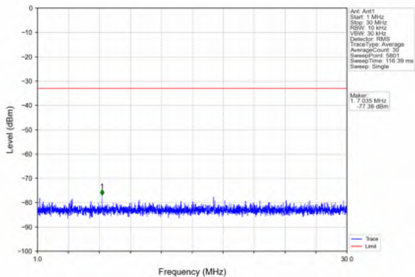
n78e_15kHz_SISO_NTNV_15MHz_DFT-s-OFDM QPSK_3457.5MHz_Inner_1RB_Left
