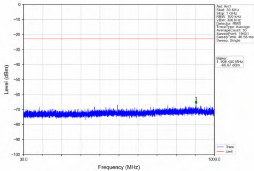
n78e_15kHz_SISO_NTNV_10MHz_CP-OFDM QPSK_3544.995MHz_Outer_Full
