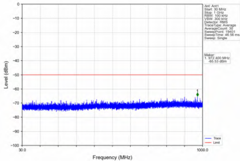
n78d_30kHz_SISO_NTNV_100MHz_DFT-s-OFDM_QPSK_3649.98MHz_Inner_1RB_Right
