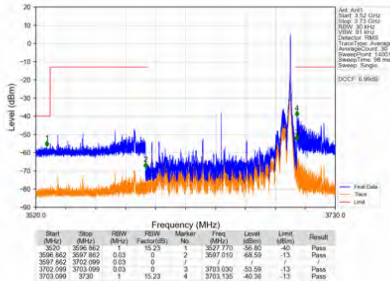
n78d_30kHz_SISO_NTNV_100MHz_DFT-s-OFDM PI/2 BPSK_3649.98MHz_Inner_1RB_Right
