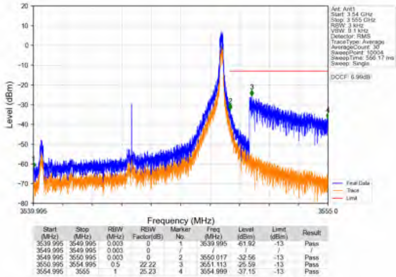
n78e_15kHz_SISO_NTNV_10MHz_DFT-s-OFDM QPSK_3544.995MHz_Edge_1RB_Right
