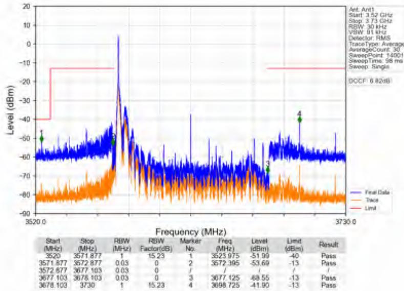
n78d_30kHz_SISO_NTNV_100MHz_DFT-s-OFDM PI/2 BPSK_3624.99MHz_Edge_1RB_Left
