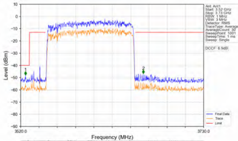
n78d_30kHz_SISO_NTNV_100MHz_CP-OFDM QPSK_3600MHz_Outer_Full
