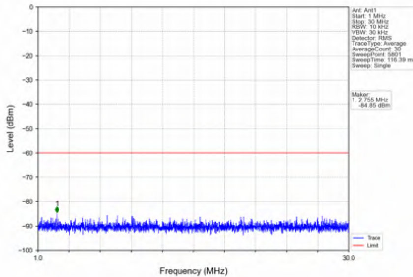
n78d_30kHz_SISO_NTNV_100MHz_DFT-s-OFDM PI/2 BPSK_3600MHz_Edge_1RB_Left
