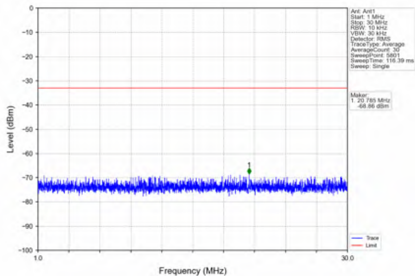
n78e_15kHz_SISO_NTNV_15MHz_CP-OFDM QPSK_3499.995MHz_Edge_1RB_Left
