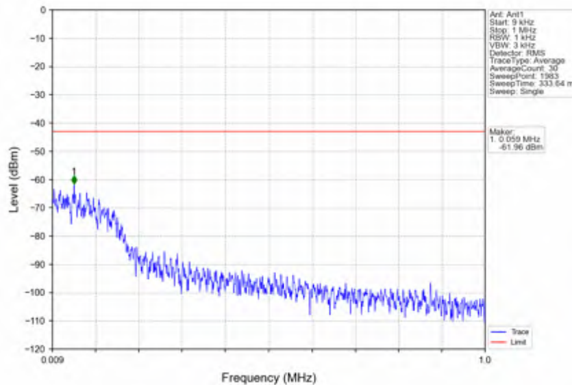
n78e_15kHz_SISO_NTV_10MHz_CP-OFDM_QPSK_3455.01MHz_Edge_1RB_Left
