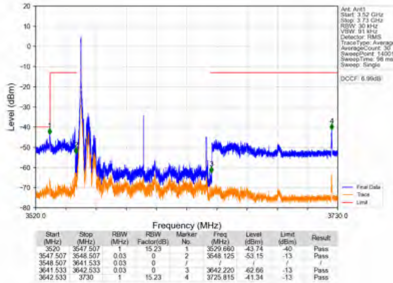
n78d_30kHz_SISO_NTV_90MHz_CP-OFDM_QPSK_3595.02MHz_Inner_1RB_Left
