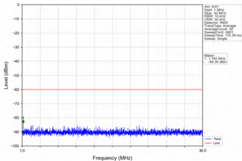
n78d_30kHz_SISO_NTNV_100MHz_DFT-s-OFDM PI/2 BPSK_3624.99MHz_Edge_1RB_Left
