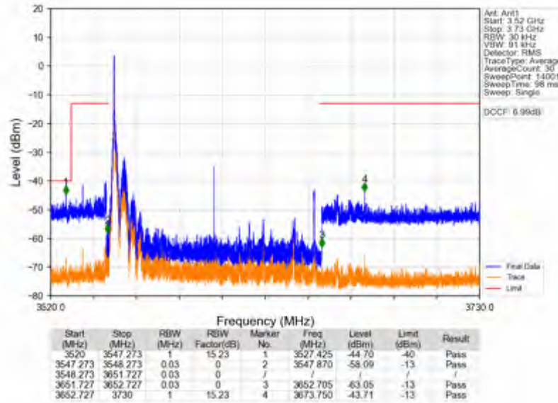
n78d_30kHz_SISO_NTNV_100MHz_CP-OFDM QPSK_3600MHz_Edge_1RB_Left
