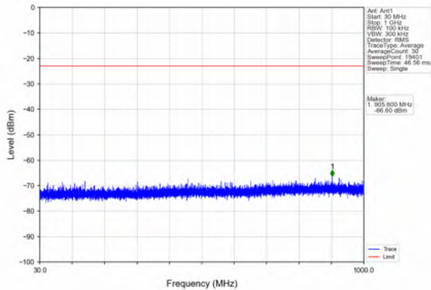
n78e_15kHz_SISO_NTNV_10MHz_CP-OFDM QPSK_3455.01MHz_Outer_Full
