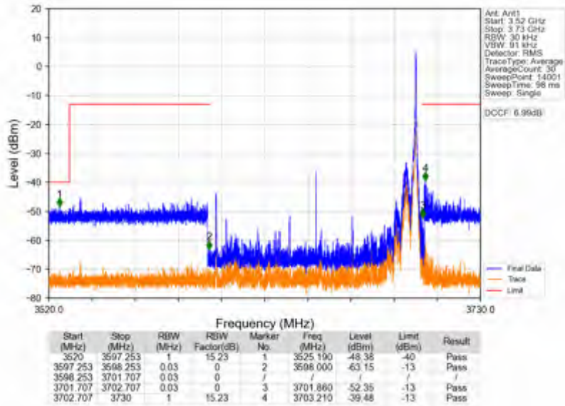
n78d_30kHz_SISO_NTNV_100MHz_DFT-s-OFDM QPSK_3649.98MHz_Inner_1RB_Right
