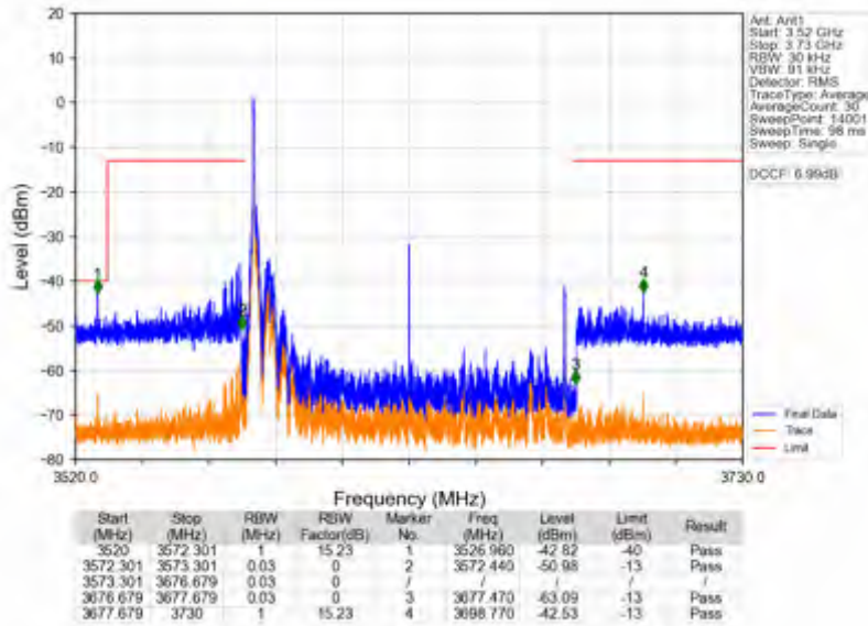
n78d_30kHz_SISO_NTNV_100MHz_CP-OFDM QPSK_3624.99MHz_Edge_1RB_Left
