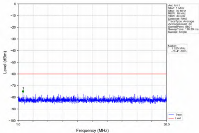
n78d_30kHz_SISO_NTNV_100MHz_DFT-s-OFDM QPSK_3600MHz_Edge_1RB_Left
