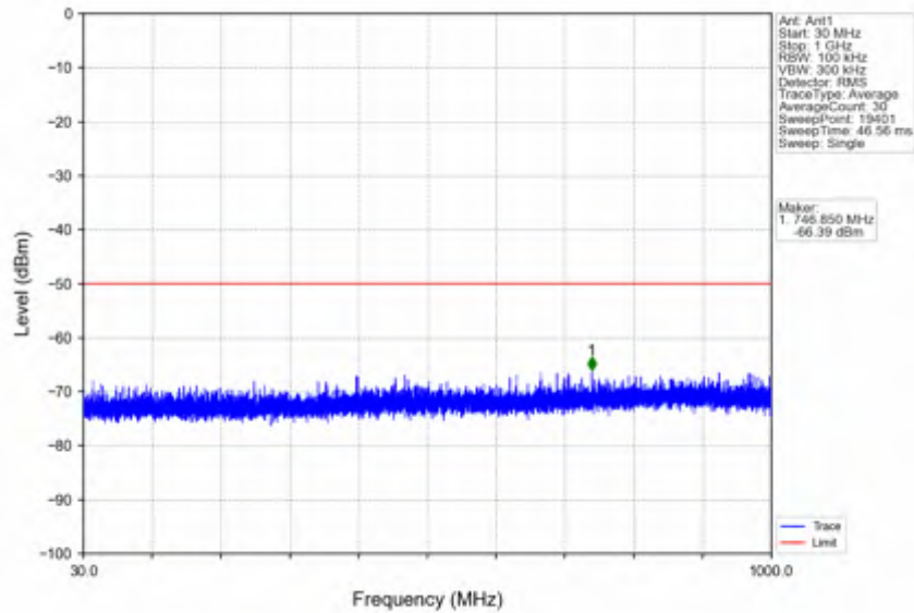
n78d_30kHz_SISO_NTNV_90MHz_DFT-s-OFDM QPSK_3654.99MHz_Edge_1RB_Right
