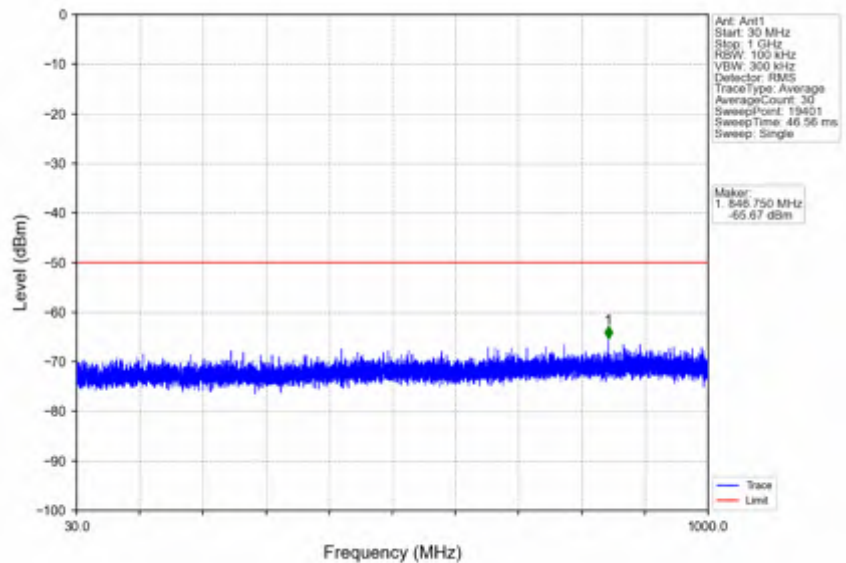
n78d_30kHz_SISO_NTNV_90MHz_CP-OFDM QPSK_3654.99MHz_Inner_1RB_Right
