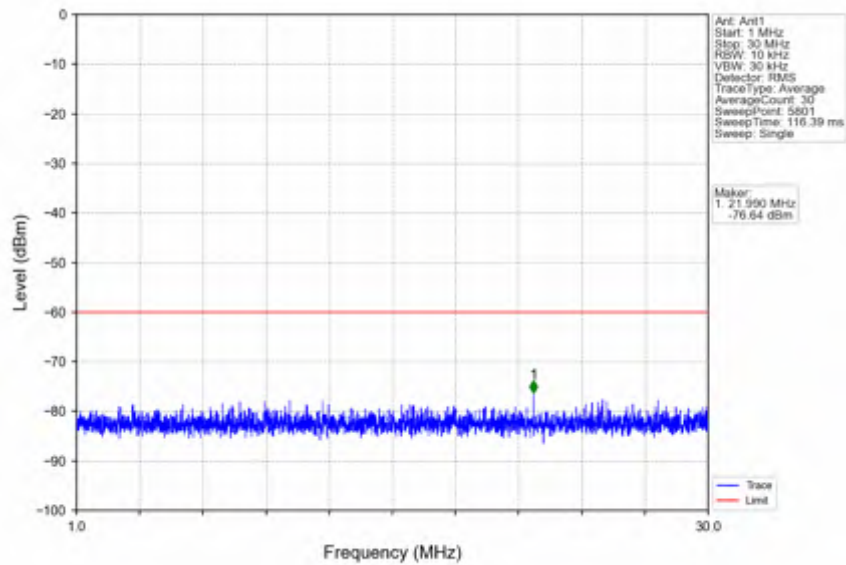
n78d_30kHz_SISO_NTNV_90MHz_CP-OFDM QPSK_3654.99MHz_Edge_1RB_Right
