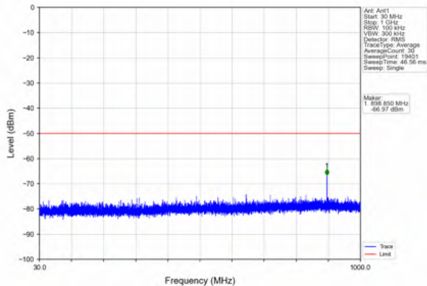
n78d_30kHz_SISO_NTNV_90MHz_DFT-s-OFDM_QPSK_3654.99MHz_Outer_Full
