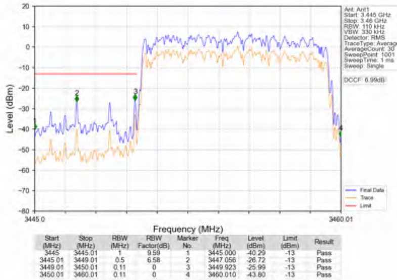
n78e_15kHz_SISO_NTNV_10MHz_DFT-s-OFDM_QPSK_3455.01MHz_Outer_Full
