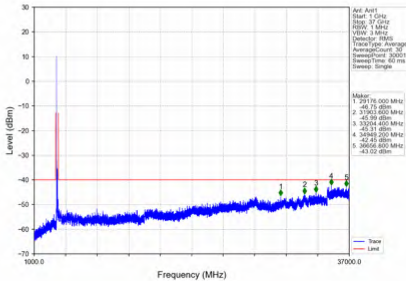
n78d_30kHz_SISO_NTNV_100MHz_CP-OFDM QPSK_3624.99MHz_Edge_1RB_Left
