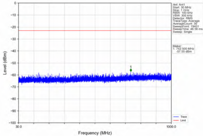
n78e_15kHz_SISO_NTNV_15MHz_DFT-s-OFDM QPSK_3542.49MHz_Edge_1RB_Right
