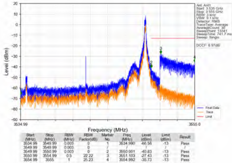
n78e_15kHz_SISO_NTV_15MHz_CP-OFDM QPSK_3542.49MHz_Inner_1RB_Right
