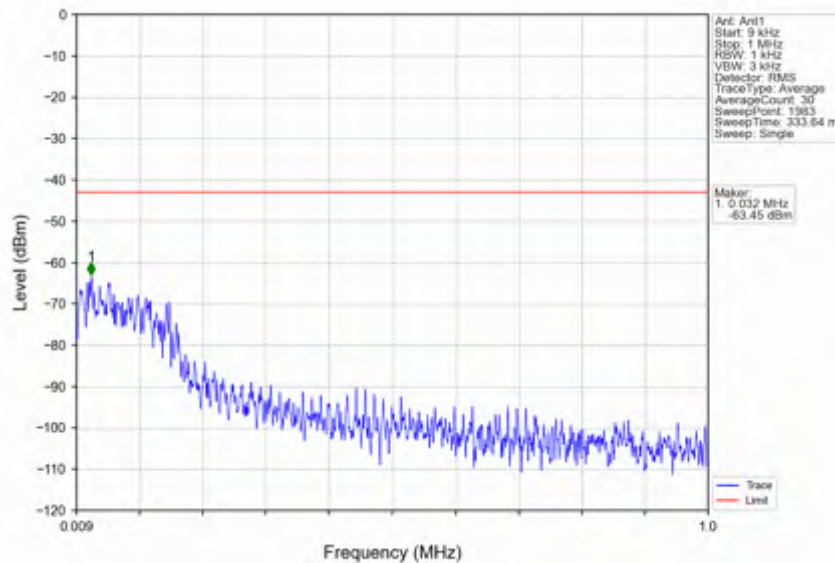
n78e_15kHz_SISO_NTV_15MHz_CP-OFDM QPSK_3542.49MHz_Edge_1RB_Right
