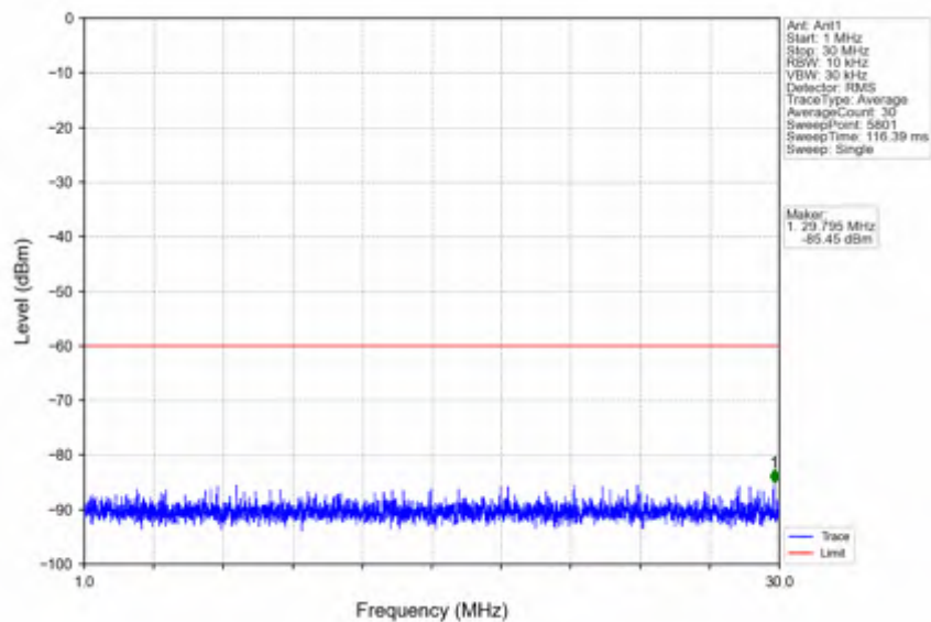
n78d_30kHz_SISO_NTNV_100MHz_DFT-s-OFDM PI/2 BPSK_3649.98MHz_Outer_Full
