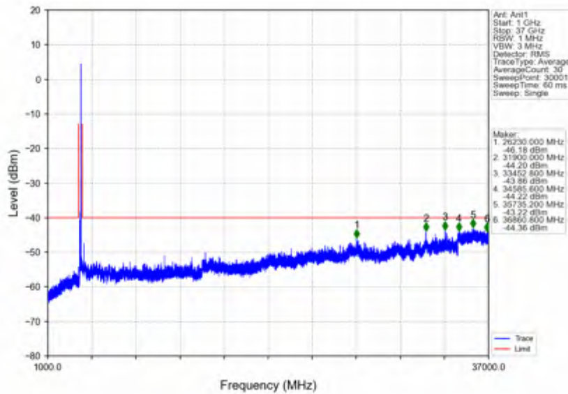
n78d_30kHz_SISO_NTV_100MHz_CP-OFDM QPSK_3649.98MHz_Outer_Full
