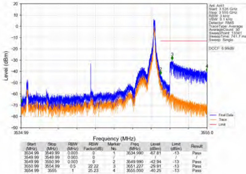
n78e_15kHz_SISO_NTNV_15MHz_DFT-s-OFDM QPSK_3542.49MHz_Inner_1RB_Right
