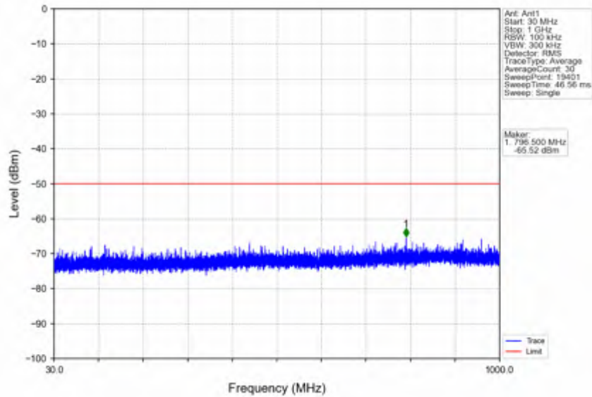
n78d_30kHz_SISO_NTNV_90MHz_CP-OFDM QPSK_3654.99MHz_Outer_Full
