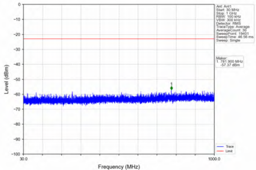
n78e_15kHz_SISO_NTNV_15MHz_CP-OFDM QPSK_3457.5MHz_Edge_1RB_Left
