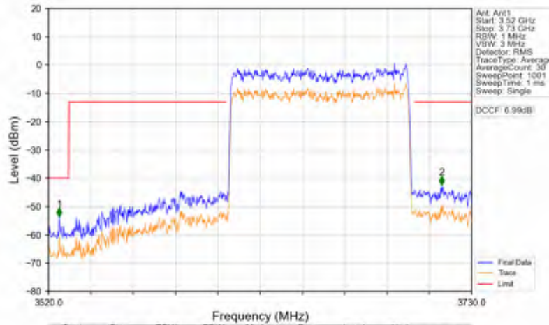
n78d_30kHz_SISO_NTNV_90MHz_DFT-s-OFDM_QPSK_3654.99MHz_Outer_Full
