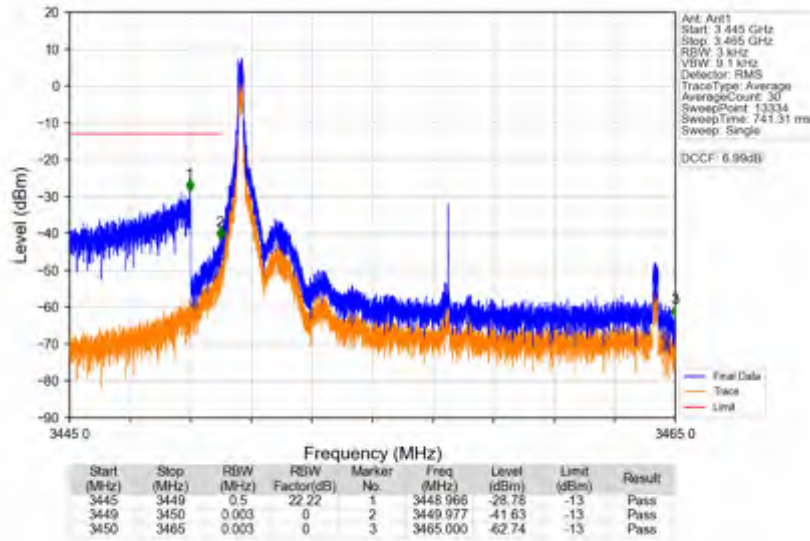
n78e_15kHz_SISO_NTNV_15MHz_CP-OFDM QPSK_3457.5MHz_Inner_1RB_Left
