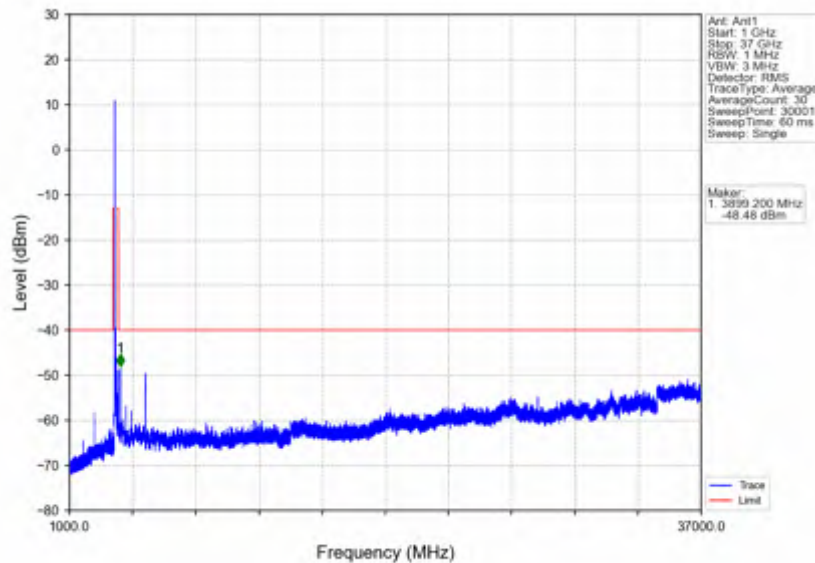
n78d_30kHz_SISO_NTNV_100MHz_DFT-s-OFDM PI/2 BPSK_3624.99MHz_Edge_1RB_Left
