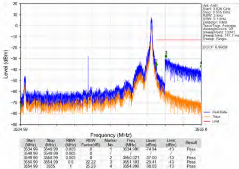
n78e_15kHz_SISO_NTNV_15MHz_DFT-s-OFDM QPSK_3542.49MHz_Edge_1RB_Right
