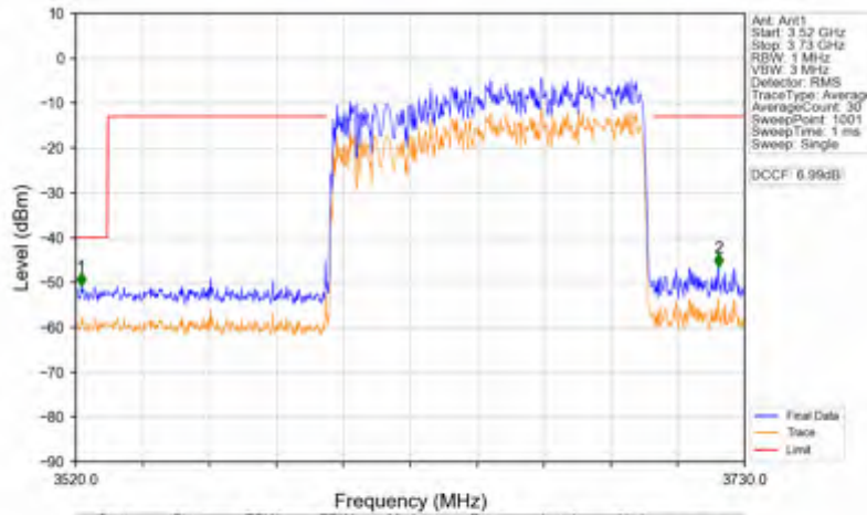
n78d_30kHz_SISO_NTNV_100MHz_DFT-s-OFDM QPSK_3649.98MHz_Outer_Full
