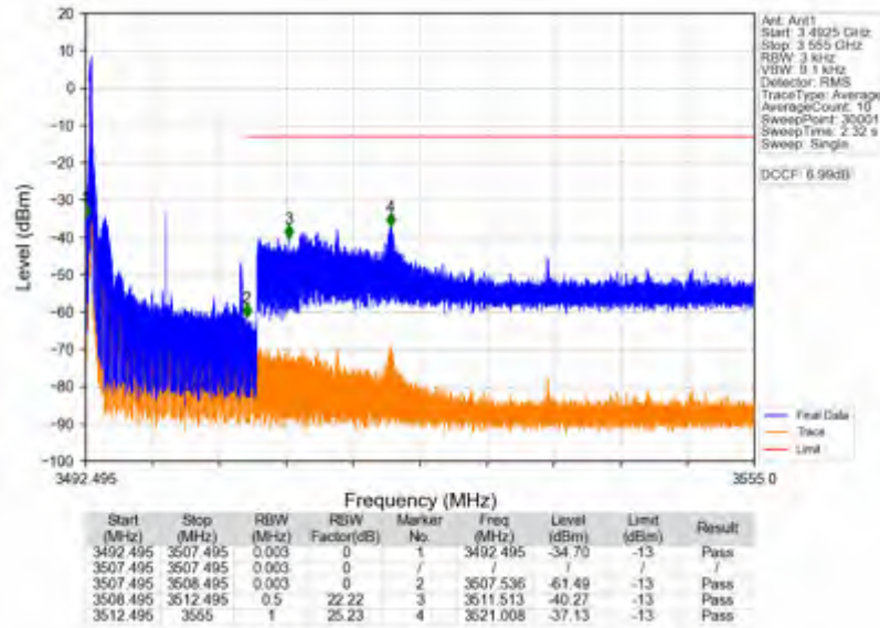
n78e_15kHz_SISO_NTNV_15MHz_DFT-s-OFDM QPSK_3499.995MHz_Edge_1RB_Left
