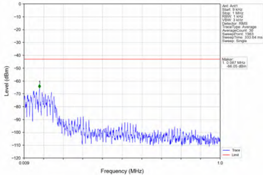
n78e_15kHz_SISO_NTNV_15MHz_DFT-s-OFDM QPSK_3542.49MHz_Edge_1RB_Right
