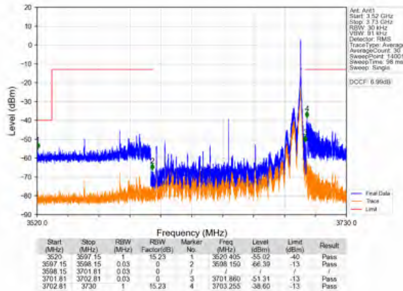
n78d_30kHz_SISO_NTNV_100MHz_DFT-s-OFDM PI/2 BPSK_3649.98MHz_Edge_1RB_Right
