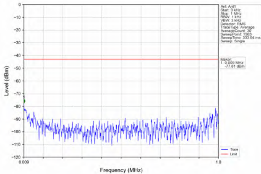
n78e_15kHz_SISO_NTNV_10MHz_DFT-s-OFDM PI/2 BPSK_3544.995MHz_Outer_Full
