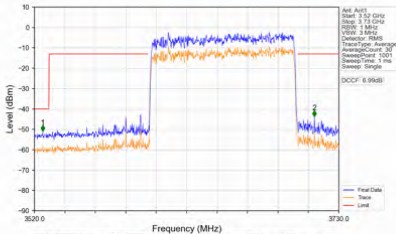
n78d_30kHz_SISO_NTV_100MHz_CP-OFDM QPSK_3649.98MHz_Outer_Full
