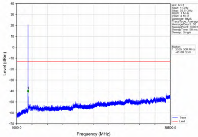
n78e_15kHz_SISO_NTV_10MHz_CP-OFDM QPSK_3544.995MHz_Outer_Full
