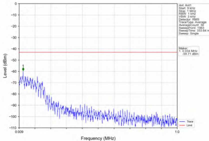
n78e_15kHz_SISO_NTNV_15MHz_CP-OFDM QPSK_3457.5MHz_Edge_1RB_Left
