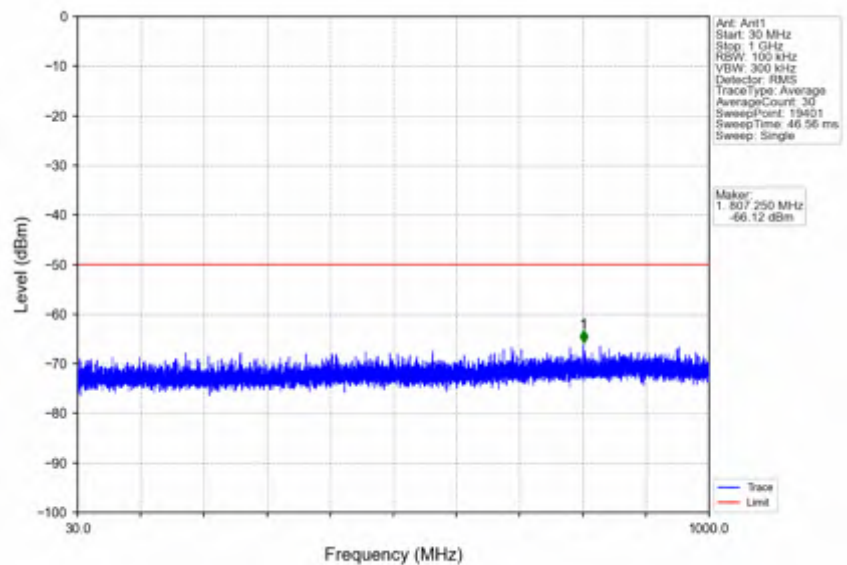
n78d_30kHz_SISO_NTNV_100MHz_CP-OFDM QPSK_3600MHz_Edge_1RB_Left
