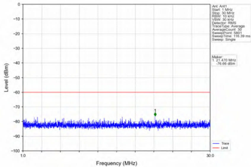
n78d_30kHz_SISO_NTNV_100MHz_CP-OFDM QPSK_3649.98MHz_Inner_1RB_Right
