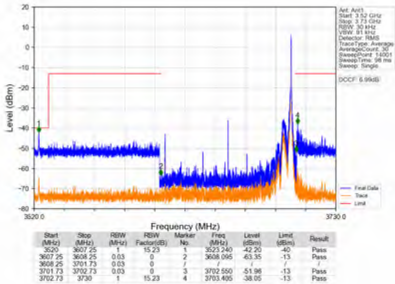
n78d_30kHz_SISO_NTNV_90MHz_DFT-s-OFDM QPSK_3654.99MHz_Edge_1RB_Right
