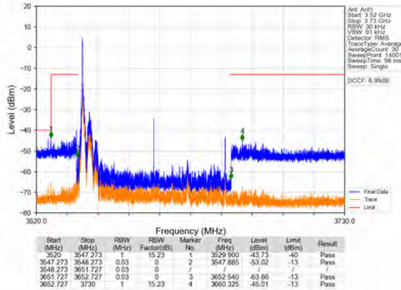
n78d_30kHz_SISO_NTNV_100MHz_CP-OFDM QPSK_3600MHz_Inner_1RB_Left
