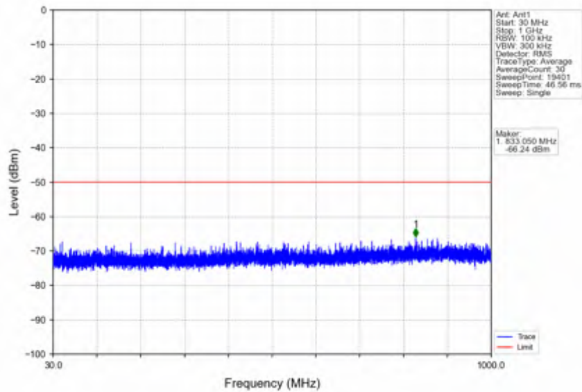
n78d_30kHz_SISO_NTV_90MHz_CP-OFDM_QPSK_3624.99MHz_Edge_1RB_Left
