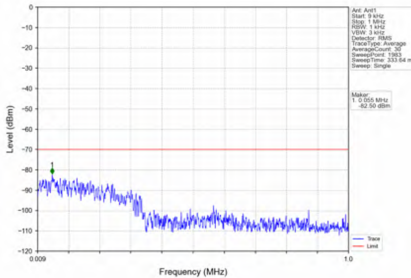
n78d_30kHz_SISO_NTNV_90MHz_CP-OFDM QPSK_3654.99MHz_Edge_1RB_Right
