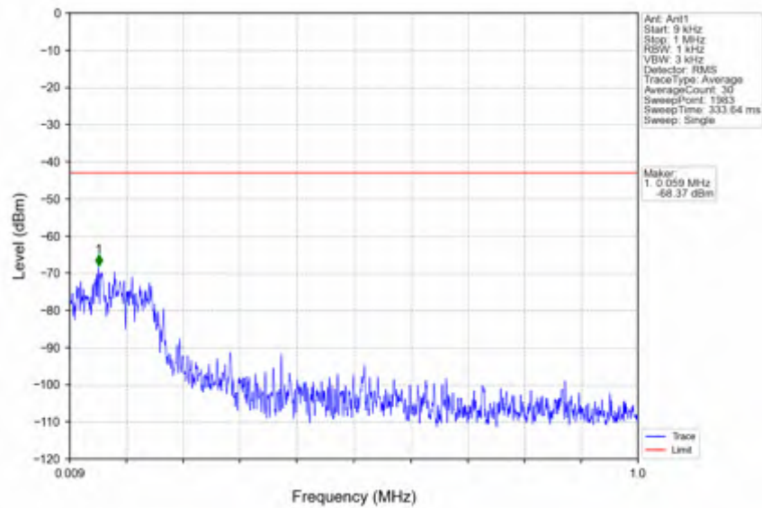
n78e_15kHz_SISO_NTNV_10MHz_DFT-s-OFDM_QPSK_3544.995MHz_Inner_1RB_Right
