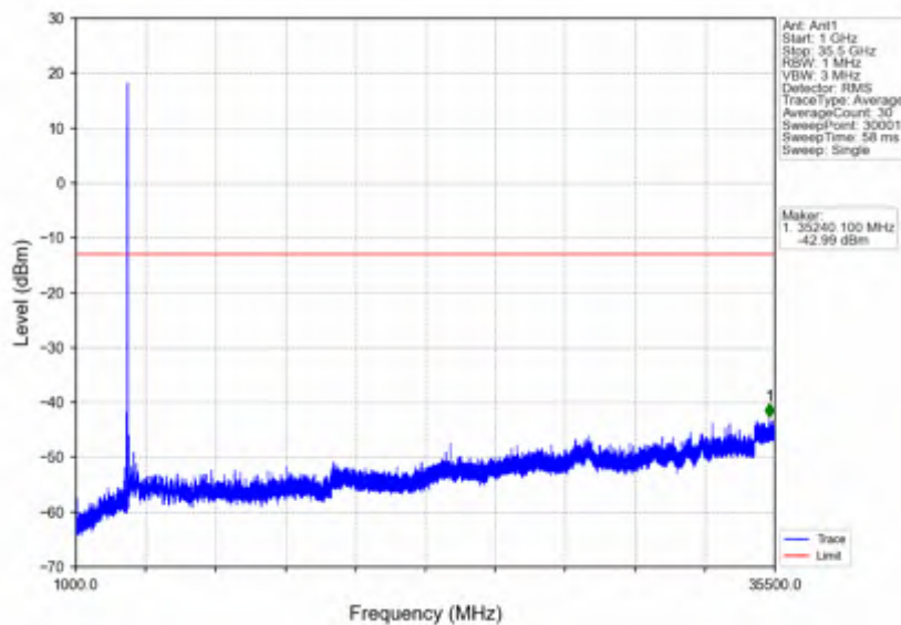
n78e_15kHz_SISO_NTV_10MHz_DFT-s-OFDM_QPSK_3544.995MHz_Edge_1RB_Right
