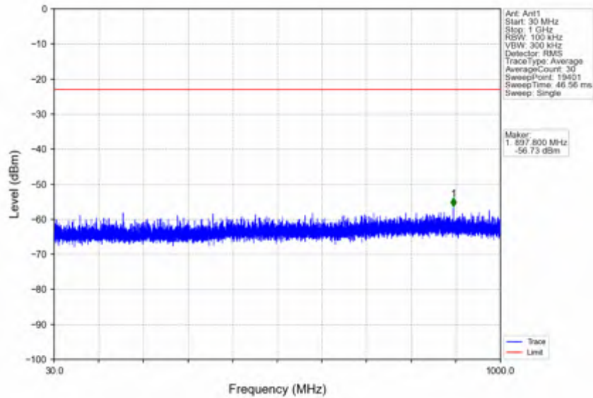
n78e_15kHz_SISO_NTNV_15MHz_CP-OFDM QPSK_3499.995MHz_Edge_1RB_Left
