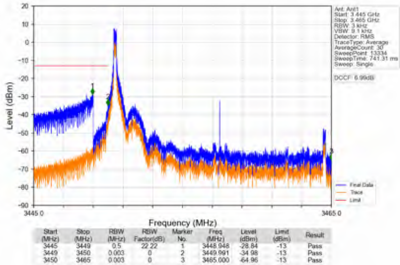
n78e_15kHz_SISO_NTNV_15MHz_DFT-s-OFDM QPSK_3457.5MHz_Edge_1RB_Left
