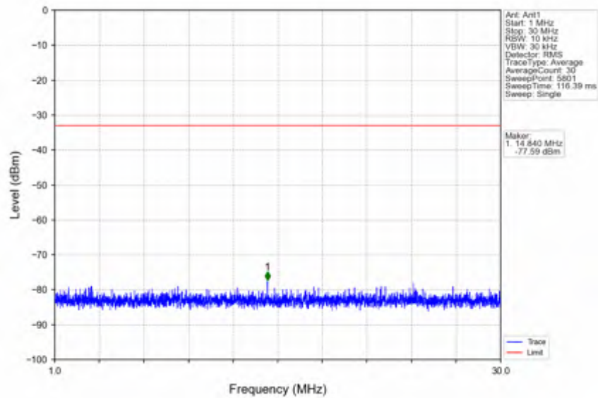
n78e_15kHz_SISO_NTNV_15MHz_DFT-s-OFDM_QPSK_3542.49MHz_Outer_Full
