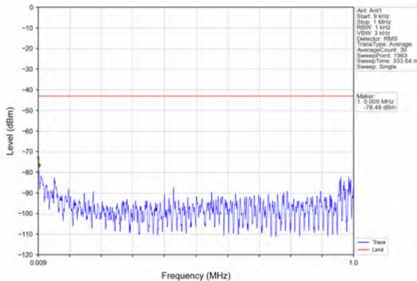
n78e_15kHz_SISO_NTNV_10MHz_DFT-s-OFDM QPSK_3544.995MHz_Outer_Full
