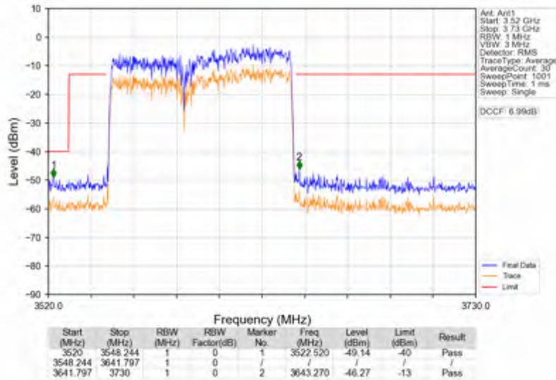
n78d_30kHz_SISO_NTNV_90MHz_CP-OFDM QPSK_3595.02MHz_Outer_Full
