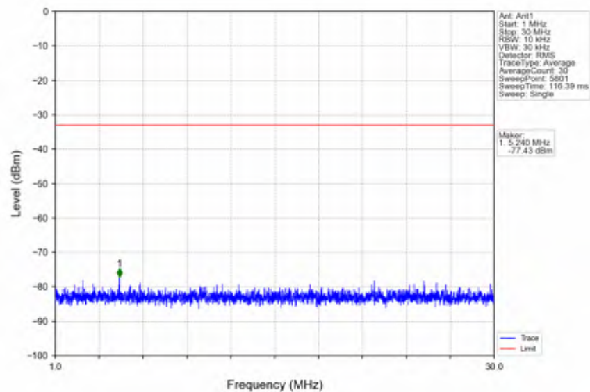
n78e_15kHz_SISO_NTNV_15MHz_CP-OFDM QPSK_3457.5MHz_Outer_Full
