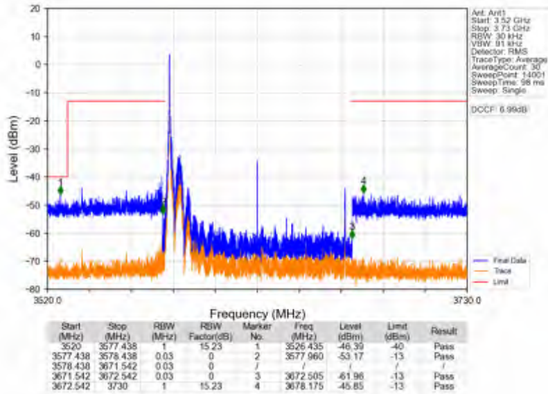
n78d_30kHz_SISO_NTV_90MHz_CP-OFDM_QPSK_3624.99MHz_Edge_1RB_Left
