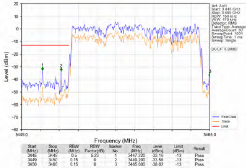
n78e_15kHz_SISO_NTNV_15MHz_DFT-s-OFDM QPSK_3457.5MHz_Outer_Full
