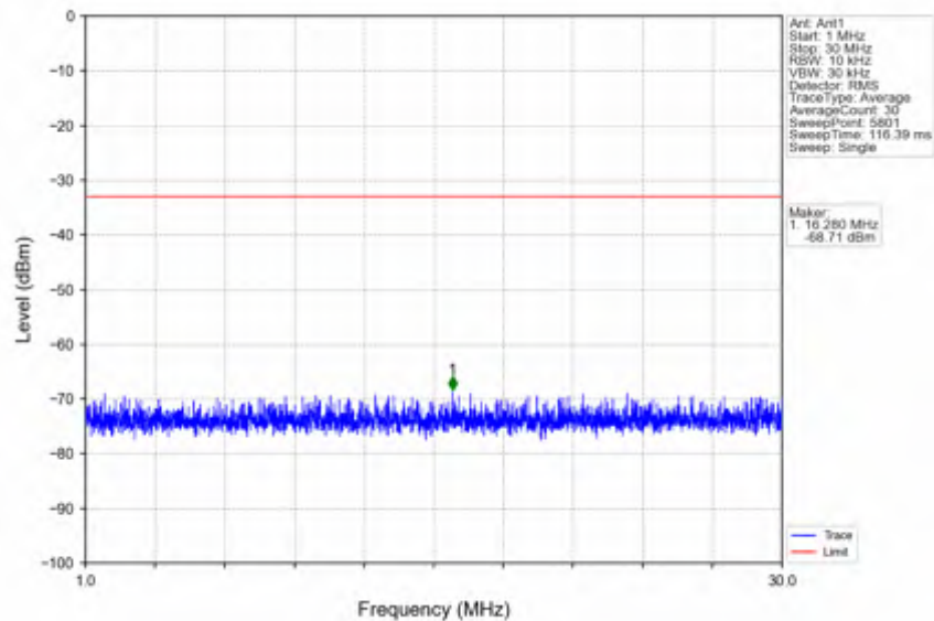
n78e_15kHz_SISO_NTNV_15MHz_DFT-s-OFDM QPSK_3457.5MHz_Edge_1RB_Left
