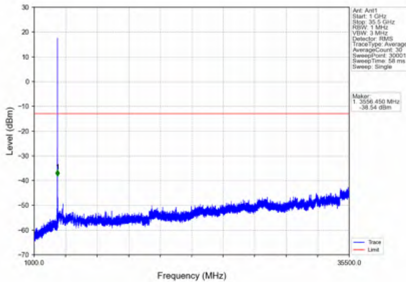
n78e_15kHz_SISO_NTNV_15MHz_DFT-s-OFDM PI/2 BPSK_3542.49MHz_Outer_Full
