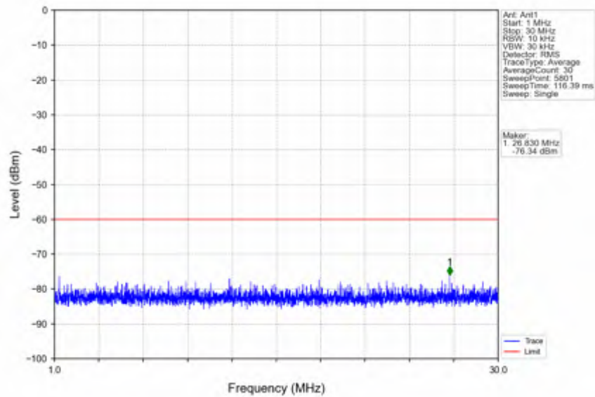
n78d_30kHz_SISO_NTNV_100MHz_DFT-s-OFDM QPSK_3600MHz_Outer_Full
