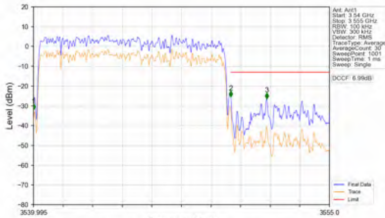
n78e_15kHz_SISO_NTV_10MHz_CP-OFDM QPSK_3544.995MHz_Outer_Full
