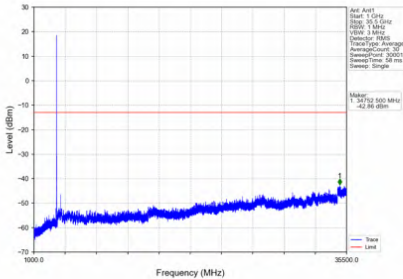
n78e_15kHz_SISO_NTNV_15MHz_DFT-s-OFDM QPSK_3542.49MHz_Edge_1RB_Right
