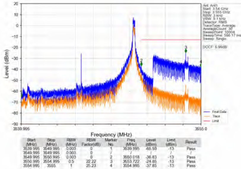
n78e_15kHz_SISO_NTNV_10MHz_DFT-s-OFDM PI/2 BPSK_3544.995MHz_Inner_1RB_Right
