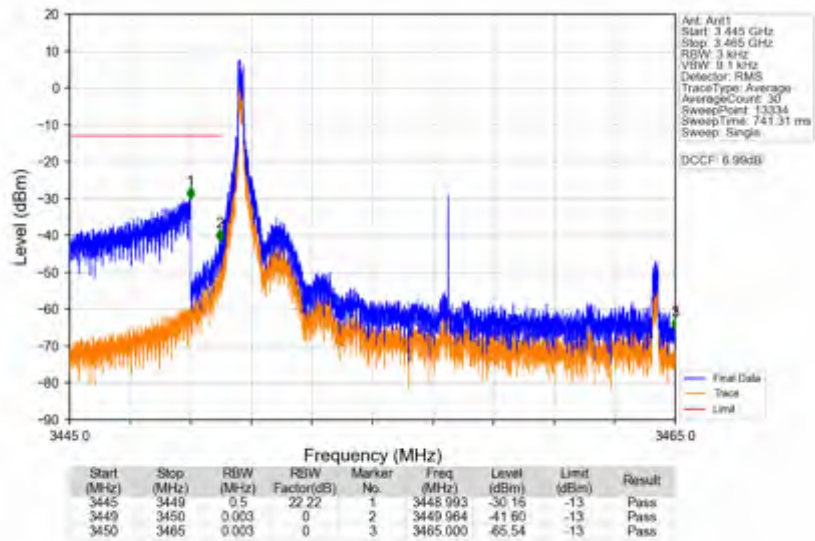
n78e_15kHz_SISO_NTNV_15MHz_DFT-s-OFDM QPSK_3457.5MHz_Inner_1RB_Left
