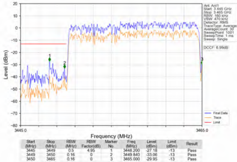
n78e_15kHz_SISO_NTNV_15MHz_CP-OFDM QPSK_3457.5MHz_Outer_Full
