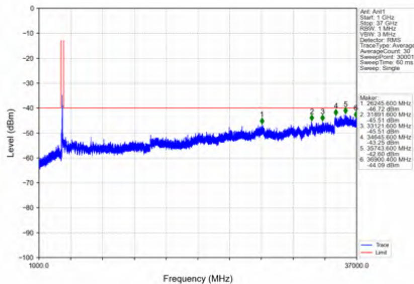
n78d_30kHz_SISO_NTNV_100MHz_CP-OFDM QPSK_3624.99MHz_Edge_1RB_Left
