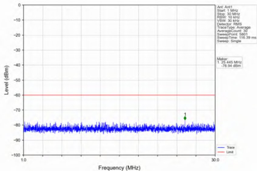
n78d_30kHz_SISO_NTNV_90MHz_CP-OFDM QPSK_3654.99MHz_Outer_Full
