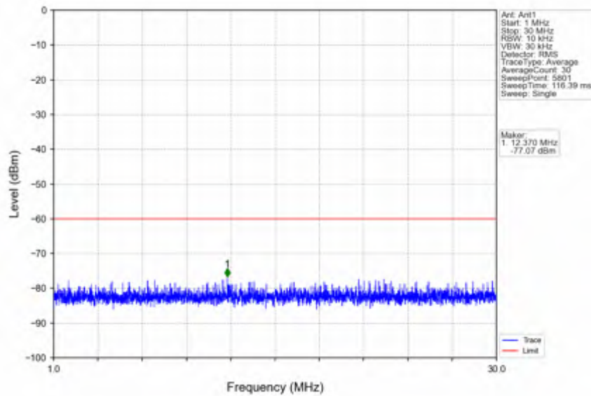
n78d_30kHz_SISO_NTNV_100MHz_DFT-s-OFDM_QPSK_3649.98MHz_Outer_Full
