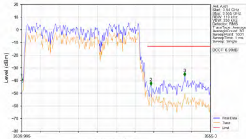
n78e_15kHz_SISO_NTNV_10MHz_DFT-s-OFDM PI/2 BPSK_3544.995MHz_Outer_Full
