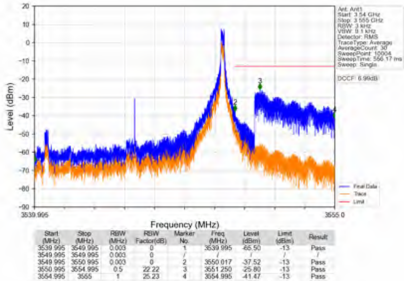
n78e_15kHz_SISO_NTNV_10MHz_DFT-s-OFDM QPSK_3544.995MHz_Inner_1RB_Right
