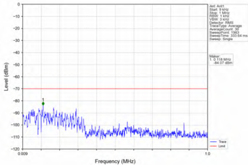
n78d_30kHz_SISO_NTNV_100MHz_DFT-s-OFDM_QPSK_3649.98MHz_Inner_1RB_Right
