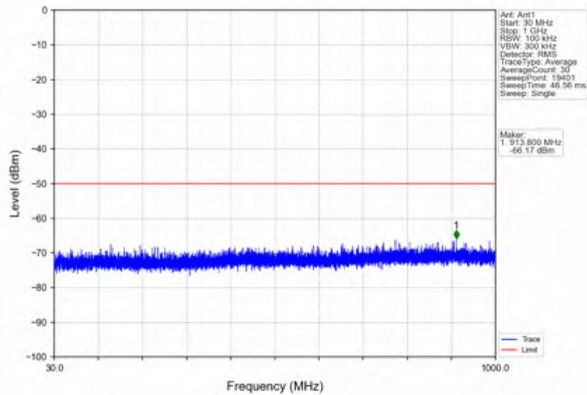
n78d_30kHz_SISO_NTNV_100MHz_CP-OFDM QPSK_3624.99MHz_Edge_1RB_Left
