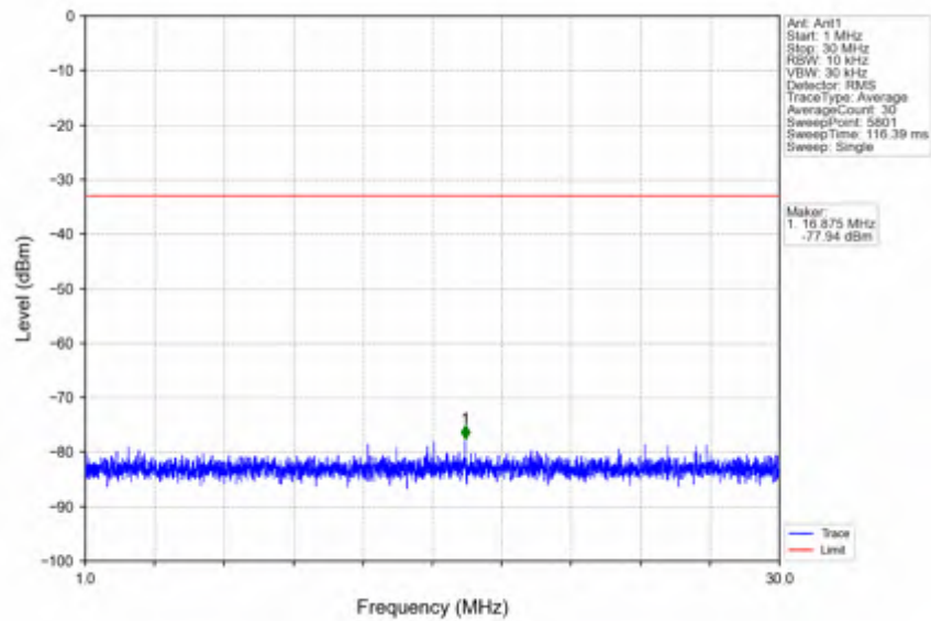
n78e_15kHz_SISO_NTNV_15MHz_DFT-s-OFDM_QPSK_3457.5MHz_Outer_Full
