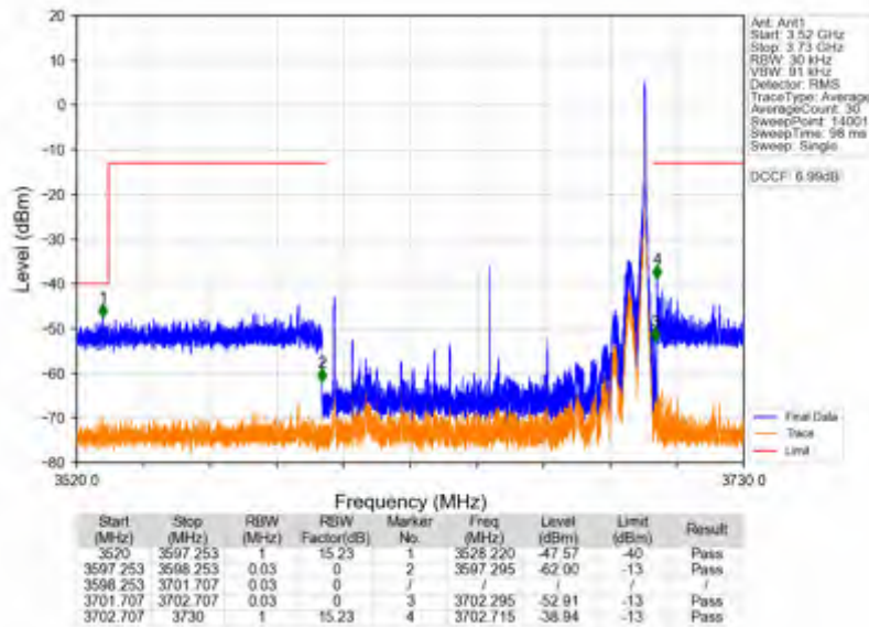
n78d_30kHz_SISO_NTNV_100MHz_DFT-s-OFDM QPSK_3649.98MHz_Edge_1RB_Right
