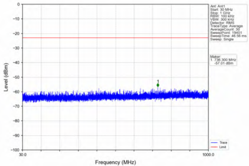
n78e_15kHz_SISO_NTNV_10MHz_DFT-s-OFDM PI/2 BPSK_3544.995MHz_Edge_1RB_Right
