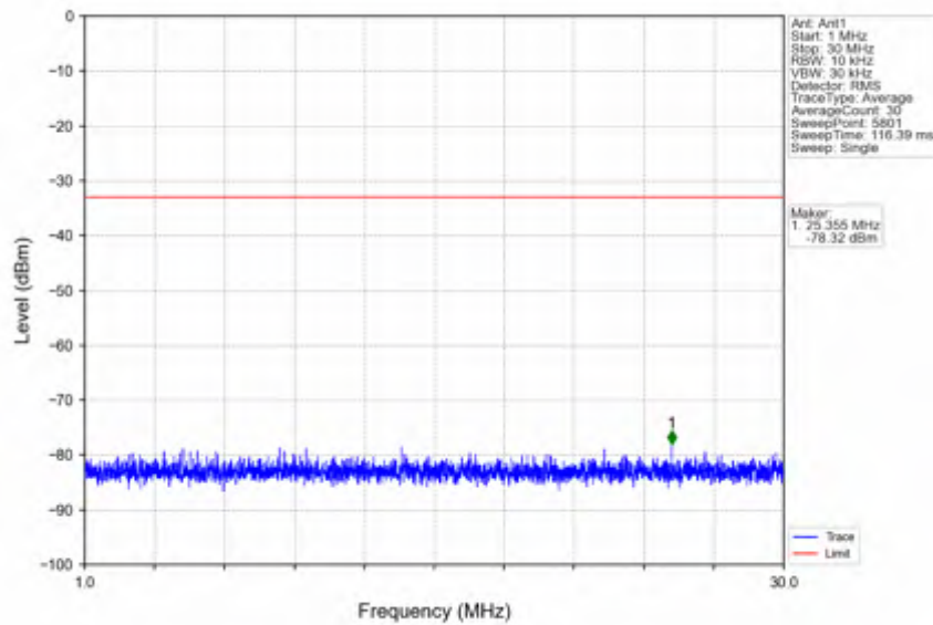
n78e_15kHz_SISO_NTNV_10MHz_DFT-s-OFDM QPSK_3544.995MHz_Outer_Full
