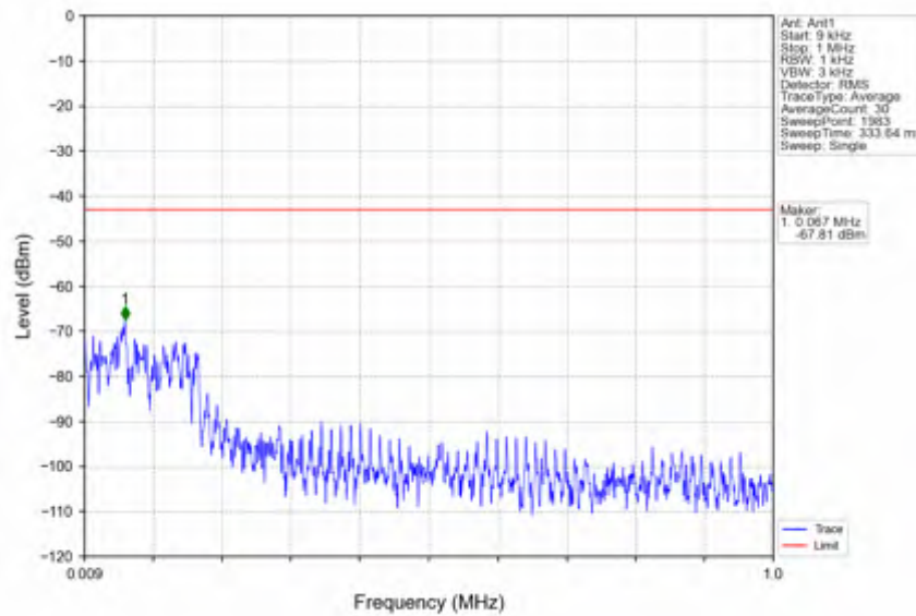
n78e_15kHz_SISO_NTNV_15MHz_DFT-s-OFDM PI/2 BPSK_3499.995MHz_Edge_1RB_Left
