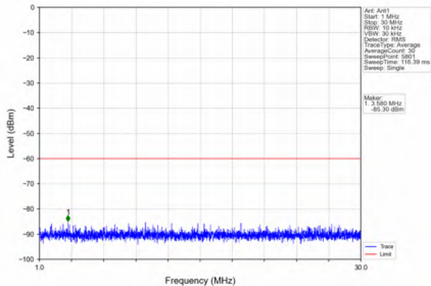
n78d_30kHz_SISO_NTNV_100MHz_DFT-s-OFDM PI/2 BPSK_3600MHz_Outer_Full
