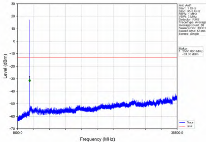
n78e_15kHz_SISO_NTV_10MHz_DFT-s-OFDM_QPSK_3544.995MHz_Inner_1RB_Right
