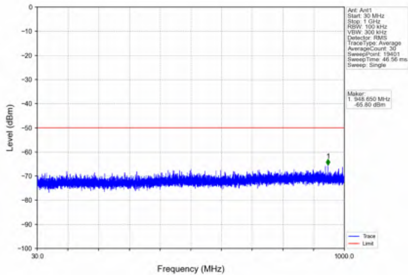
n78d_30kHz_SISO_NTV_100MHz_DFT-s-OFDM_QPSK_3649.98MHz_Edge_1RB_Right
