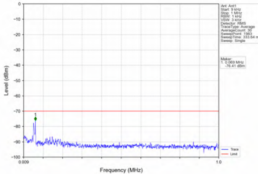
n78d_30kHz_SISO_NTV_90MHz_CP-OFDM_QPSK_3595.02MHz_Inner_1RB_Left
