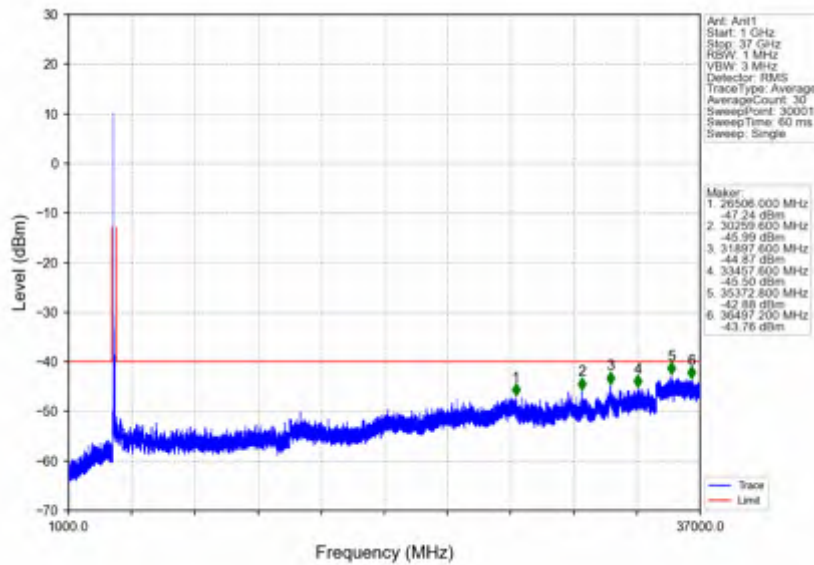
n78d_30kHz_SISO_NTNV_90MHz_CP-OFDM QPSK_3595.02MHz_Outer_Full
