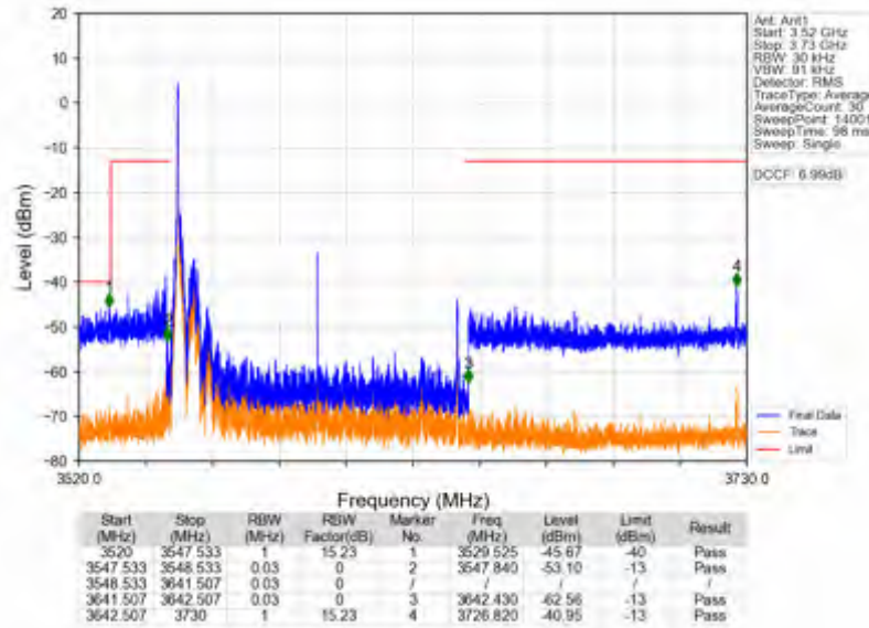
n78d_30kHz_SISO_NTV_90MHz_CP-OFDM_QPSK_3595.02MHz_Edge_1RB_Left
