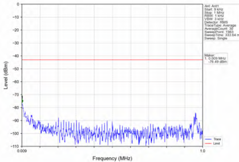
n78e_15kHz_SISO_NTNV_15MHz_DFT-s-OFDM QPSK_3457.5MHz_Outer_Full
