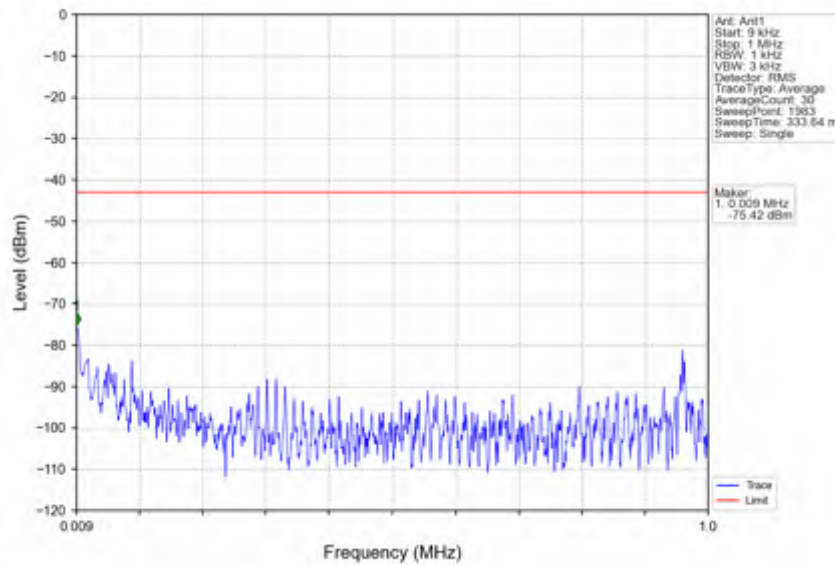
n78e_15kHz_SISO_NTNV_15MHz_DFT-s-OFDM_QPSK_3542.49MHz_Outer_Full
