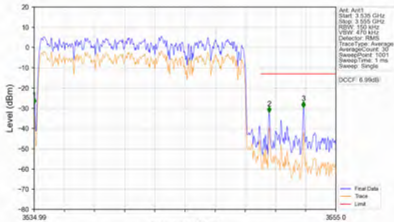
n78e_15kHz_SISO_NTNV_15MHz_DFT-s-OFDM PI/2 BPSK_3542.49MHz_Outer_Full
