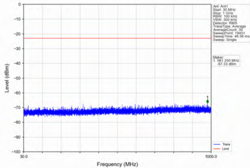
n78e_15kHz_SISO_NTNV_15MHz_CP-OFDM QPSK_3457.5MHz_Outer_Full
