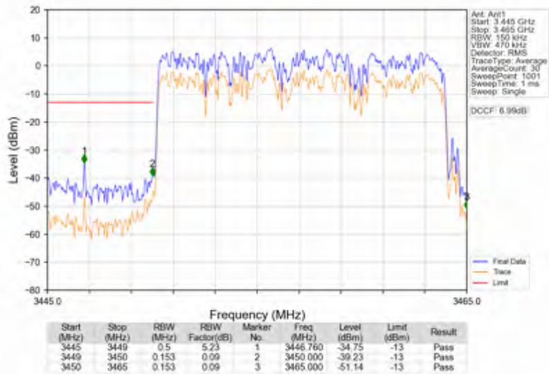
n78e_15kHz_SISO_NTNV_15MHz_DFT-s-OFDM PI/2 BPSK_3457.5MHz_Outer_Full
