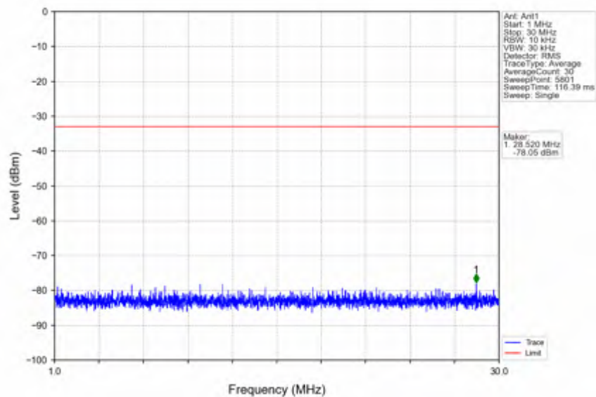
n78e_15kHz_SISO_NTNV_15MHz_DFT-s-OFDM QPSK_3542.49MHz_Inner_1RB_Right
