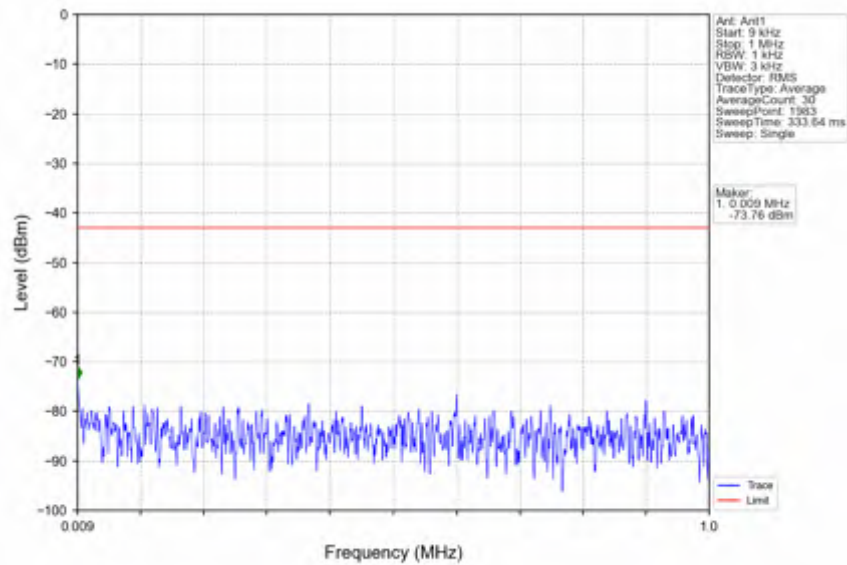
n78e_15kHz_SISO_NTNV_10MHz_CP-OFDM QPSK_3455.01MHz_Outer_Full
