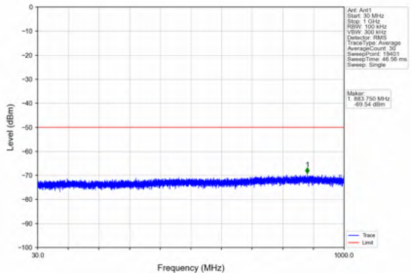
n78d_30kHz_SISO_NTVV_90MHz_CP-OFDM_QPSK_3595.02MHz_Inner_1RB_Left
