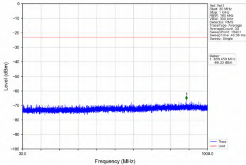
n78e_15kHz_SISO_NTNV_15MHz_DFT-s-OFDM QPSK_3457.5MHz_Inner_1RB_Left
