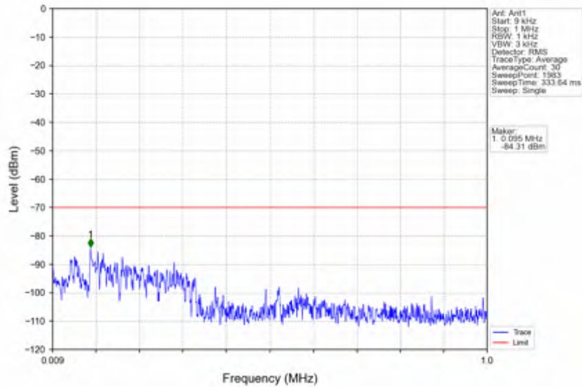
n78d_30kHz_SISO_NTV_100MHz_DFT-s-OFDM_QPSK_3649.98MHz_Edge_1RB_Right
