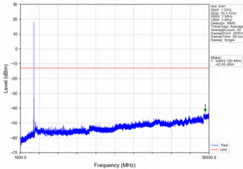
n78e_15kHz_SISO_NTNV_15MHz_DFT-s-OFDM PI/2 BPSK_3499.995MHz_Edge_1RB_Left
