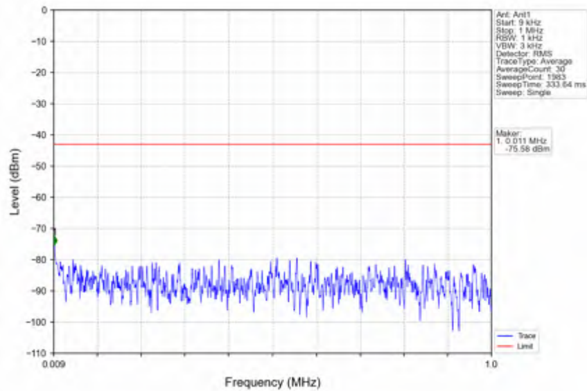
n78e_15kHz_SISO_NTNV_15MHz_CP-OFDM QPSK_3542.49MHz_Outer_Full
