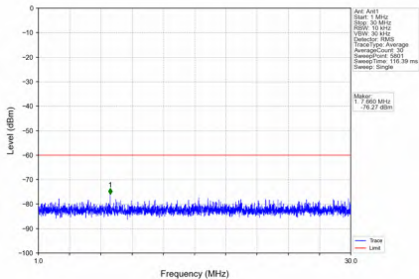
n78d_30kHz_SISO_NTNV_90MHz_CP-OFDM QPSK_3595.02MHz_Outer_Full
