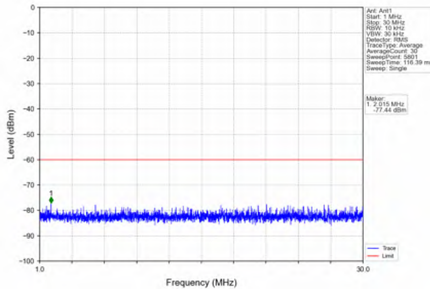
n78d_30kHz_SISO_NTNV_100MHz_DFT-s-OFDM QPSK_3624.99MHz_Edge_1RB_Left
