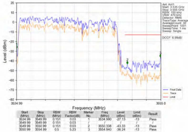
n78e_15kHz_SISO_NTNV_15MHz_DFT-s-OFDM_QPSK_3542.49MHz_Outer_Full
