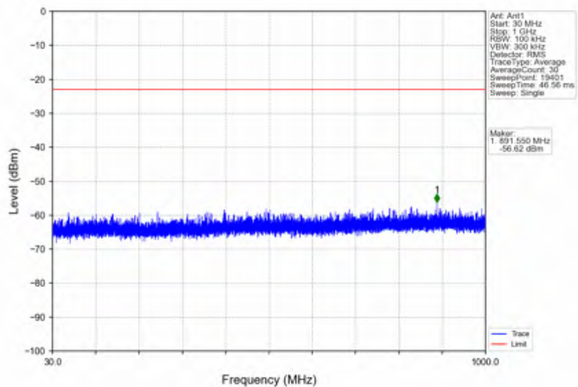
n78e_15kHz_SISO_NTNV_15MHz_DFT-s-OFDM PI/2 BPSK_3457.5MHz_Edge_1RB_Left
