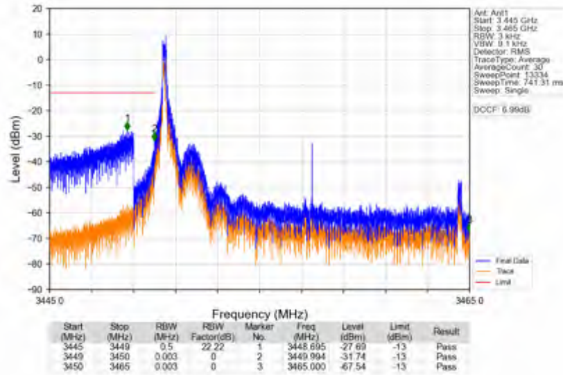
n78e_15kHz_SISO_NTNV_15MHz_CP-OFDM QPSK_3457.5MHz_Edge_1RB_Left
