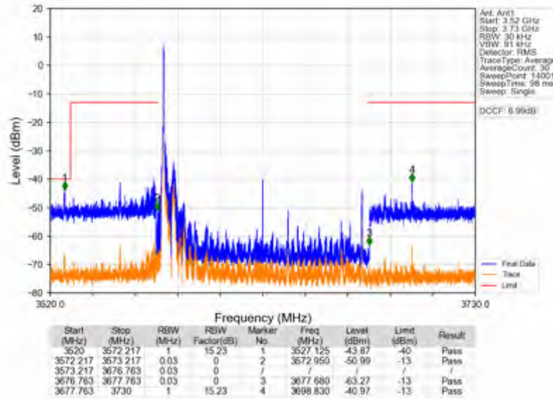
n78d_30kHz_SISO_NTNV_100MHz_DFT-s-OFDM QPSK_3624.99MHz_Edge_1RB_Left
