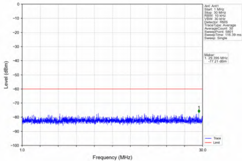
n78d_30kHz_SISO_NTVV_90MHz_CP-OFDM QPSK_3595.02MHz_Edge_1RB_Left
