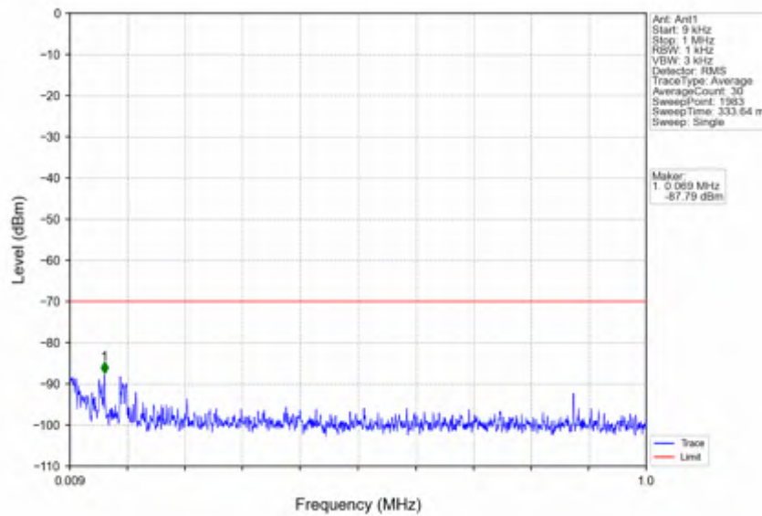
n78d_30kHz_SISO_NTNV_90MHz_DFT-s-OFDM_QPSK_3654.99MHz_Outer_Full
