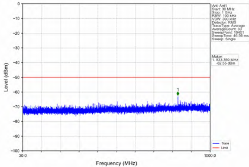
n78d_30kHz_SISO_NTNV_90MHz_DFT-s-OFDM QPSK_3654.99MHz_Inner_1RB_Right
