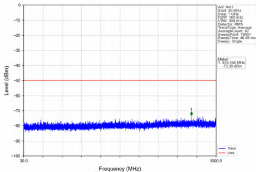
n78d_30kHz_SISO_NTNV_100MHz_DFT-s-OFDM PI/2 BPSK_3600MHz_Inner_1RB_Left
