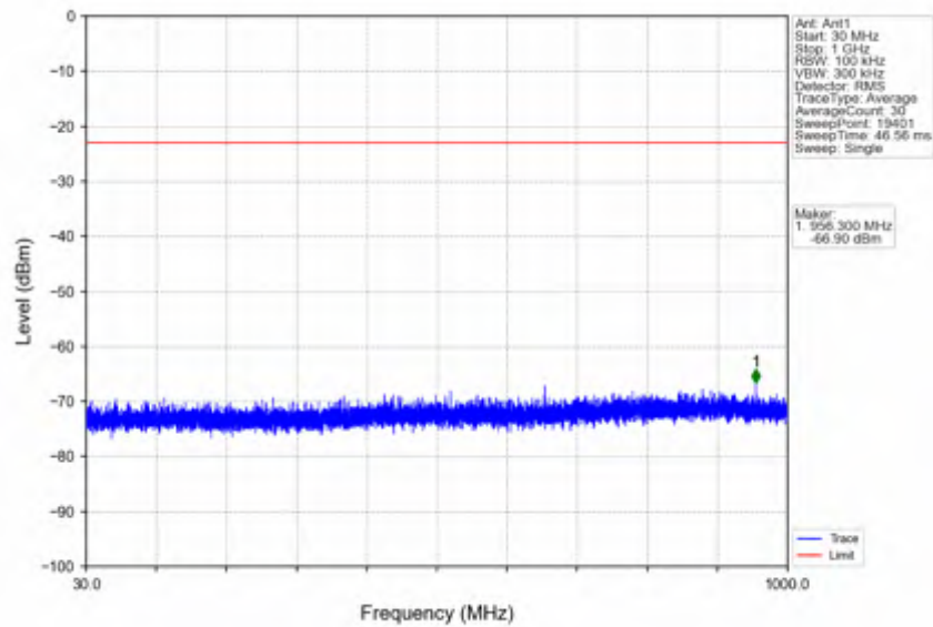
n78e_15kHz_SISO_NTNV_15MHz_CP-OFDM QPSK_3542.49MHz_Outer_Full
