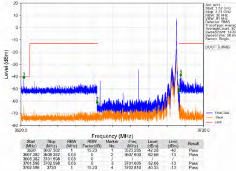
n78d_30kHz_SISO_NTNV_90MHz_CP-OFDM QPSK_3654.99MHz_Edge_1RB_Right
