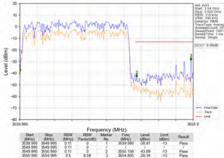
n78e_15kHz_SISO_NTNV_10MHz_DFT-s-OFDM QPSK_3544.995MHz_Outer_Full
