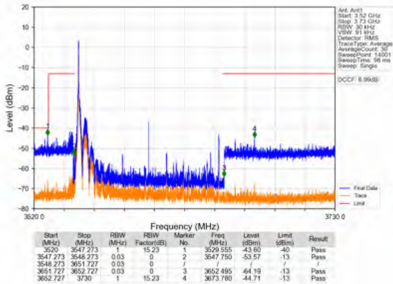
n78d_30kHz_SISO_NTNV_100MHz_DFT-s-OFDM QPSK_3600MHz_Edge_1RB_Left
