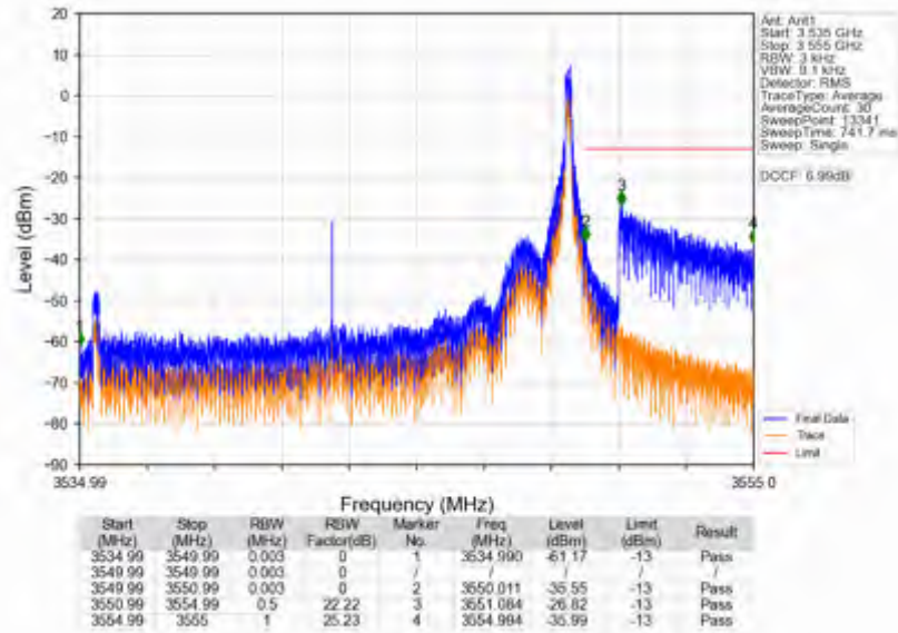
n78e_15kHz_SISO_NTV_15MHz_CP-OFDM QPSK_3542.49MHz_Edge_1RB_Right
