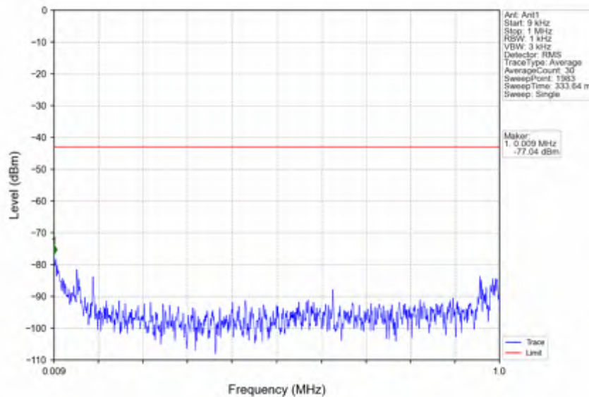
n78e_15kHz_SISO_NTNV_10MHz_DFT-s-OFDM_QPSK_3455.01MHz_Outer_Full
