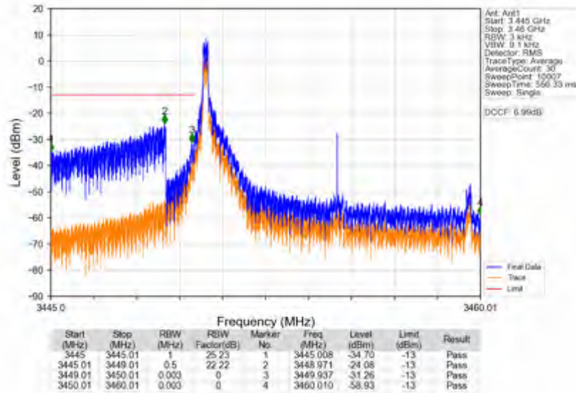
n78e_15kHz_SISO_NTV_10MHz_CP-OFDM_QPSK_3455.01MHz_Edge_1RB_Left
