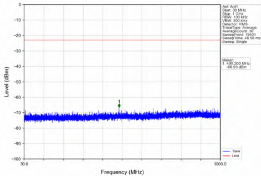
n78e_15kHz_SISO_NTNV_15MHz_DFT-s-OFDM QPSK_3542.49MHz_Inner_1RB_Right
