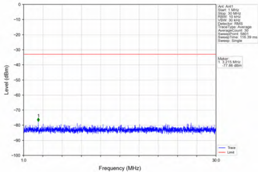
n78e_15kHz_SISO_NTNV_10MHz_DFT-s-OFDM_QPSK_3455.01MHz_Outer_Full
