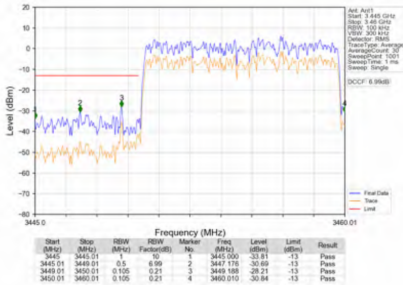
n78e_15kHz_SISO_NTNV_10MHz_CP-OFDM QPSK_3455.01MHz_Outer_Full
