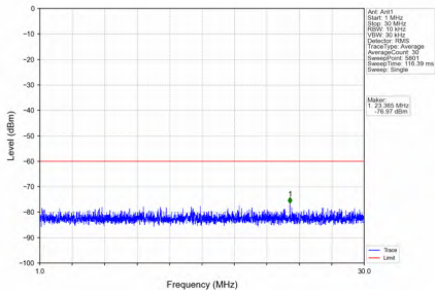
n78d_30kHz_SISO_NTNV_100MHz_CP-OFDM QPSK_3624.99MHz_Edge_1RB_Left
