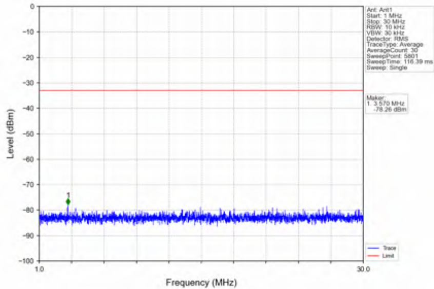
n78e_15kHz_SISO_NTNV_15MHz_CP-OFDM QPSK_3457.5MHz_Inner_1RB_Left
