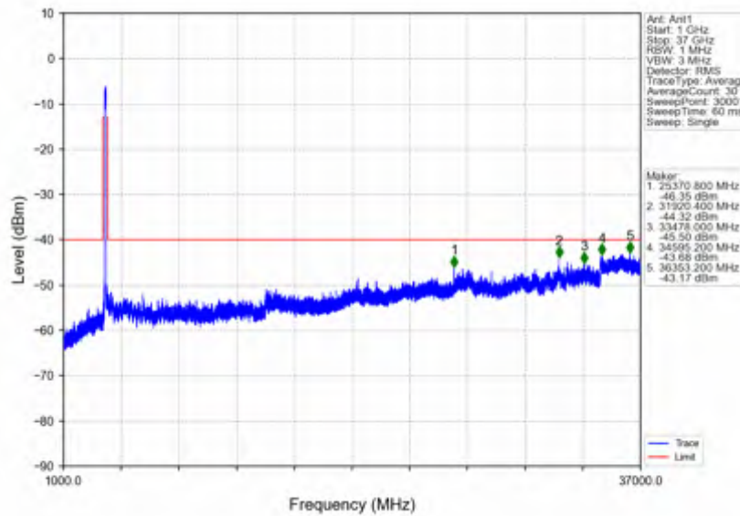
n78d_30kHz_SISO_NTNV_100MHz_DFT-s-OFDM QPSK_3600MHz_Inner_1RB_Left
