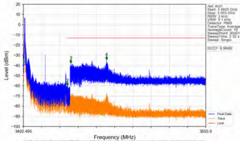
n78e_15kHz_SISO_NTNV_15MHz_CP-OFDM QPSK_3499.995MHz_Edge_1RB_Left
