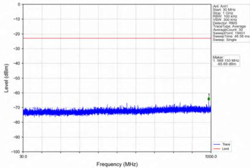
n78e_15kHz_SISO_NTV_10MHz_DFT-s-OFDM_QPSK_3544.995MHz_Inner_1RB_Right
