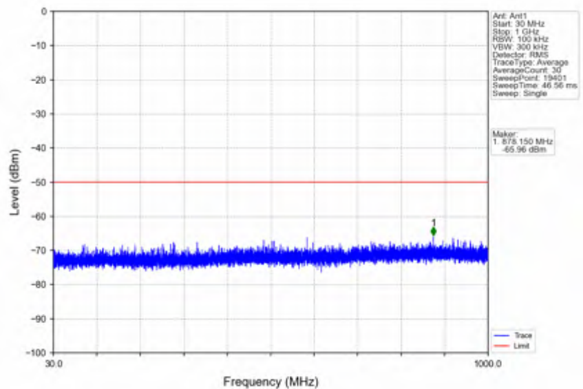
n78d_30kHz_SISO_NTNV_100MHz_CP-OFDM QPSK_3649.98MHz_Edge_1RB_Right
