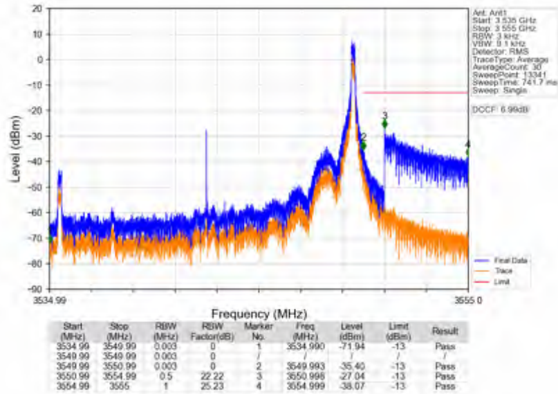
n78e_15kHz_SISO_NTNV_15MHz_DFT-s-OFDM PI/2 BPSK_3542.49MHz_Edge_1RB_Right
