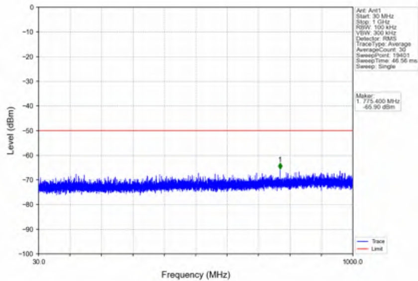
n78d_30kHz_SISO_NTNV_100MHz_CP-OFDM QPSK_3649.98MHz_Outer_Full
