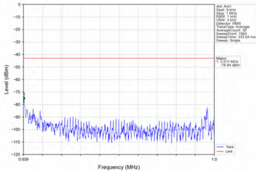
n78e_15kHz_SISO_NTNV_15MHz_DFT-s-OFDM PI/2 BPSK_3542.49MHz_Outer_Full
