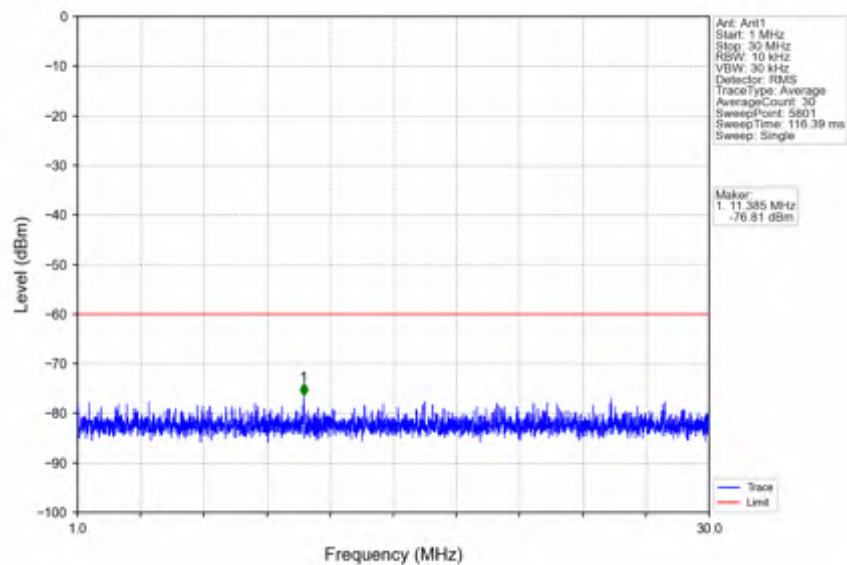
n78d_30kHz_SISO_NTV_90MHz_CP-OFDM QPSK_3624.99MHz_Edge_1RB_Left
