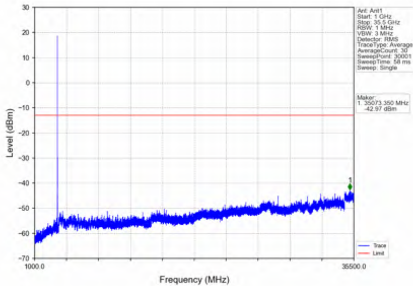
n78e_15kHz_SISO_NTNV_15MHz_DFT-s-OFDM PI/2 BPSK_3457.5MHz_Outer_Full
