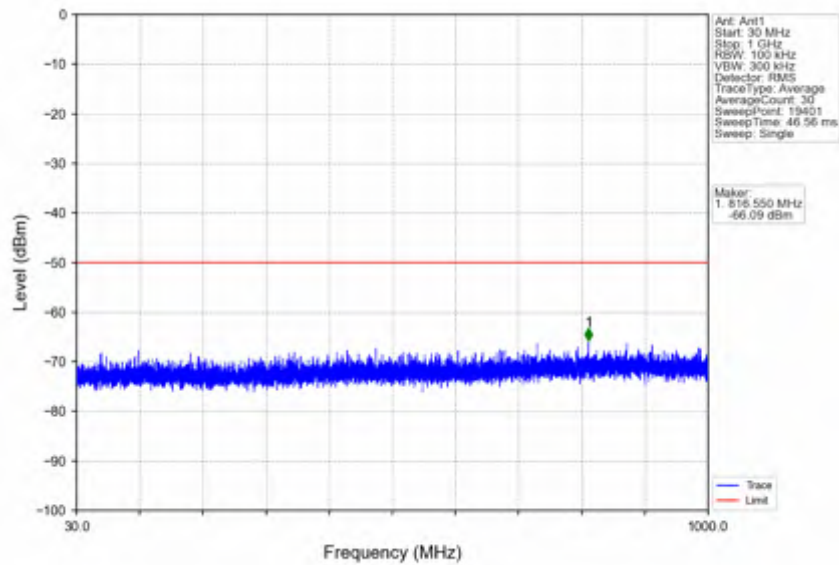
n78d_30kHz_SISO_NTNV_100MHz_DFT-s-OFDM QPSK_3600MHz_Inner_1RB_Left
