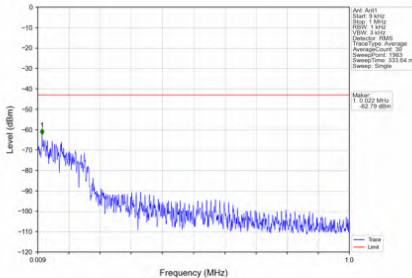
n78e_15kHz_SISO_NTV_15MHz_CP-OFDM QPSK_3542.49MHz_Inner_1RB_Right
