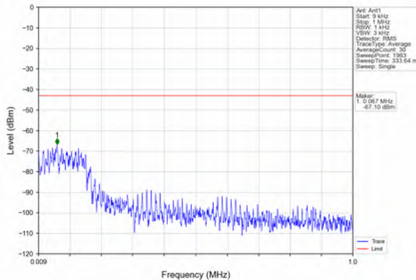
n78e_15kHz_SISO_NTNV_15MHz_DFT-s-OFDM QPSK_3499.995MHz_Edge_1RB_Left
