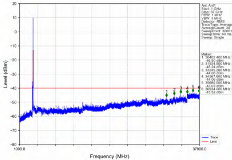
n78d_30kHz_SISO_NTNV_90MHz_CP-OFDM QPSK_3654.99MHz_Outer_Full
