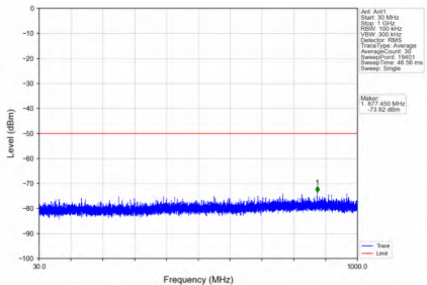
n78d_30kHz_SISO_NTNV_100MHz_DFT-s-OFDM PI/2 BPSK_3649.98MHz_Inner_1RB_Right
