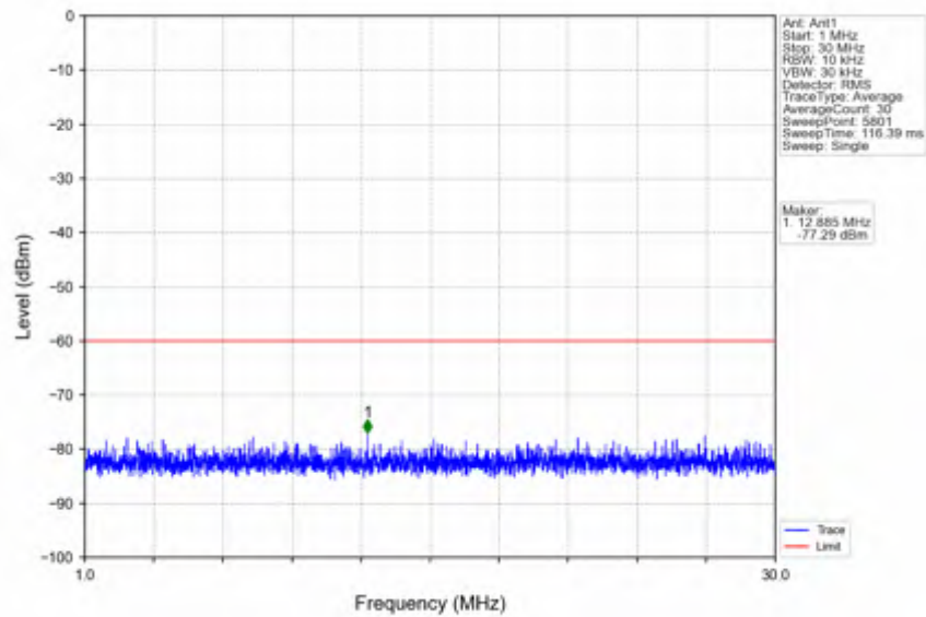
n78d_30kHz_SISO_NTNV_100MHz_CP-OFDM QPSK_3600MHz_Inner_1RB_Left
