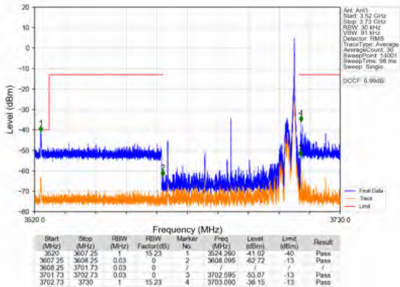
n78d_30kHz_SISO_NTNV_90MHz_DFT-s-OFDM QPSK_3654.99MHz_Inner_1RB_Right
