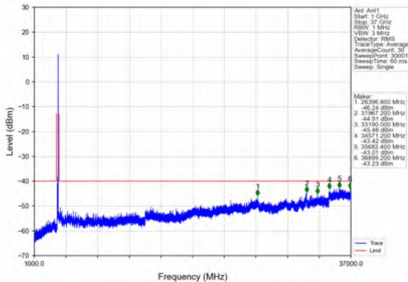
n78d_30kHz_SISO_NTV_100MHz_DFT-s-OFDM_QPSK_3649.98MHz_Edge_1RB_Right
