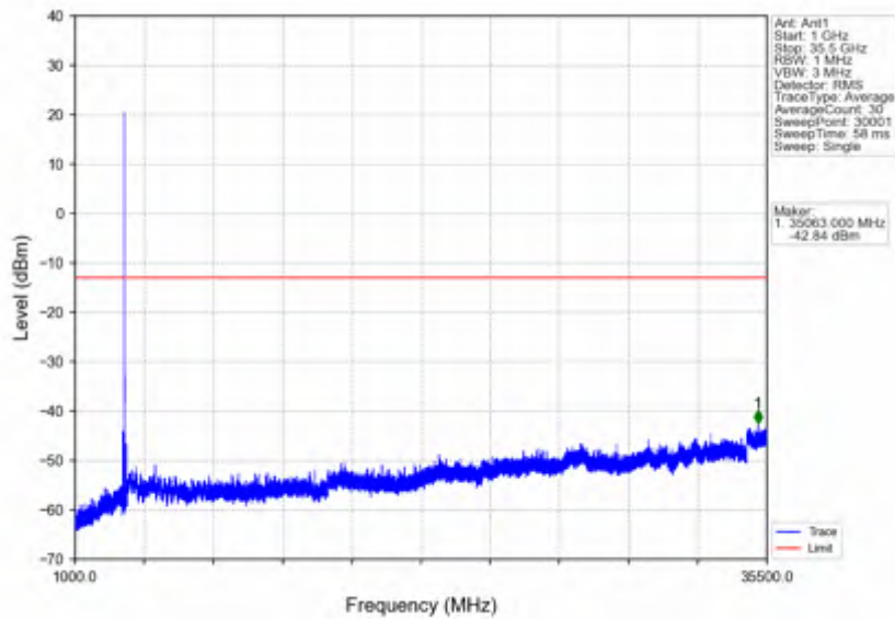
n78e_15kHz_SISO_NTNV_10MHz_DFT-s-OFDM PI/2 BPSK_3455.01MHz_Outer_Full
