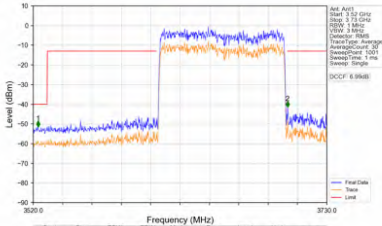
n78d_30kHz_SISO_NTNV_90MHz_CP-OFDM QPSK_3654.99MHz_Outer_Full
