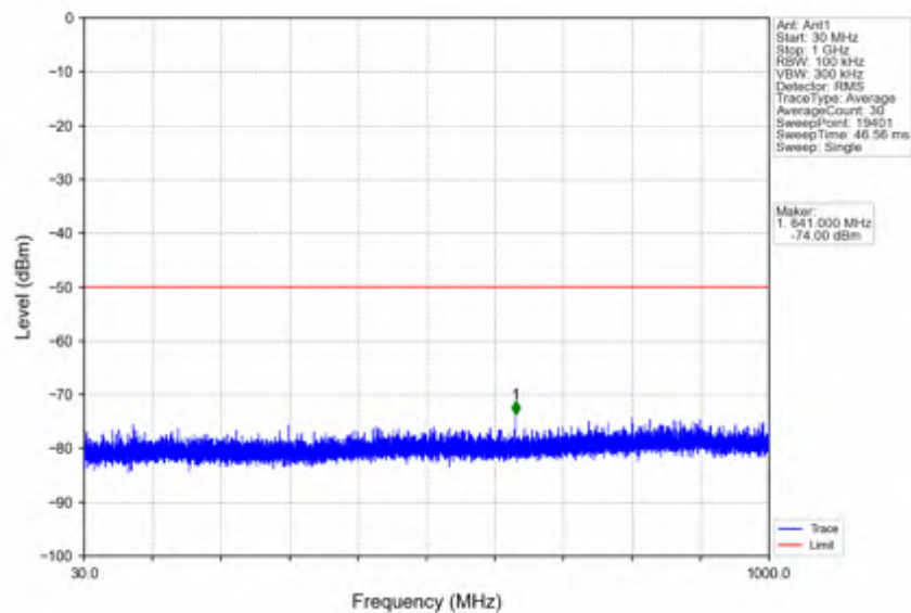
n78d_30kHz_SISO_NTNV_100MHz_DFT-s-OFDM PI/2 BPSK_3649.98MHz_Edge_1RB_Right
