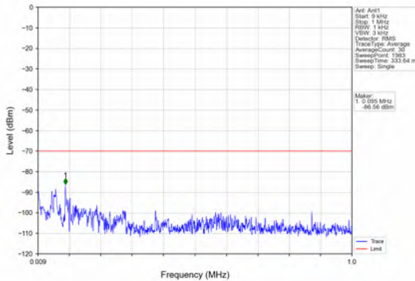
n78d_30kHz_SISO_NTNV_100MHz_DFT-s-OFDM QPSK_3649.98MHz_Outer_Full
