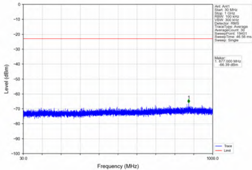
n78e_15kHz_SISO_NTNV_10MHz_DFT-s-OFDM PI/2 BPSK_3455.01MHz_Outer_Full
