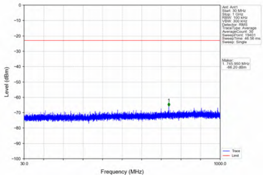
n78e_15kHz_SISO_NTNV_15MHz_DFT-s-OFDM PI/2 BPSK_3542.49MHz_Inner_1RB_Right
