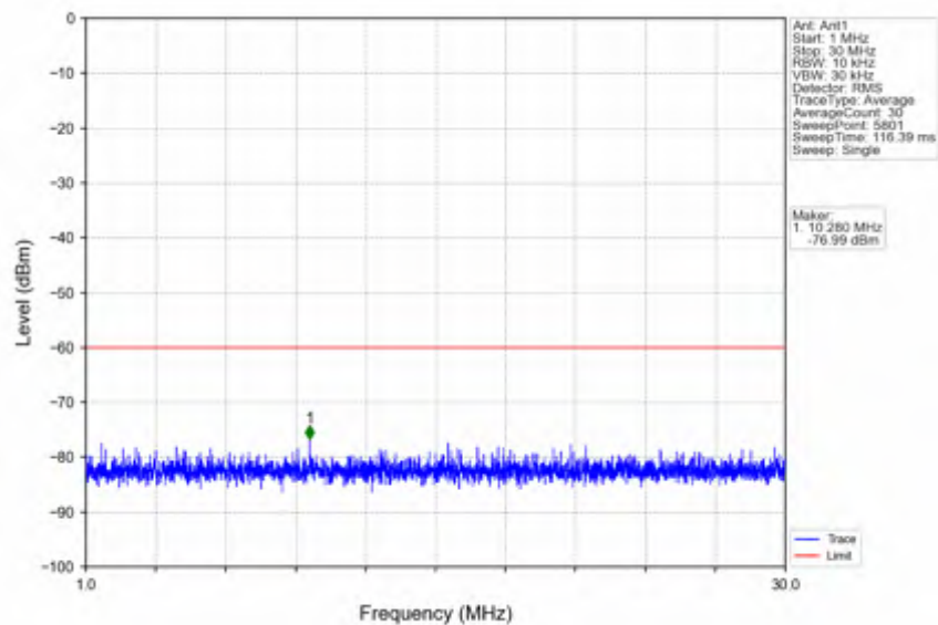
n78d_30kHz_SISO_NTNV_100MHz_CP-OFDM QPSK_3649.98MHz_Outer_Full
