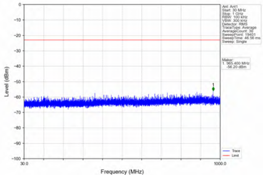
n78e_15kHz_SISO_NTNV_10MHz_CP-OFDM QPSK_3544.995MHz_Edge_1RB_Right
