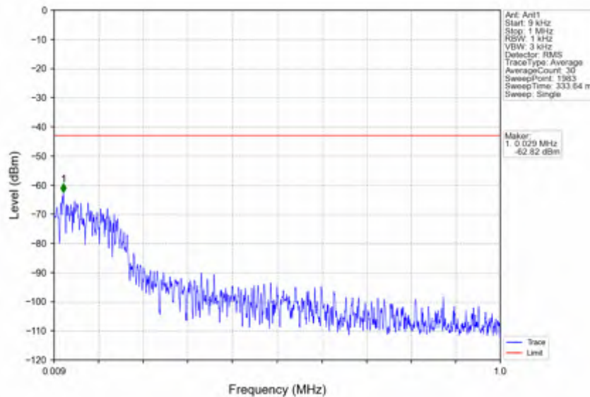
n78e_15kHz_SISO_NTNV_15MHz_CP-OFDM QPSK_3457.5MHz_Inner_1RB_Left
