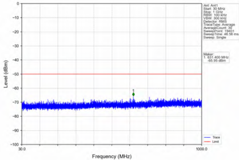
n78d_30kHz_SISO_NTNV_100MHz_DFT-s-OFDM QPSK_3600MHz_Edge_1RB_Left
