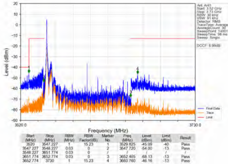
n78d_30kHz_SISO_NTNV_100MHz_DFT-s-OFDM PI/2 BPSK_3600MHz_Inner_1RB_Left
