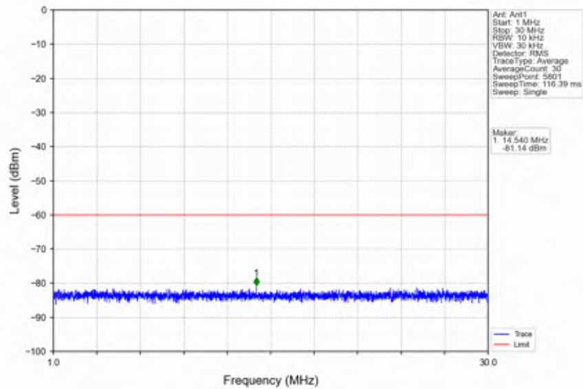
n78d_30kHz_SISO_NTNV_60MHz_DFT-s-OFDM_QPSK_3624.99MHz_Edge_1RB_Left
