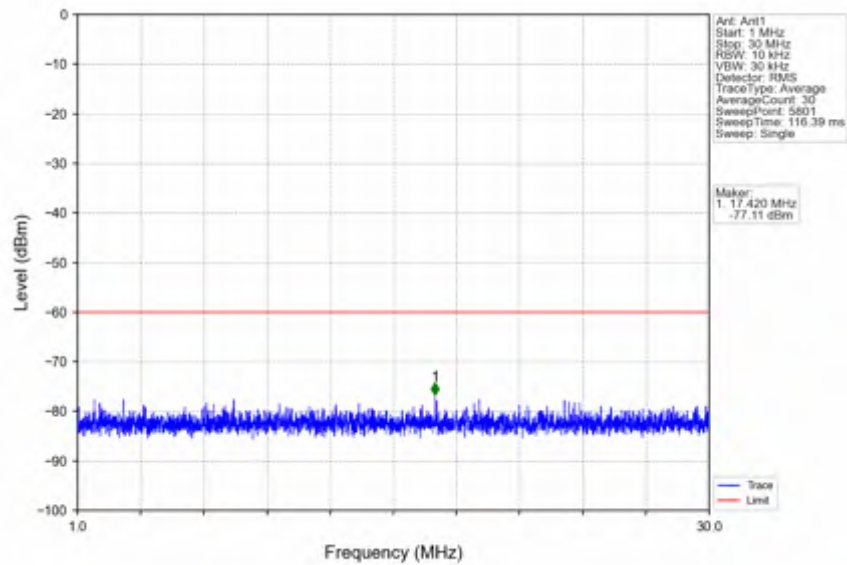
n78d_30kHz_SISO_NTNV_60MHz_CP-OFDM QPSK_3669.99MHz_Edge_1RB_Right
