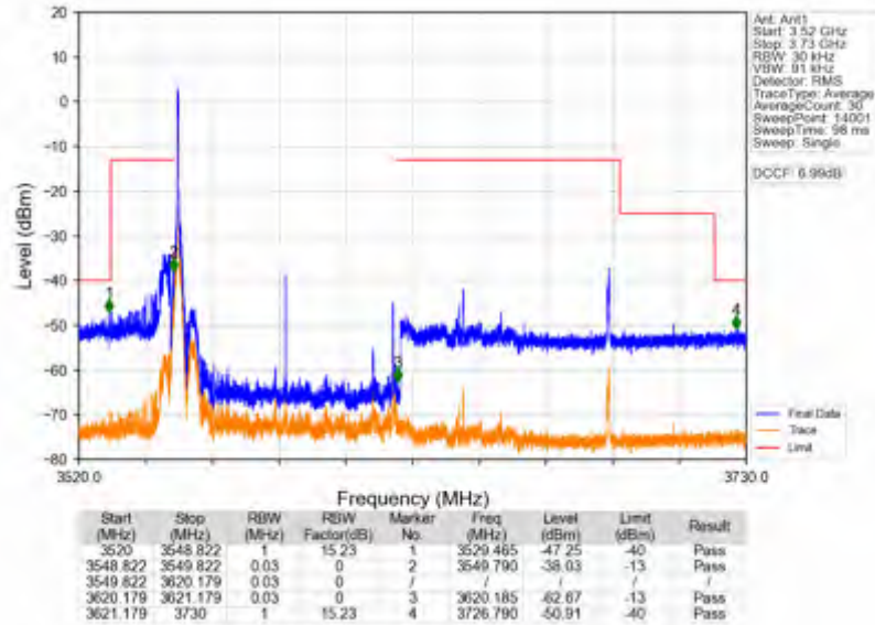
n78d_30kHz_SISO_NTNV_70MHz_DFT-s-OFDM PI/2 BPSK_3585MHz_Edge_1RB_Left
