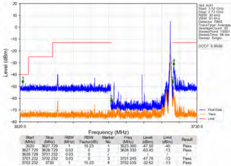
n78d_30kHz_SISO_NTNV_70MHz_DFT-s-OFDM QPSK_3664.98MHz_Inner_1RB_Right
