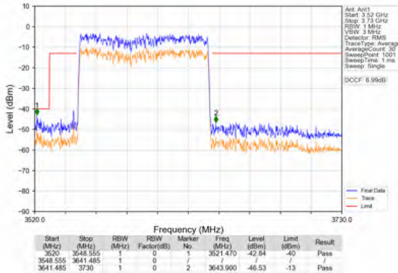
n78d_30kHz_SISO_NTNV_90MHz_DFT-s-OFDM_QPSK_3595.02MHz_Outer_Full
