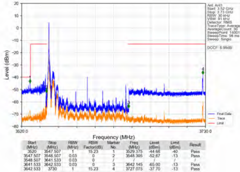
n78d_30kHz_SISO_NTNV_90MHz_DFT-s-OFDM PI/2 BPSK_3595.02MHz_Edge_1RB_Left
