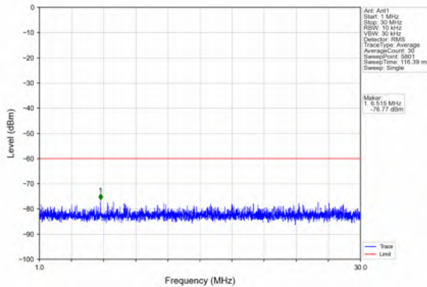
n78d_30kHz_SISO_NTNV_70MHz_DFT-s-OFDM_QPSK_3664.98MHz_Outer_Full
