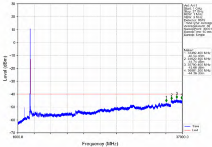
n78d_30kHz_SISO_NTNV_80MHz_DFT-s-OFDM PI/2 BPSK_3660MHz_Outer_Full
