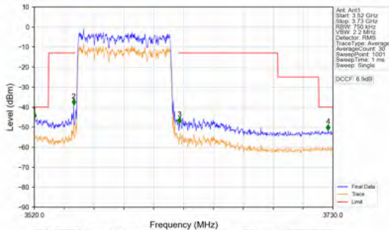
n78d_30kHz_SISO_NTNV_70MHz_DFT-s-OFDM PI/2 BPSK_3585MHz_Outer_Full
