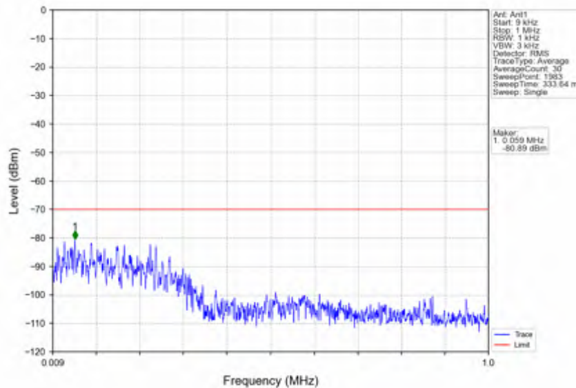
n78d_30kHz_SISO_NTV_70MHz_CP-OFDM QPSK_3664.98MHz_Edge_1RB_Right
