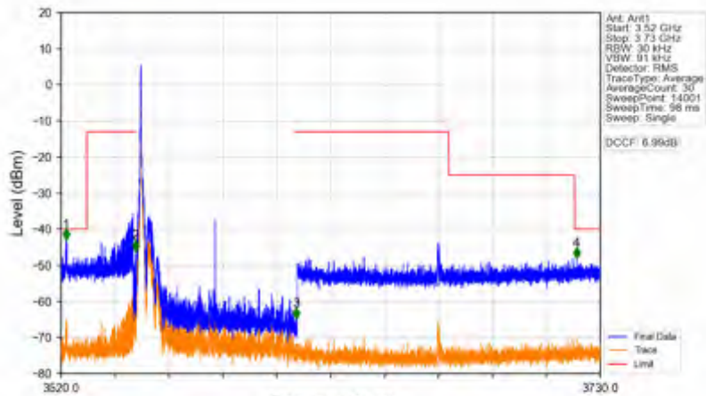
n78d_30kHz_SISO_NTNV_60MHz_DFT-s-OFDM QPSK_3580.02MHz_Edge_1RB_Left
