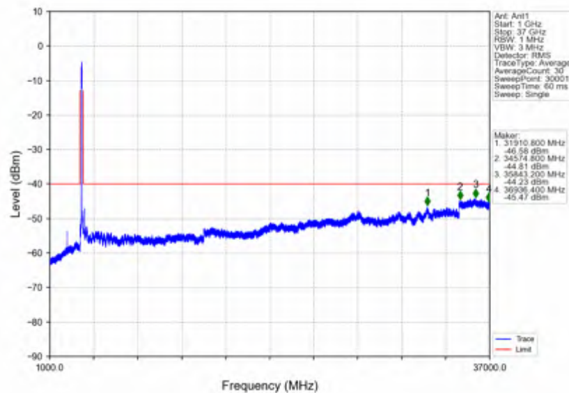
n78d_30kHz_SISO_NTNV_90MHz_DFT-s-OFDM PI/2 BPSK_3595.02MHz_Outer_Full
