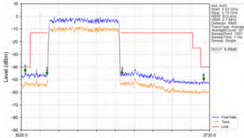
n78d_30kHz_SISO_NTNV_80MHz_DFT-s-OFDM PI/2 BPSK_3590.01MHz_Outer_Full
