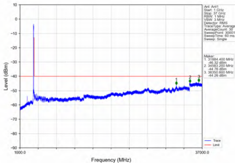
n78d_30kHz_SISO_NTNV_70MHz_DFT-s-OFDM PI/2 BPSK_3664.98MHz_Outer_Full
