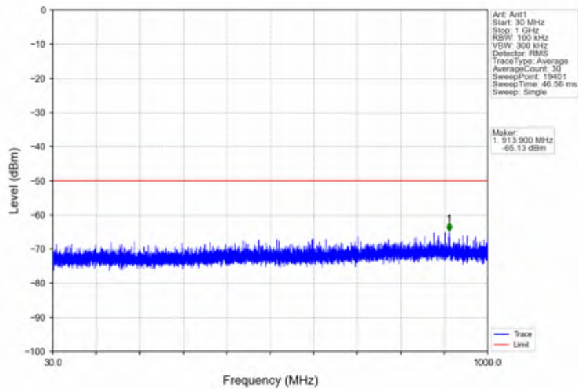
n78d_30kHz_SISO_NTNV_60MHz_DFT-s-OFDM_QPSK_3580.02MHz_Inner_1RB_Left
