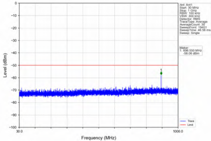
n78d_30kHz_SISO_NTV_70MHz_DFT-s-OFDM_QPSK_3585MHz_Inner_1RB_Left
