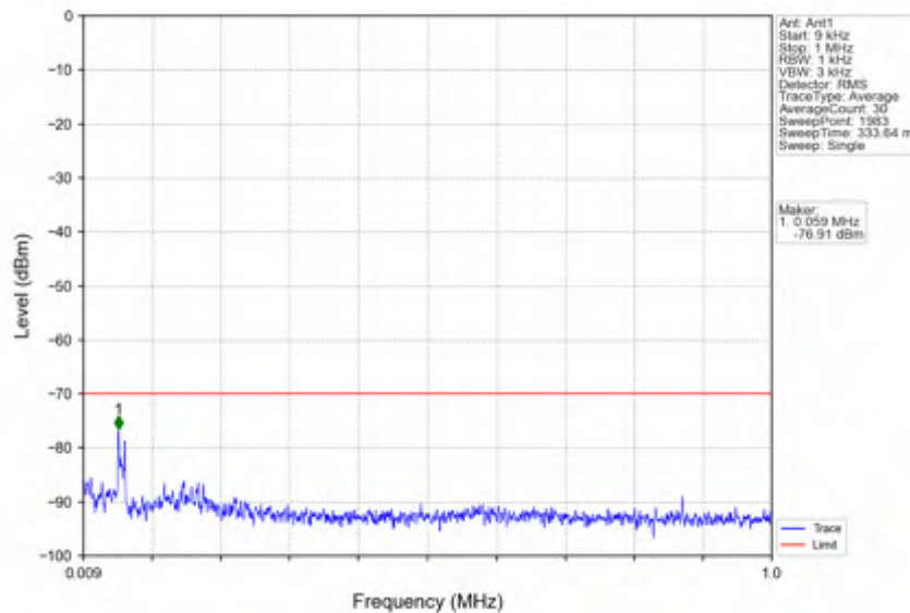
n78d_30kHz_SISO_NTV_60MHz_CP-OFDM_QPSK_3580.02MHz_Edge_1RB_Left
