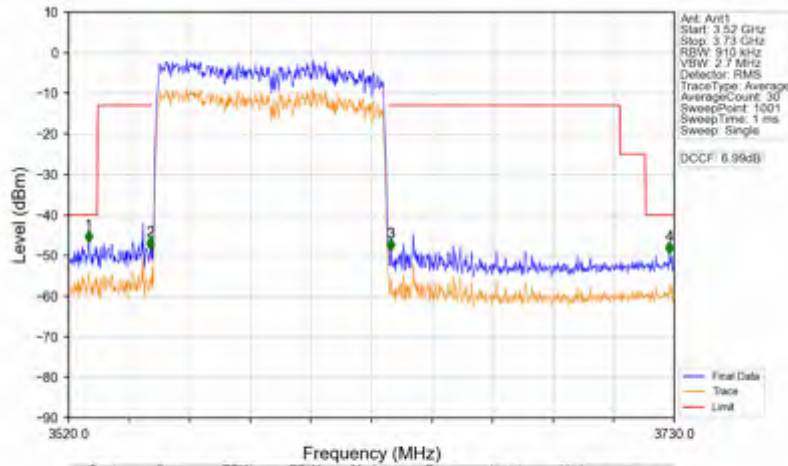
n78d_30kHz_SISO_NTNV_80MHz_CP-OFDM QPSK_3590.01MHz_Outer_Full
