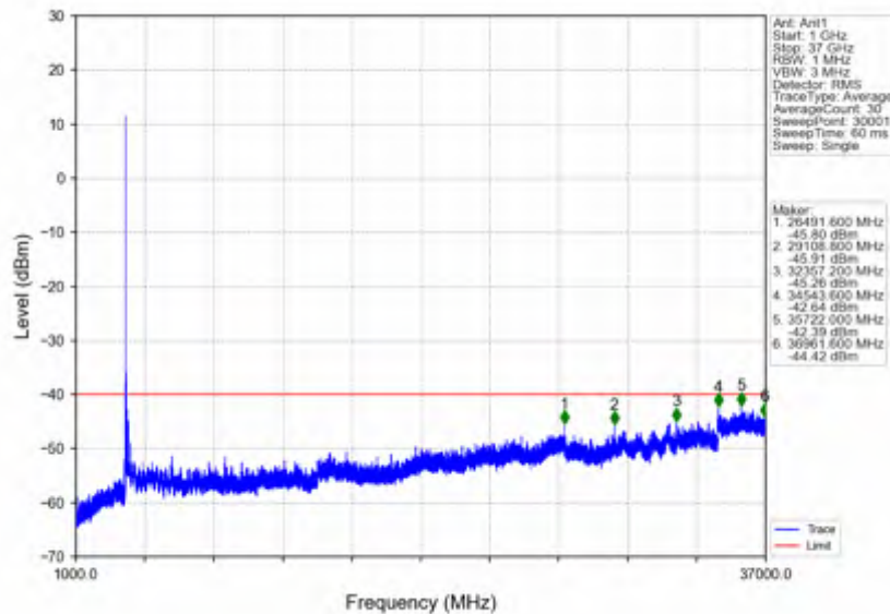
n78d_30kHz_SISO_NTVV_70MHz_CP-OFDM QPSK_3624.99MHz_Edge_1RB_Left
