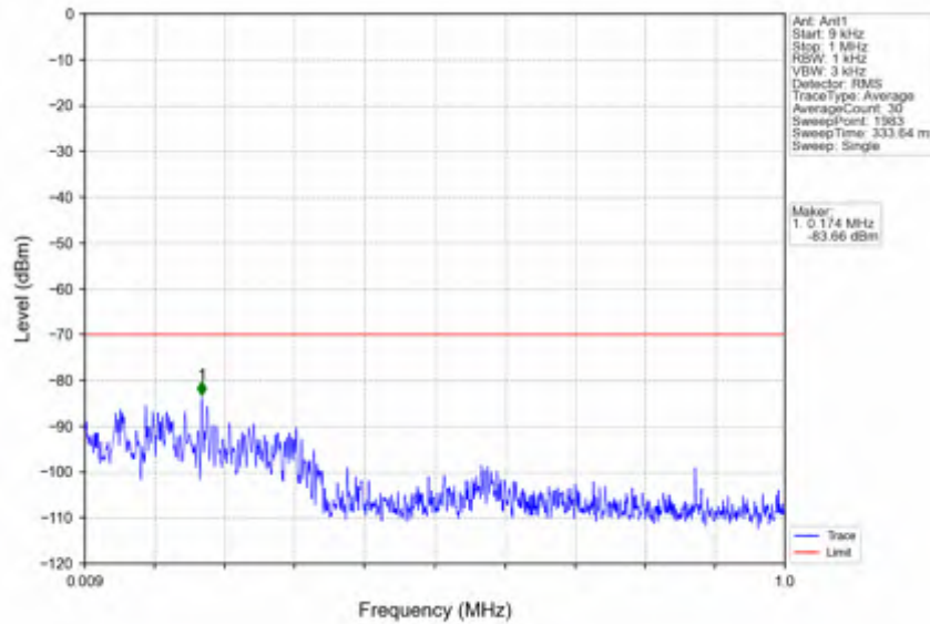
n78d_30kHz_SISO_NTNV_60MHz_DFT-s-OFDM QPSK_3669.99MHz_Edge_1RB_Right
