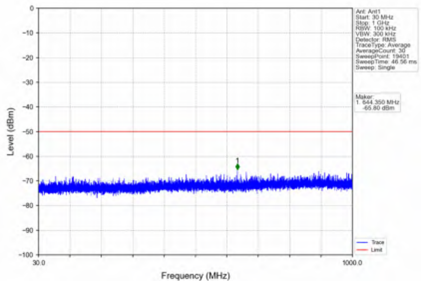
n78d_30kHz_SISO_NTNV_70MHz_DFT-s-OFDM_QPSK_3585MHz_Outer_Full
