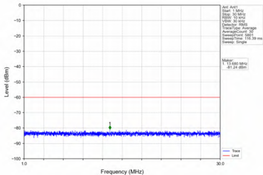
n78d_30kHz_SISO_NTNV_90MHz_DFT-s-OFDM PI/2 BPSK_3595.02MHz_Outer_Full
