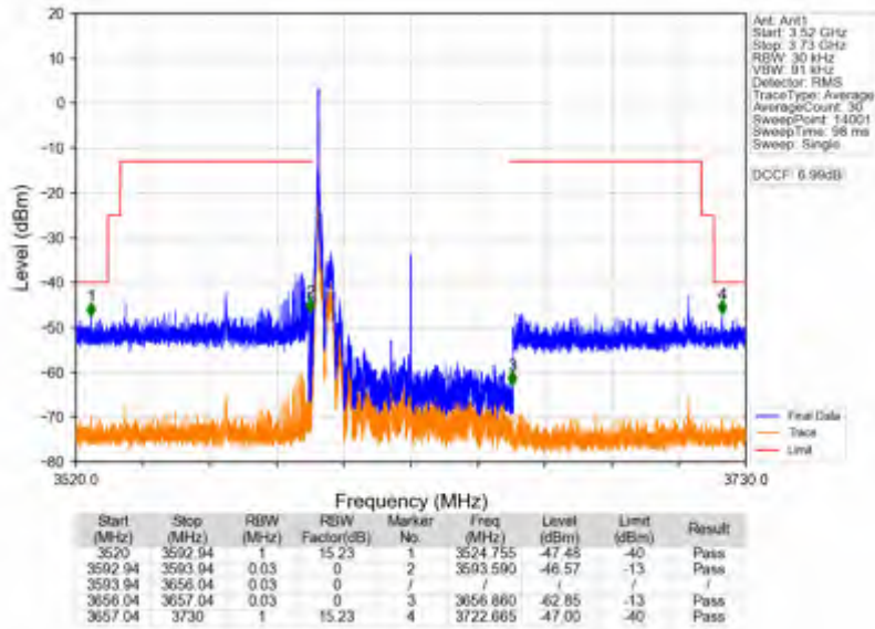
n78d_30kHz_SISO_NTV_60MHz_CP-OFDM_QPSK_3624.99MHz_Edge_1RB_Left
