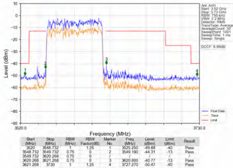
n78d_30kHz_SISO_NTNV_70MHz_DFT-s-OFDM_QPSK_3585MHz_Outer_Full
