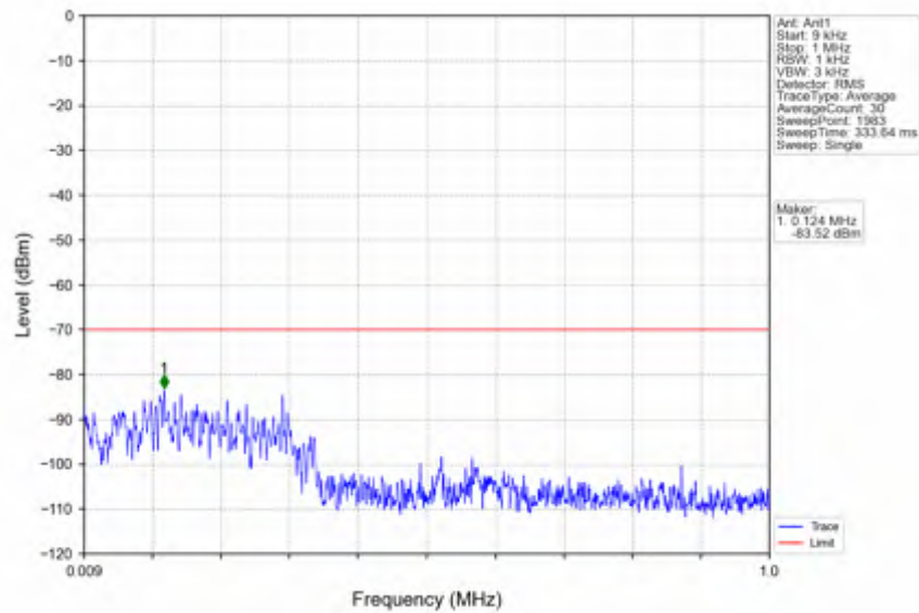
n78d_30kHz_SISO_NTNV_60MHz_DFT-s-OFDM_QPSK_3580.02MHz_Edge_1RB_Left
