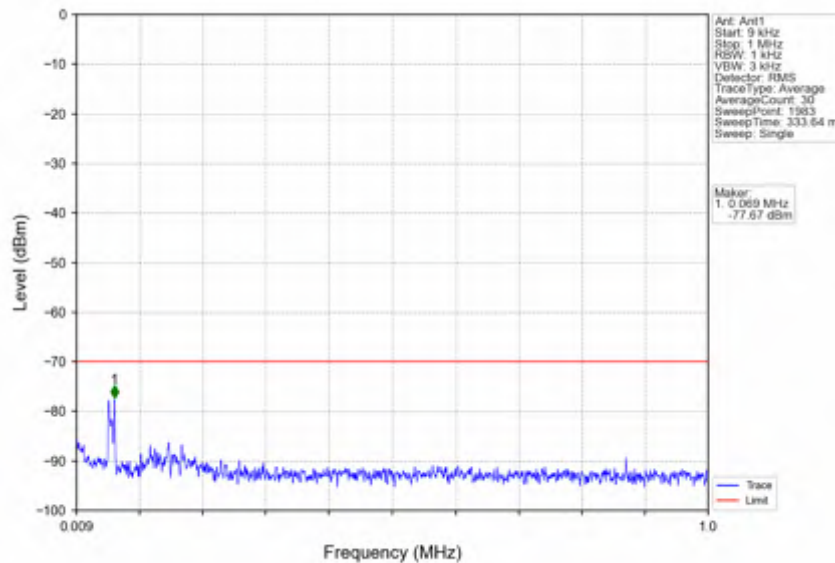
n78d_30kHz_SISO_NTNV_60MHz_DFT-s-OFDM_QPSK_3624.99MHz_Edge_1RB_Left
