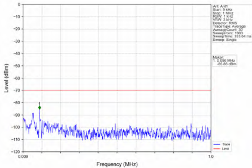
n78d_30kHz_SISO_NTNV_70MHz_CP-OFDM QPSK_3585MHz_Outer_Full
