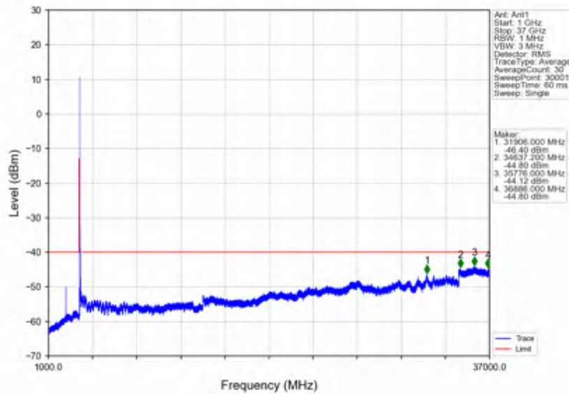
n78d_30kHz_SISO_NTNV_60MHz_DFT-s-OFDM PI/2 BPSK_3624.99MHz_Edge_1RB_Left
