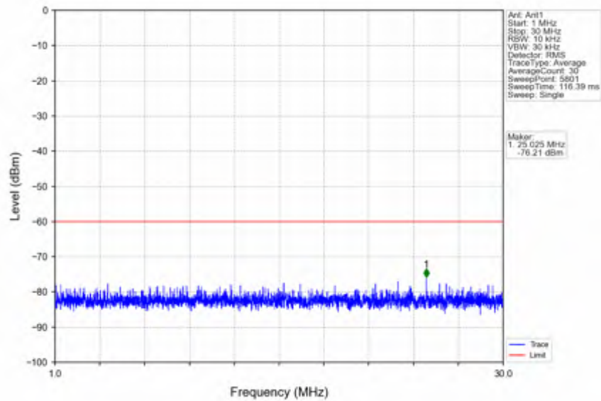
n78d_30kHz_SISO_NTVV_80MHz_CP-OFDM_QPSK_3590.01MHz_Edge_1RB_Left
