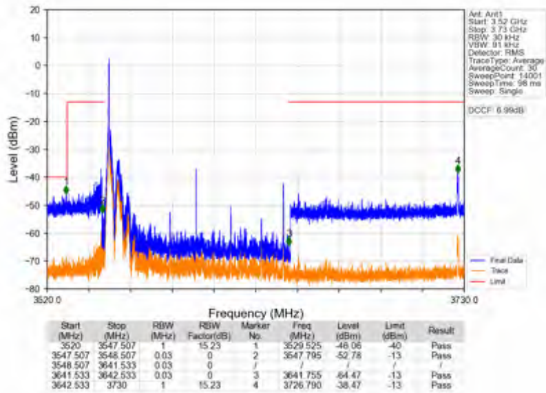
n78d_30kHz_SISO_NTNV_90MHz_DFT-s-OFDM QPSK_3595.02MHz_Edge_1RB_Left
