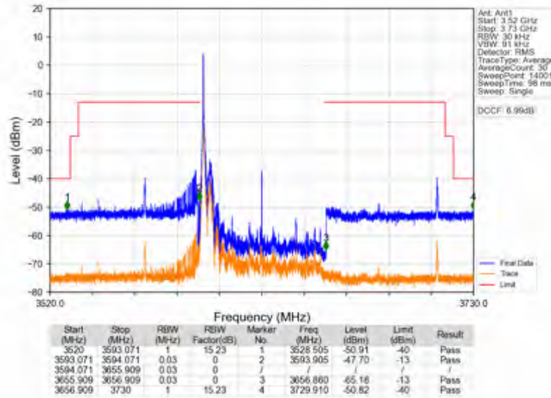
n78d_30kHz_SISO_NTNV_60MHz_DFT-s-OFDM_QPSK_3624.99MHz_Edge_1RB_Left
