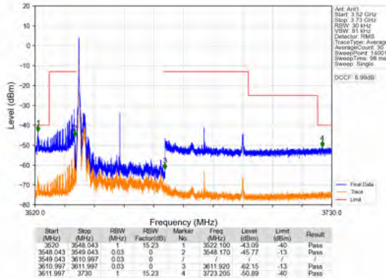
n78d_30kHz_SISO_NTV_60MHz_CP-OFDM_QPSK_3580.02MHz_Edge_1RB_Left
