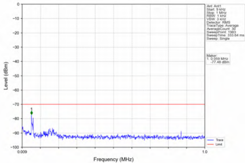
n78d_30kHz_SISO_NTNV_80MHz_DFT-s-OFDM PI/2 BPSK_3660MHz_Outer_Full
