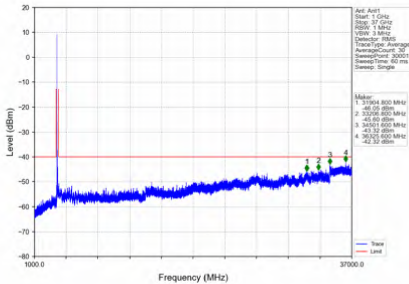
n78d_30kHz_SISO_NTNV_90MHz_DFT-s-OFDM QPSK_3595.02MHz_Edge_1RB_Left
