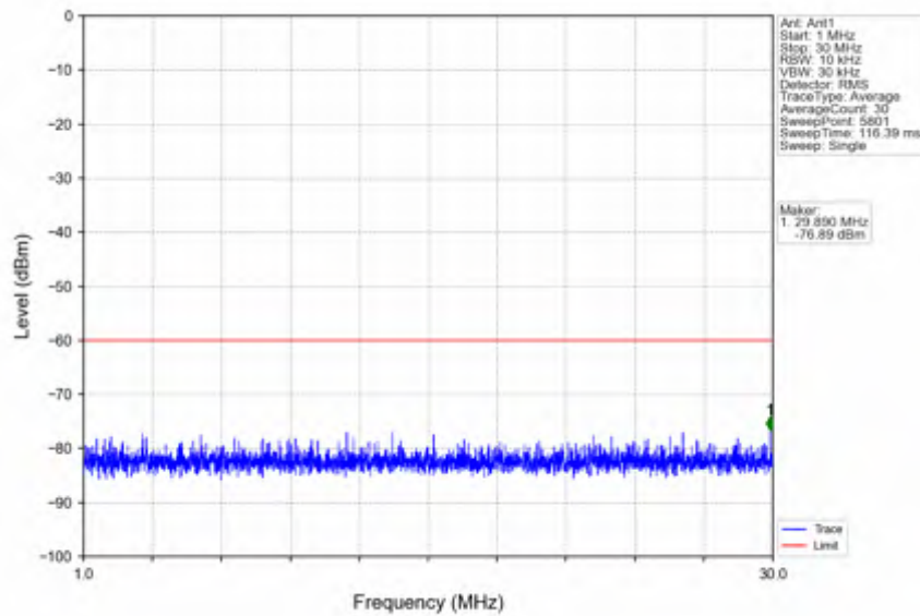
n78d_30kHz_SISO_NTNV_80MHz_DFT-s-OFDM_QPSK_3590.01MHz_Outer_Full
