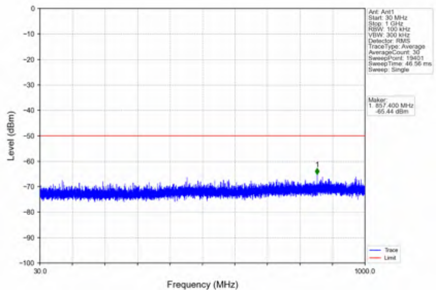
n78d_30kHz_SISO_NTNV_70MHz_CP-OFDM QPSK_3664.98MHz_Edge_1RB_Right
