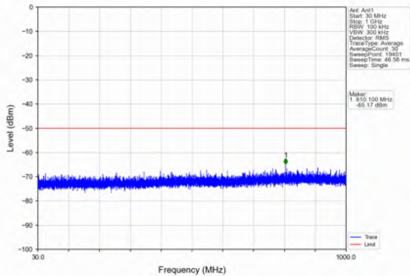
n78d_30kHz_SISO_NTV_60MHz_CP-OFDM QPSK_3624.99MHz_Edge_1RB_Left
