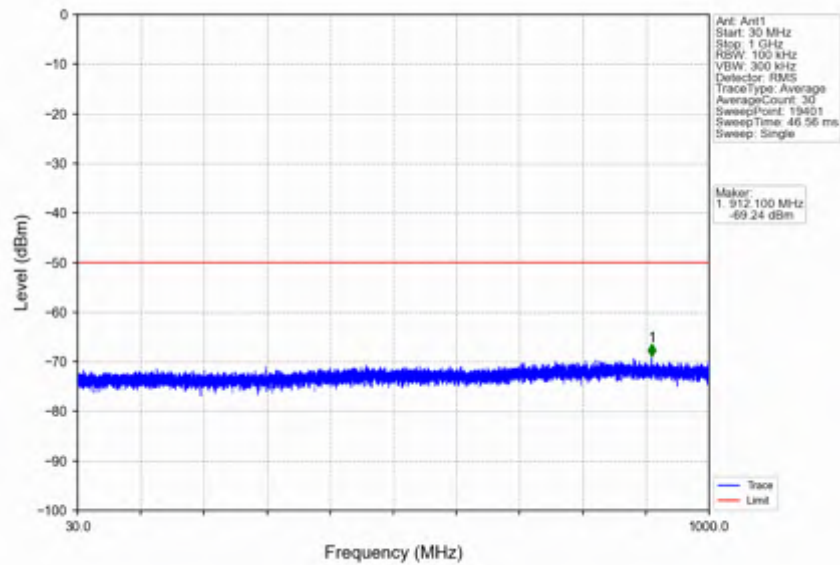
n78d_30kHz_SISO_NTNV_70MHz_DFT-s-OFDM PI/2 BPSK_3585MHz_Outer_Full
