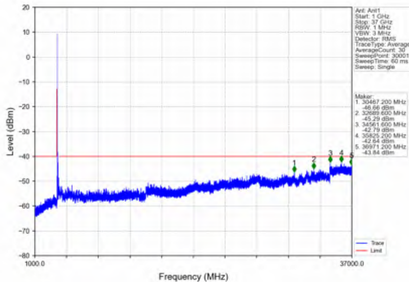
n78d_30kHz_SISO_NTV_70MHz_DFT-s-OFDM QPSK_3585MHz_Edge_1RB_Left
