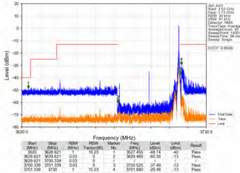
n78d_30kHz_SISO_NTV_70MHz_CP-OFDM QPSK_3664.98MHz_Edge_1RB_Right
