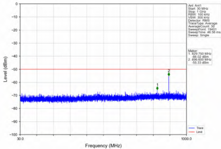
n78d_30kHz_SISO_NTNV_60MHz_DFT-s-OFDM QPSK_3669.99MHz_Inner_1RB_Right
