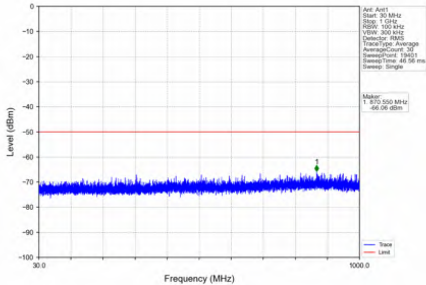
n78d_30kHz_SISO_NTNV_80MHz_CP-OFDM QPSK_3590.01MHz_Outer_Full
