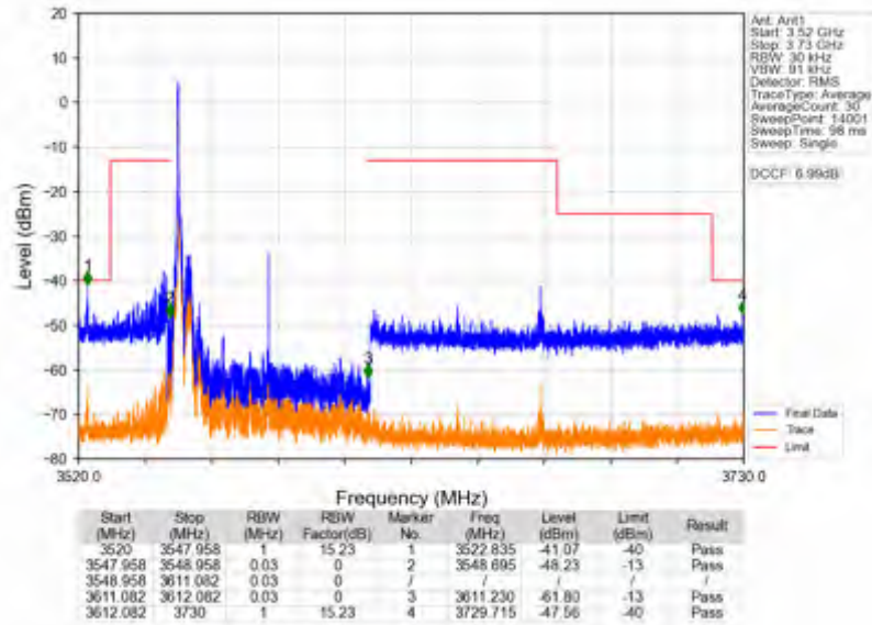
n78d_30kHz_SISO_NTV_60MHz_CP-OFDM_QPSK_3580.02MHz_Inner_1RB_Left
