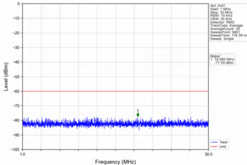
n78d_30kHz_SISO_NTNV_90MHz_DFT-s-OFDM QPSK_3595.02MHz_Inner_1RB_Left
