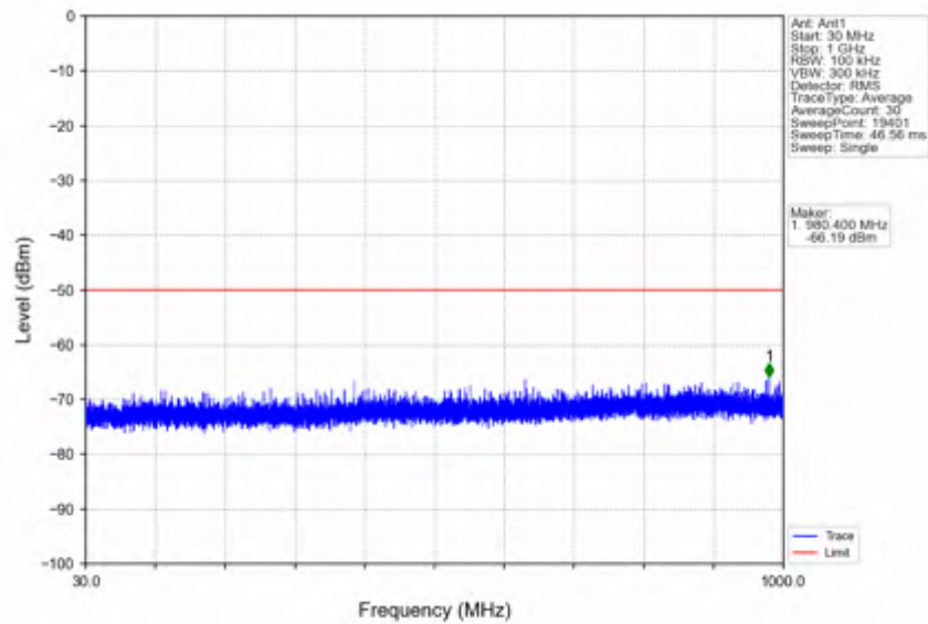
n78d_30kHz_SISO_NTNV_70MHz_CP-OFDM QPSK_3664.98MHz_Outer_Full
