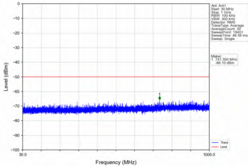
n78d_30kHz_SISO_NTVV_80MHz_CP-OFDM QPSK_3624.99MHz_Edge_1RB_Left
