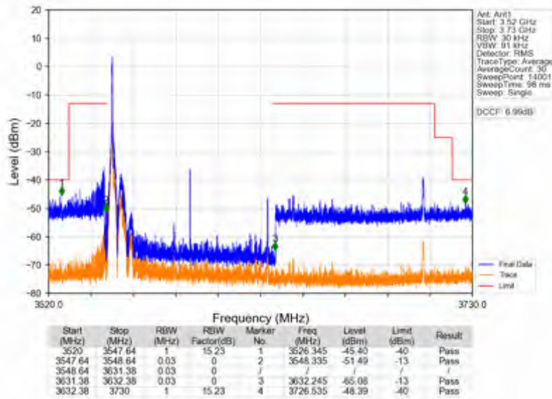
n78d_30kHz_SISO_NTNV_80MHz_DFT-s-OFDM QPSK_3590.01MHz_Inner_1RB_Left
