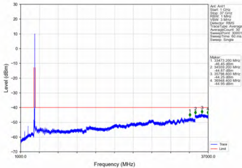
n78d_30kHz_SISO_NTNV_90MHz_DFT-s-OFDM PI/2 BPSK_3654.99MHz_Outer_Full
