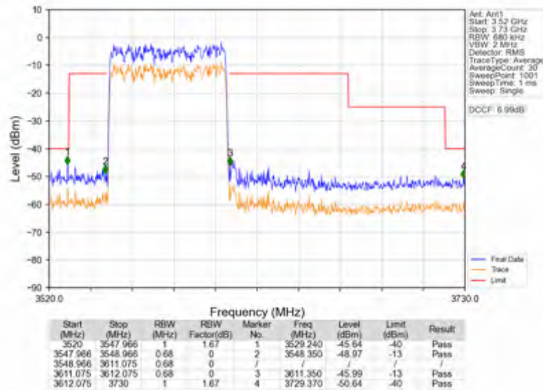
n78d_30kHz_SISO_NTNV_60MHz_DFT-s-OFDM_QPSK_3580.02MHz_Outer_Full
