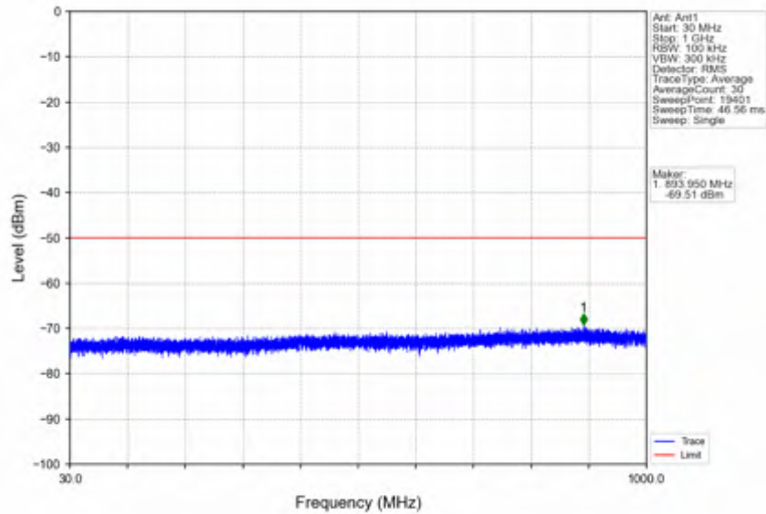
n78d_30kHz_SISO_NTNV_90MHz_DFT-s-OFDM PI/2 BPSK_3654.99MHz_Outer_Full
