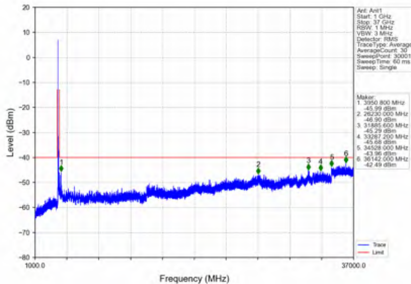
n78d_30kHz_SISO_NTVV_80MHz_CP-OFDM QPSK_3624.99MHz_Edge_1RB_Left
