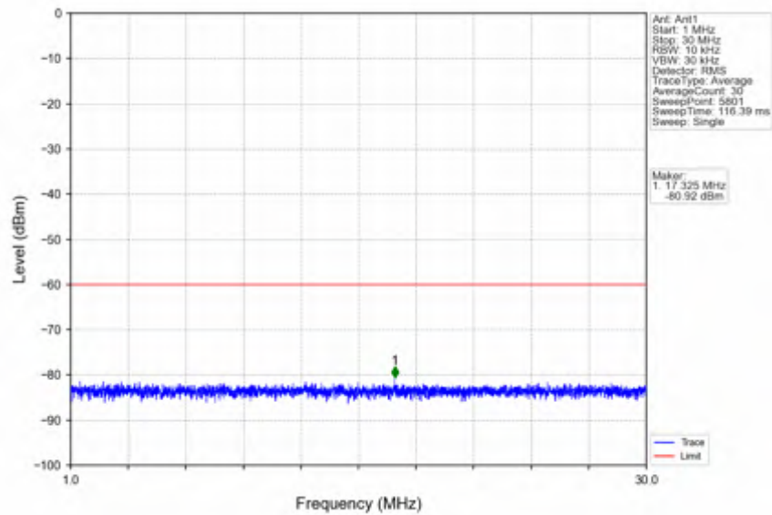
n78d_30kHz_SISO_NTNV_80MHz_DFT-s-OFDM_PI/2_BPSK_3660MHz_Inner_1RB_Right
