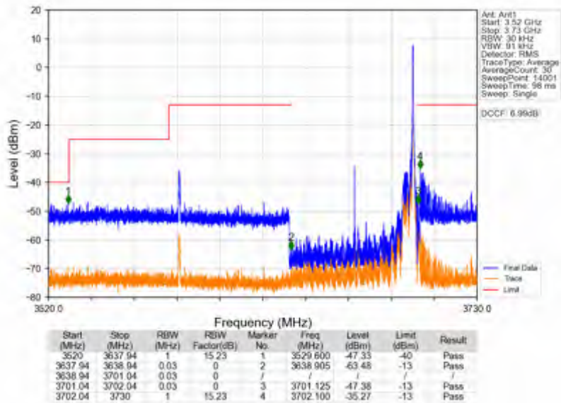
n78d_30kHz_SISO_NTNV_60MHz_DFT-s-OFDM_QPSK_3669.99MHz_Inner_1RB_Right
