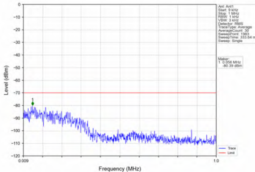
n78d_30kHz_SISO_NTV_80MHz_CP-OFDM QPSK_3590.01MHz_Edge_1RB_Left
