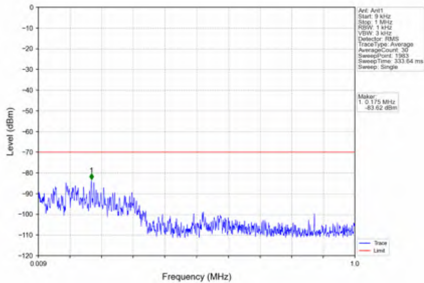
n78d_30kHz_SISO_NTNV_80MHz_DFT-s-OFDM_QPSK_3590.01MHz_Inner_1RB_Left
