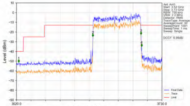
n78d_30kHz_SISO_NTNV_70MHz_CP-OFDM QPSK_3664.98MHz_Outer_Full
