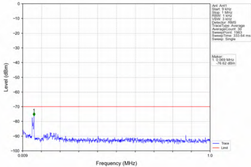
n78d_30kHz_SISO_NTNV_80MHz_DFT-s-OFDM PI/2 BPSK_3590.01MHz_Outer_Full
