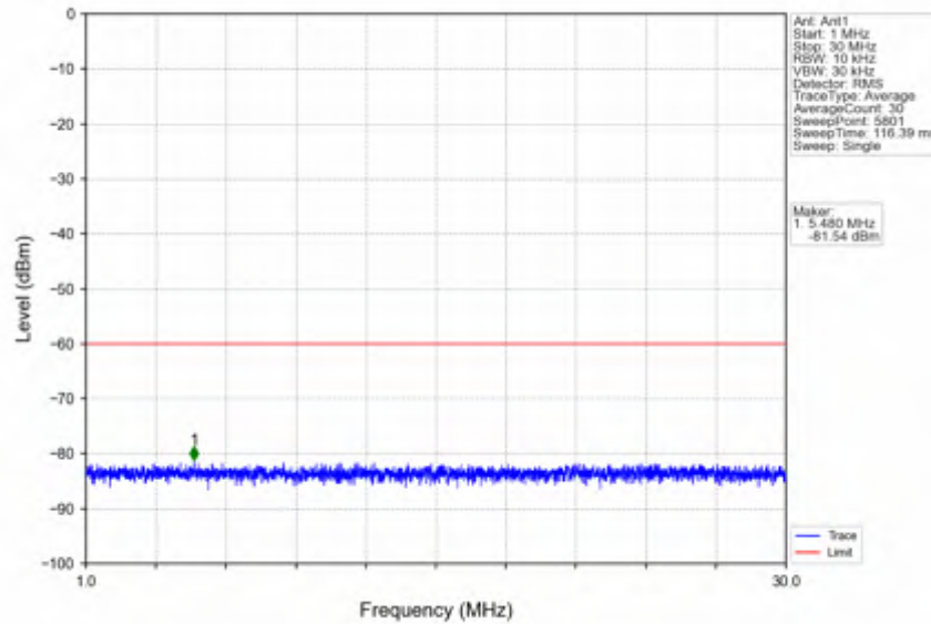
n78d_30kHz_SISO_NTNV_90MHz_DFT-s-OFDM PI/2 BPSK_3595.02MHz_Edge_1RB_Left
