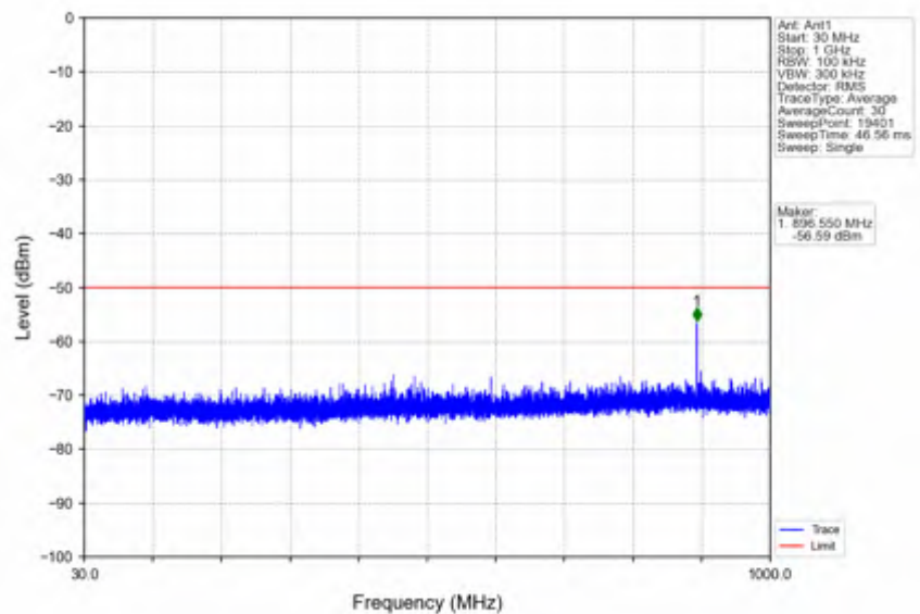
n78d_30kHz_SISO_NTNV_60MHz_CP-OFDM QPSK_3669.99MHz_Inner_1RB_Right
