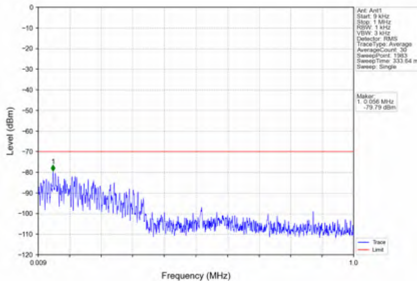
n78d_30kHz_SISO_NTNV_80MHz_CP-OFDM QPSK_3660MHz_Inner_1RB_Right
