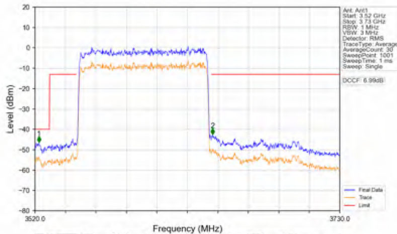
n78d_30kHz_SISO_NTNV_90MHz_DFT-s-OFDM PI/2 BPSK_3595.02MHz_Outer_Full
