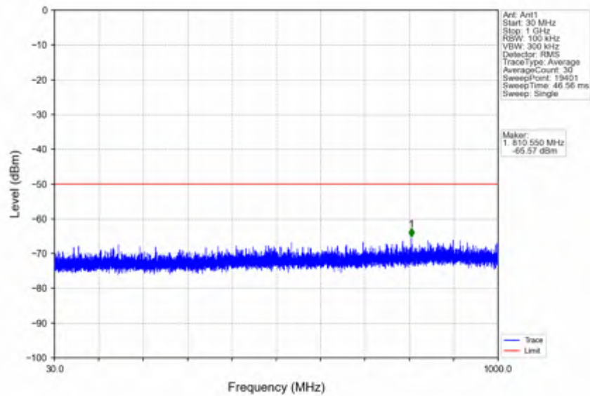
n78d_30kHz_SISO_NTNV_90MHz_DFT-s-OFDM QPSK_3595.02MHz_Inner_1RB_Left
