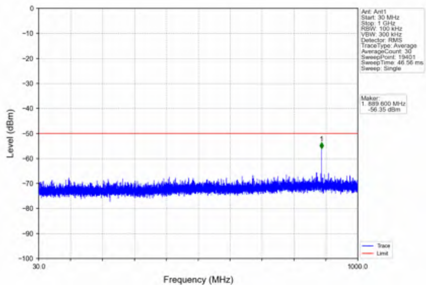
n78d_30kHz_SISO_NTNV_70MHz_DFT-s-OFDM QPSK_3624.99MHz_Edge_1RB_Left
