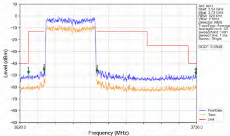
n78d_30kHz_SISO_NTNV_60MHz_CP-OFDM_QPSK_3580.02MHz_Outer_Full
