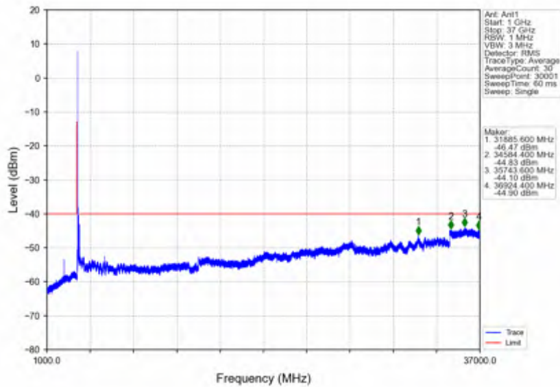
n78d_30kHz_SISO_NTNV_80MHz_DFT-s-OFDM PI/2 BPSK_3590.01MHz_Outer_Full
