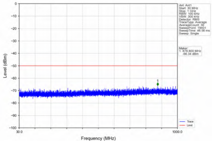
n78d_30kHz_SISO_NTVV_80MHz_CP-OFDM_QPSK_3590.01MHz_Inner_1RB_Left
