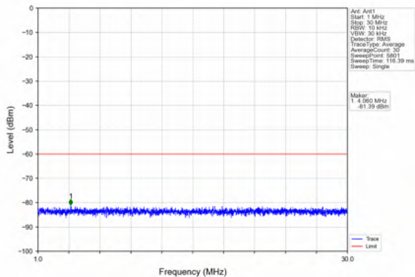
n78d_30kHz_SISO_NTNV_70MHz_DFT-s-OFDM PI/2 BPSK_3664.98MHz_Outer_Full
