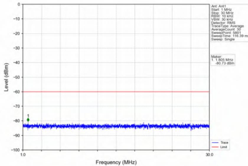
n78d_30kHz_SISO_NTNV_80MHz_DFT-s-OFDM PI/2 BPSK_3590.01MHz_Inner_1RB_Left
