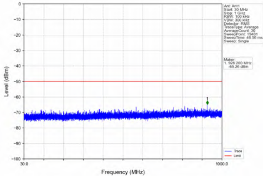
n78d_30kHz_SISO_NTVV_70MHz_CP-OFDM QPSK_3624.99MHz_Edge_1RB_Left
