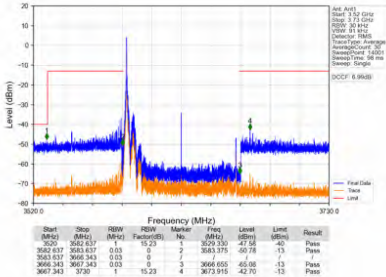
n78d_30kHz_SISO_NTV_80MHz_CP-OFDM_QPSK_3624.99MHz_Edge_1RB_Left
