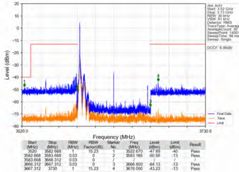
n78d_30kHz_SISO_NTNV_80MHz_DFT-s-OFDM QPSK_3624.99MHz_Edge_1RB_Left
