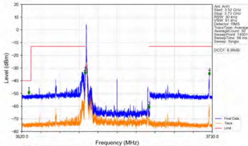
n78d_30kHz_SISO_NTNV_70MHz_DFT-s-OFDM PI/2 BPSK_3624.99MHz_Edge_1RB_Left
