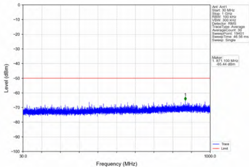
n78d_30kHz_SISO_NTNV_80MHz_DFT-s-OFDM_QPSK_3624.99MHz_Edge_1RB_Left
