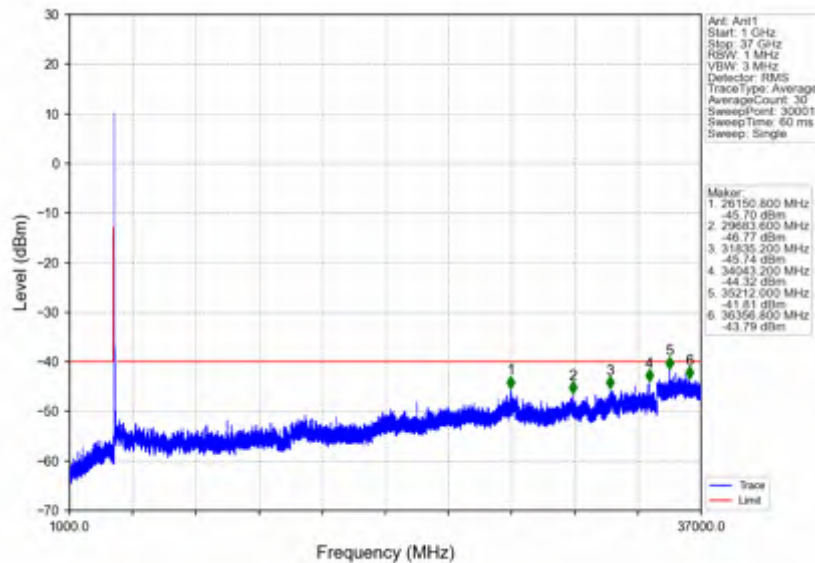
n78d_30kHz_SISO_NTNV_60MHz_DFT-s-OFDM_QPSK_3580.02MHz_Edge_1RB_Left
