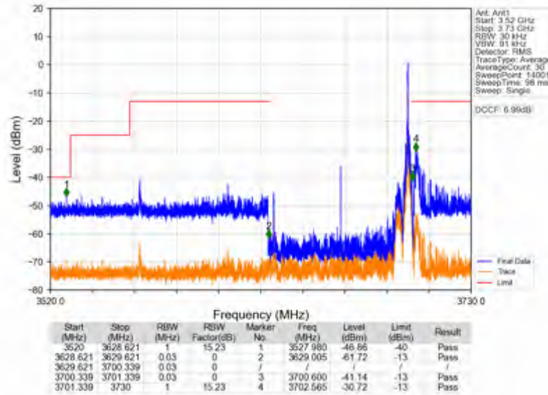
n78d_30kHz_SISO_NTNV_70MHz_CP-OFDM QPSK_3664.98MHz_Inner_1RB_Right
