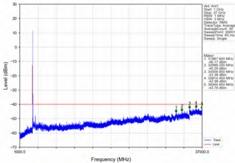
n78d_30kHz_SISO_NTV_80MHz_CP-OFDM_QPSK_3624.99MHz_Edge_1RB_Left
