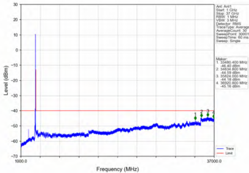
n78d_30kHz_SISO_NTNV_70MHz_DFT-s-OFDM QPSK_3585MHz_Edge_1RB_Left
