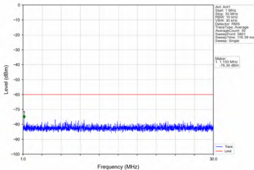
n78d_30kHz_SISO_NTV_60MHz_CP-OFDM QPSK_3624.99MHz_Edge_1RB_Left
