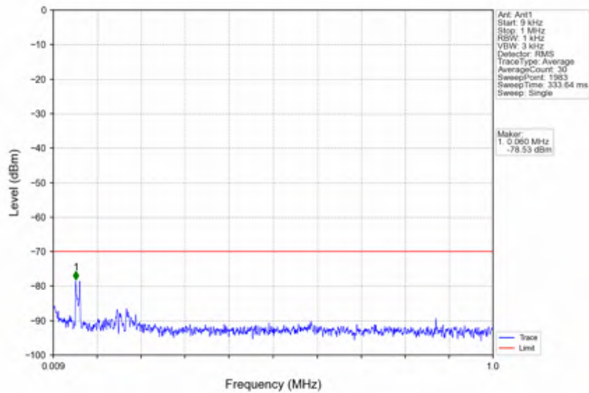
n78d_30kHz_SISO_NTNV_60MHz_DFT-s-OFDM PI/2 BPSK_3580.02MHz_Outer_Full
