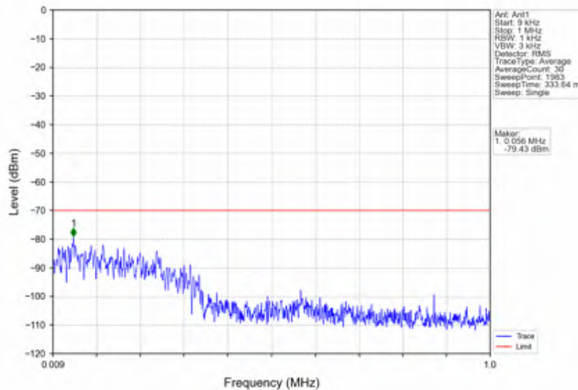
n78d_30kHz_SISO_NTVV_80MHz_CP-OFDM_QPSK_3590.01MHz_Inner_1RB_Left
