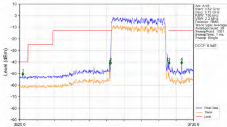
n78d_30kHz_SISO_NTNV_70MHz_DFT-s-OFDM PI/2 BPSK_3664.98MHz_Outer_Full
