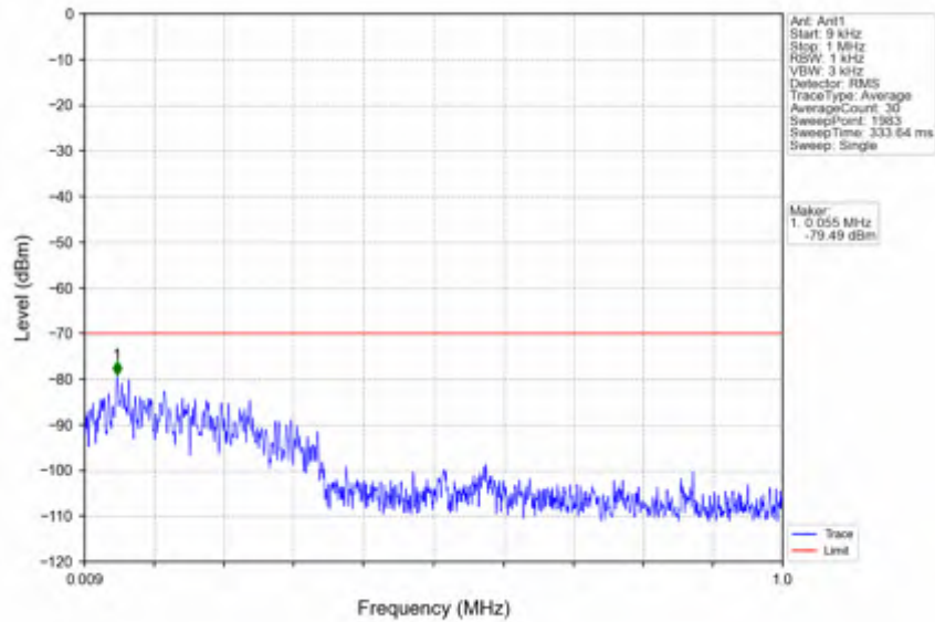
n78d_30kHz_SISO_NTV_70MHz_CP-OFDM QPSK_3624.99MHz_Edge_1RB_Left
