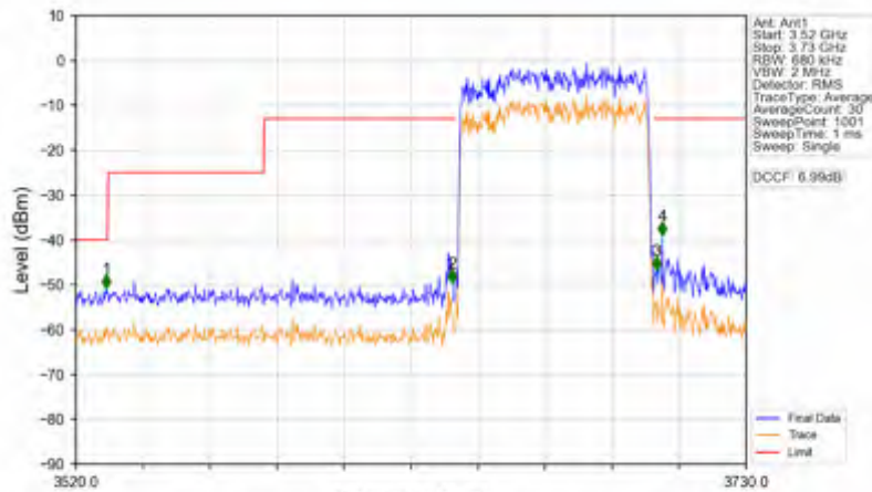
n78d_30kHz_SISO_NTNV_60MHz_CP-OFDM QPSK_3669.99MHz_Outer_Full
