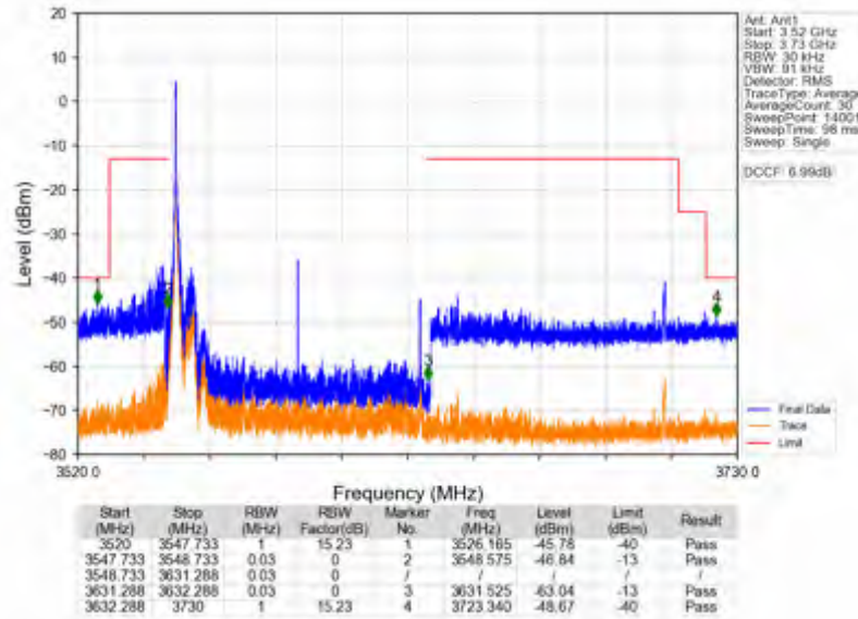
n78d_30kHz_SISO_NTV_80MHz_CP-OFDM QPSK_3590.01MHz_Edge_1RB_Left
