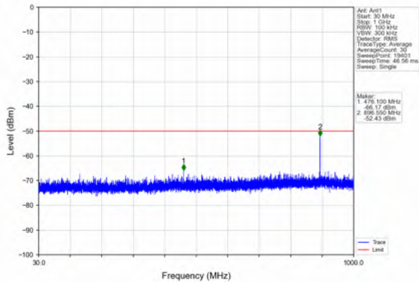
n78d_30kHz_SISO_NTNV_60MHz_CP-OFDM QPSK_3580.02MHz_Outer_Full
