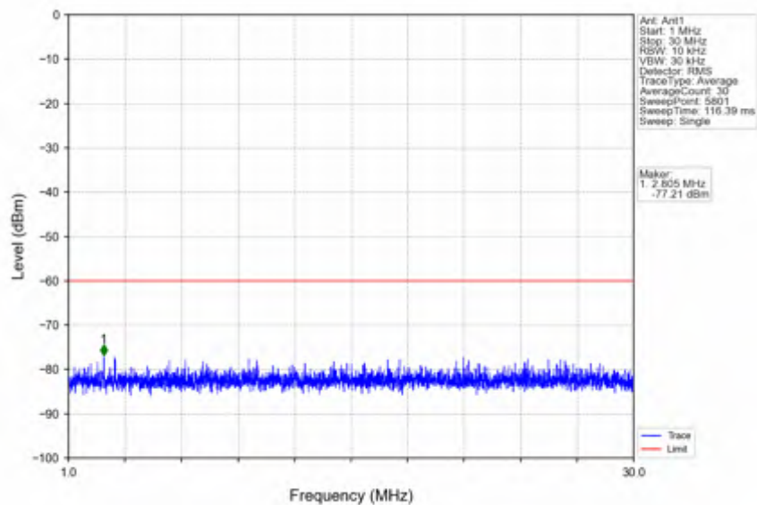
n78d_30kHz_SISO_NTNV_90MHz_DFT-s-OFDM QPSK_3595.02MHz_Edge_1RB_Left
