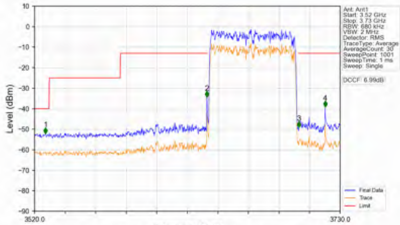
n78d_30kHz_SISO_NTNV_60MHz_DFT-s-OFDM PI/2 BPSK_3669.99MHz_Outer_Full
