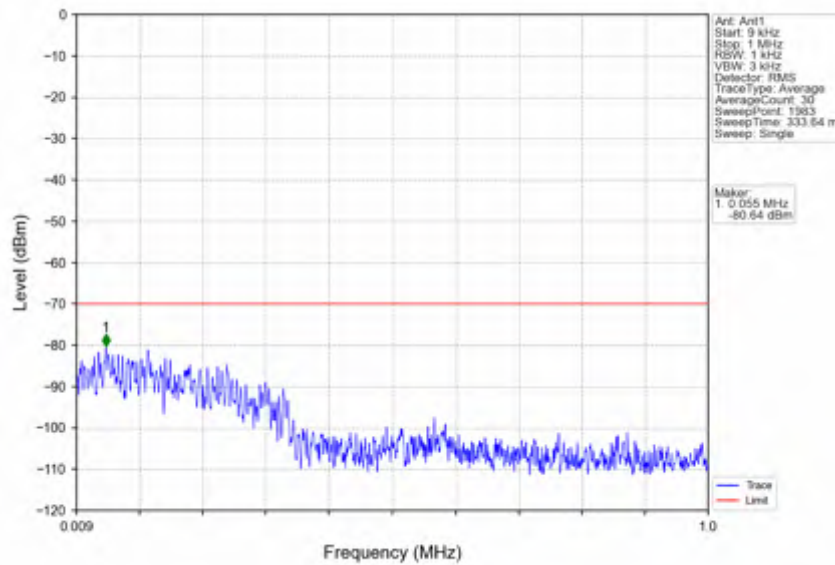
n78d_30kHz_SISO_NTV_60MHz_CP-OFDM_QPSK_3580.02MHz_Inner_1RB_Left
