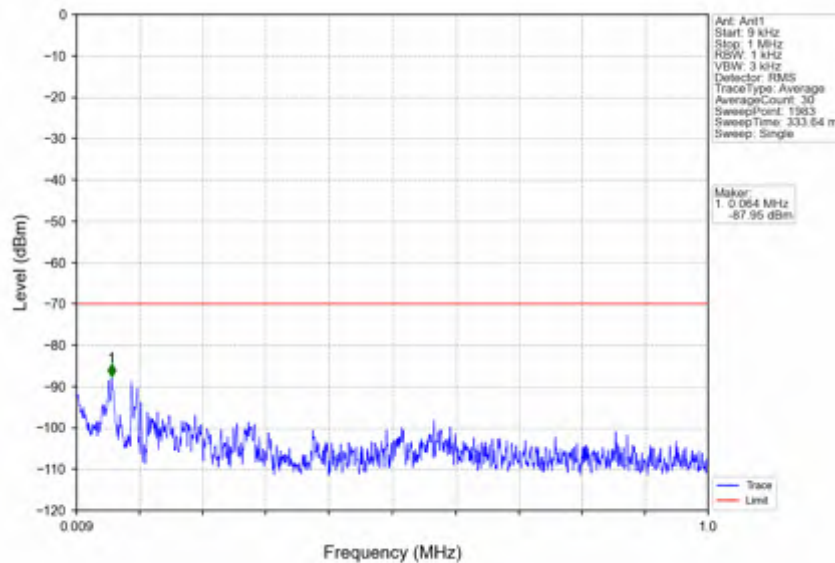
n78d_30kHz_SISO_NTNV_70MHz_DFT-s-OFDM_QPSK_3585MHz_Outer_Full
