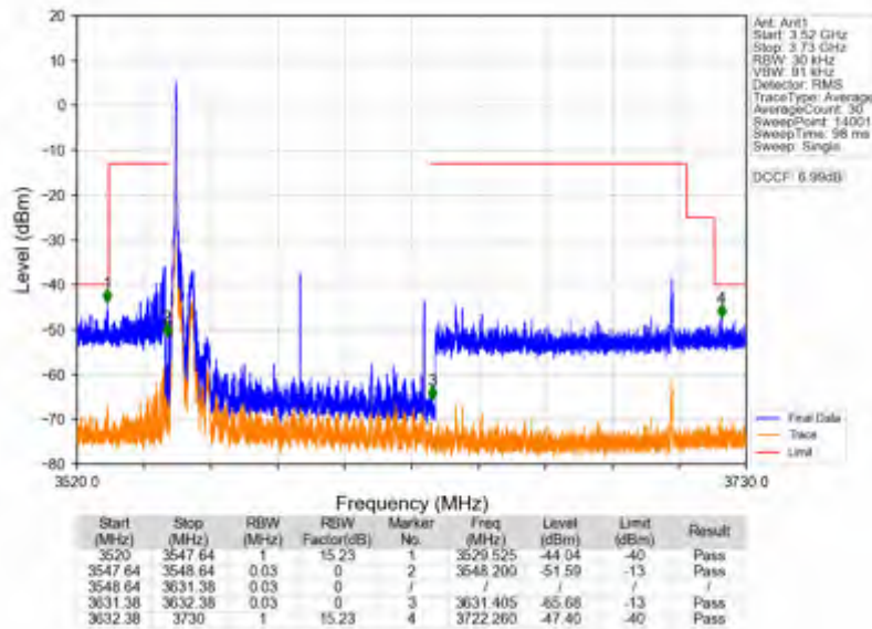
n78d_30kHz_SISO_NTNV_80MHz_DFT-s-OFDM QPSK_3590.01MHz_Edge_1RB_Left
