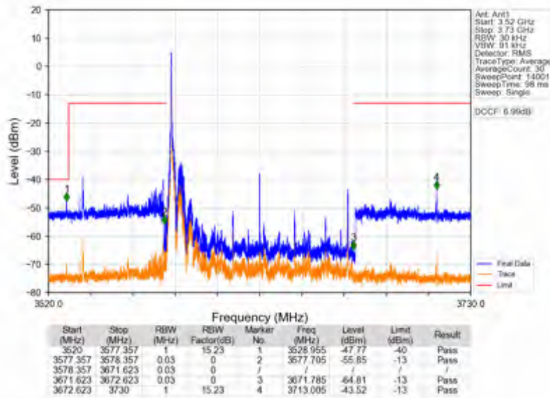
n78d_30kHz_SISO_NTNV_90MHz_DFT-s-OFDM PI/2 BPSK_3624.99MHz_Edge_1RB_Left
