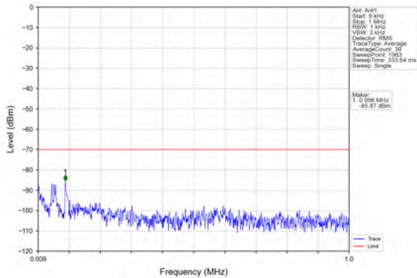
n78d_30kHz_SISO_NTNV_60MHz_CP-OFDM QPSK_3669.99MHz_Outer_Full
