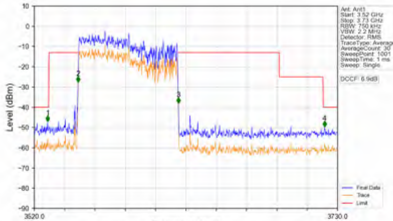
n78d_30kHz_SISO_NTNV_70MHz_CP-OFDM QPSK_3585MHz_Outer_Full
