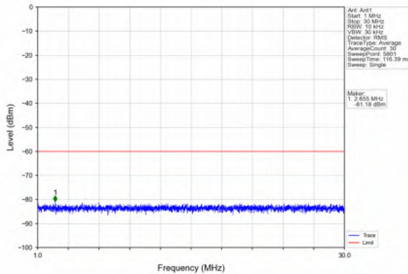
n78d_30kHz_SISO_NTNV_70MHz_DFT-s-OFDM PI/2 BPSK_3664.98MHz_Edge_1RB_Right
