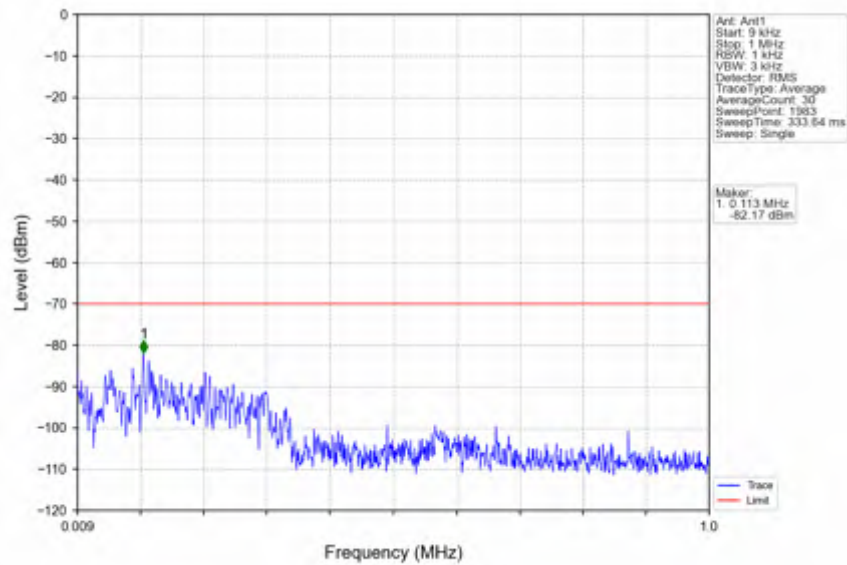
n78d_30kHz_SISO_NTNV_80MHz_DFT-s-OFDM QPSK_3660MHz_Inner_1RB_Right
