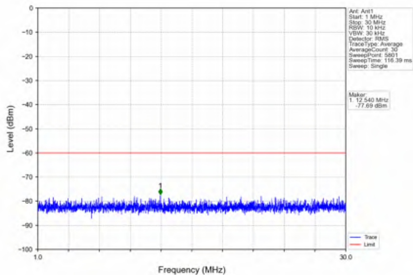
n78d_30kHz_SISO_NTVV_80MHz_CP-OFDM_QPSK_3624.99MHz_Edge_1RB_Left
