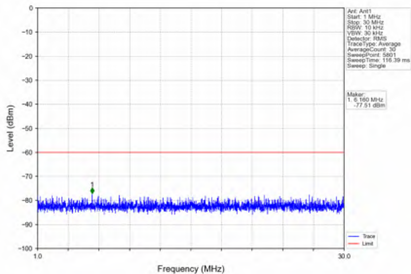
n78d_30kHz_SISO_NTNV_70MHz_CP-OFDM QPSK_3664.98MHz_Outer_Full
