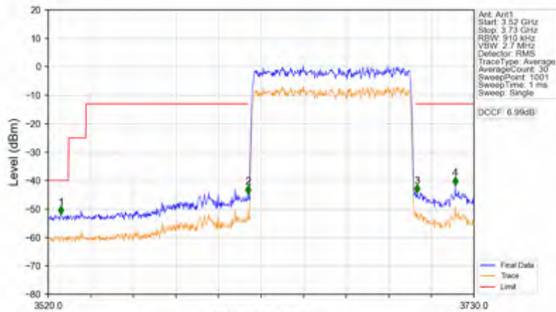
n78d_30kHz_SISO_NTNV_80MHz_DFT-s-OFDM PI/2 BPSK_3660MHz_Outer_Full
