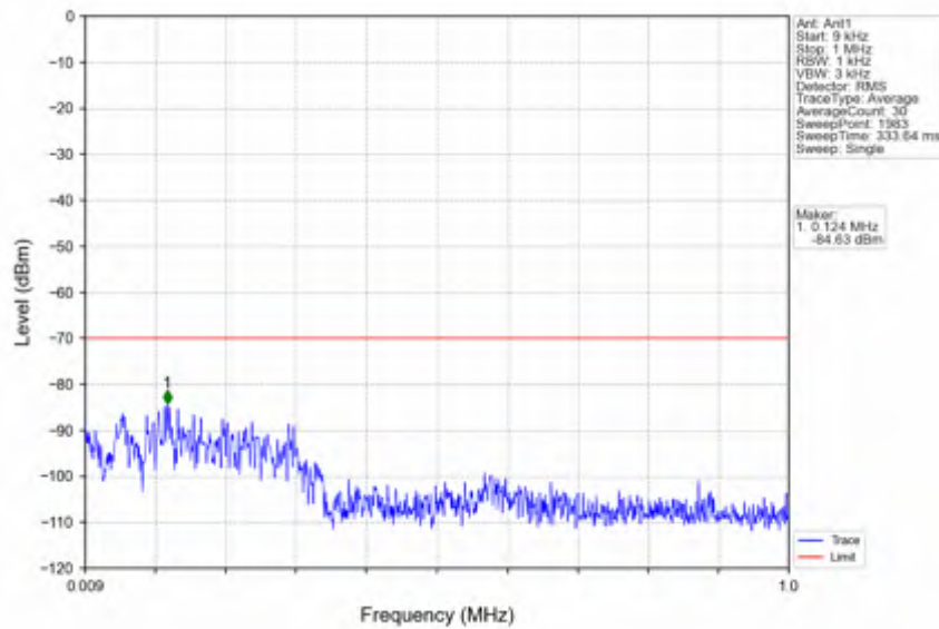
n78d_30kHz_SISO_NTNV_80MHz_DFT-s-OFDM QPSK_3660MHz_Edge_1RB_Right
