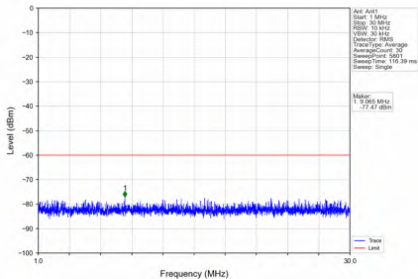
n78d_30kHz_SISO_NTNV_60MHz_CP-OFDM QPSK_3580.02MHz_Outer_Full
