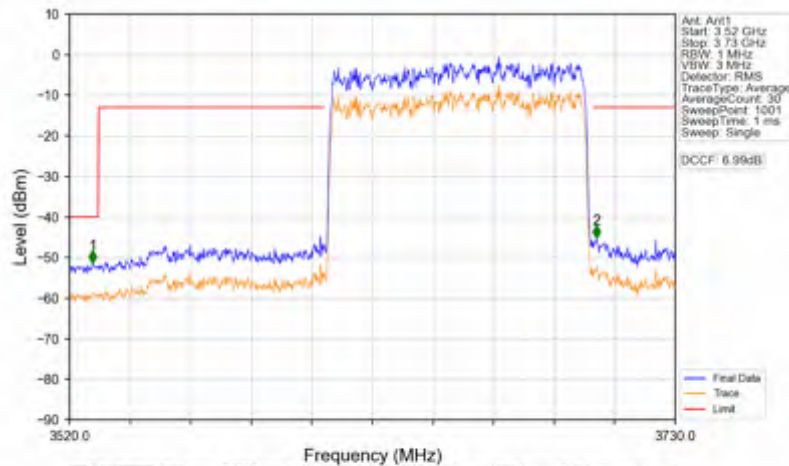
n78d_30kHz_SISO_NTNV_90MHz_DFT-s-OFDM PI/2 BPSK_3654.99MHz_Outer_Full
