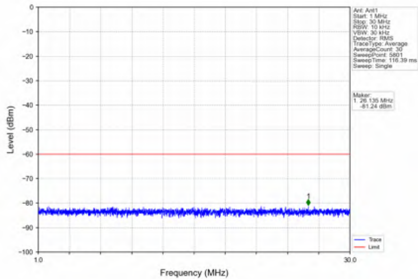
n78d_30kHz_SISO_NTV_60MHz_CP-OFDM_QPSK_3580.02MHz_Edge_1RB_Left
