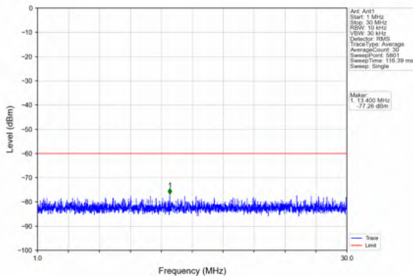
n78d_30kHz_SISO_NTNV_80MHz_DFT-s-OFDM_QPSK_3590.01MHz_Edge_1RB_Left
