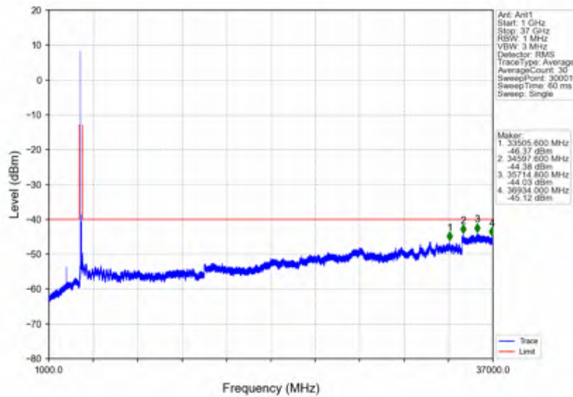
n78d_30kHz_SISO_NTNV_90MHz_DFT-s-OFDM PI/2 BPSK_3624.99MHz_Edge_1RB_Left
