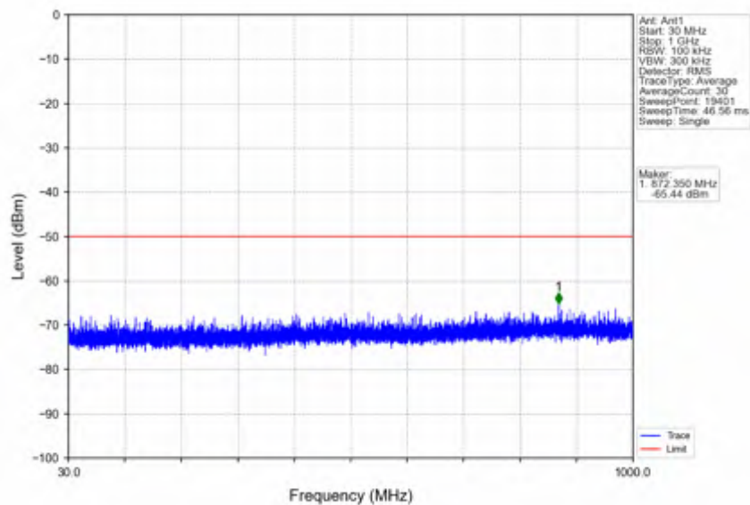
n78d_30kHz_SISO_NTNV_80MHz_CP-OFDM QPSK_3660MHz_Inner_1RB_Right
