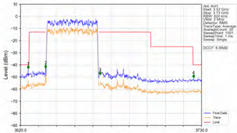
n78d_30kHz_SISO_NTNV_60MHz_DFT-s-OFDM PI/2 BPSK_3580.02MHz_Outer_Full
