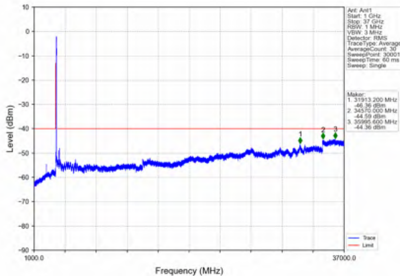
n78d_30kHz_SISO_NTNV_60MHz_DFT-s-OFDM PI/2 BPSK_3580.02MHz_Outer_Full
