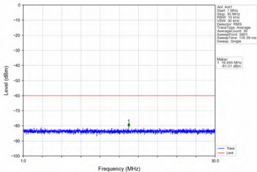
n78d_30kHz_SISO_NTNV_80MHz_DFT-s-OFDM PI/2 BPSK_3624.99MHz_Edge_1RB_Left
