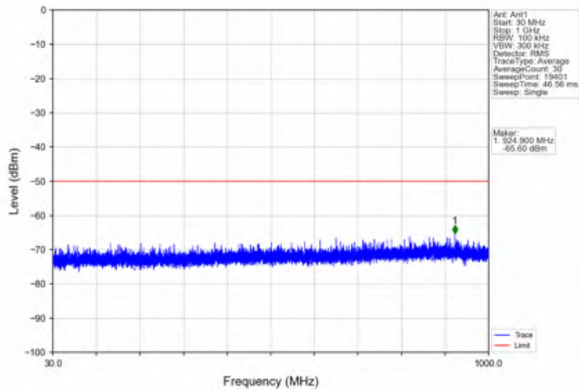
n78d_30kHz_SISO_NTNV_80MHz_DFT-s-OFDM QPSK_3590.01MHz_Inner_1RB_Left
