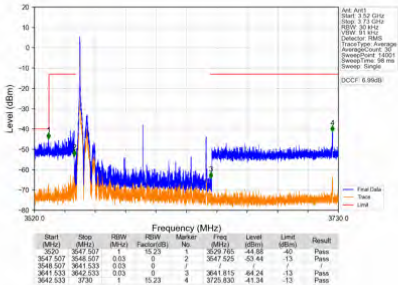
n78d_30kHz_SISO_NTNV_90MHz_DFT-s-OFDM QPSK_3595.02MHz_Inner_1RB_Left
