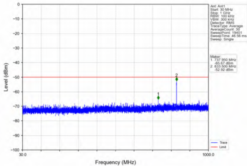
n78d_30kHz_SISO_NTNV_90MHz_DFT-s-OFDM QPSK_3595.02MHz_Edge_1RB_Left
