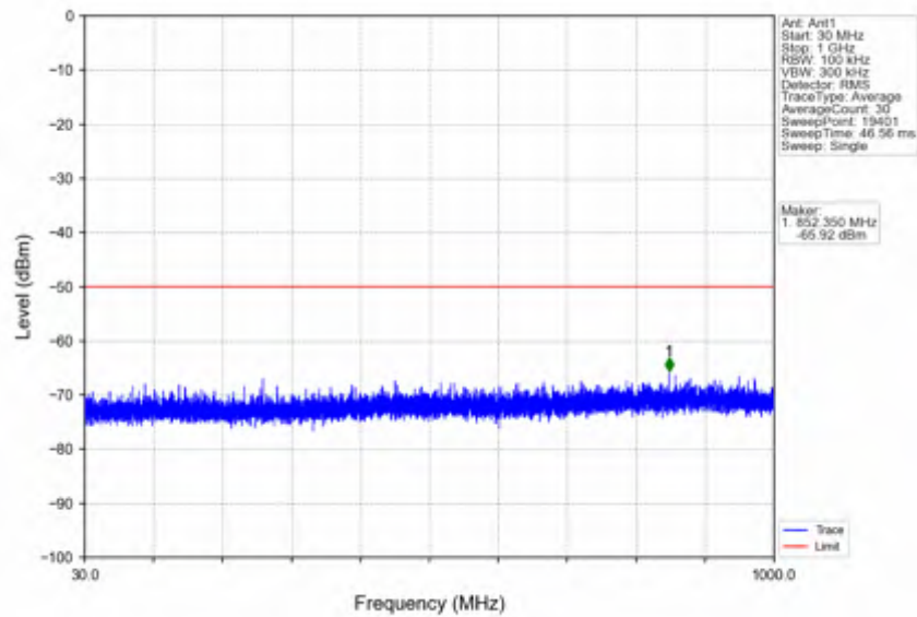
n78d_30kHz_SISO_NTNV_80MHz_DFT-s-OFDM_QPSK_3660MHz_Inner_1RB_Right
