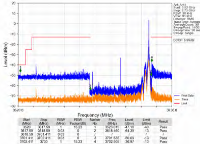
n78d_30kHz_SISO_NTNV_80MHz_CP-OFDM QPSK_3660MHz_Inner_1RB_Right
