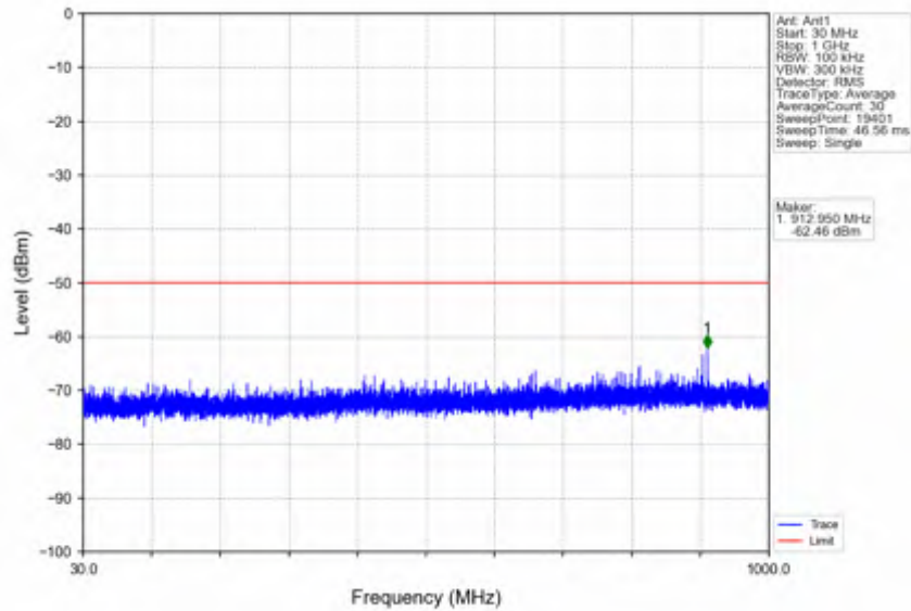
n78d_30kHz_SISO_NTNV_80MHz_DFT-s-OFDM_QPSK_3590.01MHz_Edge_1RB_Left
