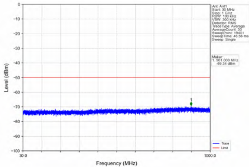
n78d_30kHz_SISO_NTNV_60MHz_DFT-s-OFDM PI/2 BPSK_3669.99MHz_Outer_Full
