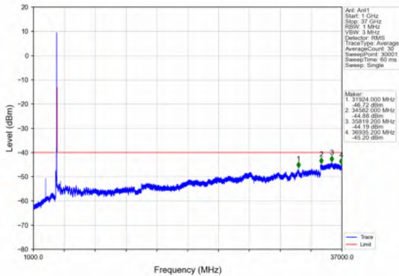
n78d_30kHz_SISO_NTNV_60MHz_DFT-s-OFDM PI/2 BPSK_3669.99MHz_Outer_Full
