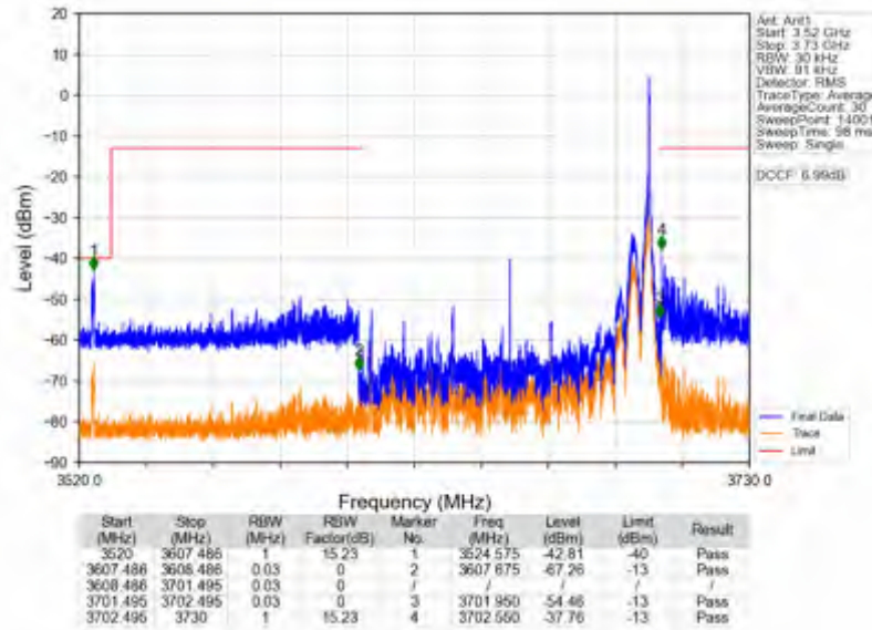
n78d_30kHz_SISO_NTNV_90MHz_DFT-s-OFDM PI/2 BPSK_3654.99MHz_Inner_1RB_Right
