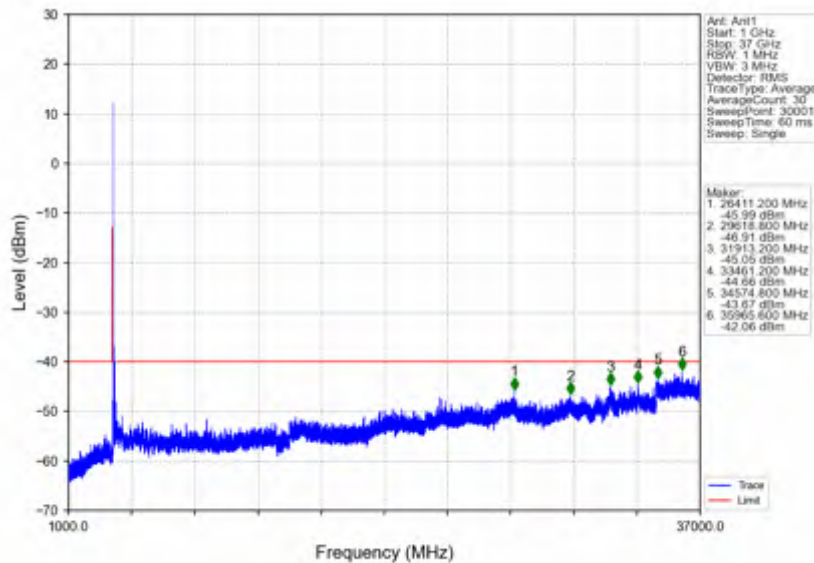
n78d_30kHz_SISO_NTV_70MHz_DFT-s-OFDM_QPSK_3585MHz_Inner_1RB_Left
