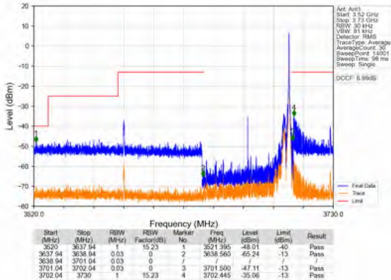
n78d_30kHz_SISO_NTNV_60MHz_DFT-s-OFDM QPSK_3669.99MHz_Edge_1RB_Right
