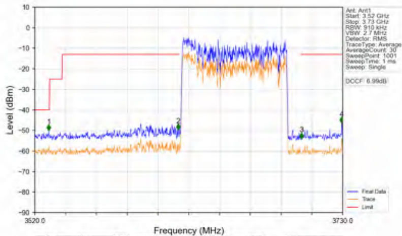
n78d_30kHz_SISO_NTNV_80MHz_CP-OFDM QPSK_3660MHz_Outer_Full
