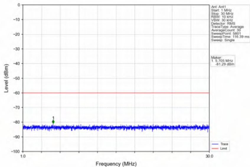
n78d_30kHz_SISO_NTNV_90MHz_DFT-s-OFDM PI/2 BPSK_3624.99MHz_Edge_1RB_Left
