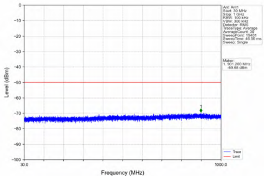
n78d_30kHz_SISO_NTV_80MHz_DFT-s-OFDM PI/2 BPSK_3660MHz_Edge_1RB_Right
