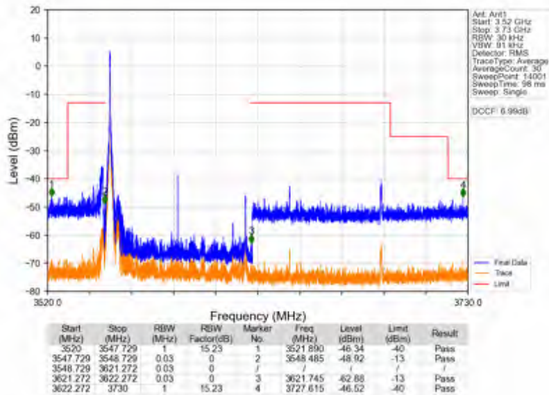
n78d_30kHz_SISO_NTNV_70MHz_DFT-s-OFDM QPSK_3585MHz_Edge_1RB_Left
