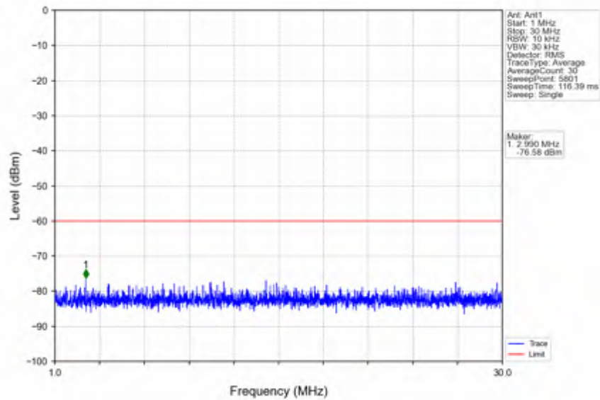
n78d_30kHz_SISO_NTNV_50MHz_CP-OFDM QPSK_3675MHz_Inner_1RB_Right
