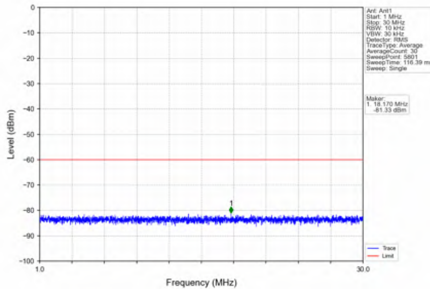
n78d_30kHz_SISO_NTNV_90MHz_DFT-s-OFDM PI/2 BPSK_3654.99MHz_Edge_1RB_Right
