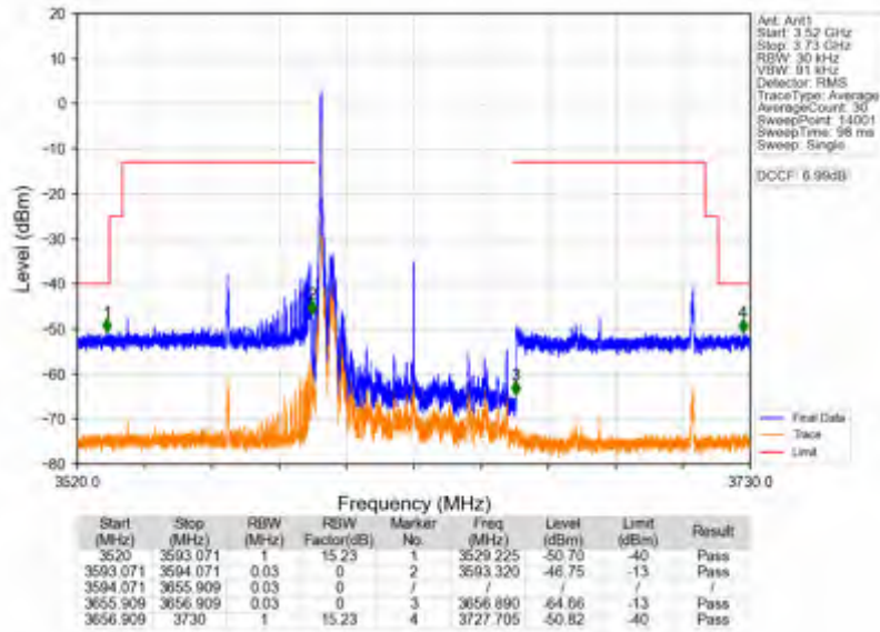
n78d_30kHz_SISO_NTNV_60MHz_DFT-s-OFDM PI/2 BPSK_3624.99MHz_Edge_1RB_Left
