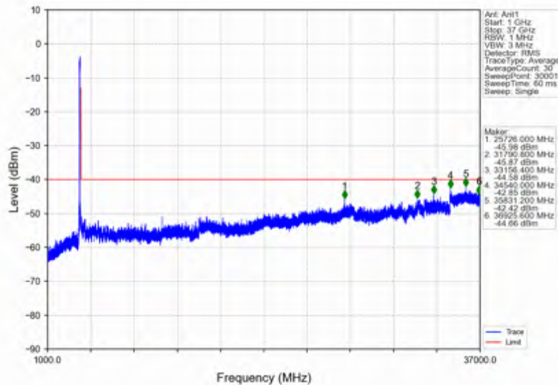
n78d_30kHz_SISO_NTNV_70MHz_CP-OFDM QPSK_3664.98MHz_Outer_Full
