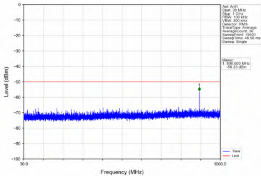
n78d_30kHz_SISO_NTV_70MHz_DFT-s-OFDM QPSK_3585MHz_Edge_1RB_Left
