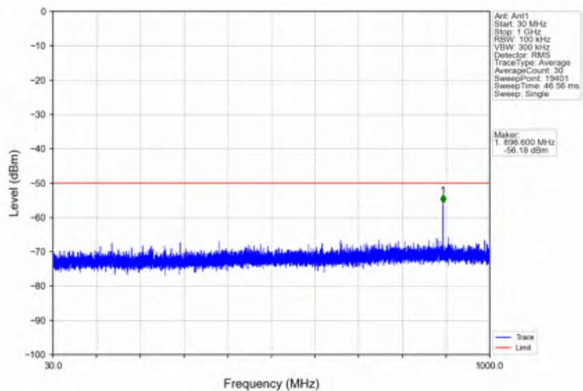
n78d_30kHz_SISO_NTV_60MHz_CP-OFDM_QPSK_3580.02MHz_Inner_1RB_Left
