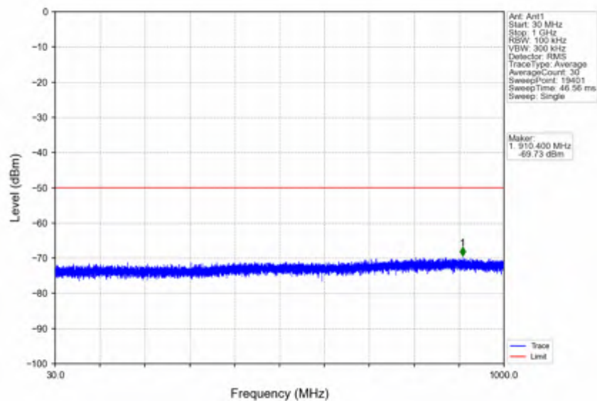
n78d_30kHz_SISO_NTNV_60MHz_DFT-s-OFDM PI/2 BPSK_3580.02MHz_Inner_1RB_Left
