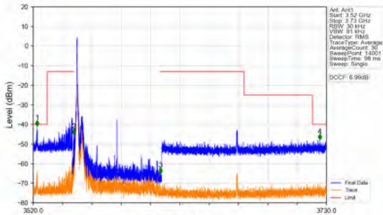
n78d_30kHz_SISO_NTNV_60MHz_DFT-s-OFDM_QPSK_3580.02MHz_Inner_1RB_Left
