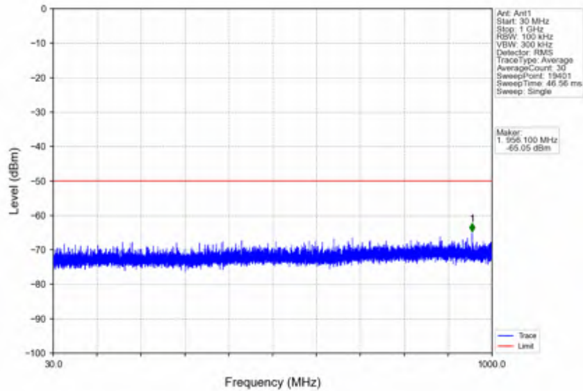
n78d_30kHz_SISO_NTNV_70MHz_DFT-s-OFDM QPSK_3664.98MHz_Inner_1RB_Right
