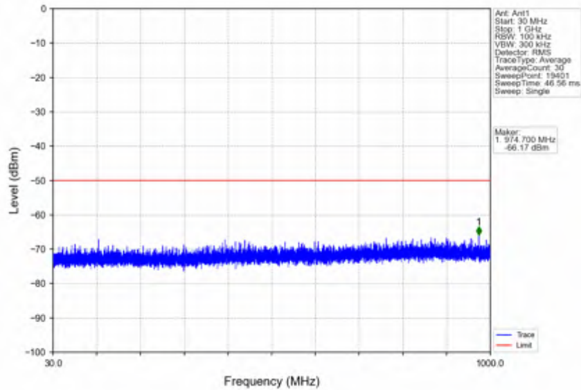
n78d_30kHz_SISO_NTNV_80MHz_DFT-s-OFDM_QPSK_3660MHz_Edge_1RB_Right
