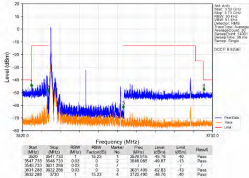
n78d_30kHz_SISO_NTVV_80MHz_CP-OFDM_QPSK_3590.01MHz_Inner_1RB_Left
