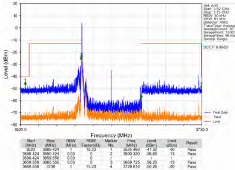
n78d_30kHz_SISO_NTV_70MHz_CP-OFDM QPSK_3624.99MHz_Edge_1RB_Left
