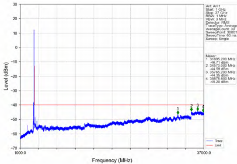
n78d_30kHz_SISO_NTNV_80MHz_DFT-s-OFDM QPSK_3590.01MHz_Edge_1RB_Left
