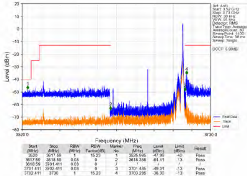
n78d_30kHz_SISO_NTNV_80MHz_CP-OFDM QPSK_3660MHz_Edge_1RB_Right
