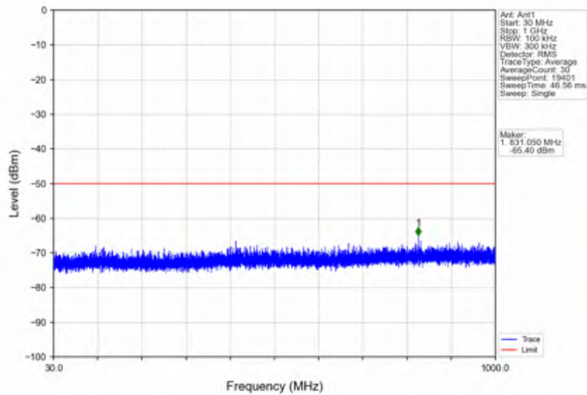
n78d_30kHz_SISO_NTNV_60MHz_DFT-s-OFDM_QPSK_3580.02MHz_Edge_1RB_Left
