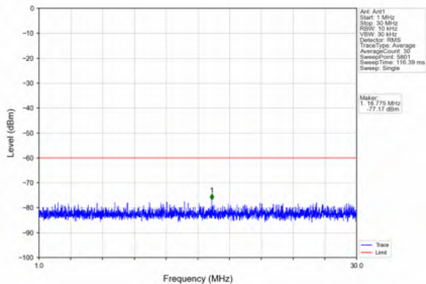
n78d_30kHz_SISO_NTNV_60MHz_DFT-s-OFDM_QPSK_3580.02MHz_Inner_1RB_Left
