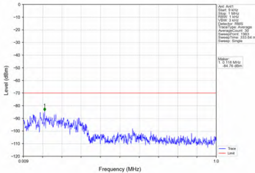
n78d_30kHz_SISO_NTNV_80MHz_DFT-s-OFDM QPSK_3624.99MHz_Edge_1RB_Left
