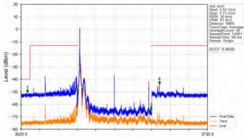
n78d_30kHz_SISO_NTNV_80MHz_DFT-s-OFDM PI/2 BPSK_3624.99MHz_Edge_1RB_Left
