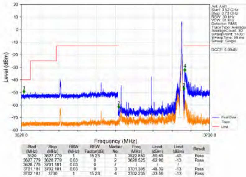
n78d_30kHz_SISO_NTNV_70MHz_DFT-s-OFDM QPSK_3664.98MHz_Edge_1RB_Right
