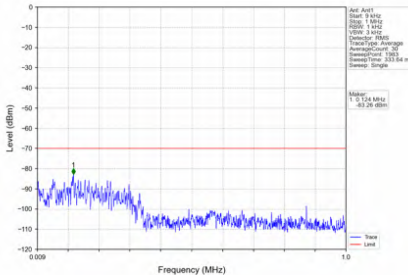
n78d_30kHz_SISO_NTNV_70MHz_DFT-s-OFDM_QPSK_3624.99MHz_Edge_1RB_Left
