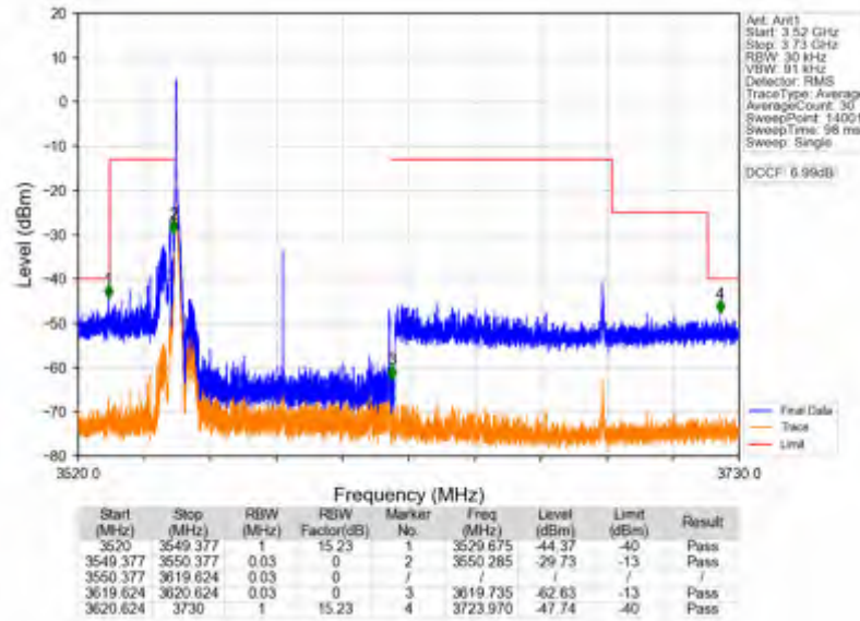
n78d_30kHz_SISO_NTNV_70MHz_CP-OFDM_QPSK_3585MHz_Edge_1RB_Left
