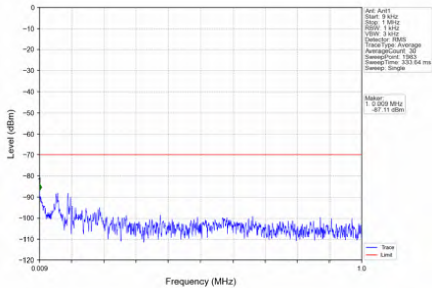
n78d_30kHz_SISO_NTNV_80MHz_CP-OFDM QPSK_3590.01MHz_Outer_Full
