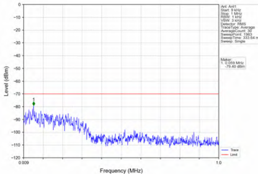
n78d_30kHz_SISO_NTNV_70MHz_CP-OFDM QPSK_3664.98MHz_Inner_1RB_Right
