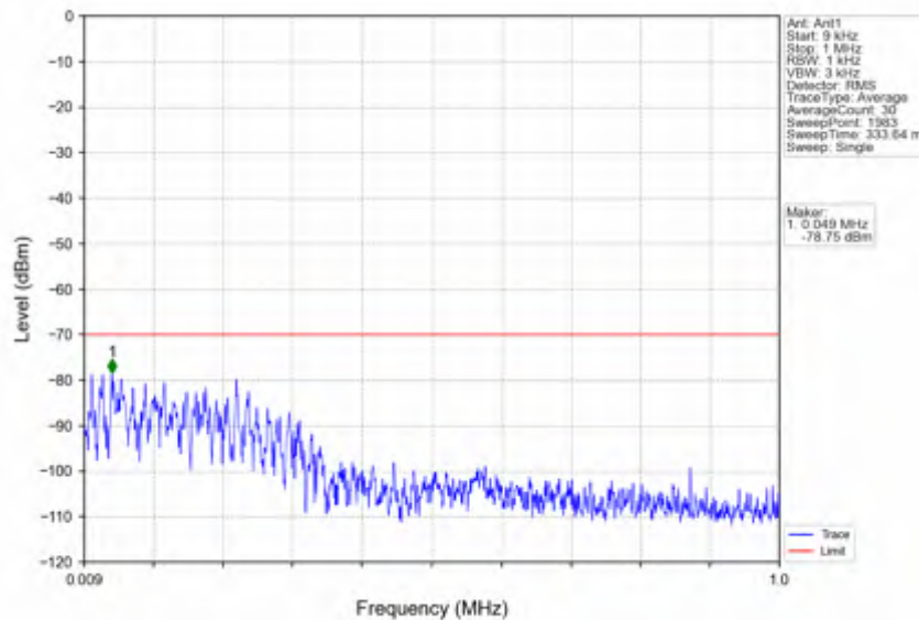
n78d_30kHz_SISO_NTV_50MHz_CP-OFDM QPSK_3575.01MHz_Edge_1RB_Left
