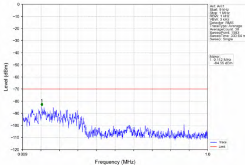
n78d_30kHz_SISO_NTNV_25MHz_DFT-s-OFDM QPSK_3624.99MHz_Edge_1RB_Left
