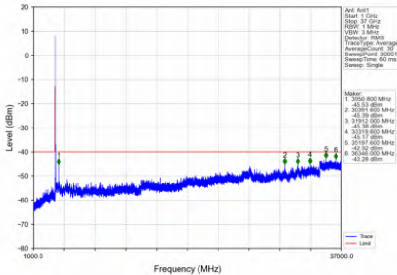
n78d_30kHz_SISO_NTNV_50MHz_CP-OFDM QPSK_3575.01MHz_Outer_Full
