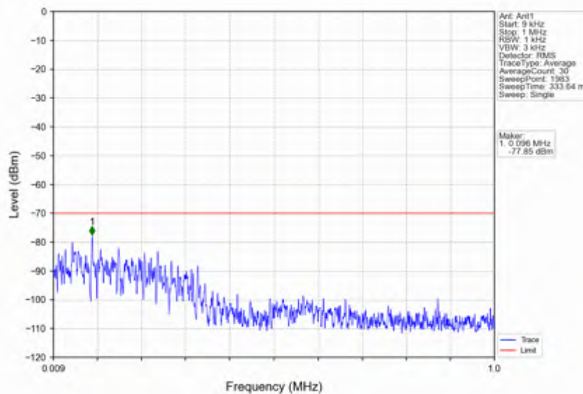
n78d_30kHz_SISO_NTNV_50MHz_CP-OFDM QPSK_3675MHz_Edge_1RB_Right
