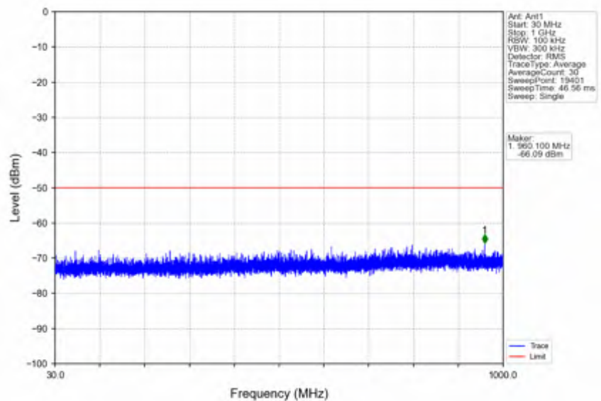
n78d_30kHz_SISO_NTNV_25MHz_DFT-s-OFDM QPSK_3624.99MHz_Edge_1RB_Left
