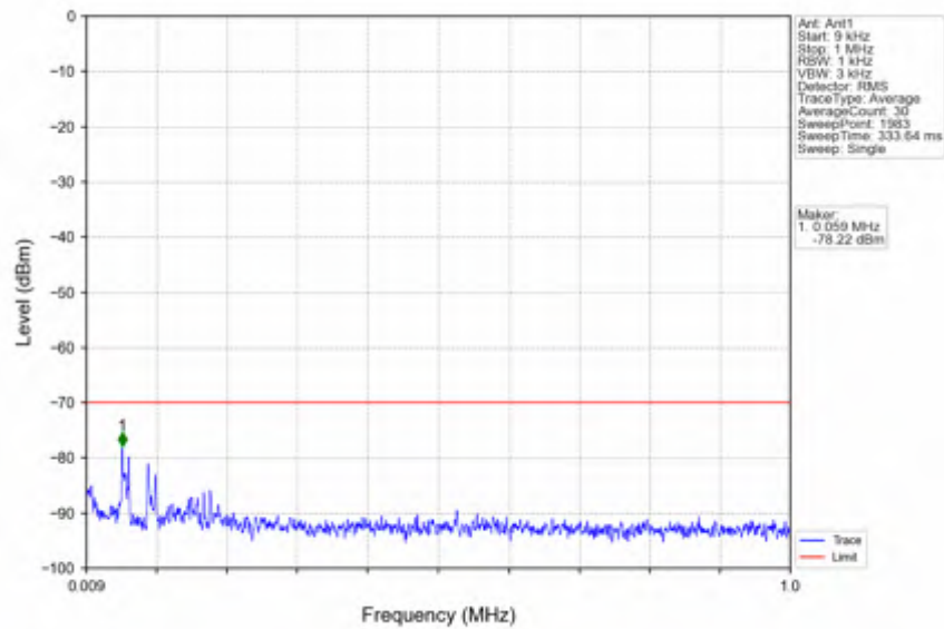
n78d_30kHz_SISO_NTNV_40MHz_DFT-s-OFDM PI/2 BPSK_3624.99MHz_Edge_1RB_Left
