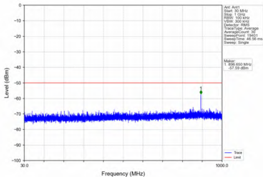
n78d_30kHz_SISO_NTNV_40MHz_CP-OFDM QPSK_3570MHz_Edge_1RB_Left
