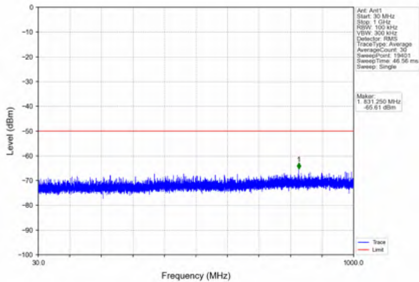
n78d_30kHz_SISO_NTNV_30MHz_DFT-s-OFDM QPSK_3684.99MHz_Edge_1RB_Right
