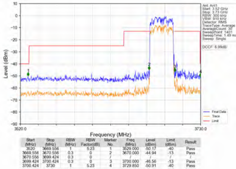
n78d_30kHz_SISO_NTNV_30MHz_DFT-s-OFDM_QPSK_3684.99MHz_Outer_Full
