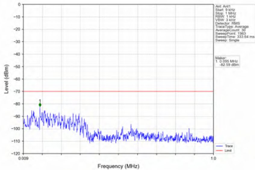
n78d_30kHz_SISO_NTNV_50MHz_DFT-s-OFDM_QPSK_3675MHz_Inner_1RB_Right
