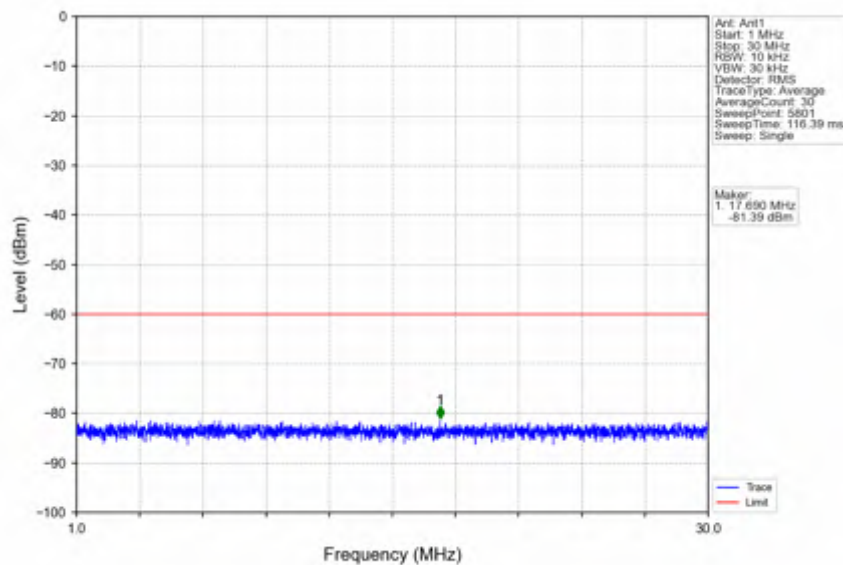
n78d_30kHz_SISO_NTNV_50MHz_DFT-s-OFDM PI/2 BPSK_3624.99MHz_Edge_1RB_Left
