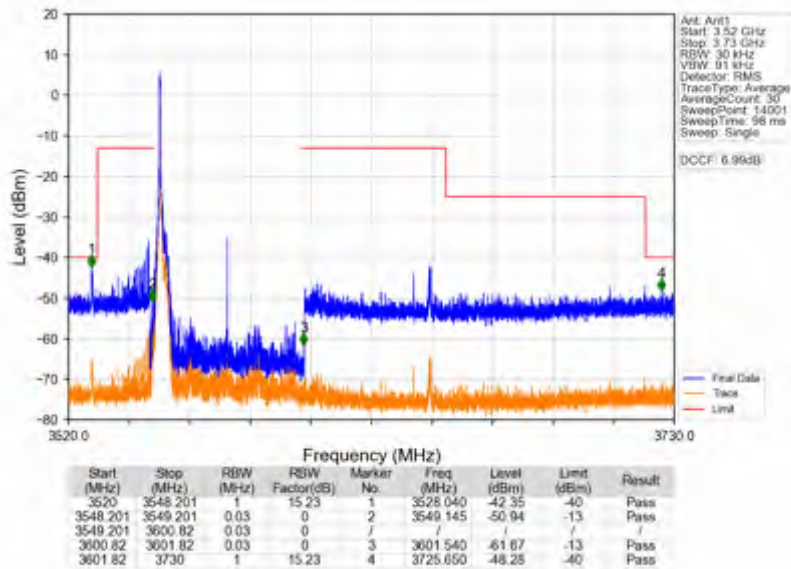
n78d_30kHz_SISO_NTNV_50MHz_DFT-s-OFDM_QPSK_3575.01MHz_Inner_1RB_Left
