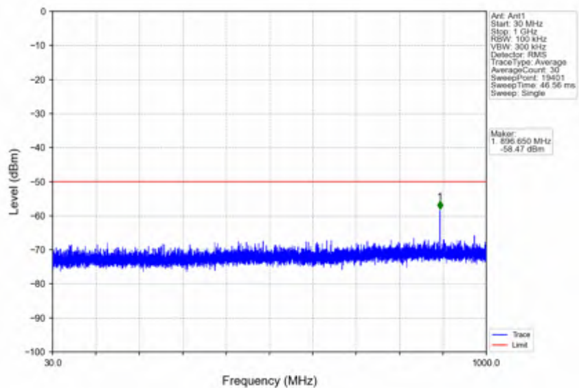
n78d_30kHz_SISO_NTNV_50MHz_DFT-s-OFDM QPSK_3624.99MHz_Edge_1RB_Left
