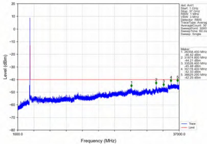
n78d_30kHz_SISO_NTNV_50MHz_CP-OFDM QPSK_3675MHz_Outer_Full
