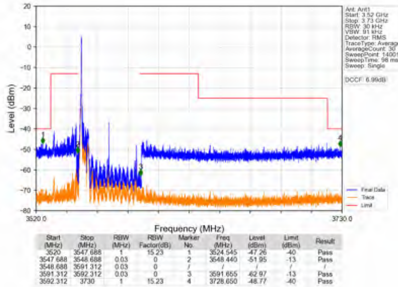
n78d_30kHz_SISO_NTNV_40MHz_CP-OFDM_QPSK_3570MHz_Edge_1RB_Left
