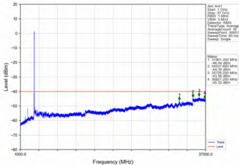
n78d_30kHz_SISO_NTNV_30MHz_DFT-s-OFDM PI/2 BPSK_3684.99MHz_Outer_Full
