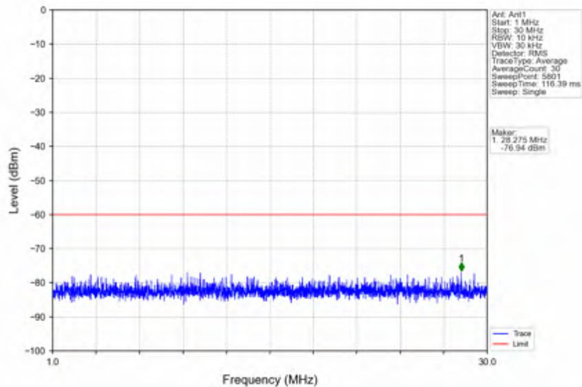
n78d_30kHz_SISO_NTV_40MHz_DFT-s-OFDM QPSK_3570MHz_Edge_1RB_Left
