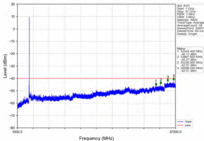
n78d_30kHz_SISO_NTNV_30MHz_DFT-s-OFDM QPSK_3684.99MHz_Edge_1RB_Right
