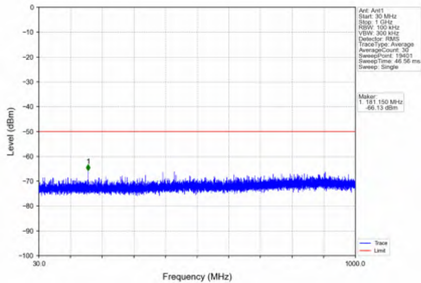
n78d_30kHz_SISO_NTNV_50MHz_DFT-s-OFDM_QPSK_3575.01MHz_Inner_1RB_Left
