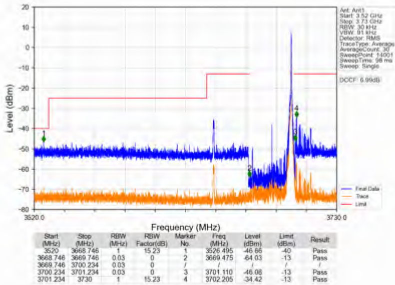
n78d_30kHz_SISO_NTNV_30MHz_DFT-s-OFDM_QPSK_3684.99MHz_Inner_1RB_Right
