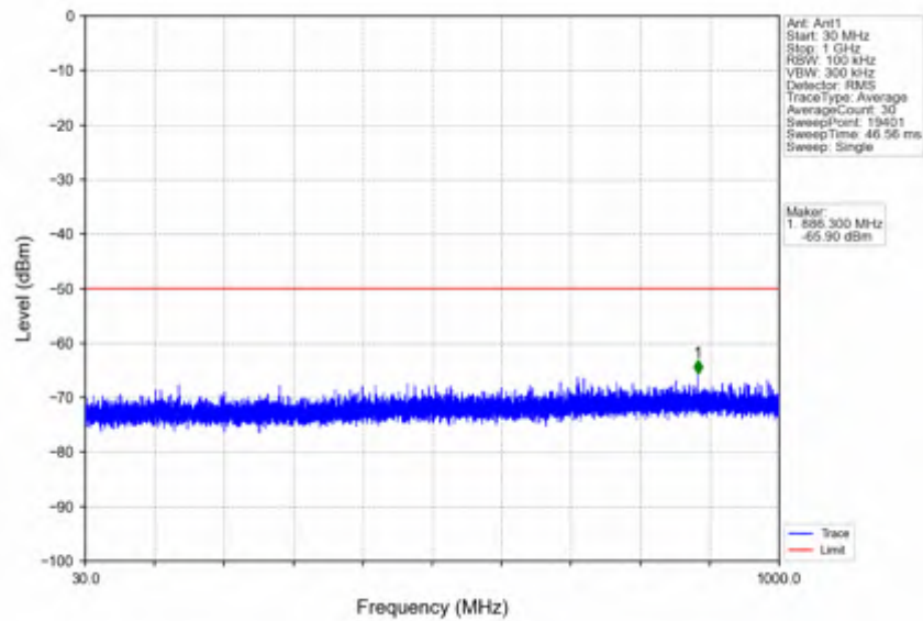
n78d_30kHz_SISO_NTNV_25MHz_DFT-s-OFDM QPSK_3687.48MHz_Edge_1RB_Right
