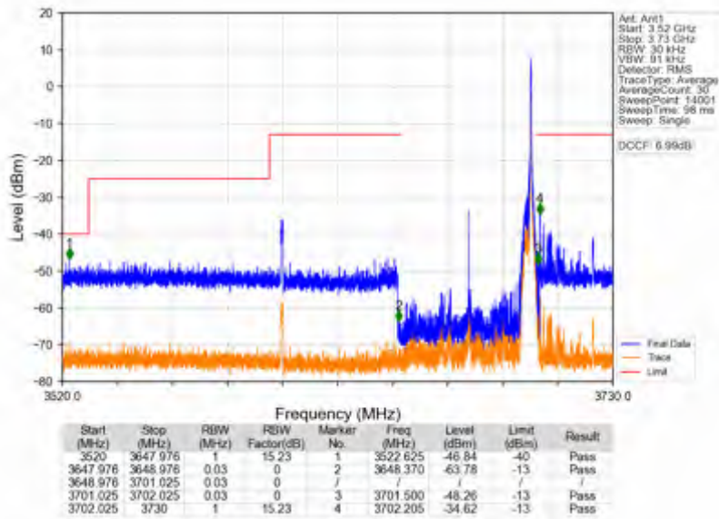
n78d_30kHz_SISO_NTNV_50MHz_DFT-s-OFDM_QPSK_3675MHz_Edge_1RB_Right
