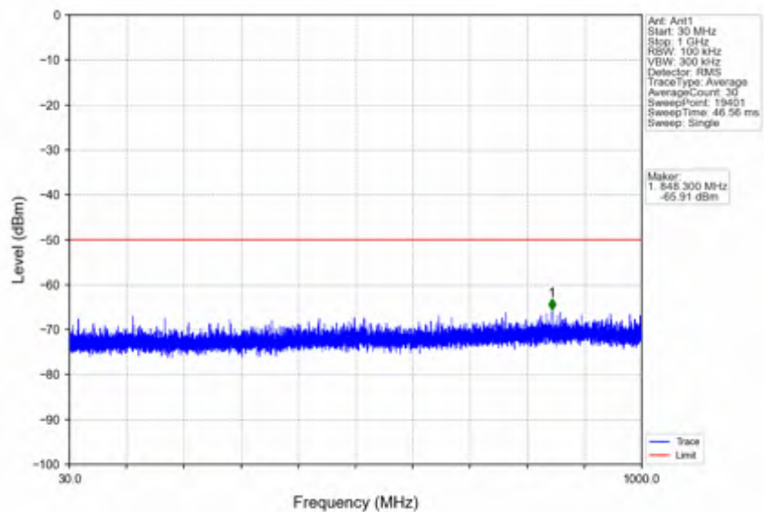
n78d_30kHz_SISO_NTNV_30MHz_CP-OFDM QPSK_3684.99MHz_Edge_1RB_Right
