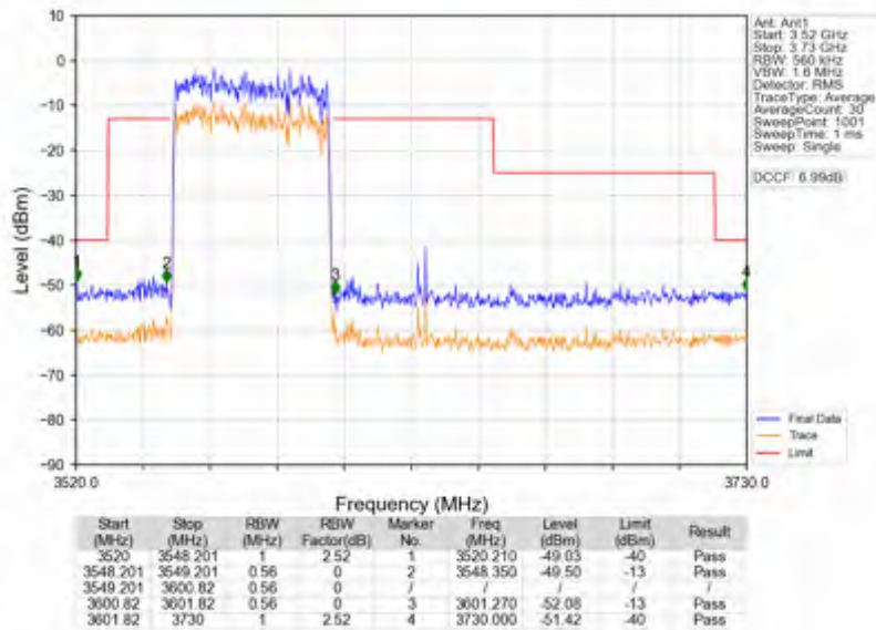
n78d_30kHz_SISO_NTNV_50MHz_CP-OFDM QPSK_3575.01MHz_Outer_Full
