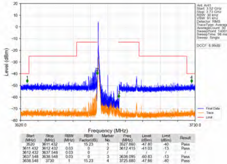
n78d_30kHz_SISO_NTNV_25MHz_DFT-s-OFDM QPSK_3624.99MHz_Edge_1RB_Left
