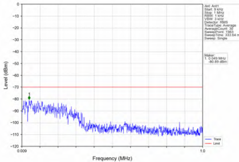
n78d_30kHz_SISO_NTV_30MHz_CP-OFDM_QPSK_3565.02MHz_Inner_1RB_Left
