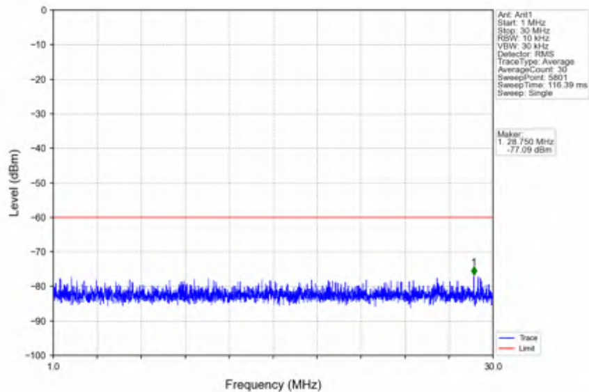
n78d_30kHz_SISO_NTV_30MHz_CP-OFDM QPSK_3624.99MHz_Edge_1RB_Left
