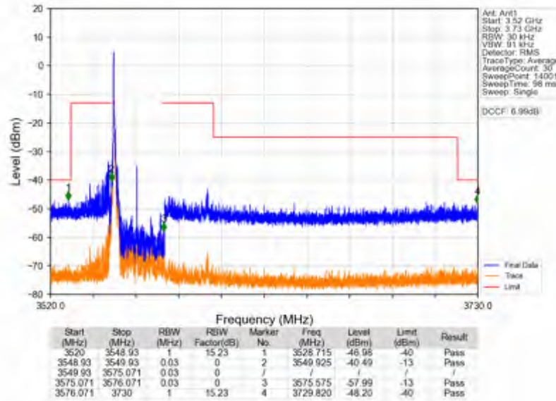
n78d_30kHz_SISO_NTNV_25MHz_CP-OFDM QPSK_3562.5MHz_Edge_1RB_Left
