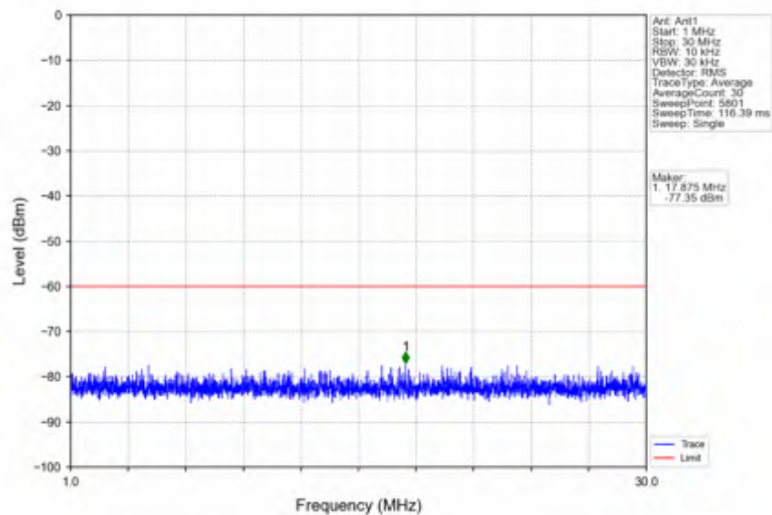
n78d_30kHz_SISO_NTNV_30MHz_DFT-s-OFDM QPSK_3684.99MHz_Edge_1RB_Right
