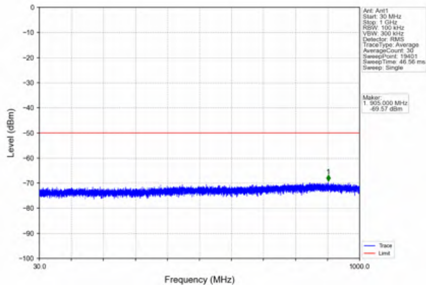
n78d_30kHz_SISO_NTNV_40MHz_DFT-s-OFDM PI/2 BPSK_3679.98MHz_Inner_1RB_Right
