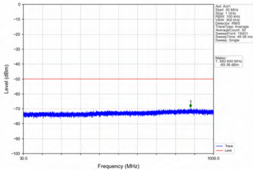
n78d_30kHz_SISO_NTNV_50MHz_DFT-s-OFDM PI/2 BPSK_3575.01MHz_Outer_Full
