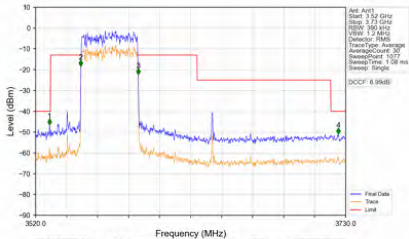
n78d_30kHz_SISO_NTNV_40MHz_CP-OFDM QPSK_3570MHz_Outer_Full
