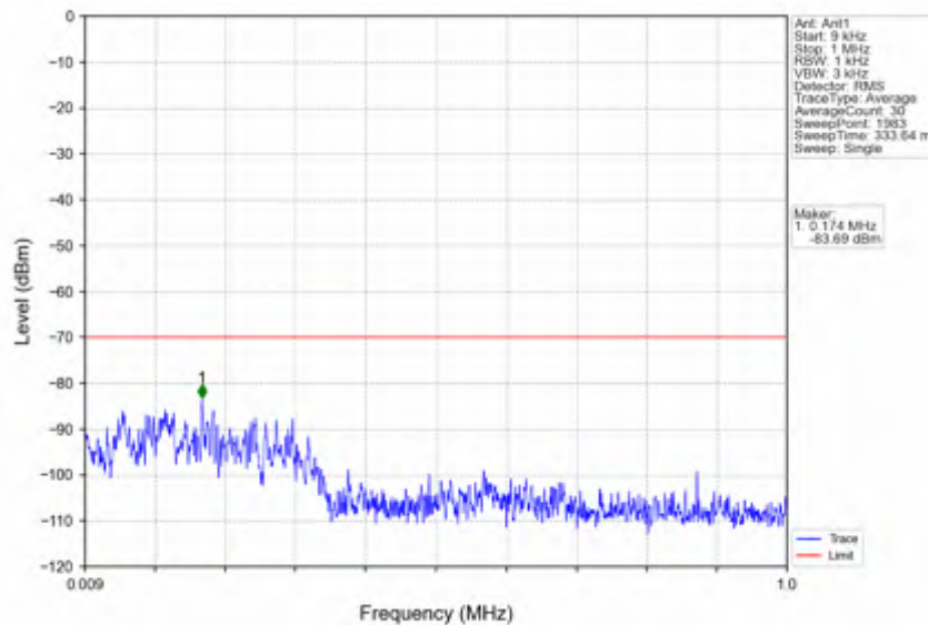
n78d_30kHz_SISO_NTNV_40MHz_DFT-s-OFDM QPSK_3624.99MHz_Edge_1RB_Left
