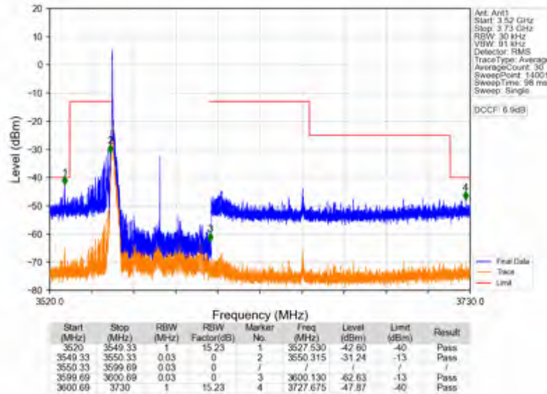
n78d_30kHz_SISO_NTV_50MHz_CP-OFDM QPSK_3575.01MHz_Edge_1RB_Left
