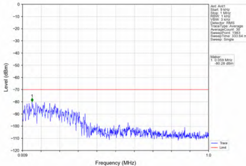
n78d_30kHz_SISO_NTV_30MHz_CP-OFDM QPSK_3565.02MHz_Edge_1RB_Left
