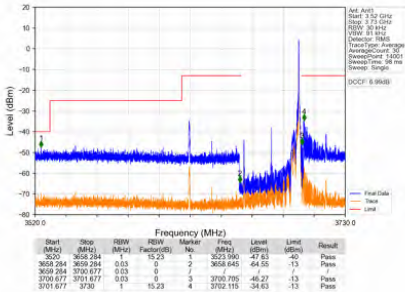
n78d_30kHz_SISO_NTNV_40MHz_DFT-s-OFDM QPSK_3679.98MHz_Inner_1RB_Right
