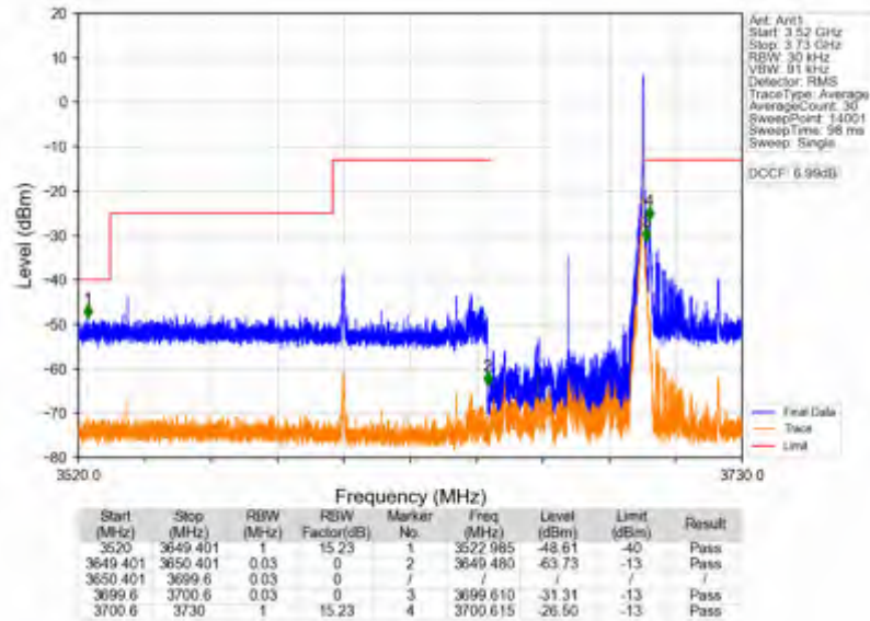
n78d_30kHz_SISO_NTNV_50MHz_CP-OFDM QPSK_3675MHz_Edge_1RB_Right
