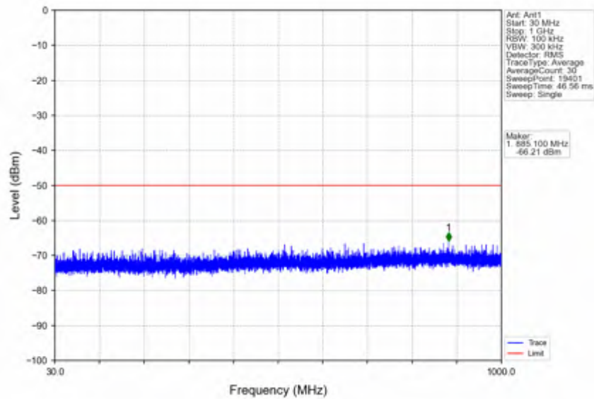
n78d_30kHz_SISO_NTV_25MHz_CP-OFDM QPSK_3624.99MHz_Edge_1RB_Left
