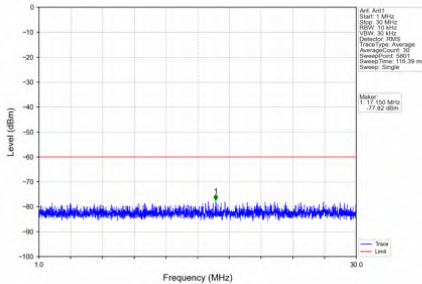
n78d_30kHz_SISO_NTNV_30MHz_CP-OFDM QPSK_3684.99MHz_Inner_1RB_Right
