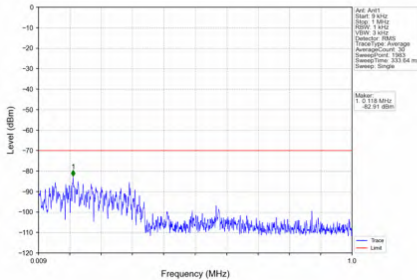
n78d_30kHz_SISO_NTNV_30MHz_DFT-s-OFDM QPSK_3565.02MHz_Edge_1RB_Left
