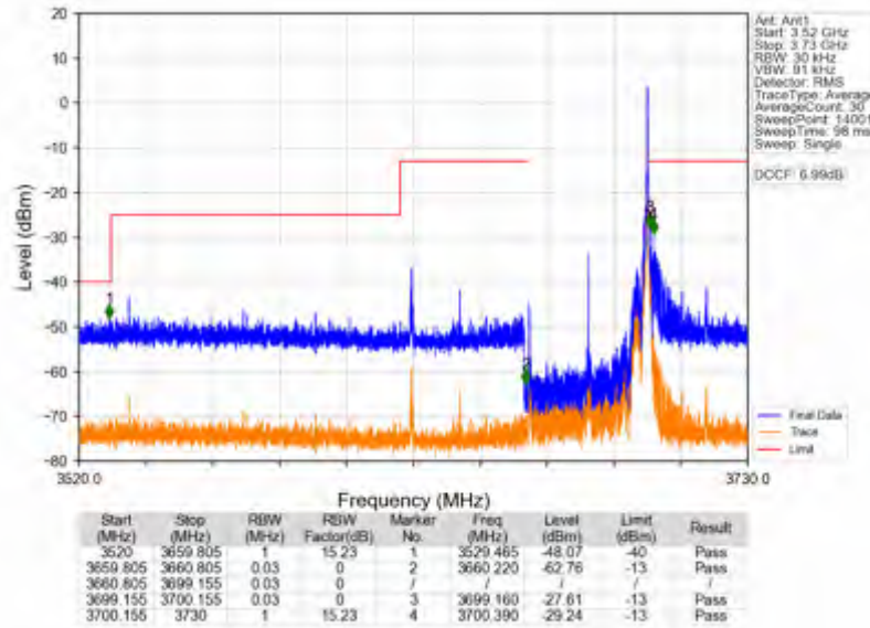
n78d_30kHz_SISO_NTNV_40MHz_CP-OFDM QPSK_3679.98MHz_Inner_1RB_Right
