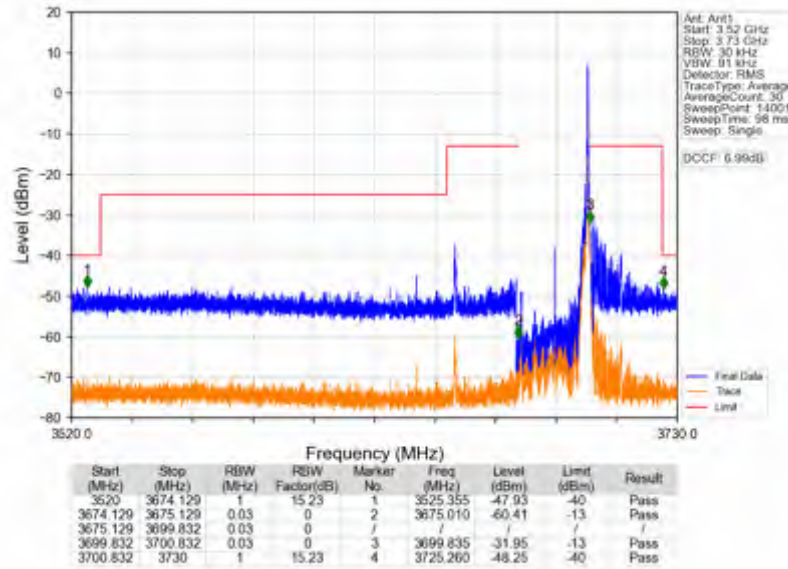
n78d_30kHz_SISO_NTV_25MHz_CP-OFDM QPSK_3687.48MHz_Edge_1RB_Right
