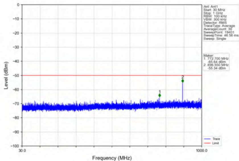
n78d_30kHz_SISO_NTNV_30MHz_DFT-s-OFDM_QPSK_3624.99MHz_Edge_1RB_Left
