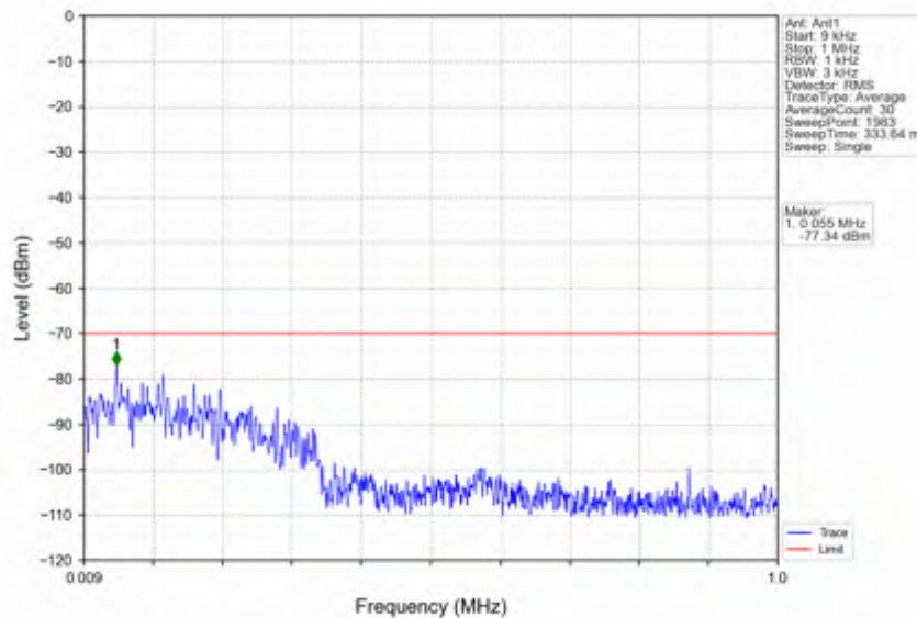
n78d_30kHz_SISO_NTNV_25MHz_CP-OFDM QPSK_3562.5MHz_Edge_1RB_Left
