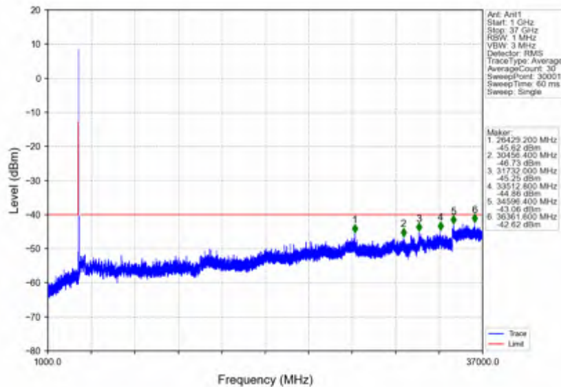
n78d_30kHz_SISO_NTVV_40MHz_DFT-s-OFDM_QPSK_3570MHz_Edge_1RB_Left
