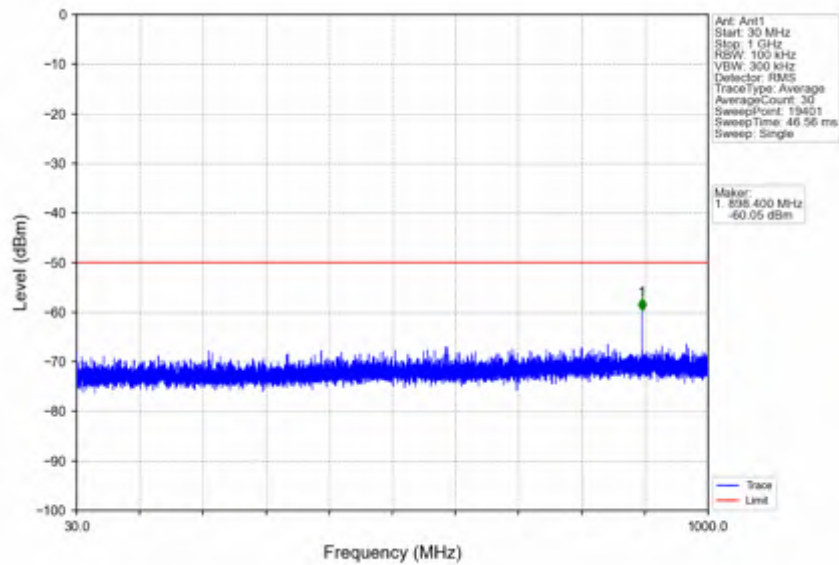
n78d_30kHz_SISO_NTNV_30MHz_DFT-s-OFDM QPSK_3565.02MHz_Inner_1RB_Left
