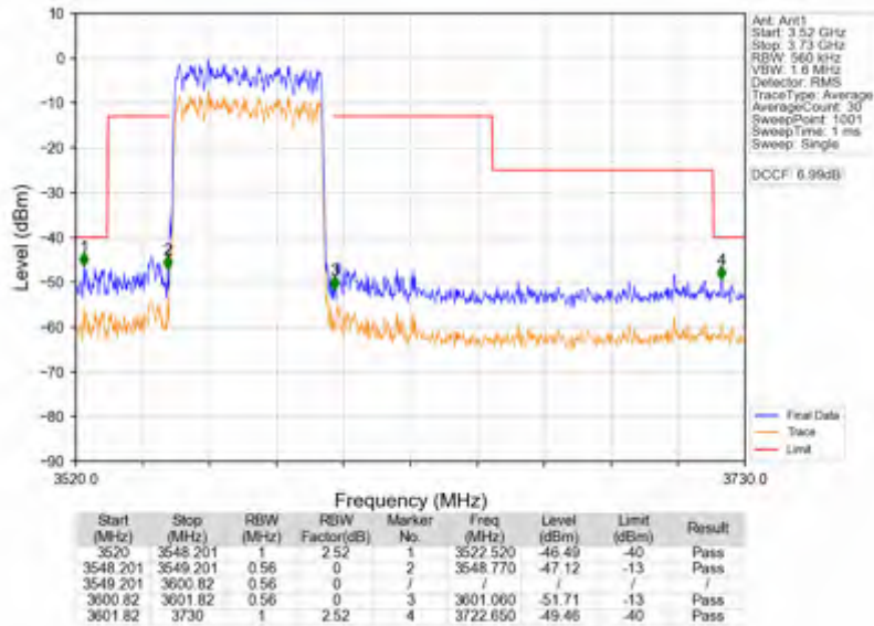
n78d_30kHz_SISO_NTNV_50MHz_DFT-s-OFDM_QPSK_3575.01MHz_Outer_Full
