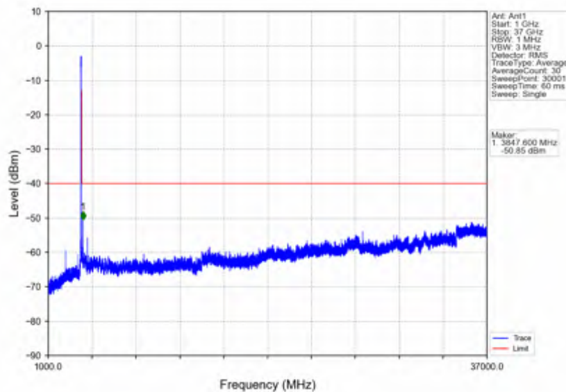
n78d_30kHz_SISO_NTNV_40MHz_DFT-s-OFDM PI/2 BPSK_3679.98MHz_Outer_Full
