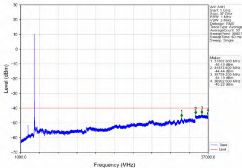
n78d_30kHz_SISO_NTNV_50MHz_DFT-s-OFDM PI/2 BPSK_3624.99MHz_Edge_1RB_Left
