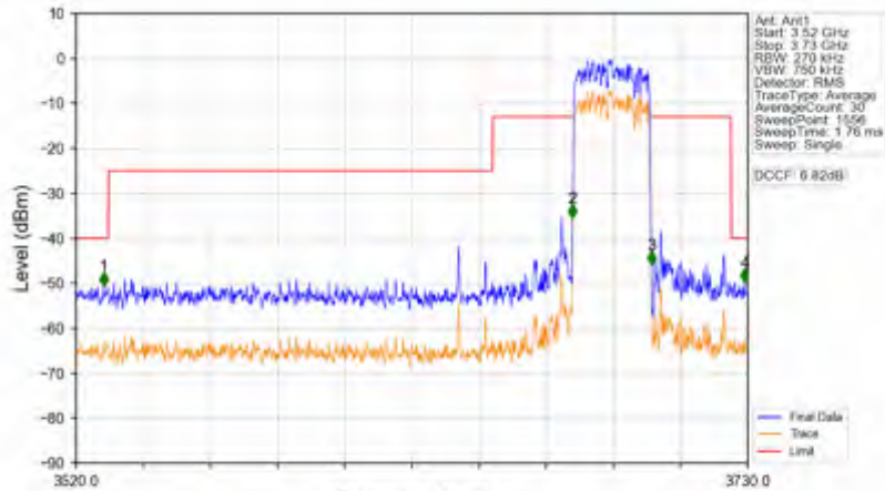
n78d_30kHz_SISO_NTNV_25MHz_CP-OFDM QPSK_3687.48MHz_Outer_Full
