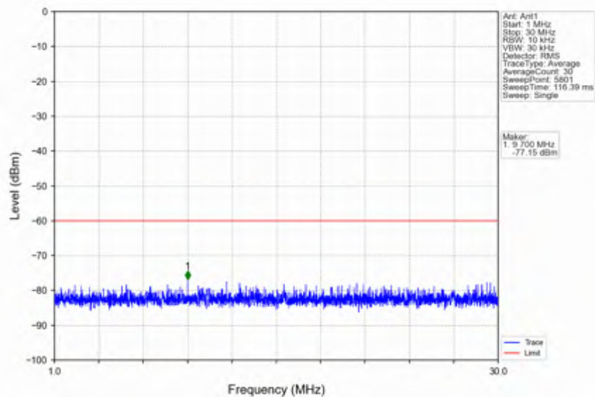
n78d_30kHz_SISO_NTNV_25MHz_DFT-s-OFDM QPSK_3687.48MHz_Edge_1RB_Right
