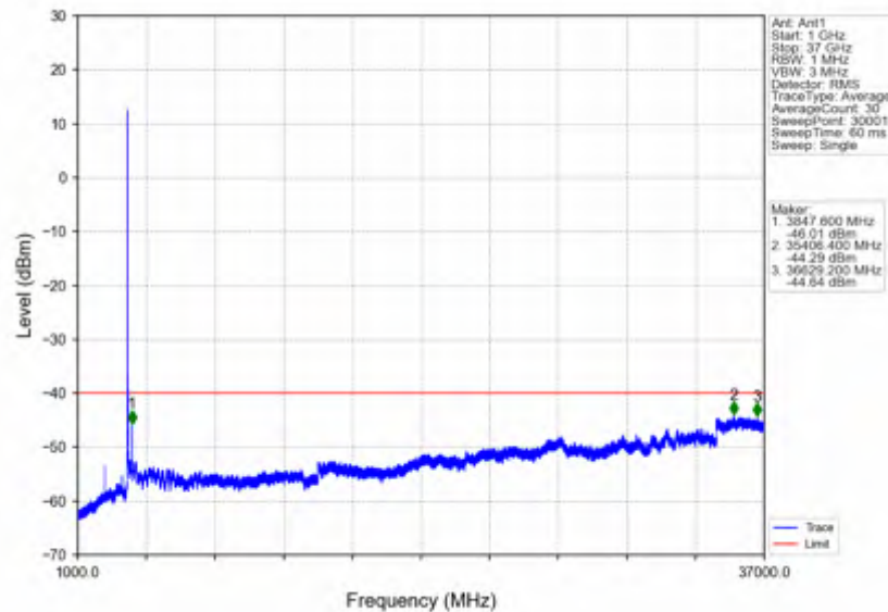
n78d_30kHz_SISO_NTVV_40MHz_CP-OFDM QPSK_3624.99MHz_Edge_1RB_Left
