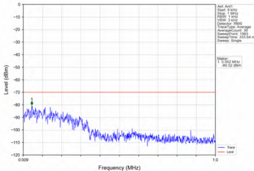
n78d_30kHz_SISO_NTV_25MHz_CP-OFDM QPSK_3687.48MHz_Edge_1RB_Right
