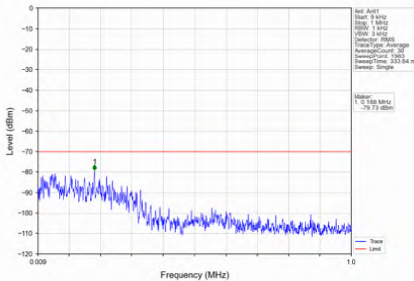
n78d_30kHz_SISO_NTV_50MHz_CP-OFDM_QPSK_3575.01MHz_Inner_1RB_Left
