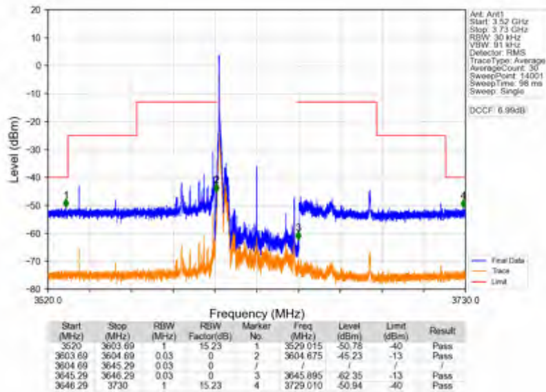
n78d_30kHz_SISO_NTV_40MHz_CP-OFDM QPSK_3624.99MHz_Edge_1RB_Left
