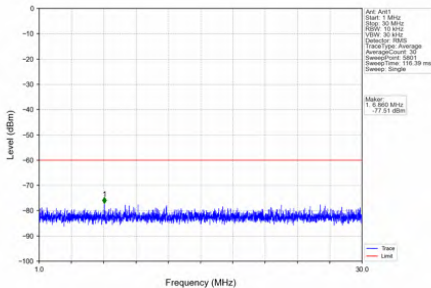
n78d_30kHz_SISO_NTNV_50MHz_DFT-s-OFDM QPSK_3575.01MHz_Edge_1RB_Left
