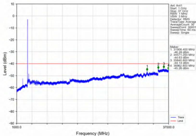
n78d_30kHz_SISO_NTNV_30MHz_DFT-s-OFDM PI/2 BPSK_3565.02MHz_Outer_Full
