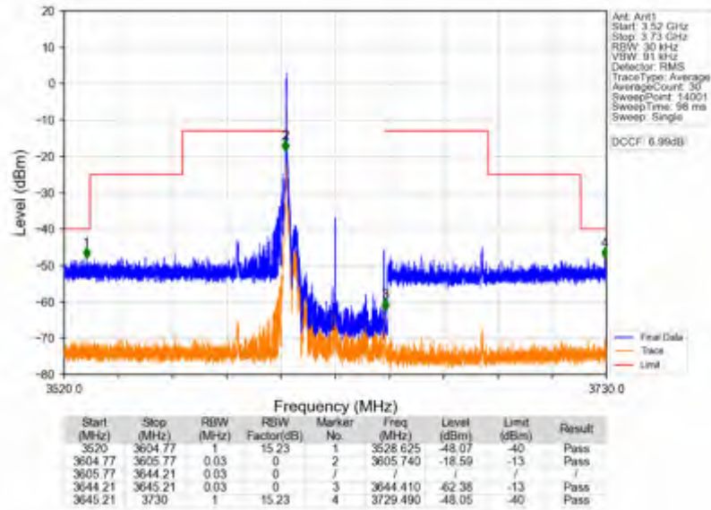
n78d_30kHz_SISO_NTNV_40MHz_DFT-s-OFDM QPSK_3624.99MHz_Edge_1RB_Left
