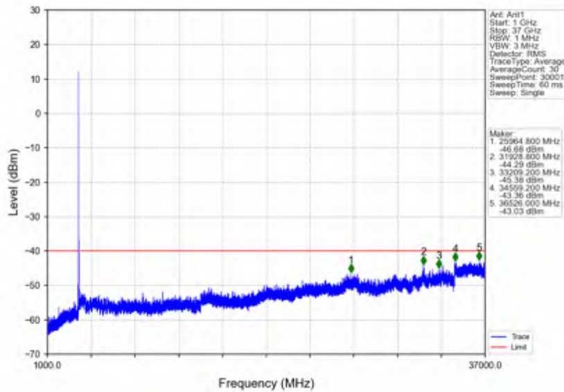
n78d_30kHz_SISO_NTV_30MHz_CP-OFDM_QPSK_3624.99MHz_Edge_1RB_Left
