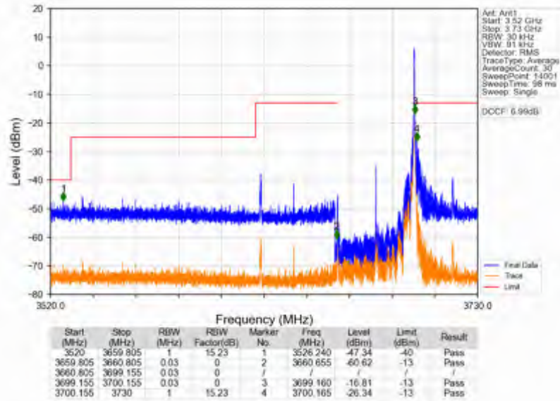
n78d_30kHz_SISO_NTNV_40MHz_CP-OFDM QPSK_3679.98MHz_Edge_1RB_Right
