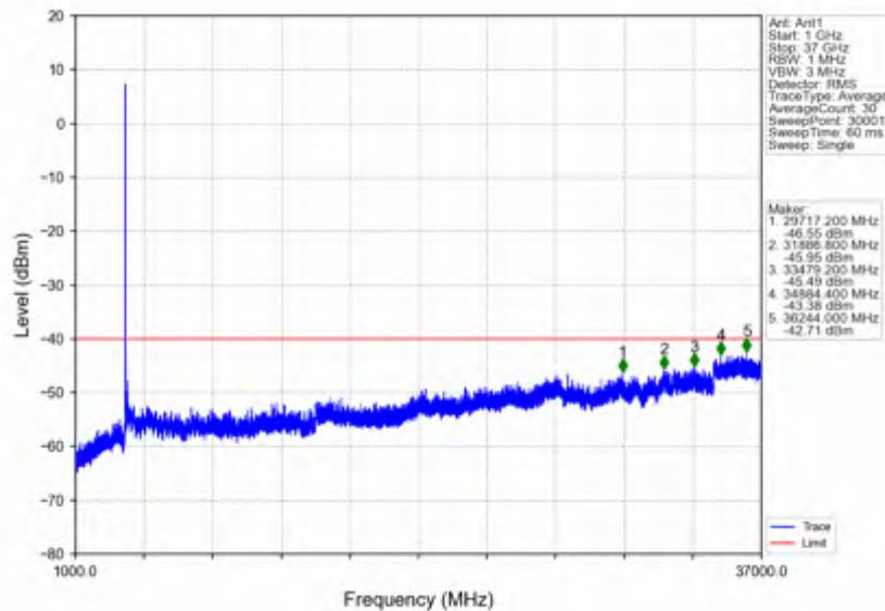
n78d_30kHz_SISO_NTV_25MHz_CP-OFDM QPSK_3624.99MHz_Edge_1RB_Left
