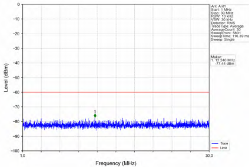
n78d_30kHz_SISO_NTNV_40MHz_CP-OFDM QPSK_3570MHz_Inner_1RB_Left
