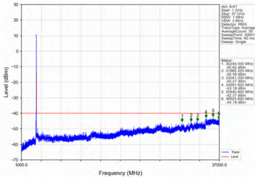
n78d_30kHz_SISO_NTNV_40MHz_CP-OFDM QPSK_3679.98MHz_Outer_Full
