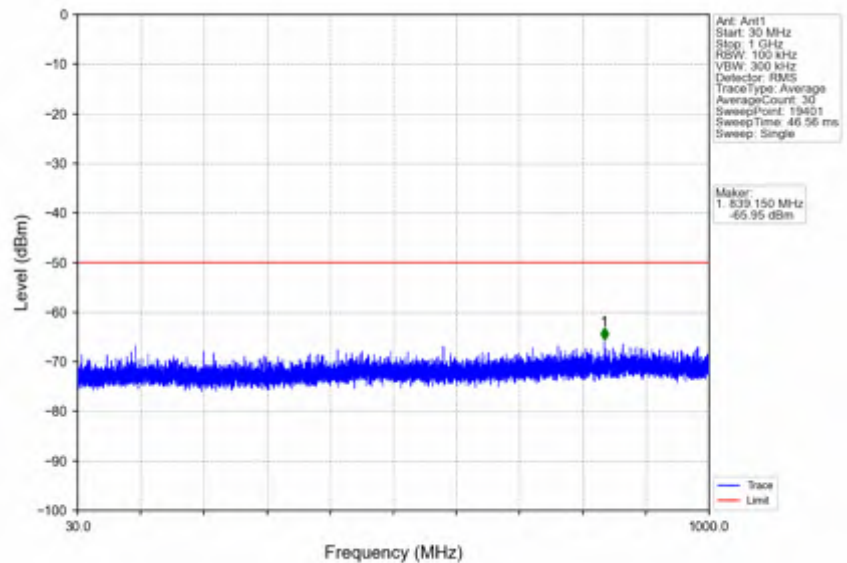
n78d_30kHz_SISO_NTNV_25MHz_CP-OFDM QPSK_3687.48MHz_Inner_1RB_Right
