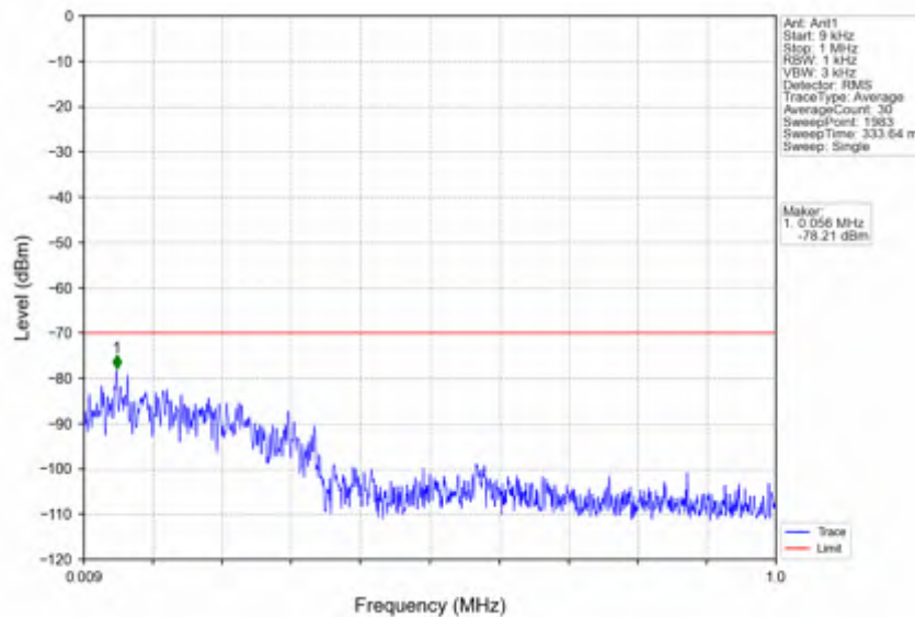
n78d_30kHz_SISO_NTNV_40MHz_CP-OFDM_QPSK_3570MHz_Edge_1RB_Left
