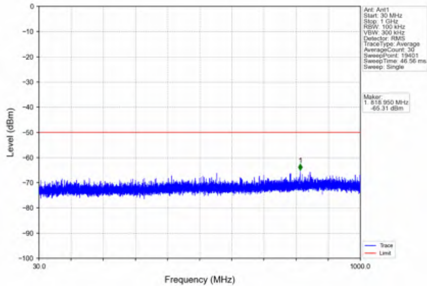
n78d_30kHz_SISO_NTNV_30MHz_DFT-s-OFDM QPSK_3684.99MHz_Inner_1RB_Right
