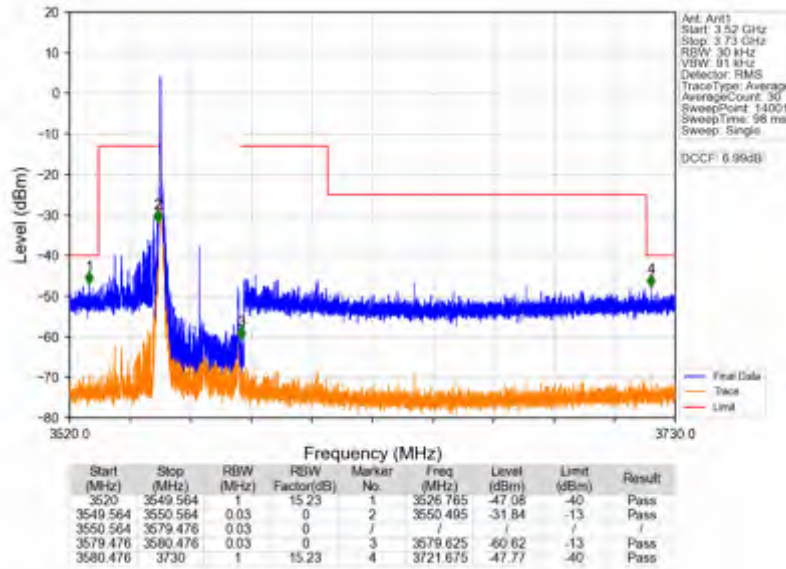
n78d_30kHz_SISO_NTV_30MHz_CP-OFDM_QPSK_3565.02MHz_Inner_1RB_Left
