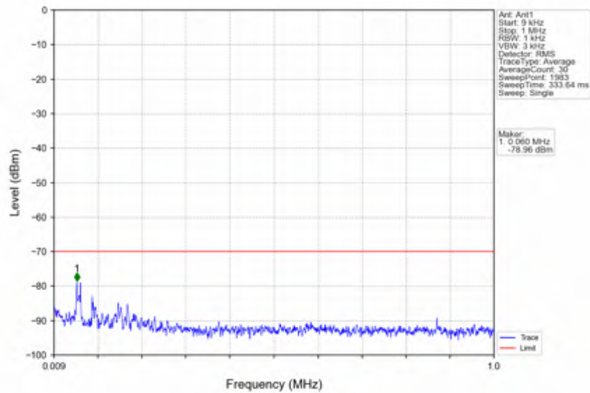
n78d_30kHz_SISO_NTVV_40MHz_CP-OFDM QPSK_3624.99MHz_Edge_1RB_Left
