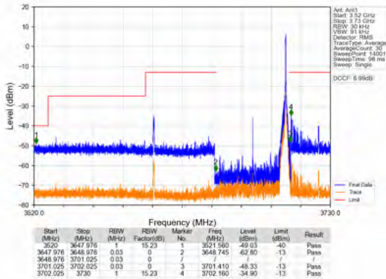
n78d_30kHz_SISO_NTNV_50MHz_DFT-s-OFDM_QPSK_3675MHz_Inner_1RB_Right
