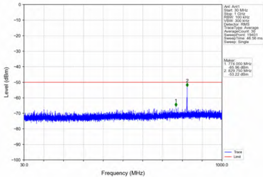
n78d_30kHz_SISO_NTNV_50MHz_DFT-s-OFDM_QPSK_3675MHz_Edge_1RB_Right
