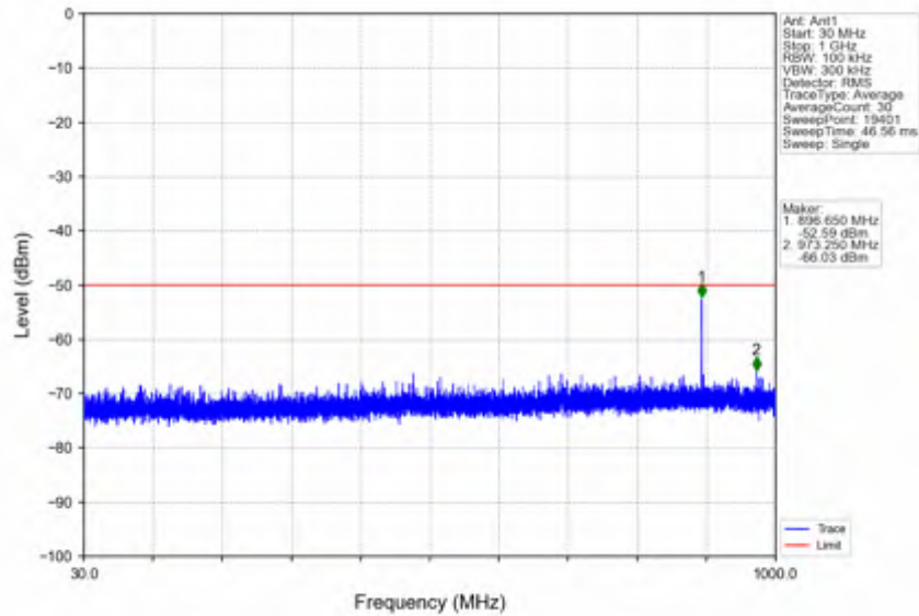
n78d_30kHz_SISO_NTVV_40MHz_DFT-s-OFDM_QPSK_3570MHz_Inner_1RB_Left
