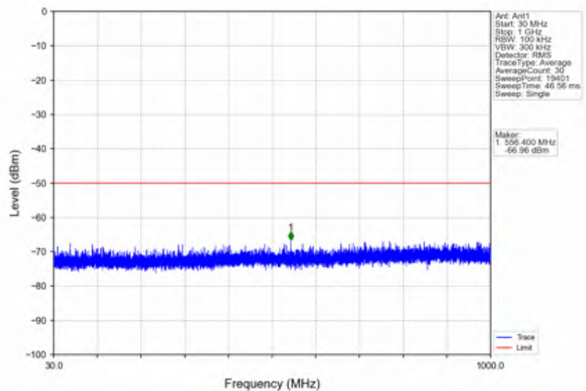
n78d_30kHz_SISO_NTVV_50MHz_CP-OFDM_QPSK_3575.01MHz_Edge_1RB_Left
