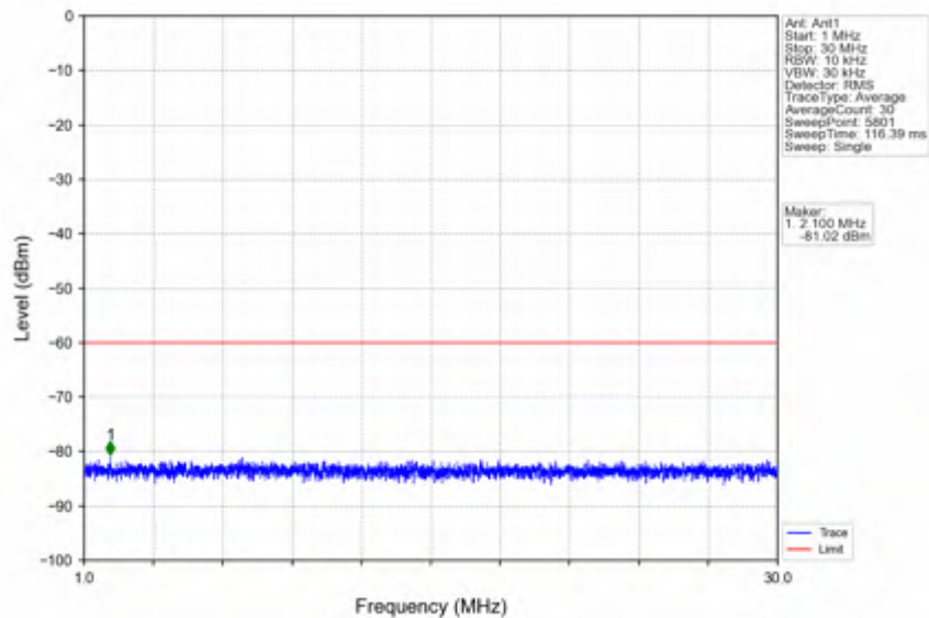
n78d_30kHz_SISO_NTNV_30MHz_DFT-s-OFDM PI/2 BPSK_3565.02MHz_Outer_Full
