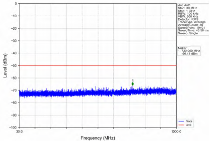
n78d_30kHz_SISO_NTVV_40MHz_DFT-s-OFDM_QPSK_3570MHz_Edge_1RB_Left
