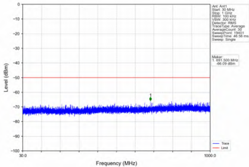
n78d_30kHz_SISO_NTNV_25MHz_CP-OFDM QPSK_3687.48MHz_Outer_Full
