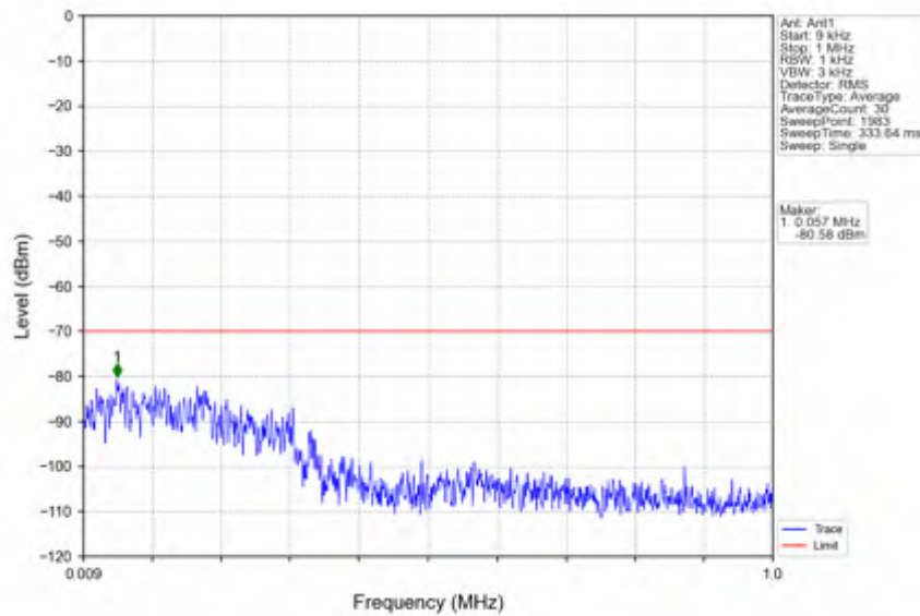
n78d_30kHz_SISO_NTV_25MHz_CP-OFDM QPSK_3624.99MHz_Edge_1RB_Left
