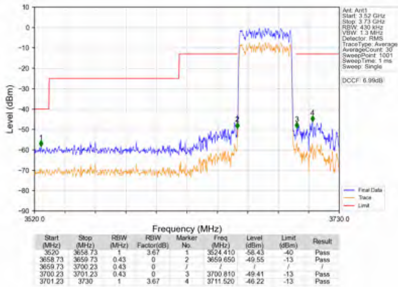
n78d_30kHz_SISO_NTNV_40MHz_DFT-s-OFDM PI/2 BPSK_3679.98MHz_Outer_Full
