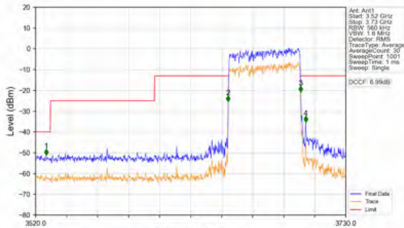
n78d_30kHz_SISO_NTNV_50MHz_CP-OFDM QPSK_3675MHz_Outer_Full
