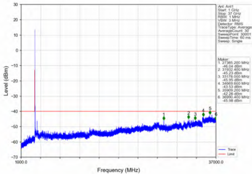
n78d_30kHz_SISO_NTV_50MHz_CP-OFDM_QPSK_3624.99MHz_Edge_1RB_Left
