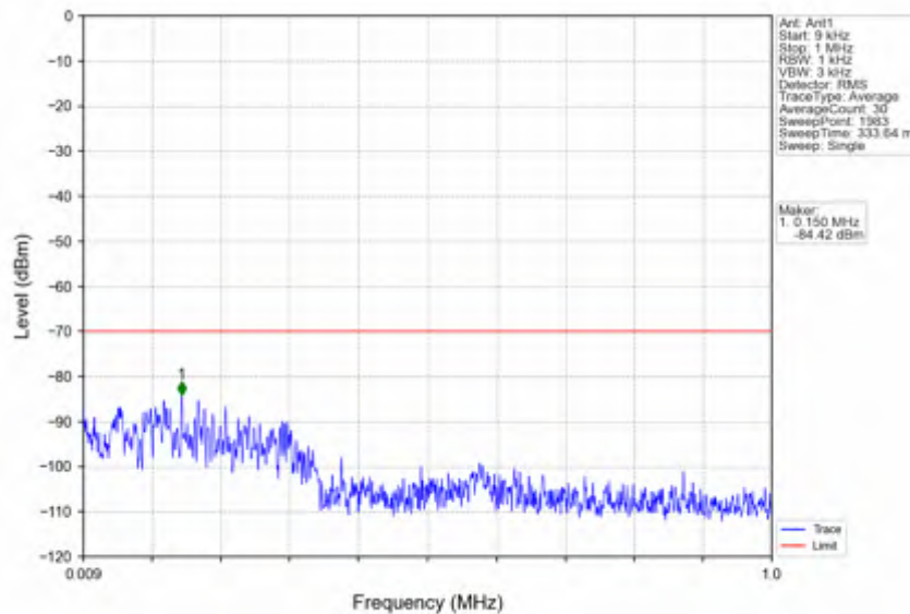
n78d_30kHz_SISO_NTNV_30MHz_DFT-s-OFDM QPSK_3624.99MHz_Edge_1RB_Left
