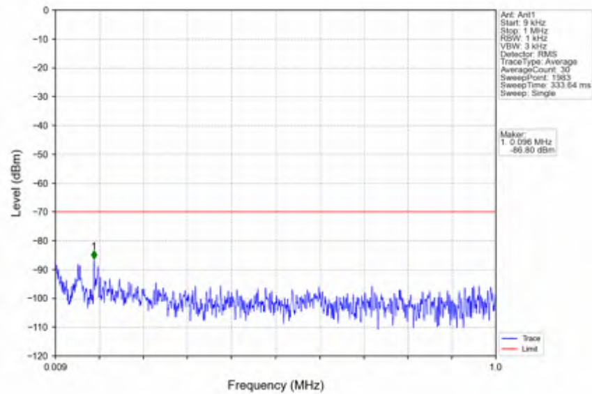
n78d_30kHz_SISO_NTNV_25MHz_CP-OFDM QPSK_3562.5MHz_Outer_Full
