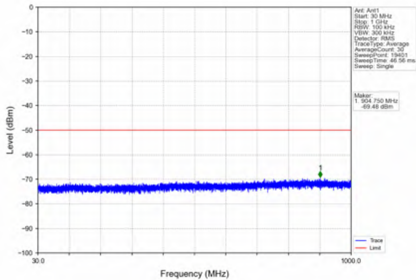
n78d_30kHz_SISO_NTNV_30MHz_DFT-s-OFDM PI/2 BPSK_3684.99MHz_Outer_Full
