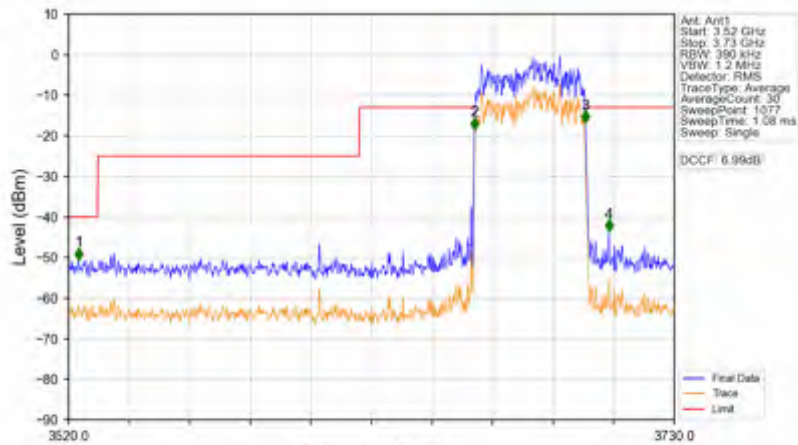
n78d_30kHz_SISO_NTNV_40MHz_CP-OFDM QPSK_3679.98MHz_Outer_Full
