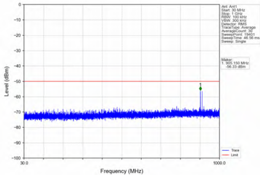
n78d_30kHz_SISO_NTVV_50MHz_CP-OFDM QPSK_3624.99MHz_Edge_1RB_Left
