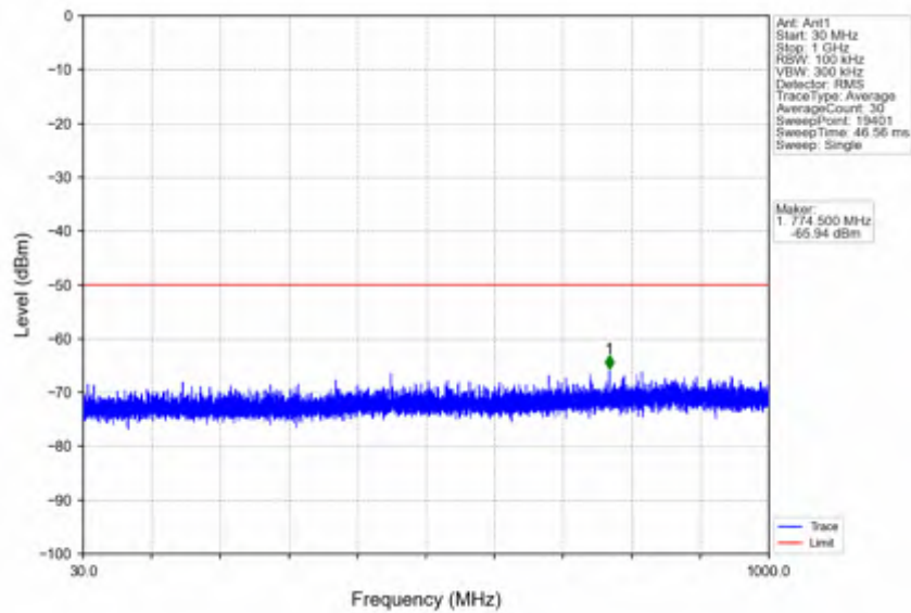
n78d_30kHz_SISO_NTV_30MHz_CP-OFDM QPSK_3624.99MHz_Edge_1RB_Left
