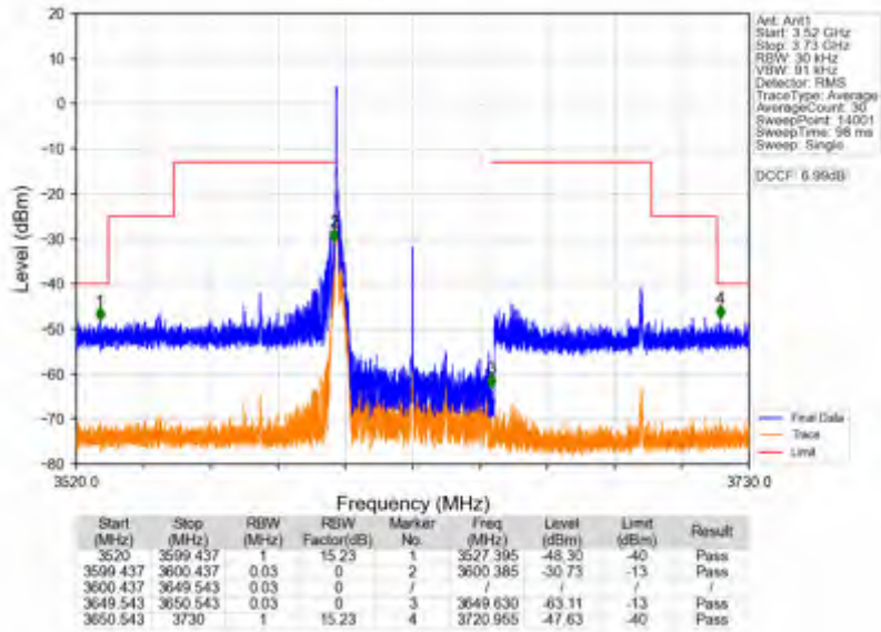
n78d_30kHz_SISO_NTV_50MHz_CP-OFDM_QPSK_3624.99MHz_Edge_1RB_Left
