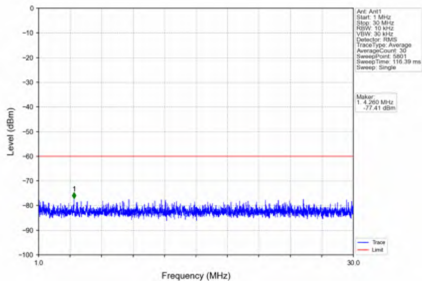
n78d_30kHz_SISO_NTNV_30MHz_DFT-s-OFDM QPSK_3565.02MHz_Inner_1RB_Left
