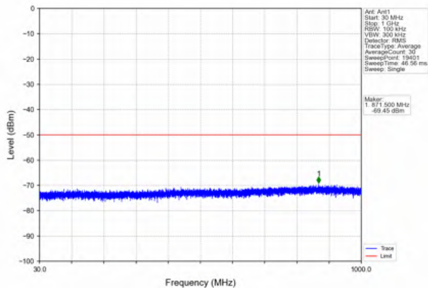
n78d_30kHz_SISO_NTV_50MHz_DFT-s-OFDM_PI/2_BPSK_3675MHz_Inner_1RB_Right
