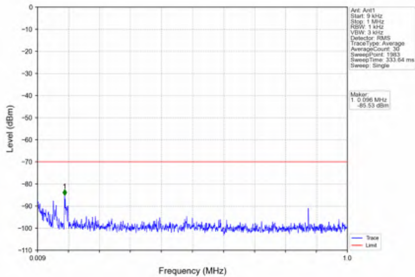
n78d_30kHz_SISO_NTNV_40MHz_DFT-s-OFDM PI/2 BPSK_3679.98MHz_Outer_Full
