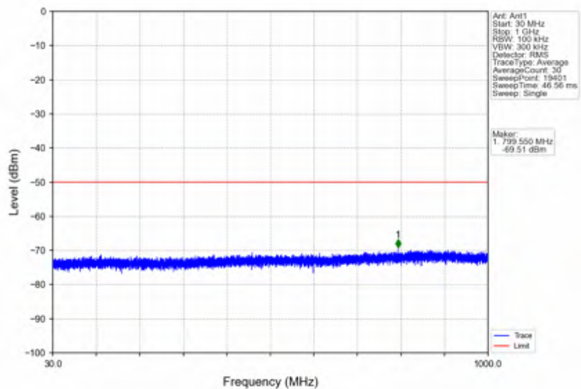
n78d_30kHz_SISO_NTNV_40MHz_DFT-s-OFDM_QPSK_3679.98MHz_Outer_Full
