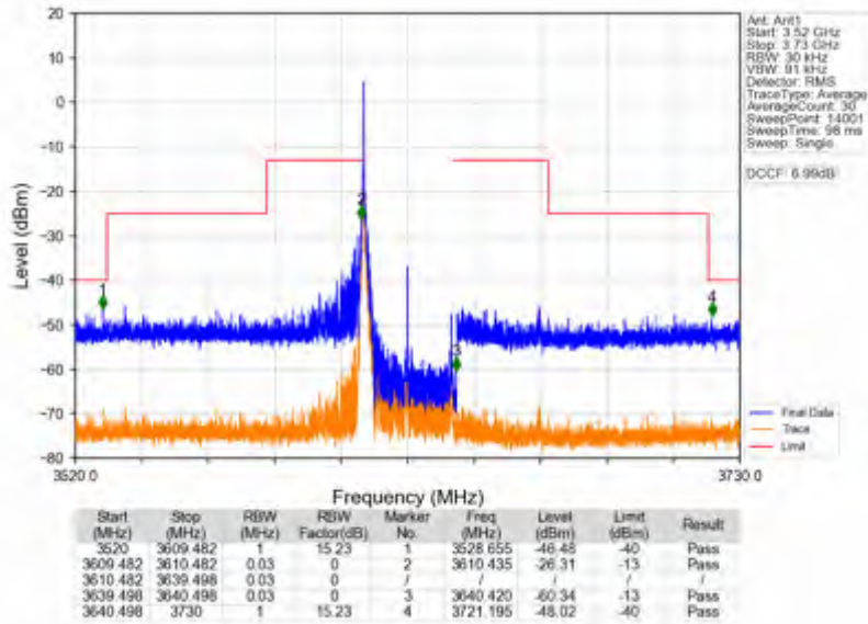
n78d_30kHz_SISO_NTV_30MHz_CP-OFDM_QPSK_3624.99MHz_Edge_1RB_Left
