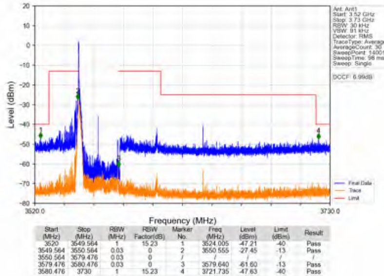
n78d_30kHz_SISO_NTV_30MHz_CP-OFDM QPSK_3565.02MHz_Edge_1RB_Left
