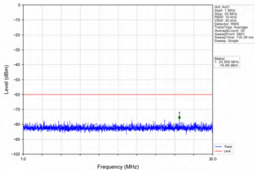
n78d_30kHz_SISO_NTNV_25MHz_CP-OFDM QPSK_3687.48MHz_Outer_Full
