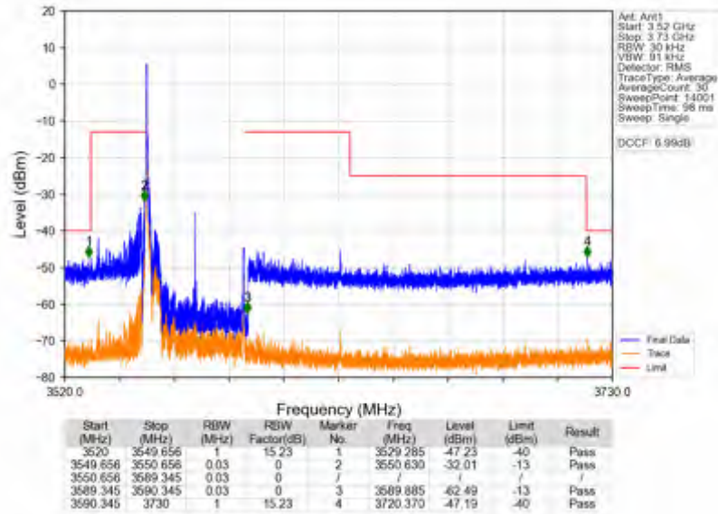
n78d_30kHz_SISO_NTNV_40MHz_CP-OFDM_QPSK_3570MHz_Inner_1RB_Left
