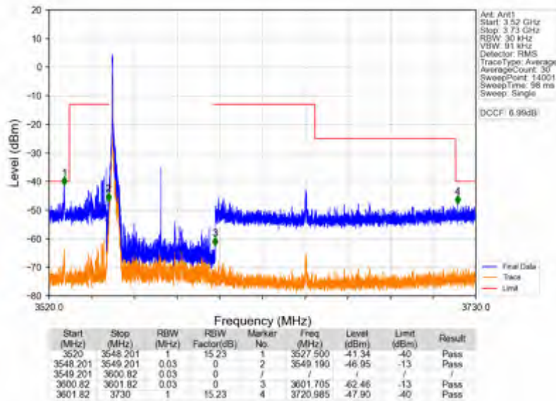
n78d_30kHz_SISO_NTNV_50MHz_DFT-s-OFDM QPSK_3575.01MHz_Edge_1RB_Left
