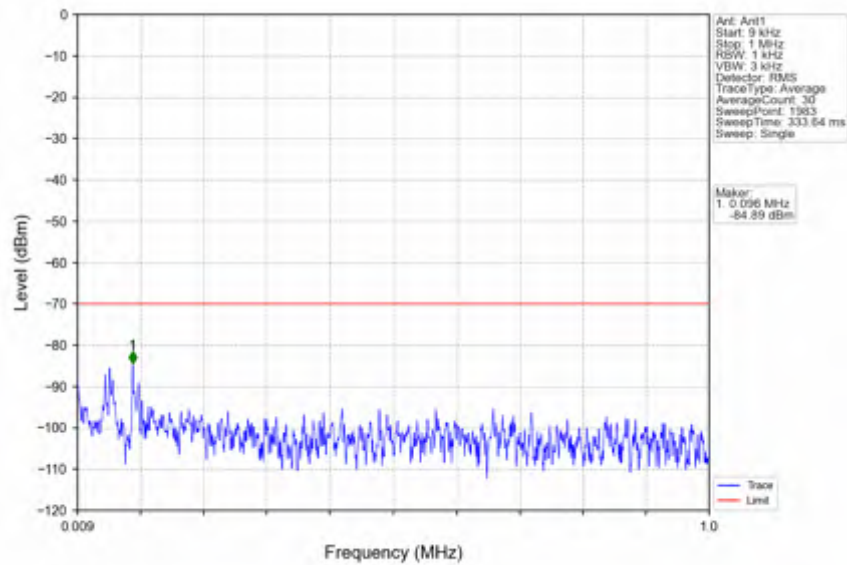
n78d_30kHz_SISO_NTNV_30MHz_CP-OFDM QPSK_3565.02MHz_Outer_Full
