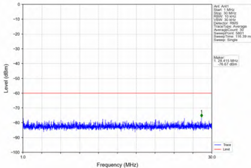
n78d_30kHz_SISO_NTNV_40MHz_DFT-s-OFDM QPSK_3679.98MHz_Inner_1RB_Right
