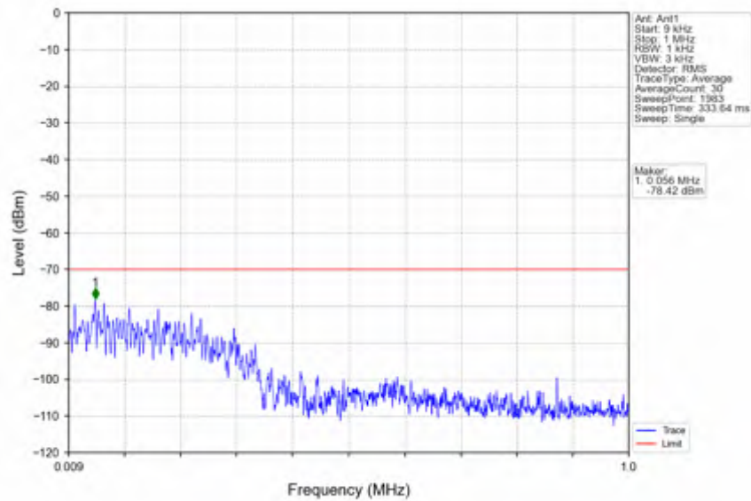
n78d_30kHz_SISO_NTVV_50MHz_CP-OFDM QPSK_3624.99MHz_Edge_1RB_Left
