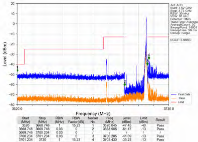
n78d_30kHz_SISO_NTNV_30MHz_DFT-s-OFDM QPSK_3684.99MHz_Edge_1RB_Right
