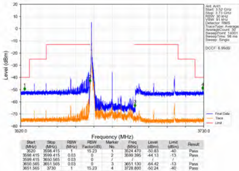
n78d_30kHz_SISO_NTNV_50MHz_DFT-s-OFDM PI/2 BPSK_3624.99MHz_Edge_1RB_Left
