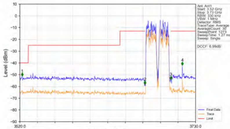
n78d_30kHz_SISO_NTNV_30MHz_DFT-s-OFDM PI/2 BPSK_3684.99MHz_Outer_Full
