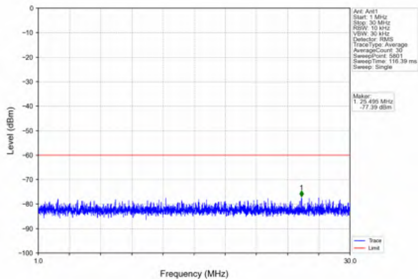
n78d_30kHz_SISO_NTNV_30MHz_DFT-s-OFDM QPSK_3684.99MHz_Inner_1RB_Right
