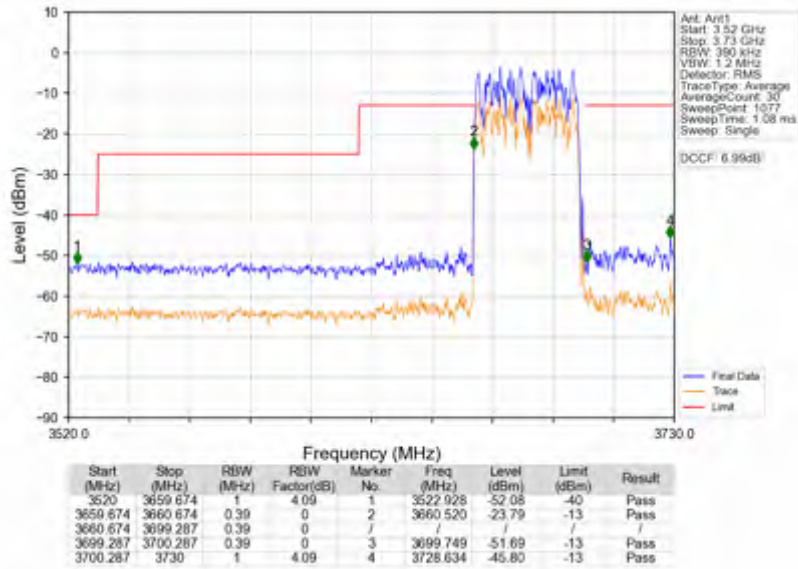
n78d_30kHz_SISO_NTNV_40MHz_DFT-s-OFDM QPSK_3679.98MHz_Outer_Full
