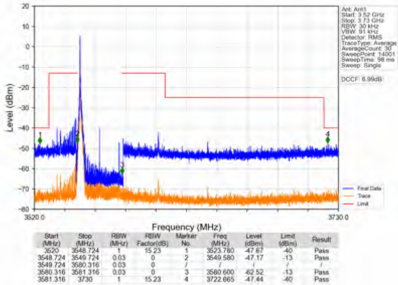
n78d_30kHz_SISO_NTNV_30MHz_DFT-s-OFDM QPSK_3565.02MHz_Inner_1RB_Left
