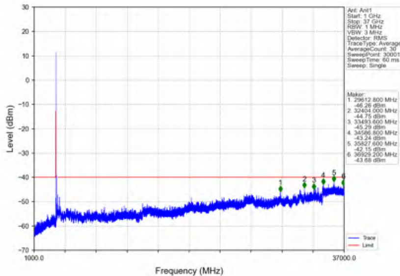
n78d_30kHz_SISO_NTVV_40MHz_DFT-s-OFDM_QPSK_3570MHz_Inner_1RB_Left
