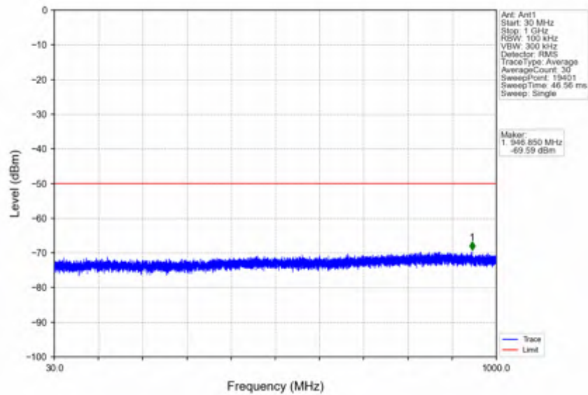
n78d_30kHz_SISO_NTVV_40MHz_CP-OFDM QPSK_3624.99MHz_Edge_1RB_Left
