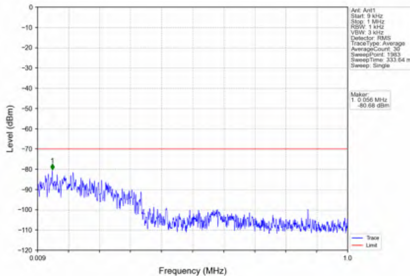
n78d_30kHz_SISO_NTNV_40MHz_CP-OFDM QPSK_3679.98MHz_Inner_1RB_Right
