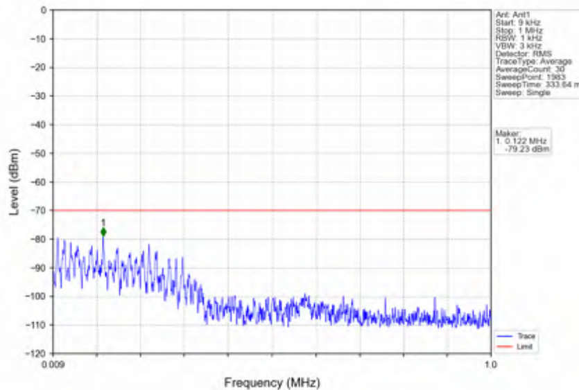
n78d_30kHz_SISO_NTV_30MHz_CP-OFDM QPSK_3684.99MHz_Edge_1RB_Right
