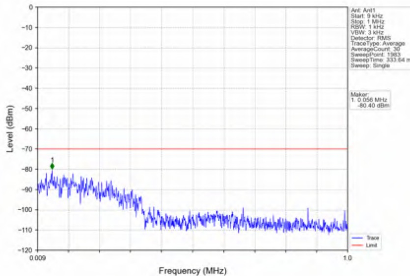
n78d_30kHz_SISO_NTNV_40MHz_CP-OFDM QPSK_3679.98MHz_Edge_1RB_Right
