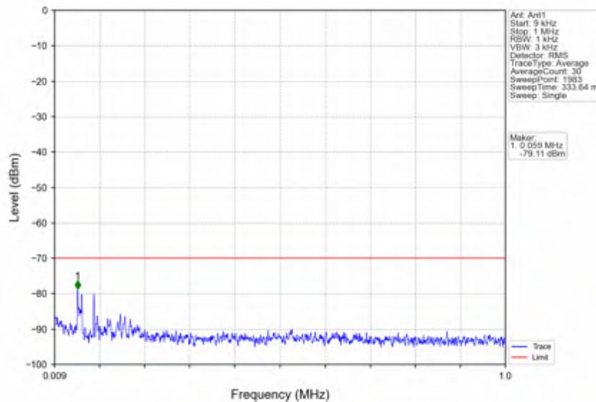
n78d_30kHz_SISO_NTNV_40MHz_DFT-s-OFDM PI/2 BPSK_3679.98MHz_Edge_1RB_Right
