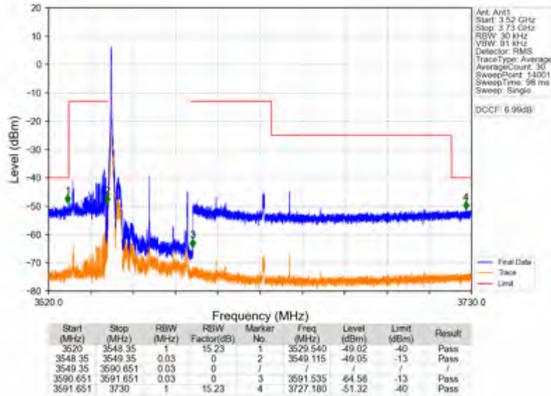
n78d_30kHz_SISO_NTNV_40MHz_DFT-s-OFDM PI/2 BPSK_3570MHz_Edge_1RB_Left
