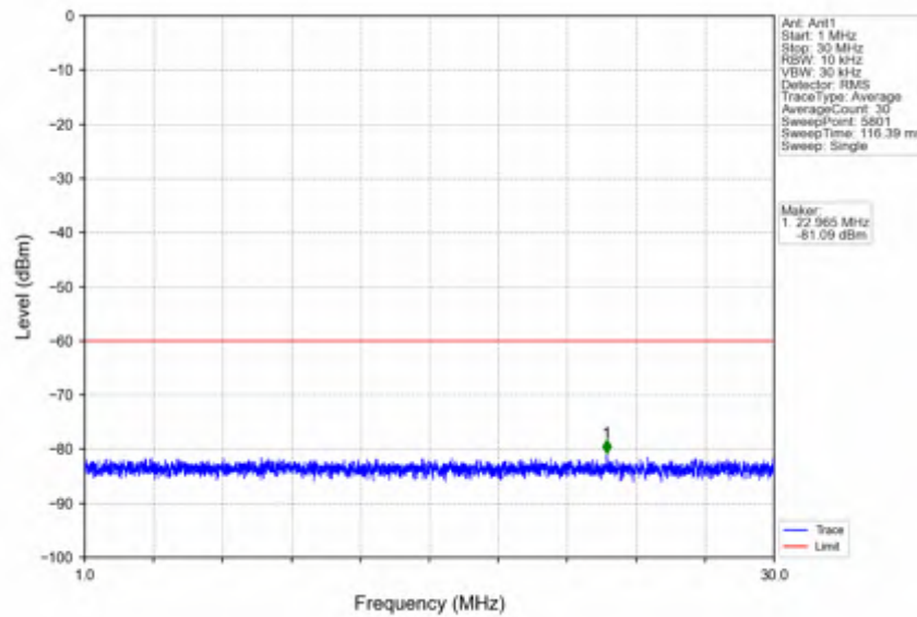
n78d_30kHz_SISO_NTNV_30MHz_DFT-s-OFDM PI/2 BPSK_3684.99MHz_Edge_1RB_Right
