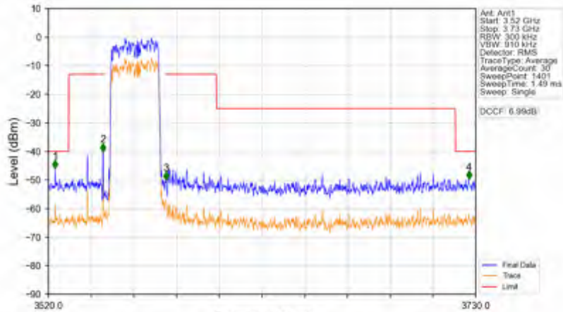
n78d_30kHz_SISO_NTNV_25MHz_CP-OFDM QPSK_3562.5MHz_Outer_Full
