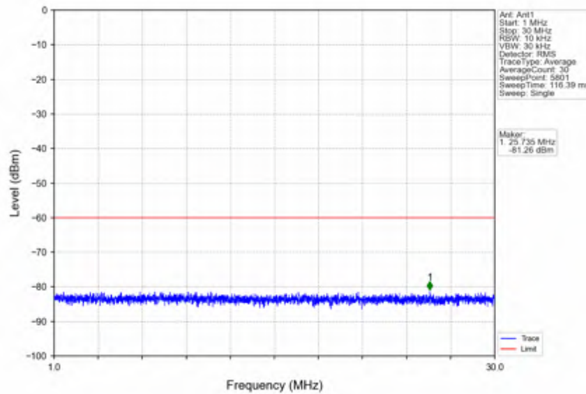
n78d_30kHz_SISO_NTNV_30MHz_DFT-s-OFDM PI/2 BPSK_3565.02MHz_Inner_1RB_Left
