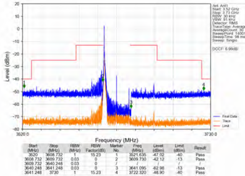
n78d_30kHz_SISO_NTNV_30MHz_DFT-s-OFDM QPSK_3624.99MHz_Edge_1RB_Left
