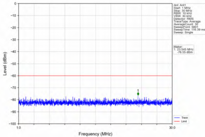
n78d_30kHz_SISO_NTNV_30MHz_DFT-s-OFDM_QPSK_3684.99MHz_Outer_Full
