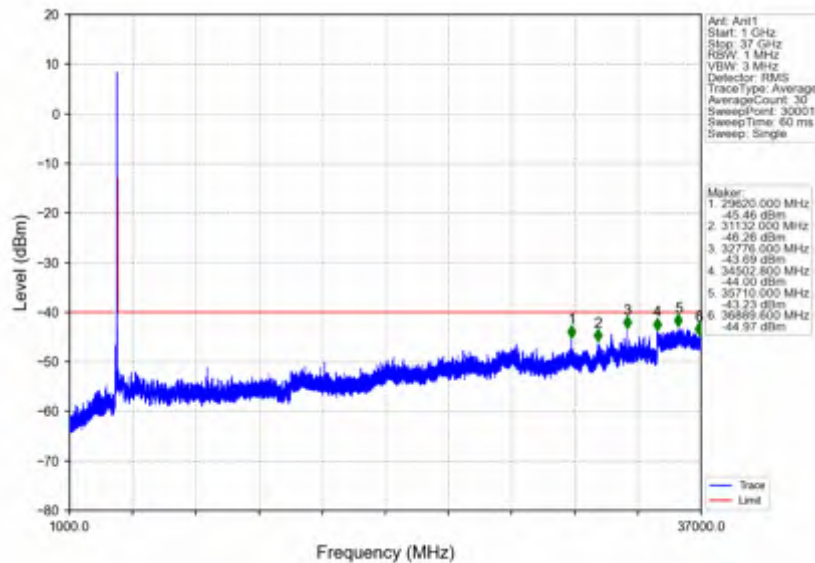
n78d_30kHz_SISO_NTNV_50MHz_DFT-s-OFDM_QPSK_3675MHz_Edge_1RB_Right
