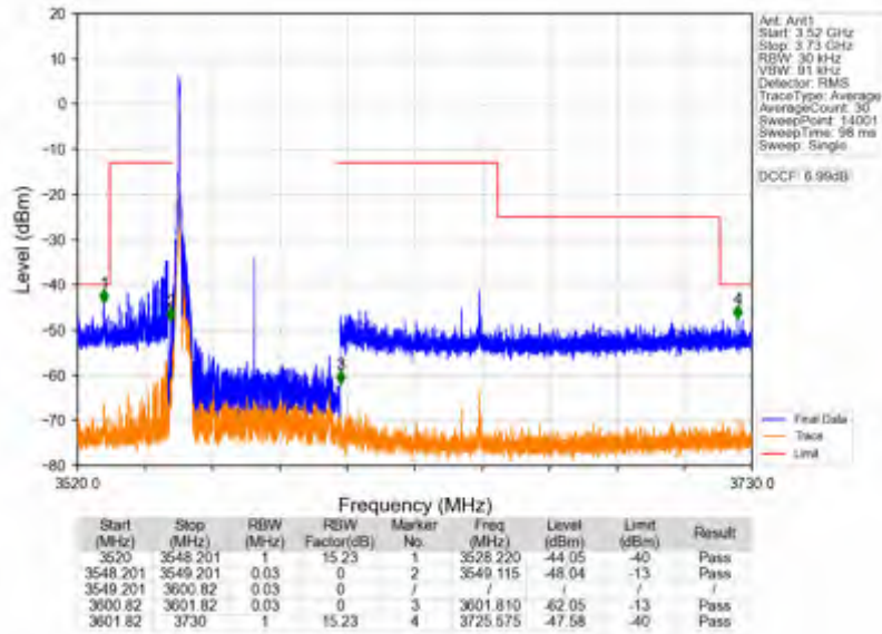
n78d_30kHz_SISO_NTV_50MHz_CP-OFDM_QPSK_3575.01MHz_Inner_1RB_Left
