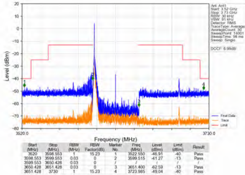
n78d_30kHz_SISO_NTNV_50MHz_DFT-s-OFDM_QPSK_3624.99MHz_Edge_1RB_Left
