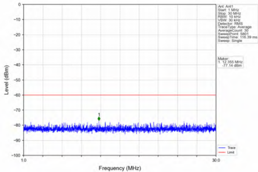
n78d_30kHz_SISO_NTNV_25MHz_CP-OFDM QPSK_3562.5MHz_Inner_1RB_Left
