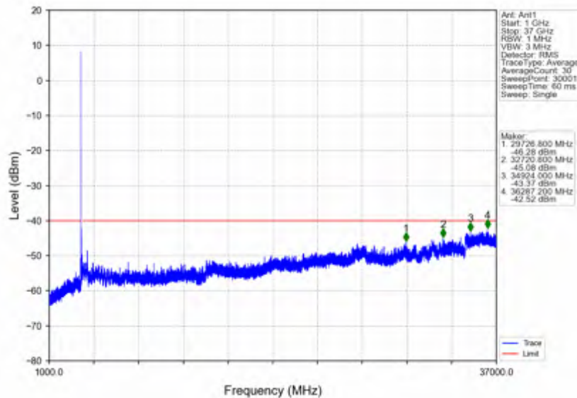
n78d_30kHz_SISO_NTNV_30MHz_DFT-s-OFDM QPSK_3565.02MHz_Edge_1RB_Left
