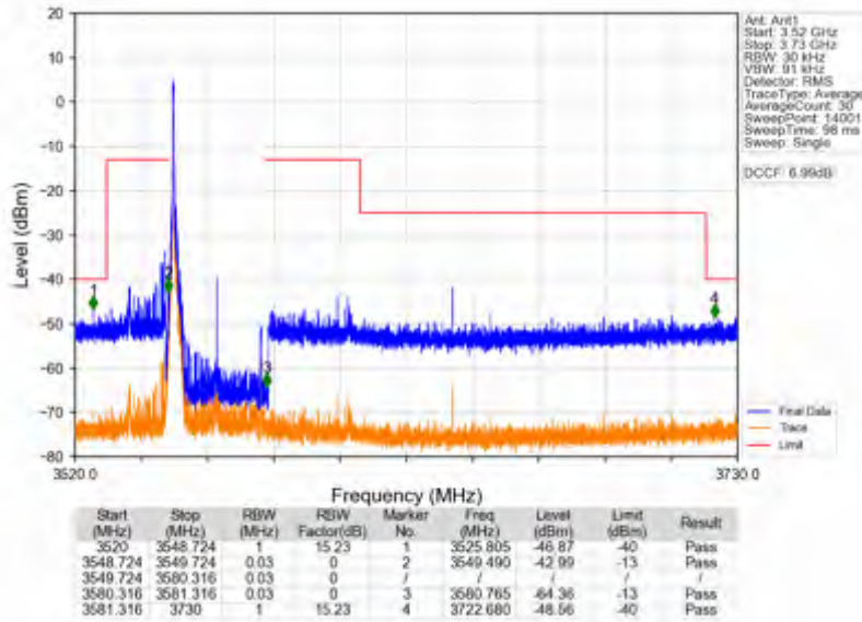
n78d_30kHz_SISO_NTNV_30MHz_DFT-s-OFDM QPSK_3565.02MHz_Edge_1RB_Left
