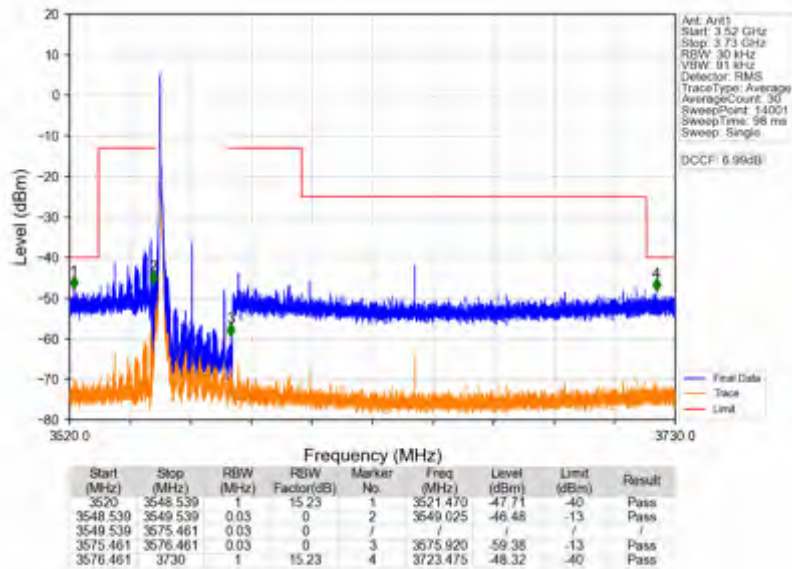
n78d_30kHz_SISO_NTNV_25MHz_DFT-s-OFDM QPSK_3562.5MHz_Inner_1RB_Left
