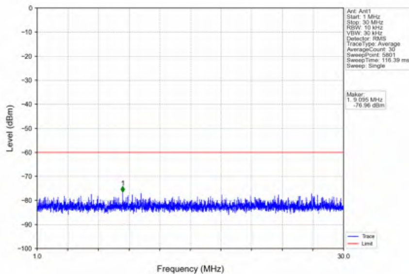
n78d_30kHz_SISO_NTNV_50MHz_DFT-s-OFDM QPSK_3575.01MHz_Inner_1RB_Left
