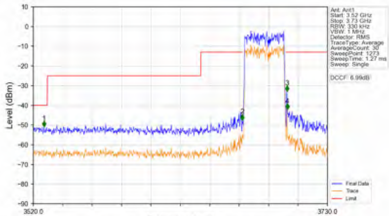
n78d_30kHz_SISO_NTNV_30MHz_CP-OFDM QPSK_3684.99MHz_Outer_Full
