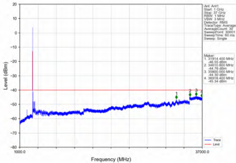
n78d_30kHz_SISO_NTNV_50MHz_DFT-s-OFDM PI/2 BPSK_3575.01MHz_Outer_Full
