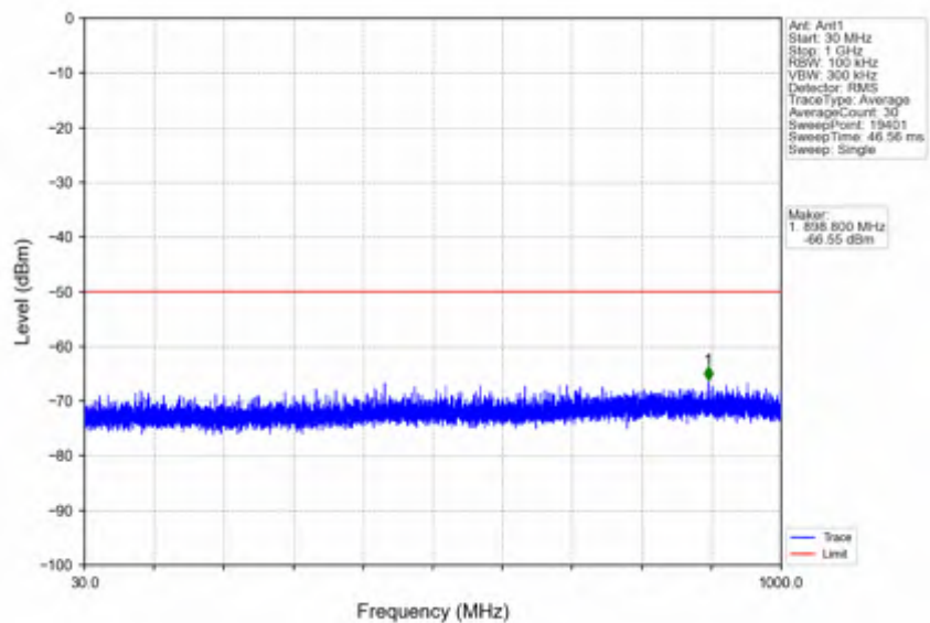
n78d_30kHz_SISO_NTNV_40MHz_DFT-s-OFDM_QPSK_3624.99MHz_Edge_1RB_Left
