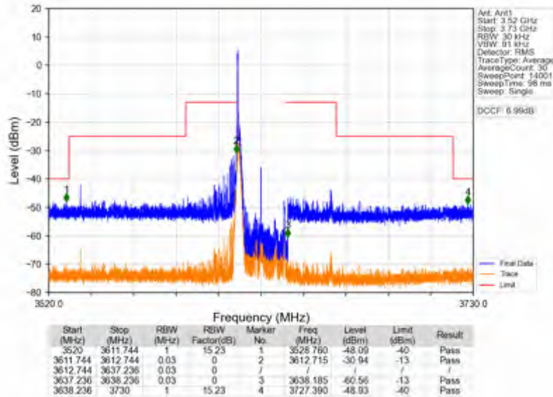
n78d_30kHz_SISO_NTNV_25MHz_CP-OFDM QPSK_3624.99MHz_Edge_1RB_Left
