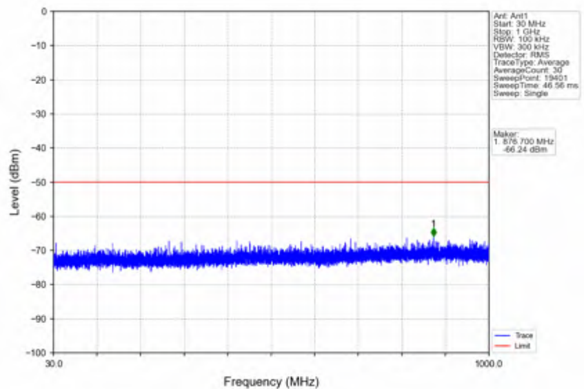
n78d_30kHz_SISO_NTVV_30MHz_CP-OFDM QPSK_3565.02MHz_Edge_1RB_Left
