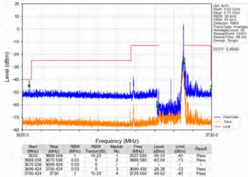
n78d_30kHz_SISO_NTV_30MHz_CP-OFDM QPSK_3684.99MHz_Edge_1RB_Right
