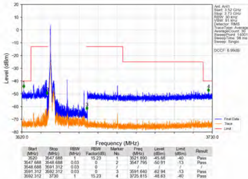
n78d_30kHz_SISO_NTNV_40MHz_DFT-s-OFDM QPSK_3570MHz_Inner_1RB_Left
