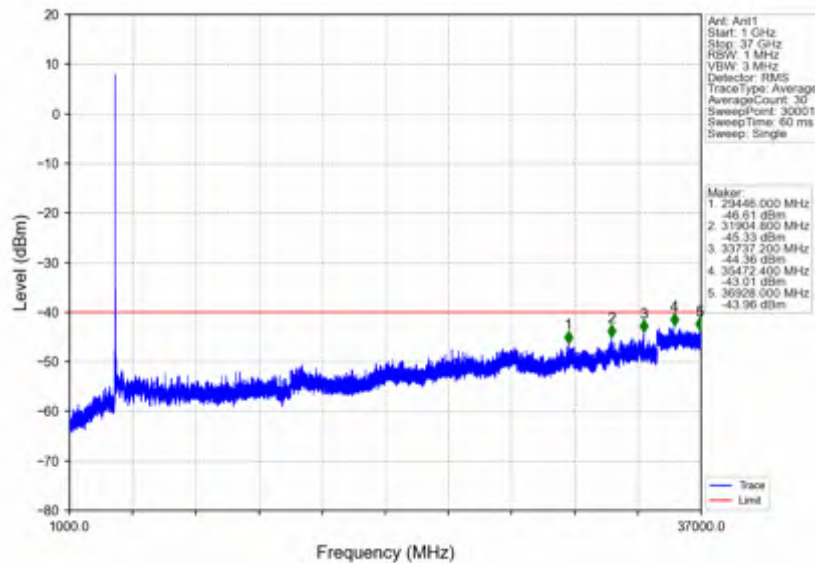
n78d_30kHz_SISO_NTVV_50MHz_CP-OFDM QPSK_3624.99MHz_Edge_1RB_Left
