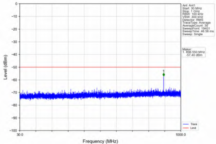
n78d_30kHz_SISO_NTNV_40MHz_DFT-s-OFDM_QPSK_3570MHz_Outer_Full
