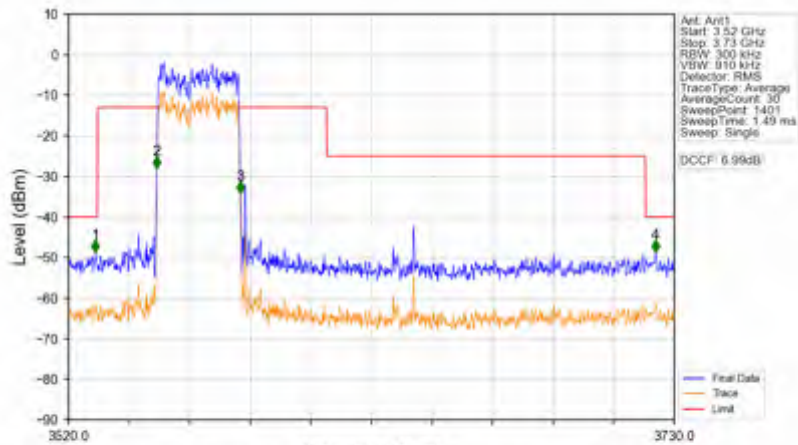
n78d_30kHz_SISO_NTNV_30MHz_CP-OFDM QPSK_3565.02MHz_Outer_Full
