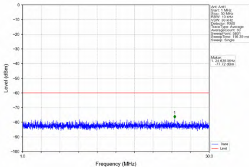
n78d_30kHz_SISO_NTNV_40MHz_DFT-s-OFDM QPSK_3679.98MHz_Edge_1RB_Right
