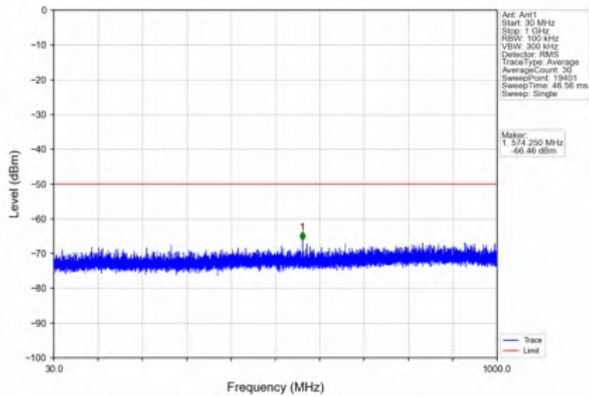
n78d_30kHz_SISO_NTNV_25MHz_DFT-s-OFDM QPSK_3687.48MHz_Inner_1RB_Right
