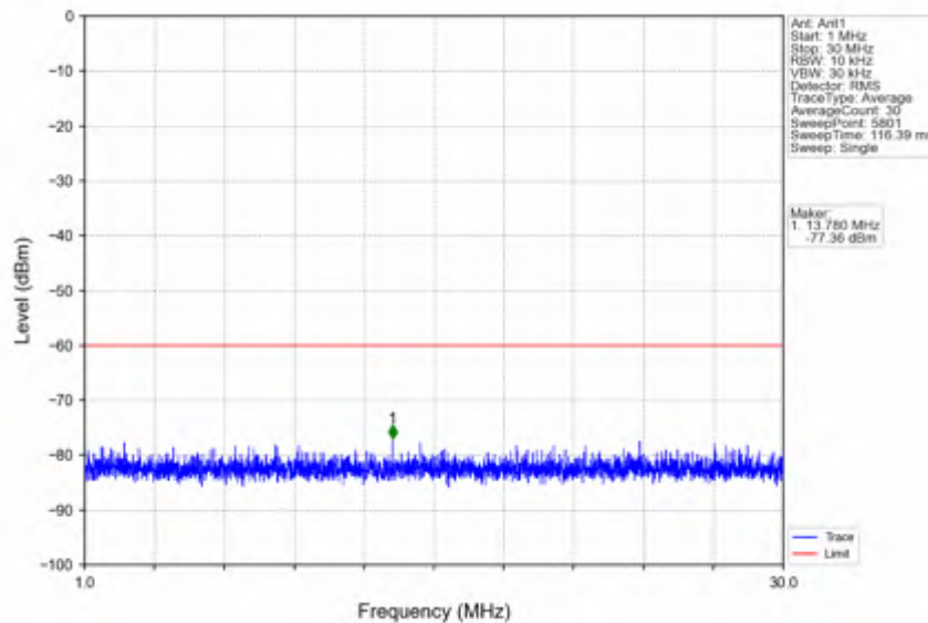
n78d_30kHz_SISO_NTNV_25MHz_DFT-s-OFDM QPSK_3562.5MHz_Inner_1RB_Left
