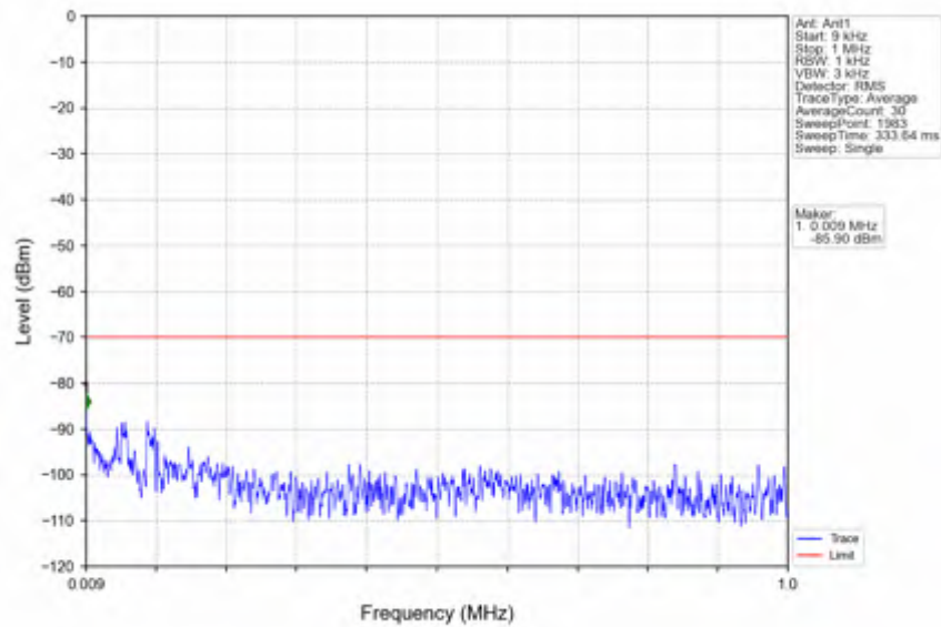
n78d_30kHz_SISO_NTNV_40MHz_CP-OFDM QPSK_3679.98MHz_Outer_Full
