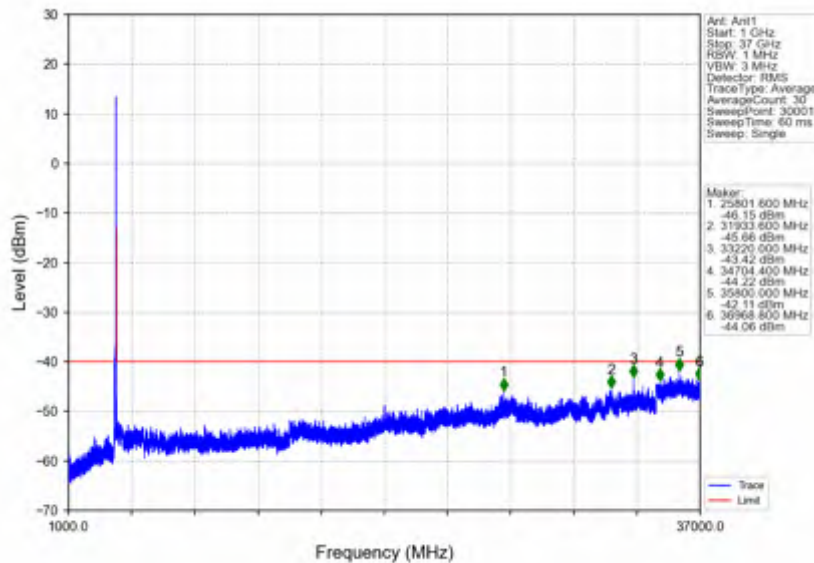
n78d_30kHz_SISO_NTNV_40MHz_DFT-s-OFDM QPSK_3679.98MHz_Edge_1RB_Right
