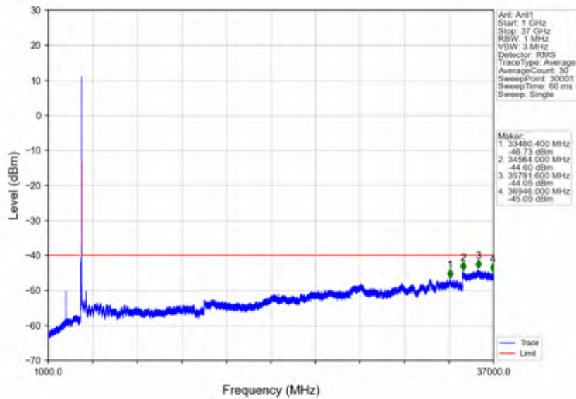
n78d_30kHz_SISO_NTNV_40MHz_DFT-s-OFDM QPSK_3570MHz_Edge_1RB_Left
