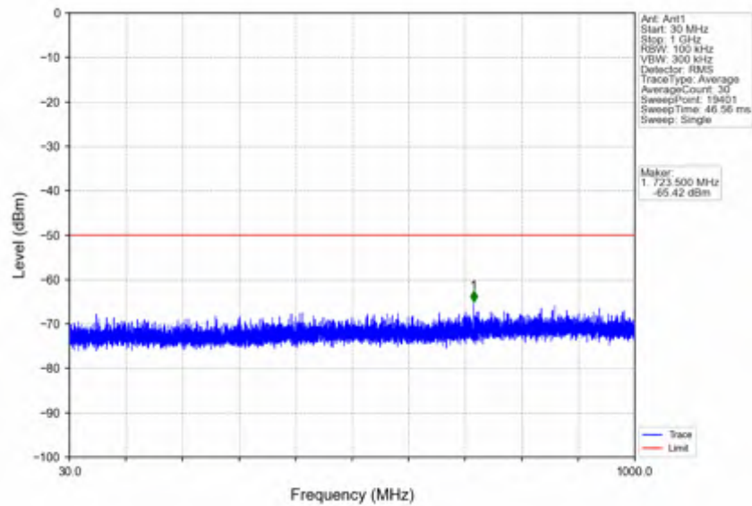
n78d_30kHz_SISO_NTNV_40MHz_CP-OFDM QPSK_3679.98MHz_Outer_Full
