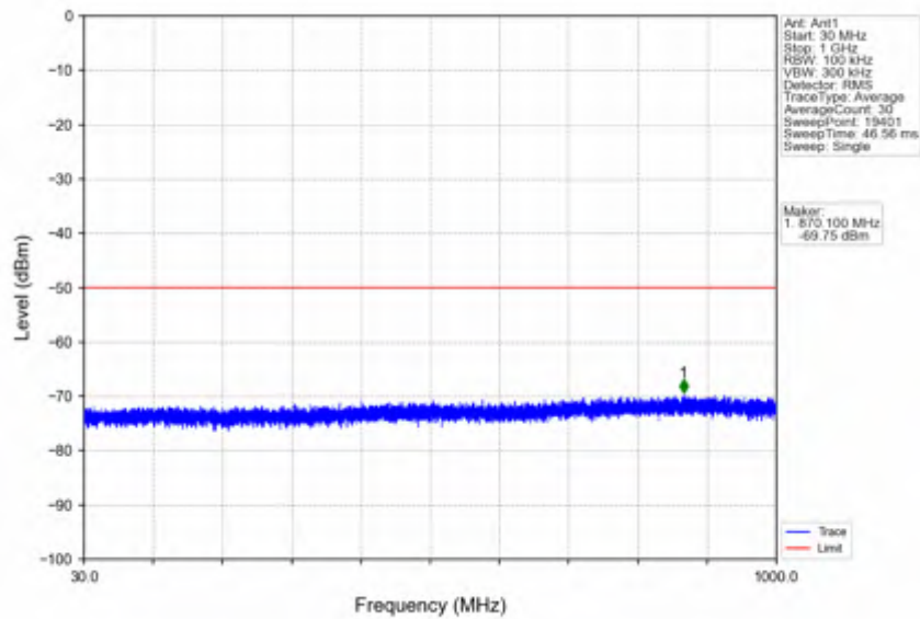
n78d_30kHz_SISO_NTNV_50MHz_DFT-s-OFDM PI/2 BPSK_3675MHz_Outer_Full
