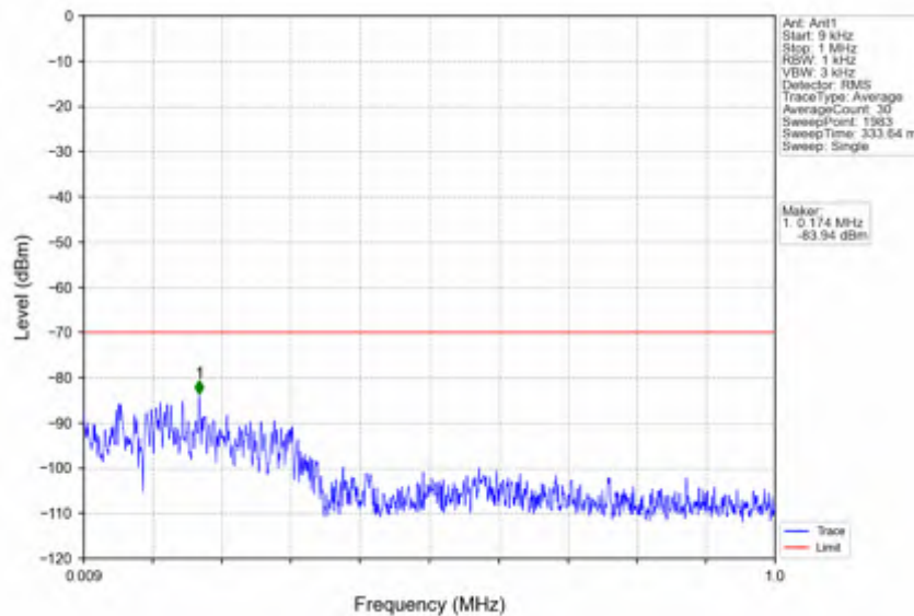
n78d_30kHz_SISO_NTNV_50MHz_DFT-s-OFDM_QPSK_3624.99MHz_Edge_1RB_Left
