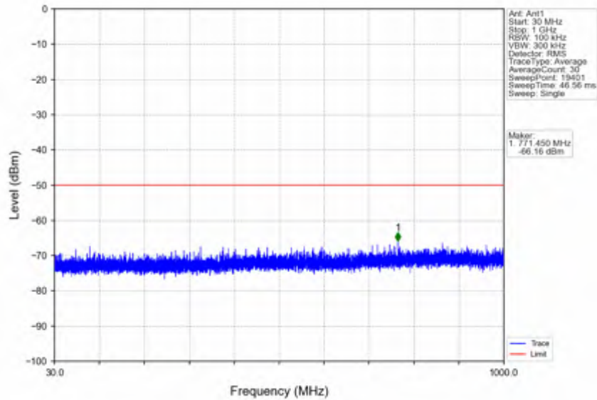
n78d_30kHz_SISO_NTNV_40MHz_DFT-s-OFDM QPSK_3679.98MHz_Edge_1RB_Right
