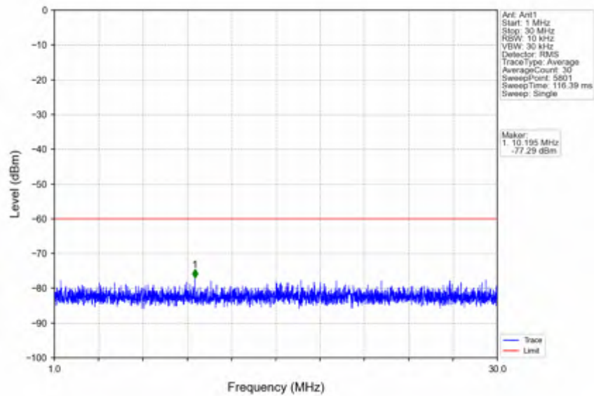
n78d_30kHz_SISO_NTNV_50MHz_CP-OFDM QPSK_3675MHz_Edge_1RB_Right
