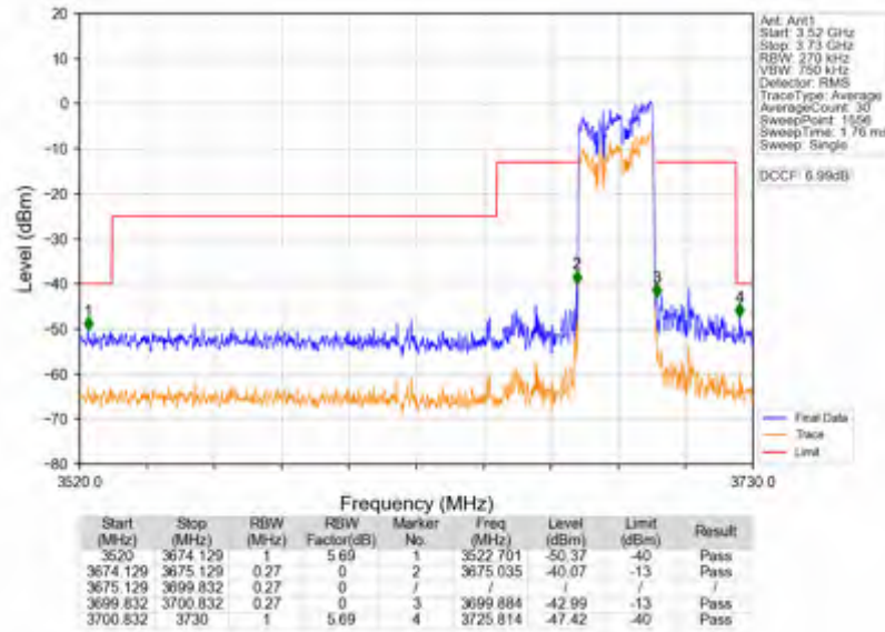
n78d_30kHz_SISO_NTNV_25MHz_DFT-s-OFDM QPSK_3687.48MHz_Outer_Full
