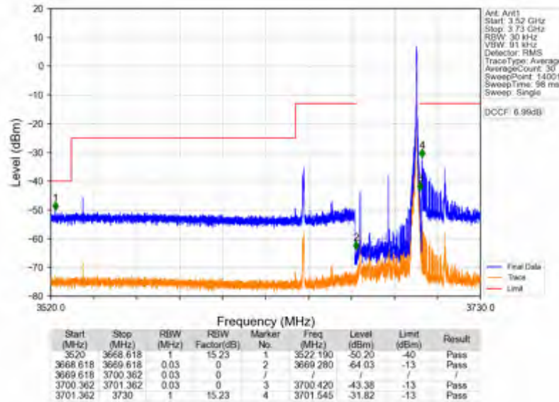
n78d_30kHz_SISO_NTNV_30MHz_DFT-s-OFDM PI/2 BPSK_3684.99MHz_Edge_1RB_Right
