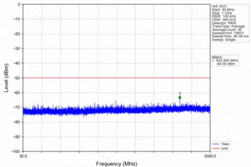
n78d_30kHz_SISO_NTVV_50MHz_CP-OFDM QPSK_3575.01MHz_Inner_1RB_Left
