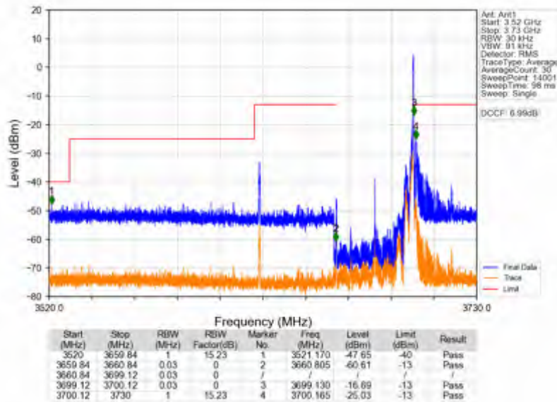
n78d_30kHz_SISO_NTNV_40MHz_DFT-s-OFDM QPSK_3679.98MHz_Edge_1RB_Right
