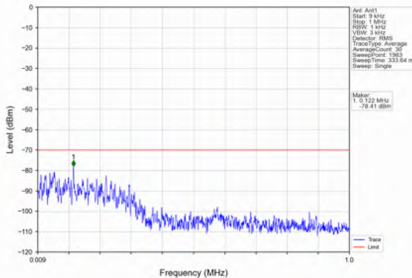
n78d_30kHz_SISO_NTV_30MHz_CP-OFDM QPSK_3684.99MHz_Inner_1RB_Right
