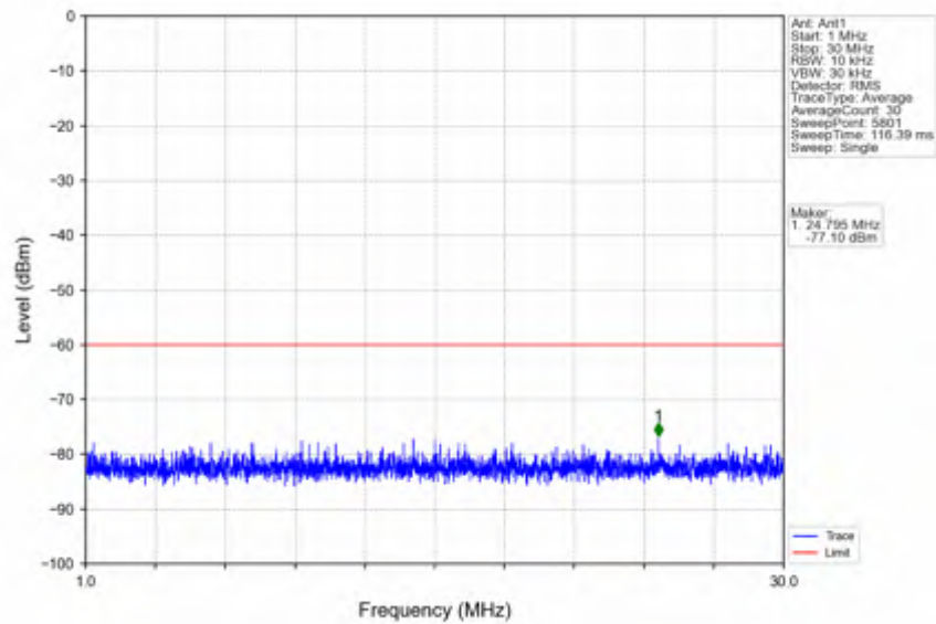
n78d_30kHz_SISO_NTNV_25MHz_CP-OFDM QPSK_3562.5MHz_Edge_1RB_Left
