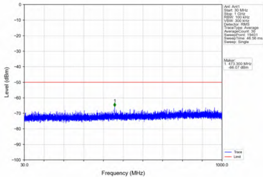
n78d_30kHz_SISO_NTNV_50MHz_DFT-s-OFDM QPSK_3675MHz_Inner_1RB_Right
