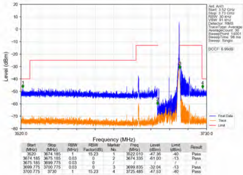
n78d_30kHz_SISO_NTNV_25MHz_DFT-s-OFDM QPSK_3687.48MHz_Edge_1RB_Right
