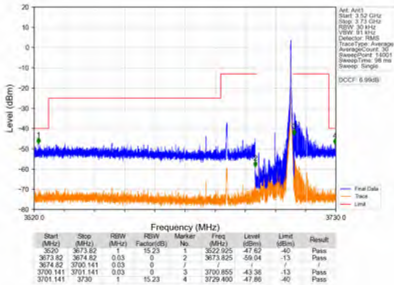
n78d_30kHz_SISO_NTNV_25MHz_DFT-s-OFDM QPSK_3687.48MHz_Inner_1RB_Right
