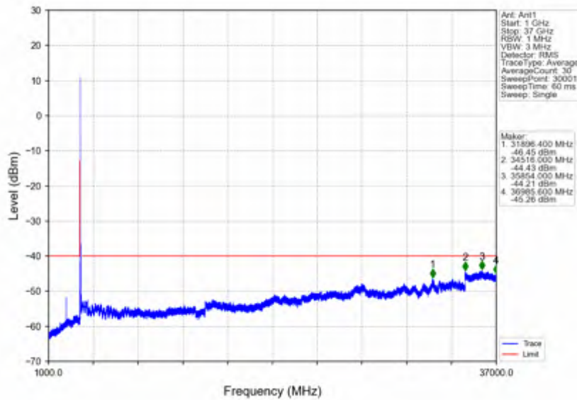
n78d_30kHz_SISO_NTNV_40MHz_DFT-s-OFDM PI/2 BPSK_3624.99MHz_Edge_1RB_Left
