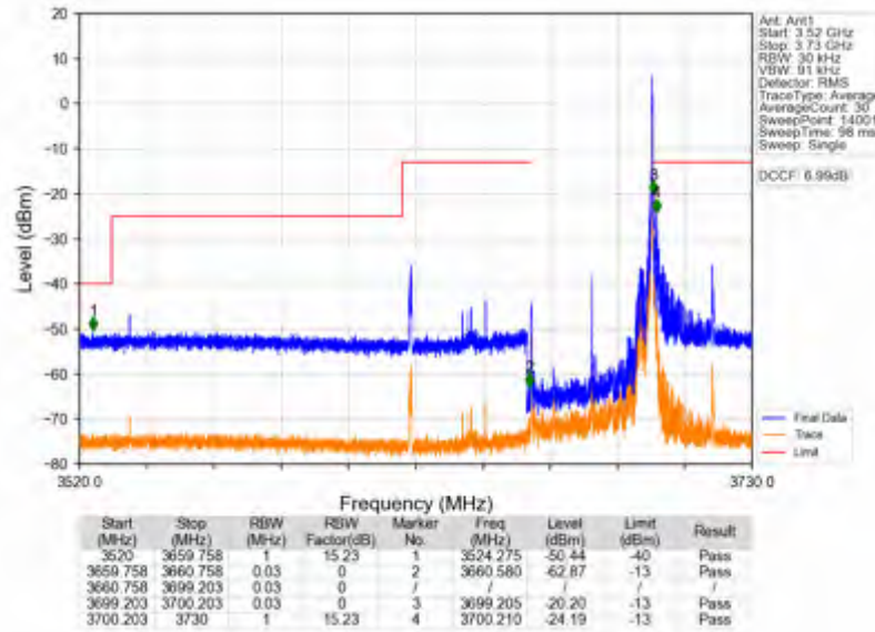
n78d_30kHz_SISO_NTNV_40MHz_DFT-s-OFDM PI/2 BPSK_3679.98MHz_Edge_1RB_Right
