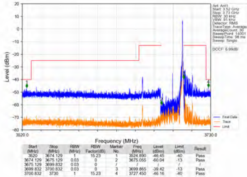
n78d_30kHz_SISO_NTNV_25MHz_CP-OFDM QPSK_3687.48MHz_Inner_1RB_Right
