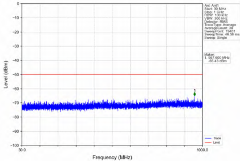
n78d_30kHz_SISO_NTNV_30MHz_CP-OFDM QPSK_3565.02MHz_Outer_Full
