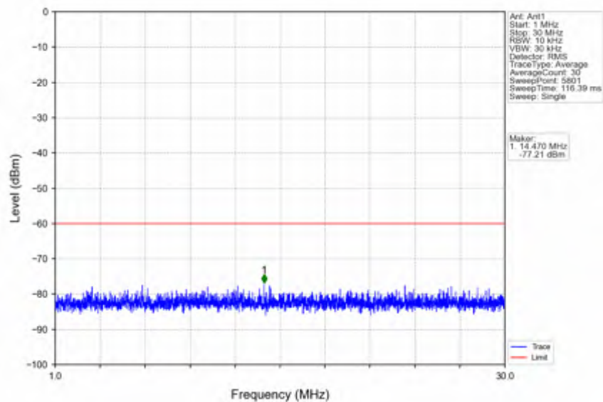
n78d_30kHz_SISO_NTNV_50MHz_CP-OFDM QPSK_3575.01MHz_Outer_Full
