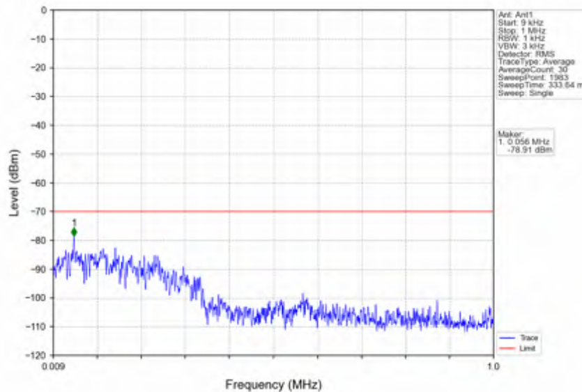
n78d_30kHz_SISO_NTNV_25MHz_CP-OFDM QPSK_3687.48MHz_Inner_1RB_Right
