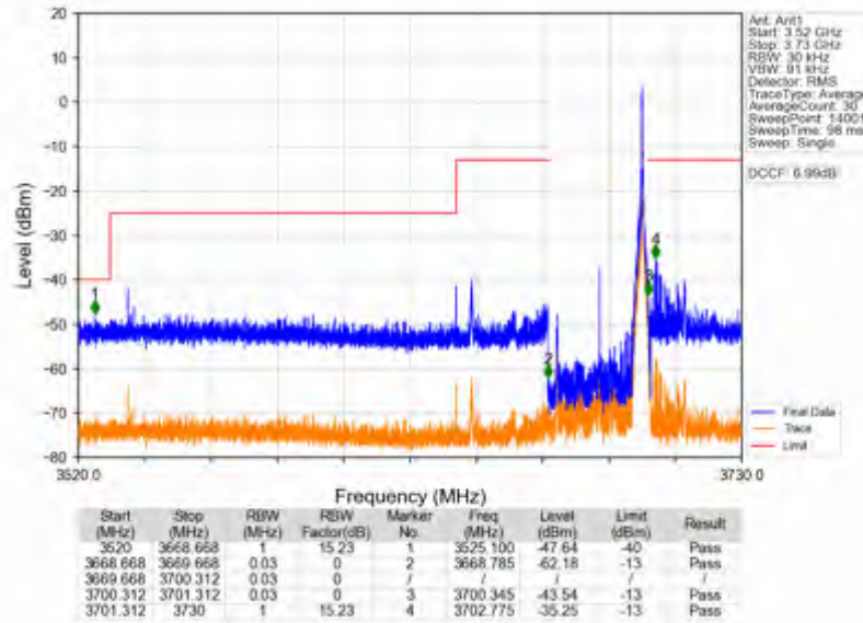
n78d_30kHz_SISO_NTV_30MHz_CP-OFDM QPSK_3684.99MHz_Inner_1RB_Right
