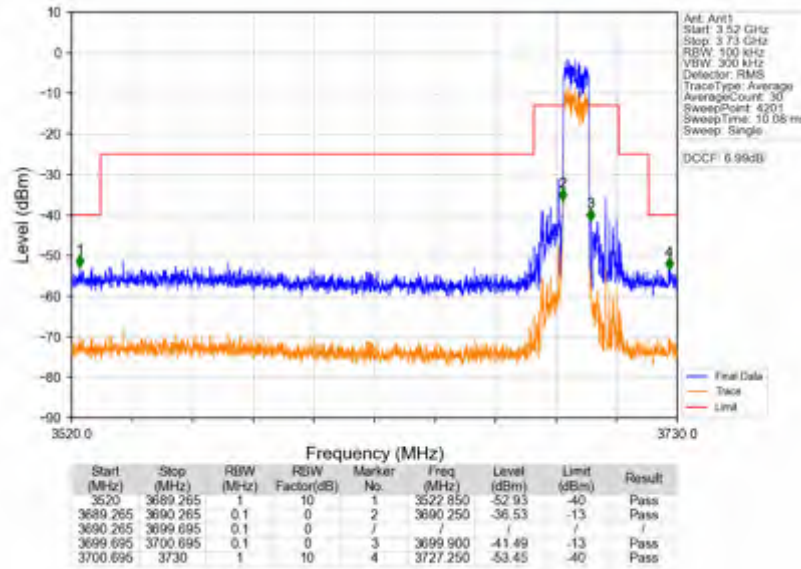
n78d_30kHz_SISO_NTNV_10MHz_DFT-s-OFDM_QPSK_3694.98MHz_Outer_Full
