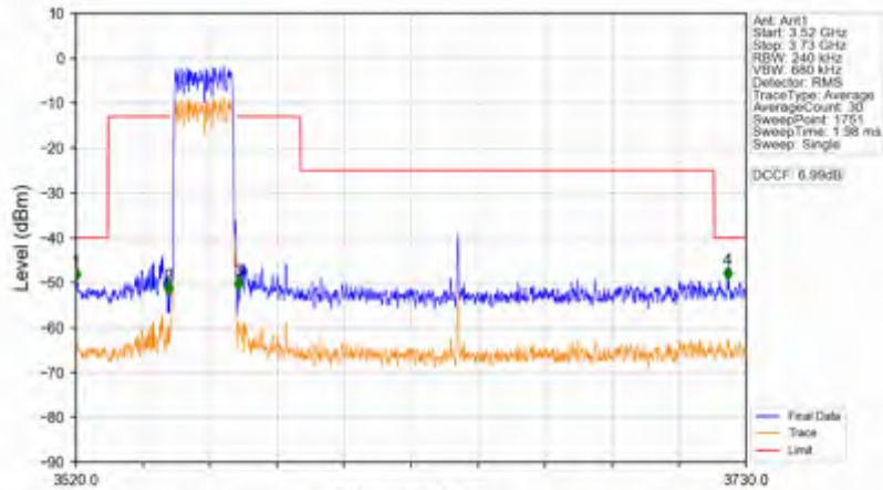
n78d_30kHz_SISO_NTNV_20MHz_CP-OFDM QPSK_3560.01MHz_Outer_Full
