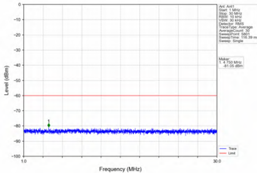
n78d_30kHz_SISO_NTNV_25MHz_DFT-s-OFDM PI/2 BPSK_3562.5MHz_Edge_1RB_Left
