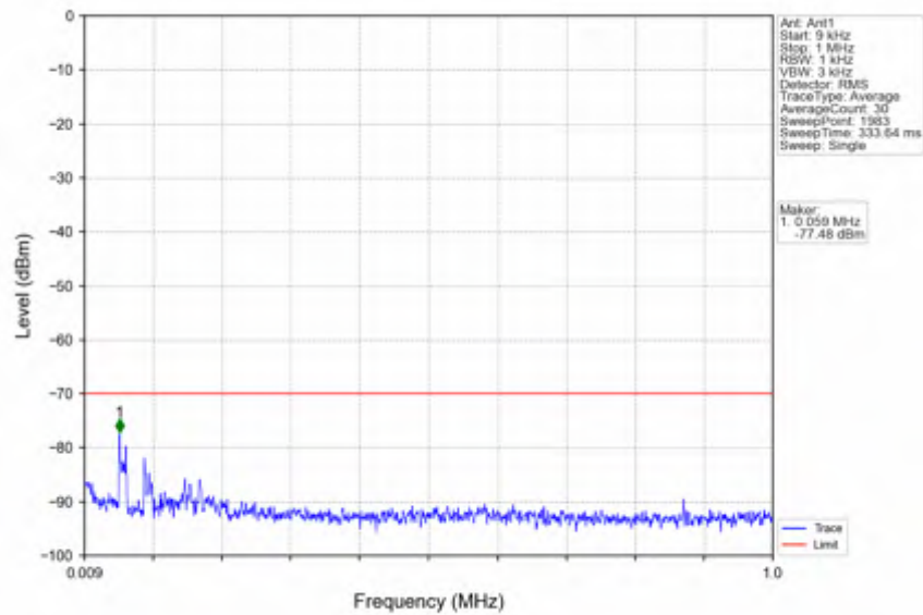
n78d_30kHz_SISO_NTNV_20MHz_DFT-s-OFDM PI/2 BPSK_3624.99MHz_Edge_1RB_Left
