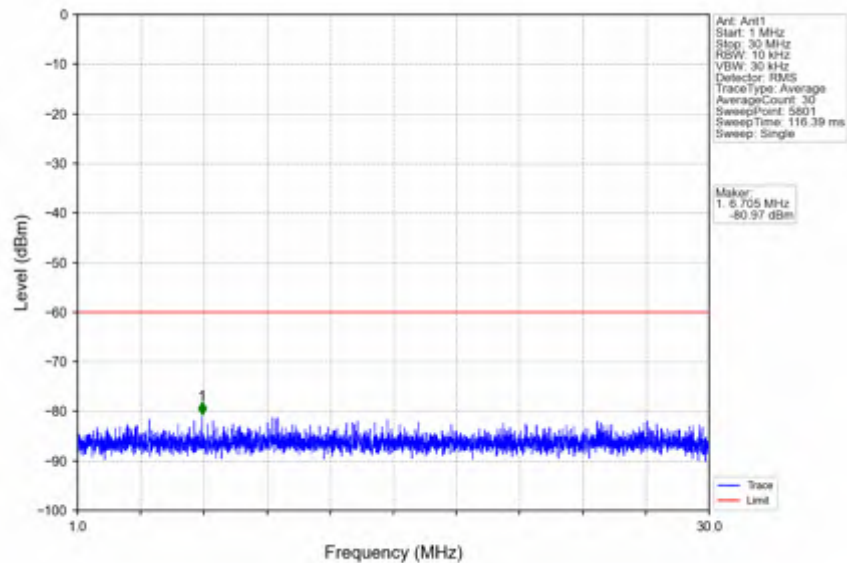
n78d_30kHz_SISO_NTNV_10MHz_CP-OFDM QPSK_3555MHz_Outer_Full
