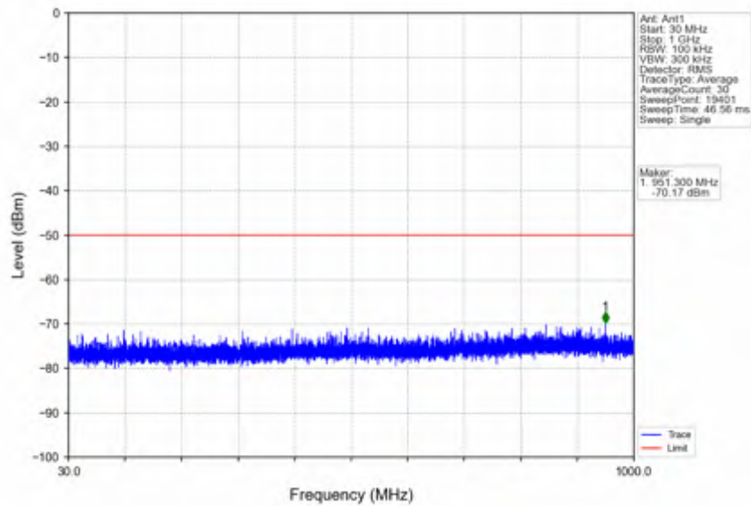
n78d_30kHz_SISO_NTNV_10MHz_DFT-s-OFDM QPSK_3694.98MHz_Inner_1RB_Right
