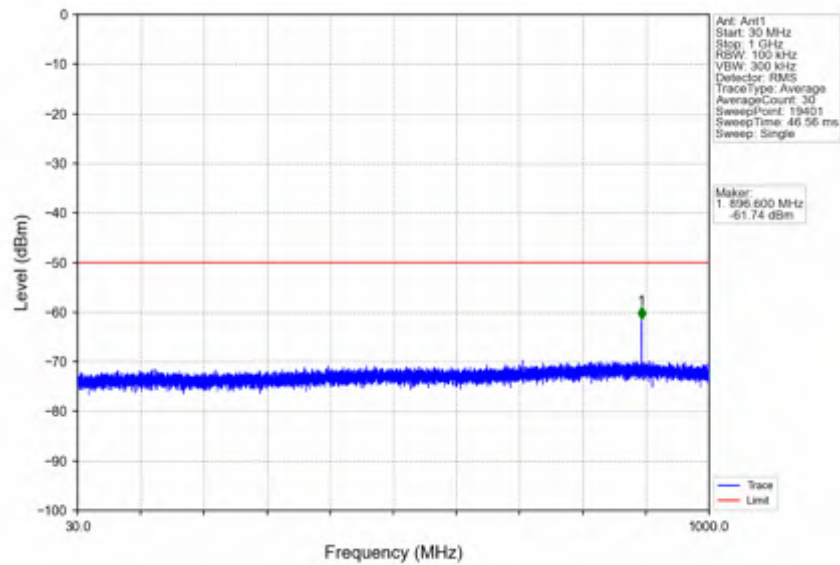
n78d_30kHz_SISO_NTNV_10MHz_DFT-s-OFDM PI/2 BPSK_3555MHz_Outer_Full
