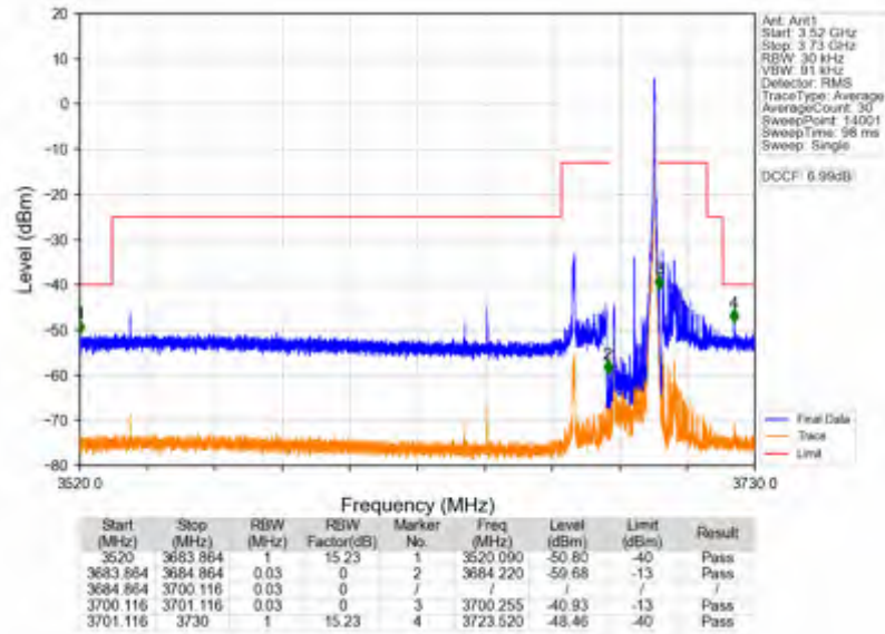
n78d_30kHz_SISO_NTNV_15MHz_DFT-s-OFDM PI/2 BPSK_3692.49MHz_Inner_1RB_Right
