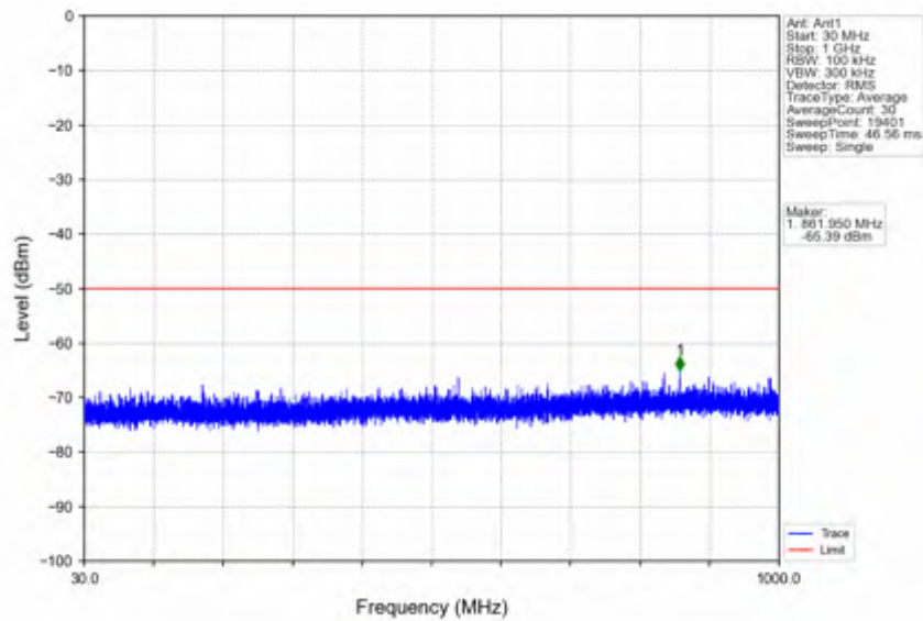
n78d_30kHz_SISO_NTNV_20MHz_DFT-s-OFDM_QPSK_3690MHz_Inner_1RB_Right
