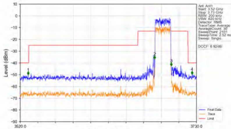
n78d_30kHz_SISO_NTNV_20MHz_CP-OFDM QPSK_3690MHz_Outer_Full
