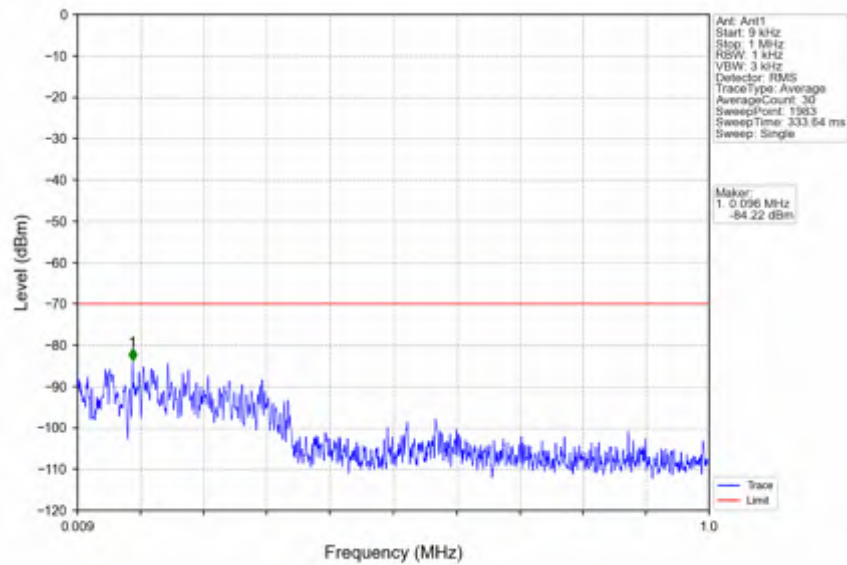
n78d_30kHz_SISO_NTNV_25MHz_DFT-s-OFDM QPSK_3562.5MHz_Edge_1RB_Left
