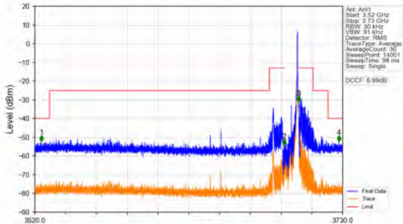
n78d_30kHz_SISO_NTNV_10MHz_DFT-s-OFDM QPSK_3694.98MHz_Edge_1RB_Right
