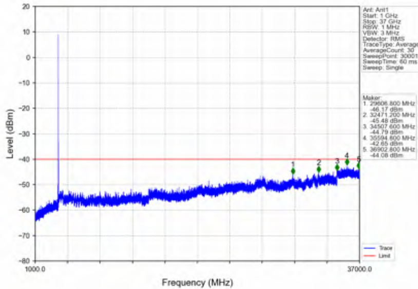
n78d_30kHz_SISO_NTV_20MHz_CP-OFDM_QPSK_3624.99MHz_Edge_1RB_Left
