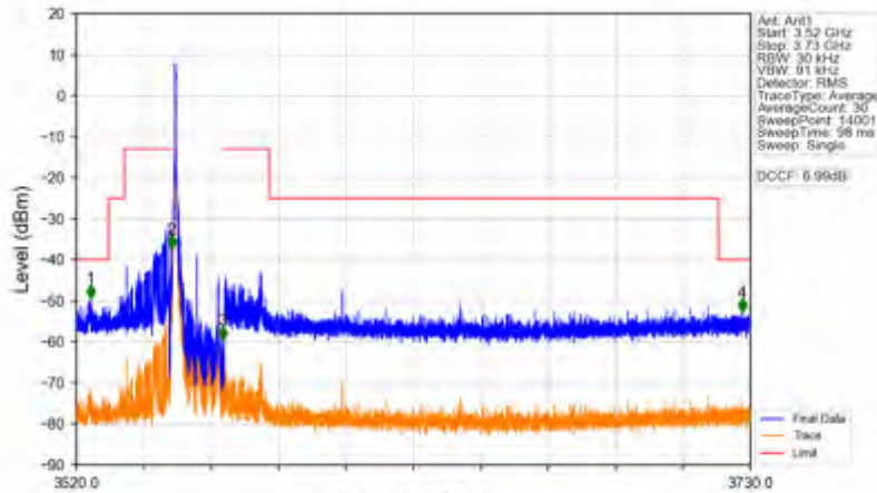
n78d_30kHz_SISO_NTNV_15MHz_DFT-s-OFDM QPSK_3557.52MHz_Edge_1RB_Left
