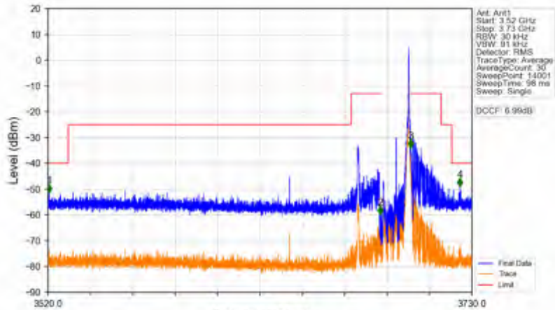
n78d_30kHz_SISO_NTNV_15MHz_DFT-s-OFDM QPSK_3692.49MHz_Inner_1RB_Right
