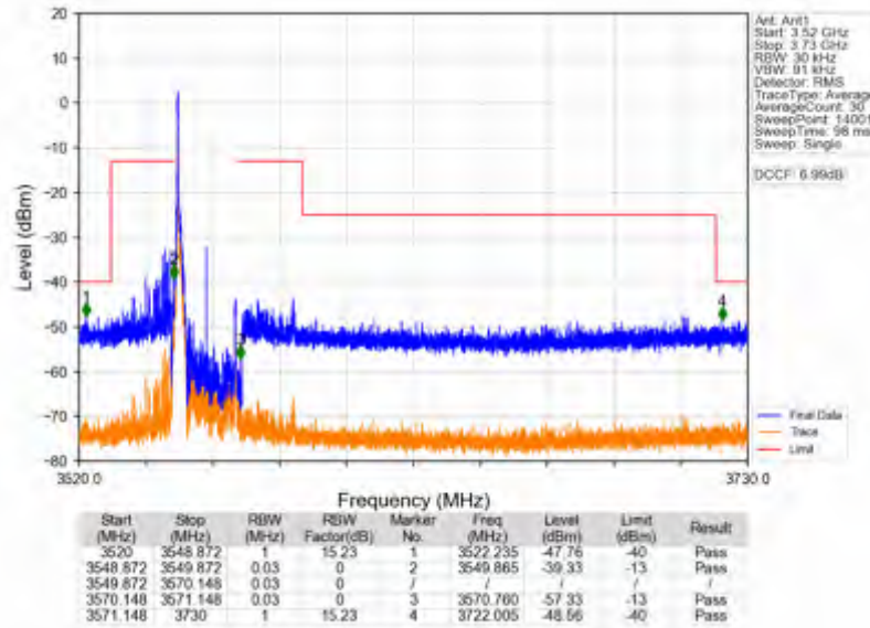
n78d_30kHz_SISO_NTV_20MHz_CP-OFDM_QPSK_3560.01MHz_Edge_1RB_Left
