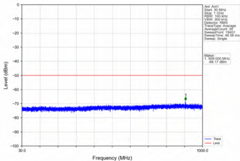
n78d_30kHz_SISO_NTNV_15MHz_DFT-s-OFDM PI/2 BPSK_3692.49MHz_Inner_1RB_Right
