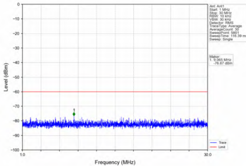
n78d_30kHz_SISO_NTNV_20MHz_CP-OFDM QPSK_3560.01MHz_Inner_1RB_Left
