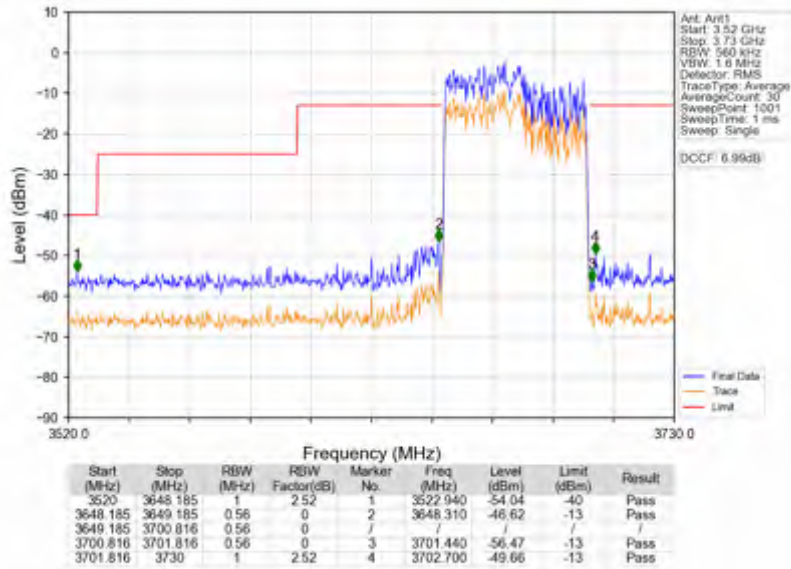
n78d_15kHz_SISO_NTNV_50MHz_CP-OFDM QPSK_3675MHz_Outer_Full
