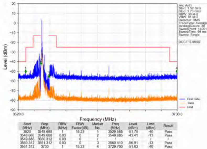
n78d_30kHz_SISO_NTNV_10MHz_DFT-s-OFDM QPSK_3555MHz_Inner_1RB_Left
