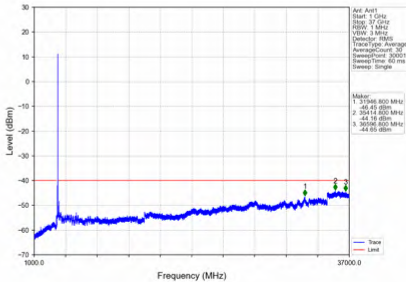
n78d_30kHz_SISO_NTNV_25MHz_DFT-s-OFDM PI/2 BPSK_3687.48MHz_Outer_Full
