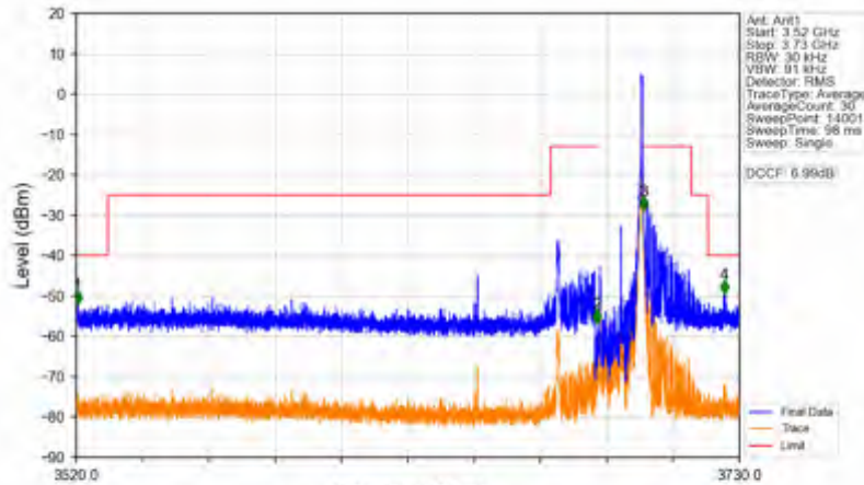
n78d_30kHz_SISO_NTNV_15MHz_DFT-s-OFDM QPSK_3692.49MHz_Edge_1RB_Right
