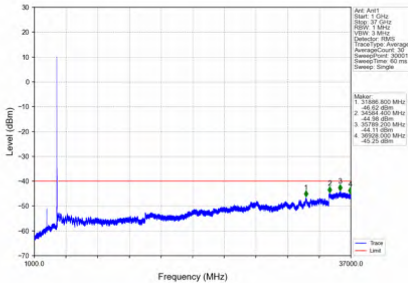
n78d_30kHz_SISO_NTNV_20MHz_DFT-s-OFDM PI/2 BPSK_3624.99MHz_Edge_1RB_Left
