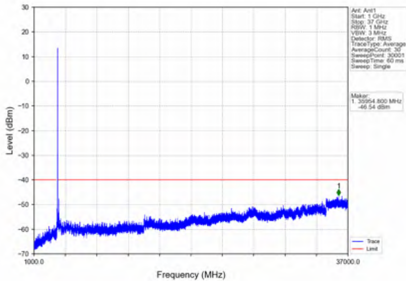
n78d_30kHz_SISO_NTNV_15MHz_CP-OFDM QPSK_3692.49MHz_Outer_Full
