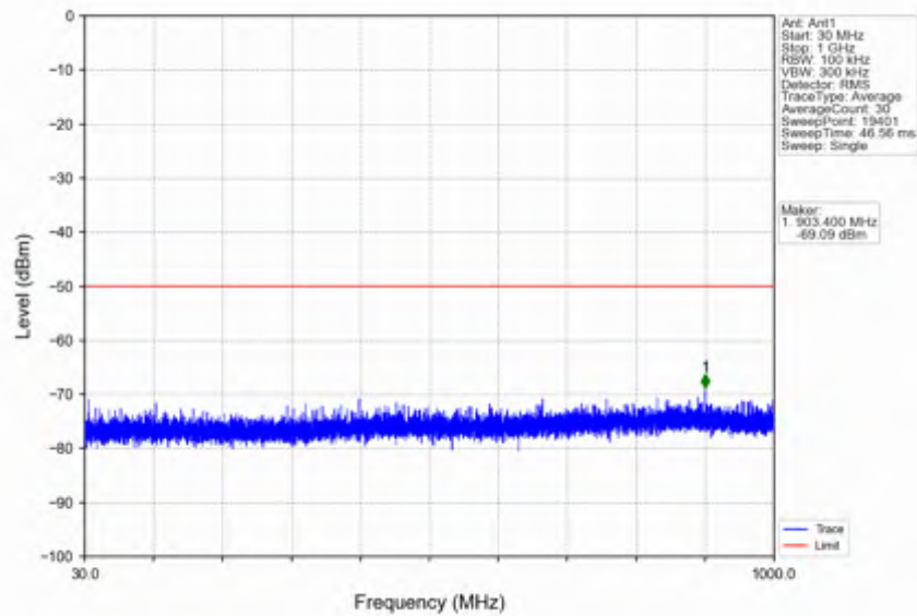
n78d_30kHz_SISO_NTNV_15MHz_DFT-s-OFDM_QPSK_3557.52MHz_Inner_1RB_Left
