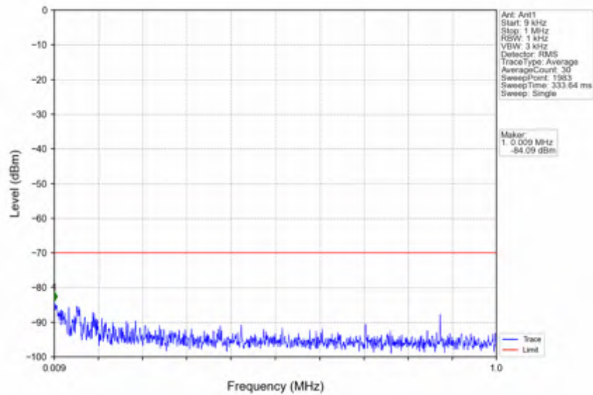
n78d_30kHz_SISO_NTNV_15MHz_DFT-s-OFDM QPSK_3557.52MHz_Inner_1RB_Left
