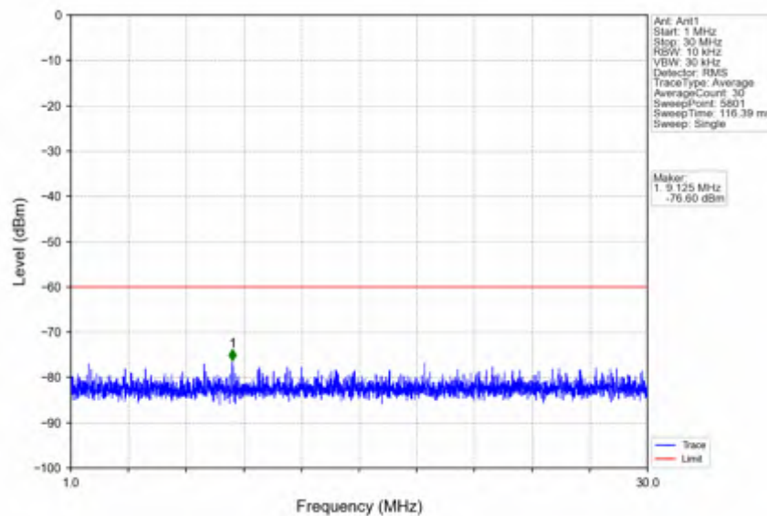
n78d_30kHz_SISO_NTNV_20MHz_DFT-s-OFDM_QPSK_3560.01MHz_Inner_1RB_Left
