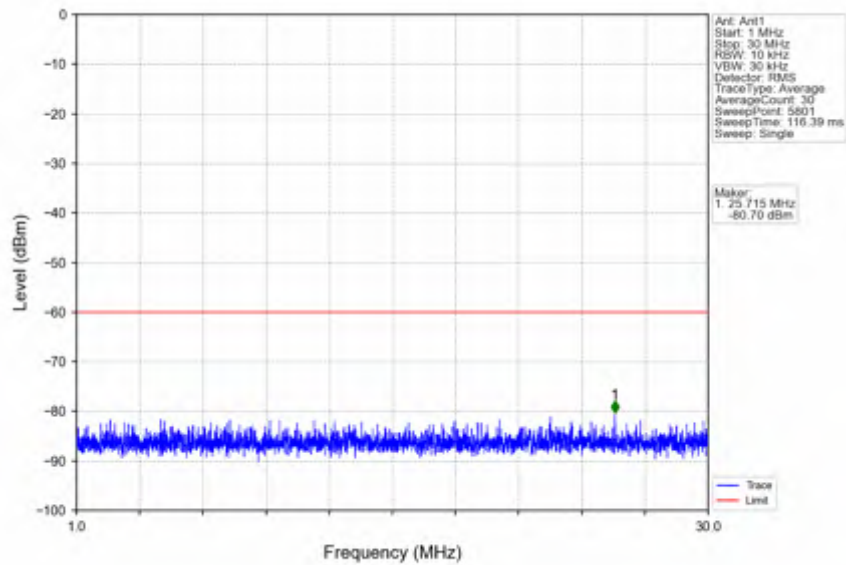
n78d_30kHz_SISO_NTNV_15MHz_CP-OFDM_QPSK_3557.52MHz_Inner_1RB_Left
