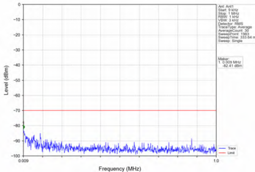
n78d_30kHz_SISO_NTV_10MHz_CP-OFDM QPSK_3694.98MHz_Inner_1RB_Right
