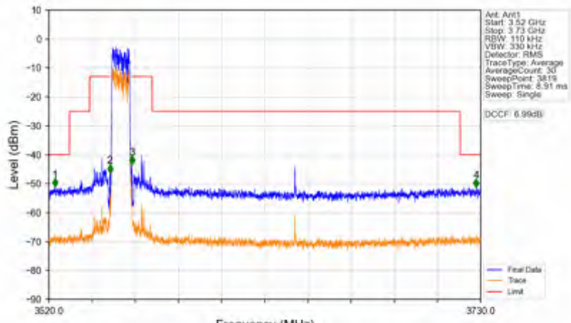
n78d_30kHz_SISO_NTNV_10MHz_DFT-s-OFDM PI/2 BPSK_3555MHz_Outer_Full
