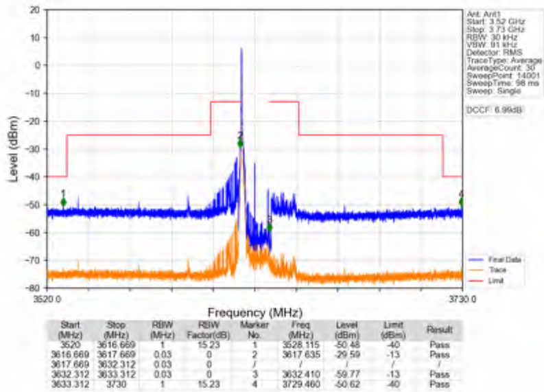
n78d_30kHz_SISO_NTNV_15MHz_DFT-s-OFDM PI/2 BPSK_3624.99MHz_Edge_1RB_Left
