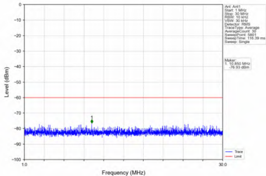
n78d_30kHz_SISO_NTNV_20MHz_CP-OFDM QPSK_3560.01MHz_Outer_Full
