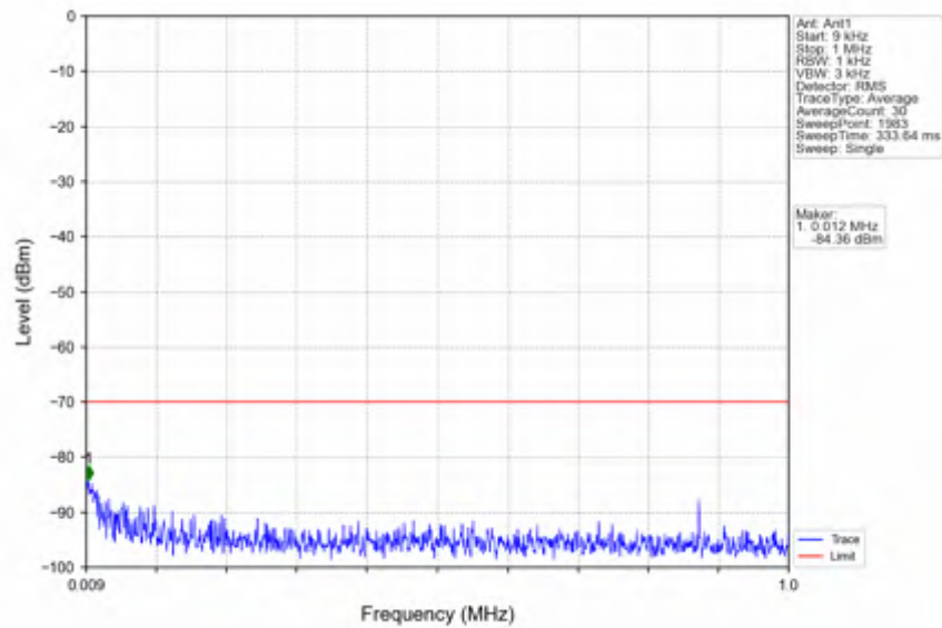
n78d_15kHz_SISO_NTNV_50MHz_CP-OFDM QPSK_3675MHz_Outer_Full
