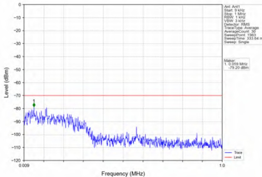
n78d_30kHz_SISO_NTV_20MHz_CP-OFDM_QPSK_3560.01MHz_Inner_1RB_Left
