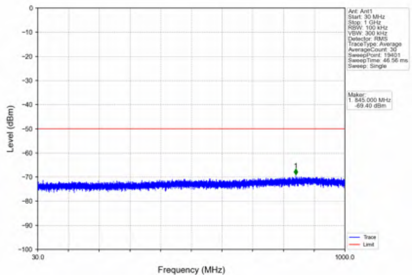
n78d_30kHz_SISO_NTNV_20MHz_DFT-s-OFDM_PI/2_BPSK_3690MHz_Inner_1RB_Right
