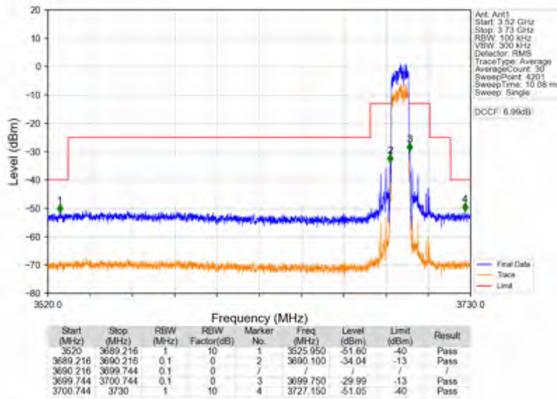
n78d_30kHz_SISO_NTNV_10MHz_DFT-s-OFDM PI/2 BPSK_3694.98MHz_Outer_Full
