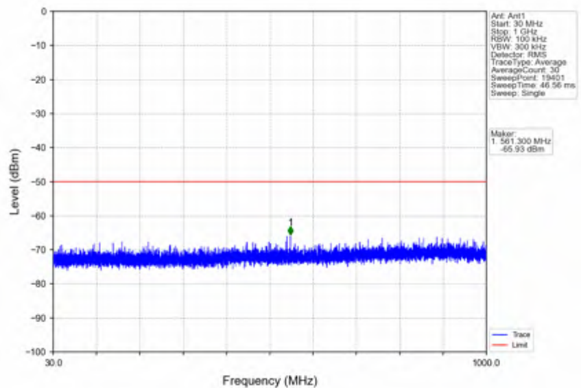
n78d_30kHz_SISO_NTNV_25MHz_DFT-s-OFDM_QPSK_3562.5MHz_Outer_Full
