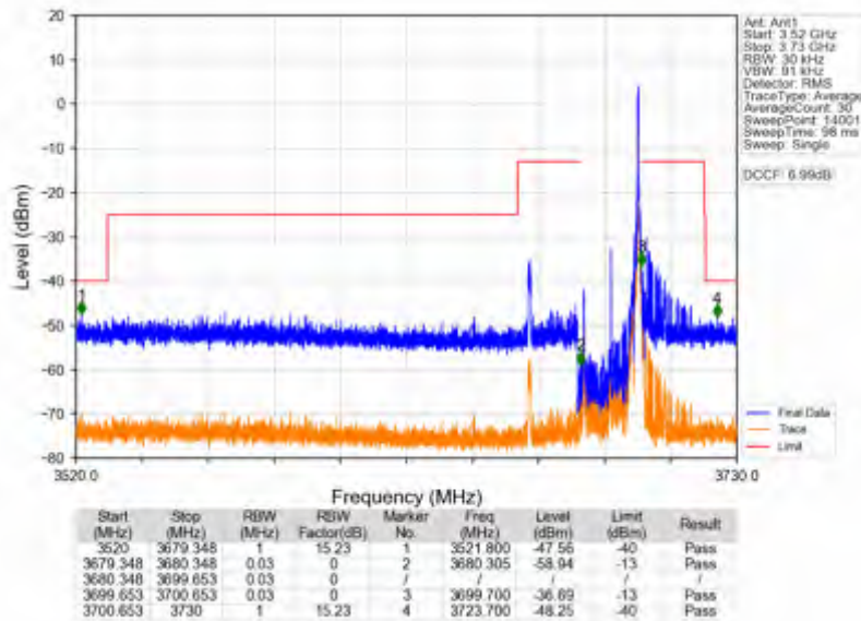
n78d_30kHz_SISO_NTNV_20MHz_DFT-s-OFDM_QPSK_3690MHz_Inner_1RB_Right
