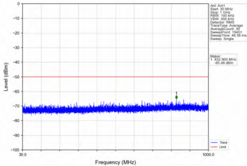
n78d_30kHz_SISO_NTVV_20MHz_CP-OFDM QPSK_3624.99MHz_Edge_1RB_Left
