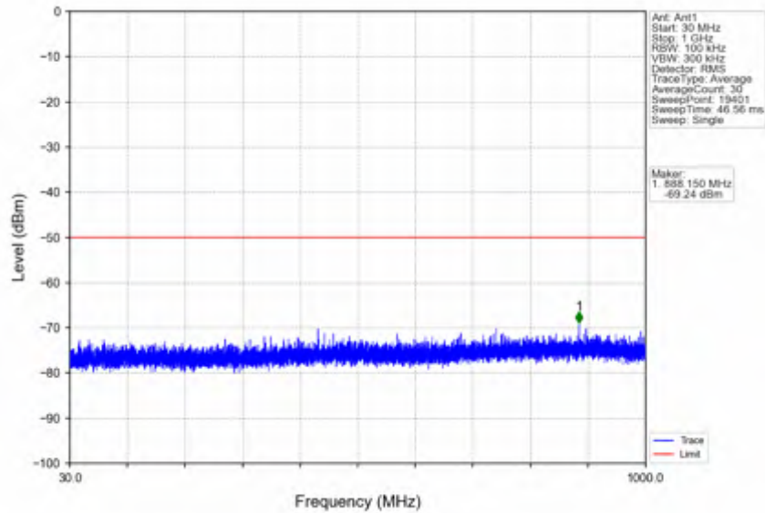
n78d_30kHz_SISO_NTVV_10MHz_DFT-s-OFDM QPSK_3555MHz_Edge_1RB_Left
