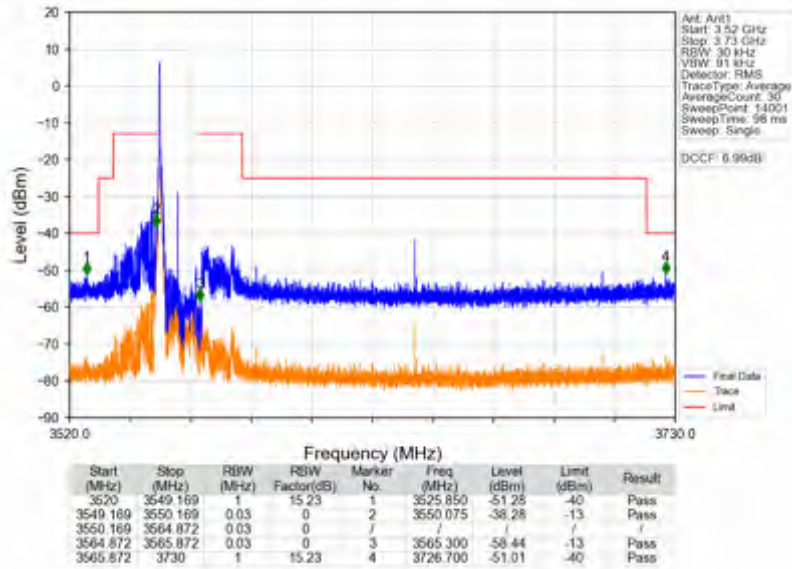
n78d_30kHz_SISO_NTV_15MHz_CP-OFDM_QPSK_3557.52MHz_Inner_1RB_Left
