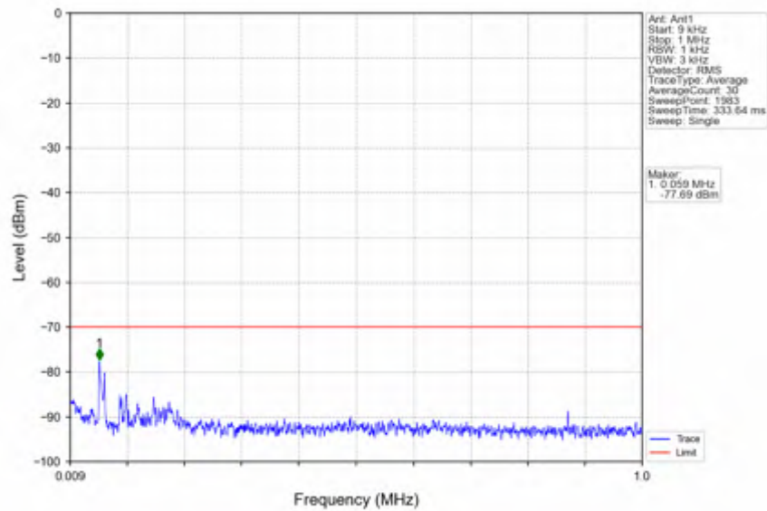
n78d_30kHz_SISO_NTNV_25MHz_DFT-s-OFDM PI/2 BPSK_3562.5MHz_Outer_Full
