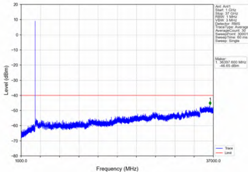
n78d_30kHz_SISO_NTVV_10MHz_CP-OFDM QPSK_3624.99MHz_Edge_1RB_Left
