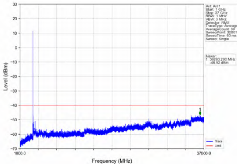
n78d_30kHz_SISO_NTVV_10MHz_DFT-s-OFDM QPSK_3555MHz_Edge_1RB_Left
