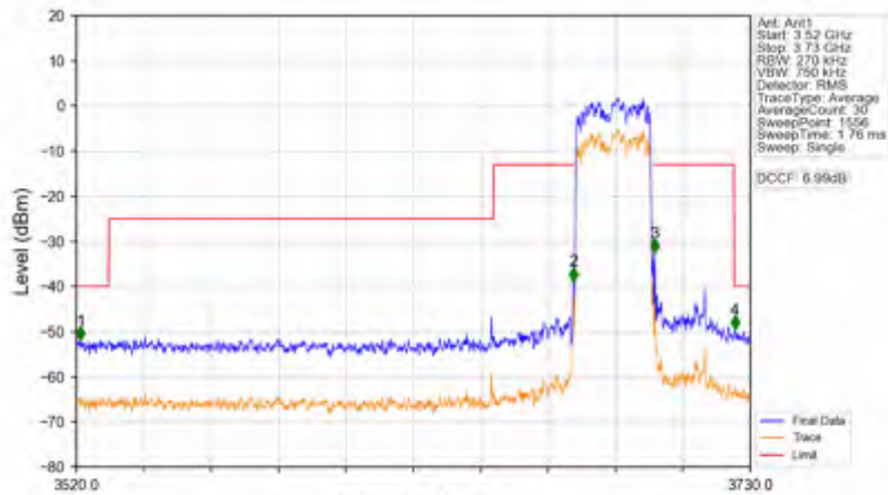
n78d_30kHz_SISO_NTNV_25MHz_DFT-s-OFDM PI/2 BPSK_3687.48MHz_Outer_Full
