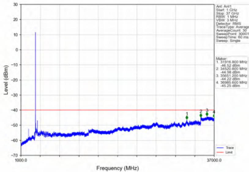
n78d_30kHz_SISO_NTNV_10MHz_DFT-s-OFDM PI/2 BPSK_3694.98MHz_Outer_Full
