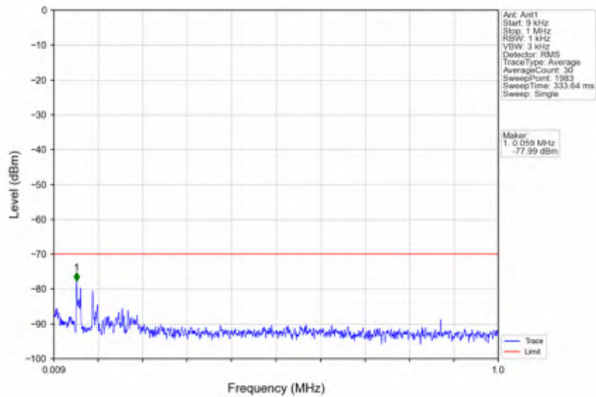
n78d_30kHz_SISO_NTNV_15MHz_DFT-s-OFDM PI/2 BPSK_3624.99MHz_Edge_1RB_Left
