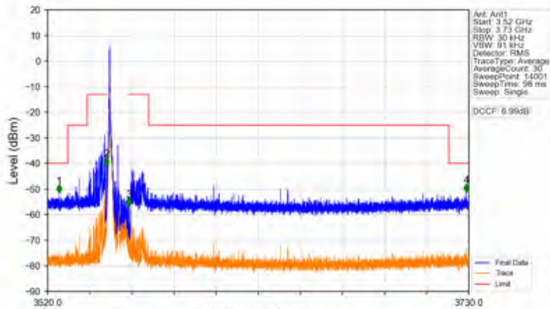
n78d_30kHz_SISO_NTV_10MHz_DFT-s-OFDM QPSK_3555MHz_Edge_1RB_Left
