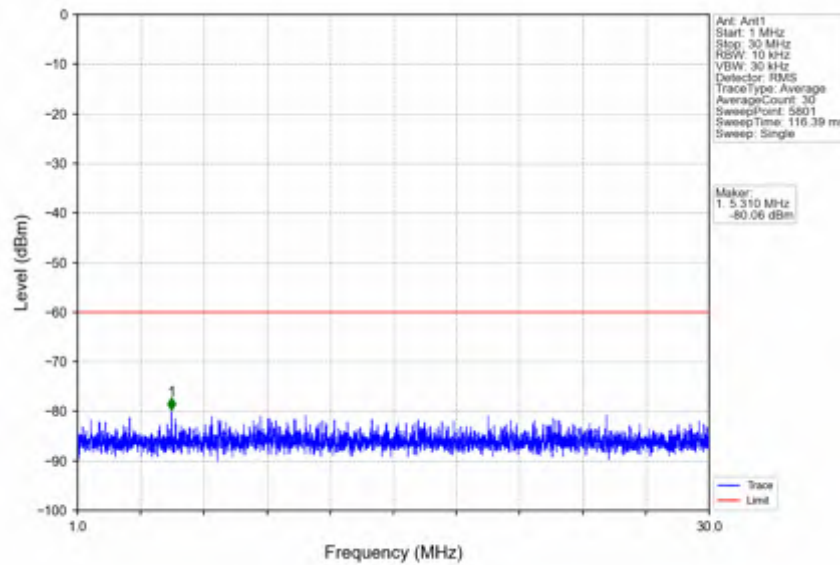
n78d_15kHz_SISO_NTNV_50MHz_CP-OFDM QPSK_3675MHz_Inner_1RB_Right
