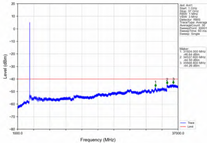
n78d_30kHz_SISO_NTNV_15MHz_DFT-s-OFDM PI/2 BPSK_3692.49MHz_Outer_Full
