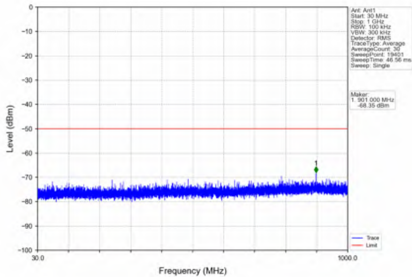
n78d_30kHz_SISO_NTNV_15MHz_DFT-s-OFDM QPSK_3692.49MHz_Inner_1RB_Right
