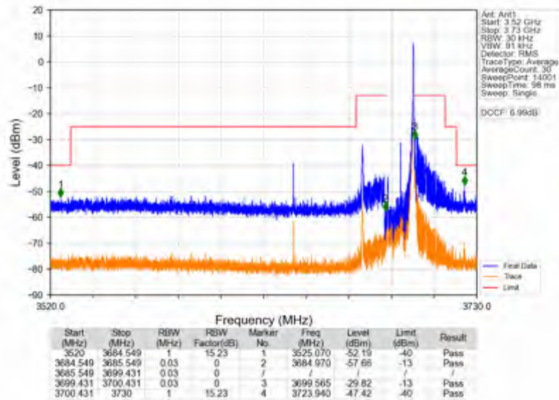
n78d_30kHz_SISO_NTNV_15MHz_CP-OFDM QPSK_3692.49MHz_Inner_1RB_Right
