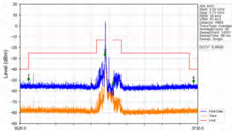
n78d_30kHz_SISO_NTV_10MHz_CP-OFDM QPSK_3624.99MHz_Edge_1RB_Left
