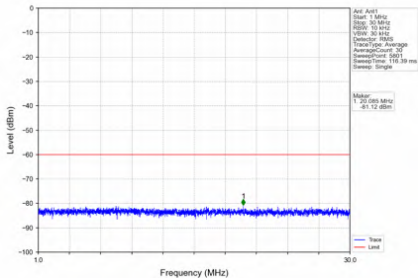
n78d_30kHz_SISO_NTNV_15MHz_DFT-s-OFDM PI/2 BPSK_3692.49MHz_Outer_Full
