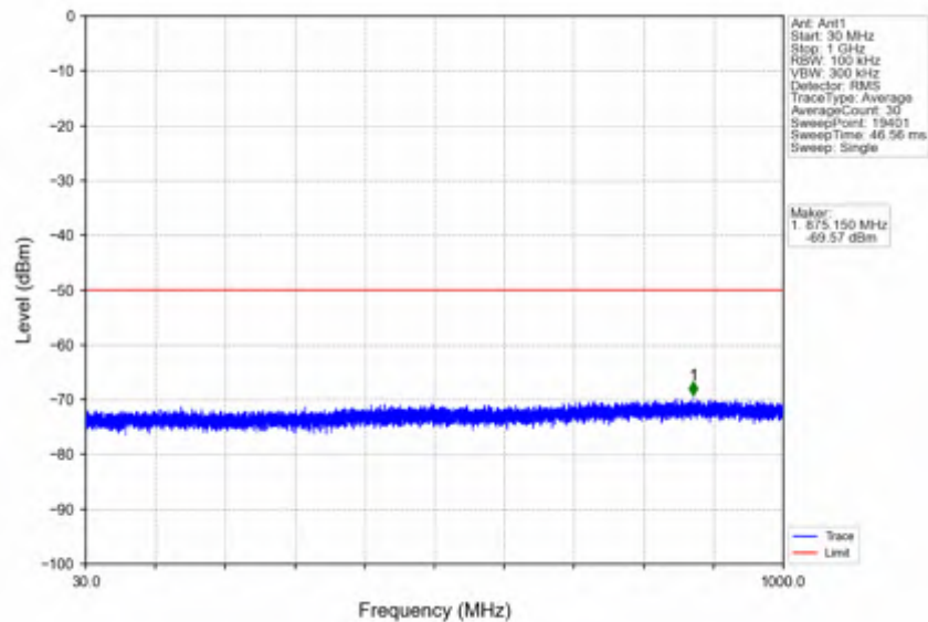
n78d_30kHz_SISO_NTNV_10MHz_DFT-s-OFDM PI/2 BPSK_3694.98MHz_Inner_1RB_Right
