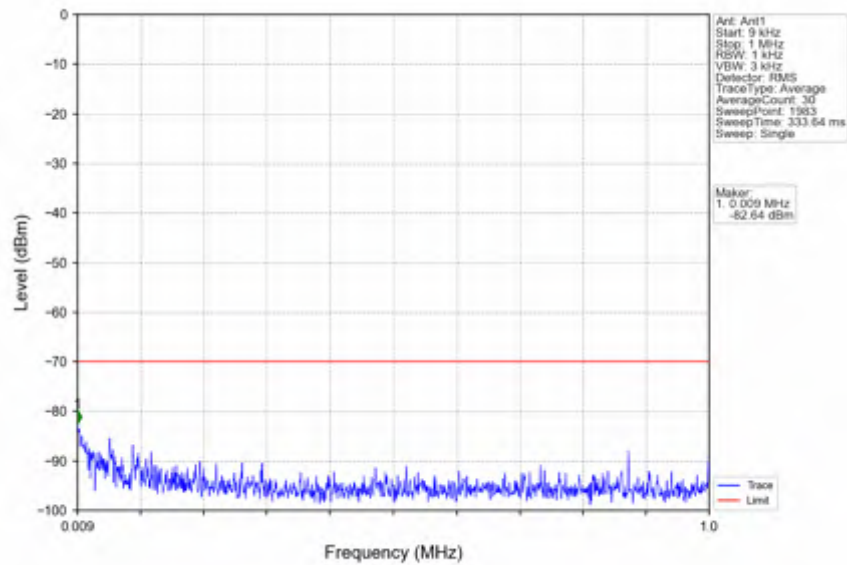
n78d_30kHz_SISO_NTNV_15MHz_DFT-s-OFDM_QPSK_3557.52MHz_Edge_1RB_Left
