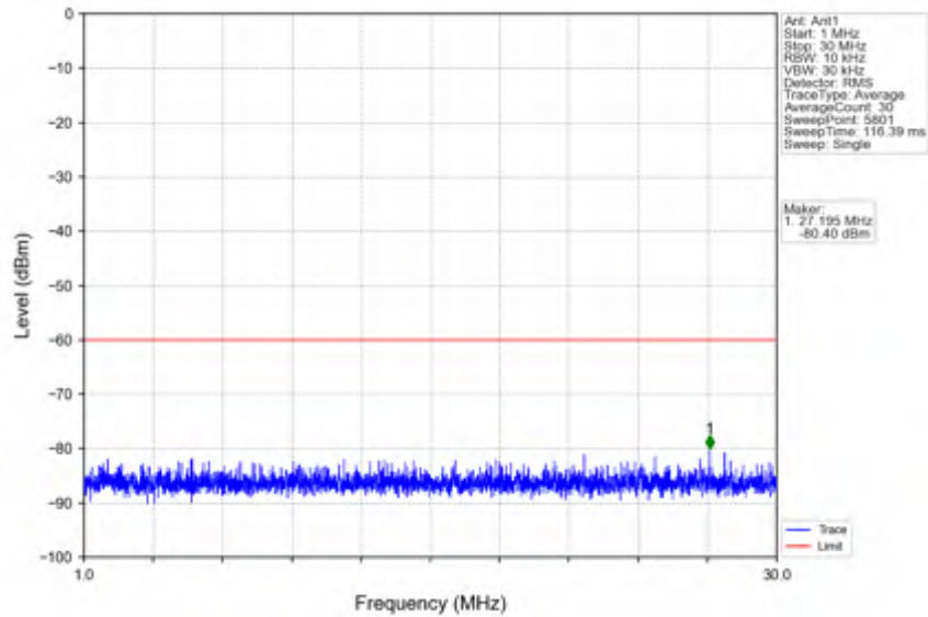
n78d_30kHz_SISO_NTNV_15MHz_DFT-s-OFDM_QPSK_3557.52MHz_Outer_Full
