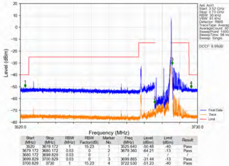
n78d_30kHz_SISO_NTV_20MHz_DFT-s-OFDM PI/2 BPSK_3690MHz_Edge_1RB_Right
