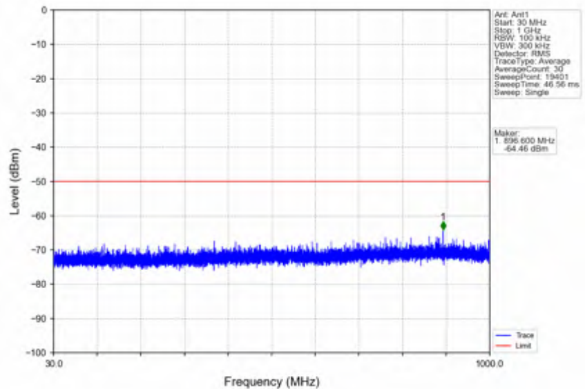
n78d_30kHz_SISO_NTNV_20MHz_CP-OFDM QPSK_3690MHz_Edge_1RB_Right
