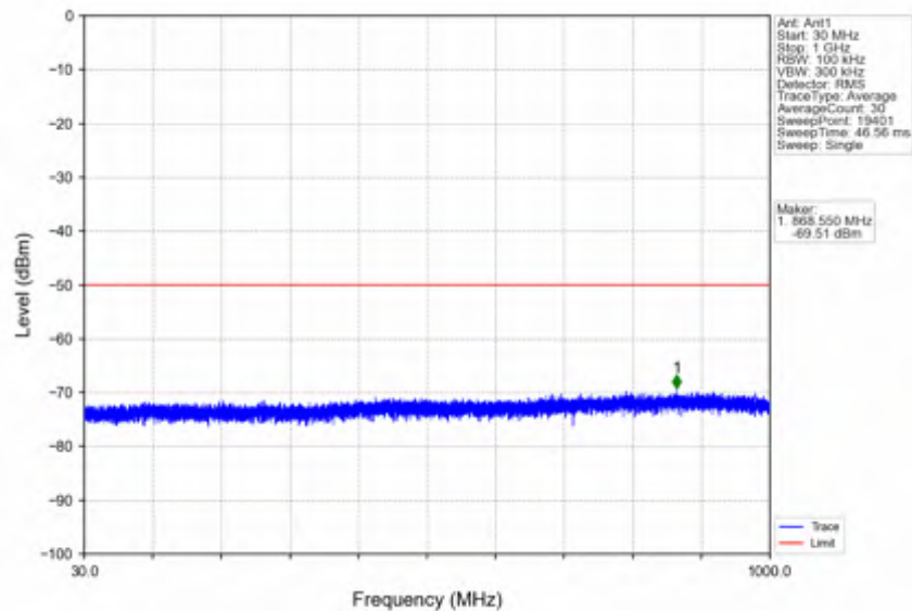
n78d_30kHz_SISO_NTNV_25MHz_DFT-s-OFDM PI/2 BPSK_3687.48MHz_Inner_1RB_Right
