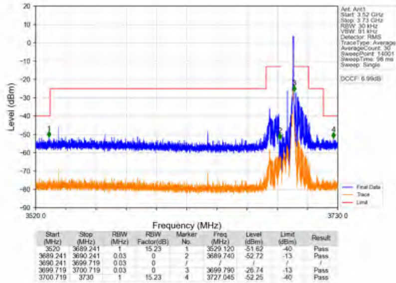
n78d_30kHz_SISO_NTV_10MHz_CP-OFDM QPSK_3694.98MHz_Edge_1RB_Right
