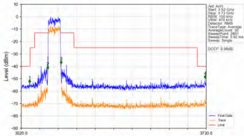
n78d_30kHz_SISO_NTNV_15MHz_CP-OFDM QPSK_3557.52MHz_Outer_Full
