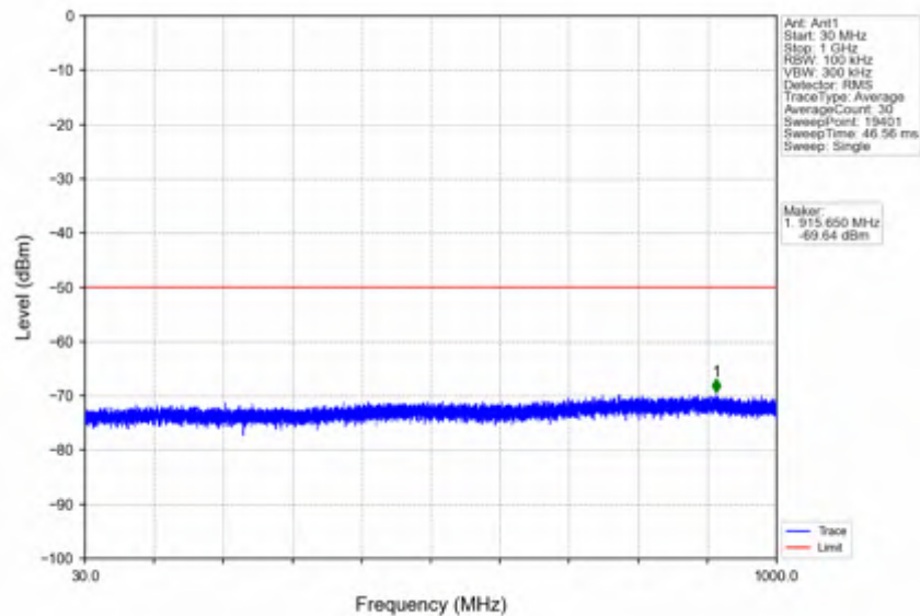
n78d_30kHz_SISO_NTNV_25MHz_DFT-s-OFDM PI/2 BPSK_3687.48MHz_Edge_1RB_Right
