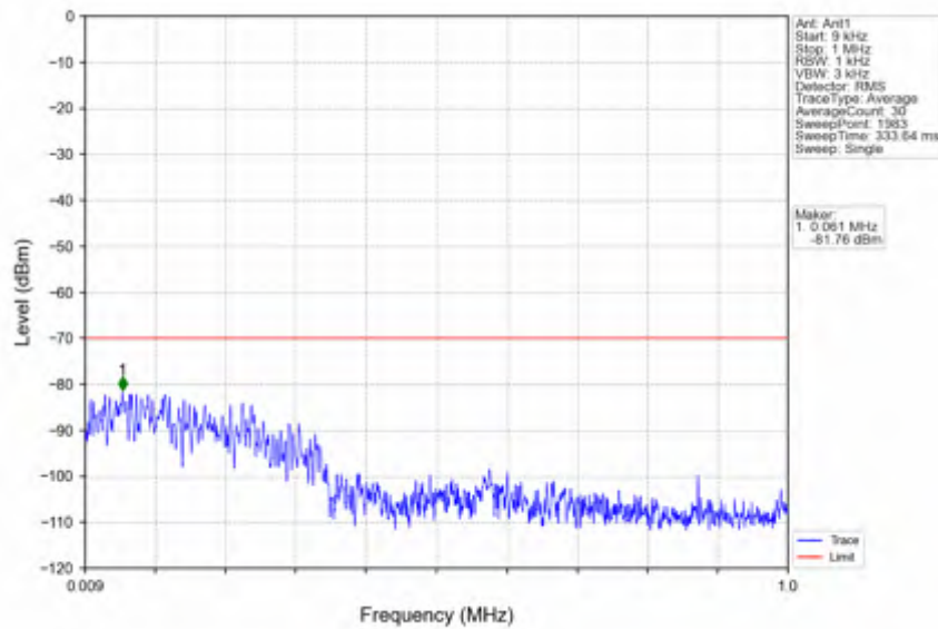
n78d_30kHz_SISO_NTVV_20MHz_CP-OFDM QPSK_3624.99MHz_Edge_1RB_Left
