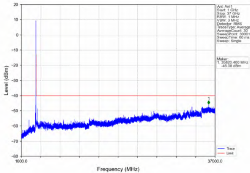
n78d_15kHz_SISO_NTNV_50MHz_CP-OFDM QPSK_3675MHz_Inner_1RB_Right
