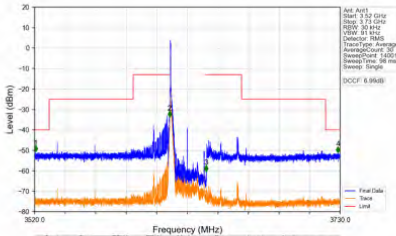
n78d_30kHz_SISO_NTNV_25MHz_DFT-s-OFDM PI/2 BPSK_3624.99MHz_Edge_1RB_Left
