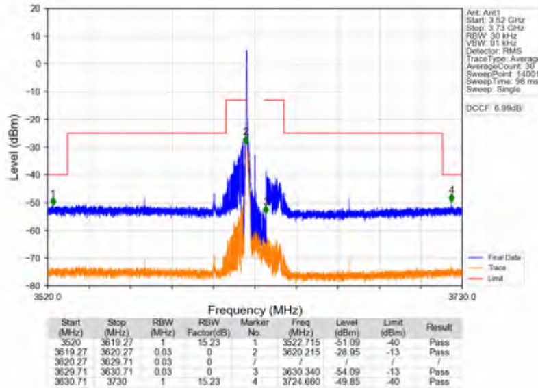
n78d_30kHz_SISO_NTNV_10MHz_DFT-s-OFDM QPSK_3624.99MHz_Edge_1RB_Left
