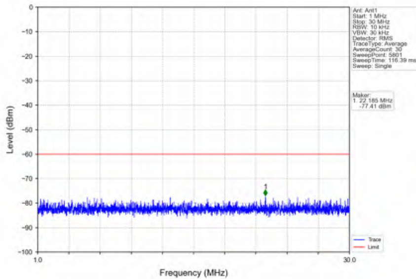
n78d_30kHz_SISO_NTNV_20MHz_DFT-s-OFDM_QPSK_3560.01MHz_Outer_Full
