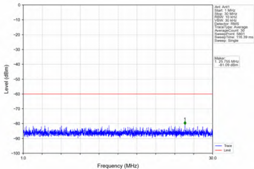
n78d_30kHz_SISO_NTNV_10MHz_CP-OFDM QPSK_3694.98MHz_Outer_Full
