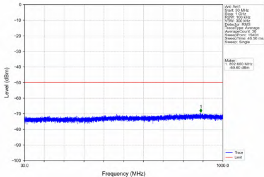
n78d_30kHz_SISO_NTNV_15MHz_DFT-s-OFDM PI/2 BPSK_3692.49MHz_Edge_1RB_Right
