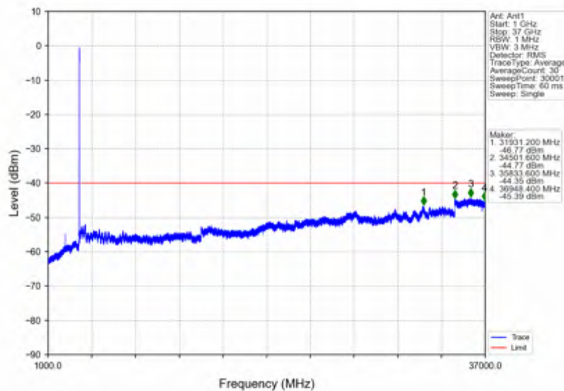
n78d_30kHz_SISO_NTNV_25MHz_DFT-s-OFDM PI/2 BPSK_3562.5MHz_Outer_Full
