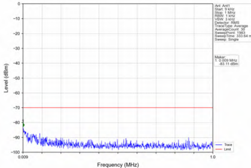
n78d_30kHz_SISO_NTV_15MHz_CP-OFDM_QPSK_3557.52MHz_Inner_1RB_Left
