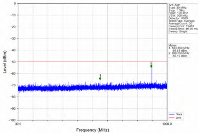
n78d_30kHz_SISO_NTNV_20MHz_DFT-s-OFDM_QPSK_3690MHz_Edge_1RB_Right
