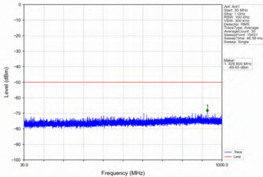
n78d_30kHz_SISO_NTNV_10MHz_DFT-s-OFDM QPSK_3555MHz_Inner_1RB_Left
