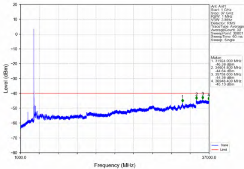
n78d_30kHz_SISO_NTNV_15MHz_DFT-s-OFDM PI/2 BPSK_3557.52MHz_Outer_Full
