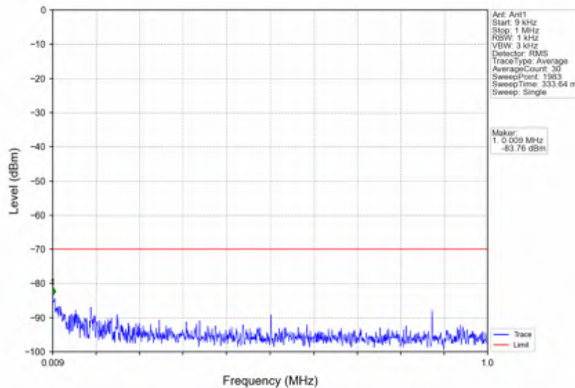
n78d_30kHz_SISO_NTNV_10MHz_DFT-s-OFDM_QPSK_3694.98MHz_Outer_Full
