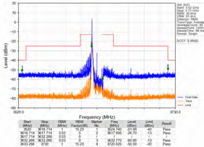
n78d_30kHz_SISO_NTNV_15MHz_DFT-s-OFDM_QPSK_3624.99MHz_Edge_1RB_Left
