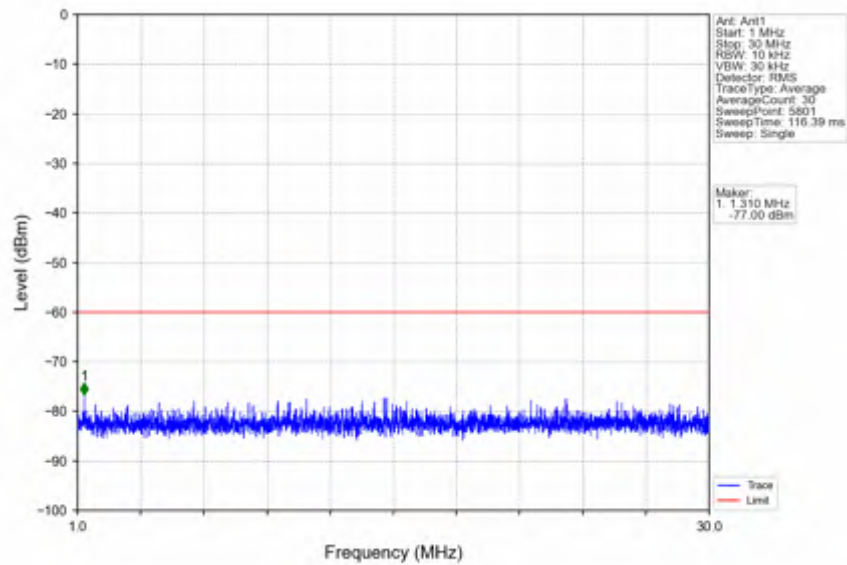
n78d_30kHz_SISO_NTNV_20MHz_DFT-s-OFDM_QPSK_3690MHz_Outer_Full
