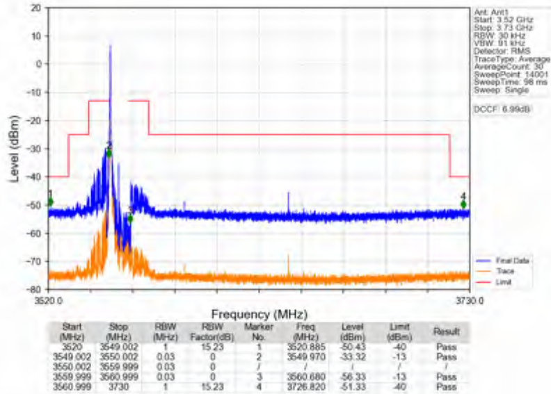
n78d_30kHz_SISO_NTNV_10MHz_DFT-s-OFDM PI/2 BPSK_3555MHz_Edge_1RB_Left
