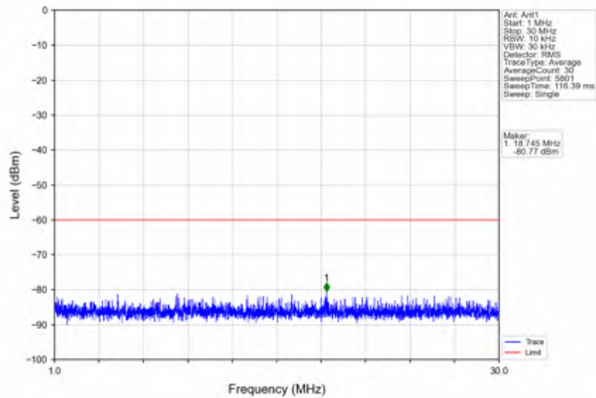
n78d_30kHz_SISO_NTNV_15MHz_DFT-s-OFDM QPSK_3624.99MHz_Edge_1RB_Left
