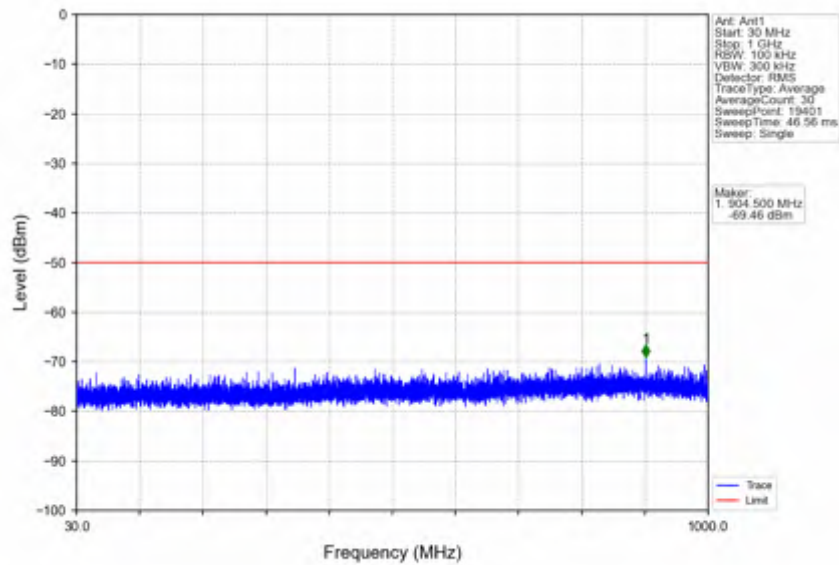
n78d_30kHz_SISO_NTV_15MHz_CP-OFDM QPSK_3624.99MHz_Edge_1RB_Left
