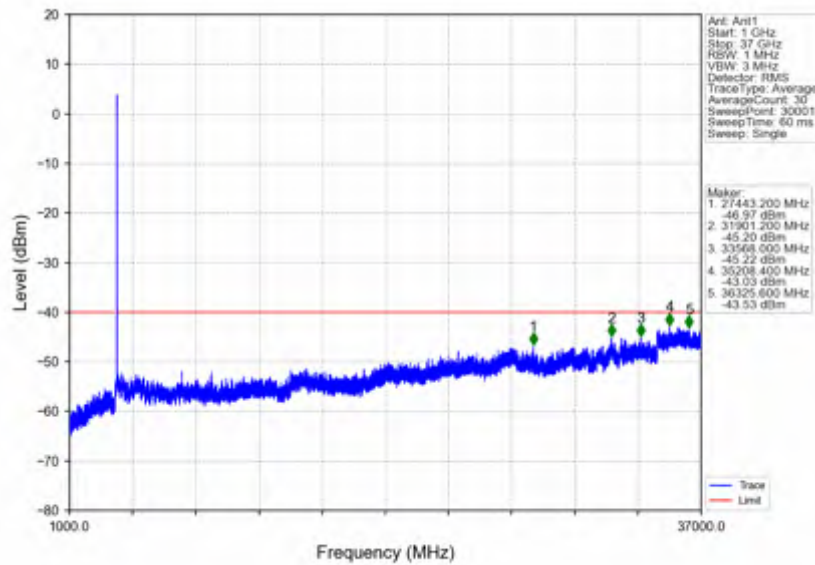
n78d_30kHz_SISO_NTNV_20MHz_DFT-s-OFDM_QPSK_3690MHz_Inner_1RB_Right
