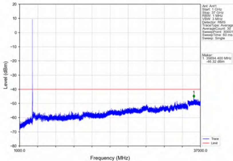
n78d_30kHz_SISO_NTNV_15MHz_DFT-s-OFDM QPSK_3557.52MHz_Edge_1RB_Left
