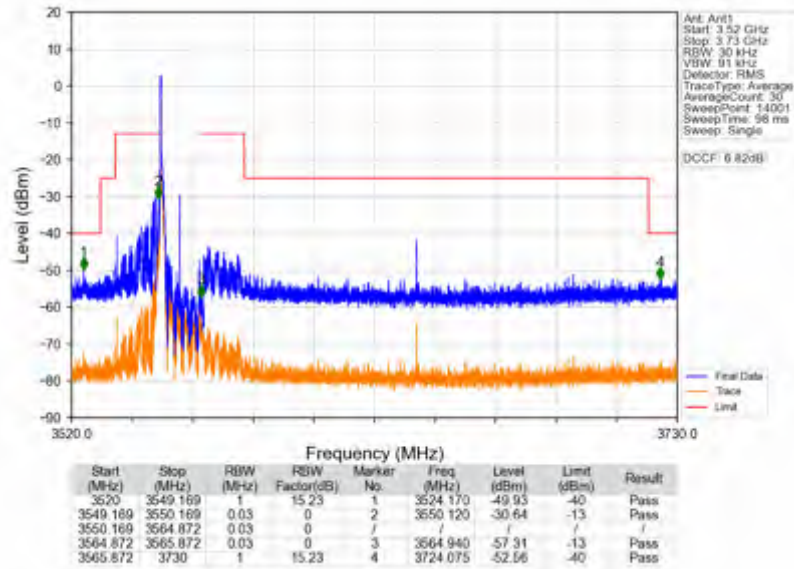
n78d_30kHz_SISO_NTV_15MHz_CP-OFDM QPSK_3557.52MHz_Edge_1RB_Left
