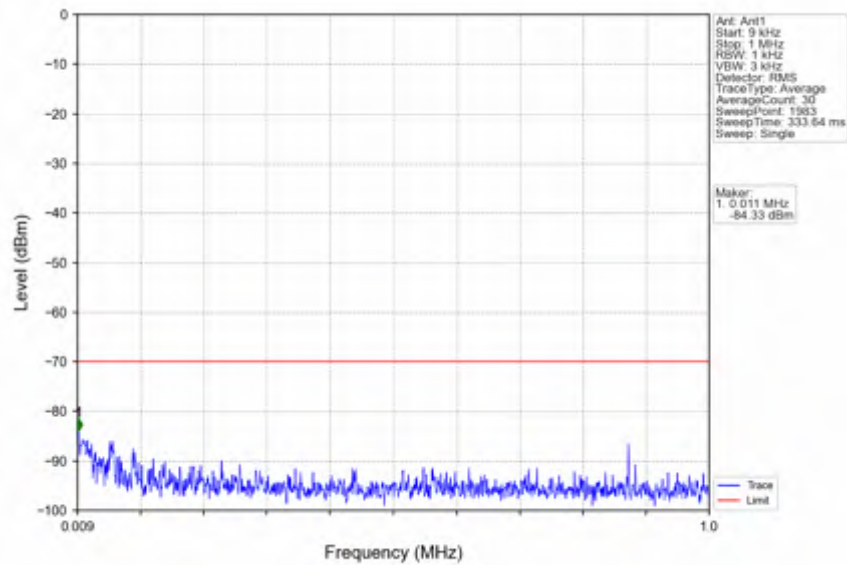
n78d_30kHz_SISO_NTNV_15MHz_CP-OFDM QPSK_3557.52MHz_Outer_Full
