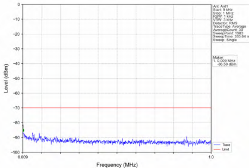
n78d_30kHz_SISO_NTNV_10MHz_DFT-s-OFDM QPSK_3624.99MHz_Edge_1RB_Left
