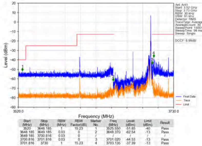
n78d_15kHz_SISO_NTNV_50MHz_CP-OFDM QPSK_3675MHz_Inner_1RB_Right
