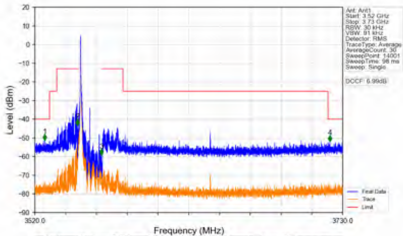
n78d_30kHz_SISO_NTNV_15MHz_DFT-s-OFDM_QPSK_3557.52MHz_Inner_1RB_Left
