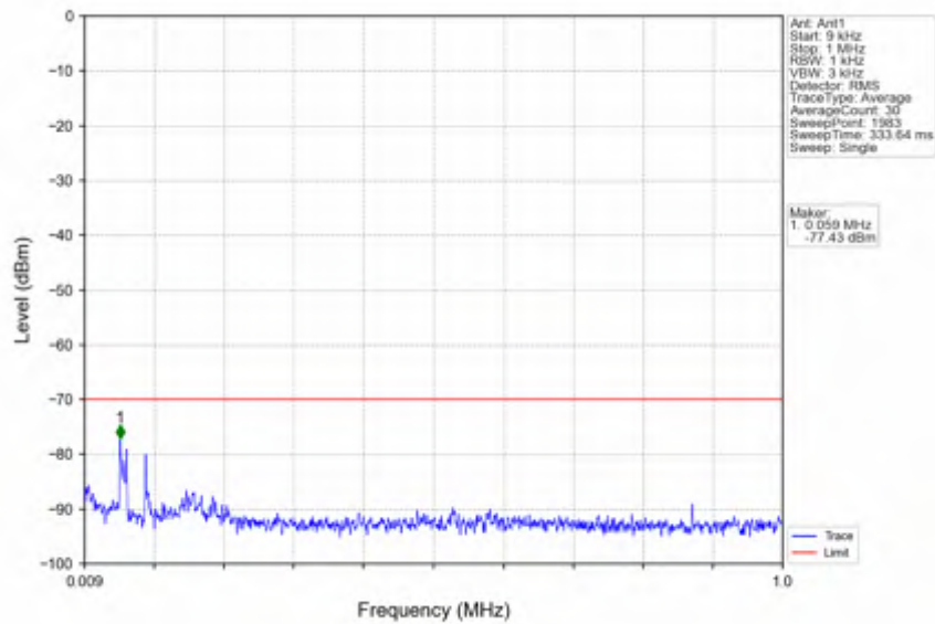
n78d_30kHz_SISO_NTNV_15MHz_DFT-s-OFDM PI/2 BPSK_3557.52MHz_Outer_Full
