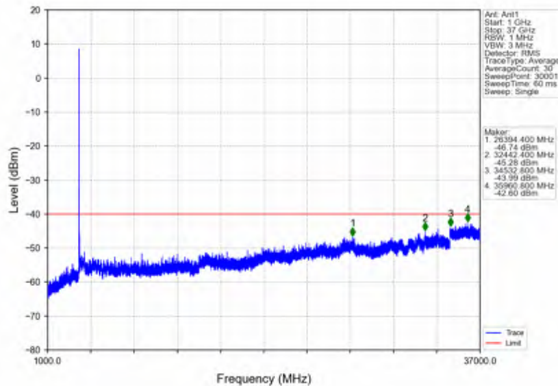
n78d_30kHz_SISO_NTVV_20MHz_CP-OFDM QPSK_3624.99MHz_Edge_1RB_Left
