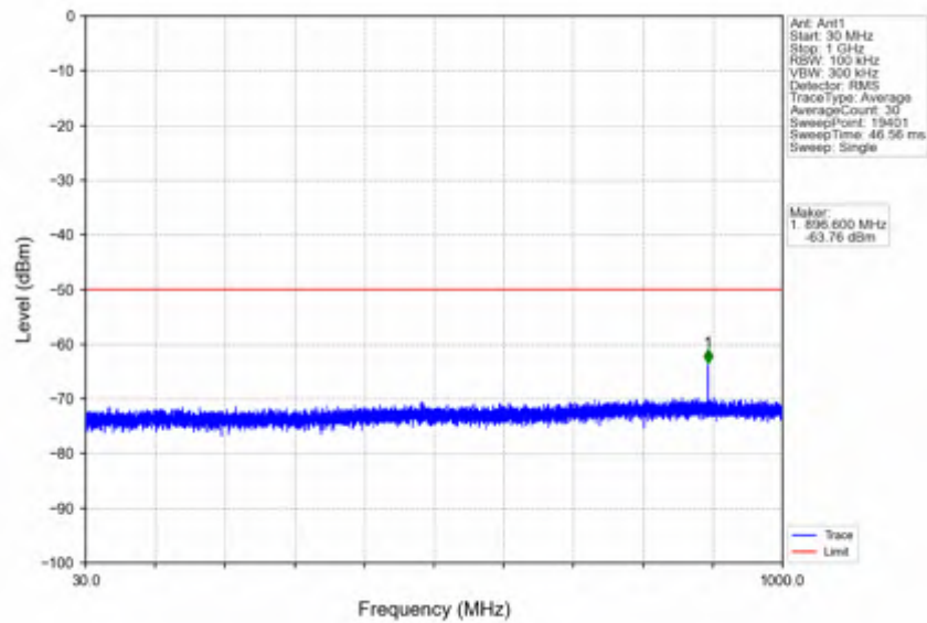
n78d_30kHz_SISO_NTNV_10MHz_DFT-s-OFDM PI/2 BPSK_3624.99MHz_Edge_1RB_Left
