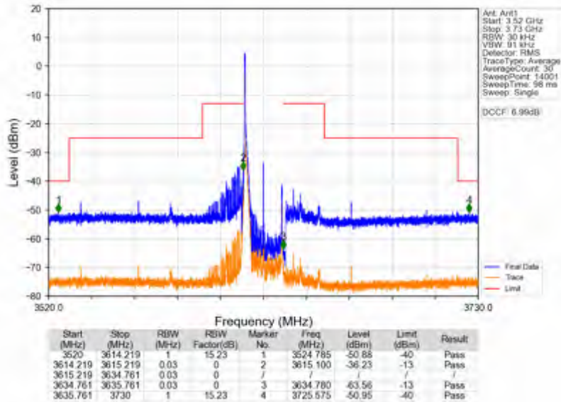
n78d_30kHz_SISO_NTNV_20MHz_DFT-s-OFDM PI/2 BPSK_3624.99MHz_Edge_1RB_Left
