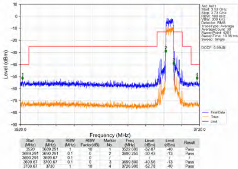
n78d_30kHz_SISO_NTNV_10MHz_CP-OFDM QPSK_3694.98MHz_Outer_Full
