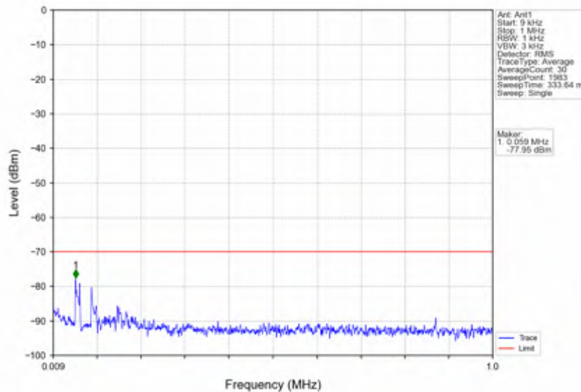
n78d_30kHz_SISO_NTNV_25MHz_DFT-s-OFDM PI/2 BPSK_3562.5MHz_Inner_1RB_Left
