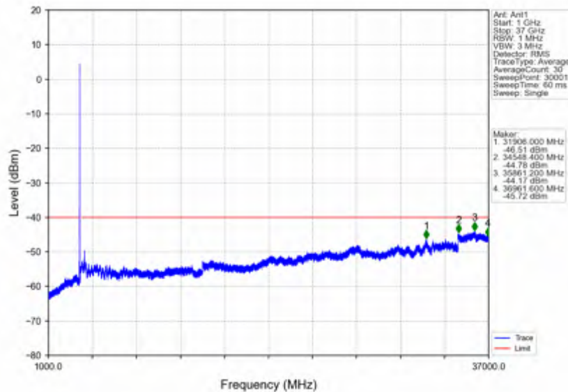
n78d_30kHz_SISO_NTNV_10MHz_DFT-s-OFDM PI/2 BPSK_3555MHz_Outer_Full
