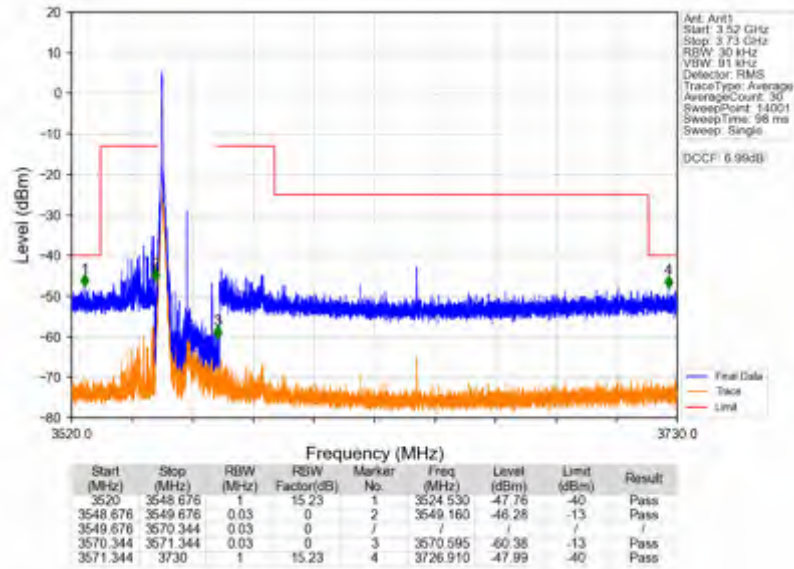
n78d_30kHz_SISO_NTV_20MHz_CP-OFDM_QPSK_3560.01MHz_Inner_1RB_Left
