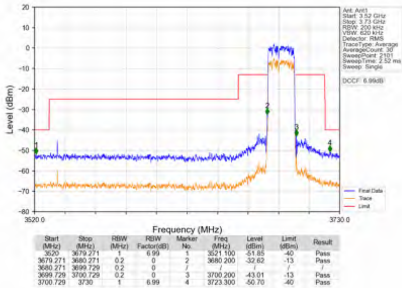
n78d_30kHz_SISO_NTNV_20MHz_DFT-s-OFDM PI/2 BPSK_3690MHz_Outer_Full
