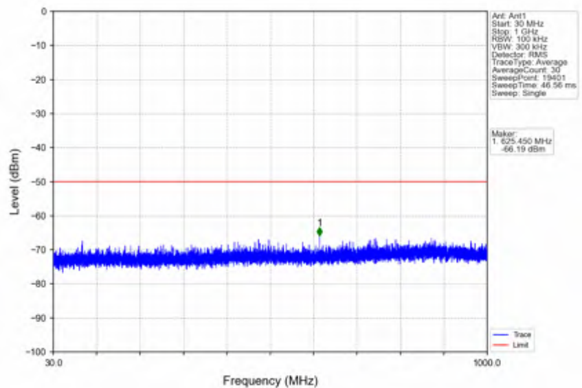
n78d_30kHz_SISO_NTNV_20MHz_DFT-s-OFDM QPSK_3624.99MHz_Edge_1RB_Left
