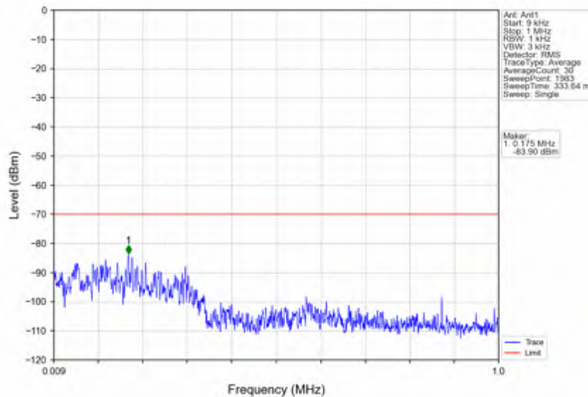
n78d_30kHz_SISO_NTNV_20MHz_DFT-s-OFDM_QPSK_3624.99MHz_Edge_1RB_Left
