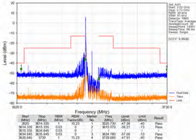
n78d_30kHz_SISO_NTV_20MHz_CP-OFDM_QPSK_3624.99MHz_Edge_1RB_Left
