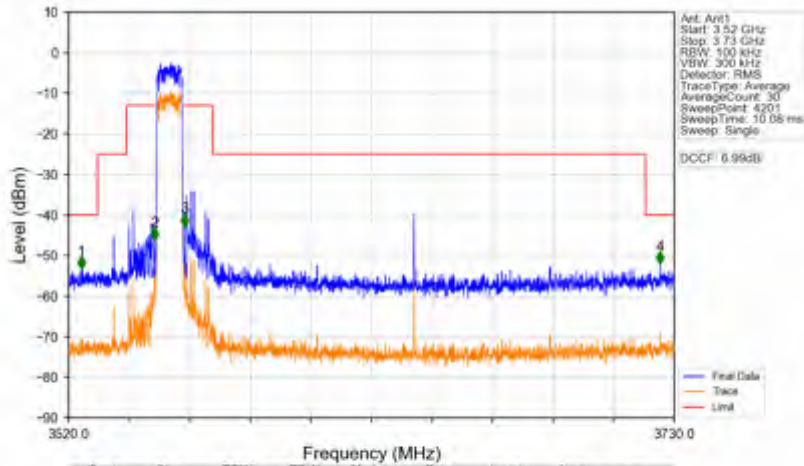
n78d_30kHz_SISO_NTNV_10MHz_CP-OFDM QPSK_3555MHz_Outer_Full
