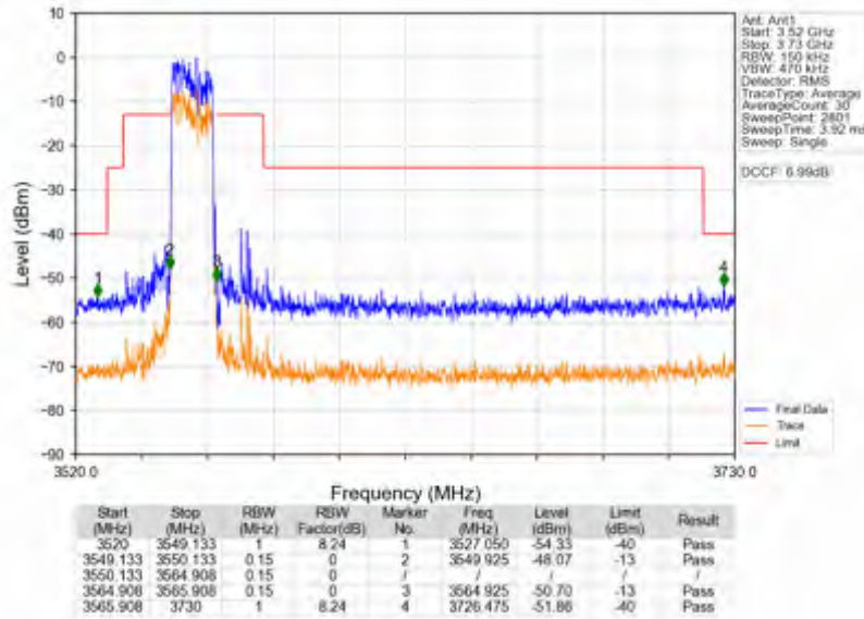
n78d_30kHz_SISO_NTNV_15MHz_DFT-s-OFDM_QPSK_3557.52MHz_Outer_Full
