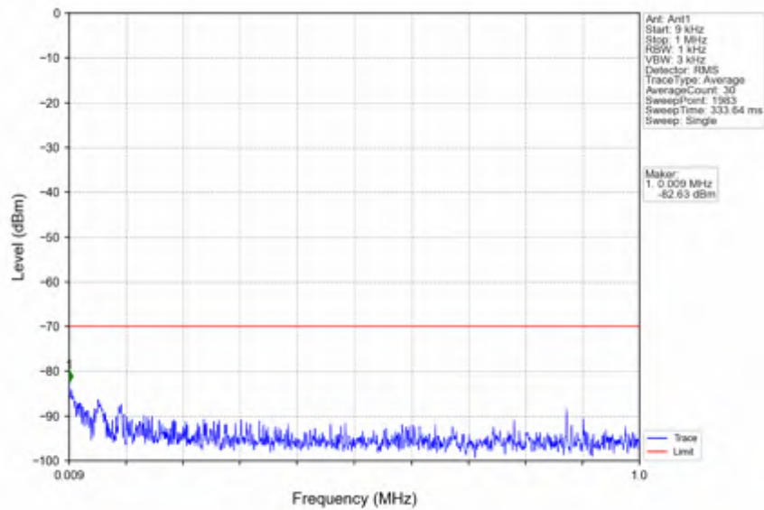
n78d_30kHz_SISO_NTVV_10MHz_DFT-s-OFDM_QPSK_3555MHz_Edge_1RB_Left
