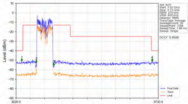
n78d_30kHz_SISO_NTNV_25MHz_DFT-s-OFDM PI/2 BPSK_3562.5MHz_Outer_Full
