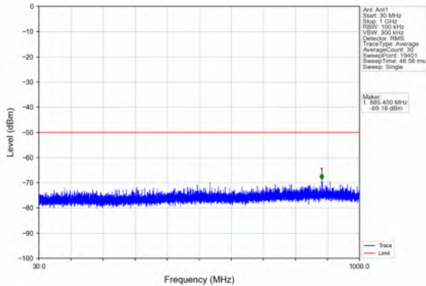
n78d_30kHz_SISO_NTNV_15MHz_DFT-s-OFDM QPSK_3692.49MHz_Edge_1RB_Right
