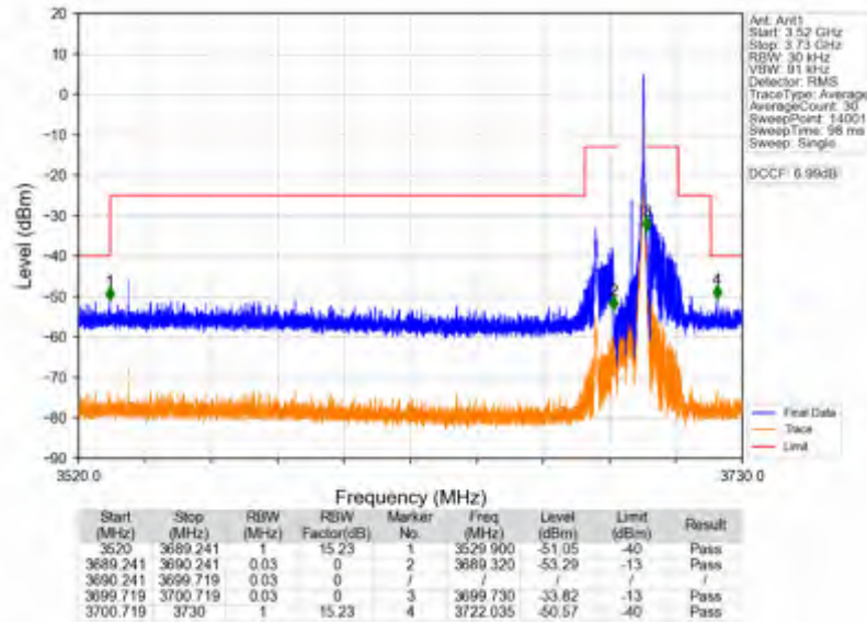
n78d_30kHz_SISO_NTV_10MHz_CP-OFDM QPSK_3694.98MHz_Inner_1RB_Right
