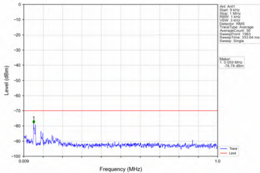
n78d_30kHz_SISO_NTNV_20MHz_DFT-s-OFDM PI/2 BPSK_3690MHz_Outer_Full
