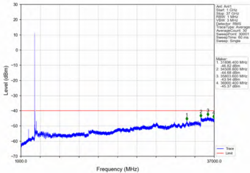
n78d_30kHz_SISO_NTNV_25MHz_DFT-s-OFDM PI/2 BPSK_3624.99MHz_Edge_1RB_Left
