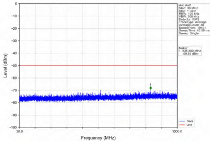
n78d_30kHz_SISO_NTVV_10MHz_CP-OFDM QPSK_3624.99MHz_Edge_1RB_Left
