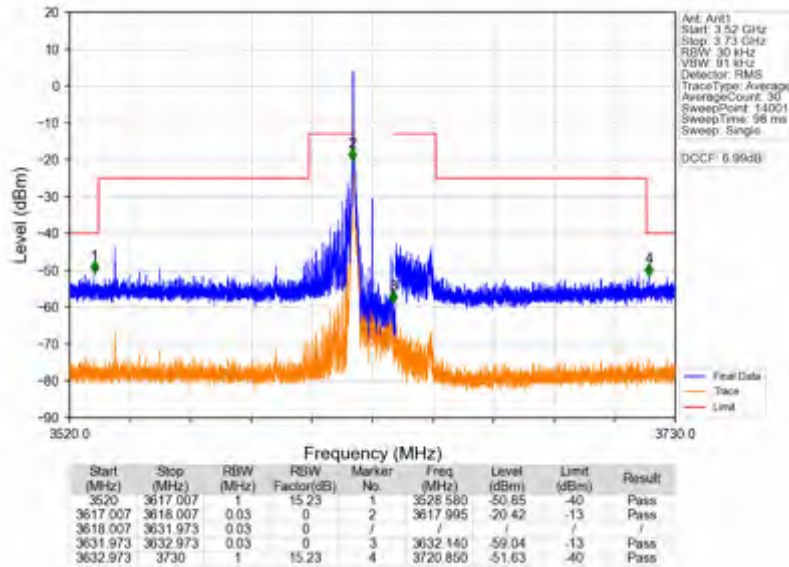
n78d_30kHz_SISO_NTVV_15MHz_CP-OFDM_QPSK_3624.99MHz_Edge_1RB_Left
