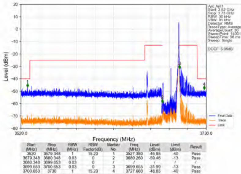
n78d_30kHz_SISO_NTNV_20MHz_DFT-s-OFDM_QPSK_3690MHz_Edge_1RB_Right
