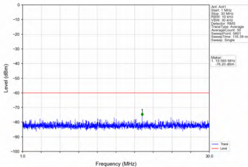
n78d_30kHz_SISO_NTNV_20MHz_DFT-s-OFDM QPSK_3560.01MHz_Edge_1RB_Left
