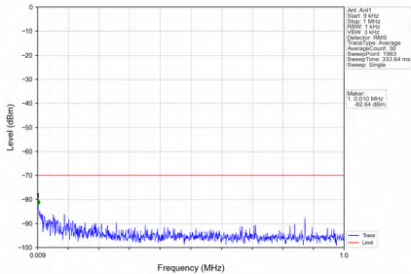
n78d_30kHz_SISO_NTV_15MHz_CP-OFDM QPSK_3624.99MHz_Edge_1RB_Left
