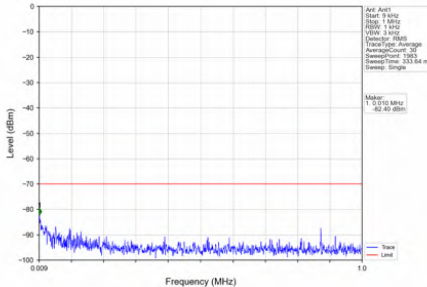
n78d_30kHz_SISO_NTNV_15MHz_DFT-s-OFDM_QPSK_3692.49MHz_Outer_Full
