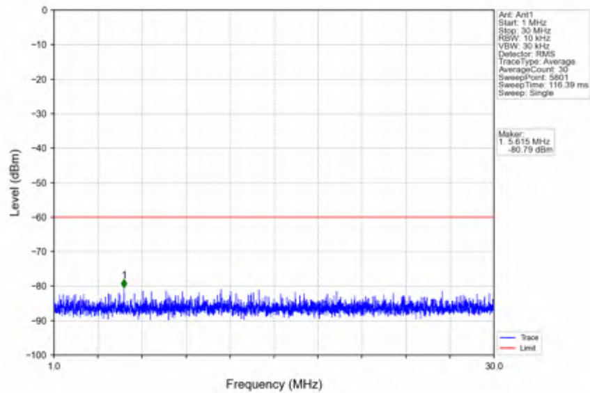
n78d_30kHz_SISO_NTNV_10MHz_DFT-s-OFDM QPSK_3555MHz_Outer_Full
