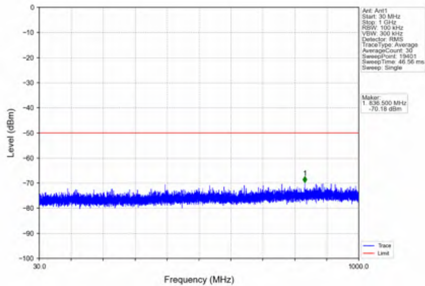
n78d_30kHz_SISO_NTNV_10MHz_CP-OFDM QPSK_3694.98MHz_Outer_Full
