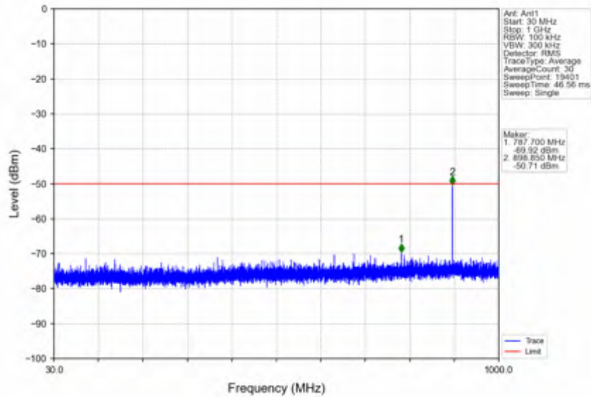
n78d_30kHz_SISO_NTNV_15MHz_DFT-s-OFDM QPSK_3557.52MHz_Edge_1RB_Left
