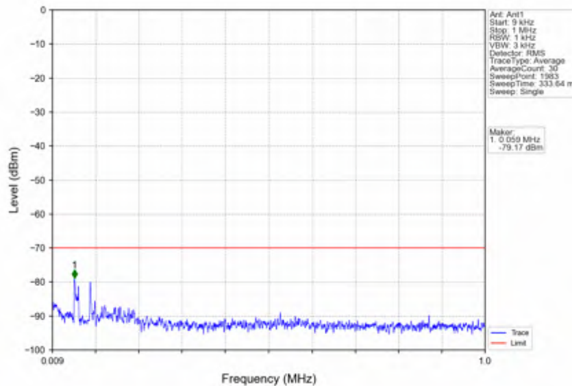
n78d_30kHz_SISO_NTV_20MHz_DFT-s-OFDM PI/2 BPSK_3690MHz_Edge_1RB_Right
