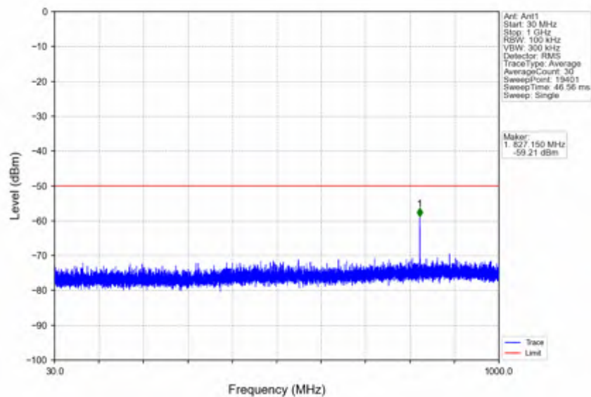
n78d_30kHz_SISO_NTNV_15MHz_CP-OFDM QPSK_3692.49MHz_Inner_1RB_Right
