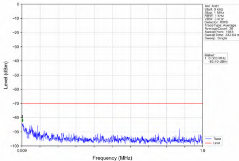
n78d_30kHz_SISO_NTV_10MHz_CP-OFDM QPSK_3694.98MHz_Edge_1RB_Right
