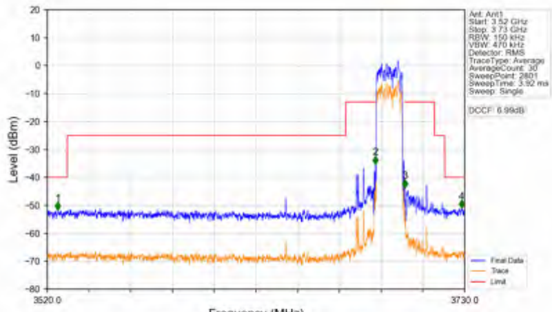
n78d_30kHz_SISO_NTNV_15MHz_DFT-s-OFDM PI/2 BPSK_3692.49MHz_Outer_Full
