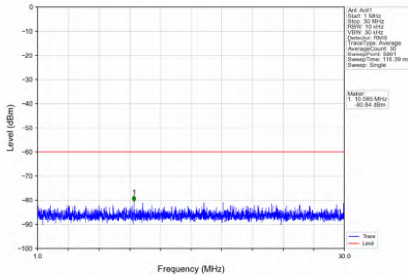
n78d_30kHz_SISO_NTNV_10MHz_CP-OFDM QPSK_3694.98MHz_Edge_1RB_Right
