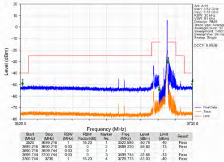
n78d_30kHz_SISO_NTNV_10MHz_DFT-s-OFDM PI/2 BPSK_3694.98MHz_Edge_1RB_Right
