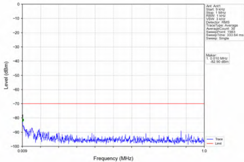
n78d_30kHz_SISO_NTVV_10MHz_CP-OFDM QPSK_3624.99MHz_Edge_1RB_Left
