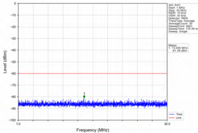
n78d_30kHz_SISO_NTV_15MHz_CP-OFDM QPSK_3557.52MHz_Edge_1RB_Left
