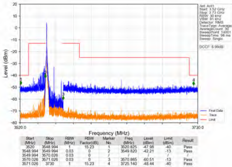
n78d_30kHz_SISO_NTNV_20MHz_DFT-s-OFDM QPSK_3560.01MHz_Inner_1RB_Left
