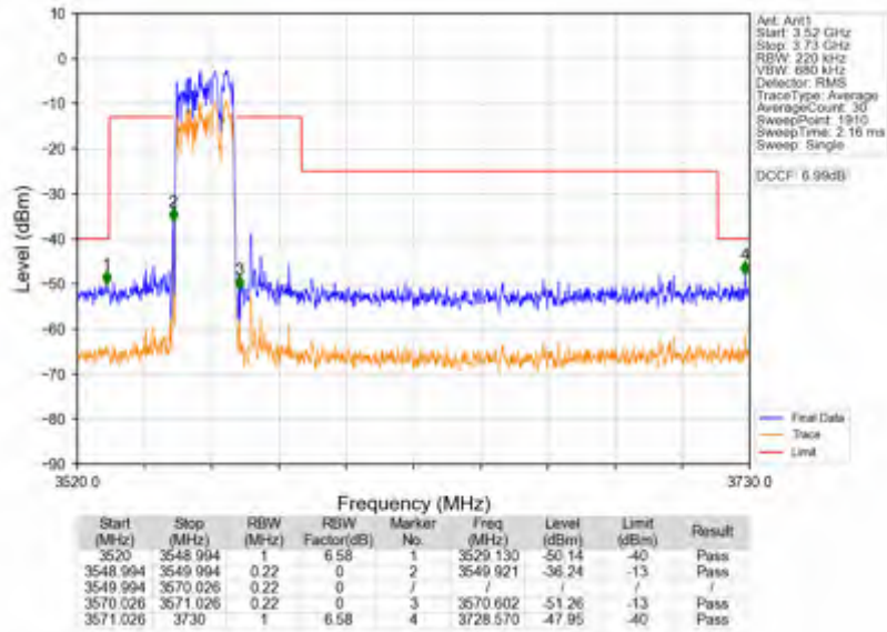
n78d_30kHz_SISO_NTNV_20MHz_DFT-s-OFDM_QPSK_3560.01MHz_Outer_Full
