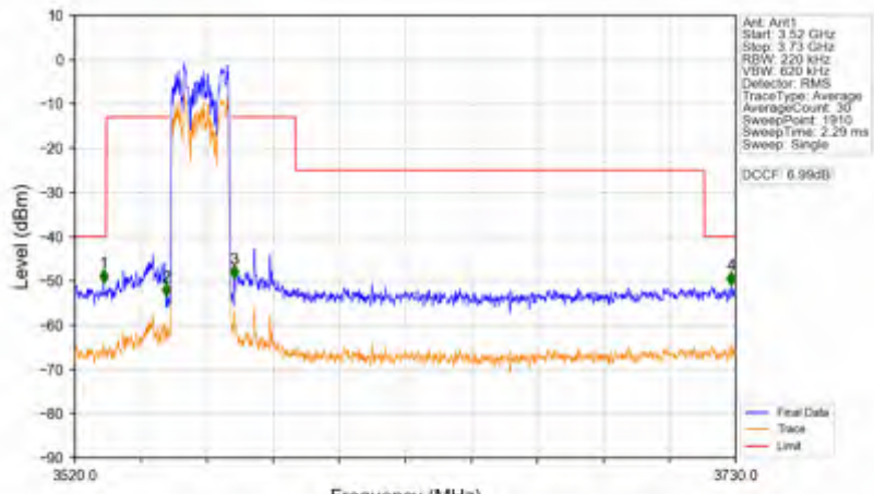
n78d_30kHz_SISO_NTNV_20MHz_DFT-s-OFDM PI/2 BPSK_3560.01MHz_Outer_Full
