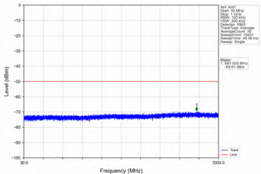
n78d_30kHz_SISO_NTNV_15MHz_DFT-s-OFDM PI/2 BPSK_3557.52MHz_Inner_1RB_Left
