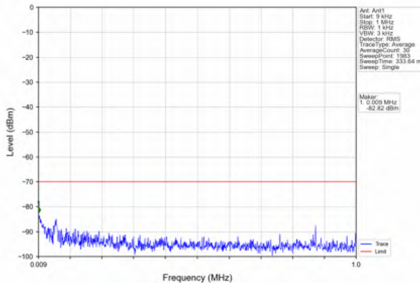
n78d_30kHz_SISO_NTV_15MHz_CP-OFDM QPSK_3557.52MHz_Edge_1RB_Left
