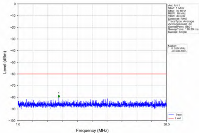
n78d_30kHz_SISO_NTNV_10MHz_DFT-s-OFDM QPSK_3555MHz_Inner_1RB_Left
