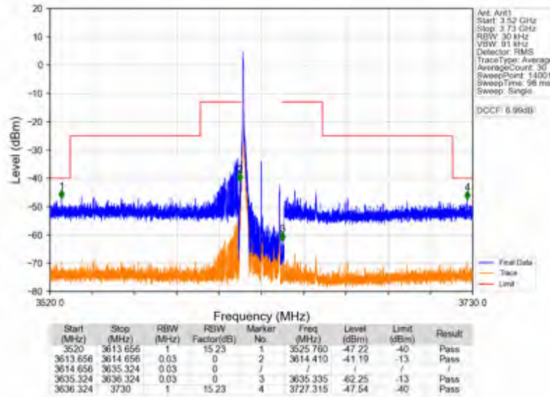
n78d_30kHz_SISO_NTNV_20MHz_DFT-s-OFDM_QPSK_3624.99MHz_Edge_1RB_Left
