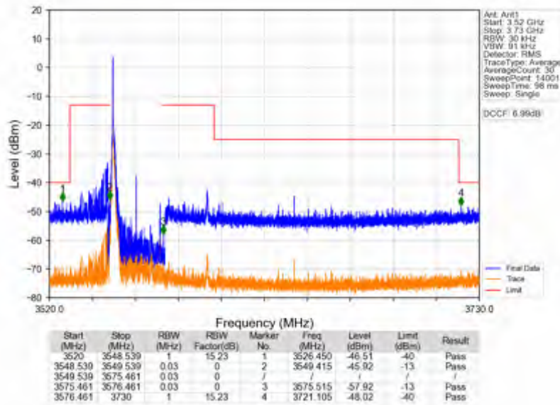
n78d_30kHz_SISO_NTNV_25MHz_DFT-s-OFDM QPSK_3562.5MHz_Edge_1RB_Left
