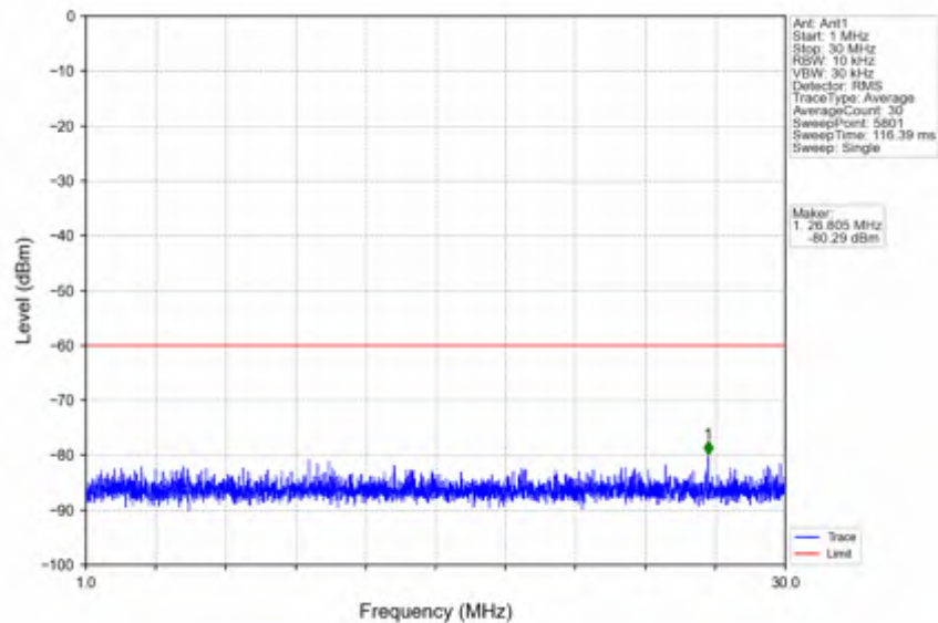
n78d_30kHz_SISO_NTNV_10MHz_DFT-s-OFDM QPSK_3694.98MHz_Inner_1RB_Right
