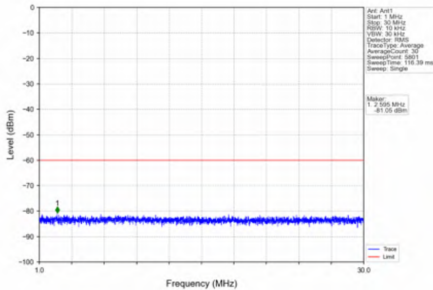
n78d_30kHz_SISO_NTNV_20MHz_DFT-s-OFDM PI/2 BPSK_3560.01MHz_Inner_1RB_Left
