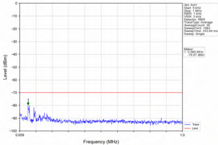
n78d_30kHz_SISO_NTNV_20MHz_DFT-s-OFDM PI/2 BPSK_3560.01MHz_Outer_Full
