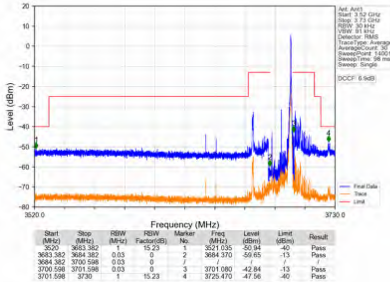
n78d_30kHz_SISO_NTNV_15MHz_DFT-s-OFDM PI/2 BPSK_3692.49MHz_Edge_1RB_Right
