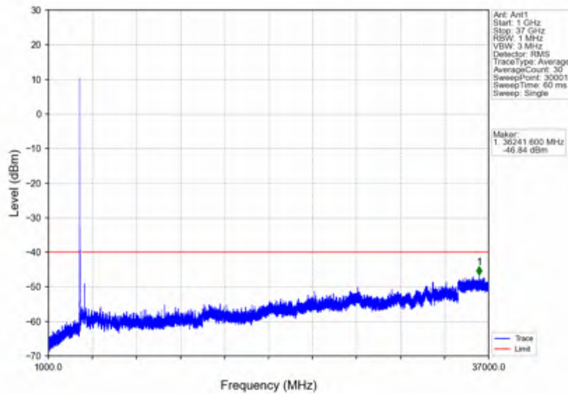
n78d_30kHz_SISO_NTVV_15MHz_CP-OFDM_QPSK_3624.99MHz_Edge_1RB_Left
