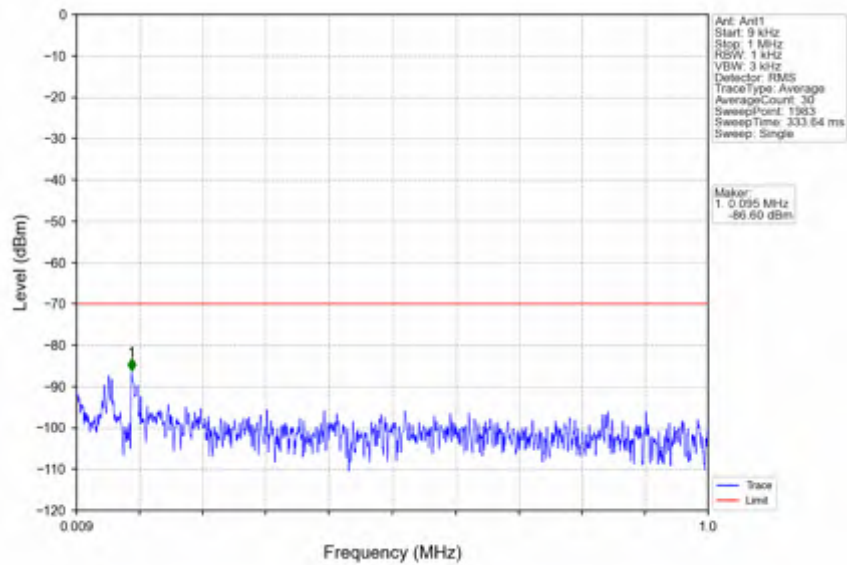
n78d_30kHz_SISO_NTNV_20MHz_CP-OFDM QPSK_3690MHz_Outer_Full
