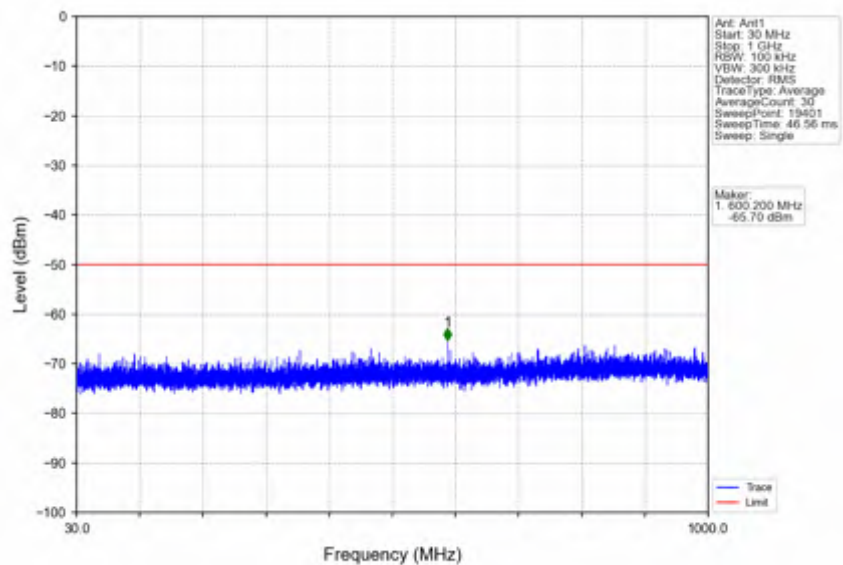
n78d_30kHz_SISO_NTVV_20MHz_CP-OFDM QPSK_3560.01MHz_Edge_1RB_Left
