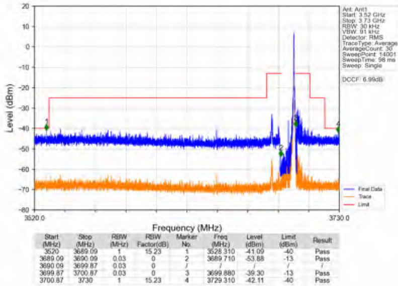
n78d_30kHz_SISO_NTNV_10MHz_DFT-s-OFDM QPSK_3694.98MHz_Inner_1RB_Right
