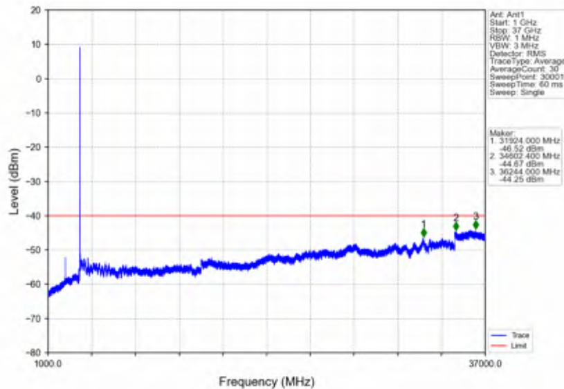
n78d_30kHz_SISO_NTNV_15MHz_DFT-s-OFDM PI/2 BPSK_3624.99MHz_Edge_1RB_Left
