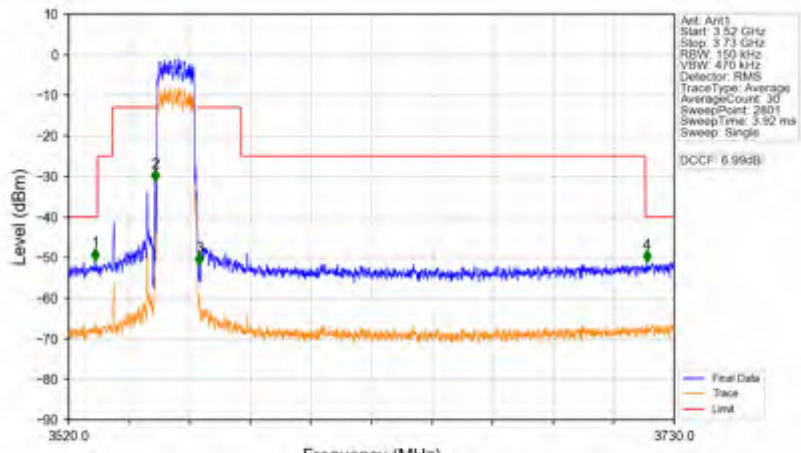
n78d_30kHz_SISO_NTNV_15MHz_DFT-s-OFDM PI/2 BPSK_3557.52MHz_Outer_Full
