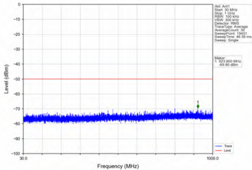
n78d_30kHz_SISO_NTNV_10MHz_CP-OFDM QPSK_3555MHz_Outer_Full
