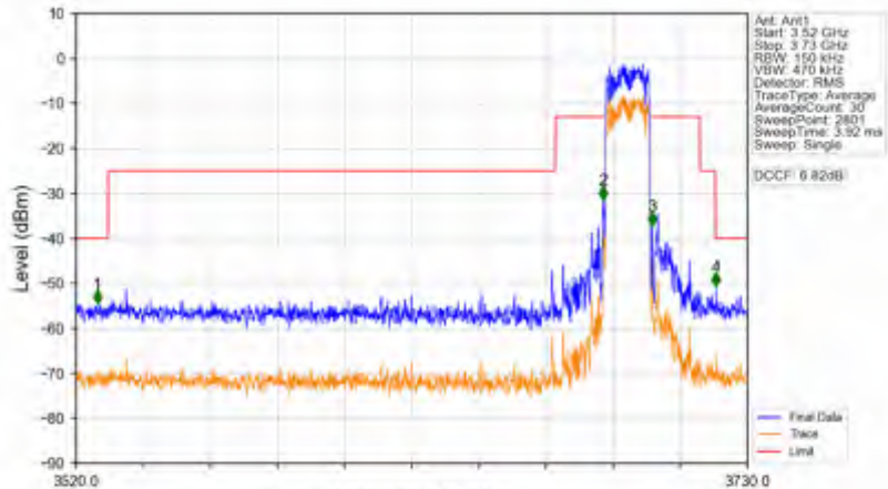
n78d_30kHz_SISO_NTNV_15MHz_CP-OFDM QPSK_3692.49MHz_Outer_Full
