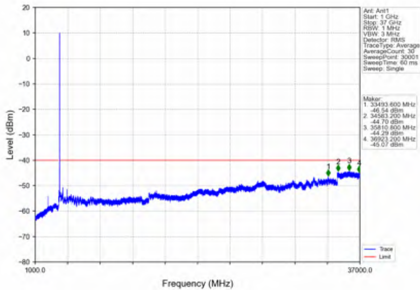
n78d_30kHz_SISO_NTV_10MHz_DFT-s-OFDM QPSK_3555MHz_Edge_1RB_Left
