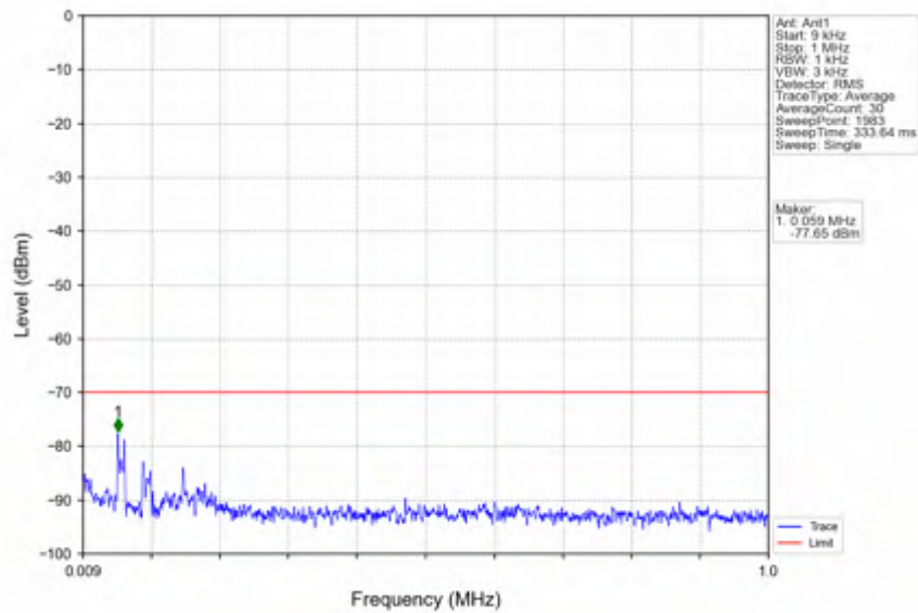
n78d_30kHz_SISO_NTNV_10MHz_DFT-s-OFDM PI/2 BPSK_3694.98MHz_Outer_Full
