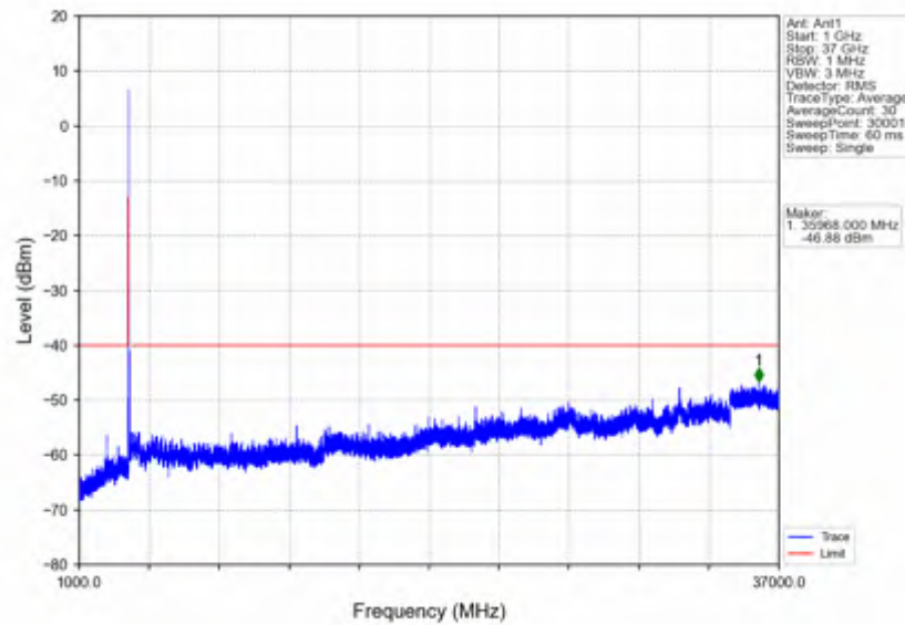
n78d_15kHz_SISO_NTVV_40MHz_DFT-s-OFDM_QPSK_3570MHz_Inner_1RB_Left
