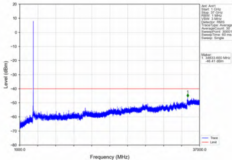
n78d_15kHz_SISO_NTV_25MHz_DFT-s-OFDM QPSK_3687.495MHz_Edge_1RB_Right
