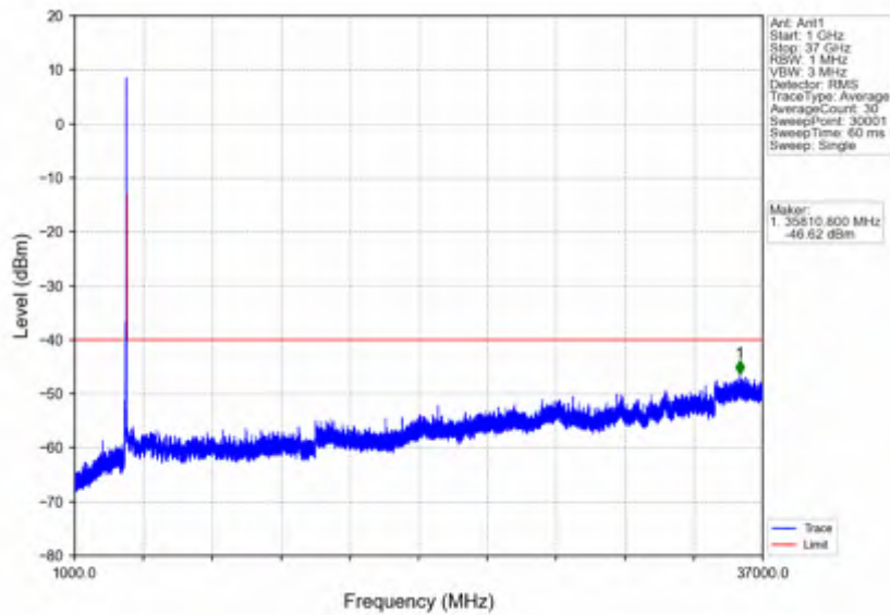
n78d_15kHz_SISO_NTV_40MHz_CP-OFDM QPSK_3679.995MHz_Outer_Full
