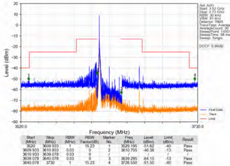
n78d_15kHz_SISO_NTNV_25MHz_DFT-s-OFDM QPSK_3625.005MHz_Edge_1RB_Left
