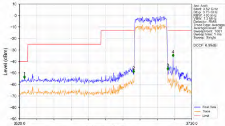
n78d_15kHz_SISO_NTV_40MHz_CP-OFDM QPSK_3679.995MHz_Outer_Full
