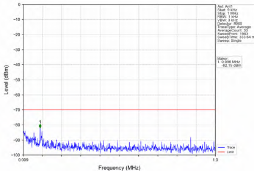
n78d_15kHz_SISO_NTV_25MHz_CP-OFDM QPSK_3687.495MHz_Edge_1RB_Right
