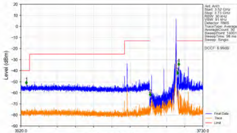
n78d_15kHz_SISO_NTNV_30MHz_DFT-s-OFDM QPSK_3684.99MHz_Inner_1RB_Right
