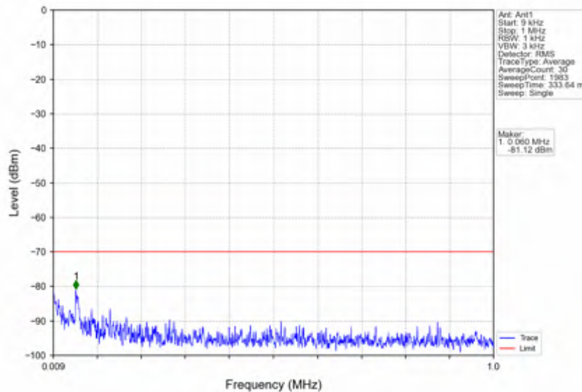
n78d_15kHz_SISO_NTNV_25MHz_CP-OFDM QPSK_3562.5MHz_Inner_1RB_Left
