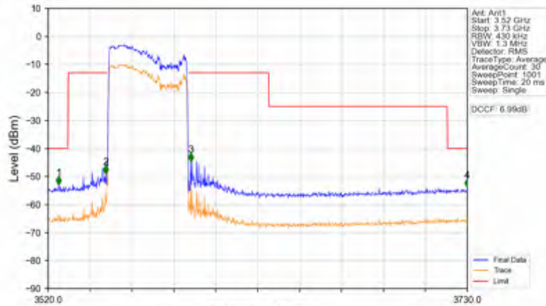
n78d_15kHz_SISO_NTNV_40MHz_CP-OFDM QPSK_3570MHz_Outer_Full
