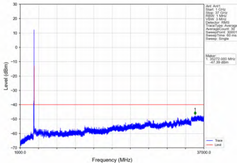
n78d_15kHz_SISO_NTV_40MHz_DFT-s-OFDM_QPSK_3679.995MHz_Inner_1RB_Right
