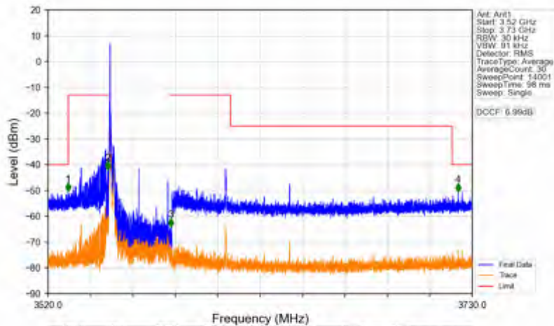
n78d_15kHz_SISO_NTNV_30MHz_DFT-s-OFDM QPSK_3565.005MHz_Edge_1RB_Left
