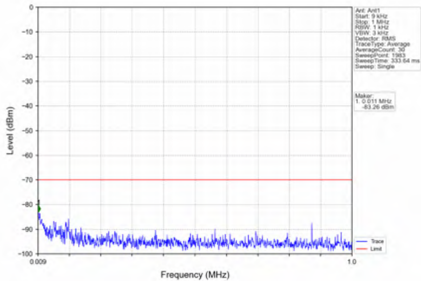
n78d_15kHz_SISO_NTVV_40MHz_DFT-s-OFDM_QPSK_3570MHz_Inner_1RB_Left
