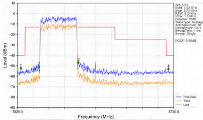
n78d_15kHz_SISO_NTV_50MHz_CP-OFDM QPSK_3575.01MHz_Outer_Full
