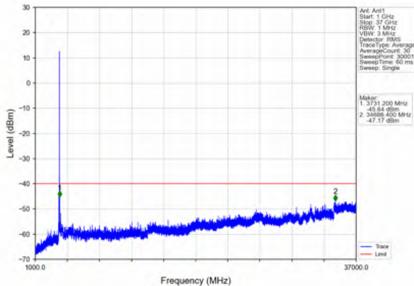
n78d_15kHz_SISO_NTV_25MHz_DFT-s-OFDM QPSK_3687.495MHz_Inner_1RB_Right
