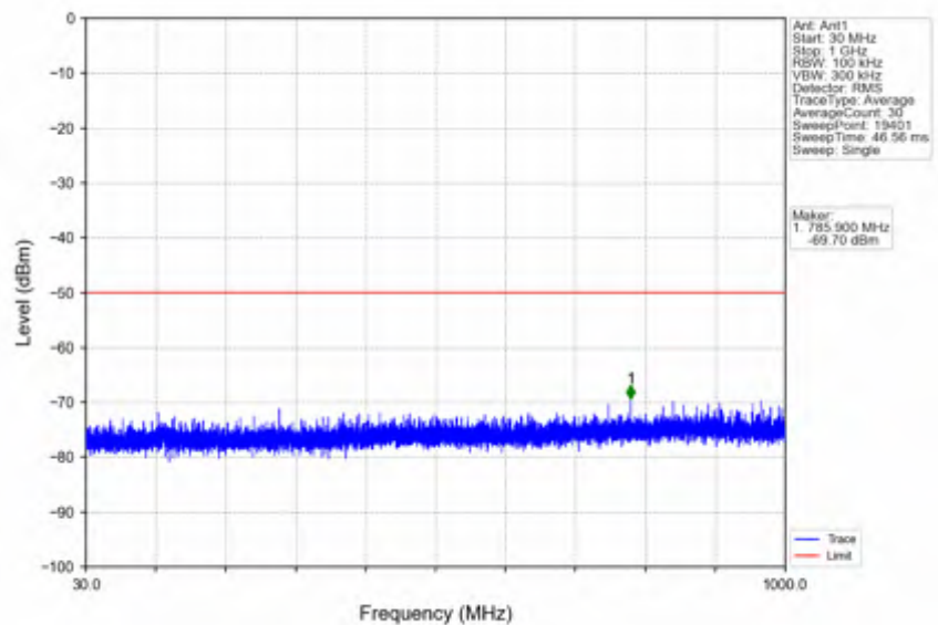
n78d_15kHz_SISO_NTNV_30MHz_CP-OFDM QPSK_3565.005MHz_Edge_1RB_Left
