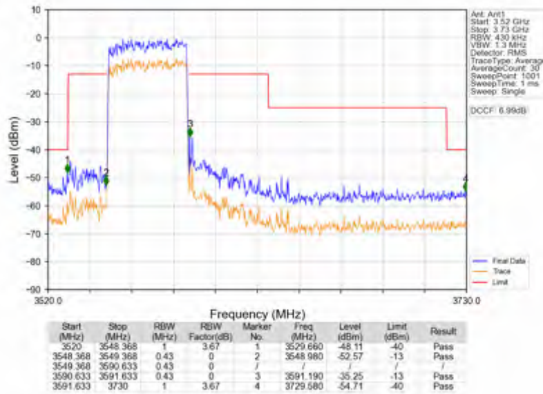
n78d_15kHz_SISO_NTNV_40MHz_DFT-s-OFDM QPSK_3570MHz_Outer_Full
