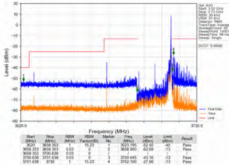
n78d_15kHz_SISO_NTV_40MHz_CP-OFDM QPSK_3679.995MHz_Inner_1RB_Right
