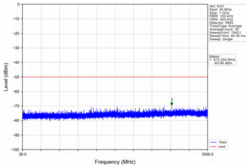
n78d_15kHz_SISO_NTNV_40MHz_DFT-s-OFDM QPSK_3625.005MHz_Edge_1RB_Left
