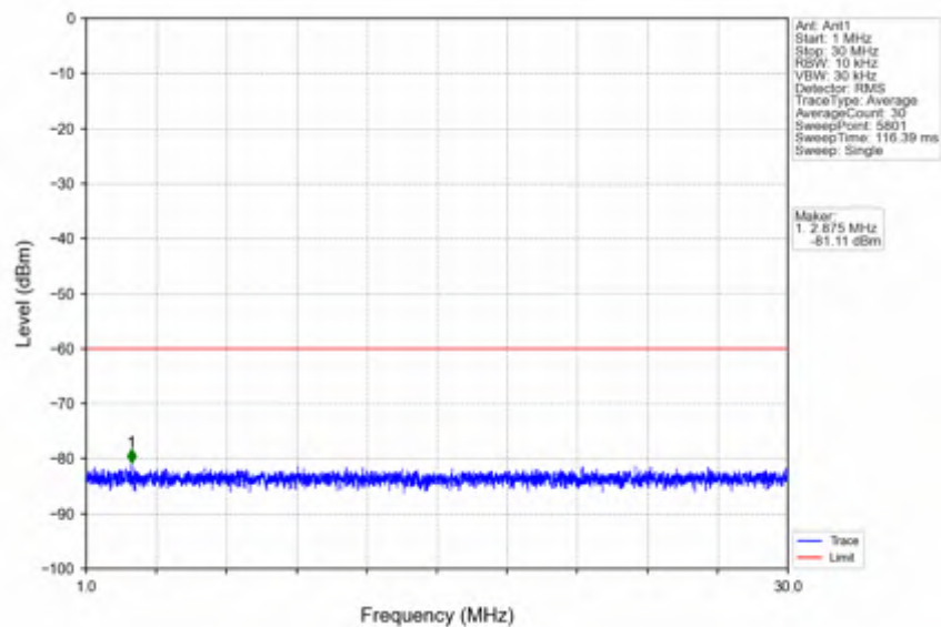
n78d_15kHz_SISO_NTNV_40MHz_DFT-s-OFDM PI/2 BPSK_3625.005MHz_Edge_1RB_Left
