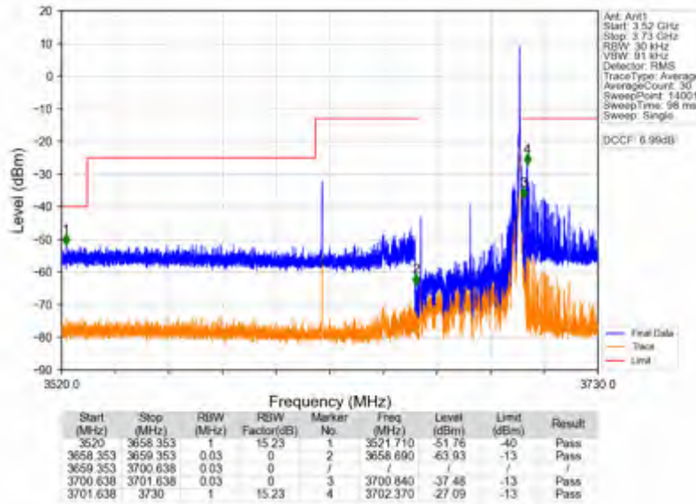
n78d_15kHz_SISO_NTNV_40MHz_CP-OFDM QPSK_3679.995MHz_Edge_1RB_Right
