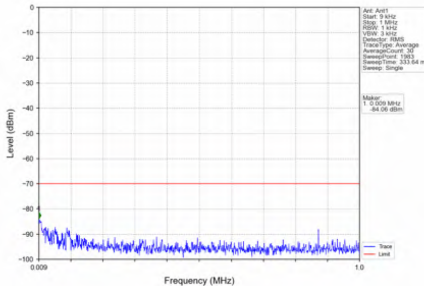
n78d_15kHz_SISO_NTNV_30MHz_DFT-s-OFDM QPSK_3565.005MHz_Outer_Full
