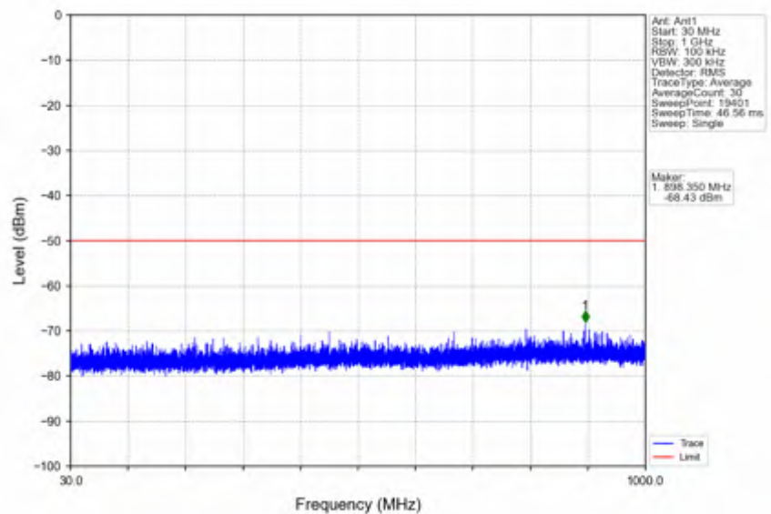
n78d_15kHz_SISO_NTNV_25MHz_CP-OFDM QPSK_3687.495MHz_Edge_1RB_Right
