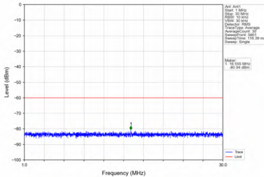
n78d_15kHz_SISO_NTNV_40MHz_DFT-s-OFDM PI/2 BPSK_3679.995MHz_Inner_1RB_Right
