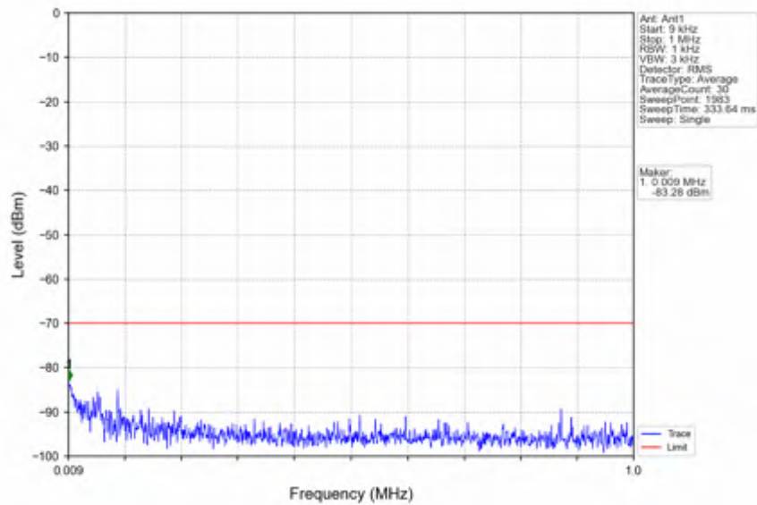
n78d_15kHz_SISO_NTNV_30MHz_DFT-s-OFDM QPSK_3565.005MHz_Inner_1RB_Left
