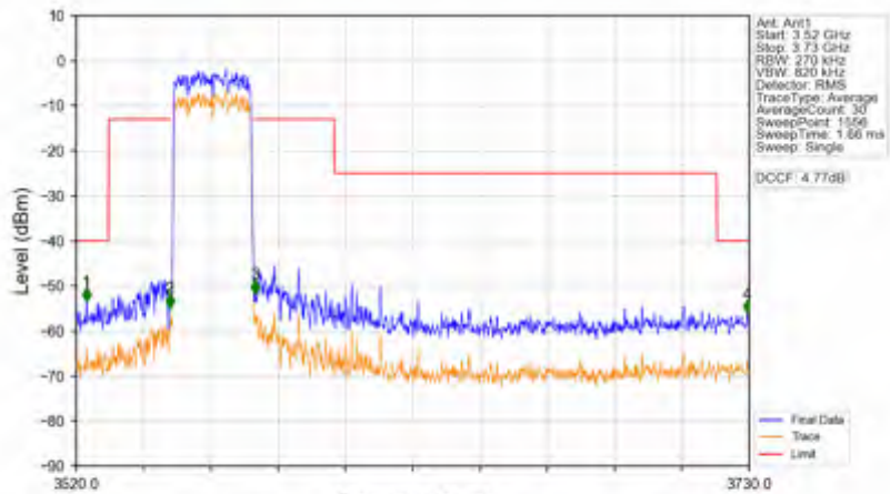
n78d_15kHz_SISO_NTNV_25MHz_CP-OFDM QPSK_3562.5MHz_Outer_Full
