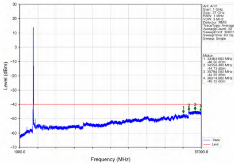
n78d_15kHz_SISO_NTNV_50MHz_DFT-s-OFDM PI/2 BPSK_3675MHz_Outer_Full
