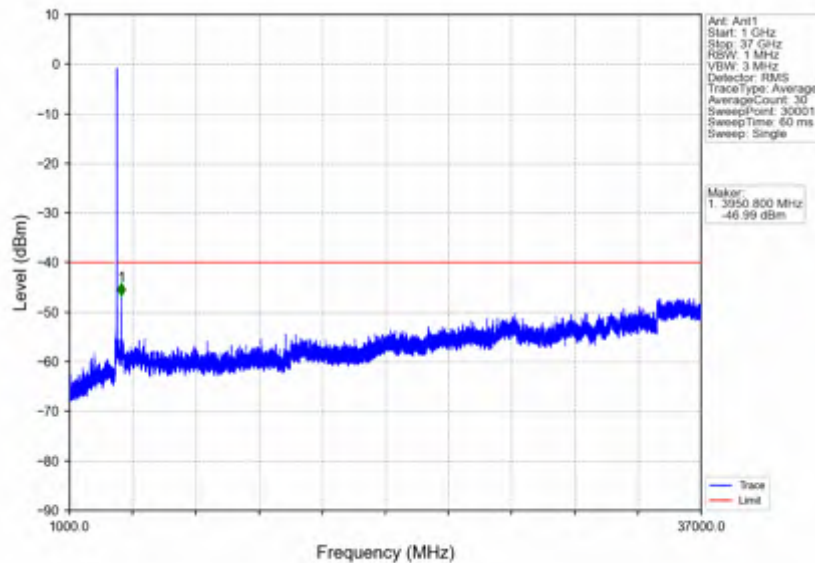
n78d_15kHz_SISO_NTNV_25MHz_CP-OFDM QPSK_3687.495MHz_Outer_Full
