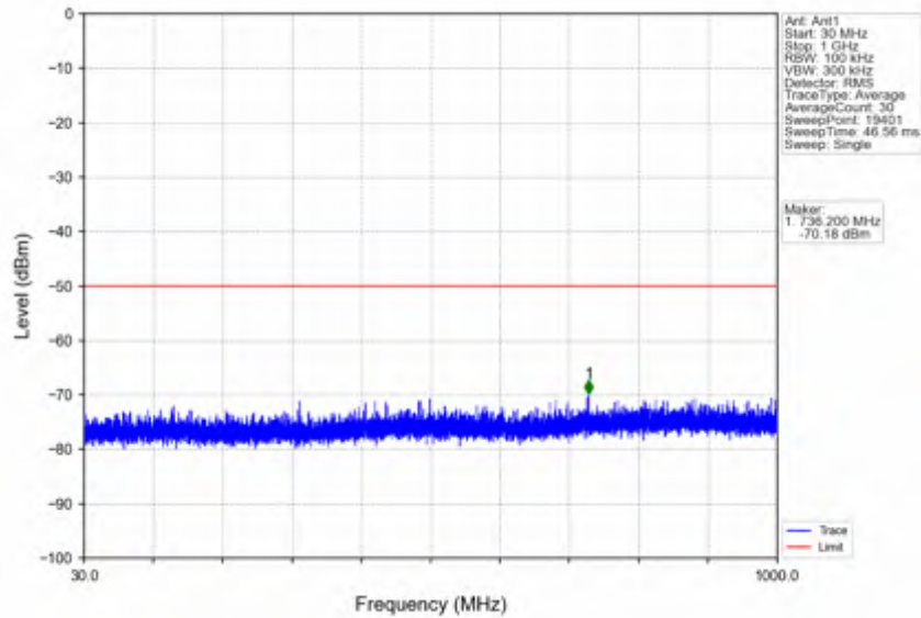
n78d_15kHz_SISO_NTV_25MHz_DFT-s-OFDM QPSK_3687.495MHz_Edge_1RB_Right
