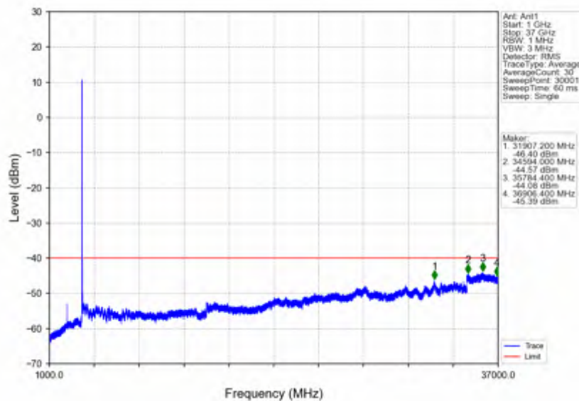
n78d_15kHz_SISO_NTNV_30MHz_DFT-s-OFDM PI/2 BPSK_3625.005MHz_Edge_1RB_Left
