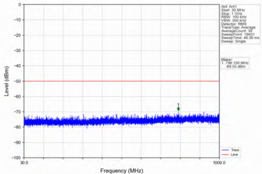
n78d_15kHz_SISO_NTV_25MHz_CP-OFDM QPSK_3687.495MHz_Inner_1RB_Right
