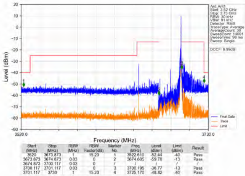
n78d_15kHz_SISO_NTNV_25MHz_DFT-s-OFDM QPSK_3687.495MHz_Edge_1RB_Right
