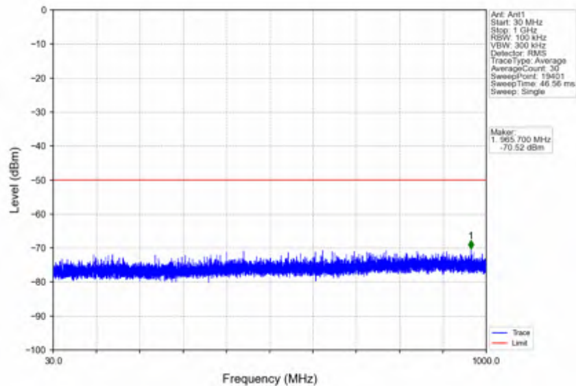
n78d_15kHz_SISO_NTNV_25MHz_CP-OFDM QPSK_3562.5MHz_Inner_1RB_Left
