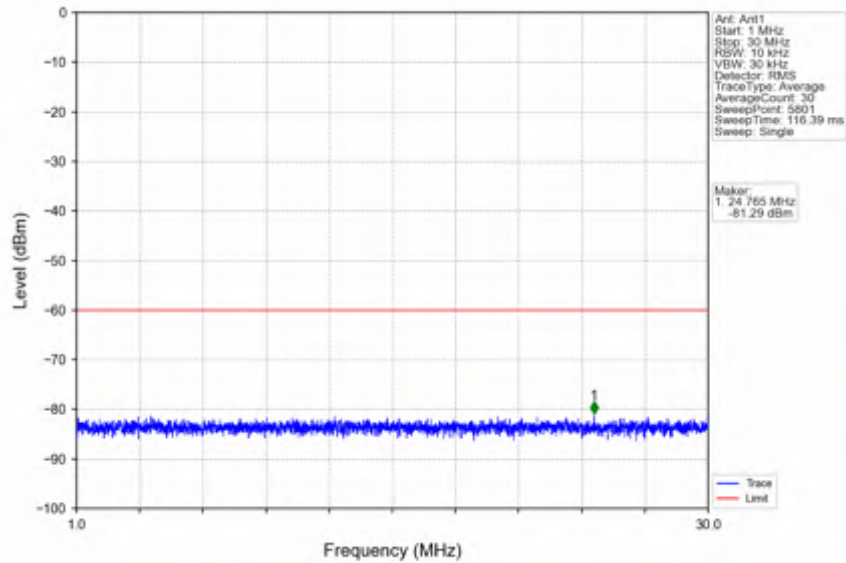
n78d_15kHz_SISO_NTNV_40MHz_DFT-s-OFDM PI/2 BPSK_3679.995MHz_Edge_1RB_Right
