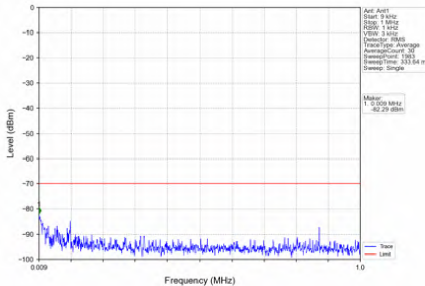
n78d_15kHz_SISO_NTV_30MHz_CP-OFDM QPSK_3684.99MHz_Edge_1RB_Right
