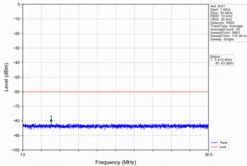
n78d_15kHz_SISO_NTNV_30MHz_DFT-s-OFDM PI/2 BPSK_3565.005MHz_Inner_1RB_Left
