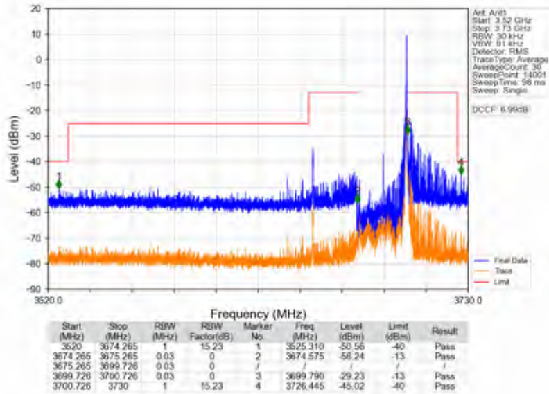
n78d_15kHz_SISO_NTV_25MHz_CP-OFDM QPSK_3687.495MHz_Inner_1RB_Right
