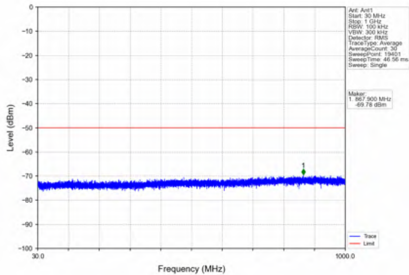
n78d_15kHz_SISO_NTNV_50MHz_DFT-s-OFDM PI/2 BPSK_3625.005MHz_Edge_1RB_Left
