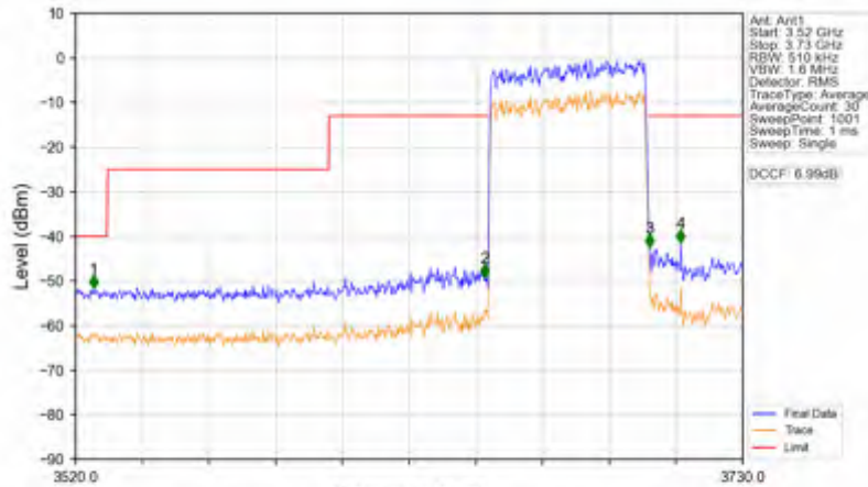
n78d_15kHz_SISO_NTNV_50MHz_DFT-s-OFDM PI/2 BPSK_3675MHz_Outer_Full
