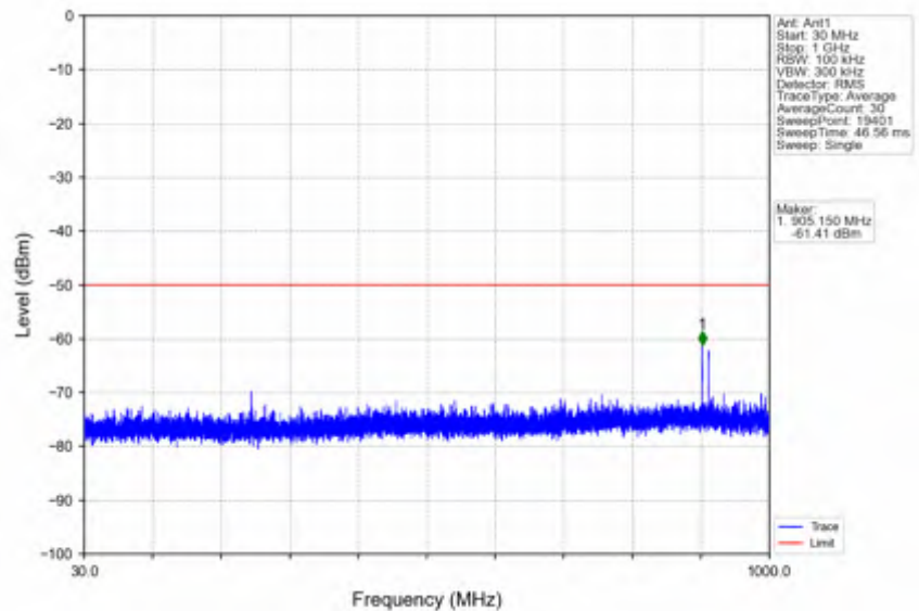
n78d_15kHz_SISO_NTNV_50MHz_CP-OFDM QPSK_3675MHz_Edge_1RB_Right
