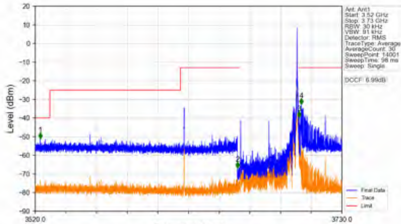
n78d_15kHz_SISO_NTNV_40MHz_DFT-s-OFDM QPSK_3679.995MHz_Edge_1RB_Right
