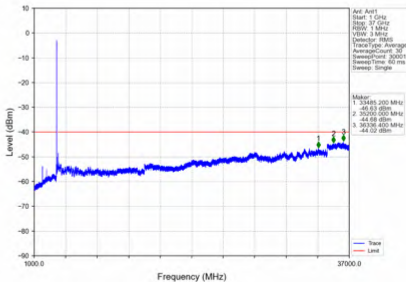
n78d_15kHz_SISO_NTNV_30MHz_DFT-s-OFDM PI/2 BPSK_3565.005MHz_Outer_Full
