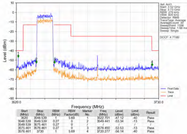
n78d_15kHz_SISO_NTNV_25MHz_DFT-s-OFDM QPSK_3562.5MHz_Outer_Full
