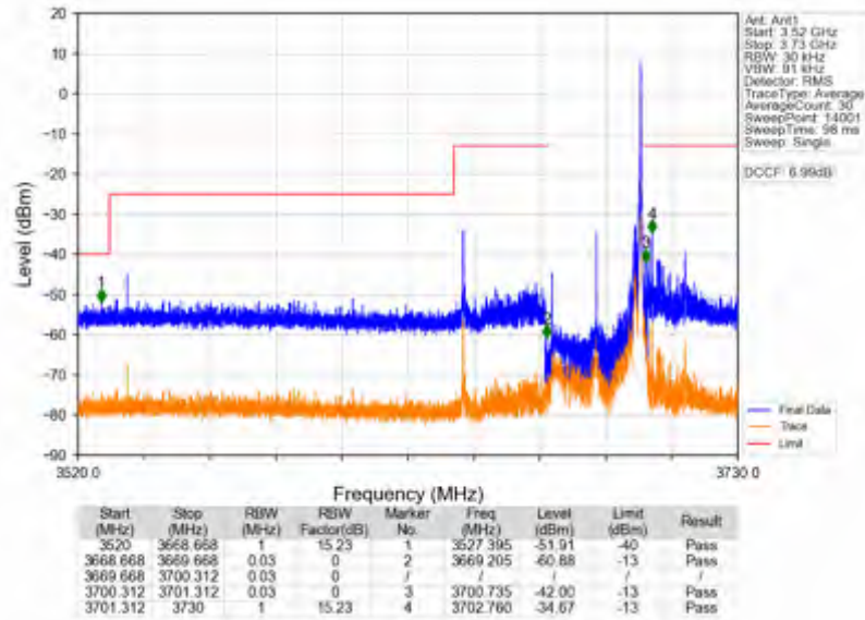
n78d_15kHz_SISO_NTV_30MHz_CP-OFDM QPSK_3684.99MHz_Inner_1RB_Right
