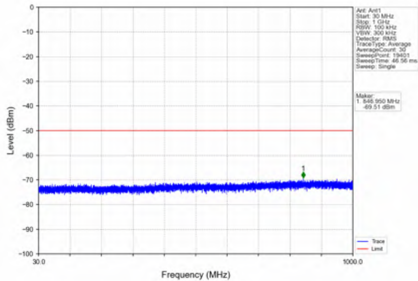
n78d_15kHz_SISO_NTVV_40MHz_DFT-s-OFDM_QPSK_3570MHz_Edge_1RB_Left
