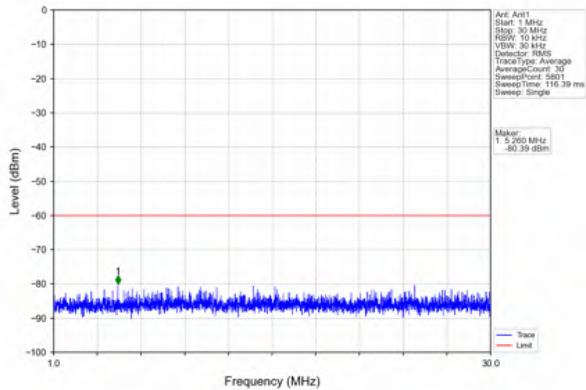
n78d_15kHz_SISO_NTNV_30MHz_CP-OFDM QPSK_3684.99MHz_Edge_1RB_Right
