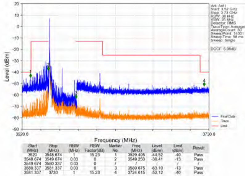
n78d_15kHz_SISO_NTNV_30MHz_CP-OFDM QPSK_3565.005MHz_Inner_1RB_Left
