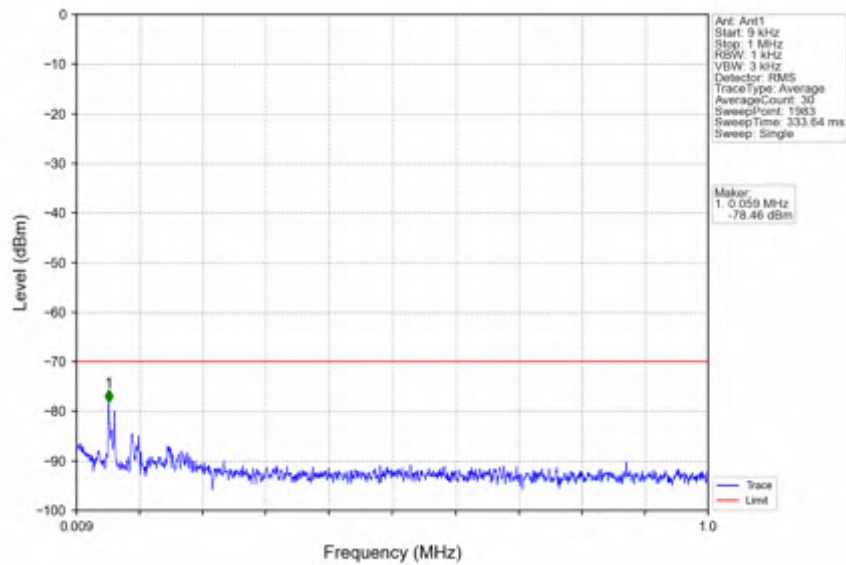
n78d_15kHz_SISO_NTNV_50MHz_DFT-s-OFDM QPSK_3575.01MHz_Edge_1RB_Left
