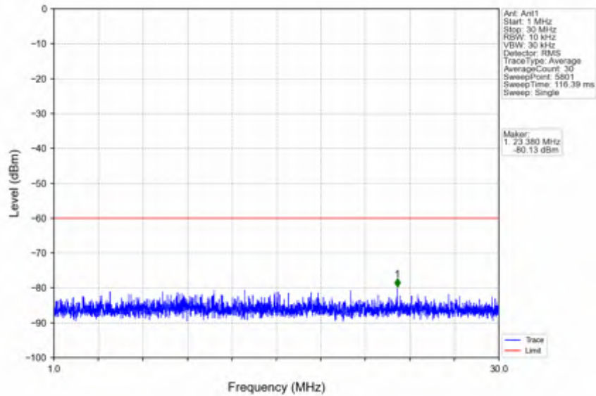
n78d_15kHz_SISO_NTNV_40MHz_CP-OFDM QPSK_3679.995MHz_Inner_1RB_Right
