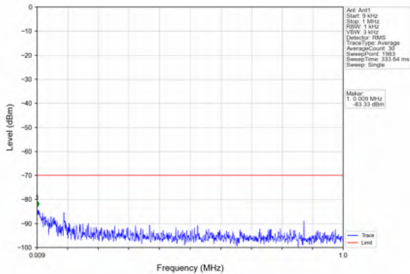
n78d_15kHz_SISO_NTNV_40MHz_CP-OFDM QPSK_3625.005MHz_Edge_1RB_Left
