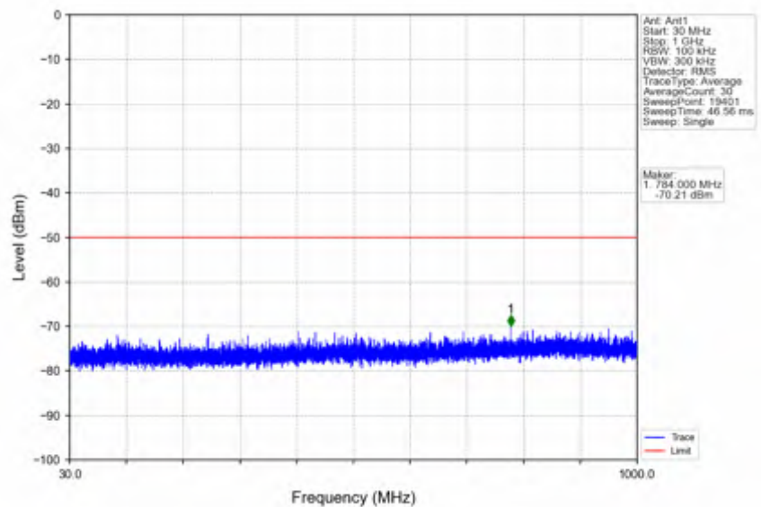
n78d_15kHz_SISO_NTNV_50MHz_DFT-s-OFDM_QPSK_3675MHz_Outer_Full
