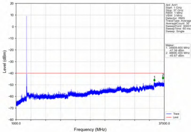
n78d_15kHz_SISO_NTNV_30MHz_DFT-s-OFDM QPSK_3565.005MHz_Edge_1RB_Left
