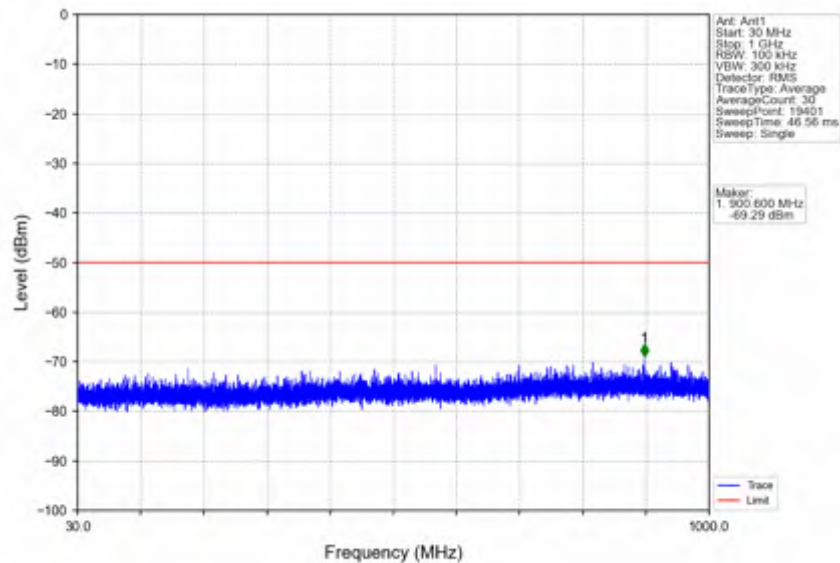
n78d_15kHz_SISO_NTNV_30MHz_DFT-s-OFDM QPSK_3625.005MHz_Edge_1RB_Left
