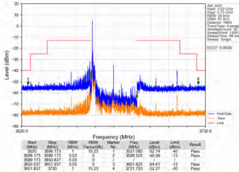
n78d_15kHz_SISO_NTNV_50MHz_DFT-s-OFDM QPSK_3625.005MHz_Edge_1RB_Left
