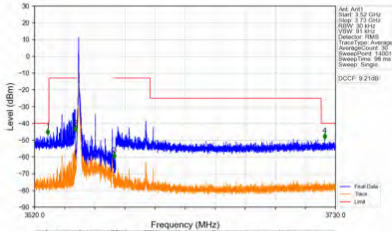
n78d_15kHz_SISO_NTNV_25MHz_DFT-s-OFDM QPSK_3562.5MHz_Inner_1RB_Left
