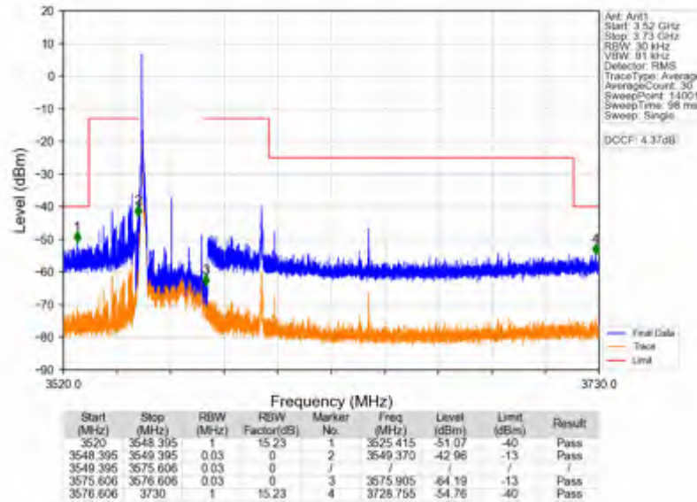
n78d_15kHz_SISO_NTNV_25MHz_CP-OFDM QPSK_3562.5MHz_Inner_1RB_Left
