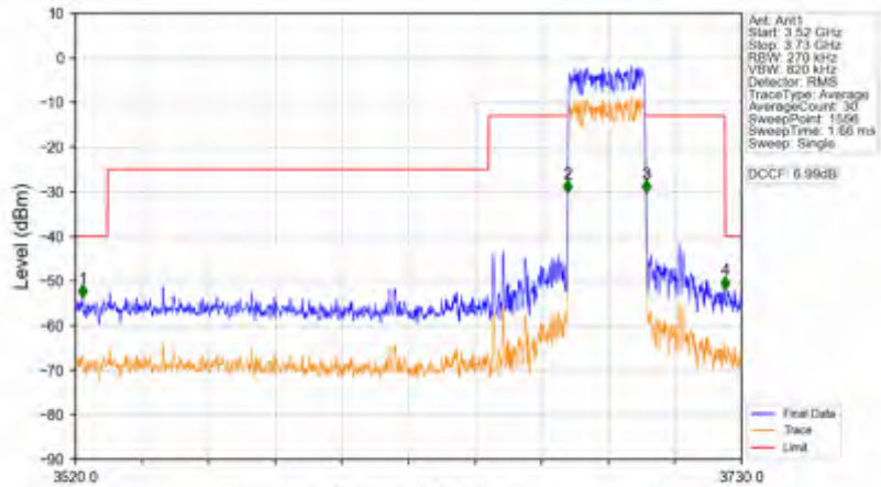
n78d_15kHz_SISO_NTV_25MHz_CP-OFDM QPSK_3687.495MHz_Outer_Full
