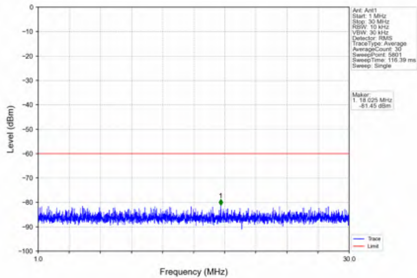
n78d_15kHz_SISO_NTNV_30MHz_CP-OFDM QPSK_3565.005MHz_Inner_1RB_Left
