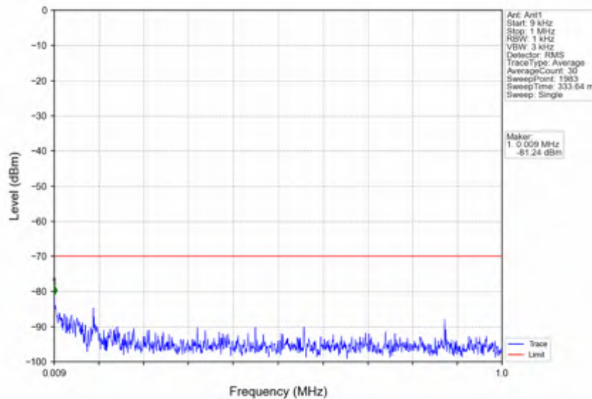
n78d_15kHz_SISO_NTV_40MHz_CP-OFDM QPSK_3679.995MHz_Inner_1RB_Right
