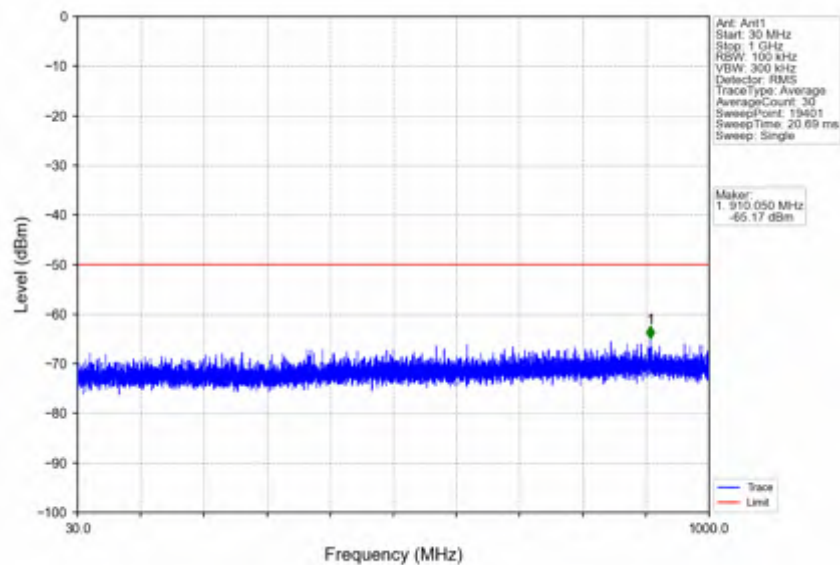
n78d_15kHz_SISO_NTNV_50MHz_CP-OFDM QPSK_3575.01MHz_Inner_1RB_Left
