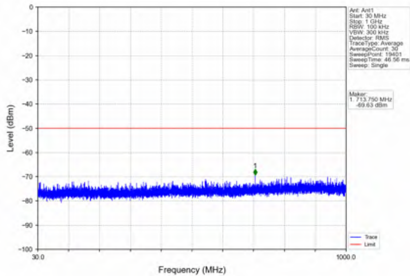
n78d_15kHz_SISO_NTNV_50MHz_DFT-s-OFDM_QPSK_3675MHz_Inner_1RB_Right
