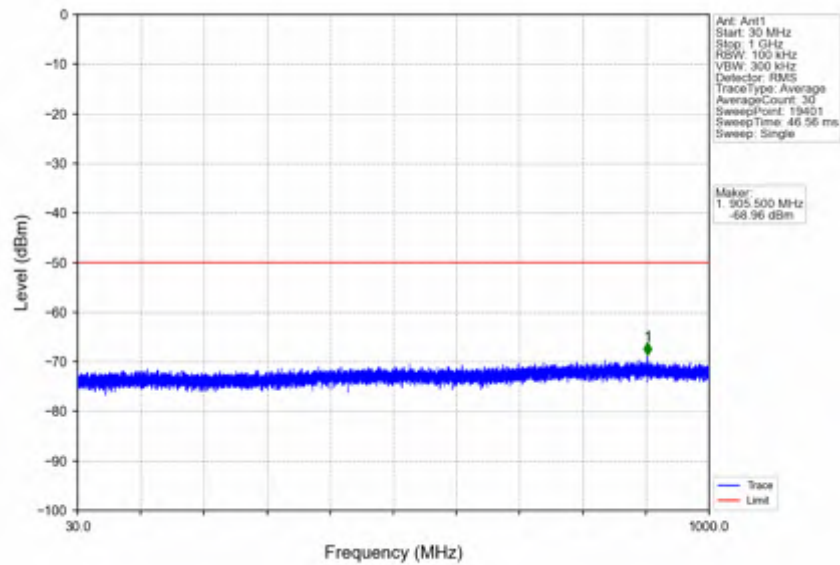
n78d_15kHz_SISO_NTNV_40MHz_DFT-s-OFDM PI/2 BPSK_3679.995MHz_Outer_Full
