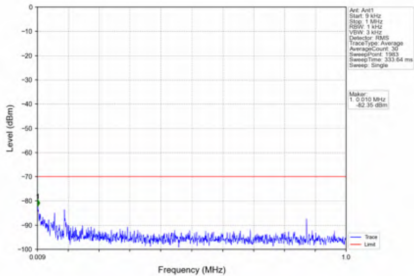
n78d_15kHz_SISO_NTV_40MHz_DFT-s-OFDM_QPSK_3679.995MHz_Edge_1RB_Right
