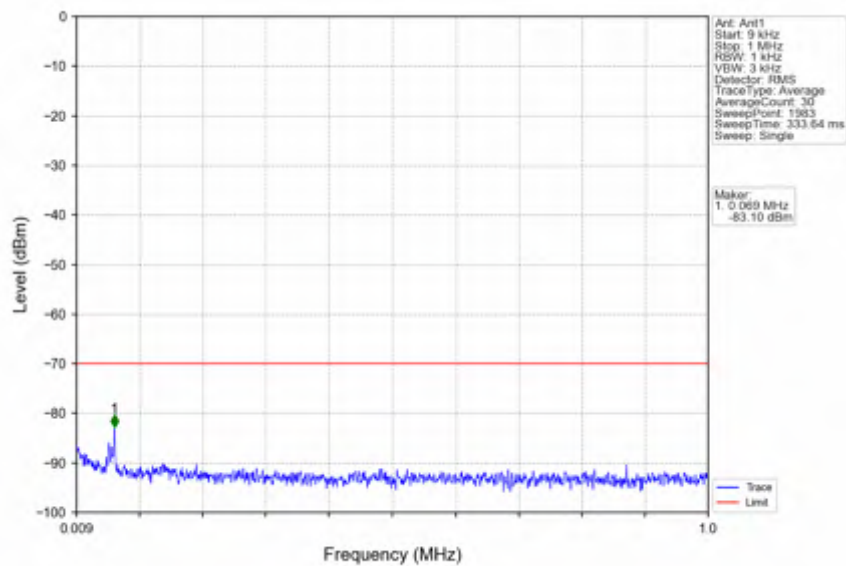
n78d_15kHz_SISO_NTNV_30MHz_DFT-s-OFDM PI/2 BPSK_3565.005MHz_Edge_1RB_Left
