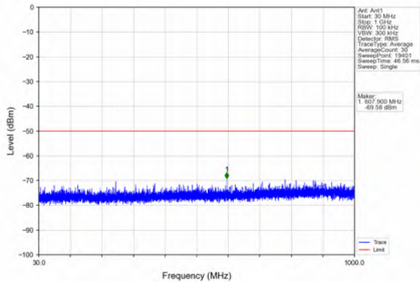
n78d_15kHz_SISO_NTVV_40MHz_DFT-s-OFDM_QPSK_3570MHz_Inner_1RB_Left
