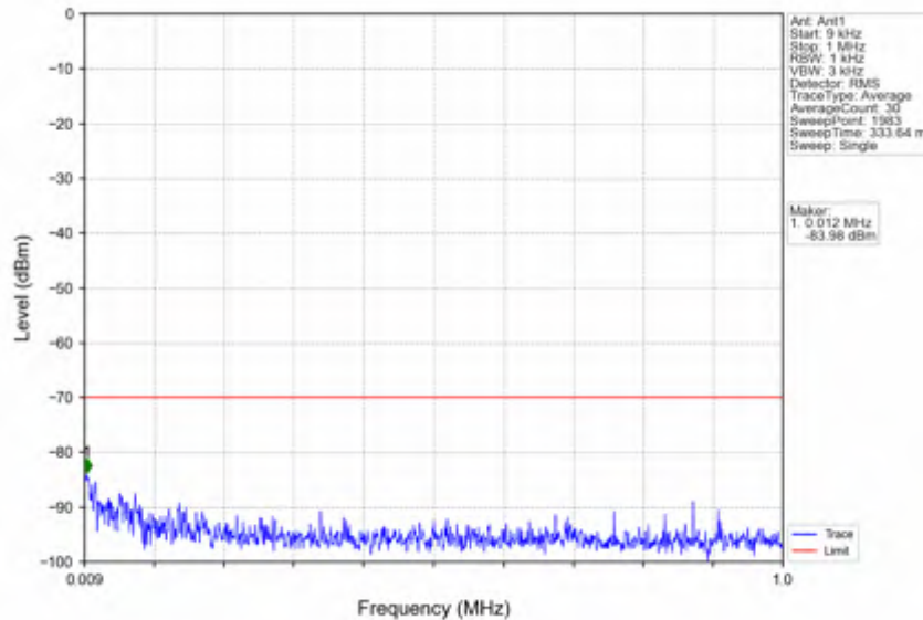
n78d_15kHz_SISO_NTNV_30MHz_DFT-s-OFDM QPSK_3625.005MHz_Edge_1RB_Left
