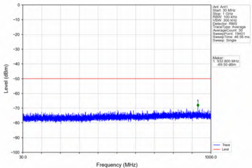
n78d_15kHz_SISO_NTNV_40MHz_CP-OFDM QPSK_3679.995MHz_Edge_1RB_Right
