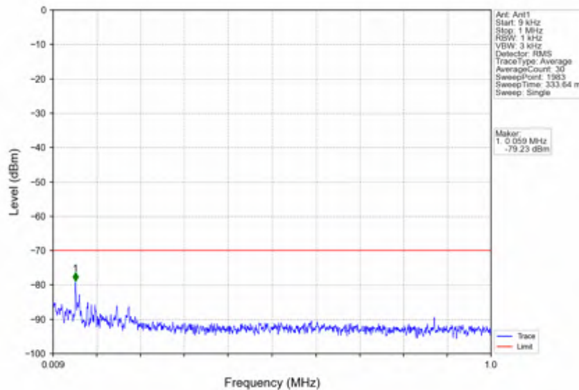
n78d_15kHz_SISO_NTV_50MHz_CP-OFDM QPSK_3575.01MHz_Edge_1RB_Left
