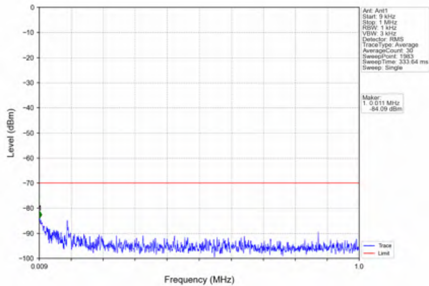
n78d_15kHz_SISO_NTNV_50MHz_DFT-s-OFDM QPSK_3675MHz_Inner_1RB_Right
