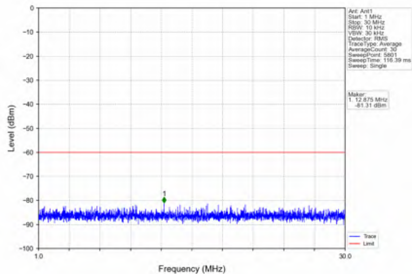
n78d_15kHz_SISO_NTNV_25MHz_CP-OFDM QPSK_3562.5MHz_Outer_Full
