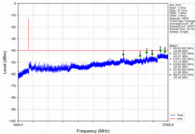
n78d_15kHz_SISO_NTV_50MHz_CP-OFDM QPSK_3625.005MHz_Edge_1RB_Left
