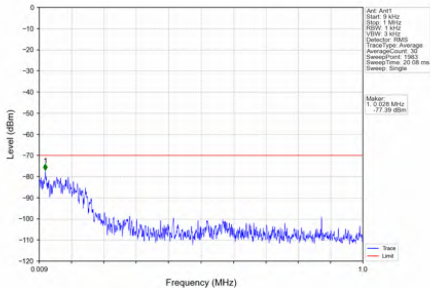
n78d_15kHz_SISO_NTV_50MHz_CP-OFDM QPSK_3575.01MHz_Inner_1RB_Left
