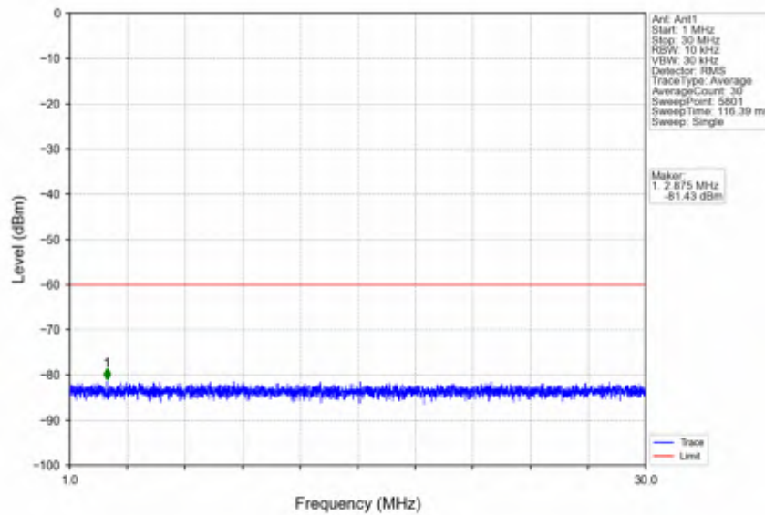
n78d_15kHz_SISO_NTNV_30MHz_DFT-s-OFDM PI/2 BPSK_3684.99MHz_Inner_1RB_Right
