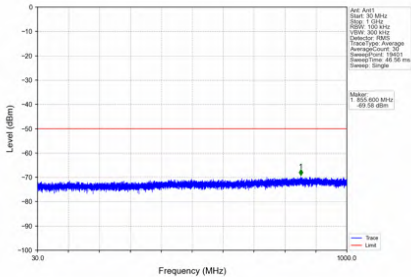
n78d_15kHz_SISO_NTNV_50MHz_DFT-s-OFDM_QPSK_3575.01MHz_Edge_1RB_Left
