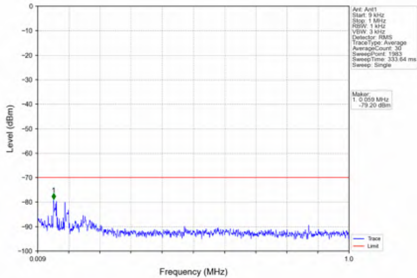
n78d_15kHz_SISO_NTV_40MHz_DFT-s-OFDM_QPSK_3570MHz_Edge_1RB_Left
