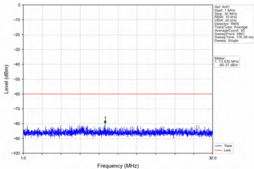
n78d_15kHz_SISO_NTNV_50MHz_DFT-s-OFDM QPSK_3575.01MHz_Inner_1RB_Left
