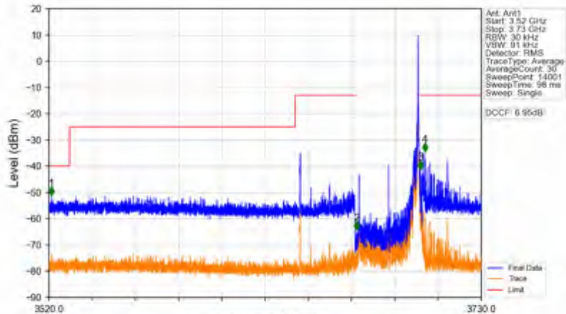
n78d_15kHz_SISO_NTNV_30MHz_DFT-s-OFDM QPSK_3684.99MHz_Edge_1RB_Right
