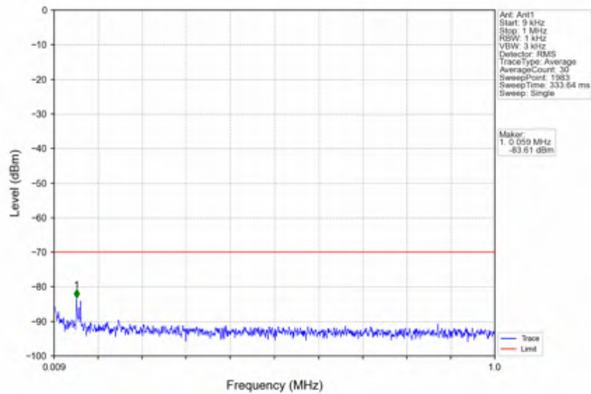
n78d_15kHz_SISO_NTNV_30MHz_DFT-s-OFDM PI/2 BPSK_3565.005MHz_Outer_Full
