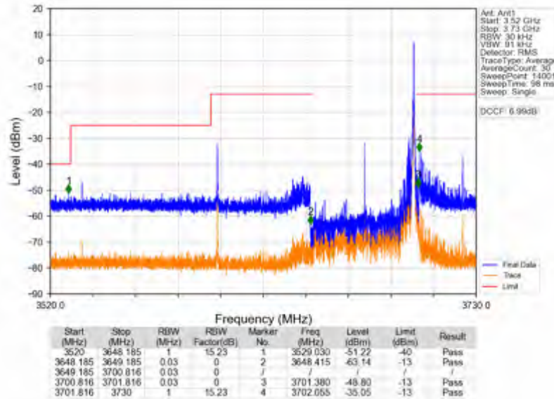
n78d_15kHz_SISO_NTNV_50MHz_CP-OFDM QPSK_3675MHz_Edge_1RB_Right
