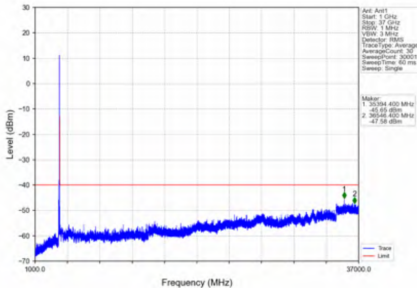
n78d_15kHz_SISO_NTV_40MHz_DFT-s-OFDM_QPSK_3679.995MHz_Edge_1RB_Right
