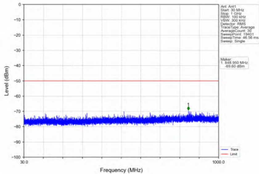
n78d_15kHz_SISO_NTNV_30MHz_DFT-s-OFDM QPSK_3565.005MHz_Inner_1RB_Left
