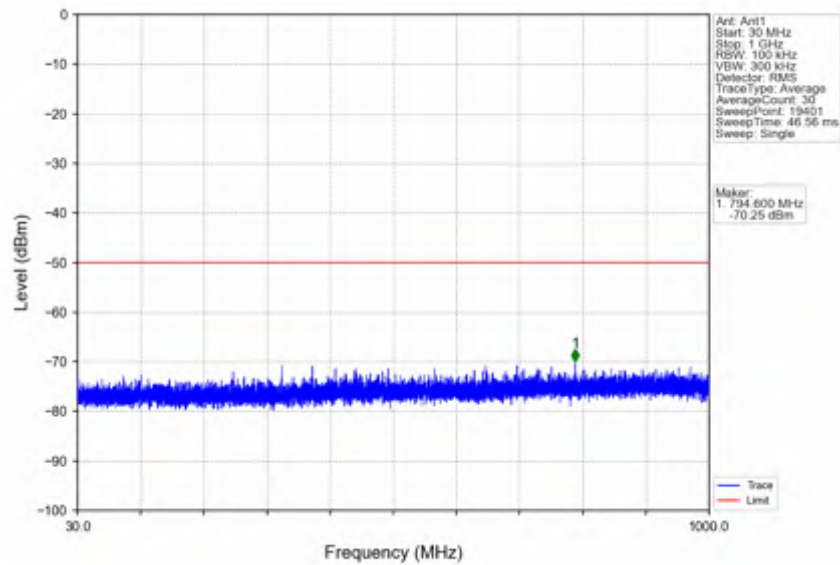
n78d_15kHz_SISO_NTNV_40MHz_CP-OFDM QPSK_3679.995MHz_Outer_Full
