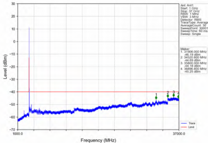
n78d_15kHz_SISO_NTVV_40MHz_DFT-s-OFDM_QPSK_3570MHz_Edge_1RB_Left
