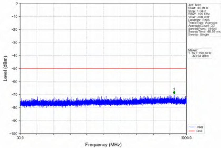
n78d_15kHz_SISO_NTV_25MHz_DFT-s-OFDM QPSK_3687.495MHz_Inner_1RB_Right
