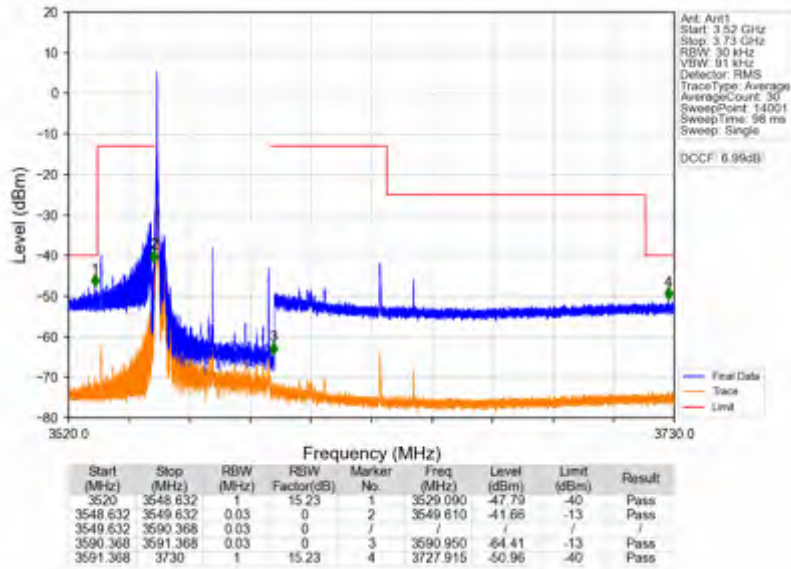
n78d_15kHz_SISO_NTNV_40MHz_DFT-s-OFDM QPSK_3570MHz_Edge_1RB_Left
