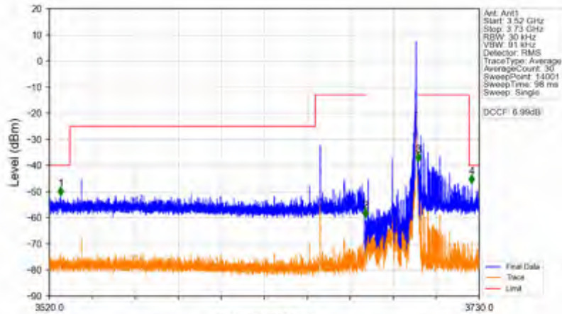
n78d_15kHz_SISO_NTNV_25MHz_DFT-s-OFDM QPSK_3687.495MHz_Inner_1RB_Right
