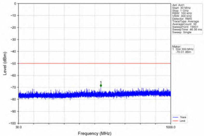
n78d_15kHz_SISO_NTNV_50MHz_DFT-s-OFDM QPSK_3625.005MHz_Edge_1RB_Left
