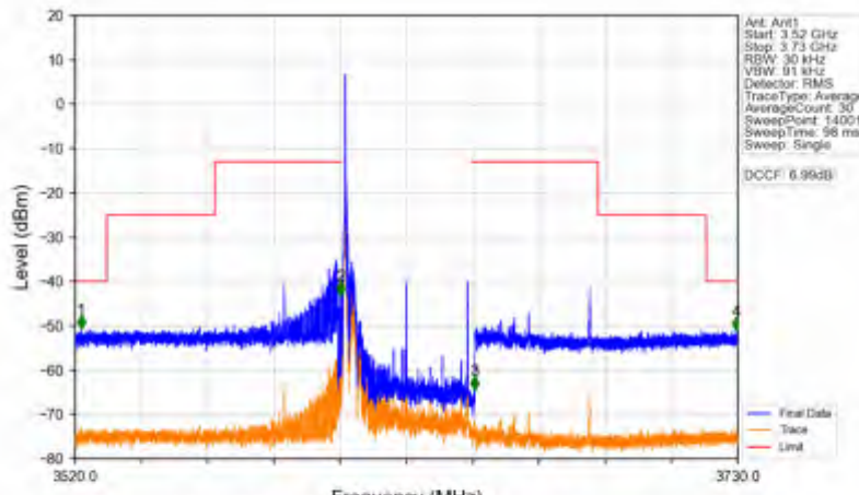
n78d_15kHz_SISO_NTNV_40MHz_DFT-s-OFDM PI/2 BPSK_3625.005MHz_Edge_1RB_Left
