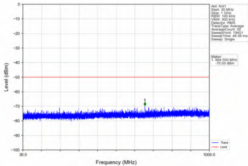
n78d_15kHz_SISO_NTNV_50MHz_CP-OFDM QPSK_3575.01MHz_Outer_Full
