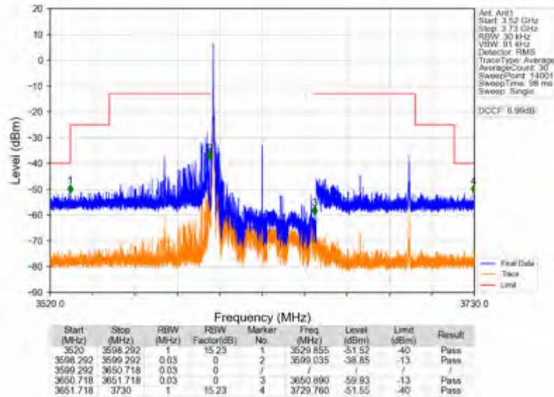
n78d_15kHz_SISO_NTV_50MHz_CP-OFDM QPSK_3625.005MHz_Edge_1RB_Left
