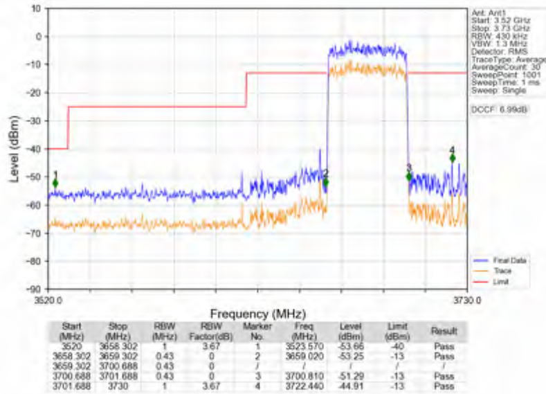
n78d_15kHz_SISO_NTNV_40MHz_DFT-s-OFDM QPSK_3679.995MHz_Outer_Full
