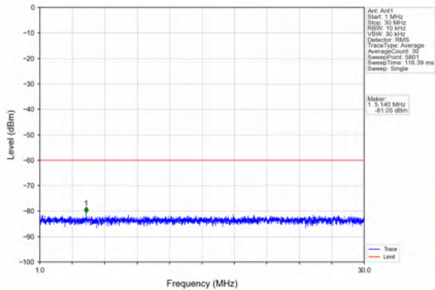
n78d_15kHz_SISO_NTV_50MHz_DFT-s-OFDM PI/2 BPSK_3675MHz_Inner_1RB_Right
