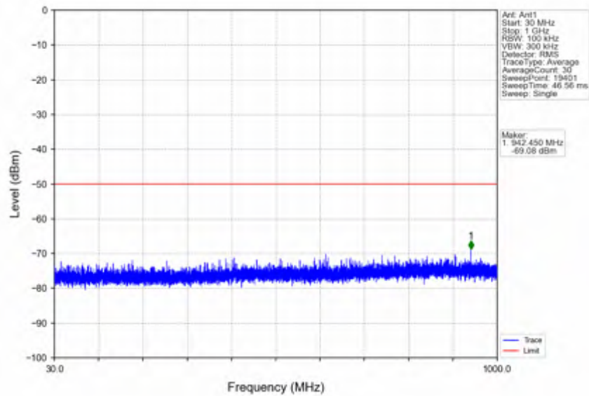
n78d_15kHz_SISO_NTNV_30MHz_CP-OFDM QPSK_3625.005MHz_Edge_1RB_Left
