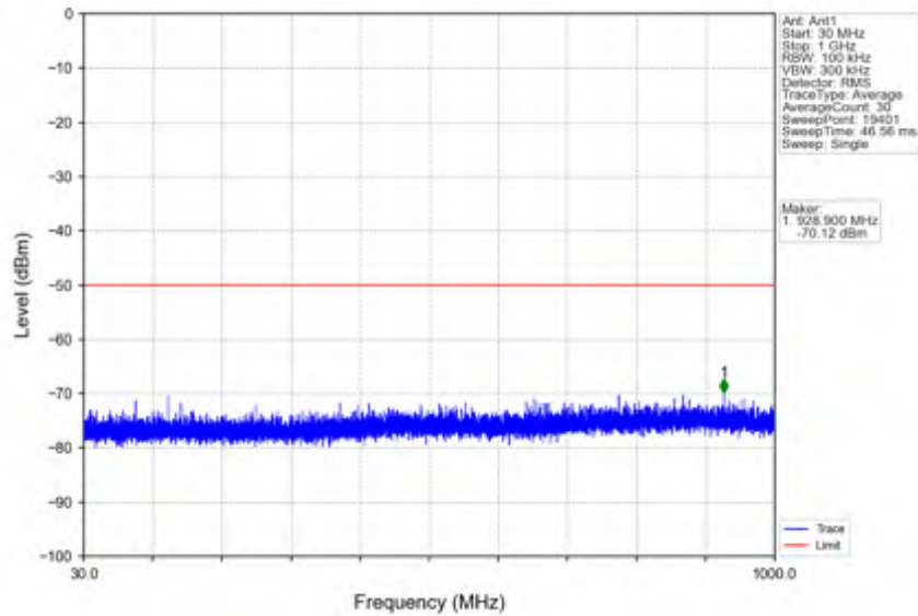
n78d_15kHz_SISO_NTV_40MHz_DFT-s-OFDM_QPSK_3679.995MHz_Edge_1RB_Right
