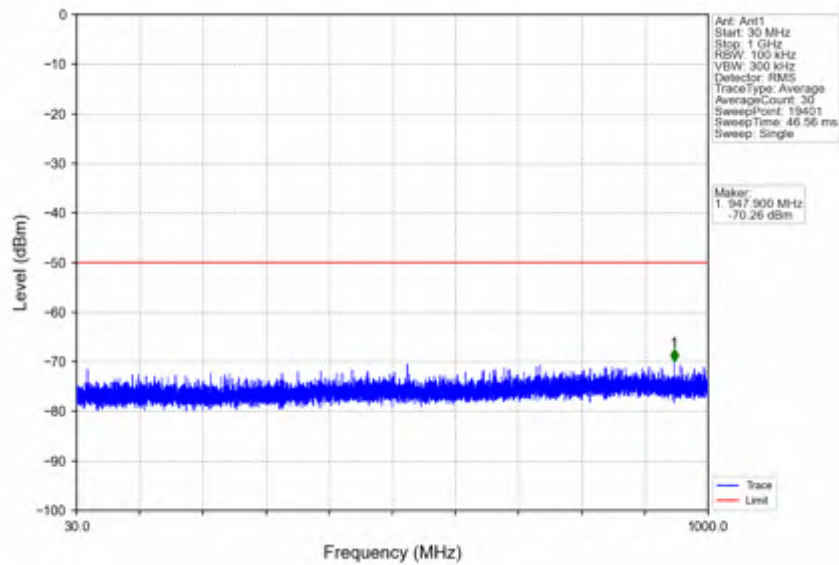
n78d_15kHz_SISO_NTNV_30MHz_DFT-s-OFDM QPSK_3565.005MHz_Edge_1RB_Left
