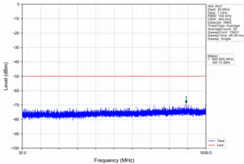
n78d_15kHz_SISO_NTNV_50MHz_CP-OFDM QPSK_3625.005MHz_Edge_1RB_Left
