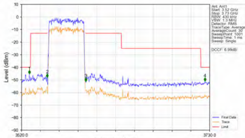
n78d_15kHz_SISO_NTNV_40MHz_DFT-s-OFDM PI/2 BPSK_3570MHz_Outer_Full
