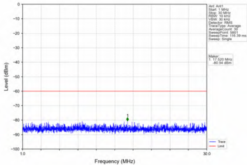
n78d_15kHz_SISO_NTNV_25MHz_DFT-s-OFDM QPSK_3687.495MHz_Outer_Full
