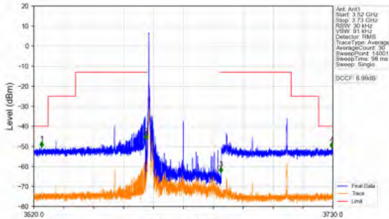
n78d_15kHz_SISO_NTNV_50MHz_DFT-s-OFDM PI/2 BPSK_3625.005MHz_Edge_1RB_Left
