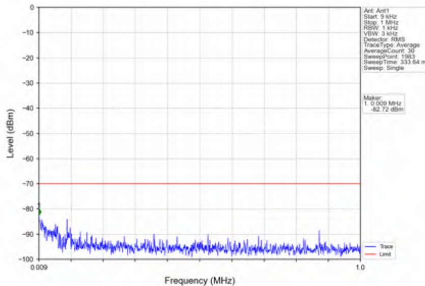
n78d_15kHz_SISO_NTV_30MHz_CP-OFDM QPSK_3684.99MHz_Inner_1RB_Right
