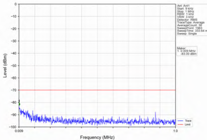
n78d_15kHz_SISO_NTNV_30MHz_CP-OFDM QPSK_3565.005MHz_Inner_1RB_Left
