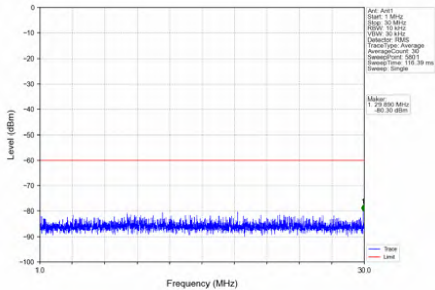
n78d_15kHz_SISO_NTNV_30MHz_CP-OFDM QPSK_3684.99MHz_Inner_1RB_Right
