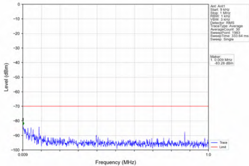
n78d_15kHz_SISO_NTNV_50MHz_CP-OFDM QPSK_3625.005MHz_Edge_1RB_Left
