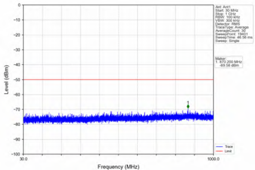
n78d_15kHz_SISO_NTNV_30MHz_DFT-s-OFDM QPSK_3565.005MHz_Outer_Full
