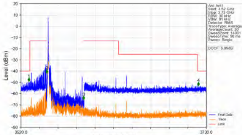
n78d_15kHz_SISO_NTNV_40MHz_DFT-s-OFDM QPSK_3570MHz_Inner_1RB_Left
