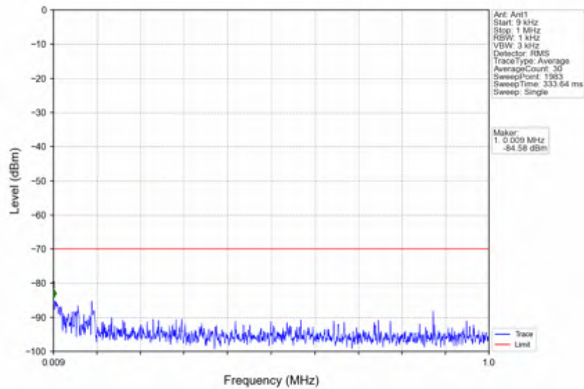
n78d_15kHz_SISO_NTNV_30MHz_CP-OFDM QPSK_3684.99MHz_Outer_Full
