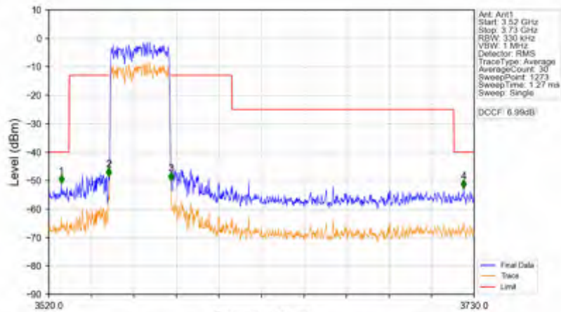
n78d_15kHz_SISO_NTNV_30MHz_CP-OFDM QPSK_3565.005MHz_Outer_Full
