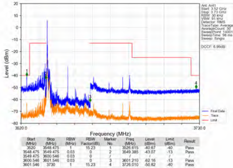
n78d_15kHz_SISO_NTV_50MHz_CP-OFDM QPSK_3575.01MHz_Edge_1RB_Left
