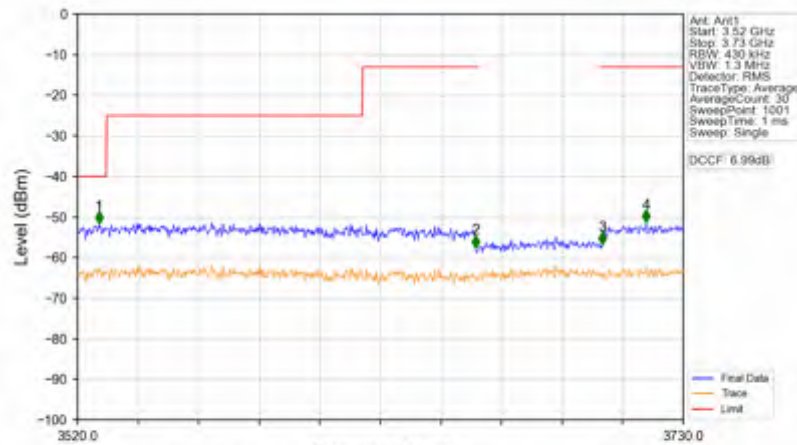
n78d_15kHz_SISO_NTNV_40MHz_DFT-s-OFDM PI/2 BPSK_3679.995MHz_Outer_Full
