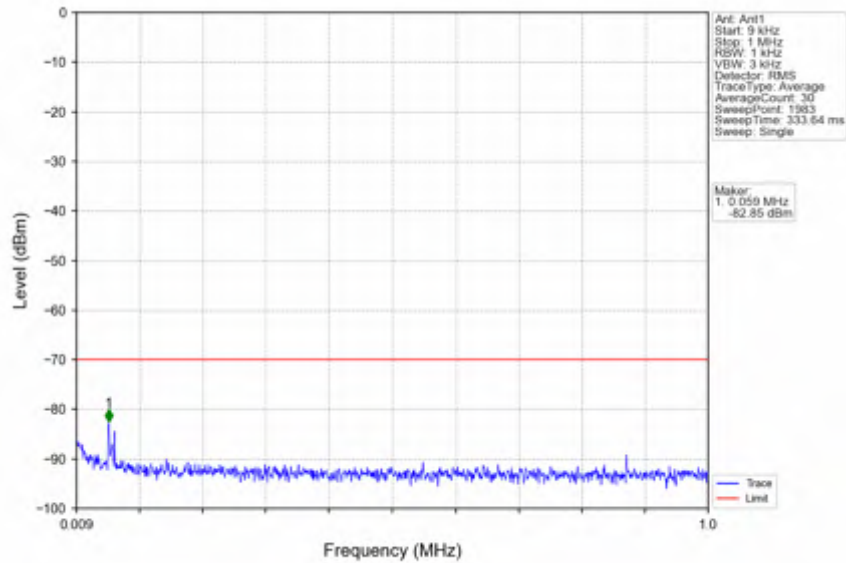
n78d_15kHz_SISO_NTNV_50MHz_DFT-s-OFDM PI/2 BPSK_3675MHz_Outer_Full
