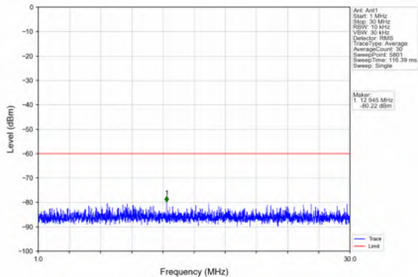
n78d_15kHz_SISO_NTNV_50MHz_CP-OFDM QPSK_3575.01MHz_Outer_Full
