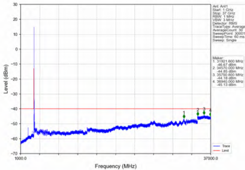
n78d_15kHz_SISO_NTV_50MHz_CP-OFDM QPSK_3575.01MHz_Outer_Full
