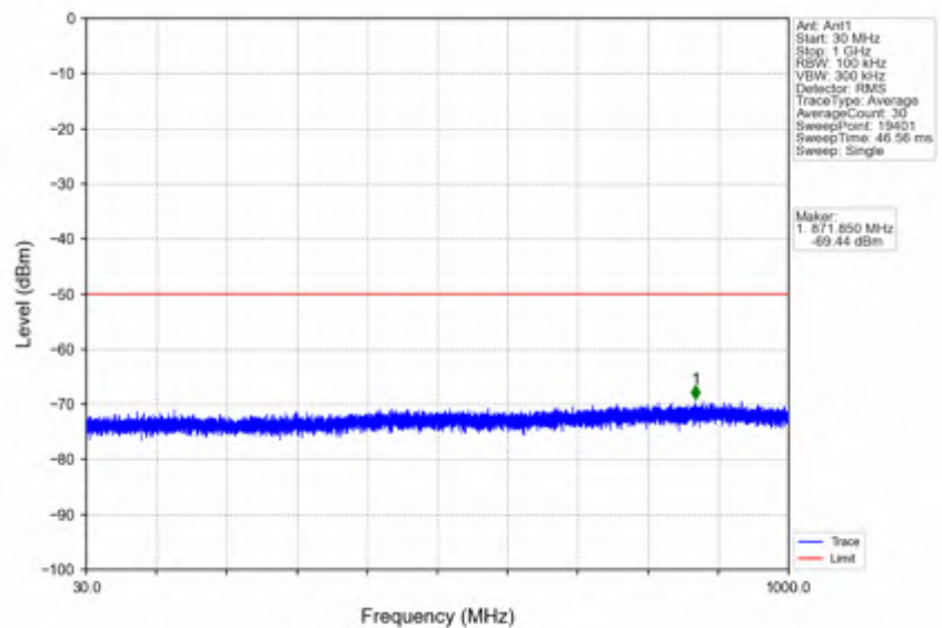
n78d_15kHz_SISO_NTV_50MHz_DFT-s-OFDM PI/2 BPSK_3675MHz_Edge_1RB_Right
