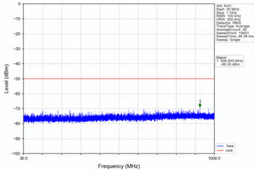
n78d_15kHz_SISO_NTV_40MHz_DFT-s-OFDM_QPSK_3679.995MHz_Inner_1RB_Right
