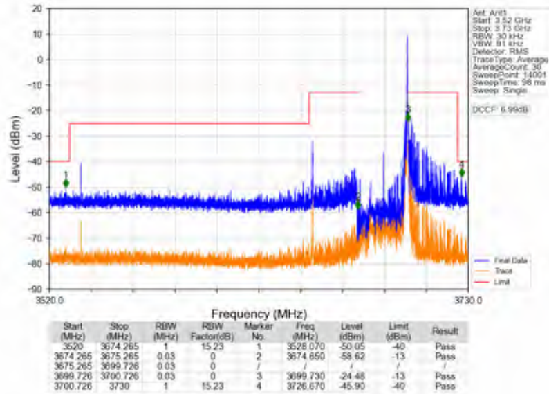
n78d_15kHz_SISO_NTV_25MHz_CP-OFDM QPSK_3687.495MHz_Edge_1RB_Right
