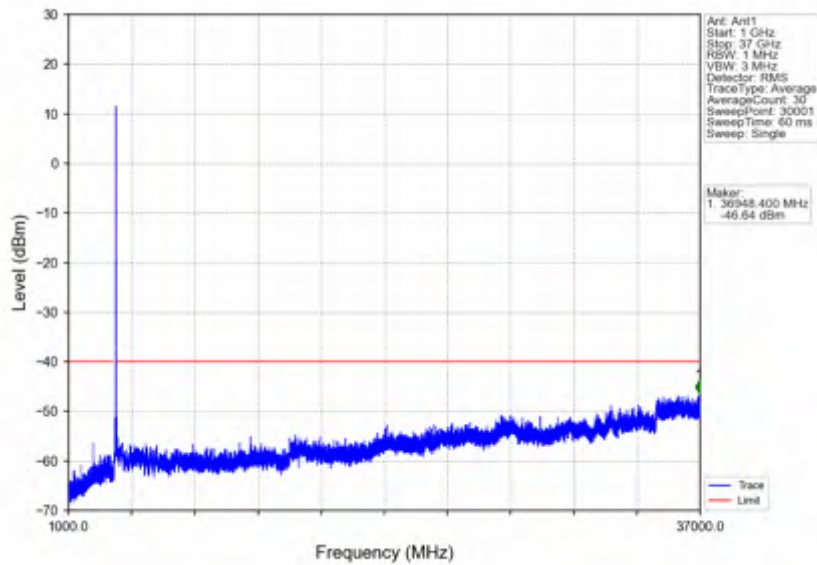
n78d_15kHz_SISO_NTV_25MHz_CP-OFDM QPSK_3687.495MHz_Outer_Full
