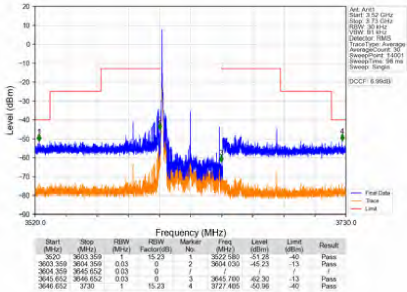
n78d_15kHz_SISO_NTNV_40MHz_CP-OFDM QPSK_3625.005MHz_Edge_1RB_Left
