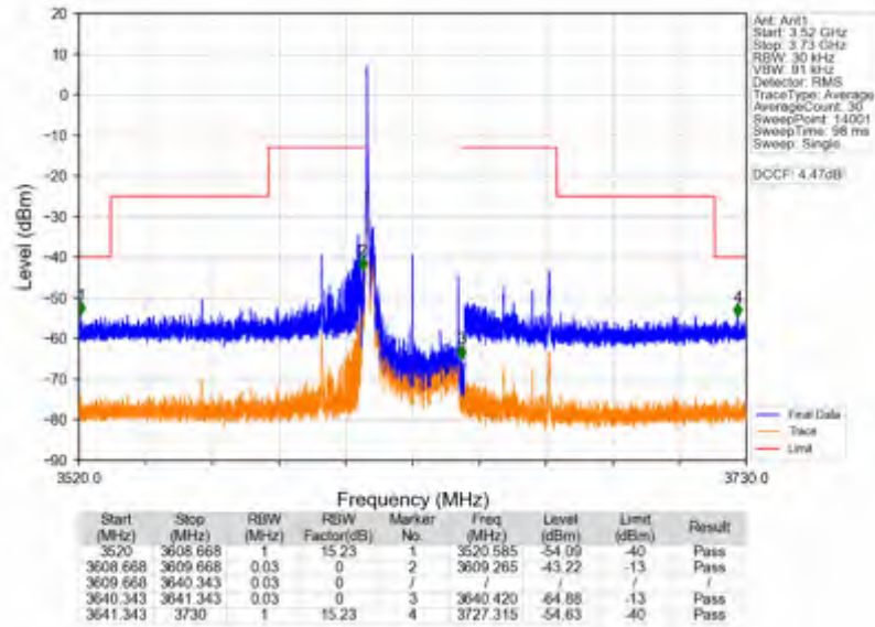
n78d_15kHz_SISO_NTNV_30MHz_DFT-s-OFDM QPSK_3625.005MHz_Edge_1RB_Left
