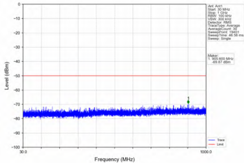
n78d_15kHz_SISO_NTNV_25MHz_CP-OFDM QPSK_3562.5MHz_Outer_Full
