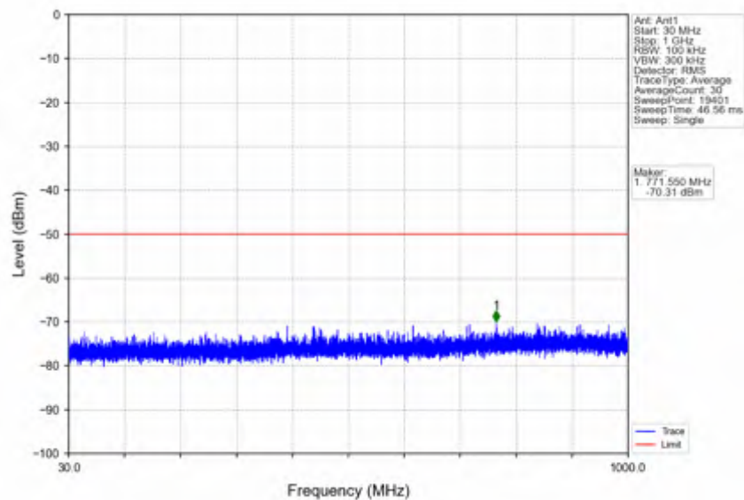
n78d_15kHz_SISO_NTNV_40MHz_DFT-s-OFDM QPSK_3679.995MHz_Outer_Full
