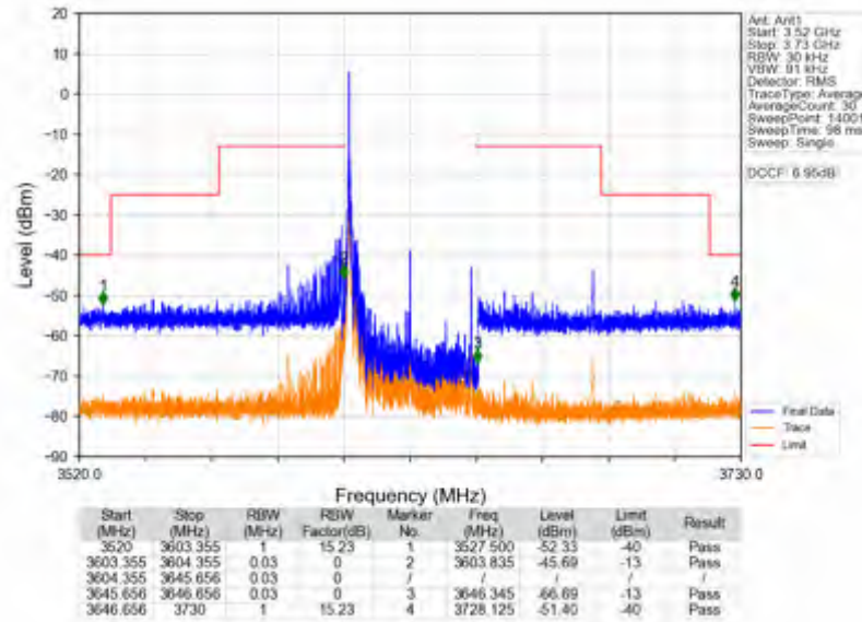
n78d_15kHz_SISO_NTNV_40MHz_DFT-s-OFDM QPSK_3625.005MHz_Edge_1RB_Left
