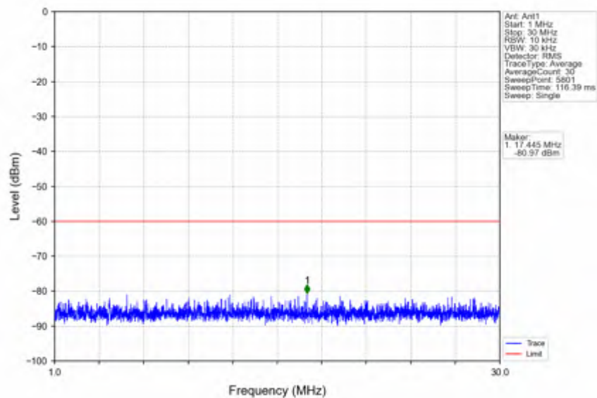
n78d_15kHz_SISO_NTNV_30MHz_CP-OFDM QPSK_3565.005MHz_Outer_Full
