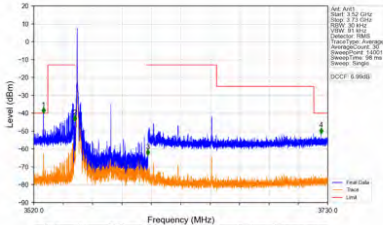
n78d_15kHz_SISO_NTNV_50MHz_DFT-s-OFDM_QPSK_3575.01MHz_Inner_1RB_Left
