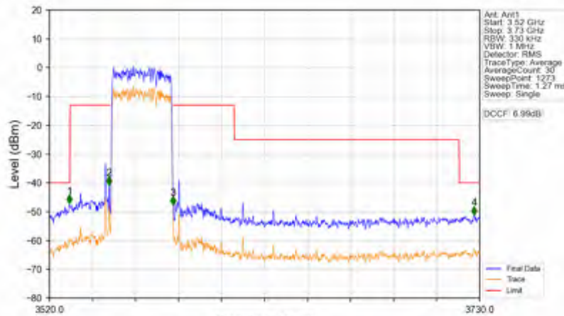
n78d_15kHz_SISO_NTNV_30MHz_DFT-s-OFDM PI/2 BPSK_3565.005MHz_Outer_Full
