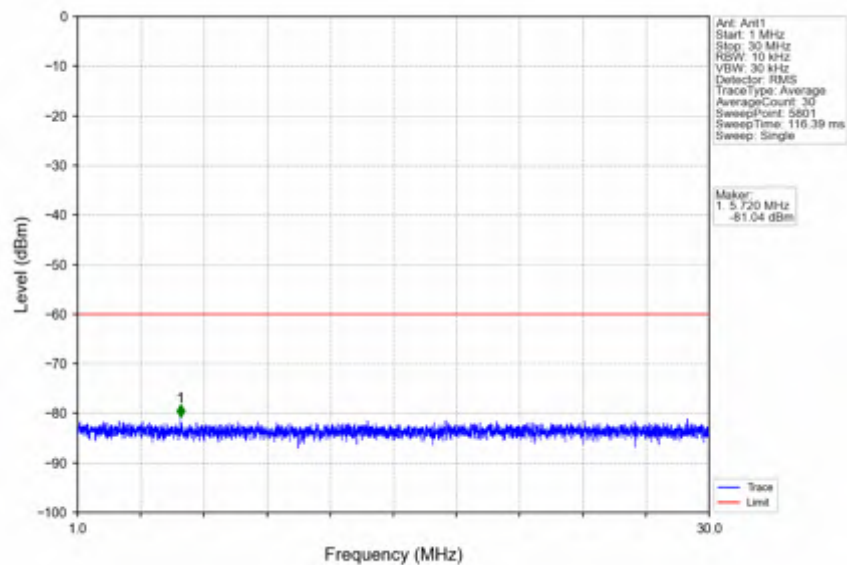
n78d_15kHz_SISO_NTNV_30MHz_DFT-s-OFDM PI/2 BPSK_3625.005MHz_Edge_1RB_Left
