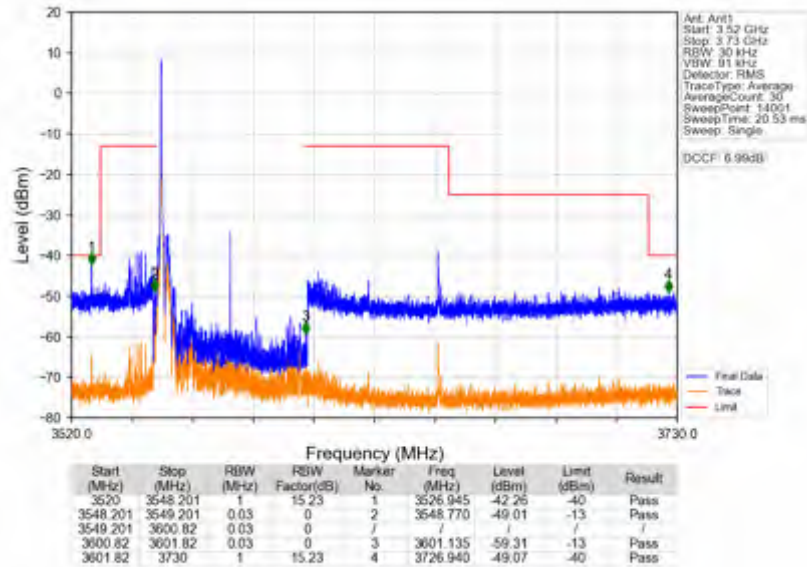
n78d_15kHz_SISO_NTV_50MHz_CP-OFDM QPSK_3575.01MHz_Inner_1RB_Left
