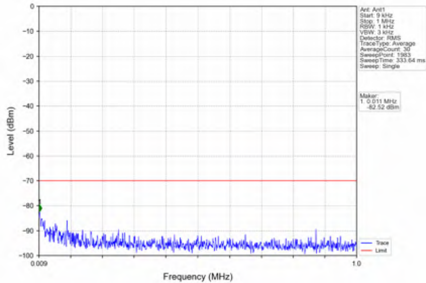
n78d_15kHz_SISO_NTV_40MHz_DFT-s-OFDM QPSK_3679.995MHz_Inner_1RB_Right
