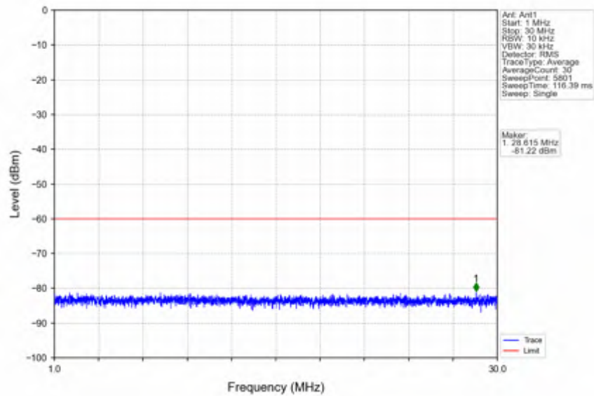
n78d_15kHz_SISO_NTNV_50MHz_DFT-s-OFDM PI/2 BPSK_3575.01MHz_Inner_1RB_Left
