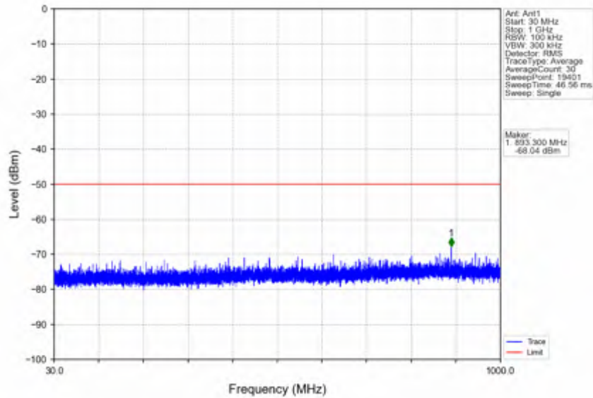
n78d_15kHz_SISO_NTNV_25MHz_DFT-s-OFDM QPSK_3562.5MHz_Inner_1RB_Left
