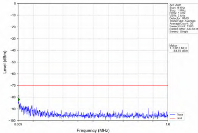
n78d_15kHz_SISO_NTNV_40MHz_CP-OFDM QPSK_3679.995MHz_Edge_1RB_Right
