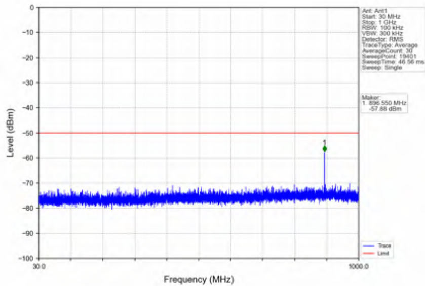
n78d_15kHz_SISO_NTNV_30MHz_DFT-s-OFDM QPSK_3684.99MHz_Inner_1RB_Right
