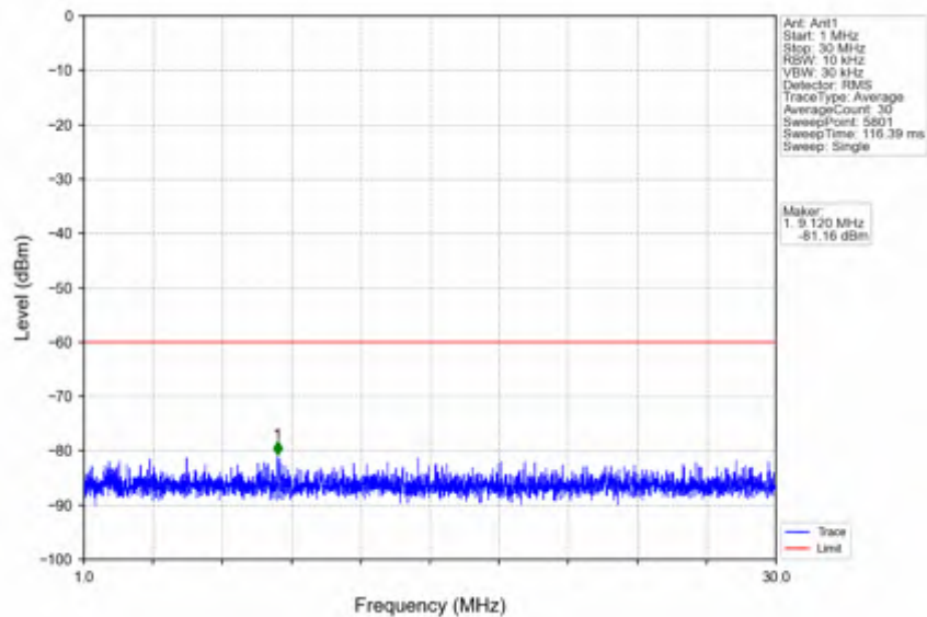
n78d_15kHz_SISO_NTNV_25MHz_DFT-s-OFDM QPSK_3562.5MHz_Inner_1RB_Left
