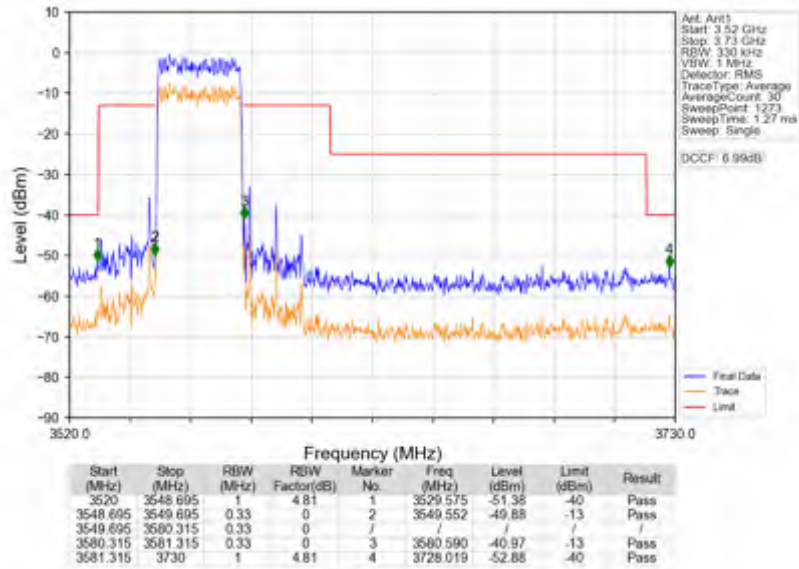
n78d_15kHz_SISO_NTNV_30MHz_DFT-s-OFDM QPSK_3565.005MHz_Outer_Full
