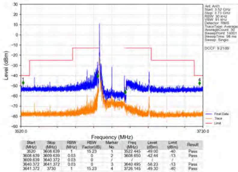
n78d_15kHz_SISO_NTNV_30MHz_CP-OFDM QPSK_3625.005MHz_Edge_1RB_Left
