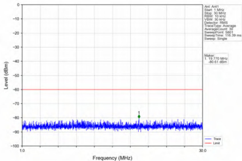
n78d_15kHz_SISO_NTV_25MHz_DFT-s-OFDM QPSK_3687.495MHz_Inner_1RB_Right
