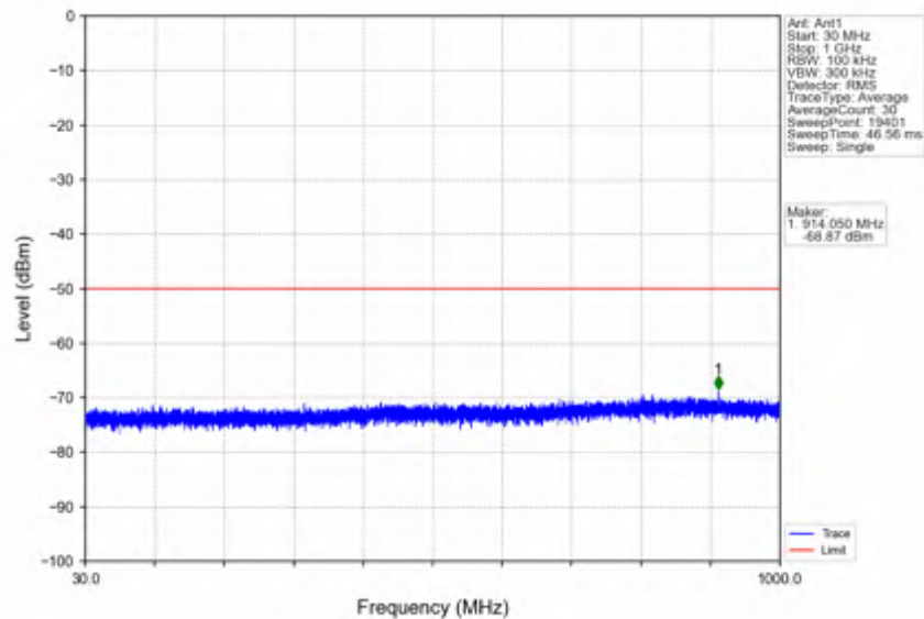
n78d_15kHz_SISO_NTNV_30MHz_DFT-s-OFDM PI/2 BPSK_3684.99MHz_Edge_1RB_Right
