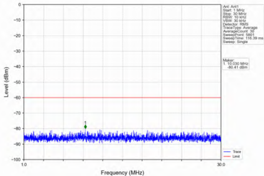
n78d_15kHz_SISO_NTV_25MHz_DFT-s-OFDM_QPSK_3687.495MHz_Edge_1RB_Right
