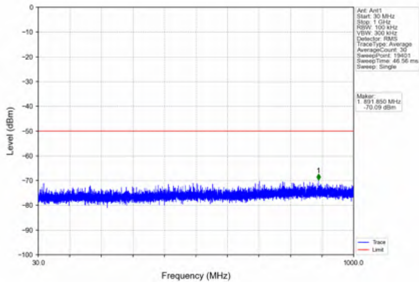
n78d_15kHz_SISO_NTNV_40MHz_CP-OFDM QPSK_3625.005MHz_Edge_1RB_Left
