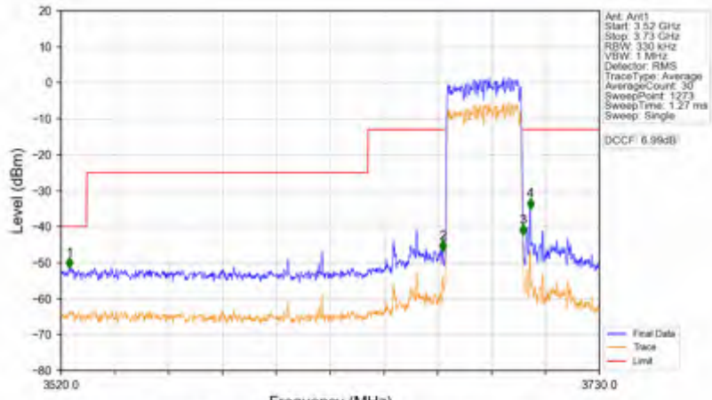
n78d_15kHz_SISO_NTNV_30MHz_DFT-s-OFDM PI/2 BPSK_3684.99MHz_Outer_Full
