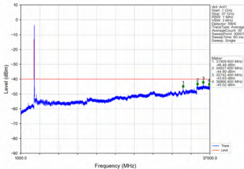
n78d_15kHz_SISO_NTNV_50MHz_DFT-s-OFDM PI/2 BPSK_3575.01MHz_Outer_Full
