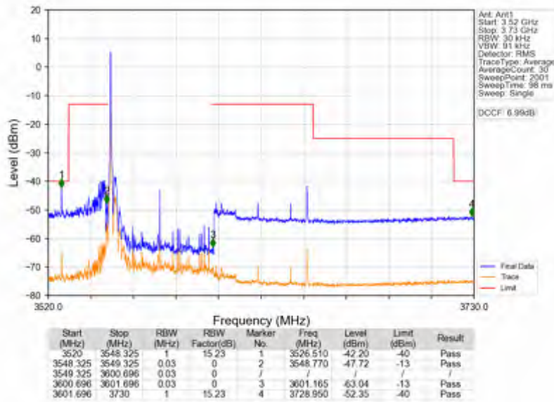
n78d_15kHz_SISO_NTNV_50MHz_DFT-s-OFDM QPSK_3575.01MHz_Edge_1RB_Left
