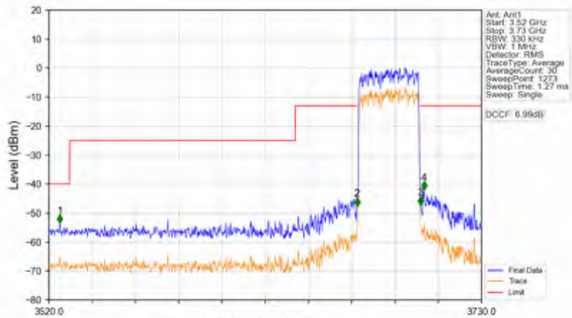
n78d_15kHz_SISO_NTNV_30MHz_CP-OFDM QPSK_3684.99MHz_Outer_Full
