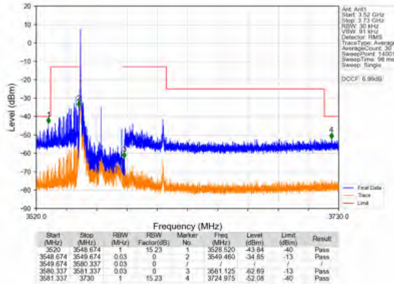
n78d_15kHz_SISO_NTNV_30MHz_CP-OFDM QPSK_3565.005MHz_Edge_1RB_Left
