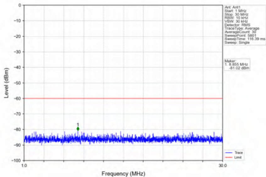
n78d_15kHz_SISO_NTNV_25MHz_CP-OFDM QPSK_3625.005MHz_Edge_1RB_Left
