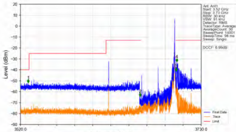
n78d_15kHz_SISO_NTNV_40MHz_DFT-s-OFDM QPSK_3679.995MHz_Inner_1RB_Right
