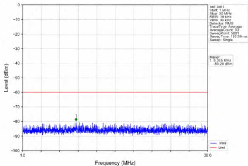
n78d_15kHz_SISO_NTNV_25MHz_CP-OFDM QPSK_3687.495MHz_Outer_Full
