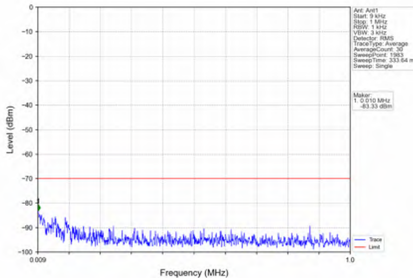
n78d_15kHz_SISO_NTV_25MHz_CP-OFDM QPSK_3687.495MHz_Inner_1RB_Right
