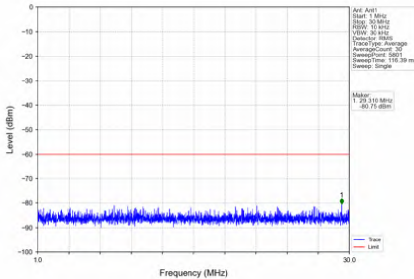
n78d_15kHz_SISO_NTNV_25MHz_DFT-s-OFDM QPSK_3625.005MHz_Edge_1RB_Left
