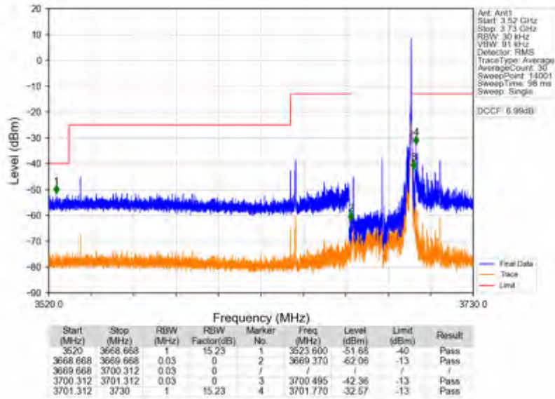
n78d_15kHz_SISO_NTV_30MHz_CP-OFDM QPSK_3684.99MHz_Edge_1RB_Right
