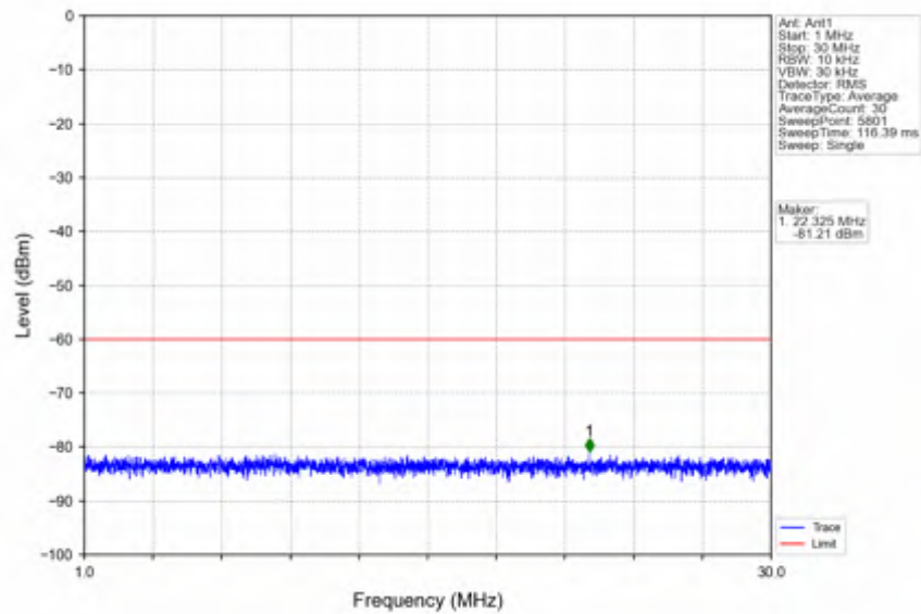
n78d_15kHz_SISO_NTVV_50MHz_CP-OFDM QPSK_3575.01MHz_Edge_1RB_Left
