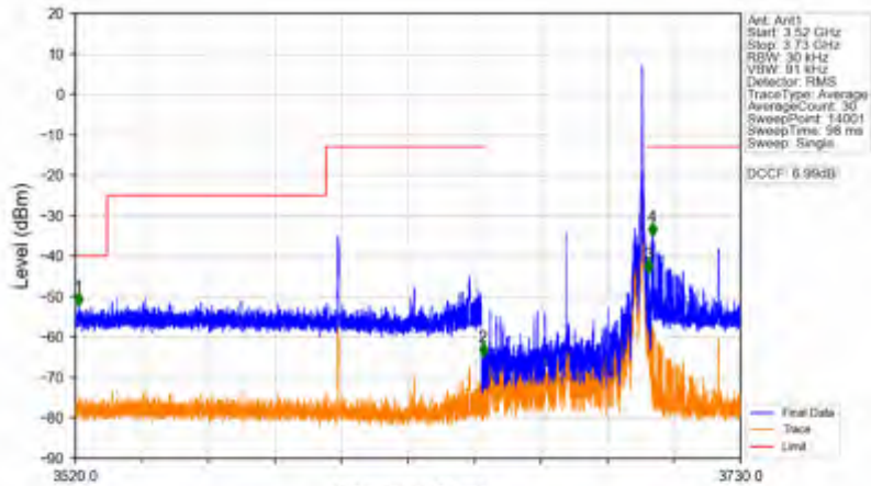
n78d_15kHz_SISO_NTNV_50MHz_DFT-s-OFDM QPSK_3675MHz_Inner_1RB_Right
