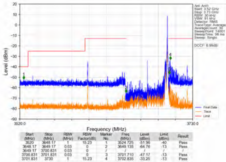
n78d_15kHz_SISO_NTNV_50MHz_DFT-s-OFDM QPSK_3675MHz_Edge_1RB_Right
