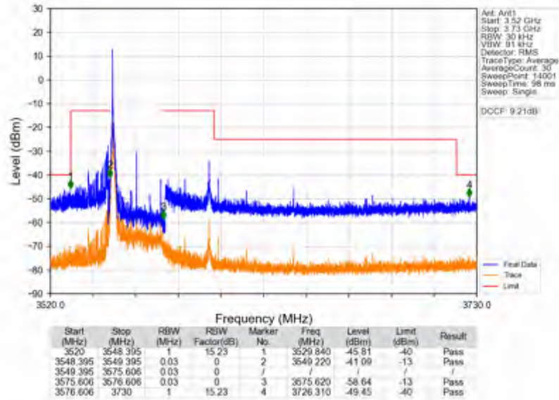
n78d_15kHz_SISO_NTNV_25MHz_CP-OFDM QPSK_3562.5MHz_Edge_1RB_Left
