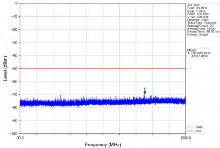
n78d_15kHz_SISO_NTNV_50MHz_DFT-s-OFDM QPSK_3575.01MHz_Inner_1RB_Left
