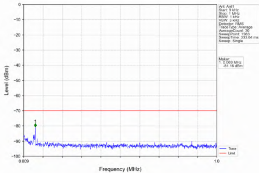
n78d_15kHz_SISO_NTNV_30MHz_DFT-s-OFDM PI/2 BPSK_3684.99MHz_Outer_Full
