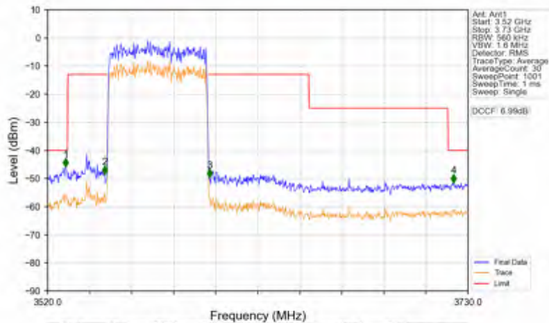
n78d_15kHz_SISO_NTNV_50MHz_DFT-s-OFDM PI/2 BPSK_3575.01MHz_Outer_Full
