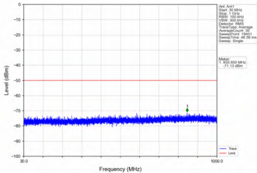
n78d_15kHz_SISO_NTVV_10MHz_DFT-s-OFDM_QPSK_3555MHz_Edge_1RB_Left
