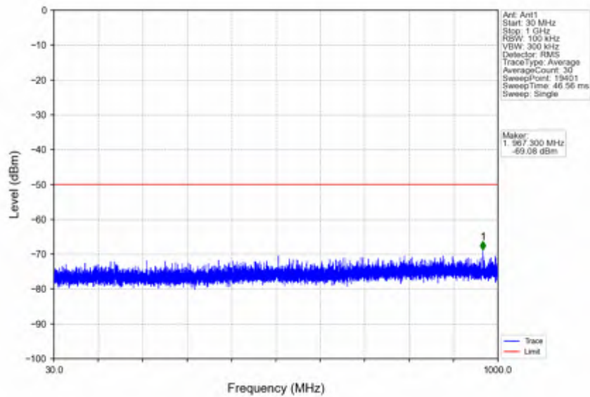
n78d_15kHz_SISO_NTNV_20MHz_DFT-s-OFDM QPSK_3560.01MHz_Inner_1RB_Left
