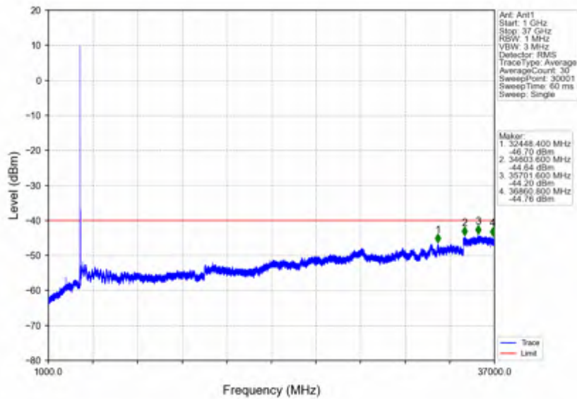
n78d_15kHz_SISO_NTNV_20MHz_DFT-s-OFDM PI/2 BPSK_3560.01MHz_Outer_Full
