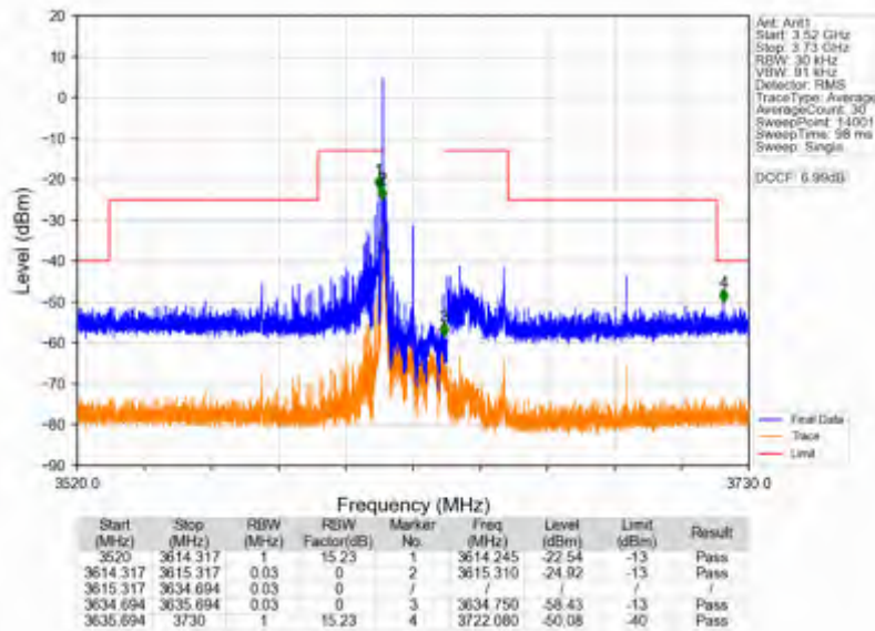
n78d_15kHz_SISO_NTNV_20MHz_CP-OFDM QPSK_3625.005MHz_Edge_1RB_Left
