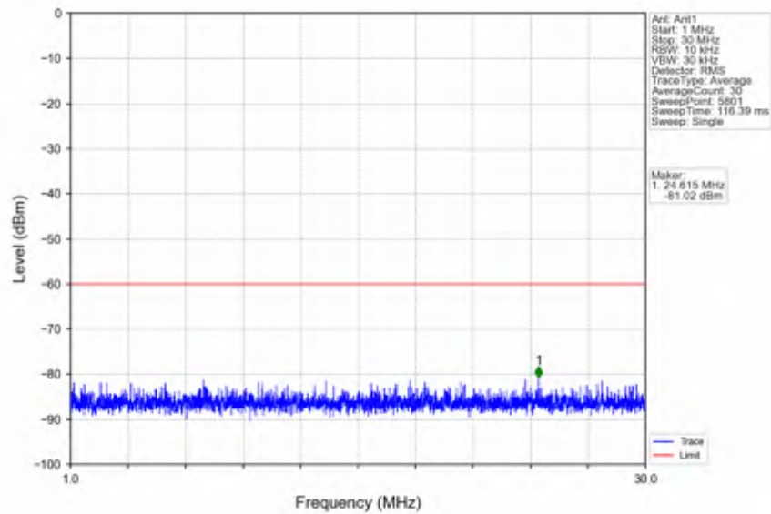
n78d_15kHz_SISO_NTNV_15MHz_CP-OFDM QPSK_3692.49MHz_Inner_1RB_Right
