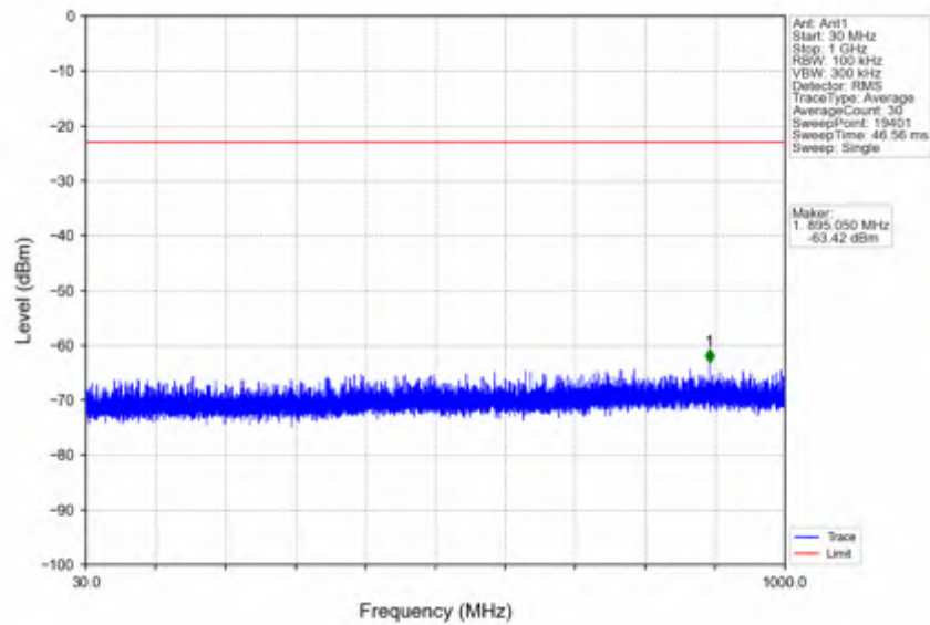
n66_30kHz_SISO_NTNV_40MHz_CP-OFDM QPSK_1745MHz_Edge_1RB_Left
