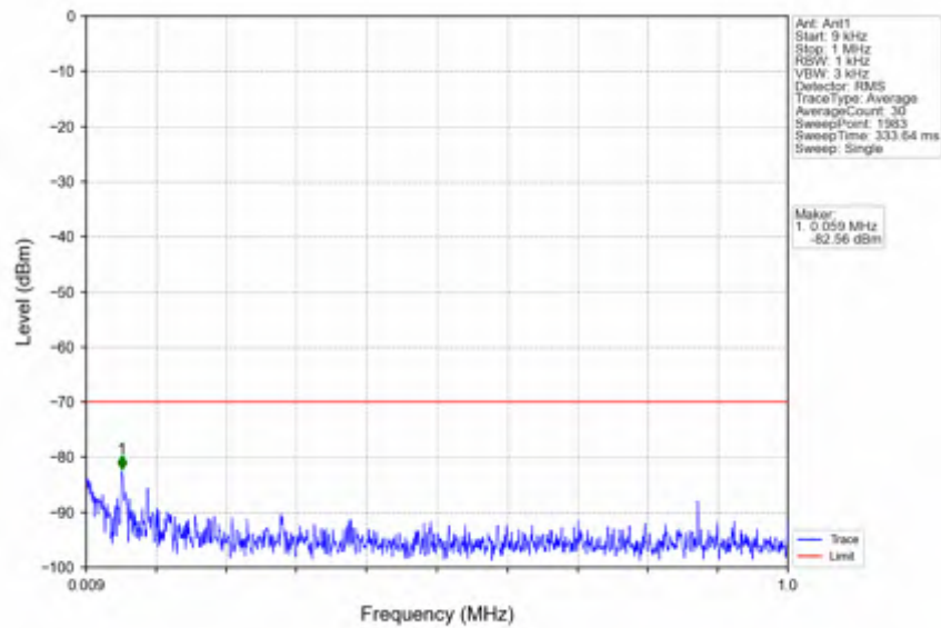
n78d_15kHz_SISO_NTNV_20MHz_DFT-s-OFDM QPSK_3560.01MHz_Edge_1RB_Left
