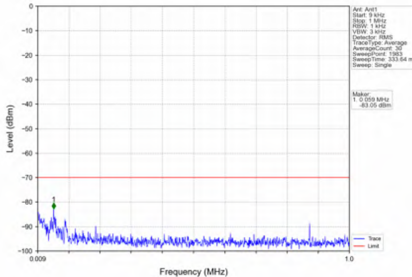
n78d_15kHz_SISO_NTV_10MHz_CP-OFDM QPSK_3694.995MHz_Edge_1RB_Right
