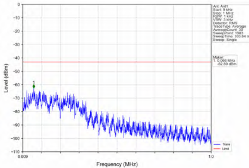
n66_30kHz_SISO_NTV_40MHz_CP-OFDM QPSK_1760MHz_Edge_1RB_Right
