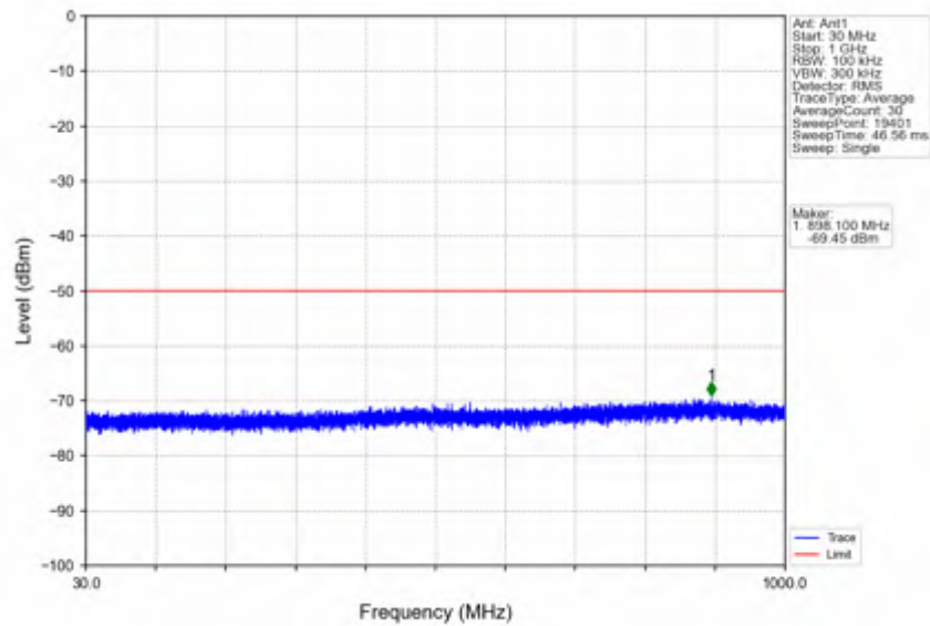
n78d_15kHz_SISO_NTNV_10MHz_DFT-s-OFDM_PI/2_BPSK_3625.005MHz_Edge_1RB_Left
