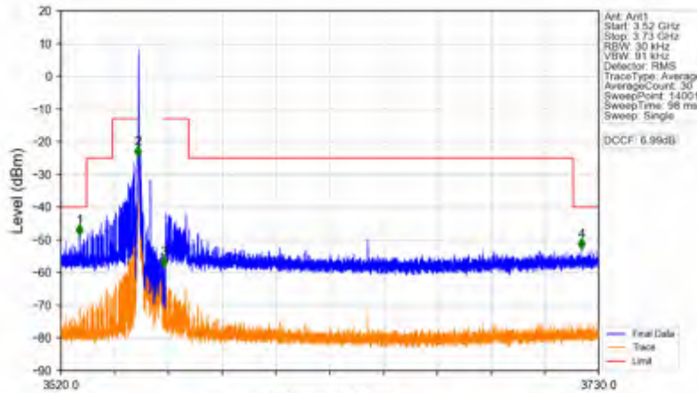
n78d_15kHz_SISO_NTNV_10MHz_DFT-s-OFDM QPSK_3555MHz_Edge_1RB_Left
