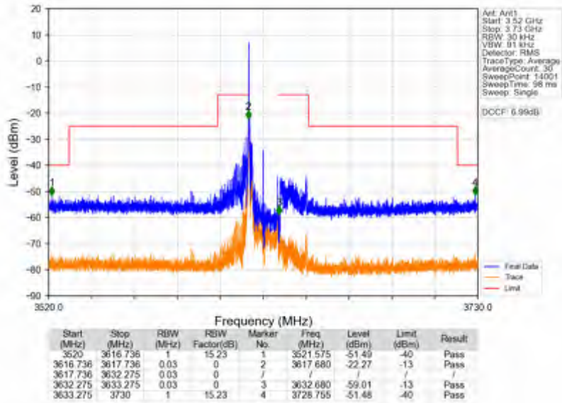
n78d_15kHz_SISO_NTNV_15MHz_CP-OFDM QPSK_3625.005MHz_Edge_1RB_Left
