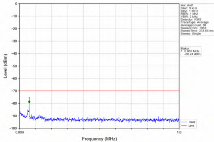
n78d_15kHz_SISO_NTNV_10MHz_DFT-s-OFDM PI/2 BPSK_3625.005MHz_Edge_1RB_Left
