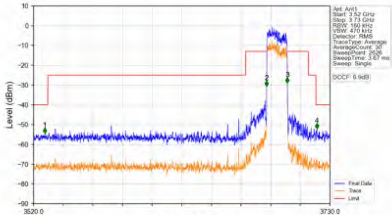
n78d_15kHz_SISO_NTNV_15MHz_CP-OFDM QPSK_3692.49MHz_Outer_Full
