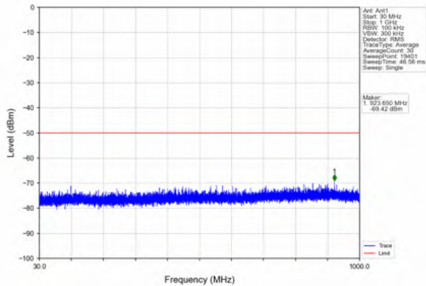
n78d_15kHz_SISO_NTNV_15MHz_CP-OFDM QPSK_3557.505MHz_Outer_Full
