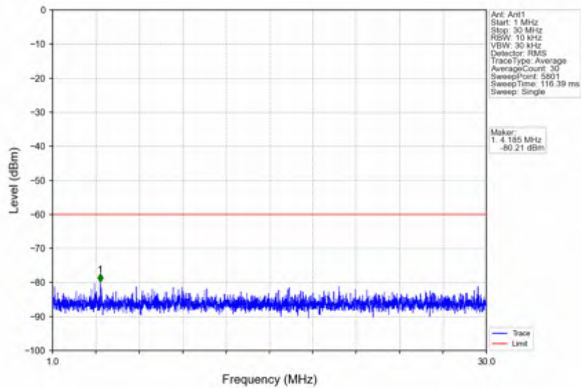
n78d_15kHz_SISO_NTV_20MHz_CP-OFDM QPSK_3560.01MHz_Edge_1RB_Left
