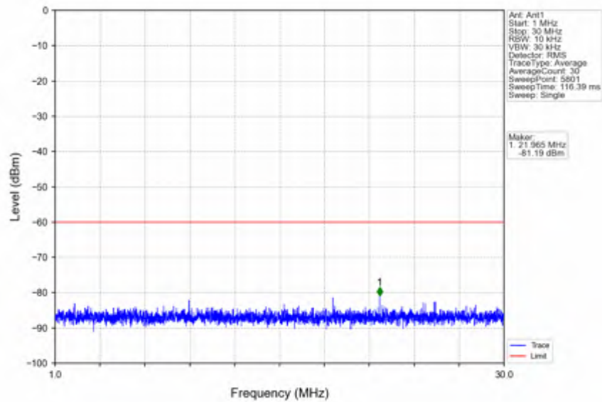
n78d_15kHz_SISO_NTNV_10MHz_CP-OFDM QPSK_3694.995MHz_Inner_1RB_Right
