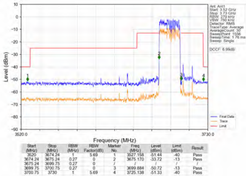
n78d_15kHz_SISO_NTNV_25MHz_DFT-s-OFDM PI/2 BPSK_3687.495MHz_Outer_Full
