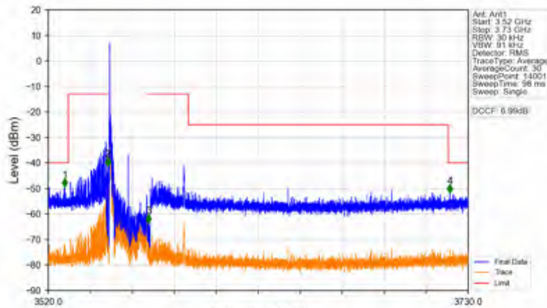
n78d_15kHz_SISO_NTNV_20MHz_DFT-s-OFDM QPSK_3560.01MHz_Inner_1RB_Left
