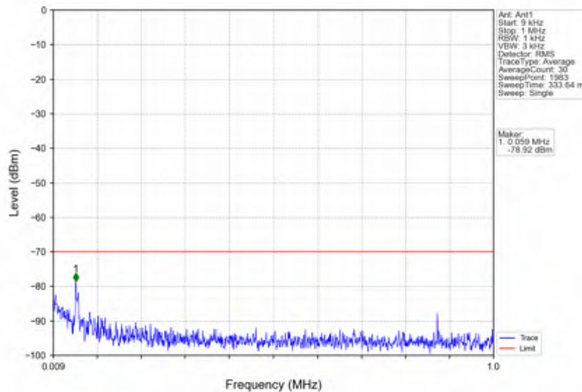
n78d_15kHz_SISO_NTNV_15MHz_CP-OFDM QPSK_3557.505MHz_Edge_1RB_Left
