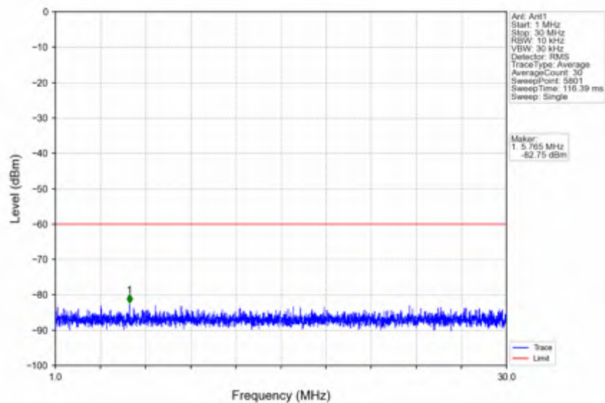
n78d_15kHz_SISO_NTVV_10MHz_DFT-s-OFDM_QPSK_3555MHz_Edge_1RB_Left
