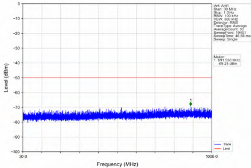
n78d_15kHz_SISO_NTNV_15MHz_DFT-s-OFDM QPSK_3692.49MHz_Inner_1RB_Right
