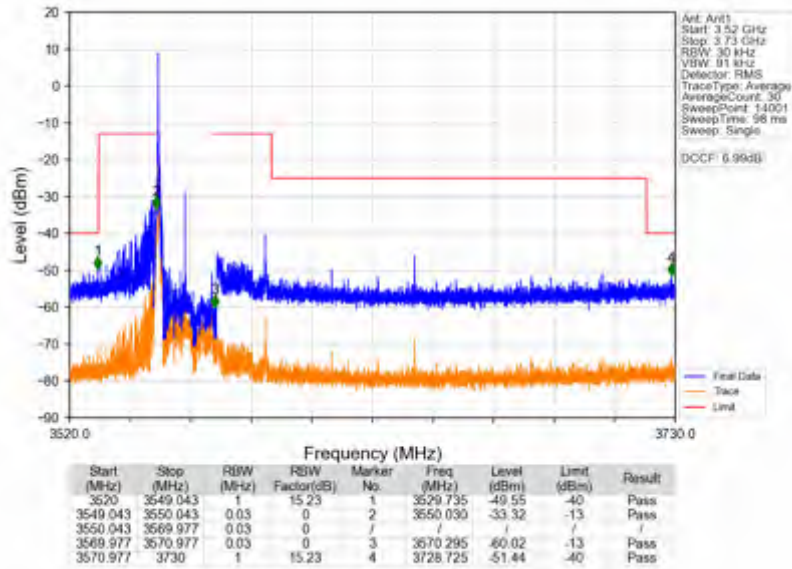
n78d_15kHz_SISO_NTV_20MHz_CP-OFDM_QPSK_3560.01MHz_Inner_1RB_Left
