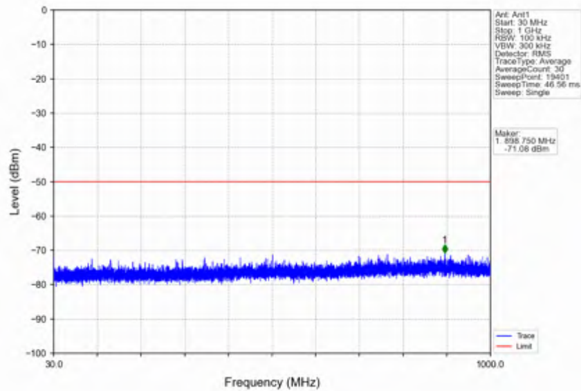
n78d_15kHz_SISO_NTNV_10MHz_CP-OFDM QPSK_3694.995MHz_Outer_Full
