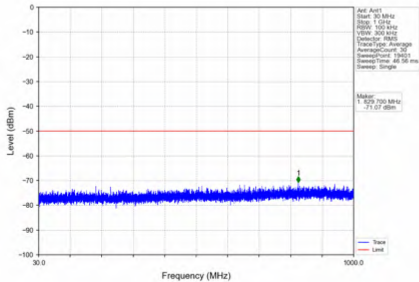
n78d_15kHz_SISO_NTNV_10MHz_CP-OFDM QPSK_3625.005MHz_Edge_1RB_Left
