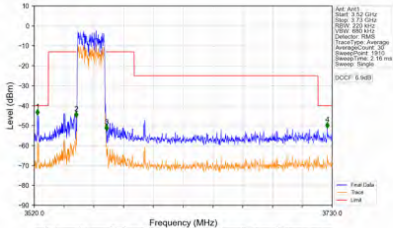
n78d_15kHz_SISO_NTNV_20MHz_CP-OFDM QPSK_3560.01MHz_Outer_Full
