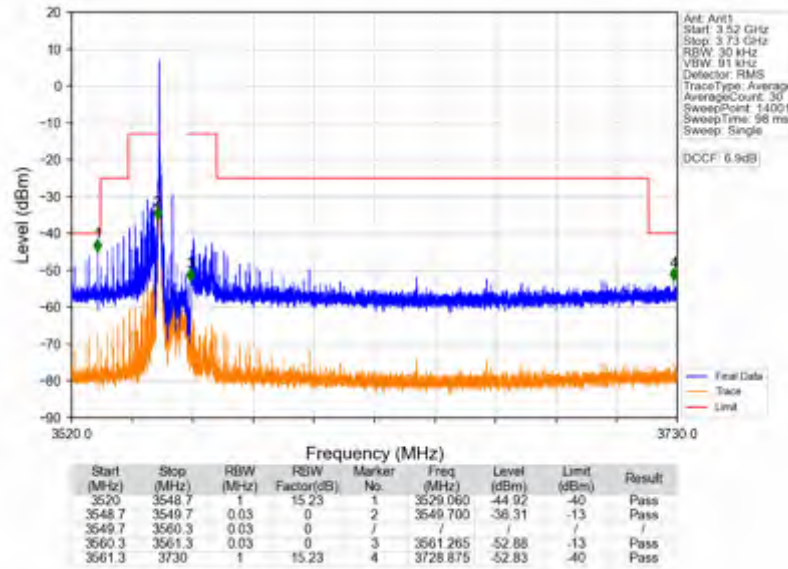
n78d_15kHz_SISO_NTNV_10MHz_CP-OFDM QPSK_3555MHz_Edge_1RB_Left
