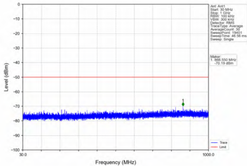
n78d_15kHz_SISO_NTV_10MHz_DFT-s-OFDM QPSK_3694.995MHz_Edge_1RB_Right
