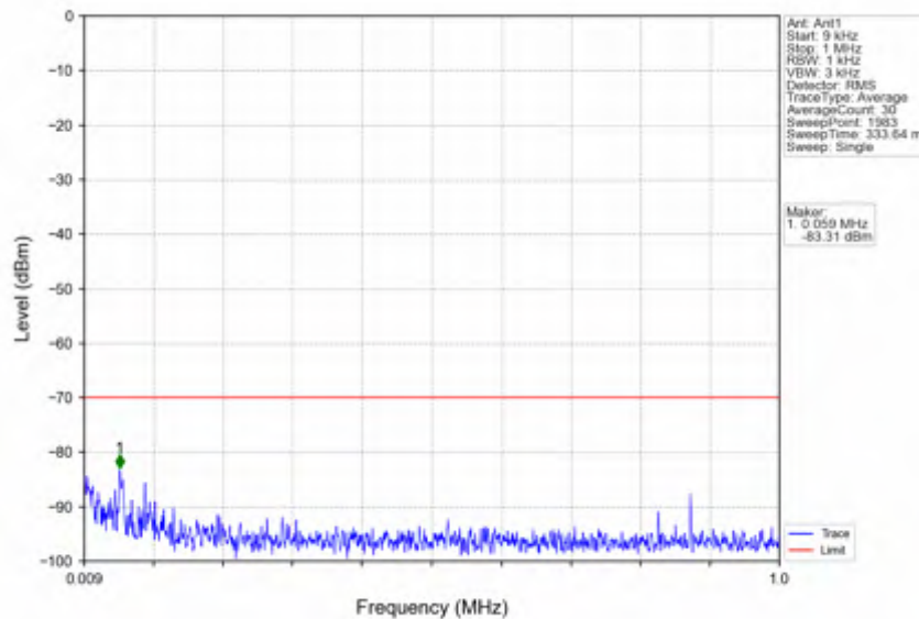
n78d_15kHz_SISO_NTNV_10MHz_DFT-s-OFDM QPSK_3625.005MHz_Edge_1RB_Left
