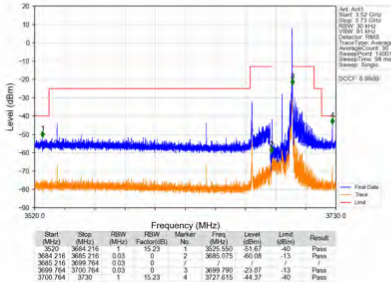
n78d_15kHz_SISO_NTV_15MHz_CP-OFDM QPSK_3692.49MHz_Edge_1RB_Right
