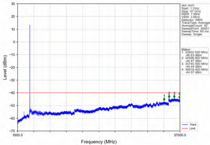
n78d_15kHz_SISO_NTNV_10MHz_DFT-s-OFDM QPSK_3555MHz_Edge_1RB_Left
