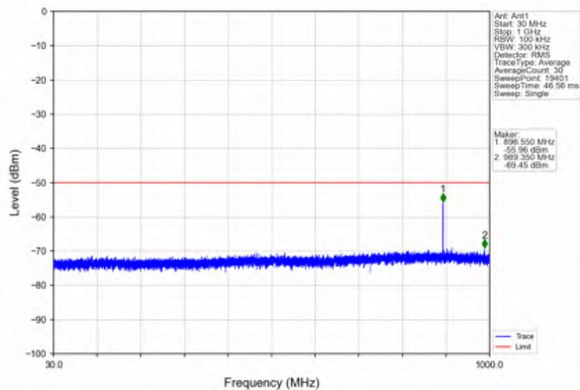
n78d_15kHz_SISO_NTNV_15MHz_DFT-s-OFDM_PI/2_BPSK_3557.505MHz_Inner_1RB_Left
