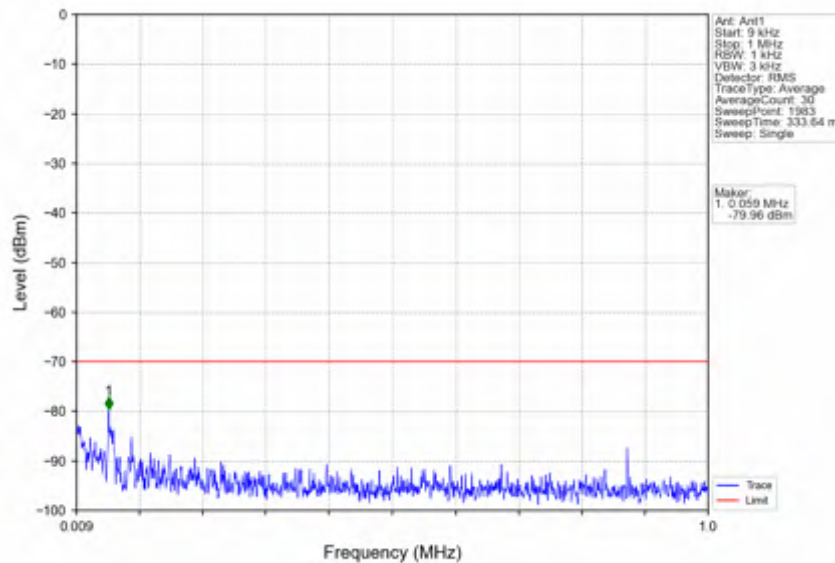
n78d_15kHz_SISO_NTNV_20MHz_CP-OFDM QPSK_3690MHz_Inner_1RB_Right
