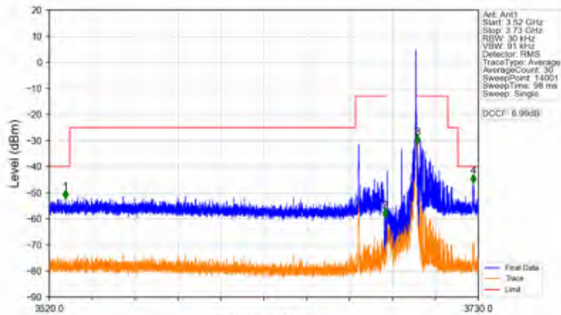
n78d_15kHz_SISO_NTNV_15MHz_DFT-s-OFDM QPSK_3692.49MHz_Edge_1RB_Right
