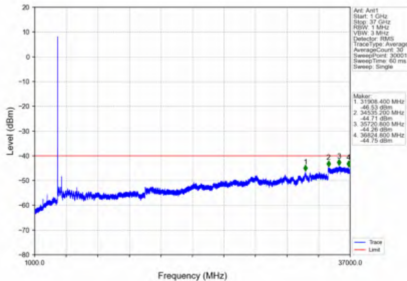
n78d_15kHz_SISO_NTNV_15MHz_DFT-s-OFDM PI/2 BPSK_3625.005MHz_Edge_1RB_Left
