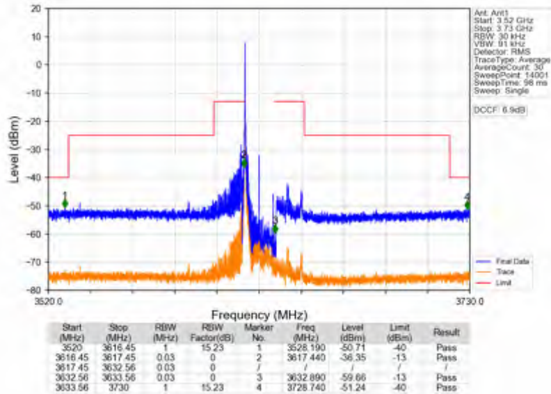
n78d_15kHz_SISO_NTNV_15MHz_DFT-s-OFDM PI/2 BPSK_3625.005MHz_Edge_1RB_Left
