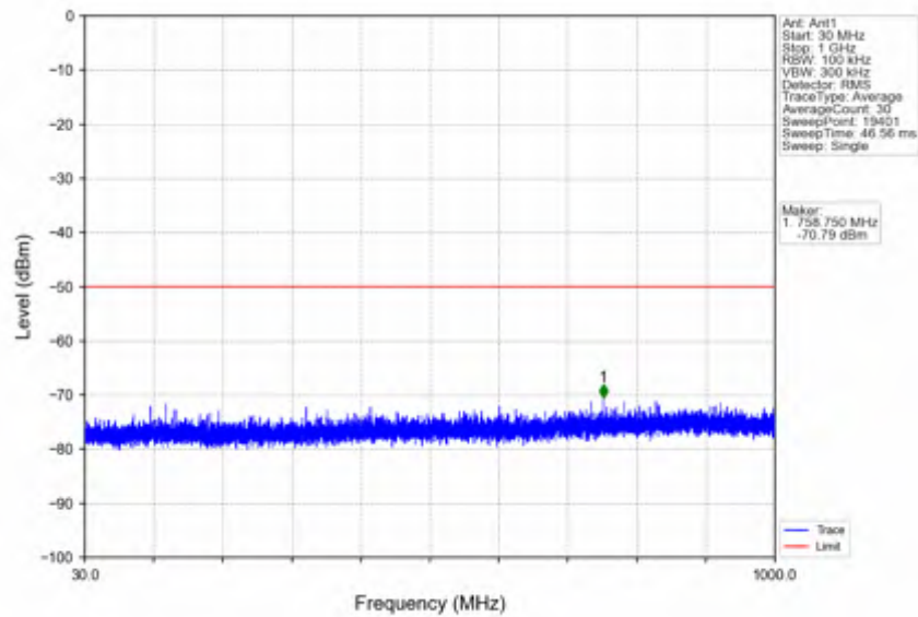
n78d_15kHz_SISO_NTNV_10MHz_CP-OFDM QPSK_3555MHz_Outer_Full
