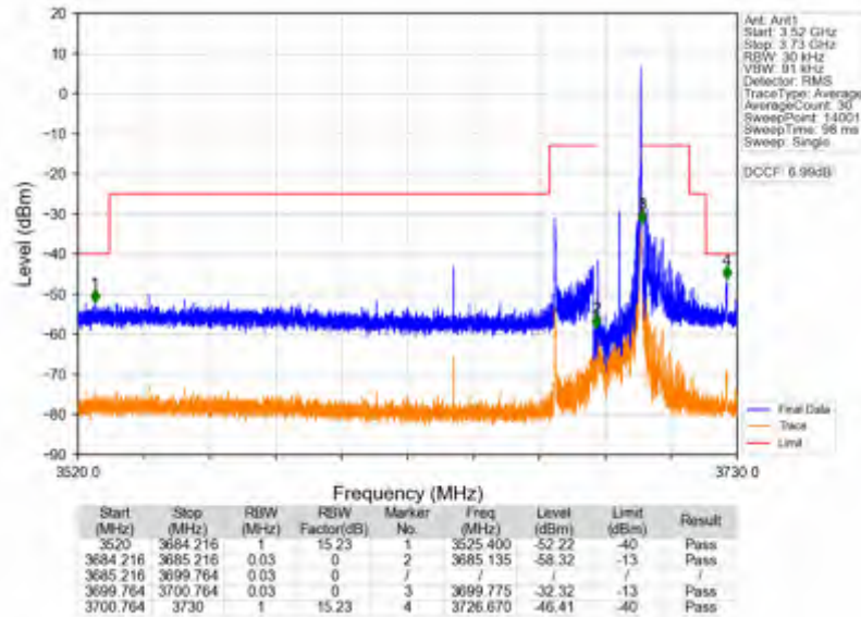
n78d_15kHz_SISO_NTV_15MHz_CP-OFDM QPSK_3692.49MHz_Inner_1RB_Right
