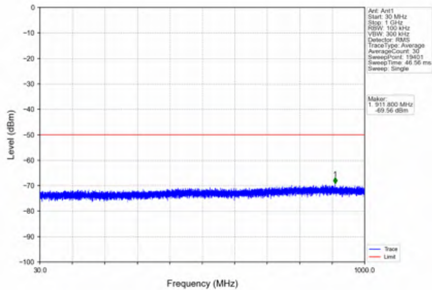
n78d_15kHz_SISO_NTNV_15MHz_DFT-s-OFDM PI/2 BPSK_3557.505MHz_Outer_Full
