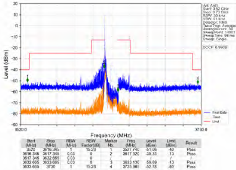
n78d_15kHz_SISO_NTNV_15MHz_DFT-s-OFDM QPSK_3625.005MHz_Edge_1RB_Left
