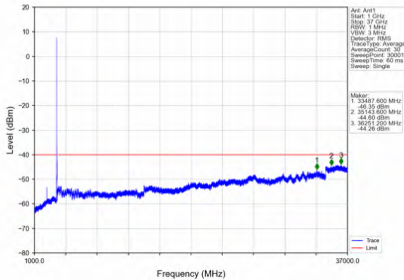
n78d_15kHz_SISO_NTNV_15MHz_DFT-s-OFDM PI/2 BPSK_3557.505MHz_Outer_Full
