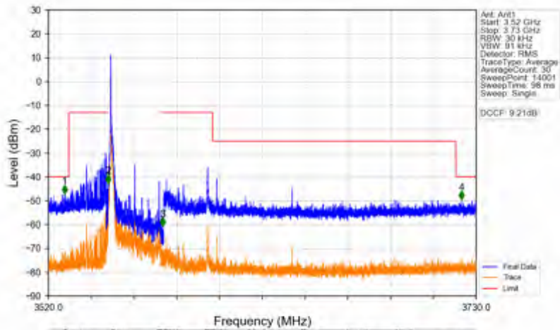
n78d_15kHz_SISO_NTNV_25MHz_DFT-s-OFDM QPSK_3562.5MHz_Edge_1RB_Left
