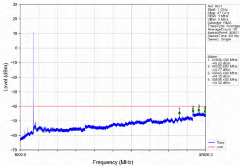
n78d_15kHz_SISO_NTNV_10MHz_DFT-s-OFDM PI/2 BPSK_3625.005MHz_Edge_1RB_Left
