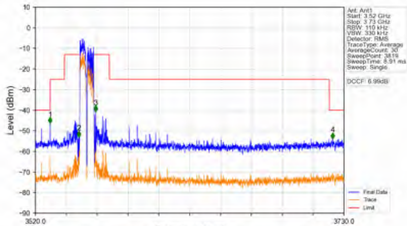
n78d_15kHz_SISO_NTNV_10MHz_CP-OFDM QPSK_3555MHz_Outer_Full
