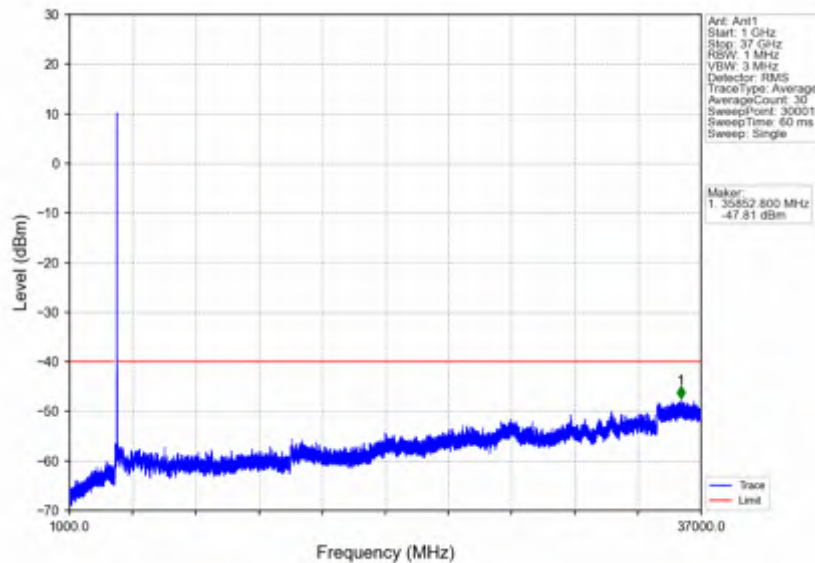
n78d_15kHz_SISO_NTV_10MHz_DFT-s-OFDM QPSK_3694.995MHz_Edge_1RB_Right
