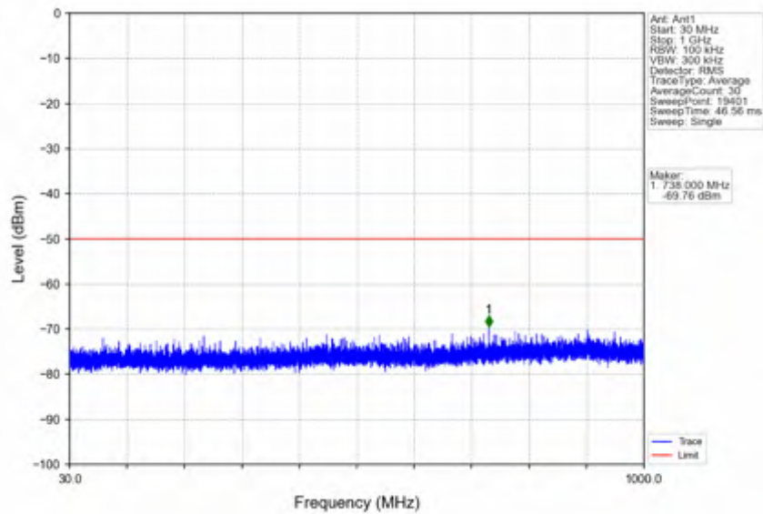
n78d_15kHz_SISO_NTNV_20MHz_DFT-s-OFDM QPSK_3690MHz_Inner_1RB_Right
