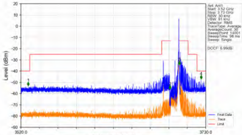
n78d_15kHz_SISO_NTNV_10MHz_DFT-s-OFDM QPSK_3694.995MHz_Inner_1RB_Right
