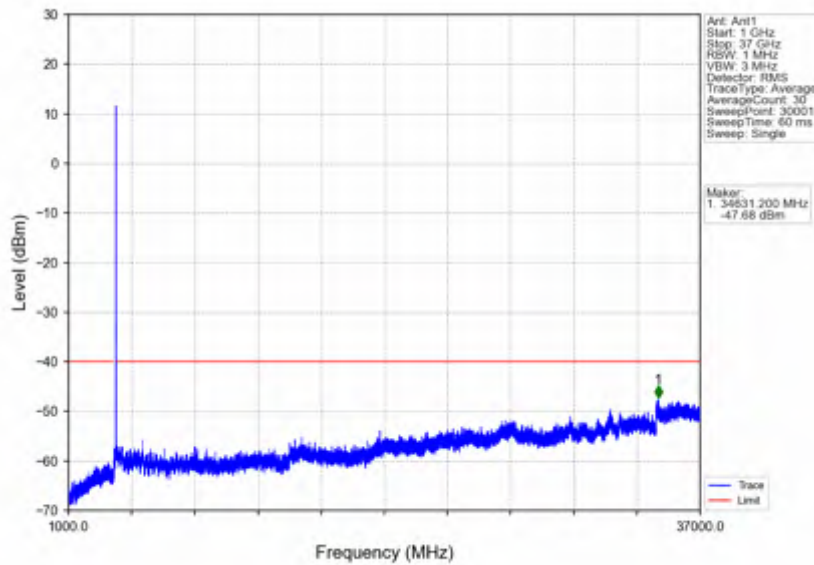
n78d_15kHz_SISO_NTV_10MHz_CP-OFDM QPSK_3694.995MHz_Outer_Full
