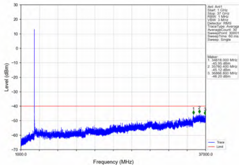
n78d_15kHz_SISO_NTNV_20MHz_CP-OFDM QPSK_3625.005MHz_Edge_1RB_Left
