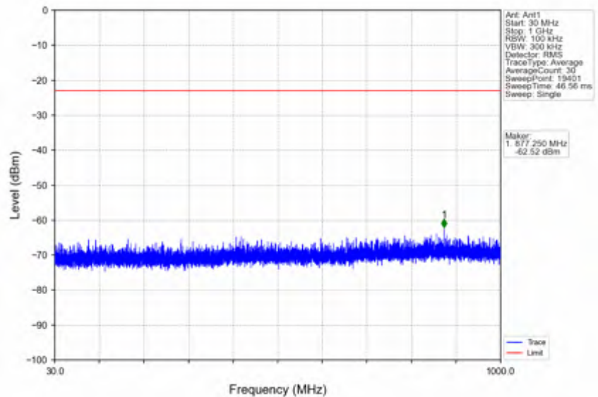
n66_30kHz_SISO_NTNV_40MHz_CP-OFDM QPSK_1760MHz_Edge_1RB_Right
