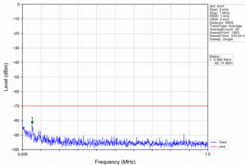
n78d_15kHz_SISO_NTV_20MHz_CP-OFDM_QPSK_3560.01MHz_Inner_1RB_Left
