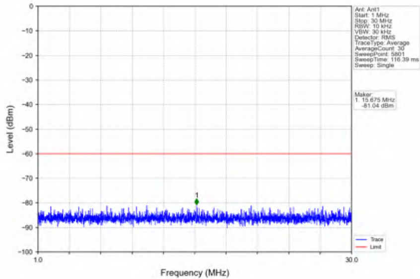
n78d_15kHz_SISO_NTNV_20MHz_CP-OFDM QPSK_3560.01MHz_Outer_Full
