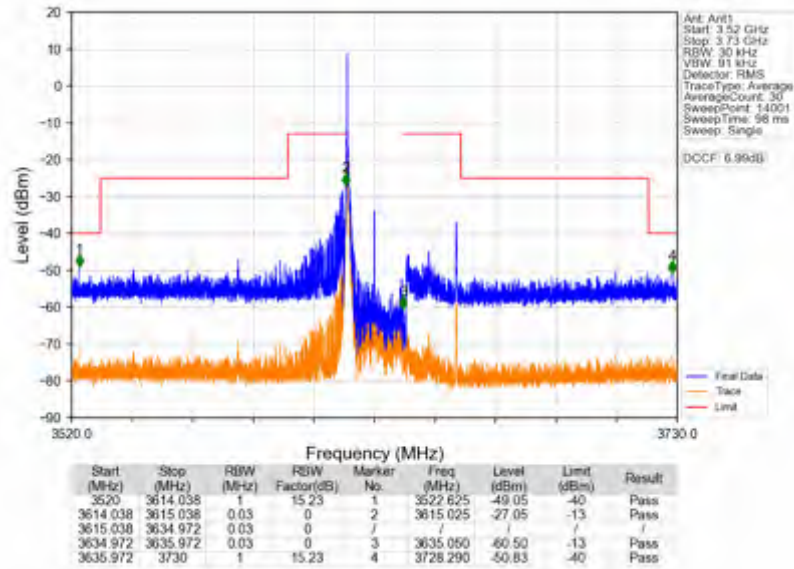
n78d_15kHz_SISO_NTNV_20MHz_DFT-s-OFDM QPSK_3625.005MHz_Edge_1RB_Left
