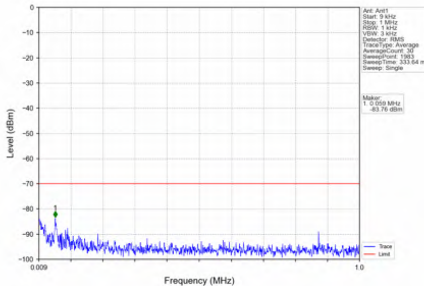
n78d_15kHz_SISO_NTNV_10MHz_CP-OFDM_QPSK_3555MHz_Inner_1RB_Left
