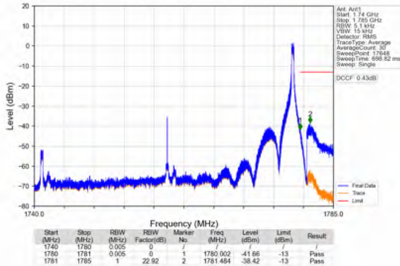
n66_30kHz_SISO_NTV_40MHz_CP-OFDM QPSK_1760MHz_Edge_1RB_Right
