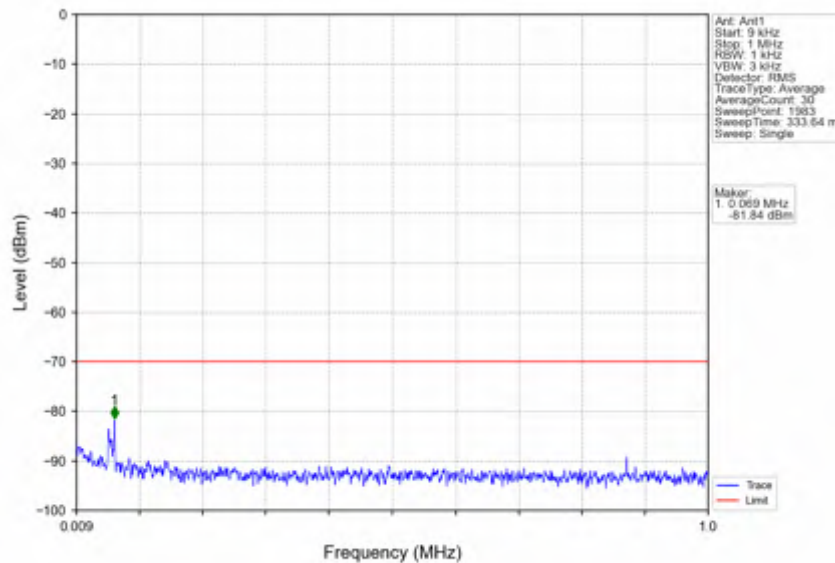
n78d_15kHz_SISO_NTV_20MHz_DFT-s-OFDM PI/2 BPSK_3690MHz_Edge_1RB_Right
