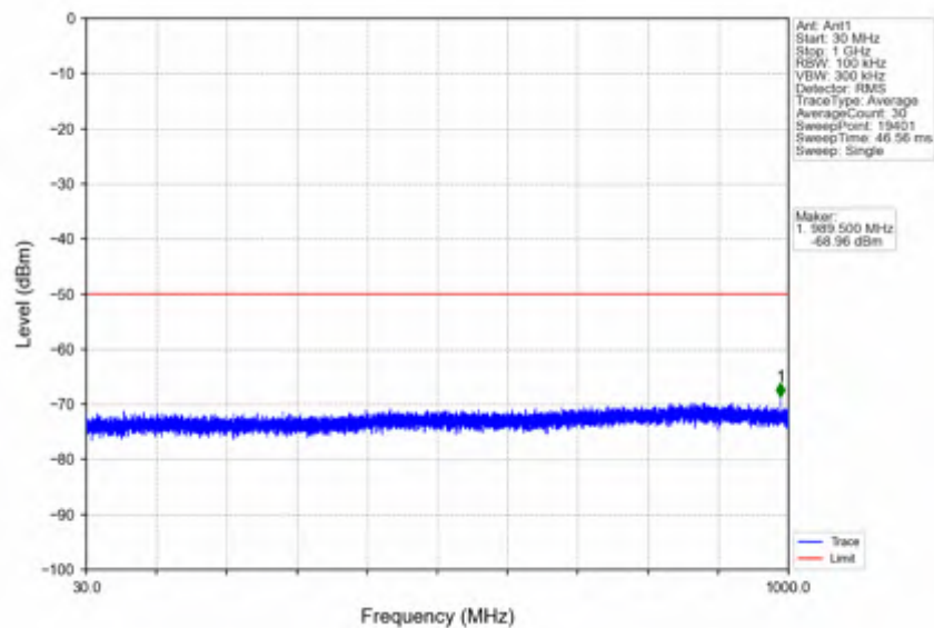
n78d_15kHz_SISO_NTNV_25MHz_DFT-s-OFDM PI/2 BPSK_3562.5MHz_Inner_1RB_Left
