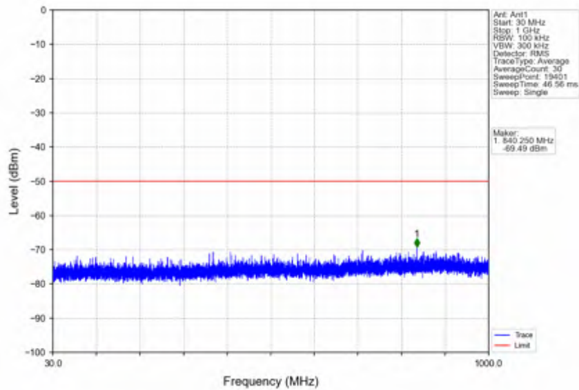
n78d_15kHz_SISO_NTNV_15MHz_CP-OFDM QPSK_3625.005MHz_Edge_1RB_Left
