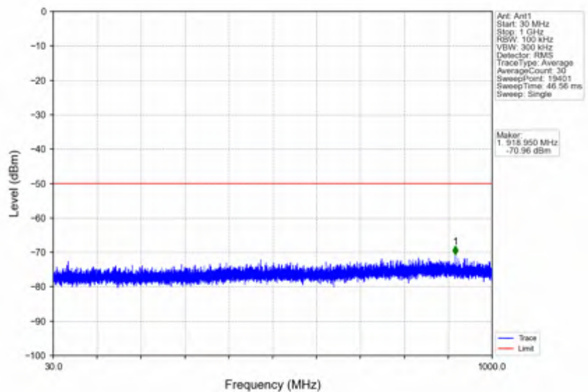
n78d_15kHz_SISO_NTNV_10MHz_CP-OFDM QPSK_3694.995MHz_Edge_1RB_Right
