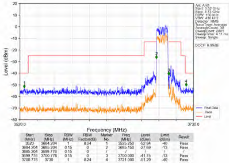
n78d_15kHz_SISO_NTNV_15MHz_DFT-s-OFDM_QPSK_3692.49MHz_Outer_Full
