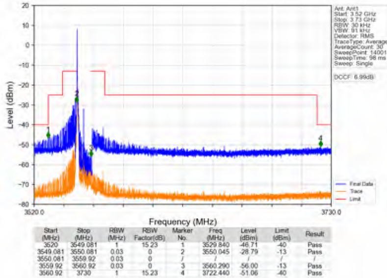
n78d_15kHz_SISO_NTNV_10MHz_DFT-s-OFDM PI/2 BPSK_3555MHz_Edge_1RB_Left
