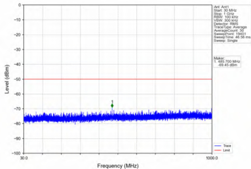
n78d_15kHz_SISO_NTNV_20MHz_DFT-s-OFDM_QPSK_3560.01MHz_Outer_Full
