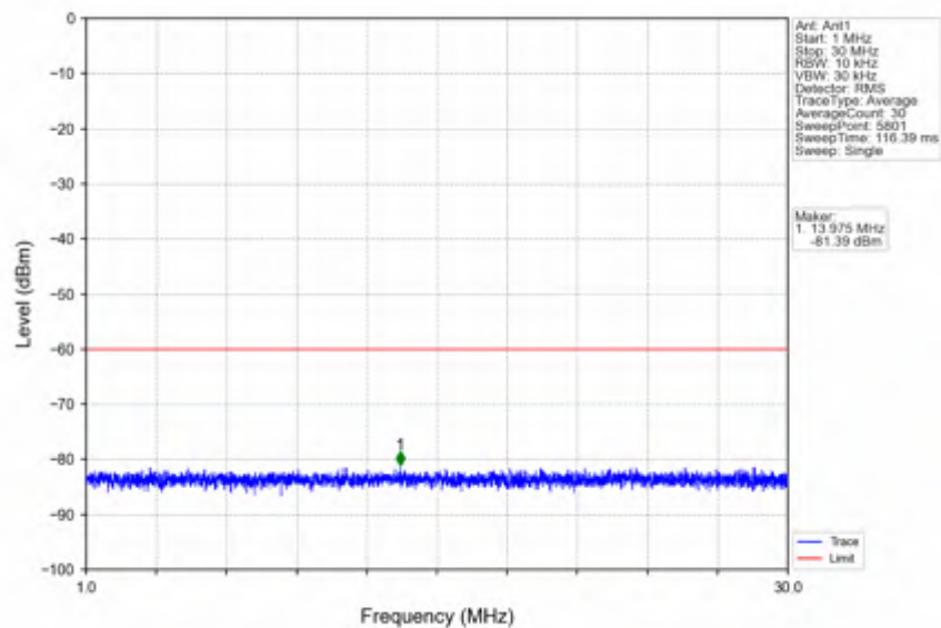
n78d_15kHz_SISO_NTNV_20MHz_DFT-s-OFDM PI/2 BPSK_3690MHz_Outer_Full
