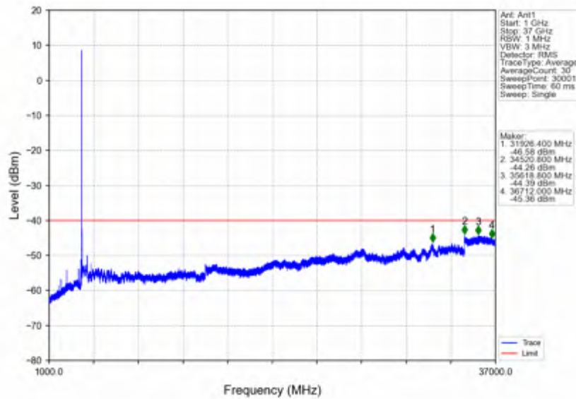
n78d_15kHz_SISO_NTNV_10MHz_DFT-s-OFDM_PI/2_BPSK_3625.005MHz_Edge_1RB_Left
