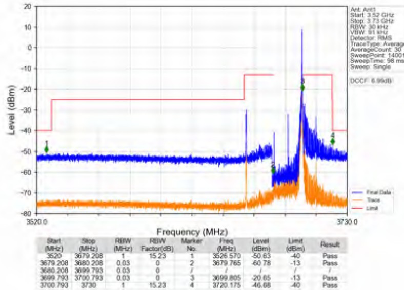
n78d_15kHz_SISO_NTV_20MHz_DFT-s-OFDM PI/2 BPSK_3690MHz_Edge_1RB_Right
