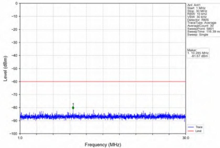
n78d_15kHz_SISO_NTNV_10MHz_DFT-s-OFDM QPSK_3694.995MHz_Outer_Full
