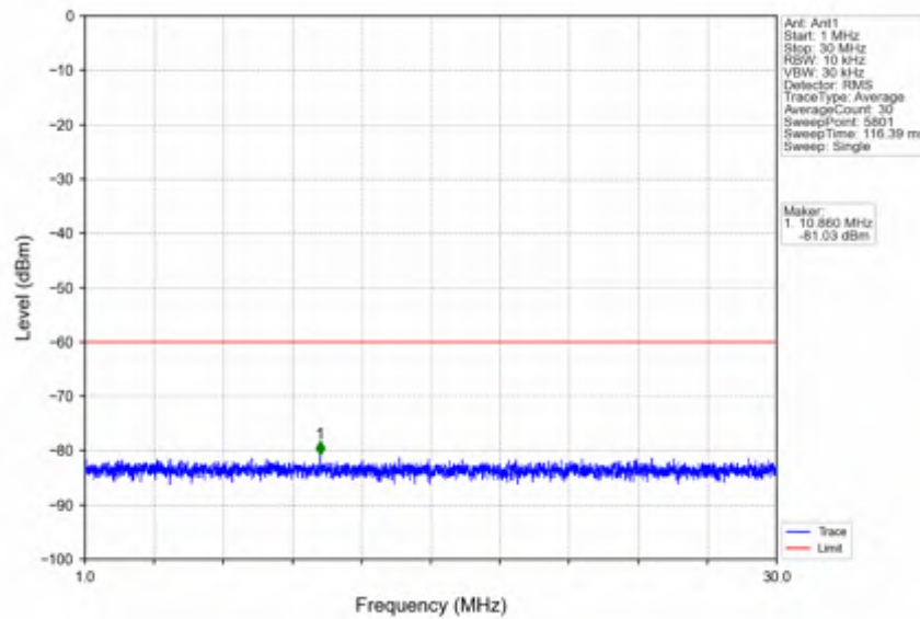
n78d_15kHz_SISO_NTNV_15MHz_DFT-s-OFDM PI/2 BPSK_3557.505MHz_Edge_1RB_Left
