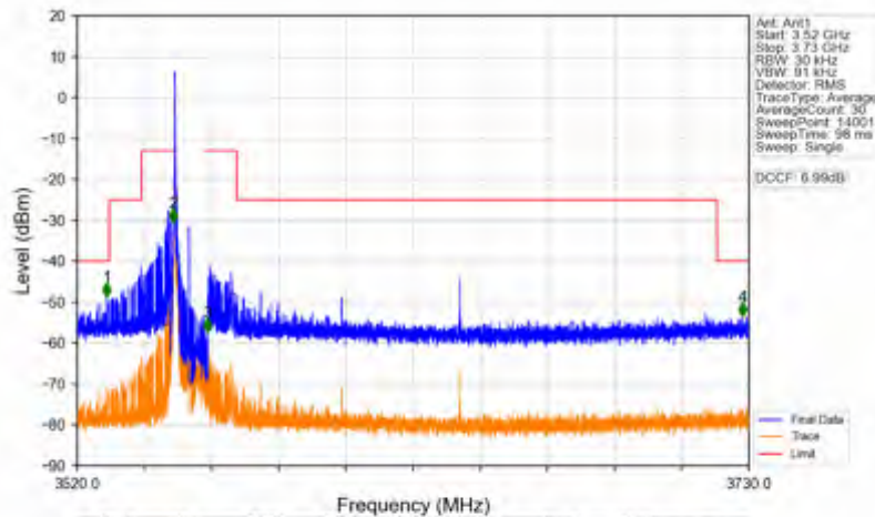
n78d_15kHz_SISO_NTNV_10MHz_DFT-s-OFDM QPSK_3555MHz_Inner_1RB_Left
