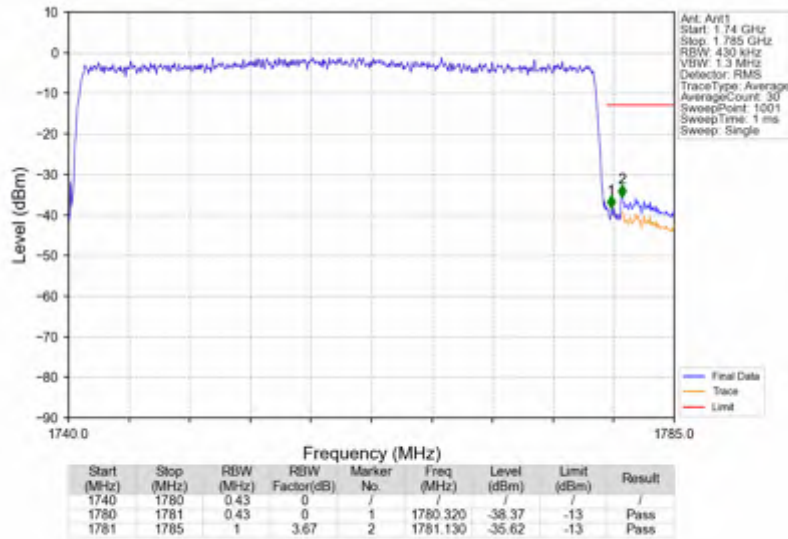
n66_30kHz_SISO_NTNV_40MHz_CP-OFDM QPSK_1760MHz_Outer_Full
