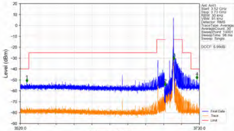
n78d_15kHz_SISO_NTNV_10MHz_DFT-s-OFDM QPSK_3694.995MHz_Edge_1RB_Right
