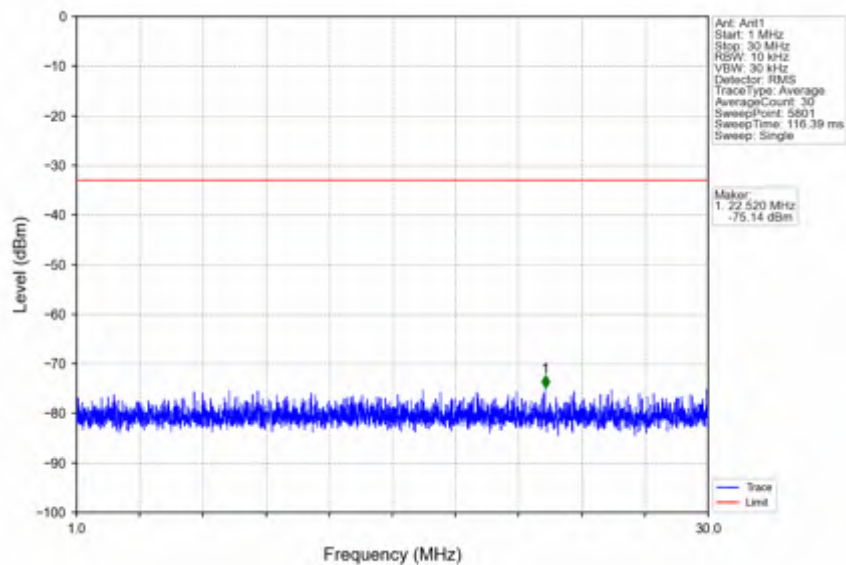
n66_30kHz_SISO_NTNV_40MHz_CP-OFDM QPSK_1760MHz_Outer_Full
