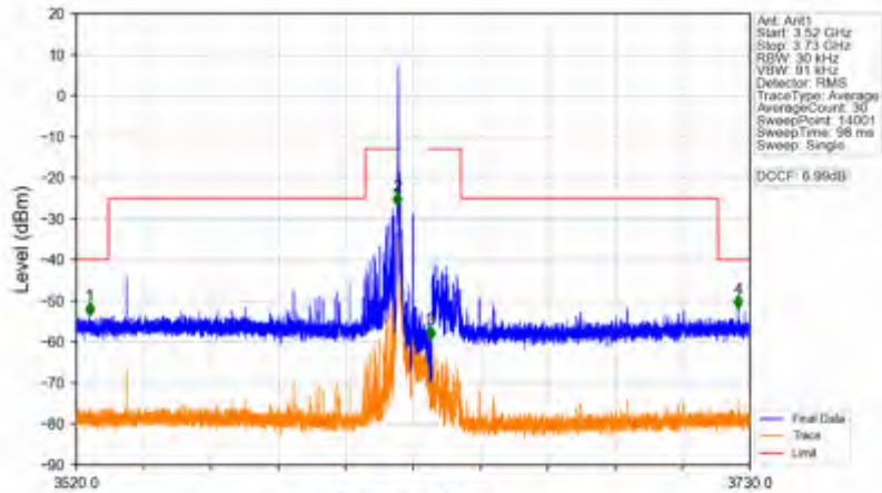
n78d_15kHz_SISO_NTNV_10MHz_CP-OFDM QPSK_3625.005MHz_Edge_1RB_Left
