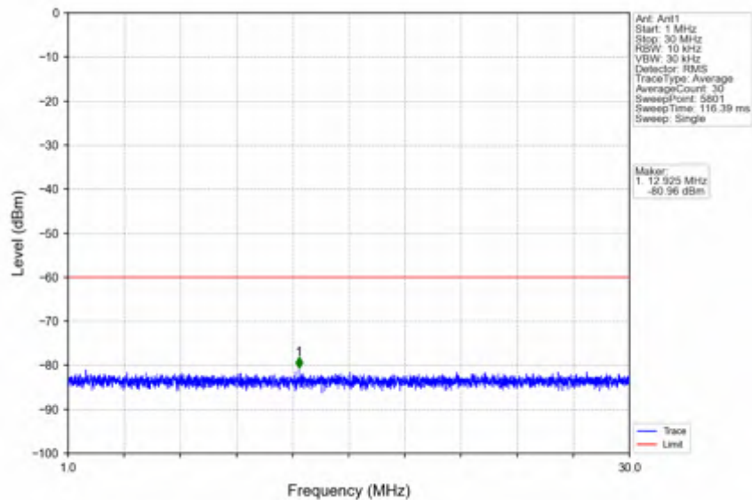
n78d_15kHz_SISO_NTNV_20MHz_DFT-s-OFDM PI/2 BPSK_3560.01MHz_Outer_Full
