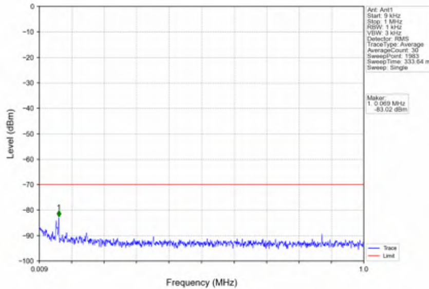
n78d_15kHz_SISO_NTV_15MHz_DFT-s-OFDM PI/2 BPSK_3557.505MHz_Inner_1RB_Left
