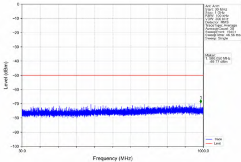
n78d_15kHz_SISO_NTNV_20MHz_DFT-s-OFDM_QPSK_3560.01MHz_Edge_1RB_Left
