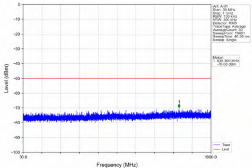
n78d_15kHz_SISO_NTNV_20MHz_CP-OFDM QPSK_3690MHz_Inner_1RB_Right
