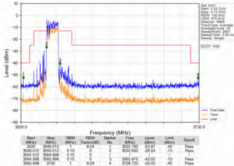
n78d_15kHz_SISO_NTNV_15MHz_DFT-s-OFDM QPSK_3557.505MHz_Outer_Full
