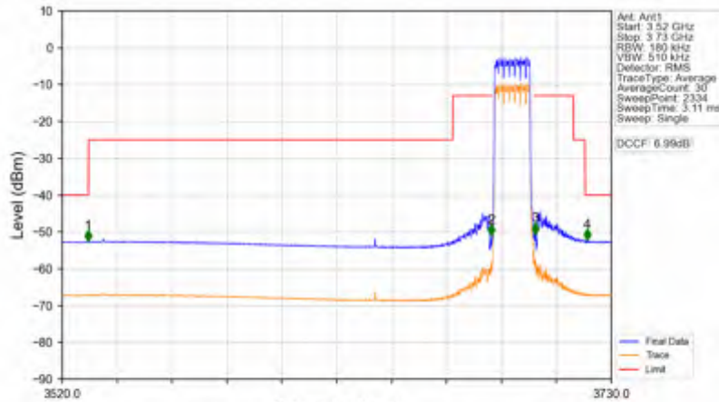
n78d_15kHz_SISO_NTNV_15MHz_DFT-s-OFDM PI/2 BPSK_3692.49MHz_Outer_Full
