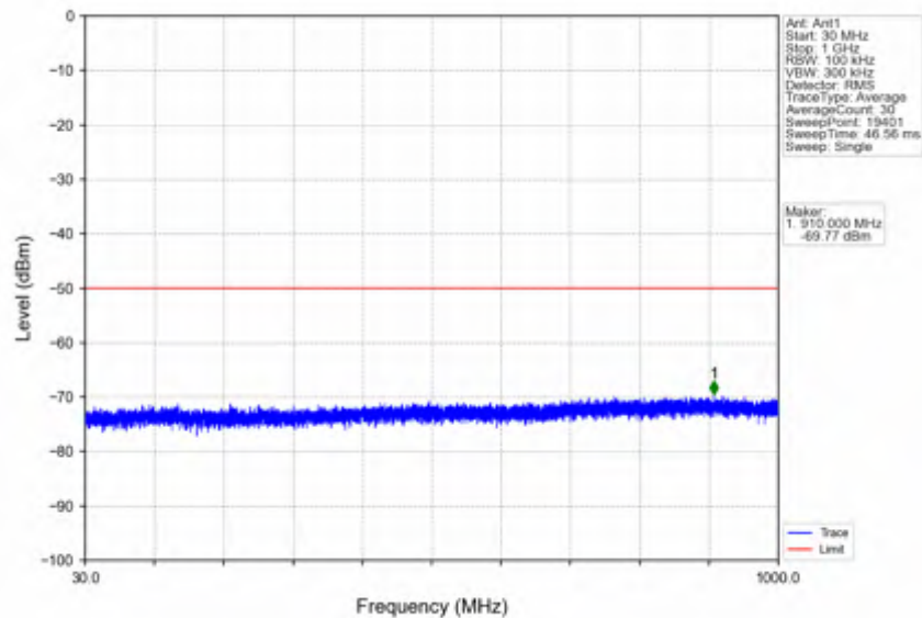
n78d_15kHz_SISO_NTNV_10MHz_DFT-s-OFDM PI/2 BPSK_3694.995MHz_Edge_1RB_Right
