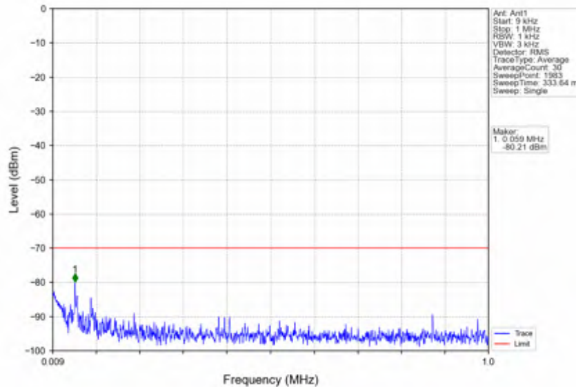
n78d_15kHz_SISO_NTV_20MHz_CP-OFDM QPSK_3560.01MHz_Edge_1RB_Left
