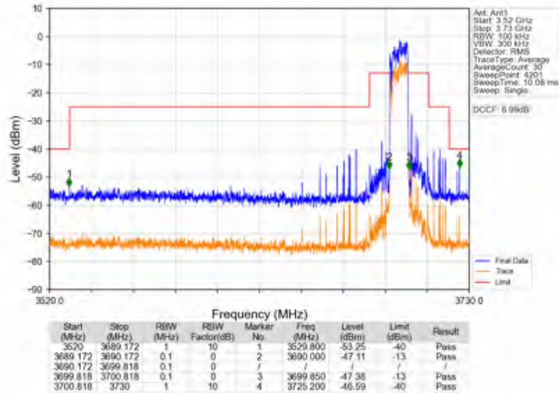
n78d_15kHz_SISO_NTNV_10MHz_DFT-s-OFDM QPSK_3694.995MHz_Outer_Full
