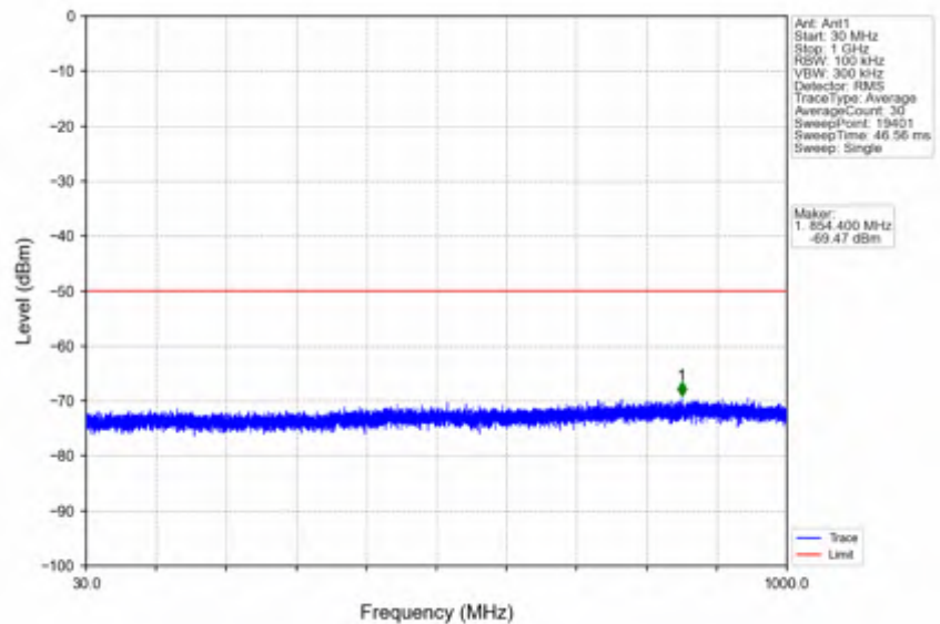
n78d_15kHz_SISO_NTNV_20MHz_DFT-s-OFDM QPSK_3690MHz_Outer_Full
