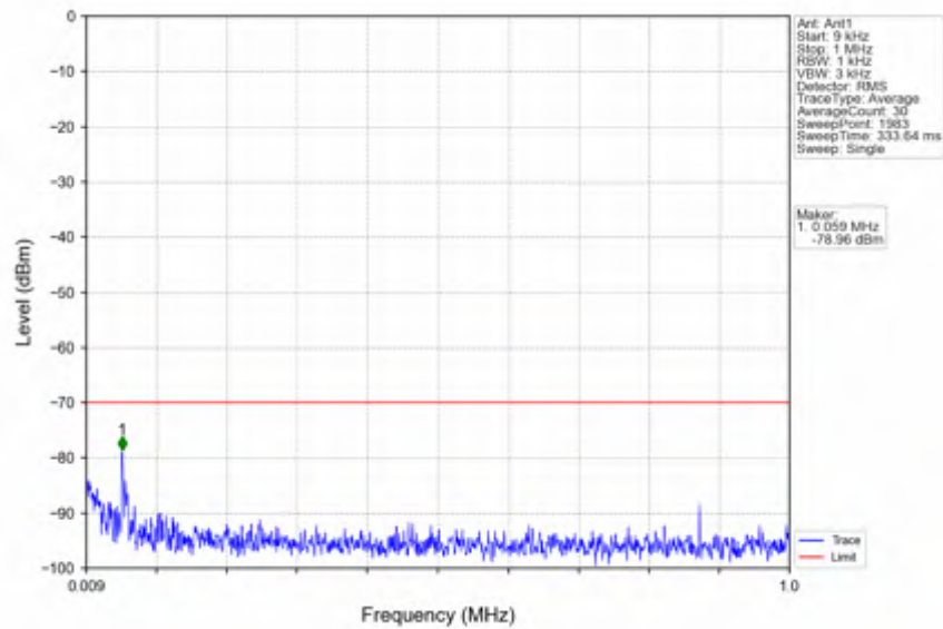
n78d_15kHz_SISO_NTNV_15MHz_CP-OFDM QPSK_3557.505MHz_Outer_Full
