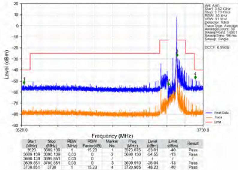
n78d_15kHz_SISO_NTV_10MHz_CP-OFDM QPSK_3694.995MHz_Edge_1RB_Right
