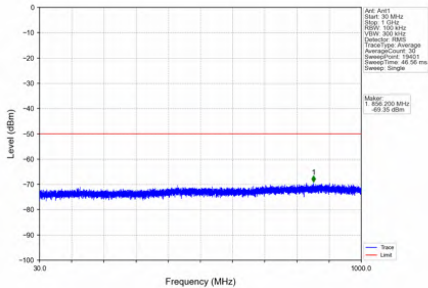
n78d_15kHz_SISO_NTNV_15MHz_DFT-s-OFDM PI/2 BPSK_3692.49MHz_Outer_Full
