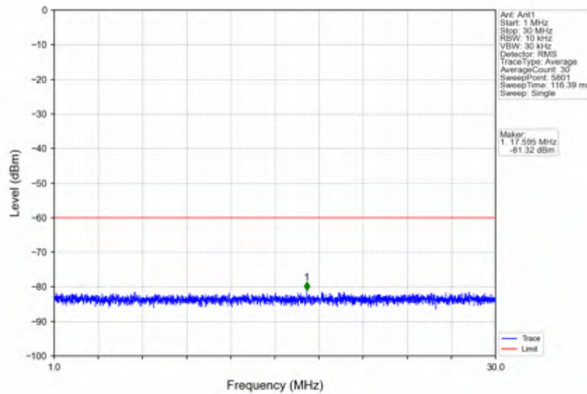
n78d_15kHz_SISO_NTNV_25MHz_DFT-s-OFDM PI/2 BPSK_3562.5MHz_Edge_1RB_Left
