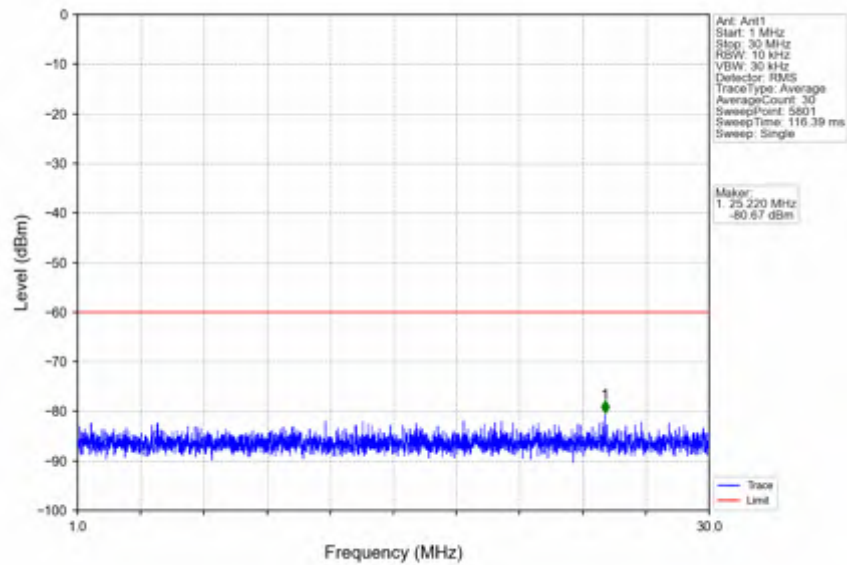
n78d_15kHz_SISO_NTNV_15MHz_CP-OFDM QPSK_3557.505MHz_Inner_1RB_Left
