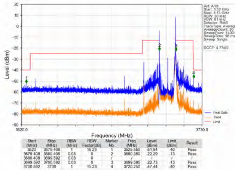
n78d_15kHz_SISO_NTNV_20MHz_CP-OFDM QPSK_3690MHz_Inner_1RB_Right
