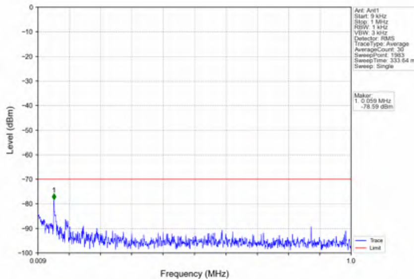
n78d_15kHz_SISO_NTV_15MHz_CP-OFDM QPSK_3692.49MHz_Inner_1RB_Right
