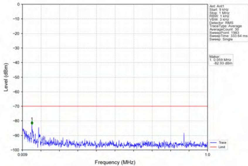
n78d_15kHz_SISO_NTVV_10MHz_DFT-s-OFDM_QPSK_3555MHz_Inner_1RB_Left
