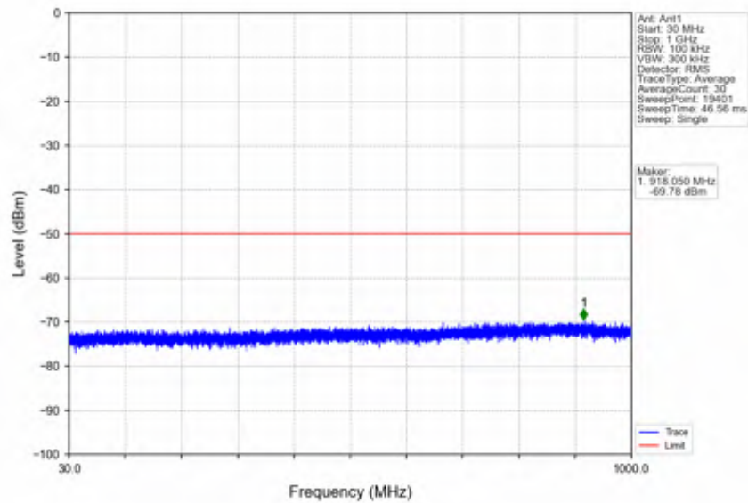
n78d_15kHz_SISO_NTNV_25MHz_DFT-s-OFDM PI/2 BPSK_3625.005MHz_Edge_1RB_Left
