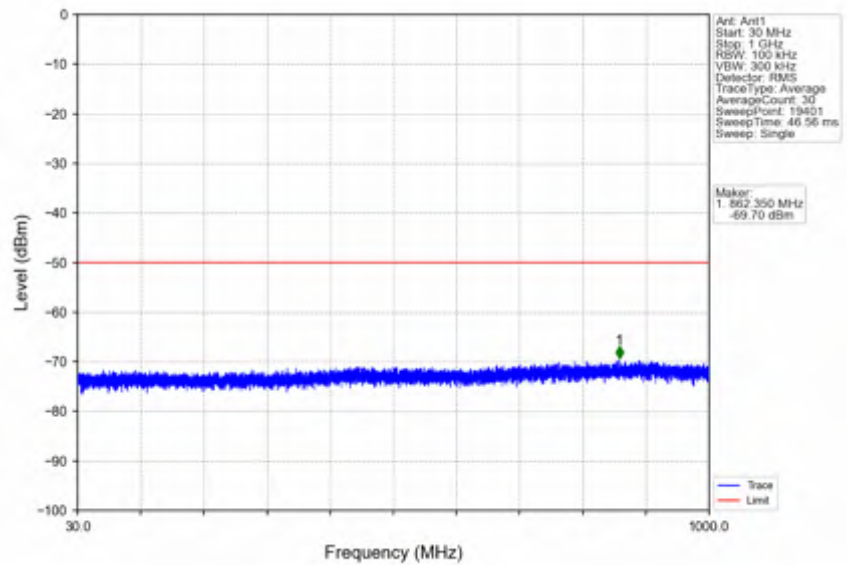
n78d_15kHz_SISO_NTNV_20MHz_CP-OFDM QPSK_3690MHz_Edge_1RB_Right
