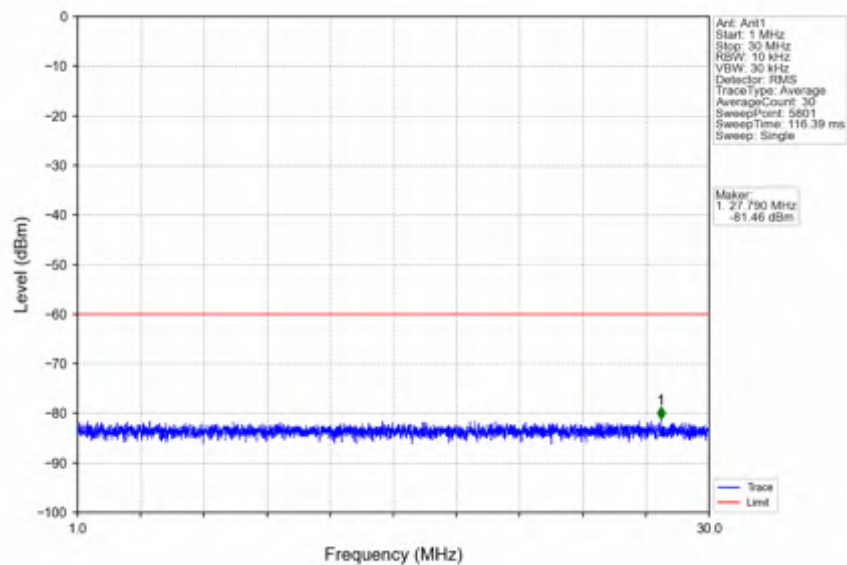
n78d_15kHz_SISO_NTNV_15MHz_DFT-s-OFDM PI/2 BPSK_3625.005MHz_Edge_1RB_Left
