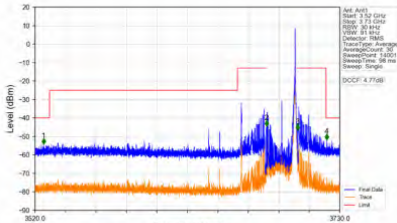
n78d_15kHz_SISO_NTNV_20MHz_DFT-s-OFDM_QPSK_3690MHz_Inner_1RB_Right
