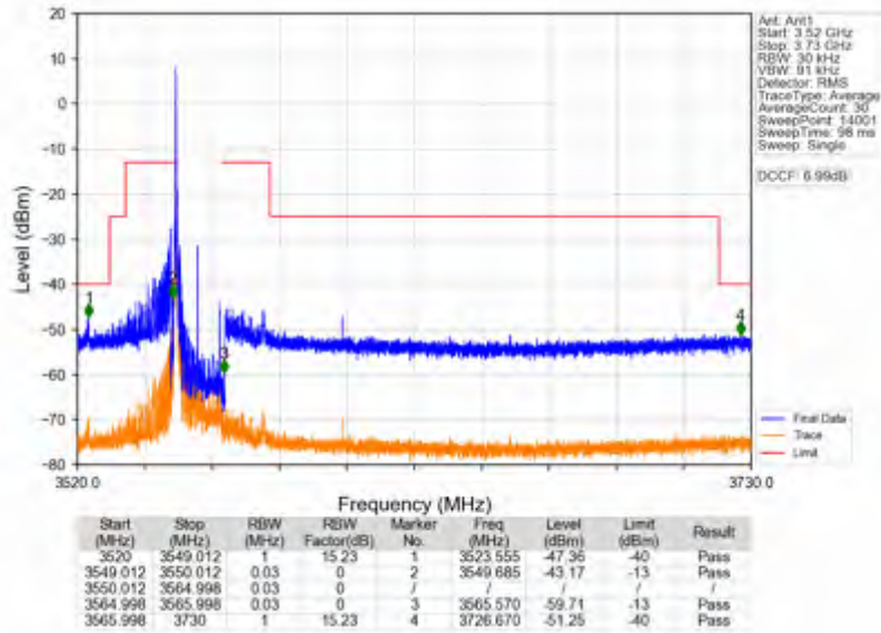
n78d_15kHz_SISO_NTV_15MHz_DFT-s-OFDM PI/2 BPSK_3557.505MHz_Inner_1RB_Left
