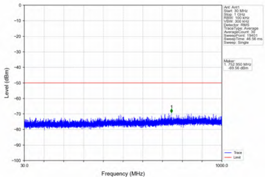
n78d_15kHz_SISO_NTNV_15MHz_CP-OFDM QPSK_3692.49MHz_Edge_1RB_Right
