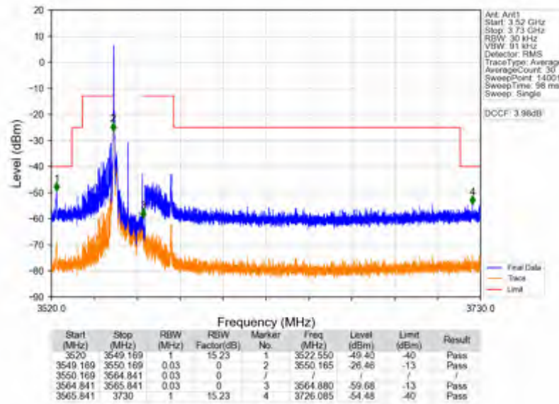
n78d_15kHz_SISO_NTNV_15MHz_CP-OFDM QPSK_3557.505MHz_Edge_1RB_Left
