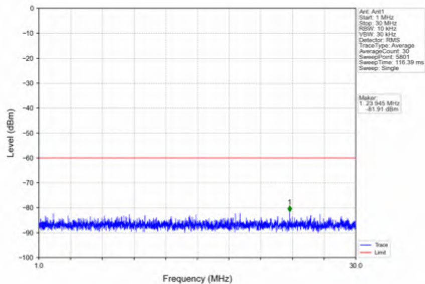
n78d_15kHz_SISO_NTV_10MHz_DFT-s-OFDM QPSK_3694.995MHz_Edge_1RB_Right
