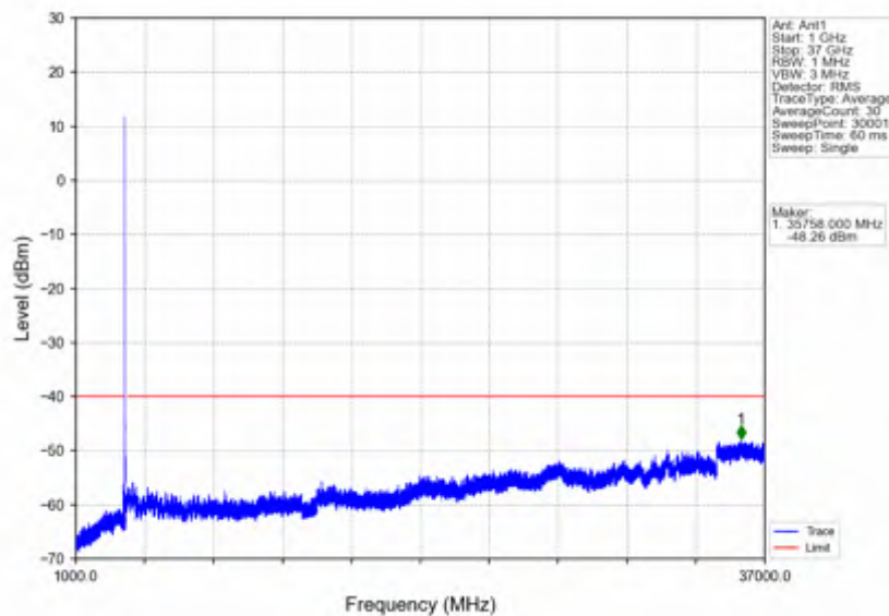
n78d_15kHz_SISO_NTVV_10MHz_DFT-s-OFDM_QPSK_3555MHz_Edge_1RB_Left
