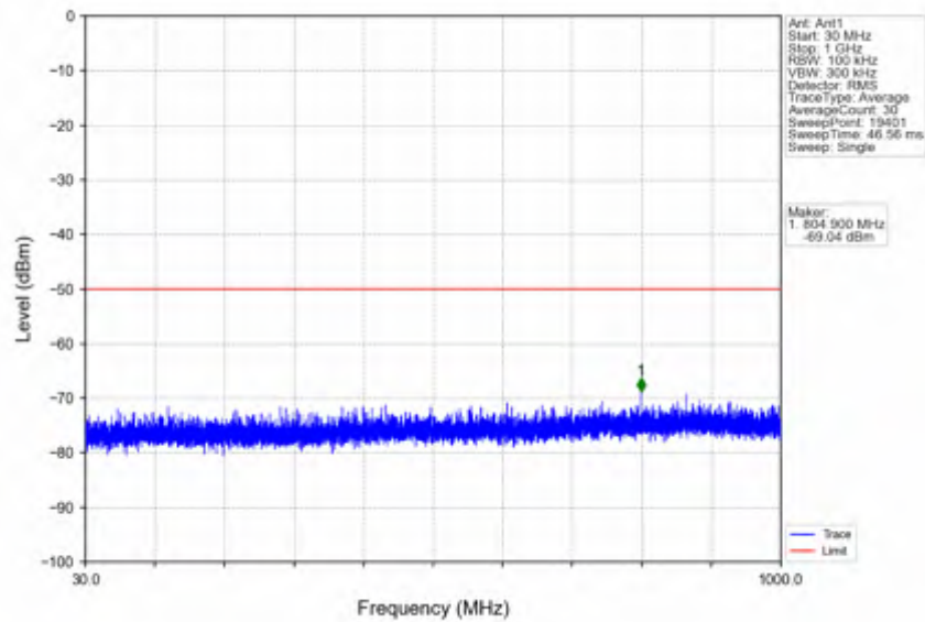
n78d_15kHz_SISO_NTNV_20MHz_CP-OFDM QPSK_3560.01MHz_Outer_Full
