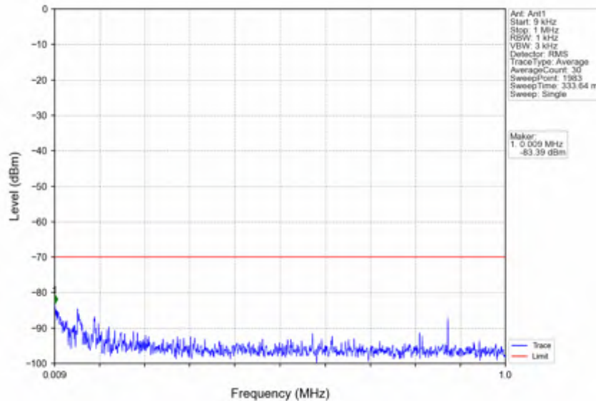
n78d_15kHz_SISO_NTV_10MHz_CP-OFDM QPSK_3694.995MHz_Inner_1RB_Right
