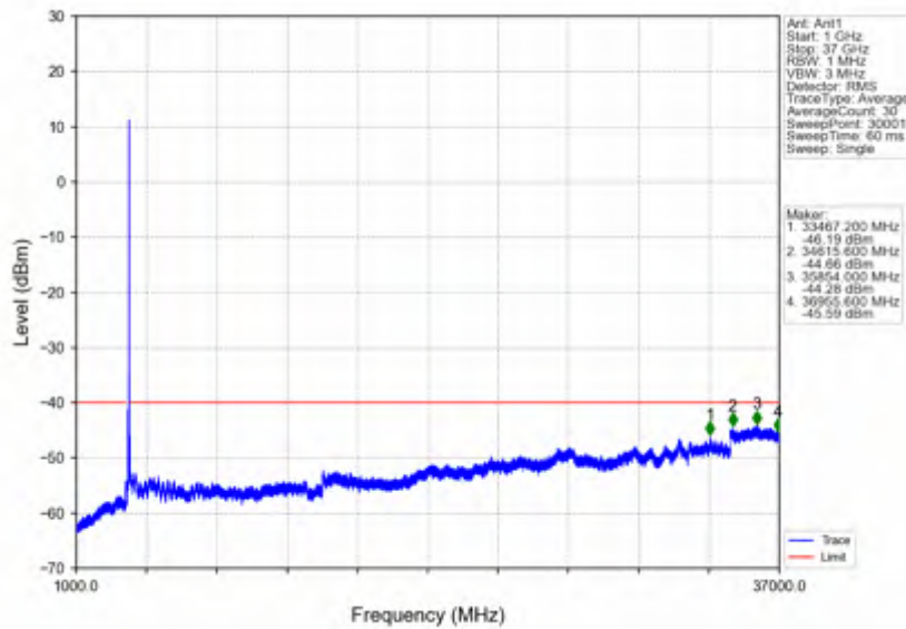
n78d_15kHz_SISO_NTNV_25MHz_DFT-s-OFDM PI/2 BPSK_3687.495MHz_Outer_Full
