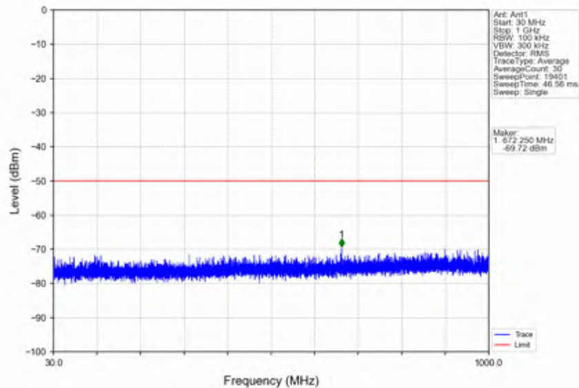
n78d_15kHz_SISO_NTNV_20MHz_CP-OFDM QPSK_3560.01MHz_Inner_1RB_Left
