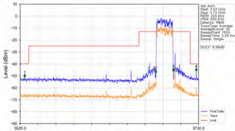
n78d_15kHz_SISO_NTNV_20MHz_CP-OFDM QPSK_3690MHz_Outer_Full
