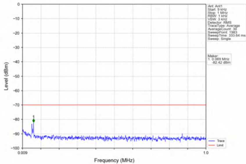
n78d_15kHz_SISO_NTNV_25MHz_DFT-s-OFDM PI/2 BPSK_3687.495MHz_Outer_Full
