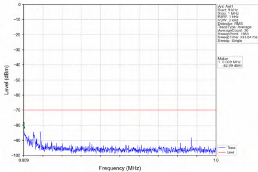
n78d_15kHz_SISO_NTV_10MHz_DFT-s-OFDM QPSK_3694.995MHz_Inner_1RB_Right
