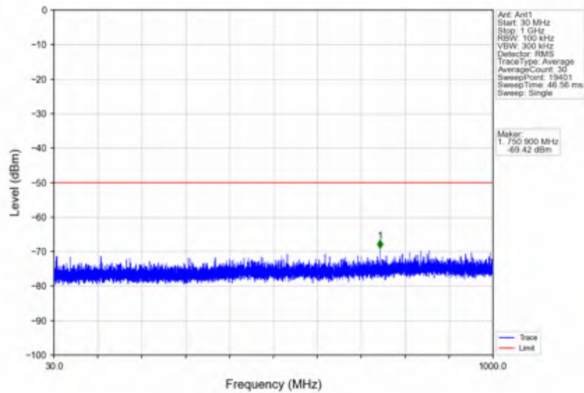
n78d_15kHz_SISO_NTNV_15MHz_CP-OFDM QPSK_3692.49MHz_Outer_Full
