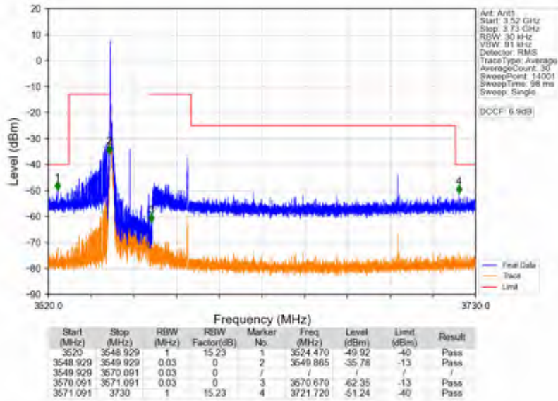
n78d_15kHz_SISO_NTNV_20MHz_DFT-s-OFDM QPSK_3560.01MHz_Edge_1RB_Left
