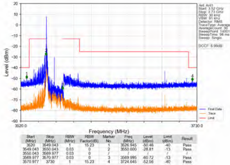
n78d_15kHz_SISO_NTV_20MHz_CP-OFDM QPSK_3560.01MHz_Edge_1RB_Left
