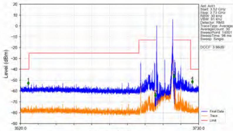
n78d_15kHz_SISO_NTNV_20MHz_DFT-s-OFDM QPSK_3690MHz_Edge_1RB_Right
