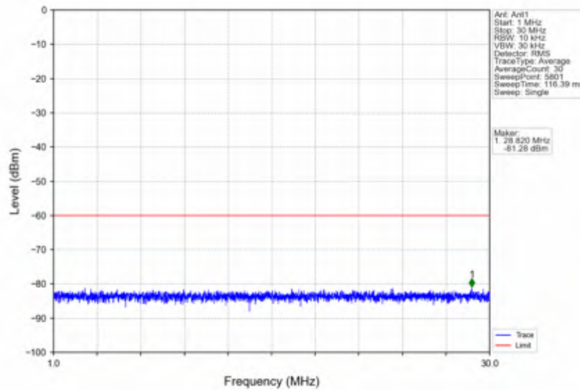
n78d_15kHz_SISO_NTV_20MHz_DFT-s-OFDM_PI/2_BPSK_3690MHz_Edge_1RB_Right
