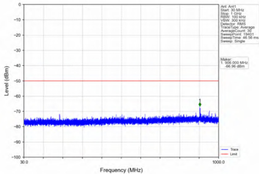
n78d_15kHz_SISO_NTNV_10MHz_DFT-s-OFDM_QPSK_3694.995MHz_Inner_1RB_Right
