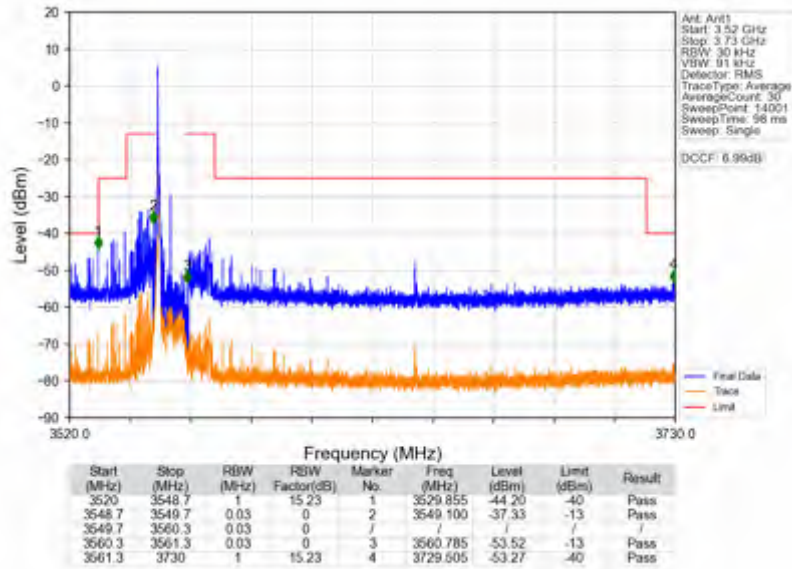
n78d_15kHz_SISO_NTNV_10MHz_CP-OFDM_QPSK_3555MHz_Inner_1RB_Left
