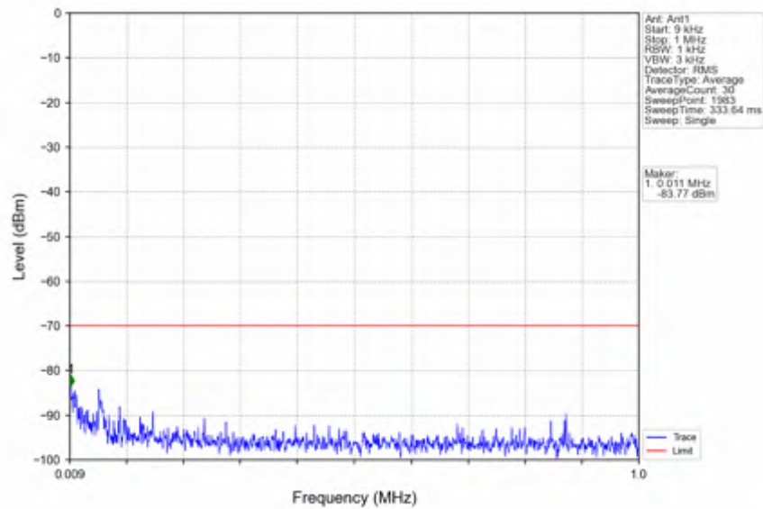
n78d_15kHz_SISO_NTNV_10MHz_CP-OFDM QPSK_3694.995MHz_Outer_Full
