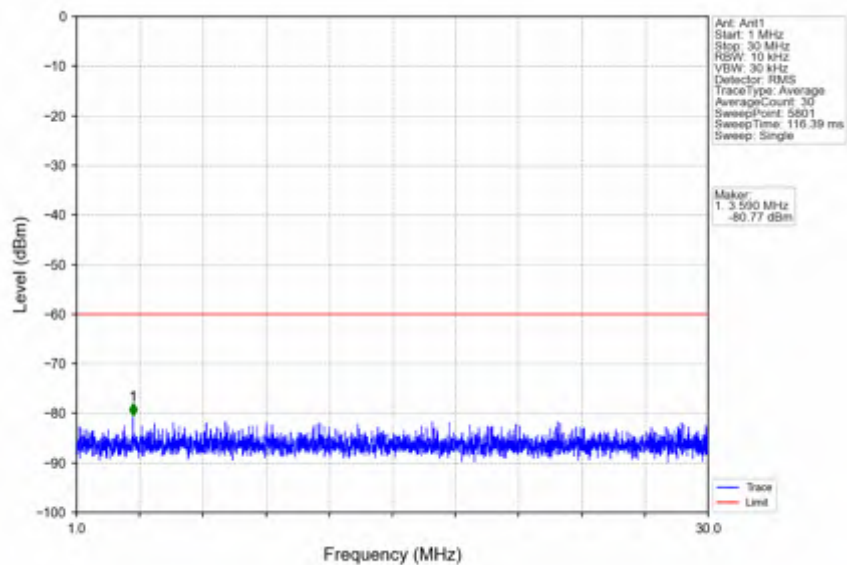
n78d_15kHz_SISO_NTNV_20MHz_DFT-s-OFDM QPSK_3560.01MHz_Inner_1RB_Left
