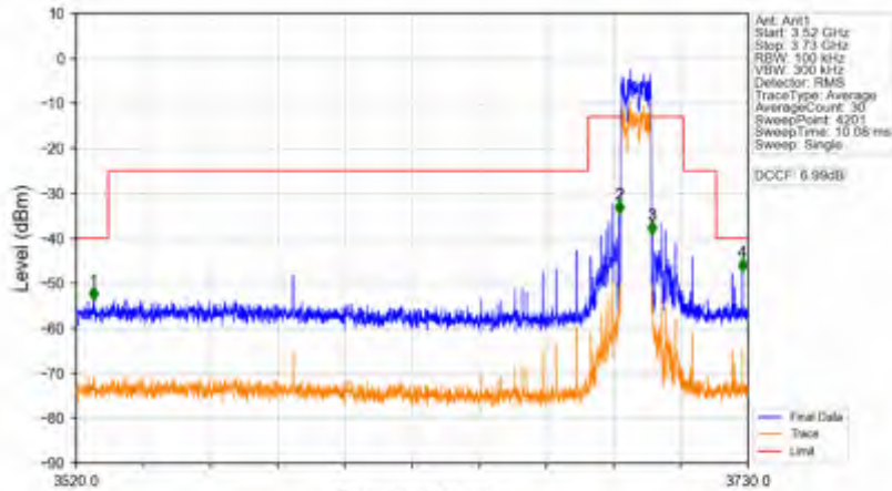
n78d_15kHz_SISO_NTV_10MHz_CP-OFDM QPSK_3694.995MHz_Outer_Full
