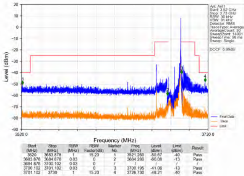
n78d_15kHz_SISO_NTNV_15MHz_DFT-s-OFDM QPSK_3692.49MHz_Inner_1RB_Right
