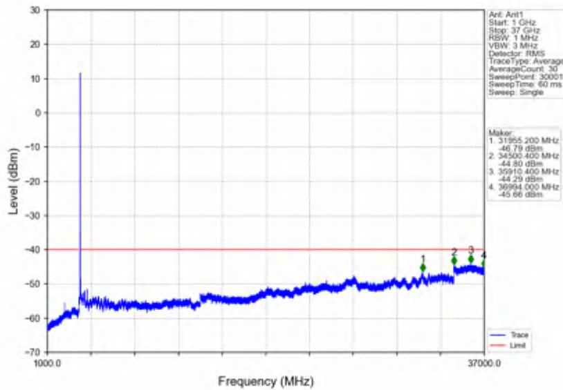
n78d_15kHz_SISO_NTNV_15MHz_DFT-s-OFDM PI/2 BPSK_3692.49MHz_Outer_Full
