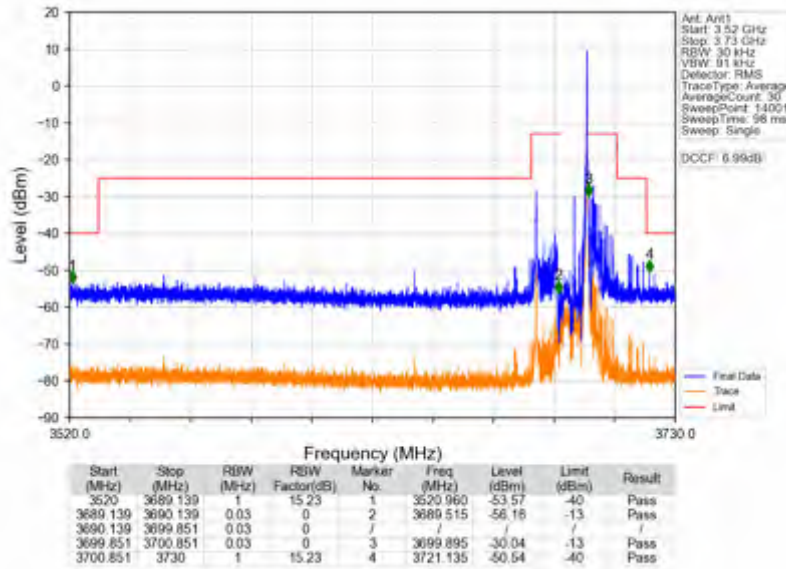
n78d_15kHz_SISO_NTV_10MHz_CP-OFDM QPSK_3694.995MHz_Inner_1RB_Right
