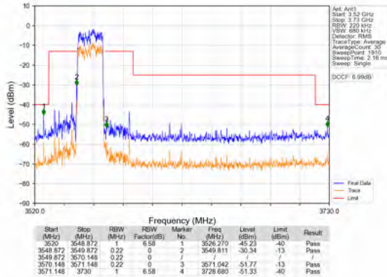
n78d_15kHz_SISO_NTNV_20MHz_DFT-s-OFDM QPSK_3560.01MHz_Outer_Full
