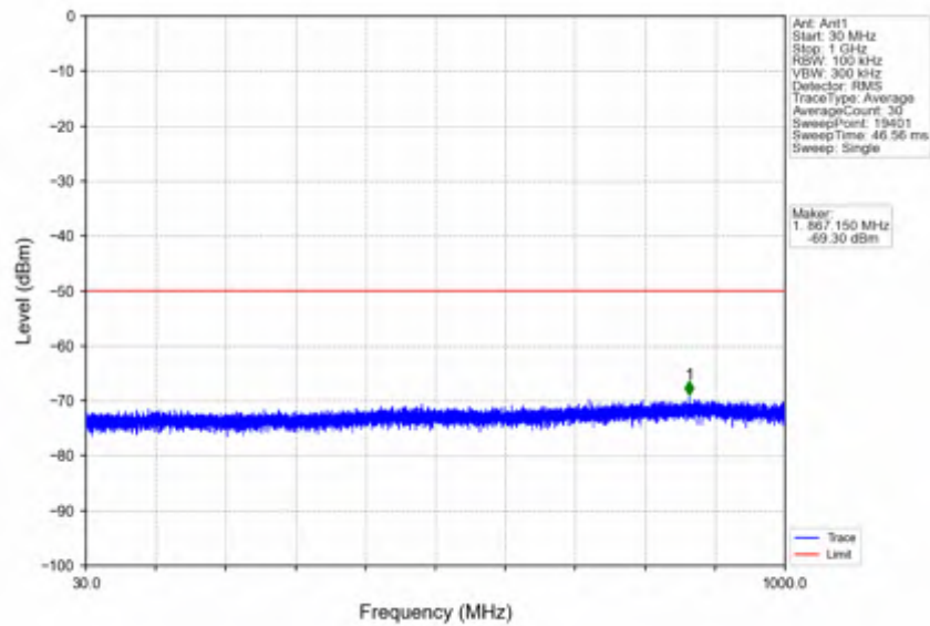
n78d_15kHz_SISO_NTNV_20MHz_DFT-s-OFDM PI/2 BPSK_3625.005MHz_Edge_1RB_Left
