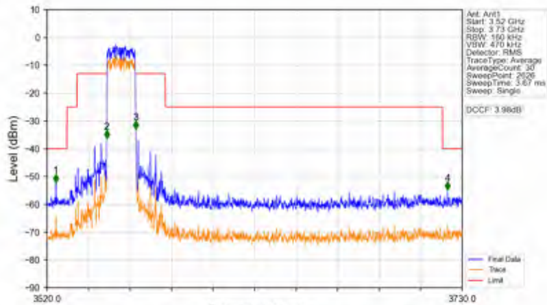
n78d_15kHz_SISO_NTNV_15MHz_CP-OFDM QPSK_3557.505MHz_Outer_Full
