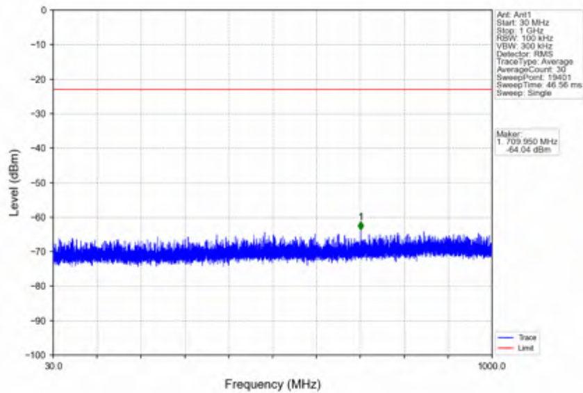
n66_30kHz_SISO_NTNV_25MHz_DFT-s-OFDM QPSK_1767.5MHz_Edge_1RB_Right
