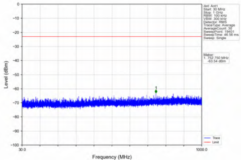
n66_30kHz_SISO_NTNV_40MHz_CP-OFDM QPSK_1730MHz_Edge_1RB_Left
