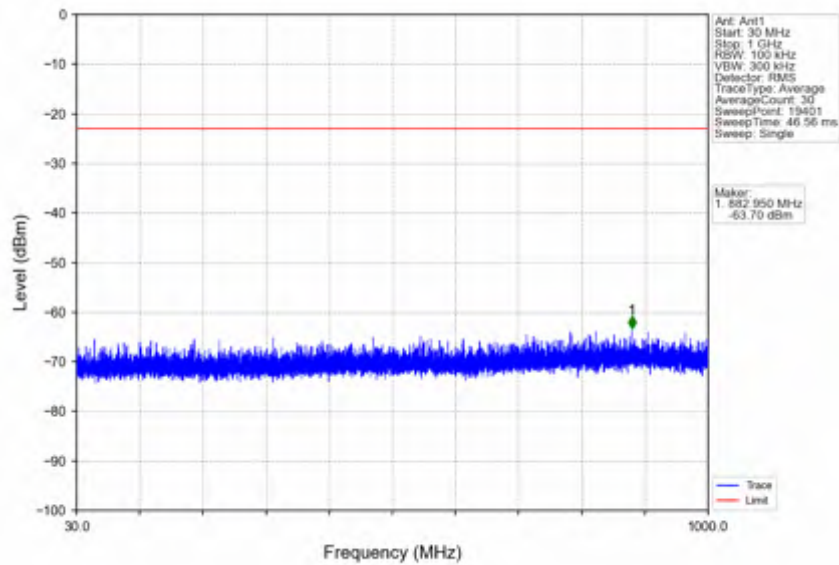
n66_30kHz_SISO_NTNV_30MHz_CP-OFDM QPSK_1725MHz_Outer_Full
