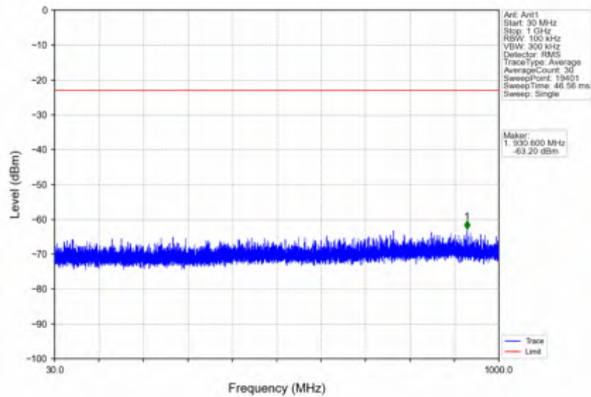
n66_30kHz_SISO_NTNV_20MHz_DFT-s-OFDM QPSK_1770MHz_Edge_1RB_Right
