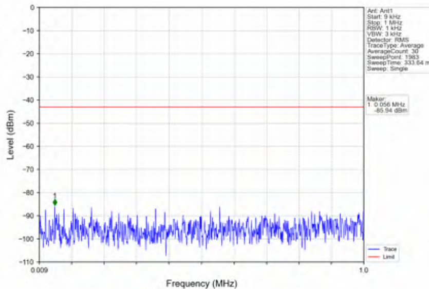
n66_30kHz_SISO_NTNV_20MHz_DFT-s-OFDM QPSK_1770MHz_Outer_Full
