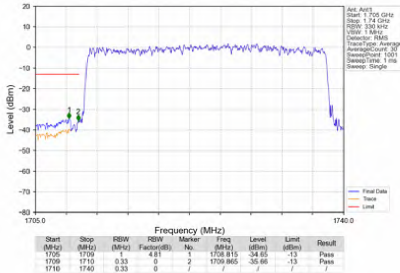
n66_30kHz_SISO_NTNV_30MHz_DFT-s-OFDM QPSK_1725MHz_Outer_Full
