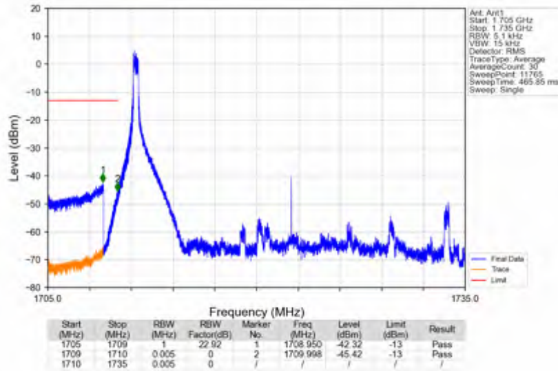
n66_30kHz_SISO_NTNV_25MHz_DFT-s-OFDM PI/2 BPSK_1722.5MHz_Inner_1RB_Left
