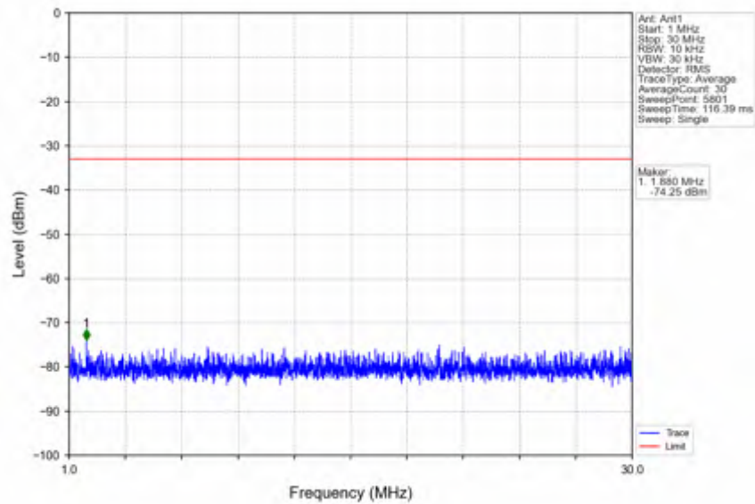
n66_30kHz_SISO_NTNV_25MHz_CP-OFDM QPSK_1767.5MHz_Inner_1RB_Right
