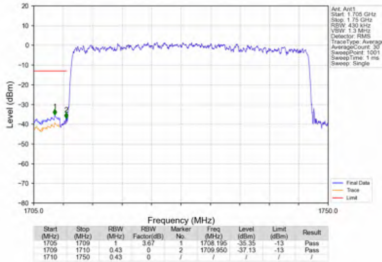
n66_30kHz_SISO_NTNV_40MHz_DFT-s-OFDM QPSK_1730MHz_Outer_Full
