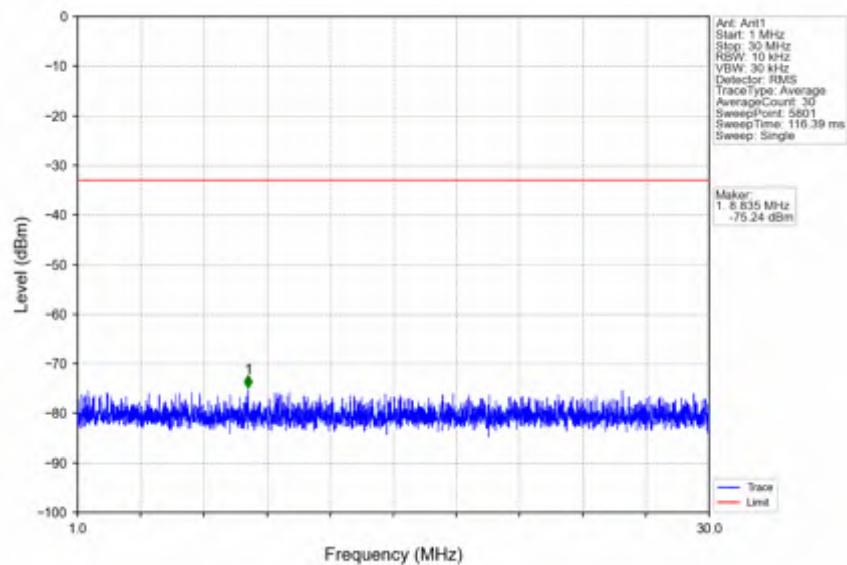
n66_30kHz_SISO_NTNV_30MHz_DFT-s-OFDM QPSK_1725MHz_Edge_1RB_Left
