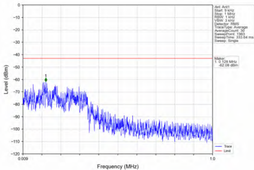
n66_30kHz_SISO_NTNV_30MHz_DFT-s-OFDM_PI/2_BPSK_1725MHz_Edge_1RB_Left
