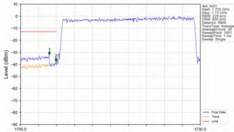
n66_30kHz_SISO_NTNV_20MHz_CP-OFDM QPSK_1720MHz_Outer_Full
