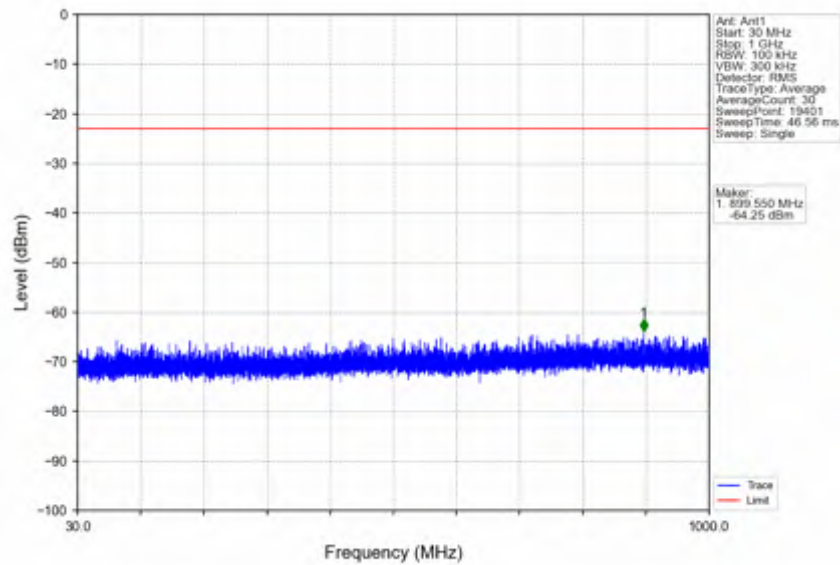
n66_30kHz_SISO_NTNV_40MHz_CP-OFDM QPSK_1730MHz_Outer_Full
