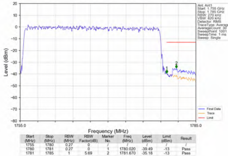
n66_30kHz_SISO_NTNV_25MHz_DFT-s-OFDM QPSK_1767.5MHz_Outer_Full
