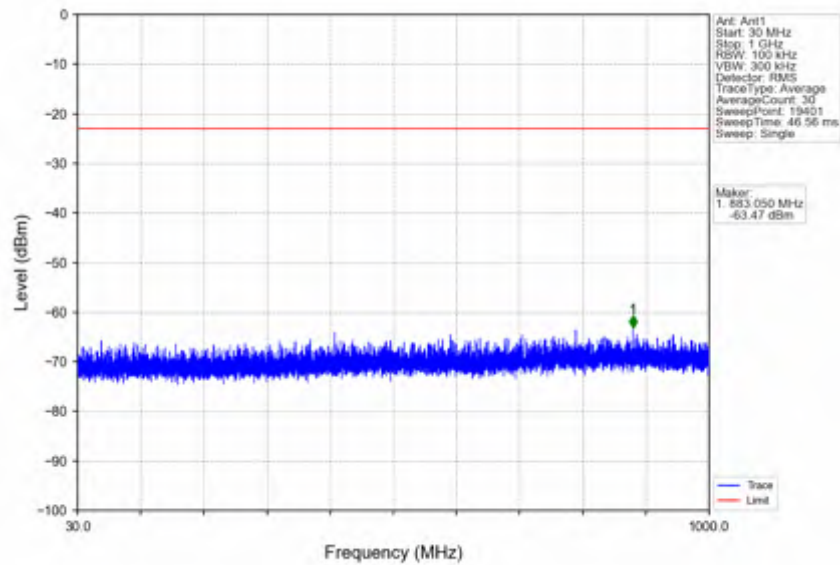
n66_30kHz_SISO_NTNV_25MHz_CP-OFDM QPSK_1722.5MHz_Outer_Full
