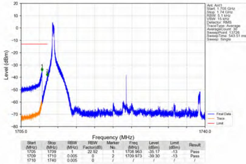
n66_30kHz_SISO_NTNV_30MHz_DFT-s-OFDM_PI/2_BPSK_1725MHz_Edge_1RB_Left
