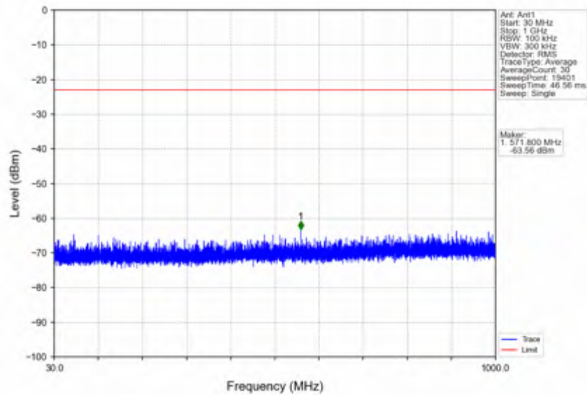
n66_30kHz_SISO_NTNV_40MHz_DFT-s-OFDM QPSK_1730MHz_Edge_1RB_Left
