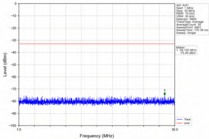
n66_30kHz_SISO_NTNV_30MHz_CP-OFDM QPSK_1725MHz_Edge_1RB_Left
