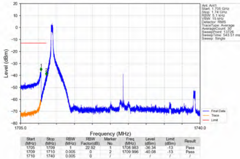
n66_30kHz_SISO_NTNV_30MHz_DFT-s-OFDM QPSK_1725MHz_Edge_1RB_Left
