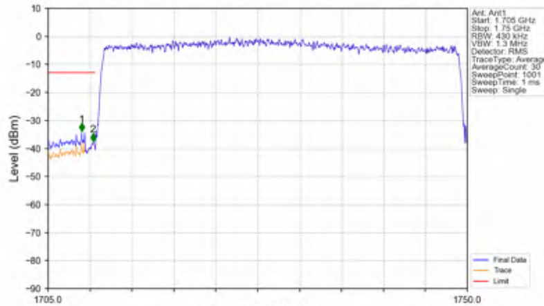
n66_30kHz_SISO_NTNV_40MHz_CP-OFDM QPSK_1730MHz_Outer_Full
