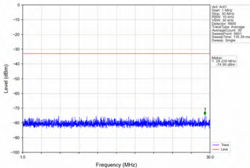
n66_30kHz_SISO_NTNV_25MHz_DFT-s-OFDM PI/2 BPSK_1767.5MHz_Outer_Full
