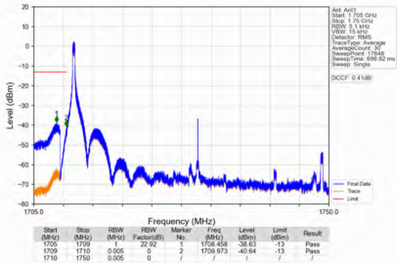
n66_30kHz_SISO_NTNV_40MHz_DFT-s-OFDM QPSK_1730MHz_Edge_1RB_Left
