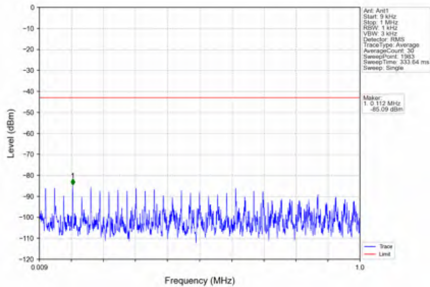
n66_30kHz_SISO_NTNV_40MHz_DFT-s-OFDM PI/2 BPSK_1760MHz_Outer_Full
