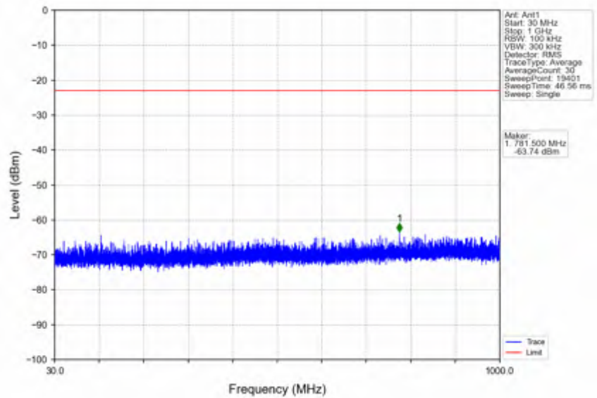
n66_30kHz_SISO_NTNV_25MHz_DFT-s-OFDM QPSK_1745MHz_Edge_1RB_Left
