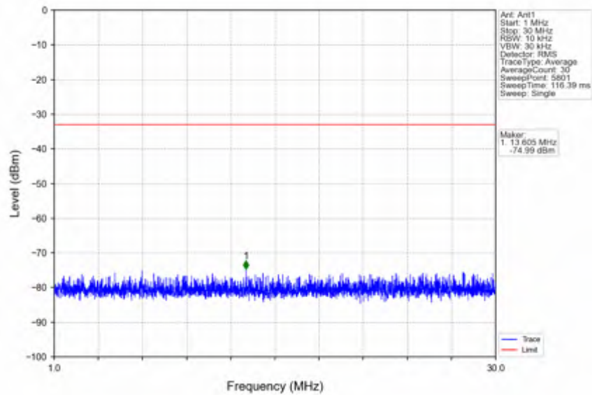
n66_30kHz_SISO_NTNV_25MHz_CP-OFDM QPSK_1722.5MHz_Inner_1RB_Left
