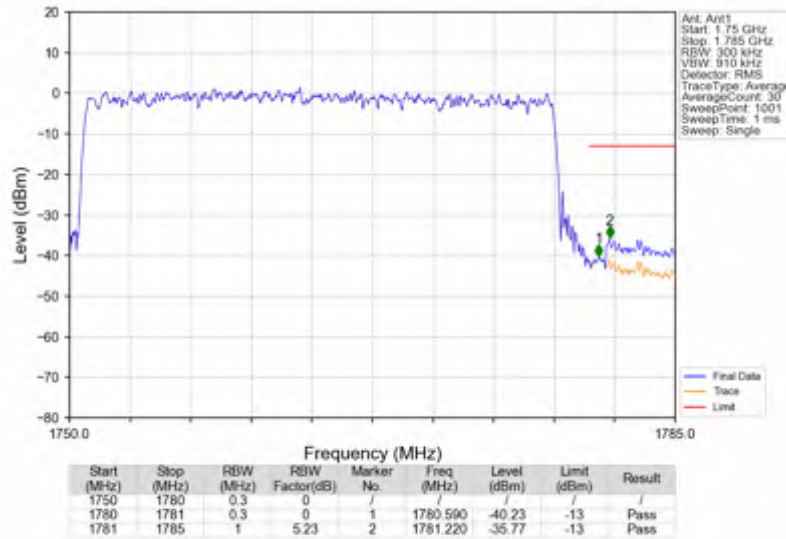
n66_30kHz_SISO_NTNV_30MHz_DFT-s-OFDM QPSK_1765MHz_Outer_Full
