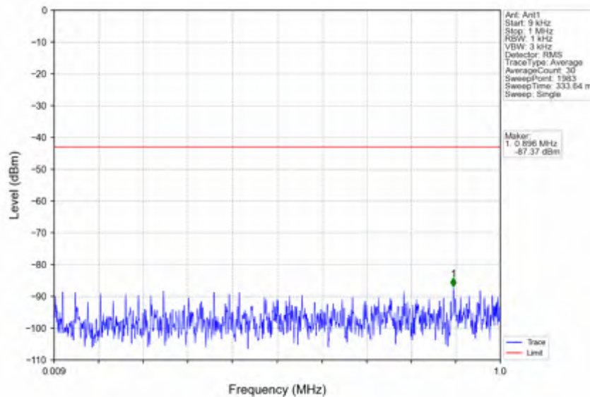
n66_30kHz_SISO_NTNV_25MHz_DFT-s-OFDM_QPSK_1722.5MHz_Outer_Full
