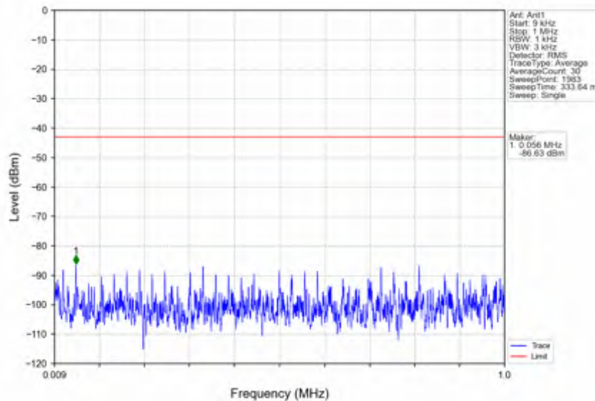
n66_30kHz_SISO_NTNV_40MHz_DFT-s-OFDM QPSK_1760MHz_Outer_Full
