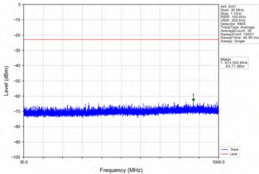
n66_30kHz_SISO_NTNV_25MHz_DFT-s-OFDM QPSK_1767.5MHz_Inner_1RB_Right
