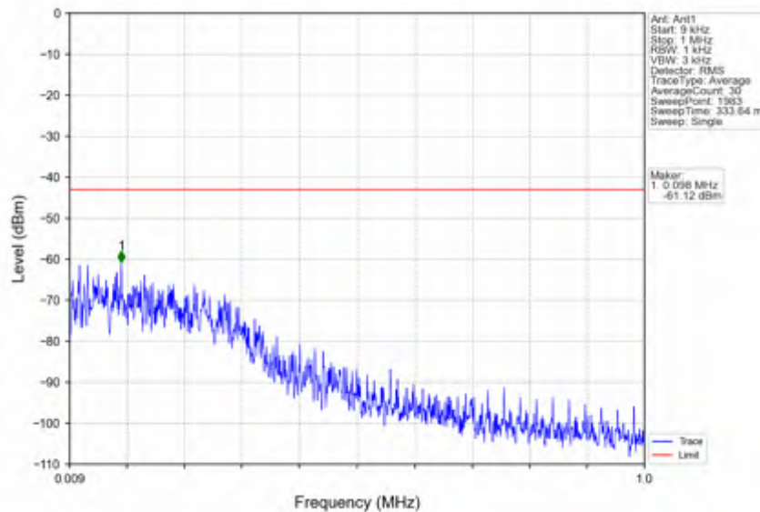
n66_30kHz_SISO_NTNV_20MHz_CP-OFDM QPSK_1770MHz_Edge_1RB_Right
