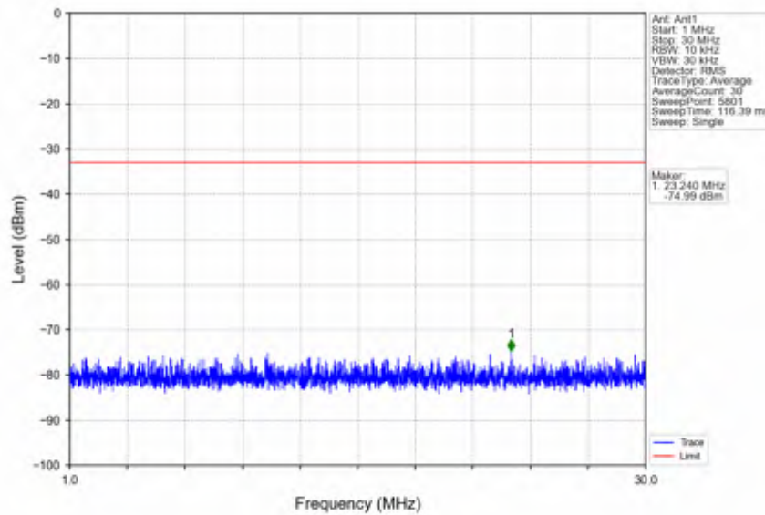
n66_30kHz_SISO_NTNV_30MHz_CP-OFDM QPSK_1765MHz_Edge_1RB_Right
