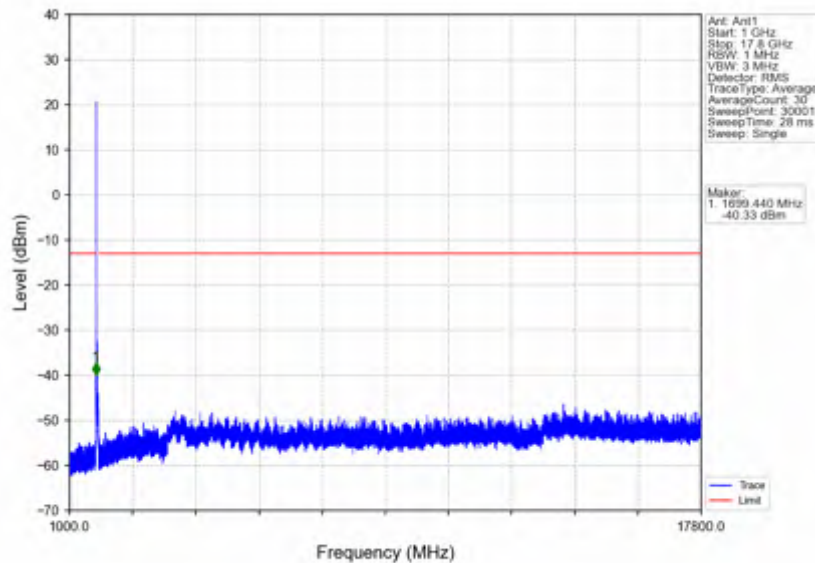
n66_30kHz_SISO_NTNV_25MHz_DFT-s-OFDM QPSK_1722.5MHz_Edge_1RB_Left
