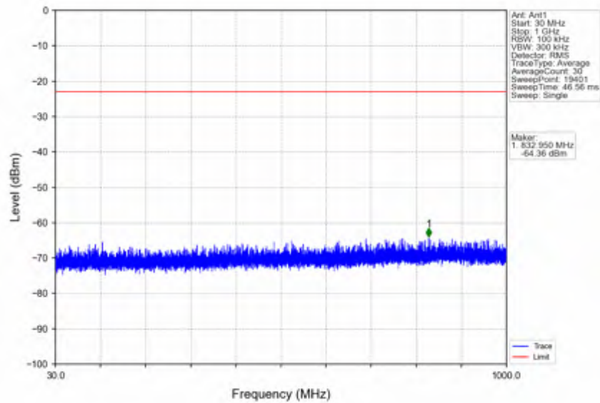
n66_30kHz_SISO_NTNV_25MHz_DFT-s-OFDM QPSK_1722.5MHz_Inner_1RB_Left
