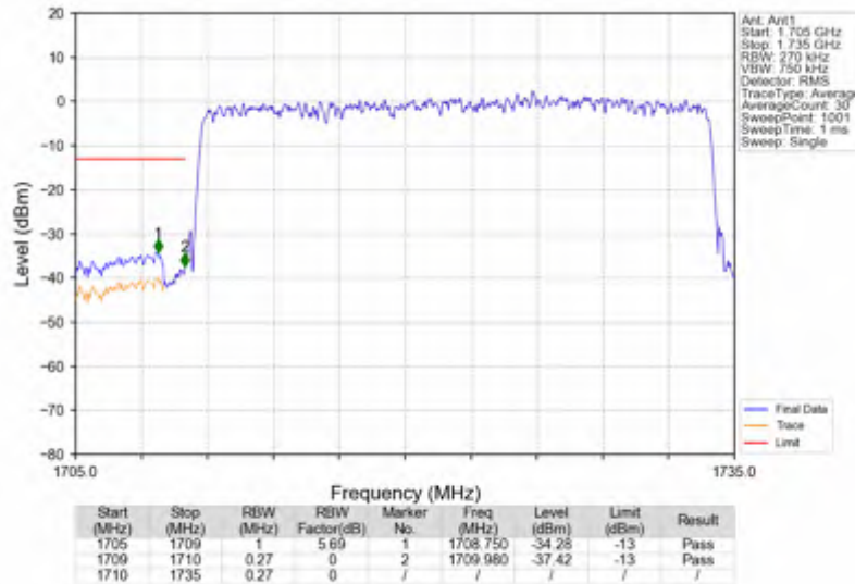
n66_30kHz_SISO_NTNV_25MHz_DFT-s-OFDM_QPSK_1722.5MHz_Outer_Full
