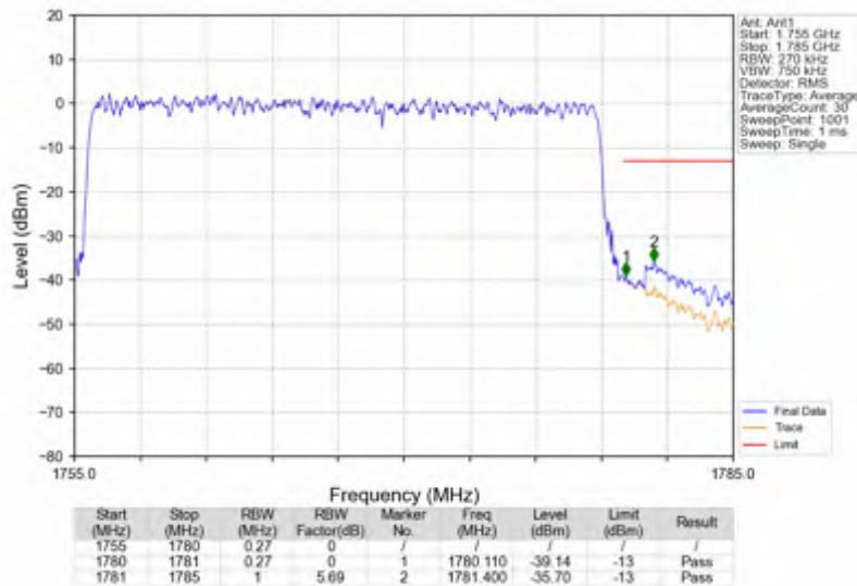
n66_30kHz_SISO_NTNV_25MHz_DFT-s-OFDM PI/2 BPSK_1767.5MHz_Outer_Full
