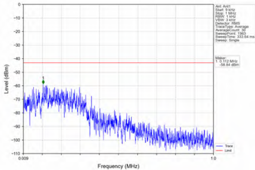
n66_30kHz_SISO_NTNV_25MHz_DFT-s-OFDM QPSK_1767.5MHz_Inner_1RB_Right
