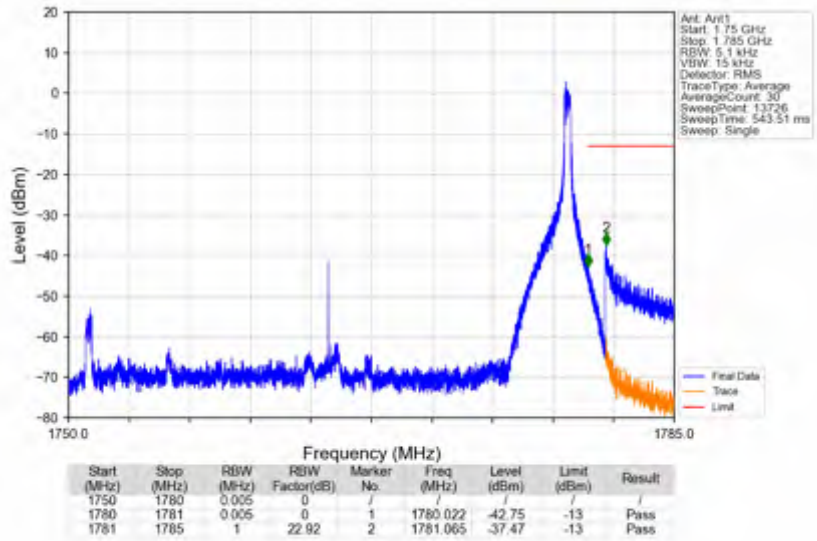
n66_30kHz_SISO_NTNV_30MHz_DFT-s-OFDM QPSK_1765MHz_Edge_1RB_Right
