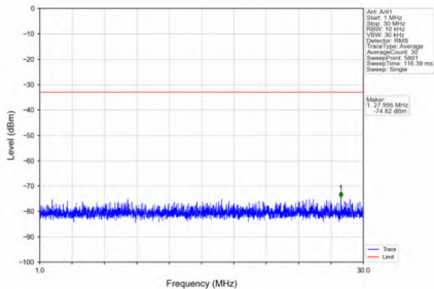
n66_30kHz_SISO_NTNV_25MHz_DFT-s-OFDM PI/2 BPSK_1722.5MHz_Outer_Full
