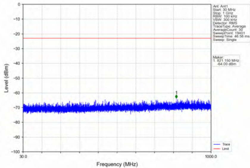
n66_30kHz_SISO_NTNV_40MHz_DFT-s-OFDM QPSK_1760MHz_Edge_1RB_Right
