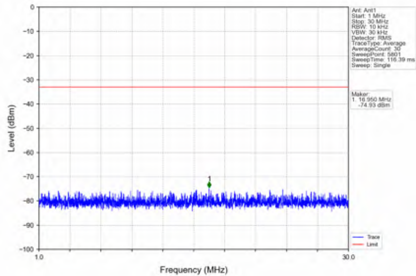
n66_30kHz_SISO_NTNV_20MHz_DFT-s-OFDM QPSK_1720MHz_Outer_Full
