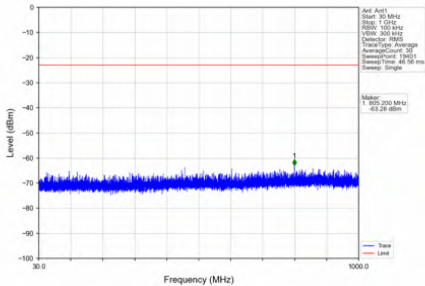
n66_30kHz_SISO_NTNV_30MHz_DFT-s-OFDM QPSK_1765MHz_Edge_1RB_Right
