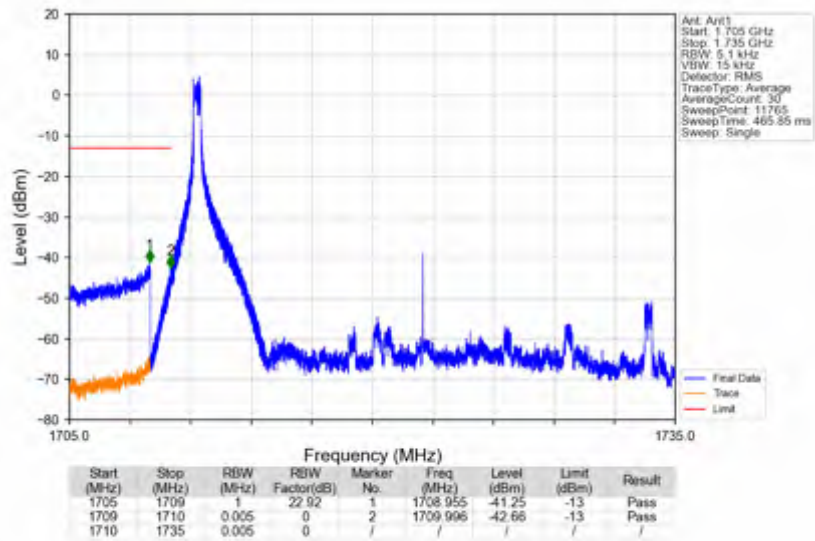
n66_30kHz_SISO_NTNV_25MHz_DFT-s-OFDM QPSK_1722.5MHz_Inner_1RB_Left
