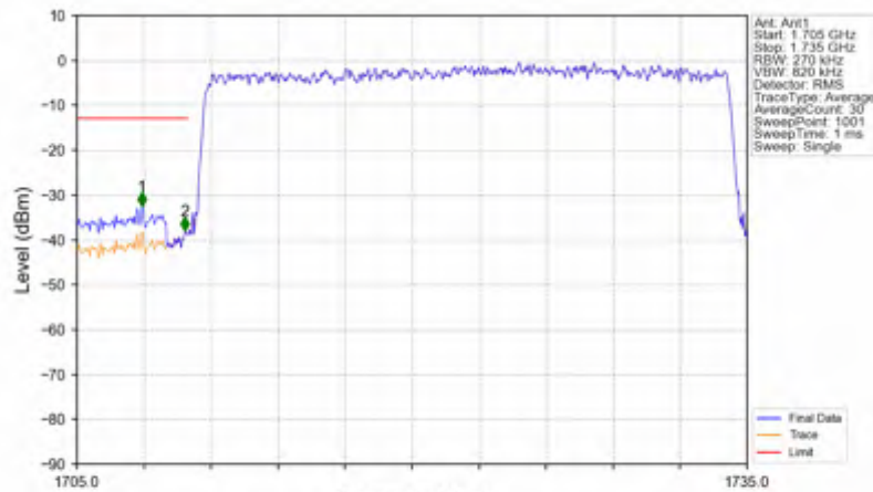
n66_30kHz_SISO_NTV_25MHz_CP-OFDM QPSK_1722.5MHz_Outer_Full
