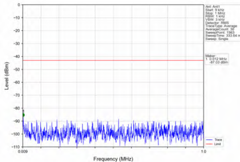
n66_30kHz_SISO_NTNV_30MHz_DFT-s-OFDM QPSK_1765MHz_Outer_Full
