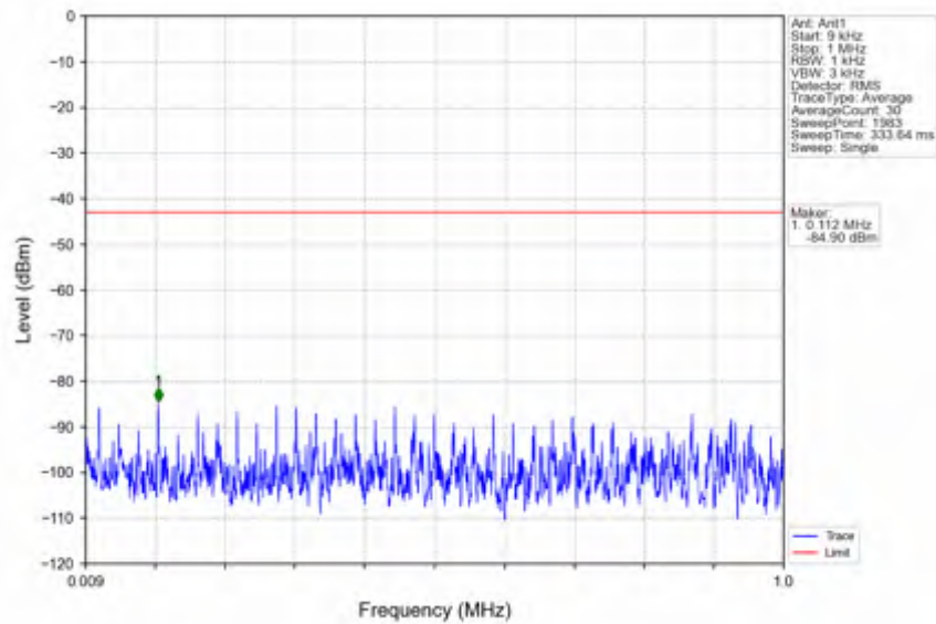
n66_30kHz_SISO_NTNV_40MHz_DFT-s-OFDM PI/2 BPSK_1730MHz_Outer_Full
