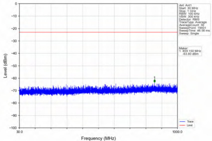
n66_30kHz_SISO_NTV_25MHz_CP-OFDM QPSK_1722.5MHz_Edge_1RB_Left
