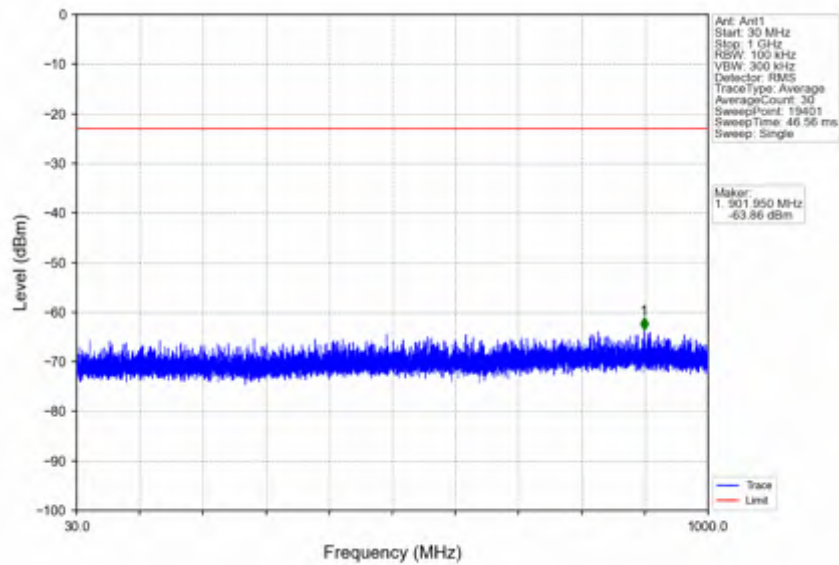
n66_30kHz_SISO_NTNV_30MHz_CP-OFDM QPSK_1745MHz_Edge_1RB_Left
