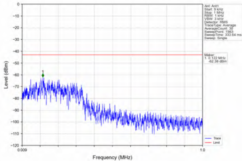
n66_30kHz_SISO_NTNV_25MHz_DFT-s-OFDM QPSK_1722.5MHz_Edge_1RB_Left
