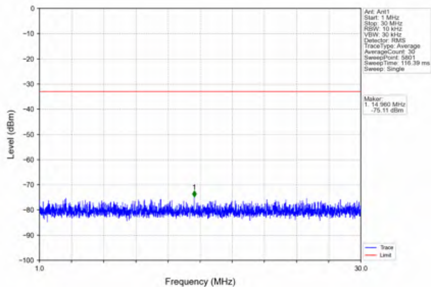
n66_30kHz_SISO_NTNV_40MHz_DFT-s-OFDM QPSK_1730MHz_Edge_1RB_Left
