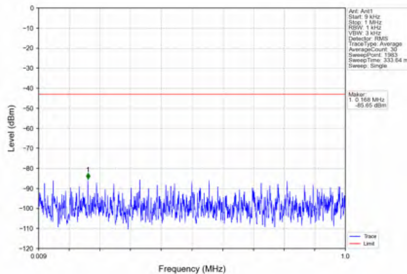
n66_30kHz_SISO_NTNV_40MHz_DFT-s-OFDM QPSK_1730MHz_Outer_Full
