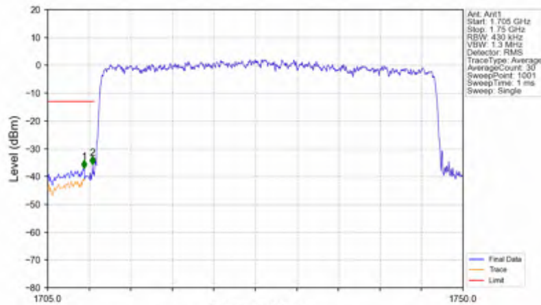
n66_30kHz_SISO_NTNV_40MHz_DFT-s-OFDM PI/2 BPSK_1730MHz_Outer_Full
