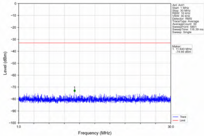
n66_30kHz_SISO_NTNV_25MHz_DFT-s-OFDM_QPSK_1722.5MHz_Outer_Full
