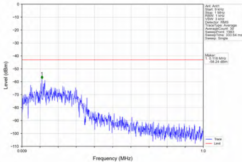
n66_30kHz_SISO_NTNV_25MHz_DFT-s-OFDM_QPSK_1722.5MHz_Inner_1RB_Left
