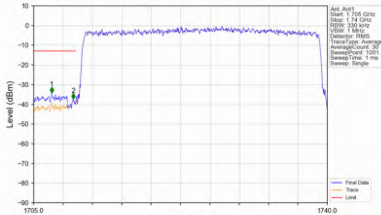
n66_30kHz_SISO_NTNV_30MHz_CP-OFDM QPSK_1725MHz_Outer_Full
