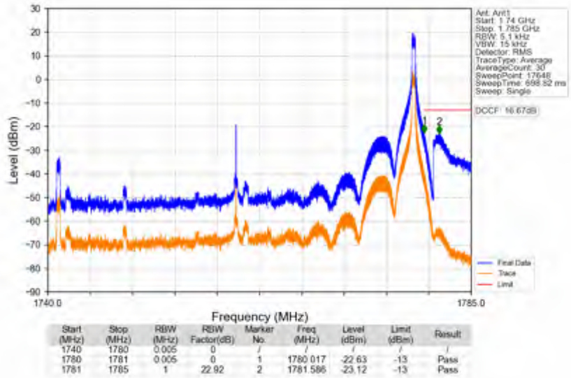
n66_30kHz_SISO_NTNV_40MHz_DFT-s-OFDM QPSK_1760MHz_Edge_1RB_Right
