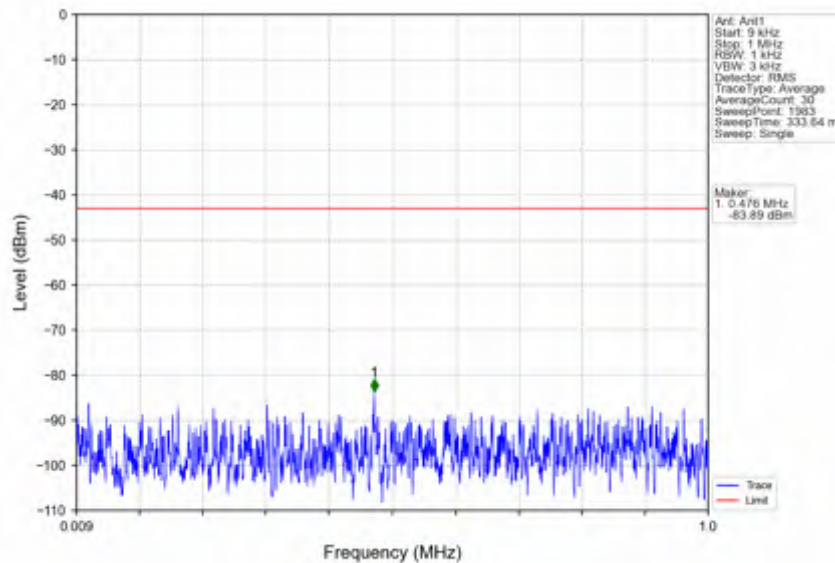
n66_30kHz_SISO_NTNV_25MHz_DFT-s-OFDM QPSK_1767.5MHz_Outer_Full
