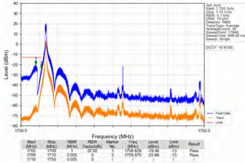
n66_30kHz_SISO_NTNV_40MHz_DFT-s-OFDM_PI/2_BPSK_1730MHz_Edge_1RB_Left
