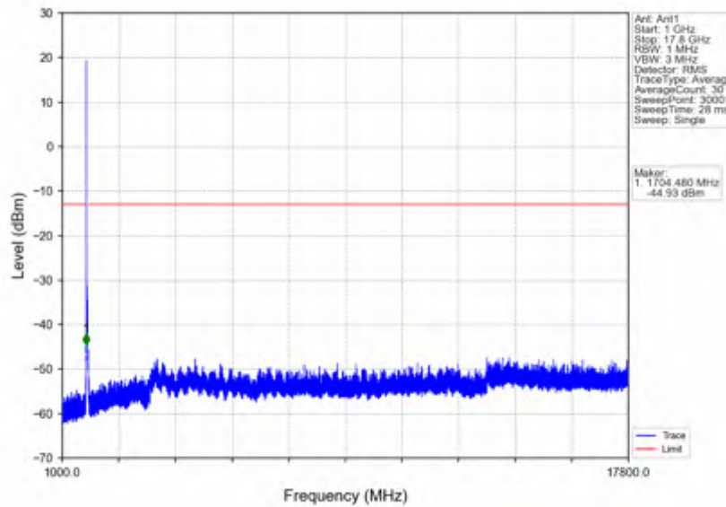
n66_30kHz_SISO_NTNV_40MHz_CP-OFDM QPSK_1730MHz_Outer_Full
