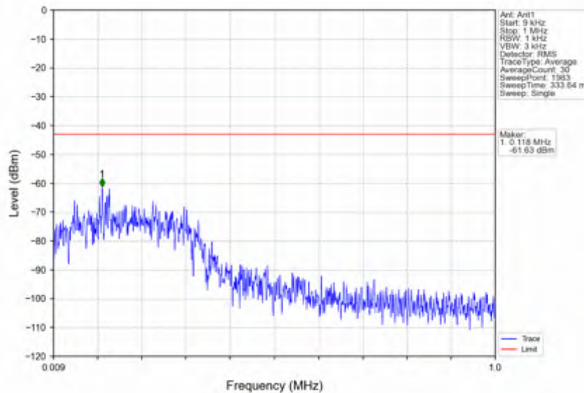
n66_30kHz_SISO_NTNV_40MHz_DFT-s-OFDM QPSK_1745MHz_Edge_1RB_Left
