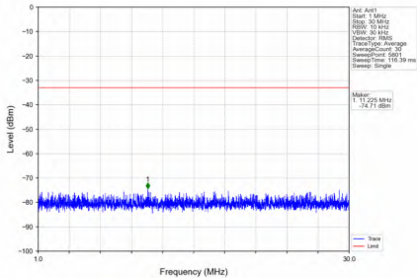
n66_30kHz_SISO_NTNV_25MHz_DFT-s-OFDM_QPSK_1767.5MHz_Outer_Full
