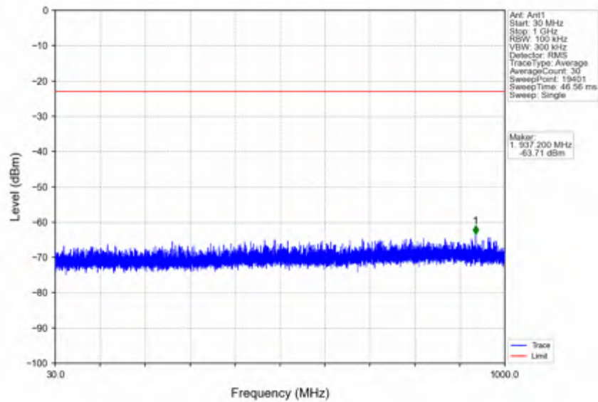
n66_30kHz_SISO_NTNV_30MHz_DFT-s-OFDM_QPSK_1725MHz_Inner_1RB_Left
