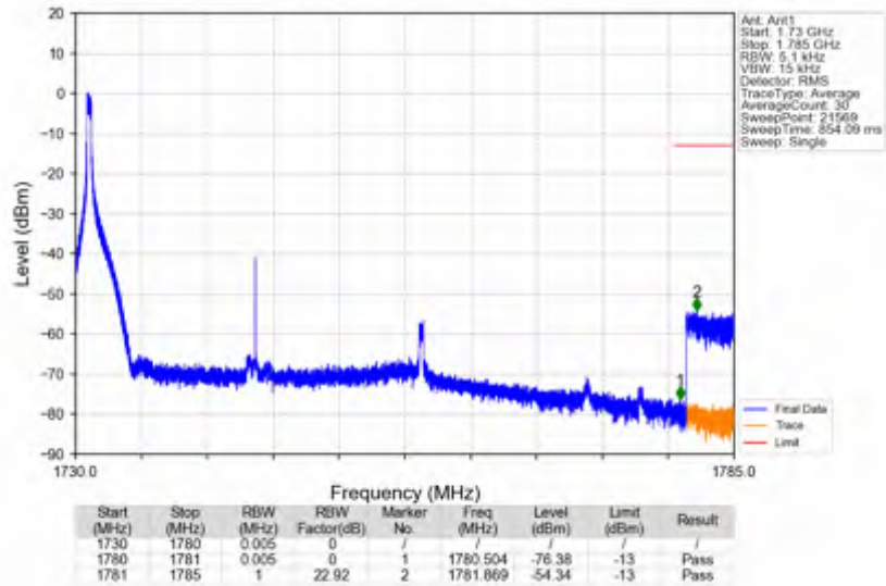
n66_30kHz_SISO_NTNV_30MHz_CP-OFDM QPSK_1745MHz_Edge_1RB_Left
