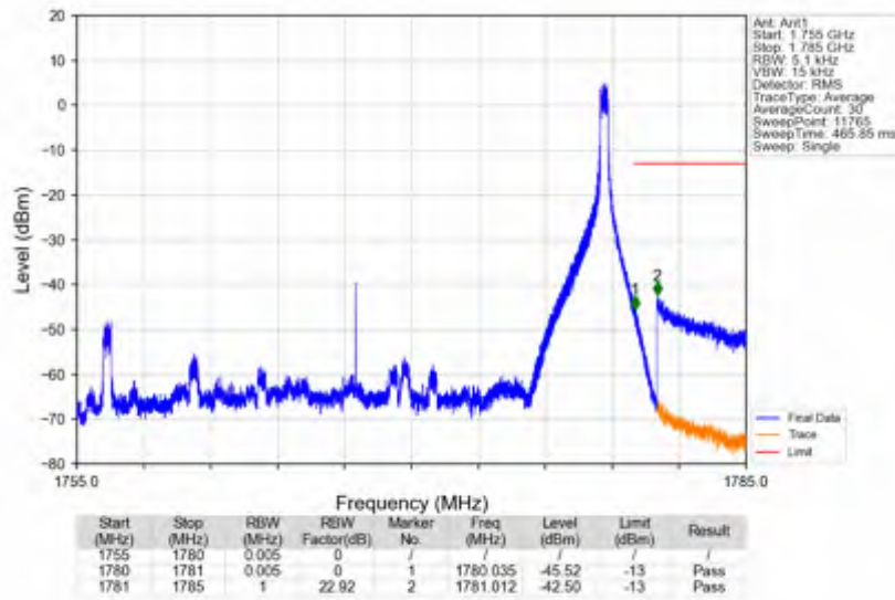
n66_30kHz_SISO_NTNV_25MHz_DFT-s-OFDM QPSK_1767.5MHz_Inner_1RB_Right
