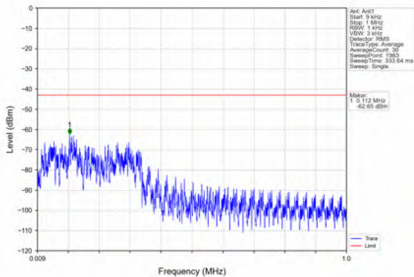
n66_30kHz_SISO_NTNV_40MHz_DFT-s-OFDM_PI/2_BPSK_1730MHz_Edge_1RB_Left
