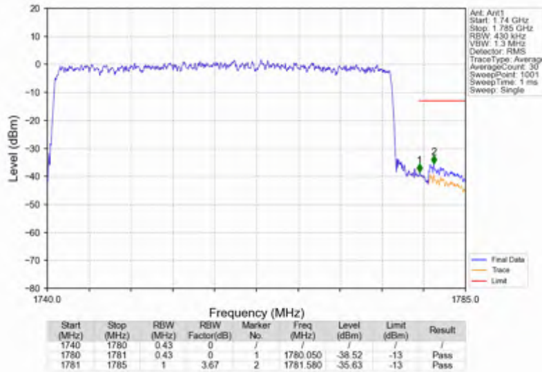
n66_30kHz_SISO_NTNV_40MHz_DFT-s-OFDM QPSK_1760MHz_Outer_Full
