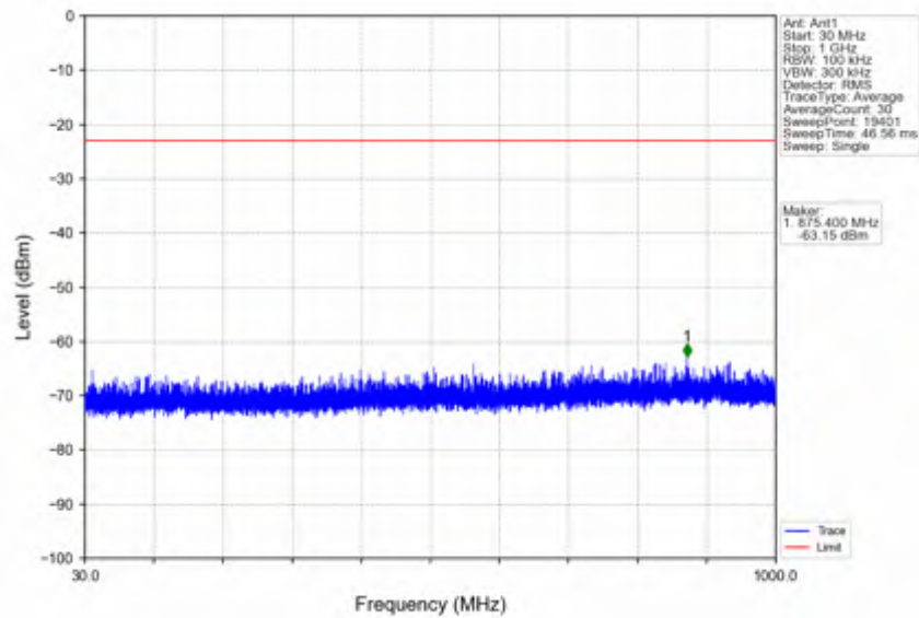
n66_30kHz_SISO_NTNV_20MHz_CP-OFDM QPSK_1720MHz_Outer_Full
