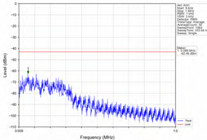
n66_30kHz_SISO_NTNV_40MHz_CP-OFDM QPSK_1730MHz_Edge_1RB_Left
