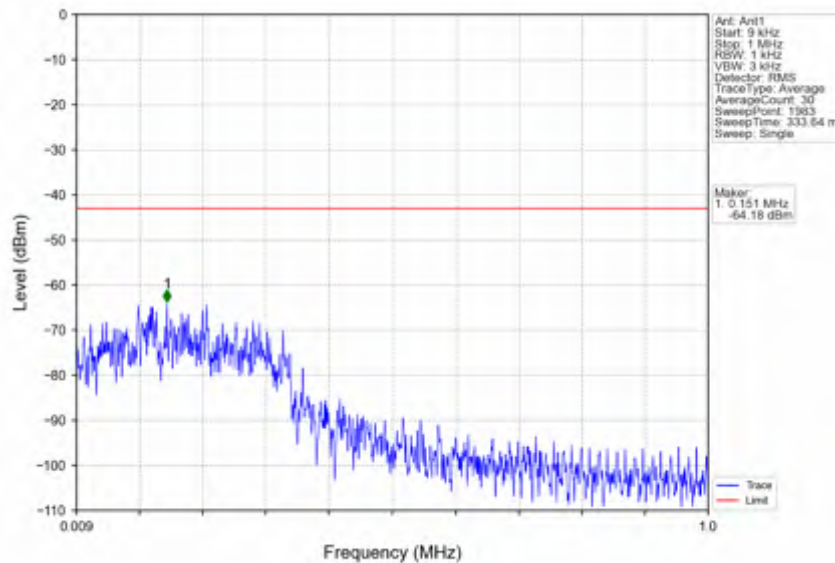
n66_30kHz_SISO_NTNV_30MHz_DFT-s-OFDM QPSK_1745MHz_Edge_1RB_Left
