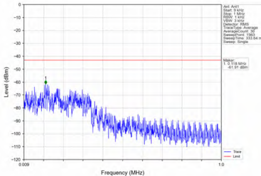
n66_30kHz_SISO_NTNV_25MHz_DFT-s-OFDM PI/2 BPSK_1767.5MHz_Edge_1RB_Right
