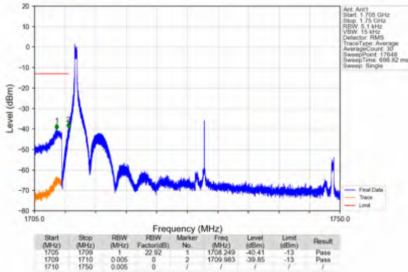
n66_30kHz_SISO_NTNV_40MHz_CP-OFDM QPSK_1730MHz_Edge_1RB_Left
