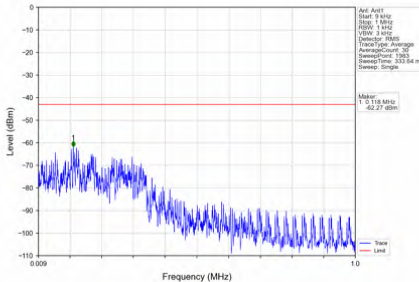
n66_30kHz_SISO_NTNV_30MHz_DFT-s-OFDM PI/2 BPSK_1765MHz_Edge_1RB_Right
