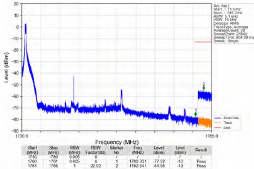
n66_30kHz_SISO_NTNV_30MHz_DFT-s-OFDM QPSK_1745MHz_Edge_1RB_Left
