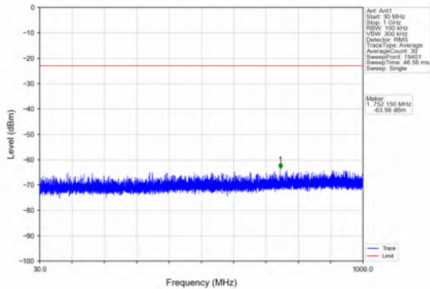
n66_30kHz_SISO_NTNV_25MHz_DFT-s-OFDM QPSK_1722.5MHz_Edge_1RB_Left
