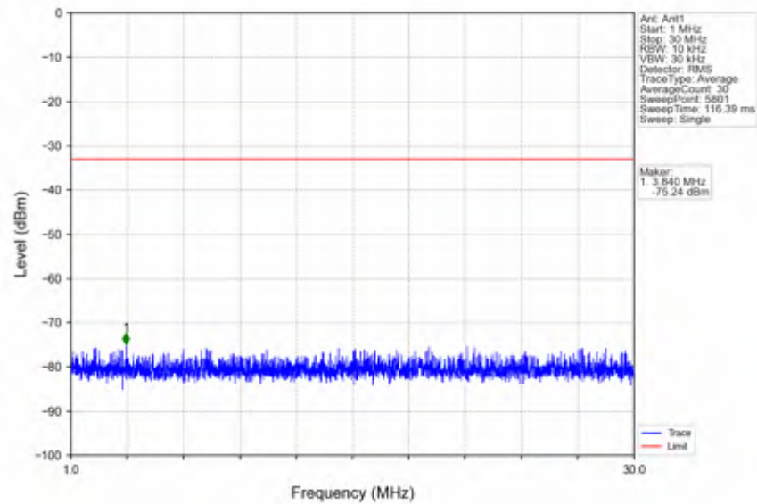
n66_30kHz_SISO_NTNV_40MHz_DFT-s-OFDM QPSK_1760MHz_Outer_Full
