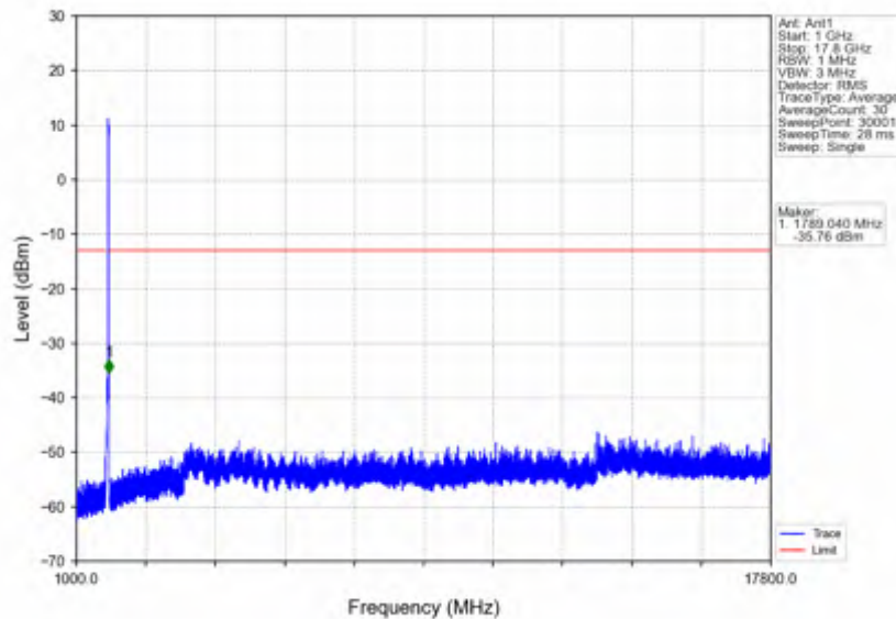
n66_30kHz_SISO_NTNV_25MHz_DFT-s-OFDM PI/2 BPSK_1767.5MHz_Outer_Full
