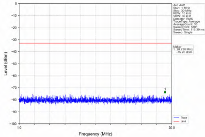
n66_30kHz_SISO_NTNV_40MHz_DFT-s-OFDM QPSK_1730MHz_Outer_Full
