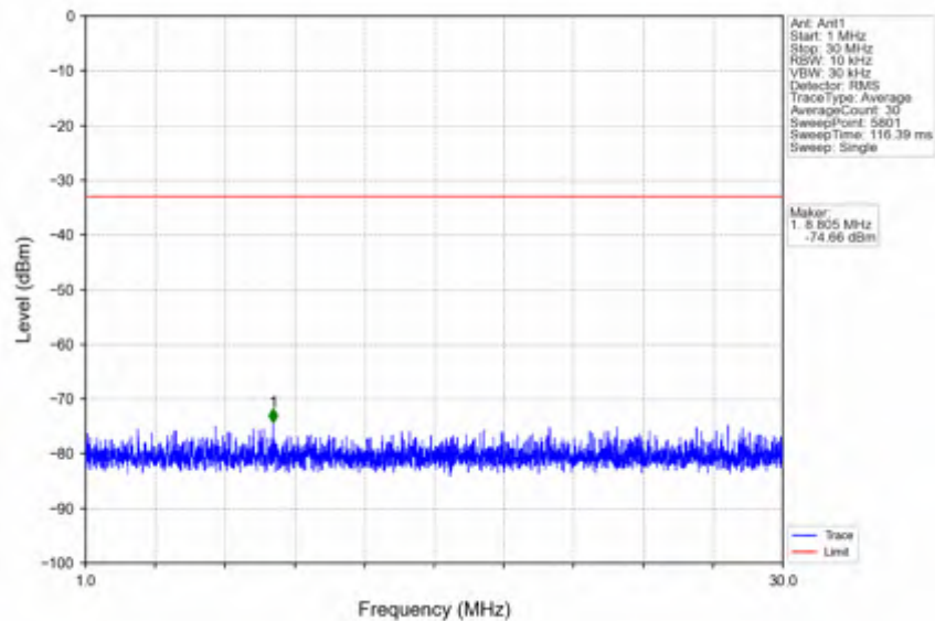
n66_30kHz_SISO_NTNV_30MHz_DFT-s-OFDM QPSK_1765MHz_Edge_1RB_Right
