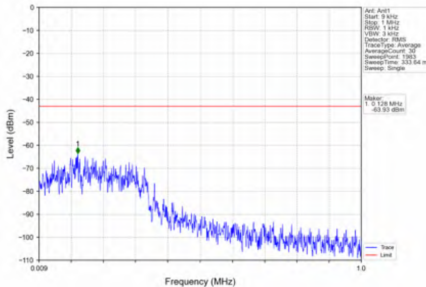
n66_30kHz_SISO_NTNV_25MHz_DFT-s-OFDM QPSK_1745MHz_Edge_1RB_Left
