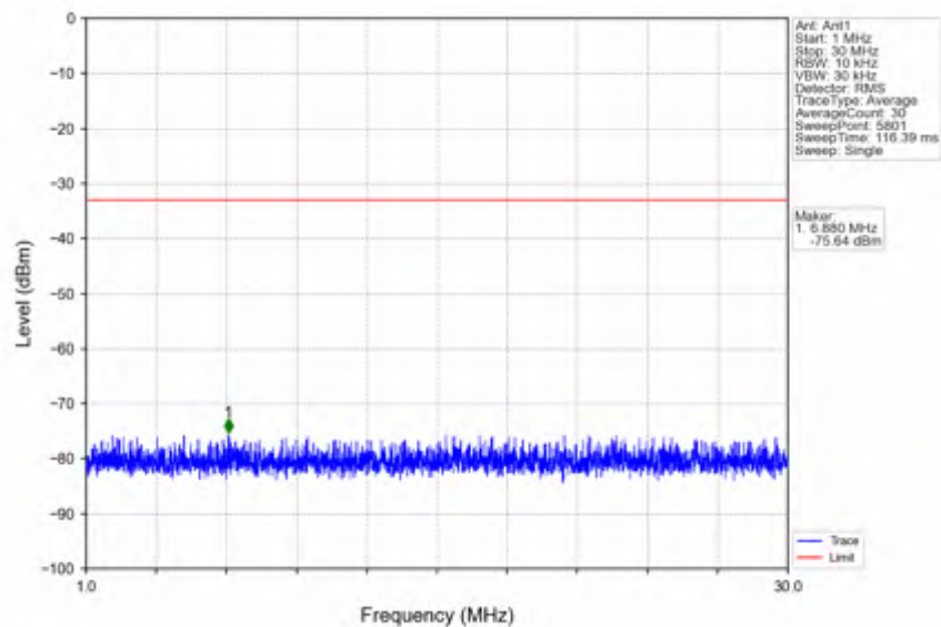
n66_30kHz_SISO_NTV_20MHz_DFT-s-OFDM_QPSK_1770MHz_Edge_1RB_Right
