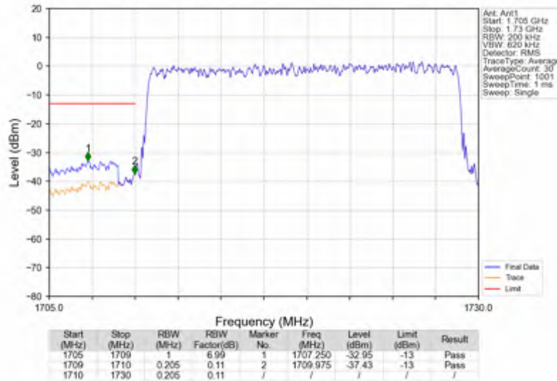
n66_30kHz_SISO_NTNV_20MHz_DFT-s-OFDM QPSK_1720MHz_Outer_Full
