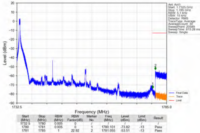
n66_30kHz_SISO_NTNV_25MHz_DFT-s-OFDM QPSK_1745MHz_Edge_1RB_Left
