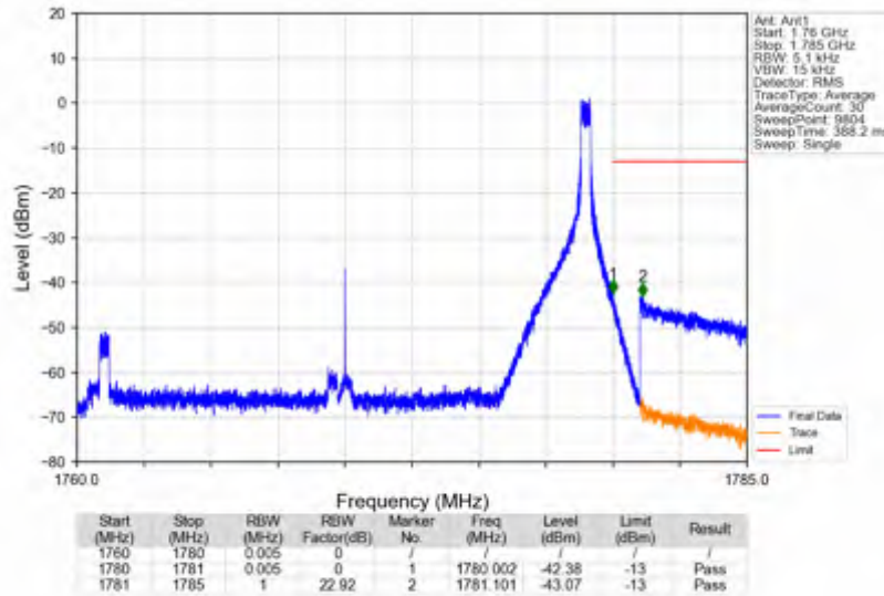
n66_30kHz_SISO_NTNV_20MHz_CP-OFDM QPSK_1770MHz_Edge_1RB_Right
