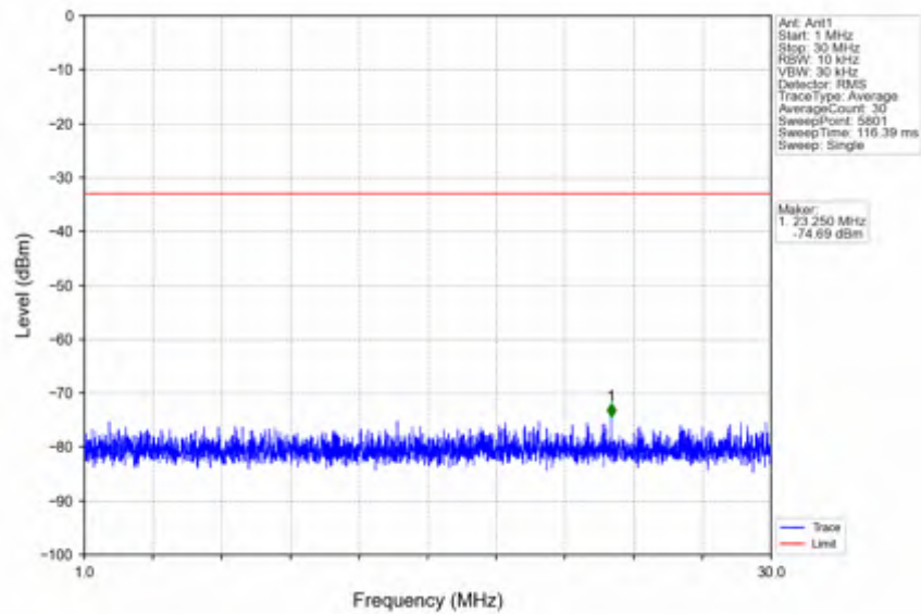
n66_30kHz_SISO_NTNV_25MHz_DFT-s-OFDM PI/2 BPSK_1767.5MHz_Inner_1RB_Right
