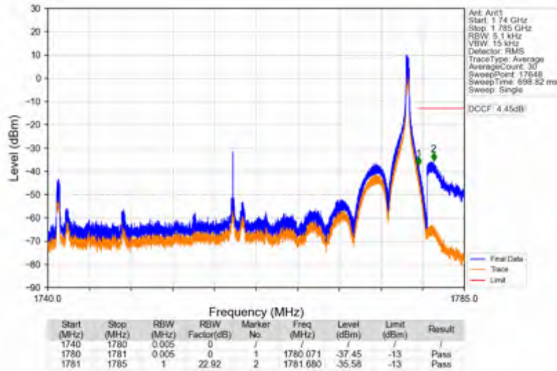
n66_30kHz_SISO_NTNV_40MHz_DFT-s-OFDM PI/2 BPSK_1760MHz_Edge_1RB_Right
