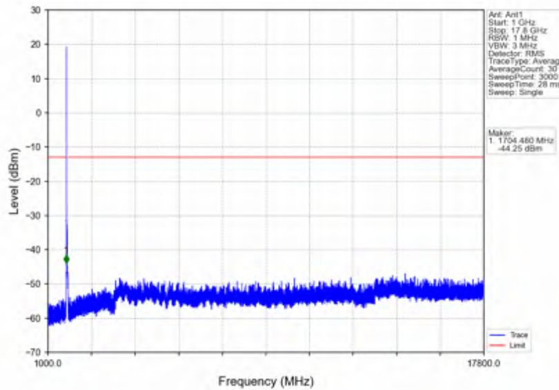
n66_30kHz_SISO_NTNV_30MHz_CP-OFDM QPSK_1725MHz_Outer_Full
