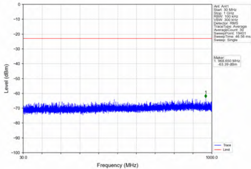
n66_30kHz_SISO_NTNV_30MHz_DFT-s-OFDM PI/2 BPSK_1765MHz_Outer_Full
