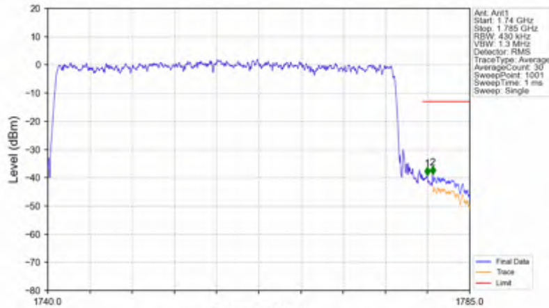
n66_30kHz_SISO_NTNV_40MHz_DFT-s-OFDM PI/2 BPSK_1760MHz_Outer_Full
