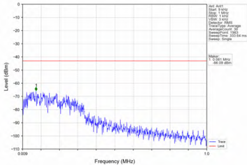
n66_30kHz_SISO_NTNV_40MHz_CP-OFDM QPSK_1745MHz_Edge_1RB_Left
