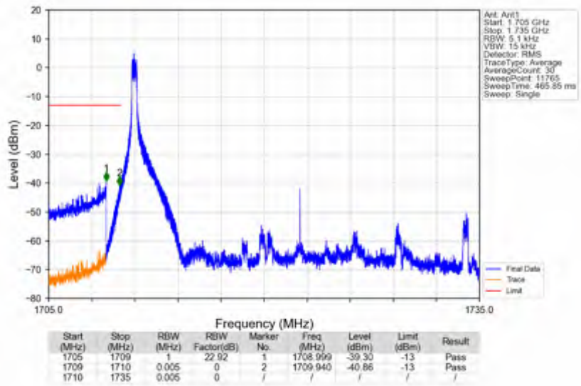
n66_30kHz_SISO_NTNV_25MHz_DFT-s-OFDM QPSK_1722.5MHz_Edge_1RB_Left
