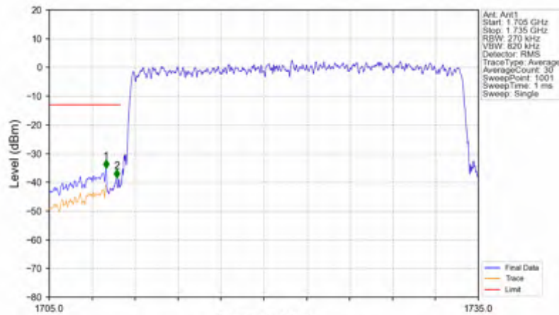
n66_30kHz_SISO_NTNV_25MHz_DFT-s-OFDM PI/2 BPSK_1722.5MHz_Outer_Full
