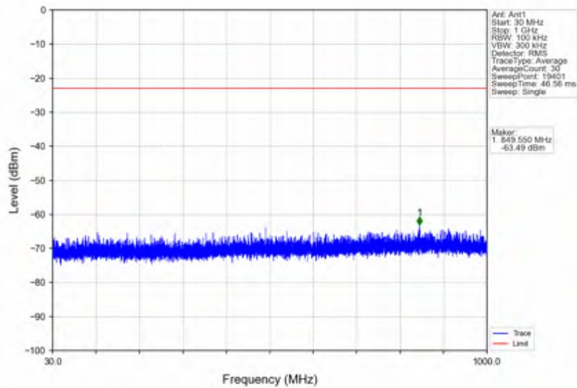
n66_30kHz_SISO_NTNV_30MHz_DFT-s-OFDM QPSK_1725MHz_Edge_1RB_Left
