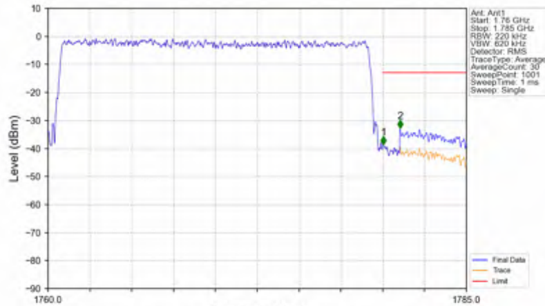
n66_30kHz_SISO_NTNV_20MHz_CP-OFDM QPSK_1770MHz_Outer_Full
