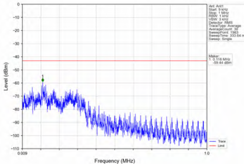
n66_30kHz_SISO_NTNV_15MHz_DFT-s-OFDM PI/2 BPSK_1772.5MHz_Inner_1RB_Right
