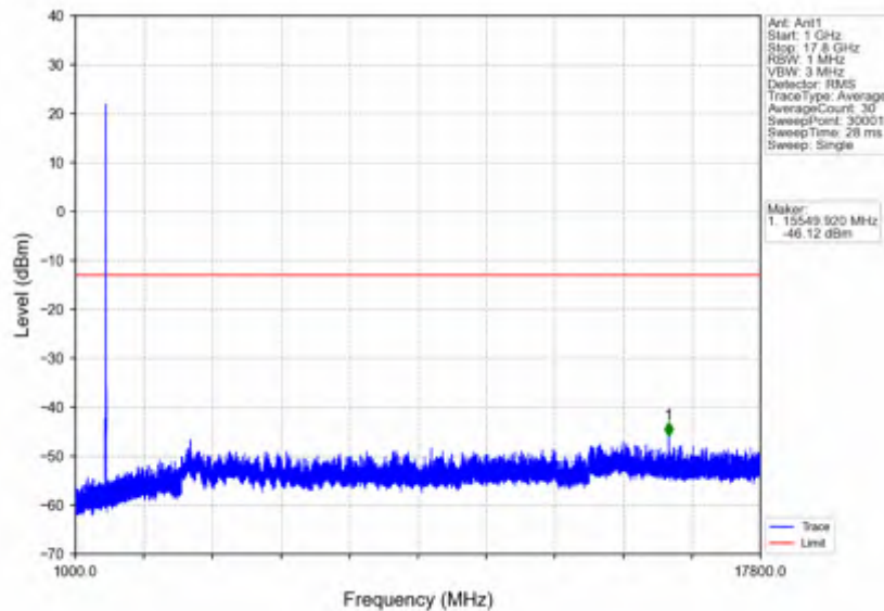
n66_30kHz_SISO_NTV_10MHz_DFT-s-OFDM PI/2 BPSK_1745MHz_Edge_1RB_Left
