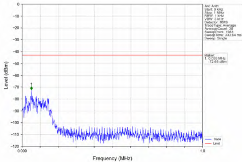
n66_15kHz_SISO_NTNV_40MHz_DFT-s-OFDM_QPSK_1760MHz_Edge_1RB_Right
