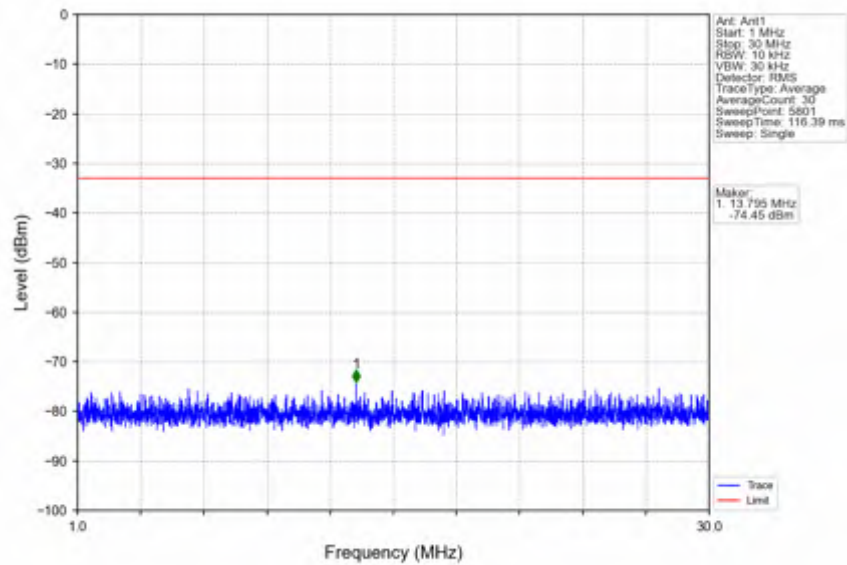
n66_15kHz_SISO_NTNV_30MHz_CP-OFDM QPSK_1765MHz_Edge_1RB_Right
