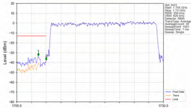
n66_30kHz_SISO_NTNV_20MHz_DFT-s-OFDM PI/2 BPSK_1720MHz_Outer_Full
