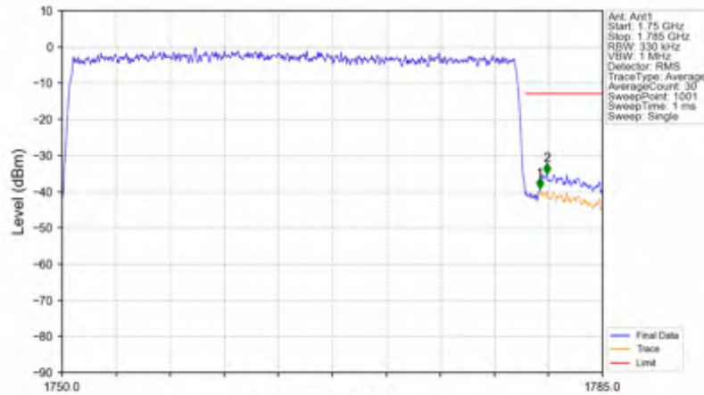
n66_15kHz_SISO_NTNV_30MHz_CP-OFDM QPSK_1765MHz_Outer_Full
