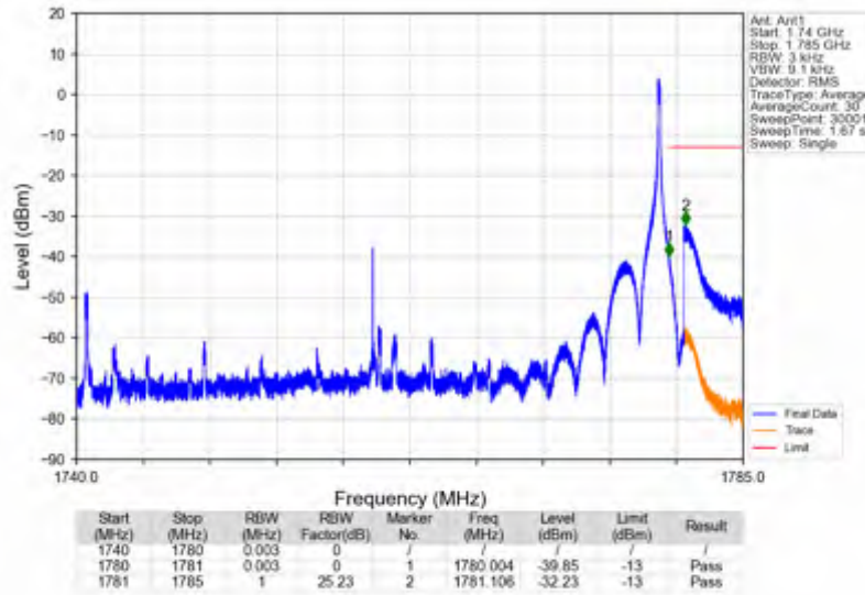
n66_15kHz_SISO_NTNV_40MHz_DFT-s-OFDM PI/2 BPSK_1760MHz_Edge_1RB_Right
