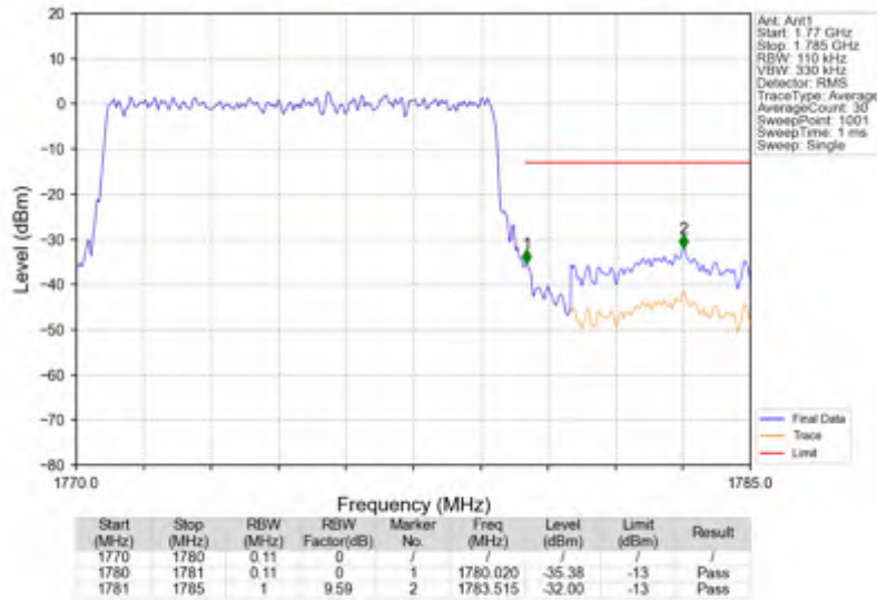
n66_30kHz_SISO_NTNV_10MHz_DFT-s-OFDM PI/2 BPSK_1775MHz_Outer_Full
