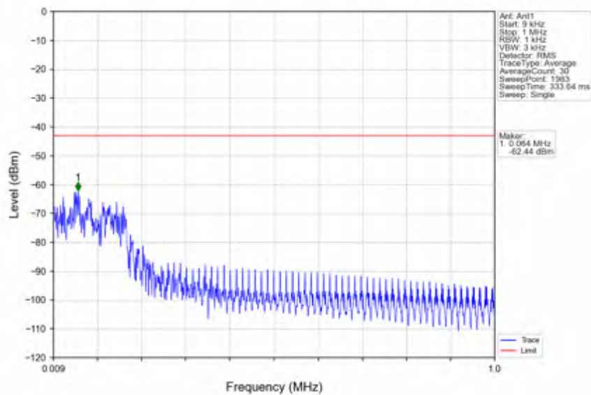
n66_15kHz_SISO_NTNV_40MHz_DFT-s-OFDM_PI/2_BPSK_1730MHz_Edge_1RB_Left
