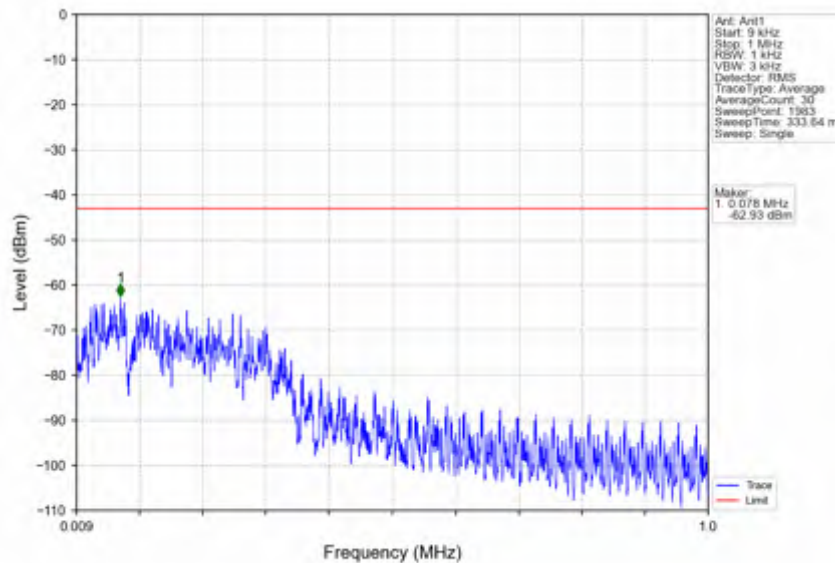
n66_30kHz_SISO_NTV_15MHz_CP-OFDM QPSK_1717.5MHz_Edge_1RB_Left
