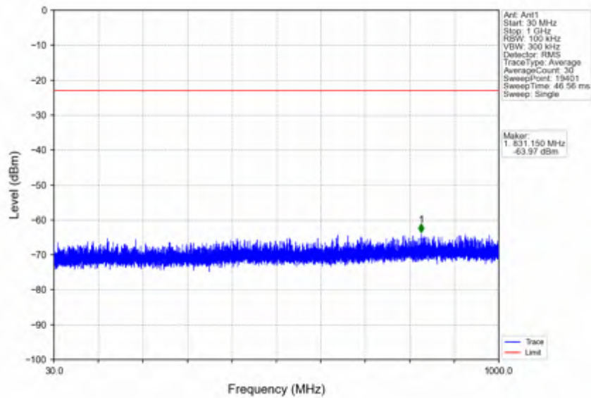
n66_30kHz_SISO_NTNV_15MHz_DFT-s-OFDM QPSK_1772.5MHz_Edge_1RB_Right
