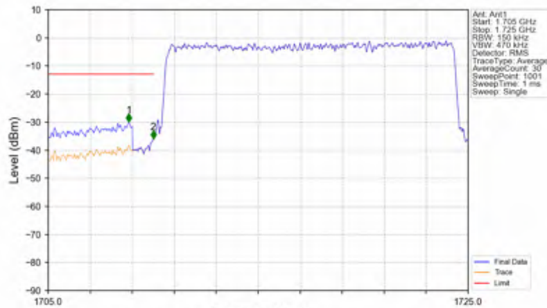
n66_30kHz_SISO_NTNV_15MHz_CP-OFDM QPSK_1717.5MHz_Outer_Full
