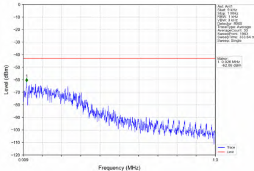
n66_30kHz_SISO_NTNV_15MHz_CP-OFDM QPSK_1772.5MHz_Edge_1RB_Right
