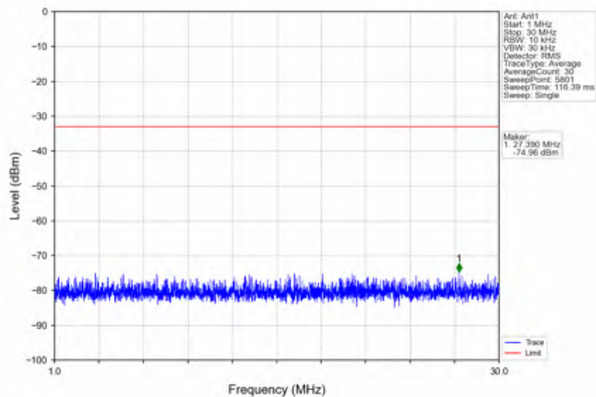
n66_15kHz_SISO_NTNV_30MHz_CP-OFDM QPSK_1745MHz_Edge_1RB_Left
