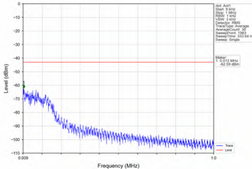
n66_15kHz_SISO_NTNV_40MHz_CP-OFDM QPSK_1730MHz_Edge_1RB_Left
