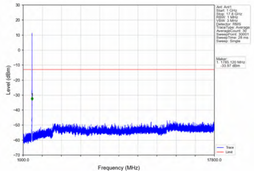
n66_30kHz_SISO_NTNV_15MHz_CP-OFDM QPSK_1772.5MHz_Outer_Full
