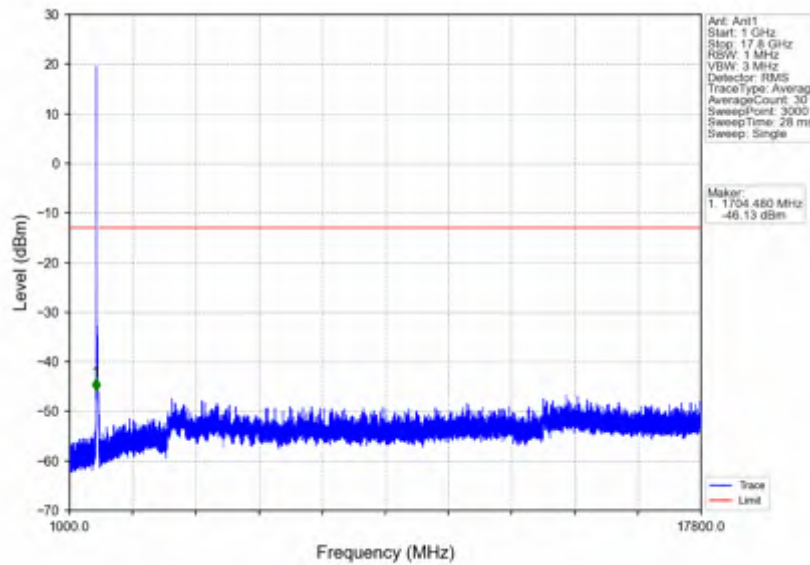
n66_15kHz_SISO_NTNV_40MHz_CP-OFDM QPSK_1730MHz_Outer_Full
