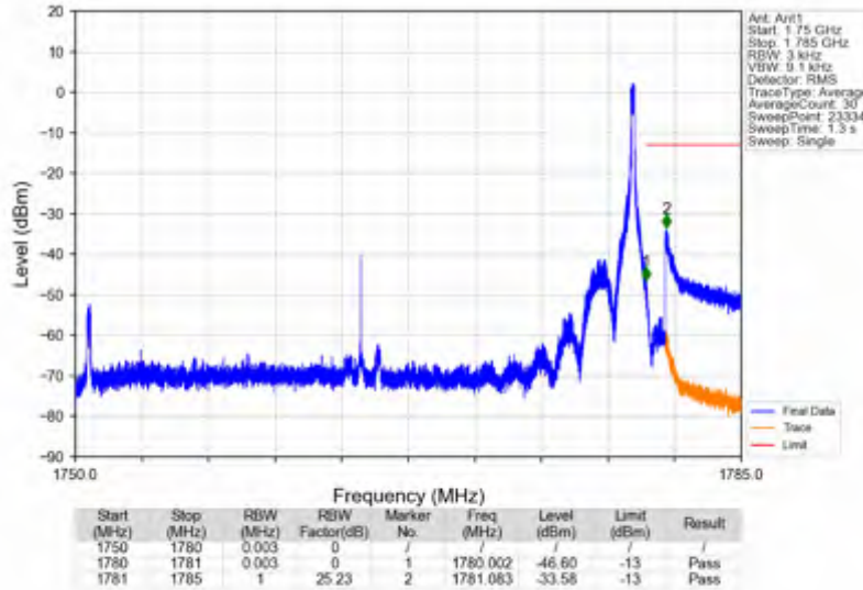
n66_15kHz_SISO_NTNV_30MHz_CP-OFDM QPSK_1765MHz_Edge_1RB_Right
