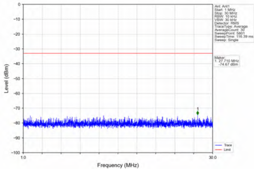
n66_15kHz_SISO_NTV_40MHz_DFT-s-OFDM PI/2 BPSK_1730MHz_Edge_1RB_Left
