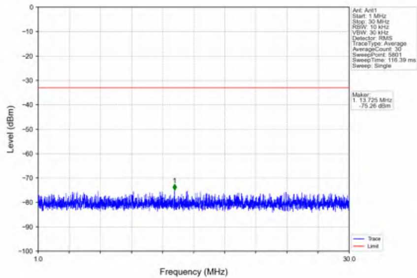
n66_30kHz_SISO_NTNV_15MHz_CP-OFDM QPSK_1772.5MHz_Inner_1RB_Right
