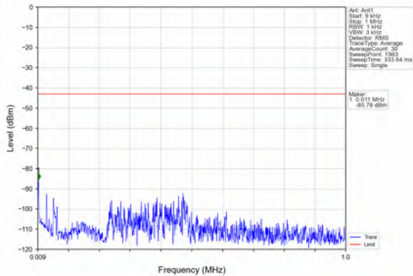
n66_30kHz_SISO_NTNV_15MHz_DFT-s-OFDM QPSK_1717.5MHz_Edge_1RB_Left
