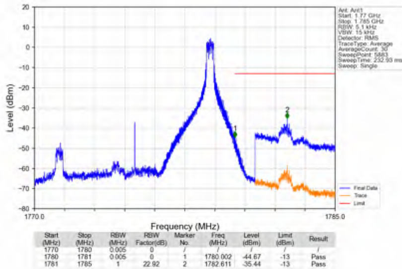
n66_30kHz_SISO_NTNV_10MHz_DFT-s-OFDM QPSK_1775MHz_Inner_1RB_Right
