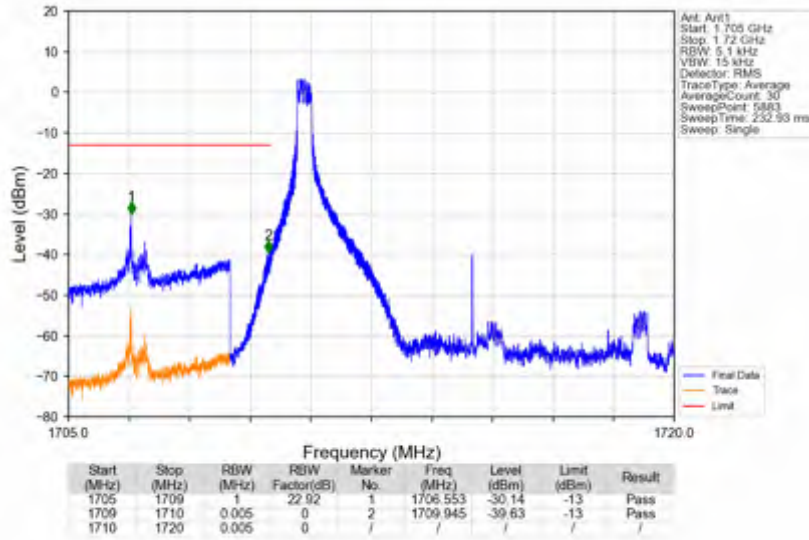
n66_30kHz_SISO_NTNV_10MHz_DFT-s-OFDM_PI/2_BPSK_1715MHz_Edge_1RB_Left
