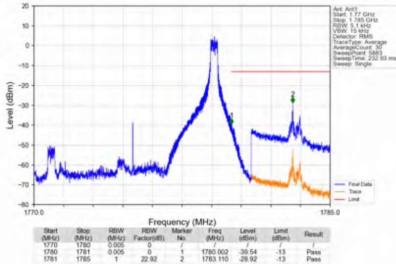
n66_30kHz_SISO_NTNV_10MHz_DFT-s-OFDM PI/2 BPSK_1775MHz_Edge_1RB_Right
