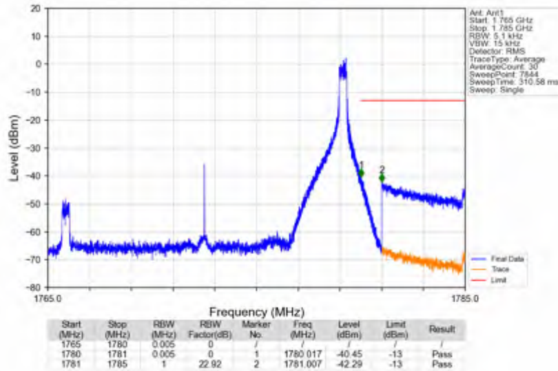
n66_30kHz_SISO_NTNV_15MHz_CP-OFDM QPSK_1772.5MHz_Edge_1RB_Right
