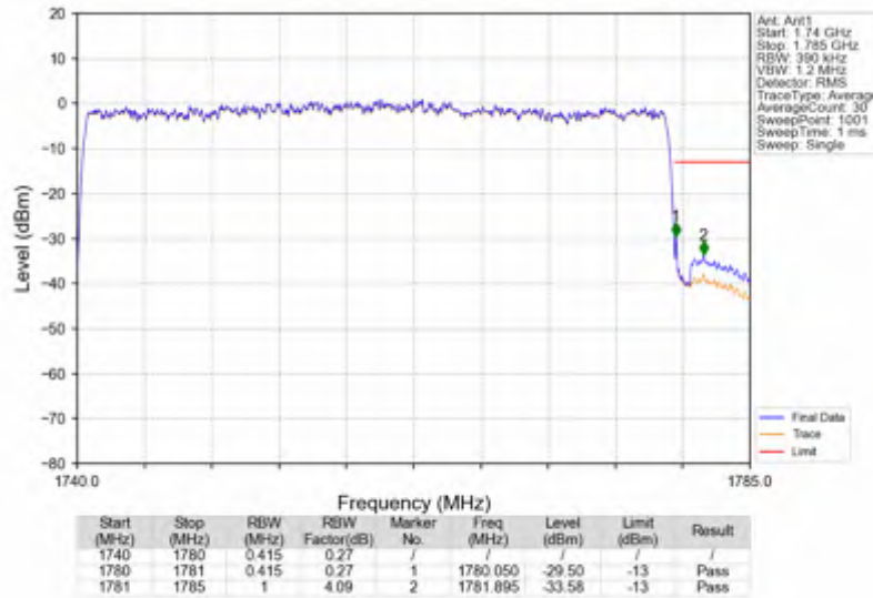
n66_15kHz_SISO_NTNV_40MHz_DFT-s-OFDM QPSK_1760MHz_Outer_Full
