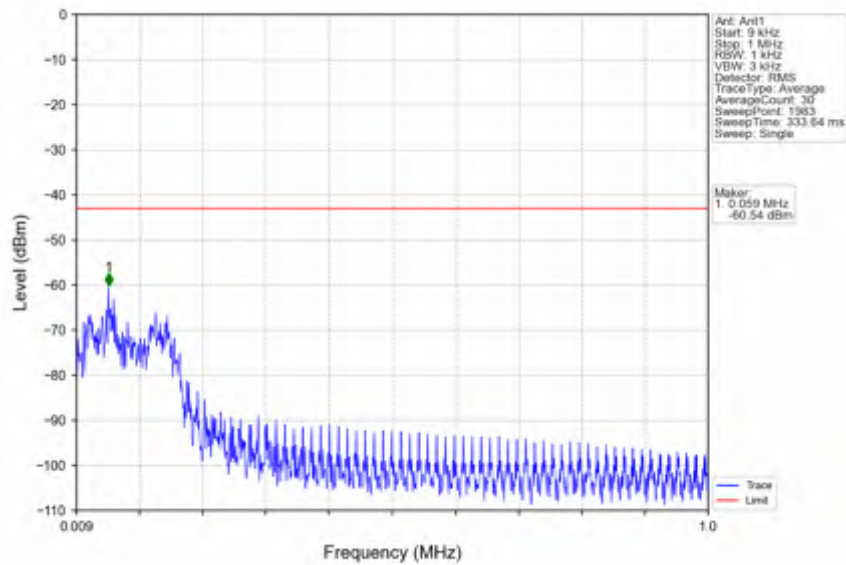
n66_15kHz_SISO_NTV_40MHz_DFT-s-OFDM PI/2 BPSK_1745MHz_Edge_1RB_Left
