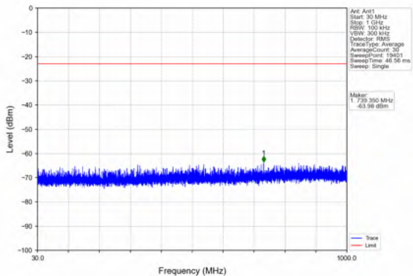
n66_30kHz_SISO_NTNV_10MHz_CP-OFDM QPSK_1775MHz_Edge_1RB_Right
