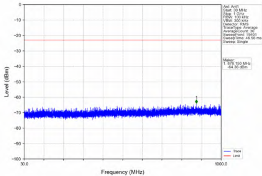
n66_15kHz_SISO_NTNV_40MHz_CP-OFDM QPSK_1730MHz_Outer_Full
