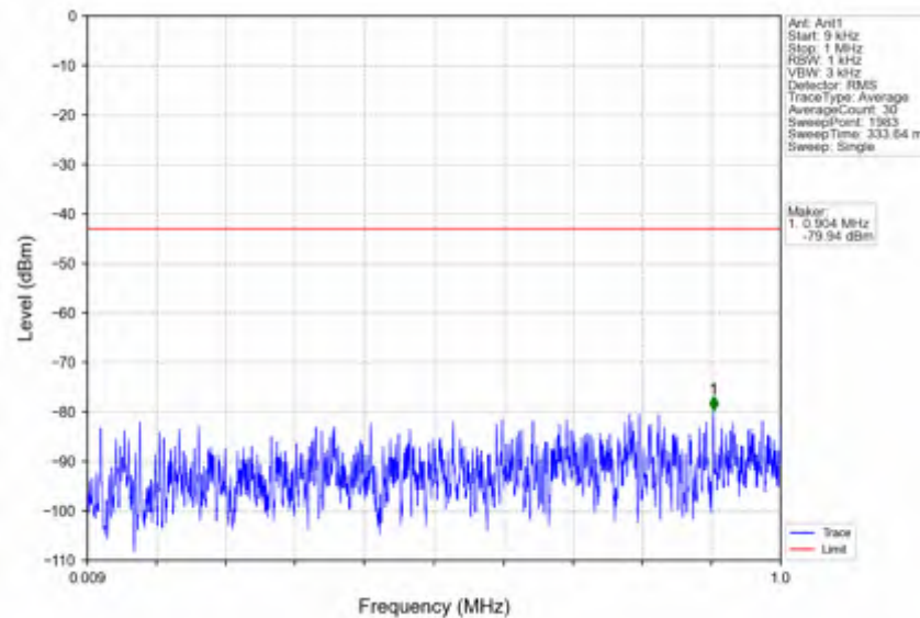
n66_30kHz_SISO_NTNV_10MHz_DFT-s-OFDM QPSK_1715MHz_Outer_Full
