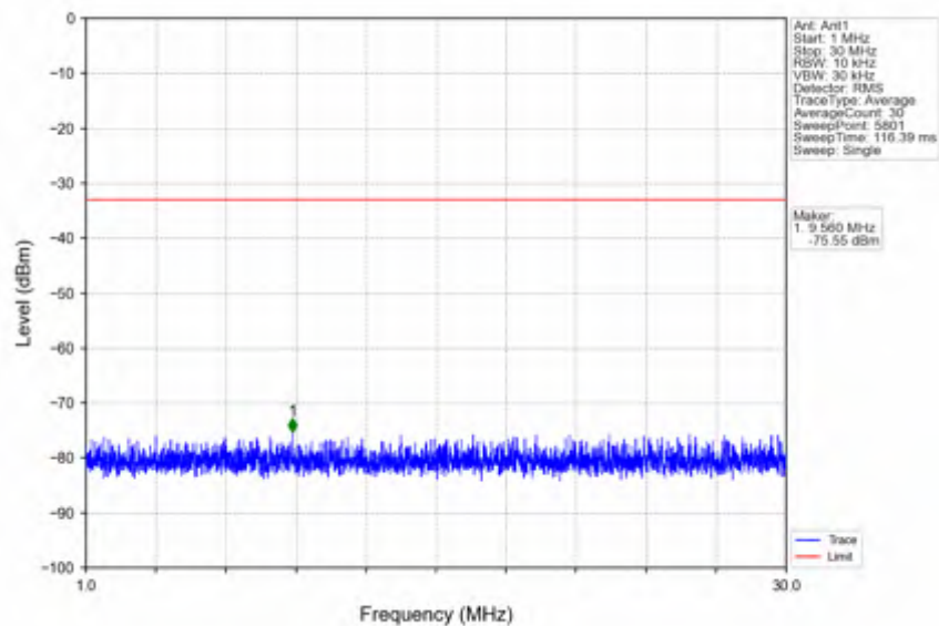
n66_15kHz_SISO_NTNV_40MHz_CP-OFDM QPSK_1745MHz_Edge_1RB_Left
