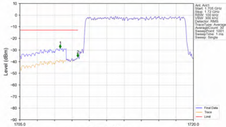
n66_30kHz_SISO_NTNV_10MHz_CP-OFDM QPSK_1715MHz_Outer_Full
