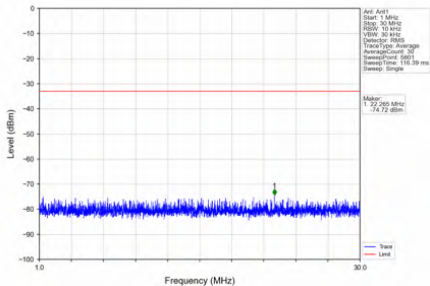
n66_30kHz_SISO_NTNV_15MHz_CP-OFDM QPSK_1745MHz_Edge_1RB_Left
