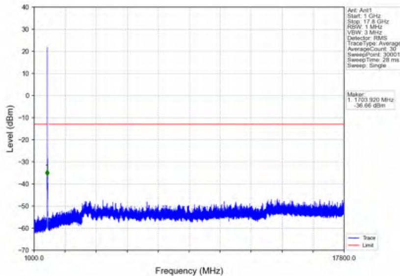
n66_30kHz_SISO_NTNV_15MHz_DFT-s-OFDM QPSK_1717.5MHz_Edge_1RB_Left
