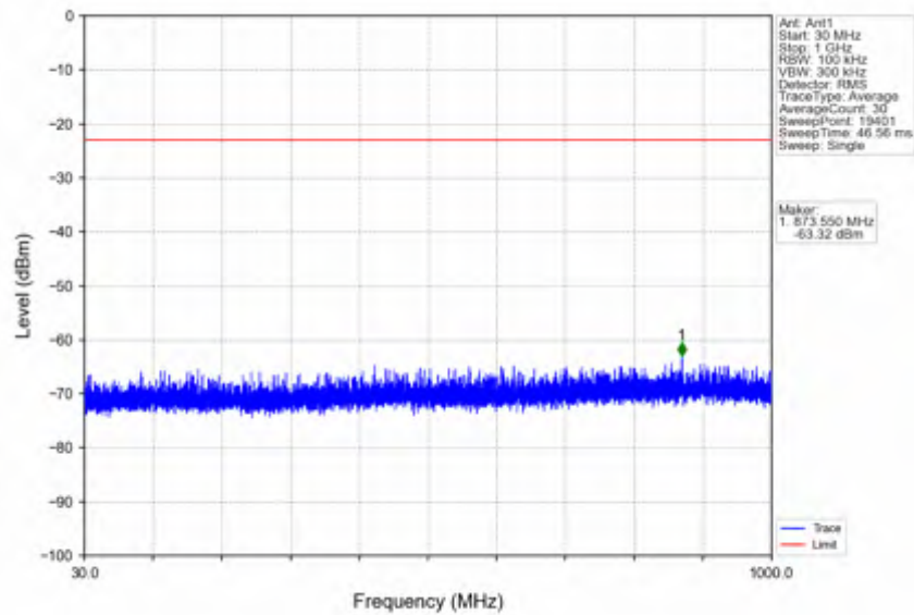
n66_30kHz_SISO_NTNV_15MHz_DFT-s-OFDM QPSK_1772.5MHz_Inner_1RB_Right
