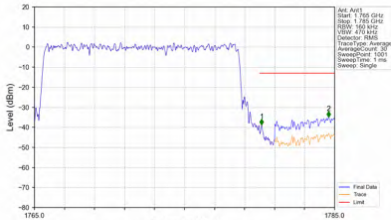
n66_30kHz_SISO_NTNV_15MHz_DFT-s-OFDM PI/2 BPSK_1772.5MHz_Outer_Full
