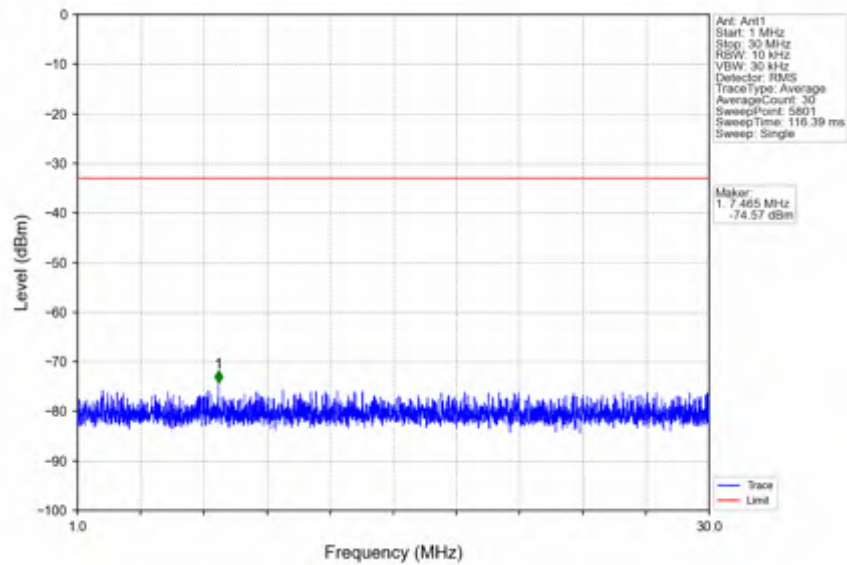
n66_30kHz_SISO_NTNV_15MHz_DFT-s-OFDM_QPSK_1772.5MHz_Outer_Full
