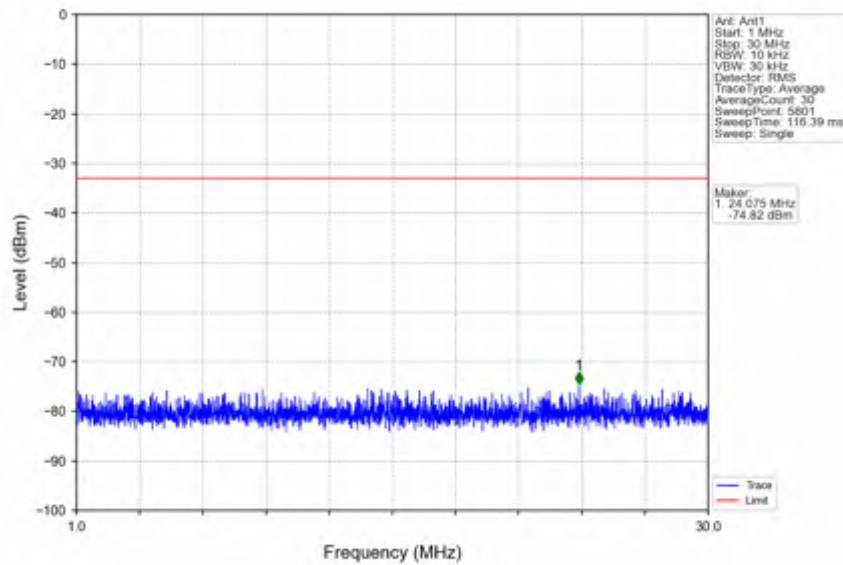
n66_30kHz_SISO_NTNV_15MHz_DFT-s-OFDM QPSK_1772.5MHz_Edge_1RB_Right
