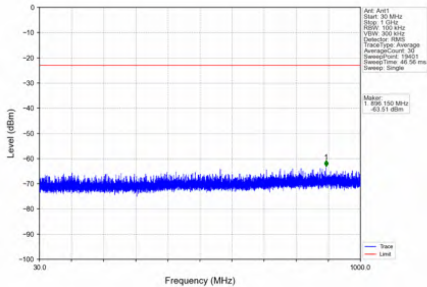
n66_30kHz_SISO_NTNV_10MHz_DFT-s-OFDM PI/2 BPSK_1775MHz_Outer_Full
