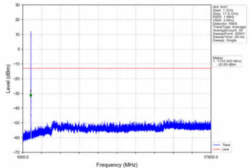
n66_30kHz_SISO_NTNV_15MHz_CP-OFDM QPSK_1717.5MHz_Outer_Full
