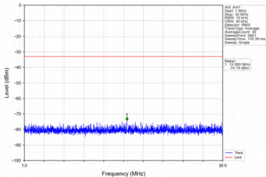
n66_30kHz_SISO_NTNV_10MHz_DFT-s-OFDM PI/2 BPSK_1715MHz_Outer_Full
