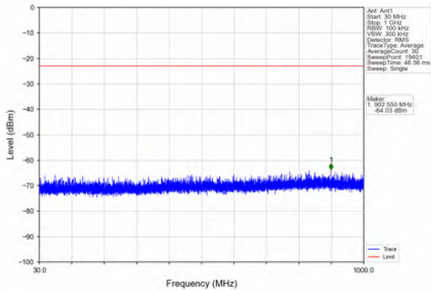
n66_15kHz_SISO_NTNV_40MHz_DFT-s-OFDM QPSK_1760MHz_Edge_1RB_Right
