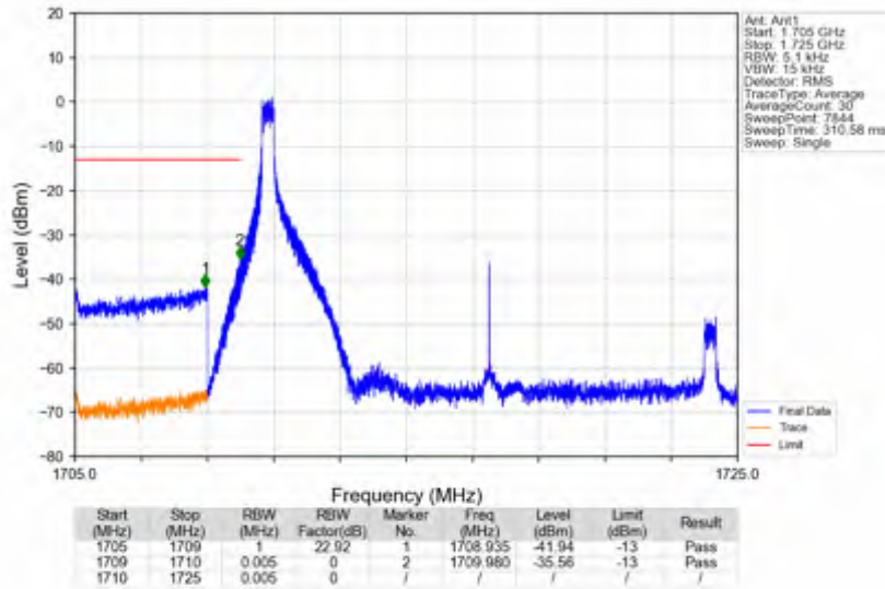
n66_30kHz_SISO_NTV_15MHz_CP-OFDM QPSK_1717.5MHz_Edge_1RB_Left
