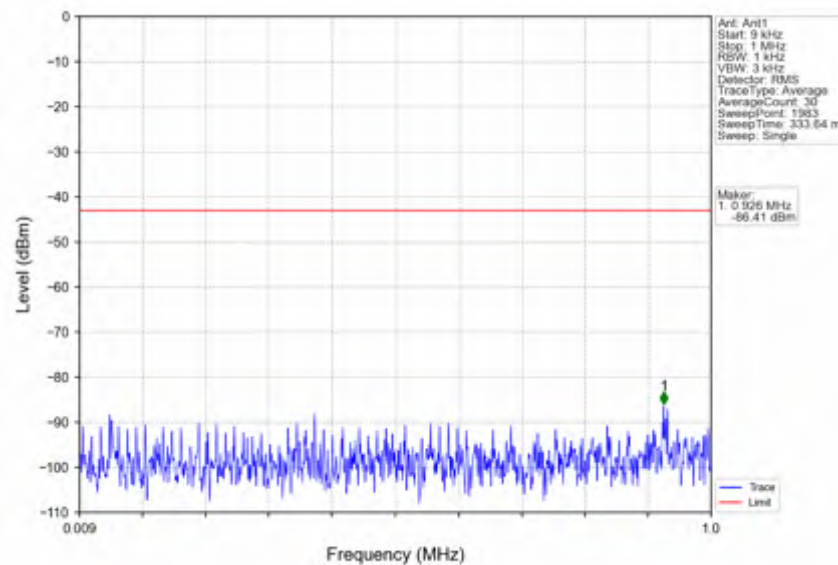
n66_15kHz_SISO_NTNV_40MHz_DFT-s-OFDM QPSK_1730MHz_Outer_Full
