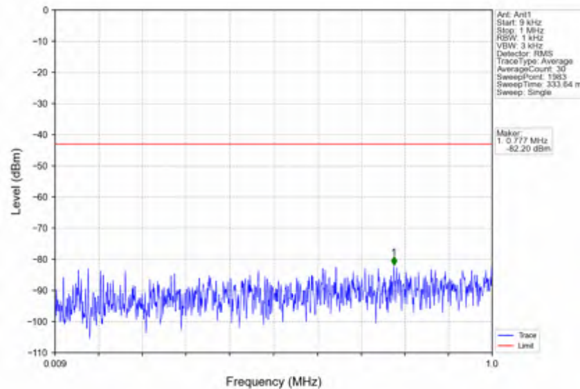
n66_30kHz_SISO_NTNV_10MHz_DFT-s-OFDM QPSK_1775MHz_Outer_Full
