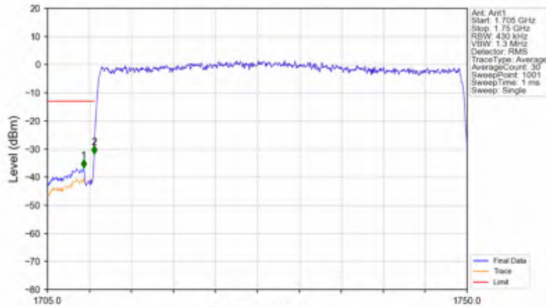
n66_15kHz_SISO_NTNV_40MHz_DFT-s-OFDM PI/2 BPSK_1730MHz_Outer_Full
