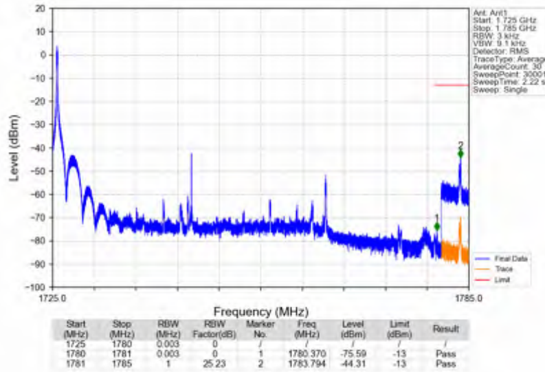
n66_15kHz_SISO_NTNV_40MHz_DFT-s-OFDM QPSK_1745MHz_Edge_1RB_Left
