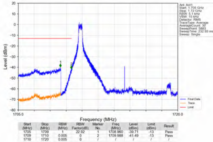
n66_30kHz_SISO_NTNV_10MHz_CP-OFDM QPSK_1715MHz_Edge_1RB_Left
