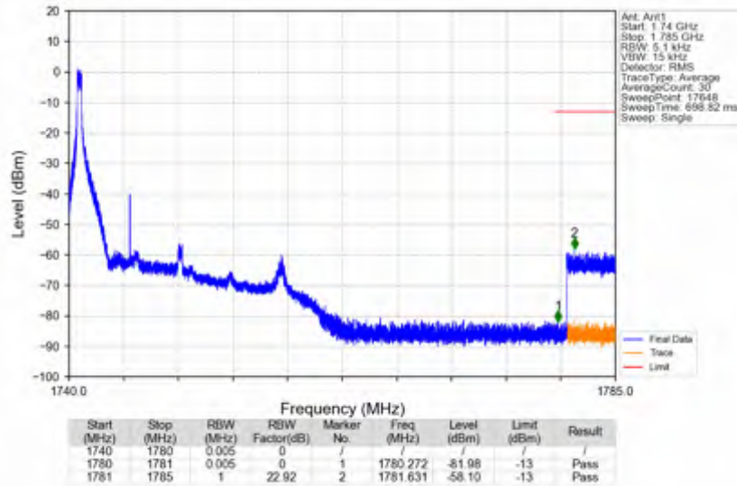
n66_30kHz_SISO_NTNV_10MHz_CP-OFDM QPSK_1745MHz_Edge_1RB_Left
