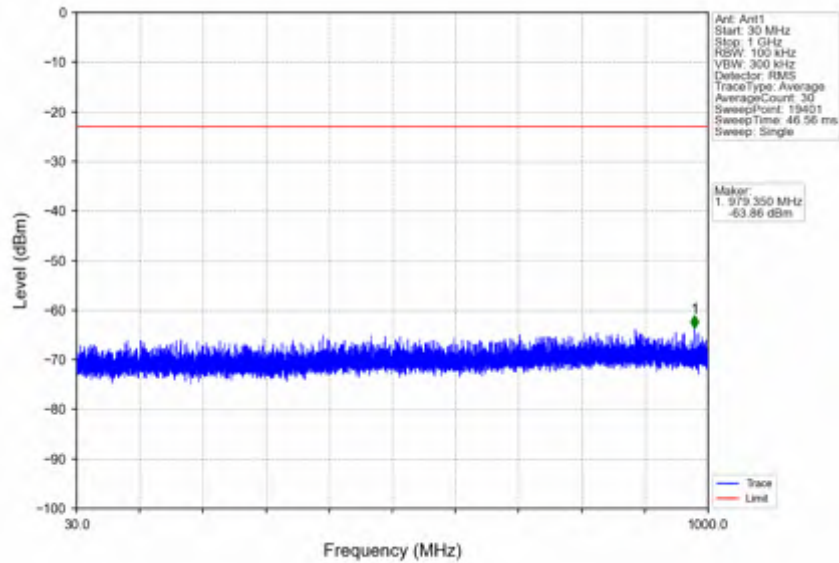
n66_30kHz_SISO_NTNV_15MHz_DFT-s-OFDM QPSK_1717.5MHz_Edge_1RB_Left
