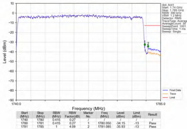
n66_15kHz_SISO_NTNV_40MHz_CP-OFDM QPSK_1760MHz_Outer_Full
