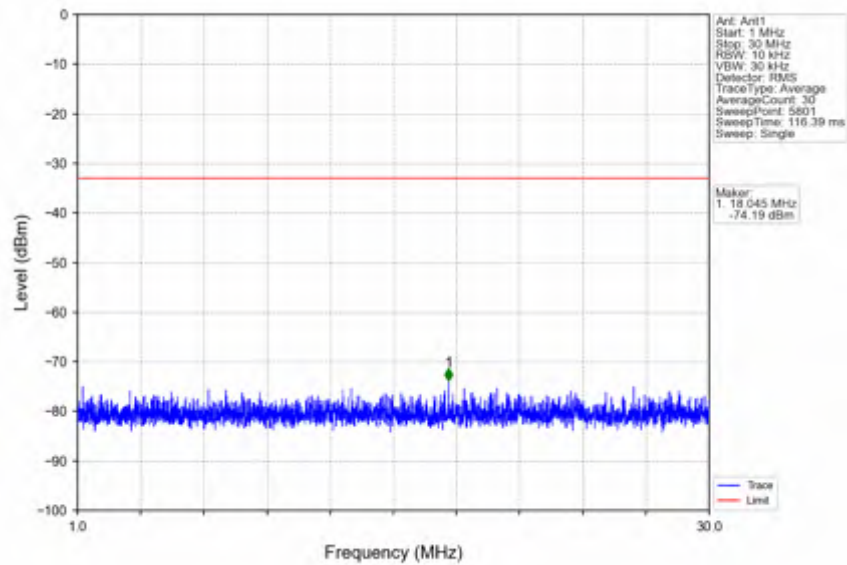
n66_15kHz_SISO_NTNV_40MHz_CP-OFDM QPSK_1730MHz_Edge_1RB_Left
