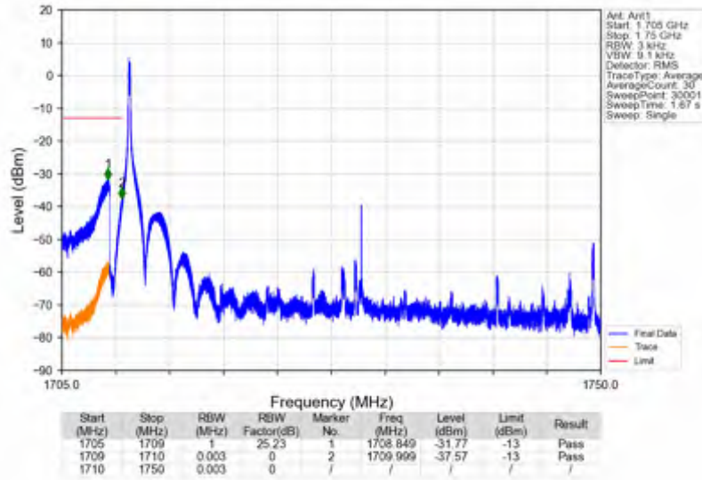
n66_15kHz_SISO_NTNV_40MHz_DFT-s-OFDM_PI/2_BPSK_1730MHz_Edge_1RB_Left
