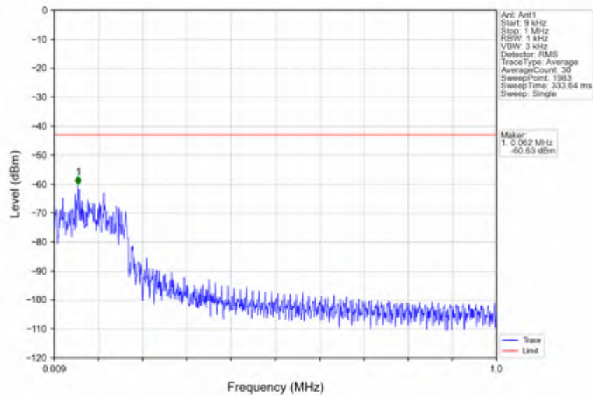
n66_15kHz_SISO_NTNV_40MHz_DFT-s-OFDM QPSK_1730MHz_Edge_1RB_Left
