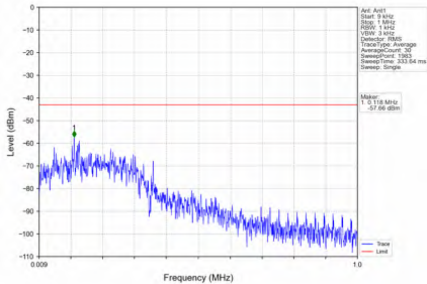
n66_30kHz_SISO_NTNV_10MHz_DFT-s-OFDM QPSK_1775MHz_Inner_1RB_Right
