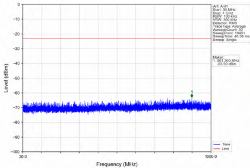
n66_15kHz_SISO_NTNV_30MHz_CP-OFDM QPSK_1745MHz_Edge_1RB_Left
