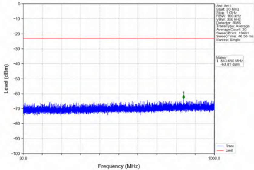
n66_30kHz_SISO_NTNV_10MHz_DFT-s-OFDM QPSK_1775MHz_Edge_1RB_Right
