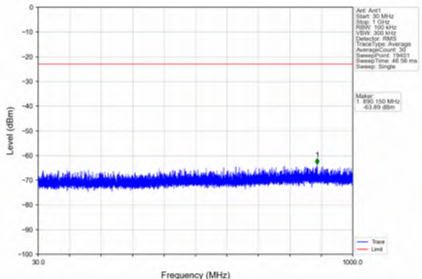
n66_15kHz_SISO_NTNV_40MHz_CP-OFDM QPSK_1760MHz_Edge_1RB_Right
