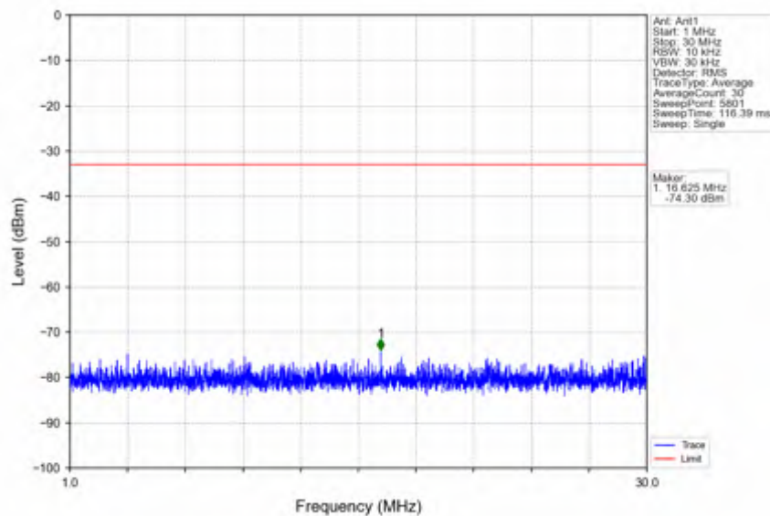
n66_30kHz_SISO_NTNV_15MHz_DFT-s-OFDM PI/2 BPSK_1772.5MHz_Outer_Full
