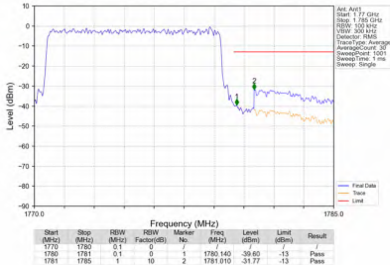
n66_30kHz_SISO_NTNV_10MHz_CP-OFDM QPSK_1775MHz_Outer_Full
