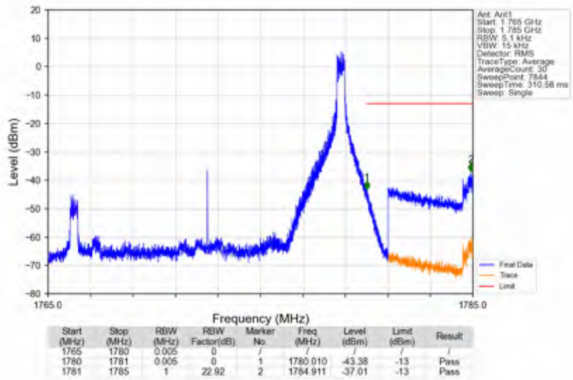
n66_30kHz_SISO_NTNV_15MHz_DFT-s-OFDM QPSK_1772.5MHz_Inner_1RB_Right
