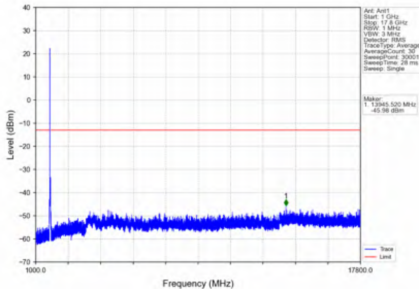
n66_15kHz_SISO_NTV_40MHz_DFT-s-OFDM PI/2 BPSK_1745MHz_Edge_1RB_Left
