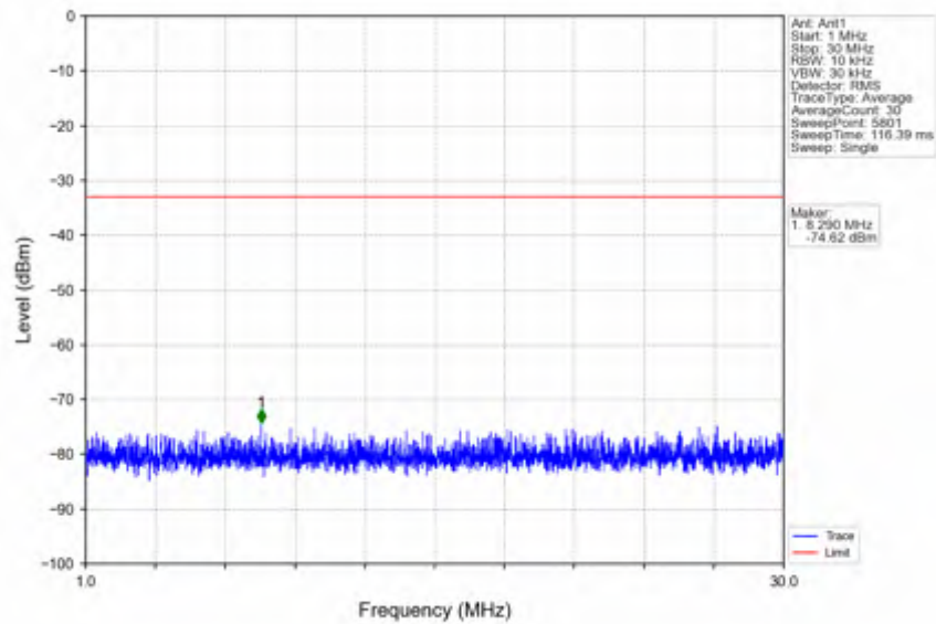
n66_30kHz_SISO_NTNV_15MHz_CP-OFDM QPSK_1772.5MHz_Edge_1RB_Right
