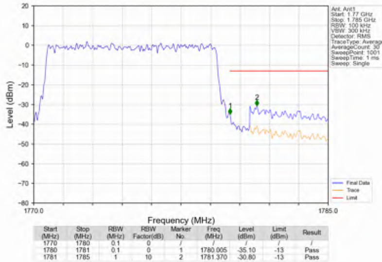
n66_30kHz_SISO_NTNV_10MHz_DFT-s-OFDM QPSK_1775MHz_Outer_Full
