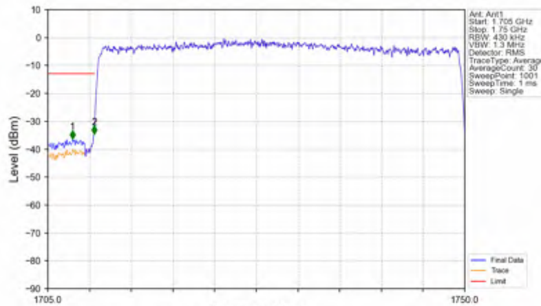
n66_15kHz_SISO_NTNV_40MHz_CP-OFDM QPSK_1730MHz_Outer_Full
