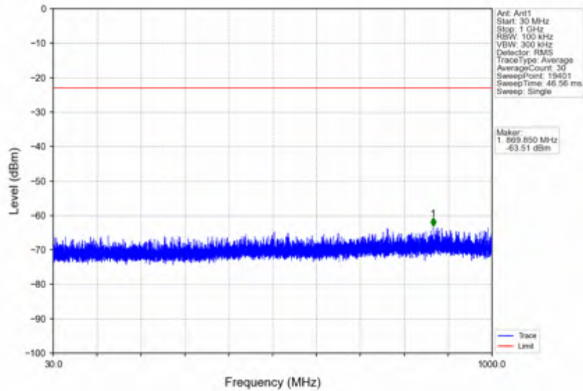
n66_30kHz_SISO_NTNV_15MHz_DFT-s-OFDM PI/2 BPSK_1717.5MHz_Outer_Full
