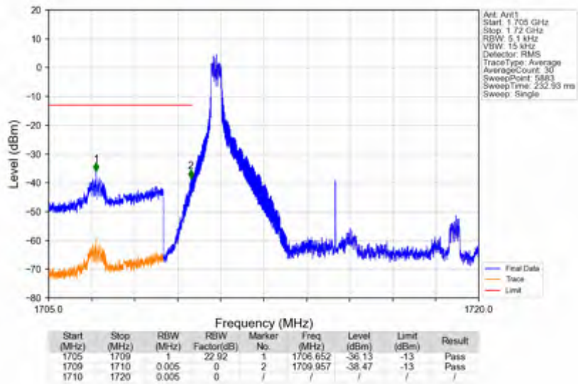
n66_30kHz_SISO_NTNV_10MHz_DFT-s-OFDM QPSK_1715MHz_Edge_1RB_Left
