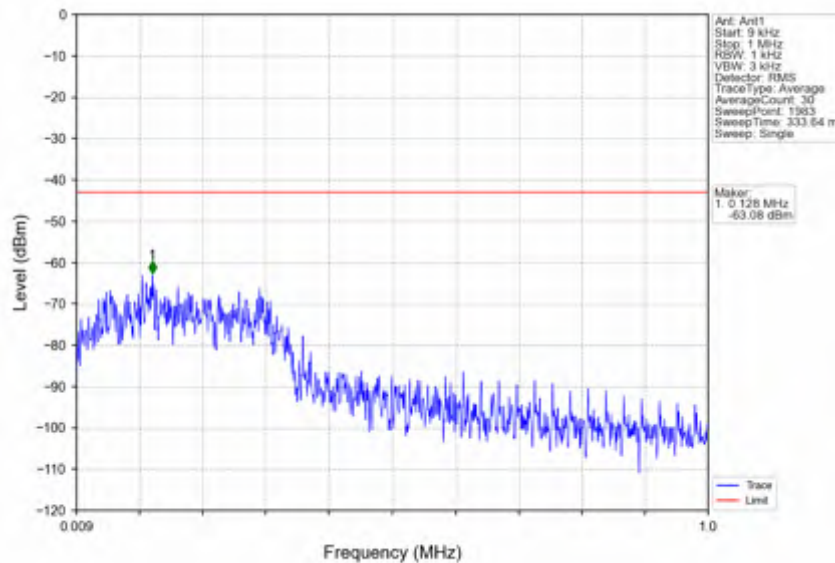
n66_30kHz_SISO_NTNV_10MHz_DFT-s-OFDM QPSK_1745MHz_Edge_1RB_Left
