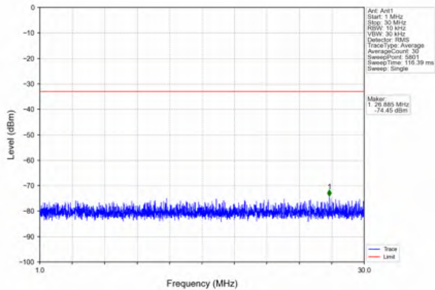
n66_30kHz_SISO_NTNV_10MHz_DFT-s-OFDM QPSK_1745MHz_Edge_1RB_Left
