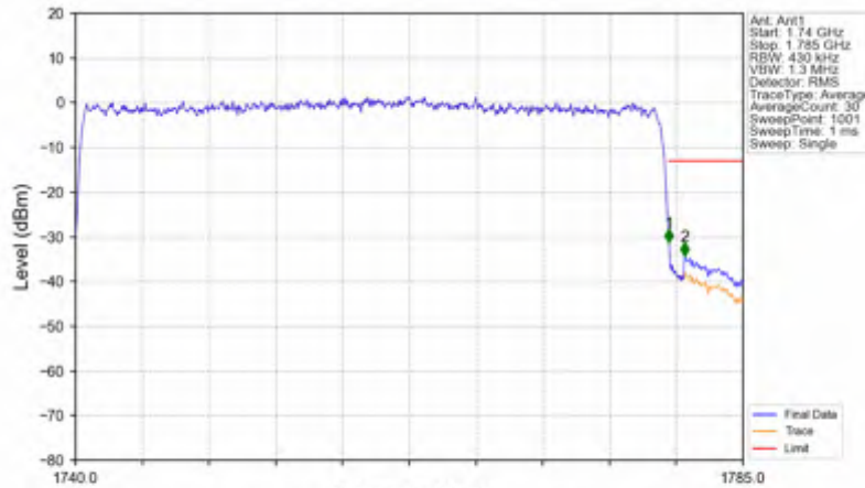
n66_15kHz_SISO_NTNV_40MHz_DFT-s-OFDM PI/2 BPSK_1760MHz_Outer_Full
