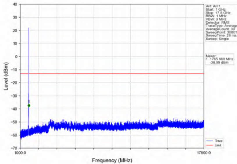
n66_30kHz_SISO_NTNV_15MHz_DFT-s-OFDM PI/2 BPSK_1772.5MHz_Outer_Full
