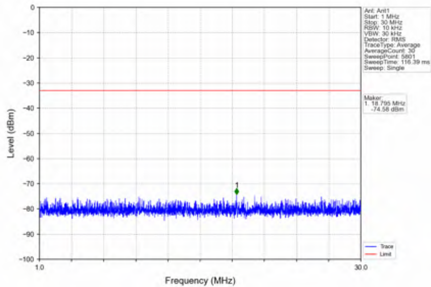
n66_30kHz_SISO_NTNV_15MHz_DFT-s-OFDM PI/2 BPSK_1772.5MHz_Edge_1RB_Right
