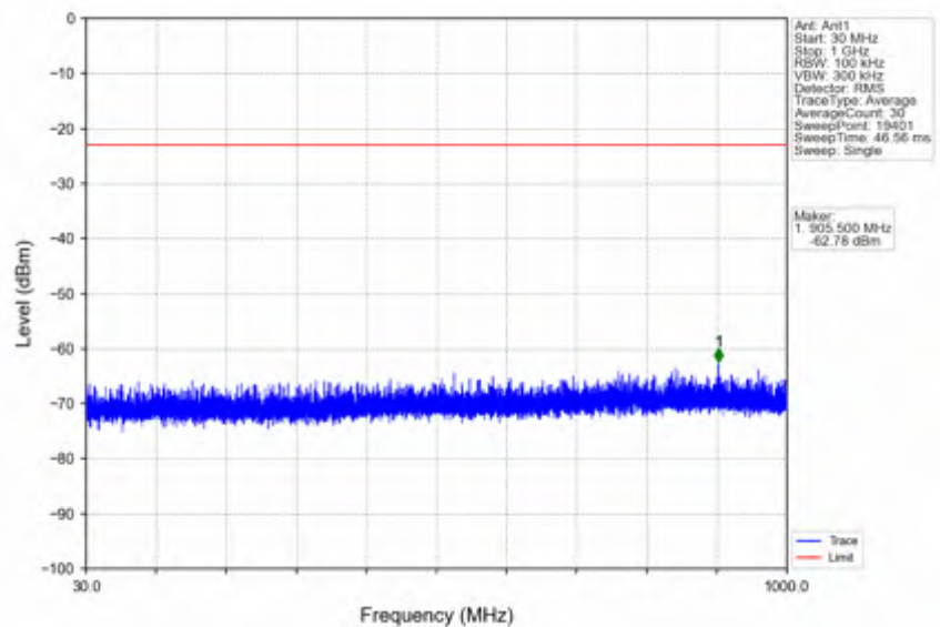
n66_30kHz_SISO_NTV_15MHz_CP-OFDM QPSK_1717.5MHz_Edge_1RB_Left
