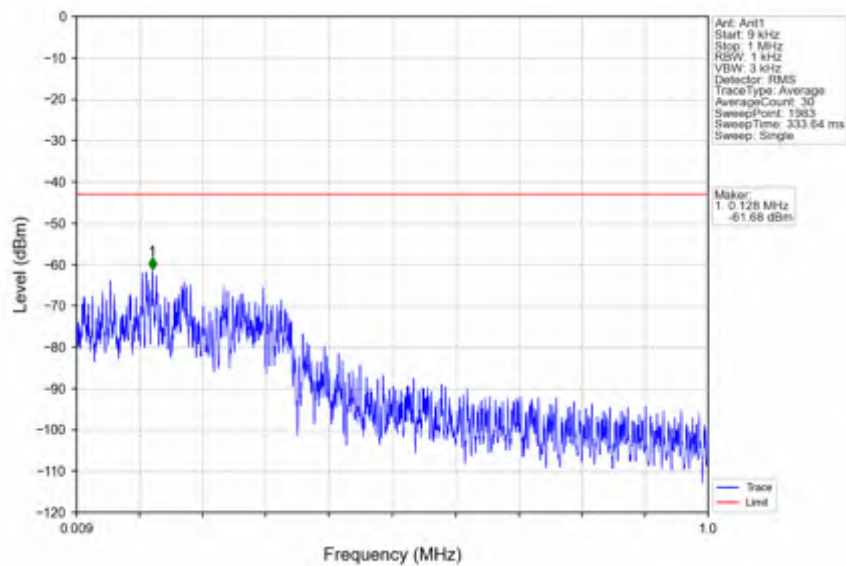
n66_30kHz_SISO_NTNV_10MHz_DFT-s-OFDM_PI/2_BPSK_1715MHz_Edge_1RB_Left
