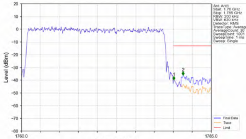
n66_30kHz_SISO_NTNV_20MHz_DFT-s-OFDM PI/2 BPSK_1770MHz_Outer_Full
