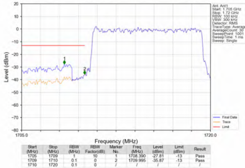
n66_30kHz_SISO_NTNV_10MHz_DFT-s-OFDM QPSK_1715MHz_Outer_Full
