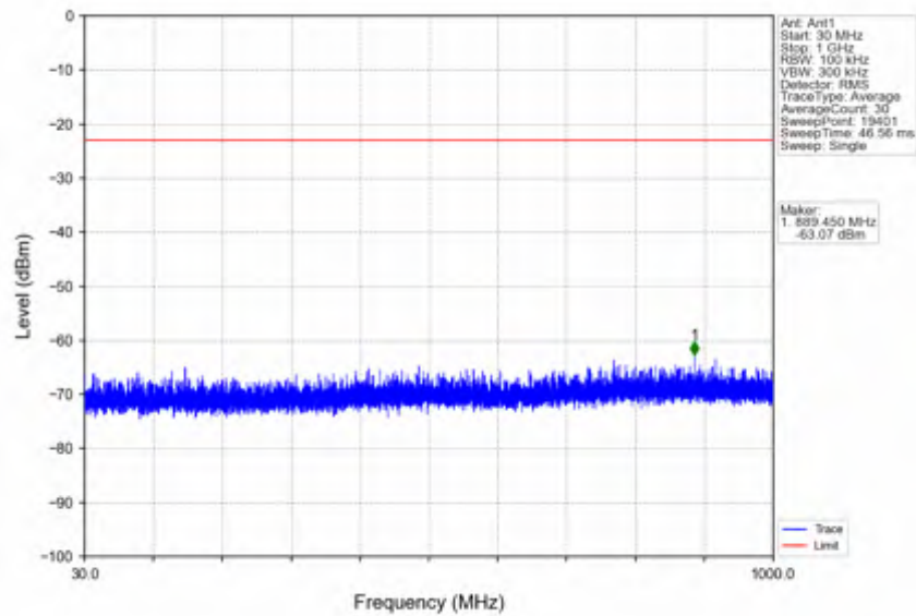
n66_30kHz_SISO_NTNV_10MHz_DFT-s-OFDM QPSK_1715MHz_Edge_1RB_Left
