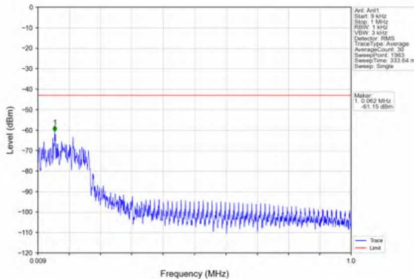
n66_15kHz_SISO_NTNV_40MHz_DFT-s-OFDM QPSK_1745MHz_Edge_1RB_Left
