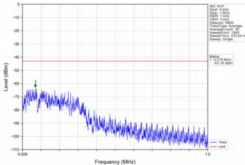
n66_30kHz_SISO_NTNV_10MHz_CP-OFDM QPSK_1715MHz_Edge_1RB_Left
