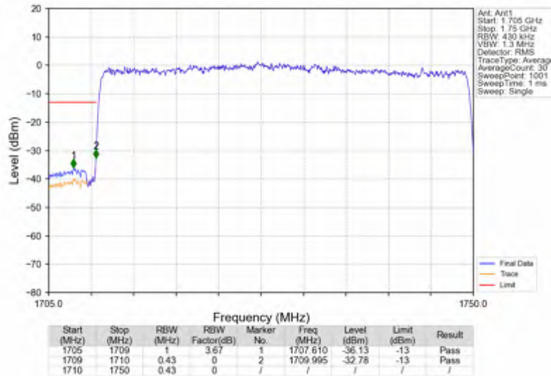
n66_15kHz_SISO_NTNV_40MHz_DFT-s-OFDM QPSK_1730MHz_Outer_Full
