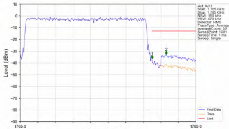
n66_30kHz_SISO_NTNV_15MHz_CP-OFDM QPSK_1772.5MHz_Outer_Full
