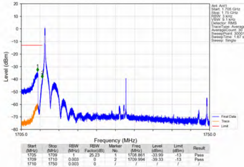
n66_15kHz_SISO_NTNV_40MHz_CP-OFDM QPSK_1730MHz_Edge_1RB_Left
