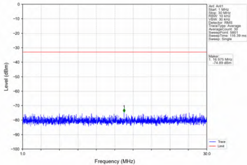
n66_15kHz_SISO_NTNV_40MHz_DFT-s-OFDM QPSK_1745MHz_Edge_1RB_Left
