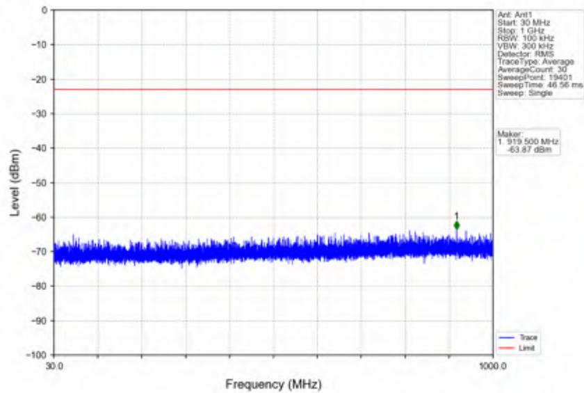
n66_30kHz_SISO_NTNV_10MHz_CP-OFDM QPSK_1745MHz_Edge_1RB_Left
