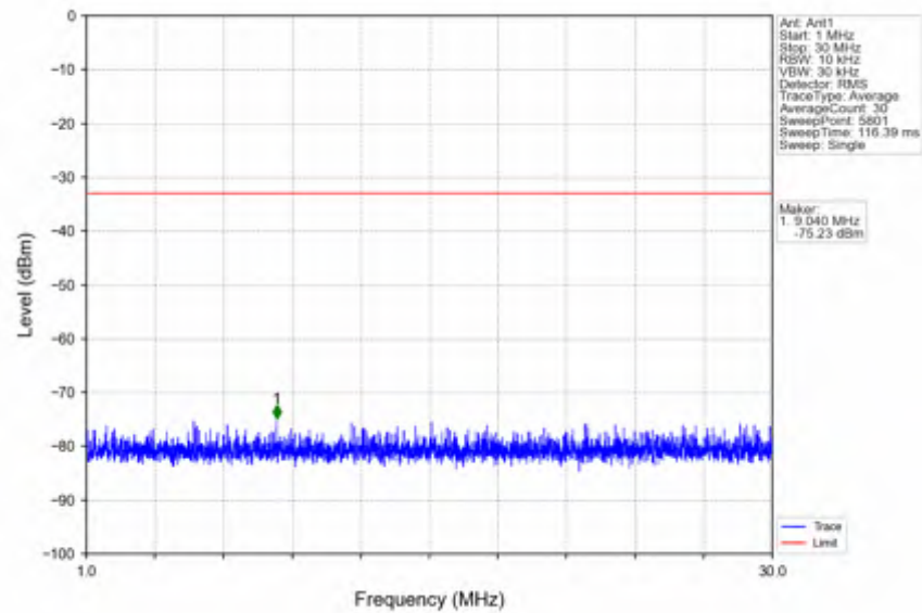
n66_15kHz_SISO_NTNV_40MHz_DFT-s-OFDM QPSK_1760MHz_Outer_Full
