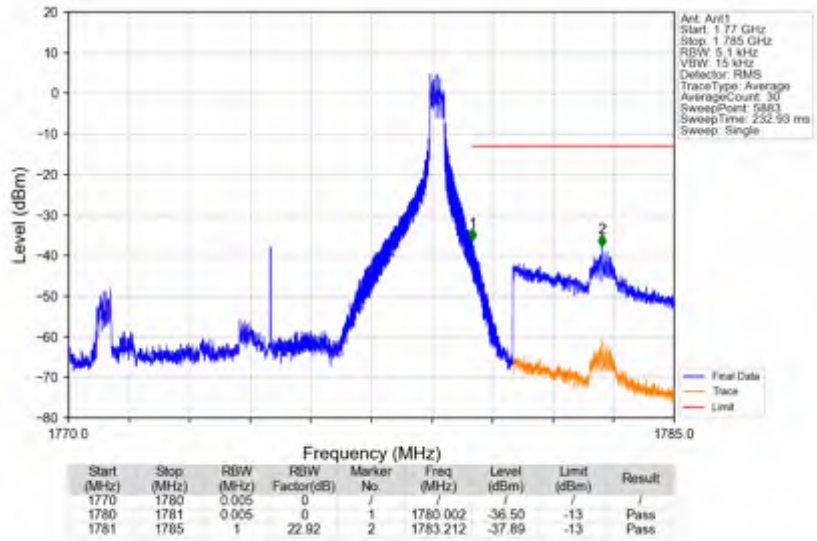
n66_30kHz_SISO_NTNV_10MHz_DFT-s-OFDM QPSK_1775MHz_Edge_1RB_Right
