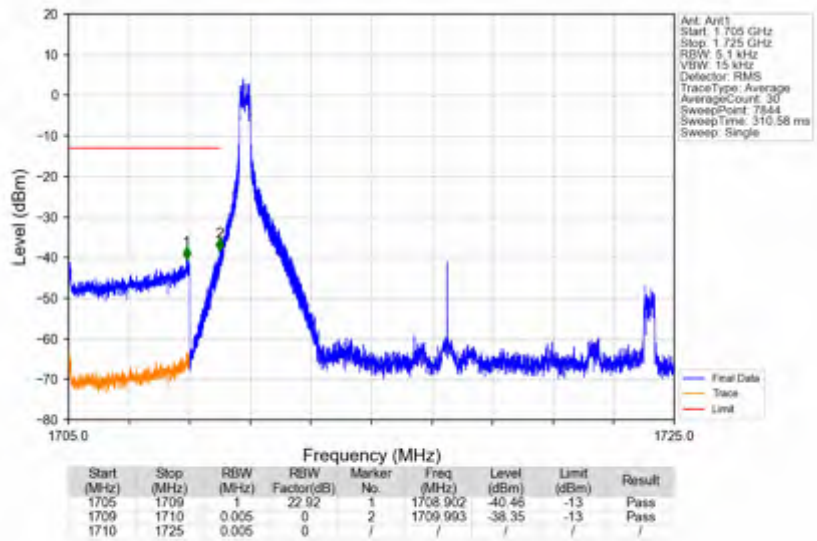
n66_30kHz_SISO_NTNV_15MHz_DFT-s-OFDM QPSK_1717.5MHz_Edge_1RB_Left
