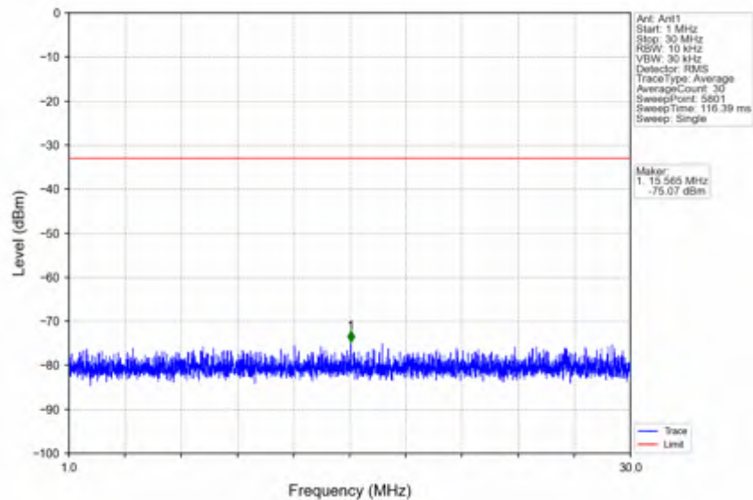
n66_30kHz_SISO_NTNV_20MHz_DFT-s-OFDM PI/2 BPSK_1720MHz_Outer_Full
