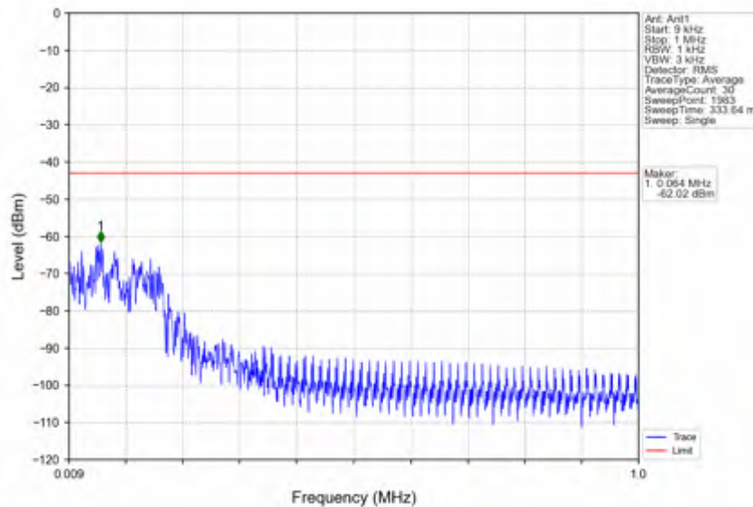
n66_15kHz_SISO_NTNV_40MHz_DFT-s-OFDM PI/2 BPSK_1760MHz_Edge_1RB_Right
