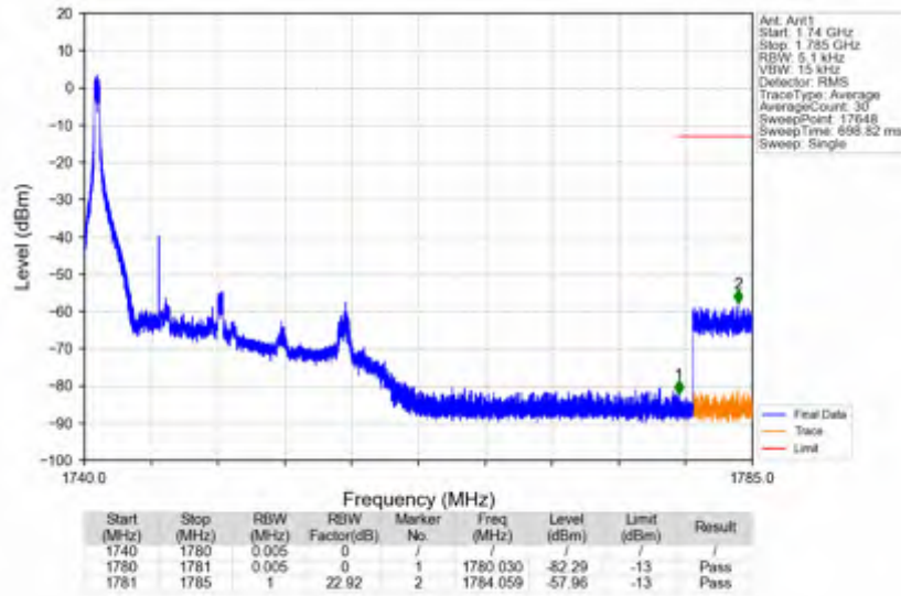
n66_30kHz_SISO_NTNV_10MHz_DFT-s-OFDM QPSK_1745MHz_Edge_1RB_Left
