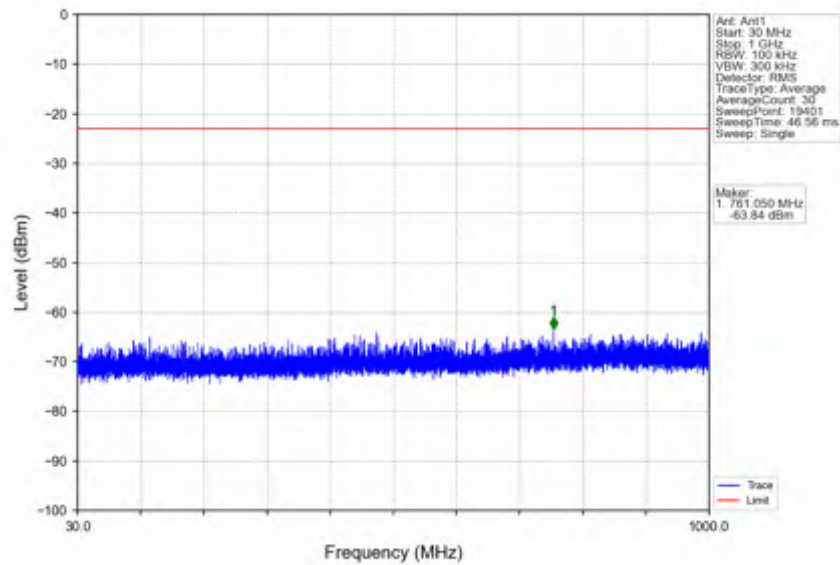
n66_30kHz_SISO_NTV_10MHz_DFT-s-OFDM PI/2 BPSK_1745MHz_Edge_1RB_Left
