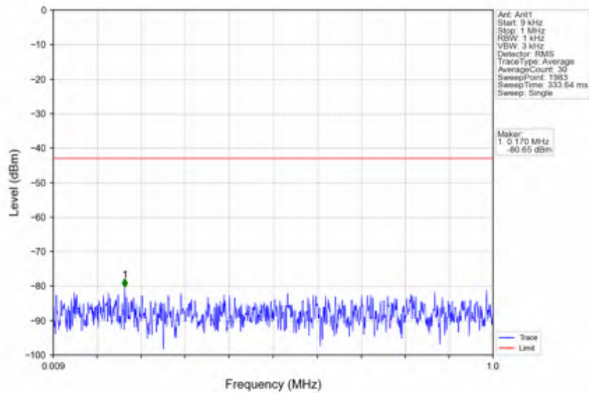
n66_15kHz_SISO_NTNV_25MHz_CP-OFDM QPSK_1722.5MHz_Outer_Full
