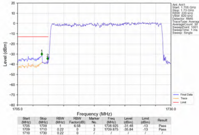
n66_15kHz_SISO_NTNV_20MHz_DFT-s-OFDM QPSK_1720MHz_Outer_Full
