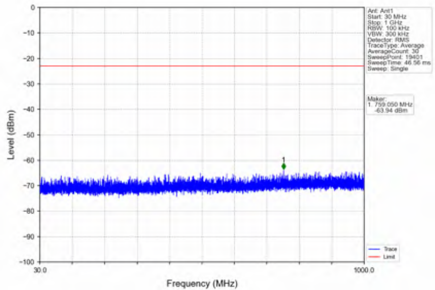
n66_15kHz_SISO_NTNV_30MHz_DFT-s-OFDM_QPSK_1745MHz_Edge_1RB_Left
