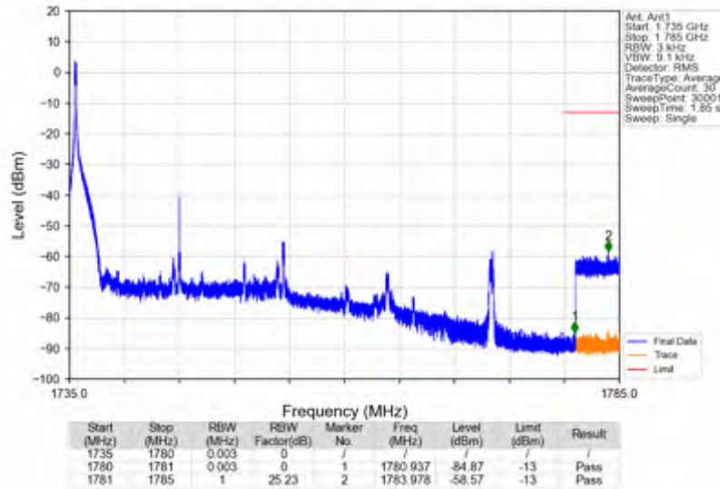
n66_15kHz_SISO_NTNV_20MHz_DFT-s-OFDM QPSK_1745MHz_Edge_1RB_Left
