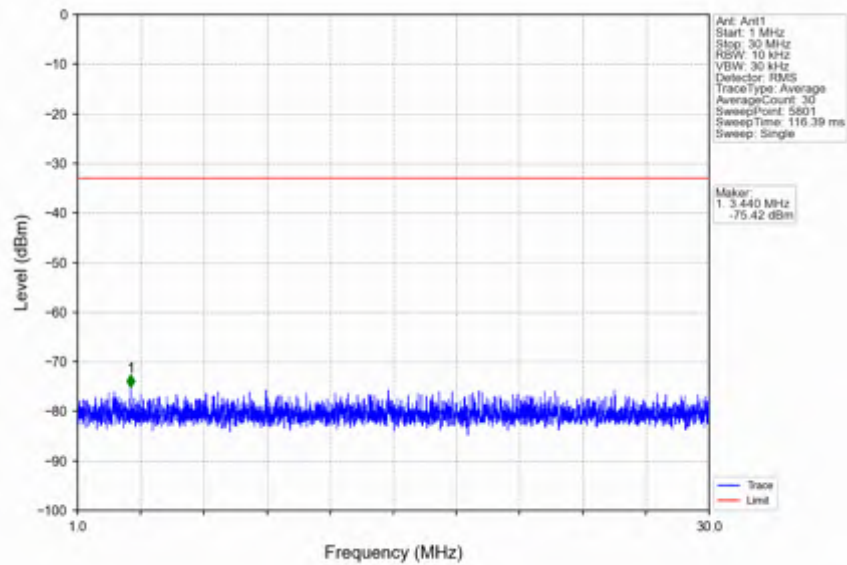
n66_15kHz_SISO_NTNV_25MHz_DFT-s-OFDM QPSK_1745MHz_Edge_1RB_Left
