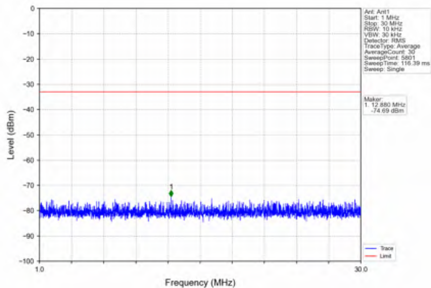
n66_15kHz_SISO_NTNV_25MHz_CP-OFDM QPSK_1745MHz_Edge_1RB_Left
