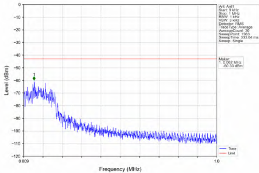
n66_15kHz_SISO_NTVV_30MHz_DFT-s-OFDM QPSK_1765MHz_Edge_1RB_Right
