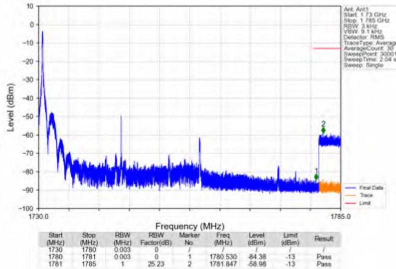
n66_15kHz_SISO_NTNV_30MHz_DFT-s-OFDM QPSK_1745MHz_Edge_1RB_Left
