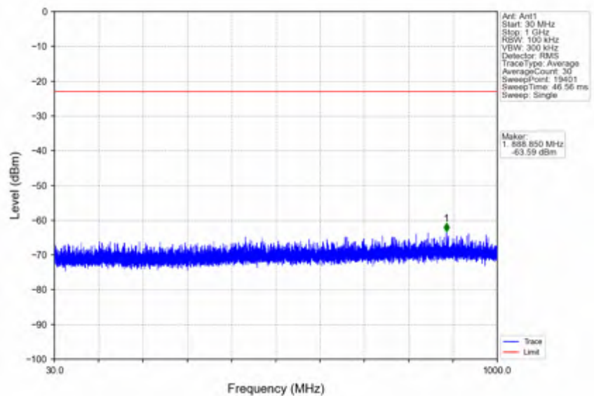
n66_15kHz_SISO_NTNV_30MHz_CP-OFDM QPSK_1725MHz_Edge_1RB_Left
