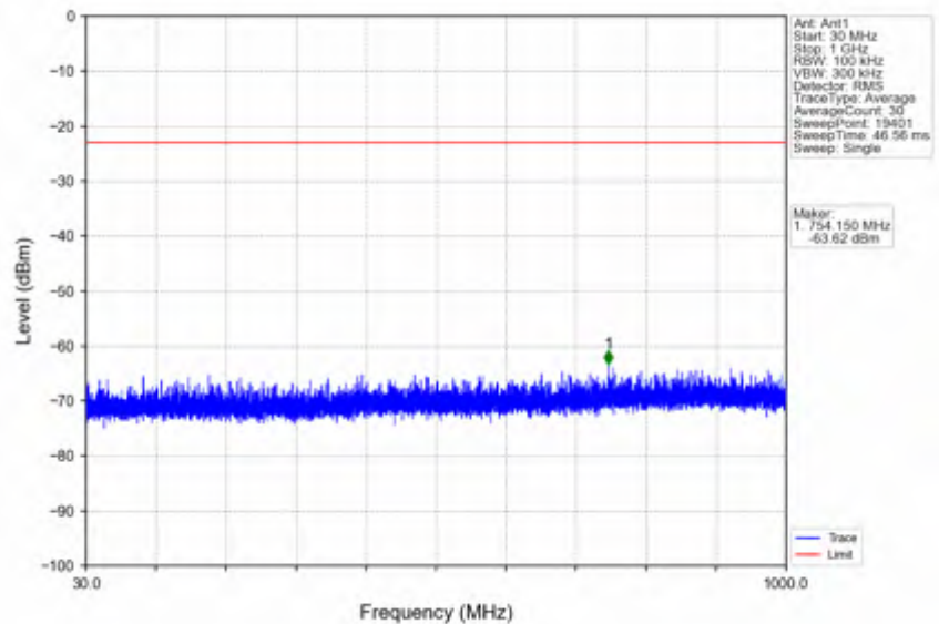
n66_15kHz_SISO_NTNV_25MHz_CP-OFDM QPSK_1767.5MHz_Edge_1RB_Right
