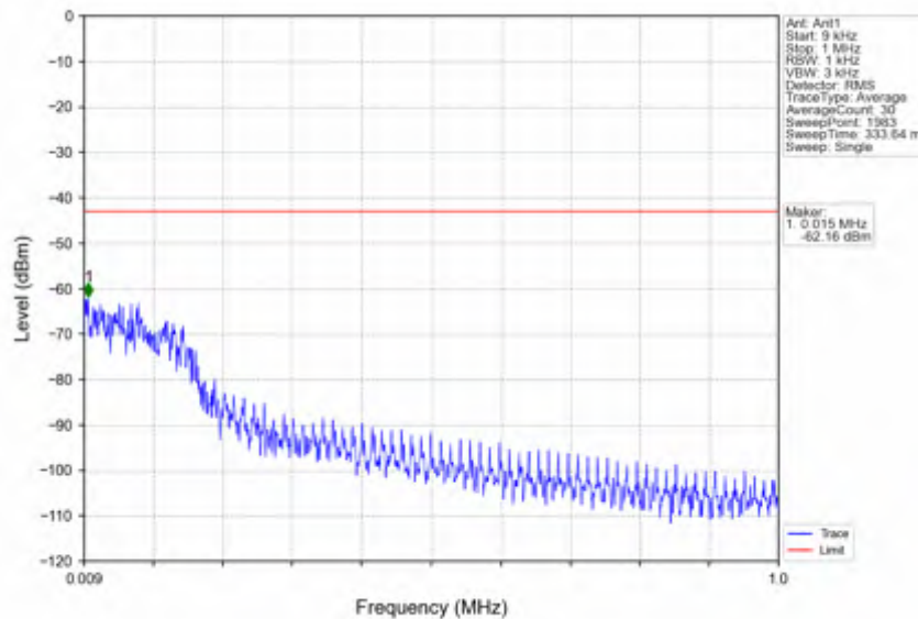
n66_15kHz_SISO_NTV_15MHz_CP-OFDM QPSK_1717.5MHz_Edge_1RB_Left
