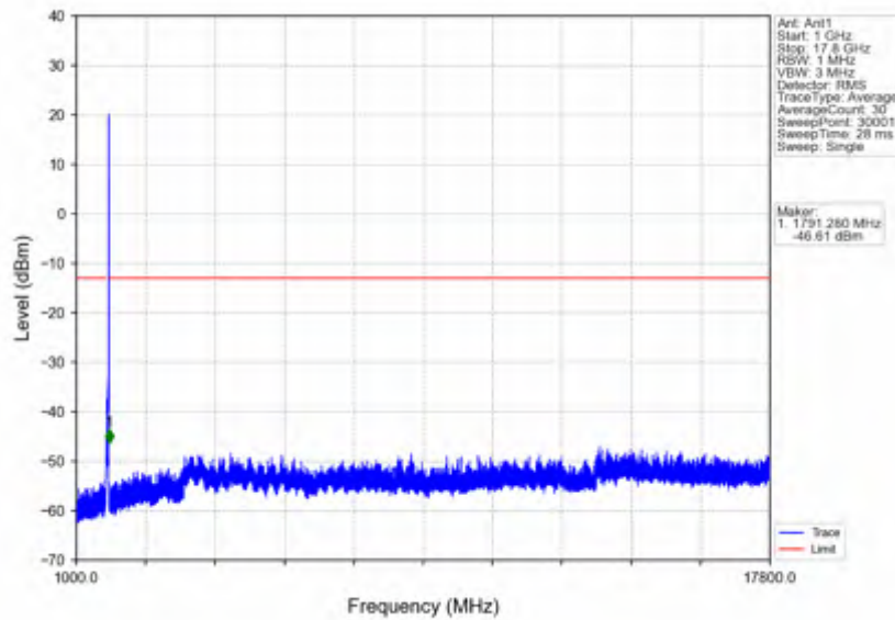
n66_15kHz_SISO_NTNV_25MHz_CP-OFDM QPSK_1767.5MHz_Outer_Full
