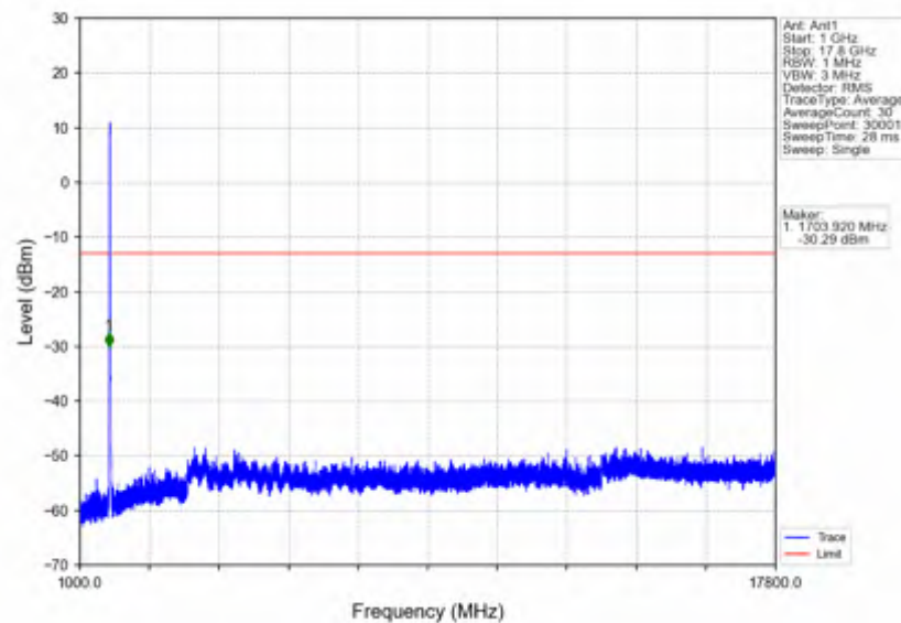
n66_15kHz_SISO_NTNV_15MHz_CP-OFDM QPSK_1717.5MHz_Outer_Full
