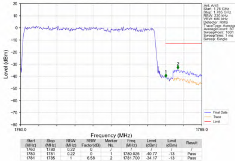
n66_15kHz_SISO_NTNV_20MHz_DFT-s-OFDM QPSK_1770MHz_Outer_Full
