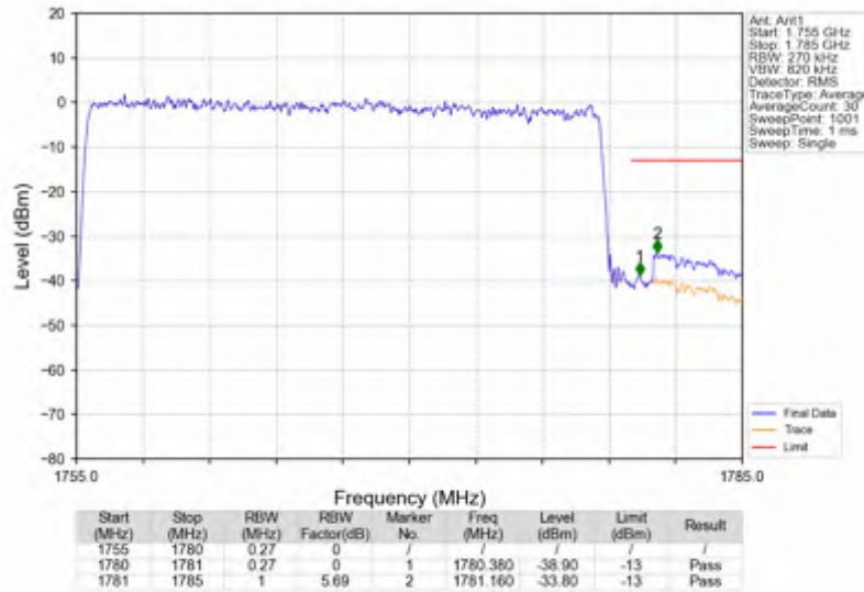
n66_15kHz_SISO_NTNV_25MHz_DFT-s-OFDM_QPSK_1767.5MHz_Outer_Full
