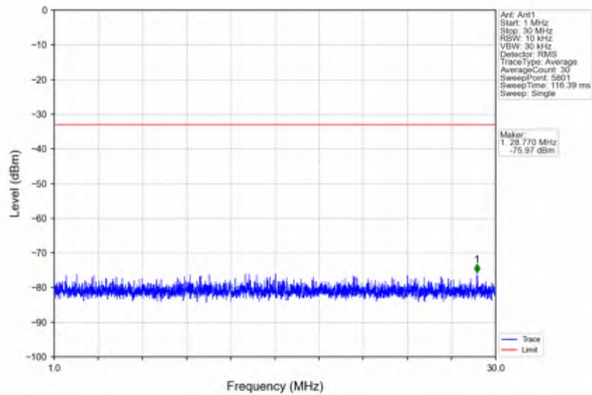
n66_15kHz_SISO_NTNV_15MHz_DFT-s-OFDM_QPSK_1772.5MHz_Outer_Full
