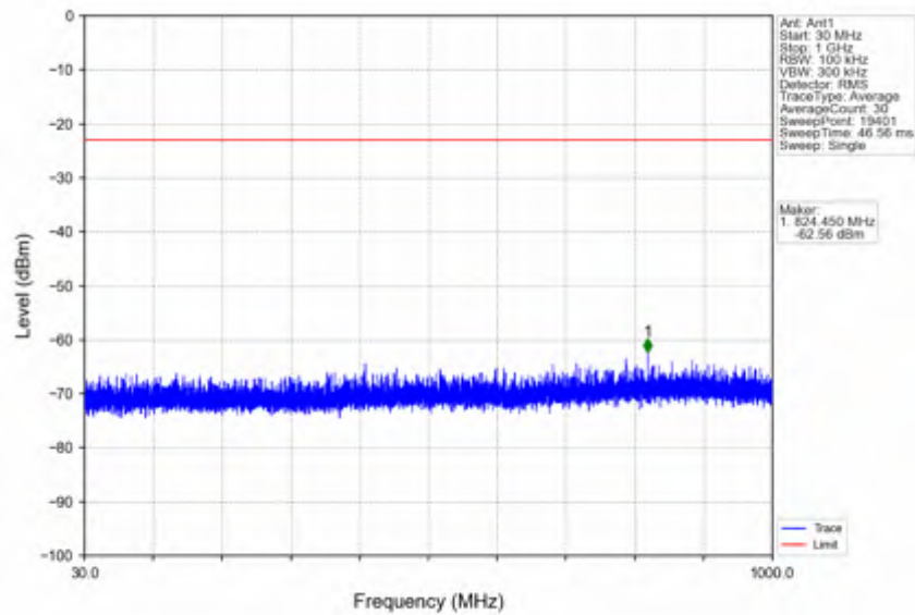
n66_15kHz_SISO_NTNV_20MHz_CP-OFDM QPSK_1745MHz_Edge_1RB_Left
