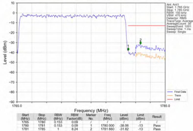
n66_15kHz_SISO_NTNV_15MHz_CP-OFDM QPSK_1772.5MHz_Outer_Full
