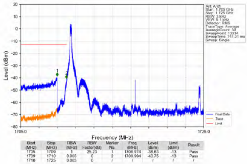
n66_15kHz_SISO_NTNV_15MHz_DFT-s-OFDM QPSK_1717.5MHz_Edge_1RB_Left
