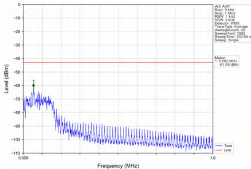
n66_15kHz_SISO_NTNV_30MHz_DFT-s-OFDM QPSK_1745MHz_Edge_1RB_Left
