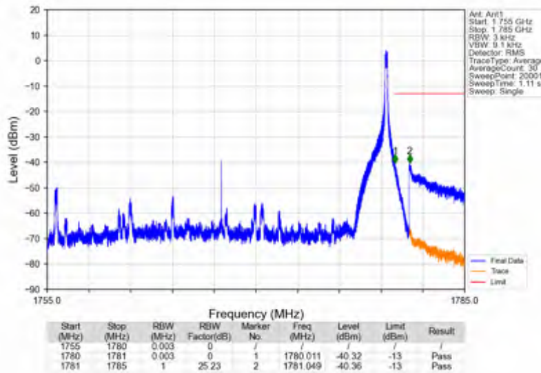
n66_15kHz_SISO_NTNV_25MHz_DFT-s-OFDM QPSK_1767.5MHz_Edge_1RB_Right
