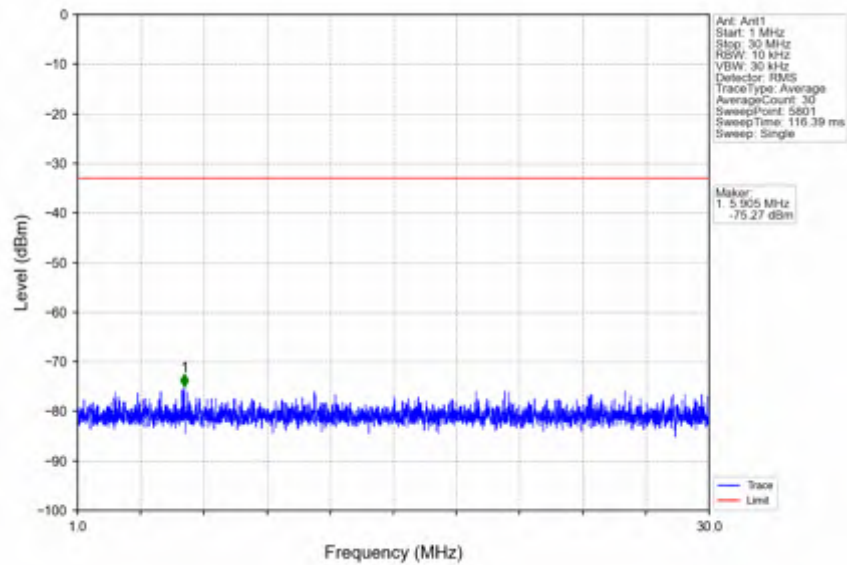
n66_15kHz_SISO_NTNV_15MHz_DFT-s-OFDM_QPSK_1717.5MHz_Outer_Full
