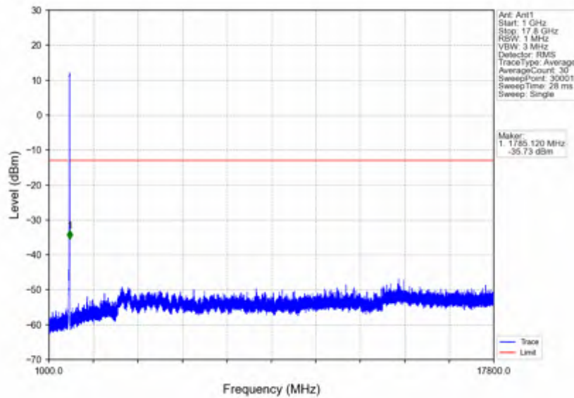
n66_15kHz_SISO_NTNV_15MHz_DFT-s-OFDM QPSK_1772.5MHz_Inner_1RB_Right
