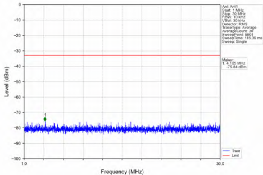
n66_15kHz_SISO_NTNV_15MHz_DFT-s-OFDM QPSK_1772.5MHz_Inner_1RB_Right
