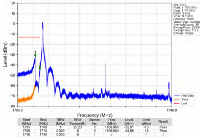
n66_15kHz_SISO_NTNV_30MHz_CP-OFDM QPSK_1725MHz_Edge_1RB_Left
