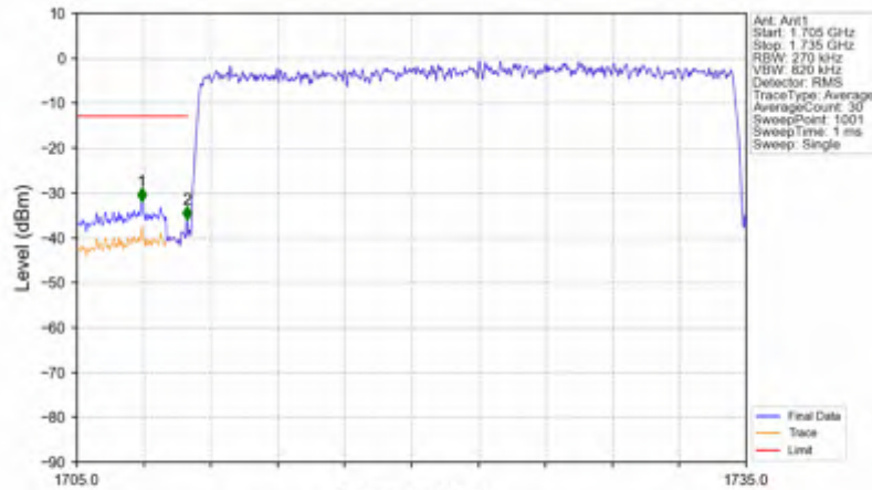
n66_15kHz_SISO_NTV_25MHz_CP-OFDM QPSK_1722.5MHz_Outer_Full
