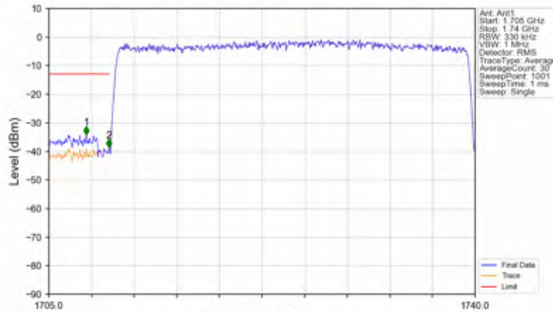
n66_15kHz_SISO_NTNV_30MHz_CP-OFDM QPSK_1725MHz_Outer_Full
