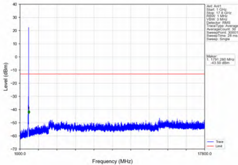
n66_15kHz_SISO_NTNV_25MHz_DFT-s-OFDM PI/2 BPSK_1767.5MHz_Outer_Full
