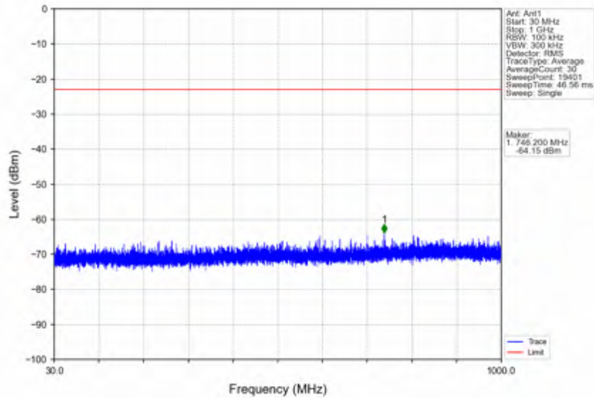
n66_15kHz_SISO_NTNV_15MHz_DFT-s-OFDM QPSK_1772.5MHz_Inner_1RB_Right
