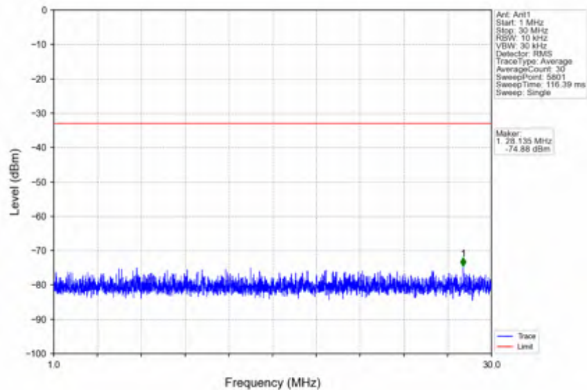
n66_15kHz_SISO_NTNV_25MHz_DFT-s-OFDM QPSK_1767.5MHz_Edge_1RB_Right
