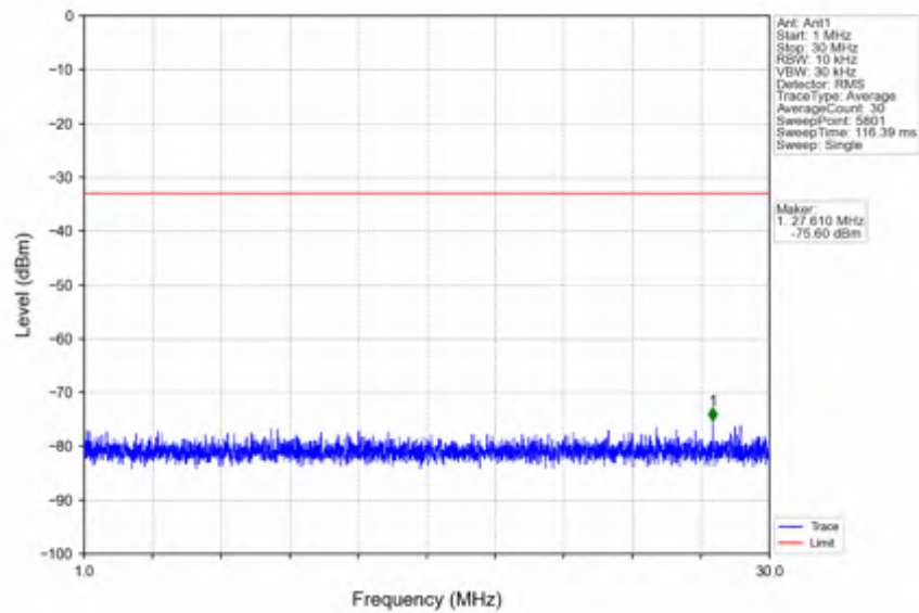
n66_15kHz_SISO_NTNV_25MHz_CP-OFDM QPSK_1767.5MHz_Inner_1RB_Right
