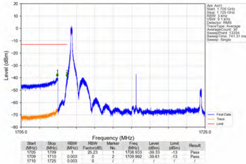
n66_15kHz_SISO_NTV_15MHz_CP-OFDM QPSK_1717.5MHz_Edge_1RB_Left
