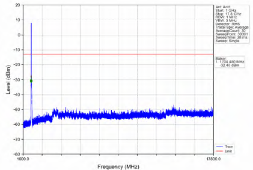
n66_15kHz_SISO_NTNV_25MHz_CP-OFDM QPSK_1722.5MHz_Outer_Full
