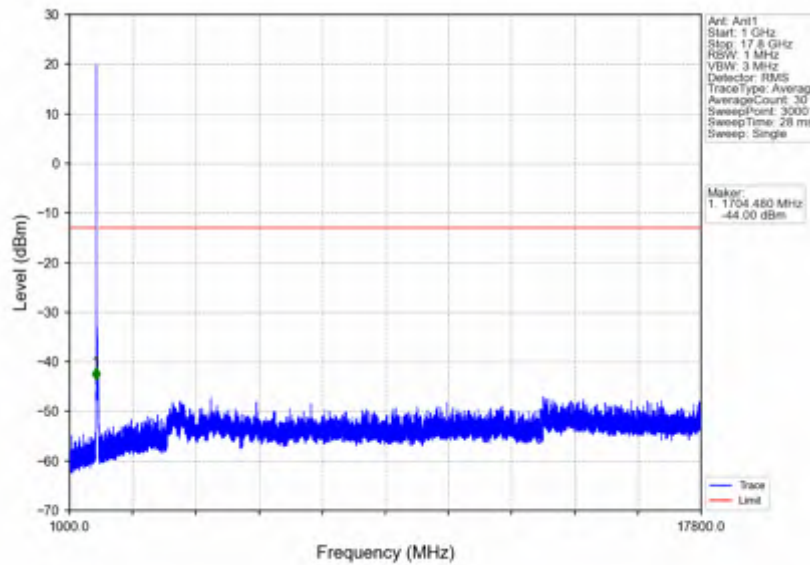
n66_15kHz_SISO_NTNV_30MHz_CP-OFDM QPSK_1725MHz_Outer_Full
