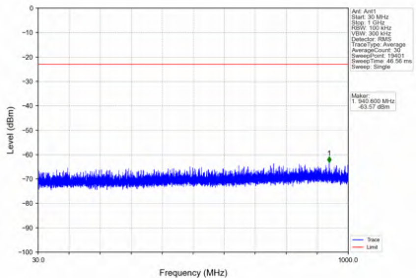
n66_15kHz_SISO_NTNV_15MHz_DFT-s-OFDM QPSK_1745MHz_Edge_1RB_Left
