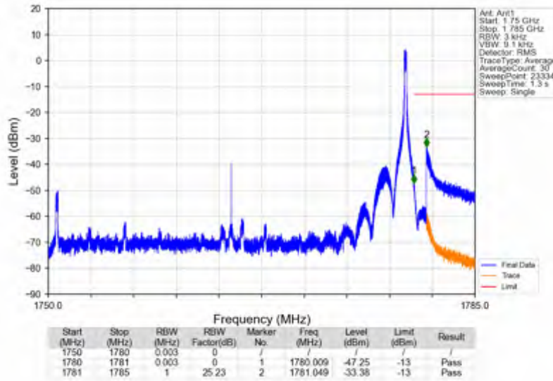
n66_15kHz_SISO_NTNV_30MHz_DFT-s-OFDM QPSK_1765MHz_Edge_1RB_Right
