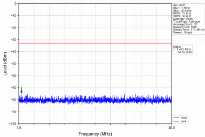
n66_15kHz_SISO_NTV_25MHz_CP-OFDM QPSK_1722.5MHz_Edge_1RB_Left
