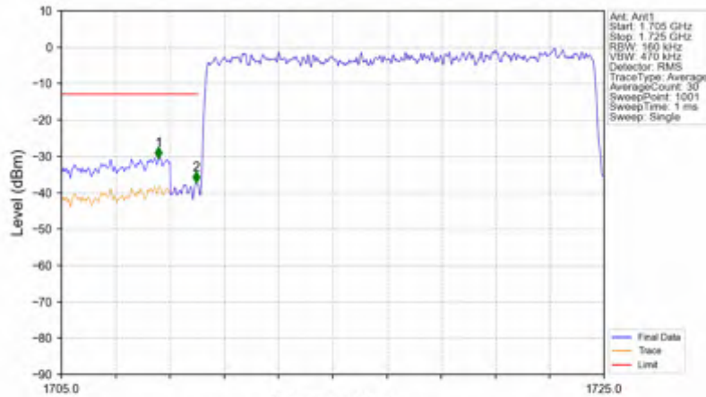
n66_15kHz_SISO_NTNV_15MHz_CP-OFDM QPSK_1717.5MHz_Outer_Full
