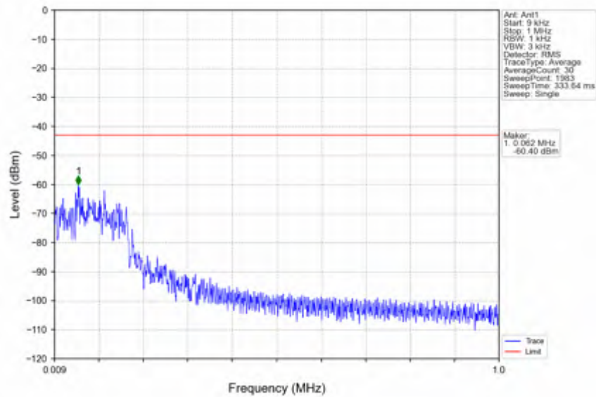
n66_15kHz_SISO_NTV_20MHz_DFT-s-OFDM_QPSK_1770MHz_Edge_1RB_Right
