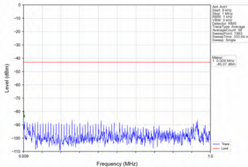
n66_15kHz_SISO_NTNV_30MHz_DFT-s-OFDM QPSK_1765MHz_Outer_Full
