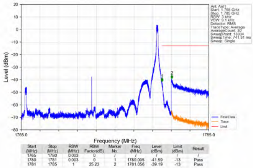
n66_15kHz_SISO_NTNV_15MHz_DFT-s-OFDM QPSK_1772.5MHz_Edge_1RB_Right
