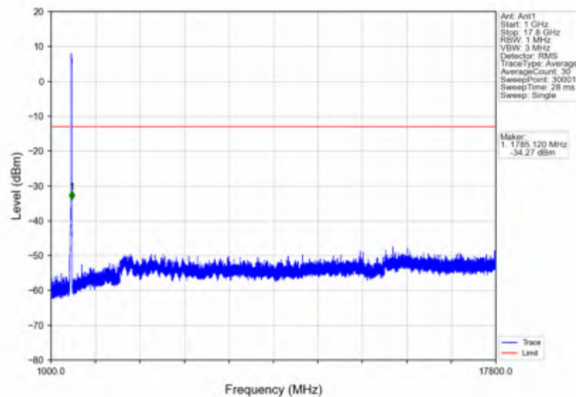
n66_15kHz_SISO_NTNV_25MHz_CP-OFDM QPSK_1767.5MHz_Outer_Full
