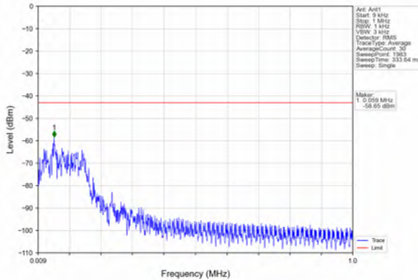
n66_15kHz_SISO_NTNV_25MHz_DFT-s-OFDM_QPSK_1722.5MHz_Inner_1RB_Left
