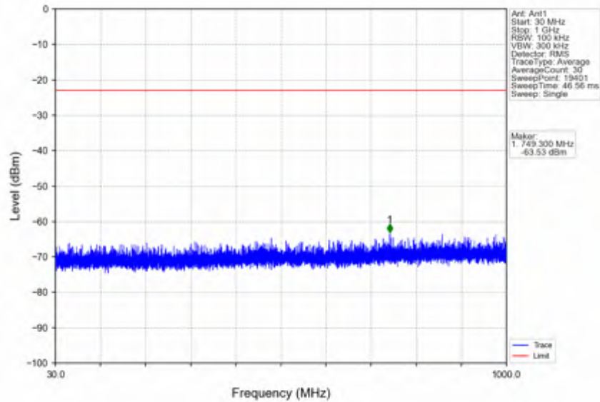
n66_15kHz_SISO_NTNV_15MHz_DFT-s-OFDM QPSK_1717.5MHz_Edge_1RB_Left
