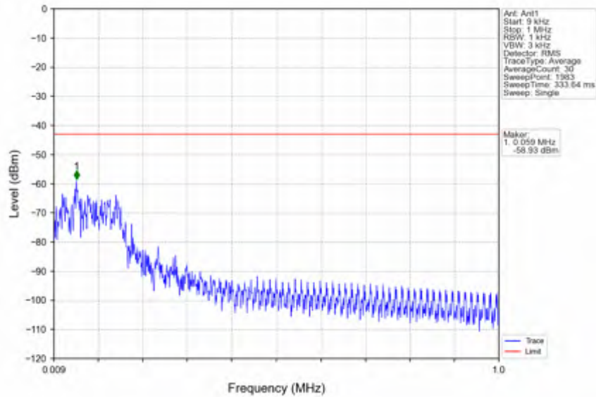
n66_15kHz_SISO_NTV_30MHz_DFT-s-OFDM_QPSK_1765MHz_Inner_1RB_Right
