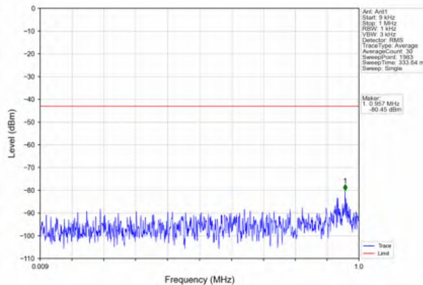
n66_15kHz_SISO_NTNV_20MHz_DFT-s-OFDM QPSK_1720MHz_Outer_Full
