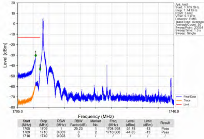
n66_15kHz_SISO_NTNV_30MHz_DFT-s-OFDM_PI/2_BPSK_1725MHz_Edge_1RB_Left
