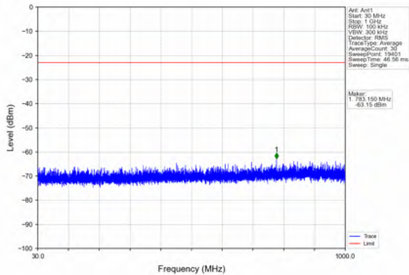
n66_15kHz_SISO_NTNV_25MHz_DFT-s-OFDM QPSK_1722.5MHz_Edge_1RB_Left
