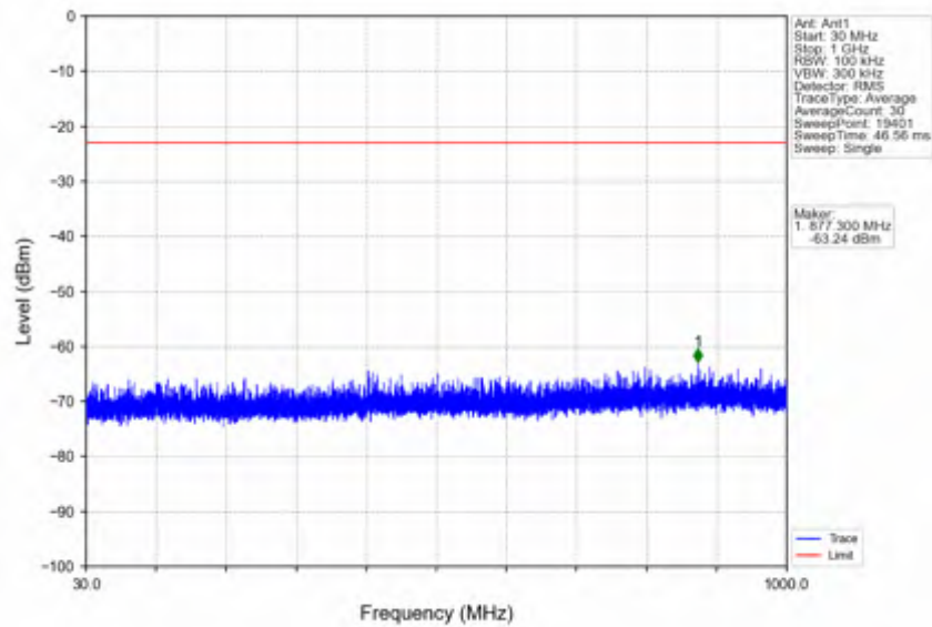
n66_15kHz_SISO_NTNV_30MHz_DFT-s-OFDM QPSK_1765MHz_Edge_1RB_Right
