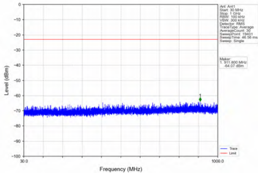
n66_15kHz_SISO_NTNV_30MHz_DFT-s-OFDM QPSK_1725MHz_Edge_1RB_Left
