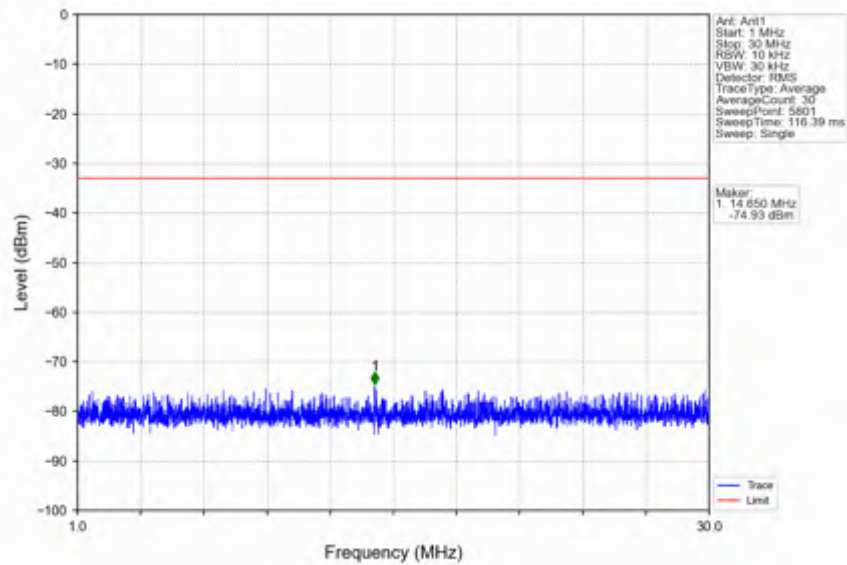
n66_15kHz_SISO_NTNV_20MHz_DFT-s-OFDM QPSK_1745MHz_Edge_1RB_Left
