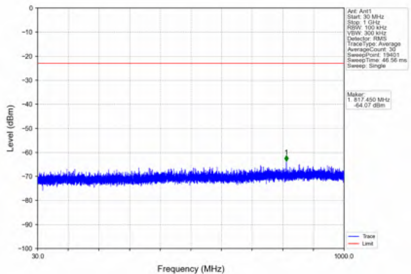
n66_15kHz_SISO_NTNV_25MHz_DFT-s-OFDM_QPSK_1767.5MHz_Outer_Full
