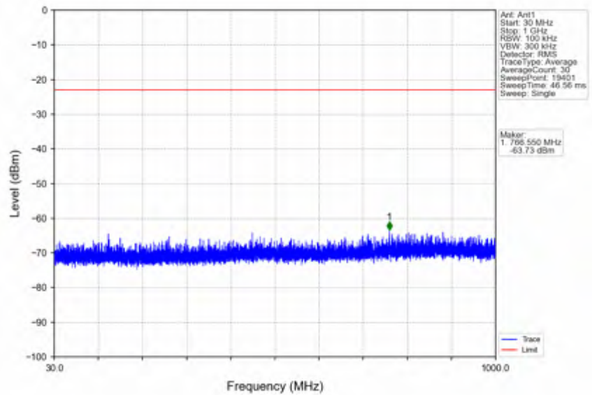
n66_15kHz_SISO_NTVV_15MHz_CP-OFDM QPSK_1717.5MHz_Edge_1RB_Left
