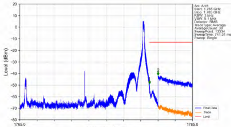
n66_15kHz_SISO_NTNV_15MHz_DFT-s-OFDM QPSK_1772.5MHz_Inner_1RB_Right
