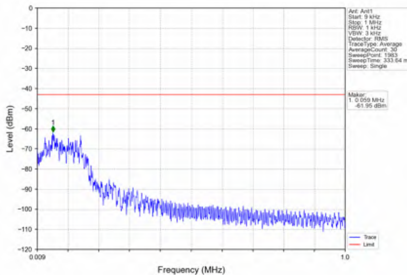
n66_15kHz_SISO_NTNV_20MHz_DFT-s-OFDM QPSK_1745MHz_Edge_1RB_Left
