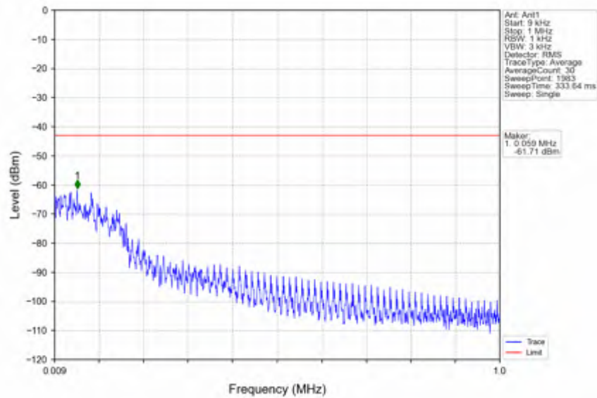
n66_15kHz_SISO_NTNV_15MHz_CP-OFDM QPSK_1745MHz_Edge_1RB_Left
