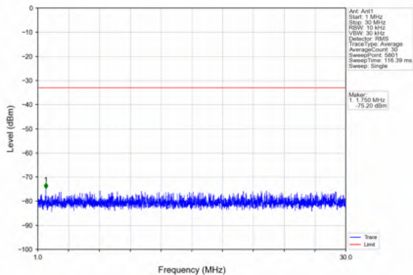
n66_15kHz_SISO_NTNV_30MHz_DFT-s-OFDM QPSK_1725MHz_Edge_1RB_Left
