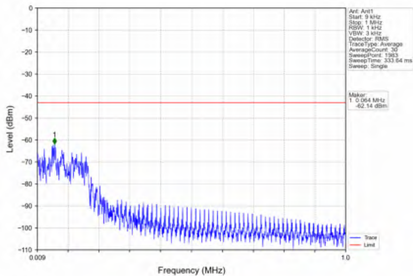
n66_15kHz_SISO_NTNV_30MHz_DFT-s-OFDM_PI/2_BPSK_1725MHz_Edge_1RB_Left
