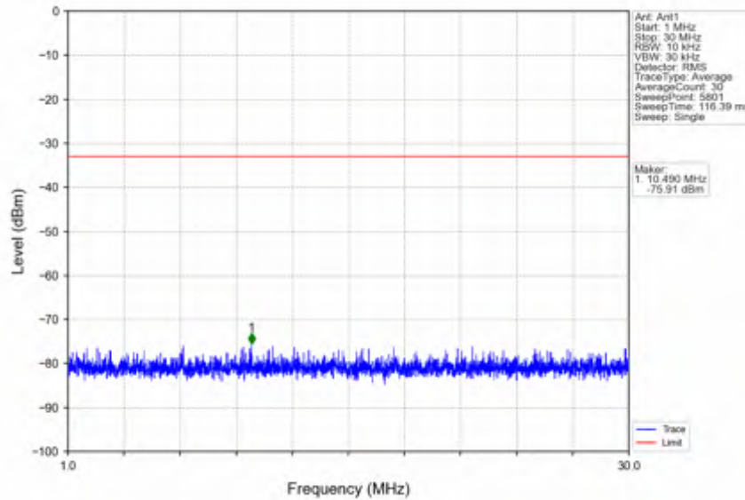
n66_15kHz_SISO_NTNV_25MHz_DFT-s-OFDM PI/2 BPSK_1767.5MHz_Inner_1RB_Right
