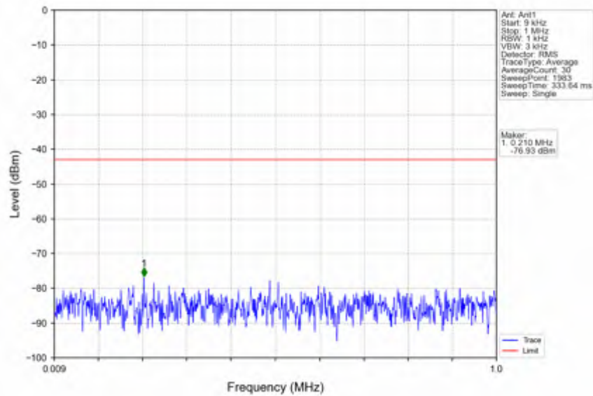
n66_15kHz_SISO_NTNV_15MHz_CP-OFDM QPSK_1772.5MHz_Outer_Full
