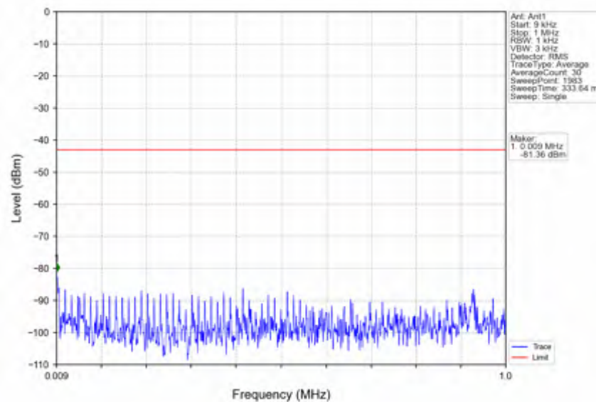
n66_15kHz_SISO_NTNV_30MHz_DFT-s-OFDM QPSK_1725MHz_Outer_Full
