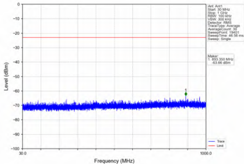
n66_15kHz_SISO_NTNV_15MHz_DFT-s-OFDM PI/2 BPSK_1772.5MHz_Inner_1RB_Right
