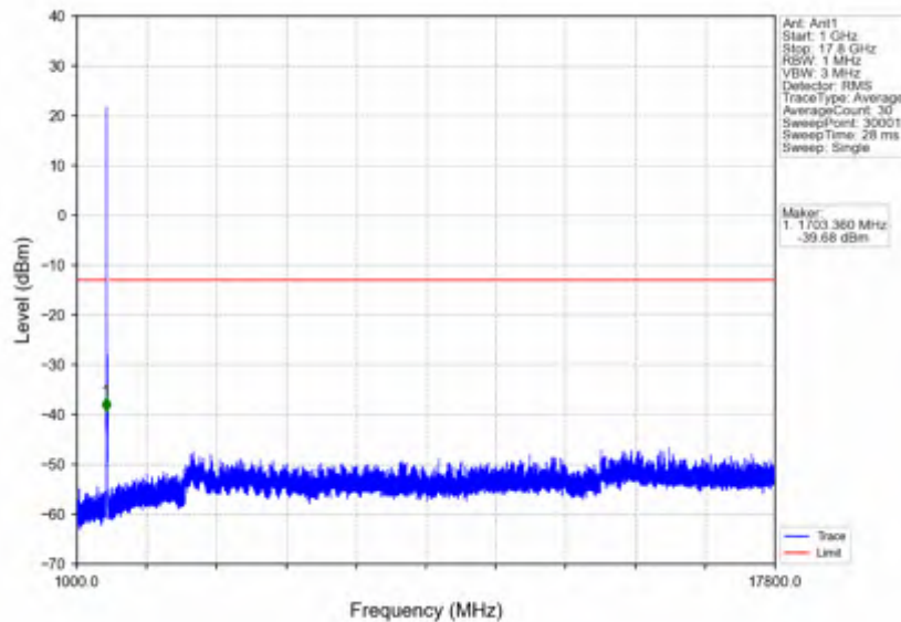
n66_15kHz_SISO_NTNV_15MHz_DFT-s-OFDM QPSK_1717.5MHz_Edge_1RB_Left
