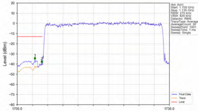
n66_15kHz_SISO_NTNV_25MHz_DFT-s-OFDM PI/2 BPSK_1722.5MHz_Outer_Full
