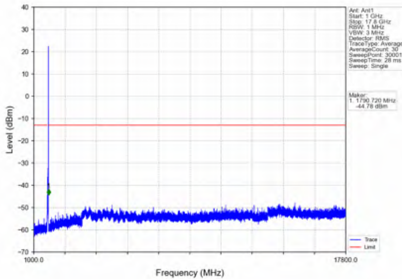
n66_15kHz_SISO_NTNV_25MHz_DFT-s-OFDM QPSK_1722.5MHz_Edge_1RB_Left
