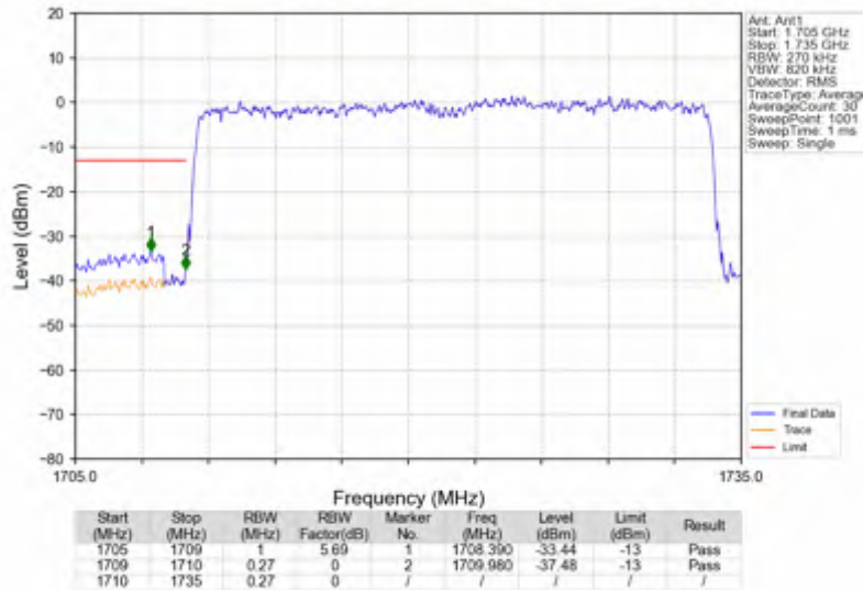
n66_15kHz_SISO_NTNV_25MHz_DFT-s-OFDM_QPSK_1722.5MHz_Outer_Full
