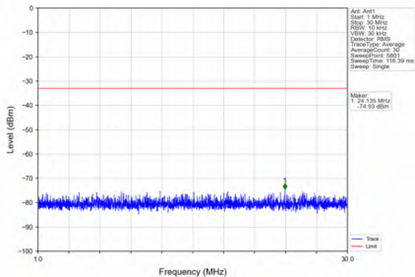
n66_15kHz_SISO_NTNV_25MHz_DFT-s-OFDM QPSK_1722.5MHz_Edge_1RB_Left
