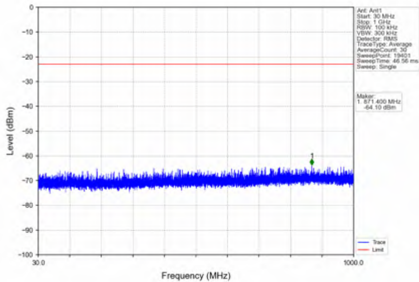
n66_15kHz_SISO_NTNV_25MHz_DFT-s-OFDM QPSK_1767.5MHz_Edge_1RB_Right
