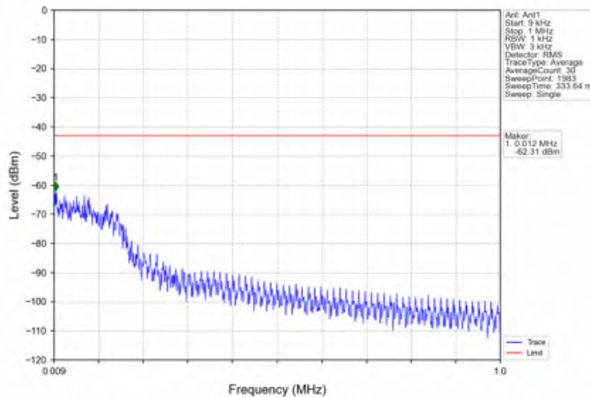
n66_15kHz_SISO_NTNV_30MHz_CP-OFDM QPSK_1725MHz_Edge_1RB_Left
