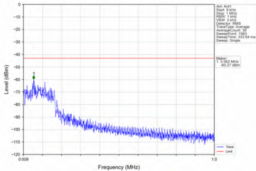
n66_15kHz_SISO_NTNV_15MHz_DFT-s-OFDM QPSK_1772.5MHz_Edge_1RB_Right
