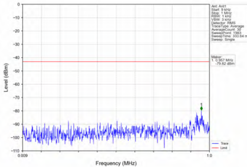
n66_15kHz_SISO_NTNV_20MHz_DFT-s-OFDM QPSK_1770MHz_Outer_Full
