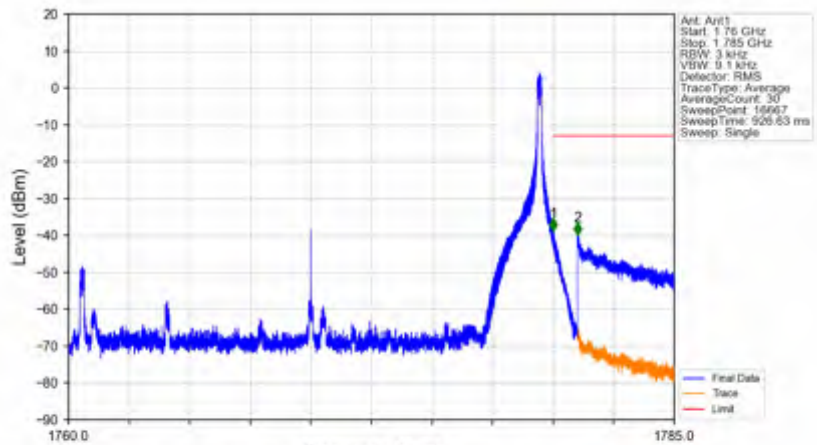
n66_15kHz_SISO_NTNV_20MHz_DFT-s-OFDM QPSK_1770MHz_Edge_1RB_Right
