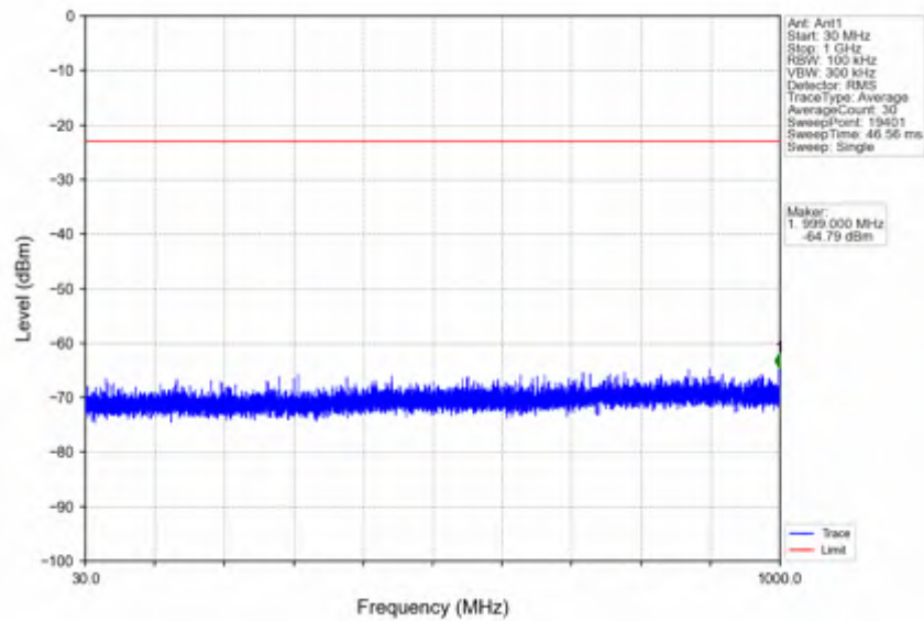
n66_15kHz_SISO_NTNV_15MHz_CP-OFDM QPSK_1717.5MHz_Outer_Full
