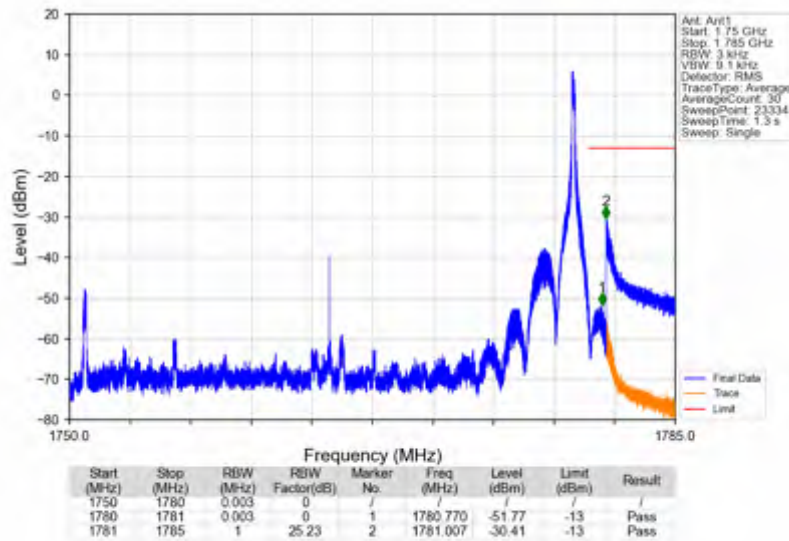
n66_15kHz_SISO_NTNV_30MHz_DFT-s-OFDM QPSK_1765MHz_Inner_1RB_Right
