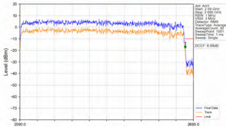
n41_30kHz_SISO_NTNV_100MHz_CP-OFDM QPSK_2640MHz_Outer_Full
