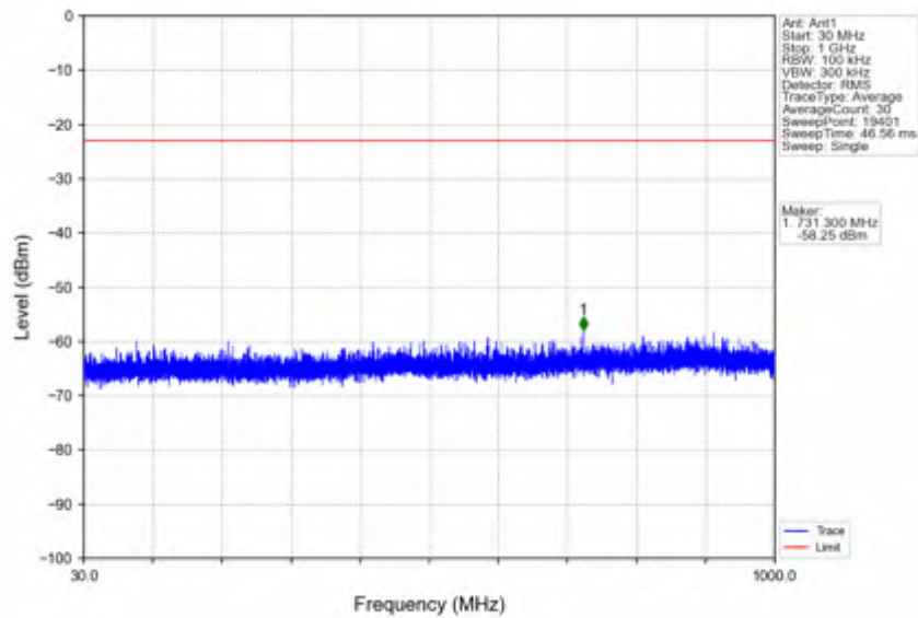
n41_30kHz_SISO_NTV_100MHz_CP-OFDM QPSK_2592.99MHz_Edge_1RB_Left
