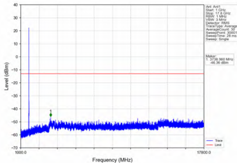
n66_15kHz_SISO_NTV_10MHz_DFT-s-OFDM PI/2 BPSK_1745MHz_Edge_1RB_Left
