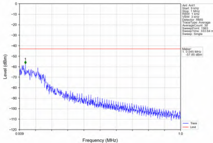
n66_15kHz_SISO_NTNV_5MHz_CP-OFDM QPSK_1777.5MHz_Inner_1RB_Right
