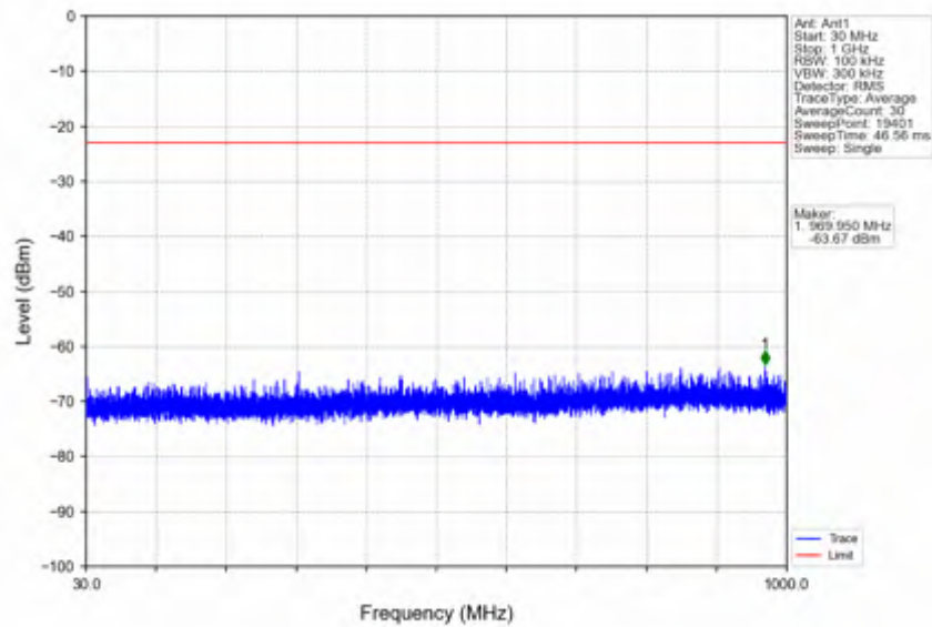
n66_15kHz_SISO_NTNV_5MHz_DFT-s-OFDM QPSK_1777.5MHz_Edge_1RB_Right
