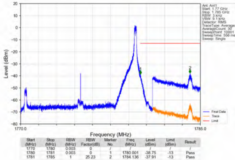
n66_15kHz_SISO_NTV_10MHz_CP-OFDM QPSK_1775MHz_Edge_1RB_Right
