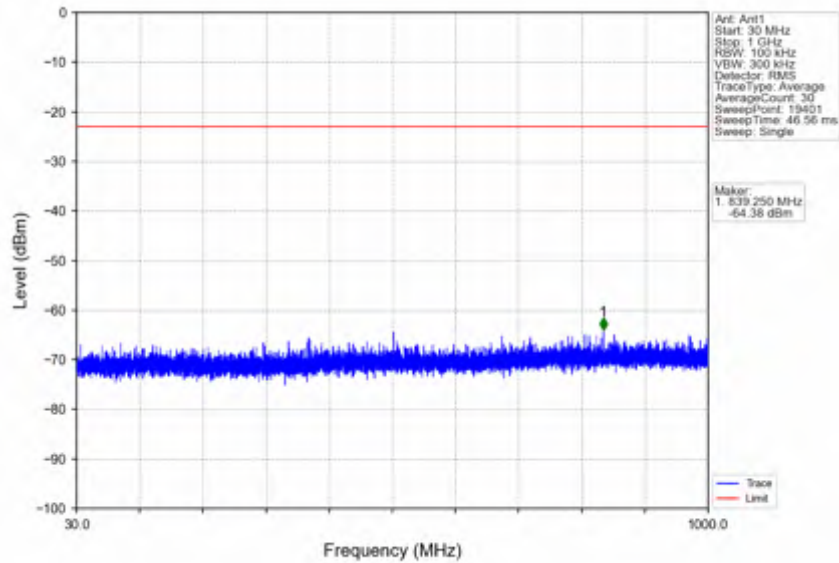
n66_15kHz_SISO_NTNV_5MHz_DFT-s-OFDM QPSK_1777.5MHz_Inner_1RB_Right
