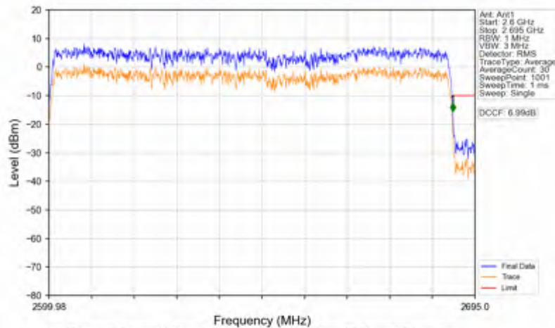
n41_30kHz_SISO_NTV_90MHz_CP-OFDM QPSK_2644.98MHz_Outer_Full
