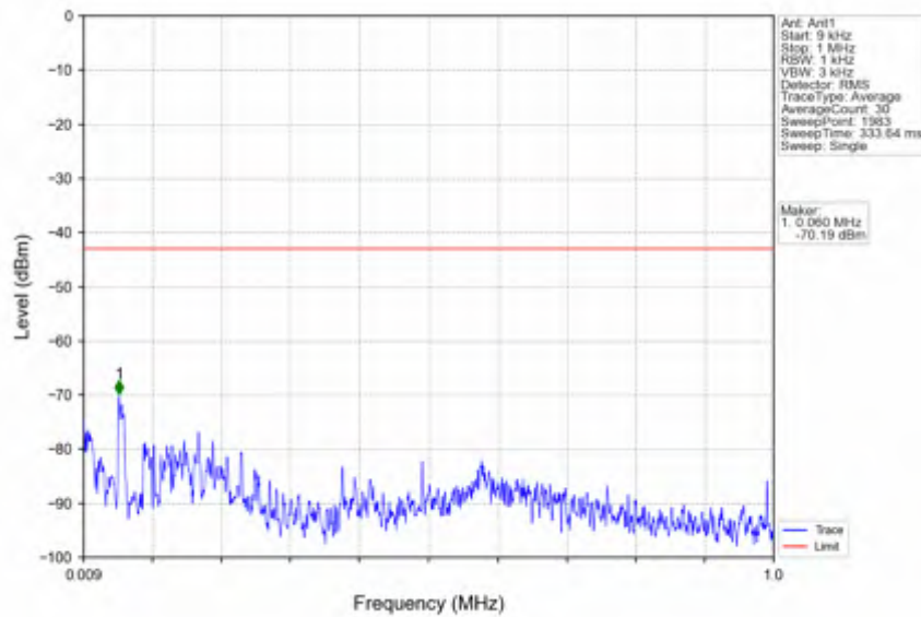
n41_30kHz_SISO_NTNV_100MHz_DFT-s-OFDM PI/2 BPSK_2640MHz_Outer_Full
