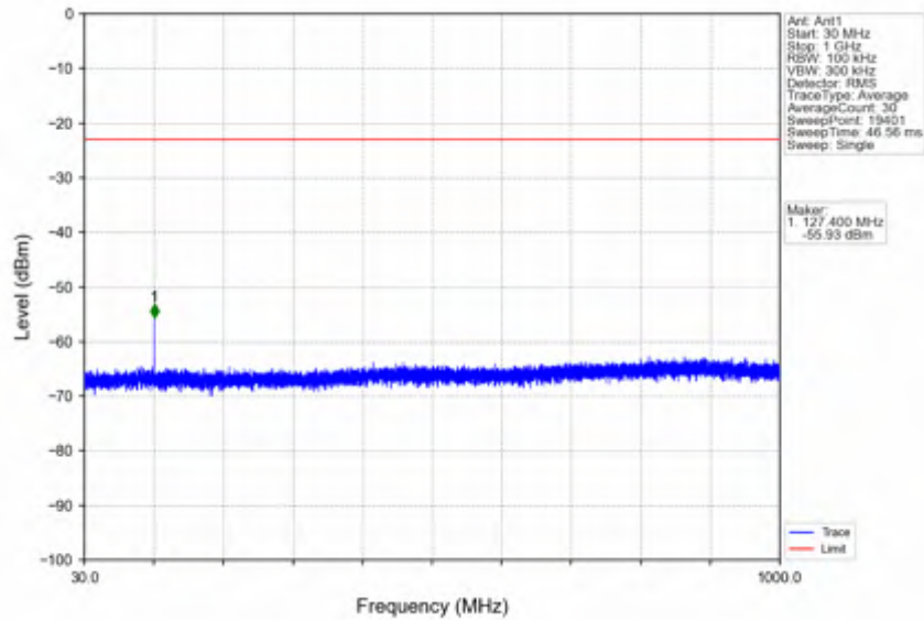
n41_30kHz_SISO_NTNV_100MHz_DFT-s-OFDM QPSK_2640MHz_Inner_1RB_Right
