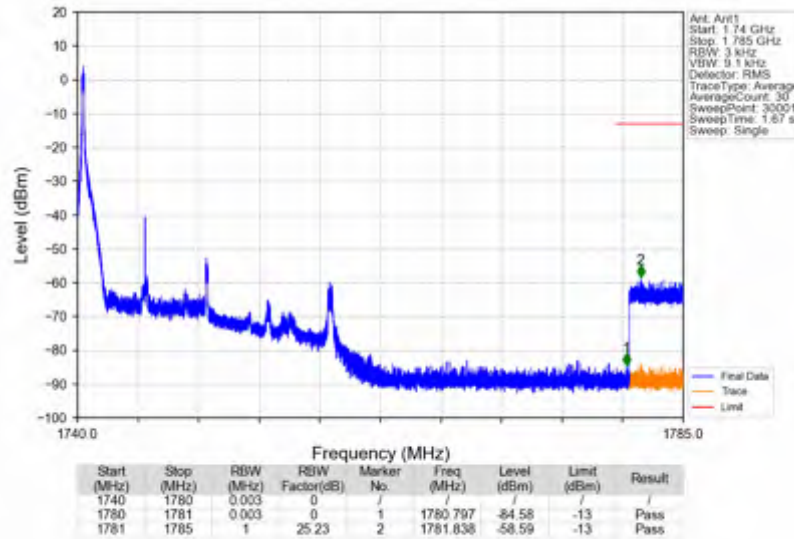
n66_15kHz_SISO_NTNV_10MHz_DFT-s-OFDM QPSK_1745MHz_Edge_1RB_Left
