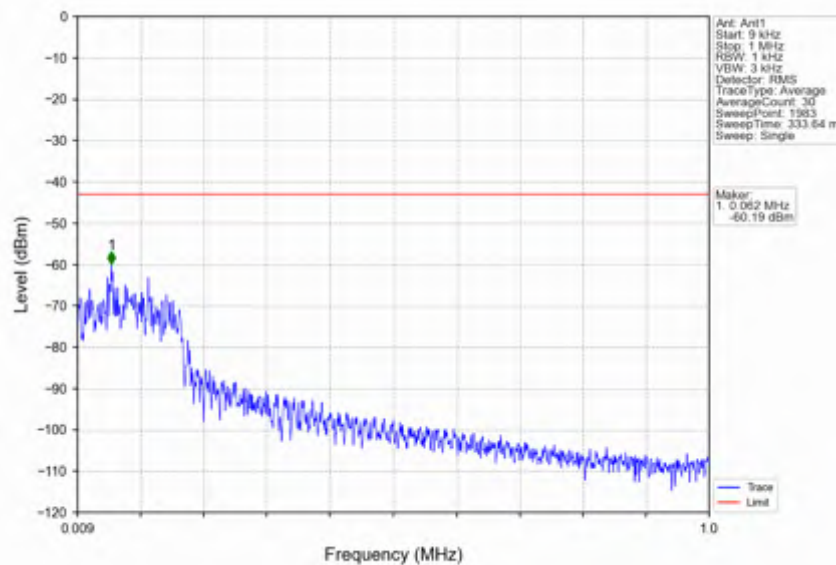
n66_15kHz_SISO_NTV_5MHz_DFT-s-OFDM QPSK_1745MHz_Edge_1RB_Left
