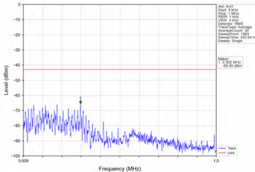
n41_30kHz_SISO_NTNV_100MHz_DFT-s-OFDM_PI/2_BPSK_2640MHz_Inner_1RB_Right
