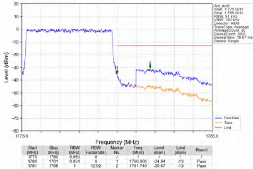
n66_15kHz_SISO_NTNV_5MHz_DFT-s-OFDM QPSK_1777.5MHz_Outer_Full
