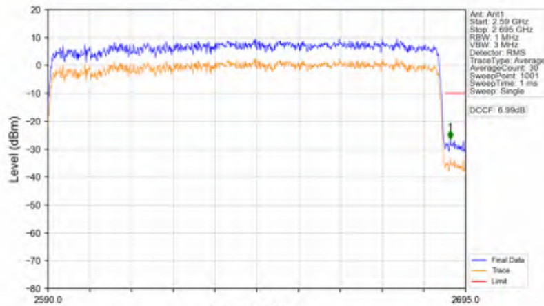
n41_30kHz_SISO_NTNV_100MHz_DFT-s-OFDM PI/2 BPSK_2640MHz_Outer_Full
