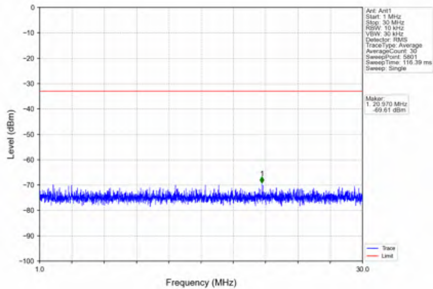
n41_30kHz_SISO_NTNV_100MHz_CP-OFDM QPSK_2640MHz_Edge_1RB_Right
