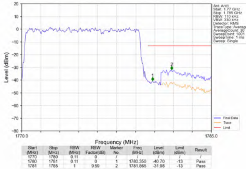
n66_15kHz_SISO_NTNV_10MHz_DFT-s-OFDM QPSK_1775MHz_Outer_Full
