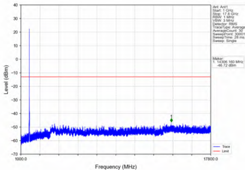
n66_15kHz_SISO_NTV_15MHz_DFT-s-OFDM PI/2 BPSK_1745MHz_Edge_1RB_Left
