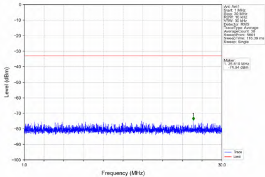
n66_15kHz_SISO_NTNV_10MHz_CP-OFDM QPSK_1715MHz_Edge_1RB_Left
