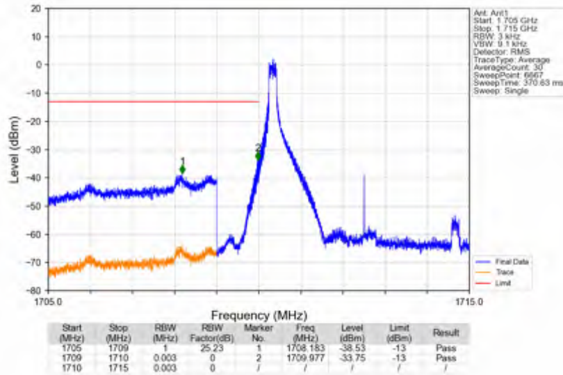
n66_15kHz_SISO_NTNV_5MHz_CP-OFDM QPSK_1712.5MHz_Edge_1RB_Left
