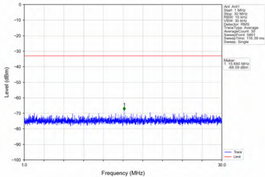
n41_30kHz_SISO_NTNV_100MHz_CP-OFDM QPSK_2546.01MHz_Edge_1RB_Left
