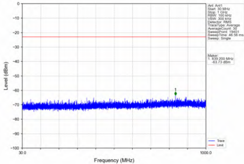
n66_15kHz_SISO_NTNV_5MHz_DFT-s-OFDM QPSK_1712.5MHz_Inner_1RB_Left
