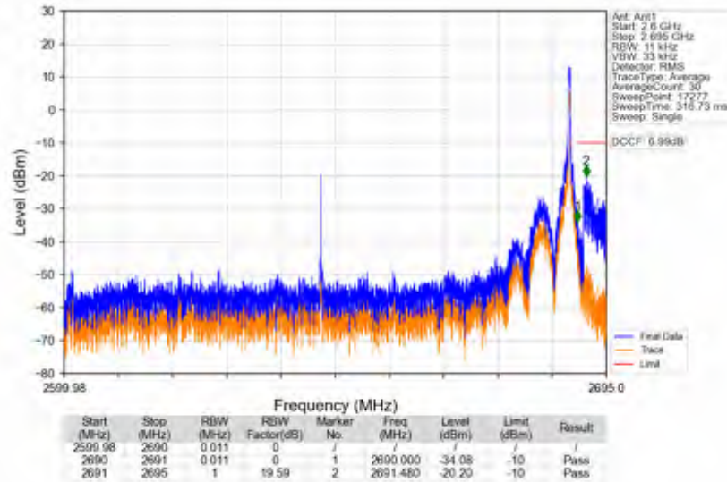
n41_30kHz_SISO_NTV_90MHz_CP-OFDM QPSK_2644.98MHz_Inner_1RB_Right
