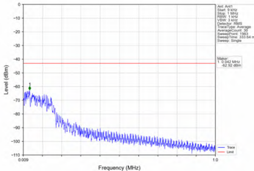
n66_15kHz_SISO_NTV_10MHz_CP-OFDM QPSK_1775MHz_Edge_1RB_Right
