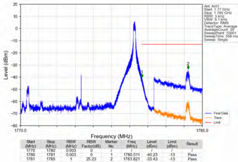
n66_15kHz_SISO_NTNV_10MHz_DFT-s-OFDM QPSK_1775MHz_Inner_1RB_Right
