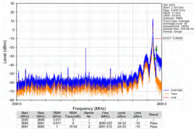
n41_30kHz_SISO_NTNV_100MHz_DFT-s-OFDM QPSK_2640MHz_Inner_1RB_Right
