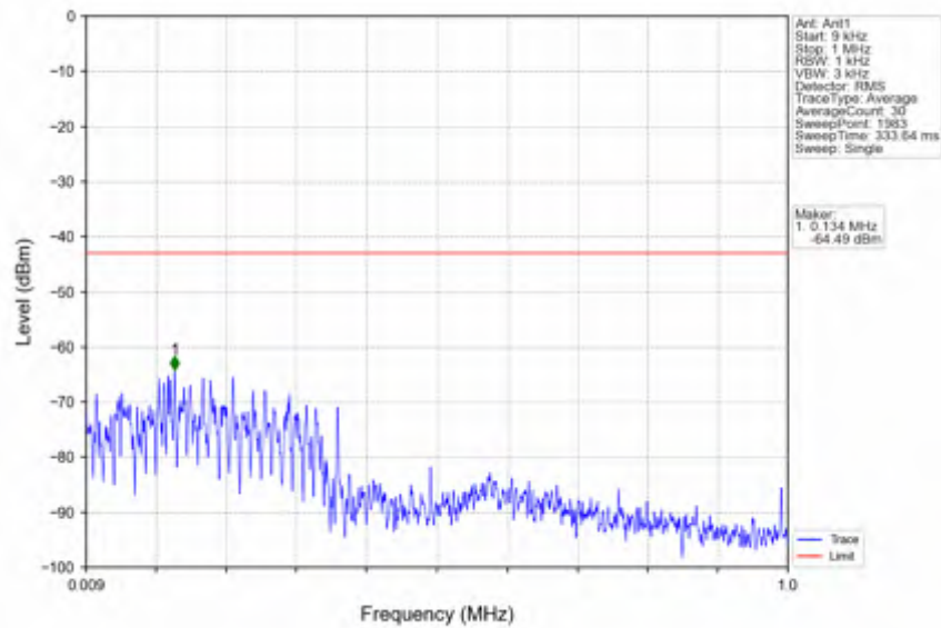
n41_30kHz_SISO_NTNV_100MHz_DFT-s-OFDM QPSK_2640MHz_Inner_1RB_Right
