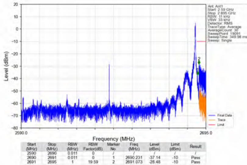
n41_30kHz_SISO_NTNV_100MHz_CP-OFDM QPSK_2640MHz_Edge_1RB_Right
