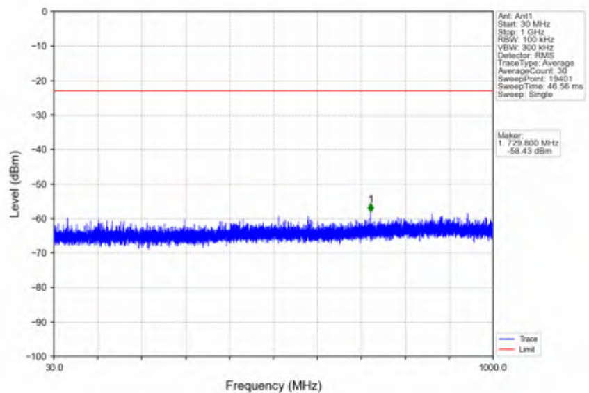
n41_30kHz_SISO_NTNV_100MHz_DFT-s-OFDM QPSK_2592.99MHz_Edge_1RB_Left
