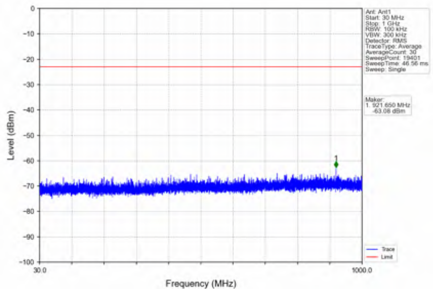
n66_15kHz_SISO_NTNV_5MHz_DFT-s-OFDM QPSK_1777.5MHz_Outer_Full
