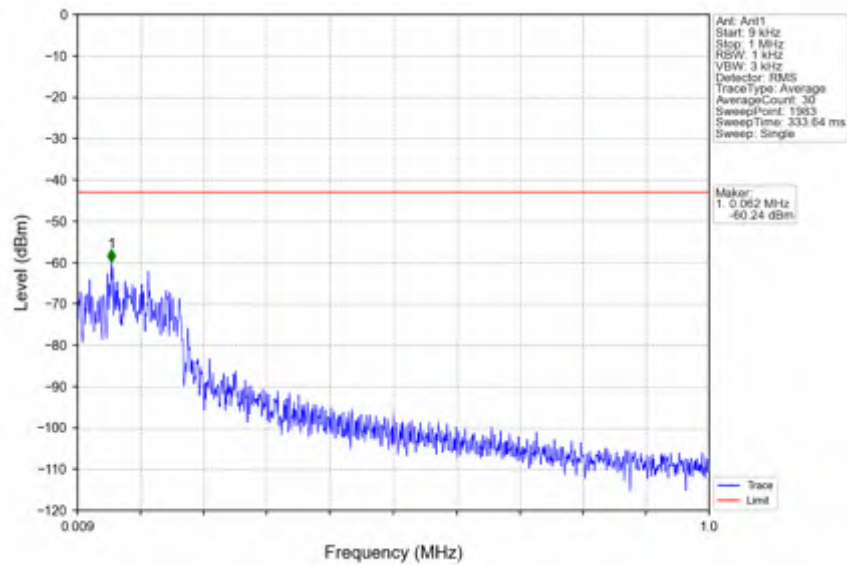
n66_15kHz_SISO_NTNV_5MHz_DFT-s-OFDM QPSK_1777.5MHz_Edge_1RB_Right
