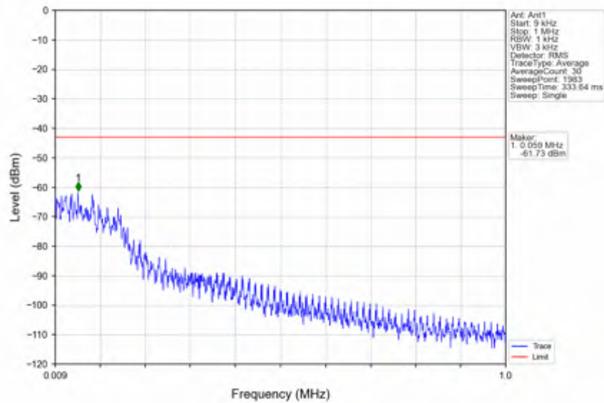
n66_15kHz_SISO_NTNV_5MHz_CP-OFDM QPSK_1745MHz_Edge_1RB_Left
