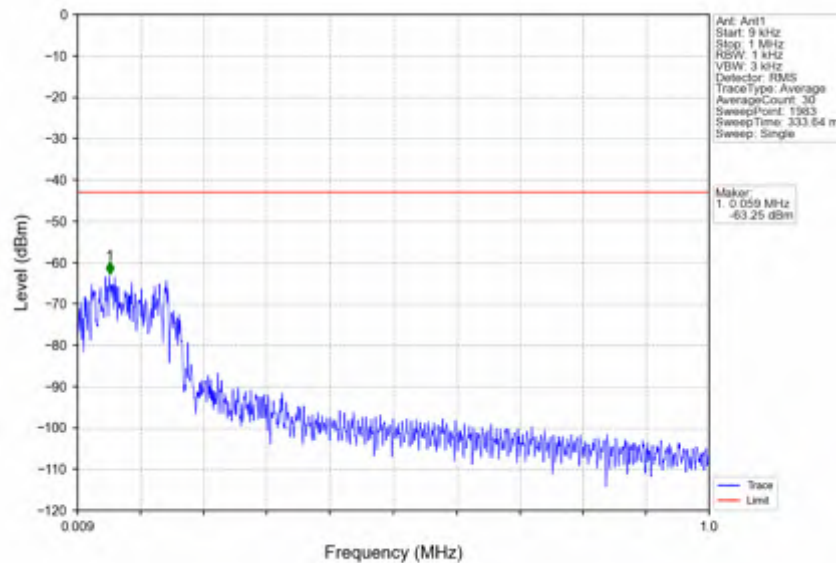
n66_15kHz_SISO_NTNV_10MHz_DFT-s-OFDM QPSK_1745MHz_Edge_1RB_Left
