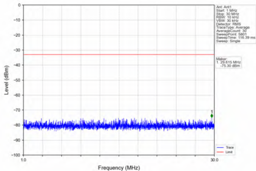
n66_15kHz_SISO_NTNV_10MHz_CP-OFDM QPSK_1745MHz_Edge_1RB_Left
