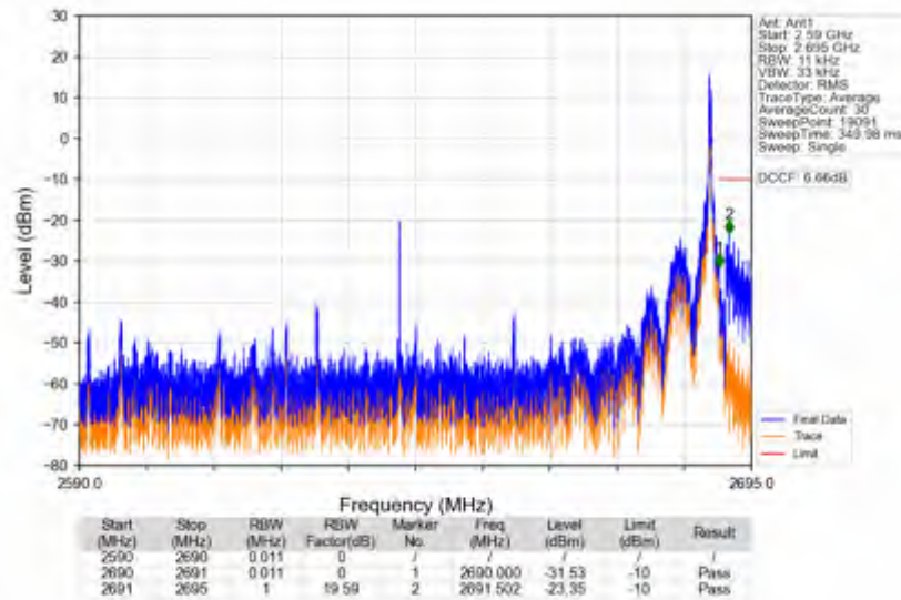
n41_30kHz_SISO_NTNV_100MHz_DFT-s-OFDM_PI/2_BPSK_2640MHz_Inner_1RB_Right
