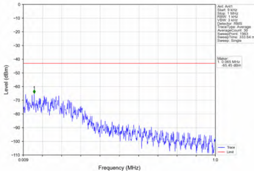
n41_30kHz_SISO_NTNV_90MHz_CP-OFDM QPSK_2644.98MHz_Edge_1RB_Right
