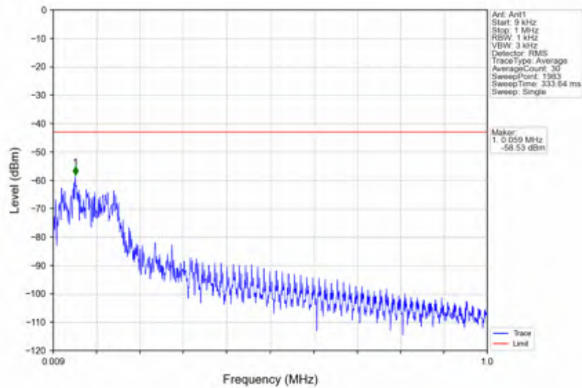
n66_15kHz_SISO_NTNV_5MHz_DFT-s-OFDM QPSK_1712.5MHz_Inner_1RB_Left
