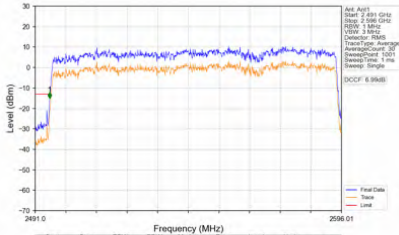
n41_30kHz_SISO_NTNV_100MHz_DFT-s-OFDM_QPSK_2546.01MHz_Outer_Full
