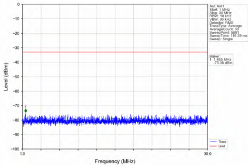
n66_15kHz_SISO_NTNV_5MHz_CP-OFDM QPSK_1777.5MHz_Edge_1RB_Right
