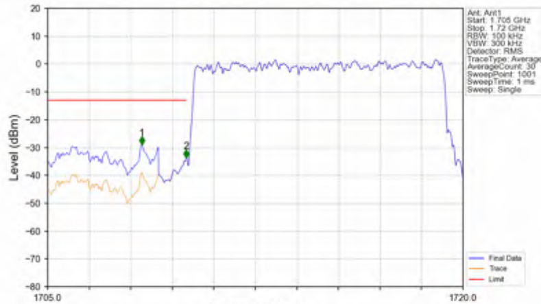
n66_15kHz_SISO_NTNV_10MHz_DFT-s-OFDM PI/2 BPSK_1715MHz_Outer_Full
