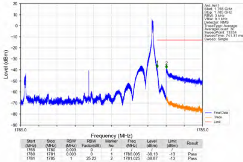
n66_15kHz_SISO_NTNV_15MHz_DFT-s-OFDM PI/2 BPSK_1772.5MHz_Edge_1RB_Right
