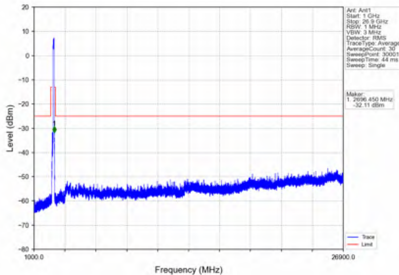
n41_30kHz_SISO_NTNV_100MHz_DFT-s-OFDM PI/2 BPSK_2640MHz_Outer_Full
