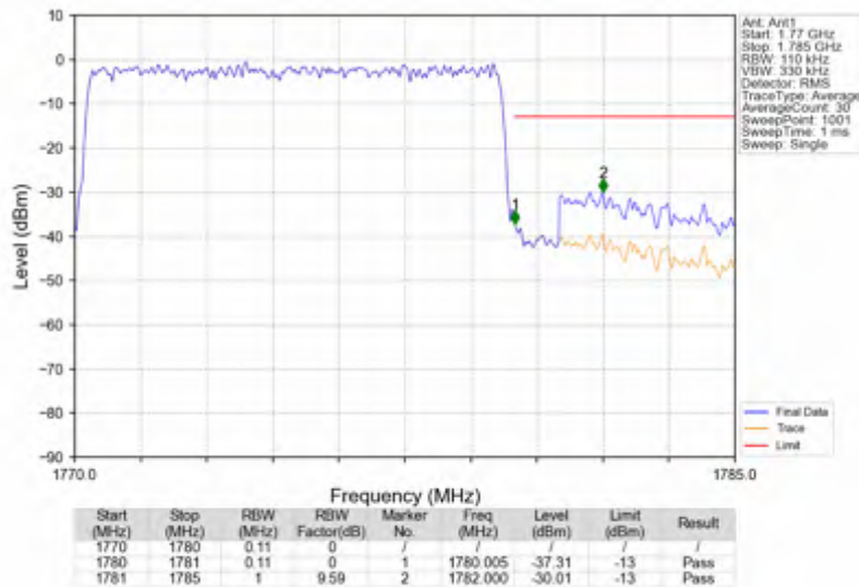
n66_15kHz_SISO_NTNV_10MHz_CP-OFDM QPSK_1775MHz_Outer_Full
