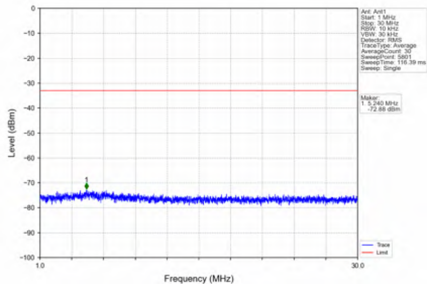
n41_30kHz_SISO_NTNV_90MHz_CP-OFDM QPSK_2644.98MHz_Outer_Full
