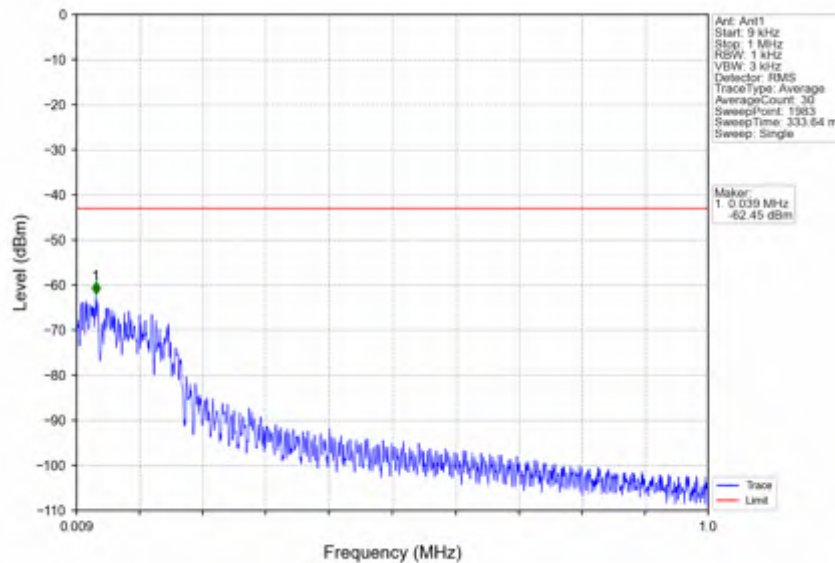
n66_15kHz_SISO_NTNV_10MHz_CP-OFDM QPSK_1715MHz_Edge_1RB_Left
