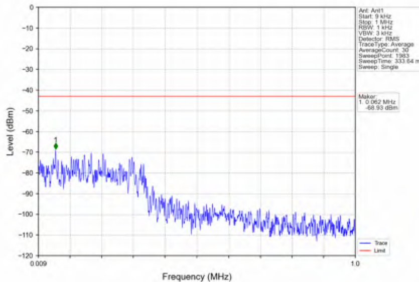
n41_30kHz_SISO_NTNV_100MHz_DFT-s-OFDM QPSK_2592.99MHz_Edge_1RB_Left
