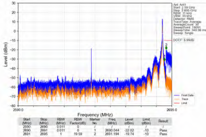
n41_30kHz_SISO_NTNV_100MHz_CP-OFDM QPSK_2640MHz_Inner_1RB_Right
