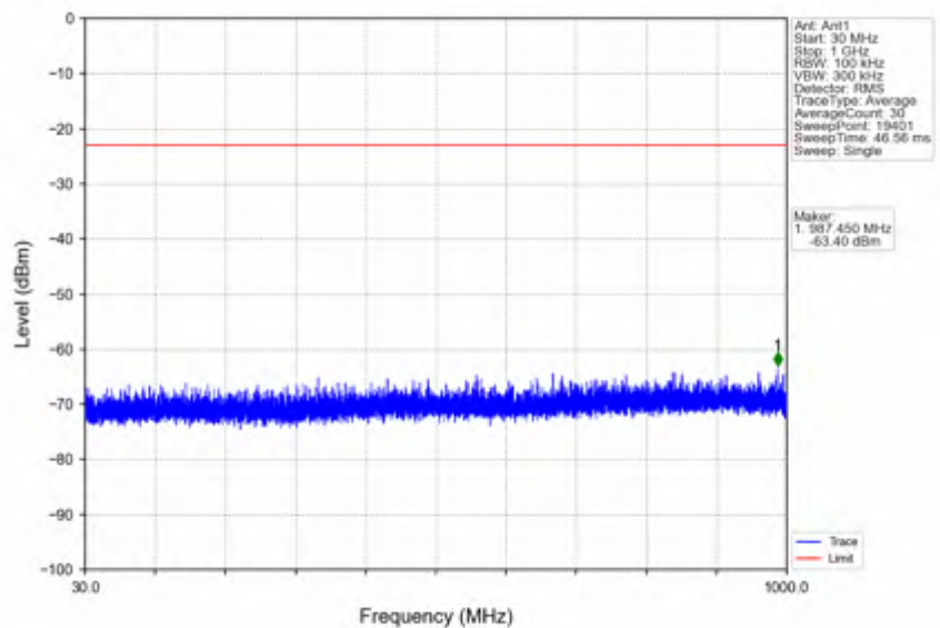
n66_15kHz_SISO_NTV_5MHz_DFT-s-OFDM QPSK_1745MHz_Edge_1RB_Left
