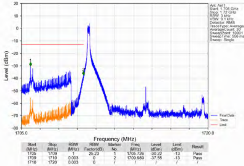
n66_15kHz_SISO_NTNV_10MHz_DFT-s-OFDM_PI/2_BPSK_1715MHz_Edge_1RB_Left
