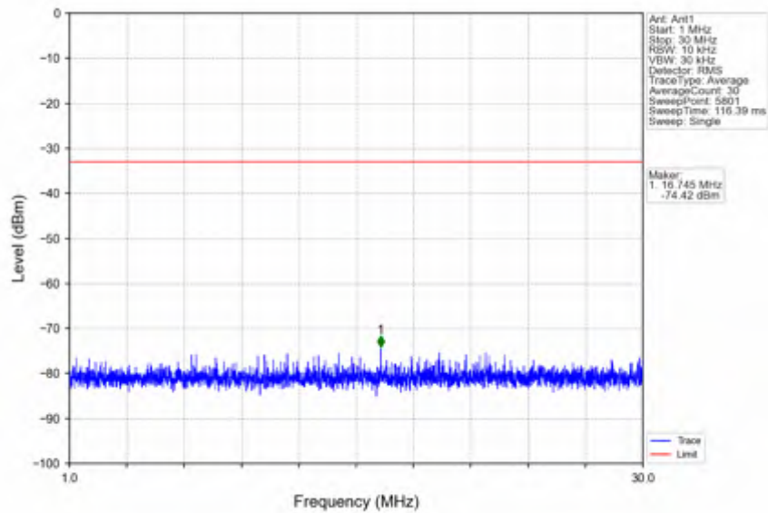
n66_15kHz_SISO_NTNV_5MHz_DFT-s-OFDM PI/2 BPSK_1777.5MHz_Inner_1RB_Right
