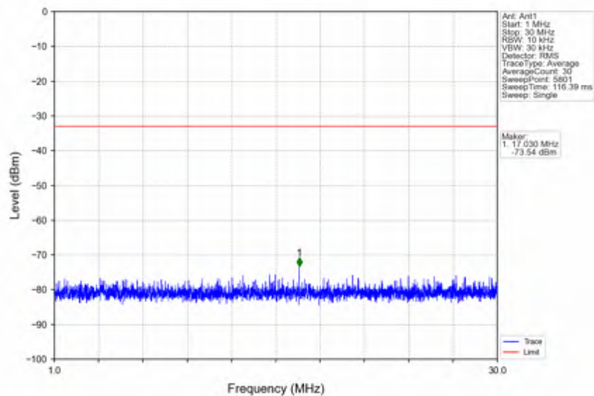
n66_15kHz_SISO_NTNV_5MHz_DFT-s-OFDM QPSK_1777.5MHz_Inner_1RB_Right
