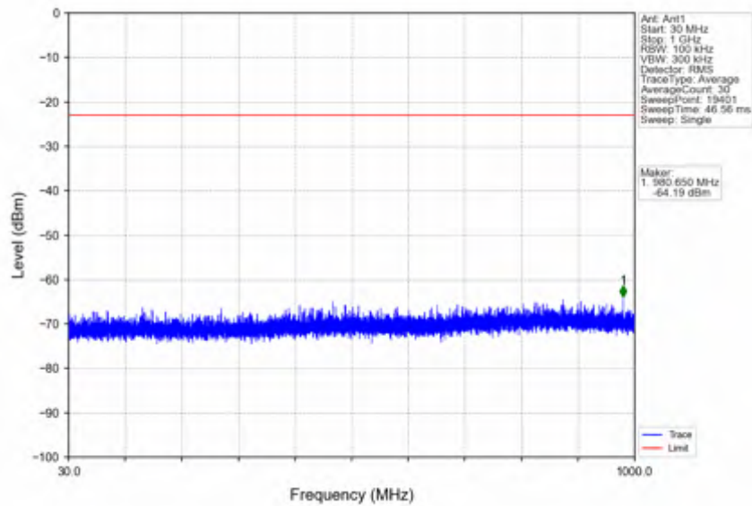
n66_15kHz_SISO_NTNV_10MHz_DFT-s-OFDM PI/2 BPSK_1775MHz_Outer_Full
