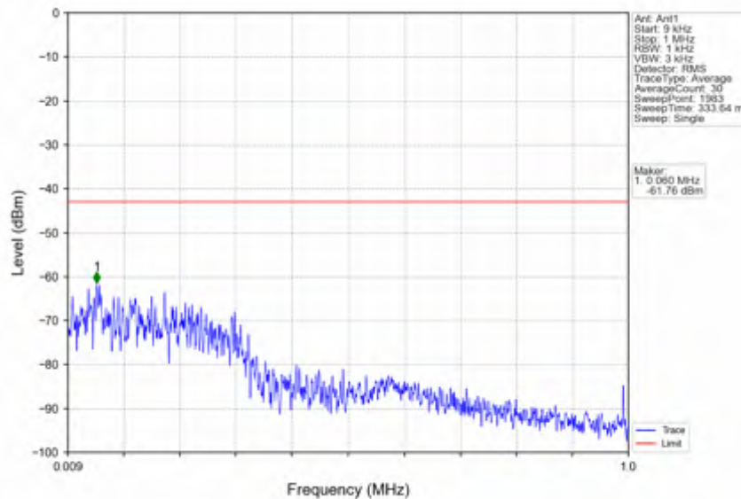
n41_30kHz_SISO_NTNV_100MHz_CP-OFDM QPSK_2640MHz_Inner_1RB_Right
