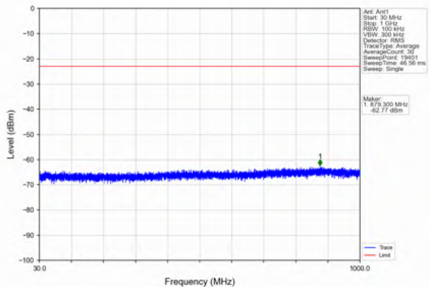
n41_30kHz_SISO_NTNV_100MHz_DFT-s-OFDM QPSK_2640MHz_Outer_Full
