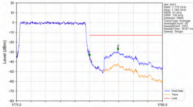
n66_15kHz_SISO_NTNV_5MHz_DFT-s-OFDM PI/2 BPSK_1777.5MHz_Outer_Full
