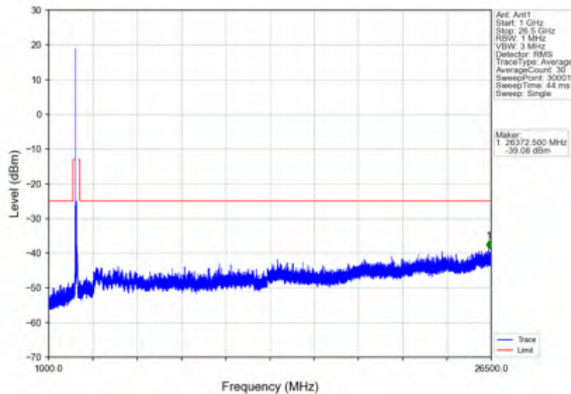
n41_30kHz_SISO_NTV_100MHz_CP-OFDM QPSK_2592.99MHz_Edge_1RB_Left
