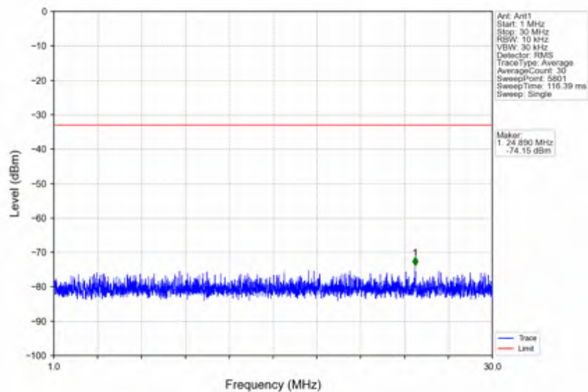
n66_15kHz_SISO_NTV_10MHz_DFT-s-OFDM PI/2 BPSK_1745MHz_Edge_1RB_Left
