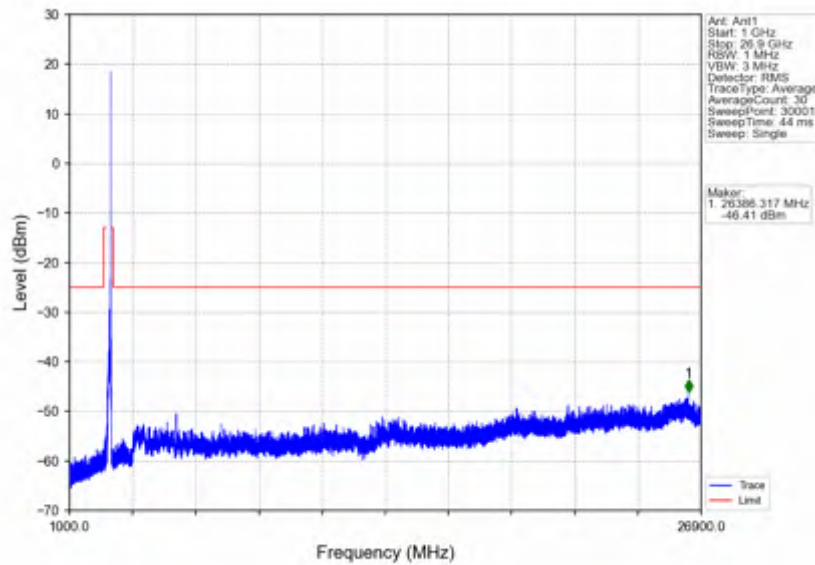
n41_30kHz_SISO_NTNV_100MHz_CP-OFDM QPSK_2640MHz_Inner_1RB_Right
