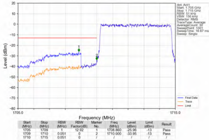
n66_15kHz_SISO_NTNV_5MHz_DFT-s-OFDM QPSK_1712.5MHz_Outer_Full
