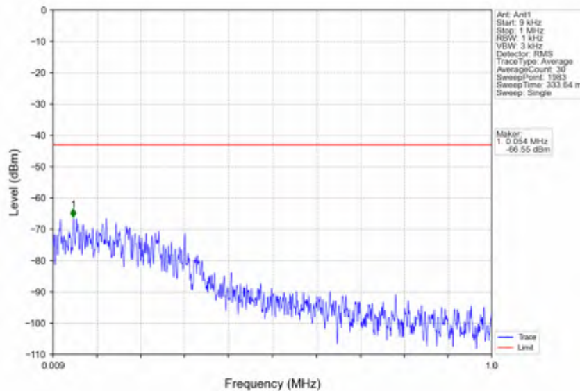
n41_30kHz_SISO_NTNV_100MHz_CP-OFDM QPSK_2640MHz_Edge_1RB_Right
