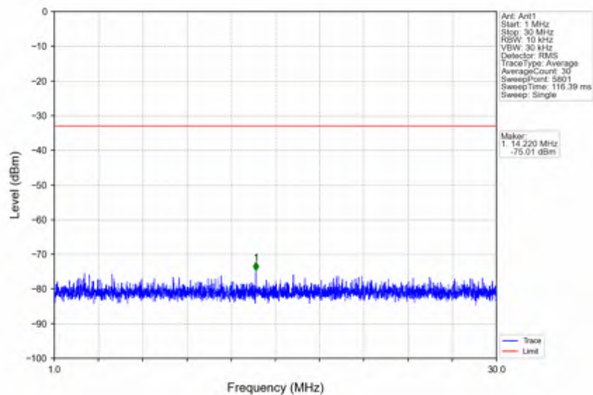
n66_15kHz_SISO_NTNV_10MHz_CP-OFDM QPSK_1715MHz_Outer_Full
