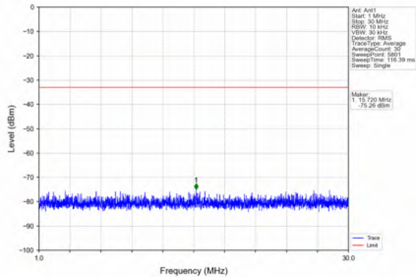
n66_15kHz_SISO_NTNV_5MHz_CP-OFDM QPSK_1712.5MHz_Edge_1RB_Left
