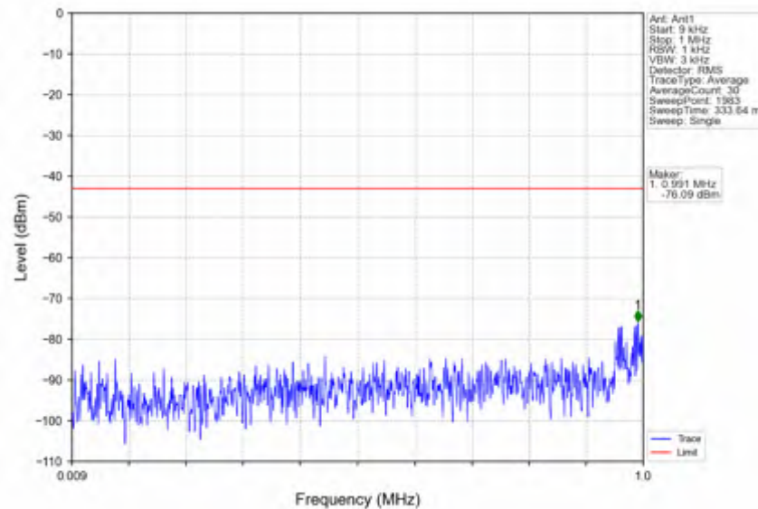
n66_15kHz_SISO_NTNV_10MHz_DFT-s-OFDM QPSK_1715MHz_Outer_Full
