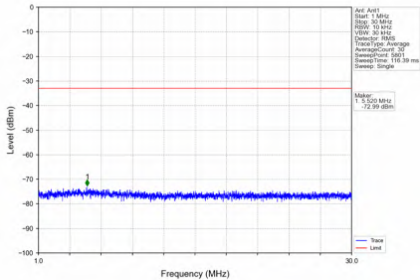
n41_30kHz_SISO_NTNV_100MHz_DFT-s-OFDM PI/2 BPSK_2640MHz_Inner_1RB_Right
