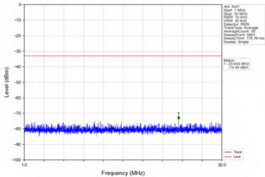
n66_15kHz_SISO_NTNV_10MHz_CP-OFDM QPSK_1775MHz_Edge_1RB_Right
