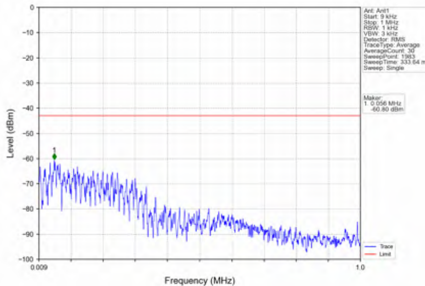
n41_30kHz_SISO_NTV_90MHz_CP-OFDM QPSK_2644.98MHz_Inner_1RB_Right
