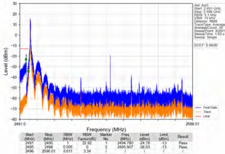
n41_30kHz_SISO_NTNV_100MHz_DFT-s-OFDM PI/2 BPSK_2546.01MHz_Inner_1RB_Left
