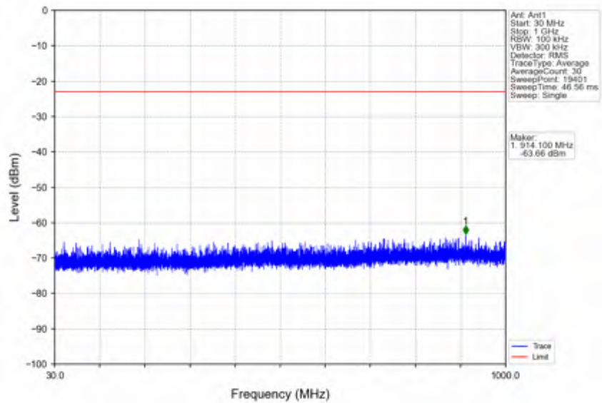
n66_15kHz_SISO_NTNV_10MHz_DFT-s-OFDM QPSK_1715MHz_Edge_1RB_Left
