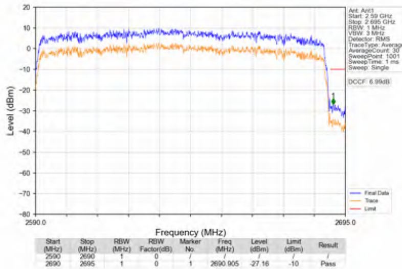
n41_30kHz_SISO_NTNV_100MHz_DFT-s-OFDM QPSK_2640MHz_Outer_Full
