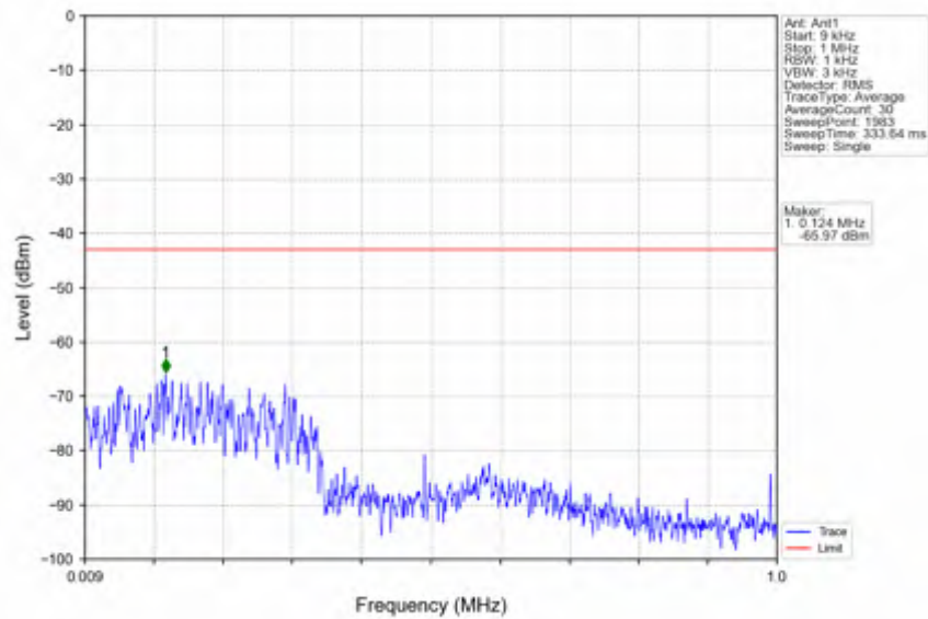
n41_30kHz_SISO_NTNV_100MHz_DFT-s-OFDM QPSK_2546.01MHz_Inner_1RB_Left
