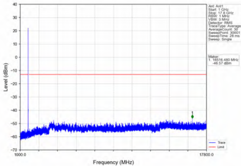
n66_15kHz_SISO_NTNV_5MHz_DFT-s-OFDM PI/2 BPSK_1712.5MHz_Outer_Full
