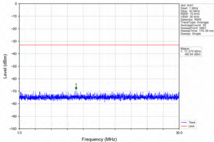
n41_30kHz_SISO_NTNV_100MHz_DFT-s-OFDM QPSK_2640MHz_Edge_1RB_Right
