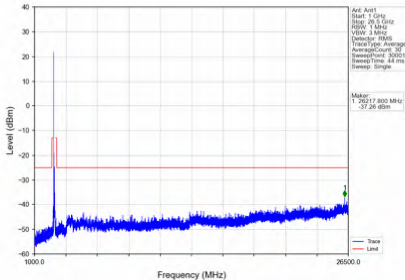
n41_30kHz_SISO_NTNV_100MHz_DFT-s-OFDM PI/2 BPSK_2592.99MHz_Edge_1RB_Left
