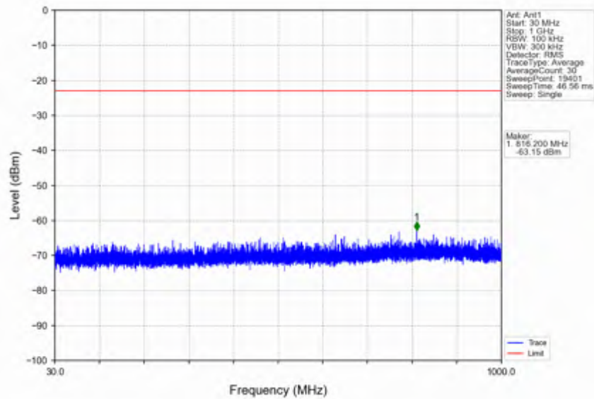
n66_15kHz_SISO_NTNV_5MHz_DFT-s-OFDM QPSK_1712.5MHz_Edge_1RB_Left
