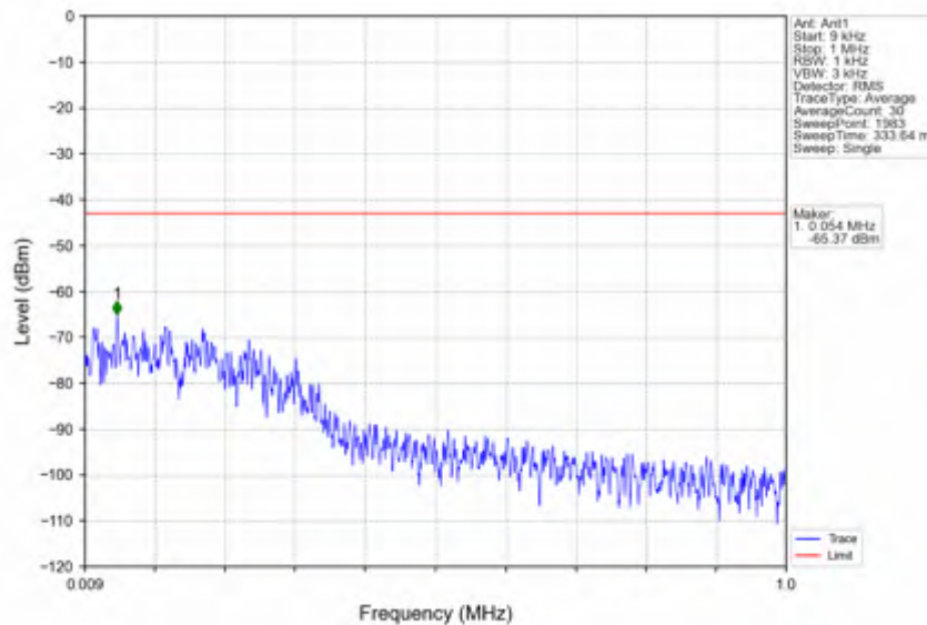
n41_30kHz_SISO_NTV_100MHz_CP-OFDM QPSK_2546.01MHz_Edge_1RB_Left
