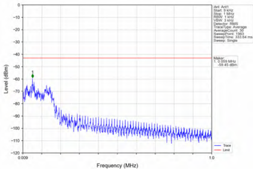
n66_15kHz_SISO_NTNV_10MHz_DFT-s-OFDM_PI/2_BPSK_1715MHz_Edge_1RB_Left
