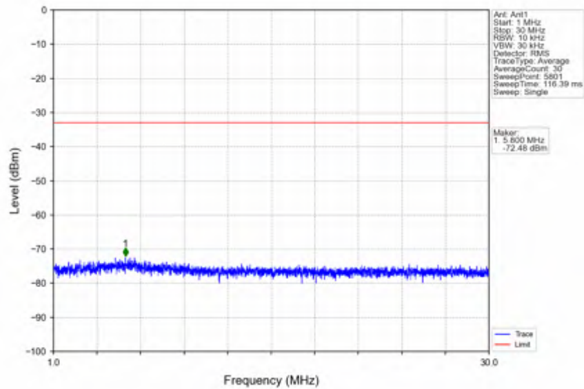
n41_30kHz_SISO_NTNV_90MHz_CP-OFDM QPSK_2644.98MHz_Inner_1RB_Right
