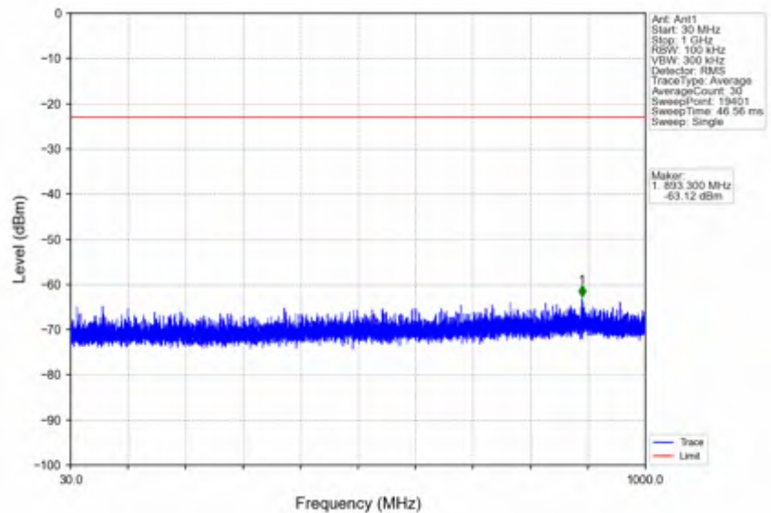
n66_15kHz_SISO_NTNV_10MHz_DFT-s-OFDM QPSK_1745MHz_Edge_1RB_Left
