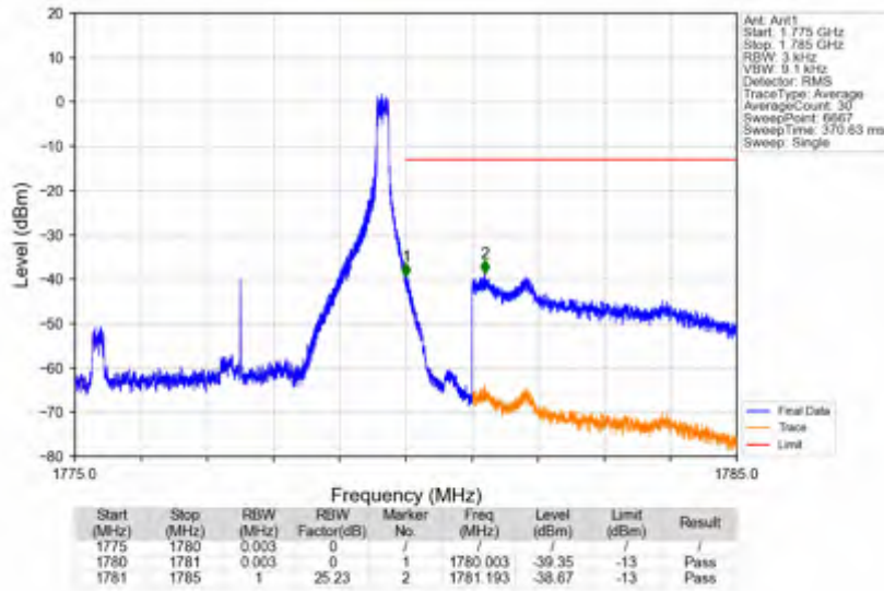
n66_15kHz_SISO_NTNV_5MHz_CP-OFDM QPSK_1777.5MHz_Edge_1RB_Right
