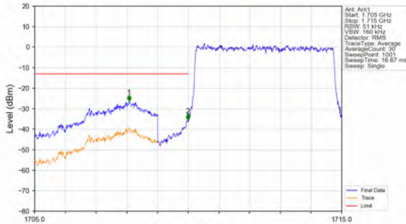
n66_15kHz_SISO_NTNV_5MHz_DFT-s-OFDM PI/2 BPSK_1712.5MHz_Outer_Full
