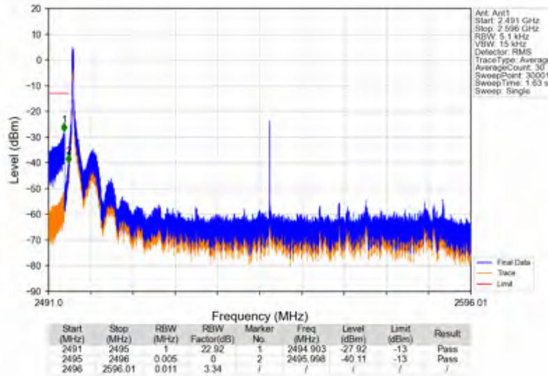
n41_30kHz_SISO_NTV_100MHz_CP-OFDM QPSK_2546.01MHz_Edge_1RB_Left
