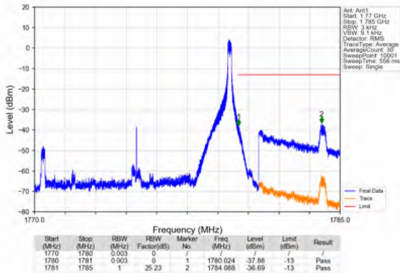
n66_15kHz_SISO_NTNV_10MHz_DFT-s-OFDM QPSK_1775MHz_Edge_1RB_Right
