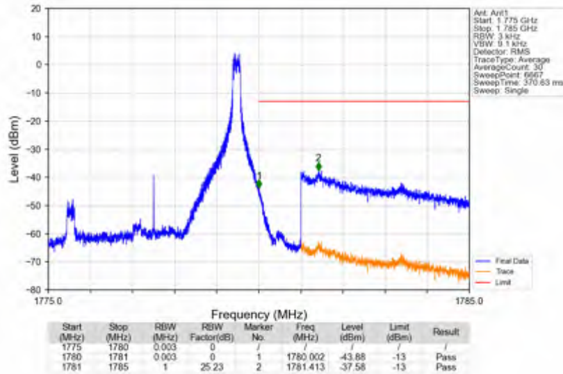
n66_15kHz_SISO_NTNV_5MHz_CP-OFDM QPSK_1777.5MHz_Inner_1RB_Right
