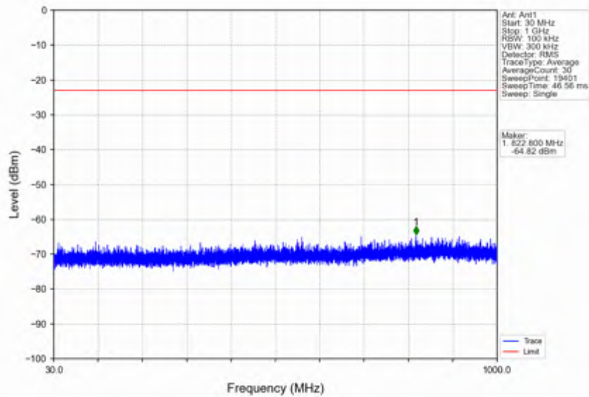
n66_15kHz_SISO_NTNV_5MHz_CP-OFDM QPSK_1777.5MHz_Outer_Full
