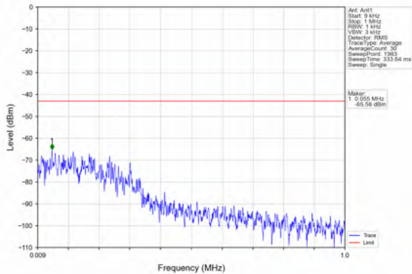
n41_30kHz_SISO_NTV_100MHz_CP-OFDM QPSK_2592.99MHz_Edge_1RB_Left
