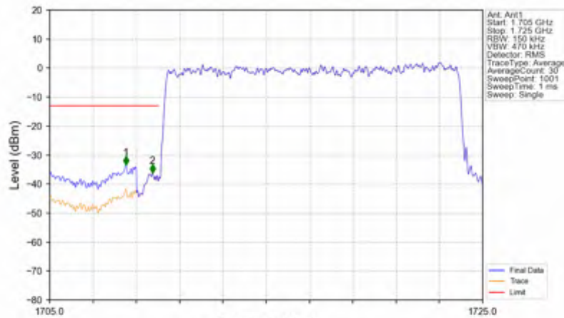
n66_15kHz_SISO_NTNV_15MHz_DFT-s-OFDM PI/2 BPSK_1717.5MHz_Outer_Full
