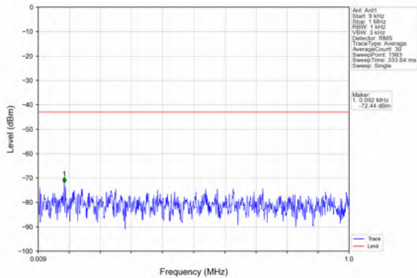
n66_15kHz_SISO_NTNV_5MHz_CP-OFDM QPSK_1712.5MHz_Outer_Full
