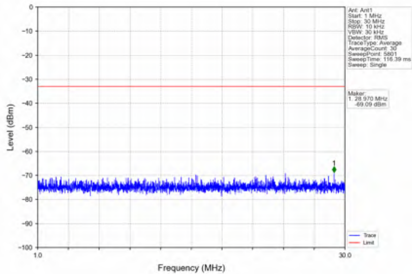
n41_30kHz_SISO_NTNV_90MHz_CP-OFDM QPSK_2644.98MHz_Edge_1RB_Right
