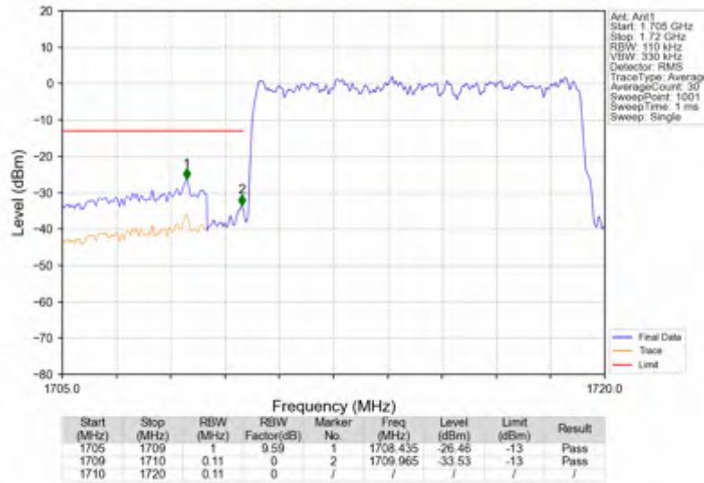
n66_15kHz_SISO_NTNV_10MHz_DFT-s-OFDM QPSK_1715MHz_Outer_Full
