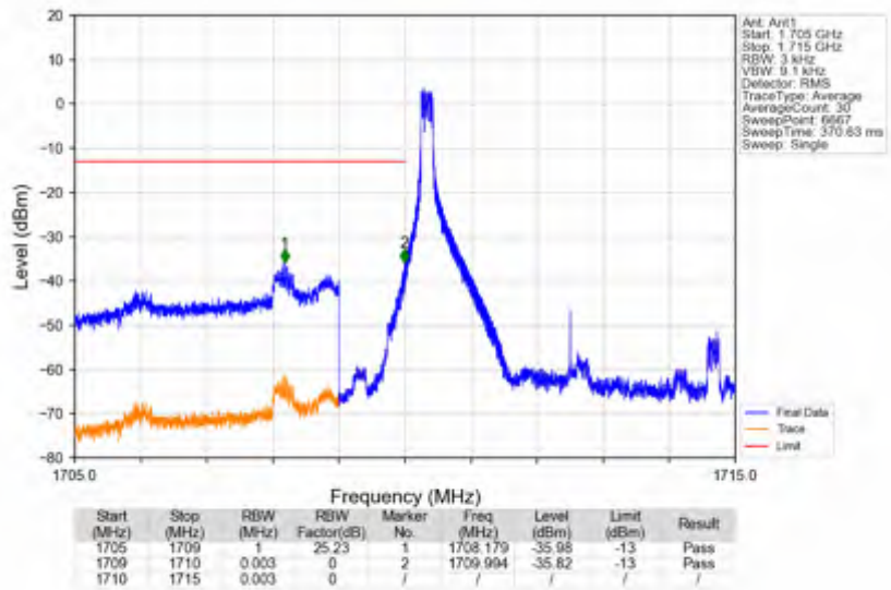
n66_15kHz_SISO_NTNV_5MHz_DFT-s-OFDM QPSK_1712.5MHz_Edge_1RB_Left
