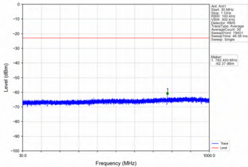
n41_30kHz_SISO_NTNV_100MHz_DFT-s-OFDM_QPSK_2546.01MHz_Inner_1RB_Left
