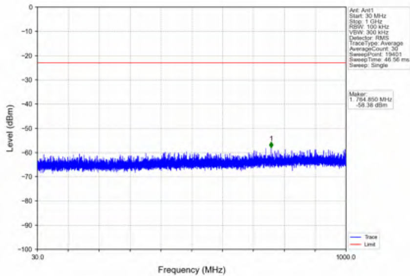
n41_30kHz_SISO_NTNV_90MHz_CP-OFDM QPSK_2592.99MHz_Edge_1RB_Left
