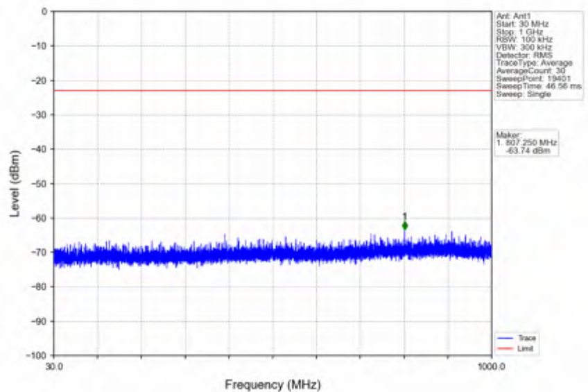
n66_15kHz_SISO_NTNV_5MHz_DFT-s-OFDM QPSK_1712.5MHz_Outer_Full
