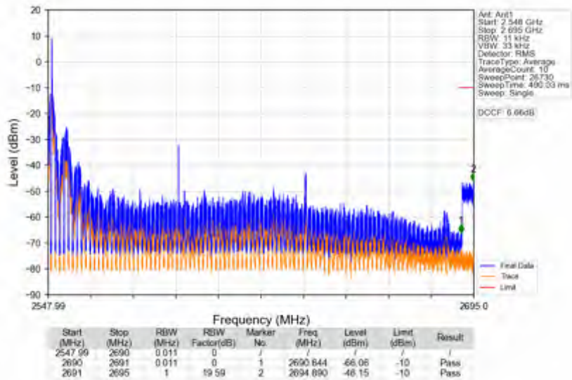
n41_30kHz_SISO_NTNV_90MHz_CP-OFDM QPSK_2592.99MHz_Edge_1RB_Left
