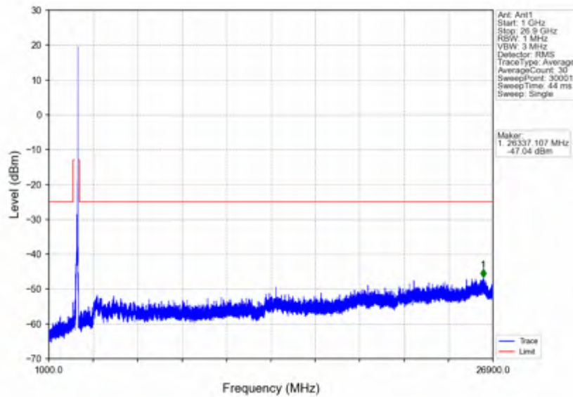
n41_30kHz_SISO_NTV_90MHz_CP-OFDM QPSK_2644.98MHz_Outer_Full
