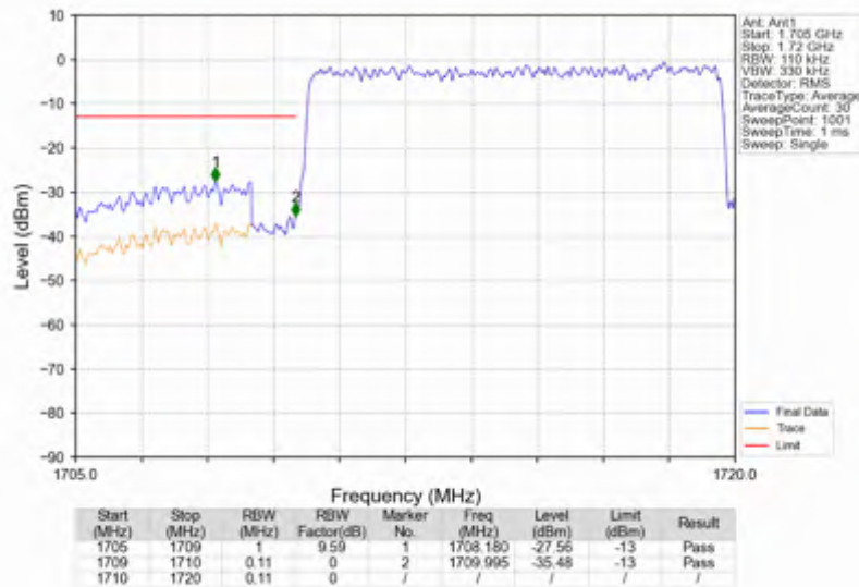
n66_15kHz_SISO_NTNV_10MHz_CP-OFDM QPSK_1715MHz_Outer_Full
