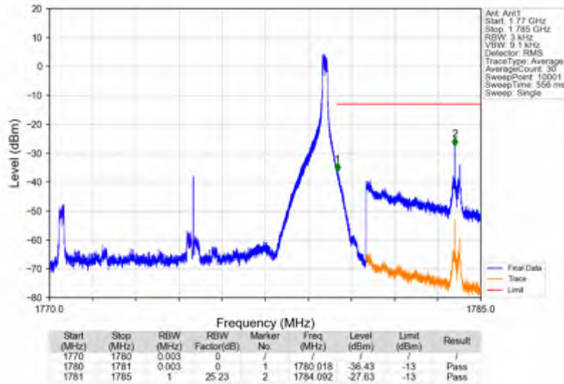
n66_15kHz_SISO_NTNV_10MHz_DFT-s-OFDM PI/2 BPSK_1775MHz_Edge_1RB_Right
