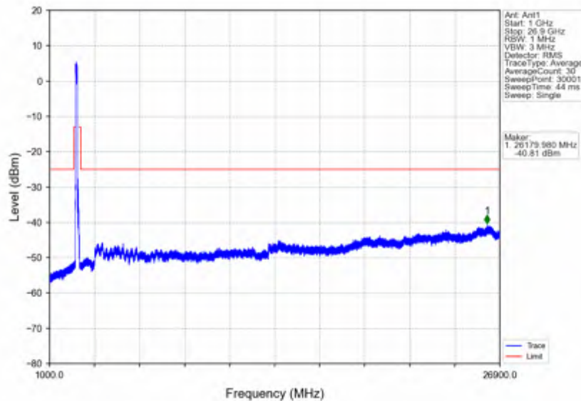
n41_30kHz_SISO_NTNV_100MHz_DFT-s-OFDM PI/2 BPSK_2546.01MHz_Outer_Full
