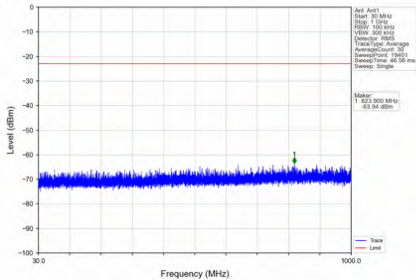
n66_15kHz_SISO_NTNV_5MHz_CP-OFDM QPSK_1745MHz_Edge_1RB_Left
