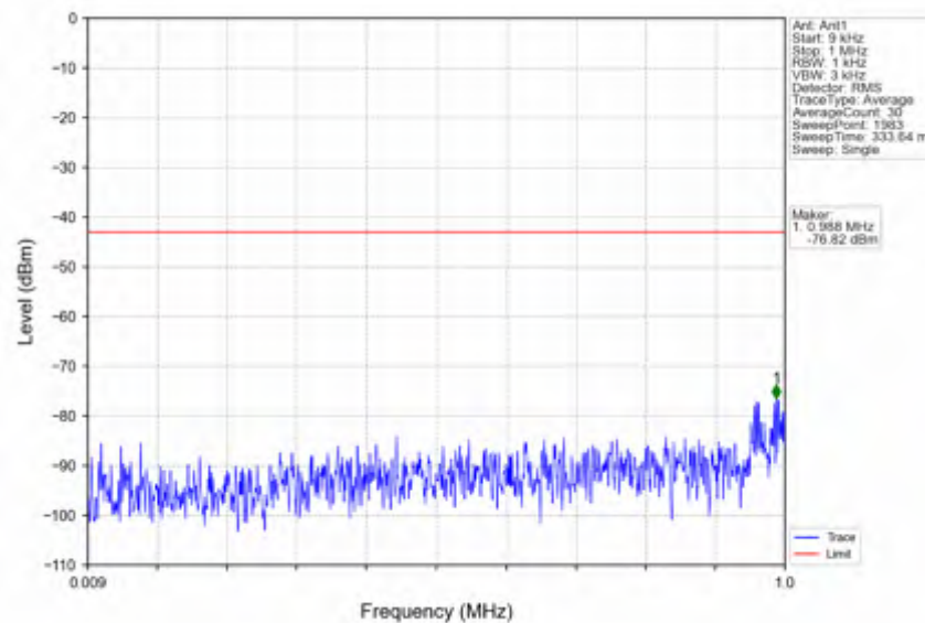
n66_15kHz_SISO_NTNV_10MHz_DFT-s-OFDM QPSK_1775MHz_Outer_Full
