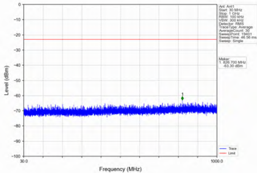
n66_15kHz_SISO_NTNV_10MHz_DFT-s-OFDM QPSK_1775MHz_Edge_1RB_Right
