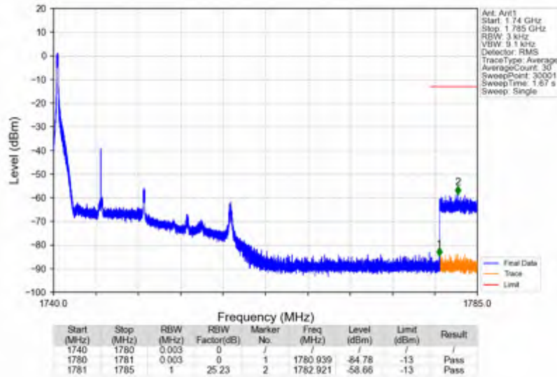
n66_15kHz_SISO_NTNV_10MHz_CP-OFDM QPSK_1745MHz_Edge_1RB_Left
