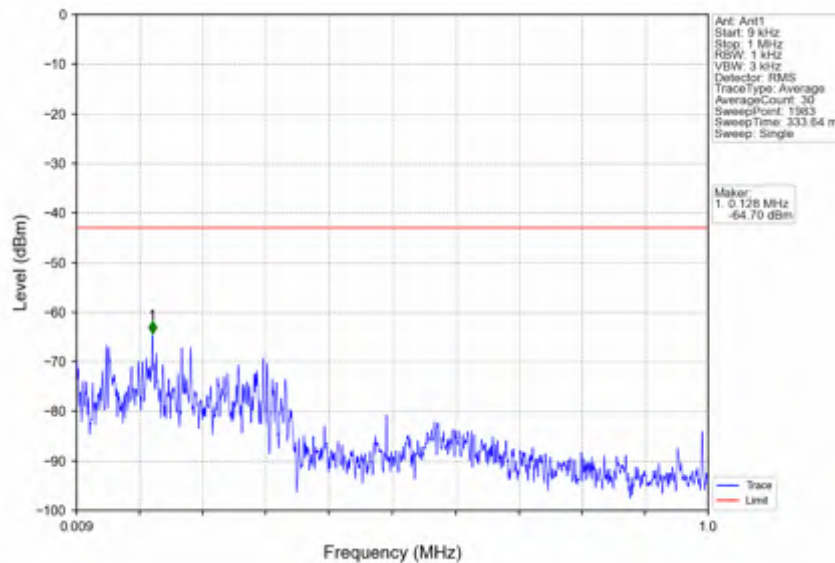
n41_30kHz_SISO_NTNV_100MHz_DFT-s-OFDM PI/2 BPSK_2546.01MHz_Inner_1RB_Left
