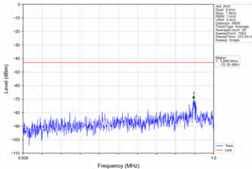
n66_15kHz_SISO_NTNV_5MHz_DFT-s-OFDM QPSK_1777.5MHz_Outer_Full
