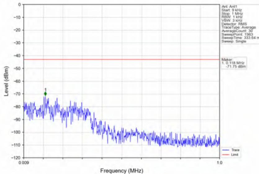
n41_30kHz_SISO_NTV_100MHz_DFT-s-OFDM PI/2 BPSK_2640MHz_Edge_1RB_Right
