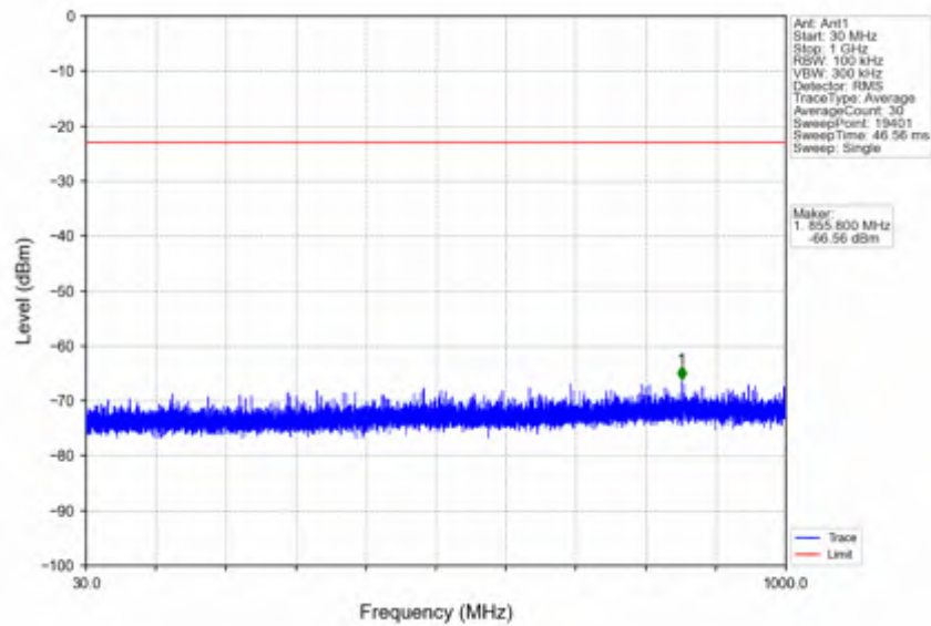
n41_30kHz_SISO_NTNV_60MHz_CP-OFDM QPSK_2526MHz_Outer_Full
