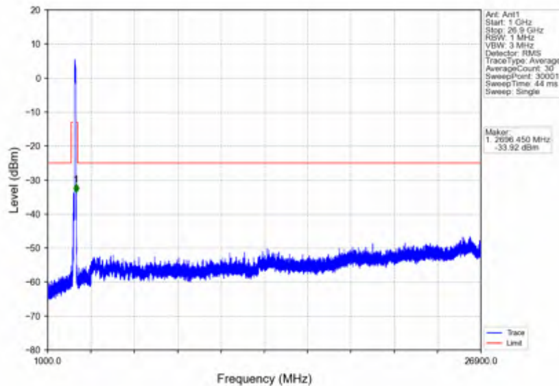
n41_30kHz_SISO_NTNV_90MHz_DFT-s-OFDM PI/2 BPSK_2644.98MHz_Outer_Full
