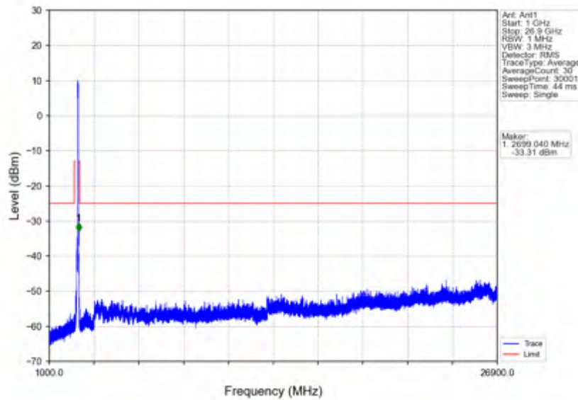
n41_30kHz_SISO_NTNV_60MHz_DFT-s-OFDM PI/2 BPSK_2659.98MHz_Outer_Full
