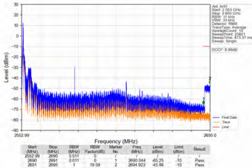
n41_30kHz_SISO_NTNV_80MHz_CP-OFDM QPSK_2592.99MHz_Edge_1RB_Left
