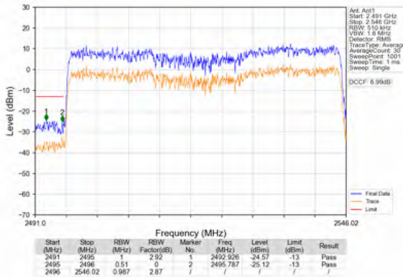
n41_30kHz_SISO_NTNV_50MHz_CP-OFDM QPSK_2521.02MHz_Outer_Full
