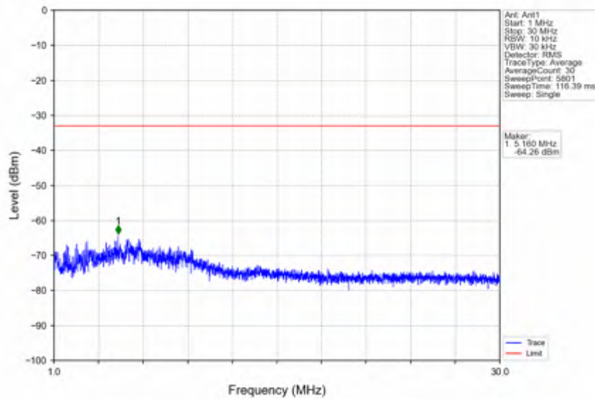
n41_30kHz_SISO_NTNV_80MHz_DFT-s-OFDM PI/2 BPSK_2649.99MHz_Inner_1RB_Right
