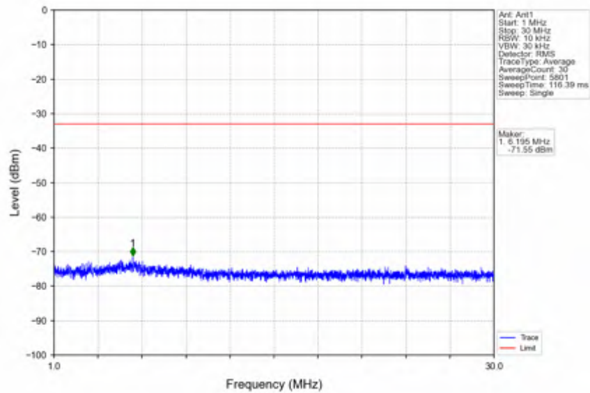
n41_30kHz_SISO_NTNV_90MHz_DFT-s-OFDM QPSK_2644.98MHz_Outer_Full
