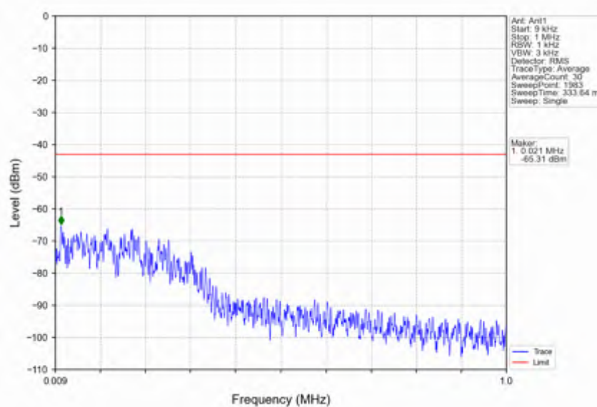
n41_30kHz_SISO_NTNV_50MHz_CP-OFDM QPSK_2521.02MHz_Edge_1RB_Left
