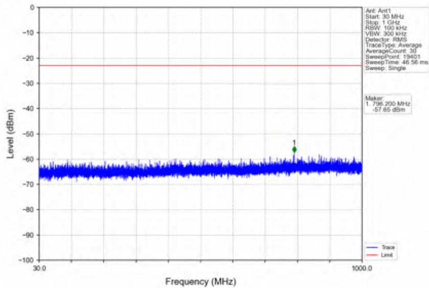
n41_30kHz_SISO_NTV_90MHz_DFT-s-OFDM QPSK_2644.98MHz_Edge_1RB_Right
