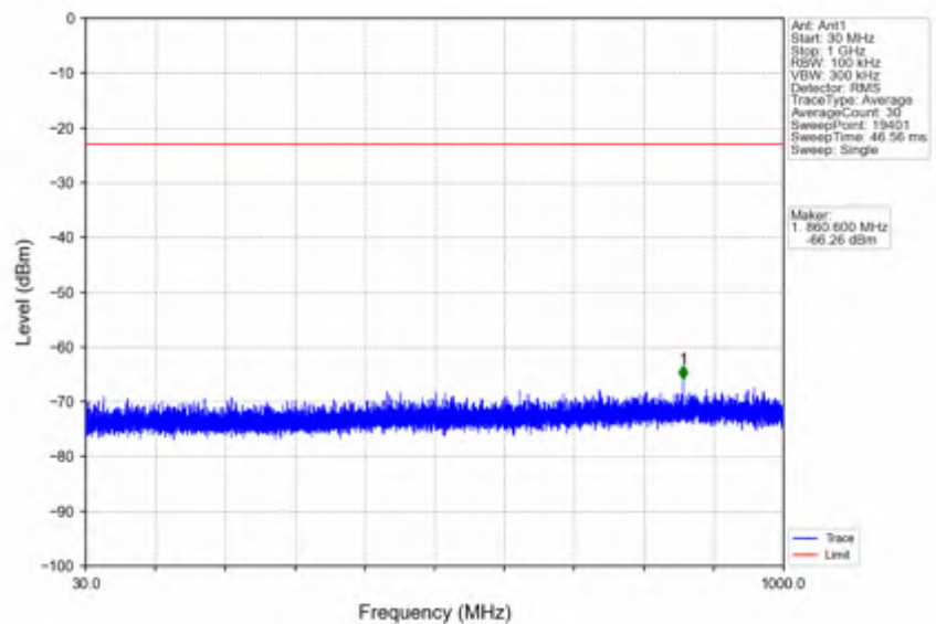
n41_30kHz_SISO_NTNV_50MHz_DFT-s-OFDM QPSK_2664.99MHz_Outer_Full
