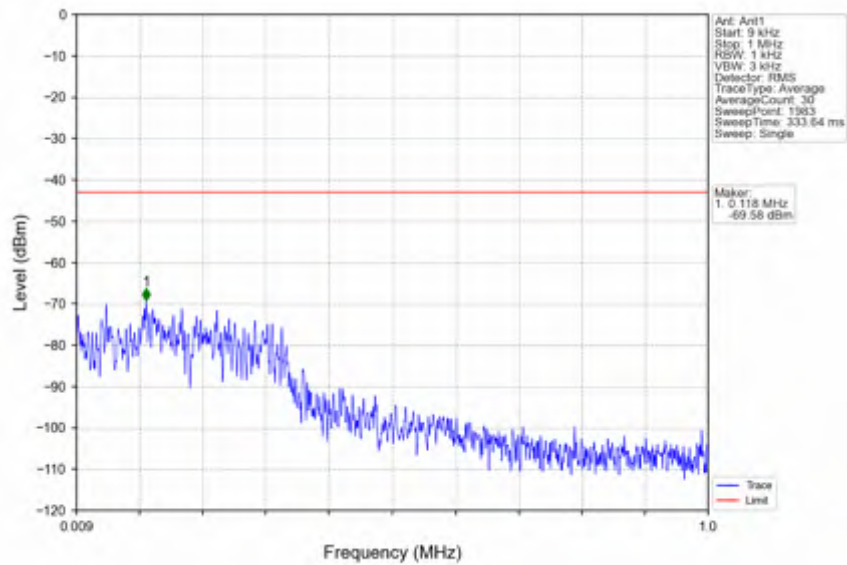
n41_30kHz_SISO_NTV_50MHz_DFT-s-OFDM_QPSK_2664.99MHz_Edge_1RB_Right
