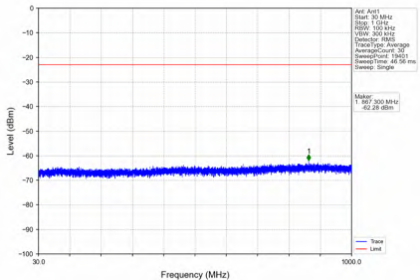
n41_30kHz_SISO_NTNV_80MHz_DFT-s-OFDM QPSK_2649.99MHz_Outer_Full
