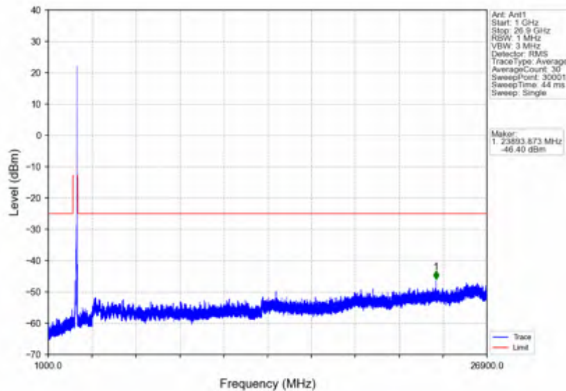
n41_30kHz_SISO_NTV_50MHz_DFT-s-OFDM QPSK_2664.99MHz_Edge_1RB_Right
