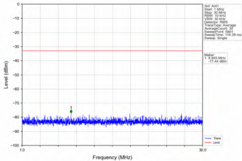
n41_30kHz_SISO_NTNV_50MHz_DFT-s-OFDM QPSK_2521.02MHz_Outer_Full
