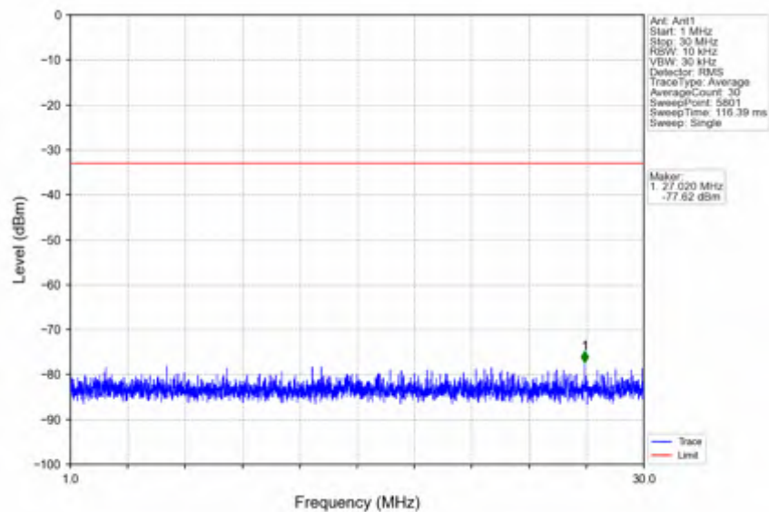
n41_30kHz_SISO_NTNV_60MHz_DFT-s-OFDM PI/2 BPSK_2659.98MHz_Outer_Full
