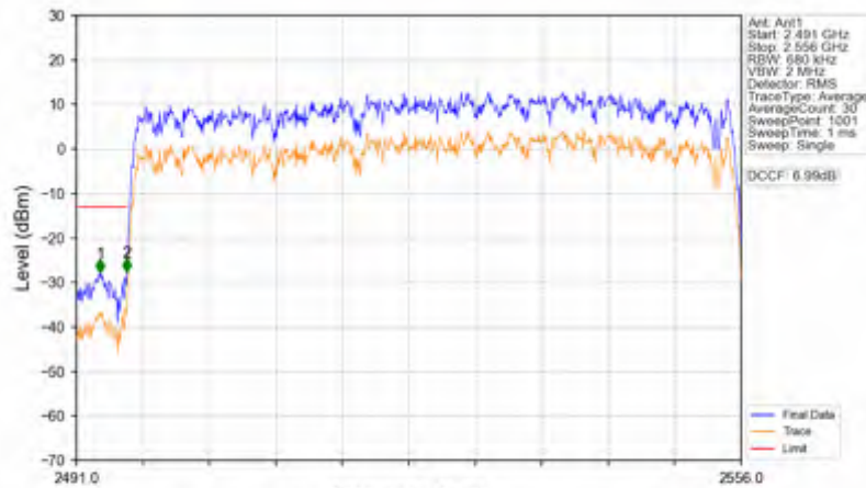
n41_30kHz_SISO_NTNV_60MHz_DFT-s-OFDM PI/2 BPSK_2526MHz_Outer_Full
