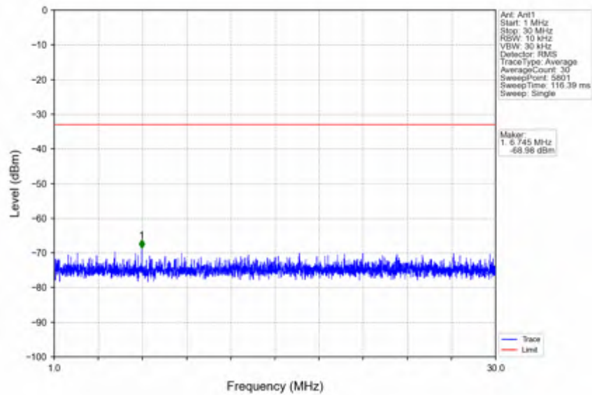
n41_30kHz_SISO_NTNV_90MHz_DFT-s-OFDM QPSK_2592.99MHz_Edge_1RB_Left
