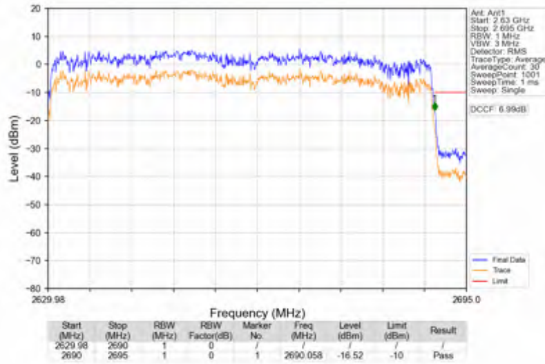
n41_30kHz_SISO_NTNV_60MHz_DFT-s-OFDM QPSK_2659.98MHz_Outer_Full
