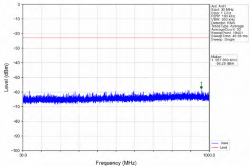
n41_30kHz_SISO_NTNV_80MHz_DFT-s-OFDM QPSK_2592.99MHz_Edge_1RB_Left
