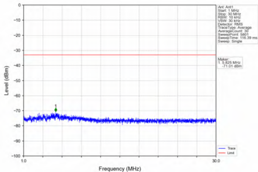
n41_30kHz_SISO_NTNV_90MHz_DFT-s-OFDM PI/2 BPSK_2644.98MHz_Outer_Full
