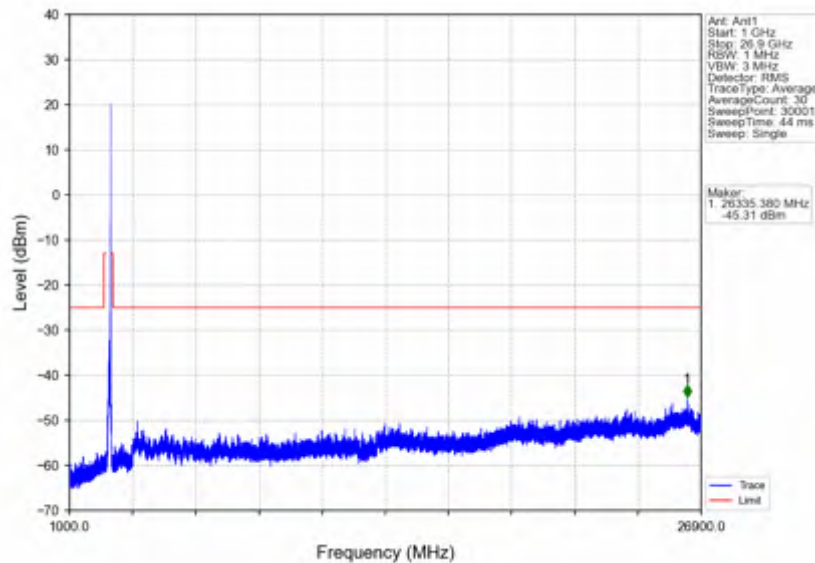
n41_30kHz_SISO_NTV_90MHz_DFT-s-OFDM QPSK_2644.98MHz_Edge_1RB_Right
