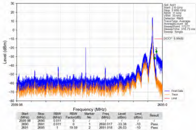
n41_30kHz_SISO_NTNV_90MHz_DFT-s-OFDM QPSK_2644.98MHz_Inner_1RB_Right
