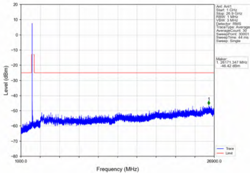
n41_30kHz_SISO_NTNV_80MHz_DFT-s-OFDM PI/2 BPSK_2592.99MHz_Edge_1RB_Left
