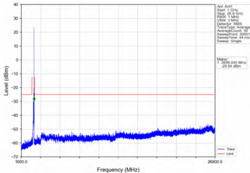
n41_30kHz_SISO_NTV_80MHz_DFT-s-OFDM_QPSK_2649.99MHz_Inner_1RB_Right
