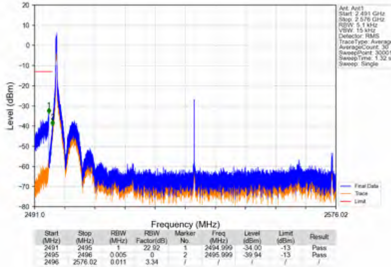
n41_30kHz_SISO_NTNV_80MHz_CP-OFDM QPSK_2536.02MHz_Edge_1RB_Left
