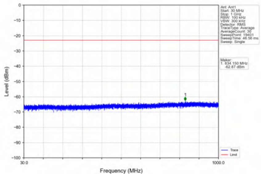
n41_30kHz_SISO_NTNV_60MHz_DFT-s-OFDM QPSK_2659.98MHz_Outer_Full
