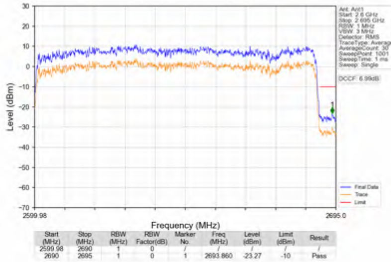
n41_30kHz_SISO_NTNV_90MHz_DFT-s-OFDM QPSK_2644.98MHz_Outer_Full
