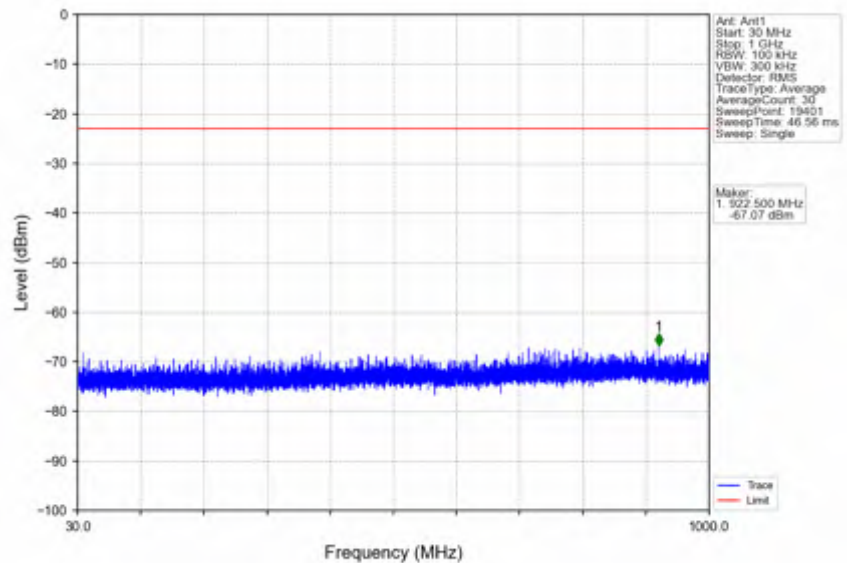
n41_30kHz_SISO_NTV_50MHz_CP-OFDM QPSK_2664.99MHz_Inner_1RB_Right
