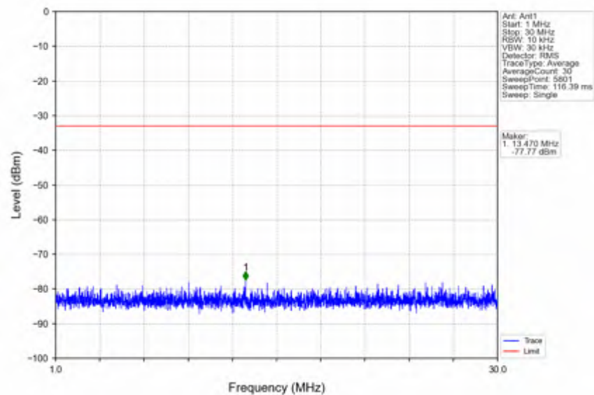
n41_30kHz_SISO_NTNV_50MHz_CP-OFDM QPSK_2521.02MHz_Outer_Full
