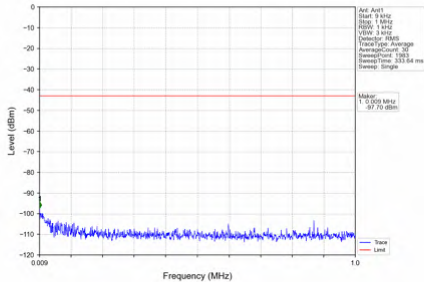
n41_30kHz_SISO_NTNV_50MHz_CP-OFDM QPSK_2664.99MHz_Outer_Full
