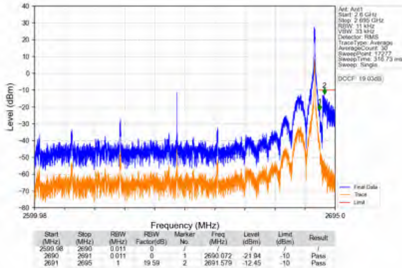
n41_30kHz_SISO_NTNV_90MHz_DFT-s-OFDM PI/2 BPSK_2644.98MHz_Inner_1RB_Right
