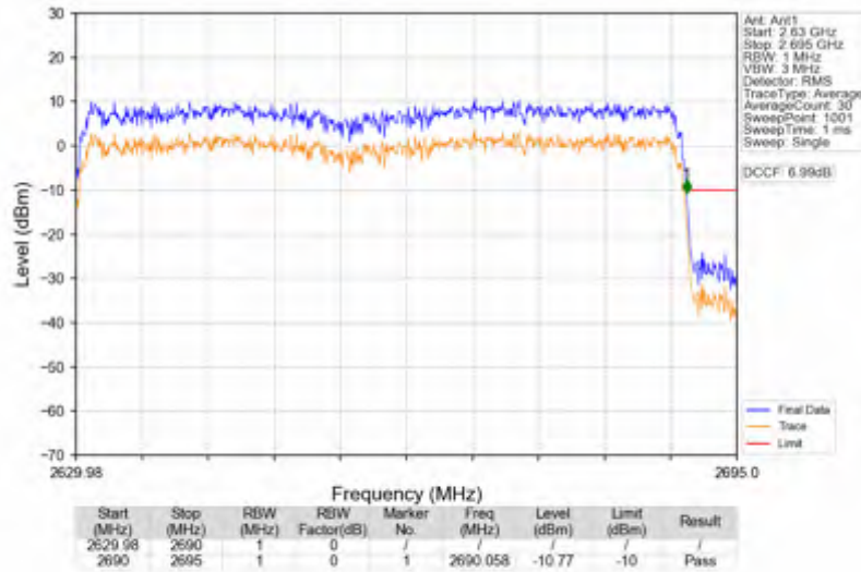
n41_30kHz_SISO_NTV_60MHz_CP-OFDM QPSK_2659.98MHz_Outer_Full
