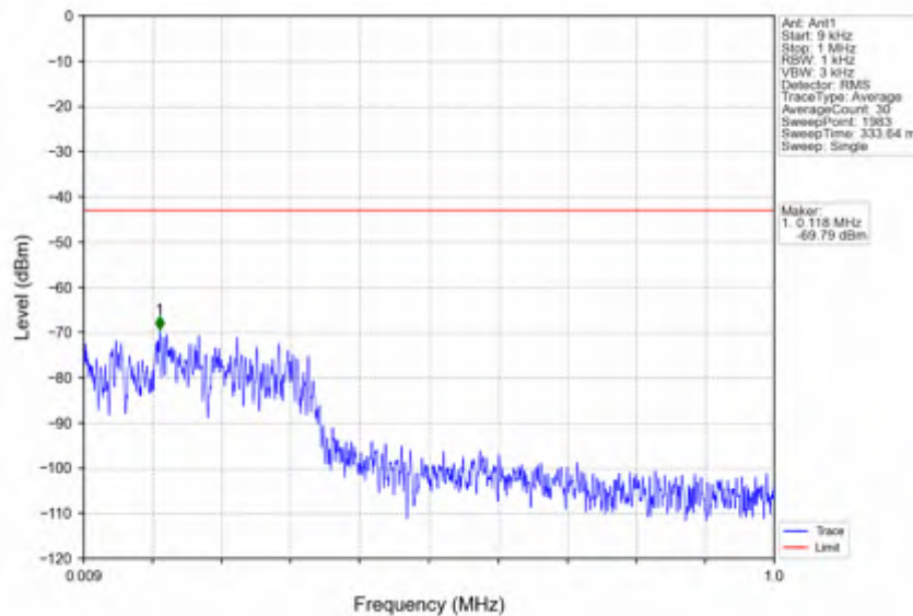
n41_30kHz_SISO_NTNV_50MHz_DFT-s-OFDM QPSK_2592.99MHz_Edge_1RB_Left
