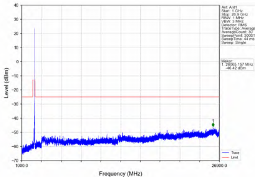
n41_30kHz_SISO_NTV_50MHz_DFT-s-OFDM QPSK_2664.99MHz_Inner_1RB_Right
