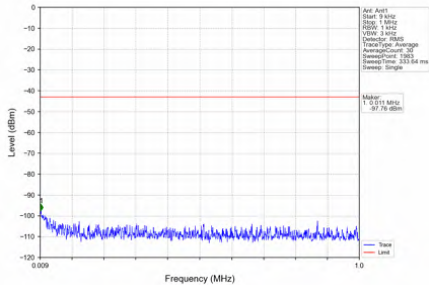
n41_30kHz_SISO_NTNV_80MHz_CP-OFDM QPSK_2536.02MHz_Outer_Full
