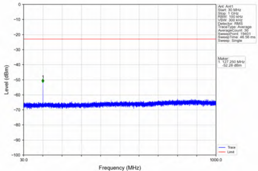
n41_30kHz_SISO_NTNV_80MHz_CP-OFDM QPSK_2649.99MHz_Inner_1RB_Right
