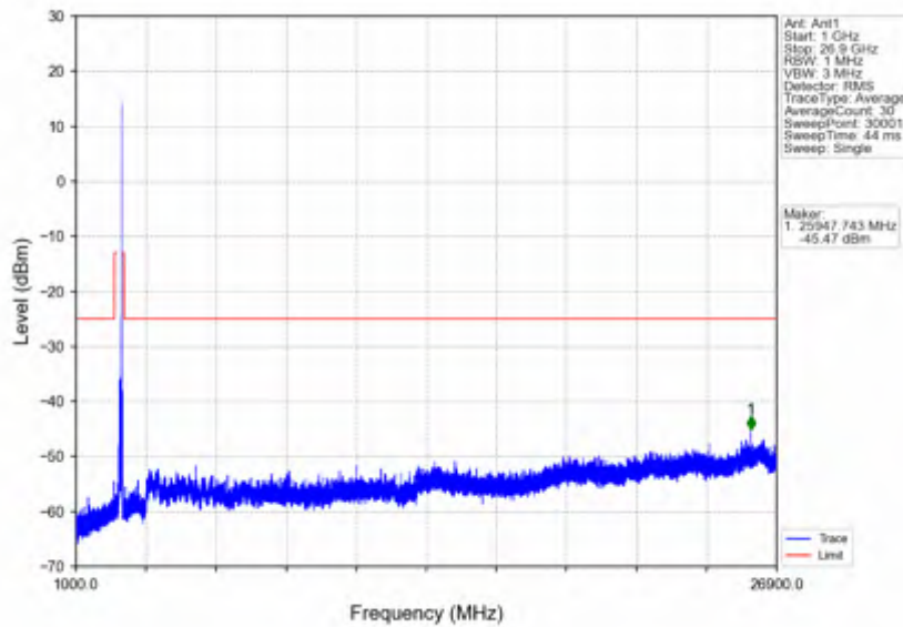
n41_30kHz_SISO_NTNV_80MHz_DFT-s-OFDM PI/2 BPSK_2649.99MHz_Outer_Full
