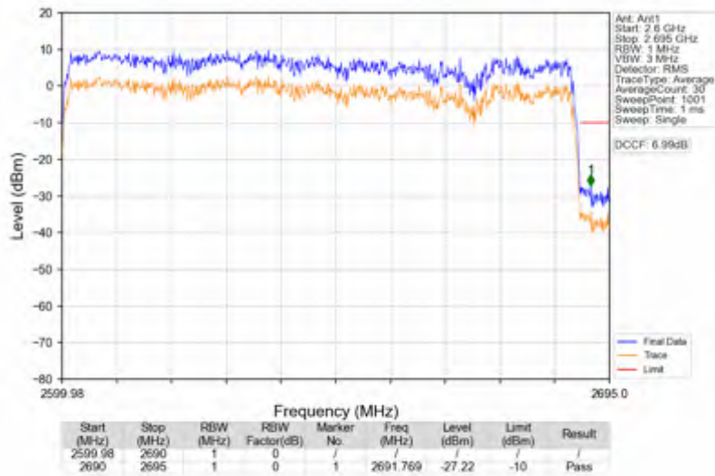
n41_30kHz_SISO_NTNV_90MHz_DFT-s-OFDM PI/2 BPSK_2644.98MHz_Outer_Full
