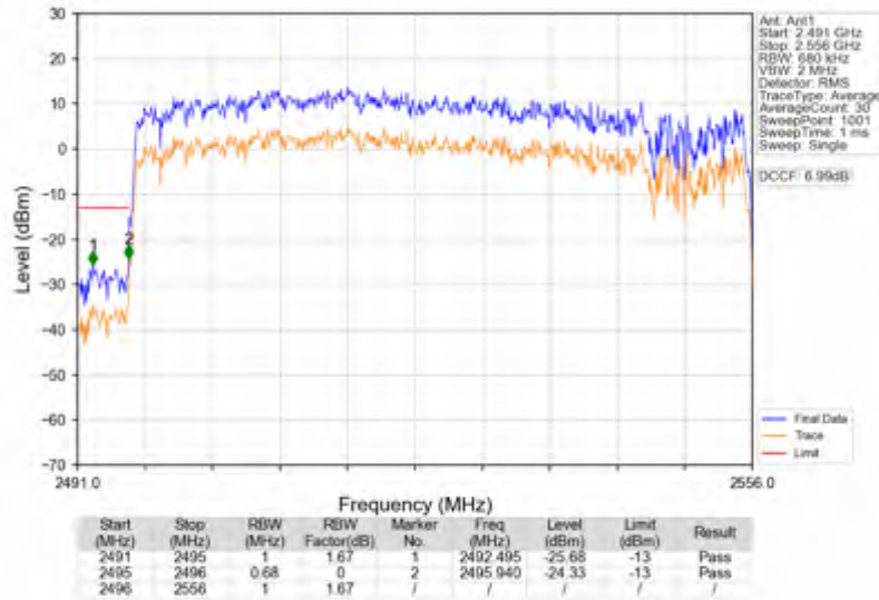
n41_30kHz_SISO_NTNV_60MHz_DFT-s-OFDM QPSK_2526MHz_Outer_Full
