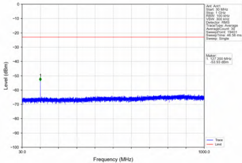
n41_30kHz_SISO_NTV_80MHz_DFT-s-OFDM_QPSK_2649.99MHz_Inner_1RB_Right
