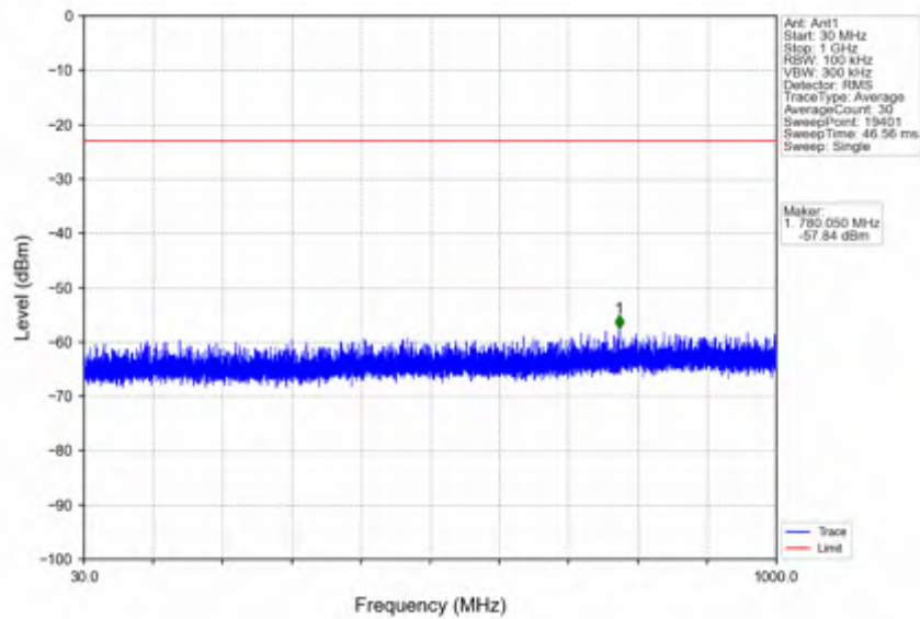
n41_30kHz_SISO_NTNV_50MHz_CP-OFDM QPSK_2592.99MHz_Edge_1RB_Left
