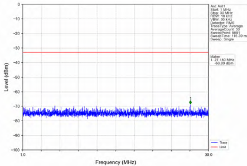
n41_30kHz_SISO_NTNV_80MHz_DFT-s-OFDM PI/2 BPSK_2536.02MHz_Edge_1RB_Left
