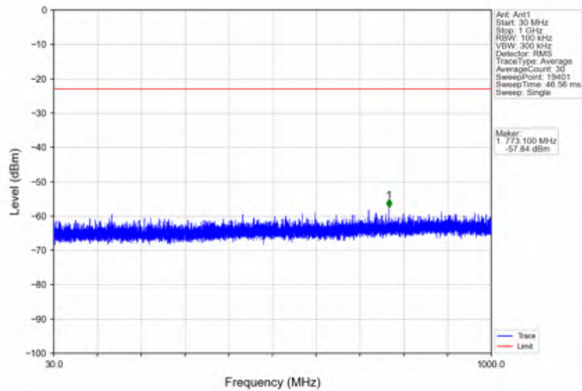
n41_30kHz_SISO_NTV_80MHz_DFT-s-OFDM QPSK_2649.99MHz_Edge_1RB_Right
