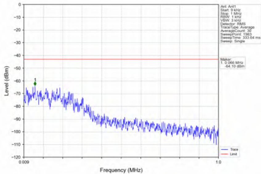
n41_30kHz_SISO_NTNV_80MHz_CP-OFDM QPSK_2592.99MHz_Edge_1RB_Left
