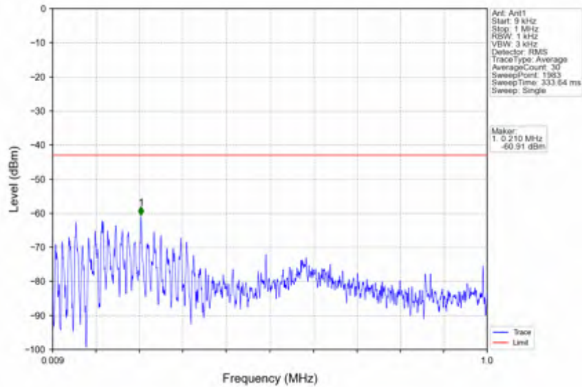
n41_30kHz_SISO_NTV_80MHz_DFT-s-OFDM QPSK_2649.99MHz_Inner_1RB_Right
