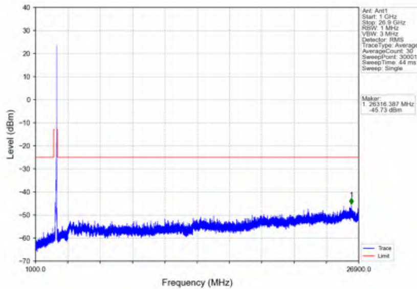
n41_30kHz_SISO_NTV_60MHz_CP-OFDM QPSK_2659.98MHz_Outer_Full
