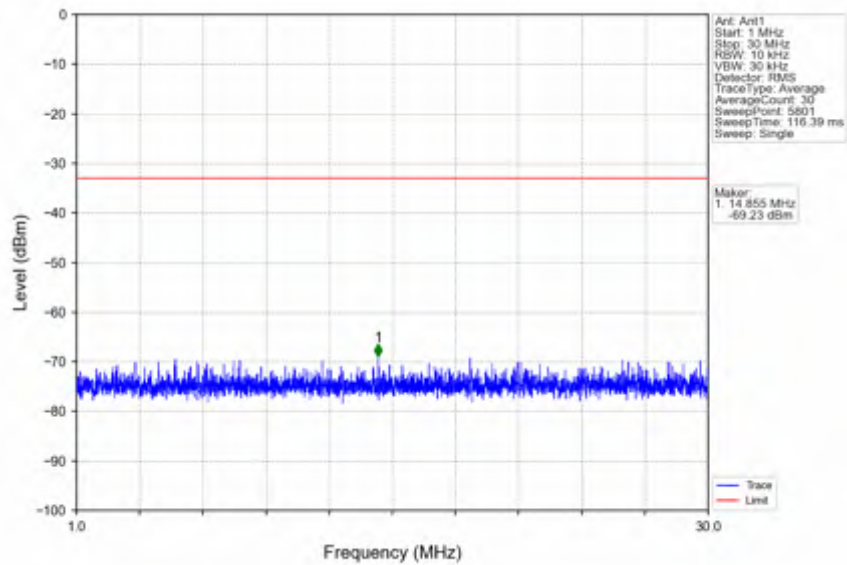
n41_30kHz_SISO_NTNV_80MHz_CP-OFDM QPSK_2536.02MHz_Edge_1RB_Left
