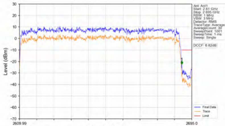
n41_30kHz_SISO_NTNV_80MHz_DFT-s-OFDM PI/2 BPSK_2649.99MHz_Outer_Full
