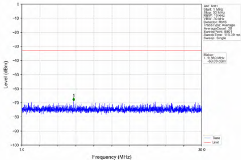
n41_30kHz_SISO_NTV_60MHz_DFT-s-OFDM_QPSK_2659.98MHz_Edge_1RB_Right
