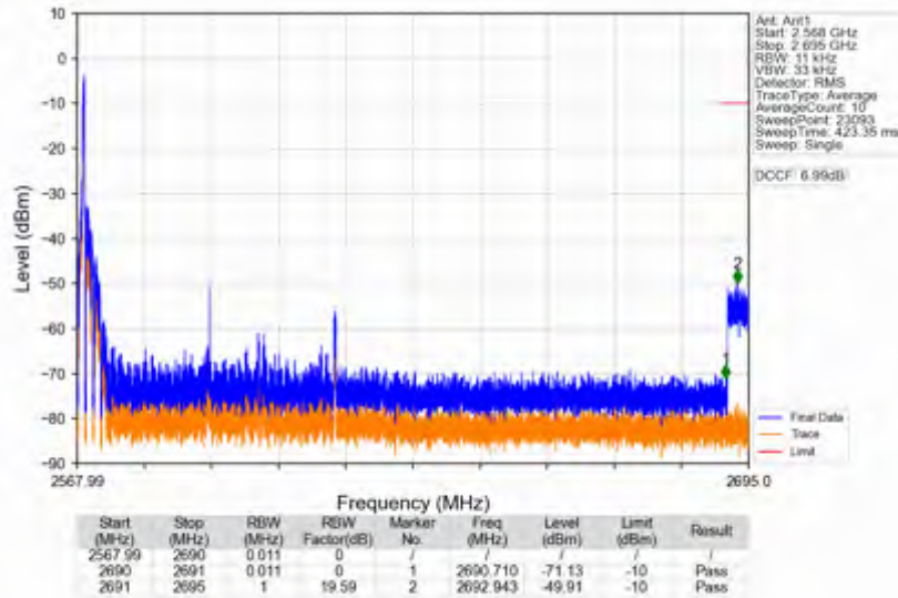
n41_30kHz_SISO_NTNV_50MHz_DFT-s-OFDM QPSK_2592.99MHz_Edge_1RB_Left
