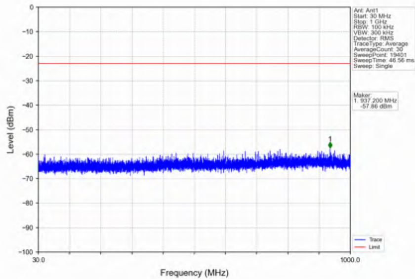
n41_30kHz_SISO_NTNV_80MHz_DFT-s-OFDM QPSK_2536.02MHz_Edge_1RB_Left
