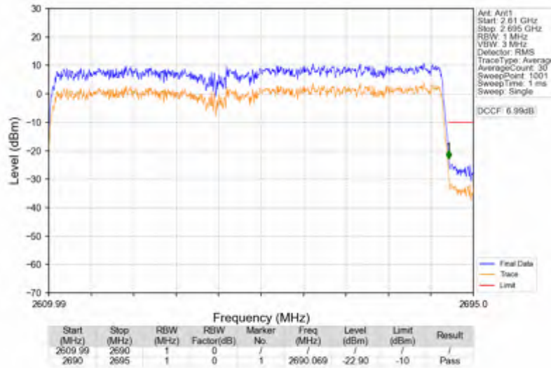
n41_30kHz_SISO_NTNV_80MHz_DFT-s-OFDM QPSK_2649.99MHz_Outer_Full
