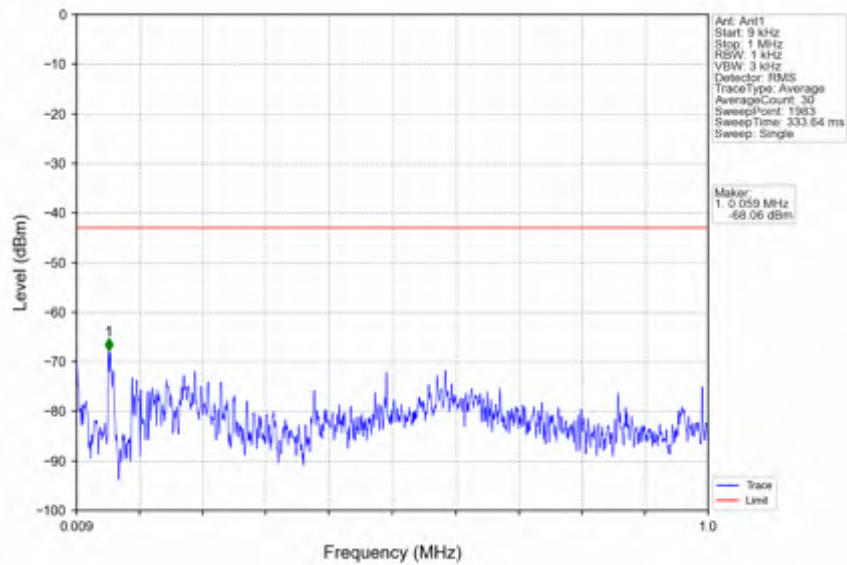
n41_30kHz_SISO_NTNV_80MHz_DFT-s-OFDM PI/2 BPSK_2649.99MHz_Outer_Full
