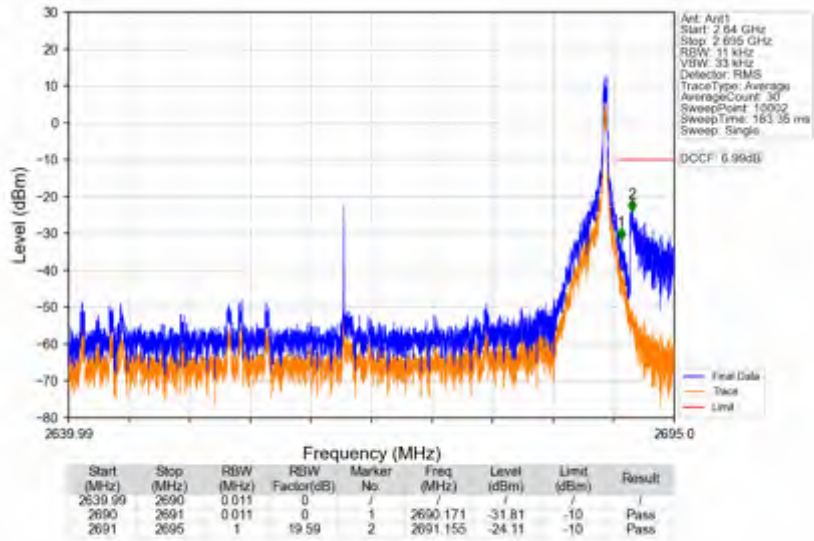
n41_30kHz_SISO_NTNV_50MHz_DFT-s-OFDM QPSK_2664.99MHz_Edge_1RB_Right
