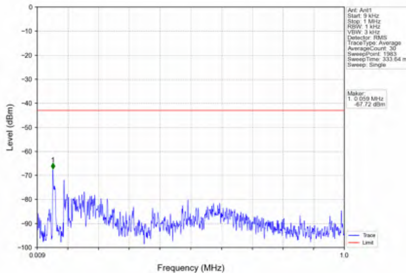
n41_30kHz_SISO_NTNV_90MHz_DFT-s-OFDM QPSK_2644.98MHz_Outer_Full
