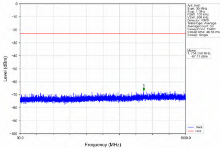
n41_30kHz_SISO_NTV_50MHz_DFT-s-OFDM QPSK_2664.99MHz_Inner_1RB_Right
