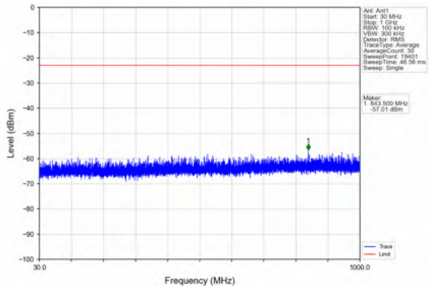
n41_30kHz_SISO_NTNV_50MHz_CP-OFDM QPSK_2521.02MHz_Edge_1RB_Left
