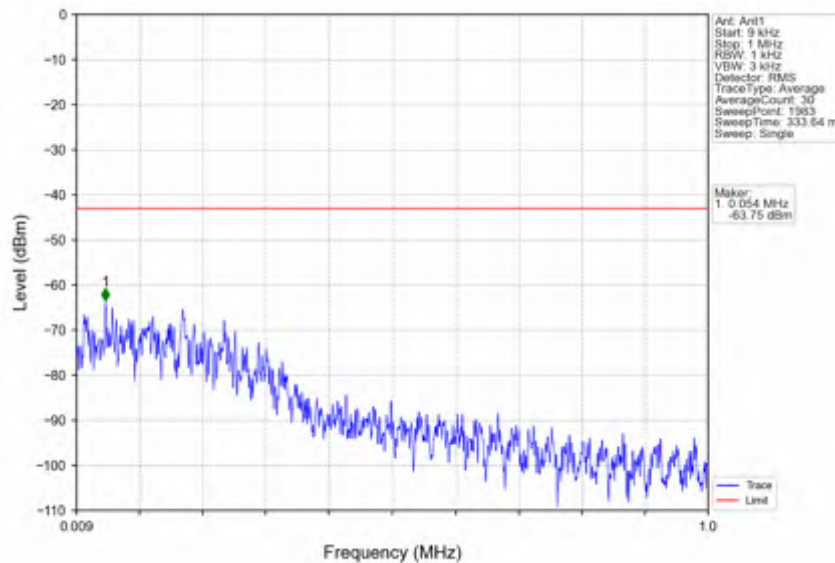
n41_30kHz_SISO_NTNV_80MHz_CP-OFDM QPSK_2649.99MHz_Edge_1RB_Right
