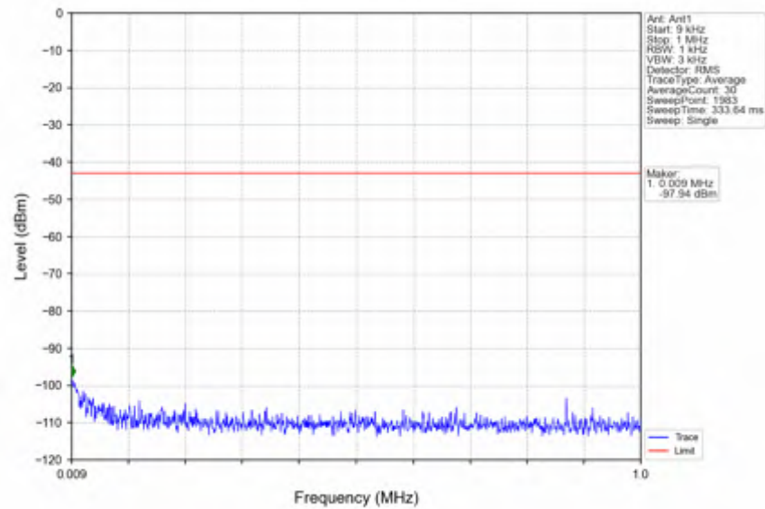
n41_30kHz_SISO_NTNV_60MHz_CP-OFDM QPSK_2659.98MHz_Outer_Full
