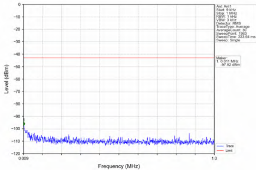
n41_30kHz_SISO_NTNV_60MHz_CP-OFDM QPSK_2526MHz_Outer_Full
