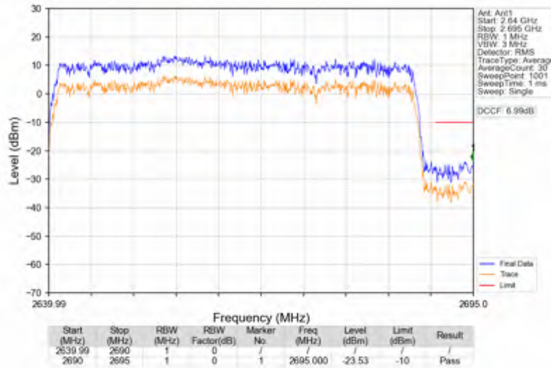
n41_30kHz_SISO_NTNV_50MHz_DFT-s-OFDM QPSK_2664.99MHz_Outer_Full
