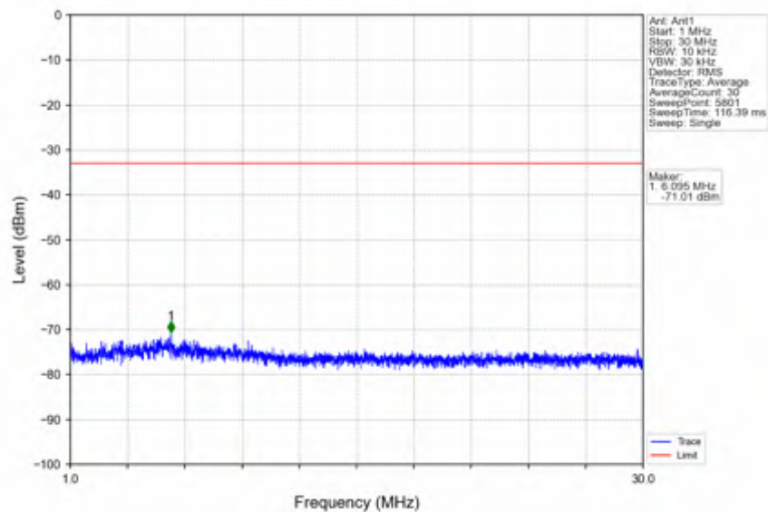
n41_30kHz_SISO_NTV_90MHz_DFT-s-OFDM_QPSK_2644.98MHz_Inner_1RB_Right
