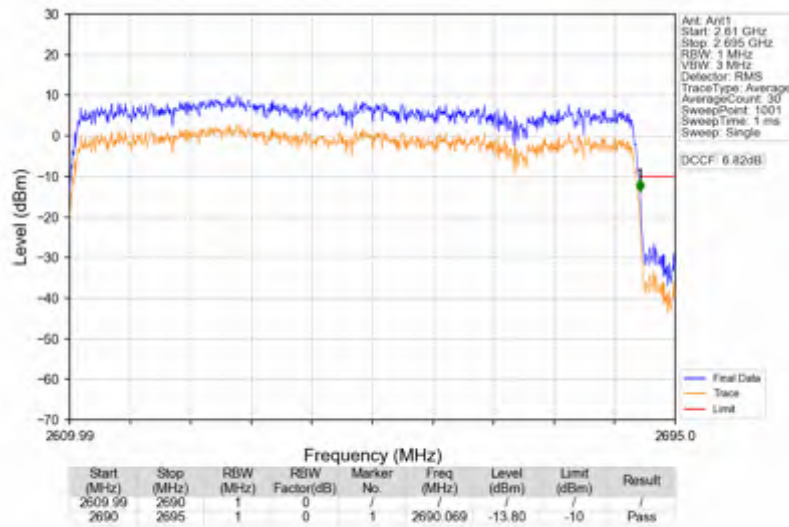
n41_30kHz_SISO_NTV_80MHz_CP-OFDM QPSK_2649.99MHz_Outer_Full
