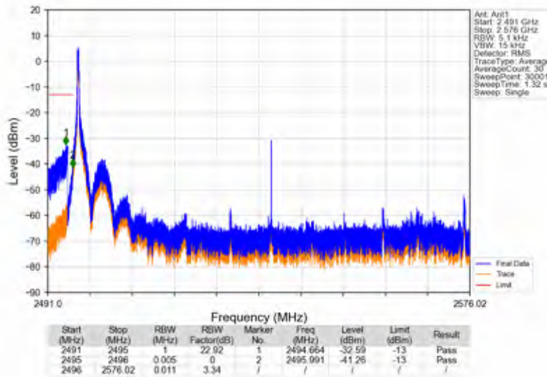
n41_30kHz_SISO_NTNV_80MHz_DFT-s-OFDM QPSK_2536.02MHz_Edge_1RB_Left
