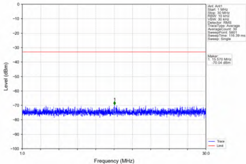
n41_30kHz_SISO_NTV_80MHz_DFT-s-OFDM_QPSK_2649.99MHz_Edge_1RB_Right
