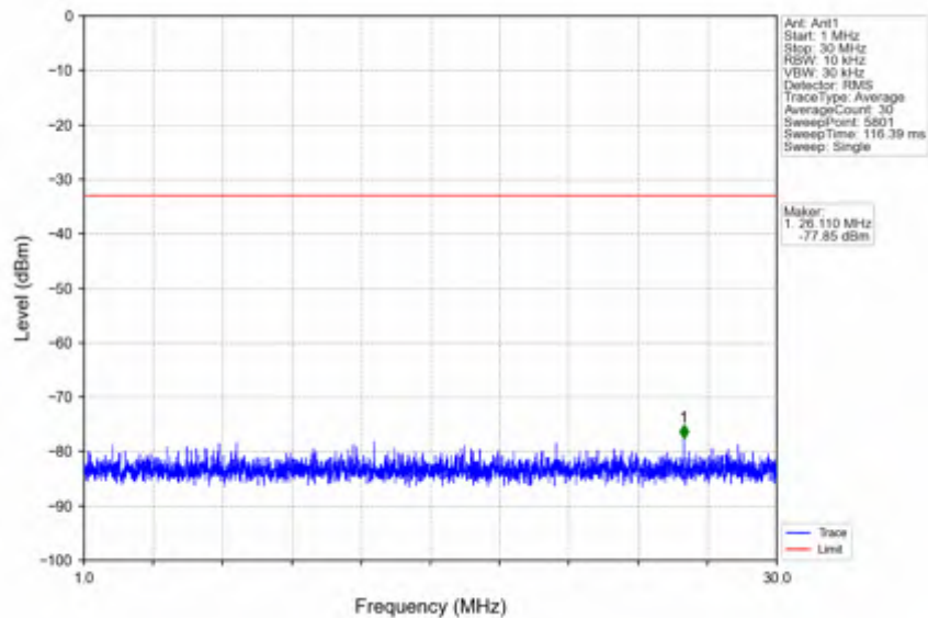
n41_30kHz_SISO_NTV_50MHz_DFT-s-OFDM_QPSK_2664.99MHz_Inner_1RB_Right
