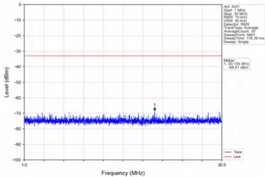
n41_30kHz_SISO_NTV_90MHz_DFT-s-OFDM QPSK_2644.98MHz_Edge_1RB_Right
