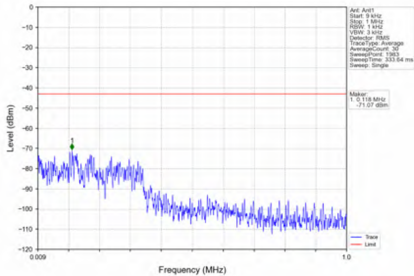
n41_30kHz_SISO_NTNV_80MHz_DFT-s-OFDM PI/2 BPSK_2592.99MHz_Edge_1RB_Left
