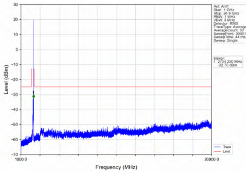
n41_30kHz_SISO_NTV_80MHz_CP-OFDM QPSK_2649.99MHz_Outer_Full
