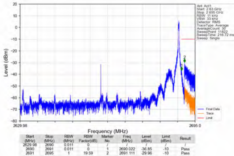
n41_30kHz_SISO_NTNV_60MHz_DFT-s-OFDM QPSK_2659.98MHz_Edge_1RB_Right
