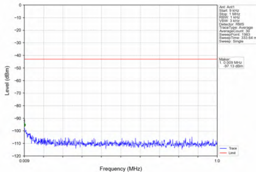
n41_30kHz_SISO_NTNV_60MHz_DFT-s-OFDM QPSK_2526MHz_Outer_Full
