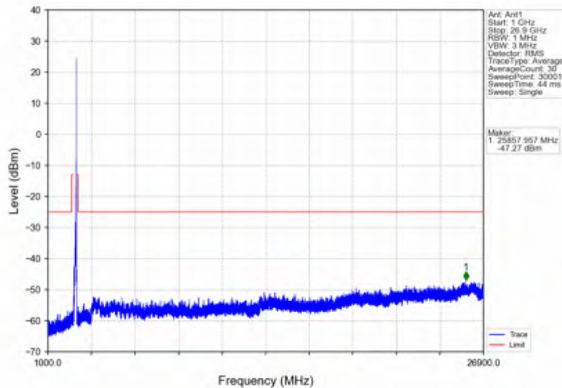
n41_30kHz_SISO_NTV_90MHz_DFT-s-OFDM_QPSK_2644.98MHz_Inner_1RB_Right
