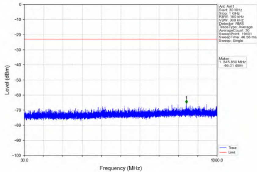
n41_30kHz_SISO_NTNV_15MHz_CP-OFDM QPSK_2682.48MHz_Outer_Full
