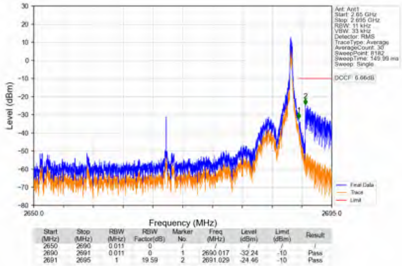
n41_30kHz_SISO_NTNV_40MHz_DFT-s-OFDM QPSK_2670MHz_Edge_1RB_Right
