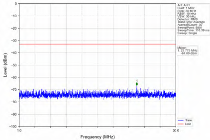
n41_30kHz_SISO_NTNV_20MHz_DFT-s-OFDM QPSK_2592.99MHz_Edge_1RB_Left
