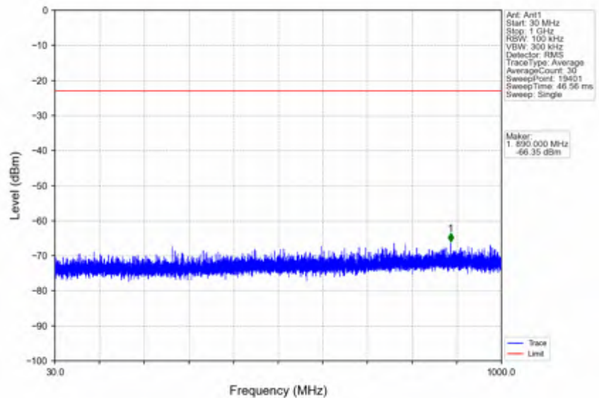
n41_30kHz_SISO_NTNV_30MHz_DFT-s-OFDM QPSK_2674.98MHz_Outer_Full
