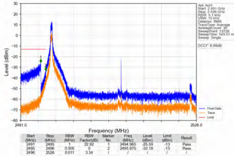
n41_30kHz_SISO_NTNV_30MHz_CP-OFDM QPSK_2511MHz_Edge_1RB_Left
