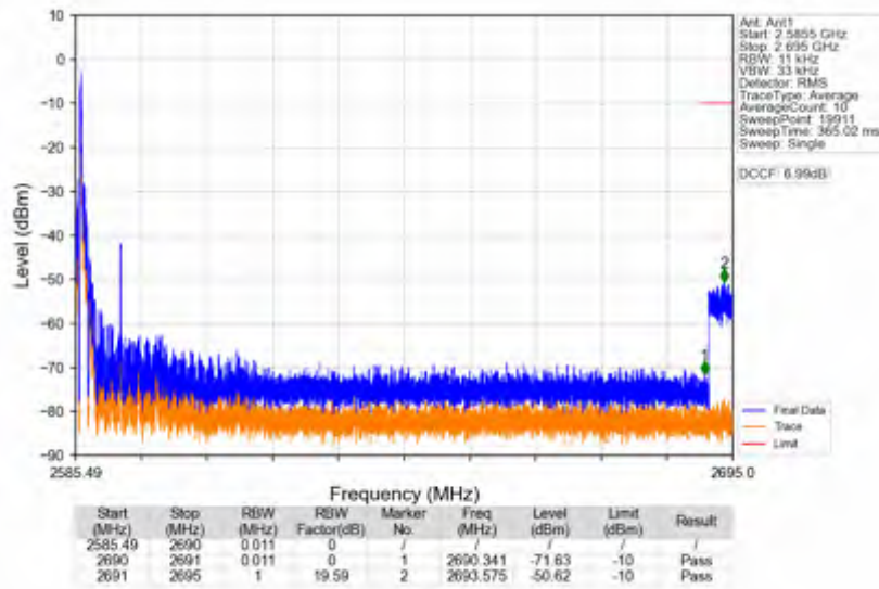
n41_30kHz_SISO_NTV_15MHz_CP-OFDM QPSK_2592.99MHz_Edge_1RB_Left
