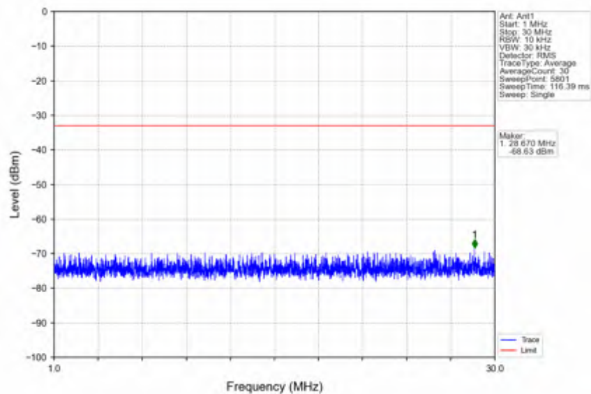
n41_30kHz_SISO_NTNV_30MHz_DFT-s-OFDM QPSK_2511MHz_Edge_1RB_Left
