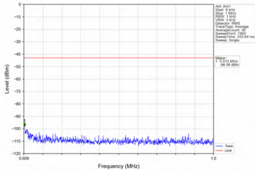
n41_30kHz_SISO_NTNV_15MHz_CP-OFDM QPSK_2682.48MHz_Outer_Full
