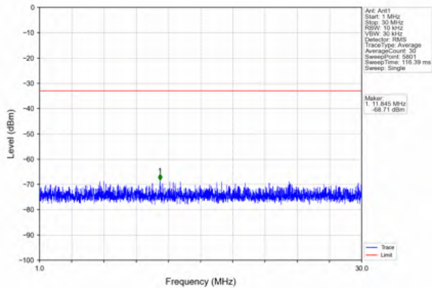
n41_30kHz_SISO_NTNV_15MHz_CP-OFDM QPSK_2682.48MHz_Edge_1RB_Right
