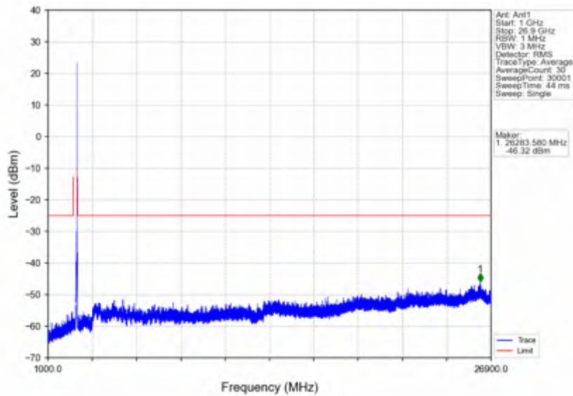
n41_30kHz_SISO_NTV_30MHz_CP-OFDM QPSK_2674.98MHz_Outer_Full
