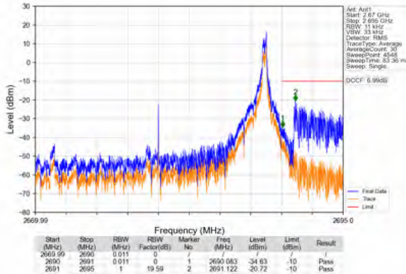
n41_30kHz_SISO_NTNV_20MHz_DFT-s-OFDM QPSK_2679.99MHz_Inner_1RB_Right
