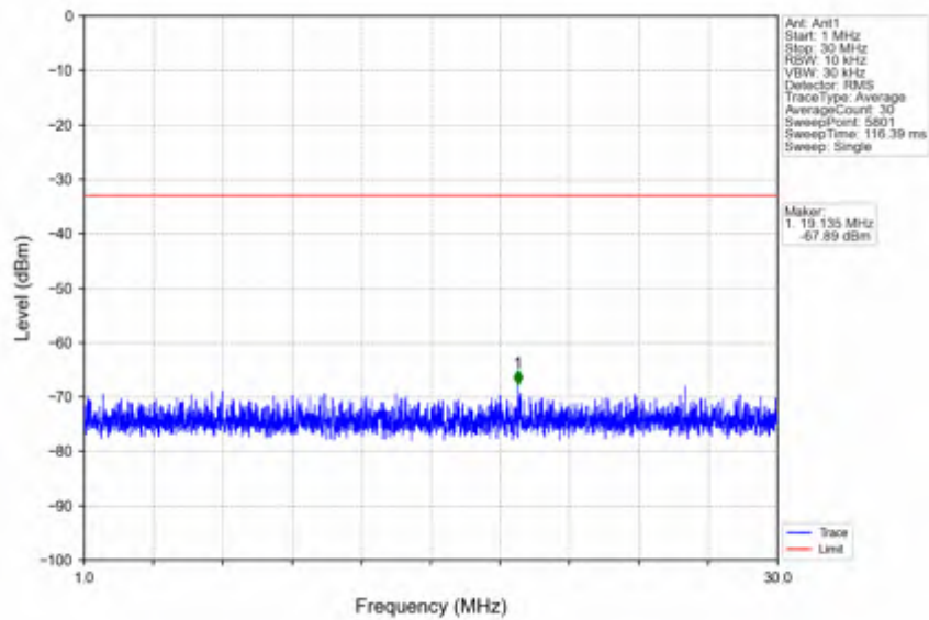
n41_30kHz_SISO_NTNV_40MHz_CP-OFDM QPSK_2670MHz_Edge_1RB_Right
