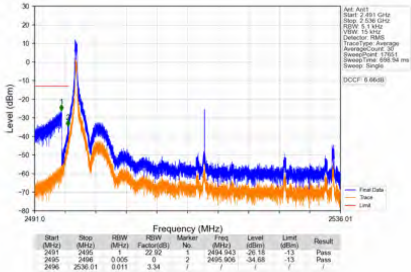
n41_30kHz_SISO_NTNV_40MHz_DFT-s-OFDM QPSK_2516.01MHz_Edge_1RB_Left
