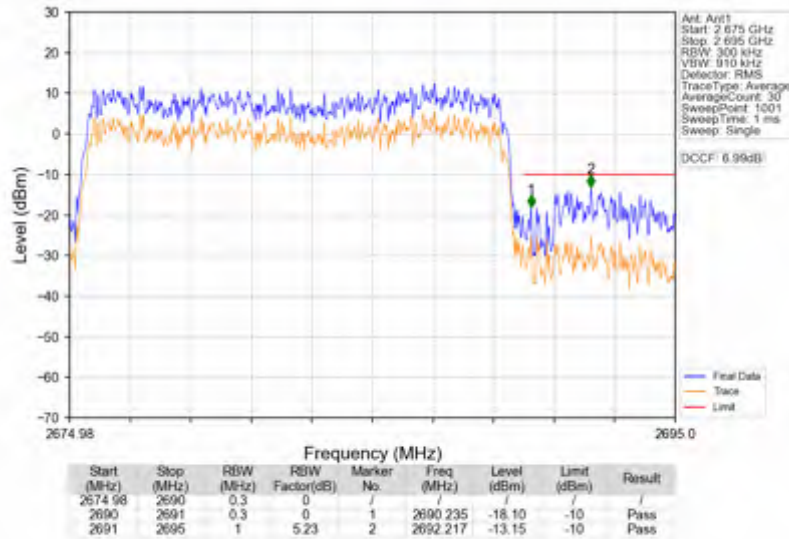
n41_30kHz_SISO_NTV_15MHz_CP-OFDM QPSK_2682.48MHz_Outer_Full
