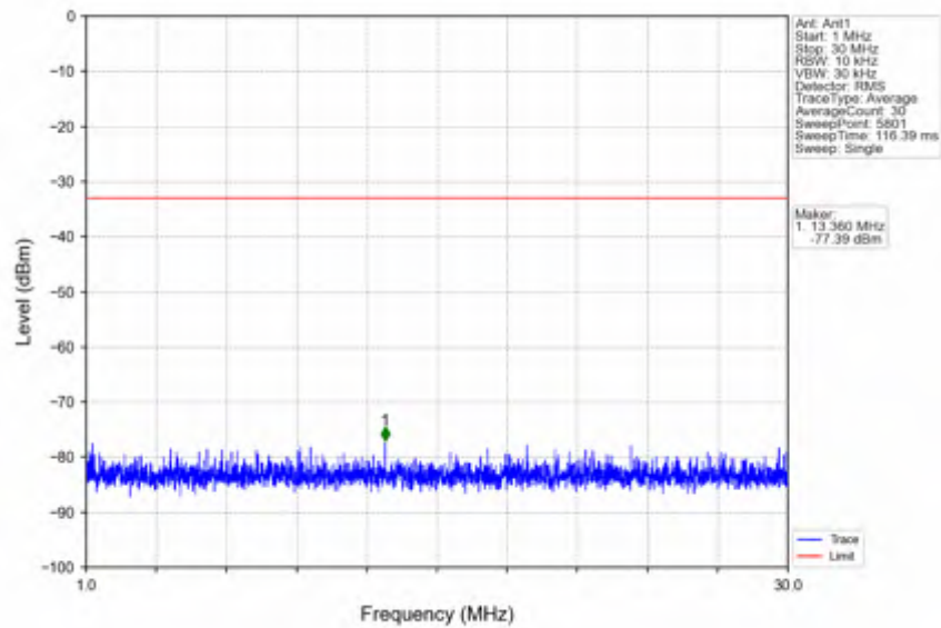
n41_30kHz_SISO_NTNV_30MHz_CP-OFDM QPSK_2674.98MHz_Inner_1RB_Right
