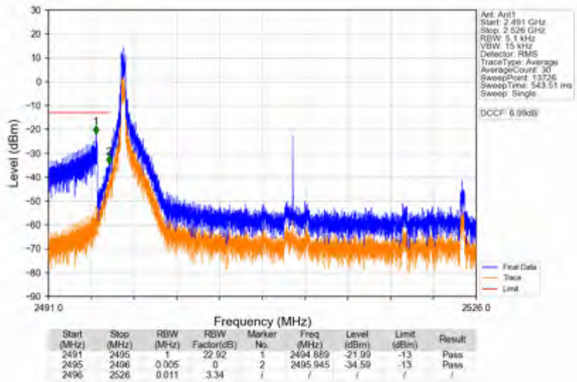
n41_30kHz_SISO_NTNV_30MHz_DFT-s-OFDM QPSK_2511MHz_Edge_1RB_Left
