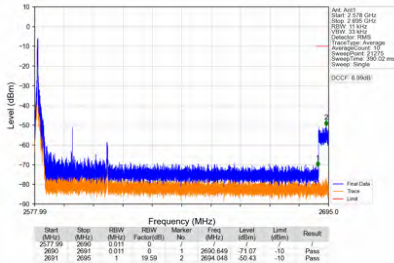
n41_30kHz_SISO_NTNV_30MHz_DFT-s-OFDM QPSK_2592.99MHz_Edge_1RB_Left
