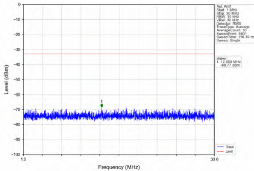
n41_30kHz_SISO_NTNV_20MHz_CP-OFDM QPSK_2679.99MHz_Edge_1RB_Right
