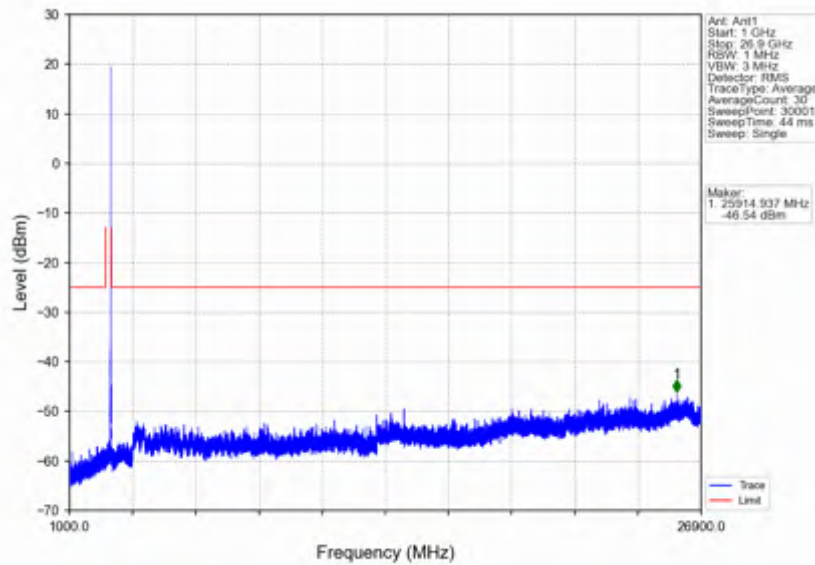
n41_30kHz_SISO_NTV_20MHz_DFT-s-OFDM QPSK_2679.99MHz_Edge_1RB_Right
