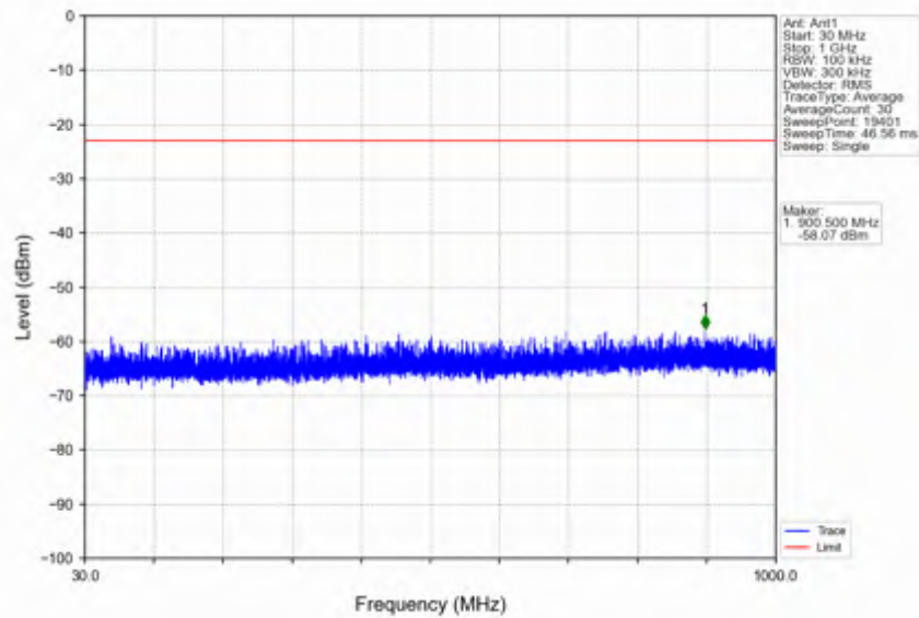
n41_30kHz_SISO_NTV_30MHz_DFT-s-OFDM QPSK_2674.98MHz_Edge_1RB_Right
