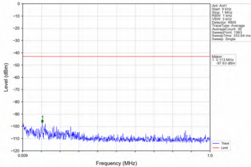
n41_30kHz_SISO_NTV_30MHz_DFT-s-OFDM_QPSK_2674.98MHz_Inner_1RB_Right
