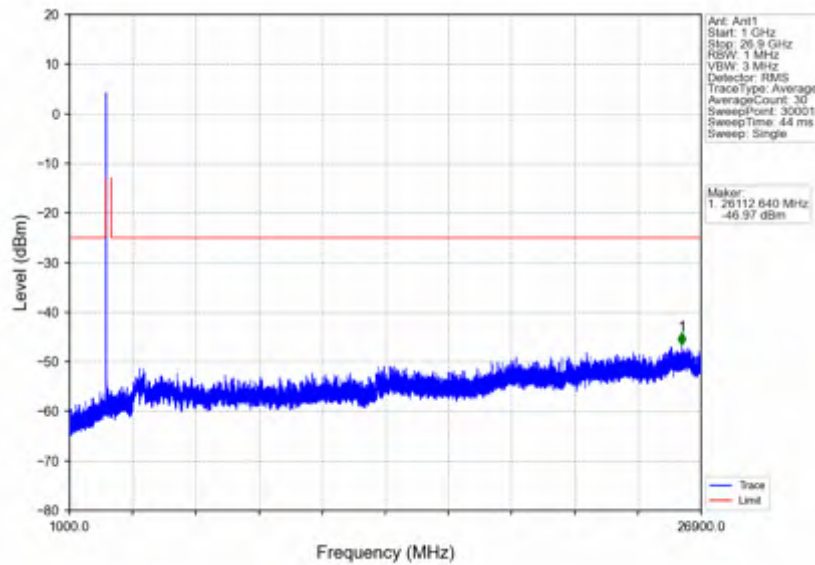
n41_30kHz_SISO_NTV_15MHz_CP-OFDM QPSK_2592.99MHz_Edge_1RB_Left
