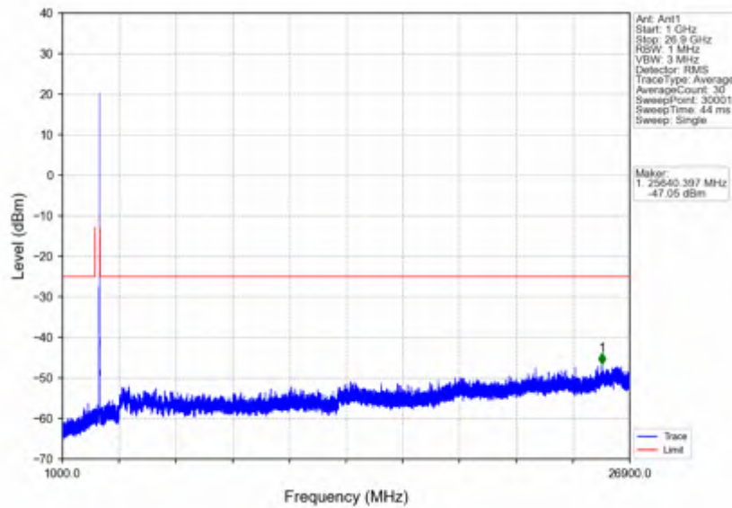
n41_30kHz_SISO_NTV_15MHz_CP-OFDM QPSK_2682.48MHz_Outer_Full
