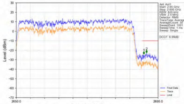
n41_30kHz_SISO_NTNV_40MHz_DFT-s-OFDM QPSK_2670MHz_Outer_Full
