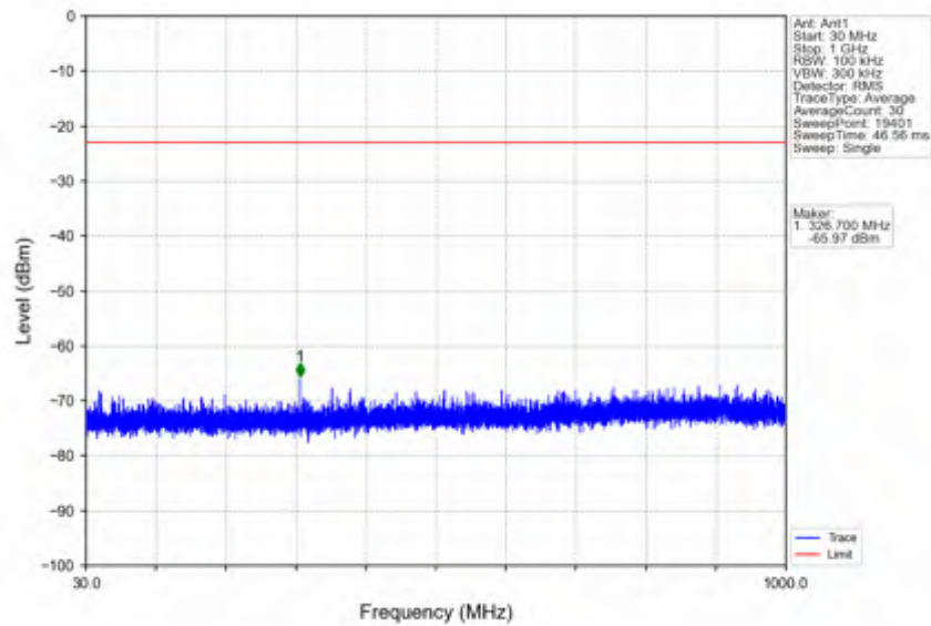
n41_30kHz_SISO_NTNV_30MHz_CP-OFDM QPSK_2511MHz_Outer_Full
