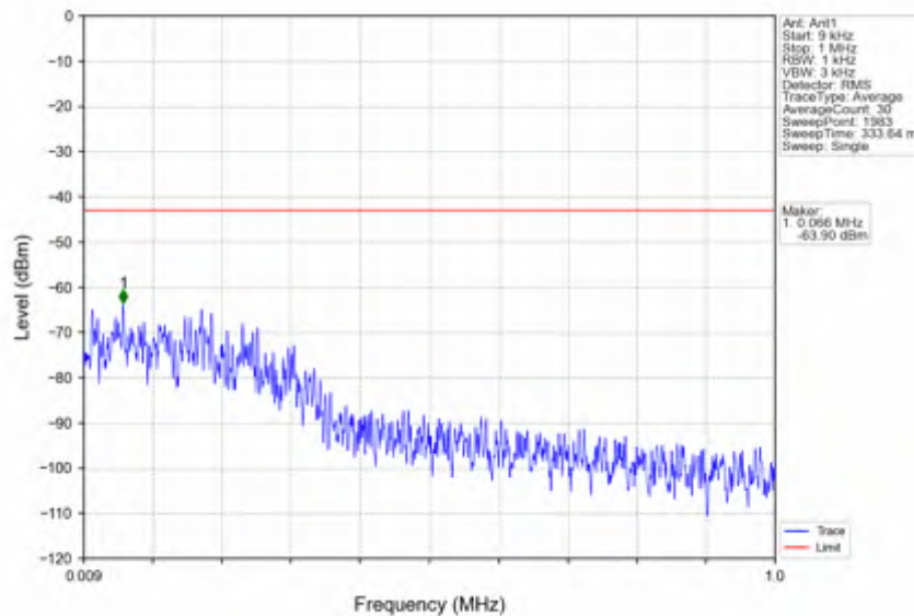
n41_30kHz_SISO_NTNV_40MHz_CP-OFDM QPSK_2516.01MHz_Edge_1RB_Left
