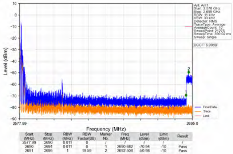
n41_30kHz_SISO_NTNV_30MHz_CP-OFDM QPSK_2592.99MHz_Edge_1RB_Left
