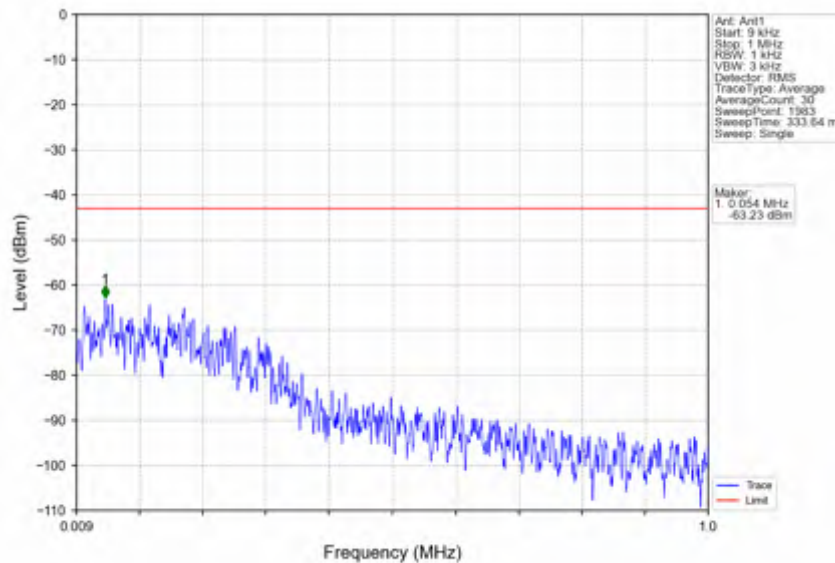
n41_30kHz_SISO_NTNV_30MHz_CP-OFDM QPSK_2674.98MHz_Edge_1RB_Right
