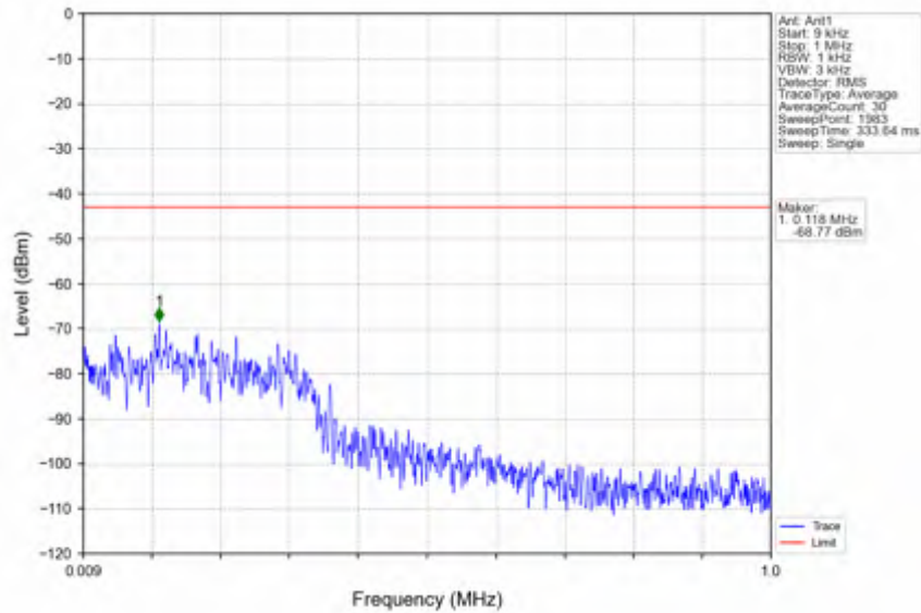
n41_30kHz_SISO_NTV_30MHz_DFT-s-OFDM_QPSK_2674.98MHz_Edge_1RB_Right
