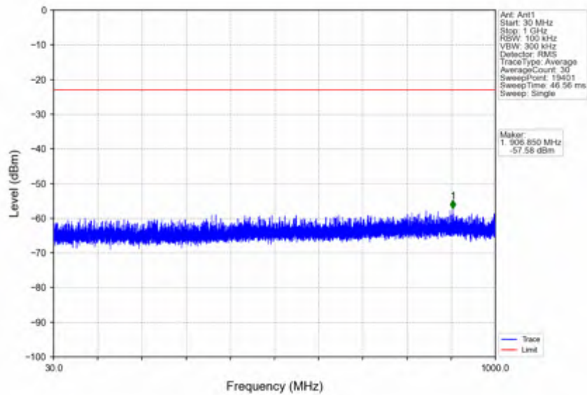
n41_30kHz_SISO_NTNV_40MHz_CP-OFDM QPSK_2592.99MHz_Edge_1RB_Left
