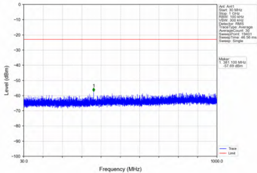
n41_30kHz_SISO_NTNV_40MHz_DFT-s-OFDM QPSK_2670MHz_Edge_1RB_Right
