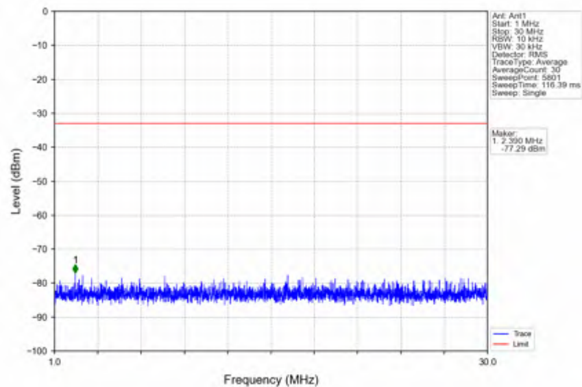
n41_30kHz_SISO_NTNV_20MHz_CP-OFDM QPSK_2679.99MHz_Outer_Full
