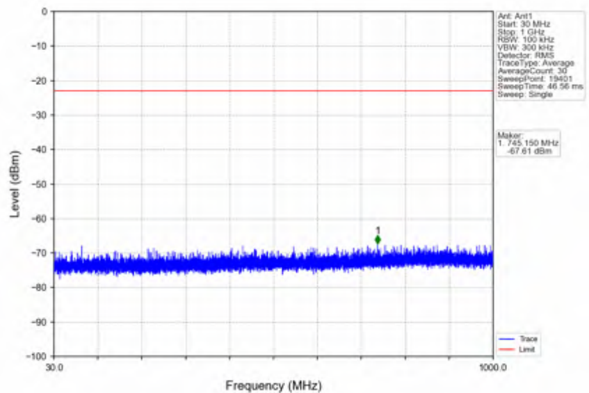
n41_30kHz_SISO_NTNV_40MHz_DFT-s-OFDM QPSK_2516.01MHz_Outer_Full
