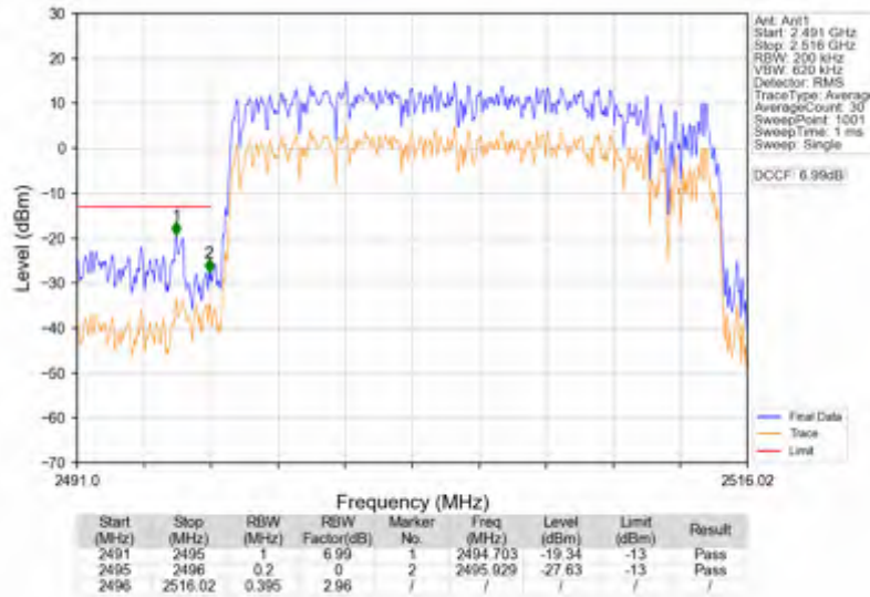
n41_30kHz_SISO_NTNV_20MHz_DFT-s-OFDM QPSK_2506.02MHz_Outer_Full
