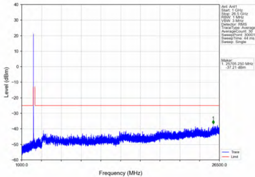
n41_30kHz_SISO_NTNV_20MHz_CP-OFDM QPSK_2506.02MHz_Outer_Full
