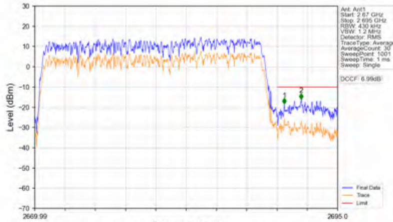
n41_30kHz_SISO_NTNV_20MHz_DFT-s-OFDM QPSK_2679.99MHz_Outer_Full
