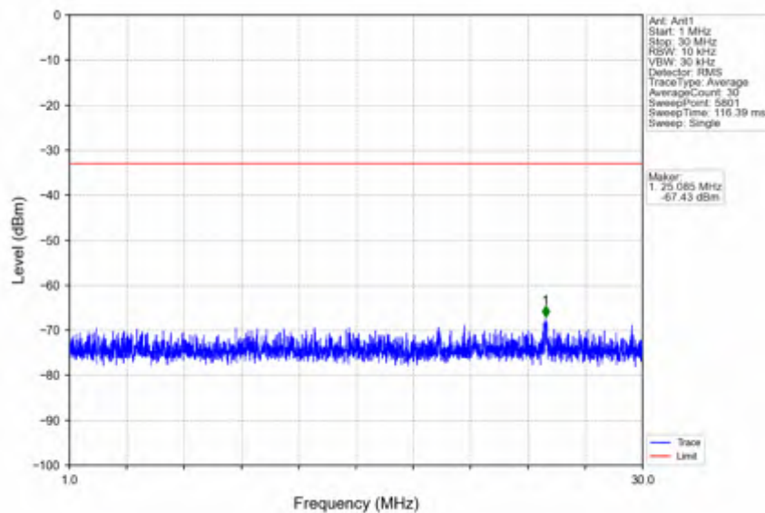
n41_30kHz_SISO_NTNV_15MHz_CP-OFDM QPSK_2592.99MHz_Edge_1RB_Left
