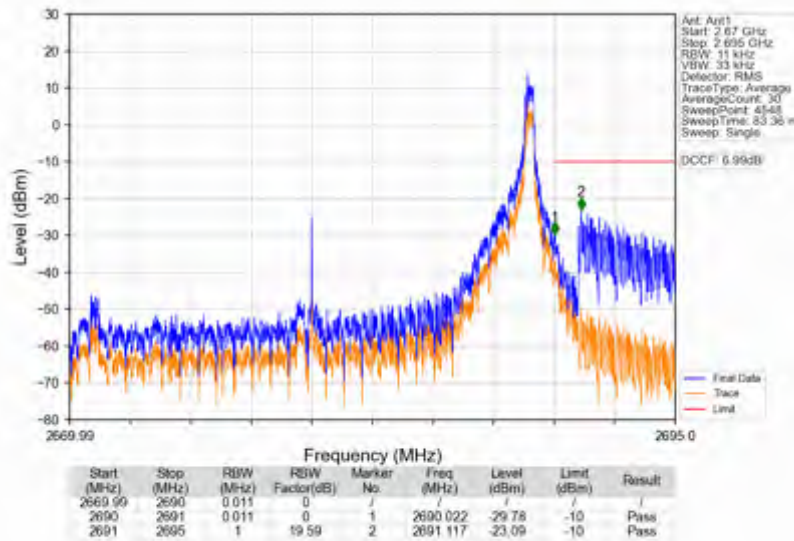
n41_30kHz_SISO_NTNV_20MHz_DFT-s-OFDM QPSK_2679.99MHz_Edge_1RB_Right
