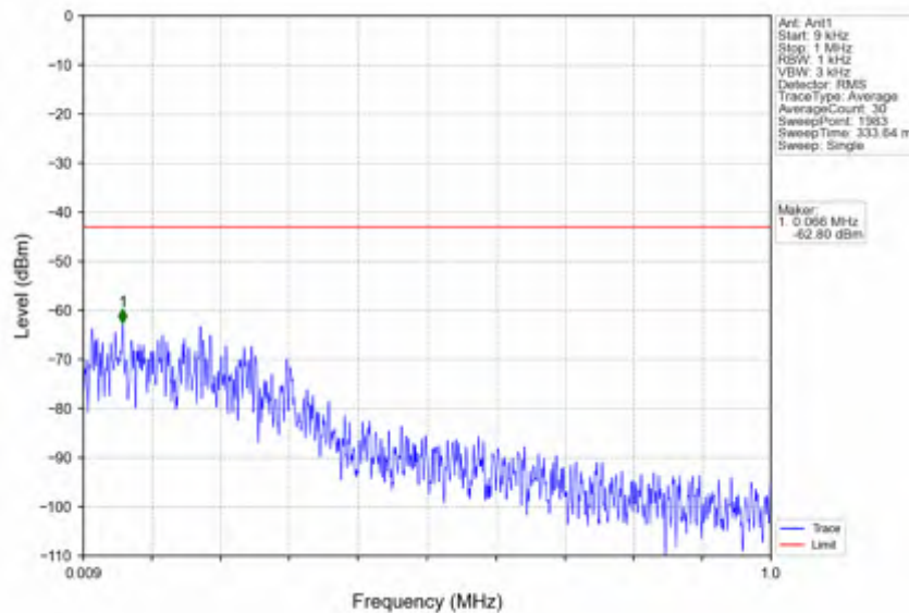
n41_30kHz_SISO_NTNV_15MHz_CP-OFDM QPSK_2682.48MHz_Edge_1RB_Right
