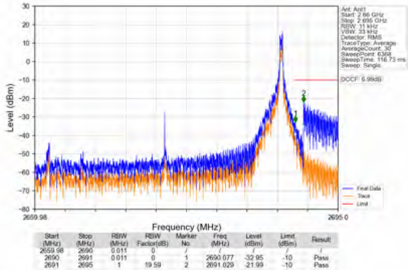
n41_30kHz_SISO_NTNV_30MHz_DFT-s-OFDM QPSK_2674.98MHz_Inner_1RB_Right
