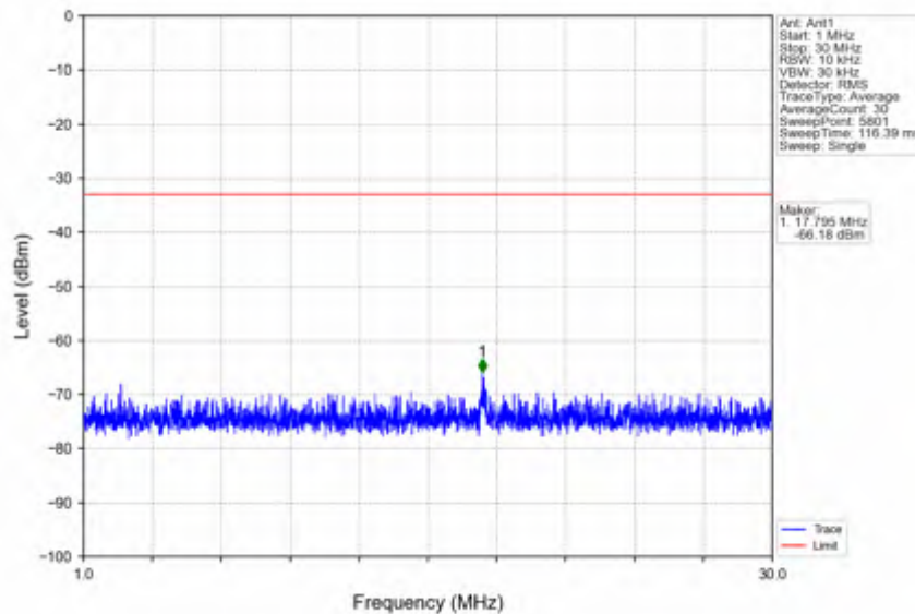
n41_30kHz_SISO_NTNV_30MHz_CP-OFDM QPSK_2592.99MHz_Edge_1RB_Left
