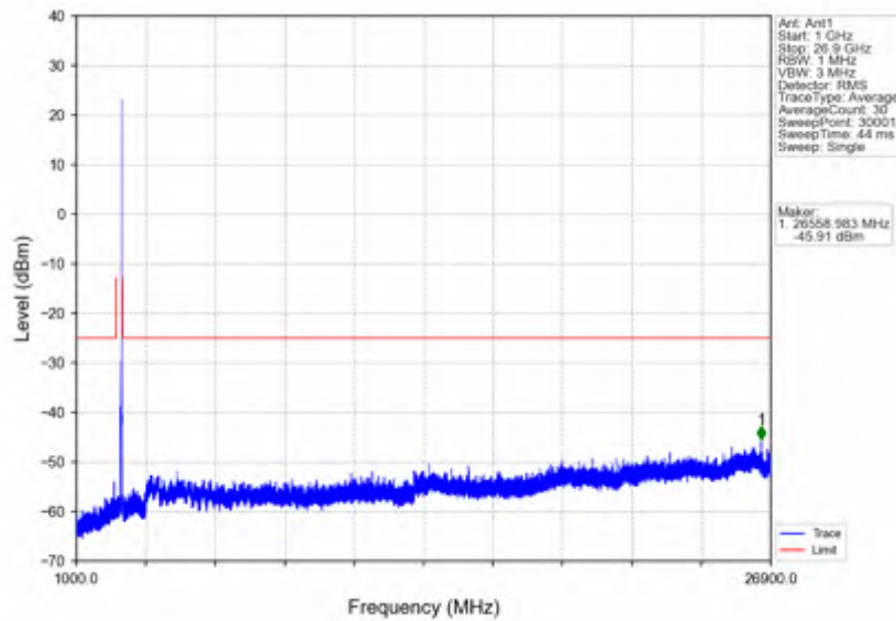
n41_30kHz_SISO_NTV_20MHz_CP-OFDM QPSK_2679.99MHz_Outer_Full
