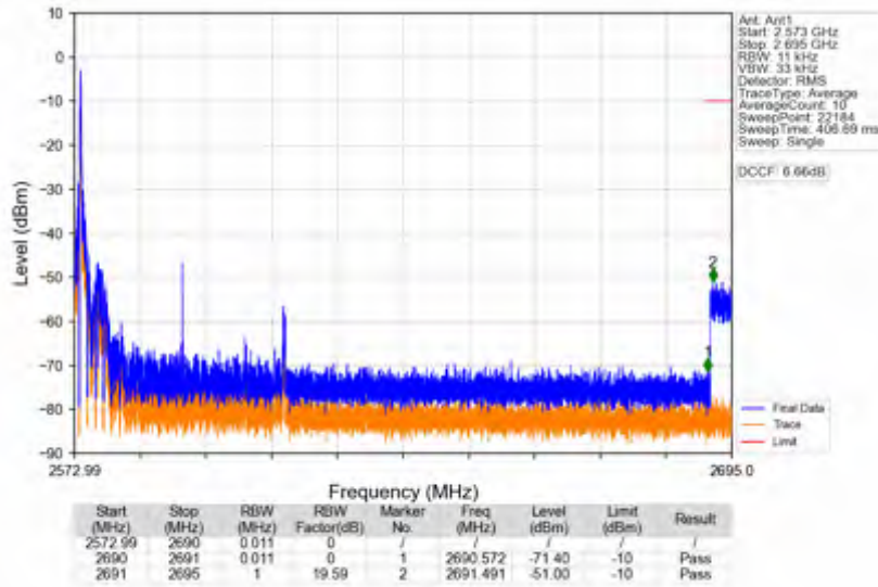
n41_30kHz_SISO_NTNV_40MHz_DFT-s-OFDM QPSK_2592.99MHz_Edge_1RB_Left
