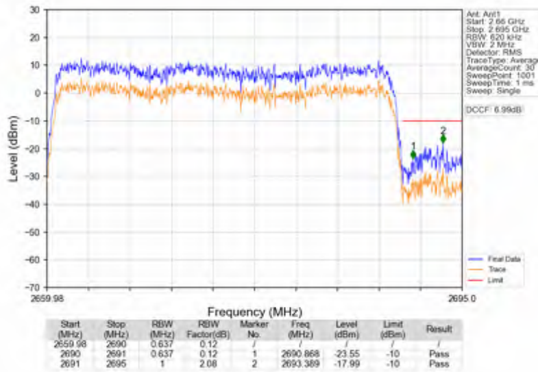
n41_30kHz_SISO_NTV_30MHz_CP-OFDM QPSK_2674.98MHz_Outer_Full
