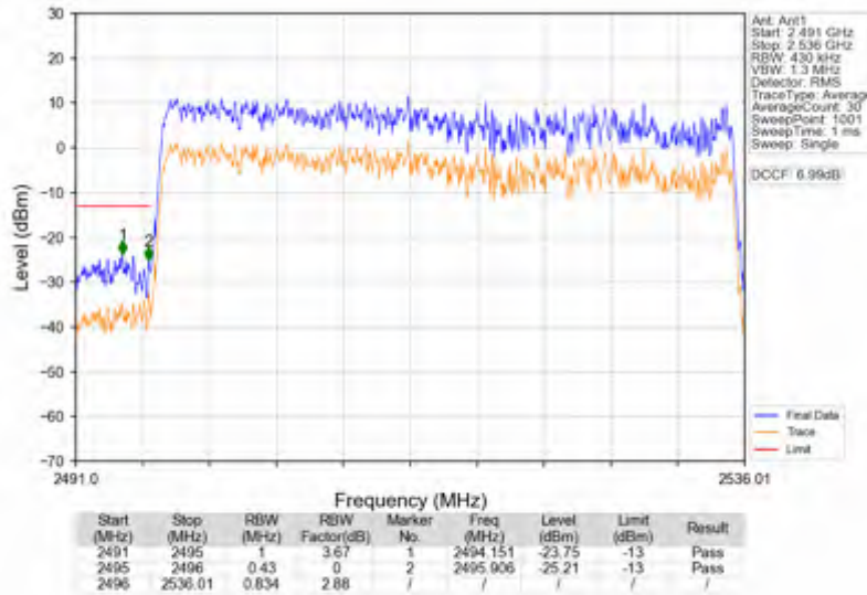
n41_30kHz_SISO_NTNV_40MHz_CP-OFDM QPSK_2516.01MHz_Outer_Full
