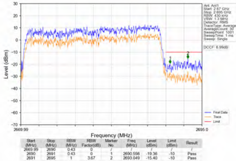
n41_30kHz_SISO_NTV_20MHz_CP-OFDM QPSK_2679.99MHz_Outer_Full
