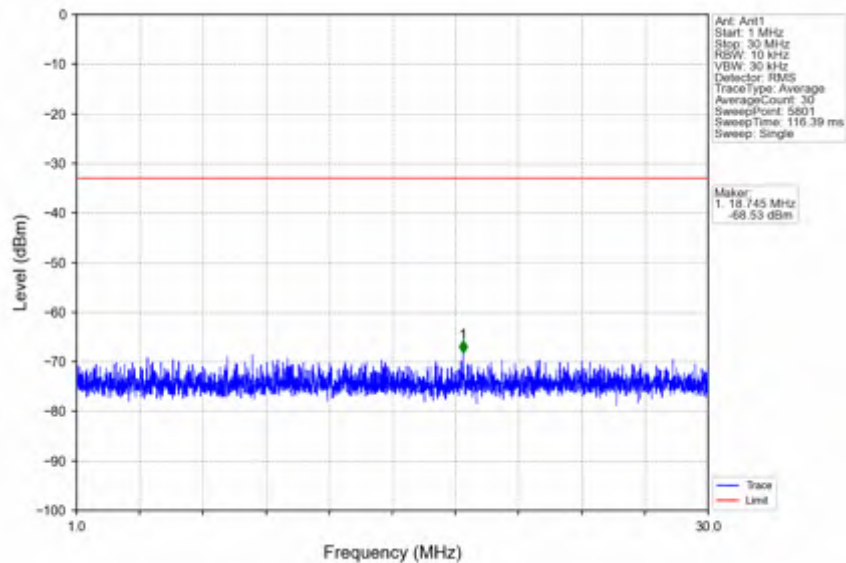
n41_30kHz_SISO_NTV_20MHz_DFT-s-OFDM_QPSK_2679.99MHz_Edge_1RB_Right
