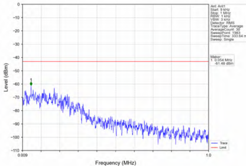
n41_30kHz_SISO_NTV_20MHz_CP-OFDM QPSK_2679.99MHz_Edge_1RB_Right
