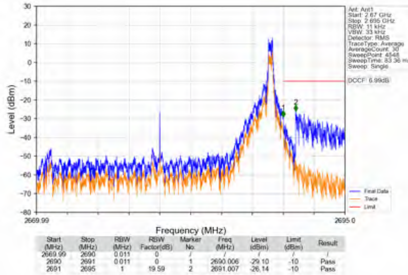
n41_30kHz_SISO_NTV_20MHz_CP-OFDM QPSK_2679.99MHz_Edge_1RB_Right
