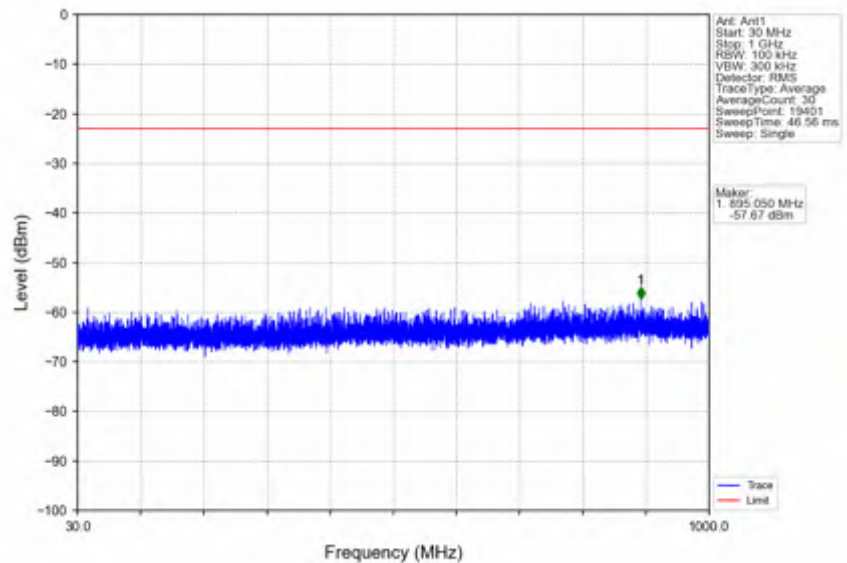
n41_30kHz_SISO_NTNV_40MHz_DFT-s-OFDM QPSK_2592.99MHz_Edge_1RB_Left
