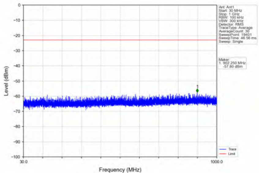
n41_30kHz_SISO_NTNV_30MHz_DFT-s-OFDM QPSK_2592.99MHz_Edge_1RB_Left
