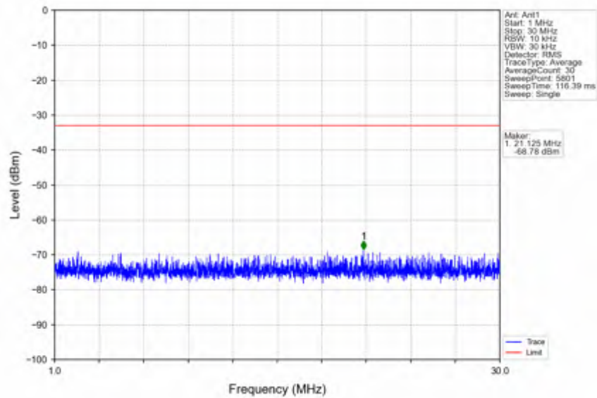
n41_30kHz_SISO_NTNV_30MHz_CP-OFDM QPSK_2511MHz_Edge_1RB_Left
