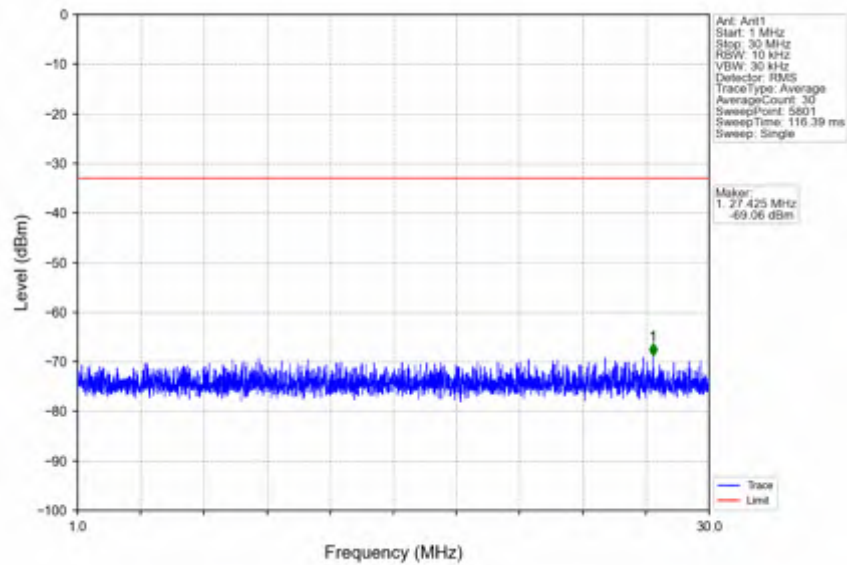
n41_30kHz_SISO_NTNV_30MHz_CP-OFDM QPSK_2674.98MHz_Edge_1RB_Right
