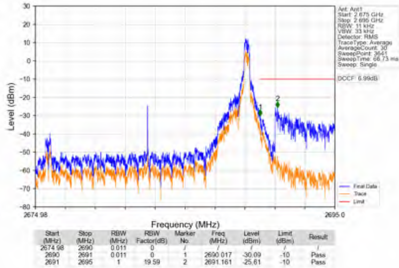
n41_30kHz_SISO_NTNV_15MHz_CP-OFDM QPSK_2682.48MHz_Edge_1RB_Right
