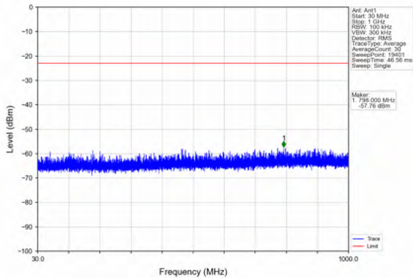
n41_30kHz_SISO_NTV_20MHz_DFT-s-OFDM QPSK_2679.99MHz_Edge_1RB_Right
