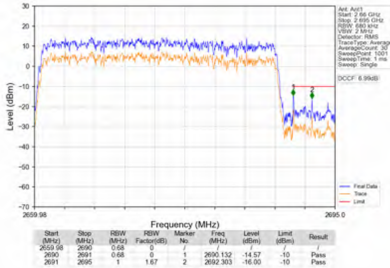
n41_30kHz_SISO_NTNV_30MHz_DFT-s-OFDM QPSK_2674.98MHz_Outer_Full
