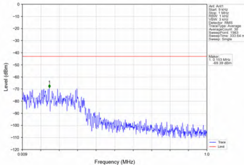
n41_30kHz_SISO_NTNV_40MHz_DFT-s-OFDM QPSK_2592.99MHz_Edge_1RB_Left
