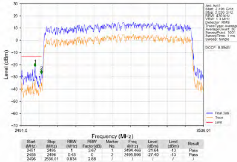
n41_30kHz_SISO_NTNV_40MHz_DFT-s-OFDM QPSK_2516.01MHz_Outer_Full
