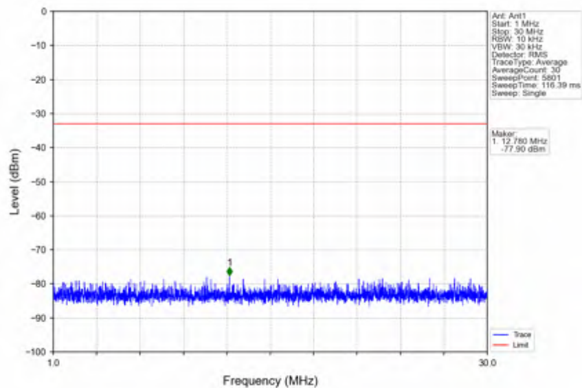
n41_30kHz_SISO_NTNV_40MHz_CP-OFDM QPSK_2670MHz_Outer_Full
