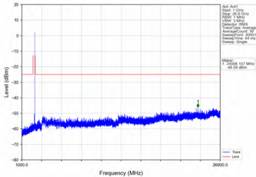
n41_15kHz_SISO_NTV_50MHz_CP-OFDM QPSK_2664.99MHz_Outer_Full
