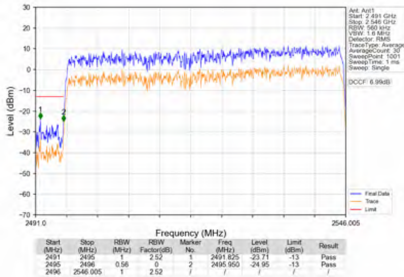
n41_15kHz_SISO_NTNV_50MHz_CP-OFDM QPSK_2521.005MHz_Outer_Full
