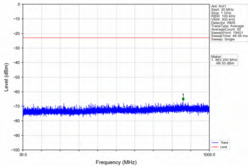
n41_30kHz_SISO_NTV_15MHz_DFT-s-OFDM_QPSK_2682.48MHz_Inner_1RB_Right
