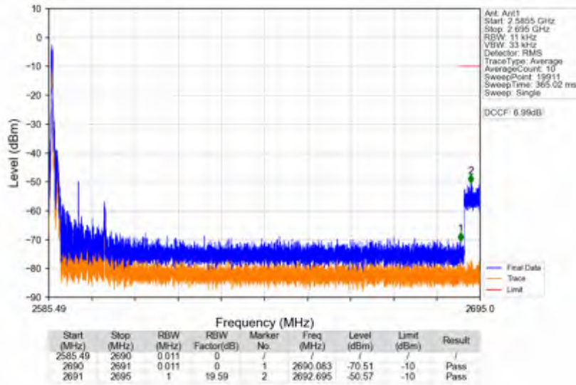
n41_30kHz_SISO_NTNV_15MHz_DFT-s-OFDM QPSK_2592.99MHz_Edge_1RB_Left
