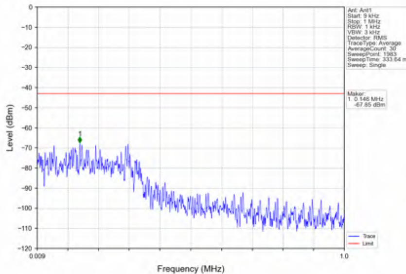
n41_30kHz_SISO_NTNV_15MHz_DFT-s-OFDM QPSK_2592.99MHz_Edge_1RB_Left
