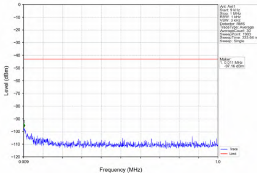
n41_30kHz_SISO_NTNV_15MHz_DFT-s-OFDM_QPSK_2503.5MHz_Outer_Full
