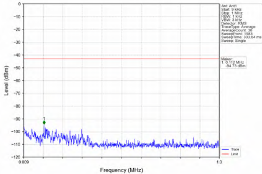
n41_30kHz_SISO_NTNV_15MHz_DFT-s-OFDM_QPSK_2503.5MHz_Inner_1RB_Left
