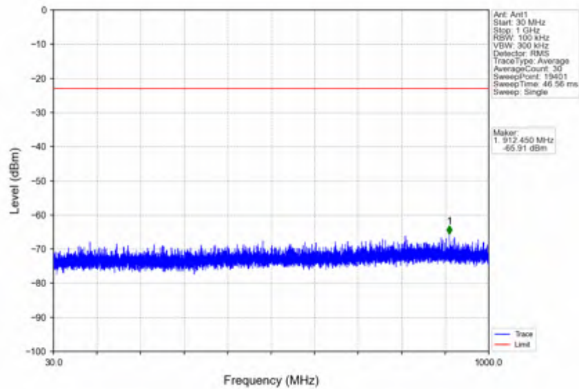
n41_15kHz_SISO_NTNV_50MHz_DFT-s-OFDM PI/2 BPSK_2521.005MHz_Outer_Full
