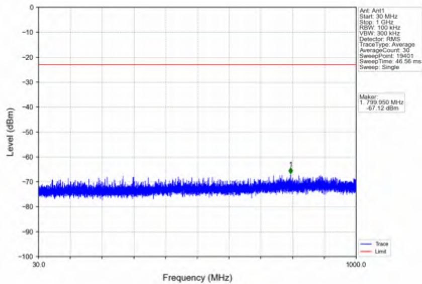
n41_30kHz_SISO_NTNV_15MHz_CP-OFDM QPSK_2503.5MHz_Outer_Full
