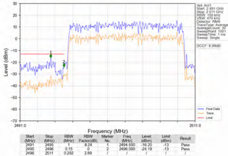
n41_30kHz_SISO_NTNV_15MHz_DFT-s-OFDM_QPSK_2503.5MHz_Outer_Full
