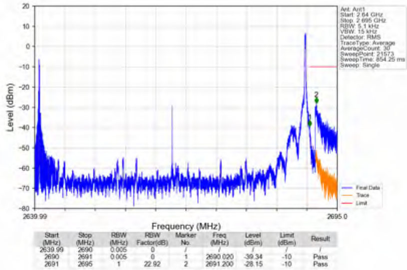
n41_15kHz_SISO_NTV_50MHz_DFT-s-OFDM QPSK_2664.99MHz_Edge_1RB_Right
