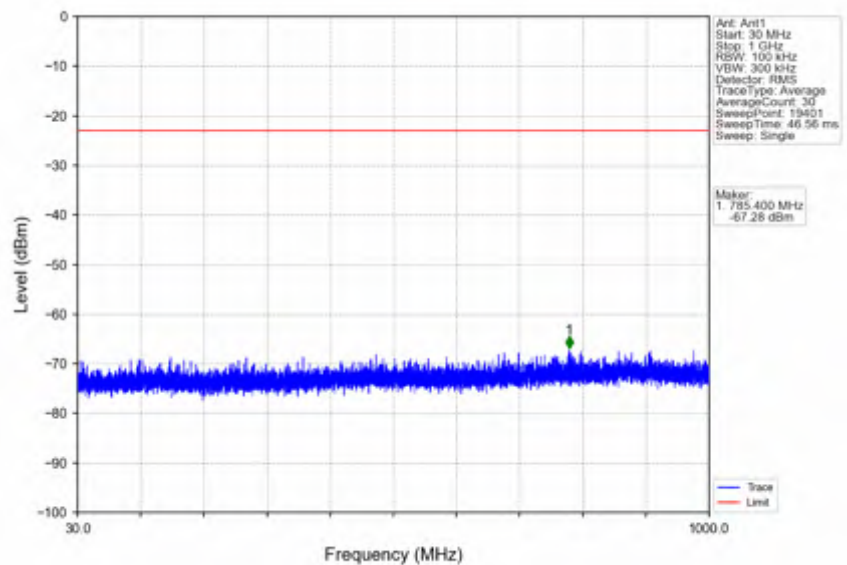
n41_15kHz_SISO_NTNV_40MHz_DFT-s-OFDM QPSK_2516.01MHz_Outer_Full
