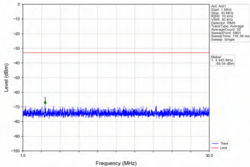
n41_30kHz_SISO_NTV_15MHz_CP-OFDM QPSK_2503.5MHz_Edge_1RB_Left
