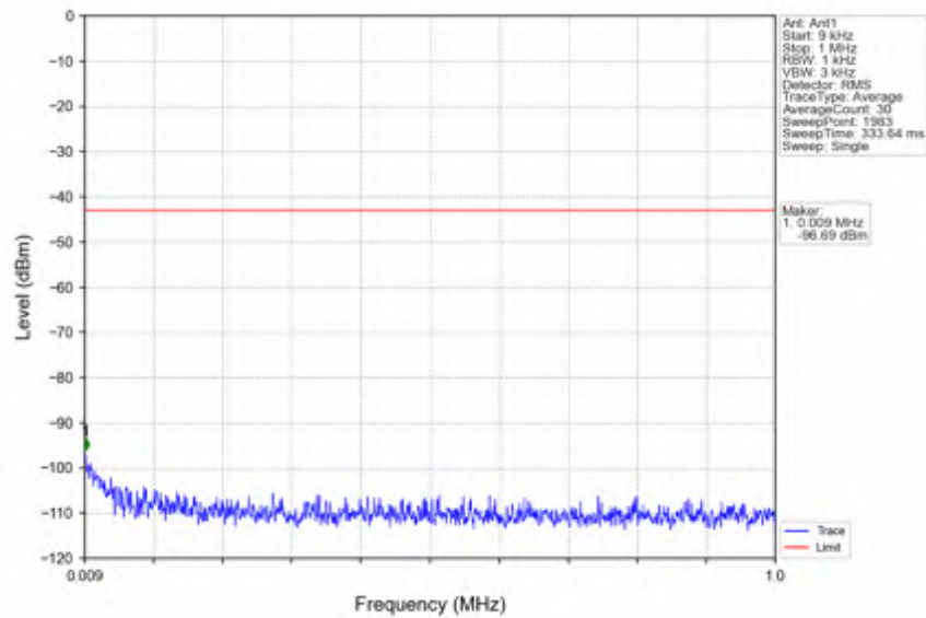
n41_30kHz_SISO_NTNV_10MHz_DFT-s-OFDM PI/2 BPSK_2685MHz_Outer_Full
