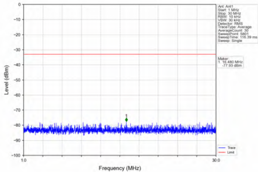
n41_15kHz_SISO_NTNV_50MHz_CP-OFDM QPSK_2664.99MHz_Inner_1RB_Right
