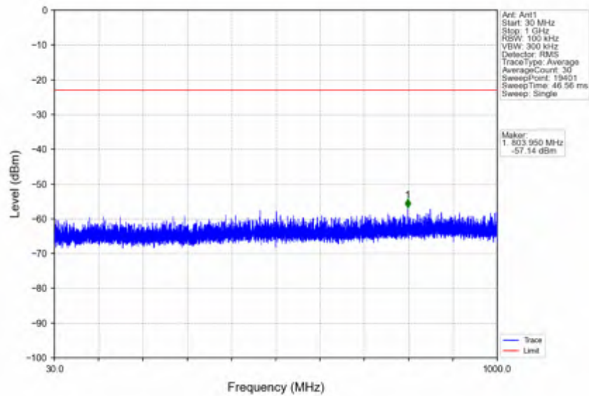
n41_30kHz_SISO_NTNV_15MHz_DFT-s-OFDM QPSK_2503.5MHz_Edge_1RB_Left
