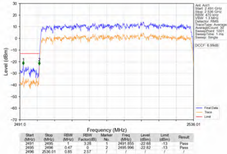
n41_15kHz_SISO_NTNV_40MHz_DFT-s-OFDM QPSK_2516.01MHz_Outer_Full
