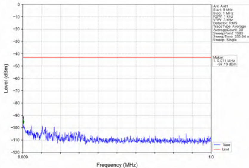
n41_30kHz_SISO_NTNV_15MHz_DFT-s-OFDM PI/2 BPSK_2682.48MHz_Inner_1RB_Right
