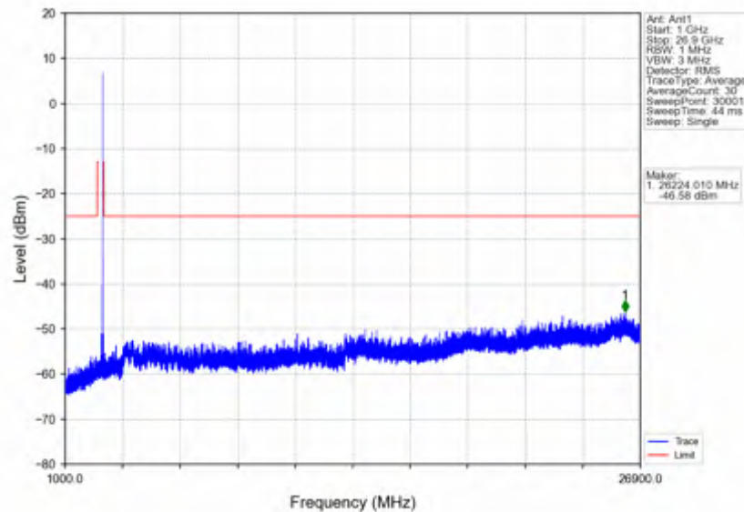
n41_15kHz_SISO_NTV_50MHz_DFT-s-OFDM QPSK_2664.99MHz_Edge_1RB_Right
