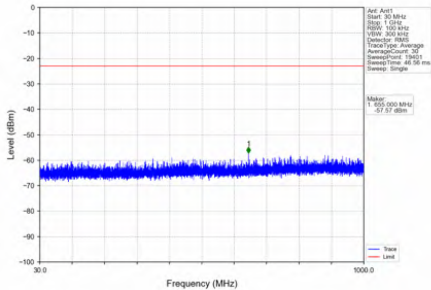
n41_15kHz_SISO_NTV_50MHz_DFT-s-OFDM QPSK_2664.99MHz_Edge_1RB_Right
