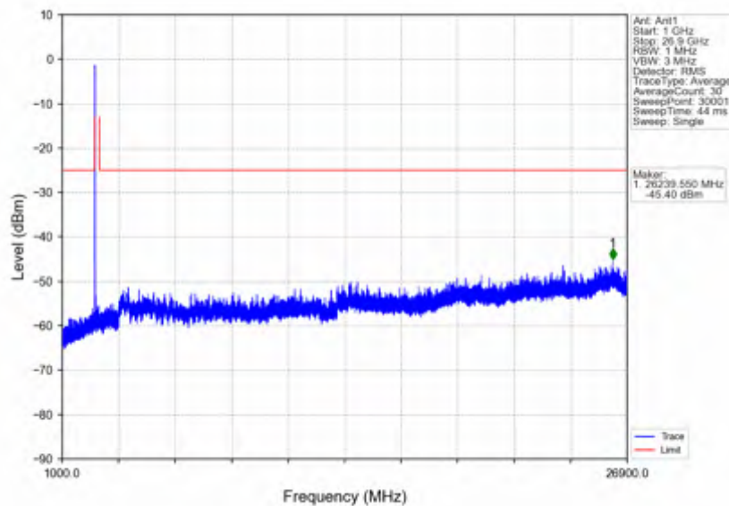
n41_30kHz_SISO_NTNV_10MHz_DFT-s-OFDM PI/2 BPSK_2501.01MHz_Outer_Full
