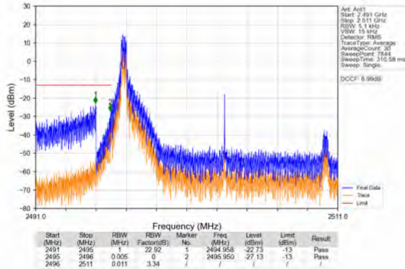
n41_30kHz_SISO_NTV_15MHz_CP-OFDM_QPSK_2503.5MHz_Edge_1RB_Left
