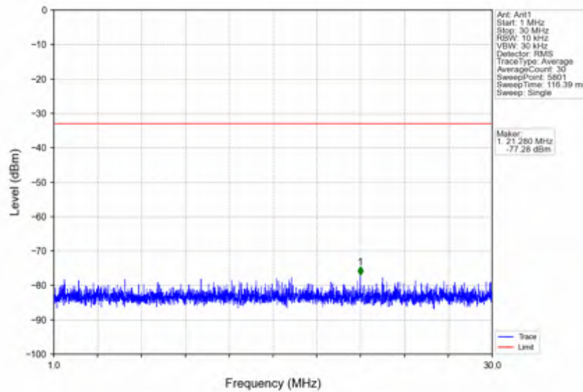
n41_15kHz_SISO_NTNV_50MHz_DFT-s-OFDM QPSK_2521.005MHz_Outer_Full
