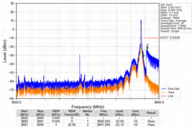
n41_15kHz_SISO_NTNV_40MHz_DFT-s-OFDM QPSK_2670MHz_Edge_1RB_Right
