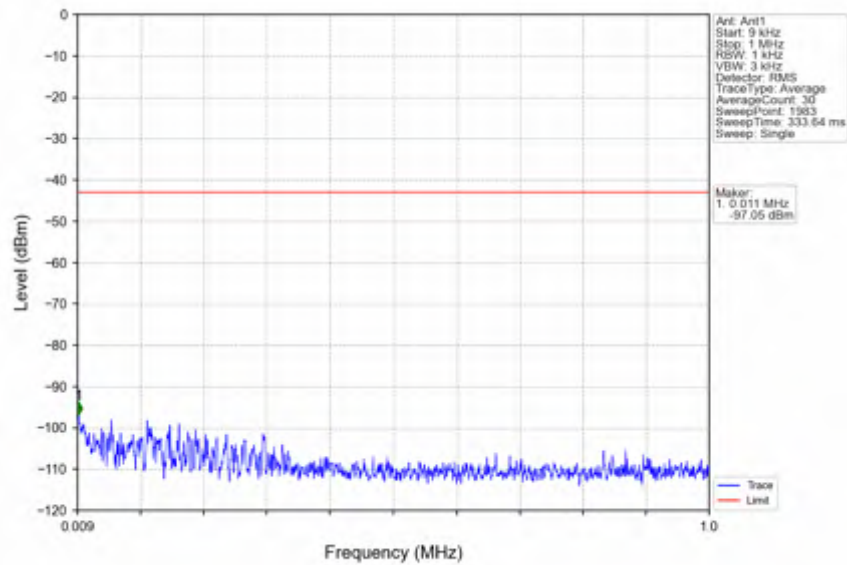
n41_30kHz_SISO_NTV_15MHz_DFT-s-OFDM_QPSK_2682.48MHz_Inner_1RB_Right
