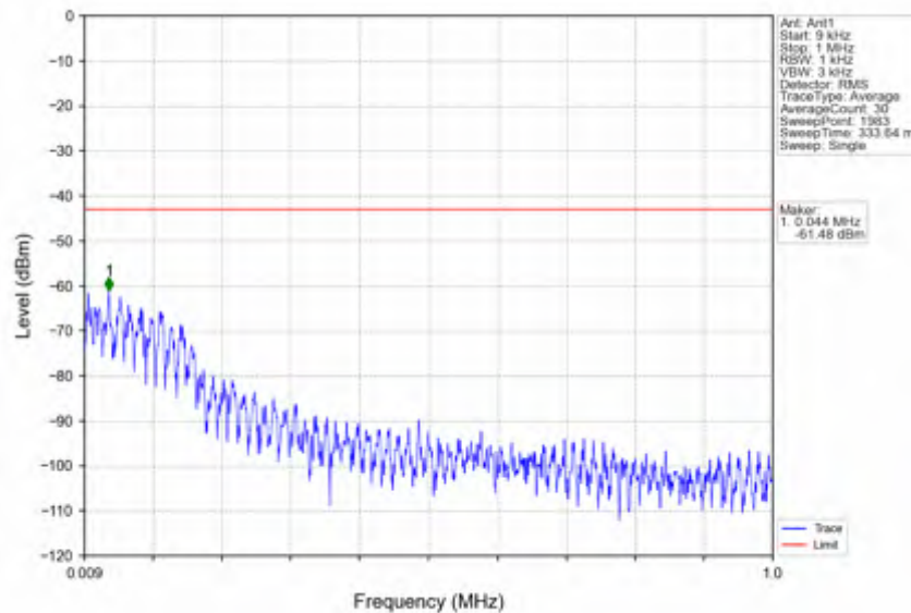
n41_15kHz_SISO_NTV_50MHz_CP-OFDM QPSK_2664.99MHz_Edge_1RB_Right
