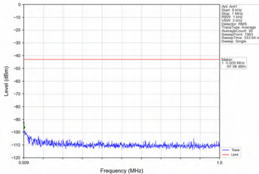
n41_30kHz_SISO_NTNV_10MHz_DFT-s-OFDM QPSK_2685MHz_Outer_Full
