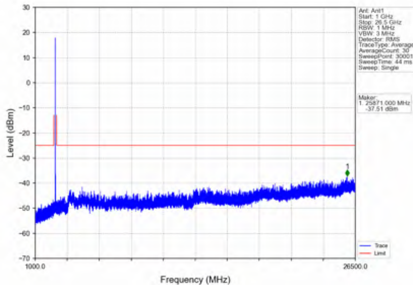
n41_30kHz_SISO_NTNV_15MHz_DFT-s-OFDM PI/2 BPSK_2592.99MHz_Edge_1RB_Left
