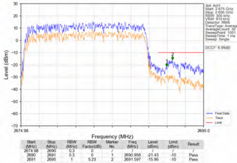
n41_30kHz_SISO_NTNV_15MHz_DFT-s-OFDM QPSK_2682.48MHz_Outer_Full
