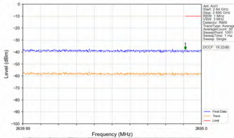
n41_15kHz_SISO_NTNV_50MHz_DFT-s-OFDM QPSK_2664.99MHz_Outer_Full
