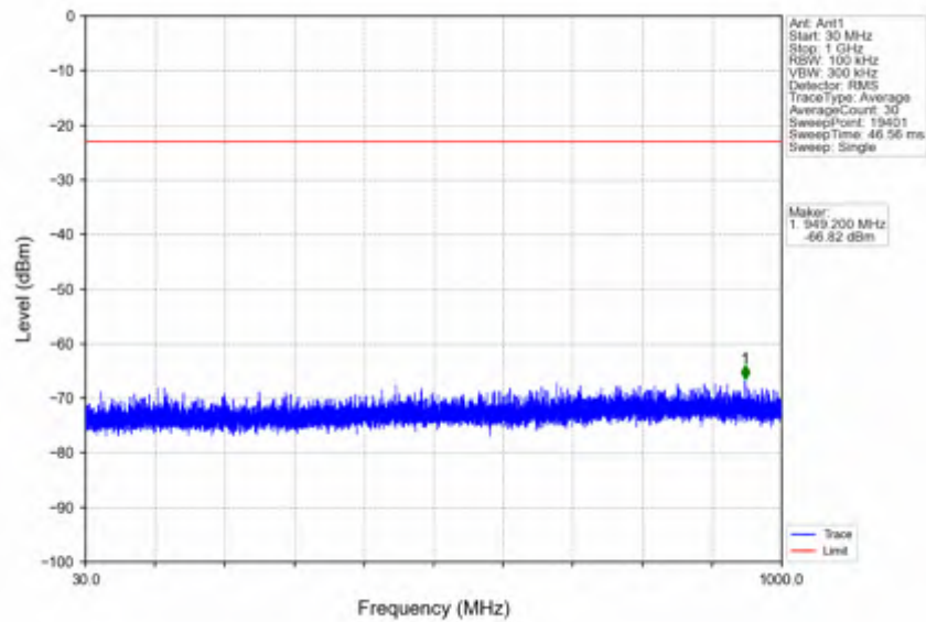
n41_30kHz_SISO_NTNV_10MHz_CP-OFDM QPSK_2685MHz_Outer_Full
