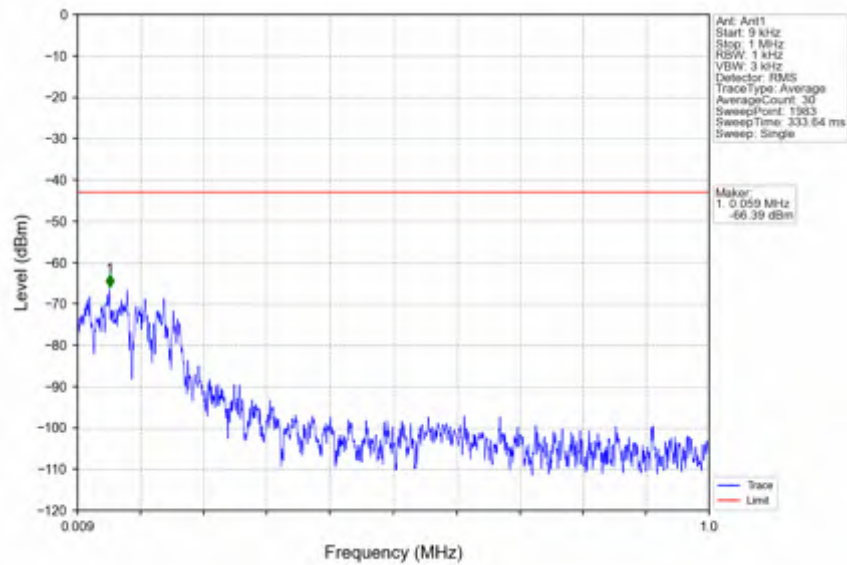
n41_15kHz_SISO_NTV_50MHz_DFT-s-OFDM QPSK_2664.99MHz_Edge_1RB_Right
