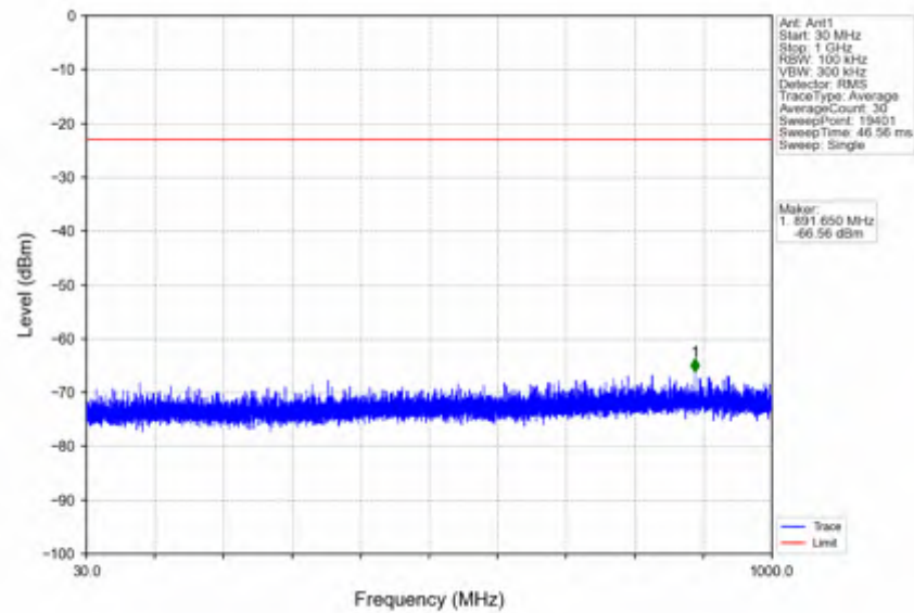
n41_30kHz_SISO_NTNV_10MHz_CP-OFDM QPSK_2501.01MHz_Outer_Full
