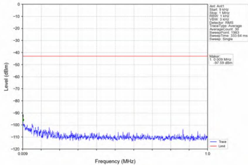
n41_15kHz_SISO_NTV_50MHz_DFT-s-OFDM QPSK_2664.99MHz_Inner_1RB_Right
