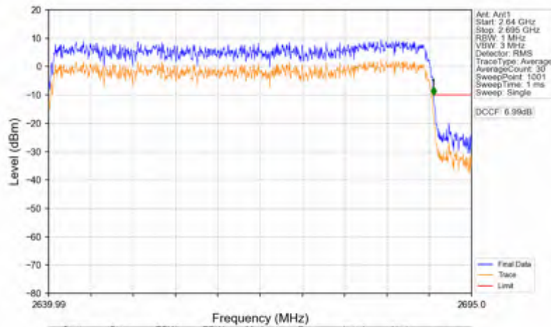
n41_15kHz_SISO_NTV_50MHz_CP-OFDM QPSK_2664.99MHz_Outer_Full
