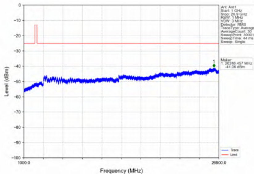
n41_15kHz_SISO_NTNV_50MHz_DFT-s-OFDM PI/2 BPSK_2664.99MHz_Outer_Full
