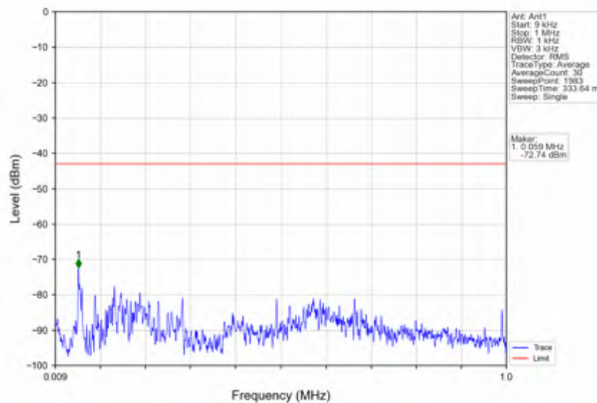
n41_15kHz_SISO_NTNV_50MHz_DFT-s-OFDM QPSK_2664.99MHz_Outer_Full
