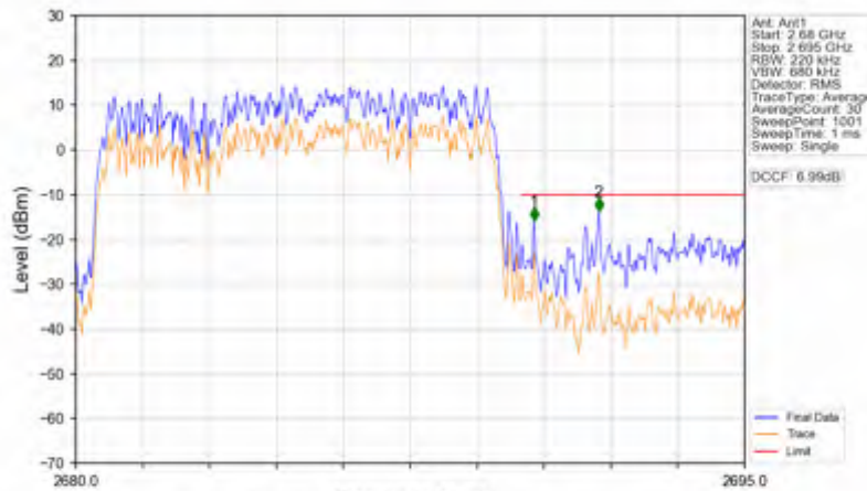
n41_30kHz_SISO_NTNV_10MHz_DFT-s-OFDM PI/2 BPSK_2685MHz_Outer_Full
