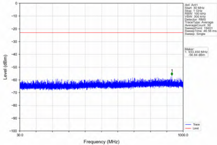
n41_30kHz_SISO_NTNV_10MHz_CP-OFDM QPSK_2592.99MHz_Edge_1RB_Left
