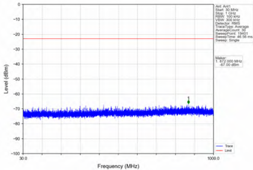
n41_30kHz_SISO_NTNV_15MHz_DFT-s-OFDM PI/2 BPSK_2682.48MHz_Outer_Full
