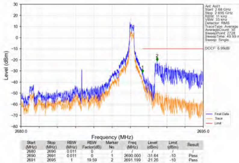
n41_30kHz_SISO_NTNV_10MHz_DFT-s-OFDM QPSK_2685MHz_Edge_1RB_Right
