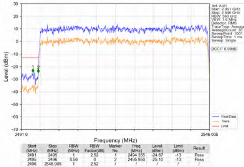
n41_15kHz_SISO_NTNV_50MHz_DFT-s-OFDM_QPSK_2521.005MHz_Outer_Full
