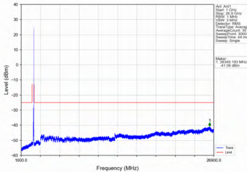
n41_15kHz_SISO_NTNV_40MHz_CP-OFDM QPSK_2670MHz_Outer_Full
