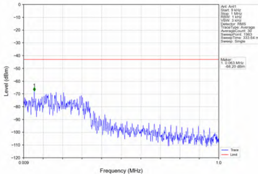
n41_30kHz_SISO_NTNV_10MHz_DFT-s-OFDM QPSK_2592.99MHz_Edge_1RB_Left
