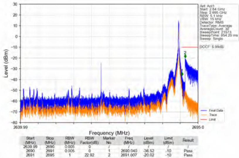
n41_15kHz_SISO_NTNV_50MHz_DFT-s-OFDM QPSK_2664.99MHz_Inner_1RB_Right
