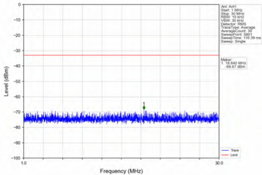
n41_15kHz_SISO_NTNV_50MHz_CP-OFDM QPSK_2664.99MHz_Edge_1RB_Right
