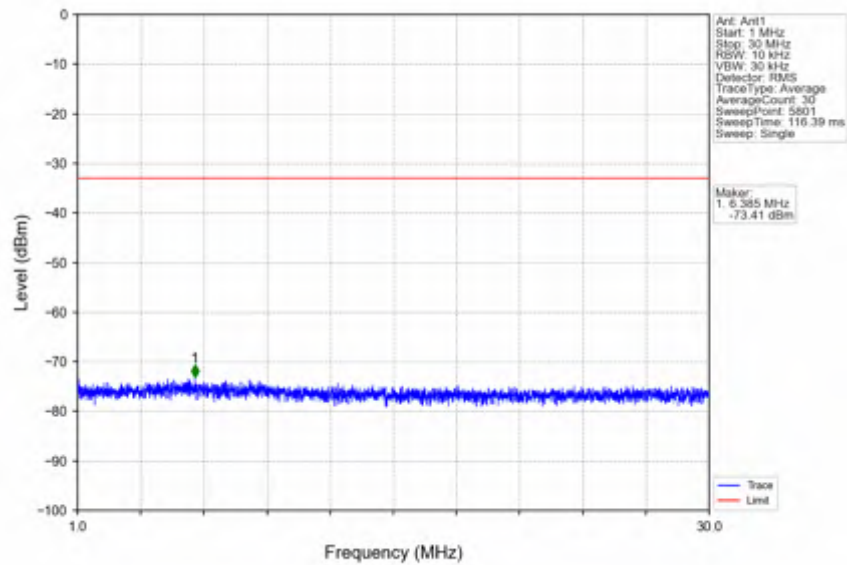
n41_15kHz_SISO_NTNV_50MHz_DFT-s-OFDM QPSK_2664.99MHz_Outer_Full
