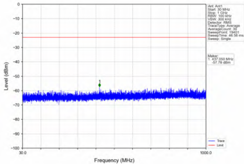
n41_15kHz_SISO_NTNV_40MHz_DFT-s-OFDM QPSK_2516.01MHz_Edge_1RB_Left
