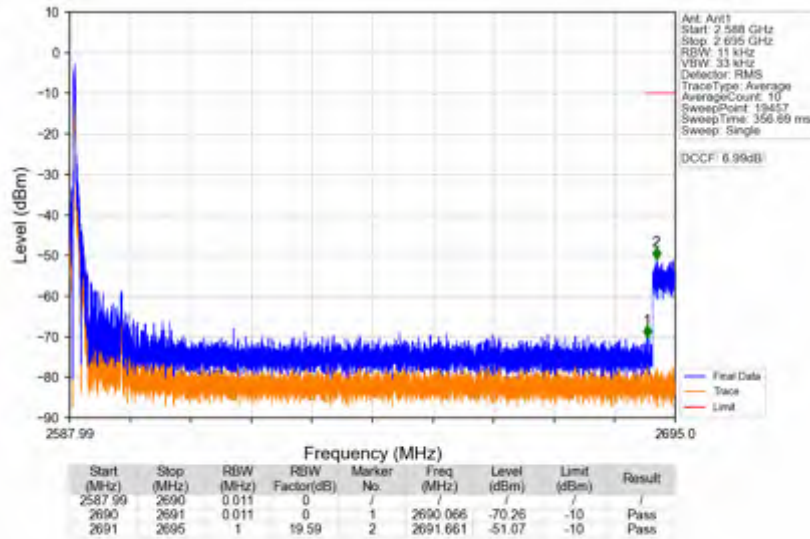
n41_30kHz_SISO_NTNV_10MHz_DFT-s-OFDM QPSK_2592.99MHz_Edge_1RB_Left
