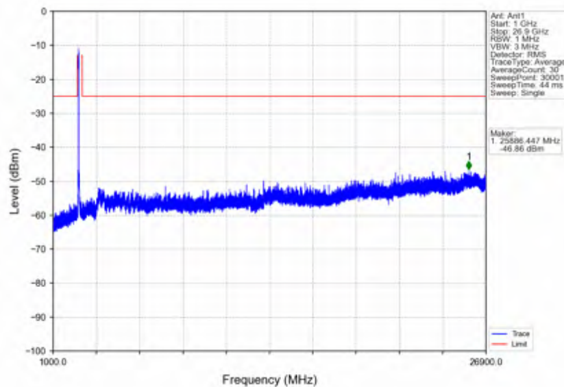
n41_15kHz_SISO_NTNV_50MHz_CP-OFDM QPSK_2521.005MHz_Outer_Full
