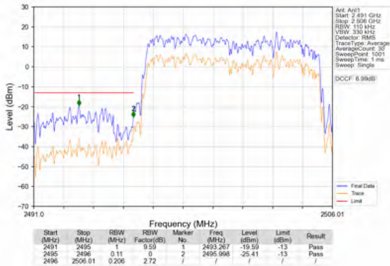
n41_30kHz_SISO_NTNV_10MHz_DFT-s-OFDM PI/2 BPSK_2501.01MHz_Outer_Full
