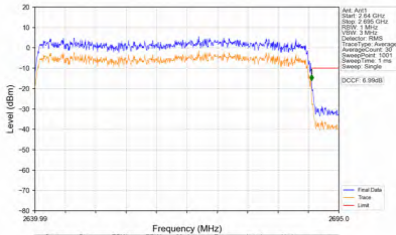
n41_15kHz_SISO_NTNV_50MHz_DFT-s-OFDM PI/2 BPSK_2664.99MHz_Outer_Full
