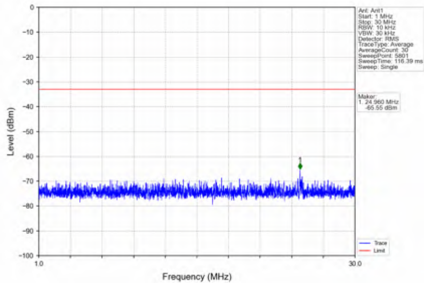
n41_30kHz_SISO_NTNV_15MHz_DFT-s-OFDM QPSK_2592.99MHz_Edge_1RB_Left
