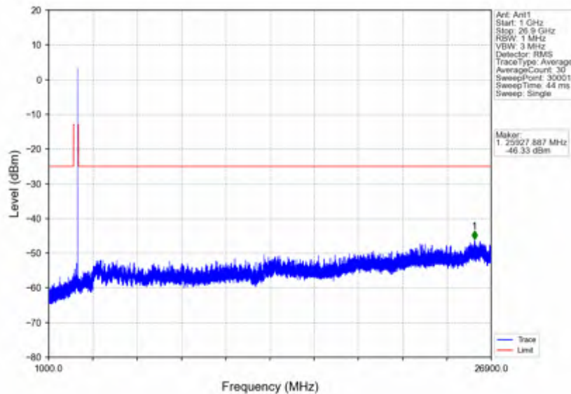
n41_15kHz_SISO_NTV_50MHz_DFT-s-OFDM QPSK_2664.99MHz_Inner_1RB_Right
