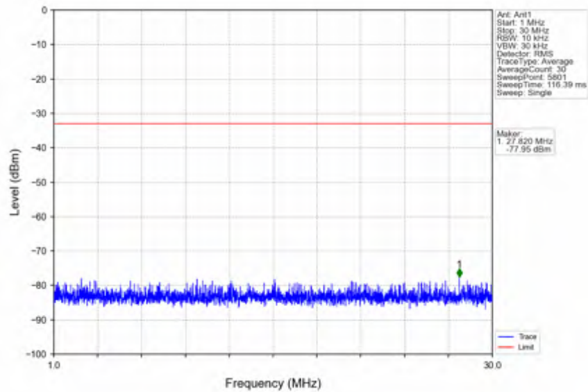
n41_30kHz_SISO_NTNV_10MHz_DFT-s-OFDM QPSK_2501.01MHz_Outer_Full
