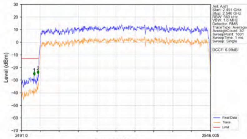
n41_15kHz_SISO_NTNV_50MHz_DFT-s-OFDM PI/2 BPSK_2521.005MHz_Outer_Full
