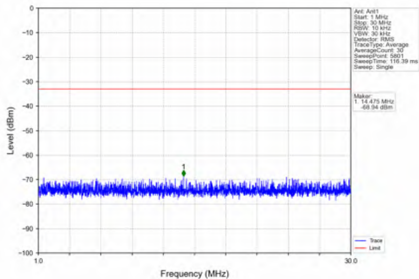
n41_15kHz_SISO_NTNV_40MHz_DFT-s-OFDM QPSK_2516.01MHz_Edge_1RB_Left
