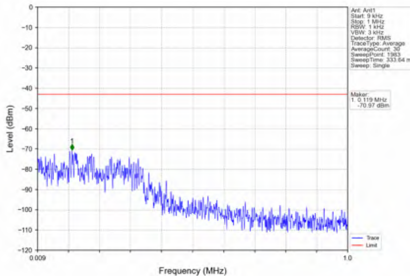
n41_30kHz_SISO_NTNV_15MHz_DFT-s-OFDM PI/2 BPSK_2682.48MHz_Edge_1RB_Right
