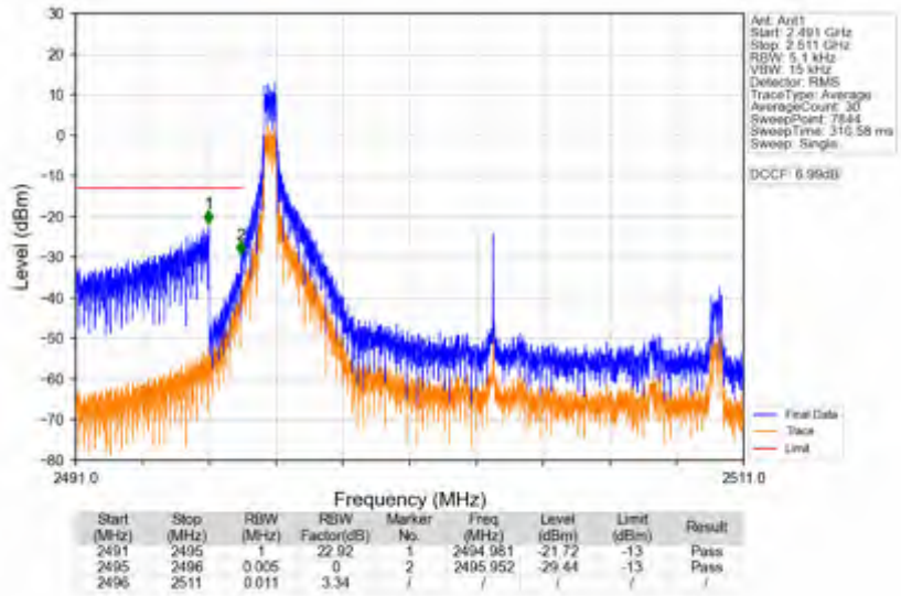
n41_30kHz_SISO_NTNV_15MHz_DFT-s-OFDM QPSK_2503.5MHz_Edge_1RB_Left
