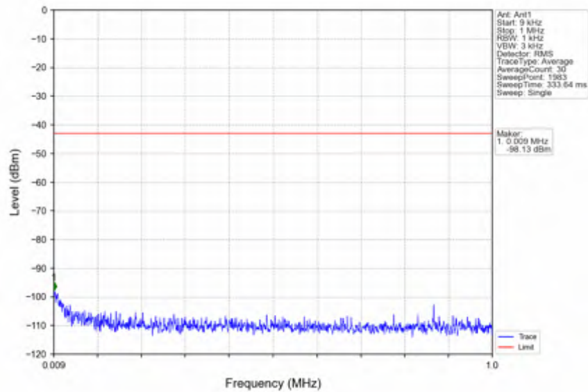
n41_15kHz_SISO_NTNV_50MHz_CP-OFDM QPSK_2521.005MHz_Outer_Full
