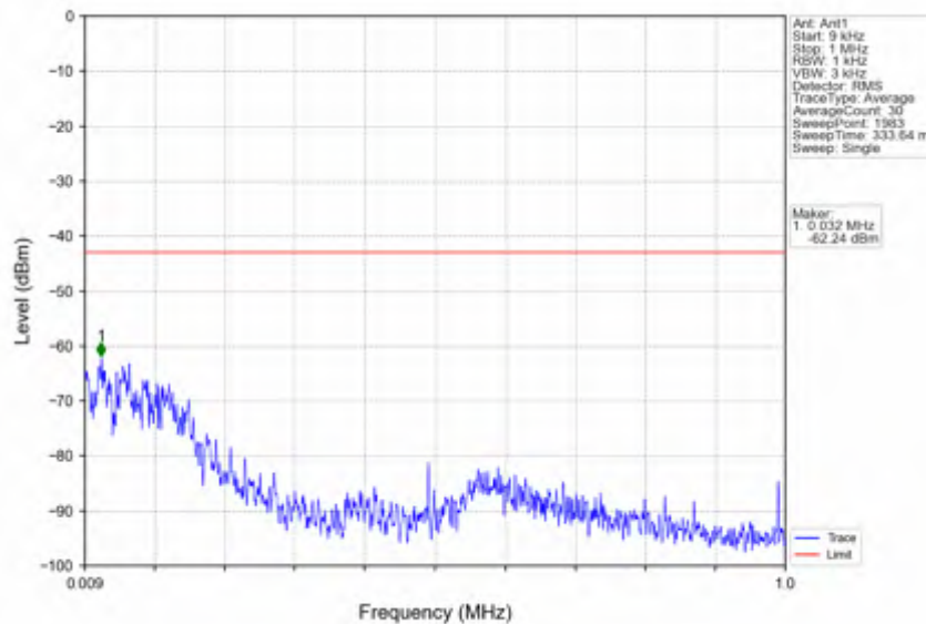
n41_15kHz_SISO_NTNV_40MHz_CP-OFDM QPSK_2670MHz_Edge_1RB_Right
