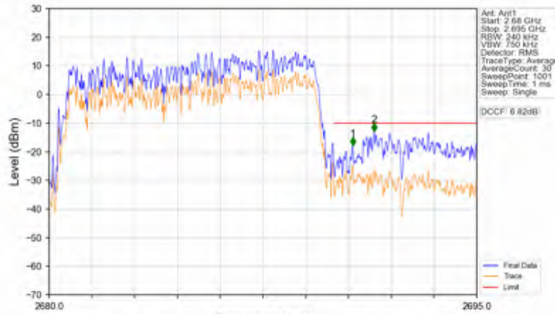
n41_30kHz_SISO_NTNV_10MHz_DFT-s-OFDM QPSK_2685MHz_Outer_Full
