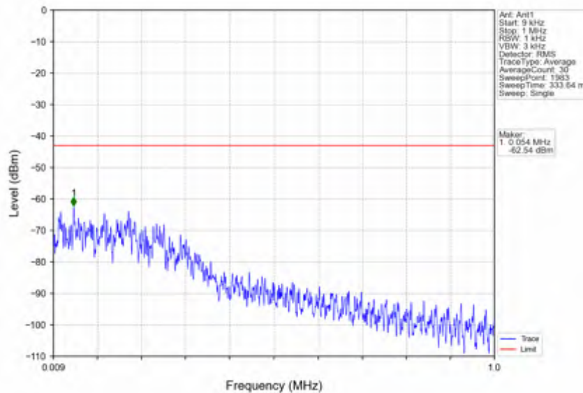
n41_30kHz_SISO_NTNV_10MHz_CP-OFDM QPSK_2685MHz_Edge_1RB_Right
