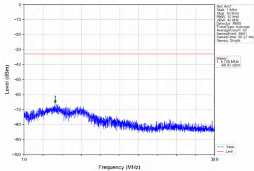
n41_15kHz_SISO_NTNV_40MHz_DFT-s-OFDM QPSK_2670MHz_Outer_Full
