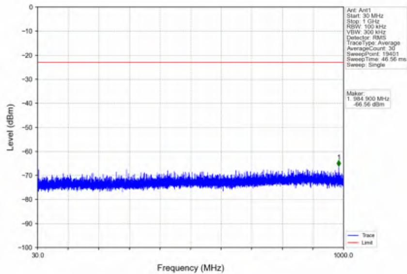
n41_30kHz_SISO_NTNV_10MHz_DFT-s-OFDM PI/2 BPSK_2501.01MHz_Outer_Full
