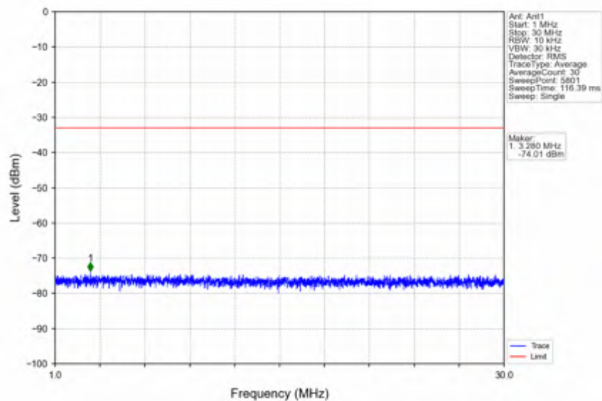
n41_15kHz_SISO_NTNV_50MHz_DFT-s-OFDM PI/2 BPSK_2664.99MHz_Outer_Full
