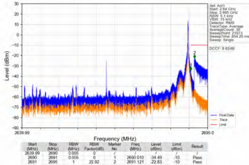
n41_15kHz_SISO_NTNV_50MHz_DFT-s-OFDM PI/2 BPSK_2664.99MHz_Edge_1RB_Right
