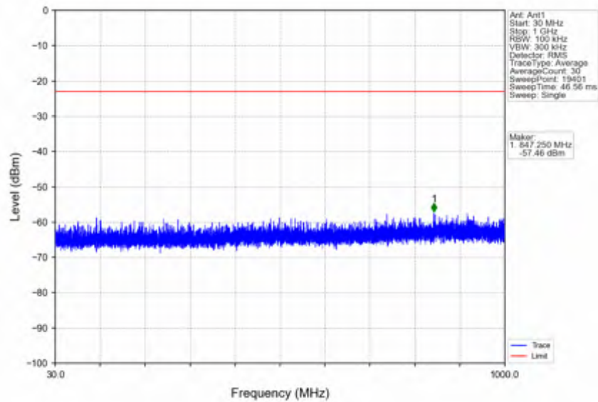
n41_15kHz_SISO_NTNV_40MHz_DFT-s-OFDM QPSK_2670MHz_Edge_1RB_Right
