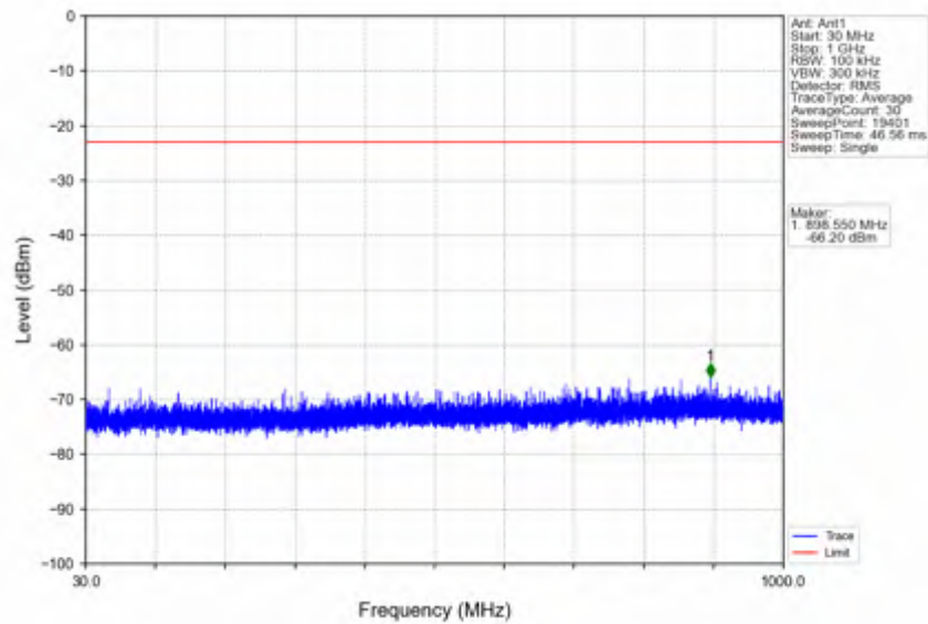
n41_30kHz_SISO_NTNV_15MHz_DFT-s-OFDM PI/2 BPSK_2503.5MHz_Outer_Full
