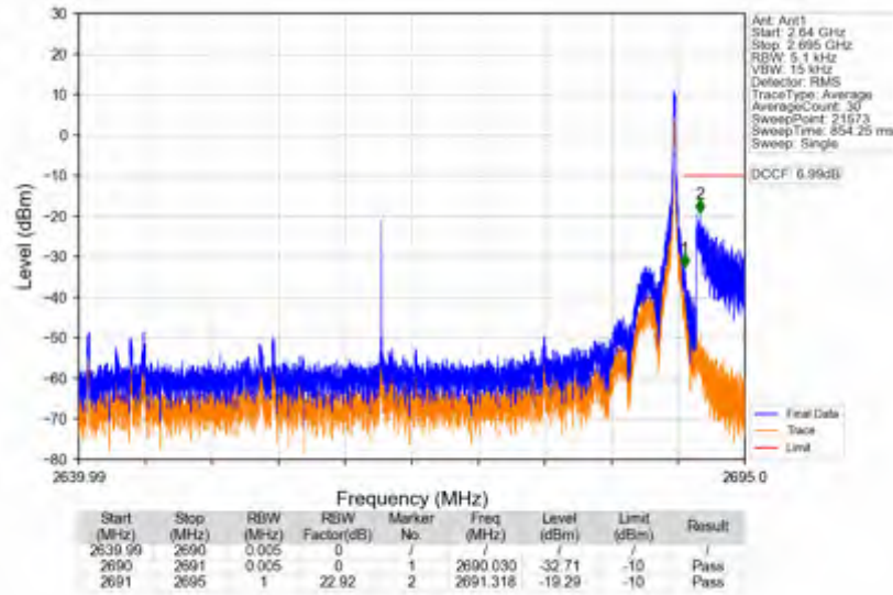
n41_15kHz_SISO_NTV_50MHz_CP-OFDM QPSK_2664.99MHz_Edge_1RB_Right
