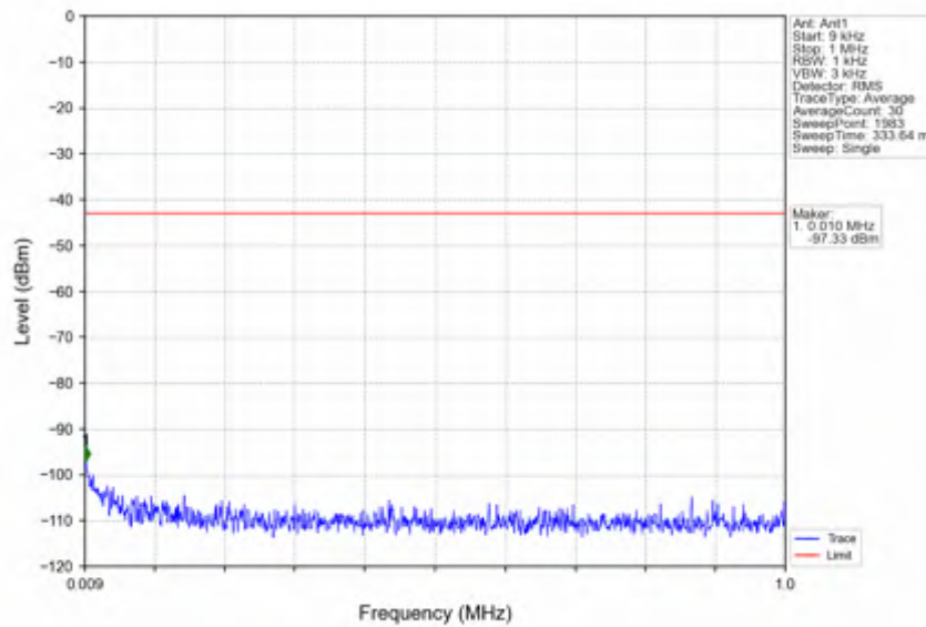
n41_15kHz_SISO_NTNV_50MHz_DFT-s-OFDM_QPSK_2521.005MHz_Outer_Full
