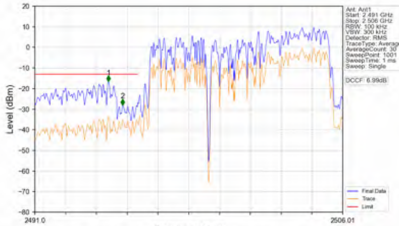
n41_30kHz_SISO_NTNV_10MHz_CP-OFDM QPSK_2501.01MHz_Outer_Full
