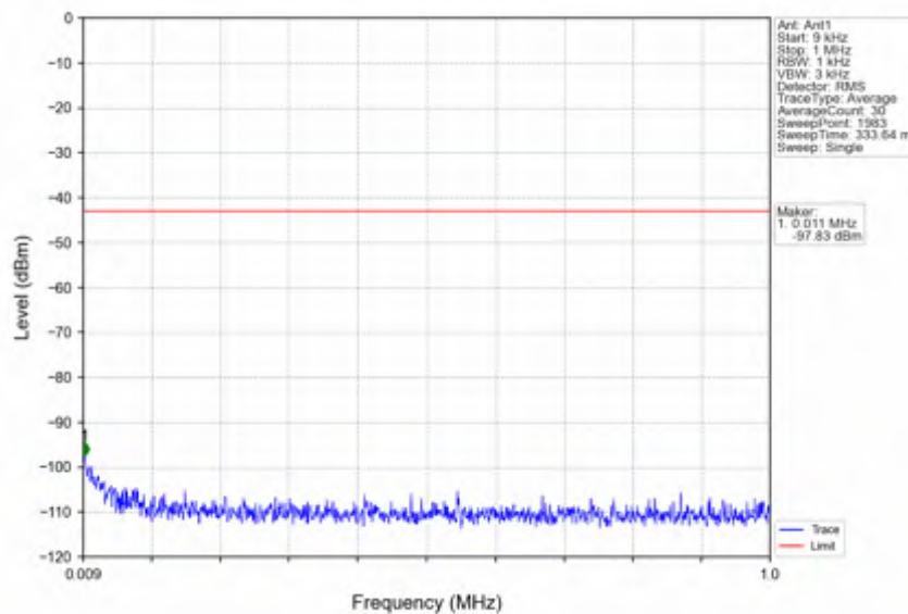
n41_15kHz_SISO_NTNV_40MHz_DFT-s-OFDM QPSK_2516.01MHz_Outer_Full
