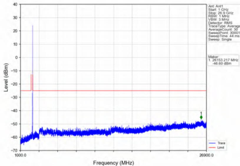
n41_30kHz_SISO_NTV_15MHz_DFT-s-OFDM_QPSK_2682.48MHz_Inner_1RB_Right
