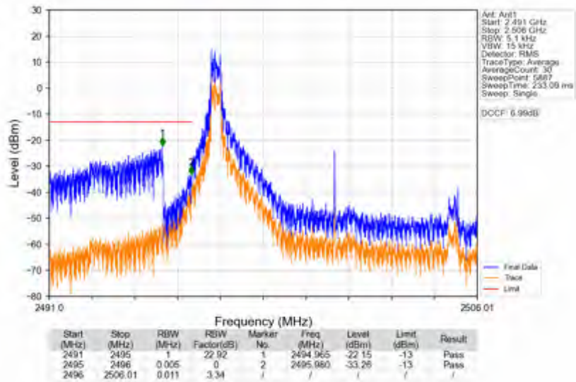
n41_30kHz_SISO_NTNV_10MHz_DFT-s-OFDM QPSK_2501.01MHz_Edge_1RB_Left
