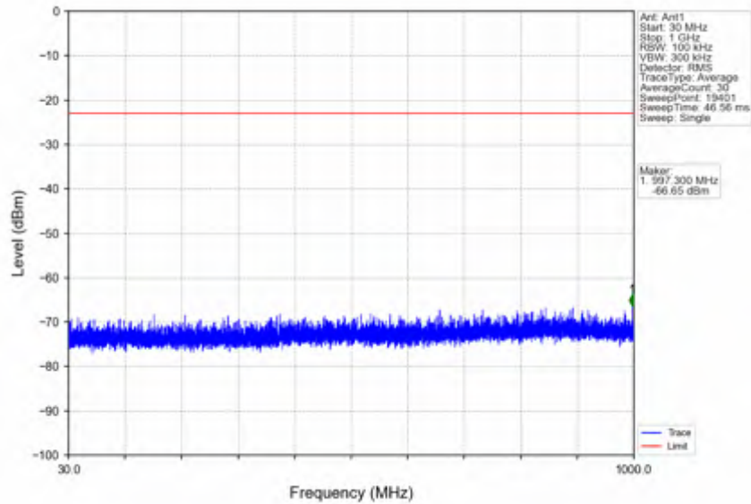
n41_15kHz_SISO_NTV_50MHz_DFT-s-OFDM QPSK_2664.99MHz_Inner_1RB_Right
