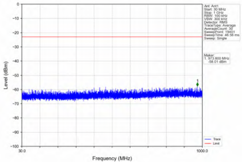
n41_30kHz_SISO_NTNV_10MHz_CP-OFDM QPSK_2501.01MHz_Edge_1RB_Left
