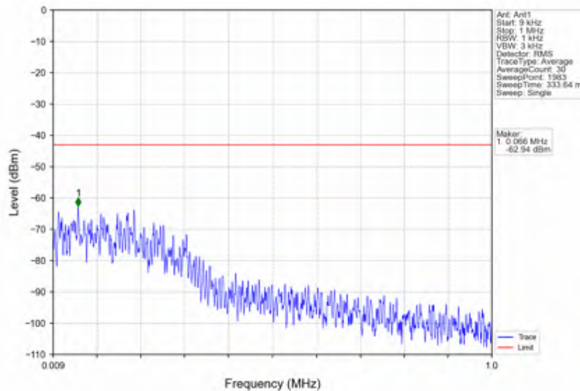
n41_30kHz_SISO_NTNV_10MHz_CP-OFDM QPSK_2501.01MHz_Edge_1RB_Left
