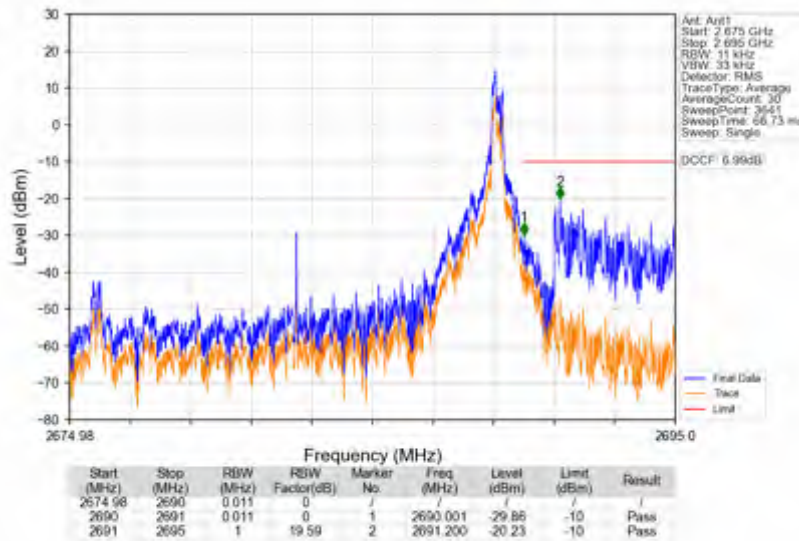
n41_30kHz_SISO_NTNV_15MHz_DFT-s-OFDM QPSK_2682.48MHz_Edge_1RB_Right
