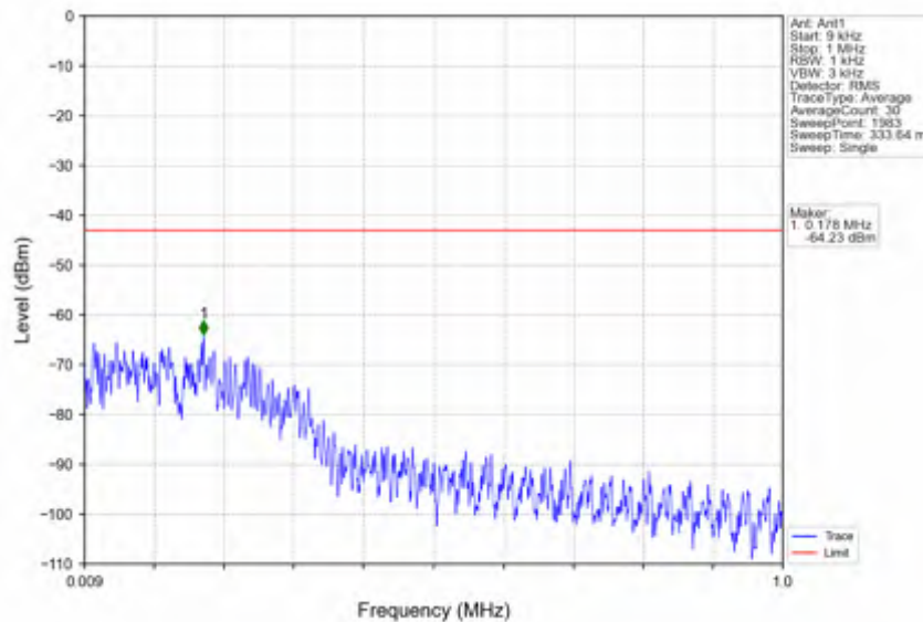
n41_30kHz_SISO_NTV_15MHz_CP-OFDM_QPSK_2503.5MHz_Edge_1RB_Left
