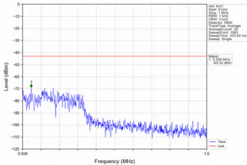
n41_30kHz_SISO_NTNV_15MHz_DFT-s-OFDM QPSK_2503.5MHz_Edge_1RB_Left
