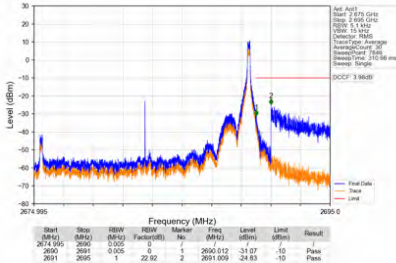
n41_15kHz_SISO_NTNV_15MHz_CP-OFDM QPSK_2682.495MHz_Edge_1RB_Right
