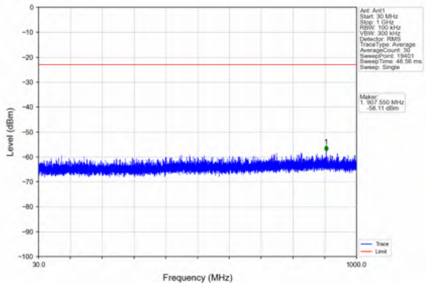
n41_15kHz_SISO_NTNV_30MHz_DFT-s-OFDM QPSK_2674.995MHz_Outer_Full
