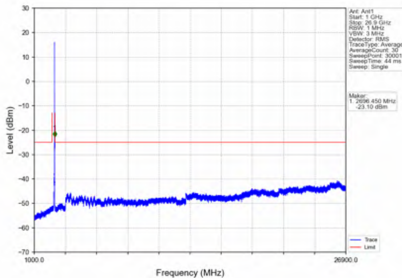
n41_15kHz_SISO_NTNV_20MHz_DFT-s-OFDM PI/2 BPSK_2679.99MHz_Outer_Full
