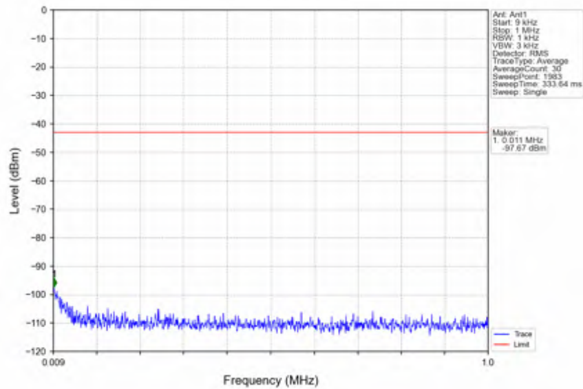
n41_15kHz_SISO_NTNV_15MHz_CP-OFDM QPSK_2682.495MHz_Outer_Full
