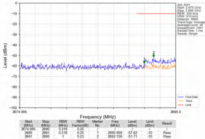
n41_15kHz_SISO_NTNV_15MHz_DFT-s-OFDM PI/2 BPSK_2682.495MHz_Outer_Full
