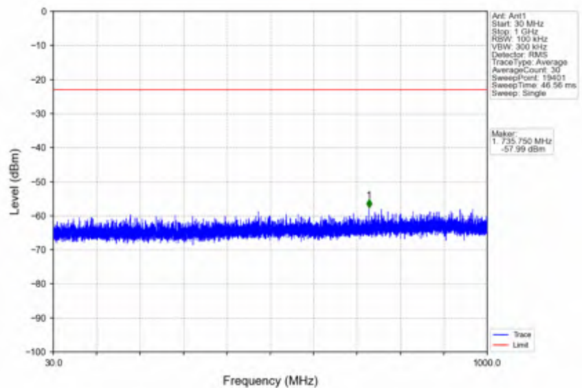
n41_15kHz_SISO_NTNV_20MHz_DFT-s-OFDM QPSK_2506.005MHz_Outer_Full
