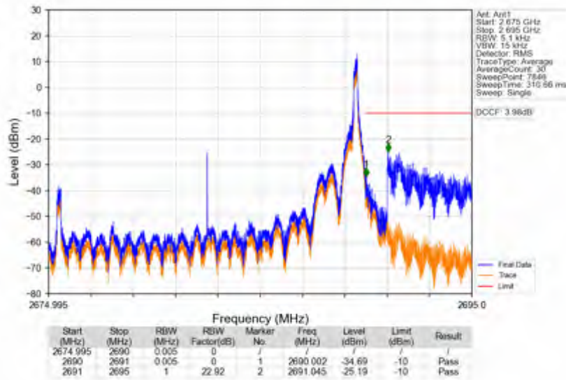
n41_15kHz_SISO_NTNV_15MHz_DFT-s-OFDM QPSK_2682.495MHz_Edge_1RB_Right
