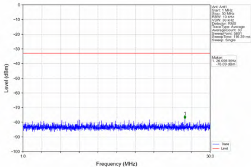
n41_15kHz_SISO_NTNV_15MHz_DFT-s-OFDM PI/2 BPSK_2682.495MHz_Outer_Full
