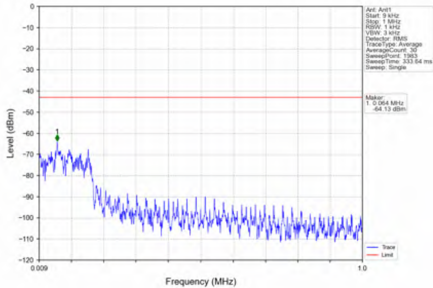
n41_15kHz_SISO_NTNV_15MHz_DFT-s-OFDM QPSK_2503.5MHz_Edge_1RB_Left
