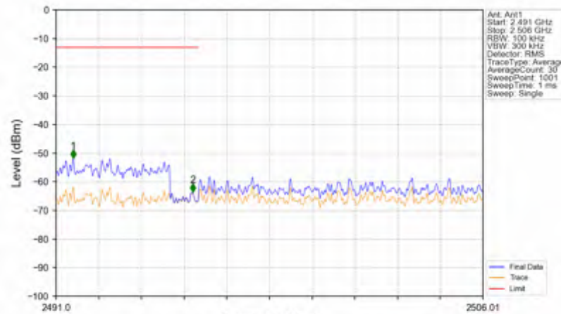
n41_15kHz_SISO_NTNV_10MHz_CP-OFDM QPSK_2501.01MHz_Outer_Full
