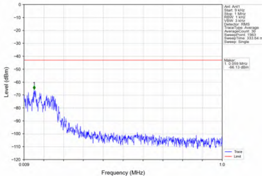
n41_15kHz_SISO_NTNV_20MHz_DFT-s-OFDM PI/2 BPSK_2679.99MHz_Edge_1RB_Right
