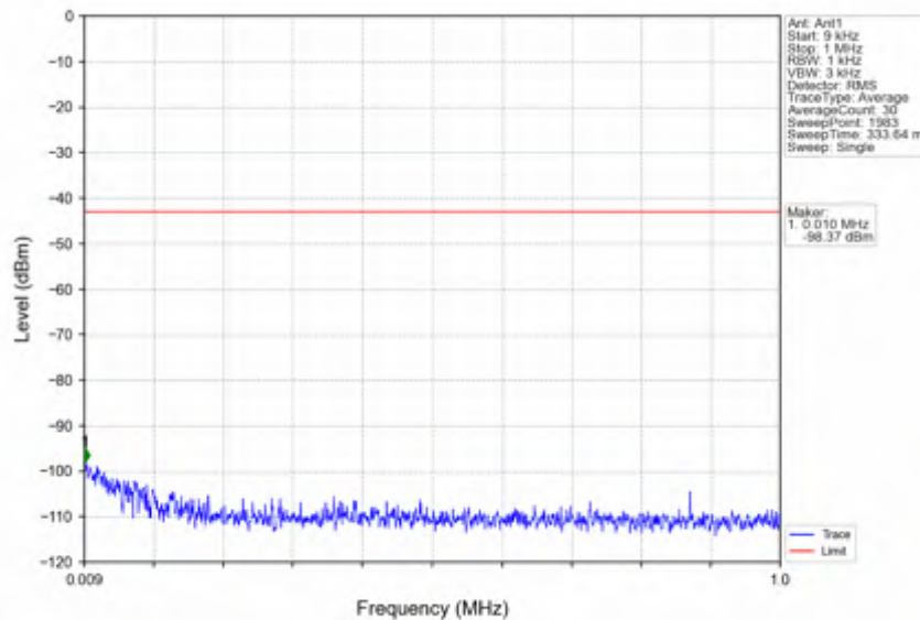
n41_15kHz_SISO_NTNV_15MHz_CP-OFDM QPSK_2682.495MHz_Inner_1RB_Right
