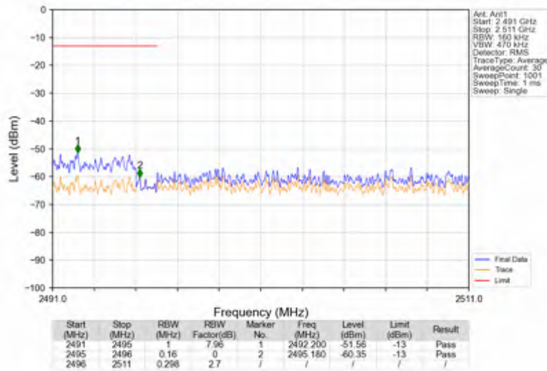
n41_15kHz_SISO_NTNV_15MHz_DFT-s-OFDM PI/2 BPSK_2503.5MHz_Outer_Full
