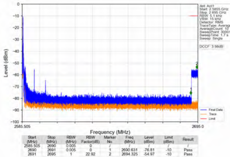
n41_15kHz_SISO_NTNV_15MHz_DFT-s-OFDM PI/2 BPSK_2593.005MHz_Edge_1RB_Left
