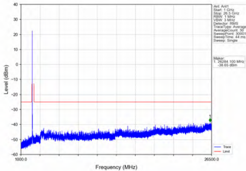
n41_15kHz_SISO_NTNV_40MHz_DFT-s-OFDM PI/2 BPSK_2516.01MHz_Outer_Full
