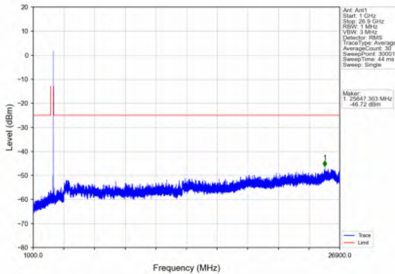
n41_15kHz_SISO_NTNV_30MHz_DFT-s-OFDM PI/2 BPSK_2674.995MHz_Outer_Full
