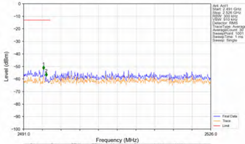
n41_15kHz_SISO_NTNV_30MHz_CP-OFDM QPSK_2511MHz_Outer_Full
