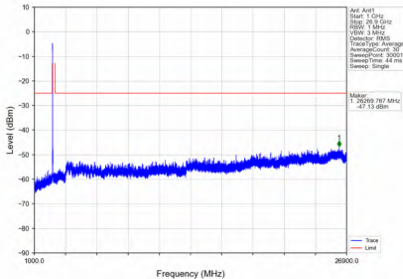
n41_15kHz_SISO_NTNV_20MHz_DFT-s-OFDM PI/2 BPSK_2506.005MHz_Outer_Full
