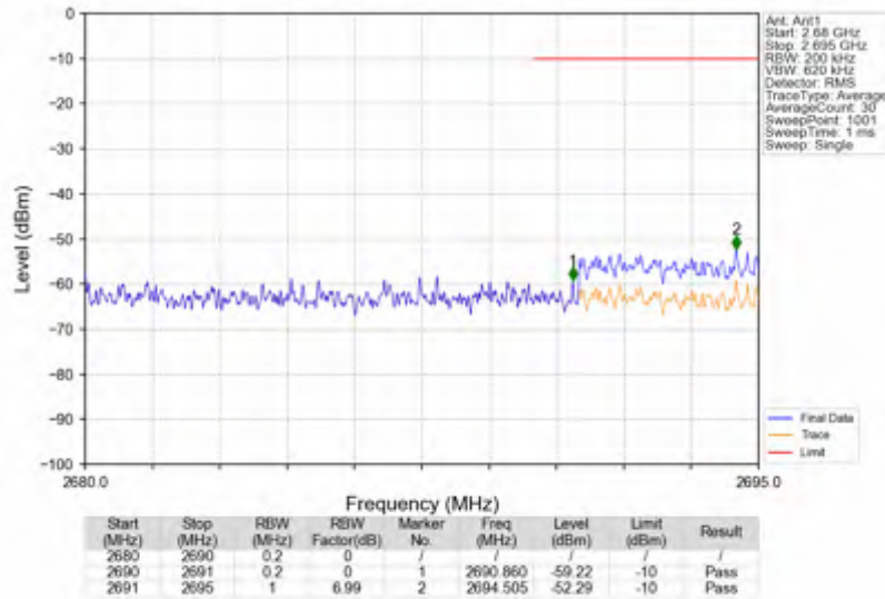
n41_15kHz_SISO_NTNV_10MHz_CP-OFDM QPSK_2685MHz_Outer_Full
