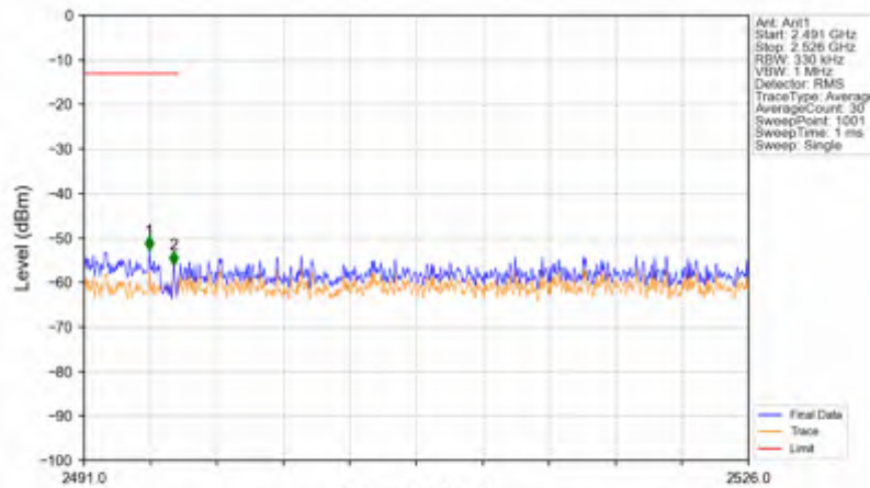
n41_15kHz_SISO_NTNV_30MHz_DFT-s-OFDM PI/2 BPSK_2511MHz_Outer_Full
