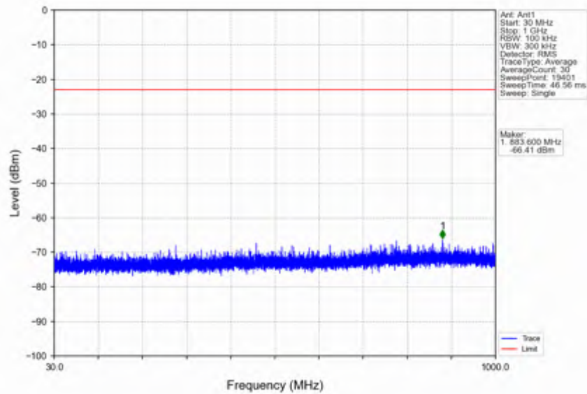
n41_15kHz_SISO_NTNV_15MHz_DFT-s-OFDM QPSK_2682.495MHz_Inner_1RB_Right
