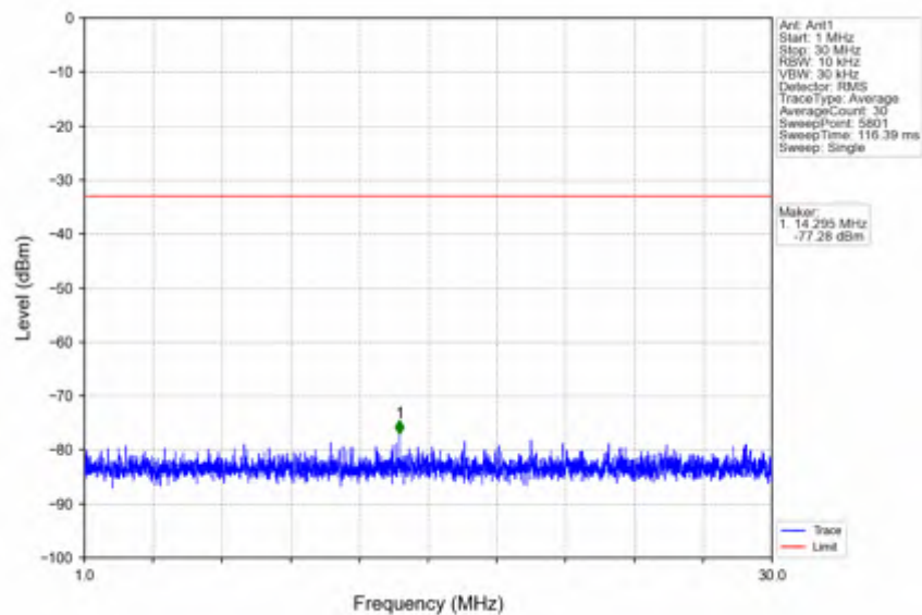
n41_15kHz_SISO_NTNV_20MHz_DFT-s-OFDM PI/2 BPSK_2506.005MHz_Outer_Full
