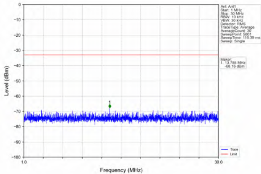
n41_15kHz_SISO_NTNV_30MHz_CP-OFDM QPSK_2674.995MHz_Edge_1RB_Right
