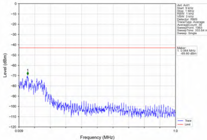
n41_15kHz_SISO_NTNV_40MHz_DFT-s-OFDM PI/2 BPSK_2670MHz_Edge_1RB_Right
