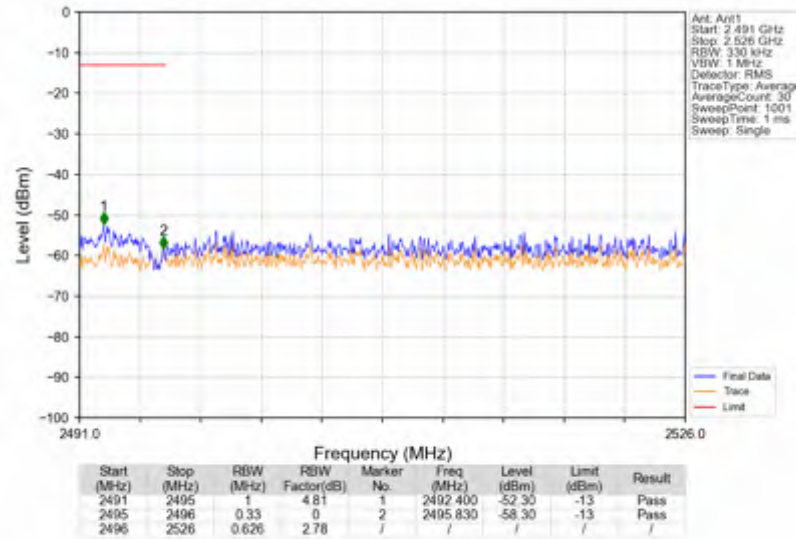
n41_15kHz_SISO_NTNV_30MHz_DFT-s-OFDM QPSK_2511MHz_Outer_Full
