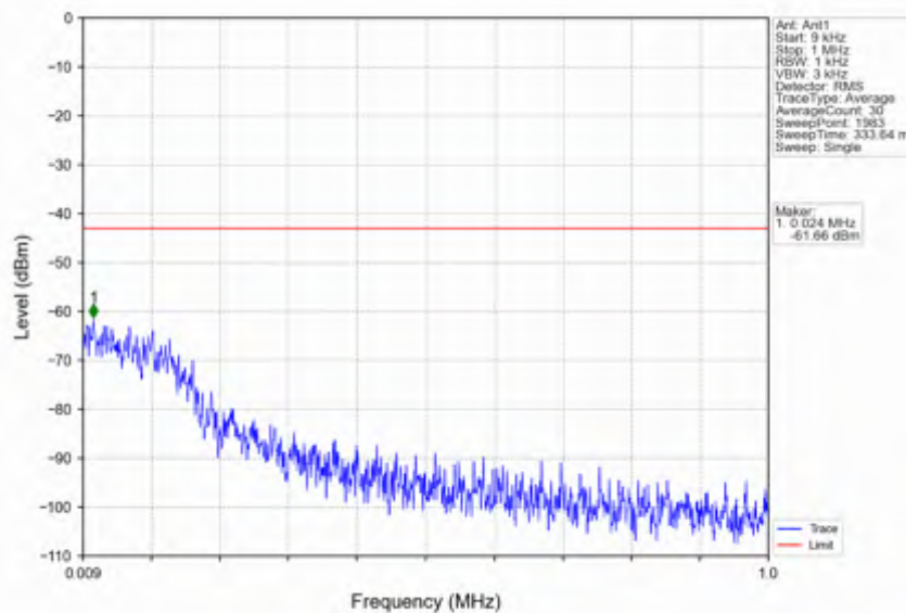
n41_15kHz_SISO_NTNV_30MHz_CP-OFDM QPSK_2674.995MHz_Edge_1RB_Right
