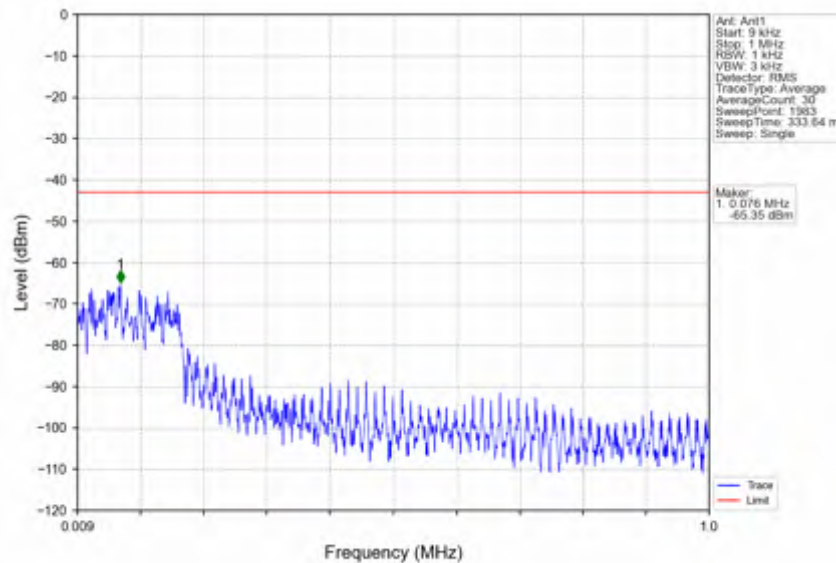
n41_15kHz_SISO_NTNV_30MHz_DFT-s-OFDM_QPSK_2593.005MHz_Edge_1RB_Left
