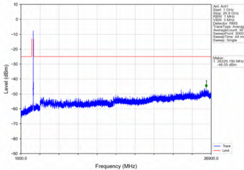
n41_15kHz_SISO_NTNV_30MHz_DFT-s-OFDM QPSK_2674.995MHz_Inner_1RB_Right
