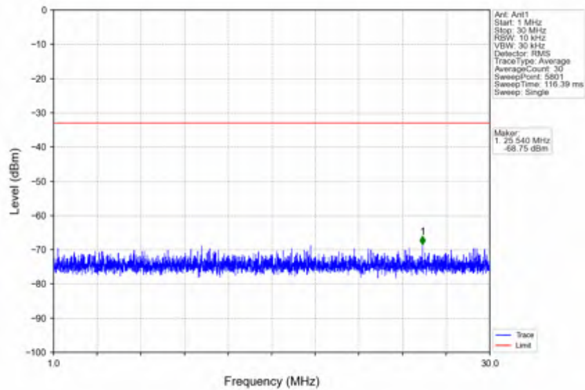
n41_15kHz_SISO_NTNV_15MHz_DFT-s-OFDM_PI/2_BPSK_2682.495MHz_Edge_1RB_Right
