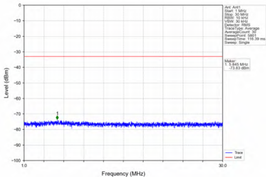
n41_15kHz_SISO_NTNV_20MHz_DFT-s-OFDM PI/2 BPSK_2679.99MHz_Outer_Full
