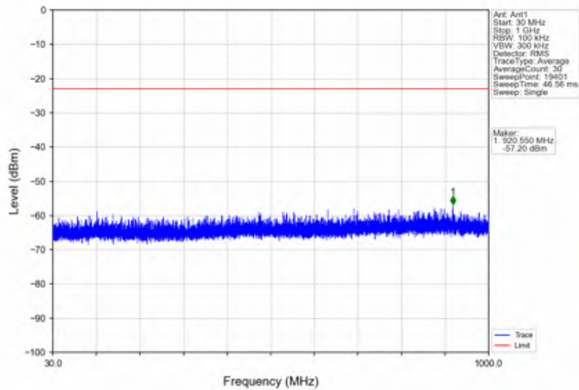
n41_15kHz_SISO_NTNV_15MHz_DFT-s-OFDM QPSK_2682.495MHz_Edge_1RB_Right
