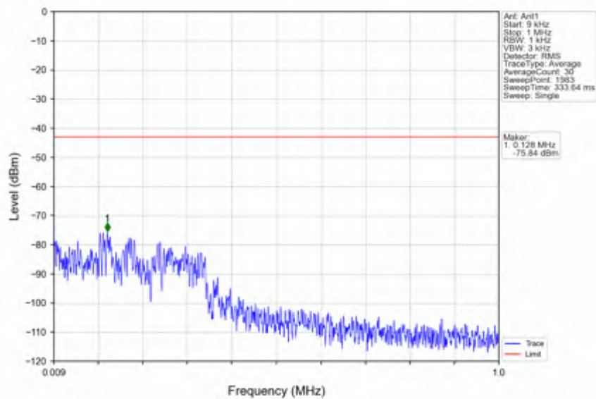
n38_30kHz_SISO_NTNV_10MHz_DFT-s-OFDM PI/2 BPSK_2575MHz_Edge_1RB_Left
