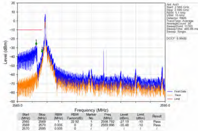
n38_15kHz_SISO_NTNV_25MHz_DFT-s-OFDM QPSK_2582.5MHz_Edge_1RB_Left
