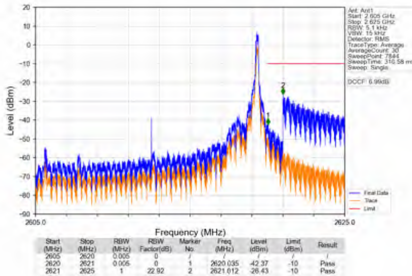
n38_15kHz_SISO_NTNV_15MHz_DFT-s-OFDM PI/2 BPSK_2612.5MHz_Inner_1RB_Right
