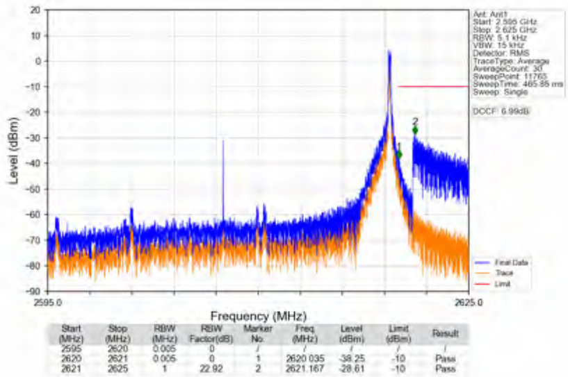
n38_15kHz_SISO_NTNV_25MHz_CP-OFDM QPSK_2607.5MHz_Edge_1RB_Right
