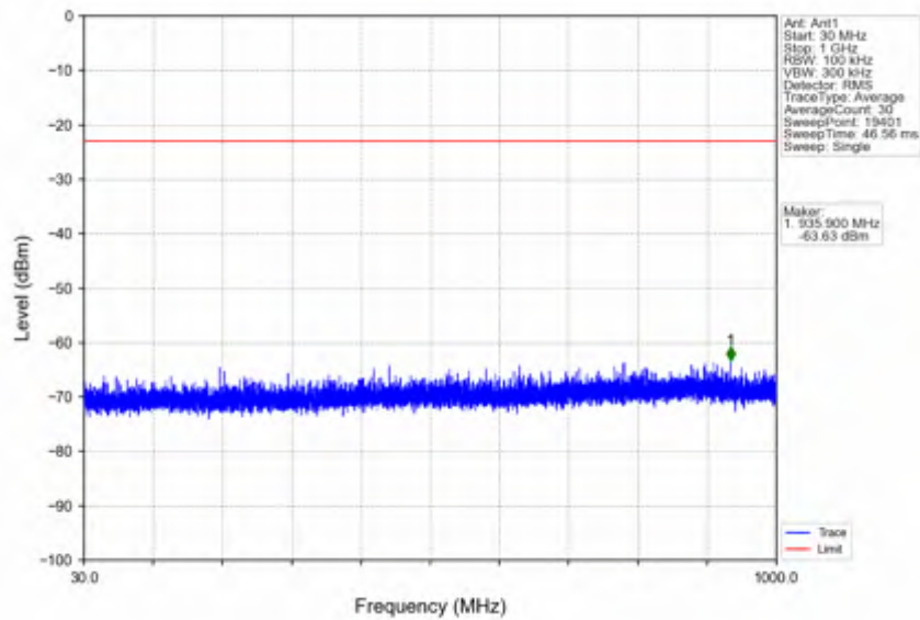
n38_15kHz_SISO_NTNV_40MHz_DFT-s-OFDM QPSK_2600MHz_Edge_1RB_Right
