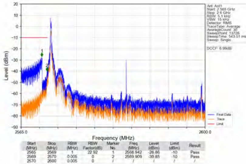
n38_15kHz_SISO_NTNV_30MHz_DFT-s-OFDM_PI/2_BPSK_2585MHz_Edge_1RB_Left
