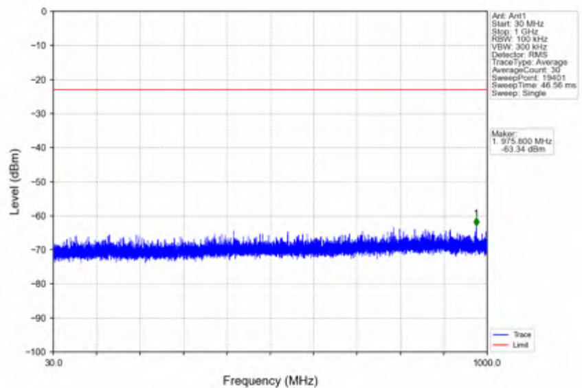
n38_15kHz_SISO_NTNV_30MHz_CP-OFDM QPSK_2585MHz_Edge_1RB_Left
