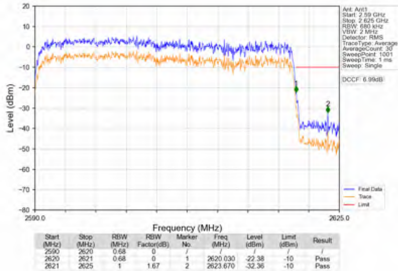
n38_15kHz_SISO_NTNV_30MHz_DFT-s-OFDM QPSK_2605MHz_Outer_Full
