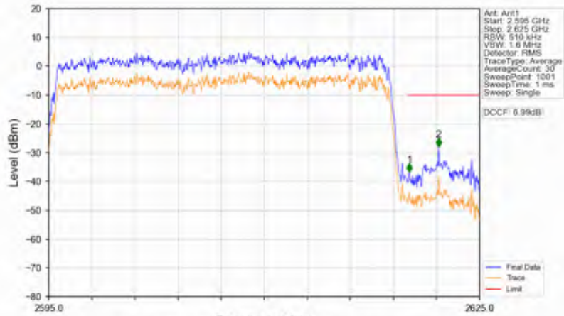
n38_15kHz_SISO_NTNV_25MHz_DFT-s-OFDM QPSK_2607.5MHz_Outer_Full
