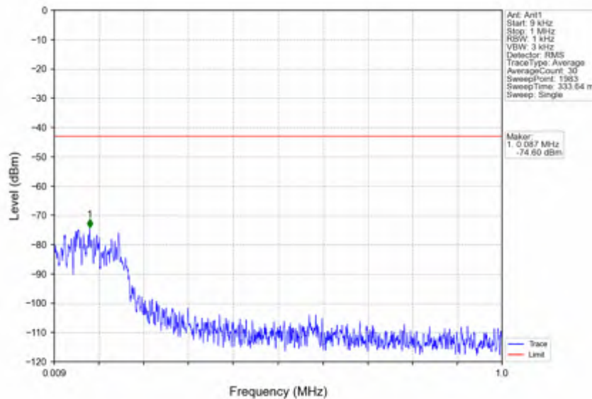
n38_15kHz_SISO_NTNV_25MHz_DFT-s-OFDM QPSK_2595MHz_Edge_1RB_Left
