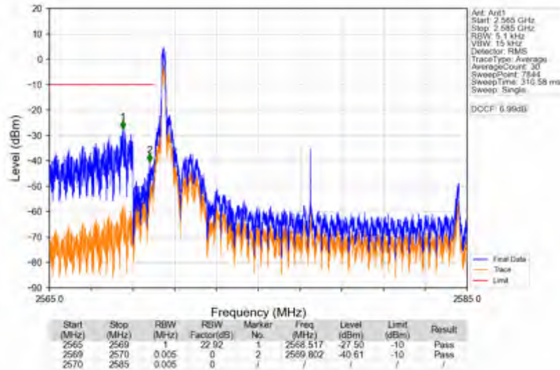
n38_15kHz_SISO_NTV_15MHz_CP-OFDM QPSK_2577.5MHz_Edge_1RB_Left
