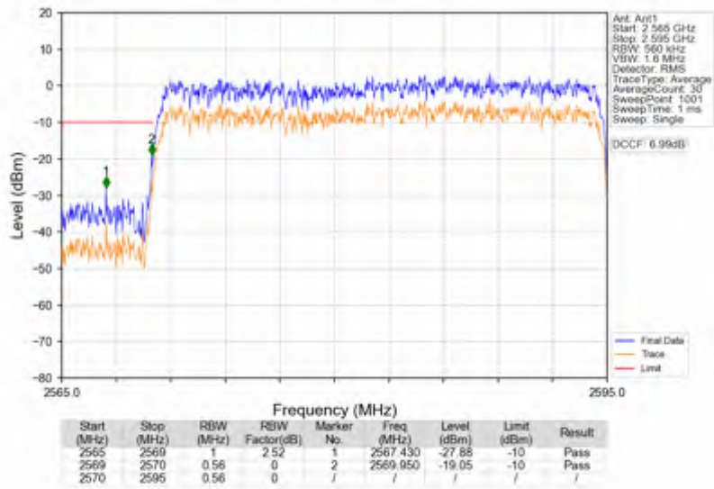
n38_15kHz_SISO_NTV_25MHz_CP-OFDM QPSK_2582.5MHz_Outer_Full
