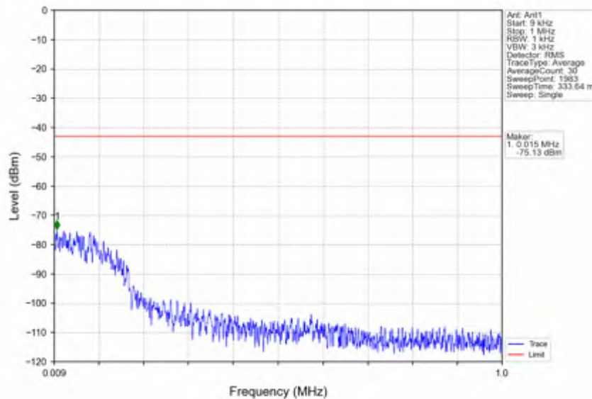
n38_15kHz_SISO_NTV_25MHz_CP-OFDM QPSK_2582.5MHz_Edge_1RB_Left
