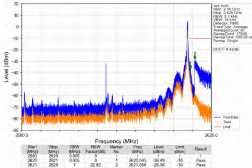
n38_15kHz_SISO_NTNV_40MHz_DFT-s-OFDM QPSK_2600MHz_Edge_1RB_Right
