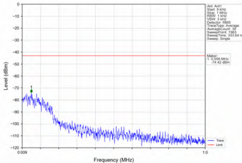
n38_15kHz_SISO_NTV_15MHz_CP-OFDM QPSK_2577.5MHz_Edge_1RB_Left
