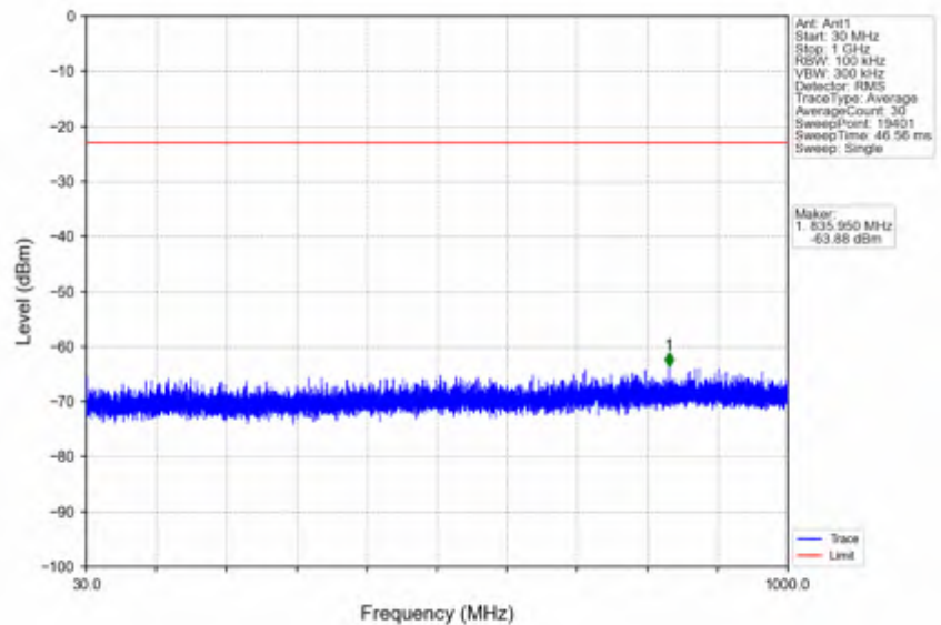
n38_15kHz_SISO_NTVV_25MHz_CP-OFDM QPSK_2582.5MHz_Edge_1RB_Left
