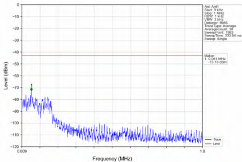
n38_15kHz_SISO_NTNV_30MHz_DFT-s-OFDM_PI/2_BPSK_2585MHz_Edge_1RB_Left
