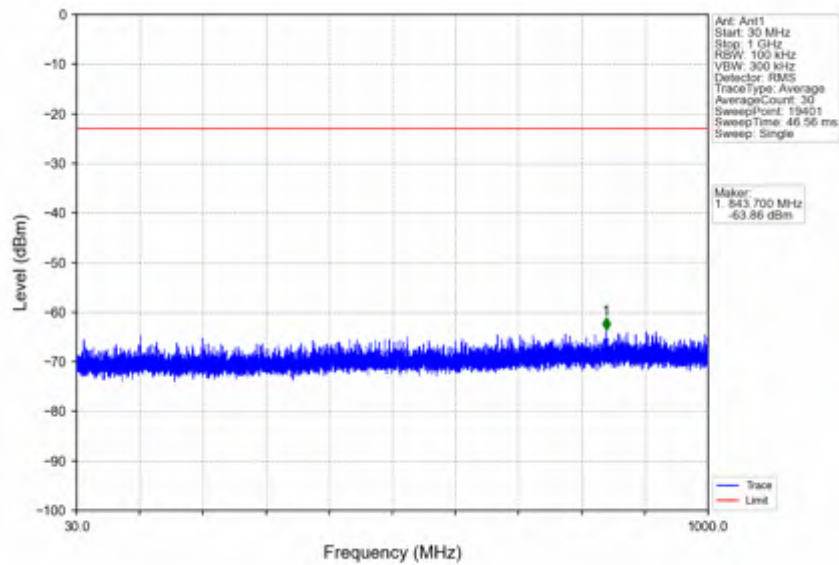
n38_15kHz_SISO_NTV_15MHz_CP-OFDM QPSK_2612.5MHz_Edge_1RB_Right
