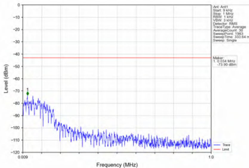
n38_15kHz_SISO_NTNV_30MHz_CP-OFDM QPSK_2585MHz_Edge_1RB_Left
