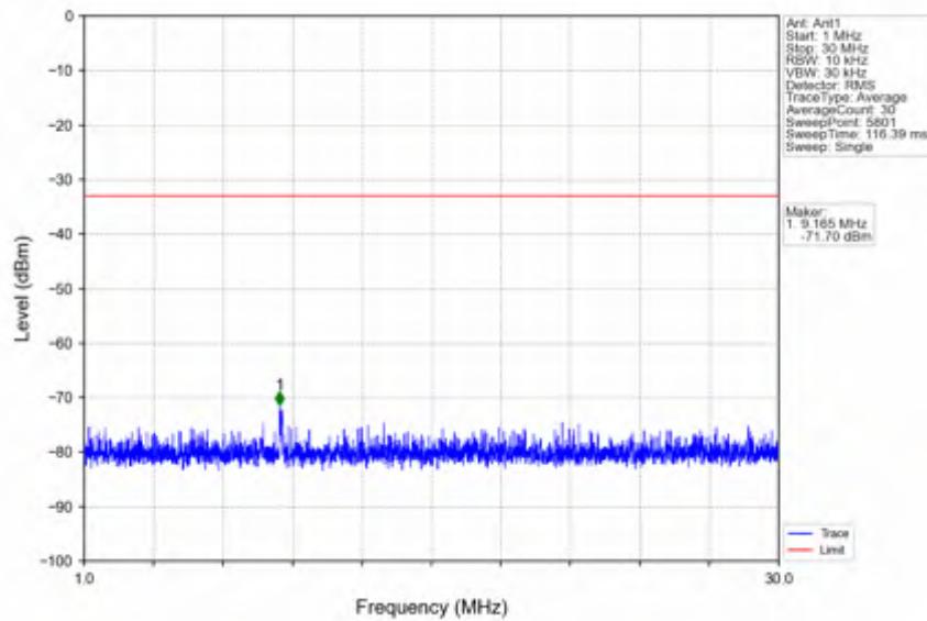
n38_15kHz_SISO_NTNV_15MHz_DFT-s-OFDM QPSK_2577.5MHz_Edge_1RB_Left
