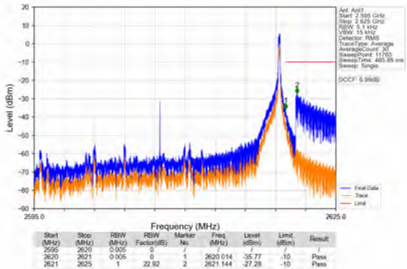
n38_15kHz_SISO_NTNV_25MHz_DFT-s-OFDM QPSK_2607.5MHz_Edge_1RB_Right
