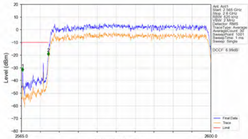
n38_15kHz_SISO_NTNV_30MHz_DFT-s-OFDM PI/2 BPSK_2585MHz_Outer_Full
