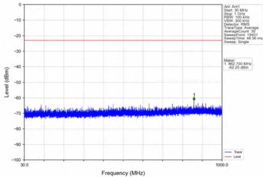
n38_15kHz_SISO_NTNV_30MHz_DFT-s-OFDM QPSK_2605MHz_Edge_1RB_Right
