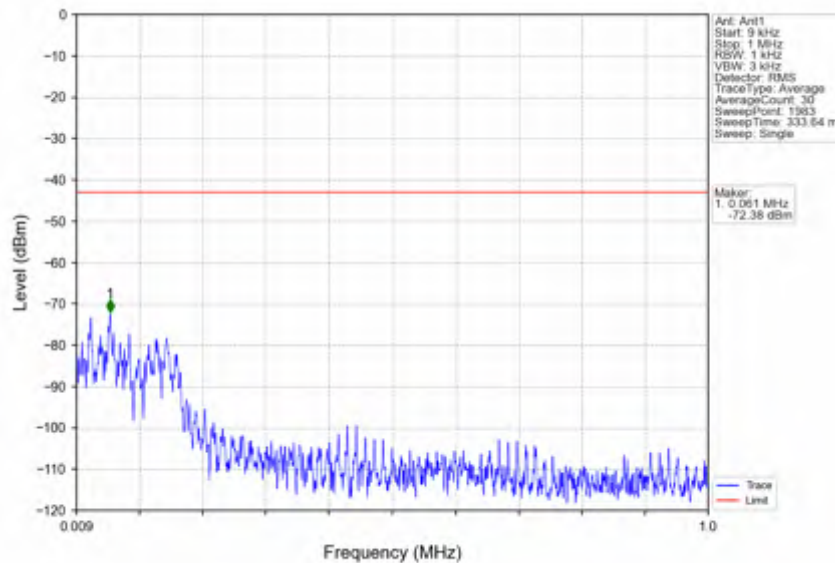
n38_15kHz_SISO_NTNV_30MHz_DFT-s-OFDM PI/2 BPSK_2595MHz_Edge_1RB_Left
