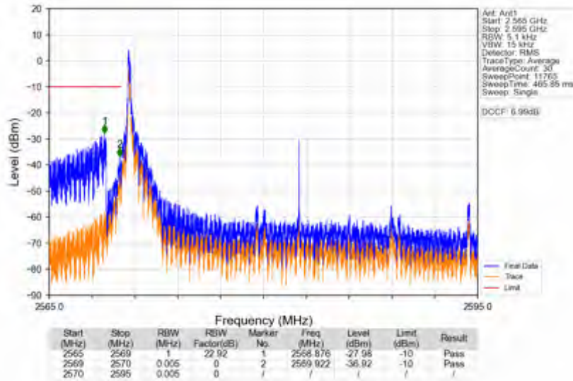
n38_15kHz_SISO_NTV_25MHz_CP-OFDM QPSK_2582.5MHz_Edge_1RB_Left
