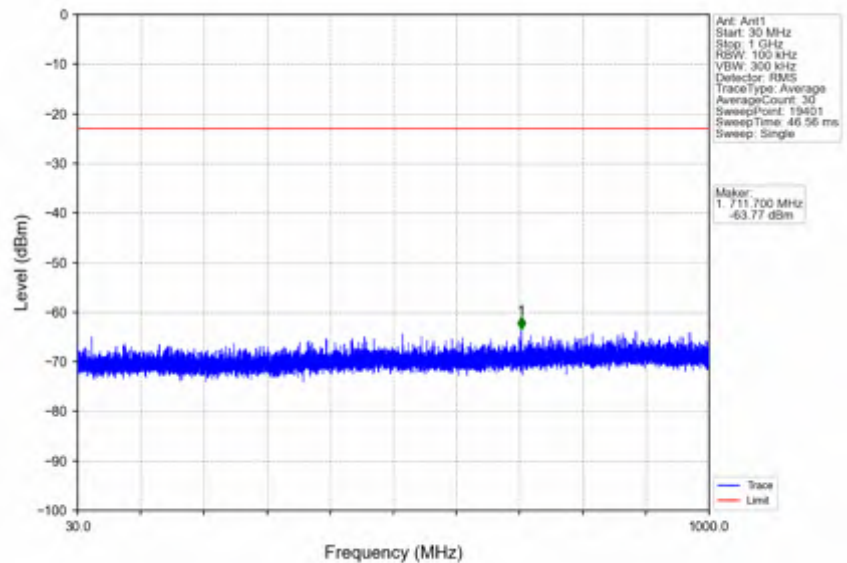
n38_15kHz_SISO_NTNV_25MHz_DFT-s-OFDM QPSK_2595MHz_Edge_1RB_Left
