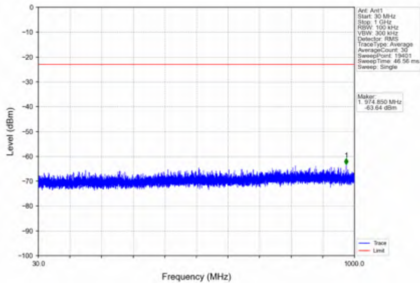
n38_15kHz_SISO_NTNV_25MHz_DFT-s-OFDM QPSK_2607.5MHz_Edge_1RB_Right
