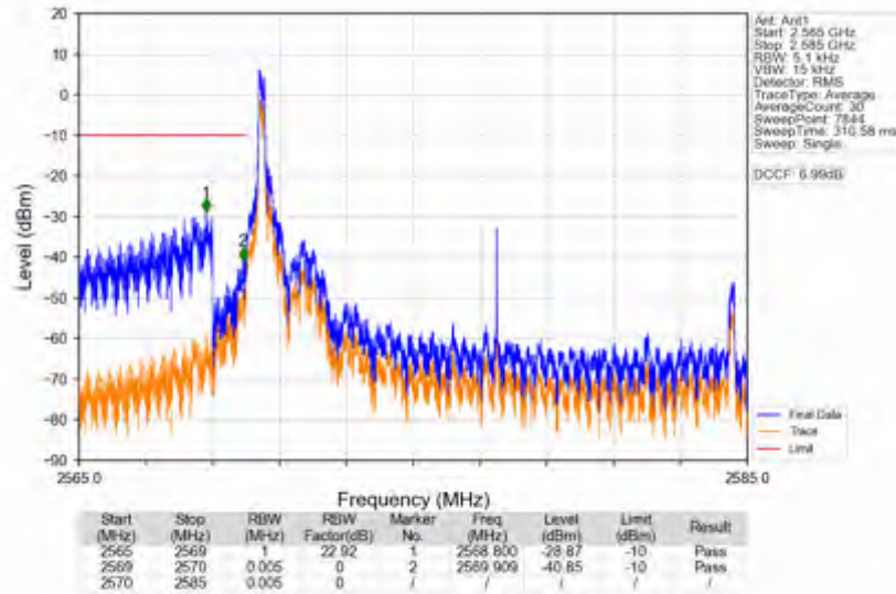
n38_15kHz_SISO_NTNV_15MHz_DFT-s-OFDM QPSK_2577.5MHz_Edge_1RB_Left
