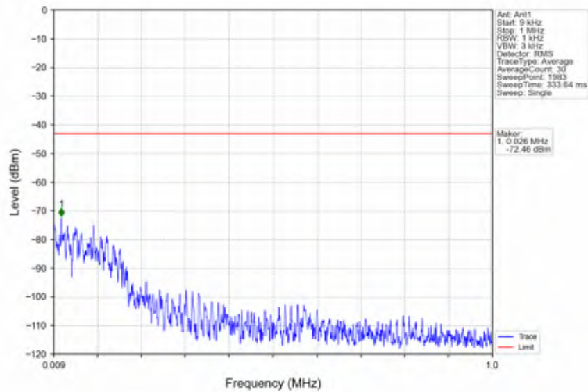
n38_15kHz_SISO_NTV_15MHz_CP-OFDM QPSK_2612.5MHz_Edge_1RB_Right
