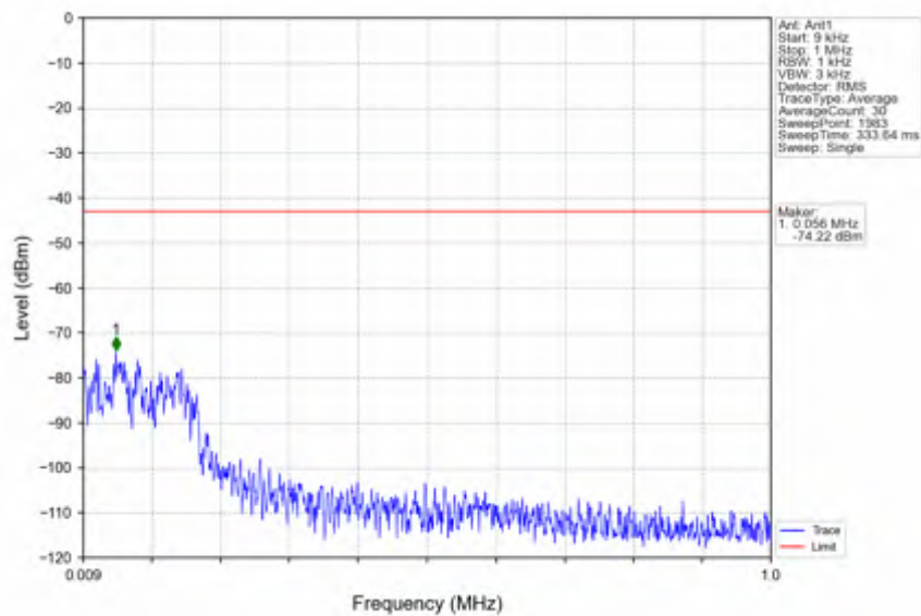
n38_15kHz_SISO_NTNV_10MHz_DFT-s-OFDM_PI/2_BPSK_2575MHz_Edge_1RB_Left
