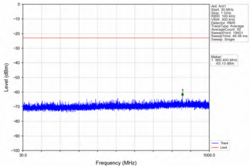
n38_15kHz_SISO_NTNV_25MHz_CP-OFDM QPSK_2595MHz_Edge_1RB_Left
