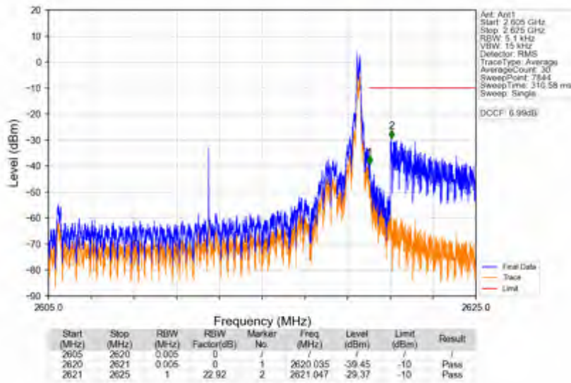
n38_15kHz_SISO_NTNV_15MHz_CP-OFDM QPSK_2612.5MHz_Edge_1RB_Right
