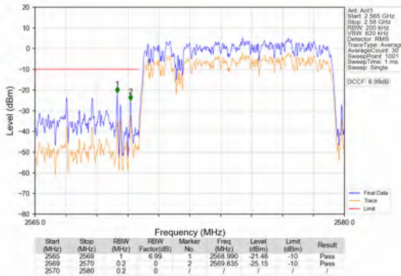
n38_15kHz_SISO_NTNV_10MHz_DFT-s-OFDM QPSK_2575MHz_Outer_Full
