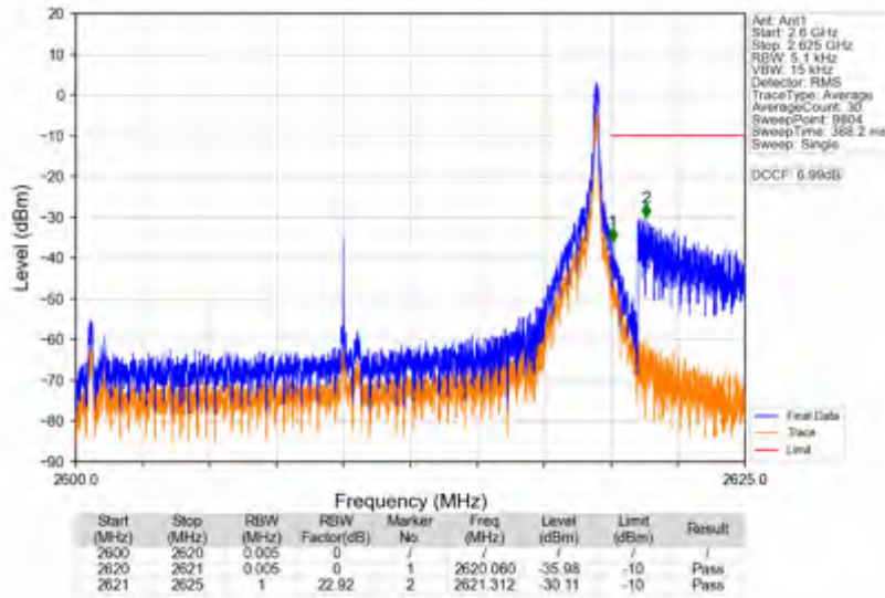
n38_15kHz_SISO_NTNV_20MHz_CP-OFDM QPSK_2610MHz_Edge_1RB_Right
