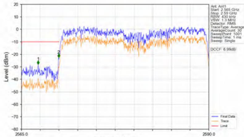
n38_15kHz_SISO_NTNV_20MHz_CP-OFDM QPSK_2580MHz_Outer_Full
