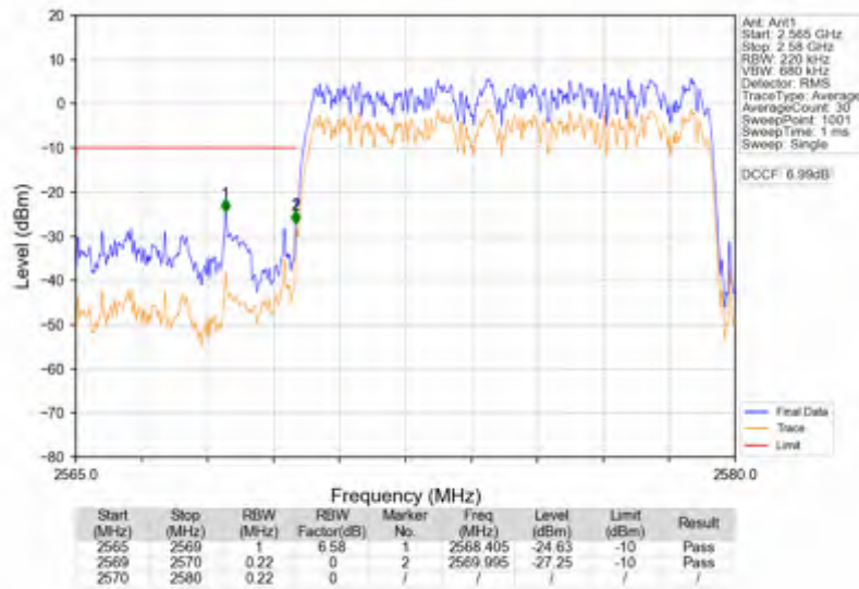
n38_15kHz_SISO_NTNV_10MHz_DFT-s-OFDM PI/2 BPSK_2575MHz_Outer_Full
