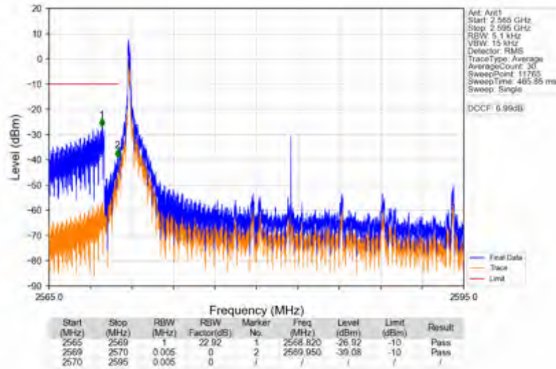
n38_15kHz_SISO_NTNV_25MHz_DFT-s-OFDM QPSK_2582.5MHz_Inner_1RB_Left
