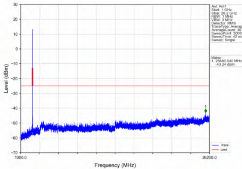
n38_15kHz_SISO_NTNV_20MHz_CP-OFDM QPSK_2580MHz_Outer_Full
