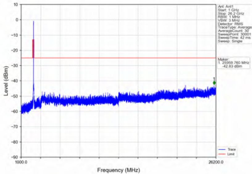
n38_15kHz_SISO_NTNV_40MHz_DFT-s-OFDM PI/2 BPSK_2600MHz_Inner_1RB_Right
