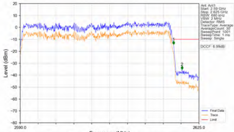
n38_15kHz_SISO_NTNV_30MHz_DFT-s-OFDM PI/2 BPSK_2605MHz_Outer_Full
