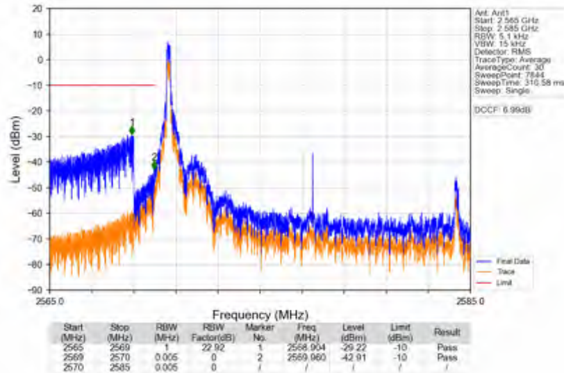
n38_15kHz_SISO_NTNV_15MHz_DFT-s-OFDM QPSK_2577.5MHz_Inner_1RB_Left
