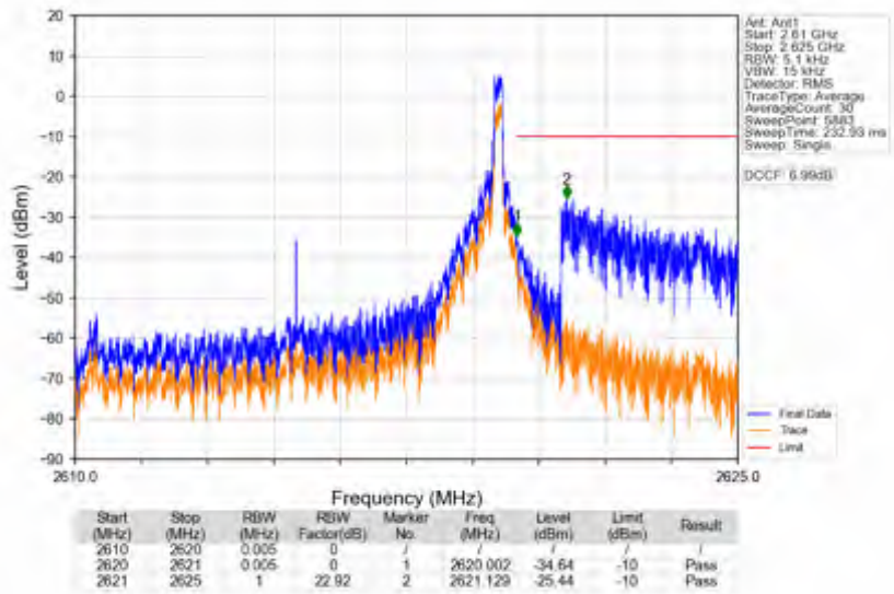
n38_15kHz_SISO_NTNV_10MHz_DFT-s-OFDM QPSK_2615MHz_Edge_1RB_Right
