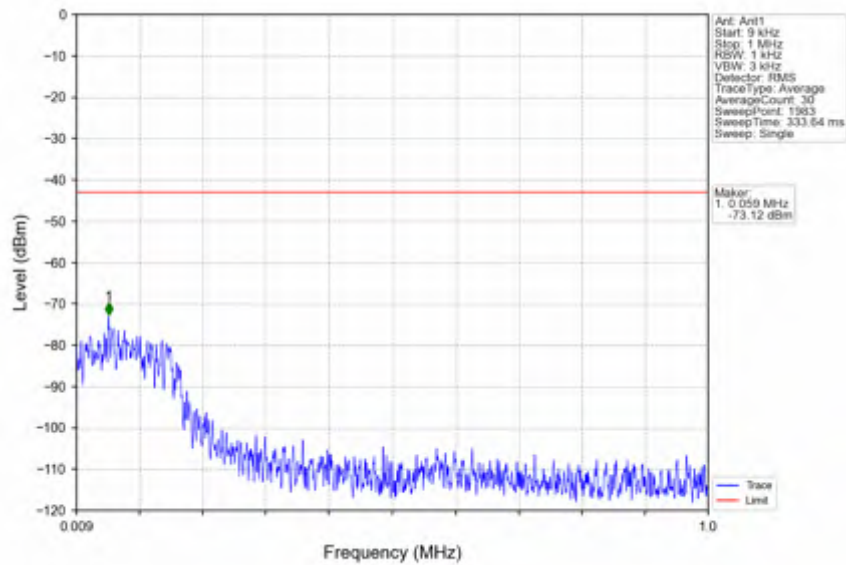
n38_15kHz_SISO_NTV_20MHz_DFT-s-OFDM QPSK_2610MHz_Edge_1RB_Right
