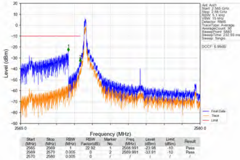
n38_15kHz_SISO_NTNV_10MHz_DFT-s-OFDM_PI/2_BPSK_2575MHz_Edge_1RB_Left
