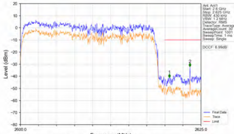
n38_15kHz_SISO_NTNV_20MHz_DFT-s-OFDM PI/2 BPSK_2610MHz_Outer_Full
