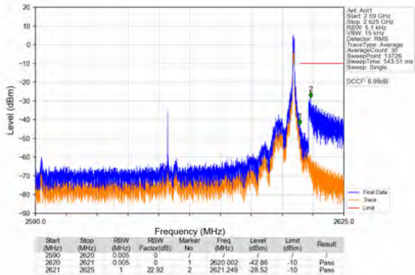
n38_15kHz_SISO_NTNV_30MHz_CP-OFDM QPSK_2605MHz_Edge_1RB_Right
