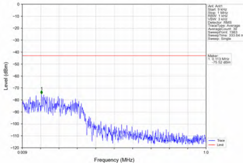
n38_30kHz_SISO_NTNV_10MHz_DFT-s-OFDM QPSK_2575MHz_Edge_1RB_Left
