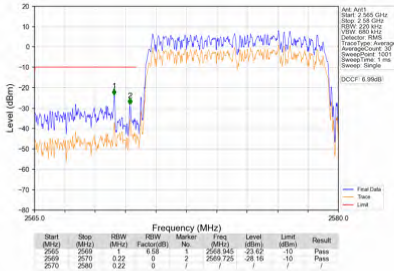
n38_30kHz_SISO_NTNV_10MHz_DFT-s-OFDM QPSK_2575MHz_Outer_Full
