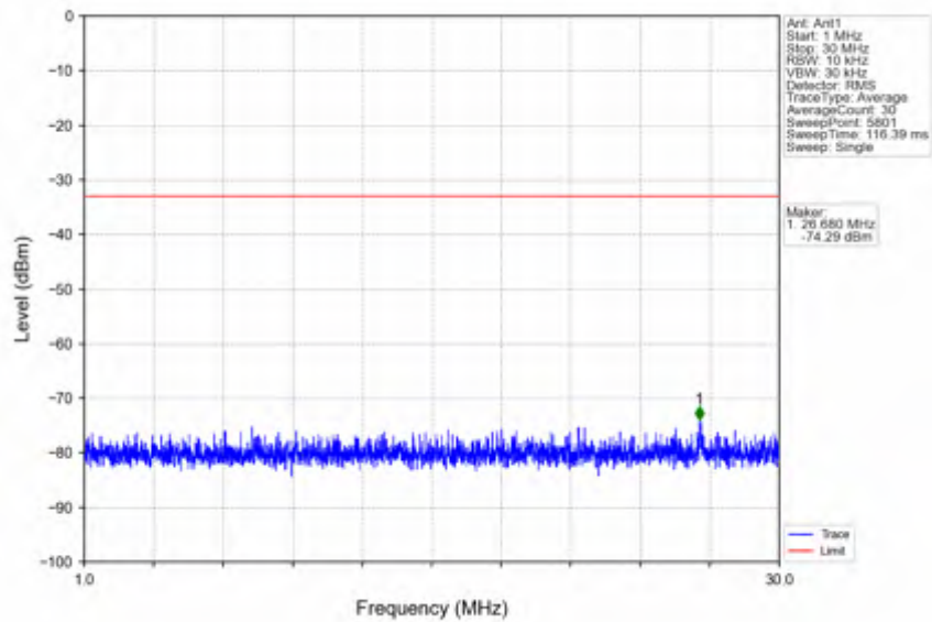
n38_15kHz_SISO_NTNV_15MHz_DFT-s-OFDM QPSK_2595MHz_Edge_1RB_Left
