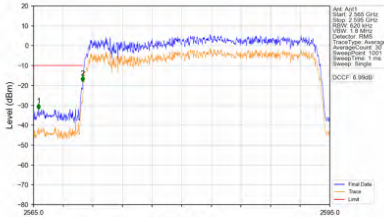
n38_15kHz_SISO_NTNV_25MHz_DFT-s-OFDM QPSK_2582.5MHz_Outer_Full
