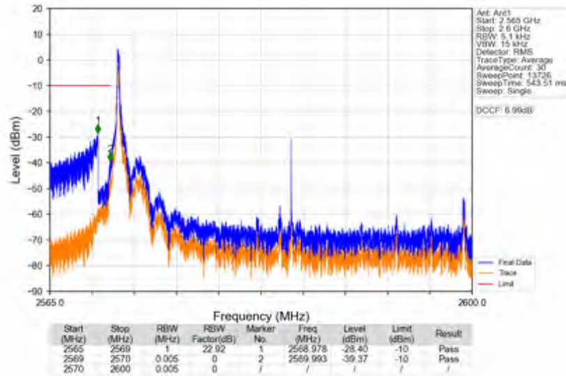
n38_15kHz_SISO_NTNV_30MHz_DFT-s-OFDM QPSK_2585MHz_Edge_1RB_Left
