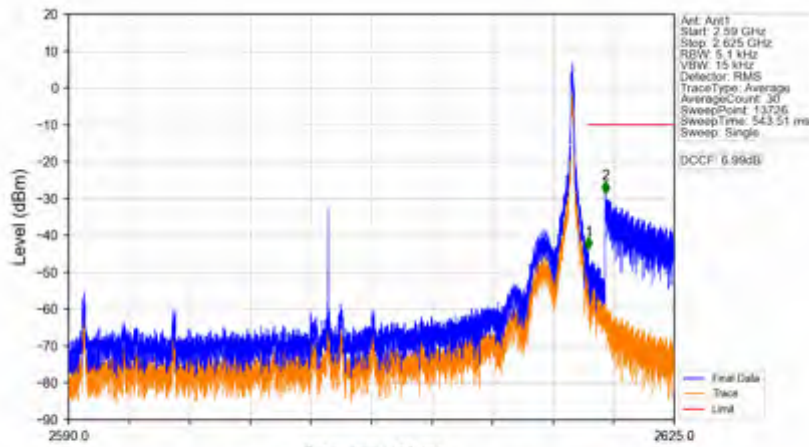
n38_15kHz_SISO_NTNV_30MHz_DFT-s-OFDM PI/2 BPSK_2605MHz_Inner_1RB_Right
