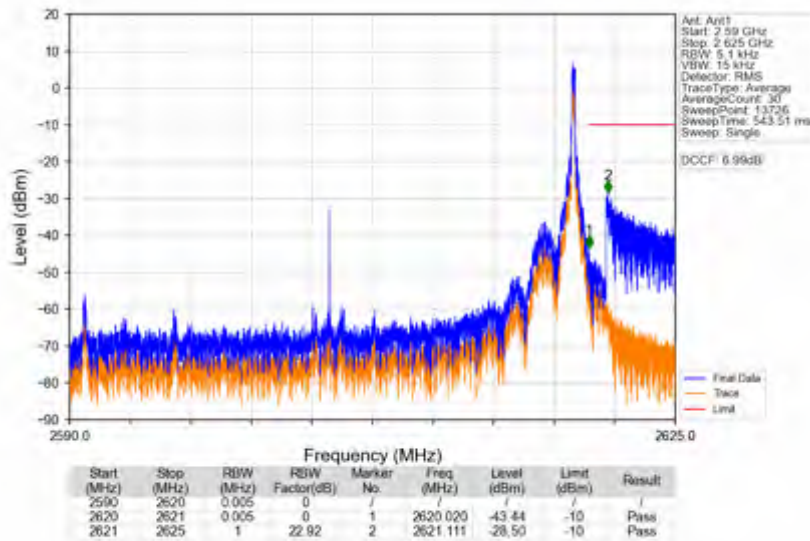
n38_15kHz_SISO_NTNV_30MHz_DFT-s-OFDM QPSK_2605MHz_Inner_1RB_Right
