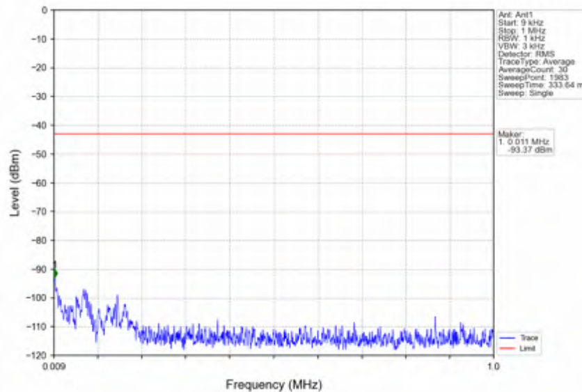
n38_15kHz_SISO_NTNV_40MHz_DFT-s-OFDM PI/2 BPSK_2600MHz_Outer_Full
