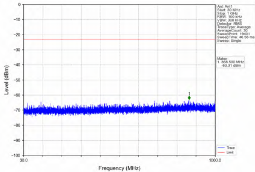
n38_15kHz_SISO_NTNV_40MHz_CP-OFDM QPSK_2600MHz_Edge_1RB_Right
