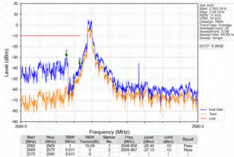
n38_30kHz_SISO_NTNV_10MHz_DFT-s-OFDM QPSK_2575MHz_Edge_1RB_Left
