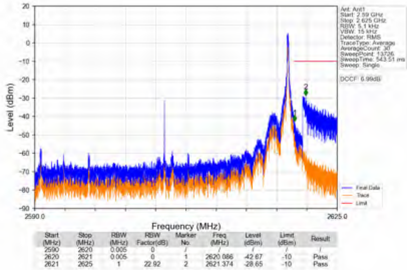
n38_15kHz_SISO_NTNV_30MHz_DFT-s-OFDM QPSK_2605MHz_Edge_1RB_Right
