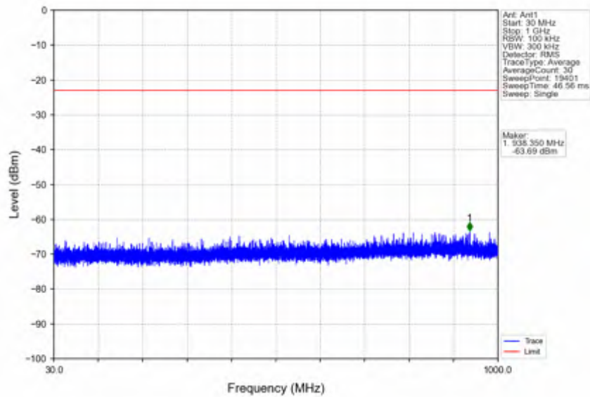
n38_15kHz_SISO_NTNV_10MHz_CP-OFDM QPSK_2615MHz_Edge_1RB_Right
