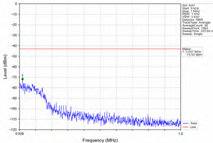
n38_15kHz_SISO_NTNV_10MHz_CP-OFDM QPSK_2575MHz_Edge_1RB_Left
