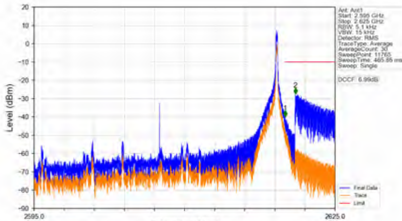
n38_15kHz_SISO_NTNV_25MHz_DFT-s-OFDM QPSK_2607.5MHz_Inner_1RB_Right
