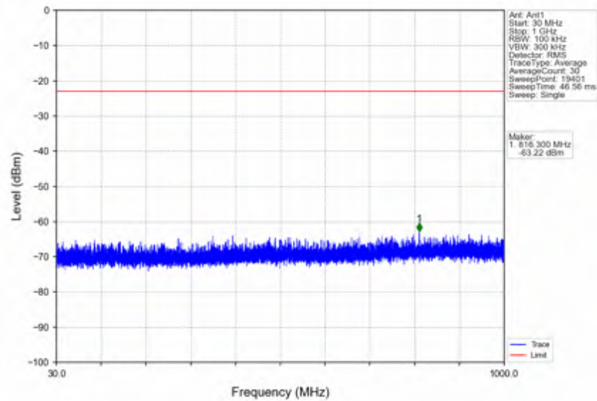
n38_15kHz_SISO_NTNV_40MHz_DFT-s-OFDM QPSK_2590MHz_Outer_Full
