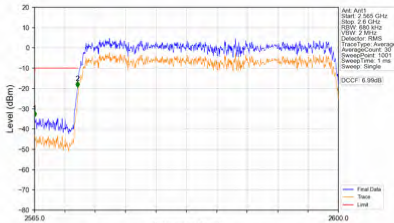
n38_15kHz_SISO_NTNV_30MHz_DFT-s-OFDM QPSK_2585MHz_Outer_Full
