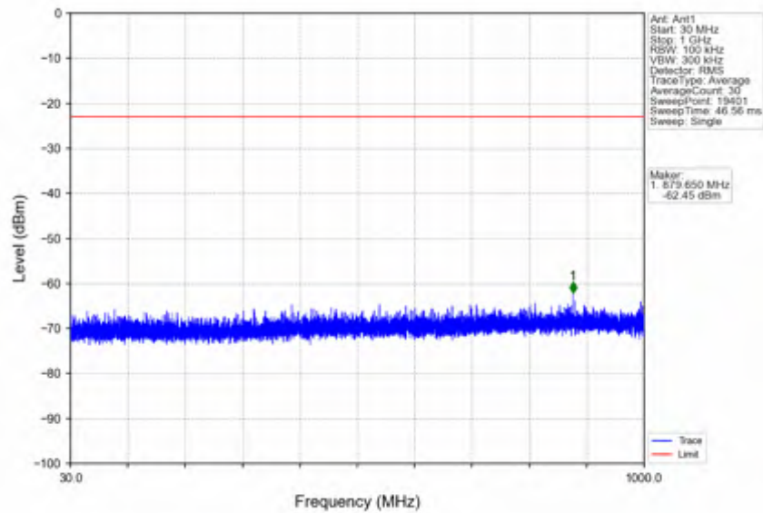
n38_15kHz_SISO_NTNV_20MHz_CP-OFDM QPSK_2610MHz_Edge_1RB_Right
