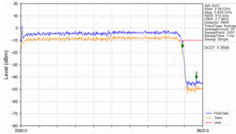
n38_15kHz_SISO_NTNV_40MHz_DFT-s-OFDM PI/2 BPSK_2600MHz_Outer_Full
