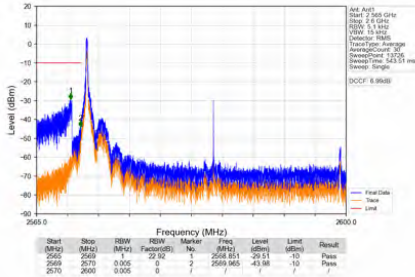
n38_15kHz_SISO_NTNV_30MHz_CP-OFDM QPSK_2585MHz_Edge_1RB_Left
