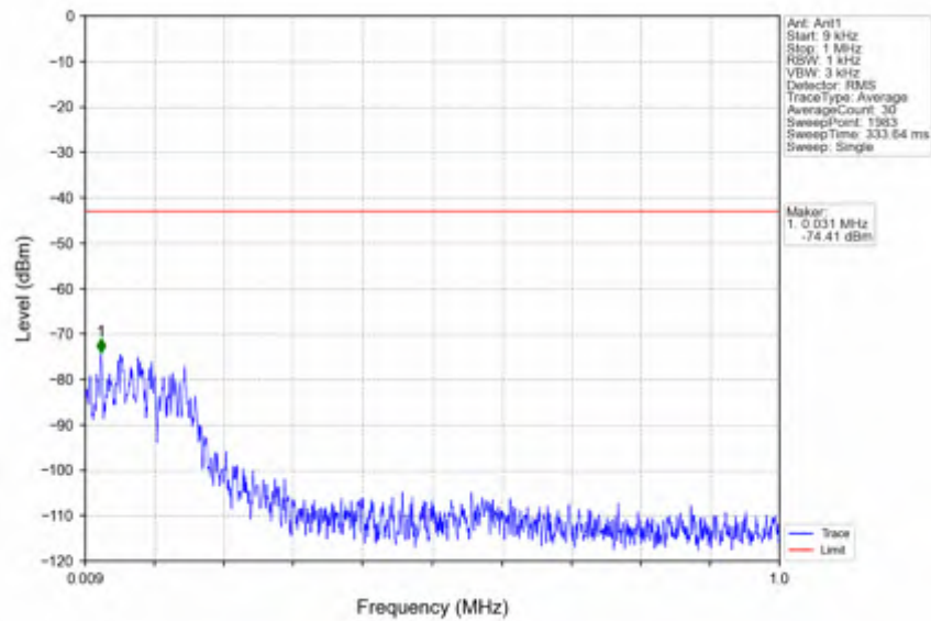
n38_15kHz_SISO_NTNV_25MHz_DFT-s-OFDM QPSK_2607.5MHz_Edge_1RB_Right
