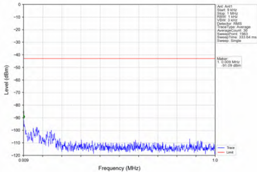
n38_15kHz_SISO_NTNV_40MHz_DFT-s-OFDM PI/2 BPSK_2590MHz_Outer_Full
