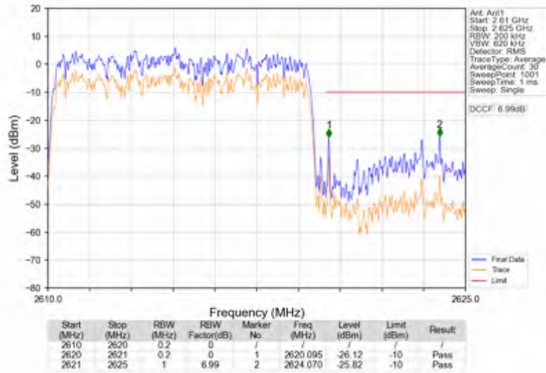
n38_15kHz_SISO_NTNV_10MHz_DFT-s-OFDM QPSK_2615MHz_Outer_Full
