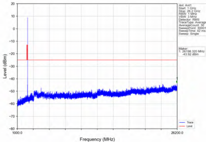
n38_15kHz_SISO_NTV_15MHz_CP-OFDM QPSK_2612.5MHz_Edge_1RB_Right
