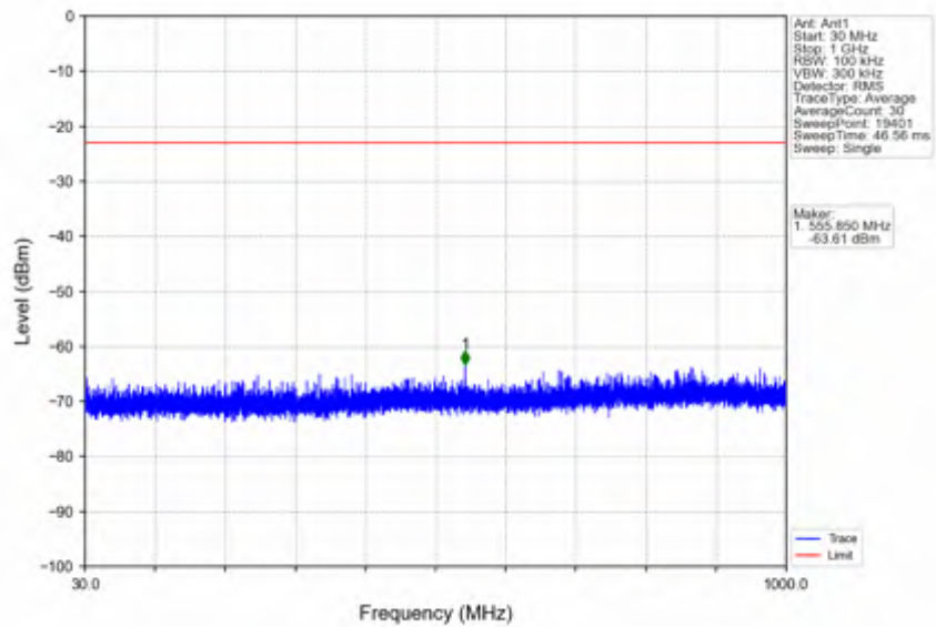
n38_15kHz_SISO_NTNV_10MHz_DFT-s-OFDM QPSK_2575MHz_Edge_1RB_Left
