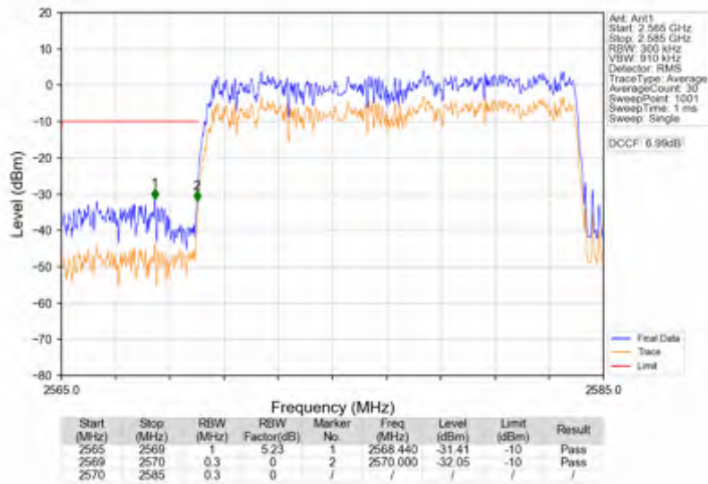
n38_15kHz_SISO_NTNV_15MHz_DFT-s-OFDM QPSK_2577.5MHz_Outer_Full
