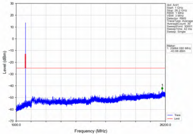
n38_15kHz_SISO_NTNV_15MHz_DFT-s-OFDM PI/2 BPSK_2577.5MHz_Outer_Full
