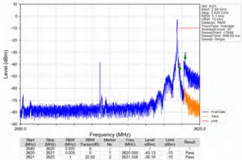
n38_15kHz_SISO_NTNV_40MHz_CP-OFDM QPSK_2600MHz_Edge_1RB_Right
