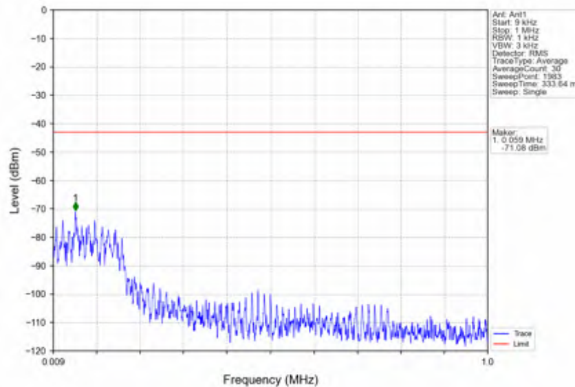
n38_15kHz_SISO_NTNV_15MHz_DFT-s-OFDM QPSK_2595MHz_Edge_1RB_Left
