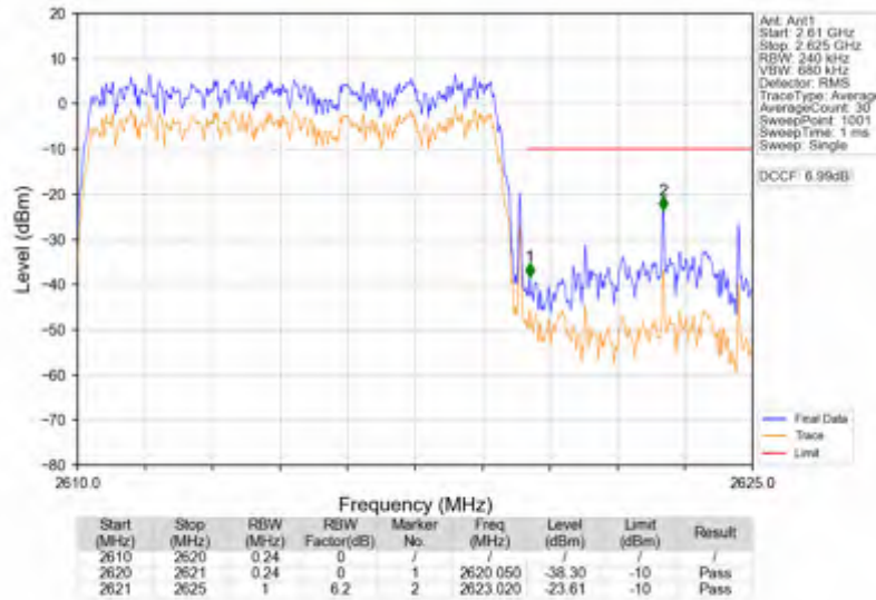
n38_15kHz_SISO_NTNV_10MHz_DFT-s-OFDM PI/2 BPSK_2615MHz_Outer_Full
