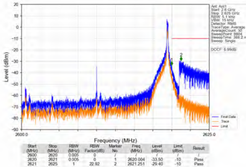
n38_15kHz_SISO_NTNV_20MHz_DFT-s-OFDM QPSK_2610MHz_Edge_1RB_Right
