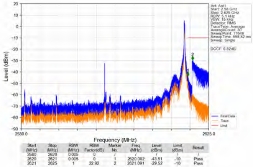
n38_15kHz_SISO_NTNV_40MHz_DFT-s-OFDM PI/2 BPSK_2600MHz_Inner_1RB_Right
