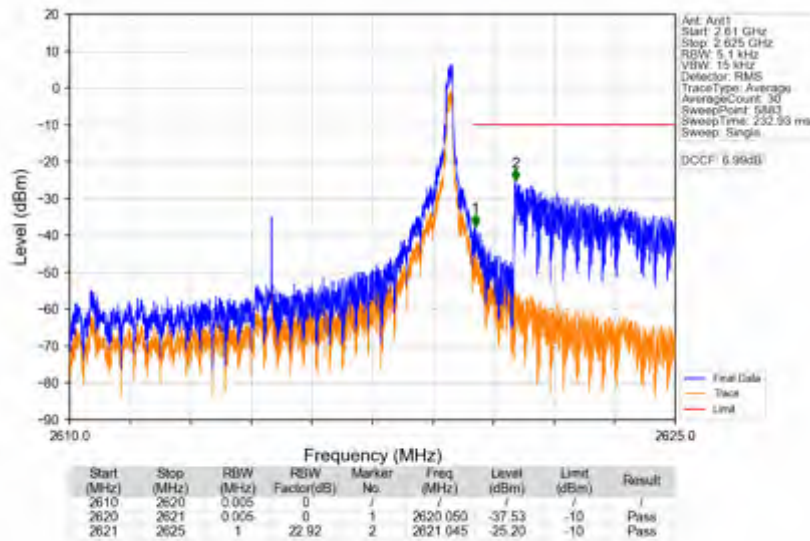
n38_15kHz_SISO_NTNV_10MHz_DFT-s-OFDM QPSK_2615MHz_Inner_1RB_Right
