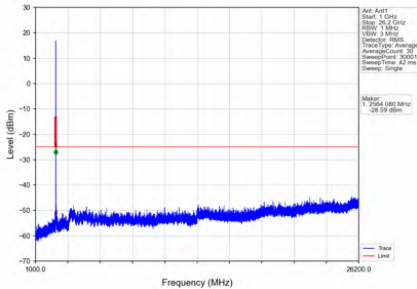
n38_15kHz_SISO_NTNV_20MHz_DFT-s-OFDM QPSK_2580MHz_Outer_Full
