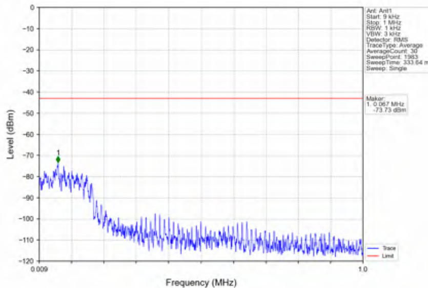
n38_15kHz_SISO_NTNV_15MHz_DFT-s-OFDM QPSK_2577.5MHz_Edge_1RB_Left
