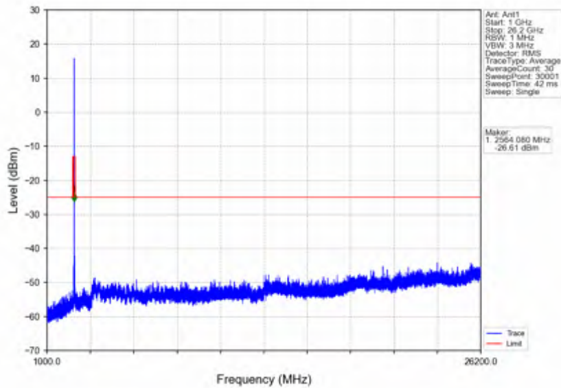
n38_15kHz_SISO_NTNV_25MHz_DFT-s-OFDM QPSK_2582.5MHz_Outer_Full
