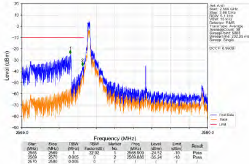
n38_15kHz_SISO_NTNV_10MHz_DFT-s-OFDM QPSK_2575MHz_Edge_1RB_Left
