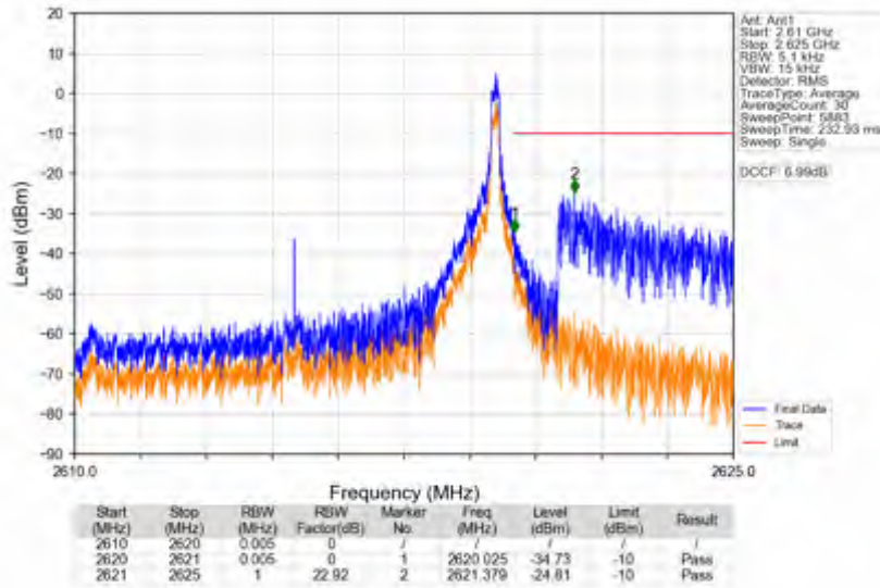
n38_15kHz_SISO_NTNV_10MHz_CP-OFDM QPSK_2615MHz_Edge_1RB_Right
