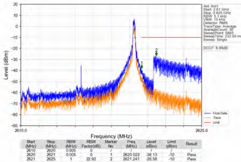
n38_15kHz_SISO_NTNV_10MHz_DFT-s-OFDM PI/2 BPSK_2615MHz_Inner_1RB_Right
