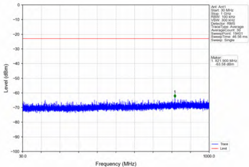
n38_15kHz_SISO_NTNV_25MHz_DFT-s-OFDM QPSK_2582.5MHz_Edge_1RB_Left
