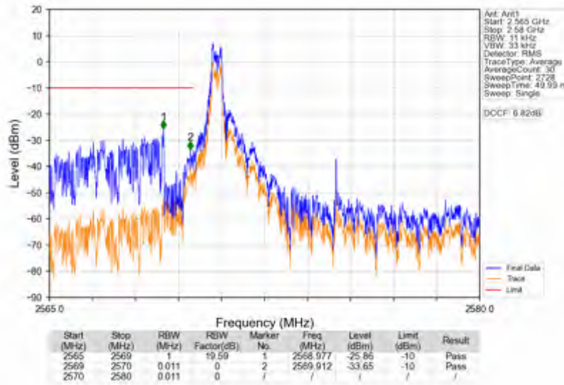
n38_30kHz_SISO_NTNV_10MHz_DFT-s-OFDM PI/2 BPSK_2575MHz_Edge_1RB_Left
