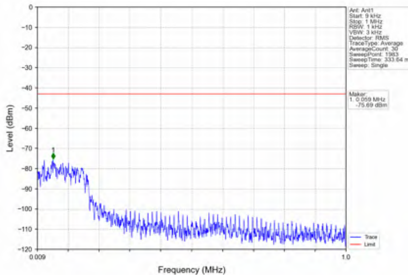
n38_15kHz_SISO_NTNV_30MHz_DFT-s-OFDM QPSK_2585MHz_Edge_1RB_Left
