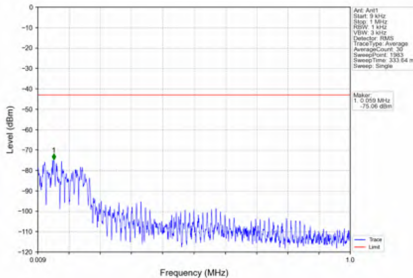
n38_15kHz_SISO_NTNV_15MHz_DFT-s-OFDM PI/2 BPSK_2595MHz_Edge_1RB_Left
