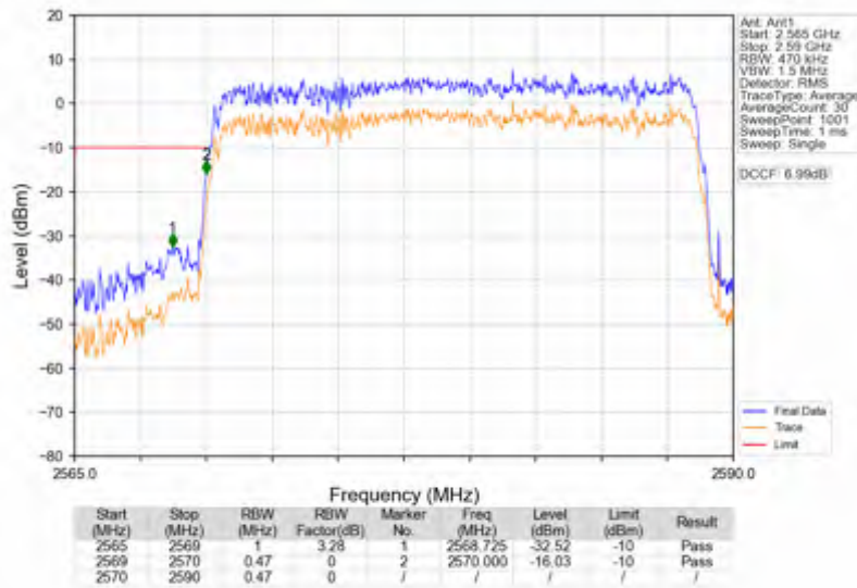
n38_15kHz_SISO_NTNV_20MHz_DFT-s-OFDM PI/2 BPSK_2580MHz_Outer_Full
