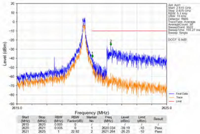
n38_15kHz_SISO_NTNV_5MHz_CP-OFDM QPSK_2617.5MHz_Inner_1RB_Right
