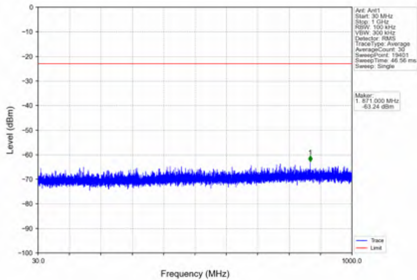
n38_15kHz_SISO_NTNV_15MHz_DFT-s-OFDM QPSK_2612.5MHz_Edge_1RB_Right
