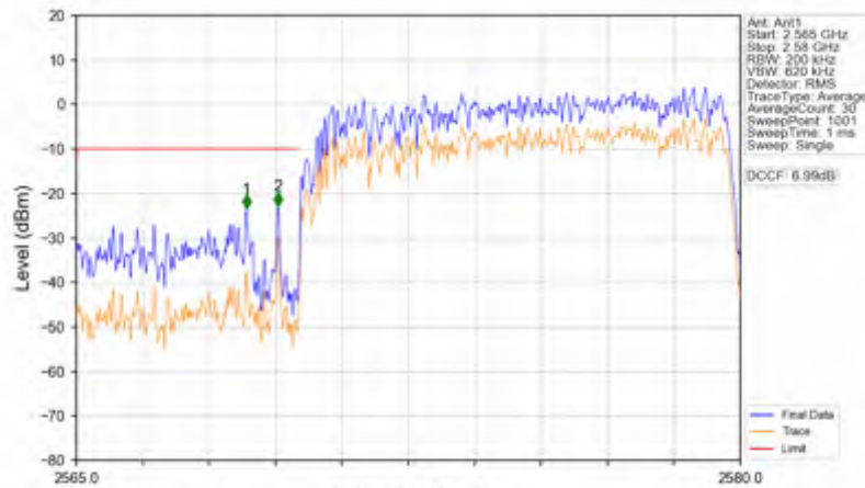
n38_15kHz_SISO_NTNV_10MHz_CP-OFDM QPSK_2575MHz_Outer_Full
