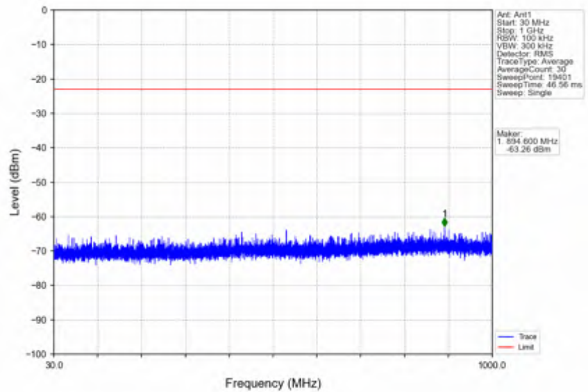
n38_15kHz_SISO_NTNV_10MHz_DFT-s-OFDM QPSK_2595MHz_Edge_1RB_Left
