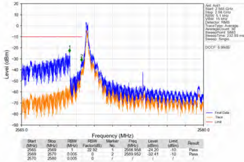
n38_15kHz_SISO_NTNV_10MHz_CP-OFDM QPSK_2575MHz_Edge_1RB_Left
