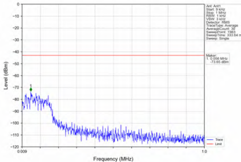
n38_15kHz_SISO_NTNV_10MHz_DFT-s-OFDM QPSK_2575MHz_Edge_1RB_Left
