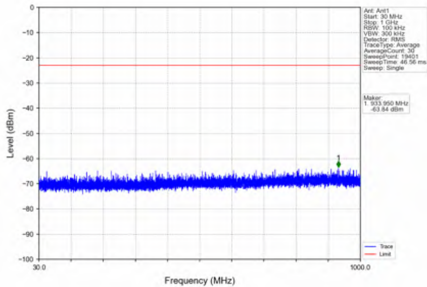
n38_15kHz_SISO_NTNV_10MHz_DFT-s-OFDM QPSK_2615MHz_Edge_1RB_Right
