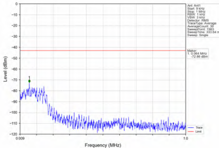
n38_15kHz_SISO_NTNV_25MHz_DFT-s-OFDM QPSK_2582.5MHz_Edge_1RB_Left
