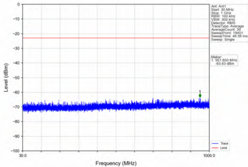
n38_15kHz_SISO_NTNV_20MHz_DFT-s-OFDM QPSK_2610MHz_Edge_1RB_Right
