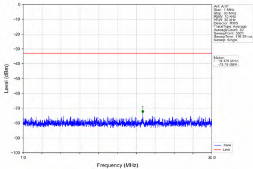
n38_15kHz_SISO_NTNV_15MHz_CP-OFDM QPSK_2595MHz_Edge_1RB_Left
