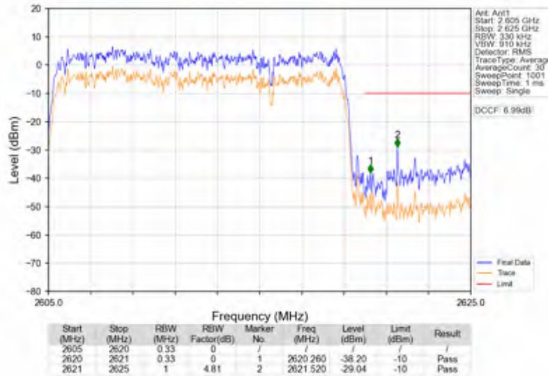
n38_15kHz_SISO_NTNV_15MHz_DFT-s-OFDM PI/2 BPSK_2612.5MHz_Outer_Full
