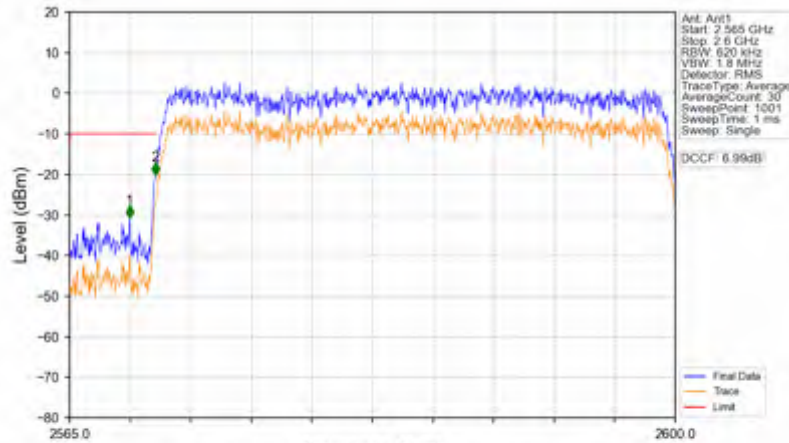
n38_15kHz_SISO_NTNV_30MHz_CP-OFDM QPSK_2585MHz_Outer_Full
