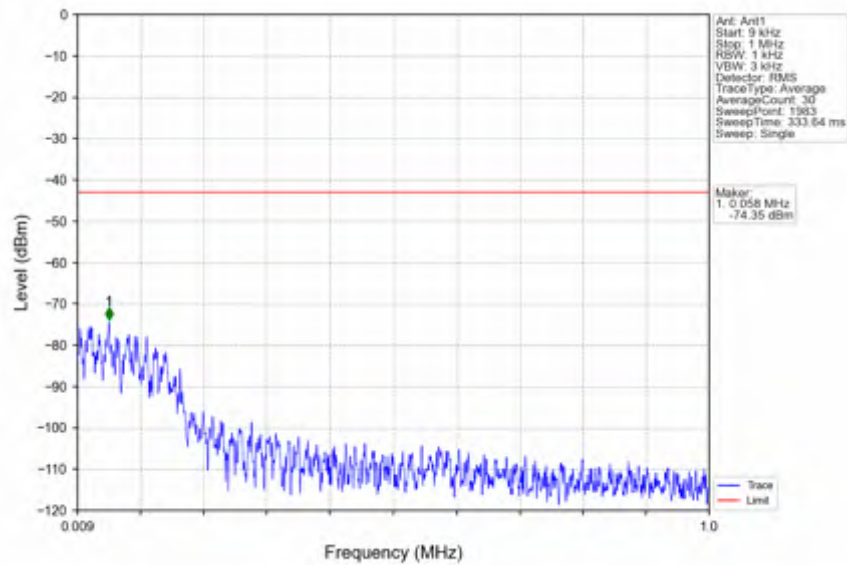
n38_15kHz_SISO_NTNV_25MHz_CP-OFDM QPSK_2607.5MHz_Edge_1RB_Right
