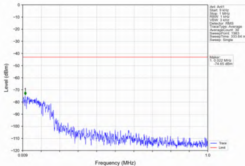
n38_15kHz_SISO_NTNV_15MHz_CP-OFDM QPSK_2595MHz_Edge_1RB_Left
