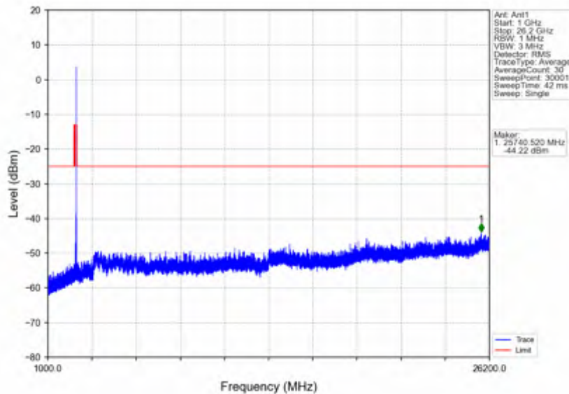
n38_15kHz_SISO_NTNV_25MHz_CP-OFDM QPSK_2607.5MHz_Edge_1RB_Right
