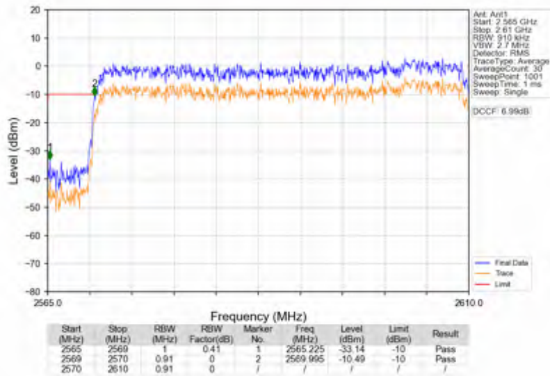
n38_15kHz_SISO_NTNV_40MHz_CP-OFDM QPSK_2590MHz_Outer_Full
