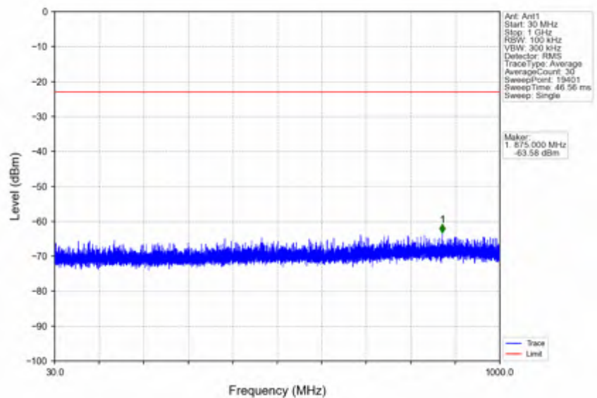
n38_15kHz_SISO_NTNV_10MHz_CP-OFDM QPSK_2575MHz_Edge_1RB_Left
