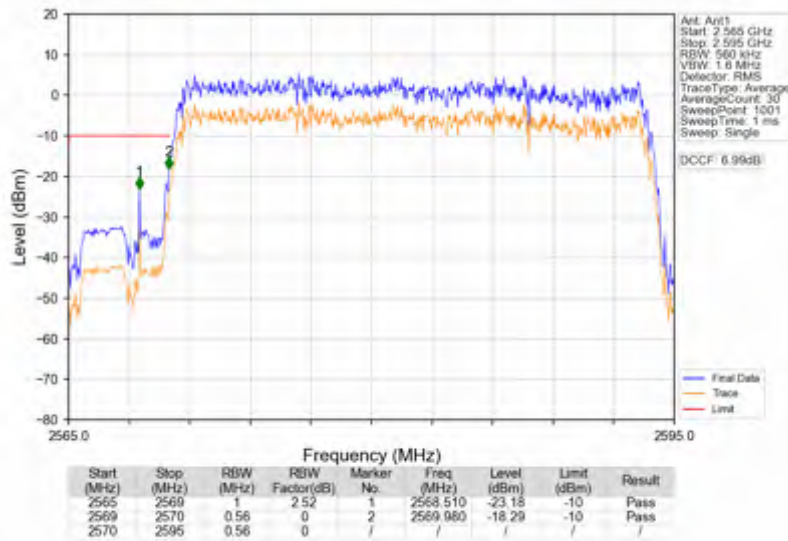
n38_15kHz_SISO_NTNV_25MHz_DFT-s-OFDM PI/2 BPSK_2582.5MHz_Outer_Full
