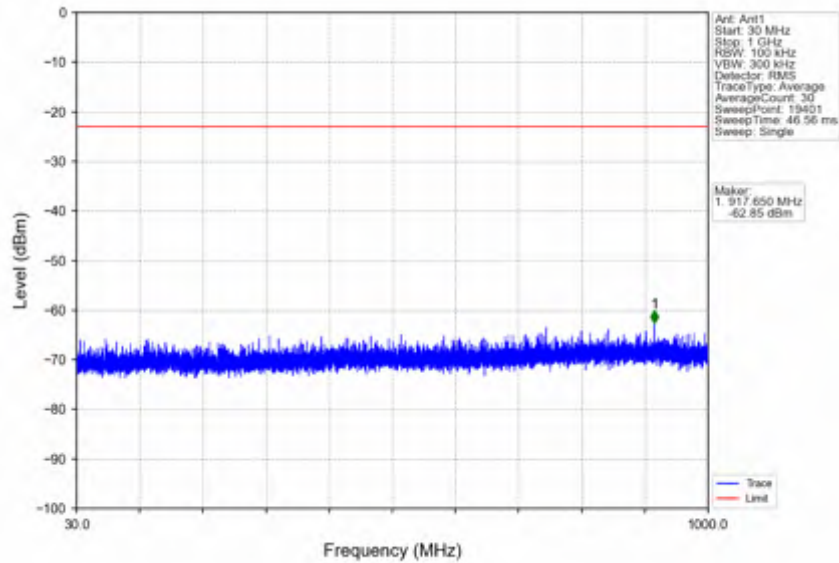
n38_15kHz_SISO_NTNV_25MHz_CP-OFDM QPSK_2607.5MHz_Edge_1RB_Right
