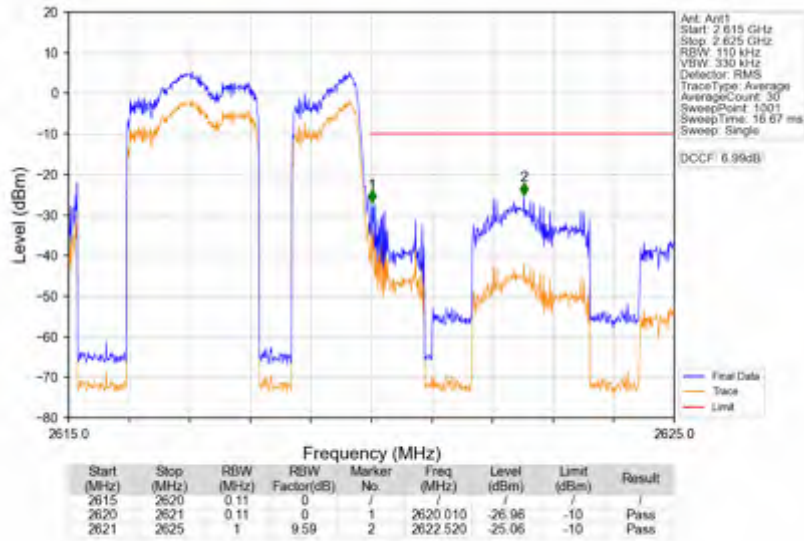
n38_15kHz_SISO_NTNV_5MHz_CP-OFDM QPSK_2617.5MHz_Outer_Full
