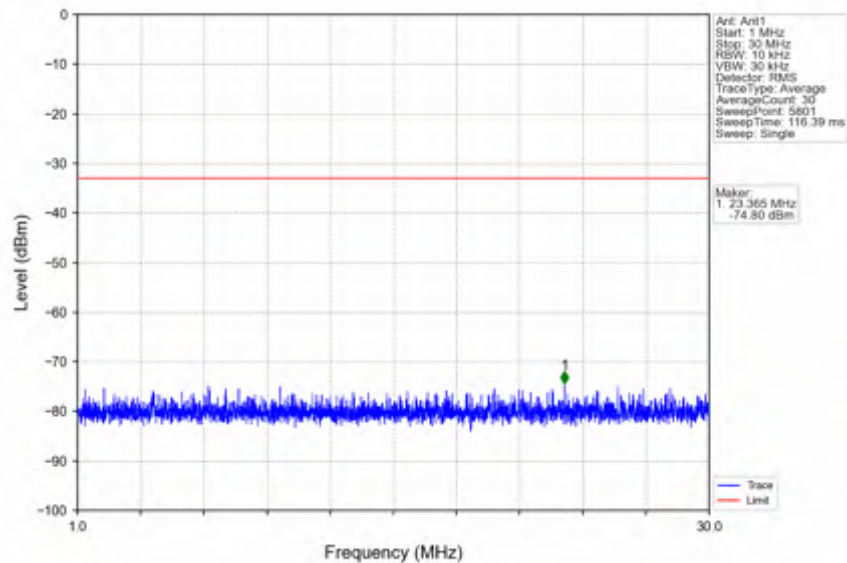
n38_15kHz_SISO_NTNV_30MHz_DFT-s-OFDM QPSK_2605MHz_Edge_1RB_Right
