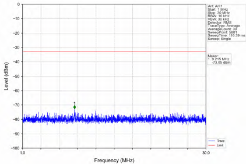
n38_15kHz_SISO_NTV_15MHz_CP-OFDM QPSK_2577.5MHz_Edge_1RB_Left
