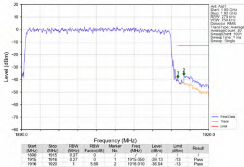
n25_30kHz_SISO_NTNV_25MHz_DFT-s-OFDM PI/2 BPSK_1902.5MHz_Outer_Full
