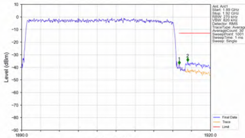
n25_30kHz_SISO_NTNV_25MHz_CP-OFDM QPSK_1902.5MHz_Outer_Full
