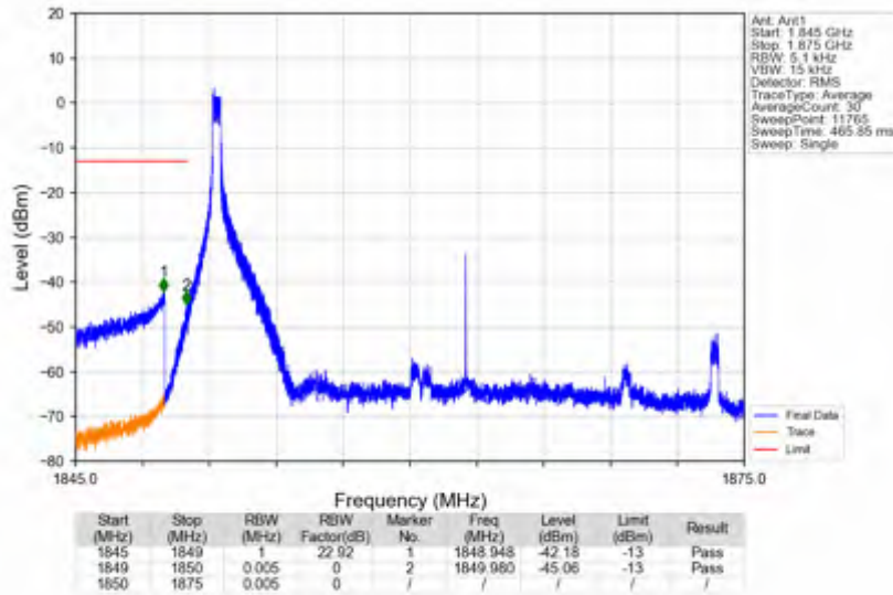
n25_30kHz_SISO_NTV_25MHz_CP-OFDM_QPSK_1862.5MHz_Inner_1RB_Left
