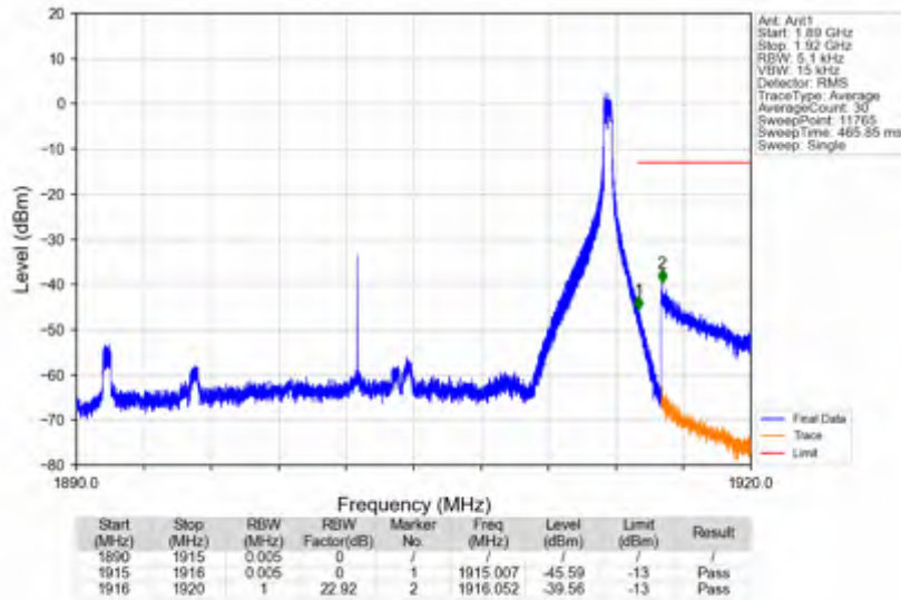
n25_30kHz_SISO_NTNV_25MHz_CP-OFDM QPSK_1902.5MHz_Inner_1RB_Right
