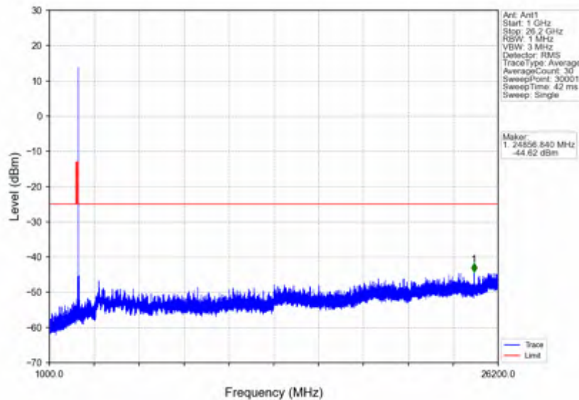
n38_15kHz_SISO_NTNV_5MHz_DFT-s-OFDM PI/2 BPSK_2617.5MHz_Edge_1RB_Right
