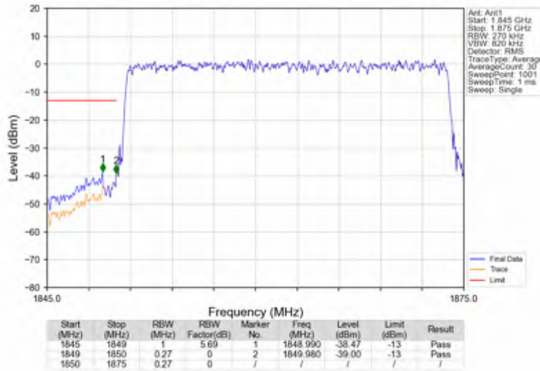
n25_30kHz_SISO_NTNV_25MHz_DFT-s-OFDM PI/2 BPSK_1862.5MHz_Outer_Full
