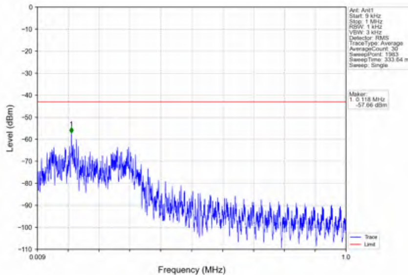
n25_30kHz_SISO_NTNV_25MHz_DFT-s-OFDM PI/2 BPSK_1902.5MHz_Inner_1RB_Right
