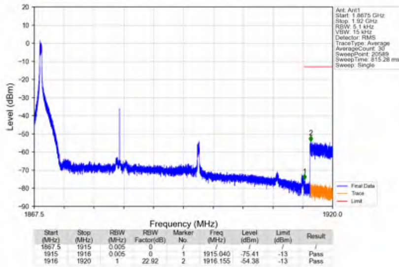
n25_30kHz_SISO_NTNV_30MHz_CP-OFDM QPSK_1882.5MHz_Edge_1RB_Left
