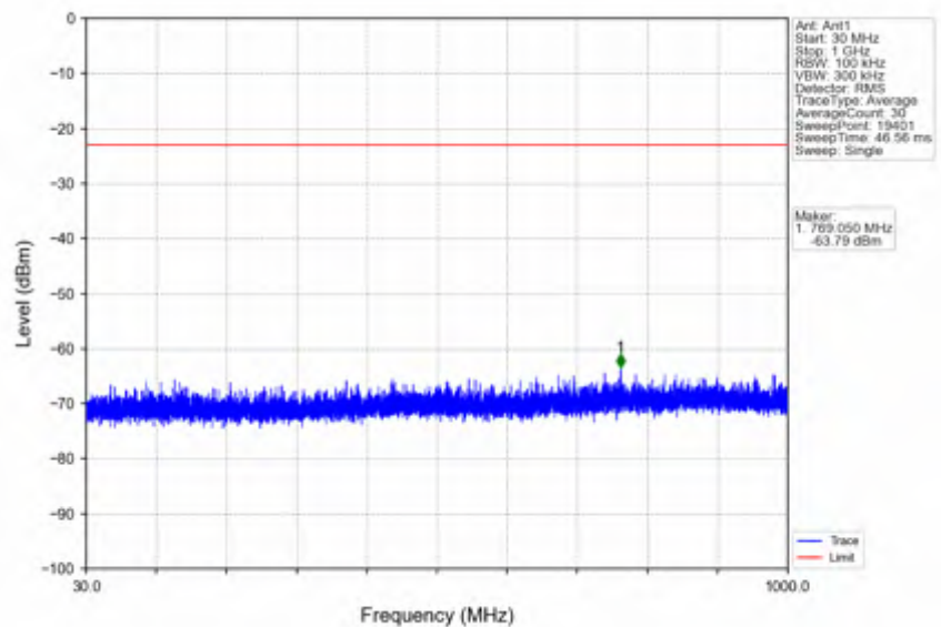
n25_30kHz_SISO_NTNV_40MHz_DFT-s-OFDM PI/2 BPSK_1870MHz_Edge_1RB_Left
