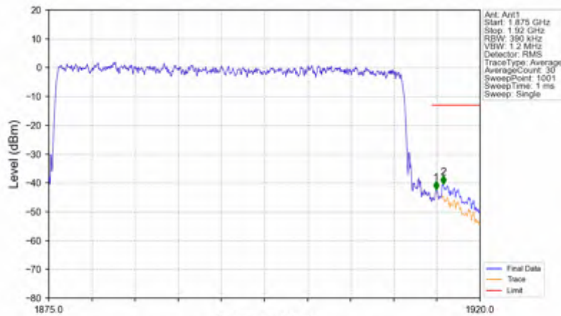
n25_30kHz_SISO_NTNV_40MHz_DFT-s-OFDM PI/2 BPSK_1895MHz_Outer_Full
