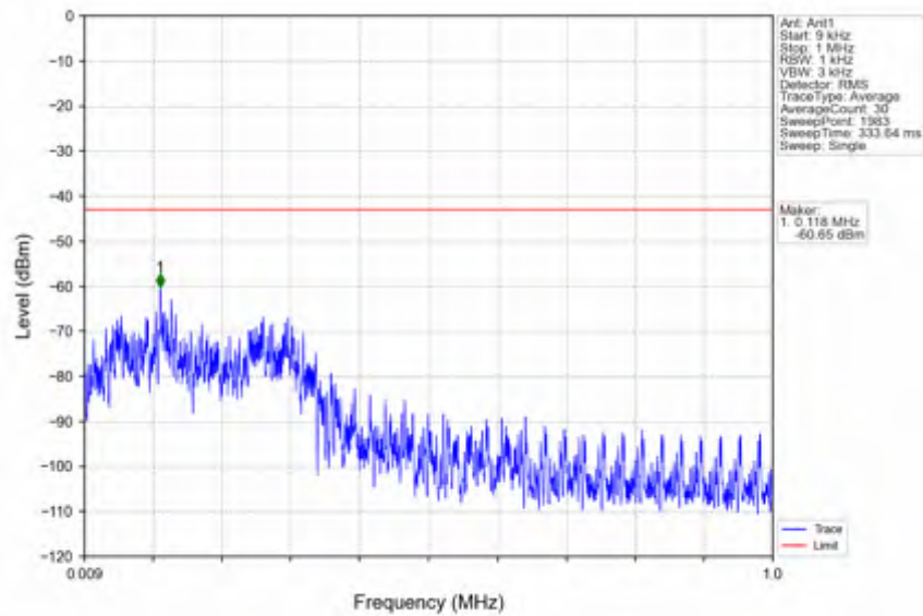
n25_30kHz_SISO_NTNV_40MHz_DFT-s-OFDM PI/2 BPSK_1882.5MHz_Edge_1RB_Left
