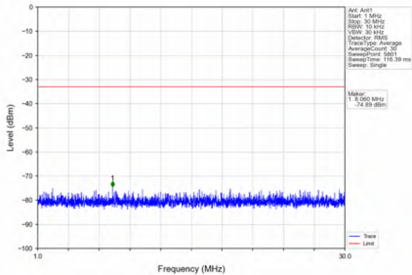
n25_30kHz_SISO_NTNV_30MHz_DFT-s-OFDM PI/2 BPSK_1865MHz_Edge_1RB_Left
