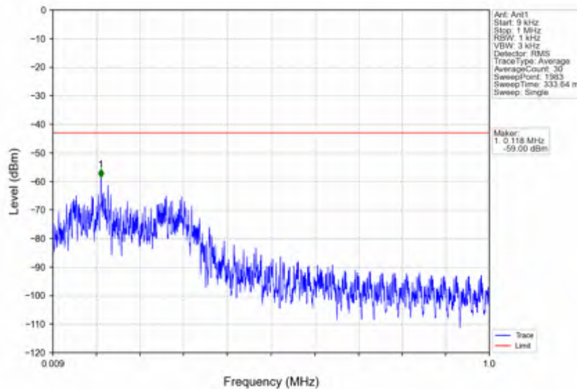
n25_30kHz_SISO_NTNV_30MHz_DFT-s-OFDM PI/2 BPSK_1900MHz_Edge_1RB_Right
