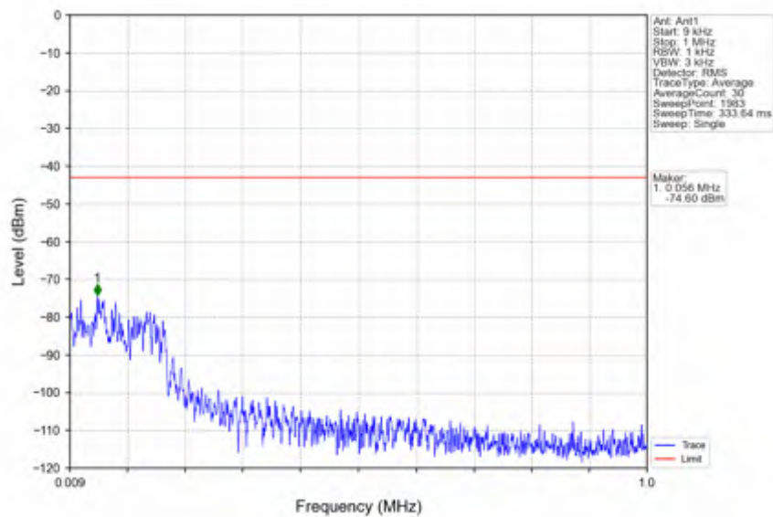
n38_15kHz_SISO_NTNV_5MHz_DFT-s-OFDM_PI/2_BPSK_2572.5MHz_Edge_1RB_Left
