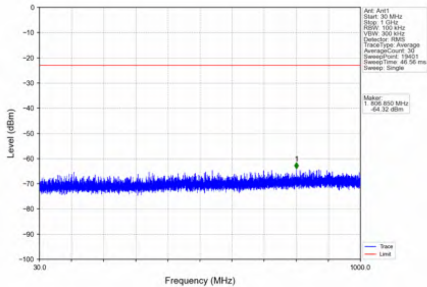
n25_30kHz_SISO_NTNV_40MHz_DFT-s-OFDM PI/2 BPSK_1895MHz_Outer_Full
