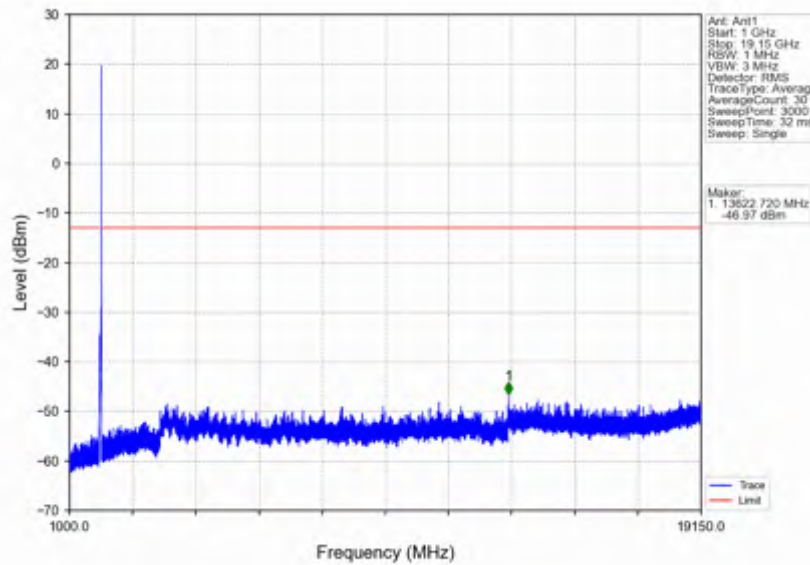
n25_30kHz_SISO_NTNV_25MHz_CP-OFDM QPSK_1902.5MHz_Outer_Full
