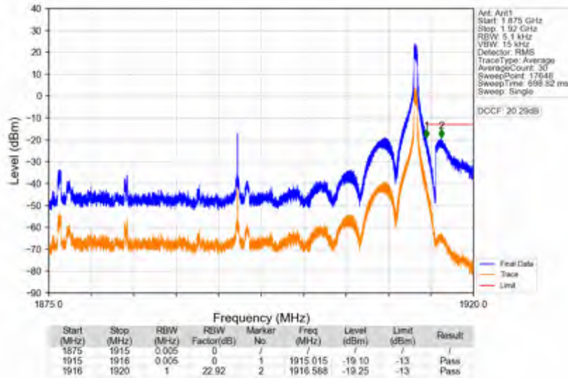
n25_30kHz_SISO_NTNV_40MHz_DFT-s-OFDM PI/2 BPSK_1895MHz_Edge_1RB_Right
