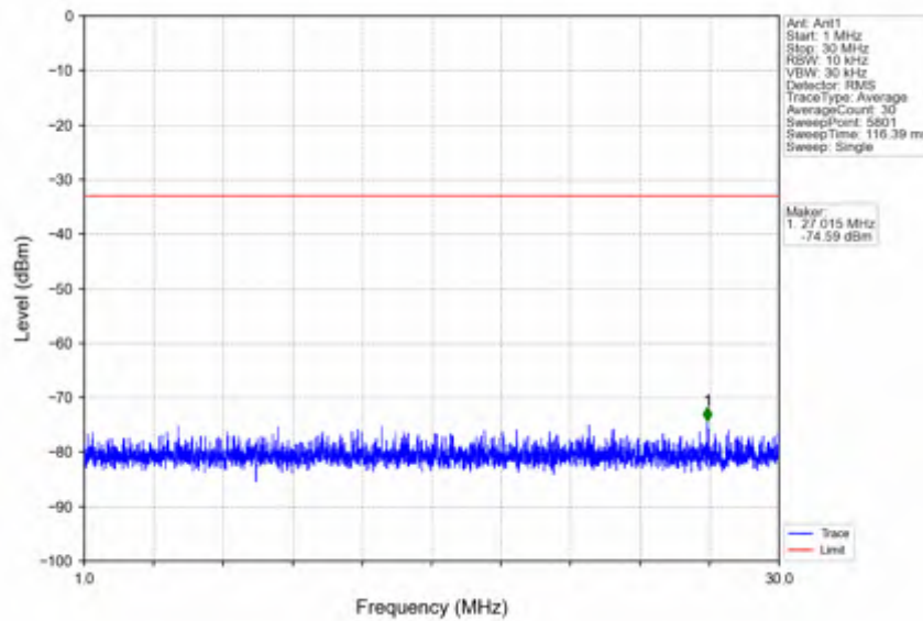
n25_30kHz_SISO_NTNV_40MHz_CP-OFDM QPSK_1895MHz_Inner_1RB_Right
