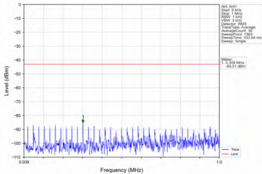
n25_30kHz_SISO_NTNV_40MHz_DFT-s-OFDM PI/2 BPSK_1870MHz_Outer_Full
