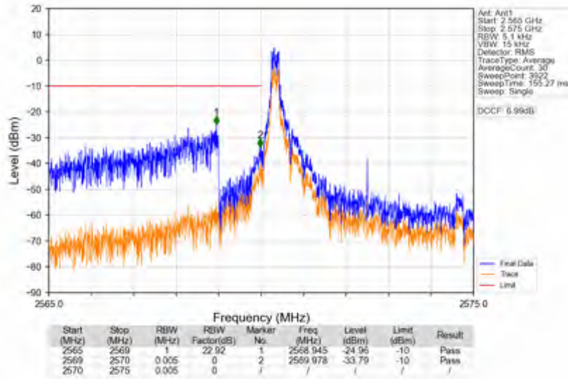
n38_15kHz_SISO_NTNV_5MHz_DFT-s-OFDM QPSK_2572.5MHz_Edge_1RB_Left
