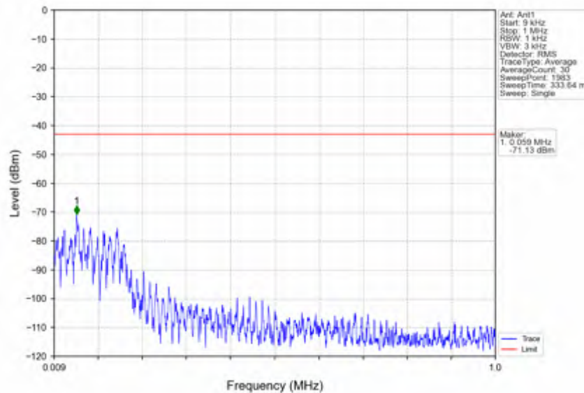
n38_15kHz_SISO_NTNV_5MHz_DFT-s-OFDM PI/2 BPSK_2595MHz_Edge_1RB_Left
