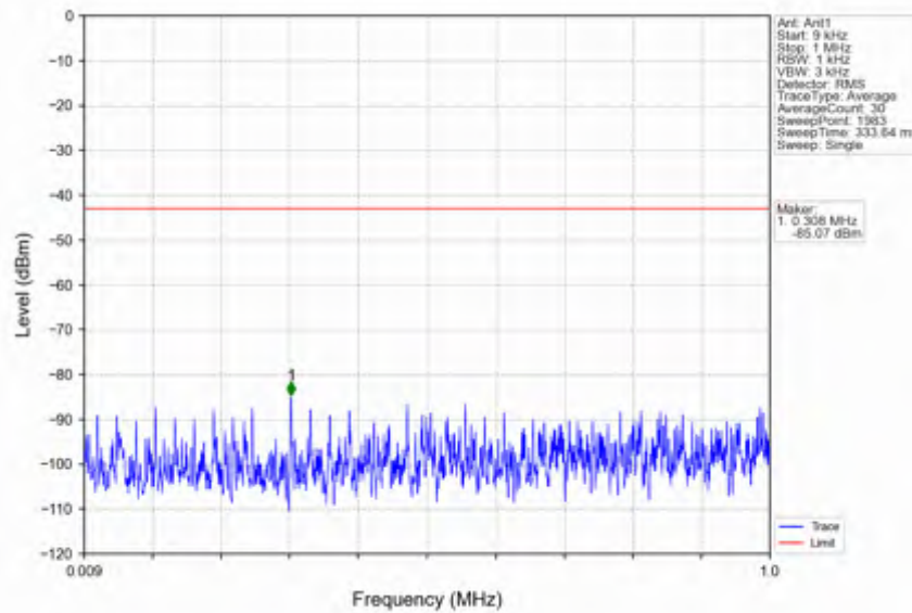
n25_30kHz_SISO_NTNV_30MHz_DFT-s-OFDM PI/2 BPSK_1865MHz_Outer_Full
