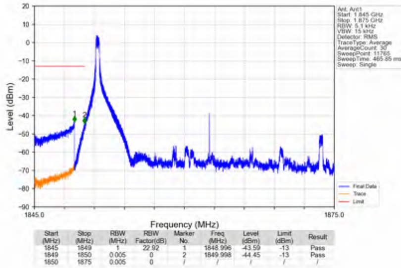
n25_30kHz_SISO_NTNV_25MHz_DFT-s-OFDM PI/2 BPSK_1862.5MHz_Inner_1RB_Left
