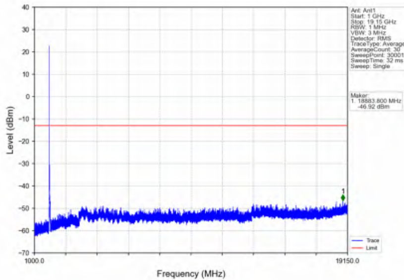
n25_30kHz_SISO_NTNV_30MHz_DFT-s-OFDM PI/2 BPSK_1882.5MHz_Edge_1RB_Left
