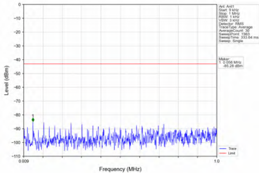
n25_30kHz_SISO_NTNV_25MHz_DFT-s-OFDM PI/2 BPSK_1902.5MHz_Outer_Full
