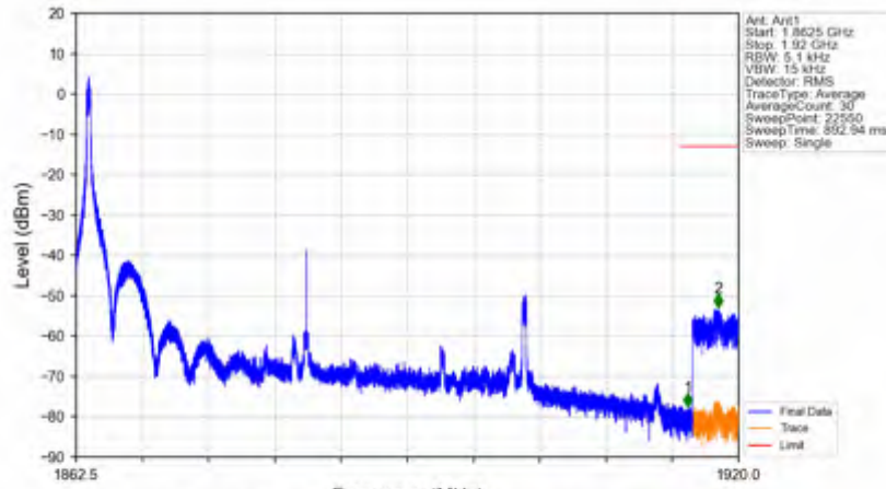
n25_30kHz_SISO_NTNV_40MHz_DFT-s-OFDM QPSK_1882.5MHz_Edge_1RB_Left
