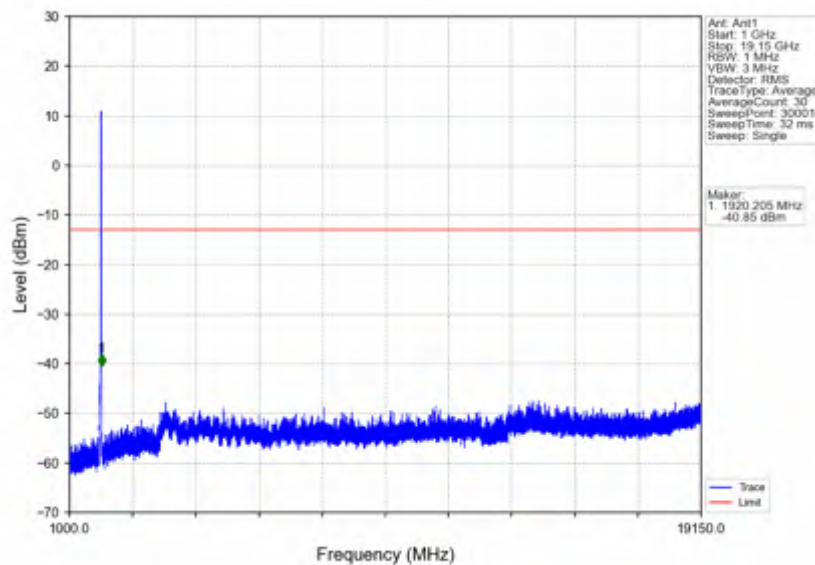
n25_30kHz_SISO_NTNV_25MHz_DFT-s-OFDM PI/2 BPSK_1902.5MHz_Outer_Full
