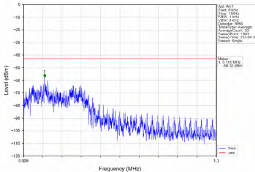
n25_30kHz_SISO_NTNV_40MHz_DFT-s-OFDM PI/2 BPSK_1895MHz_Inner_1RB_Right
