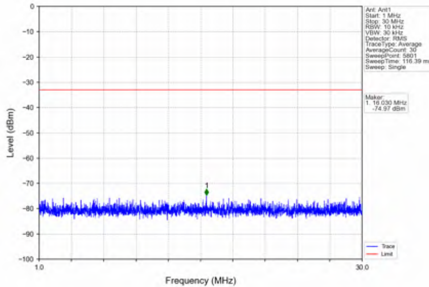
n25_30kHz_SISO_NTNV_25MHz_DFT-s-OFDM PI/2 BPSK_1902.5MHz_Edge_1RB_Right
