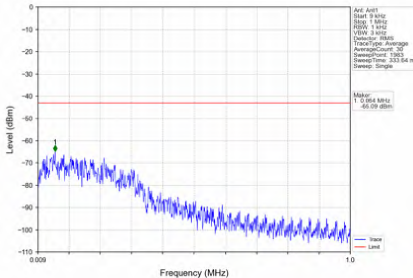
n25_30kHz_SISO_NTNV_40MHz_CP-OFDM QPSK_1870MHz_Edge_1RB_Left
