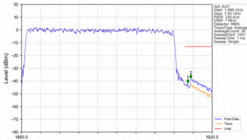
n25_30kHz_SISO_NTNV_30MHz_DFT-s-OFDM PI/2 BPSK_1900MHz_Outer_Full
