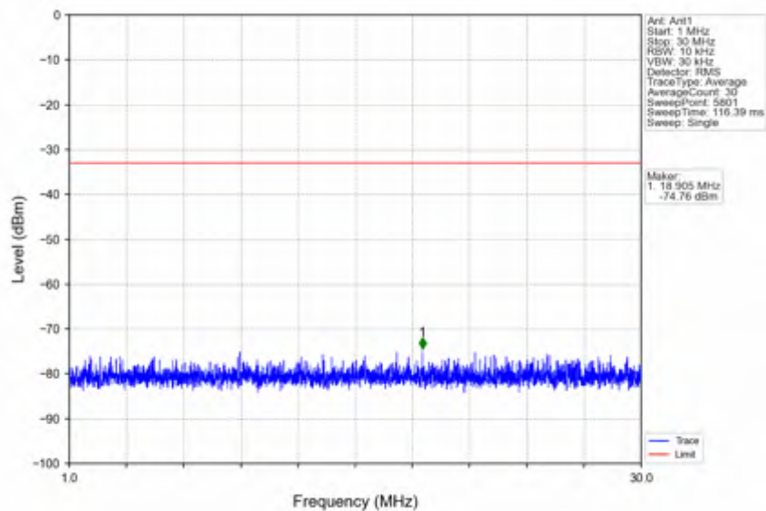
n25_30kHz_SISO_NTNV_25MHz_DFT-s-OFDM PI/2 BPSK_1862.5MHz_Outer_Full
