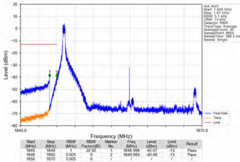
n25_30kHz_SISO_NTNV_20MHz_DFT-s-OFDM QPSK_1860MHz_Edge_1RB_Left
