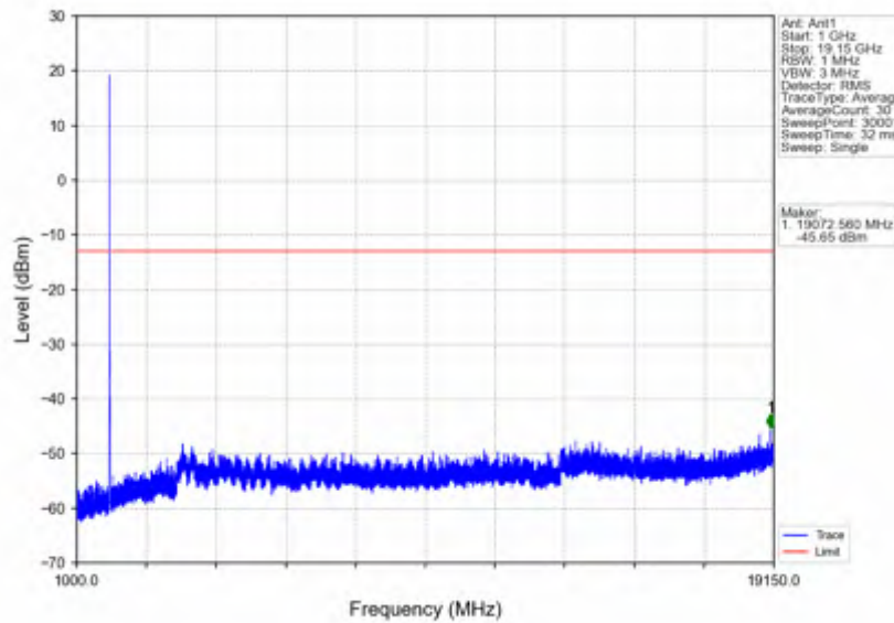
n25_30kHz_SISO_NTNV_10MHz_CP-OFDM QPSK_1855MHz_Outer_Full
