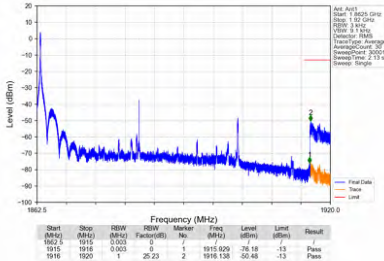
n25_15kHz_SISO_NTNV_40MHz_DFT-s-OFDM QPSK_1882.5MHz_Edge_1RB_Left
