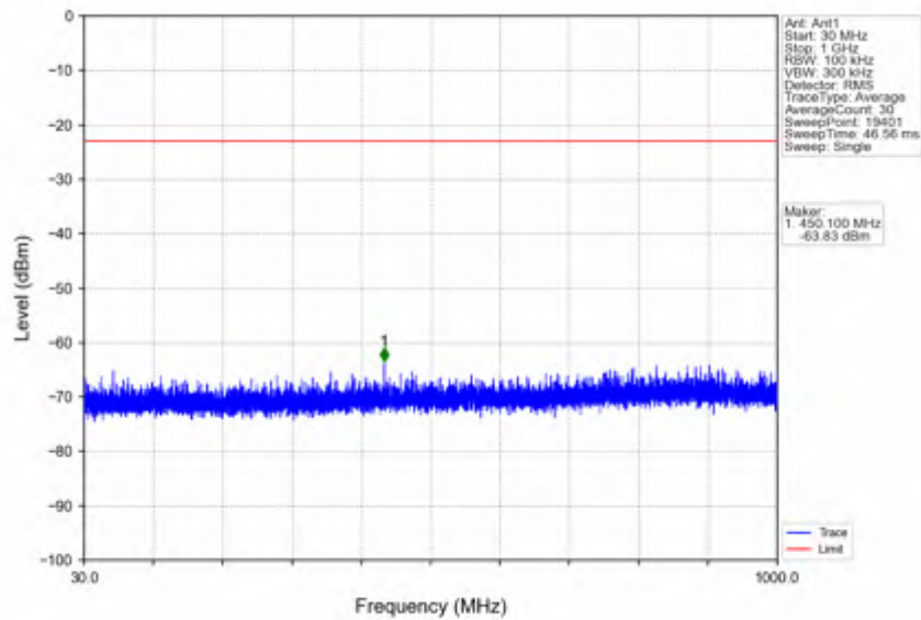
n25_30kHz_SISO_NTNV_10MHz_DFT-s-OFDM QPSK_1910MHz_Inner_1RB_Right
