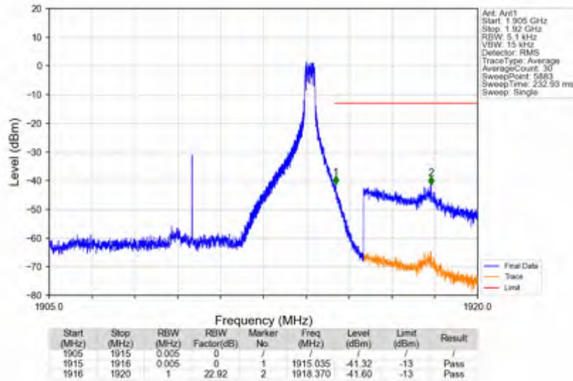
n25_30kHz_SISO_NTNV_10MHz_CP-OFDM QPSK_1910MHz_Edge_1RB_Right
