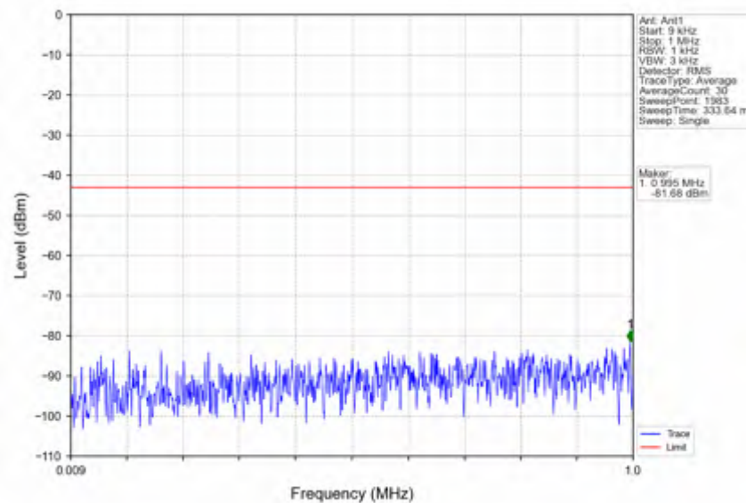
n25_30kHz_SISO_NTNV_10MHz_DFT-s-OFDM QPSK_1855MHz_Outer_Full
