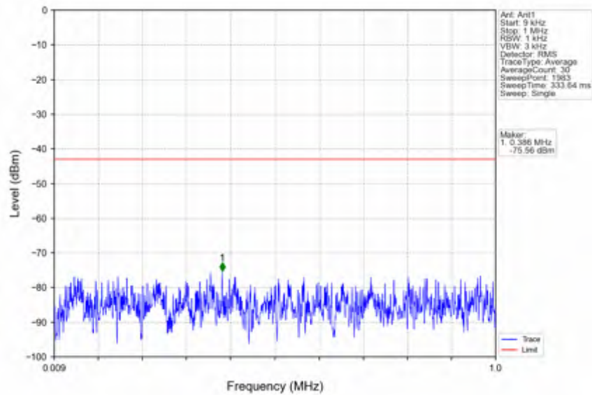
n25_30kHz_SISO_NTNV_15MHz_CP-OFDM QPSK_1857.5MHz_Outer_Full
