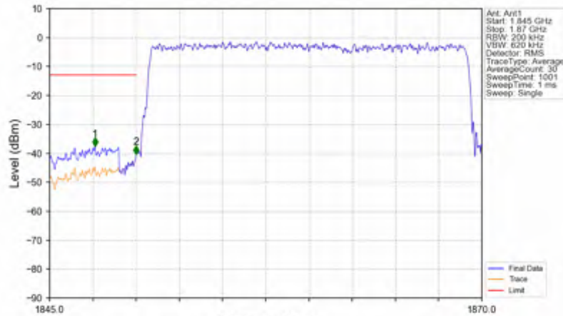
n25_30kHz_SISO_NTNV_20MHz_CP-OFDM QPSK_1860MHz_Outer_Full
