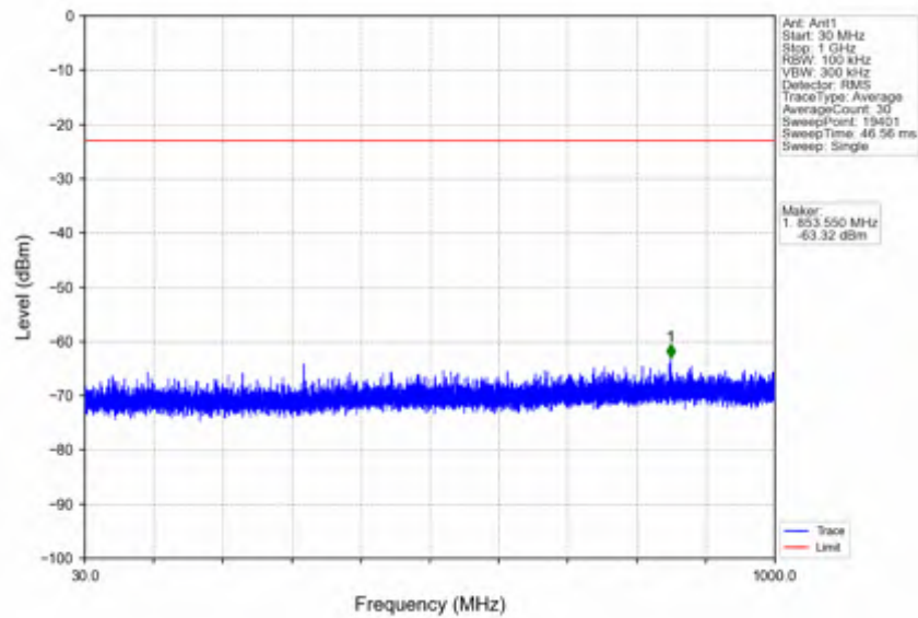
n25_30kHz_SISO_NTNV_20MHz_DFT-s-OFDM PI/2 BPSK_1860MHz_Outer_Full
