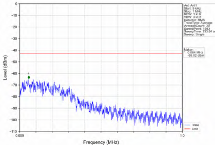
n25_30kHz_SISO_NTNV_20MHz_CP-OFDM QPSK_1860MHz_Edge_1RB_Left
