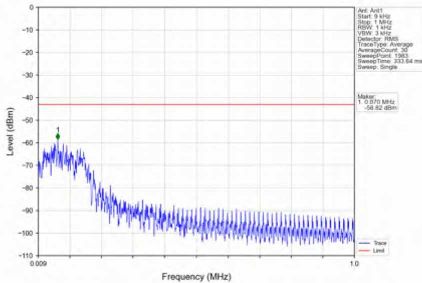
n25_15kHz_SISO_NTNV_40MHz_DFT-s-OFDM QPSK_1895MHz_Inner_1RB_Right
