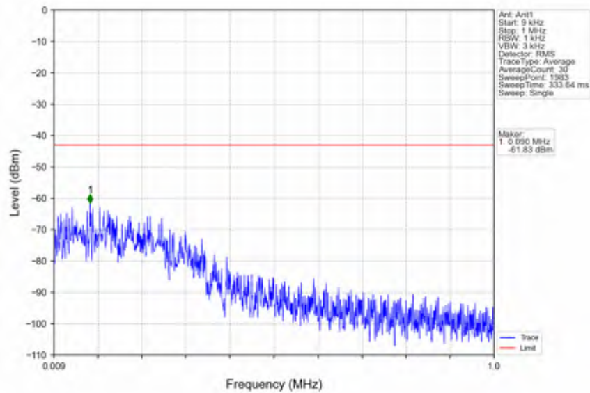
n25_30kHz_SISO_NTVV_10MHz_CP-OFDM QPSK_1882.5MHz_Edge_1RB_Left
