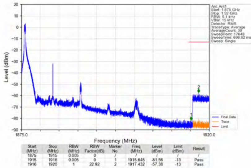
n25_30kHz_SISO_NTNV_15MHz_DFT-s-OFDM QPSK_1882.5MHz_Edge_1RB_Left
