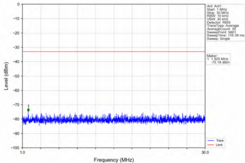
n25_30kHz_SISO_NTNV_20MHz_DFT-s-OFDM PI/2 BPSK_1882.5MHz_Edge_1RB_Left
