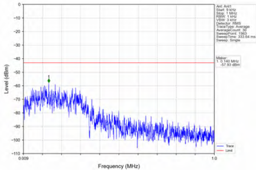
n25_30kHz_SISO_NTNV_10MHz_DFT-s-OFDM QPSK_1910MHz_Inner_1RB_Right
