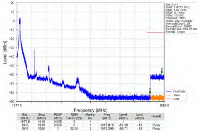
n25_30kHz_SISO_NTNV_10MHz_DFT-s-OFDM QPSK_1882.5MHz_Edge_1RB_Left
