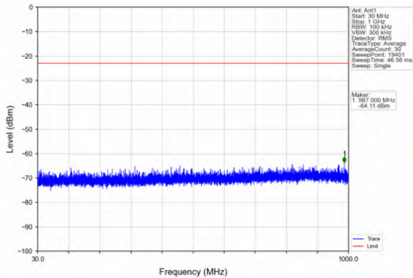
n25_30kHz_SISO_NTNV_10MHz_DFT-s-OFDM QPSK_185MHz_Edge_1RB_Left
