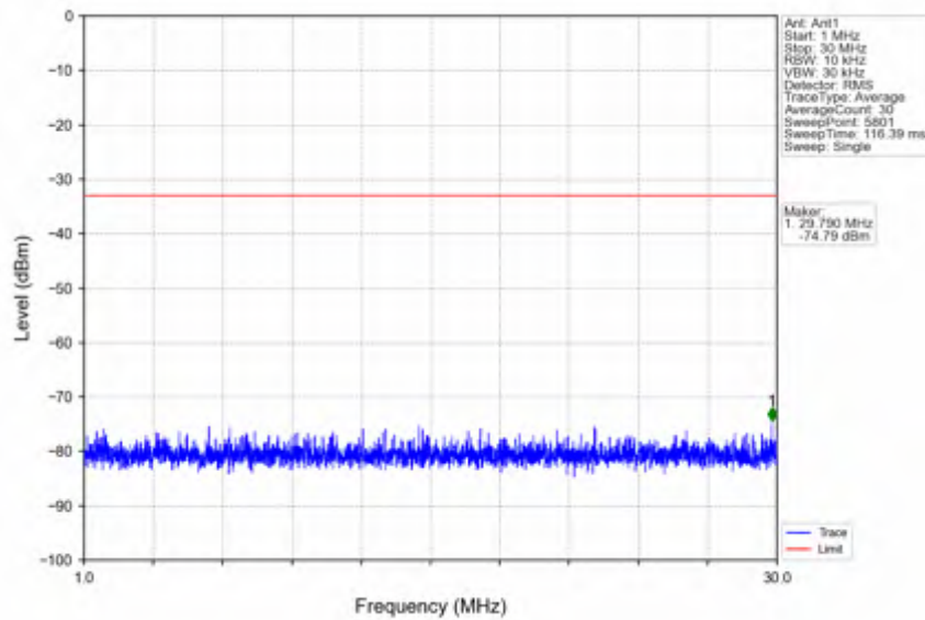
n25_30kHz_SISO_NTNV_20MHz_DFT-s-OFDM QPSK_1882.5MHz_Edge_1RB_Left
