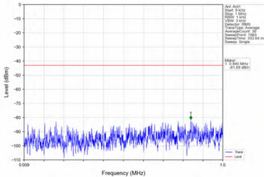
n25_30kHz_SISO_NTNV_15MHz_DFT-s-OFDM PI/2 BPSK_1857.5MHz_Outer_Full
