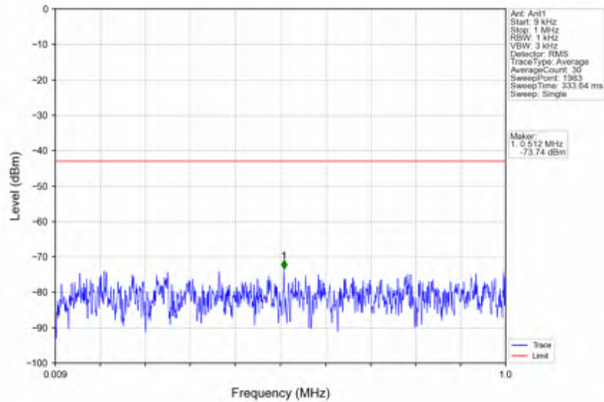
n25_30kHz_SISO_NTNV_10MHz_CP-OFDM QPSK_1910MHz_Outer_Full
