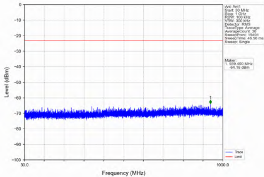
n25_30kHz_SISO_NTNV_15MHz_DFT-s-OFDM QPSK_1857.5MHz_Edge_1RB_Left
