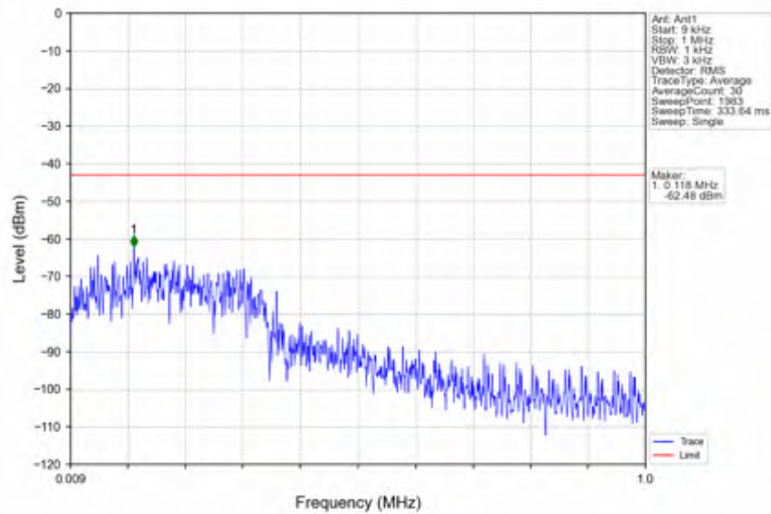
n25_30kHz_SISO_NTNV_15MHz_DFT-s-OFDM_QPSK_1857.5MHz_Edge_1RB_Left
