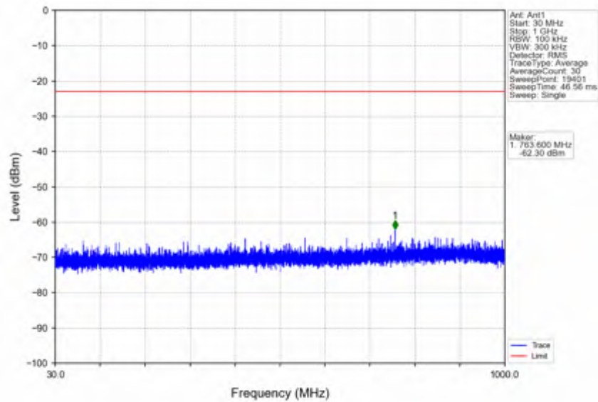
n25_30kHz_SISO_NTNV_10MHz_DFT-s-OFDM QPSK_1910MHz_Edge_1RB_Right
