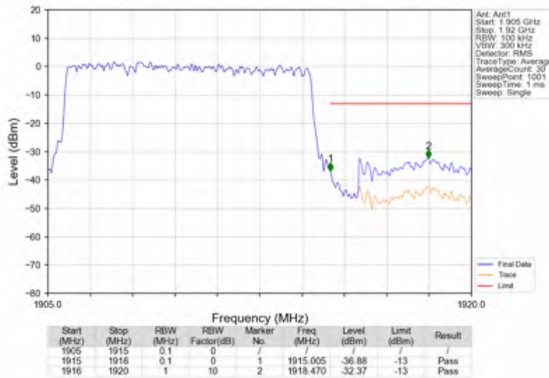
n25_30kHz_SISO_NTNV_10MHz_DFT-s-OFDM PI/2 BPSK_1910MHz_Outer_Full
