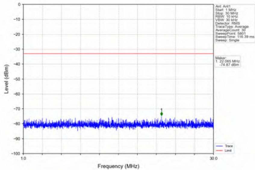
n25_30kHz_SISO_NTNV_15MHz_DFT-s-OFDM_QPSK_1907.5MHz_Outer_Full
