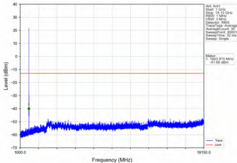
n25_30kHz_SISO_NTNV_15MHz_DFT-s-OFDM QPSK_1857.5MHz_Edge_1RB_Left
