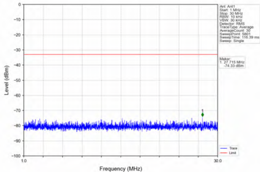
n25_15kHz_SISO_NTNV_40MHz_DFT-s-OFDM_QPSK_1895MHz_Edge_1RB_Right
