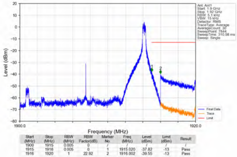
n25_30kHz_SISO_NTNV_15MHz_DFT-s-OFDM QPSK_1907.5MHz_Edge_1RB_Right
