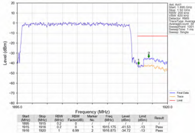
n25_30kHz_SISO_NTNV_20MHz_DFT-s-OFDM QPSK_1905MHz_Outer_Full
