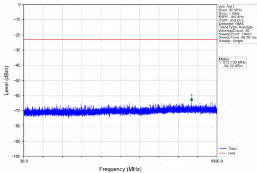
n25_15kHz_SISO_NTNV_40MHz_CP-OFDM QPSK_1870MHz_Outer_Full
