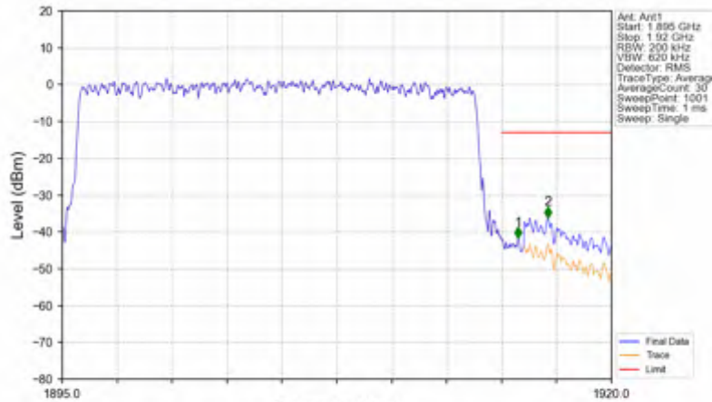
n25_30kHz_SISO_NTNV_20MHz_DFT-s-OFDM PI/2 BPSK_1905MHz_Outer_Full
