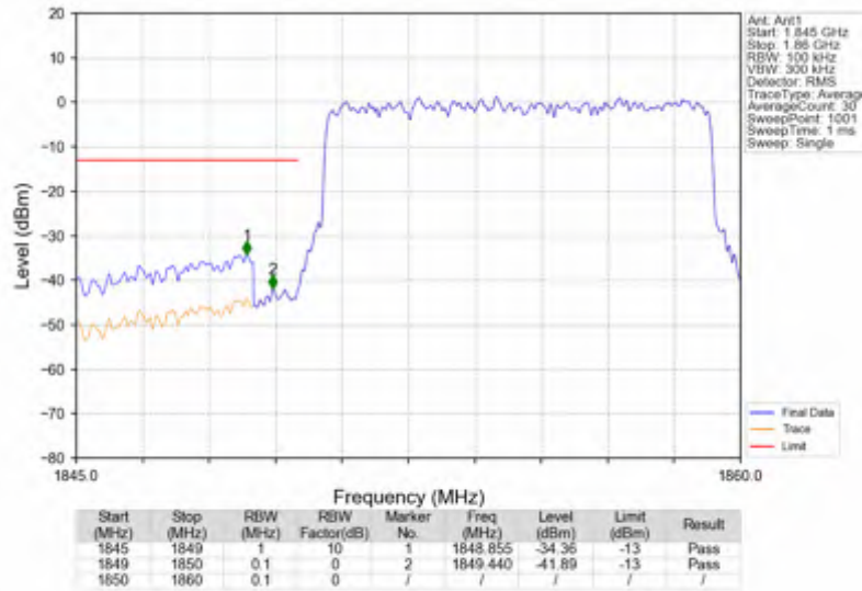
n25_30kHz_SISO_NTNV_10MHz_DFT-s-OFDM QPSK_1855MHz_Outer_Full
