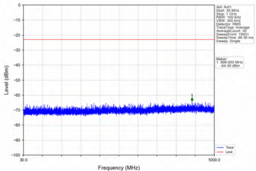
n25_30kHz_SISO_NTNV_10MHz_CP-OFDM QPSK_1910MHz_Edge_1RB_Right
