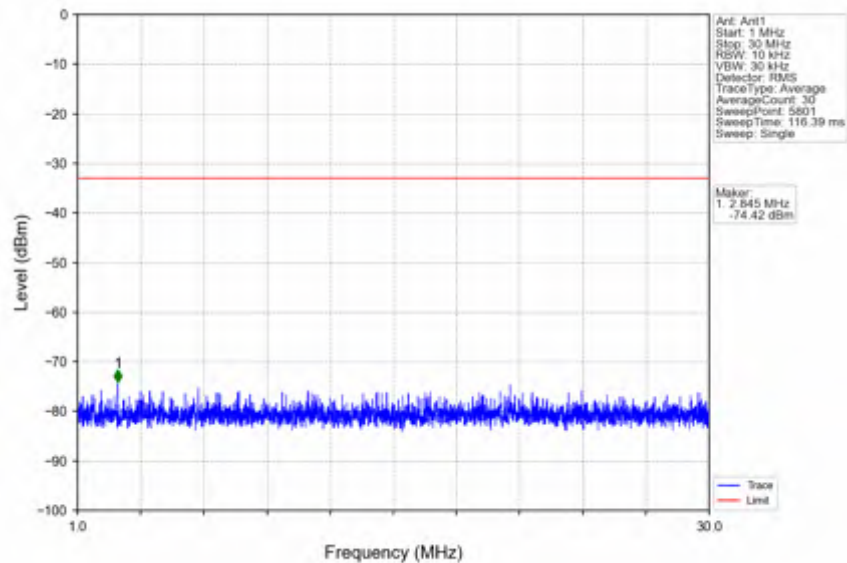
n25_30kHz_SISO_NTNV_15MHz_DFT-s-OFDM PI/2 BPSK_1882.5MHz_Edge_1RB_Left
