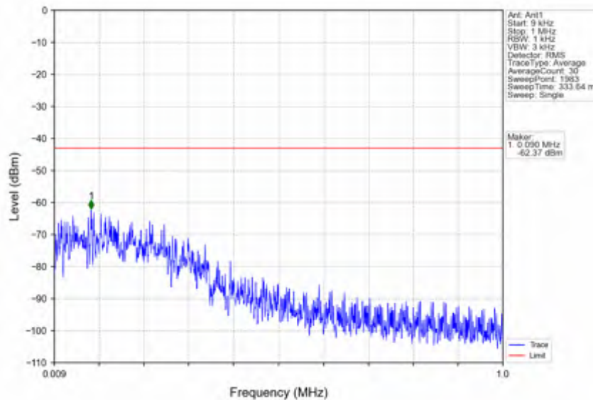
n25_30kHz_SISO_NTV_15MHz_CP-OFDM QPSK_1857.5MHz_Edge_1RB_Left
