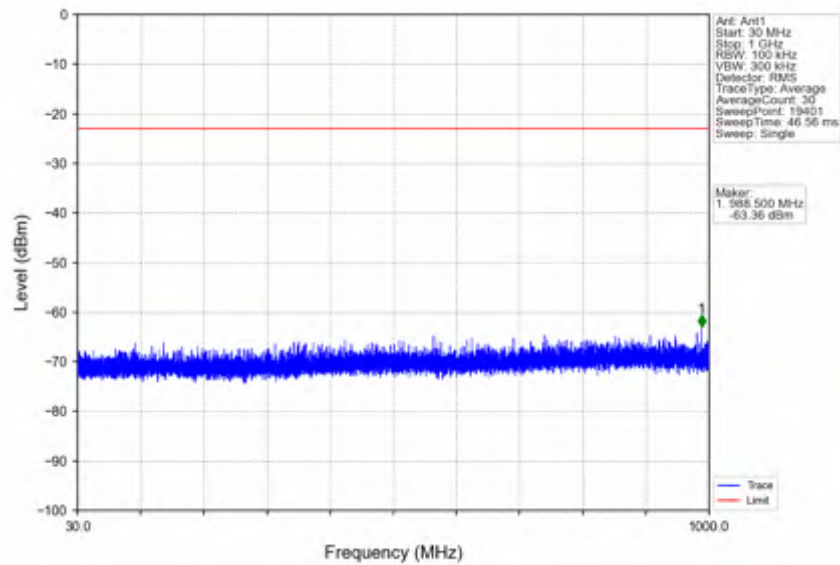
n25_30kHz_SISO_NTNV_20MHz_CP-OFDM QPSK_1860MHz_Outer_Full
