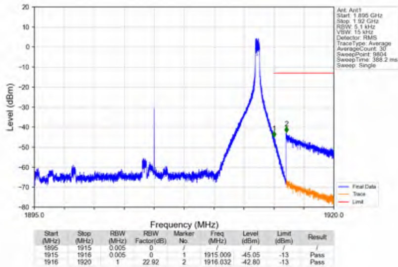
n25_30kHz_SISO_NTNV_20MHz_DFT-s-OFDM QPSK_1905MHz_Inner_1RB_Right
