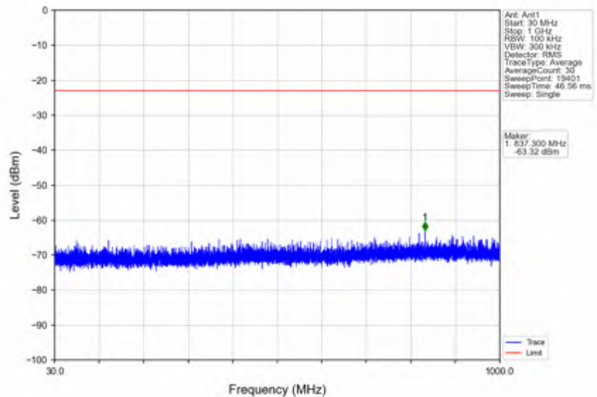
n25_15kHz_SISO_NTNV_40MHz_DFT-s-OFDM_QPSK_1882.5MHz_Edge_1RB_Left
