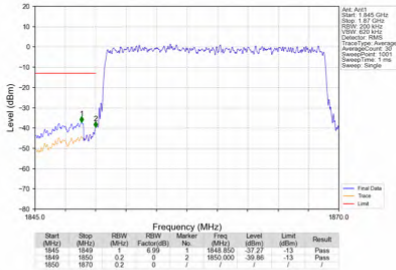
n25_30kHz_SISO_NTNV_20MHz_DFT-s-OFDM QPSK_1860MHz_Outer_Full
