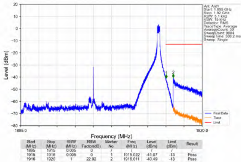
n25_30kHz_SISO_NTNV_20MHz_DFT-s-OFDM QPSK_1905MHz_Edge_1RB_Right
