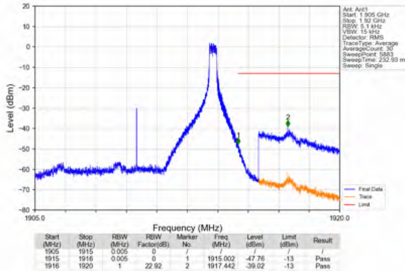
n25_30kHz_SISO_NTNV_10MHz_CP-OFDM QPSK_1910MHz_Inner_1RB_Right
