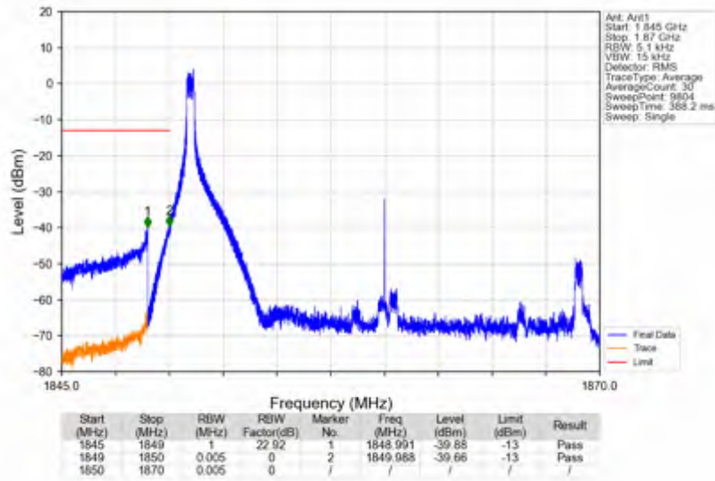
n25_30kHz_SISO_NTNV_20MHz_DFT-s-OFDM_PI/2_BPSK_1860MHz_Edge_1RB_Left
