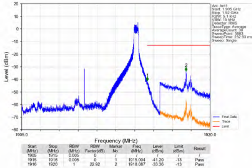
n25_30kHz_SISO_NTNV_10MHz_DFT-s-OFDM PI/2 BPSK_1910MHz_Edge_1RB_Right
