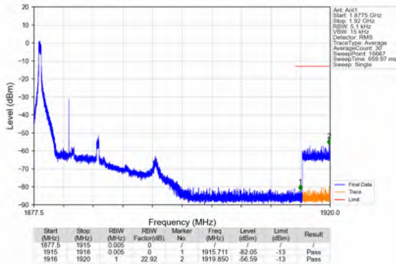
n25_30kHz_SISO_NTNV_10MHz_CP-OFDM QPSK_1882.5MHz_Edge_1RB_Left
