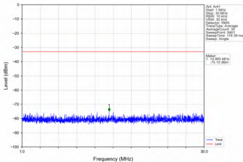
n25_30kHz_SISO_NTNV_20MHz_DFT-s-OFDM QPSK_1905MHz_Edge_1RB_Right
