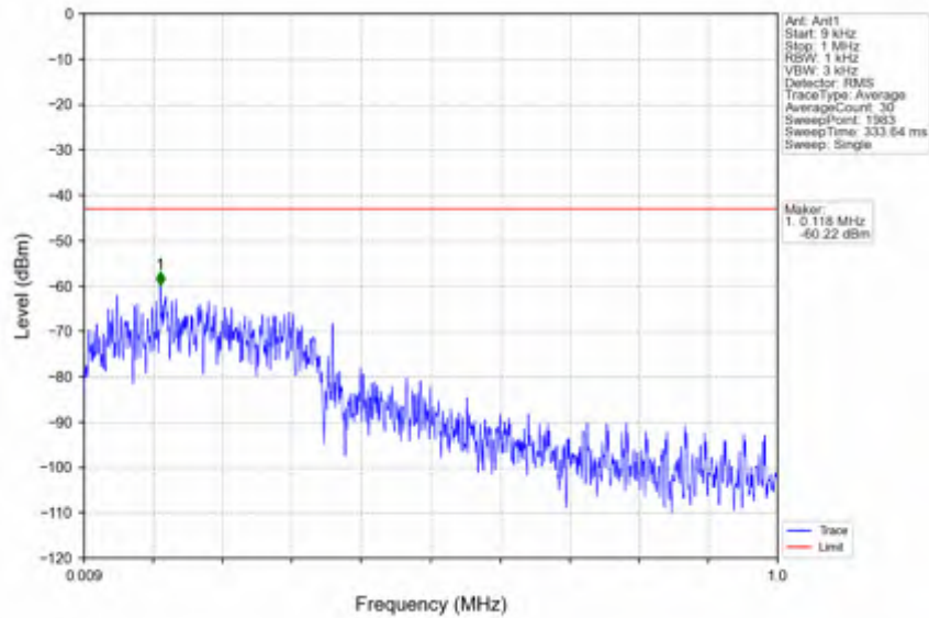
n25_30kHz_SISO_NTNV_15MHz_DFT-s-OFDM_QPSK_1857.5MHz_Inner_1RB_Left
