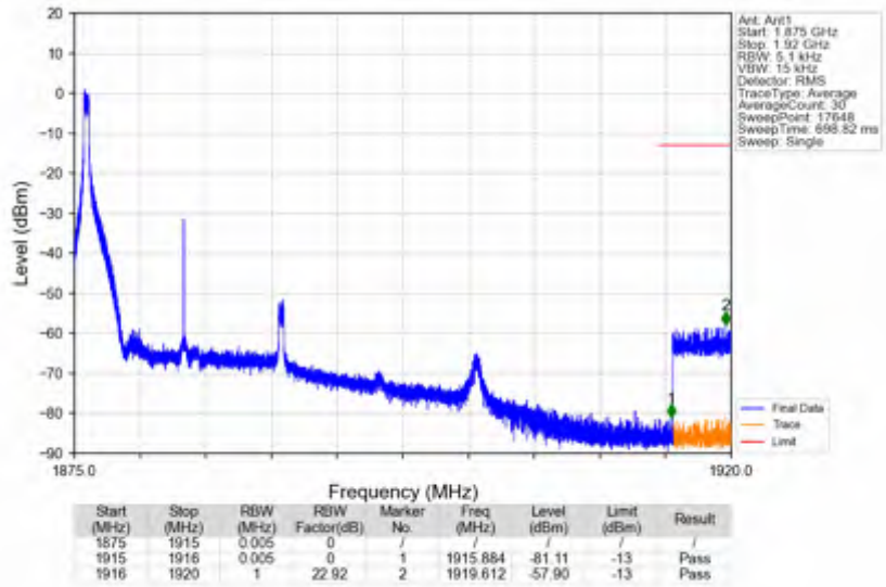
n25_30kHz_SISO_NTV_15MHz_CP-OFDM QPSK_1882.5MHz_Edge_1RB_Left
