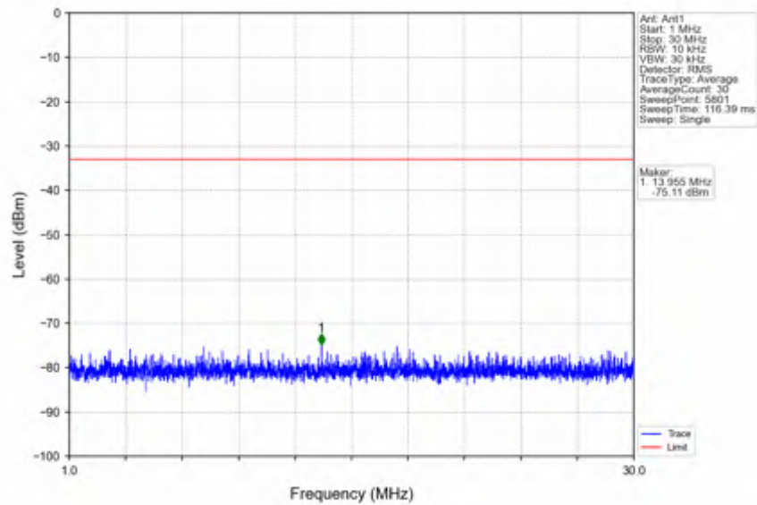
n25_15kHz_SISO_NTNV_40MHz_CP-OFDM QPSK_1870MHz_Edge_1RB_Left
