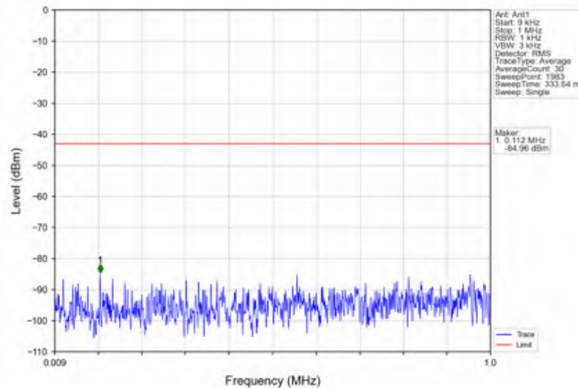
n25_30kHz_SISO_NTNV_20MHz_DFT-s-OFDM QPSK_1905MHz_Outer_Full
