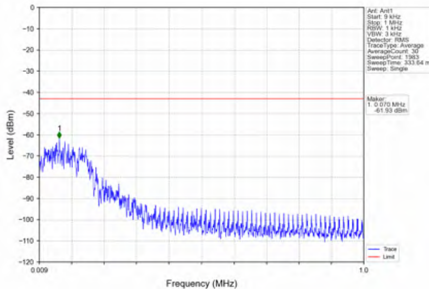
n25_15kHz_SISO_NTNV_40MHz_DFT-s-OFDM QPSK_1882.5MHz_Edge_1RB_Left
