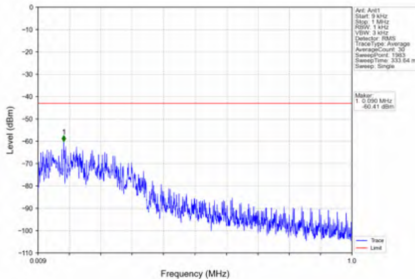
n25_30kHz_SISO_NTNV_10MHz_CP-OFDM QPSK_1910MHz_Edge_1RB_Right
