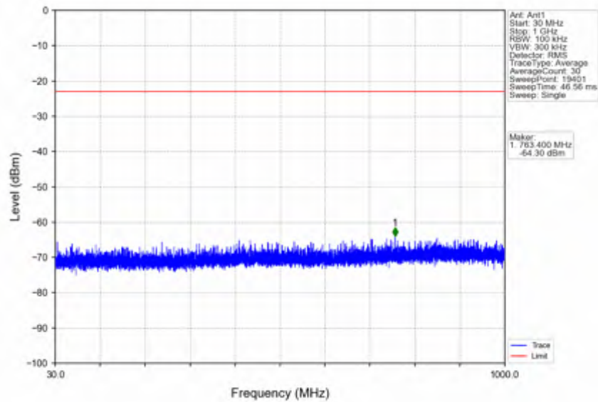
n25_30kHz_SISO_NTVV_15MHz_CP-OFDM QPSK_1882.5MHz_Edge_1RB_Left
