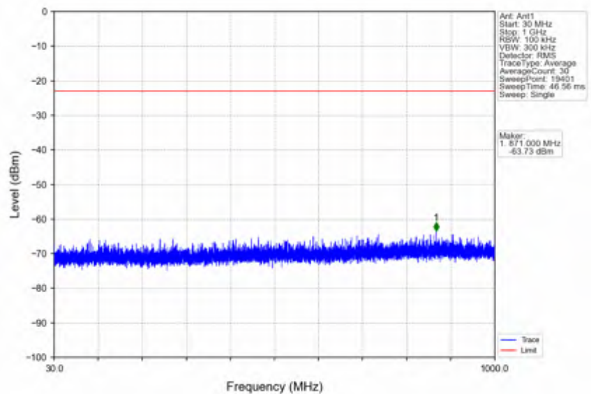
n25_30kHz_SISO_NTNV_10MHz_CP-OFDM QPSK_1855MHz_Edge_1RB_Left
