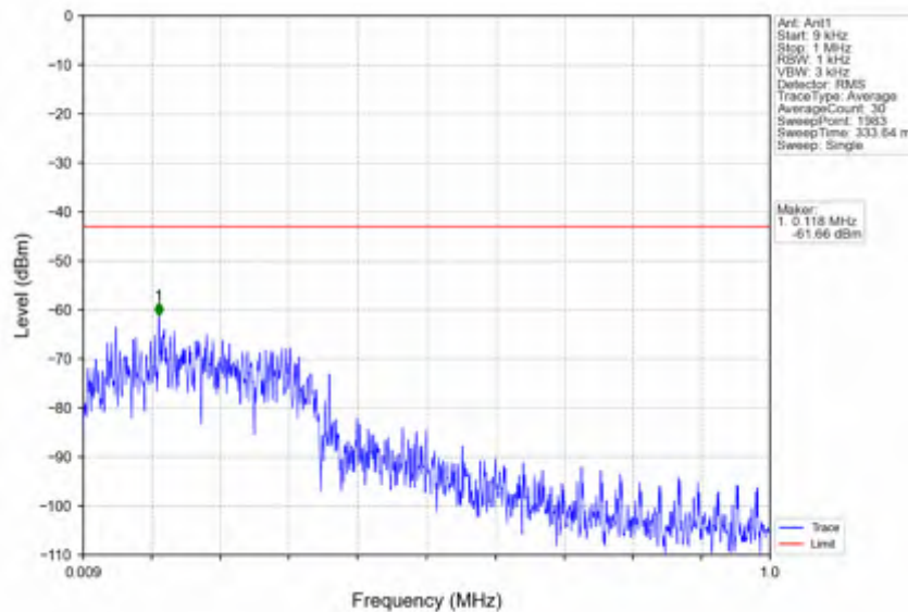
n25_30kHz_SISO_NTNV_10MHz_DFT-s-OFDM QPSK_1882.5MHz_Edge_1RB_Left
