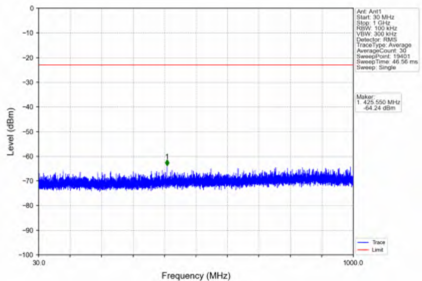
n25_15kHz_SISO_NTNV_40MHz_CP-OFDM QPSK_1895MHz_Inner_1RB_Right
