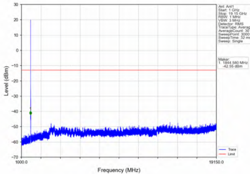
n25_30kHz_SISO_NTNV_15MHz_CP-OFDM QPSK_1857.5MHz_Outer_Full
