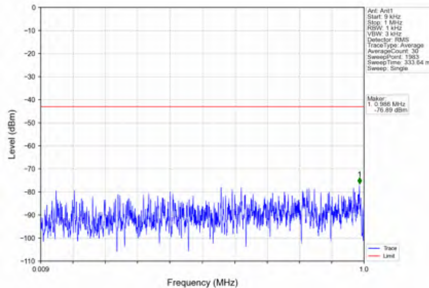
n25_30kHz_SISO_NTNV_10MHz_DFT-s-OFDM QPSK_1910MHz_Outer_Full
