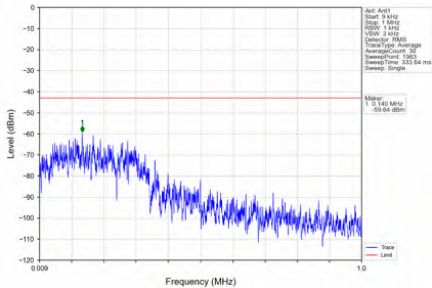
n25_30kHz_SISO_NTNV_15MHz_DFT-s-OFDM QPSK_1907.5MHz_Edge_1RB_Right
