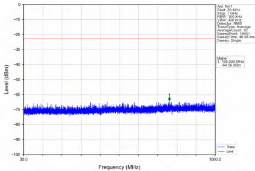
n25_15kHz_SISO_NTNV_40MHz_DFT-s-OFDM QPSK_1895MHz_Edge_1RB_Right
