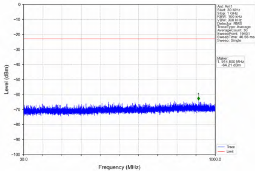
n25_30kHz_SISO_NTNV_20MHz_DFT-s-OFDM QPSK_1905MHz_Edge_1RB_Right
