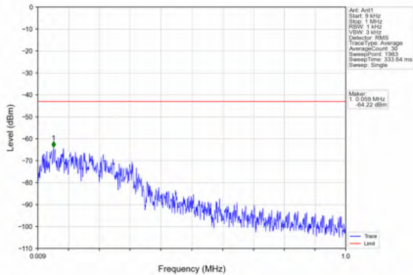
n25_30kHz_SISO_NTV_20MHz_CP-OFDM QPSK_1882.5MHz_Edge_1RB_Left
