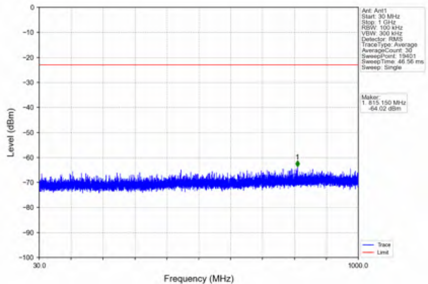
n25_30kHz_SISO_NTNV_15MHz_DFT-s-OFDM_QPSK_1882.5MHz_Edge_1RB_Left
