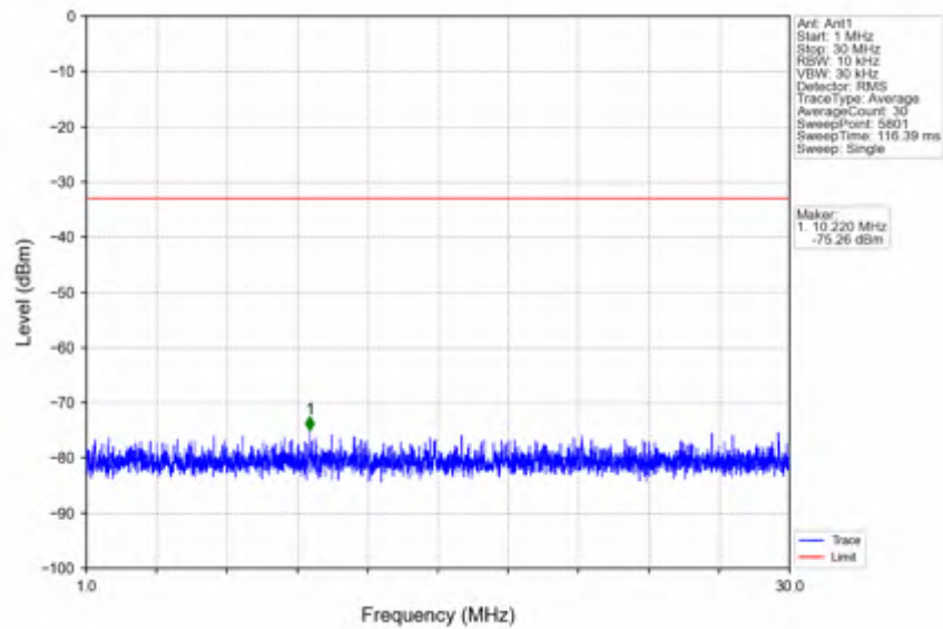
n25_30kHz_SISO_NTNV_10MHz_DFT-s-OFDM_QPSK_1882.5MHz_Edge_1RB_Left
