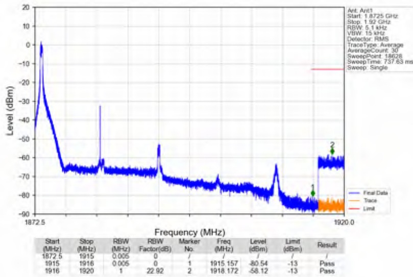
n25_30kHz_SISO_NTNV_20MHz_CP-OFDM QPSK_1882.5MHz_Edge_1RB_Left
