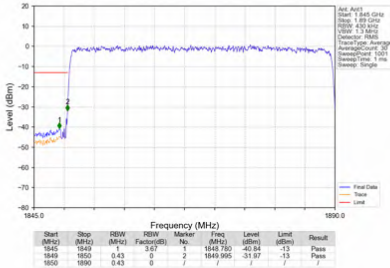
n25_15kHz_SISO_NTNV_40MHz_DFT-s-OFDM QPSK_1870MHz_Outer_Full
