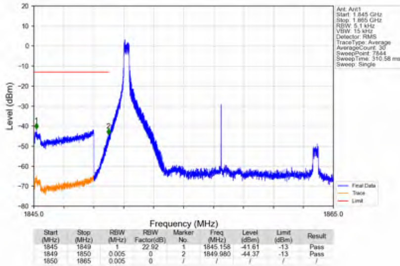
n25_30kHz_SISO_NTV_15MHz_CP-OFDM_QPSK_1857.5MHz_Inner_1RB_Left
