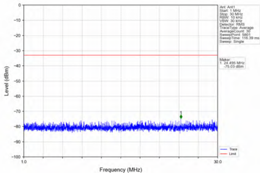
n25_30kHz_SISO_NTNV_15MHz_CP-OFDM QPSK_1907.5MHz_Outer_Full
