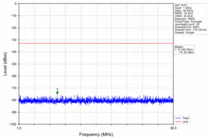
n25_30kHz_SISO_NTV_15MHz_CP-OFDM QPSK_1882.5MHz_Edge_1RB_Left
