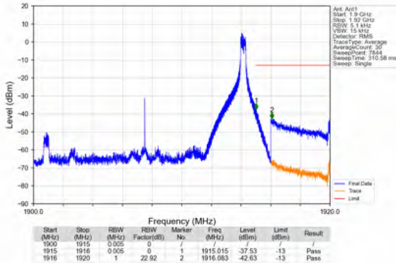
n25_30kHz_SISO_NTNV_15MHz_DFT-s-OFDM PI/2 BPSK_1907.5MHz_Edge_1RB_Right
