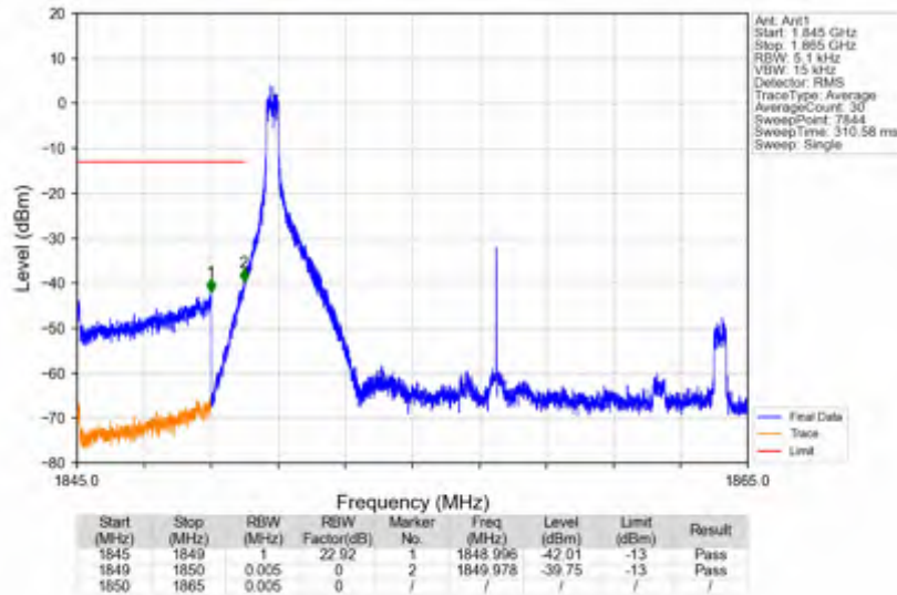
n25_30kHz_SISO_NTNV_15MHz_DFT-s-OFDM QPSK_1857.5MHz_Edge_1RB_Left
