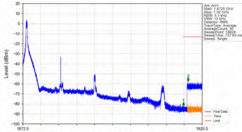
n25_30kHz_SISO_NTNV_20MHz_DFT-s-OFDM_QPSK_1882.5MHz_Edge_1RB_Left
