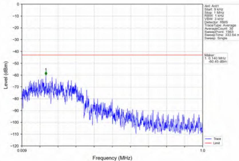
n25_30kHz_SISO_NTNV_15MHz_DFT-s-OFDM QPSK_1882.5MHz_Edge_1RB_Left
