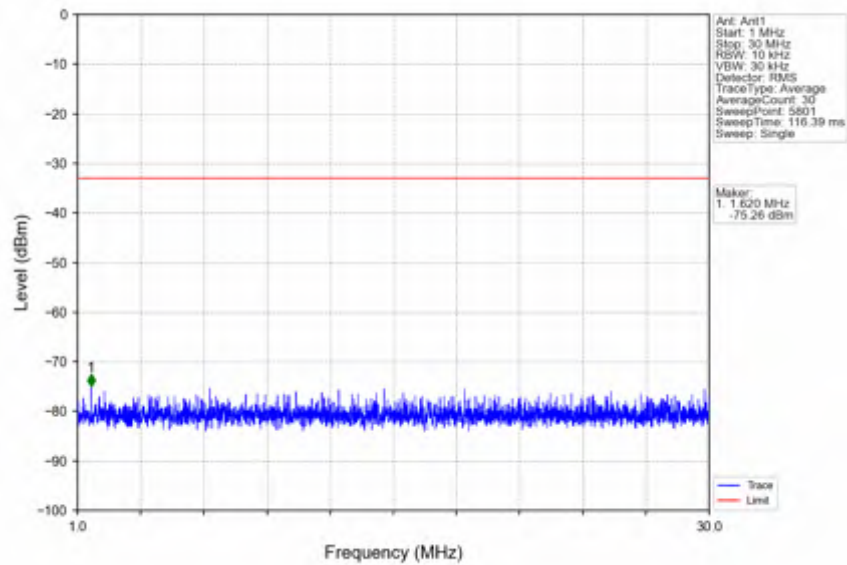
n25_30kHz_SISO_NTNV_15MHz_DFT-s-OFDM_QPSK_1857.5MHz_Outer_Full
