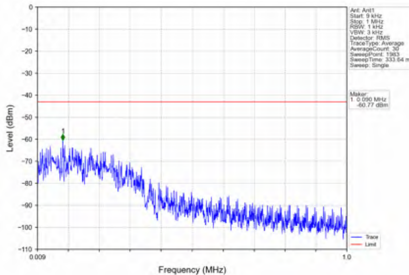
n25_30kHz_SISO_NTNV_20MHz_CP-OFDM QPSK_1905MHz_Edge_1RB_Right
