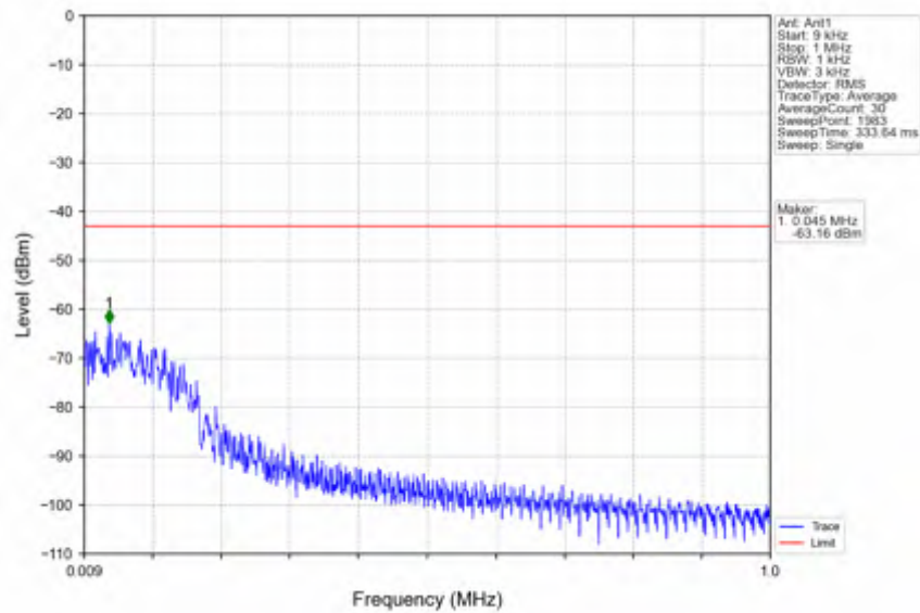
n25_15kHz_SISO_NTVV_40MHz_CP-OFDM QPSK_1882.5MHz_Edge_1RB_Left
