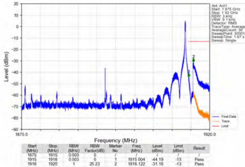
n25_15kHz_SISO_NTNV_40MHz_DFT-s-OFDM QPSK_1895MHz_Inner_1RB_Right
