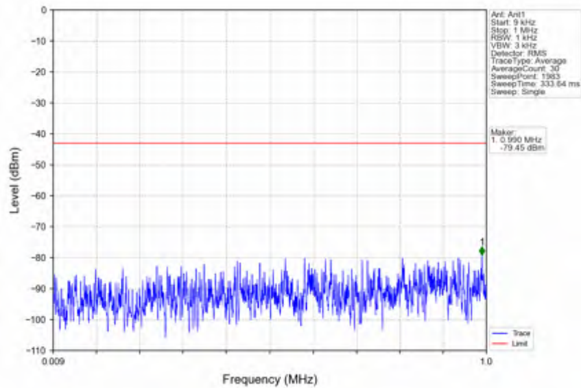
n25_30kHz_SISO_NTNV_10MHz_DFT-s-OFDM PI/2 BPSK_1855MHz_Outer_Full
