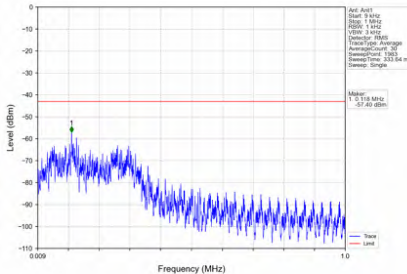
n25_30kHz_SISO_NTNV_15MHz_DFT-s-OFDM PI/2 BPSK_1907.5MHz_Inner_1RB_Right
