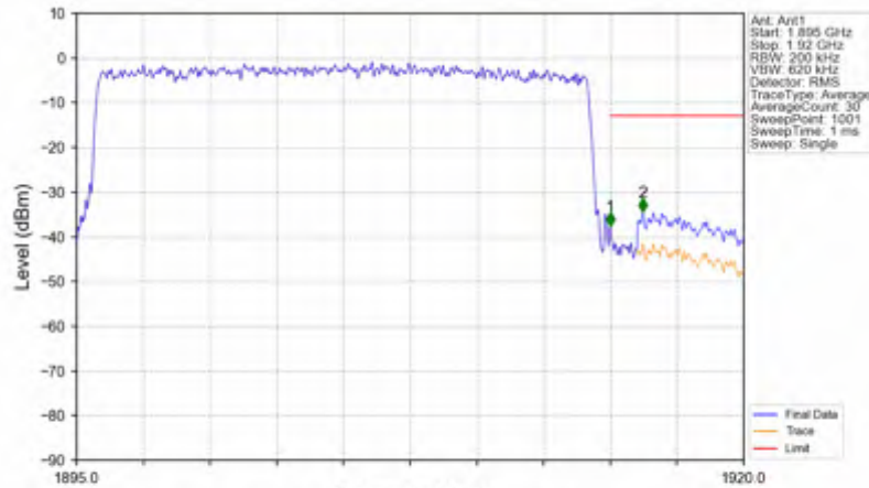
n25_30kHz_SISO_NTNV_20MHz_CP-OFDM QPSK_1905MHz_Outer_Full
