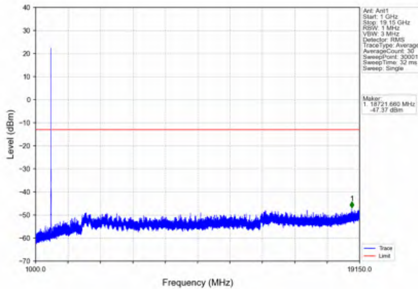
n25_30kHz_SISO_NTNV_10MHz_DFT-s-OFDM QPSK_185MHz_Edge_1RB_Left
