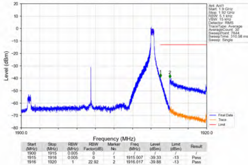
n25_30kHz_SISO_NTV_15MHz_CP-OFDM QPSK_1907.5MHz_Edge_1RB_Right
