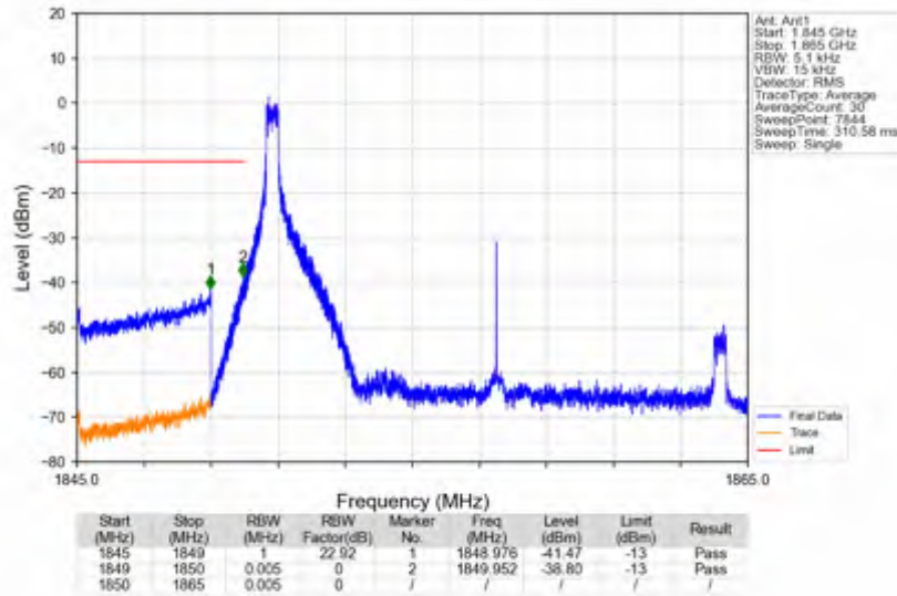
n25_30kHz_SISO_NTV_15MHz_CP-OFDM QPSK_1857.5MHz_Edge_1RB_Left
