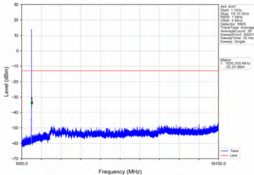
n25_30kHz_SISO_NTNV_15MHz_DFT-s-OFDM PI/2 BPSK_1907.5MHz_Outer_Full
