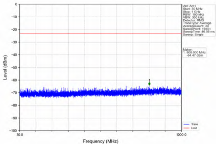
n25_30kHz_SISO_NTNV_10MHz_DFT-s-OFDM_PI/2_BPSK_1855MHz_Edge_1RB_Left
