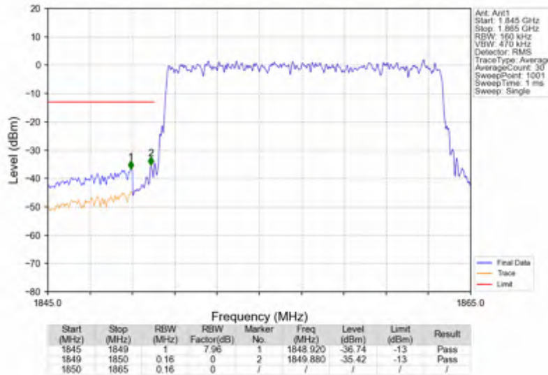
n25_30kHz_SISO_NTNV_15MHz_DFT-s-OFDM QPSK_1857.5MHz_Outer_Full
