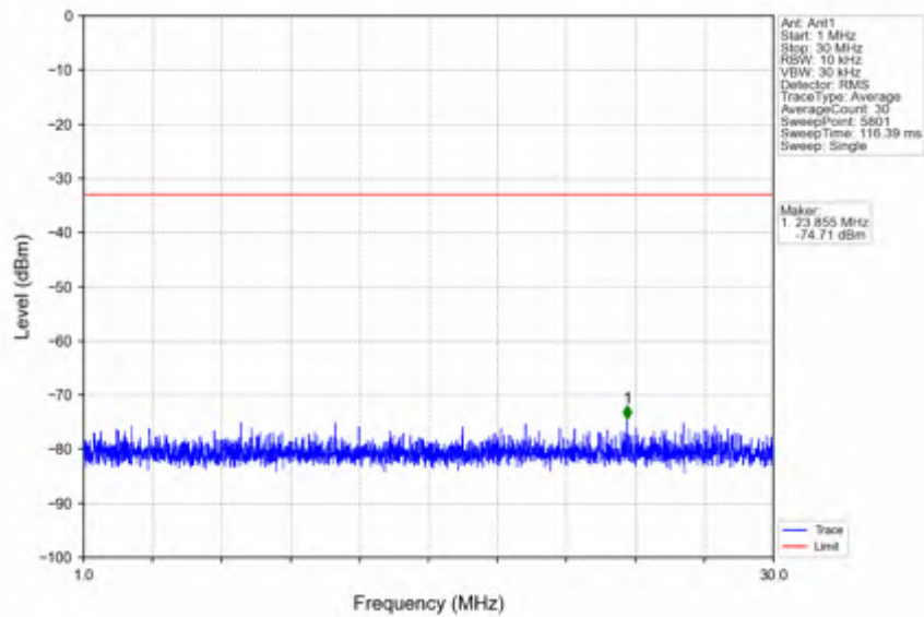
n25_30kHz_SISO_NTNV_15MHz_CP-OFDM QPSK_1907.5MHz_Edge_1RB_Right
