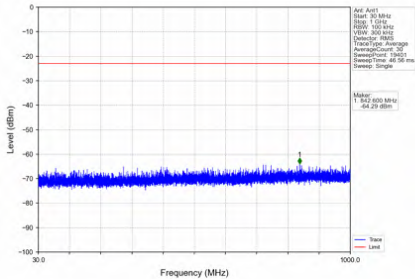
n25_30kHz_SISO_NTNV_20MHz_DFT-s-OFDM QPSK_1905MHz_Inner_1RB_Right
