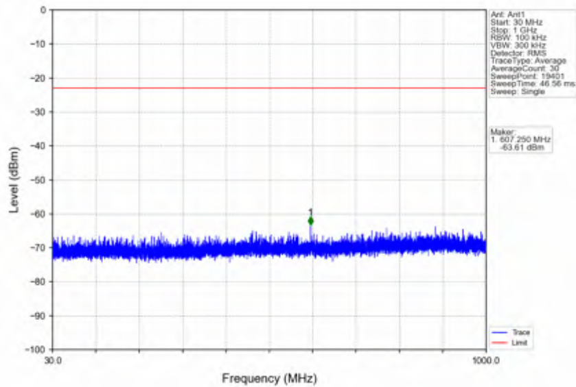
n25_30kHz_SISO_NTNV_20MHz_DFT-s-OFDM QPSK_1860MHz_Edge_1RB_Left
