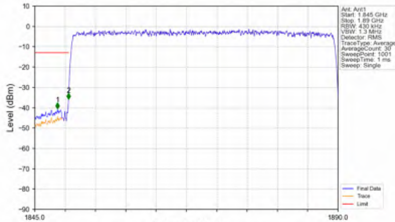
n25_15kHz_SISO_NTNV_40MHz_CP-OFDM QPSK_1870MHz_Outer_Full
