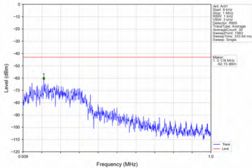
n25_30kHz_SISO_NTNV_10MHz_DFT-s-OFDM QPSK_185MHz_Edge_1RB_Left
