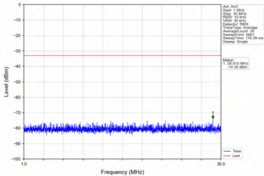
n25_30kHz_SISO_NTNV_20MHz_CP-OFDM QPSK_1905MHz_Edge_1RB_Right
