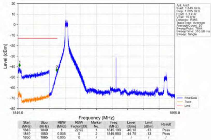
n25_30kHz_SISO_NTNV_15MHz_DFT-s-OFDM QPSK_1857.5MHz_Inner_1RB_Left
