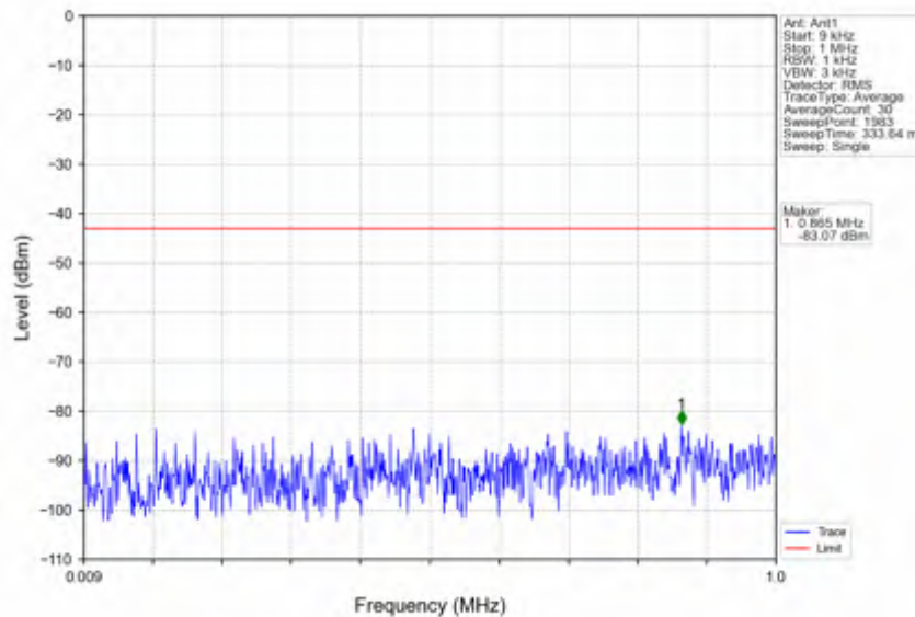
n25_30kHz_SISO_NTNV_15MHz_DFT-s-OFDM QPSK_1907.5MHz_Outer_Full
