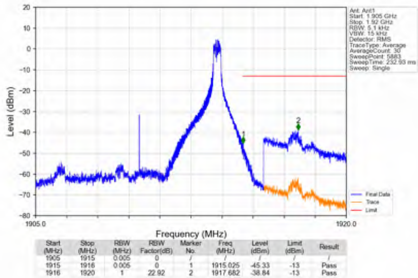
n25_30kHz_SISO_NTNV_10MHz_DFT-s-OFDM QPSK_1910MHz_Inner_1RB_Right
