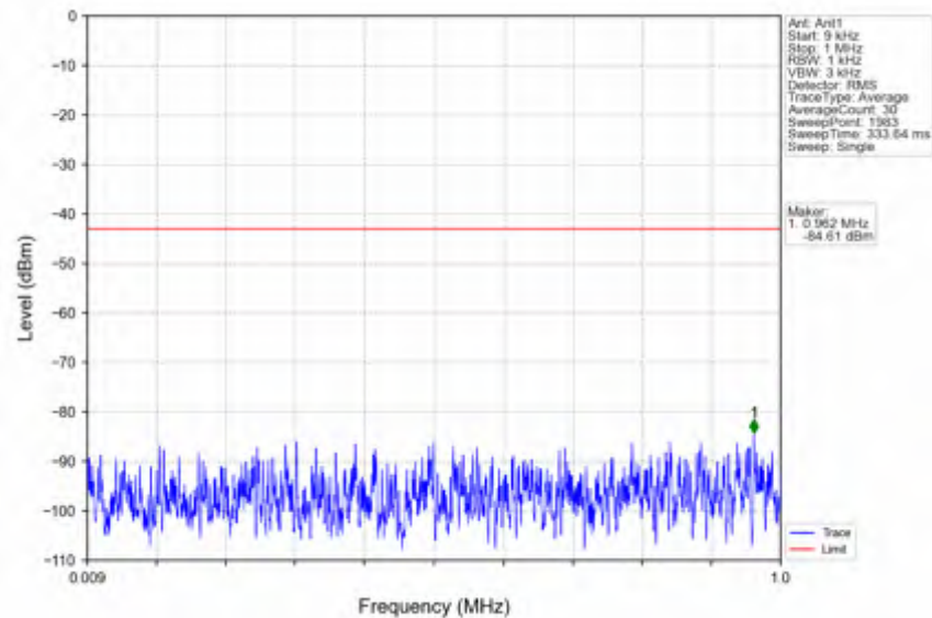
n25_30kHz_SISO_NTNV_20MHz_DFT-s-OFDM QPSK_1860MHz_Outer_Full
