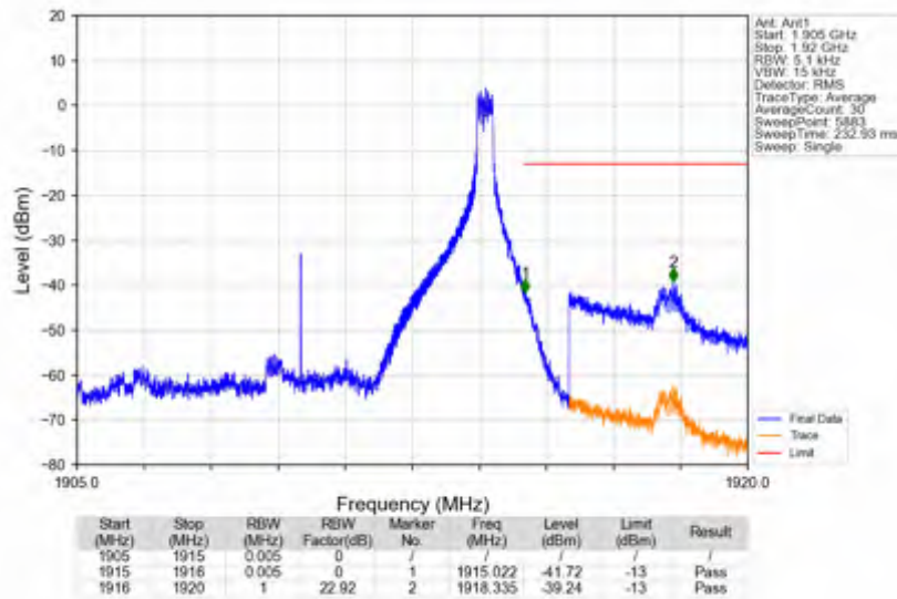
n25_30kHz_SISO_NTNV_10MHz_DFT-s-OFDM QPSK_1910MHz_Edge_1RB_Right
