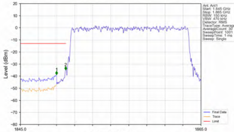
n25_30kHz_SISO_NTNV_15MHz_DFT-s-OFDM PI/2 BPSK_1857.5MHz_Outer_Full
