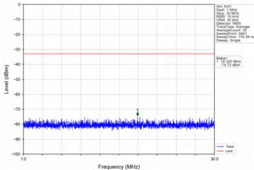
n25_30kHz_SISO_NTNV_15MHz_DFT-s-OFDM QPSK_1907.5MHz_Inner_1RB_Right
