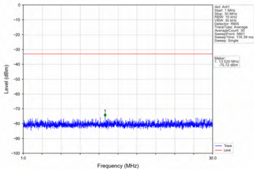
n25_30kHz_SISO_NTNV_20MHz_DFT-s-OFDM QPSK_1860MHz_Edge_1RB_Left
