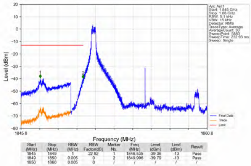
n25_30kHz_SISO_NTNV_10MHz_DFT-s-OFDM QPSK_1855MHz_Edge_1RB_Left
