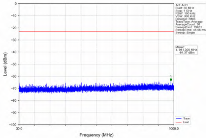
n25_15kHz_SISO_NTVV_40MHz_CP-OFDM QPSK_1882.5MHz_Edge_1RB_Left
