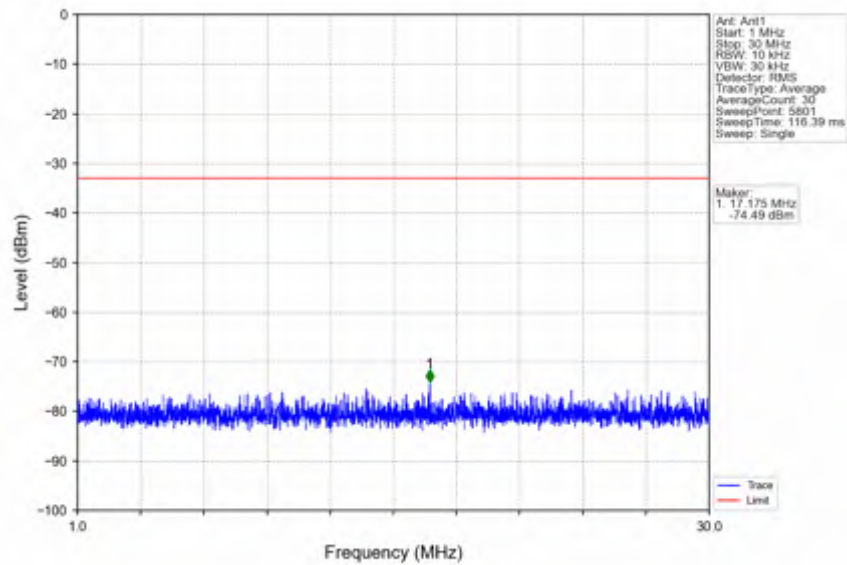
n25_30kHz_SISO_NTNV_15MHz_CP-OFDM QPSK_1857.5MHz_Inner_1RB_Left
