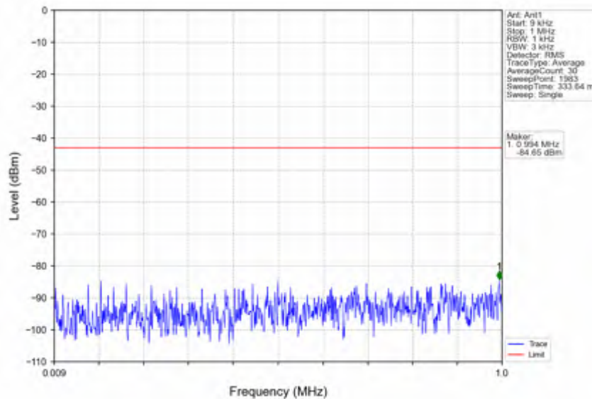
n25_30kHz_SISO_NTNV_15MHz_DFT-s-OFDM QPSK_1857.5MHz_Outer_Full
