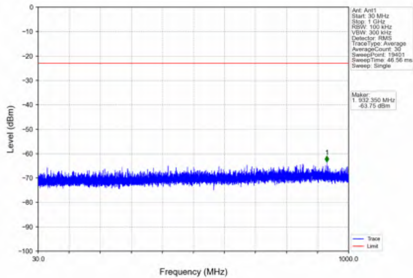
n25_30kHz_SISO_NTVV_20MHz_CP-OFDM QPSK_1882.5MHz_Edge_1RB_Left
