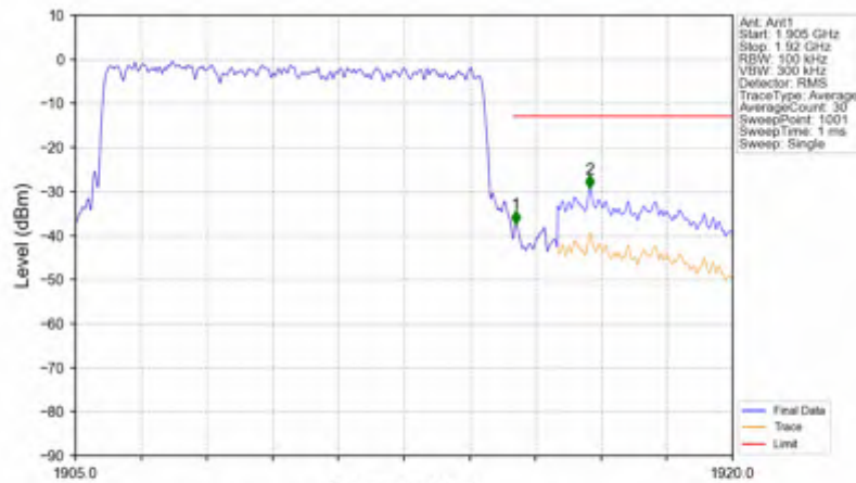
n25_30kHz_SISO_NTNV_10MHz_CP-OFDM QPSK_1910MHz_Outer_Full
