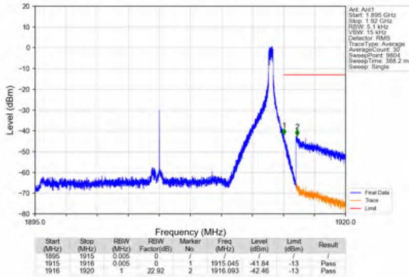
n25_30kHz_SISO_NTNV_20MHz_CP-OFDM QPSK_1905MHz_Edge_1RB_Right
