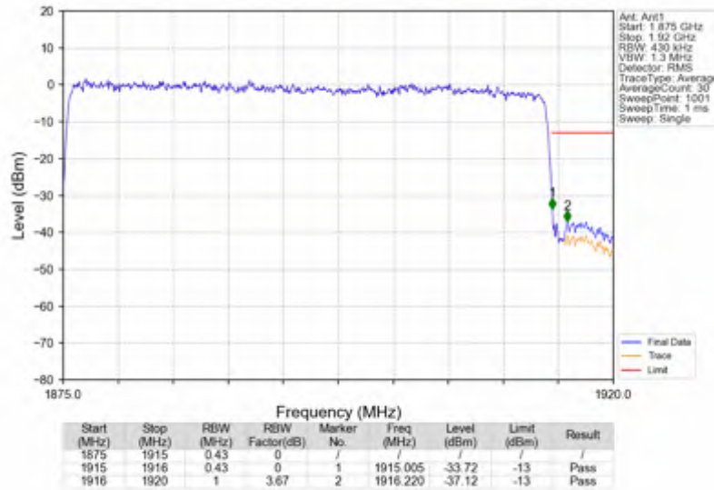
n25_15kHz_SISO_NTNV_40MHz_DFT-s-OFDM QPSK_1895MHz_Outer_Full
