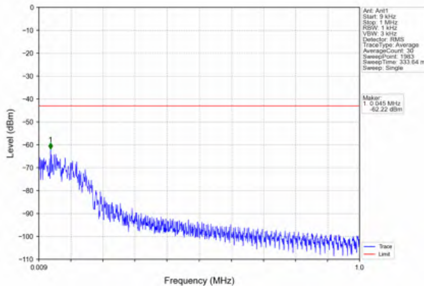
n25_15kHz_SISO_NTNV_40MHz_CP-OFDM QPSK_1870MHz_Edge_1RB_Left
