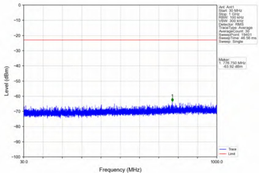
n25_30kHz_SISO_NTNV_20MHz_DFT-s-OFDM PI/2 BPSK_1860MHz_Edge_1RB_Left
