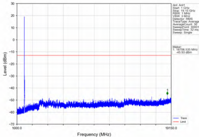
n25_15kHz_SISO_NTVV_40MHz_CP-OFDM QPSK_1882.5MHz_Edge_1RB_Left
