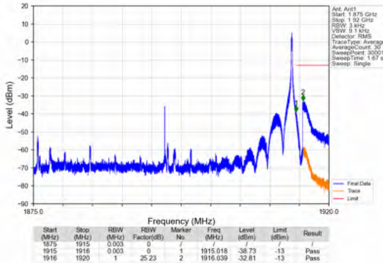
n25_15kHz_SISO_NTNV_40MHz_DFT-s-OFDM QPSK_1895MHz_Edge_1RB_Right
