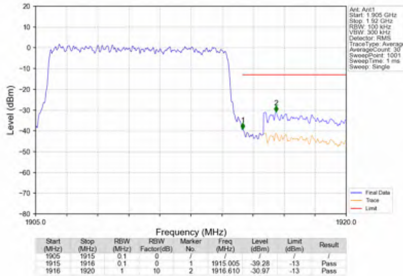
n25_30kHz_SISO_NTNV_10MHz_DFT-s-OFDM QPSK_1910MHz_Outer_Full
