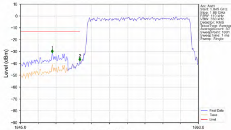
n25_30kHz_SISO_NTNV_10MHz_CP-OFDM QPSK_1855MHz_Outer_Full
