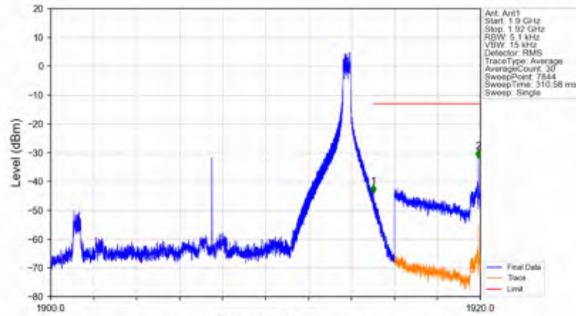
n25_30kHz_SISO_NTNV_15MHz_DFT-s-OFDM PI/2 BPSK_1907.5MHz_Inner_1RB_Right
