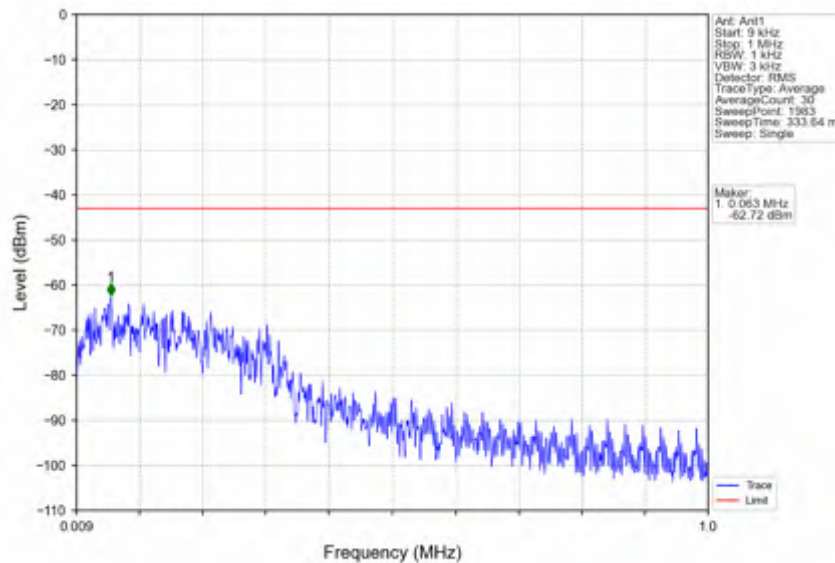
n25_30kHz_SISO_NTV_15MHz_CP-OFDM QPSK_1907.5MHz_Edge_1RB_Right
