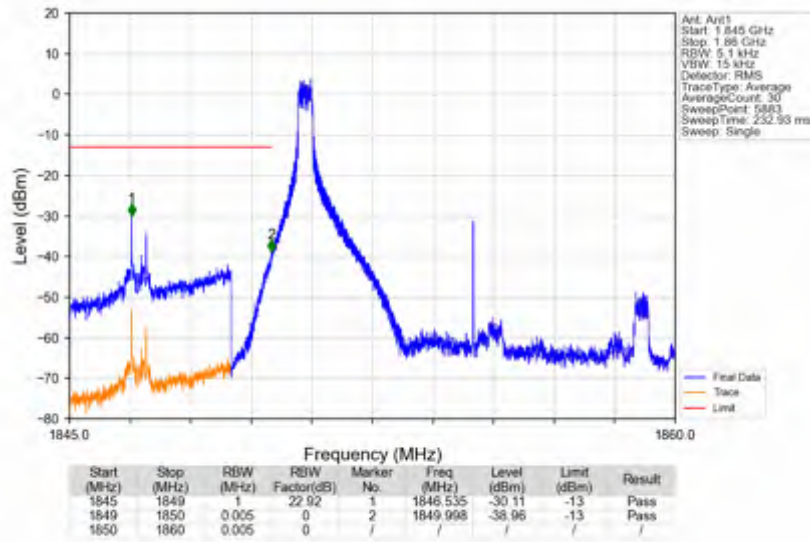
n25_30kHz_SISO_NTNV_10MHz_DFT-s-OFDM_PI/2_BPSK_1855MHz_Edge_1RB_Left
