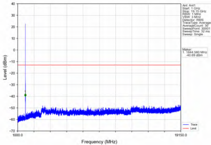
n25_30kHz_SISO_NTNV_15MHz_DFT-s-OFDM PI/2 BPSK_1882.5MHz_Edge_1RB_Left
