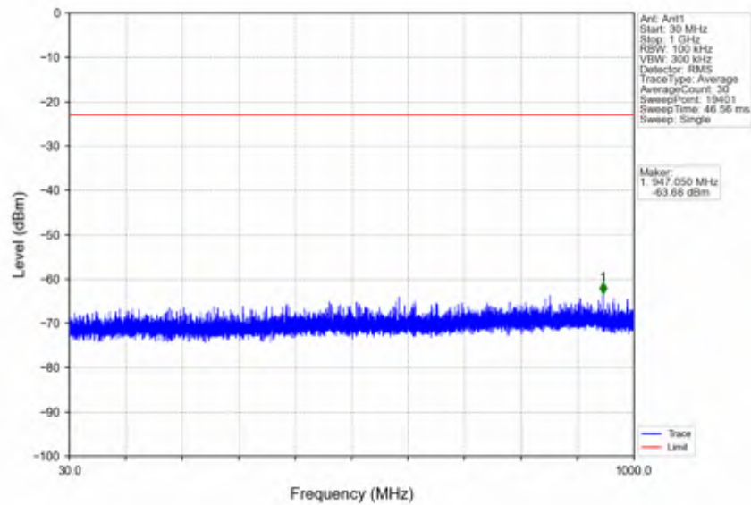
n25_30kHz_SISO_NTNV_15MHz_DFT-s-OFDM_QPSK_1857.5MHz_Inner_1RB_Left
