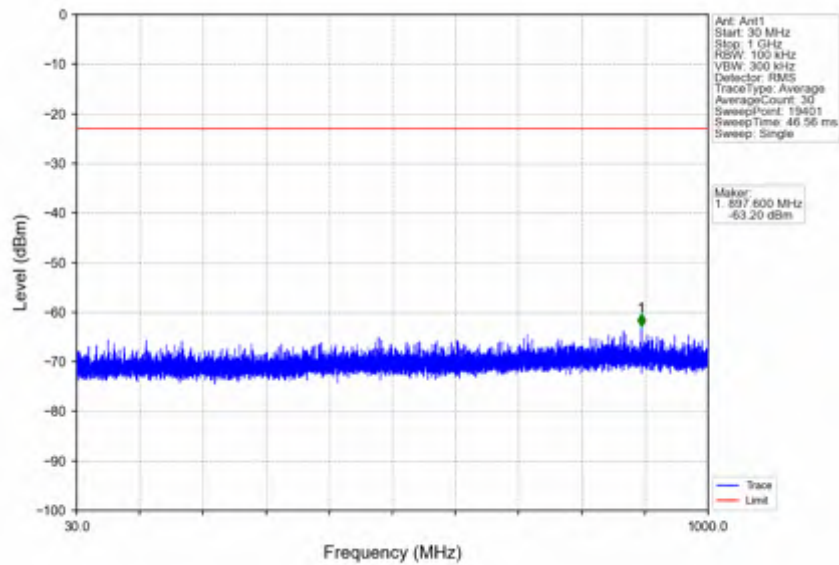
n25_30kHz_SISO_NTNV_15MHz_CP-OFDM QPSK_1907.5MHz_Outer_Full
