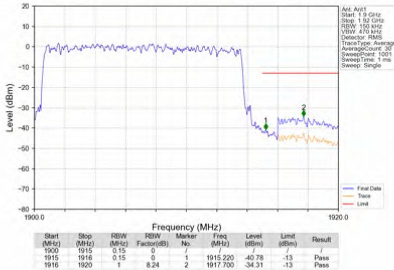
n25_30kHz_SISO_NTNV_15MHz_DFT-s-OFDM QPSK_1907.5MHz_Outer_Full
