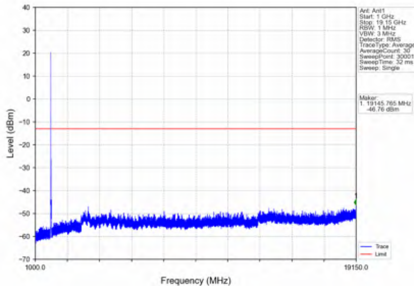
n25_30kHz_SISO_NTVV_20MHz_CP-OFDM QPSK_1882.5MHz_Edge_1RB_Left
