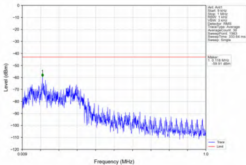
n25_30kHz_SISO_NTNV_20MHz_DFT-s-OFDM_PI/2_BPSK_1860MHz_Edge_1RB_Left
