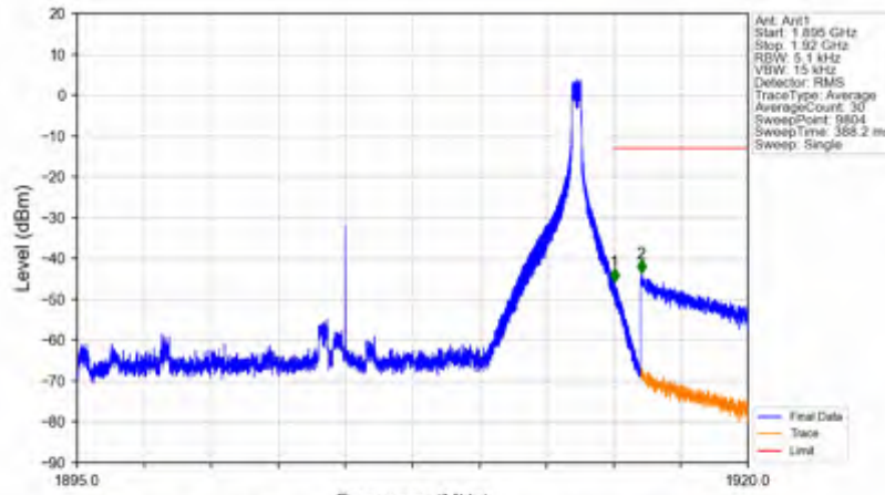
n25_30kHz_SISO_NTNV_20MHz_DFT-s-OFDM PI/2 BPSK_1905MHz_Inner_1RB_Right
