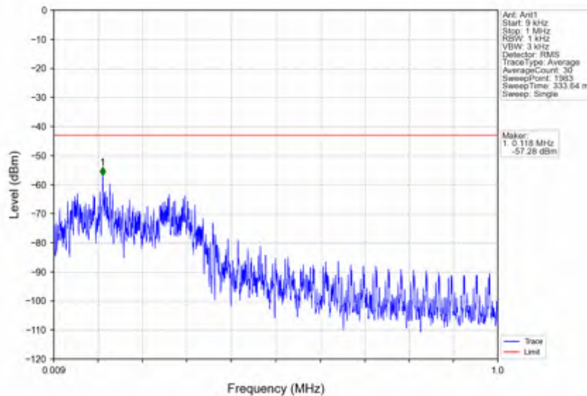
n25_30kHz_SISO_NTNV_20MHz_DFT-s-OFDM PI/2 BPSK_1905MHz_Inner_1RB_Right
