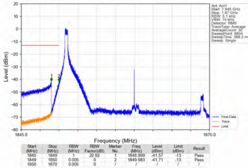
n25_30kHz_SISO_NTNV_20MHz_CP-OFDM QPSK_1860MHz_Edge_1RB_Left
