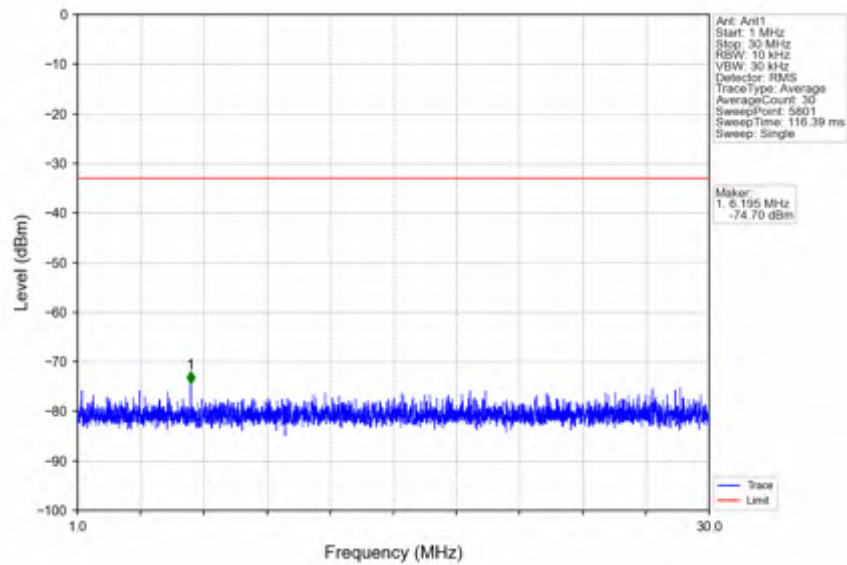
n25_30kHz_SISO_NTVV_15MHz_CP-OFDM QPSK_1857.5MHz_Edge_1RB_Left
