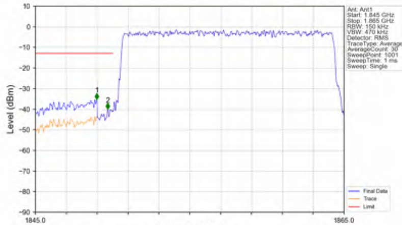
n25_30kHz_SISO_NTNV_15MHz_CP-OFDM QPSK_1857.5MHz_Outer_Full
