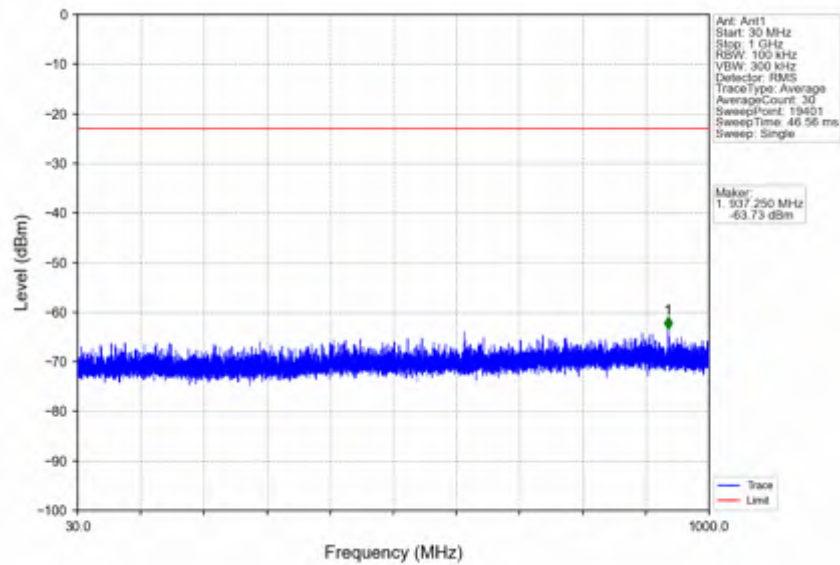
n25_30kHz_SISO_NTNV_20MHz_CP-OFDM QPSK_1905MHz_Outer_Full
