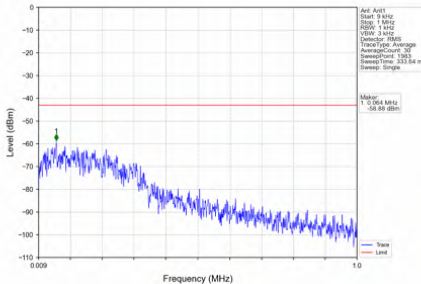
n25_30kHz_SISO_NTNV_10MHz_CP-OFDM QPSK_1910MHz_Inner_1RB_Right
