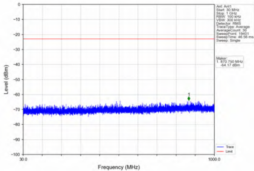
n25_30kHz_SISO_NTNV_15MHz_CP-OFDM QPSK_1857.5MHz_Outer_Full
