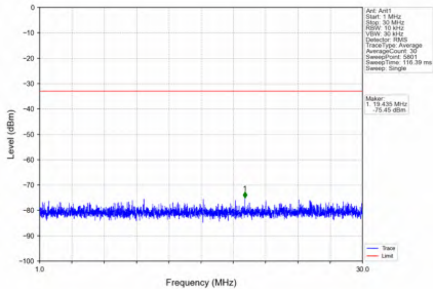
n25_15kHz_SISO_NTNV_25MHz_DFT-s-OFDM QPSK_1882.5MHz_Edge_1RB_Left
