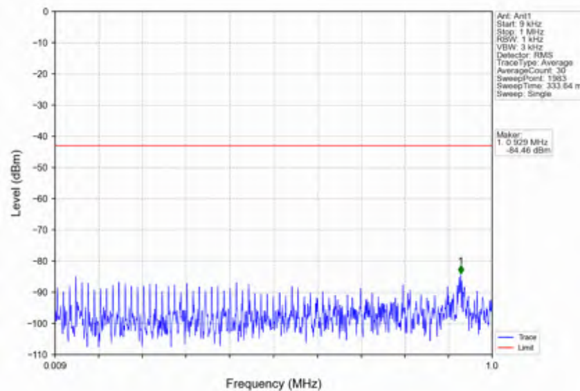
n25_15kHz_SISO_NTNV_30MHz_DFT-s-OFDM QPSK_1865MHz_Outer_Full
