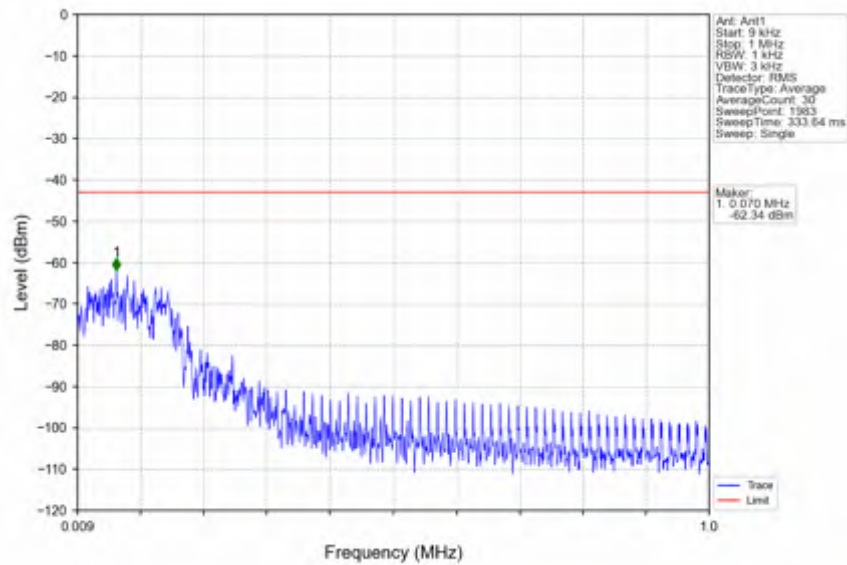
n25_15kHz_SISO_NTNV_30MHz_DFT-s-OFDM QPSK_1865MHz_Edge_1RB_Left
