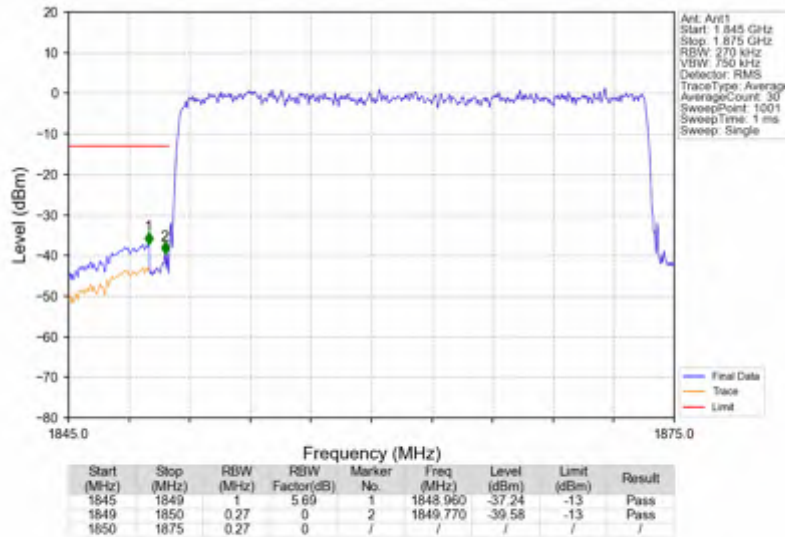
n25_15kHz_SISO_NTNV_25MHz_DFT-s-OFDM_QPSK_1862.5MHz_Outer_Full
