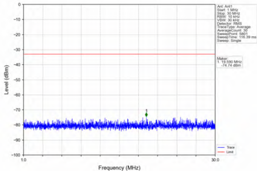
n25_15kHz_SISO_NTNV_20MHz_DFT-s-OFDM QPSK_1860MHz_Edge_1RB_Left
