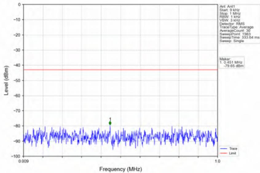
n25_15kHz_SISO_NTNV_25MHz_CP-OFDM QPSK_1862.5MHz_Outer_Full
