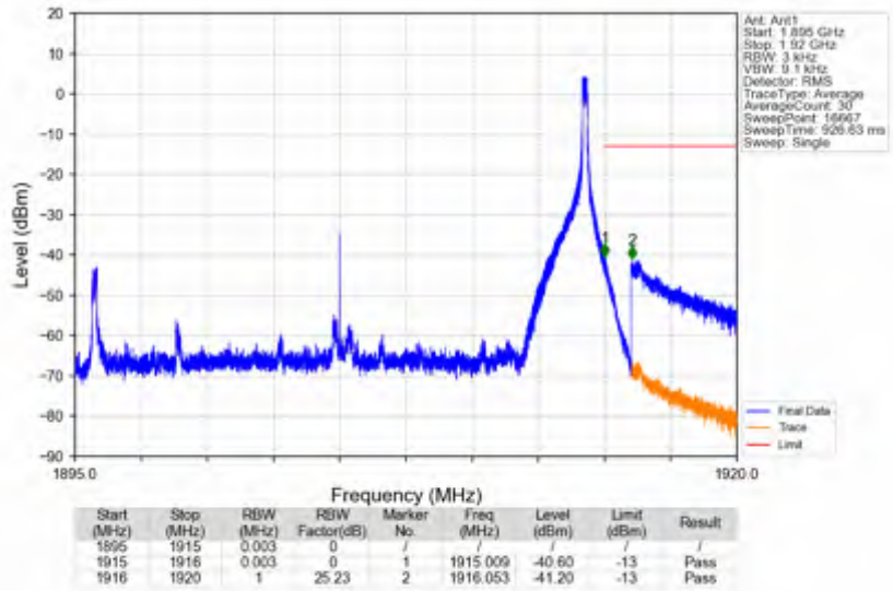
n25_15kHz_SISO_NTNV_20MHz_DFT-s-OFDM QPSK_1905MHz_Inner_1RB_Right
