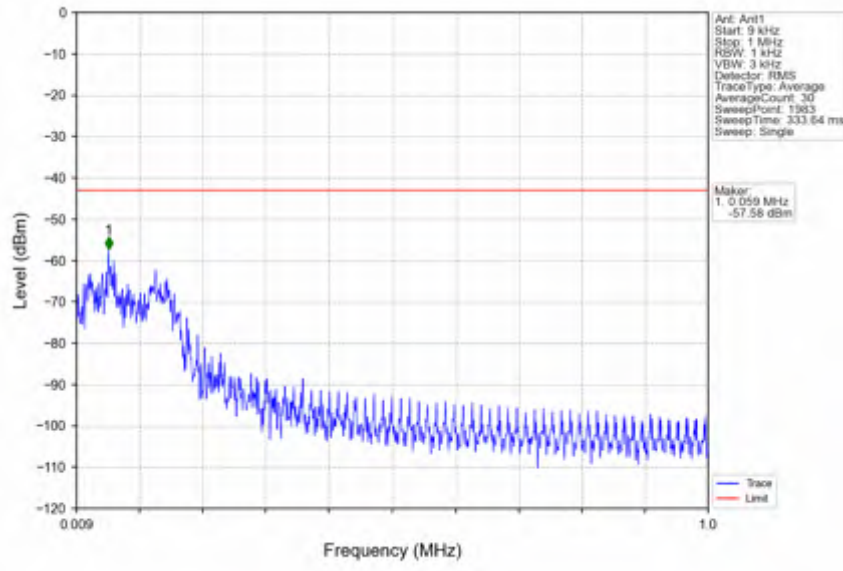
n25_15kHz_SISO_NTNV_25MHz_DFT-s-OFDM PI/2 BPSK_1902.5MHz_Inner_1RB_Right
