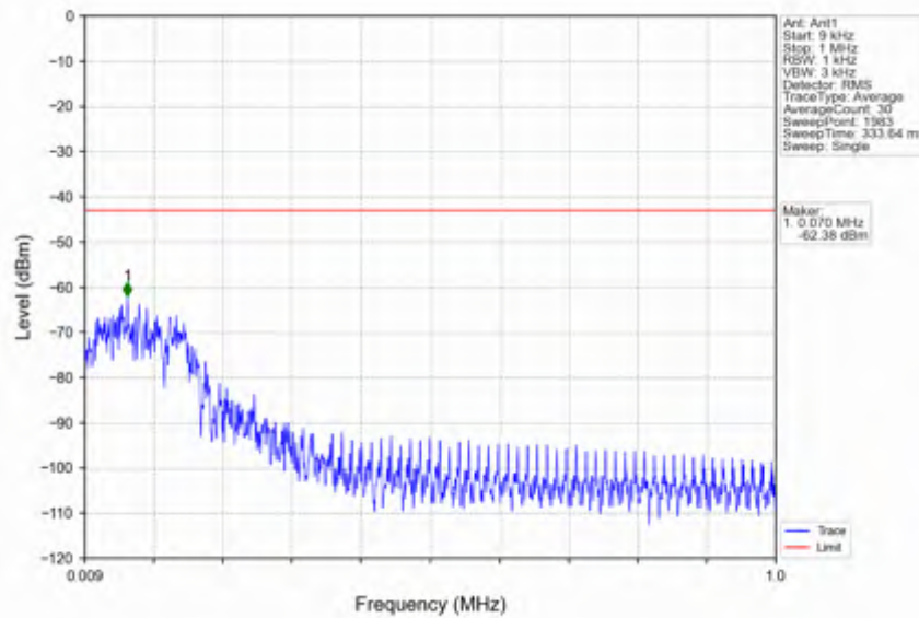
n25_15kHz_SISO_NTNV_40MHz_DFT-s-OFDM QPSK_1870MHz_Edge_1RB_Left
