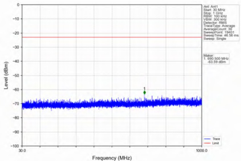
n25_15kHz_SISO_NTNV_25MHz_DFT-s-OFDM_QPSK_1862.5MHz_Outer_Full
