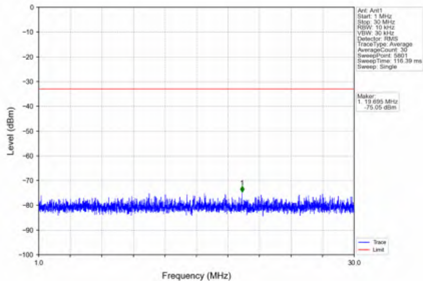
n25_15kHz_SISO_NTV_20MHz_CP-OFDM QPSK_1882.5MHz_Edge_1RB_Left
