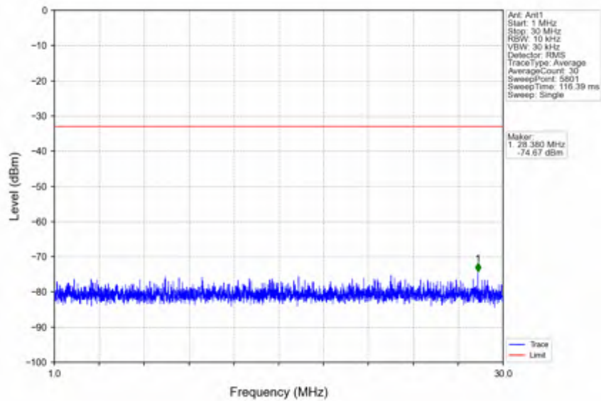
n25_15kHz_SISO_NTNV_30MHz_CP-OFDM QPSK_1900MHz_Edge_1RB_Right
