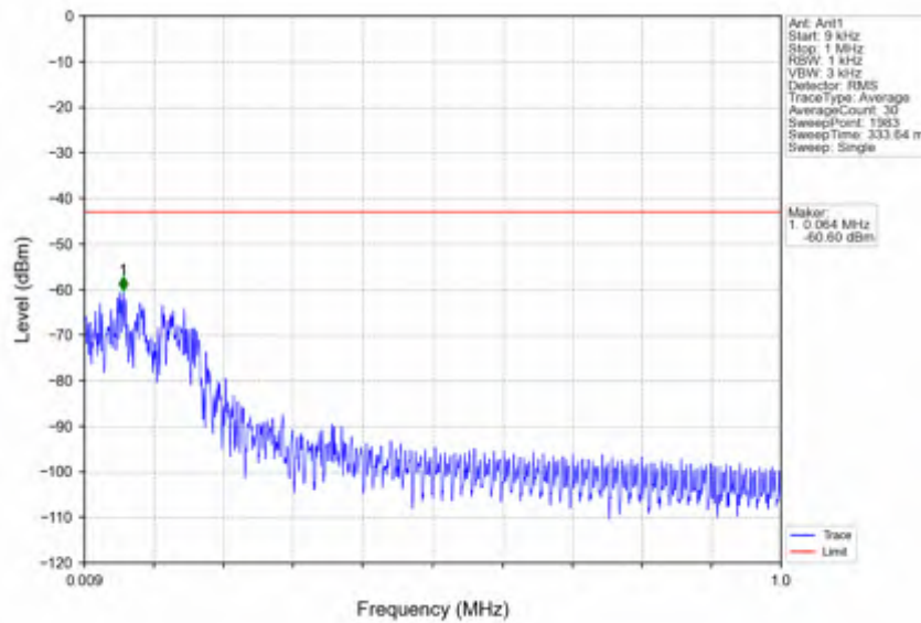
n25_15kHz_SISO_NTNV_20MHz_DFT-s-OFDM PI/2 BPSK_1905MHz_Edge_1RB_Right
