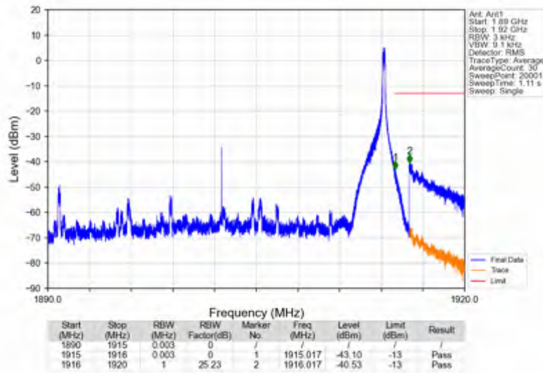
n25_15kHz_SISO_NTNV_25MHz_DFT-s-OFDM QPSK_1902.5MHz_Inner_1RB_Right
