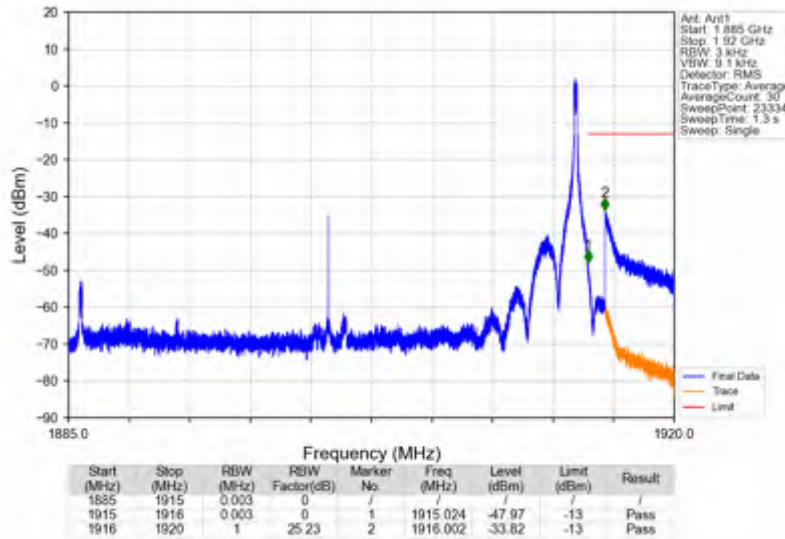
n25_15kHz_SISO_NTNV_30MHz_CP-OFDM QPSK_1900MHz_Edge_1RB_Right
