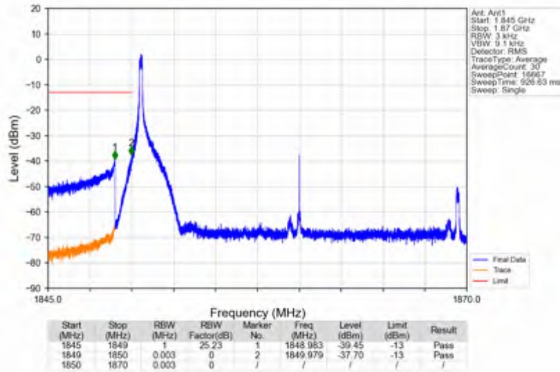
n25_15kHz_SISO_NTNV_20MHz_CP-OFDM QPSK_1860MHz_Edge_1RB_Left
