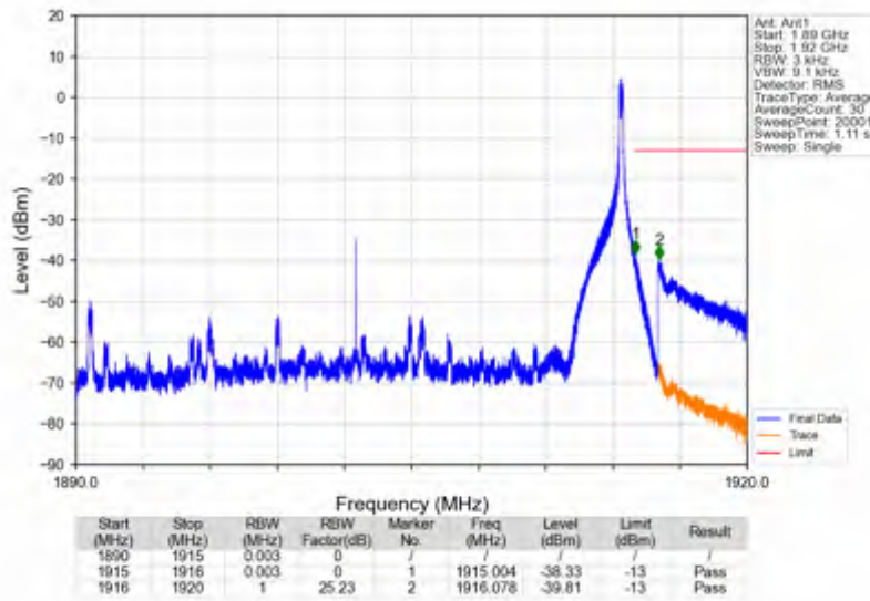
n25_15kHz_SISO_NTNV_25MHz_DFT-s-OFDM QPSK_1902.5MHz_Edge_1RB_Right
