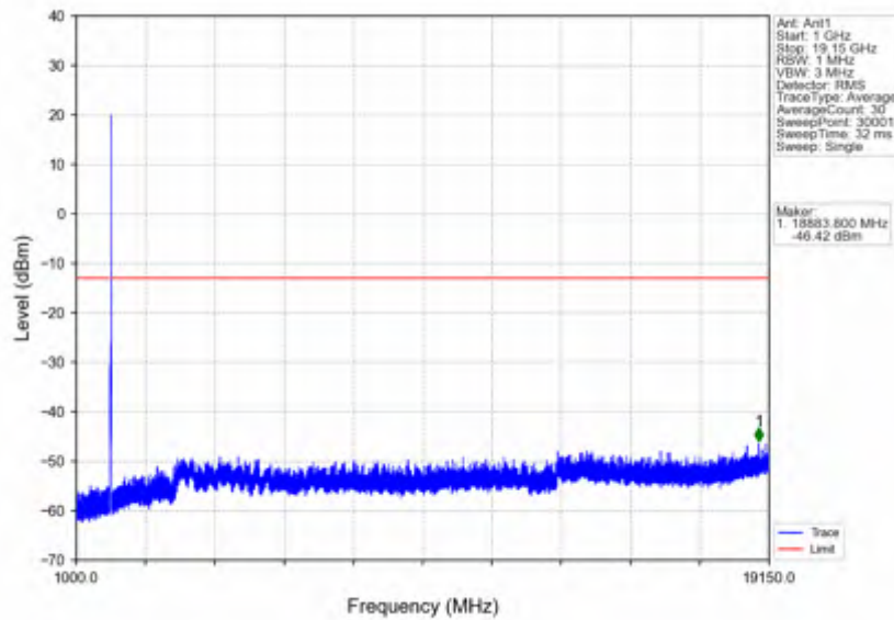
n25_15kHz_SISO_NTNV_20MHz_CP-OFDM QPSK_1905MHz_Inner_1RB_Right
