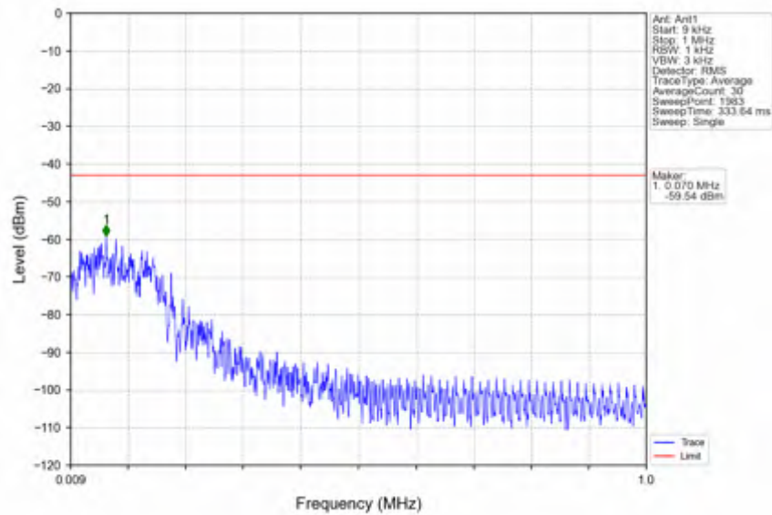
n25_15kHz_SISO_NTNV_25MHz_DFT-s-OFDM QPSK_1862.5MHz_Inner_1RB_Left
