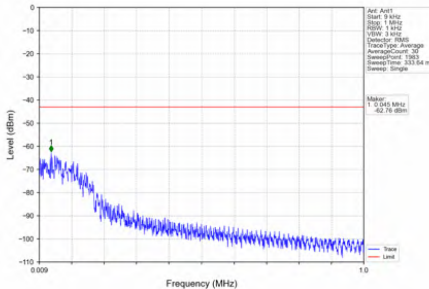
n25_15kHz_SISO_NTNV_30MHz_CP-OFDM QPSK_1865MHz_Edge_1RB_Left
