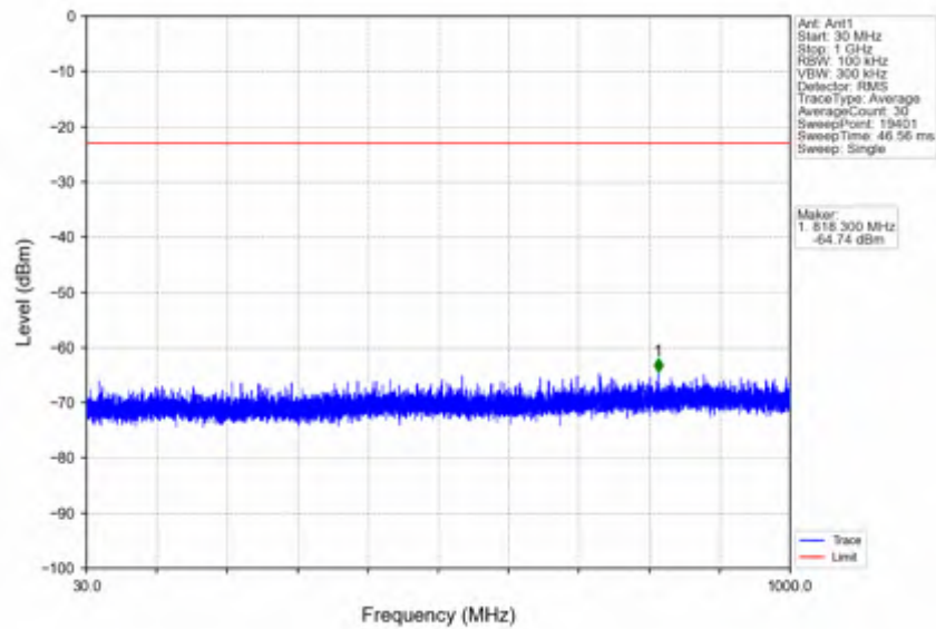
n25_15kHz_SISO_NTNV_25MHz_DFT-s-OFDM QPSK_1862.5MHz_Edge_1RB_Left
