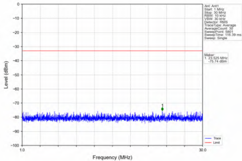
n25_15kHz_SISO_NTNV_30MHz_CP-OFDM QPSK_1900MHz_Inner_1RB_Right
