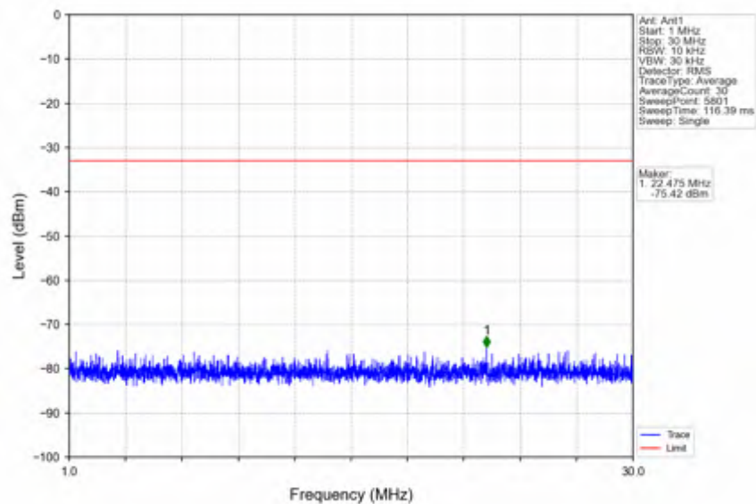
n25_15kHz_SISO_NTV_30MHz_DFT-s-OFDM QPSK_1900MHz_Inner_1RB_Right
