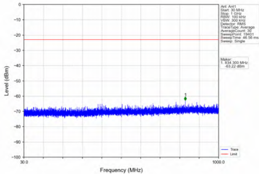
n25_15kHz_SISO_NTV_30MHz_CP-OFDM QPSK_1882.5MHz_Edge_1RB_Left
