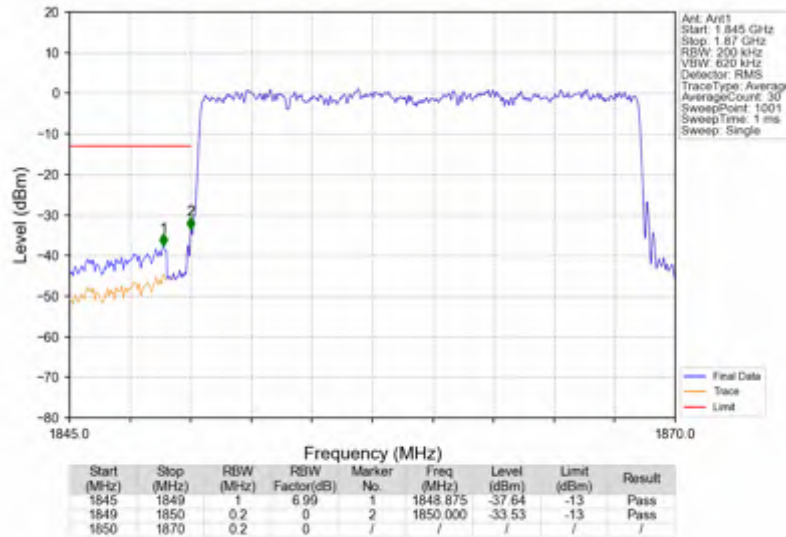
n25_15kHz_SISO_NTNV_20MHz_DFT-s-OFDM QPSK_1860MHz_Outer_Full
