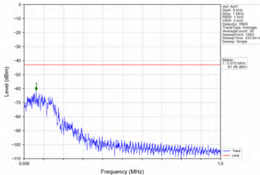
n25_15kHz_SISO_NTNV_25MHz_DFT-s-OFDM QPSK_1882.5MHz_Edge_1RB_Left
