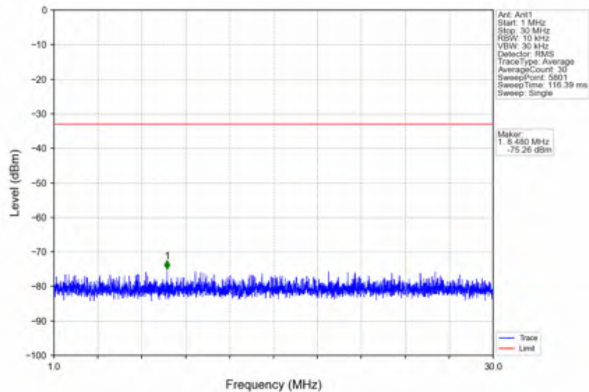
n25_15kHz_SISO_NTV_30MHz_CP-OFDM QPSK_1882.5MHz_Edge_1RB_Left
