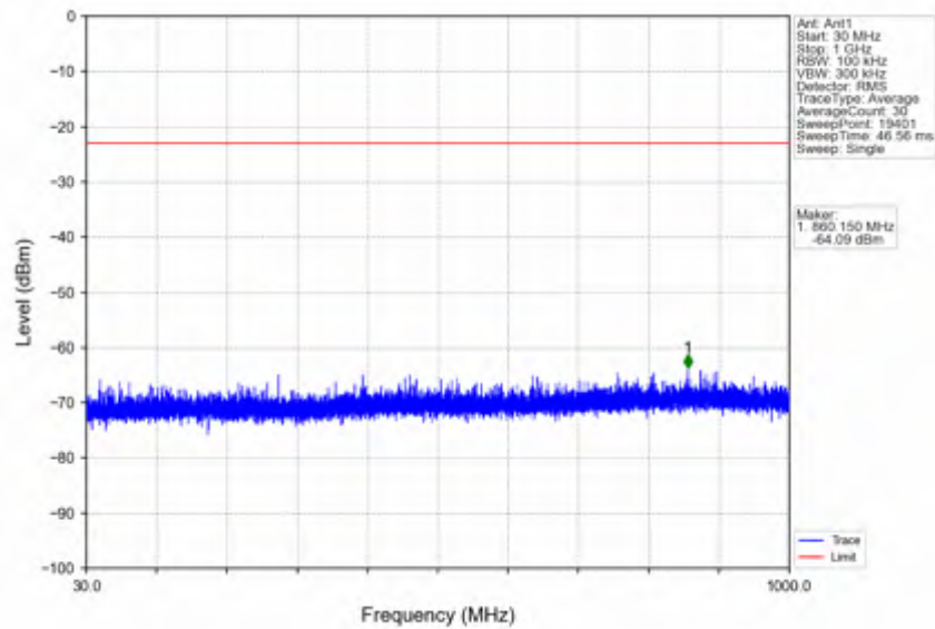
n25_15kHz_SISO_NTNV_30MHz_DFT-s-OFDM PI/2 BPSK_1882.5MHz_Edge_1RB_Left
