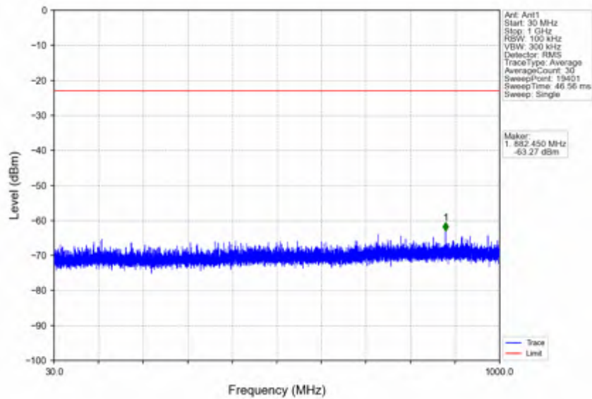
n25_15kHz_SISO_NTNV_30MHz_DFT-s-OFDM QPSK_1900MHz_Edge_1RB_Right
