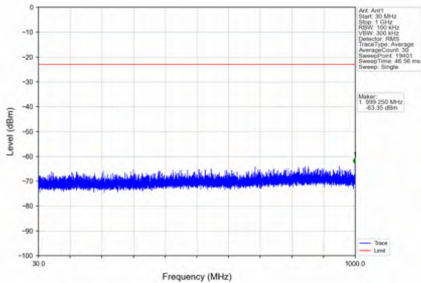
n25_15kHz_SISO_NTNV_20MHz_DFT-s-OFDM QPSK_1860MHz_Edge_1RB_Left
