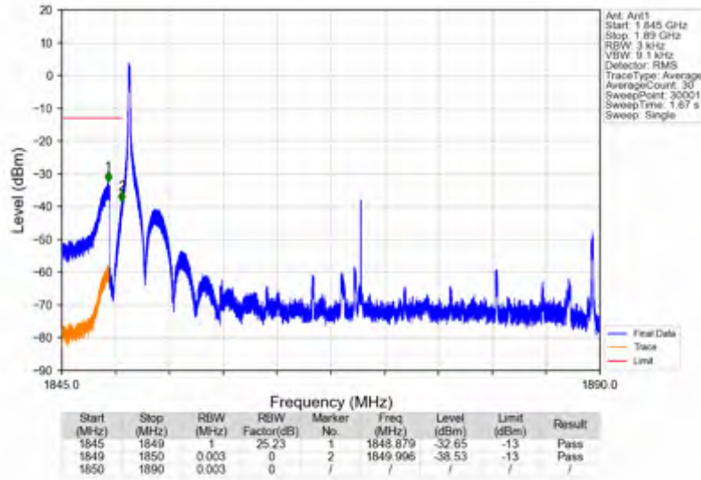
n25_15kHz_SISO_NTNV_40MHz_DFT-s-OFDM PI/2 BPSK_1870MHz_Edge_1RB_Left
