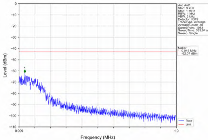
n25_15kHz_SISO_NTV_25MHz_CP-OFDM QPSK_1862.5MHz_Edge_1RB_Left
