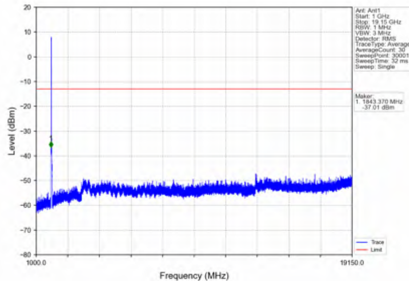
n25_15kHz_SISO_NTNV_25MHz_CP-OFDM QPSK_1862.5MHz_Outer_Full
