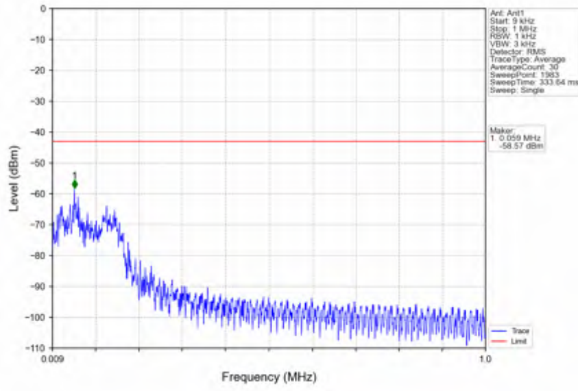
n25_15kHz_SISO_NTNV_25MHz_DFT-s-OFDM PI/2 BPSK_1902.5MHz_Edge_1RB_Right
