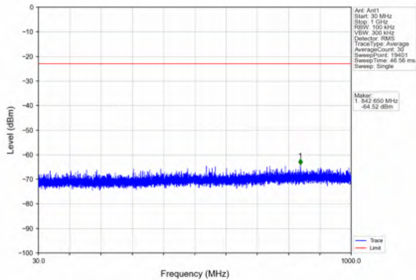
n25_15kHz_SISO_NTVV_25MHz_CP-OFDM QPSK_1882.5MHz_Edge_1RB_Left
