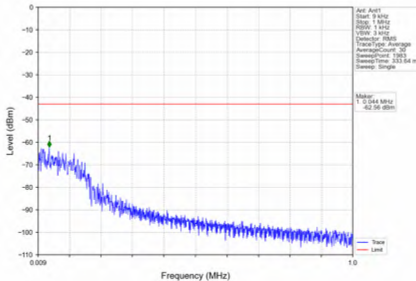
n25_15kHz_SISO_NTNV_20MHz_CP-OFDM QPSK_1860MHz_Edge_1RB_Left
