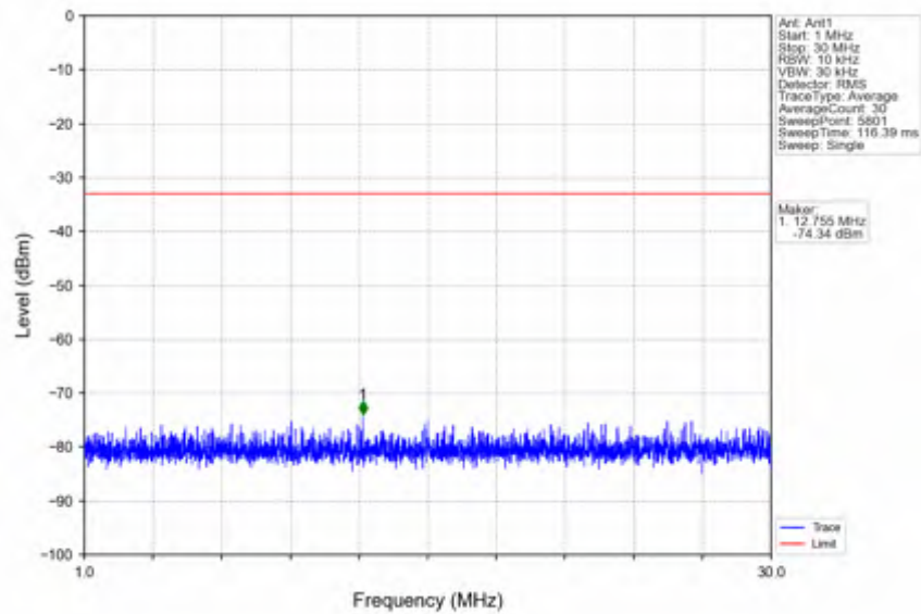
n25_15kHz_SISO_NTNV_15MHz_CP-OFDM QPSK_1907.5MHz_Edge_1RB_Right
