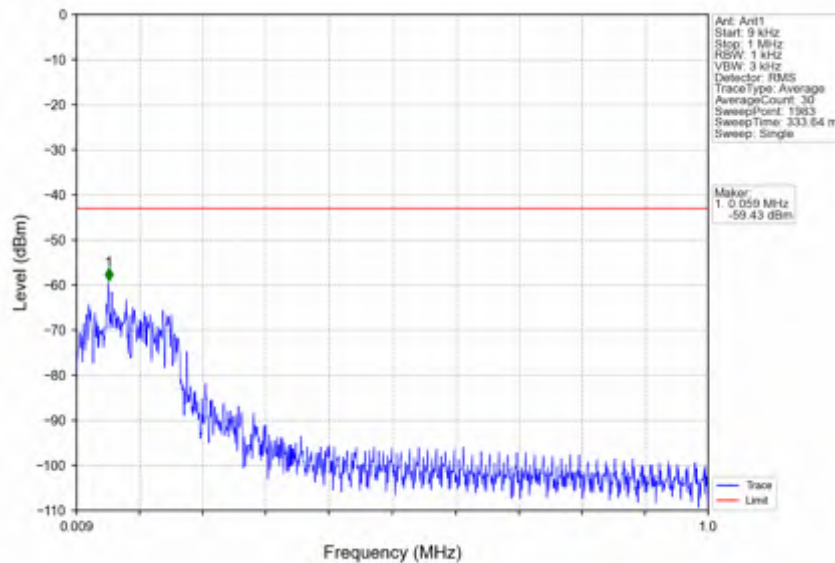
n25_15kHz_SISO_NTNV_20MHz_DFT-s-OFDM QPSK_1882.5MHz_Edge_1RB_Left
