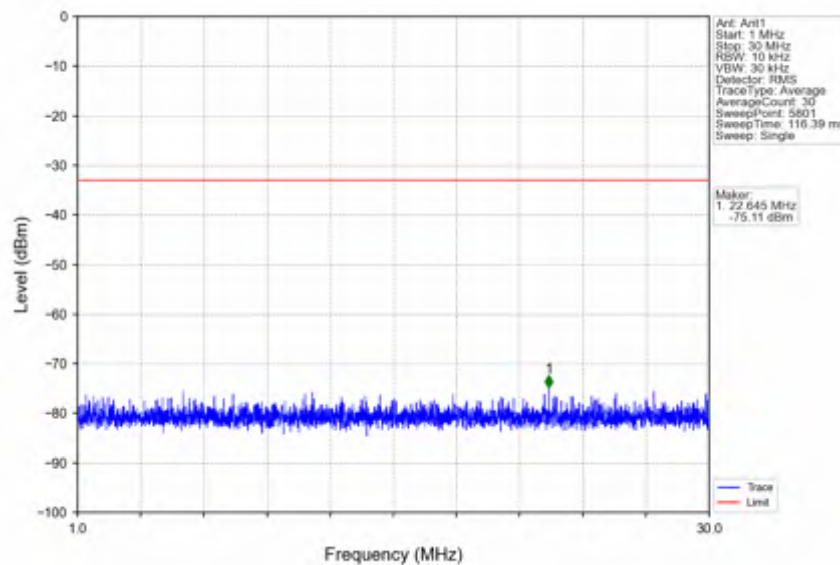
n25_15kHz_SISO_NTNV_25MHz_DFT-s-OFDM PI/2 BPSK_1862.5MHz_Outer_Full
