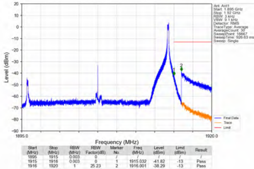
n25_15kHz_SISO_NTNV_20MHz_CP-OFDM QPSK_1905MHz_Inner_1RB_Right
