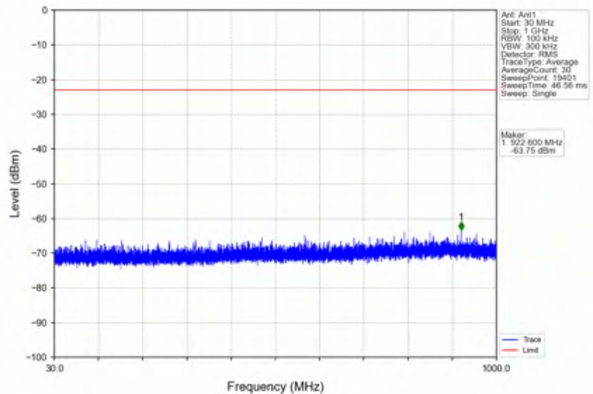
n25_15kHz_SISO_NTNV_25MHz_CP-OFDM QPSK_1862.5MHz_Inner_1RB_Left
