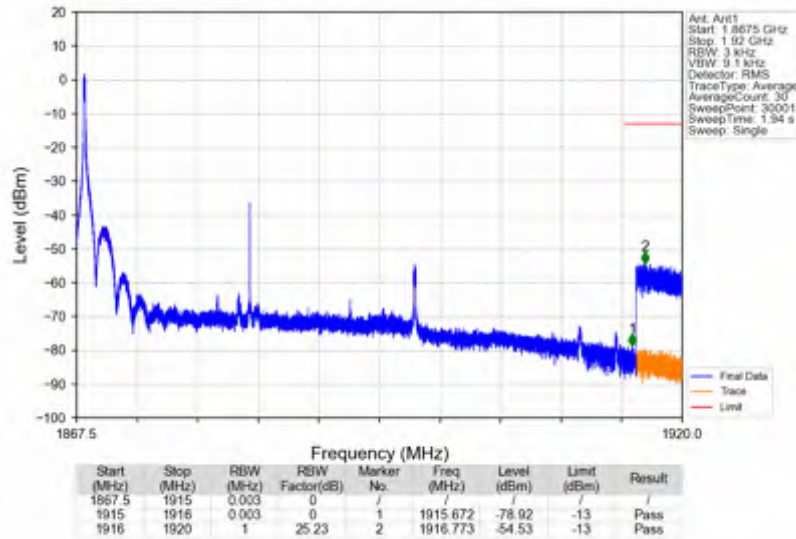
n25_15kHz_SISO_NTNV_30MHz_CP-OFDM QPSK_1882.5MHz_Edge_1RB_Left
