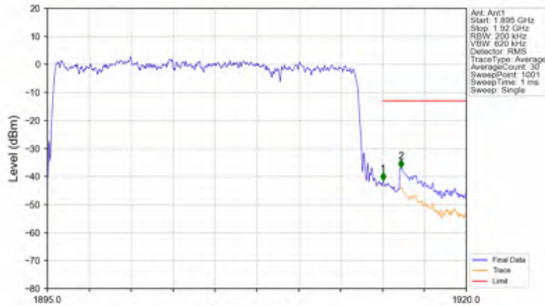
n25_15kHz_SISO_NTNV_20MHz_DFT-s-OFDM PI/2 BPSK_1905MHz_Outer_Full
