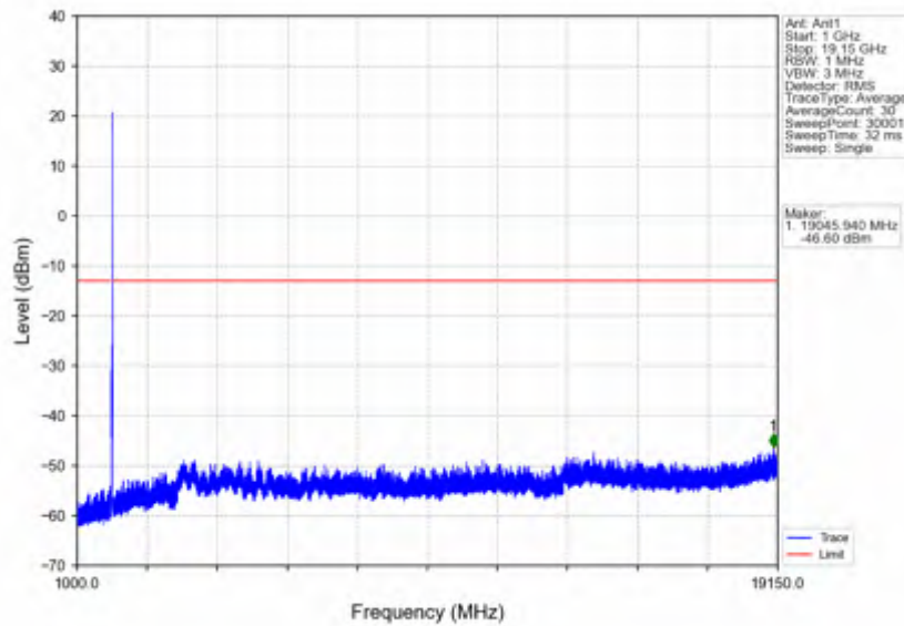
n25_15kHz_SISO_NTV_15MHz_CP-OFDM QPSK_1907.5MHz_Inner_1RB_Right
