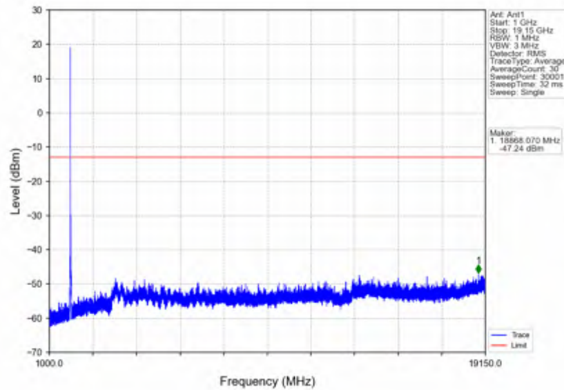
n25_15kHz_SISO_NTVV_25MHz_CP-OFDM QPSK_1882.5MHz_Edge_1RB_Left
