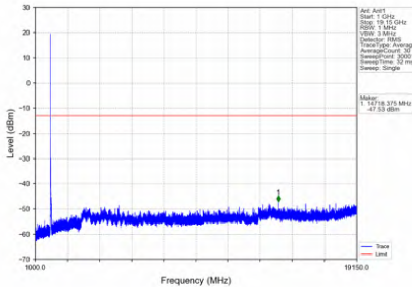
n25_15kHz_SISO_NTV_25MHz_CP-OFDM QPSK_1862.5MHz_Outer_Full
