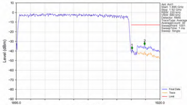
n25_15kHz_SISO_NTNV_20MHz_CP-OFDM QPSK_1905MHz_Outer_Full
