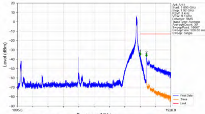
n25_15kHz_SISO_NTNV_20MHz_DFT-s-OFDM PI/2 BPSK_1905MHz_Edge_1RB_Right
