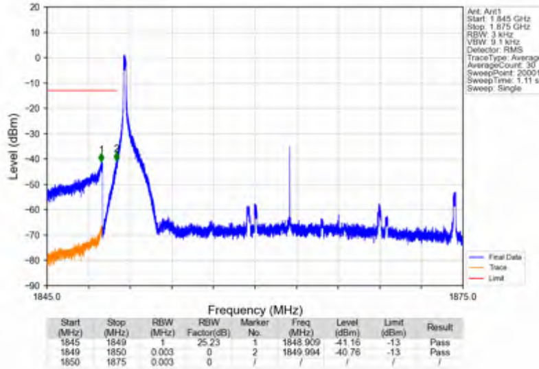
n25_15kHz_SISO_NTV_25MHz_CP-OFDM QPSK_1862.5MHz_Edge_1RB_Left
