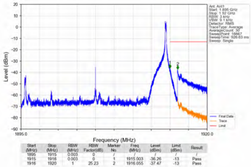
n25_15kHz_SISO_NTNV_20MHz_DFT-s-OFDM QPSK_1905MHz_Edge_1RB_Right
