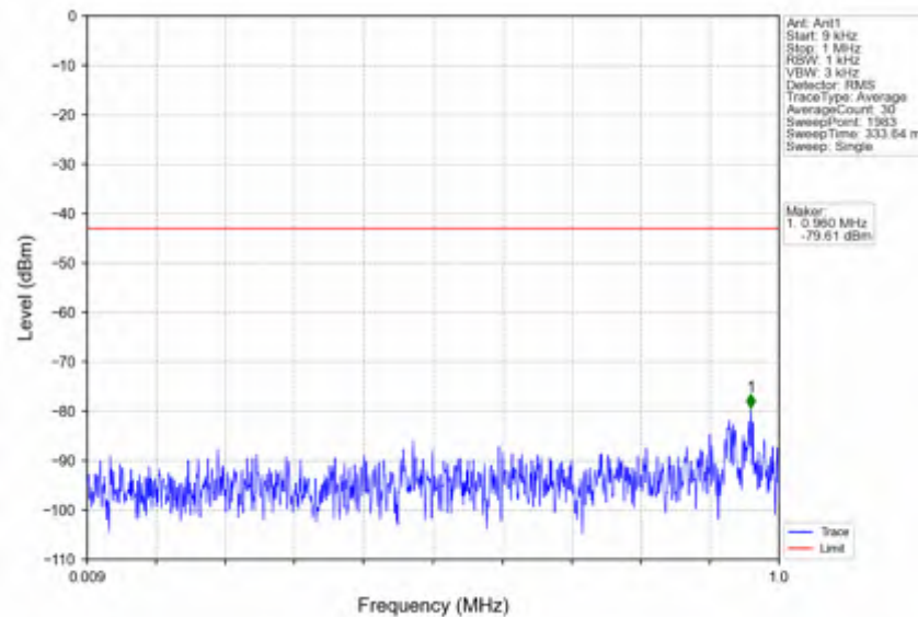
n25_15kHz_SISO_NTNV_20MHz_DFT-s-OFDM QPSK_1905MHz_Outer_Full
