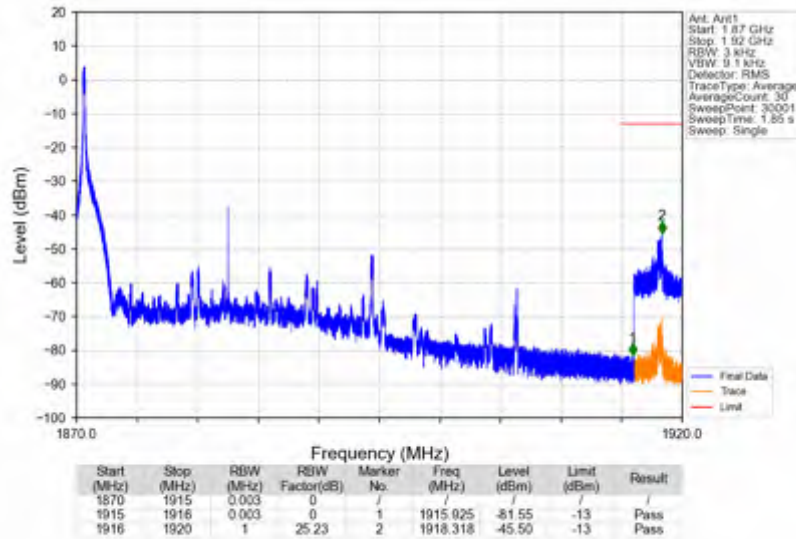
n25_15kHz_SISO_NTNV_25MHz_DFT-s-OFDM PI/2 BPSK_1882.5MHz_Edge_1RB_Left
