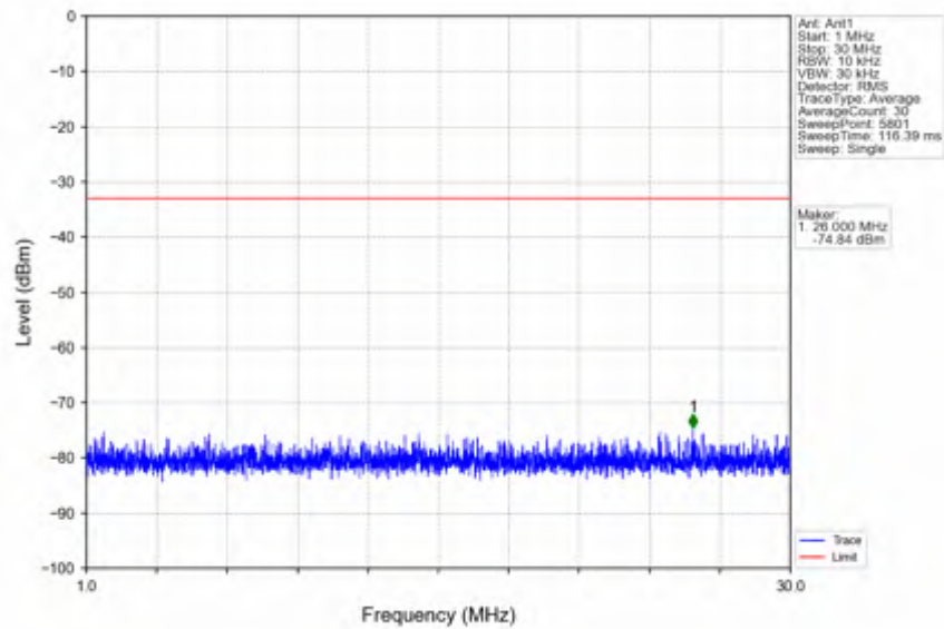
n25_15kHz_SISO_NTNV_20MHz_CP-OFDM QPSK_1860MHz_Edge_1RB_Left
