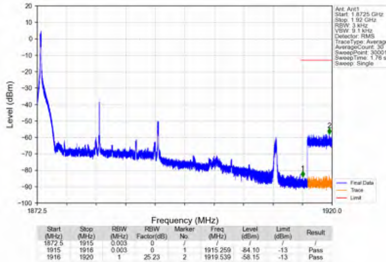
n25_15kHz_SISO_NTNV_20MHz_DFT-s-OFDM QPSK_1882.5MHz_Edge_1RB_Left
