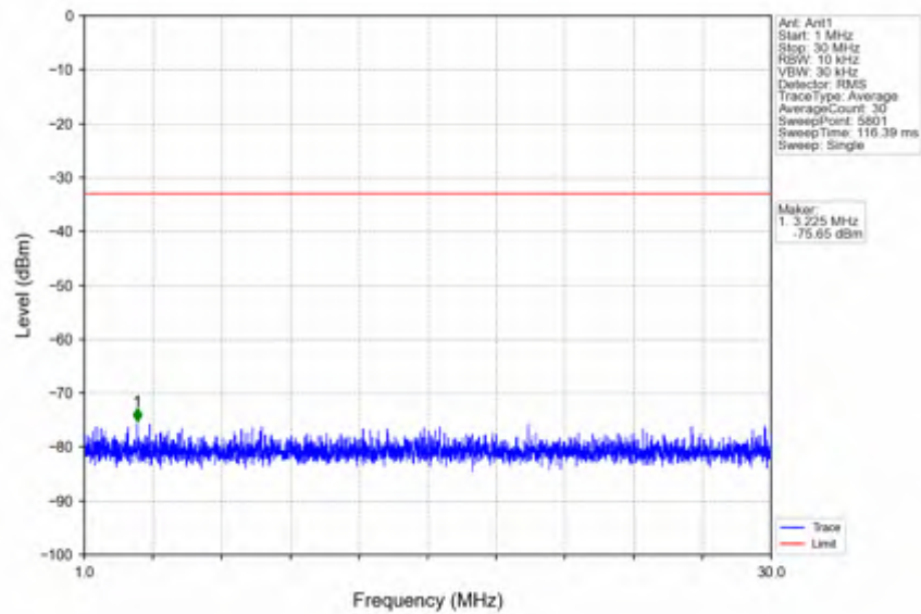
n25_15kHz_SISO_NTNV_30MHz_DFT-s-OFDM QPSK_1882.5MHz_Edge_1RB_Left
