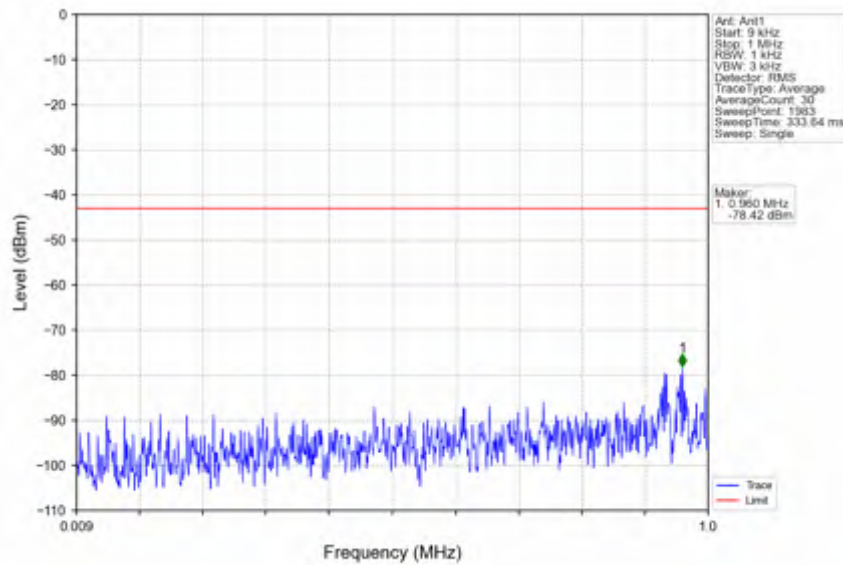
n25_15kHz_SISO_NTNV_20MHz_DFT-s-OFDM PI/2 BPSK_1860MHz_Outer_Full
