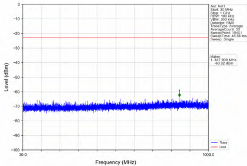
n25_15kHz_SISO_NTNV_25MHz_CP-OFDM QPSK_1862.5MHz_Outer_Full
