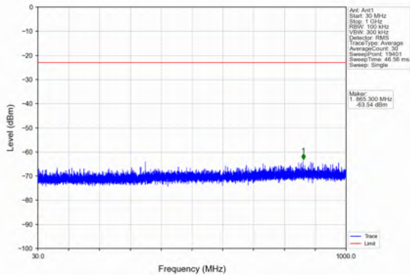
n25_15kHz_SISO_NTNV_30MHz_DFT-s-OFDM QPSK_1865MHz_Edge_1RB_Left
