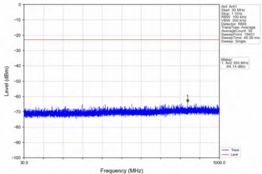
n25_15kHz_SISO_NTNV_25MHz_CP-OFDM QPSK_1902.5MHz_Inner_1RB_Right
