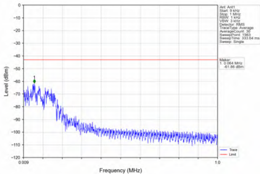
n25_15kHz_SISO_NTNV_20MHz_DFT-s-OFDM_PI/2_BPSK_1860MHz_Edge_1RB_Left
