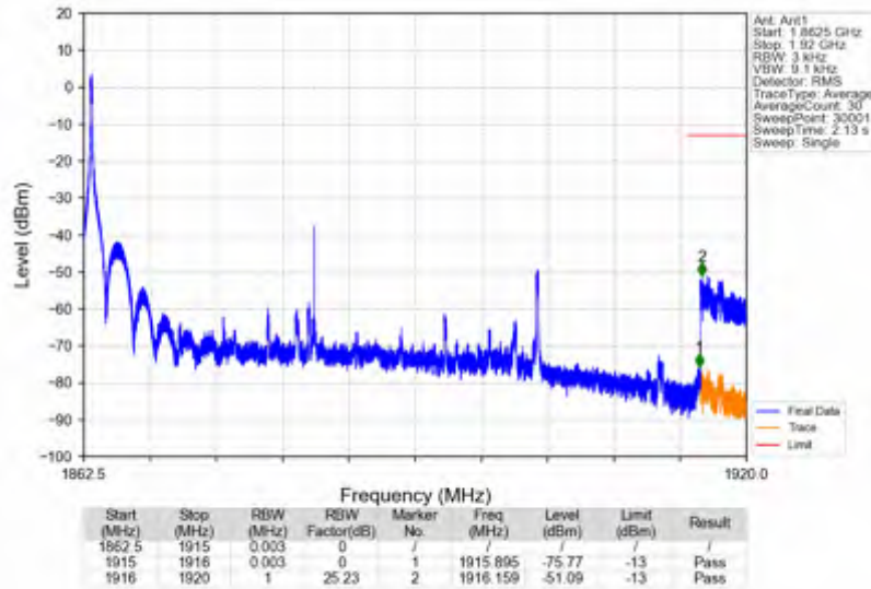
n25_15kHz_SISO_NTNV_40MHz_DFT-s-OFDM PI/2 BPSK_1882.5MHz_Edge_1RB_Left
