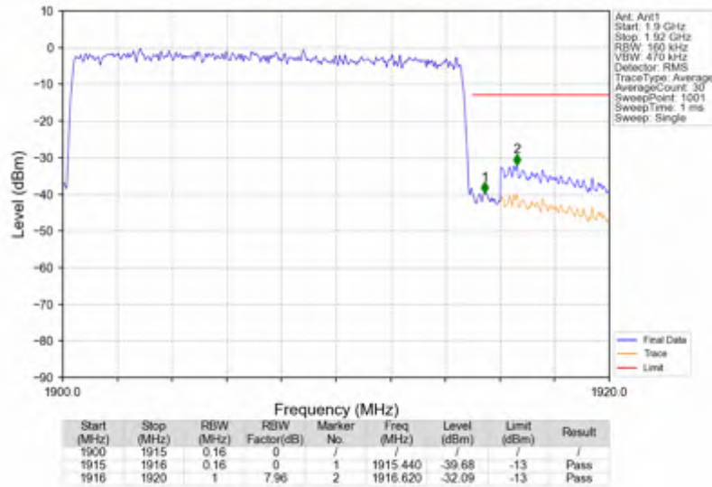
n25_15kHz_SISO_NTNV_15MHz_CP-OFDM QPSK_1907.5MHz_Outer_Full
