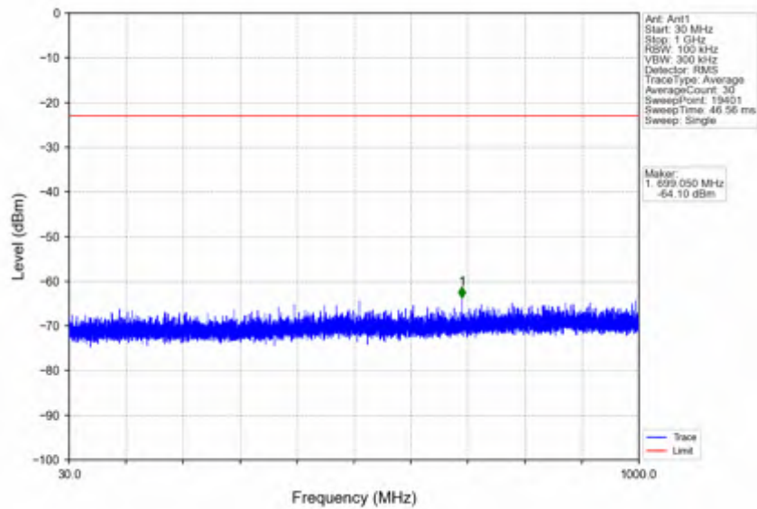
n25_15kHz_SISO_NTNV_40MHz_DFT-s-OFDM PI/2 BPSK_1895MHz_Outer_Full
