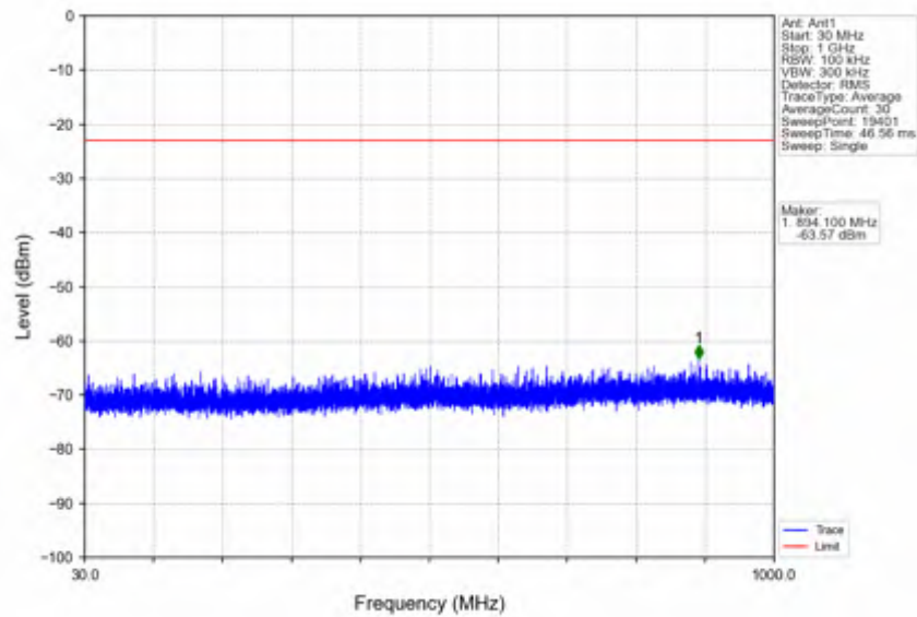
n25_15kHz_SISO_NTVV_20MHz_CP-OFDM QPSK_1882.5MHz_Edge_1RB_Left
