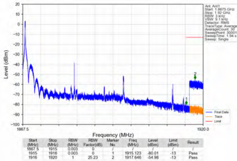
n25_15kHz_SISO_NTNV_30MHz_DFT-s-OFDM PI/2 BPSK_1882.5MHz_Edge_1RB_Left
