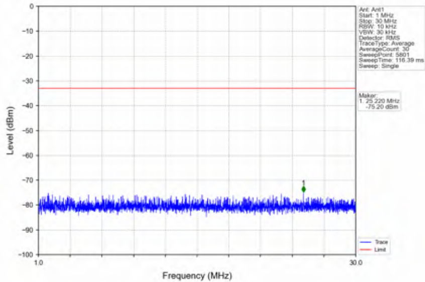
n25_15kHz_SISO_NTNV_20MHz_DFT-s-OFDM QPSK_1882.5MHz_Edge_1RB_Left
