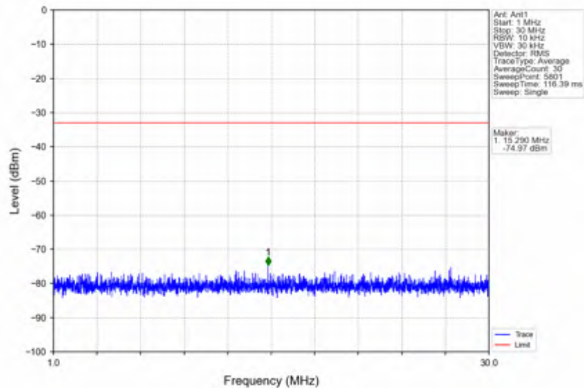
n25_15kHz_SISO_NTV_25MHz_CP-OFDM QPSK_1882.5MHz_Edge_1RB_Left
