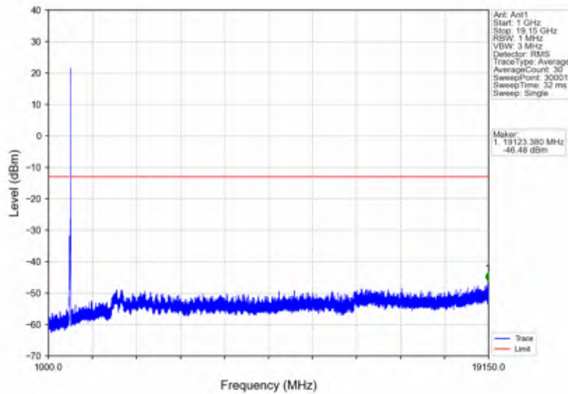
n25_15kHz_SISO_NTV_25MHz_CP-OFDM QPSK_1902.5MHz_Inner_1RB_Right
