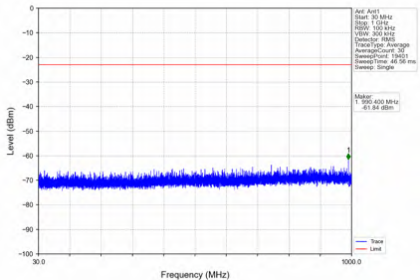
n25_15kHz_SISO_NTNV_20MHz_CP-OFDM QPSK_1905MHz_Inner_1RB_Right
