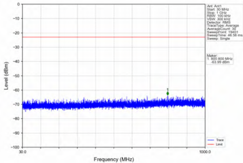
n25_15kHz_SISO_NTNV_20MHz_DFT-s-OFDM QPSK_1905MHz_Edge_1RB_Right
