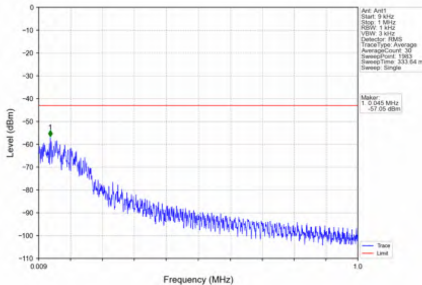
n25_15kHz_SISO_NTNV_30MHz_CP-OFDM QPSK_1900MHz_Inner_1RB_Right
