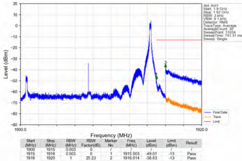
n25_15kHz_SISO_NTV_15MHz_CP-OFDM QPSK_1907.5MHz_Inner_1RB_Right
