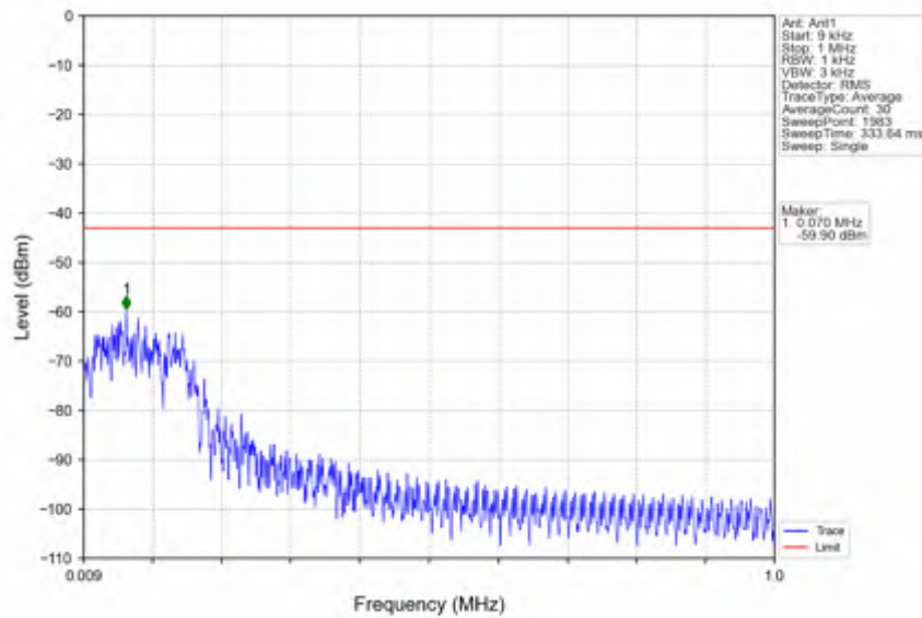
n25_15kHz_SISO_NTNV_25MHz_DFT-s-OFDM QPSK_1902.5MHz_Edge_1RB_Right
