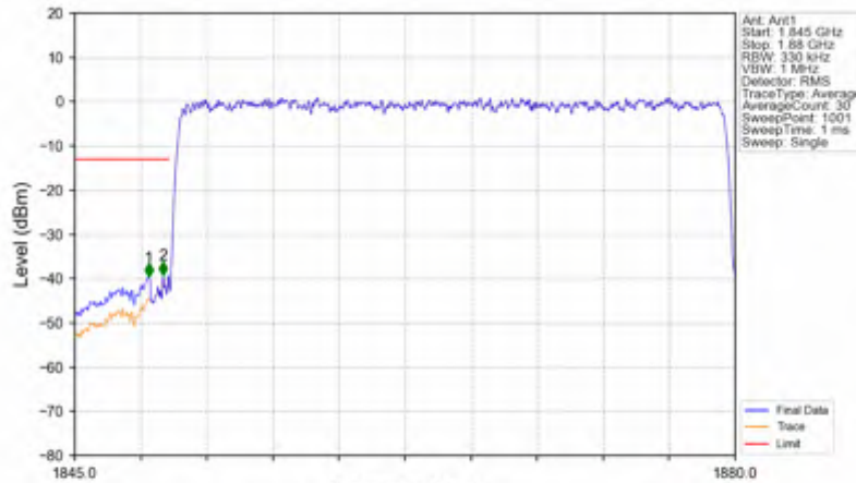
n25_15kHz_SISO_NTNV_30MHz_DFT-s-OFDM PI/2 BPSK_1865MHz_Outer_Full
