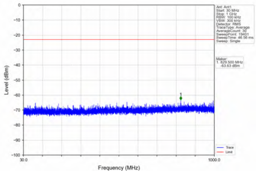
n25_15kHz_SISO_NTV_25MHz_CP-OFDM QPSK_1862.5MHz_Edge_1RB_Left
