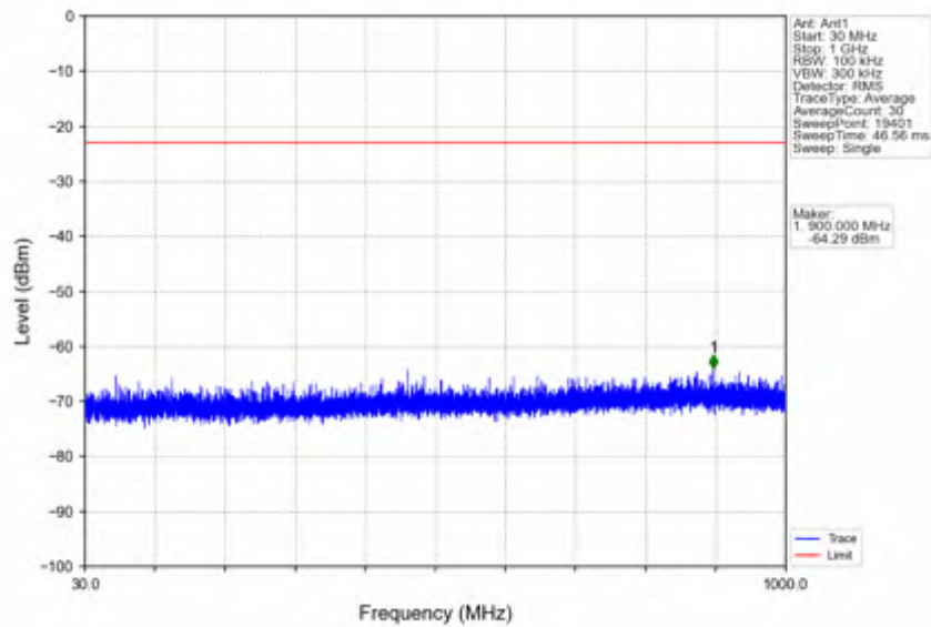
n25_15kHz_SISO_NTNV_30MHz_DFT-s-OFDM PI/2 BPSK_1865MHz_Outer_Full
