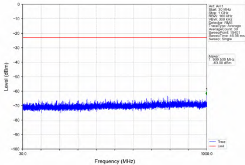
n25_15kHz_SISO_NTNV_25MHz_DFT-s-OFDM QPSK_1902.5MHz_Inner_1RB_Right
