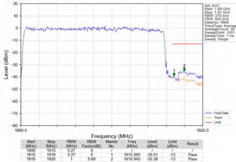
n25_15kHz_SISO_NTNV_25MHz_DFT-s-OFDM_QPSK_1902.5MHz_Outer_Full
