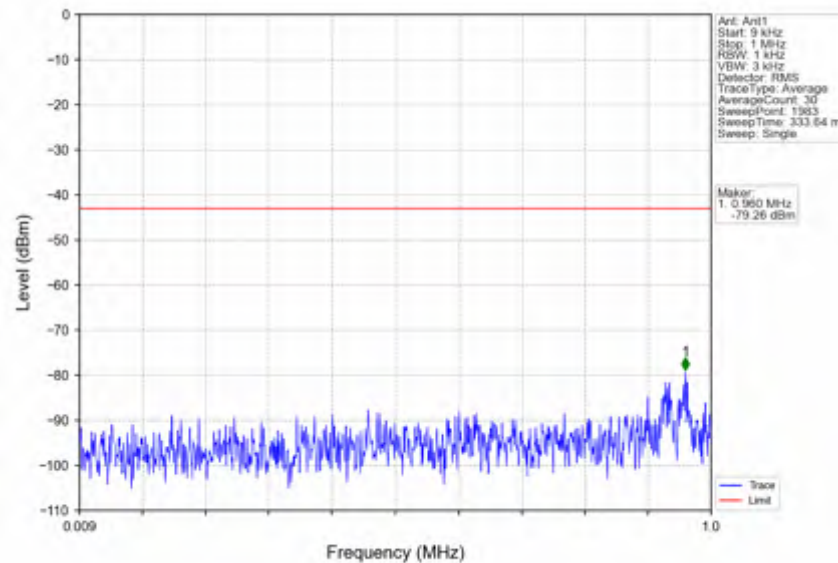
n25_15kHz_SISO_NTNV_20MHz_DFT-s-OFDM QPSK_1860MHz_Outer_Full
