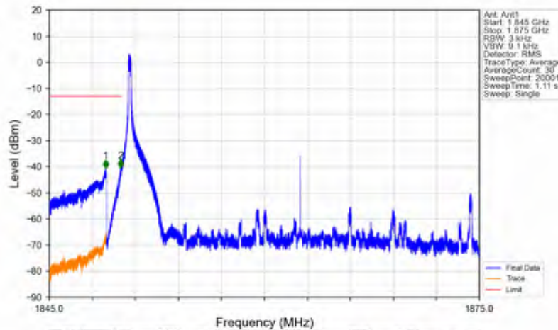
n25_15kHz_SISO_NTNV_25MHz_DFT-s-OFDM QPSK_1862.5MHz_Edge_1RB_Left
