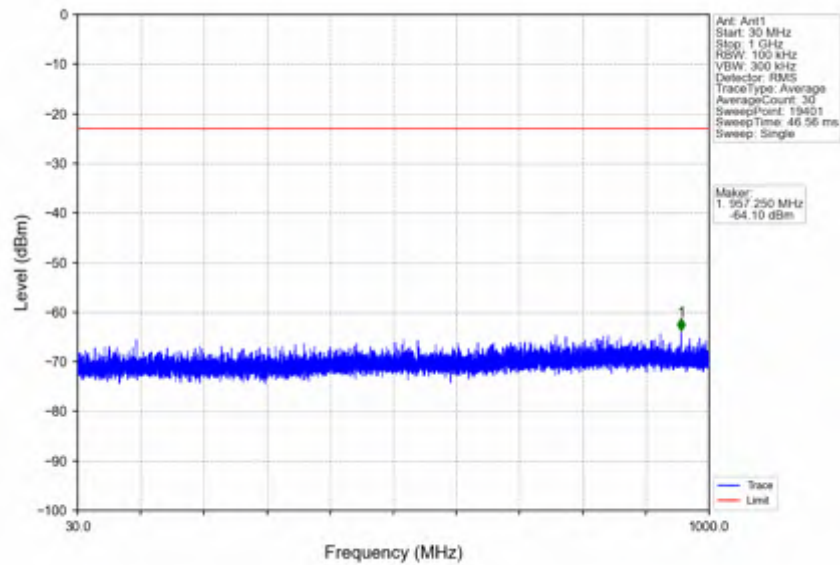
n25_15kHz_SISO_NTNV_40MHz_DFT-s-OFDM PI/2 BPSK_1870MHz_Outer_Full
