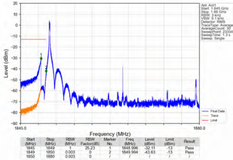
n25_15kHz_SISO_NTNV_30MHz_DFT-s-OFDM_PI/2_BPSK_1865MHz_Edge_1RB_Left
