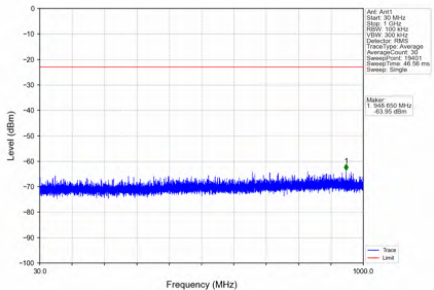
n25_15kHz_SISO_NTNV_30MHz_CP-OFDM QPSK_1865MHz_Edge_1RB_Left
