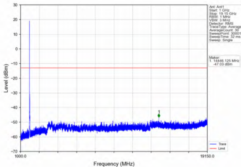
n25_15kHz_SISO_NTV_30MHz_CP-OFDM QPSK_1882.5MHz_Edge_1RB_Left
