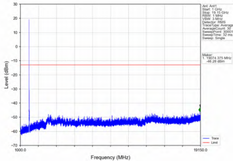
n25_15kHz_SISO_NTVV_20MHz_CP-OFDM QPSK_1882.5MHz_Edge_1RB_Left
