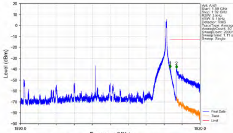
n25_15kHz_SISO_NTNV_25MHz_DFT-s-OFDM PI/2 BPSK_1902.5MHz_Edge_1RB_Right
