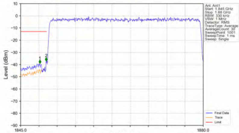
n25_15kHz_SISO_NTNV_30MHz_CP-OFDM QPSK_1865MHz_Outer_Full
