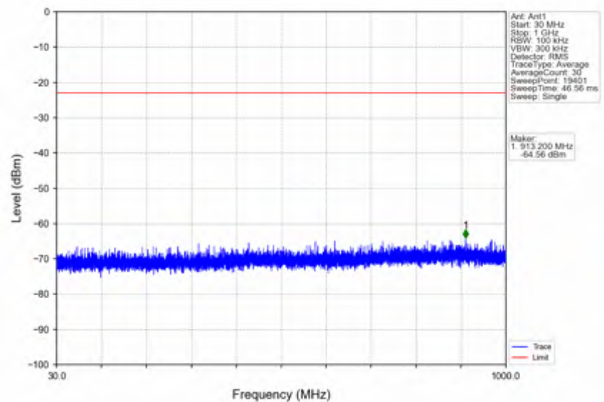
n25_15kHz_SISO_NTNV_30MHz_DFT-s-OFDM_QPSK_1865MHz_Outer_Full
