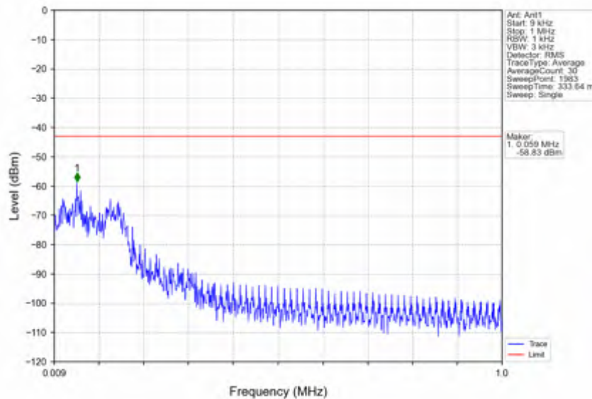
n25_15kHz_SISO_NTNV_25MHz_DFT-s-OFDM PI/2 BPSK_1862.5MHz_Inner_1RB_Left
