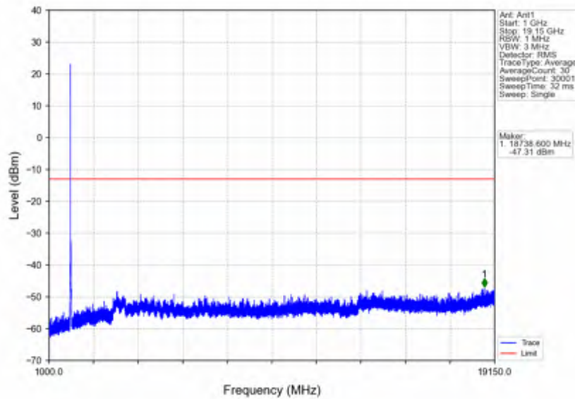
n25_15kHz_SISO_NTNV_30MHz_DFT-s-OFDM PI/2 BPSK_1882.5MHz_Edge_1RB_Left
