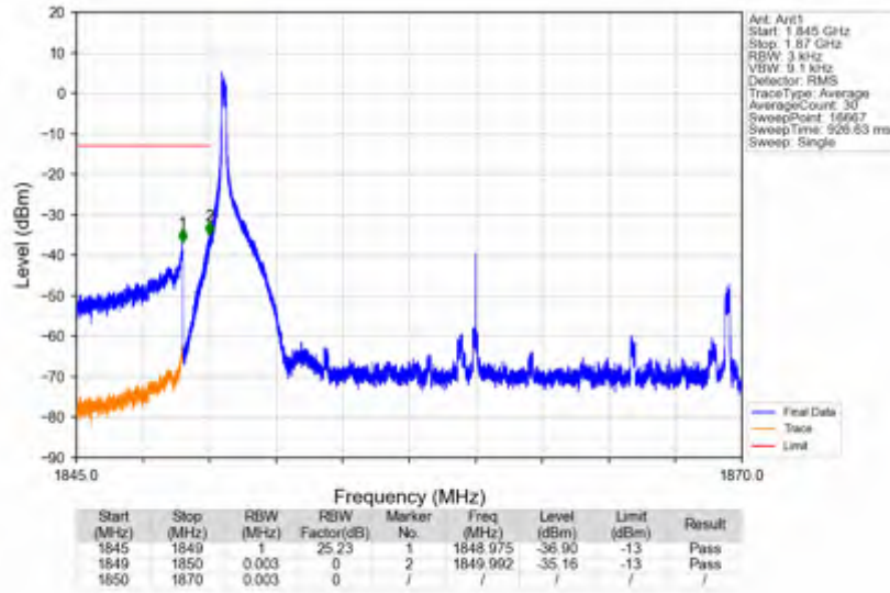
n25_15kHz_SISO_NTNV_20MHz_DFT-s-OFDM_PI/2_BPSK_1860MHz_Edge_1RB_Left
