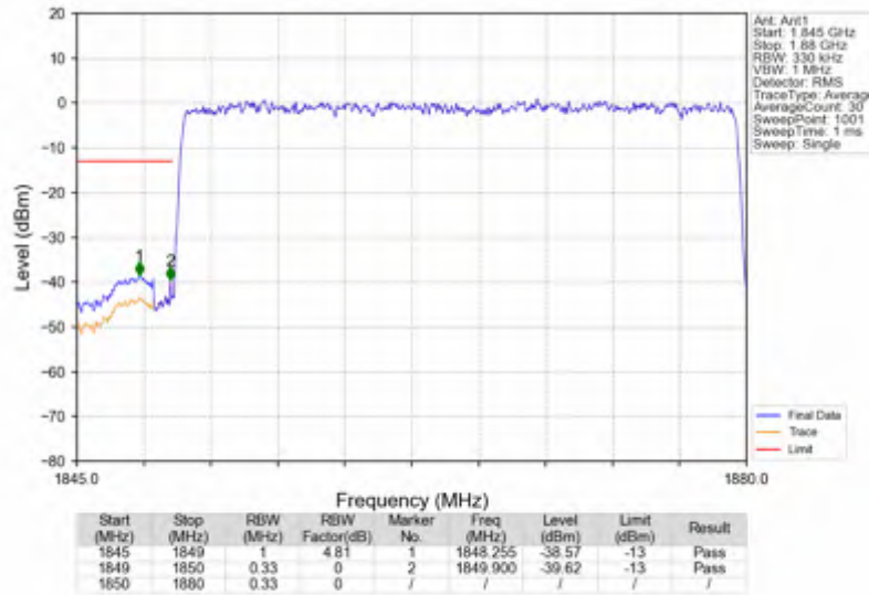
n25_15kHz_SISO_NTNV_30MHz_DFT-s-OFDM QPSK_1865MHz_Outer_Full
