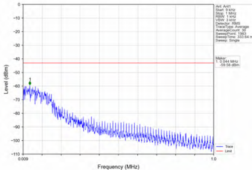
n25_15kHz_SISO_NTV_15MHz_CP-OFDM QPSK_1907.5MHz_Inner_1RB_Right
