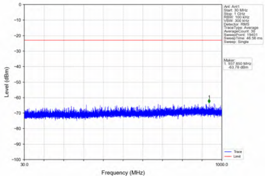
n25_15kHz_SISO_NTNV_15MHz_CP-OFDM QPSK_1907.5MHz_Inner_1RB_Right
