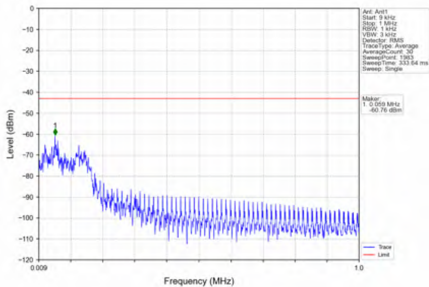
n25_15kHz_SISO_NTNV_30MHz_DFT-s-OFDM_PI/2_BPSK_1865MHz_Edge_1RB_Left
