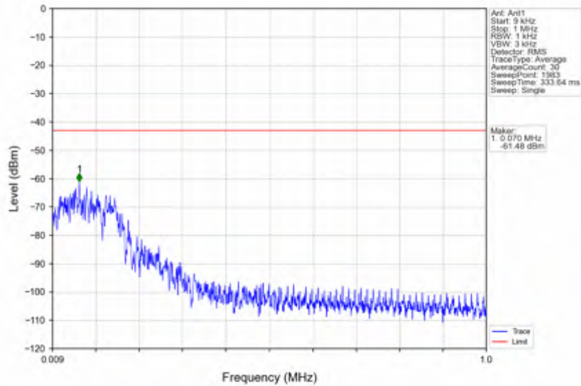
n25_15kHz_SISO_NTNV_25MHz_DFT-s-OFDM QPSK_1862.5MHz_Edge_1RB_Left
