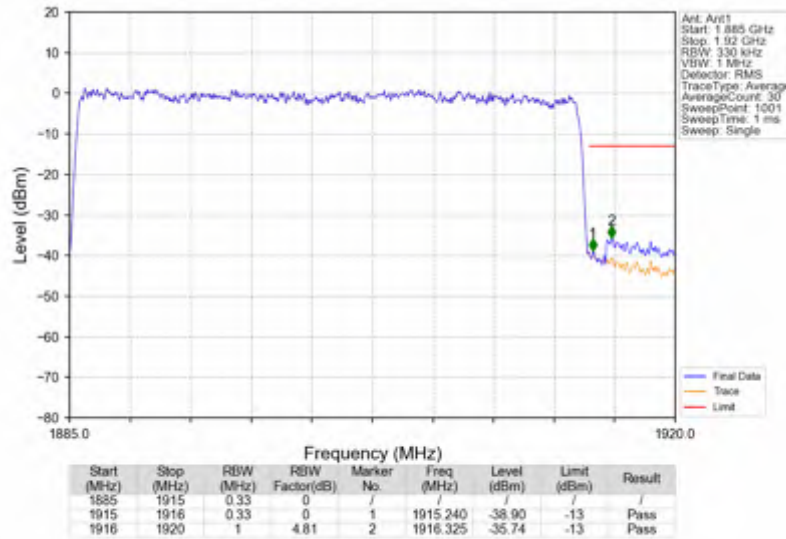
n25_15kHz_SISO_NTNV_30MHz_DFT-s-OFDM QPSK_1900MHz_Outer_Full
