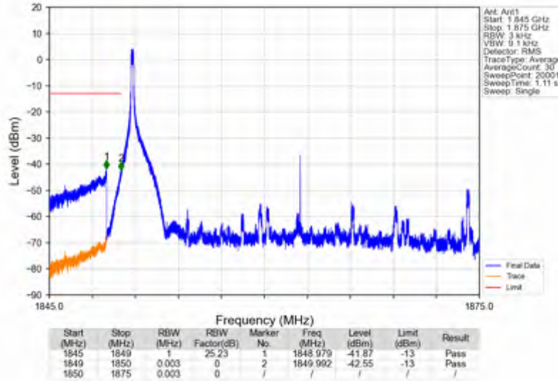
n25_15kHz_SISO_NTNV_25MHz_DFT-s-OFDM PI/2 BPSK_1862.5MHz_Inner_1RB_Left
