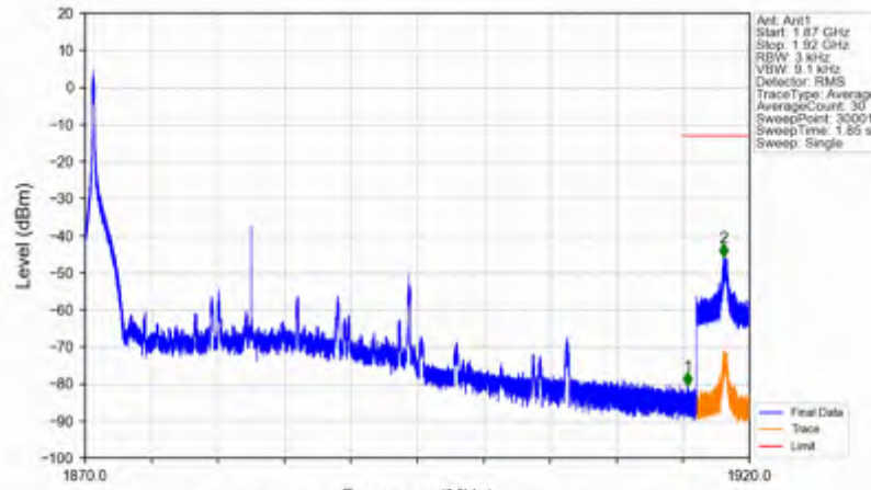
n25_15kHz_SISO_NTNV_25MHz_DFT-s-OFDM QPSK_1882.5MHz_Edge_1RB_Left
