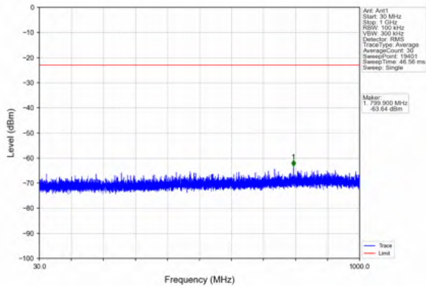
n25_15kHz_SISO_NTNV_25MHz_DFT-s-OFDM QPSK_1862.5MHz_Inner_1RB_Left
