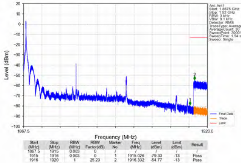
n25_15kHz_SISO_NTNV_30MHz_DFT-s-OFDM QPSK_1882.5MHz_Edge_1RB_Left
