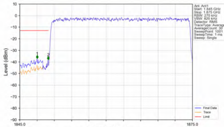
n25_15kHz_SISO_NTV_25MHz_CP-OFDM QPSK_1862.5MHz_Outer_Full
