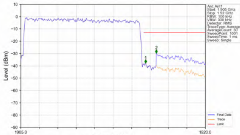
n25_15kHz_SISO_NTNV_10MHz_CP-OFDM QPSK_1910MHz_Outer_Full
