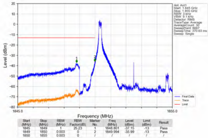
n25_15kHz_SISO_NTNV_5MHz_DFT-s-OFDM QPSK_1852.5MHz_Edge_1RB_Left
