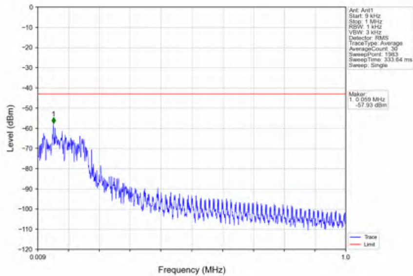
n25_15kHz_SISO_NTNV_10MHz_DFT-s-OFDM QPSK_185MHz_Inner_1RB_Left
