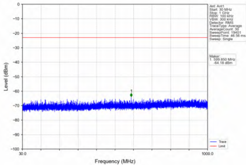
n25_15kHz_SISO_NTNV_15MHz_DFT-s-OFDM QPSK_1907.5MHz_Inner_1RB_Right
