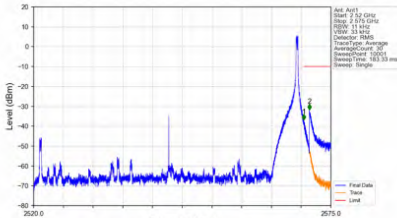
n7_30kHz_SISO_NTNV_50MHz_DFT-s-OFDM QPSK_2545MHz_Edge_1RB_Right
