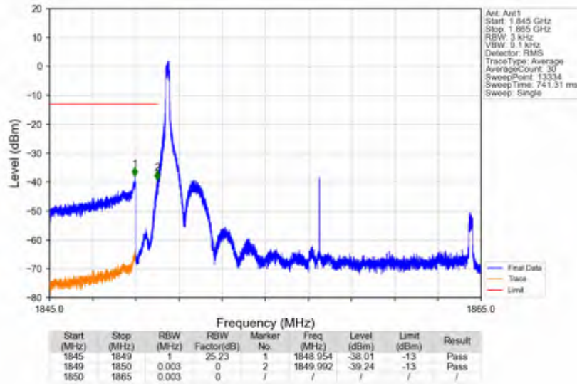
n25_15kHz_SISO_NTV_15MHz_CP-OFDM QPSK_1857.5MHz_Edge_1RB_Left
