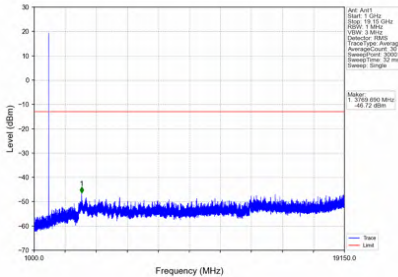
n25_15kHz_SISO_NTNV_5MHz_CP-OFDM QPSK_1852.5MHz_Outer_Full
