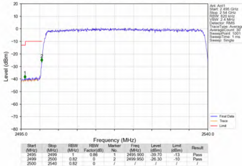
n7_30kHz_SISO_NTNV_40MHz_CP-OFDM QPSK_2520MHz_Outer_Full
