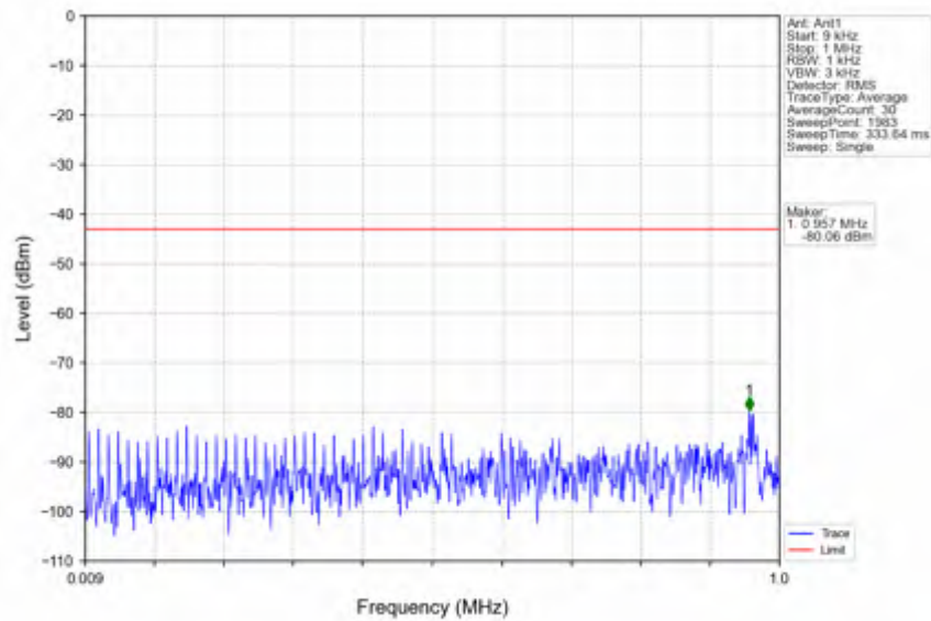
n25_15kHz_SISO_NTNV_15MHz_DFT-s-OFDM PI/2 BPSK_1857.5MHz_Outer_Full
