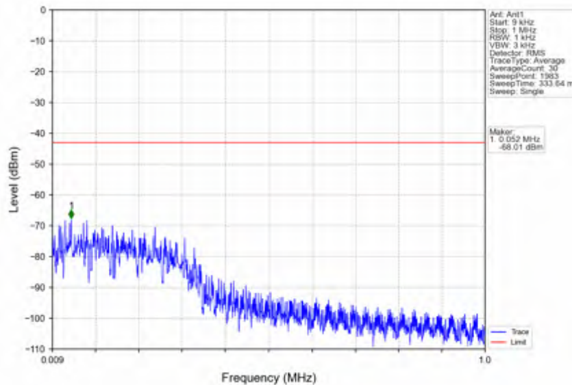
n7_30kHz_SISO_NTNV_40MHz_CP-OFDM QPSK_2535MHz_Edge_1RB_Left
