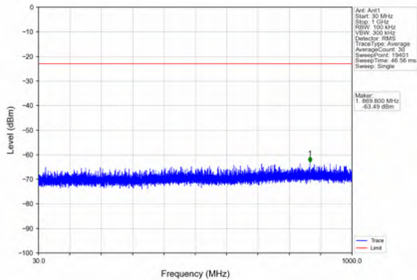
n7_30kHz_SISO_NTNV_50MHz_DFT-s-OFDM QPSK_2545MHz_Edge_1RB_Right
