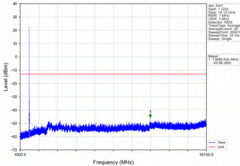
n25_15kHz_SISO_NTNV_15MHz_DFT-s-OFDM QPSK_1907.5MHz_Edge_1RB_Right
