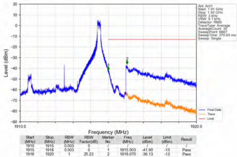
n25_15kHz_SISO_NTNV_5MHz_DFT-s-OFDM QPSK_1912.5MHz_Inner_1RB_Right
