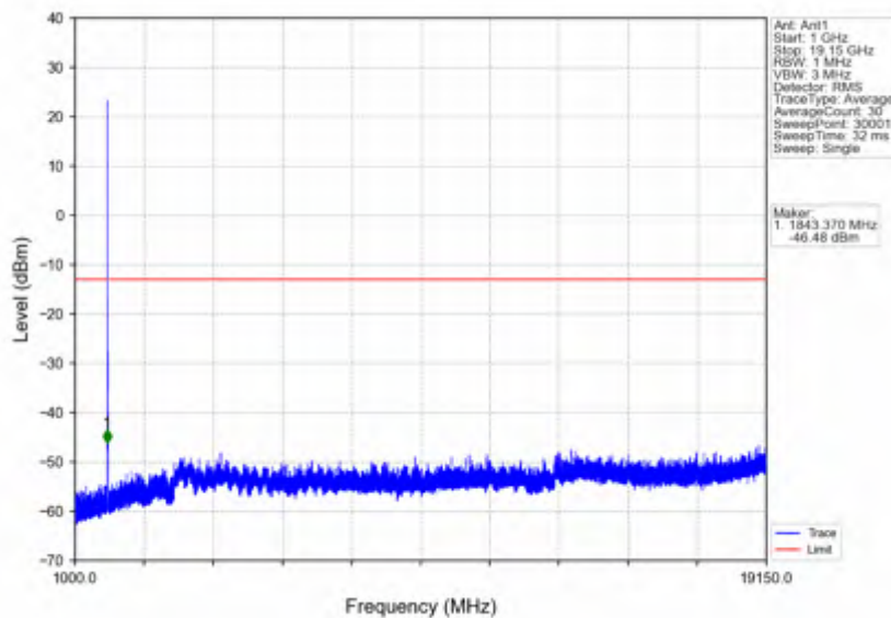
n25_15kHz_SISO_NTNV_10MHz_DFT-s-OFDM QPSK_185MHz_Inner_1RB_Left
