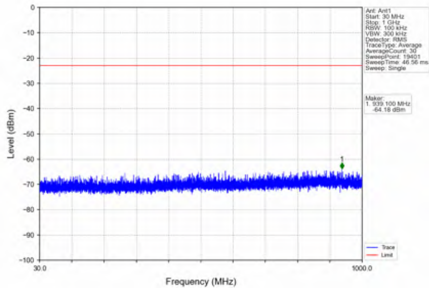
n25_15kHz_SISO_NTVV_10MHz_CP-OFDM QPSK_1882.5MHz_Edge_1RB_Left
