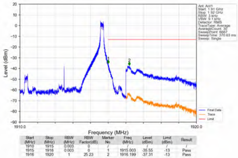
n25_15kHz_SISO_NTNV_5MHz_DFT-s-OFDM QPSK_1912.5MHz_Edge_1RB_Right
