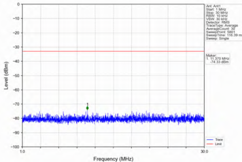
n25_15kHz_SISO_NTNV_15MHz_DFT-s-OFDM QPSK_1907.5MHz_Edge_1RB_Right
