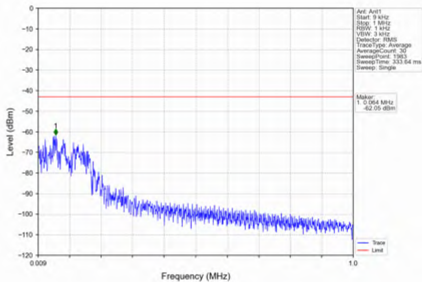
n25_15kHz_SISO_NTNV_10MHz_DFT-s-OFDM_PI/2_BPSK_1855MHz_Edge_1RB_Left
