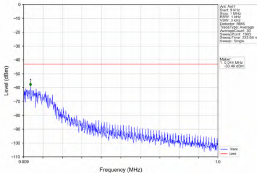
n25_15kHz_SISO_NTNV_15MHz_CP-OFDM QPSK_1857.5MHz_Inner_1RB_Left
