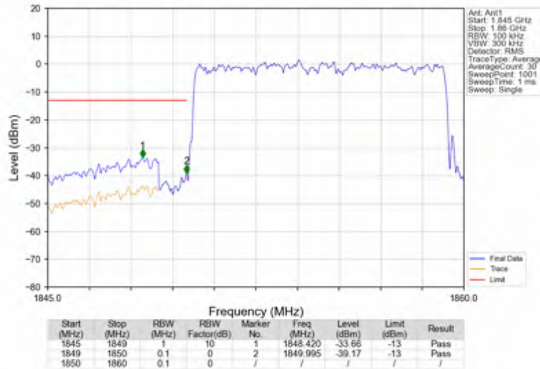
n25_15kHz_SISO_NTNV_10MHz_DFT-s-OFDM QPSK_1855MHz_Outer_Full
