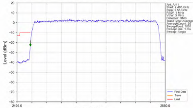
n7_30kHz_SISO_NTNV_50MHz_DFT-s-OFDM PI/2 BPSK_2525MHz_Outer_Full
