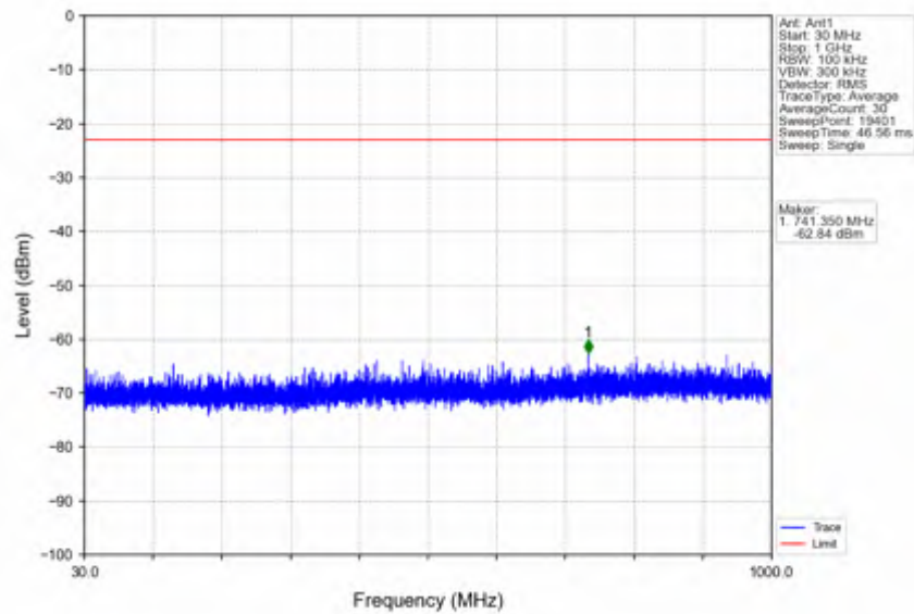
n7_30kHz_SISO_NTNV_50MHz_CP-OFDM QPSK_2545MHz_Edge_1RB_Right
