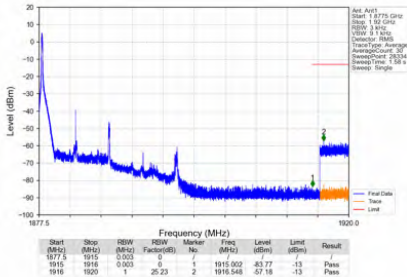
n25_15kHz_SISO_NTNV_10MHz_DFT-s-OFDM PI/2 BPSK_1882.5MHz_Edge_1RB_Left
