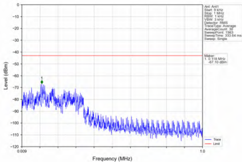
n7_30kHz_SISO_NTNV_50MHz_DFT-s-OFDM_PI/2_BPSK_2525MHz_Edge_1RB_Left
