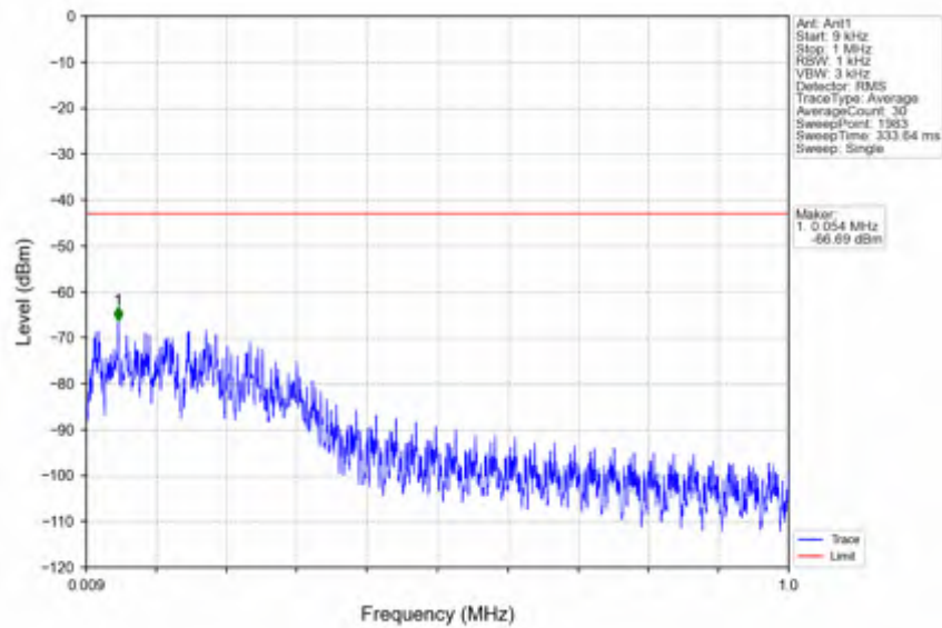
n7_30kHz_SISO_NTNV_40MHz_CP-OFDM QPSK_2550MHz_Edge_1RB_Right
