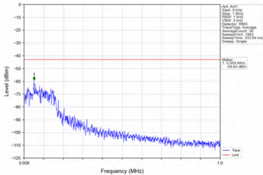
n25_15kHz_SISO_NTNV_5MHz_DFT-s-OFDM QPSK_1852.5MHz_Edge_1RB_Left
