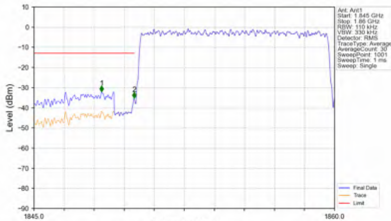
n25_15kHz_SISO_NTNV_10MHz_CP-OFDM QPSK_1855MHz_Outer_Full
