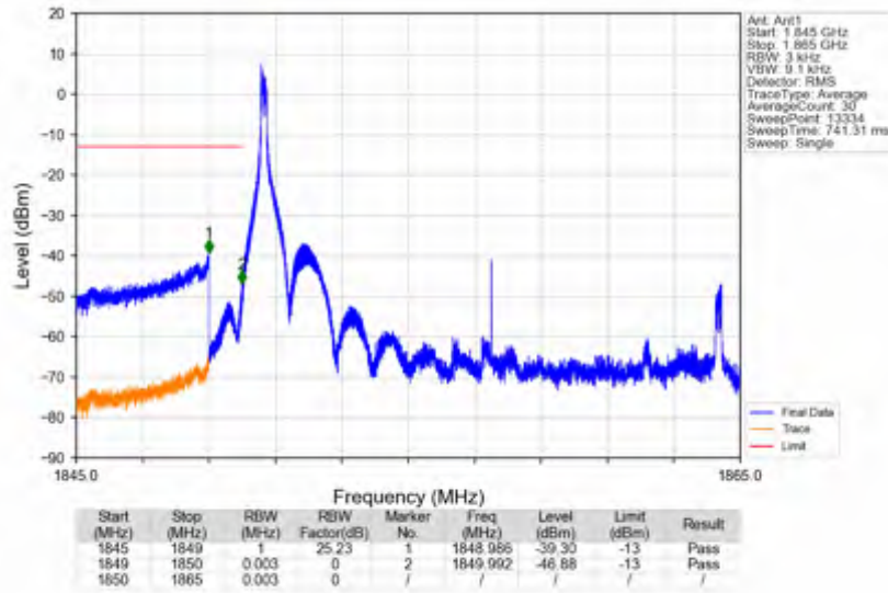
n25_15kHz_SISO_NTNV_15MHz_DFT-s-OFDM PI/2 BPSK_1857.5MHz_Inner_1RB_Left
