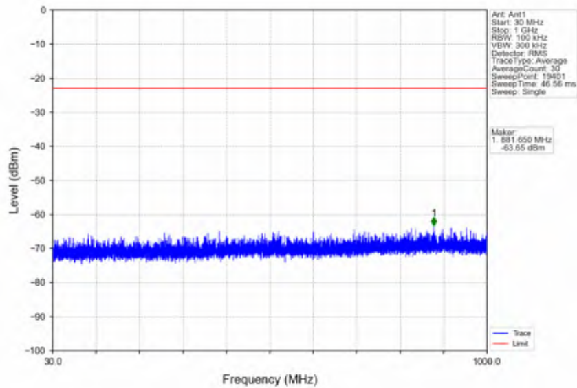
n25_15kHz_SISO_NTNV_15MHz_DFT-s-OFDM QPSK_1857.5MHz_Edge_1RB_Left
