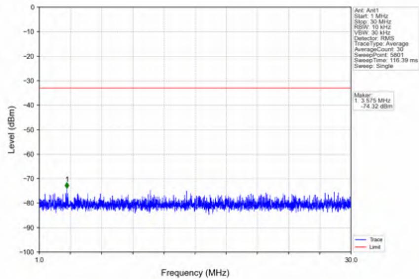
n25_15kHz_SISO_NTNV_10MHz_DFT-s-OFDM QPSK_1910MHz_Outer_Full
