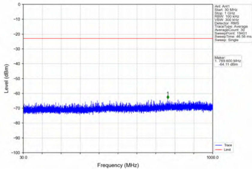
n25_15kHz_SISO_NTNV_5MHz_DFT-s-OFDM QPSK_1912.5MHz_Edge_1RB_Right
