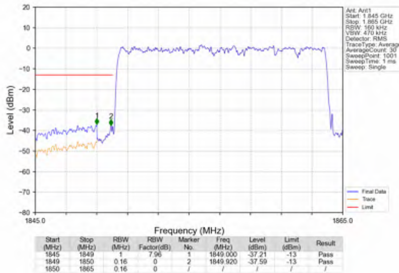
n25_15kHz_SISO_NTNV_15MHz_DFT-s-OFDM QPSK_1857.5MHz_Outer_Full
