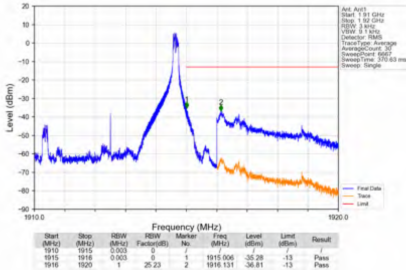
n25_15kHz_SISO_NTNV_5MHz_DFT-s-OFDM PI/2 BPSK_1912.5MHz_Edge_1RB_Right
