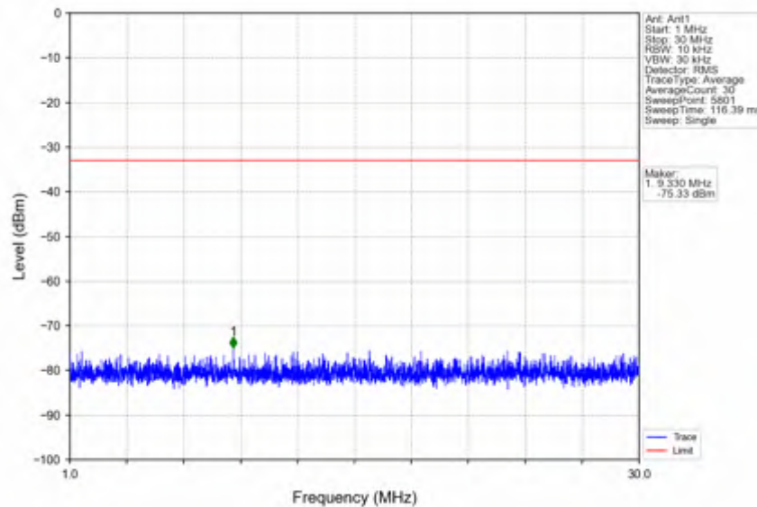
n25_15kHz_SISO_NTNV_15MHz_DFT-s-OFDM_QPSK_1857.5MHz_Inner_1RB_Left
