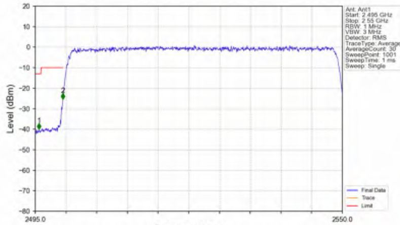
n7_30kHz_SISO_NTNV_50MHz_CP-OFDM QPSK_2525MHz_Outer_Full
