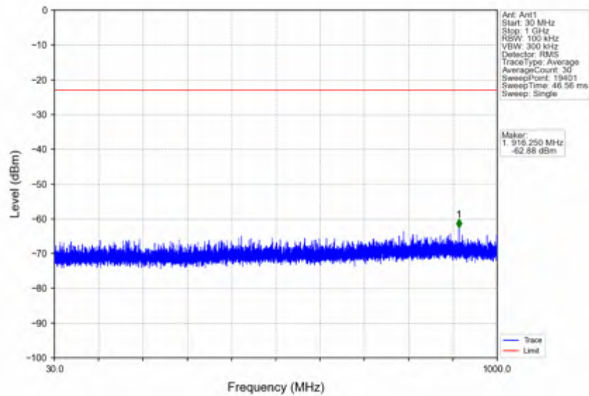
n25_15kHz_SISO_NTNV_10MHz_CP-OFDM QPSK_1855MHz_Outer_Full
