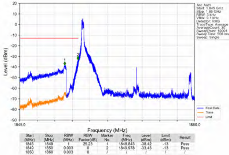
n25_15kHz_SISO_NTNV_10MHz_DFT-s-OFDM_PI/2_BPSK_1855MHz_Edge_1RB_Left
