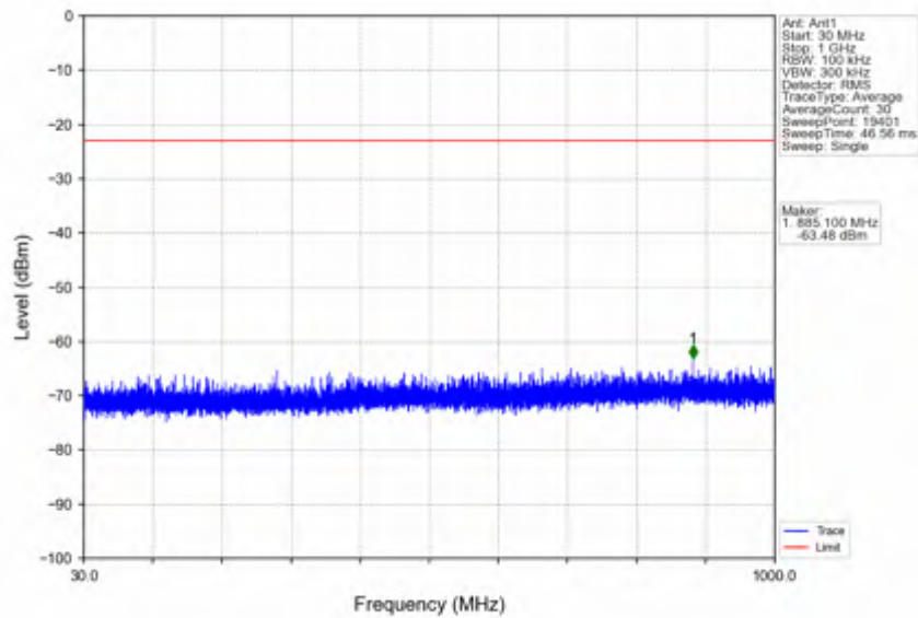
n25_15kHz_SISO_NTNV_10MHz_DFT-s-OFDM QPSK_1910MHz_Inner_1RB_Right
