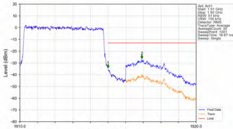
n25_15kHz_SISO_NTNV_5MHz_DFT-s-OFDM PI/2 BPSK_1912.5MHz_Outer_Full
