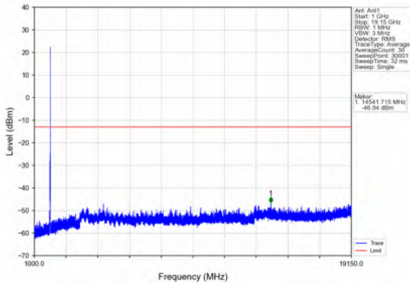
n25_15kHz_SISO_NTNV_15MHz_DFT-s-OFDM QPSK_1857.5MHz_Edge_1RB_Left
