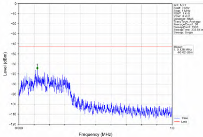
n7_30kHz_SISO_NTV_50MHz_DFT-s-OFDM QPSK_2525MHz_Edge_1RB_Left
