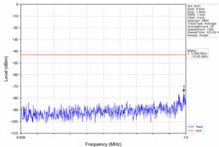
n25_15kHz_SISO_NTNV_10MHz_DFT-s-OFDM QPSK_1855MHz_Outer_Full
