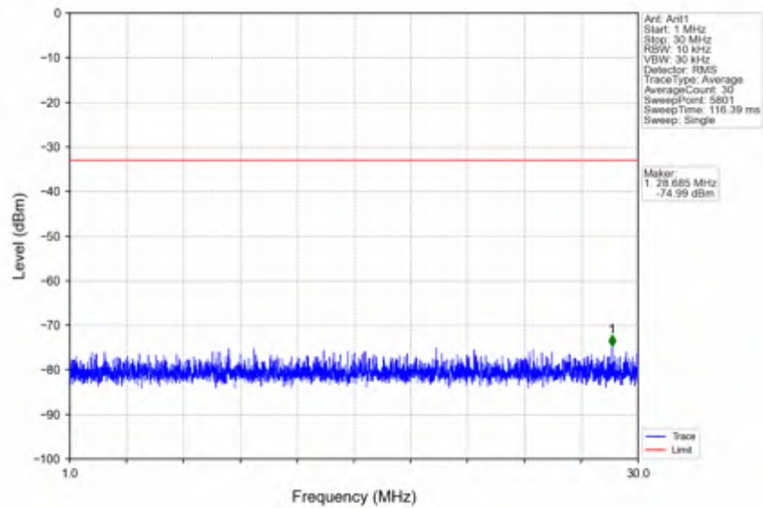
n25_15kHz_SISO_NTNV_5MHz_DFT-s-OFDM QPSK_1852.5MHz_Outer_Full
