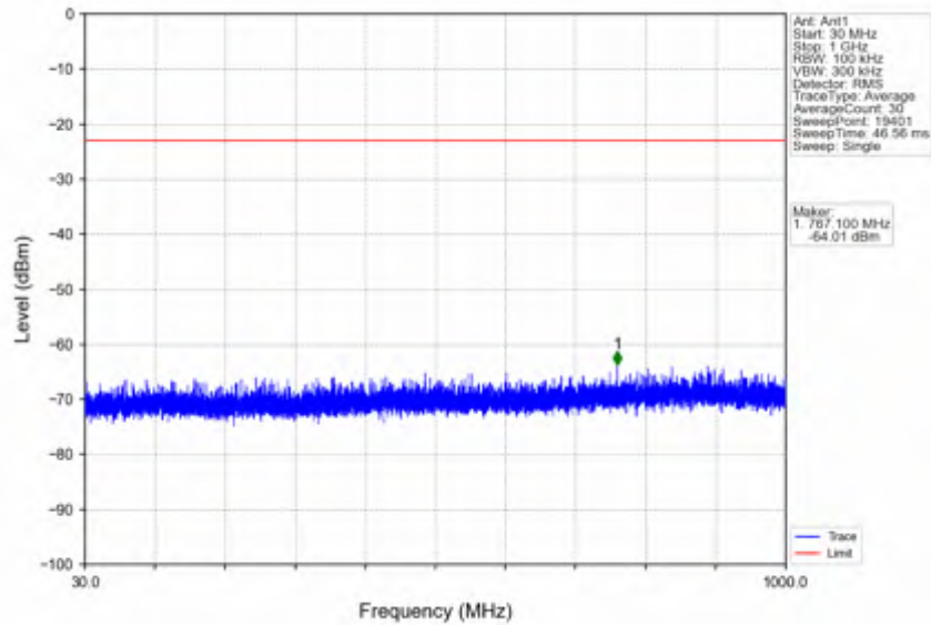
n25_15kHz_SISO_NTNV_5MHz_DFT-s-OFDM QPSK_1912.5MHz_Inner_1RB_Right
