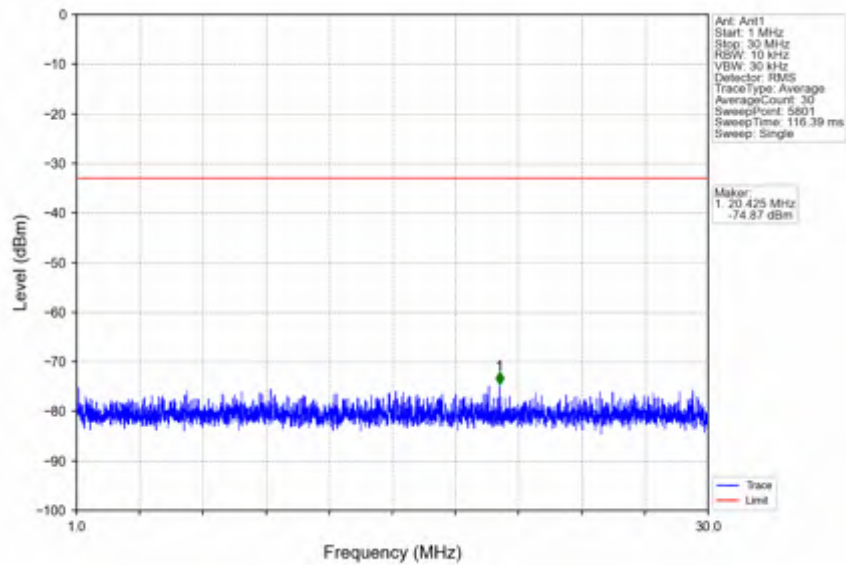
n25_15kHz_SISO_NTNV_10MHz_CP-OFDM QPSK_1910MHz_Inner_1RB_Right
