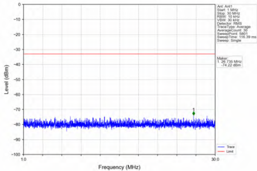
n7_30kHz_SISO_NTNV_40MHz_CP-OFDM QPSK_2535MHz_Edge_1RB_Left
