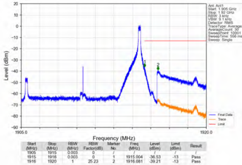
n25_15kHz_SISO_NTNV_10MHz_CP-OFDM QPSK_1910MHz_Edge_1RB_Right
