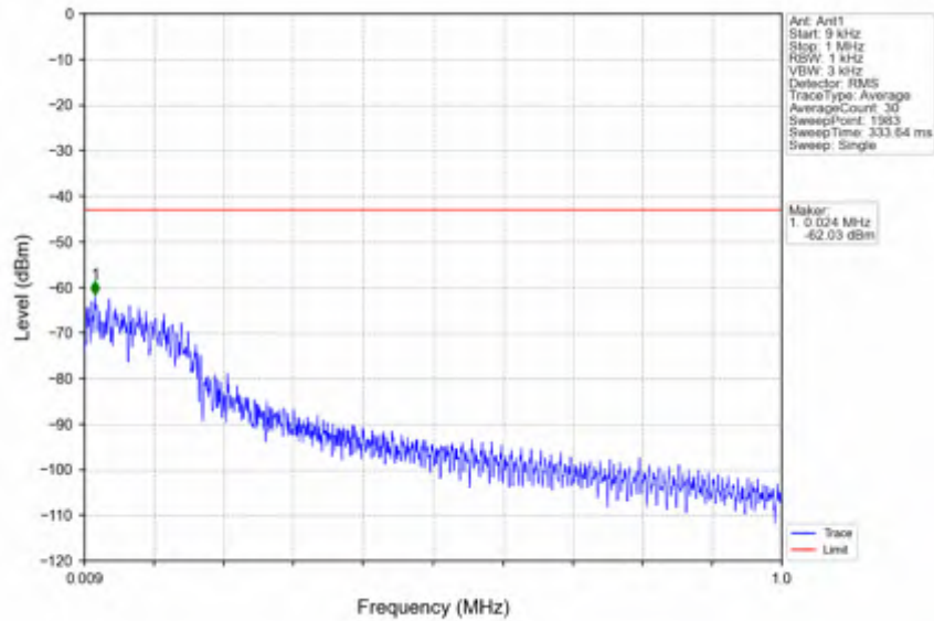
n25_15kHz_SISO_NTVV_10MHz_CP-OFDM QPSK_1882.5MHz_Edge_1RB_Left
