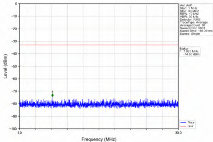
n25_15kHz_SISO_NTNV_5MHz_DFT-s-OFDM QPSK_1912.5MHz_Edge_1RB_Right
