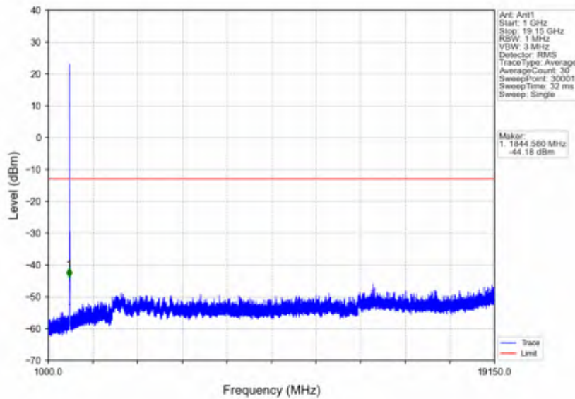
n25_15kHz_SISO_NTNV_15MHz_DFT-s-OFDM PI/2 BPSK_1882.5MHz_Edge_1RB_Left
