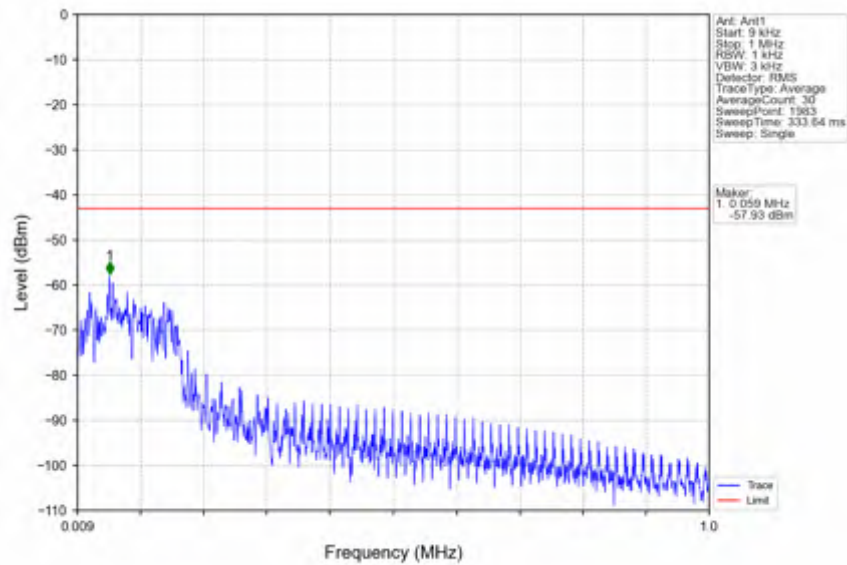
n25_15kHz_SISO_NTNV_15MHz_DFT-s-OFDM QPSK_1907.5MHz_Inner_1RB_Right
