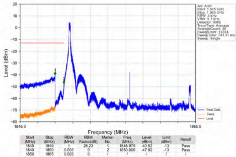
n25_15kHz_SISO_NTNV_15MHz_DFT-s-OFDM QPSK_1857.5MHz_Inner_1RB_Left
