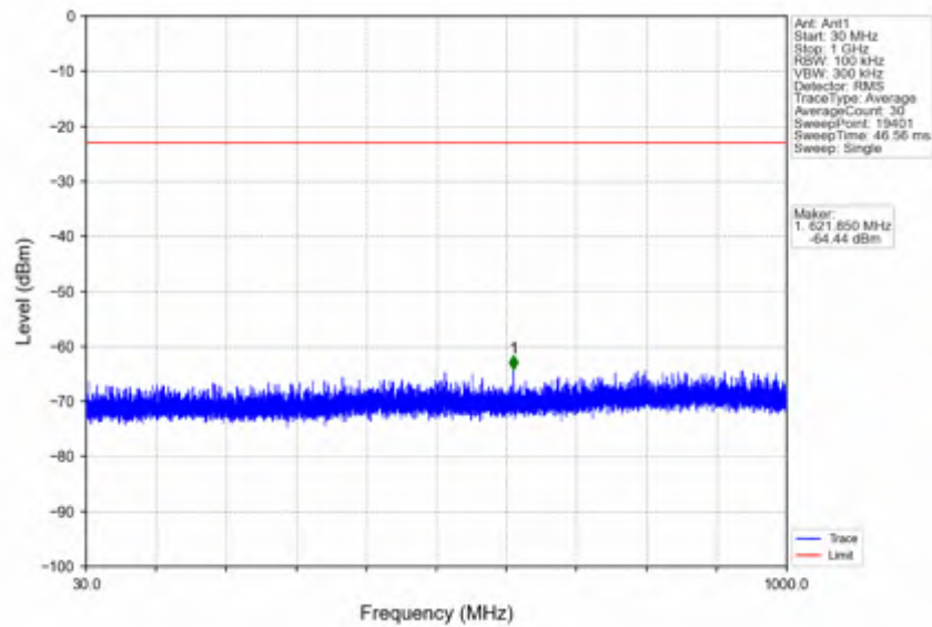
n25_15kHz_SISO_NTNV_15MHz_CP-OFDM QPSK_1857.5MHz_Outer_Full
