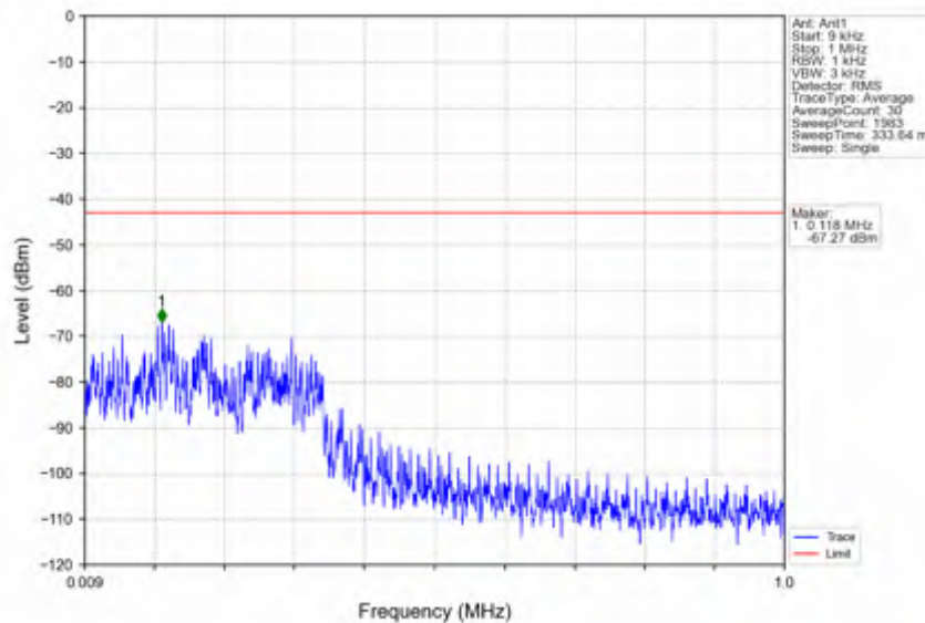
n7_30kHz_SISO_NTNV_50MHz_DFT-s-OFDM PI/2 BPSK_2535MHz_Edge_1RB_Left
