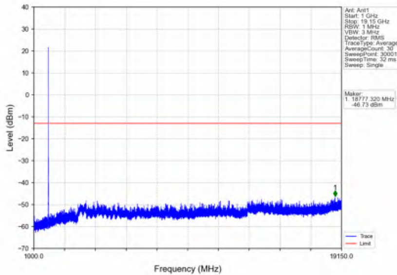
n25_15kHz_SISO_NTNV_10MHz_DFT-s-OFDM QPSK_185MHz_Edge_1RB_Left
