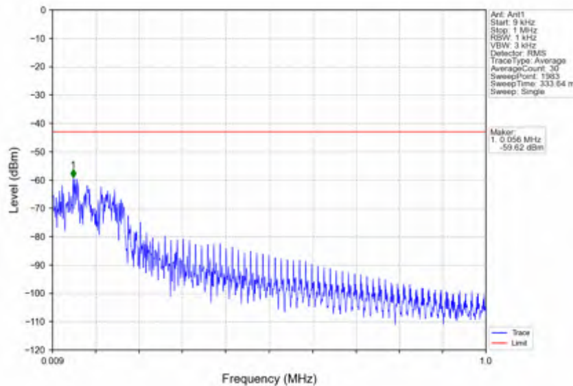
n25_15kHz_SISO_NTNV_5MHz_DFT-s-OFDM PI/2 BPSK_1912.5MHz_Inner_1RB_Right
