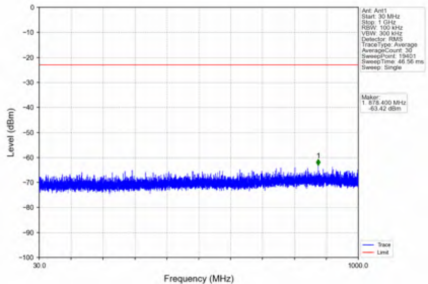
n25_15kHz_SISO_NTNV_10MHz_DFT-s-OFDM QPSK_1882.5MHz_Edge_1RB_Left
