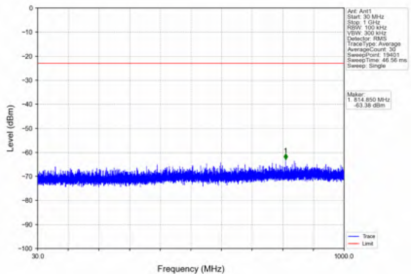
n25_15kHz_SISO_NTNV_5MHz_CP-OFDM QPSK_1912.5MHz_Inner_1RB_Right
