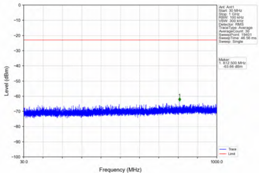
n25_15kHz_SISO_NTNV_15MHz_DFT-s-OFDM_QPSK_1857.5MHz_Outer_Full
