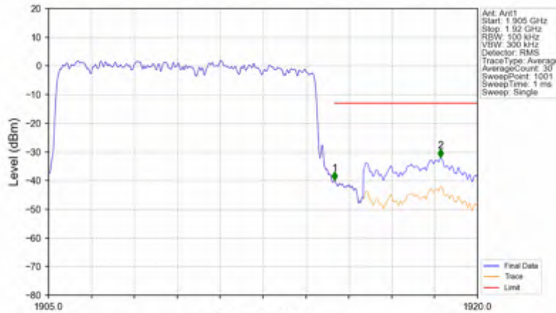
n25_15kHz_SISO_NTNV_10MHz_DFT-s-OFDM PI/2 BPSK_1910MHz_Outer_Full
