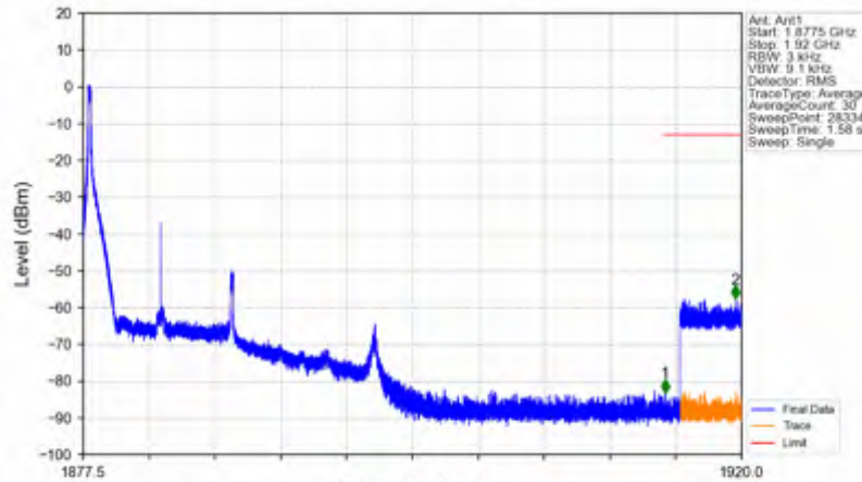
n25_15kHz_SISO_NTNV_10MHz_CP-OFDM QPSK_1882.5MHz_Edge_1RB_Left
