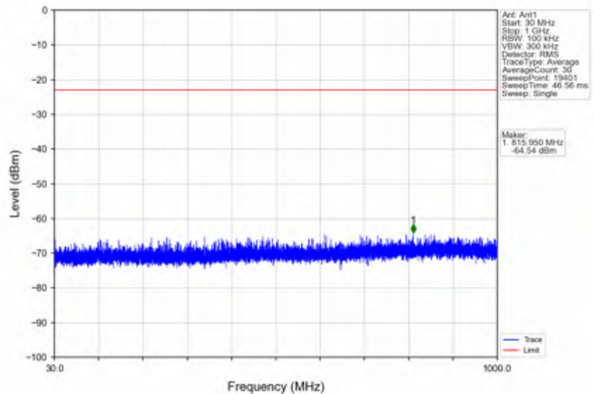
n25_15kHz_SISO_NTNV_15MHz_CP-OFDM QPSK_1857.5MHz_Inner_1RB_Left
