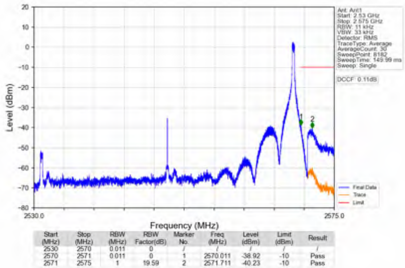
n7_30kHz_SISO_NTNV_40MHz_CP-OFDM QPSK_2550MHz_Edge_1RB_Right
