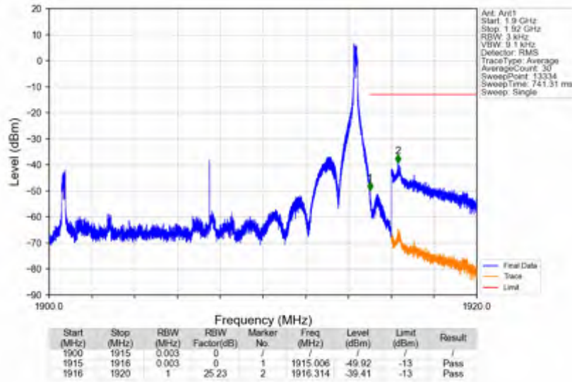
n25_15kHz_SISO_NTNV_15MHz_DFT-s-OFDM PI/2 BPSK_1907.5MHz_Inner_1RB_Right
