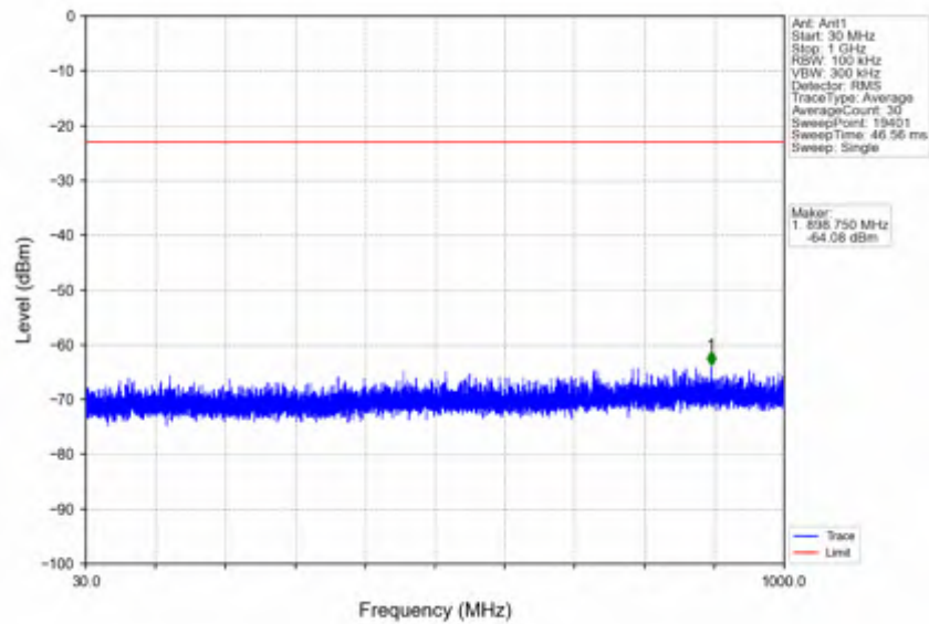
n25_15kHz_SISO_NTNV_10MHz_DFT-s-OFDM QPSK_185MHz_Edge_1RB_Left
