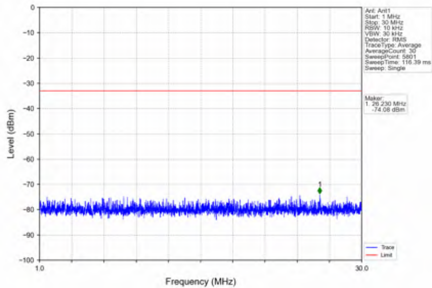
n7_30kHz_SISO_NTNV_50MHz_CP-OFDM QPSK_2525MHz_Edge_1RB_Left
