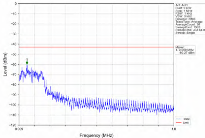
n25_15kHz_SISO_NTNV_15MHz_DFT-s-OFDM QPSK_1882.5MHz_Edge_1RB_Left
