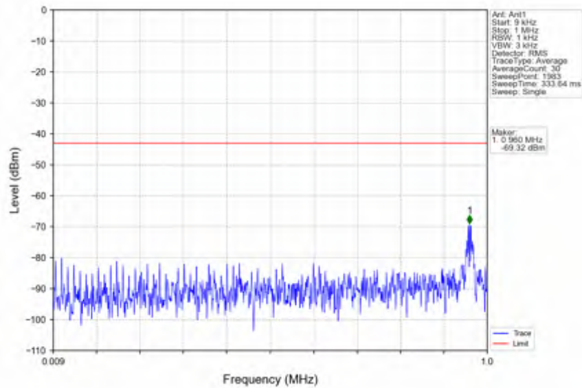
n25_15kHz_SISO_NTNV_15MHz_DFT-s-OFDM PI/2 BPSK_1907.5MHz_Outer_Full
