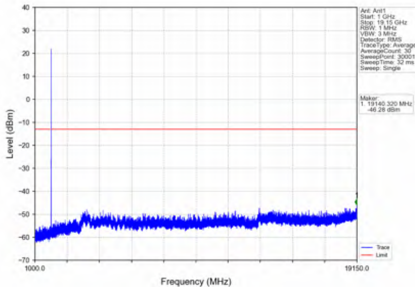
n25_15kHz_SISO_NTNV_5MHz_DFT-s-OFDM QPSK_1912.5MHz_Inner_1RB_Right
