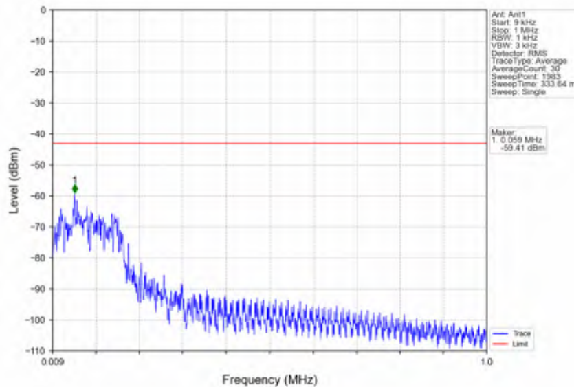
n25_15kHz_SISO_NTNV_10MHz_DFT-s-OFDM QPSK_1882.5MHz_Edge_1RB_Left
