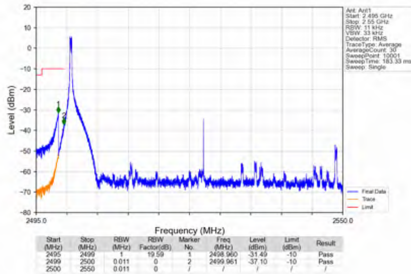
n7_30kHz_SISO_NTV_50MHz_DFT-s-OFDM QPSK_2525MHz_Edge_1RB_Left
