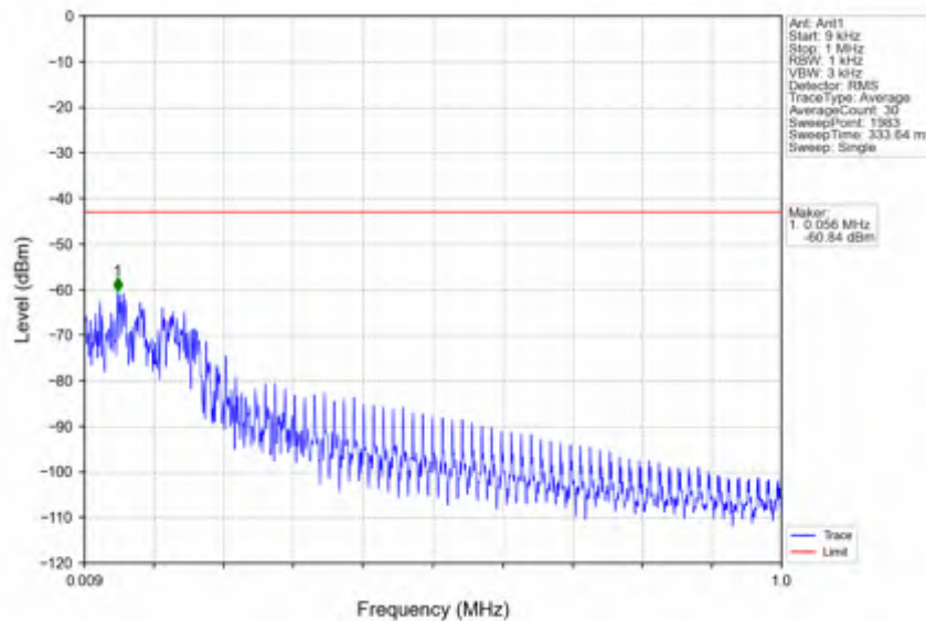
n25_15kHz_SISO_NTNV_5MHz_DFT-s-OFDM PI/2 BPSK_1852.5MHz_Inner_1RB_Left
