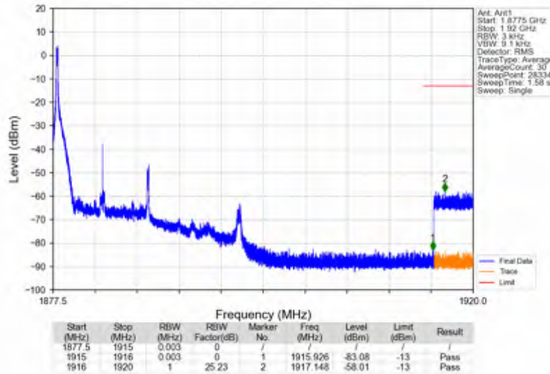
n25_15kHz_SISO_NTNV_10MHz_DFT-s-OFDM QPSK_1882.5MHz_Edge_1RB_Left
