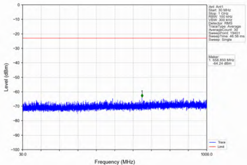
n25_15kHz_SISO_NTNV_10MHz_CP-OFDM QPSK_1855MHz_Edge_1RB_Left
