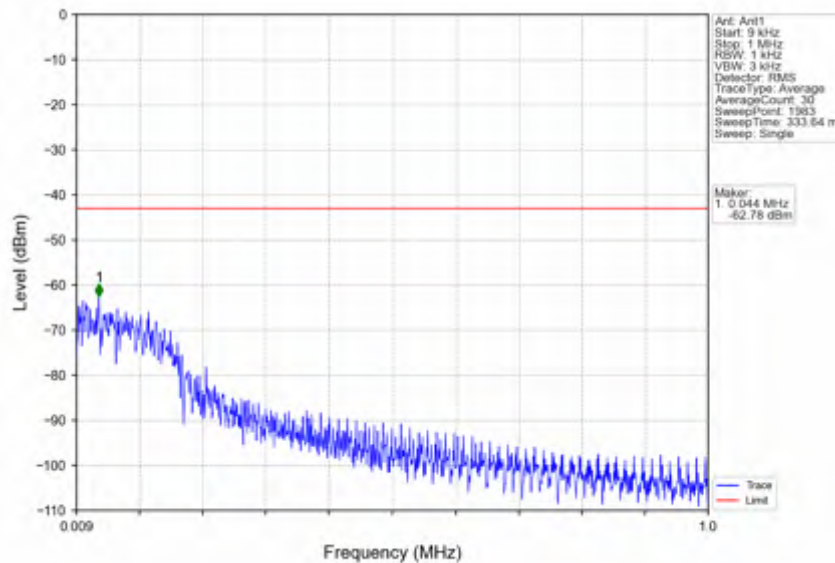
n25_15kHz_SISO_NTV_15MHz_CP-OFDM QPSK_1857.5MHz_Edge_1RB_Left
