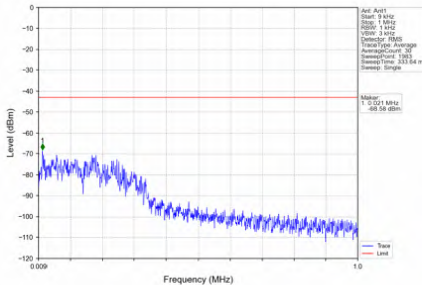
n7_30kHz_SISO_NTNV_50MHz_CP-OFDM_QPSK_2525MHz_Edge_1RB_Left
