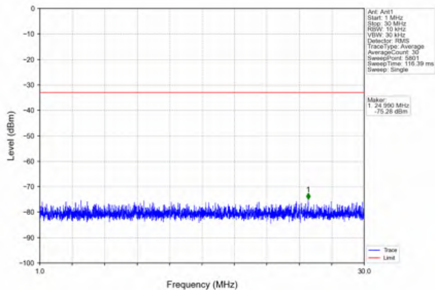
n25_15kHz_SISO_NTNV_5MHz_CP-OFDM QPSK_1912.5MHz_Outer_Full
