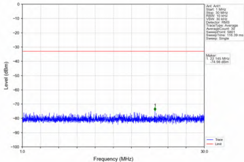
n25_15kHz_SISO_NTNV_10MHz_DFT-s-OFDM QPSK_1910MHz_Inner_1RB_Right
