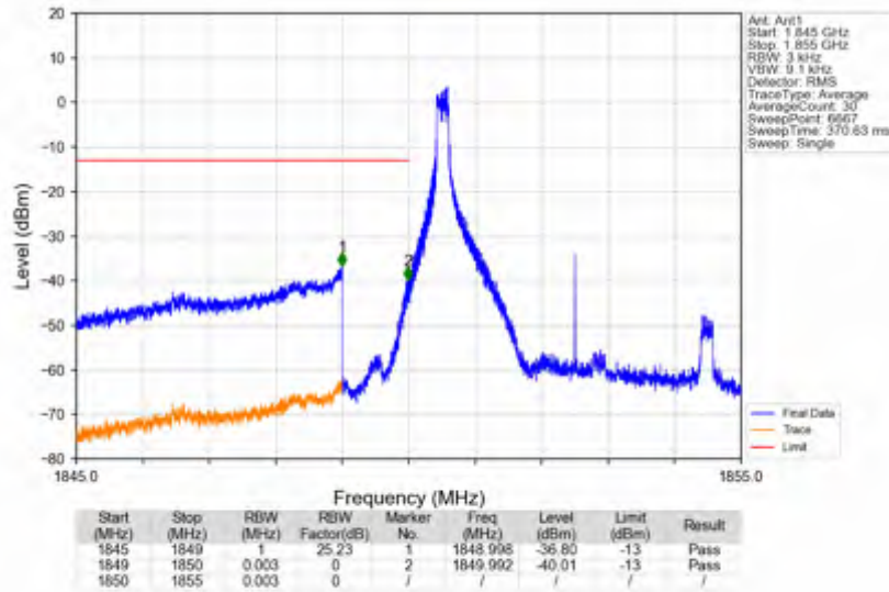
n25_15kHz_SISO_NTNV_5MHz_CP-OFDM QPSK_1852.5MHz_Inner_1RB_Left
