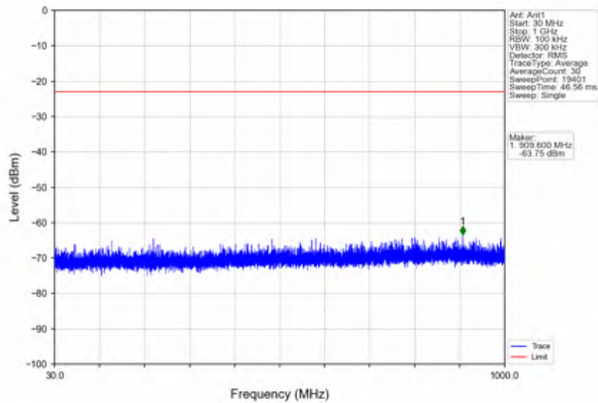
n25_15kHz_SISO_NTNV_10MHz_DFT-s-OFDM QPSK_1910MHz_Edge_1RB_Right
