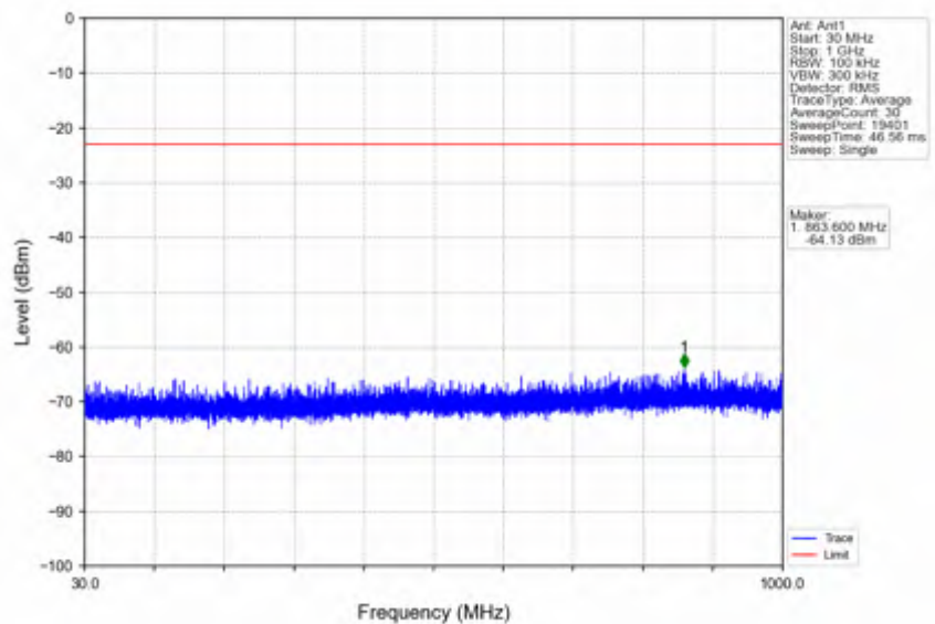
n25_15kHz_SISO_NTNV_5MHz_DFT-s-OFDM QPSK_1882.5MHz_Edge_1RB_Left
