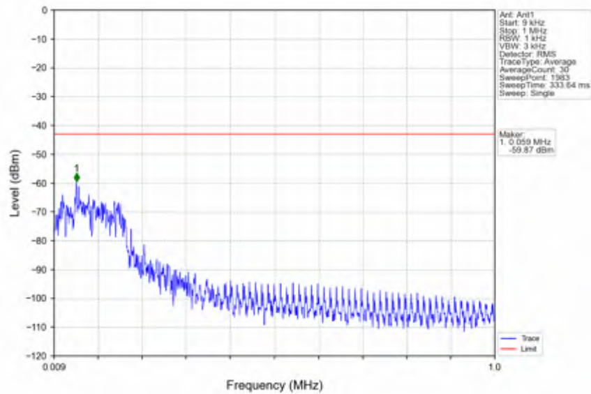
n25_15kHz_SISO_NTNV_15MHz_DFT-s-OFDM QPSK_1857.5MHz_Edge_1RB_Left
