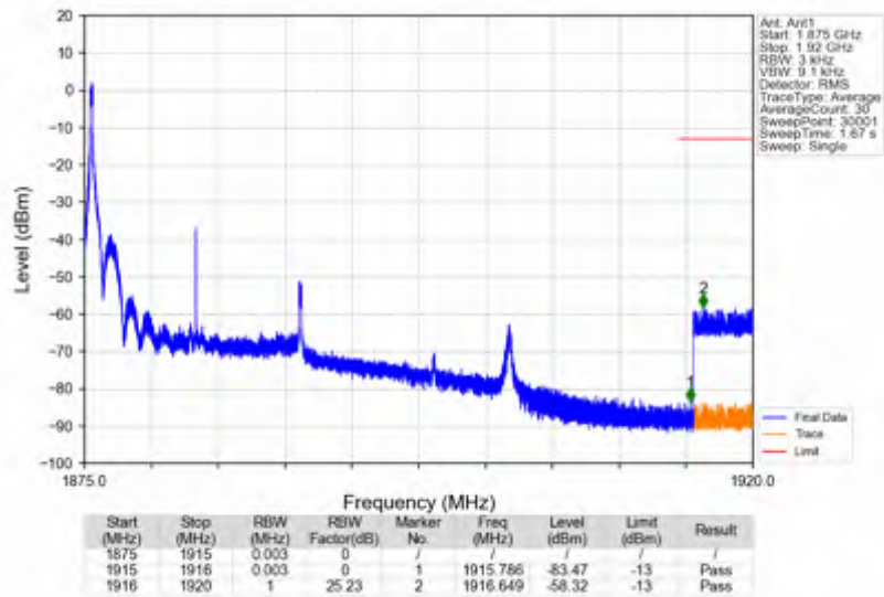
n25_15kHz_SISO_NTV_15MHz_CP-OFDM QPSK_1882.5MHz_Edge_1RB_Left
