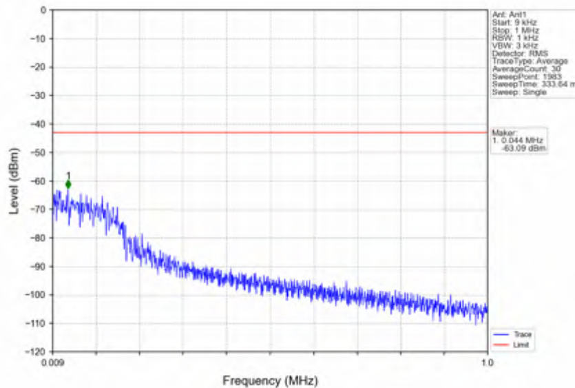
n25_15kHz_SISO_NTNV_10MHz_CP-OFDM QPSK_1855MHz_Edge_1RB_Left
