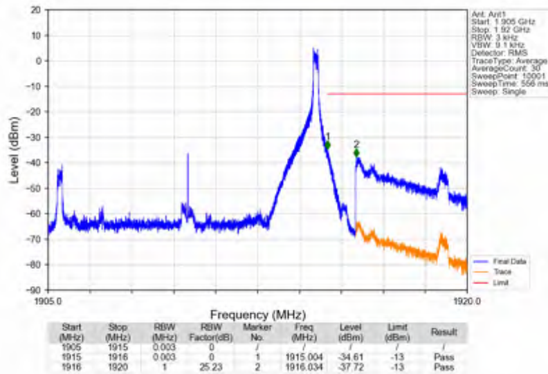
n25_15kHz_SISO_NTNV_10MHz_DFT-s-OFDM QPSK_1910MHz_Edge_1RB_Right
