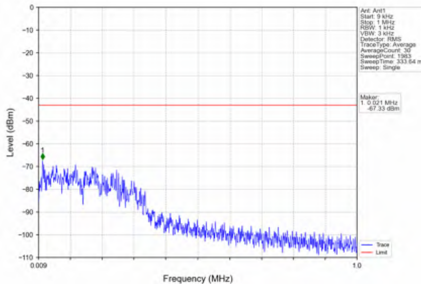
n7_30kHz_SISO_NTNV_50MHz_CP-OFDM QPSK_2535MHz_Edge_1RB_Left
