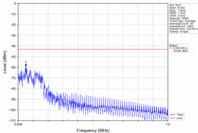
n25_15kHz_SISO_NTNV_10MHz_DFT-s-OFDM PI/2 BPSK_1910MHz_Inner_1RB_Right
