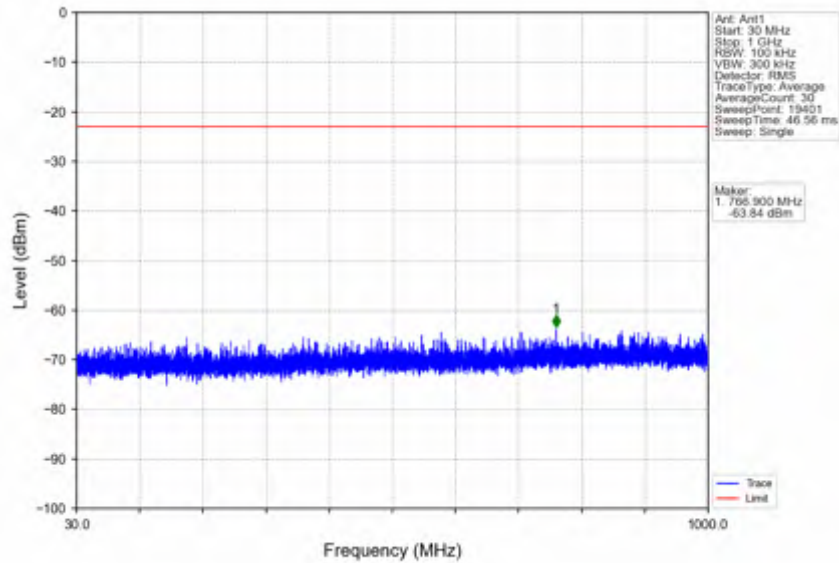
n25_15kHz_SISO_NTNV_5MHz_DFT-s-OFDM QPSK_1852.5MHz_Edge_1RB_Left
