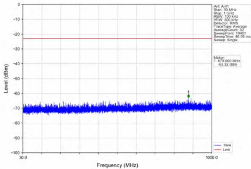
n25_15kHz_SISO_NTV_15MHz_CP-OFDM QPSK_1882.5MHz_Edge_1RB_Left
