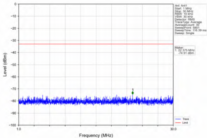
n25_15kHz_SISO_NTNV_10MHz_CP-OFDM QPSK_1910MHz_Outer_Full
