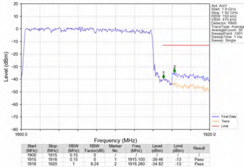
n25_15kHz_SISO_NTNV_15MHz_DFT-s-OFDM_QPSK_1907.5MHz_Outer_Full
