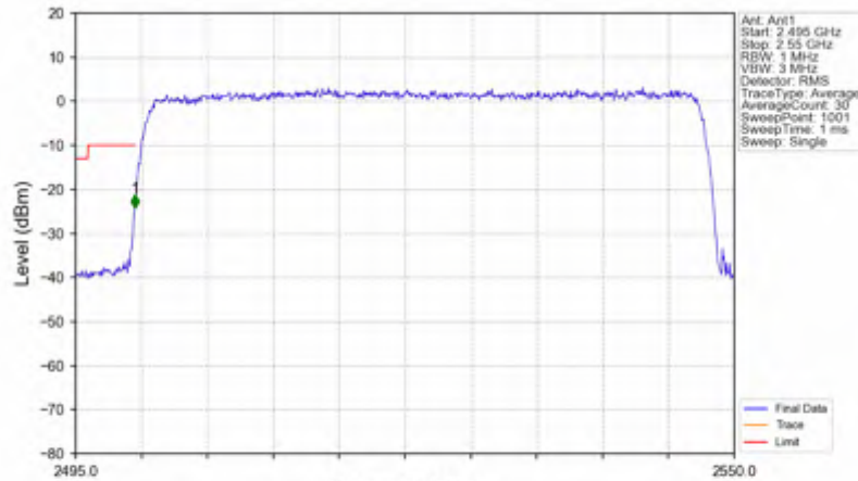
n7_30kHz_SISO_NTNV_50MHz_DFT-s-OFDM_QPSK_2525MHz_Outer_Full
