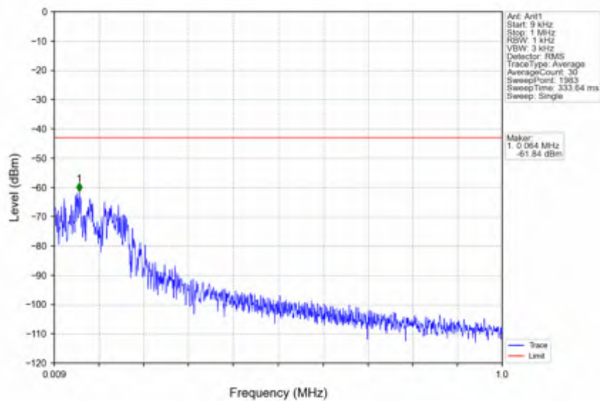
n25_15kHz_SISO_NTNV_5MHz_DFT-s-OFDM_PI/2_BPSK_1852.5MHz_Edge_1RB_Left
