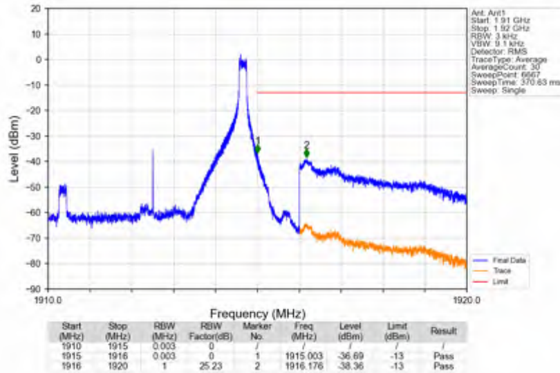
n25_15kHz_SISO_NTNV_5MHz_CP-OFDM QPSK_1912.5MHz_Edge_1RB_Right
