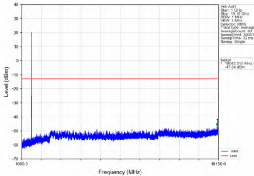
n25_15kHz_SISO_NTNV_10MHz_CP-OFDM QPSK_1910MHz_Inner_1RB_Right
