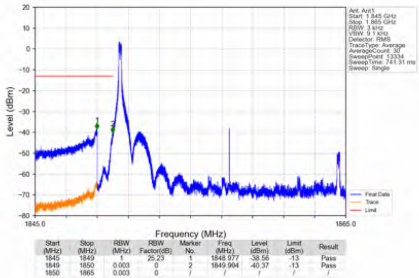
n25_15kHz_SISO_NTNV_15MHz_DFT-s-OFDM QPSK_1857.5MHz_Edge_1RB_Left
