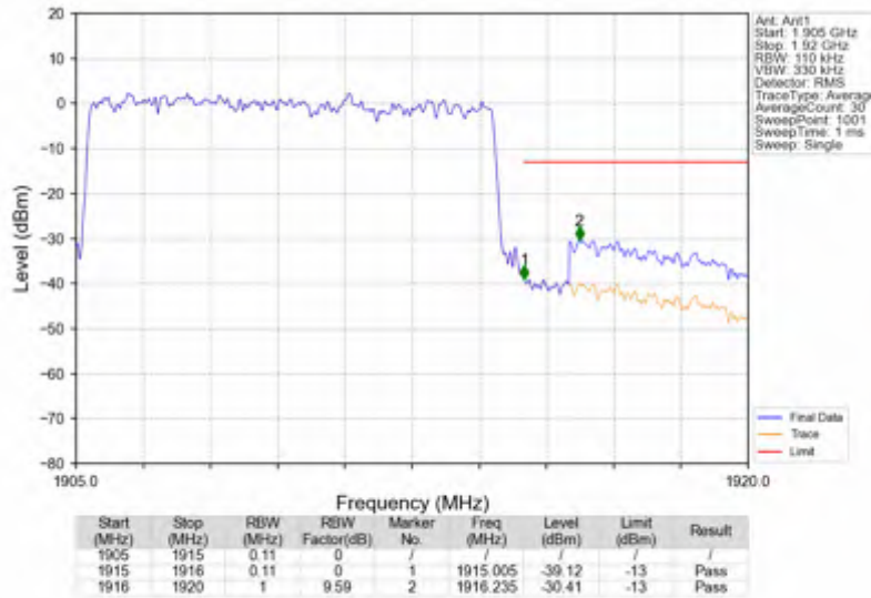
n25_15kHz_SISO_NTNV_10MHz_DFT-s-OFDM QPSK_1910MHz_Outer_Full
