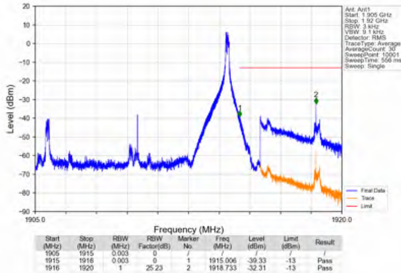
n25_15kHz_SISO_NTNV_10MHz_DFT-s-OFDM PI/2 BPSK_1910MHz_Inner_1RB_Right
