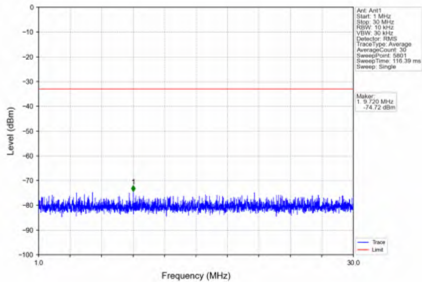
n25_15kHz_SISO_NTNV_15MHz_DFT-s-OFDM_QPSK_1907.5MHz_Outer_Full
