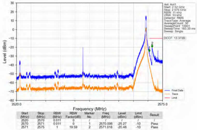
n7_30kHz_SISO_NTNV_50MHz_CP-OFDM QPSK_2545MHz_Edge_1RB_Right
