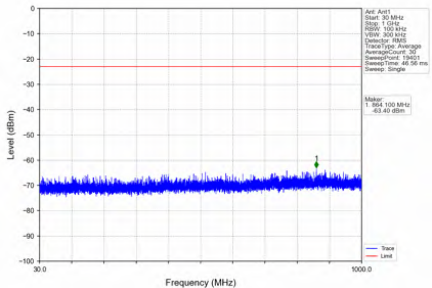
n25_15kHz_SISO_NTNV_10MHz_CP-OFDM QPSK_1910MHz_Edge_1RB_Right
