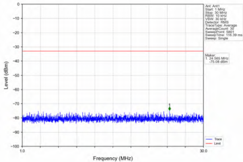
n25_15kHz_SISO_NTNV_5MHz_CP-OFDM QPSK_1852.5MHz_Edge_1RB_Left
