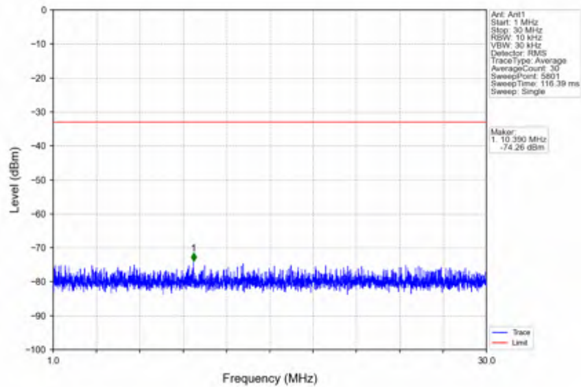
n7_30kHz_SISO_NTNV_50MHz_DFT-s-OFDM QPSK_2535MHz_Edge_1RB_Left
