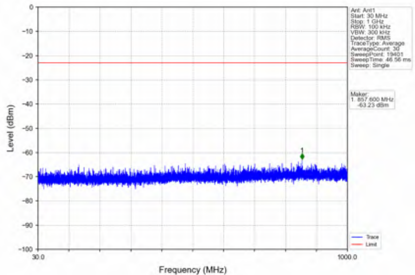
n25_15kHz_SISO_NTNV_15MHz_DFT-s-OFDM QPSK_1882.5MHz_Edge_1RB_Left
