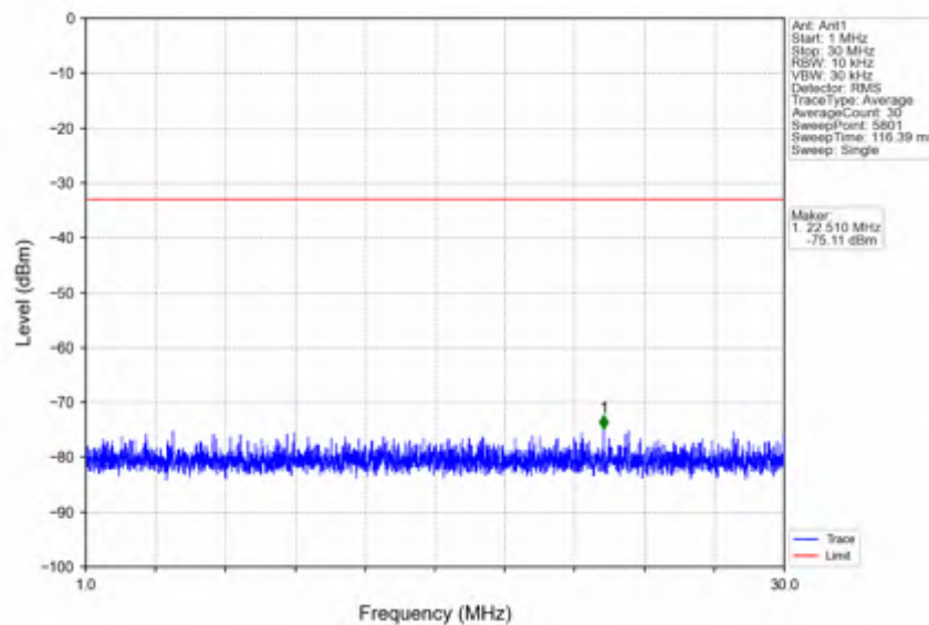
n25_15kHz_SISO_NTNV_5MHz_DFT-s-OFDM QPSK_1852.5MHz_Inner_1RB_Left
