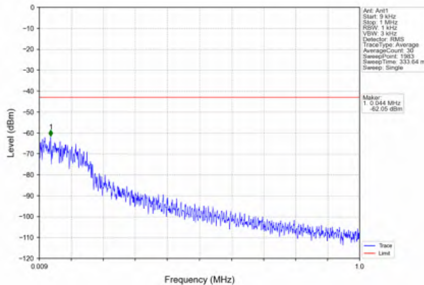
n25_15kHz_SISO_NTNV_5MHz_CP-OFDM QPSK_1912.5MHz_Edge_1RB_Right
