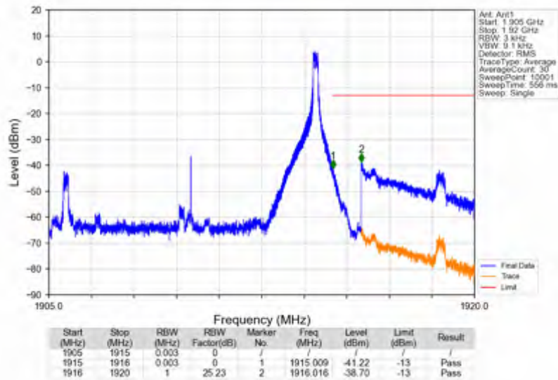
n25_15kHz_SISO_NTNV_10MHz_DFT-s-OFDM QPSK_1910MHz_Inner_1RB_Right
