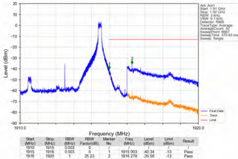
n25_15kHz_SISO_NTNV_5MHz_CP-OFDM QPSK_1912.5MHz_Inner_1RB_Right
