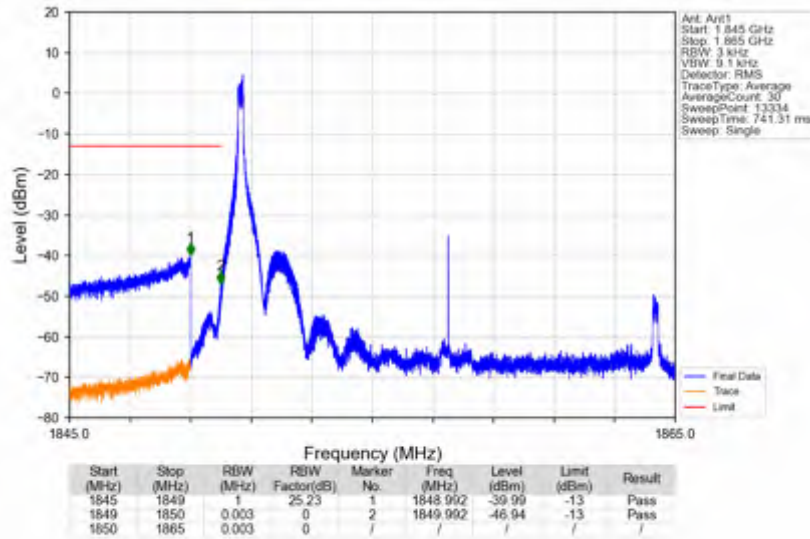
n25_15kHz_SISO_NTNV_15MHz_CP-OFDM QPSK_1857.5MHz_Inner_1RB_Left
