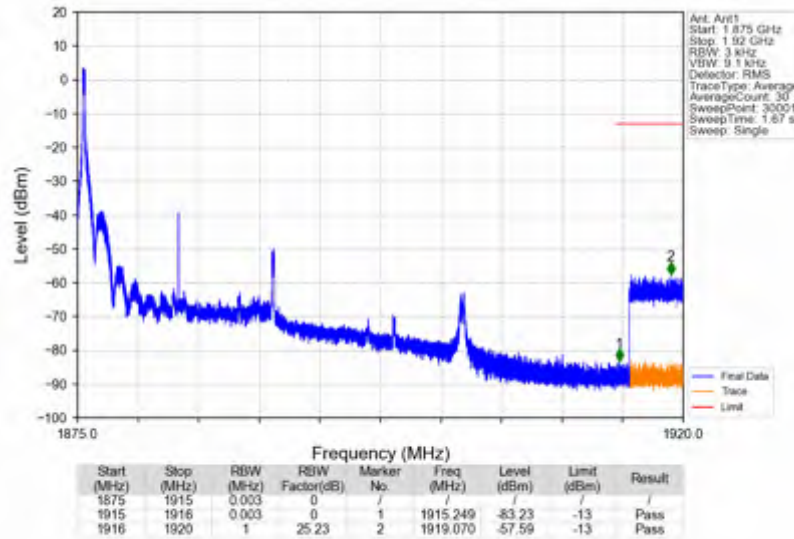
n25_15kHz_SISO_NTNV_15MHz_DFT-s-OFDM QPSK_1882.5MHz_Edge_1RB_Left
