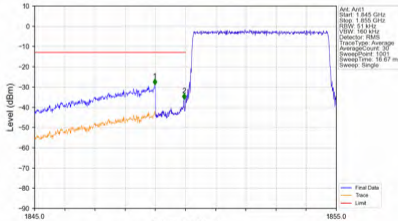
n25_15kHz_SISO_NTNV_5MHz_CP-OFDM QPSK_1852.5MHz_Outer_Full
