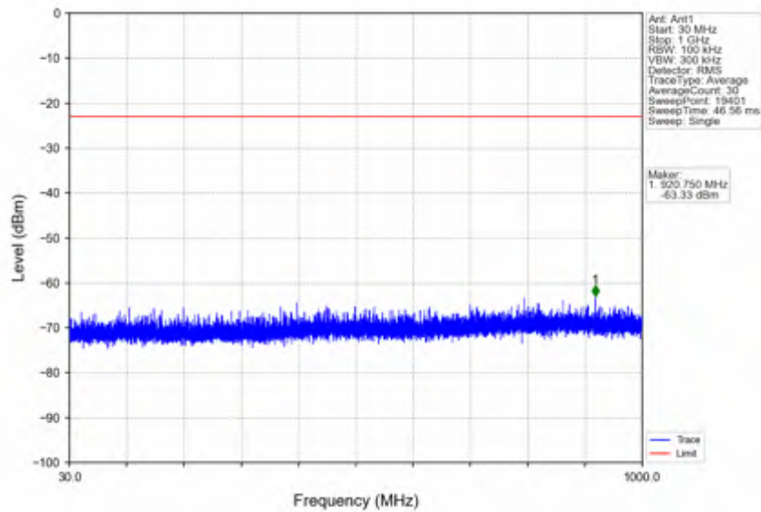
n25_15kHz_SISO_NTNV_10MHz_DFT-s-OFDM QPSK_185MHz_Inner_1RB_Left
