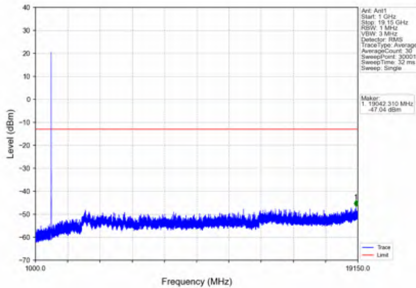
n25_15kHz_SISO_NTVV_10MHz_CP-OFDM QPSK_1882.5MHz_Edge_1RB_Left
