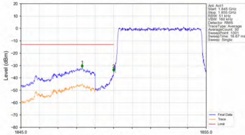
n25_15kHz_SISO_NTNV_5MHz_DFT-s-OFDM PI/2 BPSK_1852.5MHz_Outer_Full
