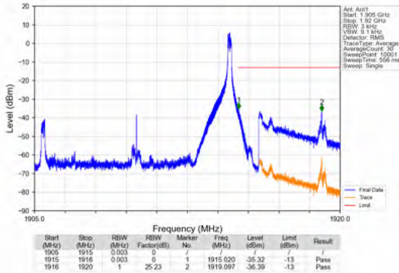
n25_15kHz_SISO_NTNV_10MHz_DFT-s-OFDM PI/2 BPSK_1910MHz_Edge_1RB_Right
