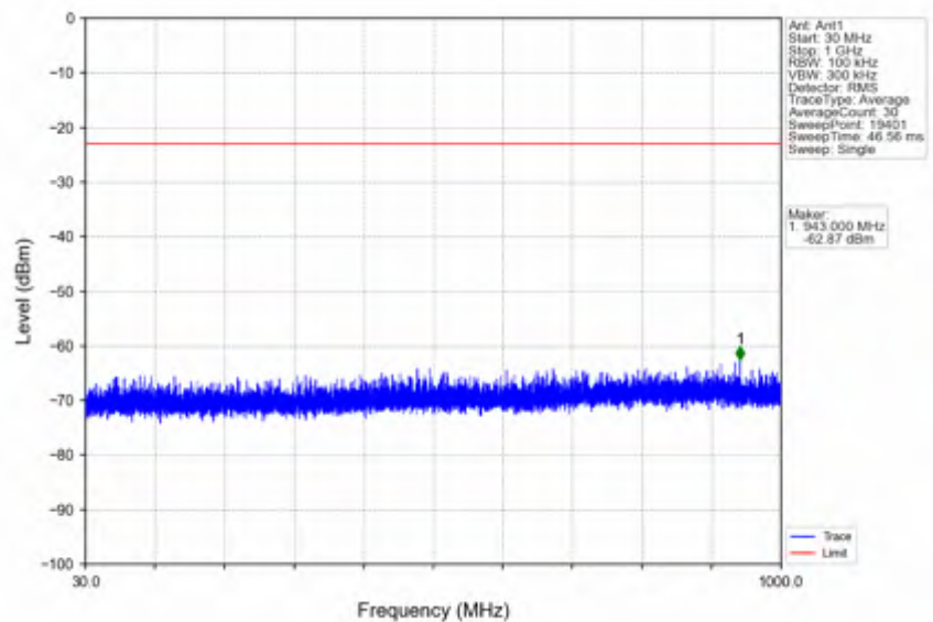
n7_30kHz_SISO_NTNV_50MHz_CP-OFDM QPSK_2535MHz_Edge_1RB_Left
