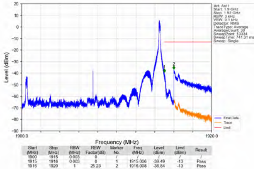
n25_15kHz_SISO_NTNV_15MHz_DFT-s-OFDM PI/2 BPSK_1907.5MHz_Edge_1RB_Right
