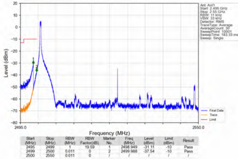
n7_30kHz_SISO_NTNV_50MHz_DFT-s-OFDM_PI/2_BPSK_2525MHz_Edge_1RB_Left
