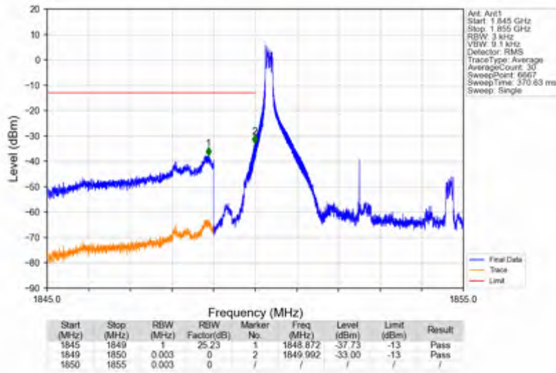
n25_15kHz_SISO_NTNV_5MHz_DFT-s-OFDM_PI/2_BPSK_1852.5MHz_Edge_1RB_Left
