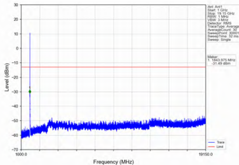
n25_15kHz_SISO_NTNV_15MHz_CP-OFDM QPSK_1857.5MHz_Outer_Full
