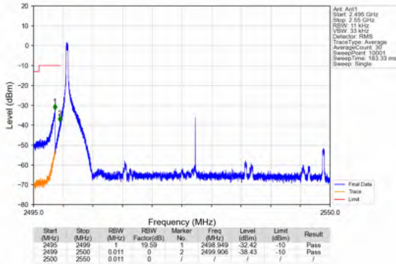
n7_30kHz_SISO_NTNV_50MHz_CP-OFDM_QPSK_2525MHz_Edge_1RB_Left
