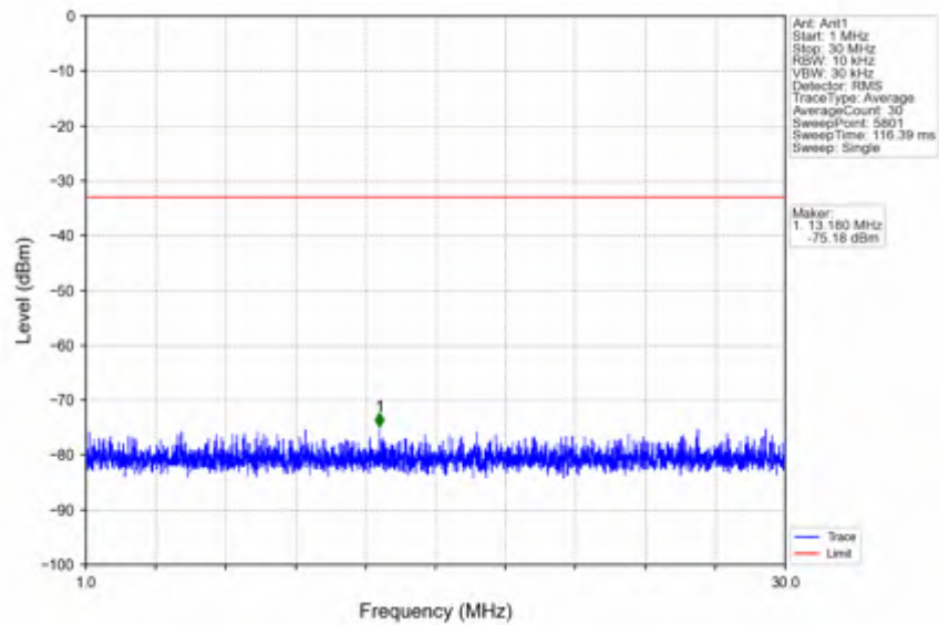
n25_15kHz_SISO_NTNV_5MHz_DFT-s-OFDM QPSK_1912.5MHz_Outer_Full
