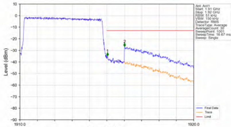
n25_15kHz_SISO_NTNV_5MHz_CP-OFDM QPSK_1912.5MHz_Outer_Full
