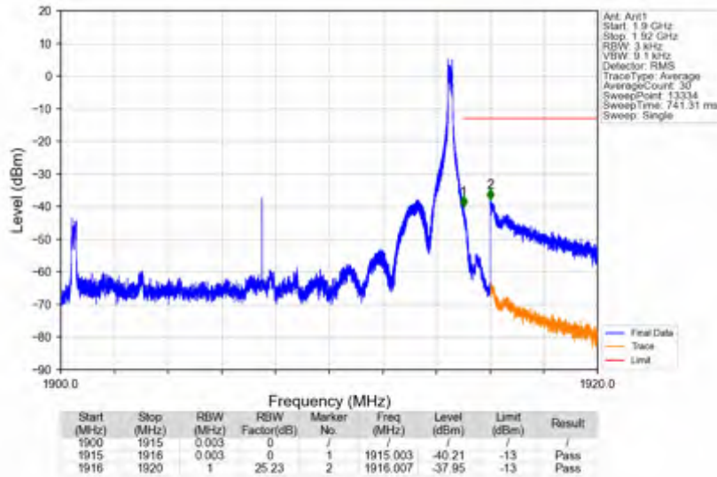
n25_15kHz_SISO_NTNV_15MHz_DFT-s-OFDM QPSK_1907.5MHz_Edge_1RB_Right
