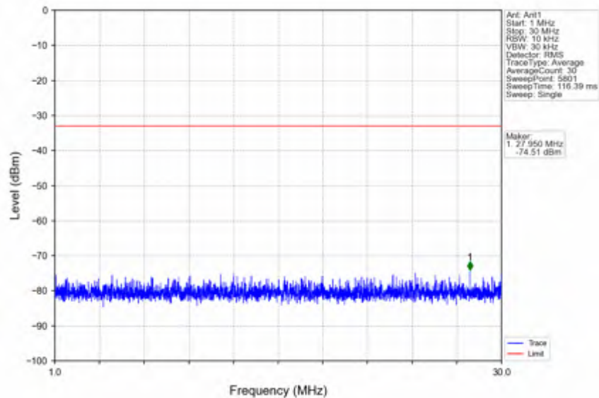
n25_15kHz_SISO_NTNV_5MHz_DFT-s-OFDM QPSK_1912.5MHz_Inner_1RB_Right
