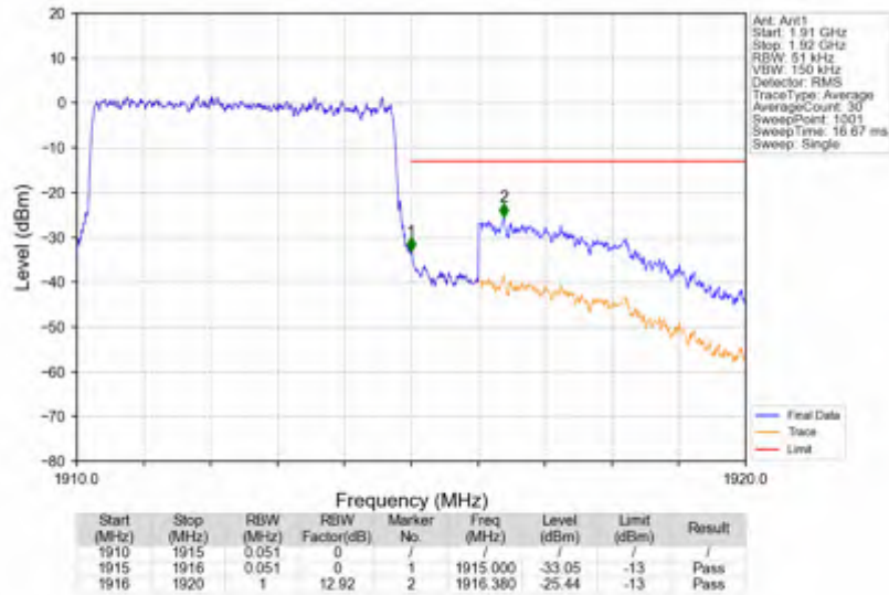
n25_15kHz_SISO_NTNV_5MHz_DFT-s-OFDM QPSK_1912.5MHz_Outer_Full
