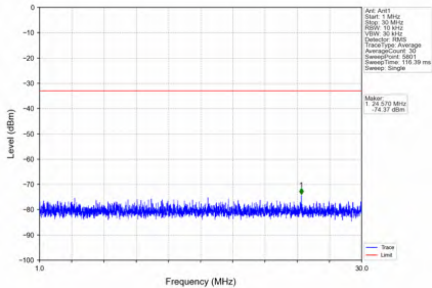
n25_15kHz_SISO_NTNV_5MHz_CP-OFDM QPSK_1852.5MHz_Inner_1RB_Left
