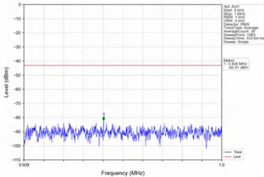
n7_30kHz_SISO_NTNV_20MHz_CP-OFDM QPSK_2535MHz_Edge_1RB_Left
