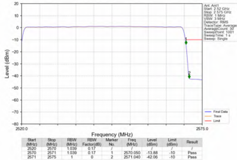
n7_15kHz_SISO_NTNV_50MHz_DFT-s-OFDM QPSK_2545MHz_Outer_Full
