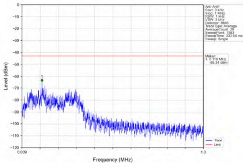
n7_30kHz_SISO_NTNV_25MHz_DFT-s-OFDM PI/2 BPSK_2512.5MHz_Edge_1RB_Left
