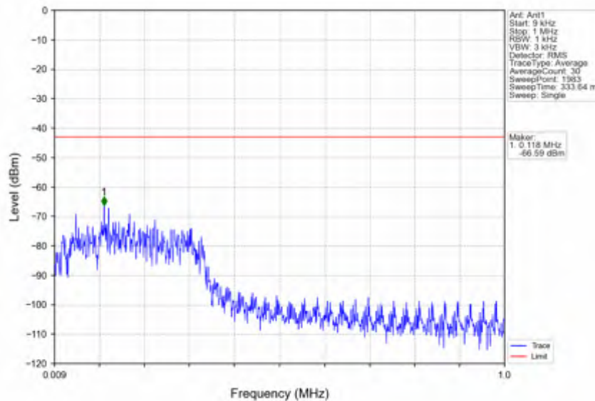
n7_30kHz_SISO_NTNV_40MHz_DFT-s-OFDM QPSK_2520MHz_Edge_1RB_Left
