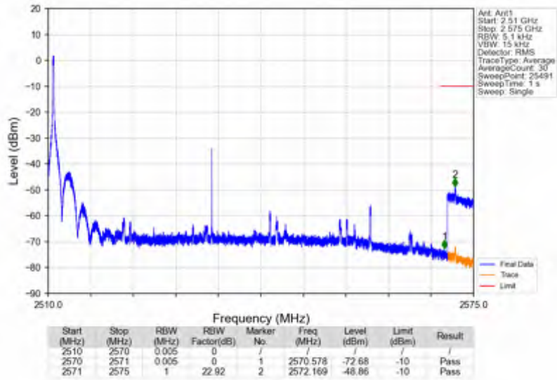
n7_15kHz_SISO_NTNV_50MHz_CP-OFDM QPSK_2535MHz_Edge_1RB_Left
