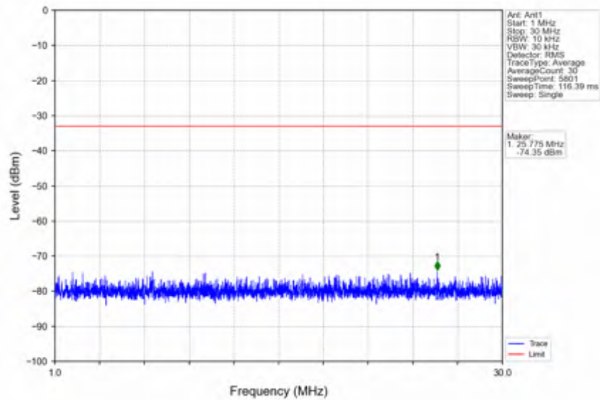
n7_30kHz_SISO_NTNV_30MHz_DFT-s-OFDM_QPSK_2535MHz_Edge_1RB_Left
