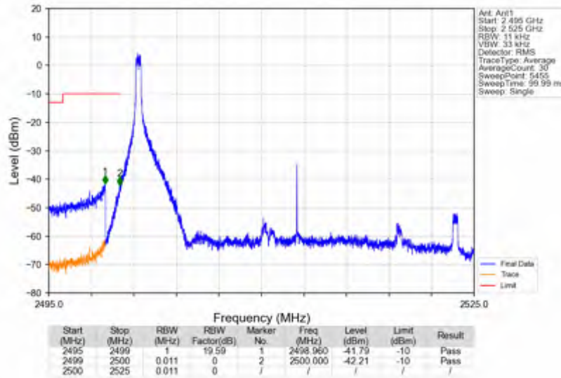
n7_30kHz_SISO_NTNV_25MHz_CP-OFDM QPSK_2512.5MHz_Inner_1RB_Left
