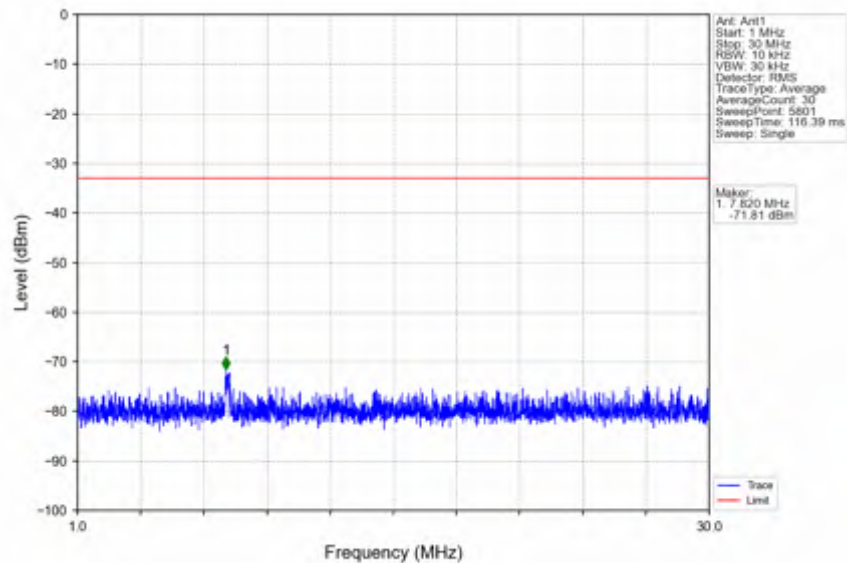
n7_30kHz_SISO_NTNV_15MHz_CP-OFDM QPSK_2562.5MHz_Edge_1RB_Right
