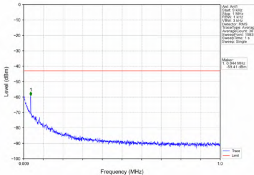
n7_15kHz_SISO_NTNV_50MHz_CP-OFDM_QPSK_2525MHz_Inner_1RB_Left
