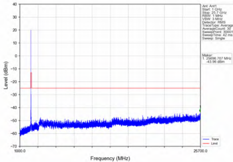
n7_30kHz_SISO_NTNV_25MHz_DFT-s-OFDM QPSK_2512.5MHz_Outer_Full
