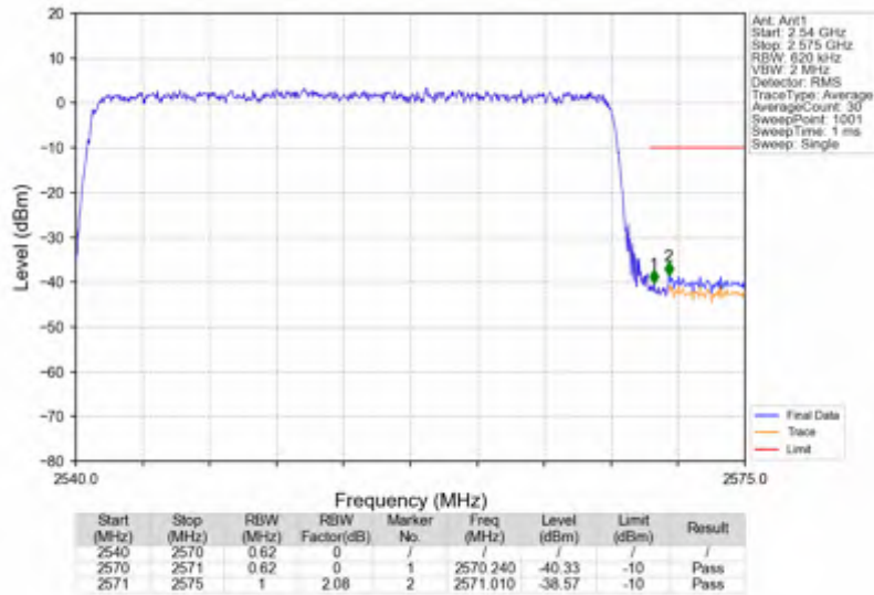
n7_30kHz_SISO_NTNV_30MHz_DFT-s-OFDM QPSK_2555MHz_Outer_Full
