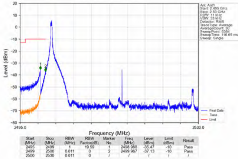
n7_30kHz_SISO_NTNV_30MHz_DFT-s-OFDM_PI/2_BPSK_2515MHz_Edge_1RB_Left
