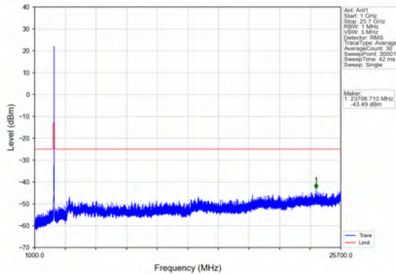
n7_30kHz_SISO_NTNV_30MHz_DFT-s-OFDM PI/2 BPSK_2555MHz_Edge_1RB_Right
