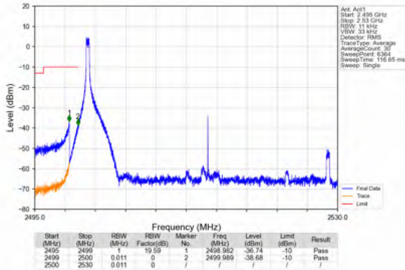
n7_30kHz_SISO_NTV_30MHz_DFT-s-OFDM QPSK_2515MHz_Edge_1RB_Left
