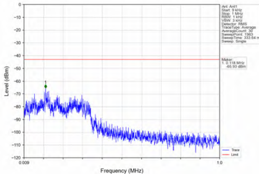
n7_30kHz_SISO_NTNV_25MHz_DFT-s-OFDM PI/2 BPSK_2535MHz_Edge_1RB_Left
