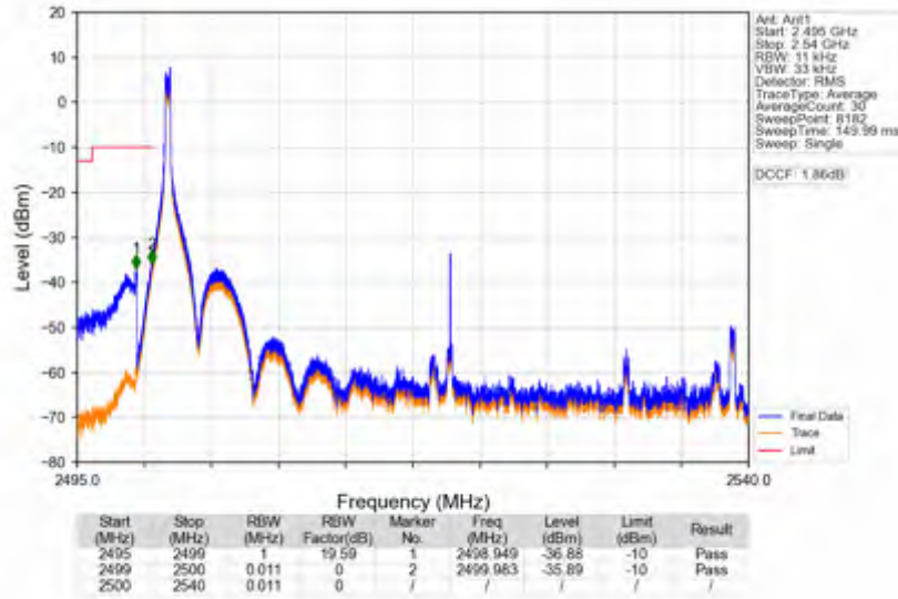
n7_30kHz_SISO_NTNV_40MHz_DFT-s-OFDM_PI/2_BPSK_2520MHz_Edge_1RB_Left
