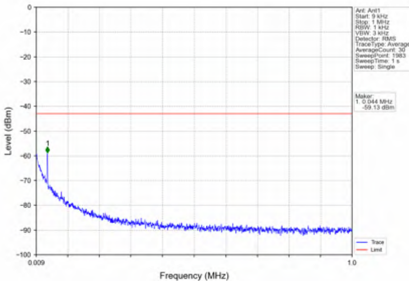
n7_15kHz_SISO_NTNV_50MHz_DFT-s-OFDM QPSK_2545MHz_Outer_Full
