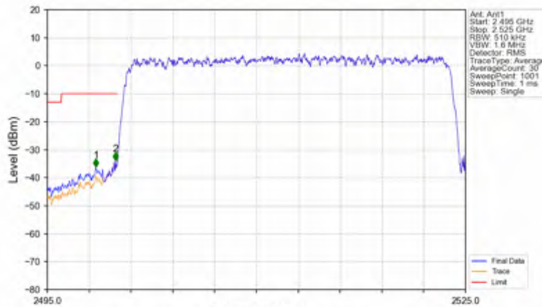
n7_30kHz_SISO_NTNV_25MHz_DFT-s-OFDM PI/2 BPSK_2512.5MHz_Outer_Full
