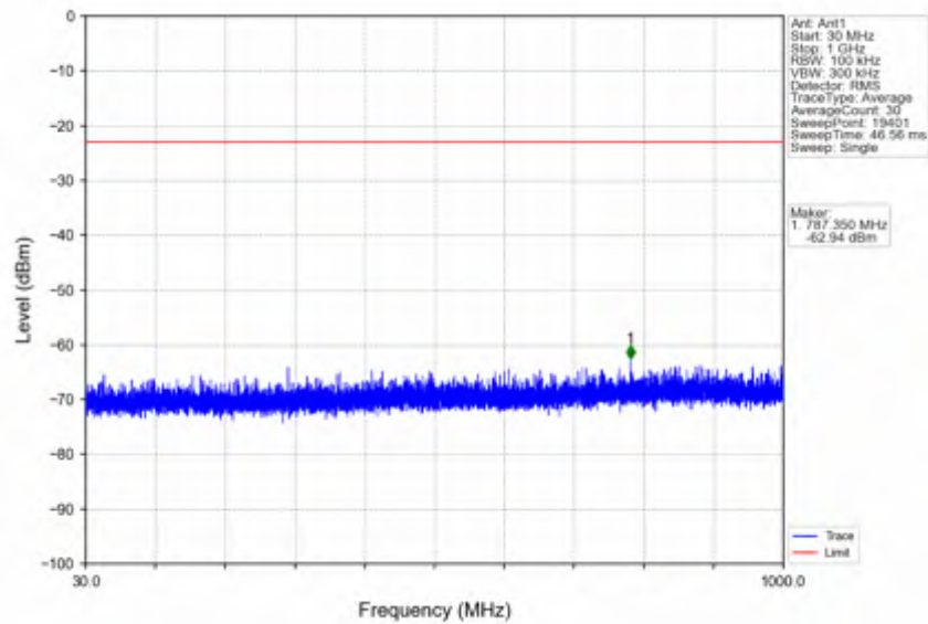
n7_30kHz_SISO_NTNV_25MHz_CP-OFDM QPSK_2557.5MHz_Edge_1RB_Right
