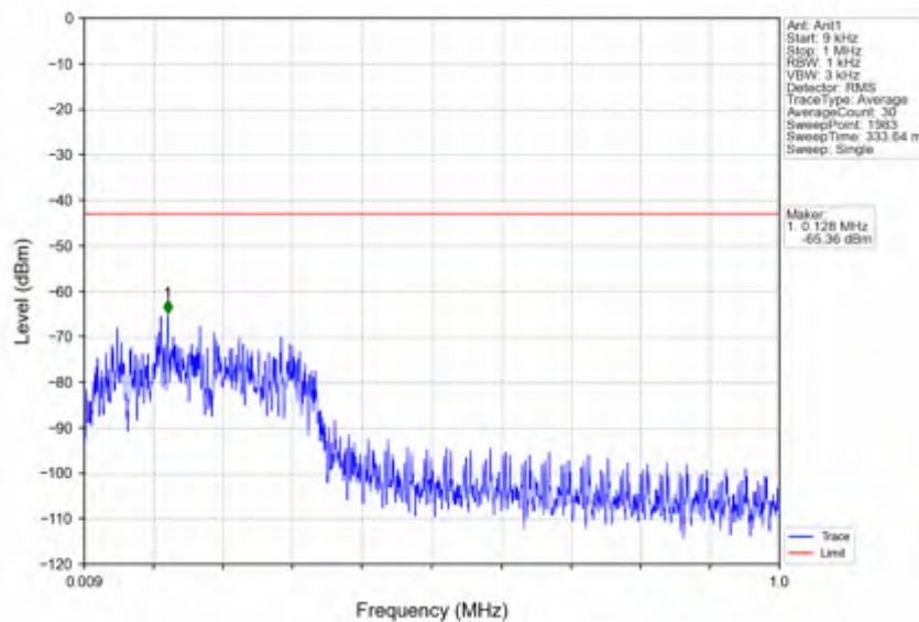
n7_30kHz_SISO_NTV_10MHz_DFT-s-OFDM QPSK_2535MHz_Edge_1RB_Left
