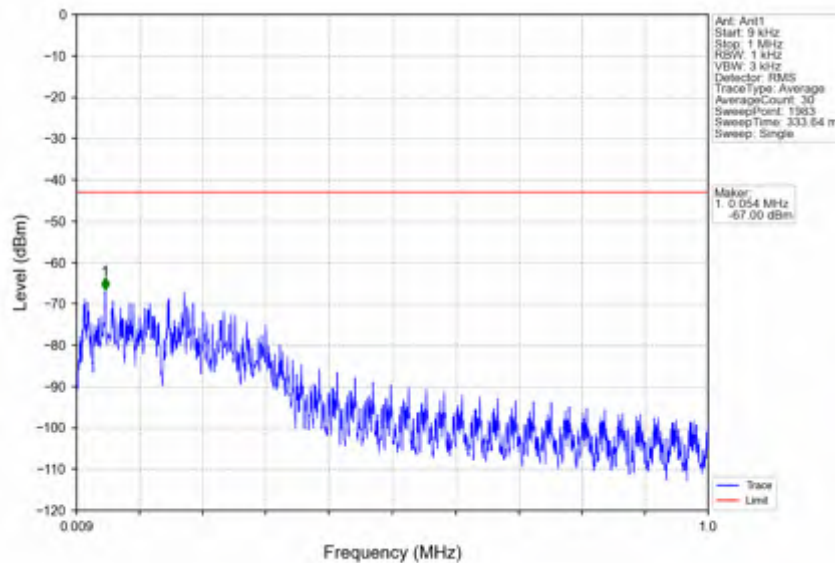
n7_30kHz_SISO_NTNV_40MHz_CP-OFDM_QPSK_2520MHz_Edge_1RB_Left
