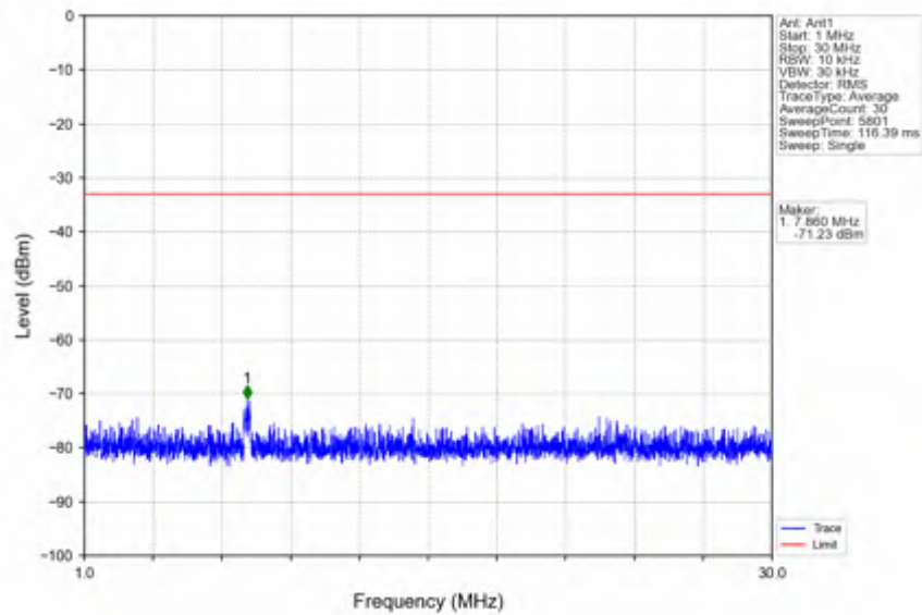
n7_30kHz_SISO_NTNV_10MHz_CP-OFDM QPSK_2565MHz_Edge_1RB_Right
