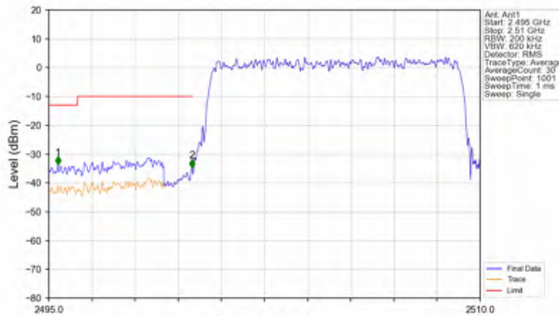
n7_30kHz_SISO_NTNV_10MHz_DFT-s-OFDM QPSK_2505MHz_Outer_Full
