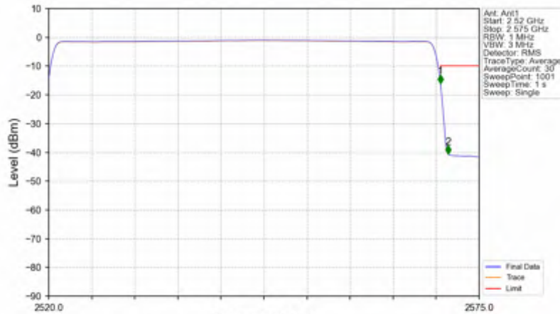
n7_15kHz_SISO_NTNV_50MHz_CP-OFDM QPSK_2545MHz_Outer_Full
