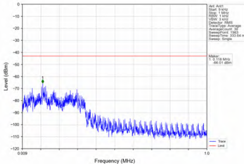
n7_30kHz_SISO_NTNV_30MHz_DFT-s-OFDM PI/2 BPSK_2535MHz_Edge_1RB_Left
