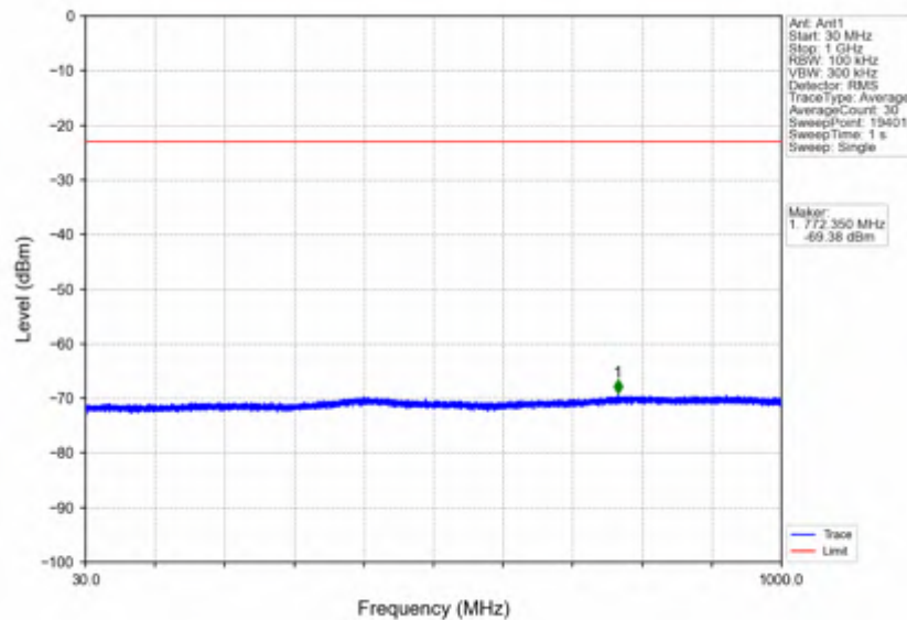
n7_15kHz_SISO_NTNV_50MHz_CP-OFDM QPSK_2545MHz_Inner_1RB_Right
