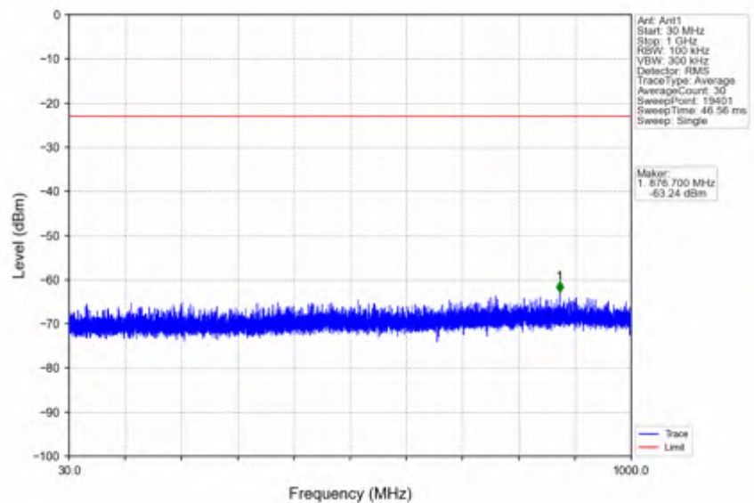
n7_30kHz_SISO_NTNV_40MHz_DFT-s-OFDM QPSK_2520MHz_Edge_1RB_Left
