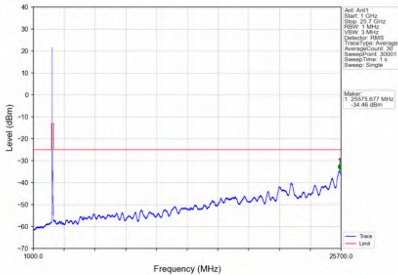
n7_15kHz_SISO_NTNV_50MHz_CP-OFDM QPSK_2535MHz_Edge_1RB_Left
