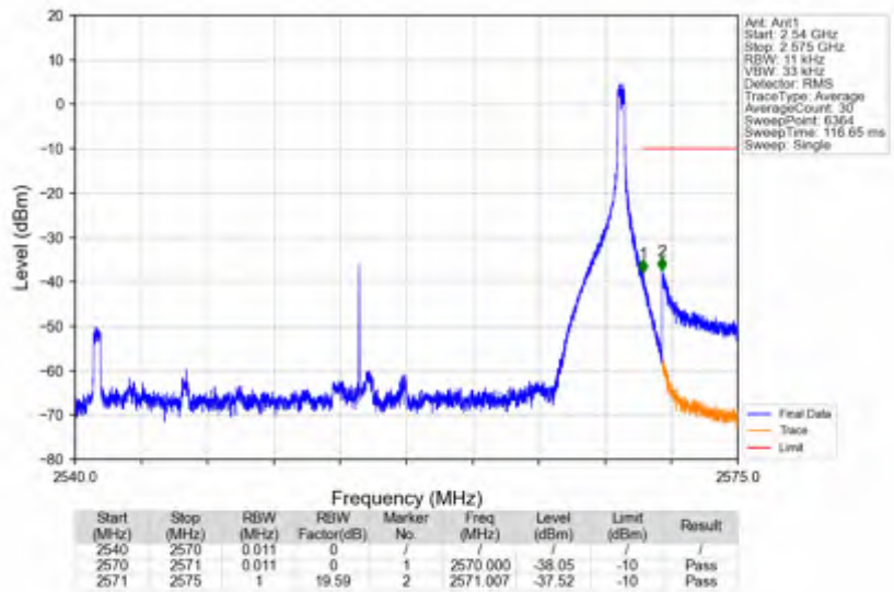
n7_30kHz_SISO_NTNV_30MHz_DFT-s-OFDM QPSK_2555MHz_Edge_1RB_Right
