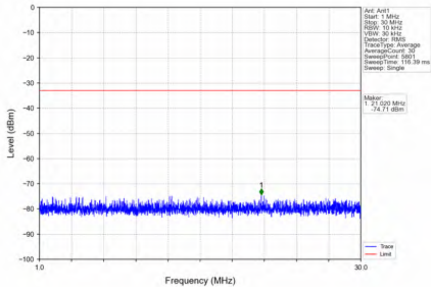
n7_30kHz_SISO_NTNV_30MHz_DFT-s-OFDM QPSK_2515MHz_Edge_1RB_Left
