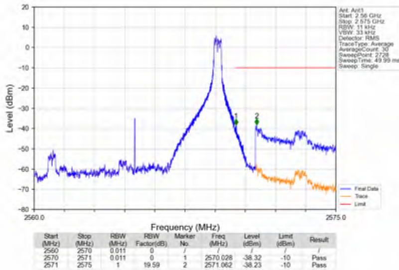
n7_30kHz_SISO_NTNV_10MHz_DFT-s-OFDM QPSK_2565MHz_Edge_1RB_Right
