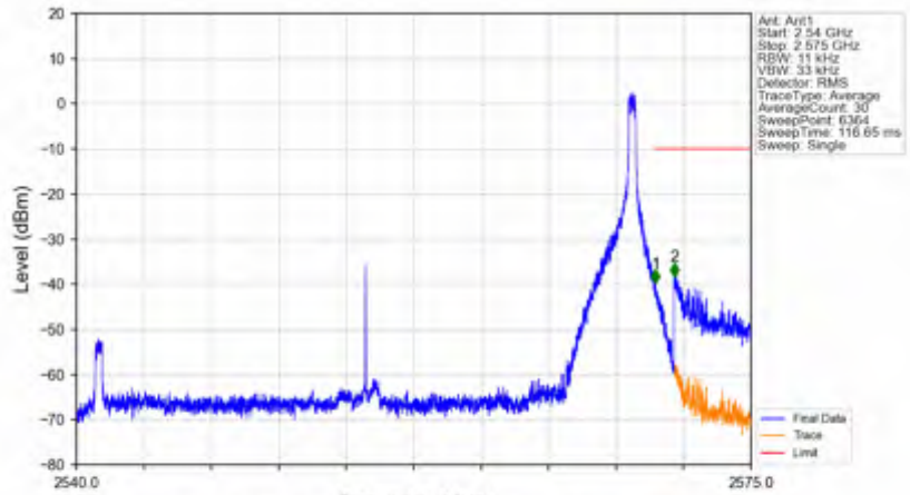
n7_30kHz_SISO_NTNV_30MHz_CP-OFDM QPSK_2555MHz_Edge_1RB_Right
