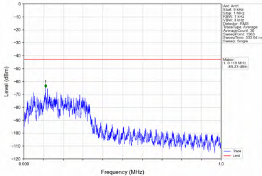
n7_30kHz_SISO_NTNV_10MHz_DFT-s-OFDM_QPSK_2565MHz_Edge_1RB_Right
