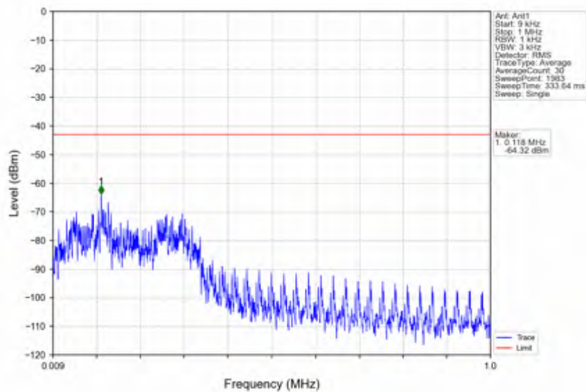
n7_30kHz_SISO_NTNV_10MHz_DFT-s-OFDM_PI/2_BPSK_2505MHz_Edge_1RB_Left
