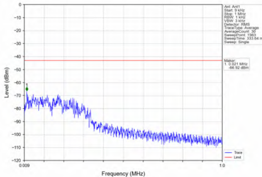
n7_30kHz_SISO_NTNV_25MHz_CP-OFDM QPSK_2535MHz_Edge_1RB_Left
