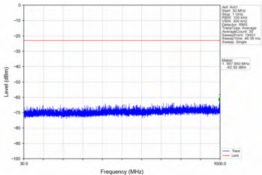
n7_30kHz_SISO_NTV_10MHz_DFT-s-OFDM QPSK_2505MHz_Edge_1RB_Left
