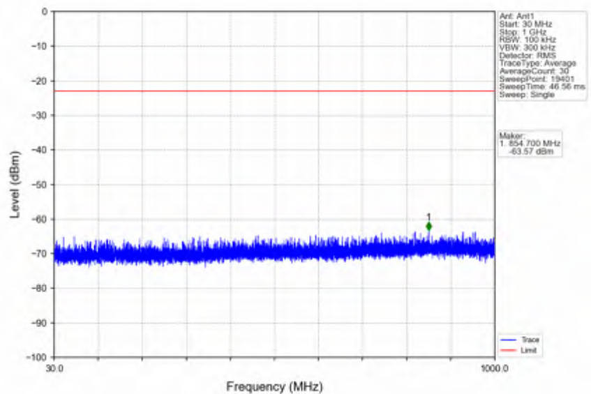
n7_30kHz_SISO_NTNV_10MHz_CP-OFDM QPSK_2535MHz_Edge_1RB_Left
