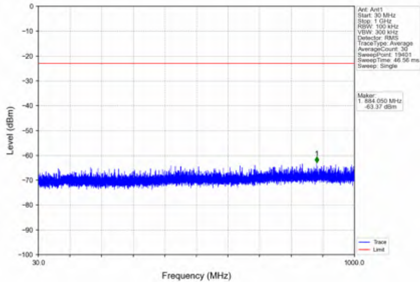
n7_30kHz_SISO_NTV_25MHz_DFT-s-OFDM QPSK_2557.5MHz_Edge_1RB_Right
