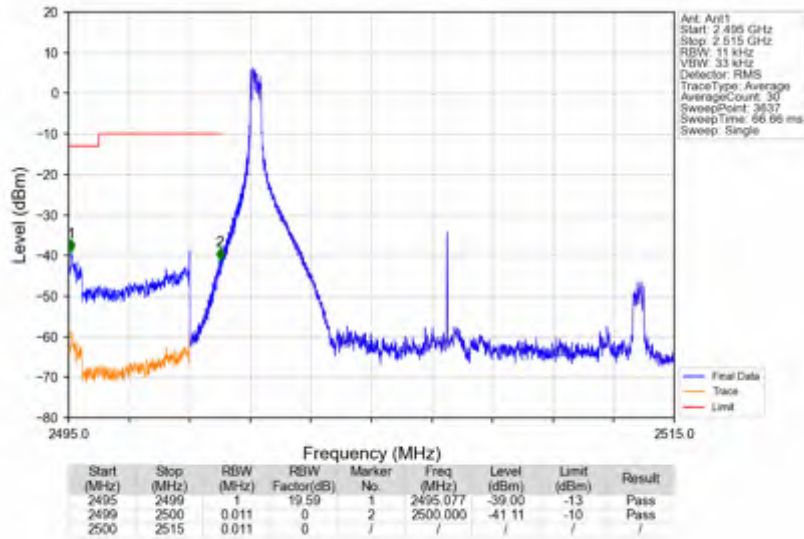
n7_30kHz_SISO_NTNV_15MHz_DFT-s-OFDM PI/2 BPSK_2507.5MHz_Inner_1RB_Left
