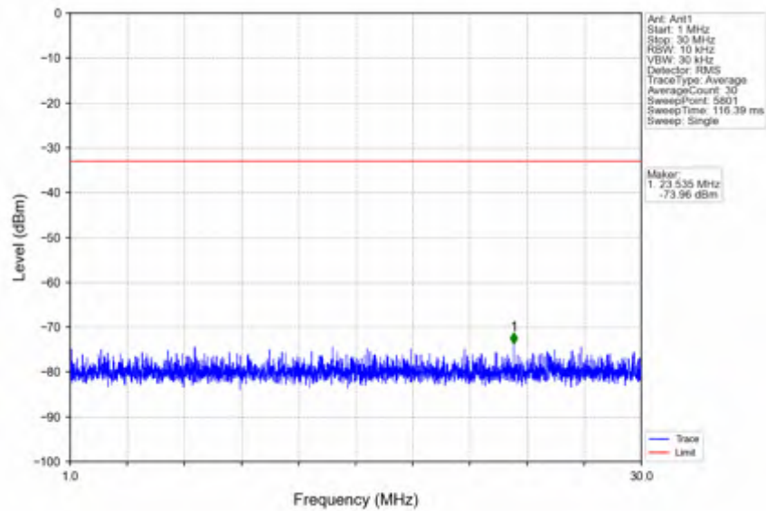
n7_30kHz_SISO_NTV_25MHz_DFT-s-OFDM QPSK_2535MHz_Edge_1RB_Left
