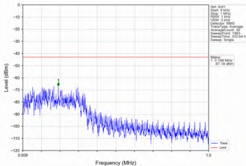
n7_30kHz_SISO_NTNV_40MHz_DFT-s-OFDM QPSK_2535MHz_Edge_1RB_Left
