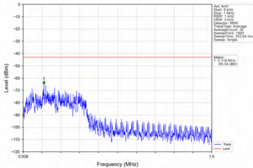
n7_30kHz_SISO_NTV_15MHz_DFT-s-OFDM_QPSK_2562.5MHz_Edge_1RB_Right
