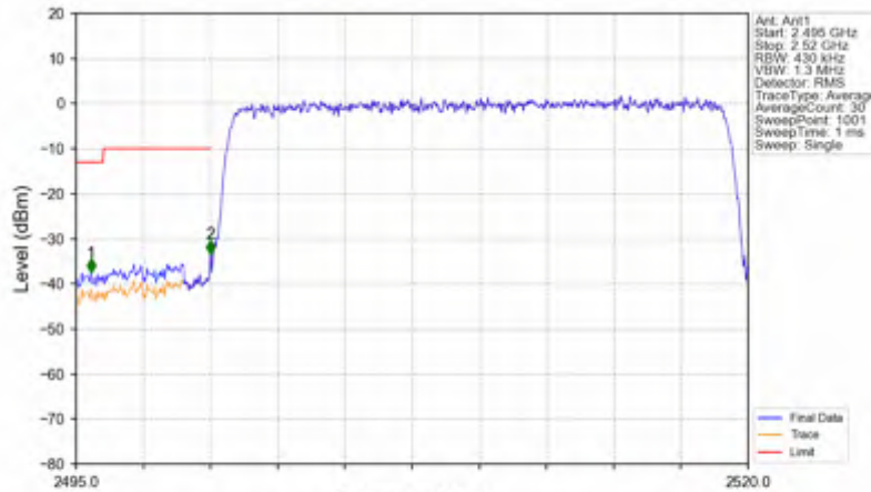
n7_30kHz_SISO_NTNV_20MHz_CP-OFDM QPSK_2510MHz_Outer_Full
