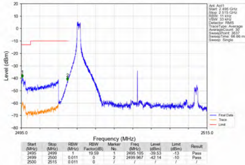
n7_30kHz_SISO_NTNV_15MHz_DFT-s-OFDM QPSK_2507.5MHz_Inner_1RB_Left
