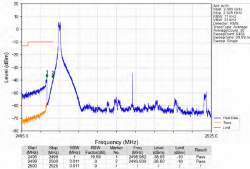
n7_30kHz_SISO_NTNV_25MHz_DFT-s-OFDM QPSK_2512.5MHz_Edge_1RB_Left
