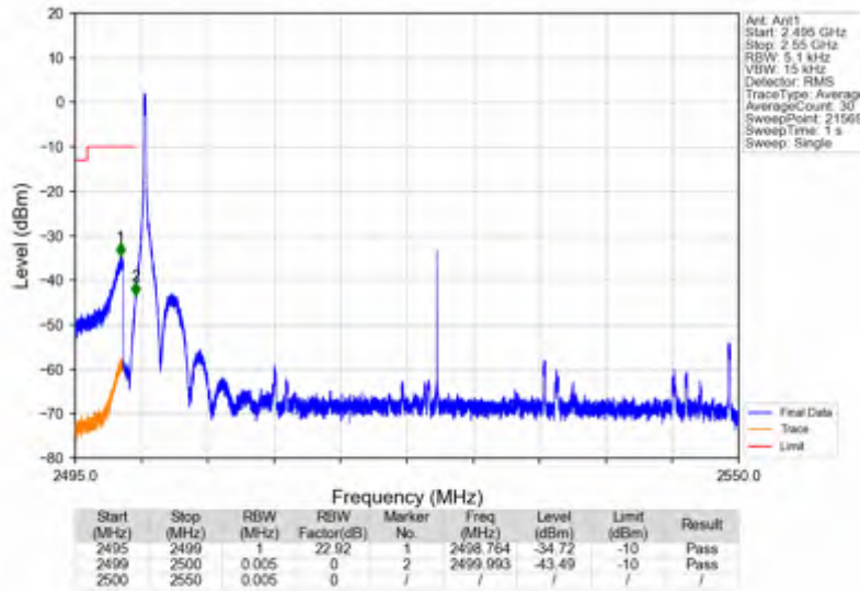
n7_15kHz_SISO_NTNV_50MHz_CP-OFDM_QPSK_2525MHz_Edge_1RB_Left
