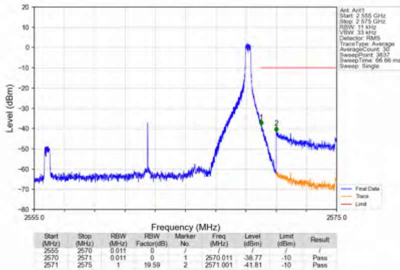
n7_30kHz_SISO_NTNV_15MHz_CP-OFDM QPSK_2562.5MHz_Edge_1RB_Right
