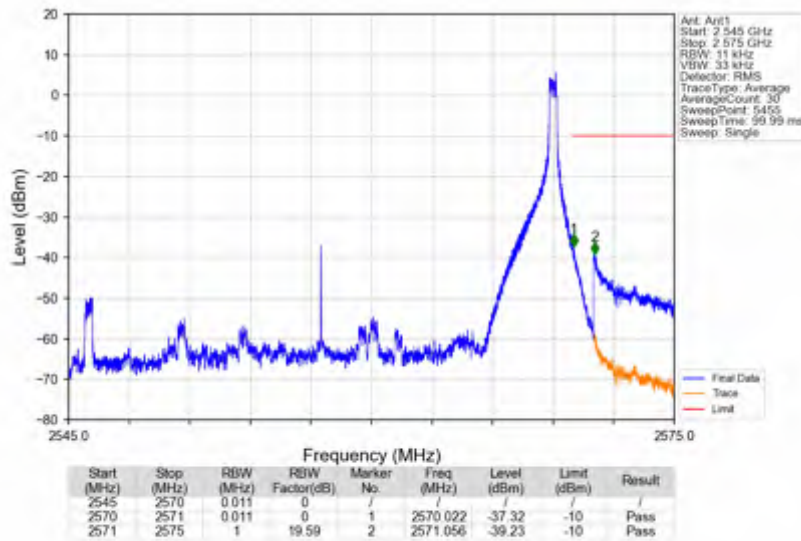
n7_30kHz_SISO_NTNV_25MHz_DFT-s-OFDM QPSK_2557.5MHz_Edge_1RB_Right
