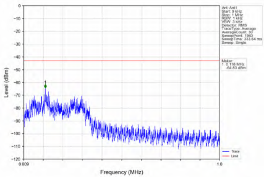
n7_30kHz_SISO_NTNV_15MHz_DFT-s-OFDM PI/2 BPSK_2507.5MHz_Edge_1RB_Left
