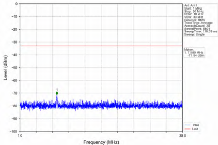
n7_30kHz_SISO_NTNV_30MHz_CP-OFDM QPSK_2555MHz_Edge_1RB_Right
