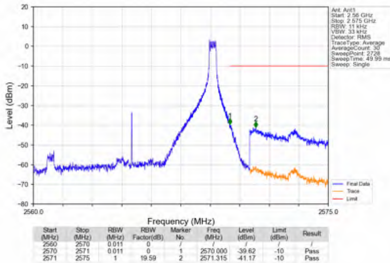
n7_30kHz_SISO_NTNV_10MHz_CP-OFDM QPSK_2565MHz_Edge_1RB_Right
