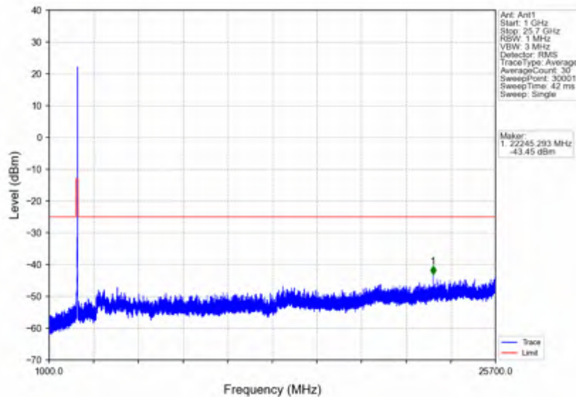
n7_30kHz_SISO_NTV_25MHz_DFT-s-OFDM QPSK_2557.5MHz_Edge_1RB_Right
