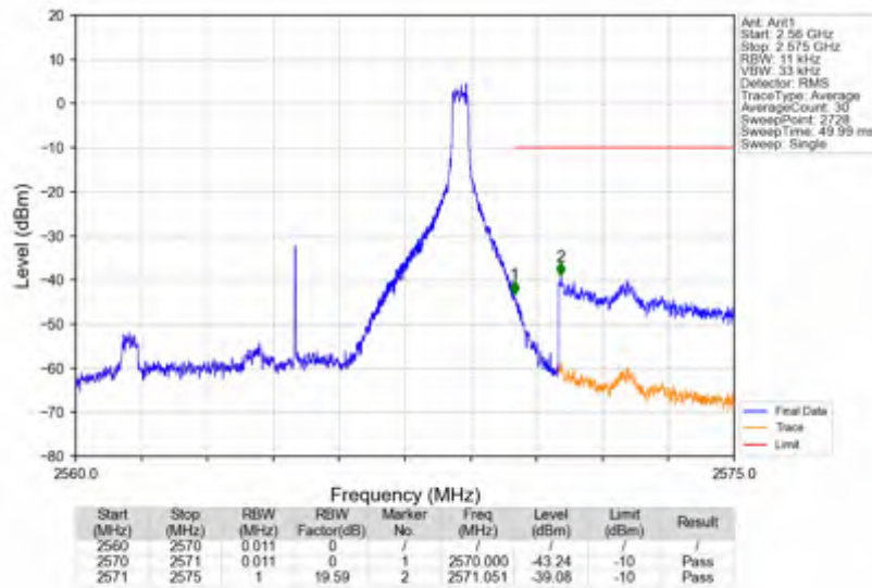
n7_30kHz_SISO_NTNV_10MHz_CP-OFDM QPSK_2565MHz_Inner_1RB_Right
