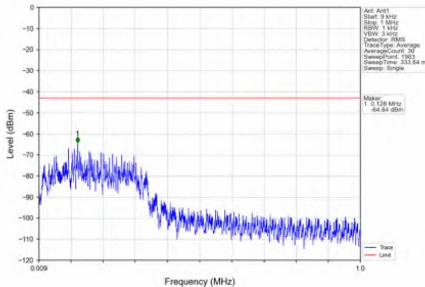
n7_30kHz_SISO_NTNV_20MHz_DFT-s-OFDM QPSK_2535MHz_Edge_1RB_Left
