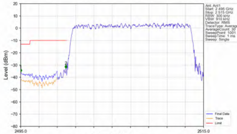
n7_30kHz_SISO_NTNV_15MHz_DFT-s-OFDM PI/2 BPSK_2507.5MHz_Outer_Full
