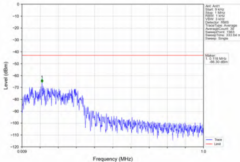
n7_30kHz_SISO_NTNV_25MHz_DFT-s-OFDM QPSK_2535MHz_Edge_1RB_Left
