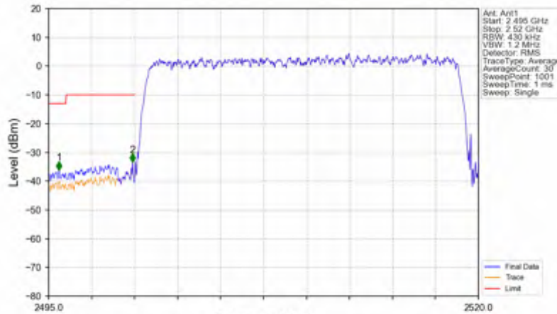
n7_30kHz_SISO_NTNV_20MHz_DFT-s-OFDM QPSK_2510MHz_Outer_Full
