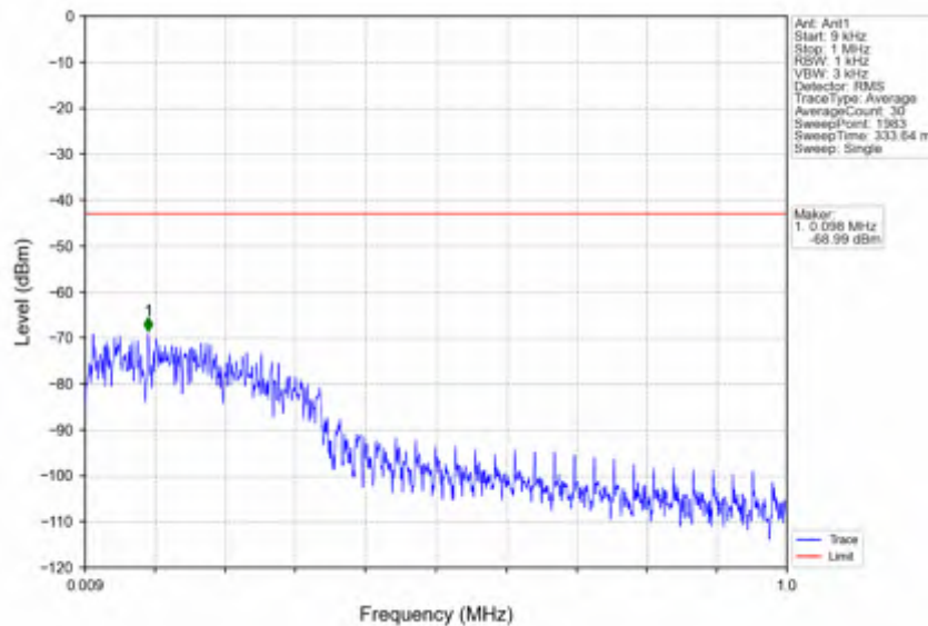
n7_30kHz_SISO_NTNV_10MHz_CP-OFDM QPSK_2535MHz_Edge_1RB_Left
