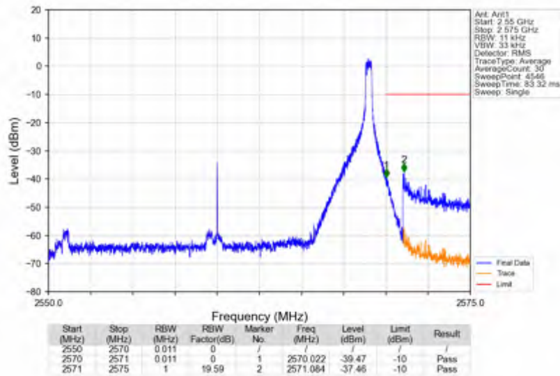
n7_30kHz_SISO_NTNV_20MHz_CP-OFDM QPSK_2560MHz_Edge_1RB_Right
