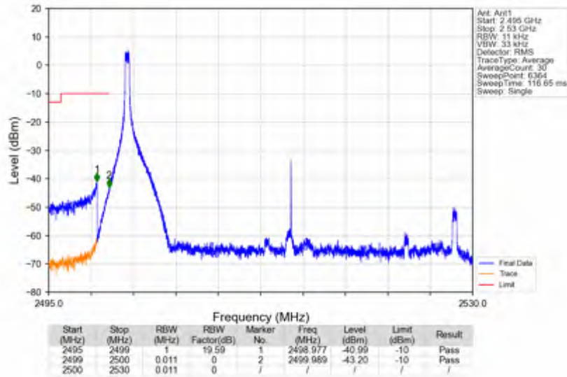
n7_30kHz_SISO_NTNV_30MHz_DFT-s-OFDM QPSK_2515MHz_Inner_1RB_Left
