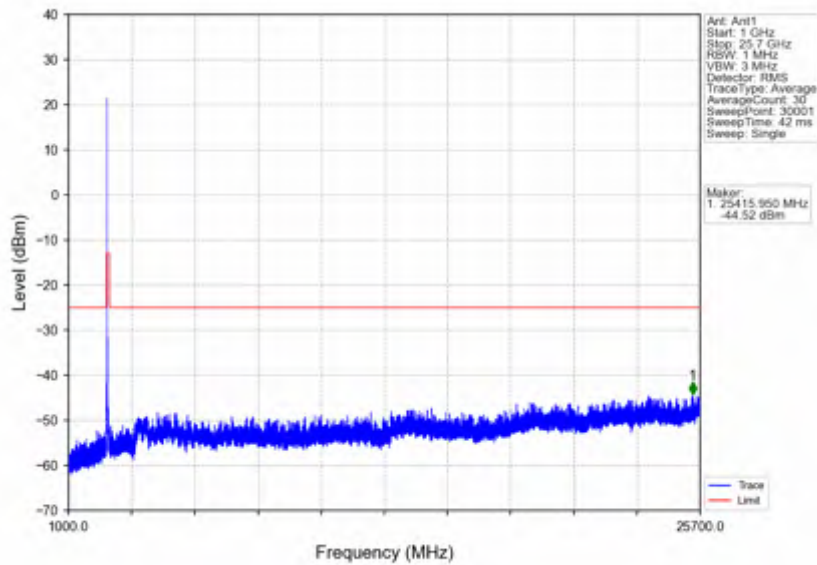
n7_30kHz_SISO_NTNV_25MHz_DFT-s-OFDM PI/2 BPSK_2512.5MHz_Outer_Full
