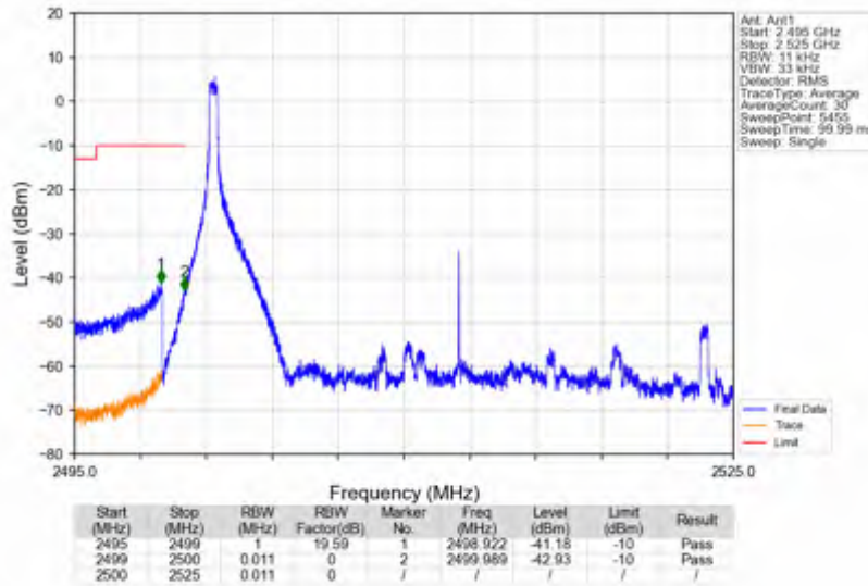
n7_30kHz_SISO_NTNV_25MHz_DFT-s-OFDM QPSK_2512.5MHz_Inner_1RB_Left
