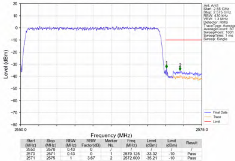
n7_30kHz_SISO_NTNV_20MHz_CP-OFDM QPSK_2560MHz_Outer_Full
