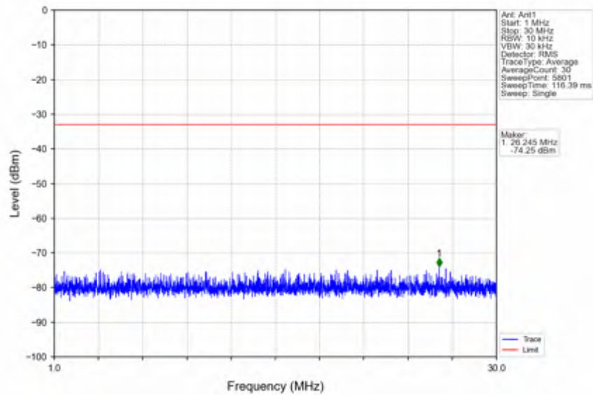
n7_30kHz_SISO_NTNV_40MHz_CP-OFDM QPSK_2520MHz_Edge_1RB_Left
