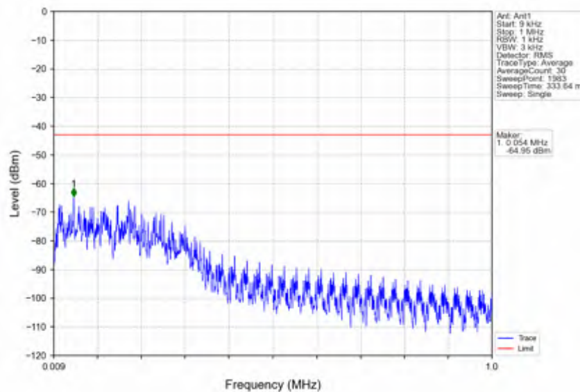
n7_30kHz_SISO_NTNV_15MHz_CP-OFDM QPSK_2535MHz_Edge_1RB_Left
