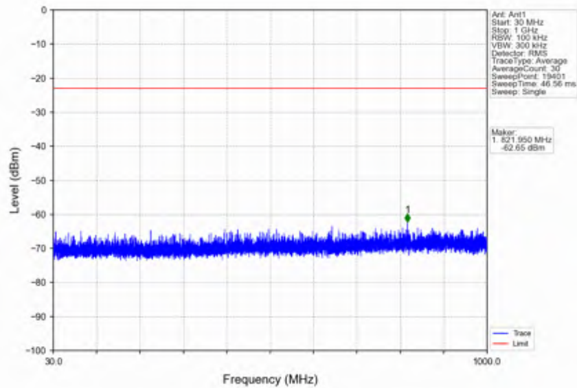
n7_30kHz_SISO_NTNV_30MHz_DFT-s-OFDM QPSK_2555MHz_Edge_1RB_Right
