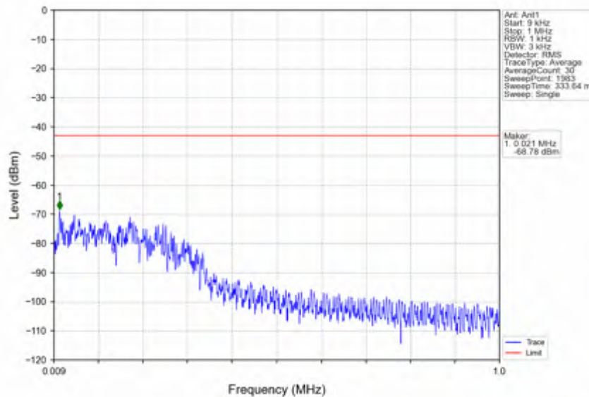
n7_30kHz_SISO_NTNV_30MHz_CP-OFDM_QPSK_2515MHz_Edge_1RB_Left
