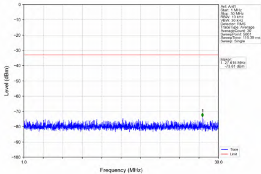
n7_30kHz_SISO_NTNV_20MHz_CP-OFDM QPSK_2535MHz_Edge_1RB_Left
