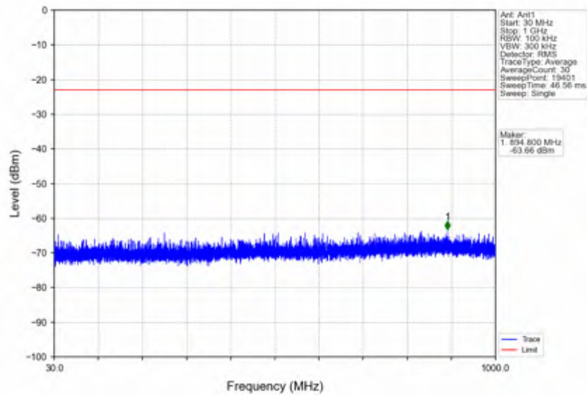
n7_30kHz_SISO_NTNV_20MHz_CP-OFDM QPSK_2560MHz_Edge_1RB_Right
