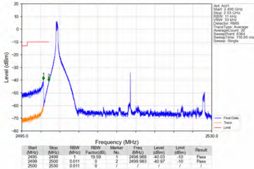
n7_30kHz_SISO_NTNV_30MHz_DFT-s-OFDM PI/2 BPSK_2515MHz_Inner_1RB_Left
