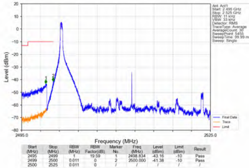
n7_30kHz_SISO_NTNV_25MHz_DFT-s-OFDM PI/2 BPSK_2512.5MHz_Inner_1RB_Left
