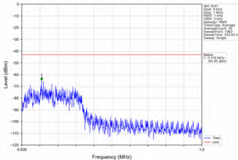
n7_30kHz_SISO_NTNV_15MHz_DFT-s-OFDM QPSK_2507.5MHz_Edge_1RB_Left
