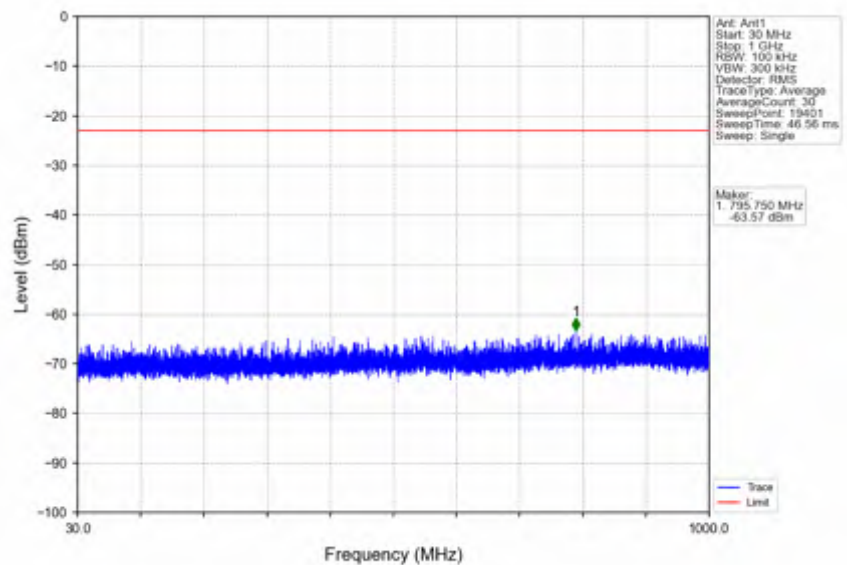
n7_30kHz_SISO_NTNV_30MHz_CP-OFDM QPSK_2535MHz_Edge_1RB_Left
