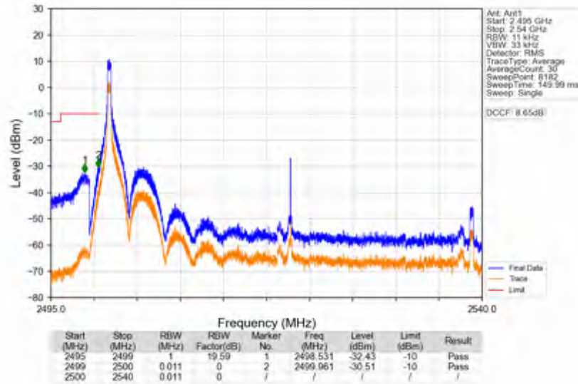
n7_30kHz_SISO_NTNV_40MHz_CP-OFDM_QPSK_2520MHz_Edge_1RB_Left
