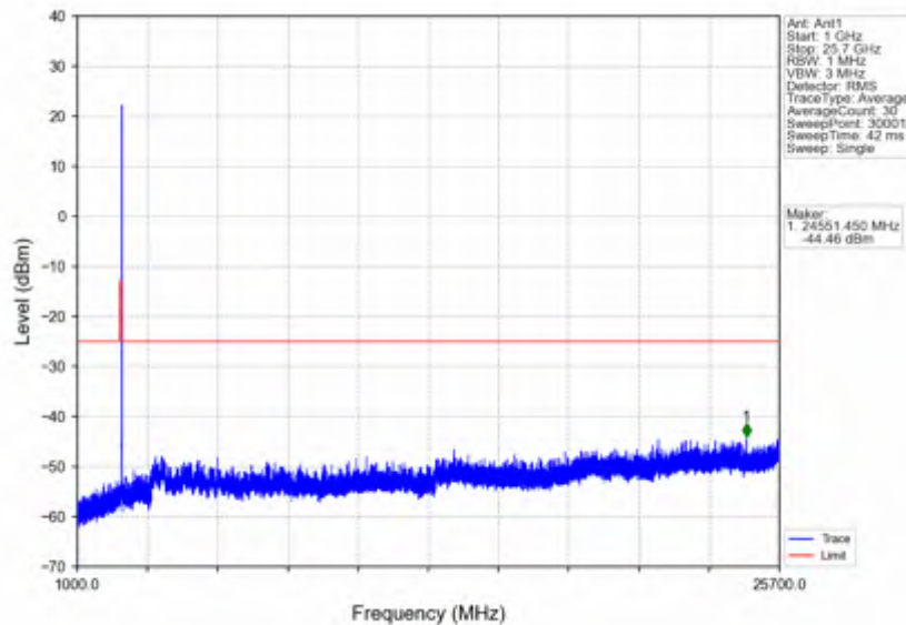
n7_30kHz_SISO_NTNV_15MHz_DFT-s-OFDM PI/2 BPSK_2562.5MHz_Edge_1RB_Right
