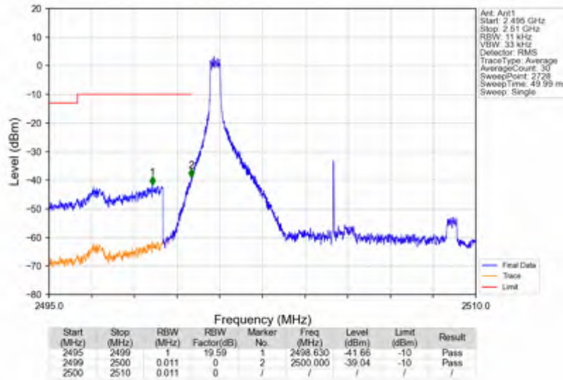
n7_30kHz_SISO_NTNV_10MHz_CP-OFDM QPSK_2505MHz_Edge_1RB_Left
