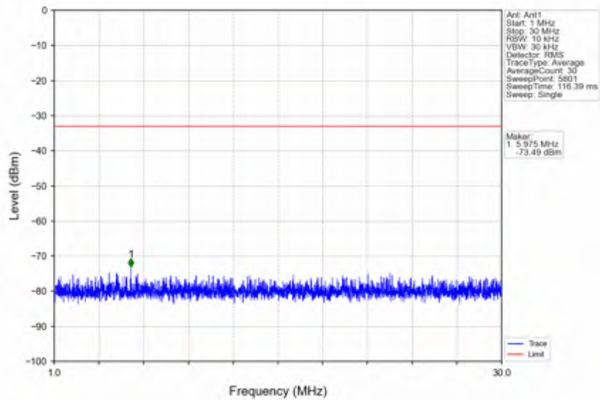
n7_30kHz_SISO_NTV_15MHz_DFT-s-OFDM QPSK_2535MHz_Edge_1RB_Left
