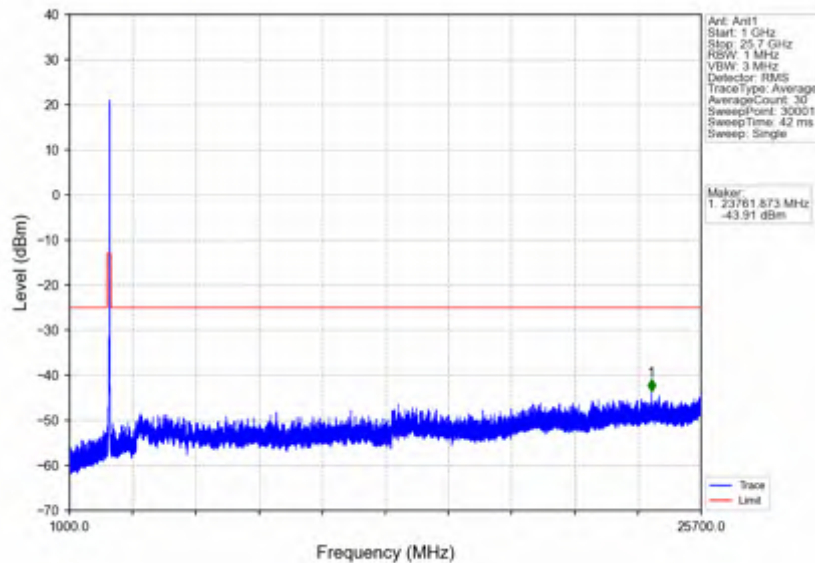
n7_30kHz_SISO_NTNV_40MHz_DFT-s-OFDM PI/2 BPSK_2550MHz_Inner_1RB_Right
