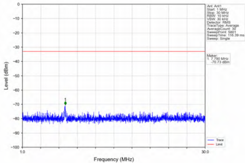
n7_30kHz_SISO_NTV_25MHz_CP-OFDM QPSK_2557.5MHz_Edge_1RB_Right
