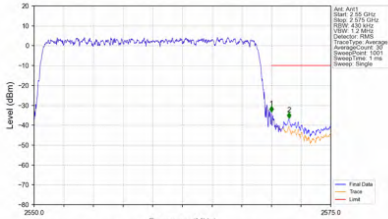
n7_30kHz_SISO_NTNV_20MHz_DFT-s-OFDM PI/2 BPSK_2560MHz_Outer_Full
