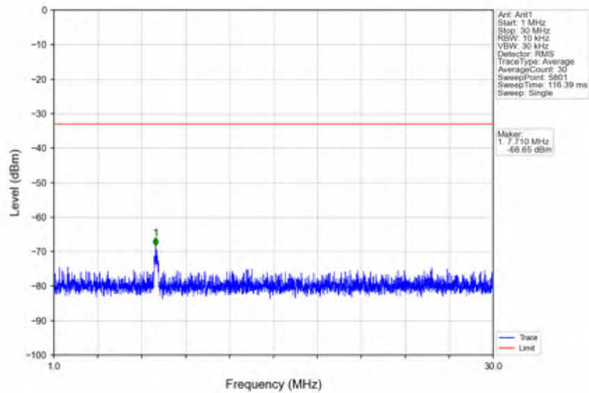
n7_30kHz_SISO_NTV_25MHz_DFT-s-OFDM QPSK_2557.5MHz_Edge_1RB_Right
