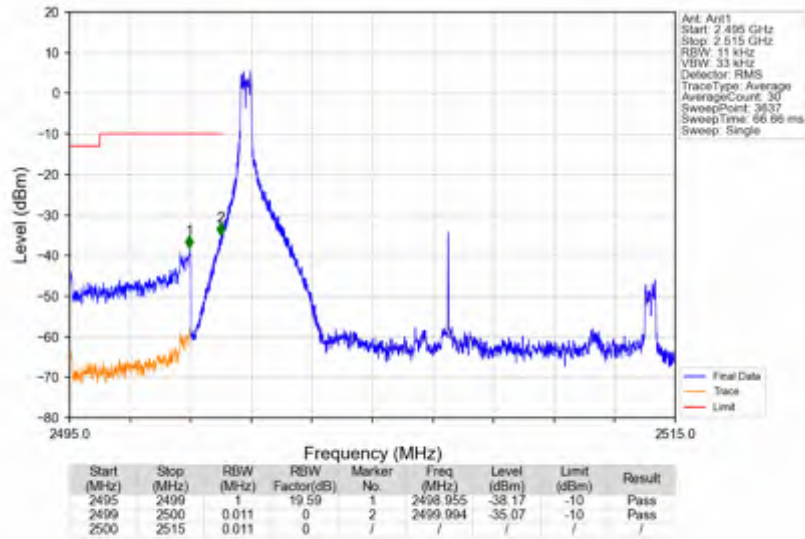
n7_30kHz_SISO_NTNV_15MHz_DFT-s-OFDM QPSK_2507.5MHz_Edge_1RB_Left
