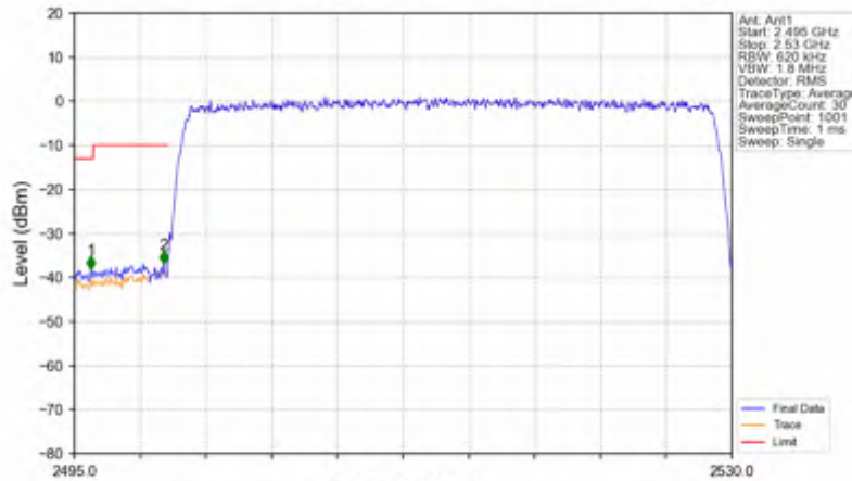
n7_30kHz_SISO_NTNV_30MHz_CP-OFDM QPSK_2515MHz_Outer_Full
