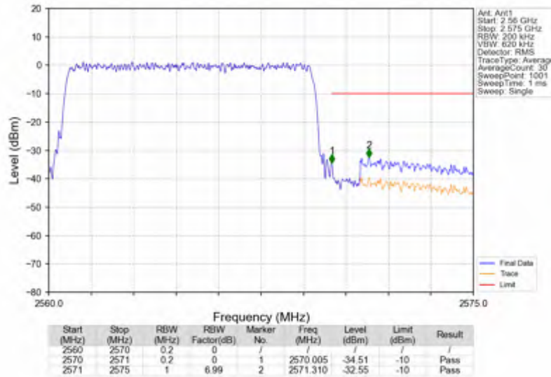
n7_30kHz_SISO_NTNV_10MHz_CP-OFDM QPSK_2565MHz_Outer_Full
