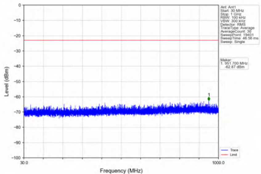
n7_30kHz_SISO_NTNV_15MHz_CP-OFDM QPSK_2535MHz_Edge_1RB_Left
