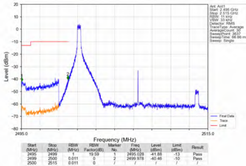
n7_30kHz_SISO_NTNV_15MHz_CP-OFDM QPSK_2507.5MHz_Inner_1RB_Left
