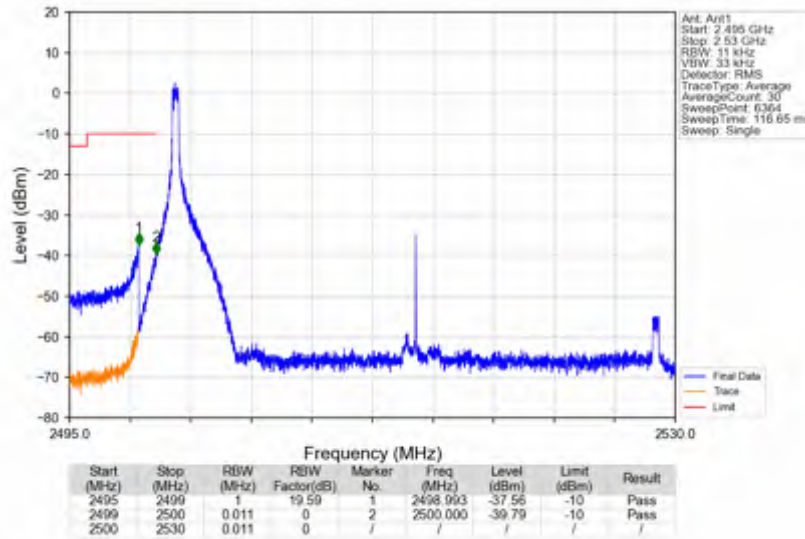
n7_30kHz_SISO_NTNV_30MHz_CP-OFDM_QPSK_2515MHz_Edge_1RB_Left
