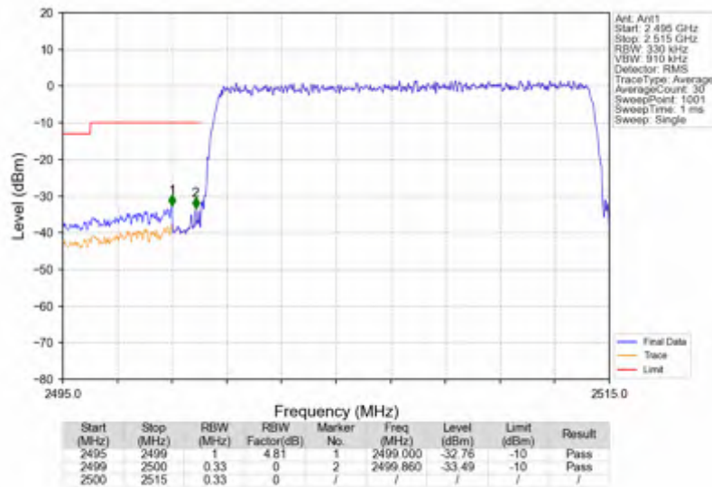
n7_30kHz_SISO_NTNV_15MHz_CP-OFDM QPSK_2507.5MHz_Outer_Full
