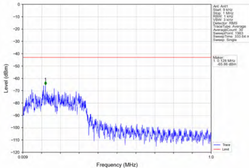
n7_30kHz_SISO_NTNV_25MHz_DFT-s-OFDM QPSK_2512.5MHz_Edge_1RB_Left
