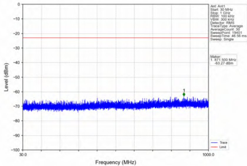
n7_30kHz_SISO_NTNV_15MHz_DFT-s-OFDM PI/2 BPSK_2562.5MHz_Edge_1RB_Right
