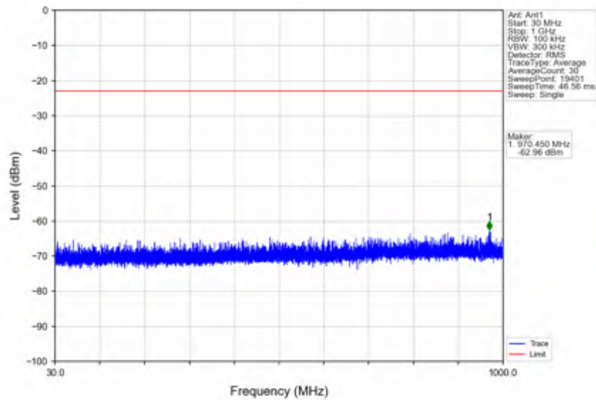
n7_30kHz_SISO_NTV_15MHz_DFT-s-OFDM QPSK_2562.5MHz_Edge_1RB_Right
