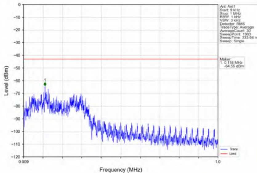
n7_30kHz_SISO_NTNV_15MHz_DFT-s-OFDM PI/2 BPSK_2535MHz_Edge_1RB_Left
