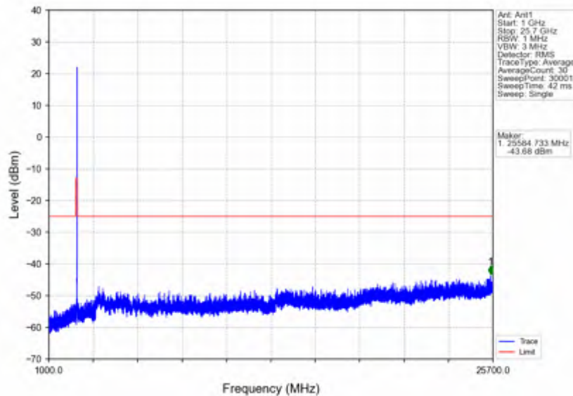
n7_30kHz_SISO_NTV_15MHz_DFT-s-OFDM QPSK_2562.5MHz_Edge_1RB_Right
