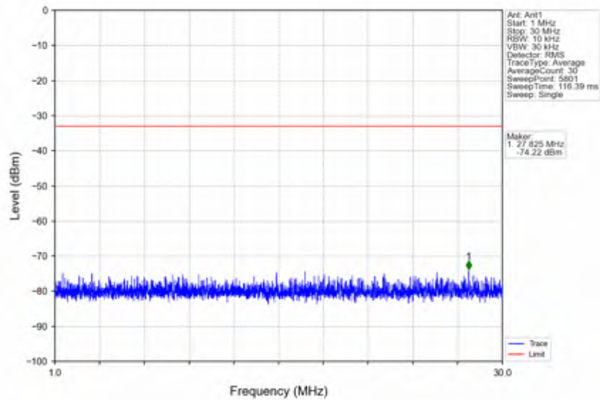
n7_30kHz_SISO_NTV_10MHz_DFT-s-OFDM QPSK_2535MHz_Edge_1RB_Left
