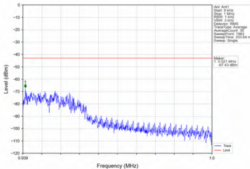
n7_30kHz_SISO_NTNV_30MHz_CP-OFDM QPSK_2535MHz_Edge_1RB_Left
