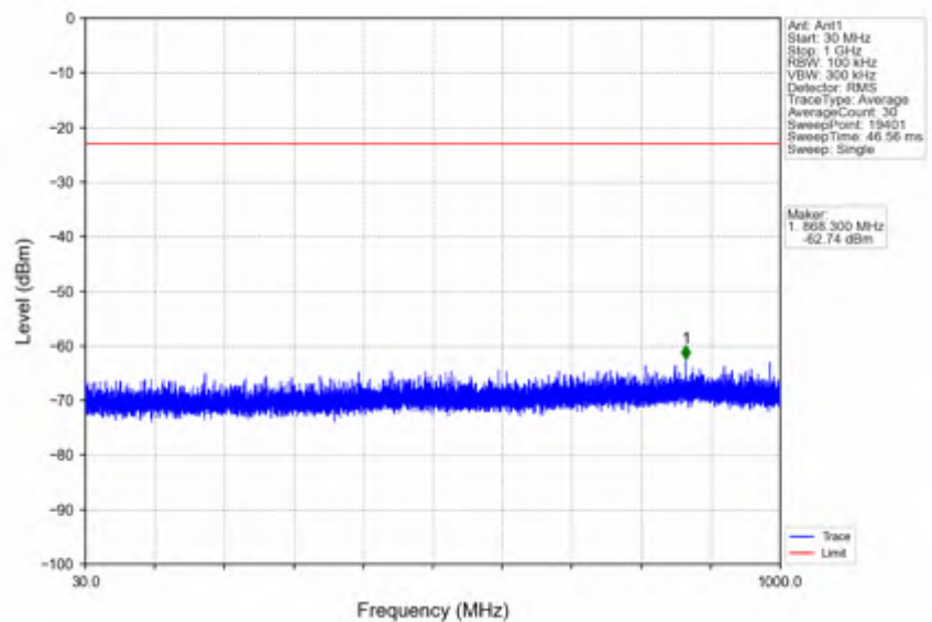
n7_30kHz_SISO_NTNV_20MHz_DFT-s-OFDM QPSK_2510MHz_Edge_1RB_Left
