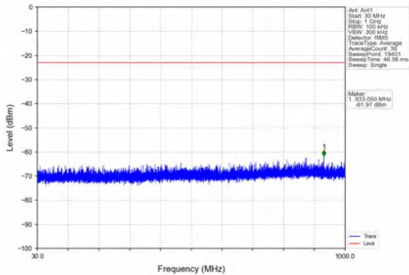
n7_30kHz_SISO_NTNV_40MHz_DFT-s-OFDM QPSK_2550MHz_Edge_1RB_Right
