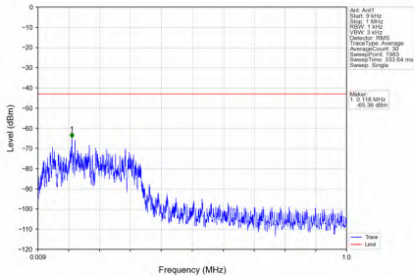
n7_30kHz_SISO_NTNV_20MHz_DFT-s-OFDM QPSK_2560MHz_Edge_1RB_Right
