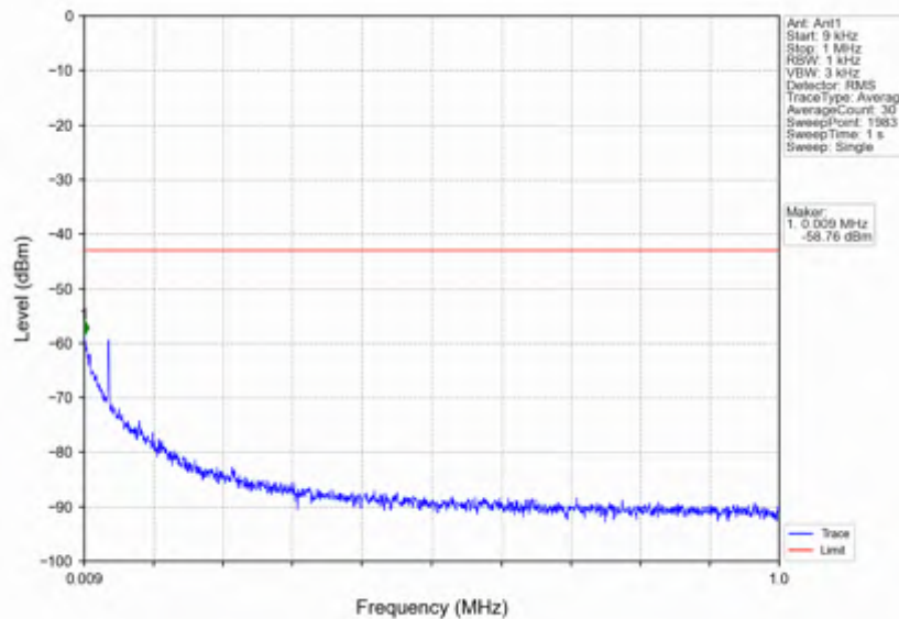
n7_15kHz_SISO_NTNV_50MHz_CP-OFDM_QPSK_2525MHz_Edge_1RB_Left
