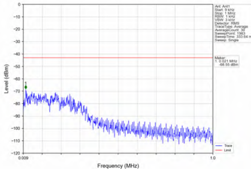
n7_30kHz_SISO_NTNV_15MHz_CP-OFDM QPSK_2507.5MHz_Edge_1RB_Left
