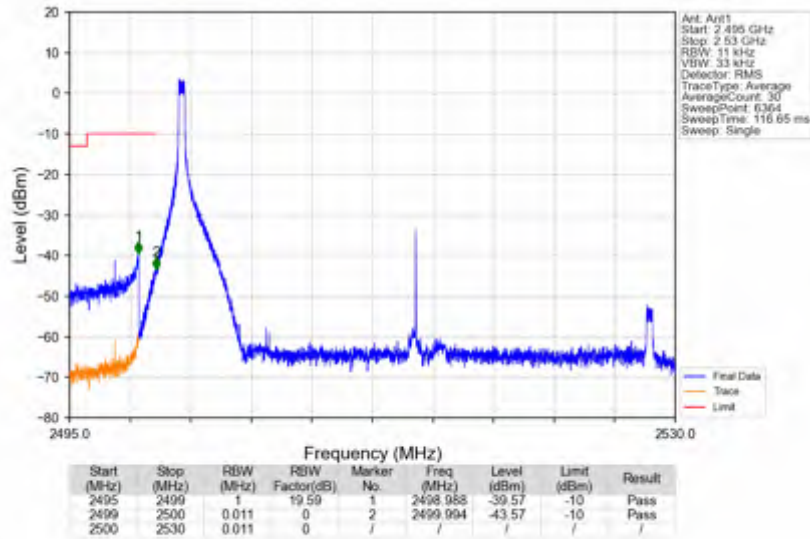
n7_30kHz_SISO_NTNV_30MHz_CP-OFDM QPSK_2515MHz_Inner_1RB_Left
