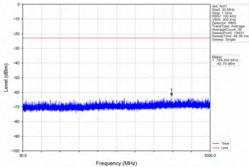
n7_30kHz_SISO_NTNV_15MHz_CP-OFDM QPSK_2562.5MHz_Edge_1RB_Right
