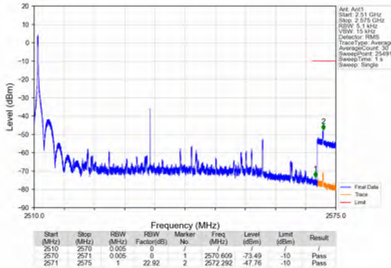
n7_15kHz_SISO_NTV_50MHz_DFT-s-OFDM QPSK_2535MHz_Edge_1RB_Left
