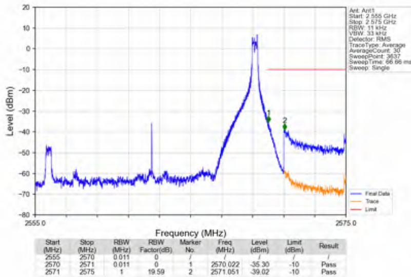
n7_30kHz_SISO_NTV_15MHz_DFT-s-OFDM QPSK_2562.5MHz_Edge_1RB_Right
