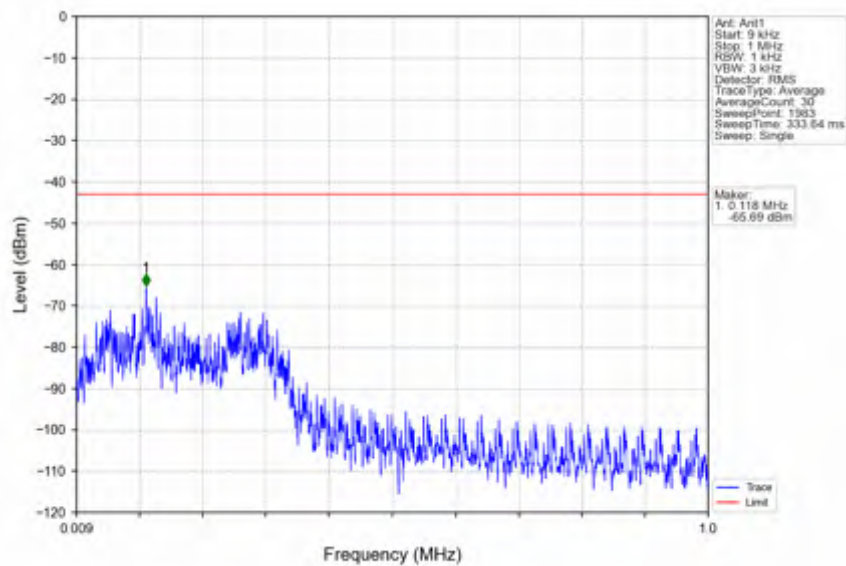
n7_30kHz_SISO_NTNV_30MHz_DFT-s-OFDM_PI/2_BPSK_2515MHz_Edge_1RB_Left
