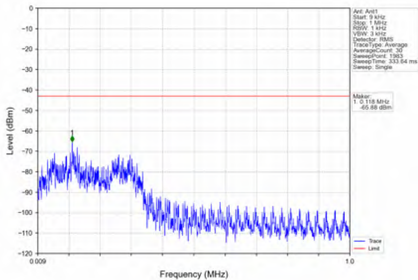
n7_30kHz_SISO_NTNV_40MHz_DFT-s-OFDM_PI/2_BPSK_2520MHz_Edge_1RB_Left
