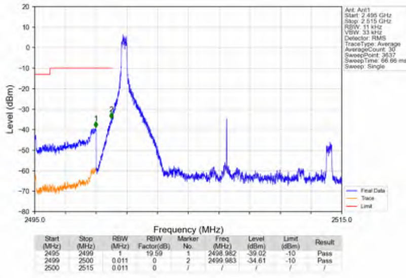
n7_30kHz_SISO_NTNV_15MHz_DFT-s-OFDM PI/2 BPSK_2507.5MHz_Edge_1RB_Left
