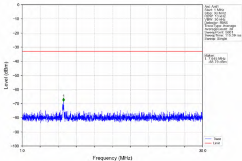
n7_30kHz_SISO_NTNV_30MHz_DFT-s-OFDM QPSK_2555MHz_Edge_1RB_Right
