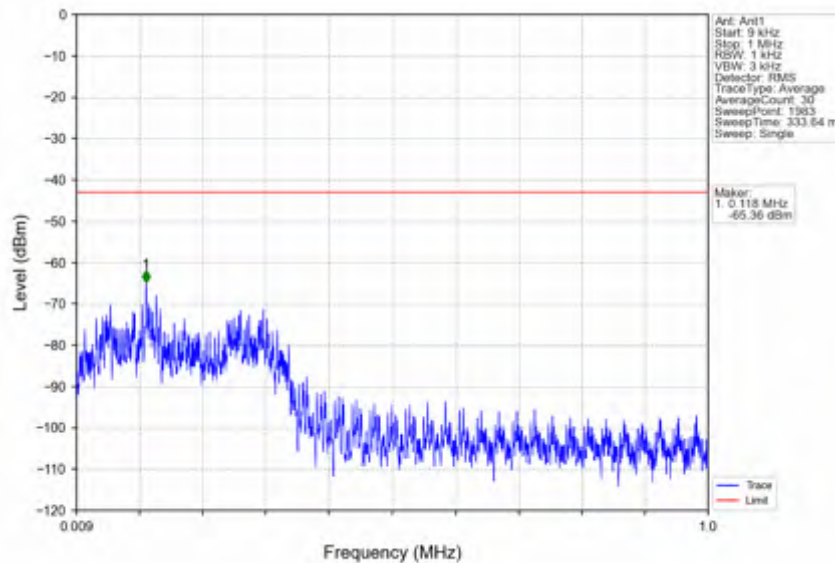
n7_30kHz_SISO_NTNV_40MHz_DFT-s-OFDM PI/2 BPSK_2535MHz_Edge_1RB_Left
