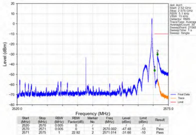
n7_15kHz_SISO_NTNV_50MHz_DFT-s-OFDM QPSK_2545MHz_Inner_1RB_Right
