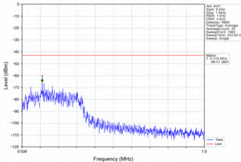
n7_30kHz_SISO_NTV_30MHz_DFT-s-OFDM QPSK_2515MHz_Edge_1RB_Left
