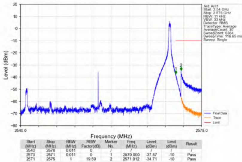
n7_30kHz_SISO_NTNV_30MHz_DFT-s-OFDM PI/2 BPSK_2555MHz_Edge_1RB_Right
