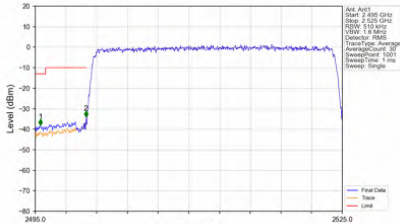
n7_30kHz_SISO_NTNV_25MHz_CP-OFDM QPSK_2512.5MHz_Outer_Full
