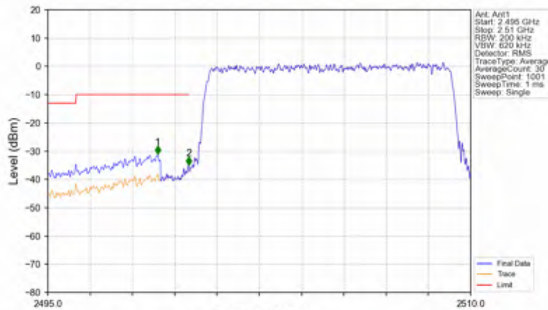
n7_30kHz_SISO_NTNV_10MHz_CP-OFDM QPSK_2505MHz_Outer_Full
