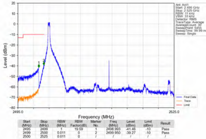
n7_30kHz_SISO_NTNV_25MHz_CP-OFDM QPSK_2512.5MHz_Edge_1RB_Left
