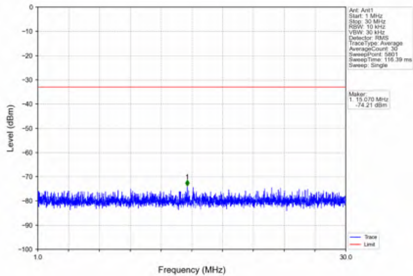
n7_30kHz_SISO_NTNV_15MHz_CP-OFDM QPSK_2507.5MHz_Edge_1RB_Left
