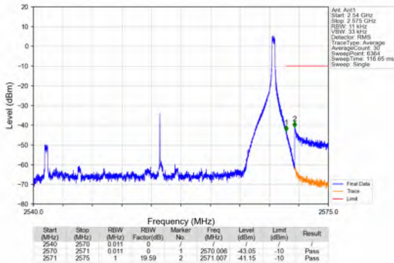
n7_30kHz_SISO_NTNV_30MHz_DFT-s-OFDM QPSK_2555MHz_Inner_1RB_Right
