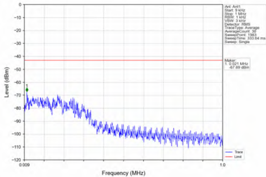
n7_30kHz_SISO_NTNV_20MHz_CP-OFDM QPSK_2560MHz_Edge_1RB_Right
