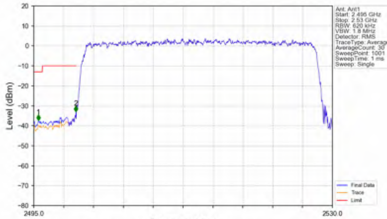
n7_30kHz_SISO_NTNV_30MHz_DFT-s-OFDM QPSK_2515MHz_Outer_Full
