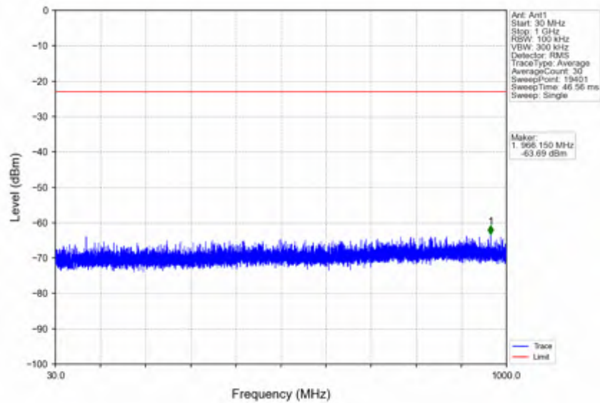
n7_30kHz_SISO_NTNV_10MHz_CP-OFDM QPSK_2565MHz_Edge_1RB_Right
