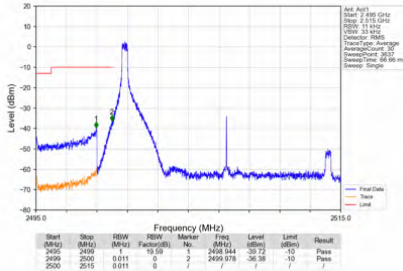
n7_30kHz_SISO_NTNV_15MHz_CP-OFDM QPSK_2507.5MHz_Edge_1RB_Left
