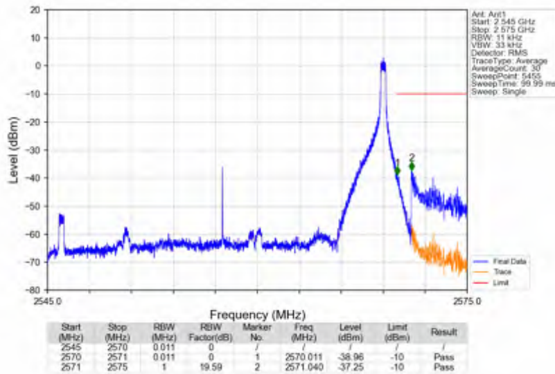
n7_30kHz_SISO_NTNV_25MHz_CP-OFDM QPSK_2557.5MHz_Edge_1RB_Right
