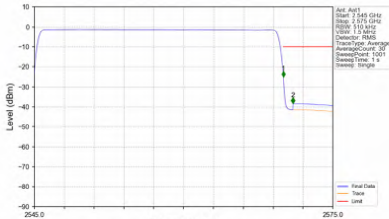
n7_15kHz_SISO_NTV_25MHz_CP-OFDM QPSK_2557.5MHz_Outer_Full
