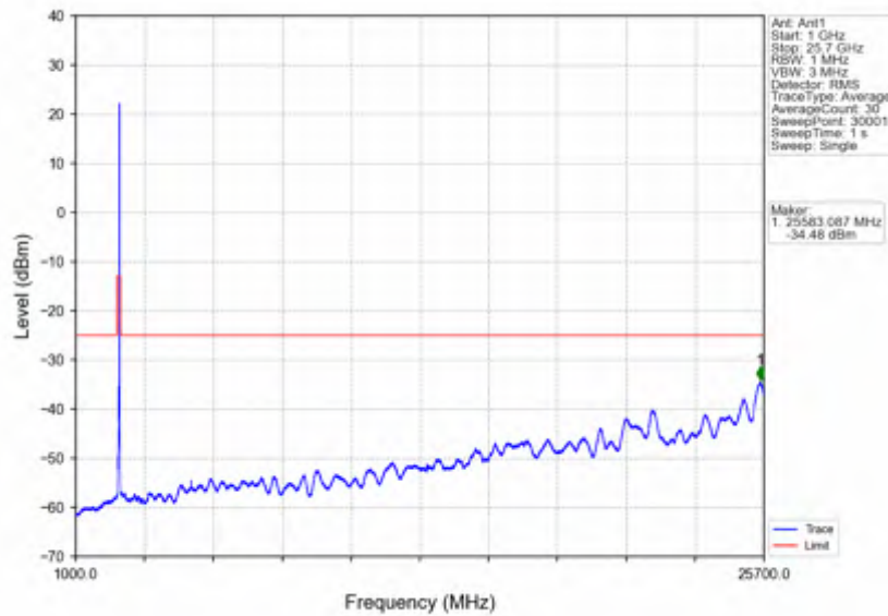
n7_15kHz_SISO_NTNV_30MHz_DFT-s-OFDM PI/2 BPSK_2555MHz_Outer_Full
