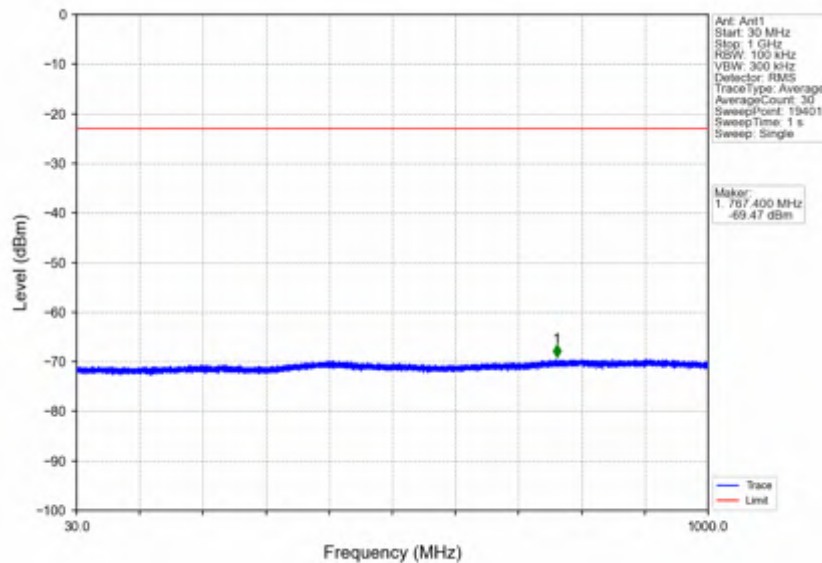
n7_15kHz_SISO_NTNV_40MHz_CP-OFDM QPSK_2550MHz_Inner_1RB_Right
