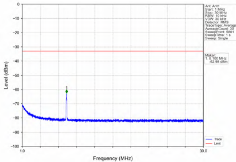
n7_15kHz_SISO_NTNV_40MHz_CP-OFDM QPSK_2550MHz_Edge_1RB_Right
