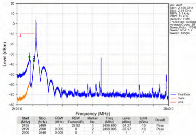
n7_15kHz_SISO_NTNV_40MHz_DFT-s-OFDM QPSK_2520MHz_Edge_1RB_Left
