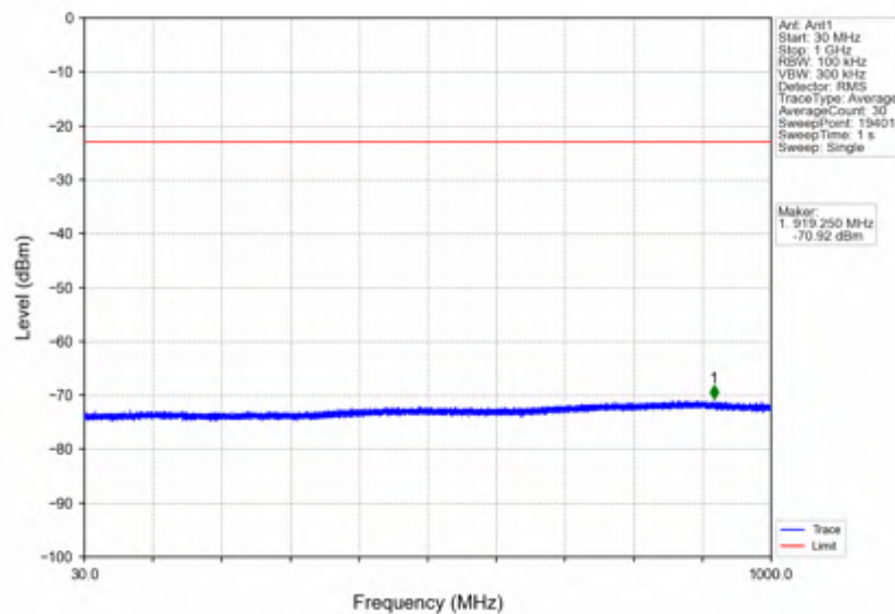
n7_15kHz_SISO_NTNV_25MHz_CP-OFDM QPSK_2512.5MHz_Inner_1RB_Left
