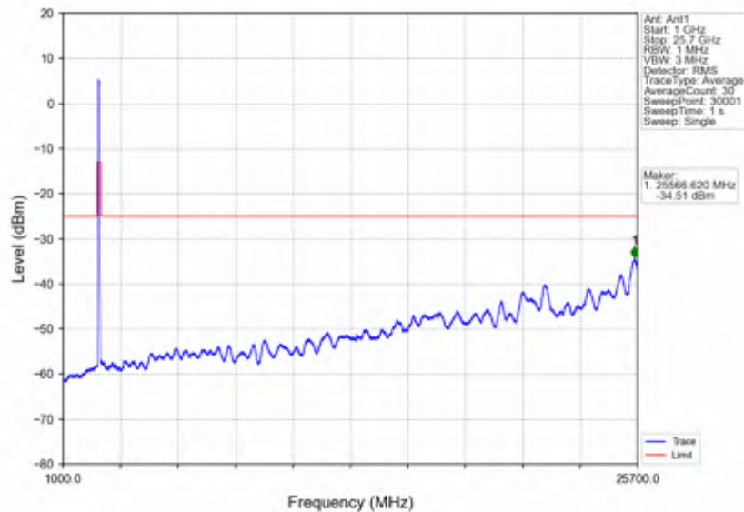
n7_15kHz_SISO_NTNV_40MHz_CP-OFDM QPSK_2520MHz_Outer_Full
