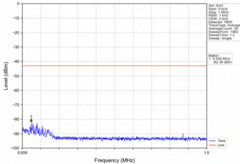
n7_15kHz_SISO_NTNV_25MHz_DFT-s-OFDM QPSK_2512.5MHz_Edge_1RB_Left
