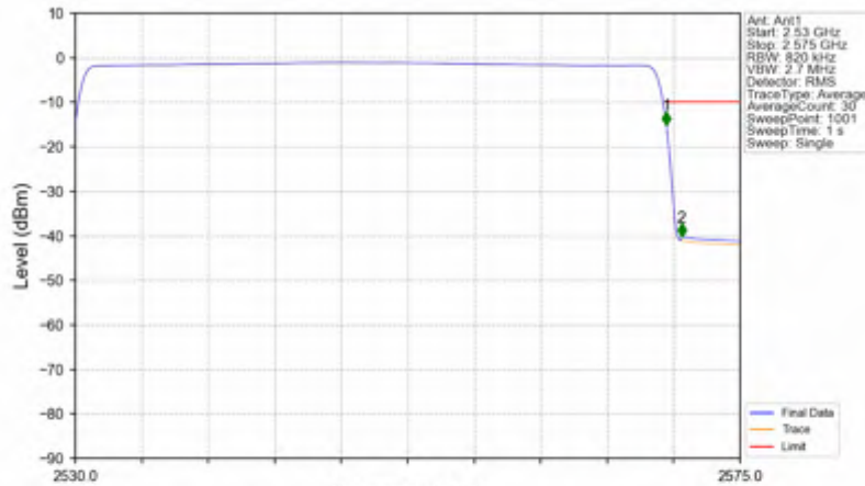
n7_15kHz_SISO_NTNV_40MHz_CP-OFDM QPSK_2550MHz_Outer_Full
