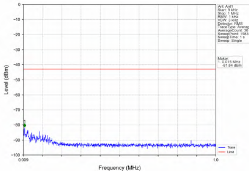
n7_15kHz_SISO_NTNV_25MHz_CP-OFDM QPSK_2512.5MHz_Edge_1RB_Left
