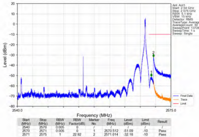
n7_15kHz_SISO_NTNV_30MHz_DFT-s-OFDM QPSK_2555MHz_Inner_1RB_Right
