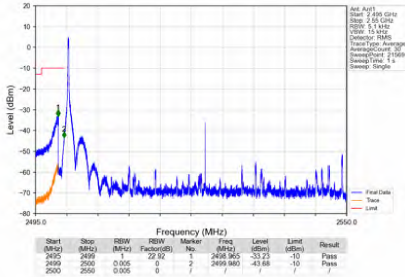
n7_15kHz_SISO_NTNV_50MHz_DFT-s-OFDM_PI/2_BPSK_2525MHz_Edge_1RB_Left
