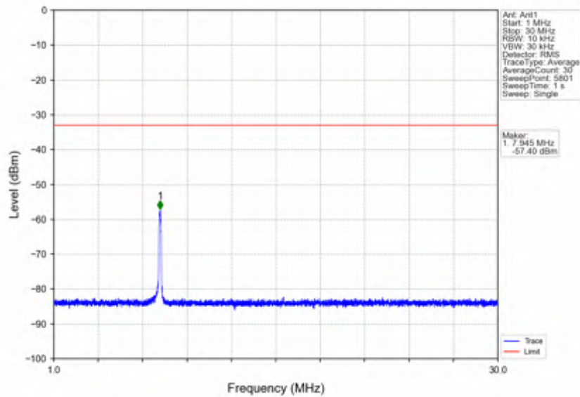
n7_15kHz_SISO_NTV_25MHz_CP-OFDM QPSK_2557.5MHz_Inner_1RB_Right
