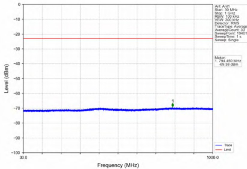
n7_15kHz_SISO_NTNV_30MHz_DFT-s-OFDM QPSK_2555MHz_Inner_1RB_Right
