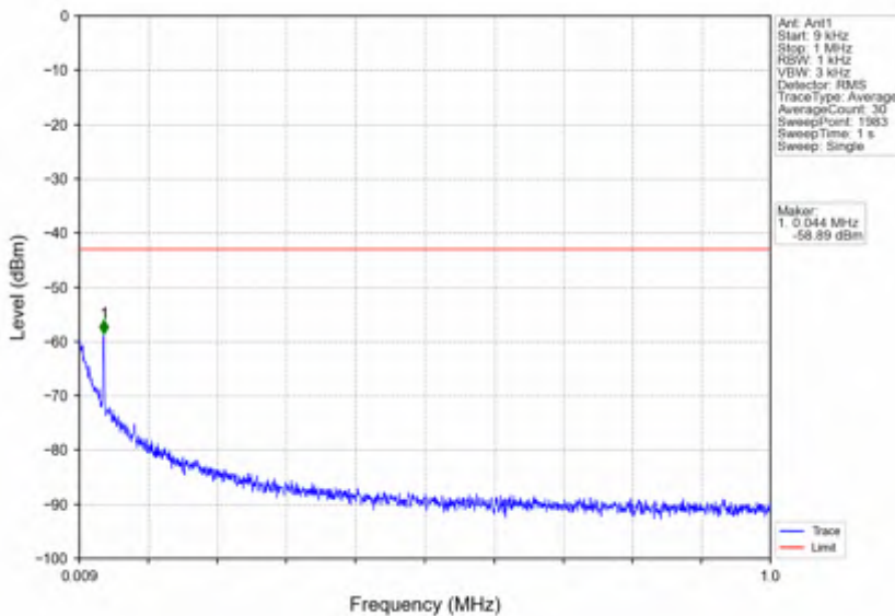
n7_15kHz_SISO_NTNV_50MHz_DFT-s-OFDM QPSK_2525MHz_Outer_Full
