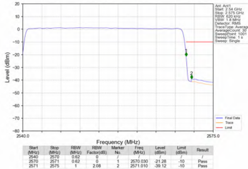
n7_15kHz_SISO_NTNV_30MHz_DFT-s-OFDM QPSK_2555MHz_Outer_Full
