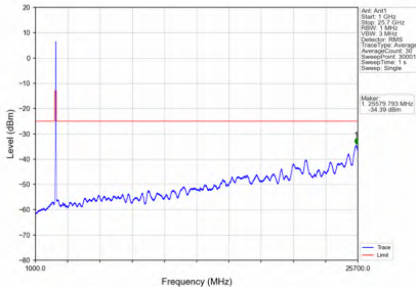
n7_15kHz_SISO_NTNV_30MHz_CP-OFDM QPSK_2555MHz_Outer_Full
