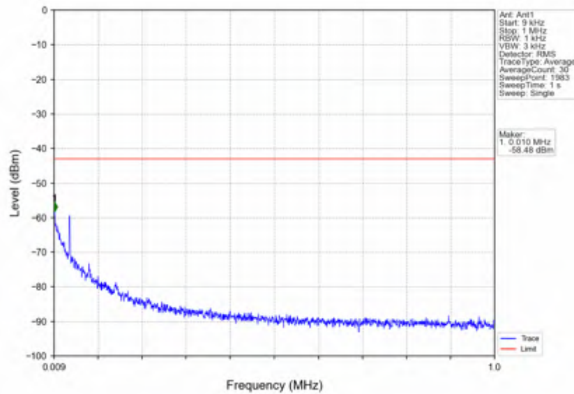
n7_15kHz_SISO_NTNV_40MHz_DFT-s-OFDM QPSK_2520MHz_Edge_1RB_Left
