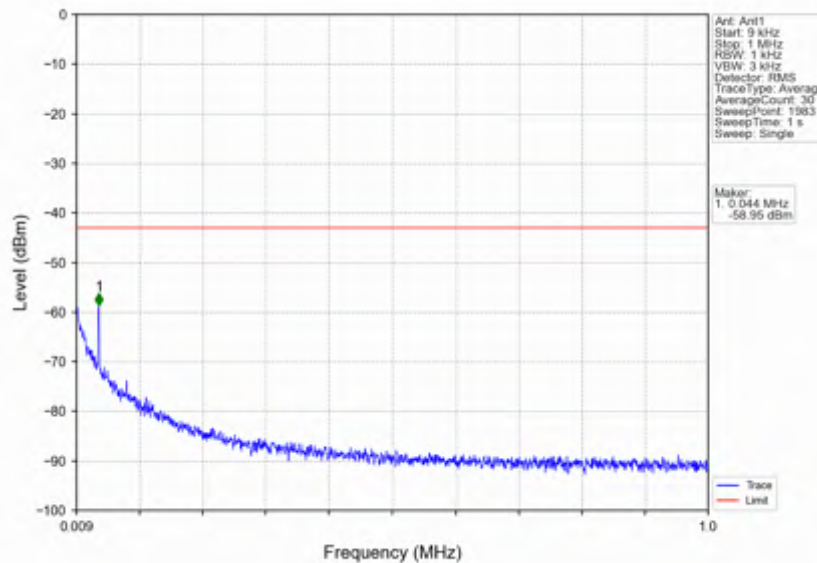
n7_15kHz_SISO_NTNV_40MHz_CP-OFDM QPSK_2520MHz_Edge_1RB_Left
