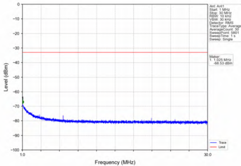
n7_15kHz_SISO_NTNV_30MHz_DFT-s-OFDM_QPSK_2555MHz_Outer_Full
