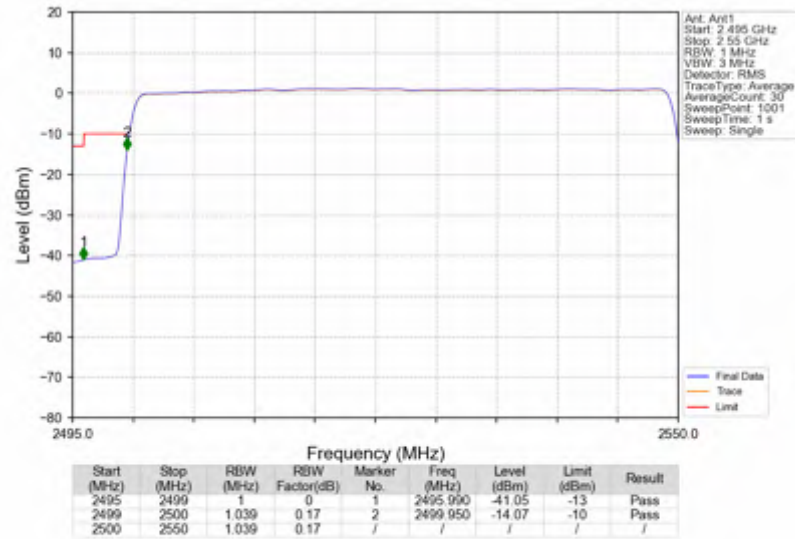
n7_15kHz_SISO_NTNV_50MHz_DFT-s-OFDM QPSK_2525MHz_Outer_Full
