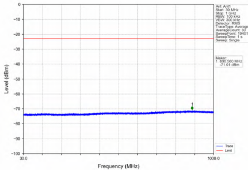
n7_15kHz_SISO_NTV_25MHz_DFT-s-OFDM QPSK_2557.5MHz_Inner_1RB_Right
