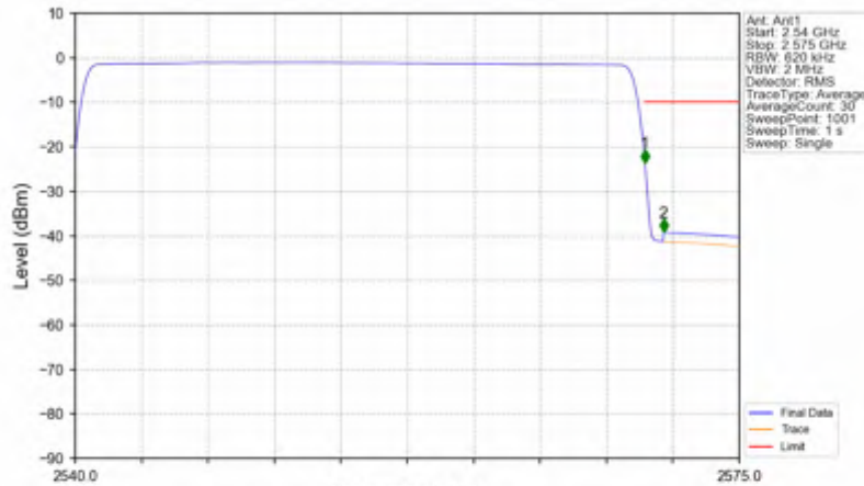
n7_15kHz_SISO_NTNV_30MHz_CP-OFDM QPSK_2555MHz_Outer_Full
