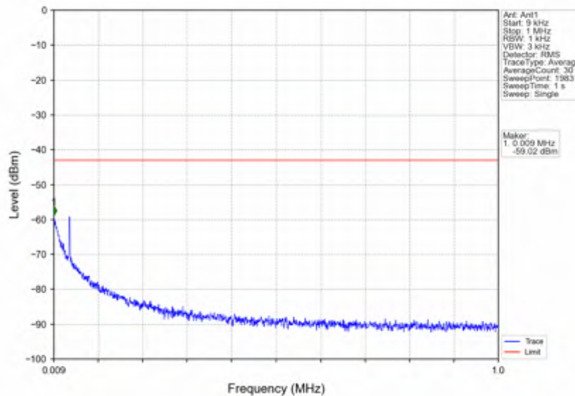
n7_15kHz_SISO_NTNV_40MHz_DFT-s-OFDM QPSK_2520MHz_Outer_Full
