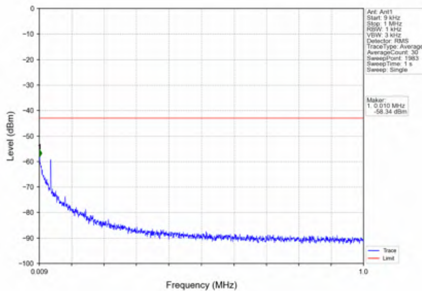
n7_15kHz_SISO_NTNV_50MHz_DFT-s-OFDM_PI/2_BPSK_2525MHz_Edge_1RB_Left
