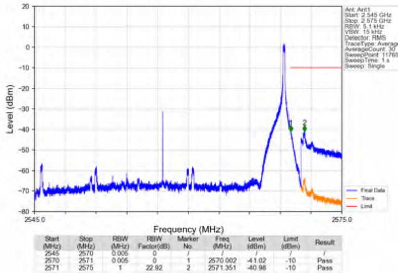
n7_15kHz_SISO_NTV_25MHz_CP-OFDM QPSK_2557.5MHz_Edge_1RB_Right
