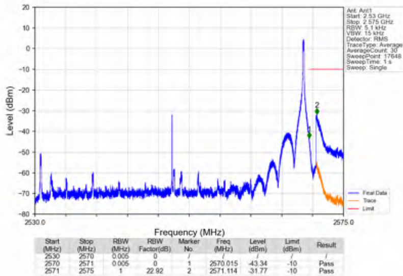
n7_15kHz_SISO_NTNV_40MHz_DFT-s-OFDM QPSK_2550MHz_Inner_1RB_Right
