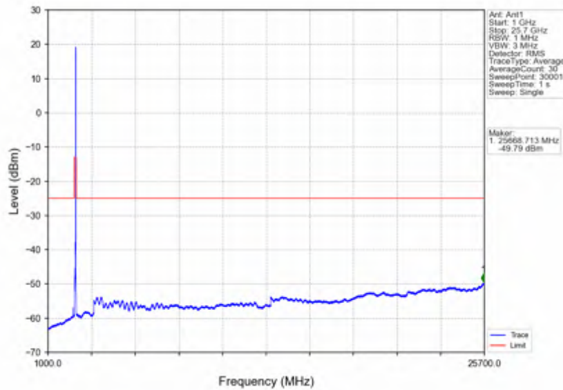
n7_15kHz_SISO_NTV_25MHz_CP-OFDM QPSK_2557.5MHz_Outer_Full
