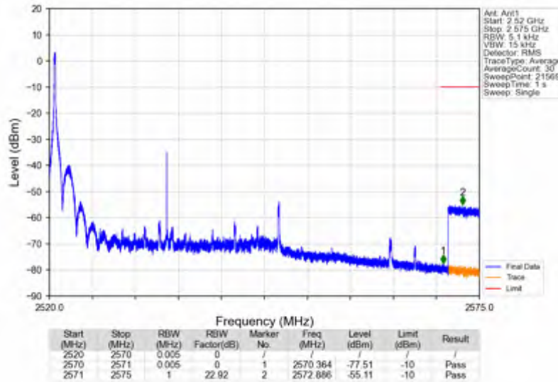
n7_15kHz_SISO_NTV_30MHz_DFT-s-OFDM QPSK_2535MHz_Edge_1RB_Left
