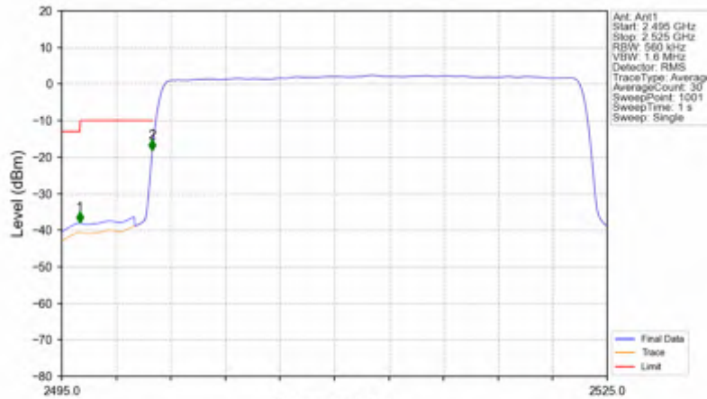
n7_15kHz_SISO_NTNV_25MHz_DFT-s-OFDM PI/2 BPSK_2512.5MHz_Outer_Full
