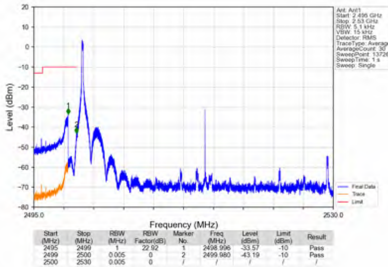
n7_15kHz_SISO_NTNV_30MHz_DFT-s-OFDM QPSK_2515MHz_Edge_1RB_Left
