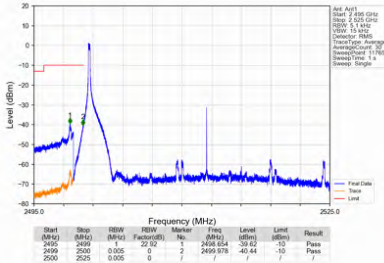
n7_15kHz_SISO_NTNV_25MHz_CP-OFDM QPSK_2512.5MHz_Edge_1RB_Left
