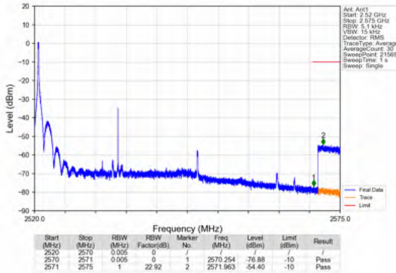
n7_15kHz_SISO_NTNV_30MHz_CP-OFDM QPSK_2535MHz_Edge_1RB_Left
