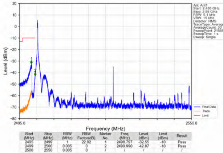
n7_15kHz_SISO_NTNV_50MHz_DFT-s-OFDM QPSK_2525MHz_Edge_1RB_Left
