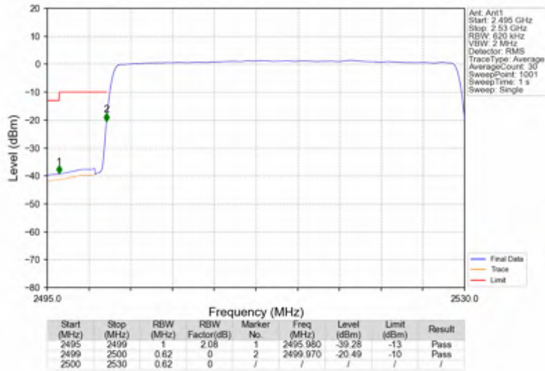
n7_15kHz_SISO_NTNV_30MHz_DFT-s-OFDM QPSK_2515MHz_Outer_Full
