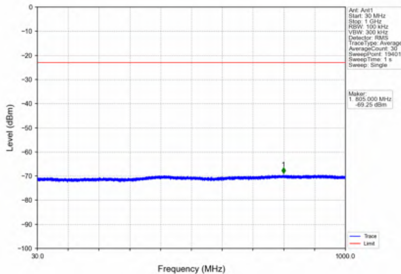
n7_15kHz_SISO_NTNV_40MHz_DFT-s-OFDM_QPSK_2550MHz_Outer_Full
