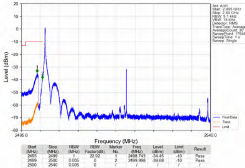
n7_15kHz_SISO_NTNV_40MHz_CP-OFDM QPSK_2520MHz_Edge_1RB_Left
