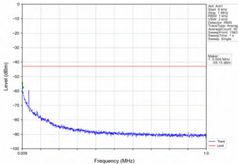
n7_15kHz_SISO_NTNV_40MHz_DFT-s-OFDM QPSK_2535MHz_Edge_1RB_Left
