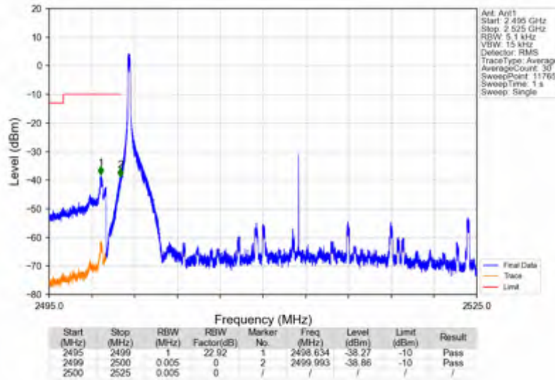
n7_15kHz_SISO_NTNV_25MHz_DFT-s-OFDM QPSK_2512.5MHz_Edge_1RB_Left
