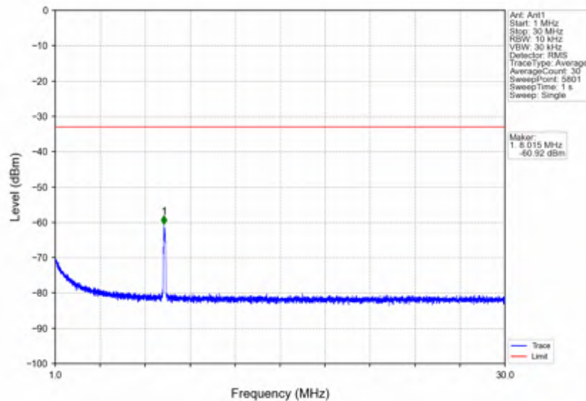
n7_15kHz_SISO_NTNV_30MHz_DFT-s-OFDM QPSK_2555MHz_Edge_1RB_Right
