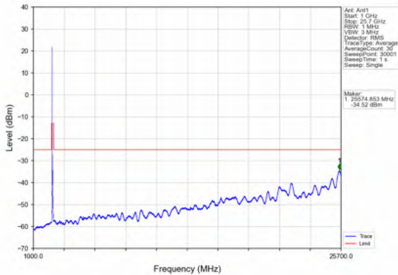
n7_15kHz_SISO_NTV_50MHz_DFT-s-OFDM QPSK_2525MHz_Edge_1RB_Left
