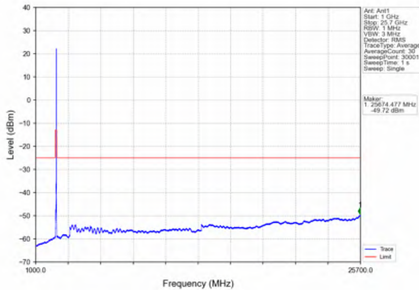
n7_15kHz_SISO_NTV_25MHz_DFT-s-OFDM QPSK_2557.5MHz_Inner_1RB_Right
