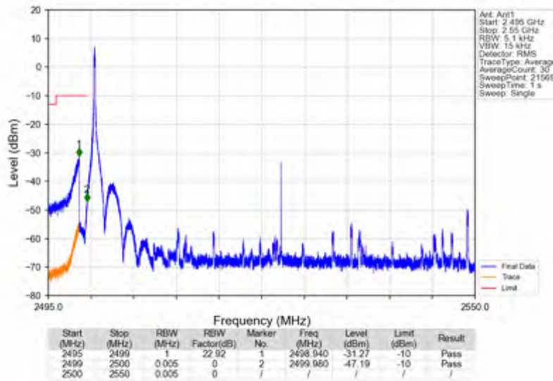
n7_15kHz_SISO_NTNV_50MHz_DFT-s-OFDM_QPSK_2525MHz_Inner_1RB_Left
