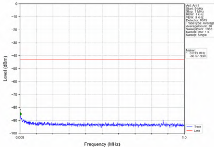
n7_15kHz_SISO_NTNV_30MHz_DFT-s-OFDM QPSK_2515MHz_Outer_Full
