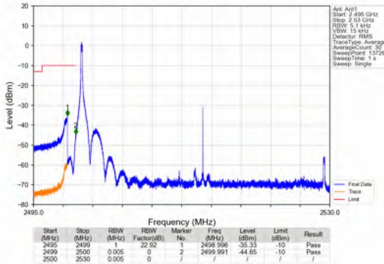
n7_15kHz_SISO_NTNV_30MHz_CP-OFDM QPSK_2515MHz_Edge_1RB_Left
