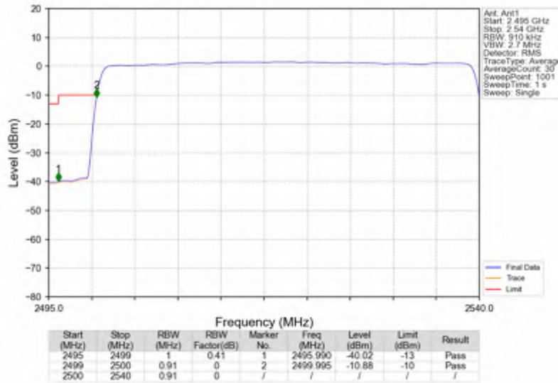
n7_15kHz_SISO_NTNV_40MHz_DFT-s-OFDM QPSK_2520MHz_Outer_Full
