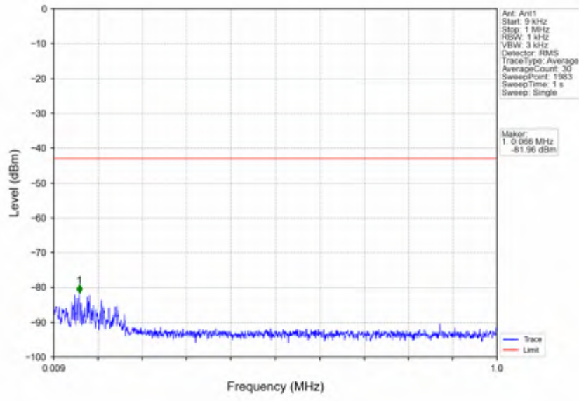
n7_15kHz_SISO_NTV_25MHz_DFT-s-OFDM QPSK_2535MHz_Edge_1RB_Left
