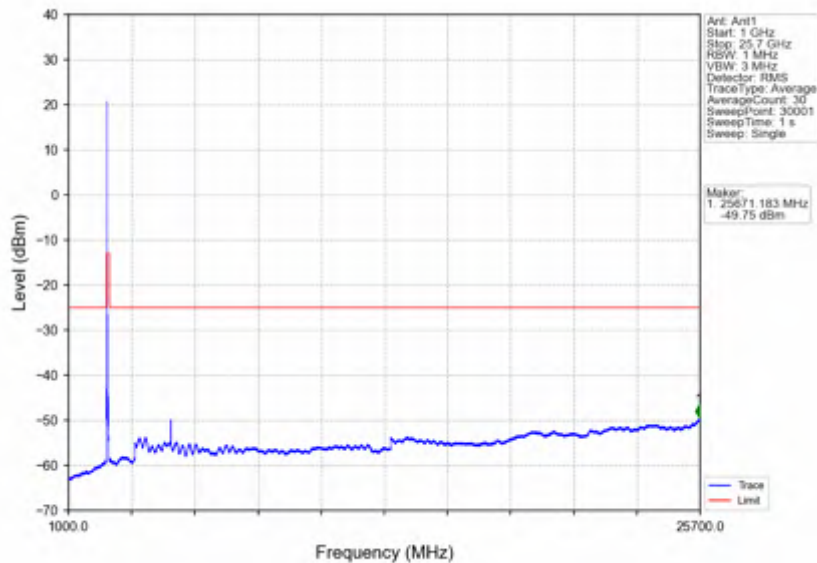
n7_15kHz_SISO_NTNV_25MHz_DFT-s-OFDM QPSK_2512.5MHz_Edge_1RB_Left
