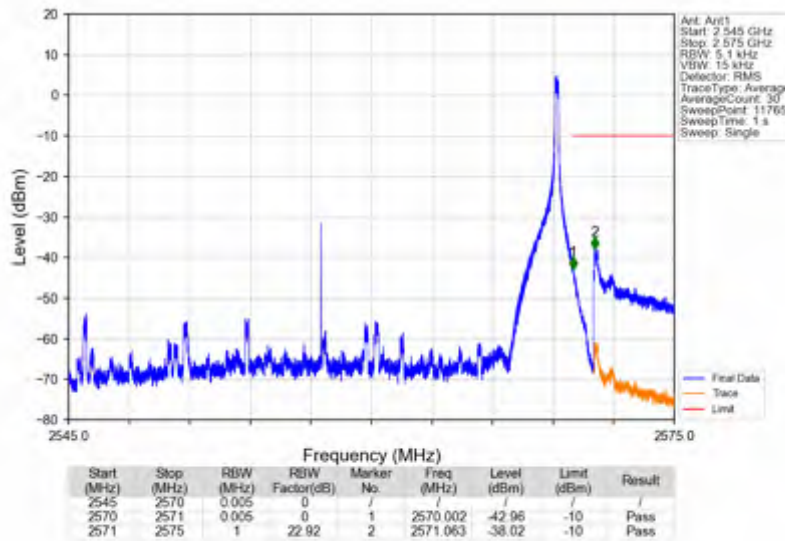
n7_15kHz_SISO_NTNV_25MHz_DFT-s-OFDM QPSK_2557.5MHz_Inner_1RB_Right
