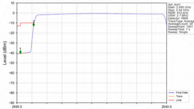
n7_15kHz_SISO_NTNV_40MHz_CP-OFDM QPSK_2520MHz_Outer_Full
