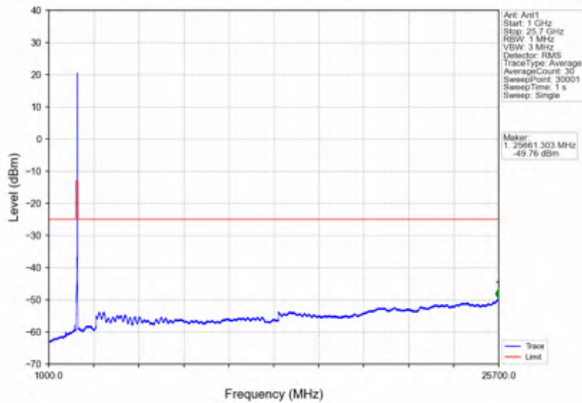
n7_15kHz_SISO_NTNV_25MHz_CP-OFDM QPSK_2557.5MHz_Inner_1RB_Right
