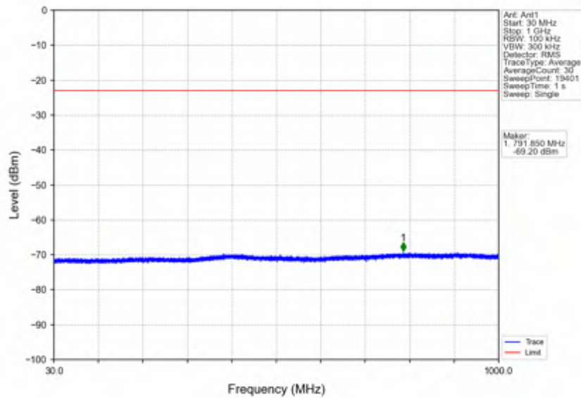
n7_15kHz_SISO_NTNV_50MHz_DFT-s-OFDM QPSK_2525MHz_Inner_1RB_Left
