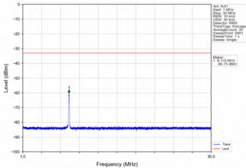
n7_15kHz_SISO_NTV_25MHz_CP-OFDM QPSK_2557.5MHz_Edge_1RB_Right
