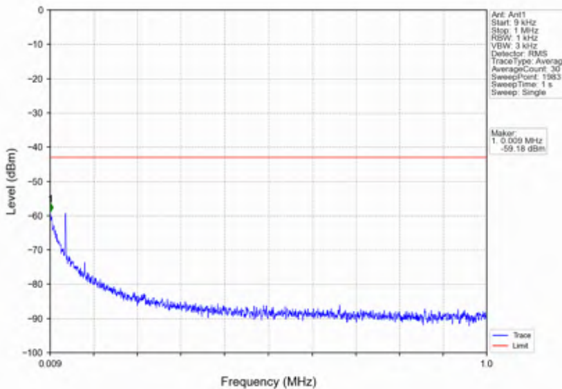
n7_15kHz_SISO_NTNV_30MHz_DFT-s-OFDM QPSK_2555MHz_Outer_Full
