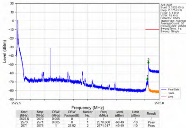
n7_15kHz_SISO_NTNV_25MHz_CP-OFDM QPSK_2535MHz_Edge_1RB_Left
