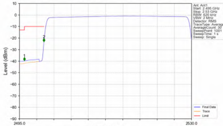
n7_15kHz_SISO_NTNV_30MHz_CP-OFDM QPSK_2515MHz_Outer_Full
