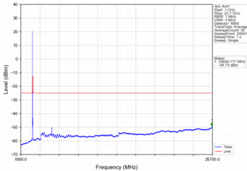
n7_15kHz_SISO_NTNV_25MHz_CP-OFDM QPSK_2535MHz_Edge_1RB_Left
