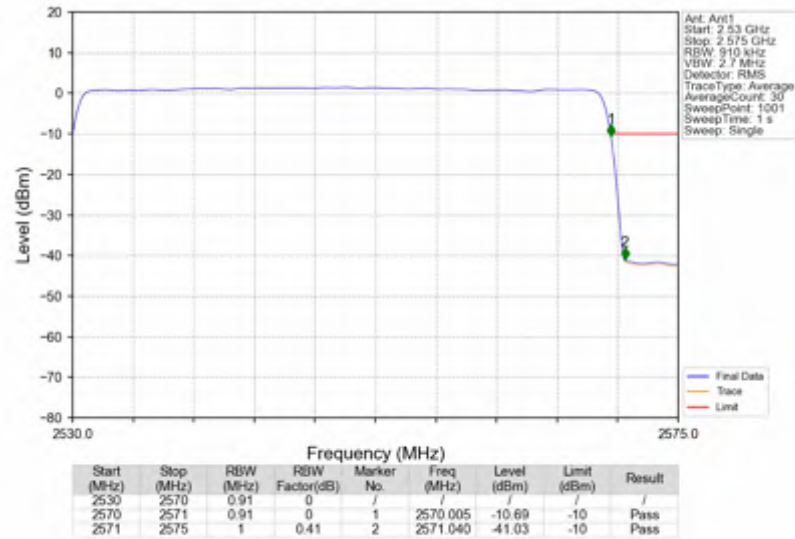
n7_15kHz_SISO_NTNV_40MHz_DFT-s-OFDM_QPSK_2550MHz_Outer_Full
