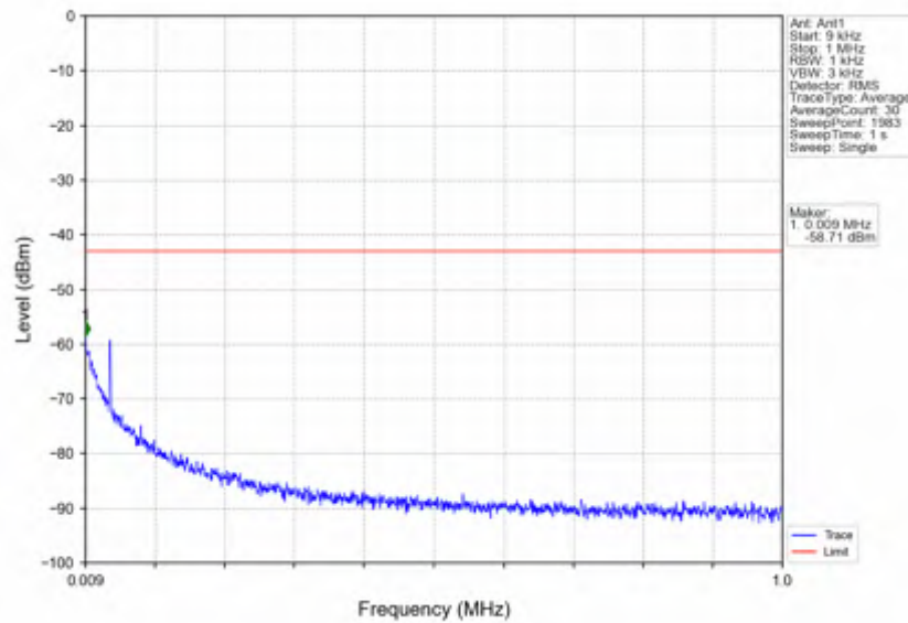
n7_15kHz_SISO_NTNV_30MHz_CP-OFDM QPSK_2515MHz_Outer_Full
