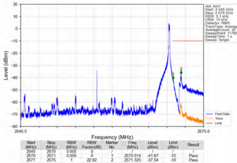
n7_15kHz_SISO_NTNV_25MHz_DFT-s-OFDM QPSK_2557.5MHz_Edge_1RB_Right
