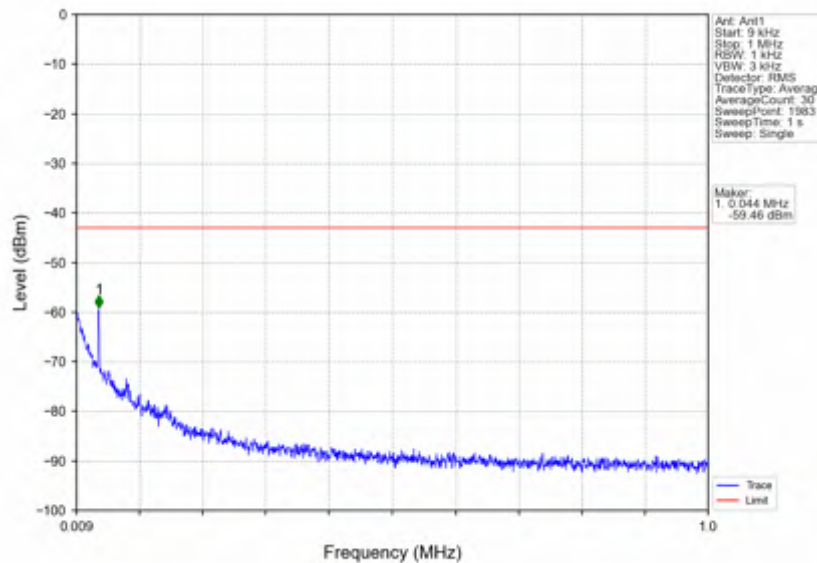
n7_15kHz_SISO_NTV_30MHz_DFT-s-OFDM QPSK_2535MHz_Edge_1RB_Left
