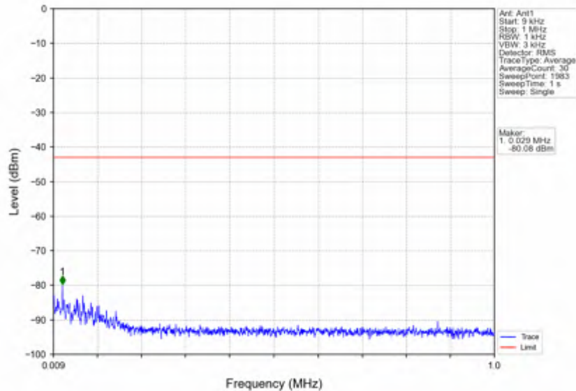
n7_15kHz_SISO_NTV_25MHz_CP-OFDM QPSK_2557.5MHz_Edge_1RB_Right
