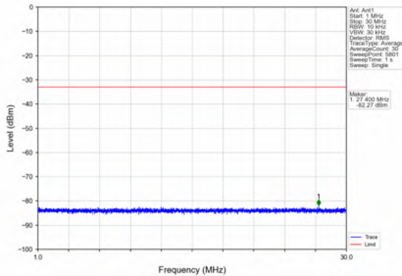
n7_15kHz_SISO_NTV_25MHz_DFT-s-OFDM QPSK_2535MHz_Edge_1RB_Left
