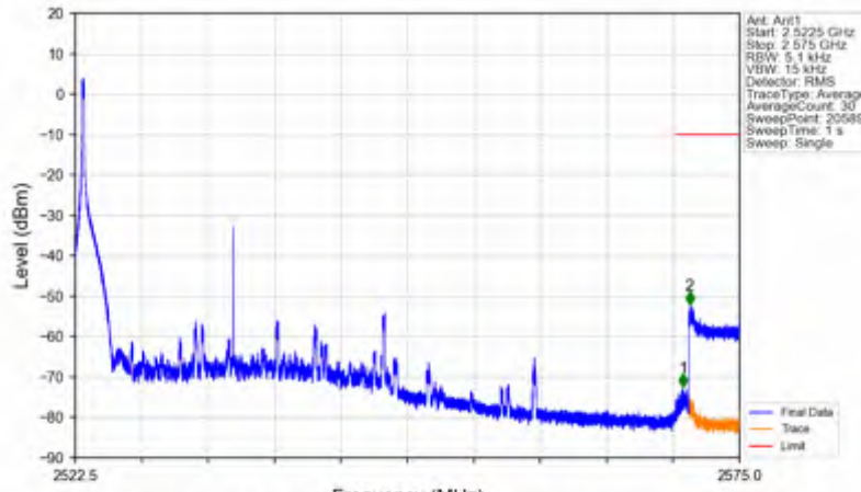
n7_15kHz_SISO_NTV_25MHz_DFT-s-OFDM QPSK_2535MHz_Edge_1RB_Left
