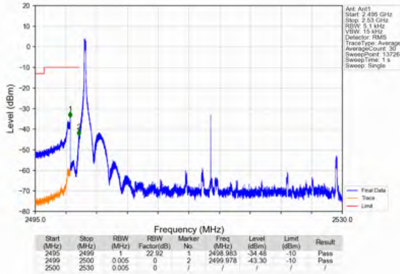
n7_15kHz_SISO_NTNV_30MHz_DFT-s-OFDM_PI/2_BPSK_2515MHz_Edge_1RB_Left
