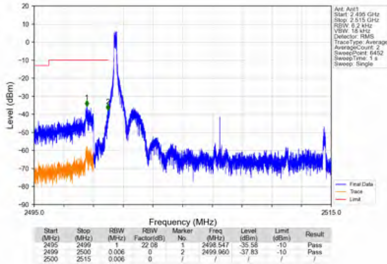
n7_15kHz_SISO_NTNV_15MHz_DFT-s-OFDM QPSK_2507.5MHz_Edge_1RB_Left
