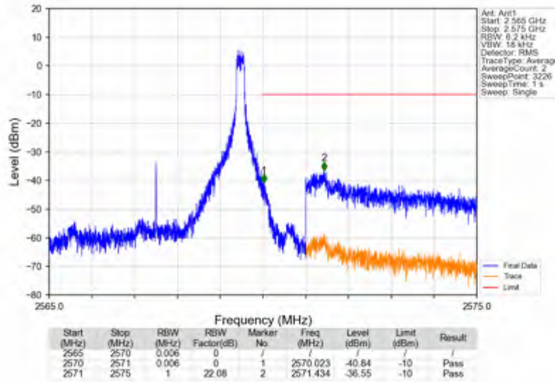
n7_15kHz_SISO_NTV_5MHz_CP-OFDM QPSK_2567.5MHz_Inner_1RB_Right
