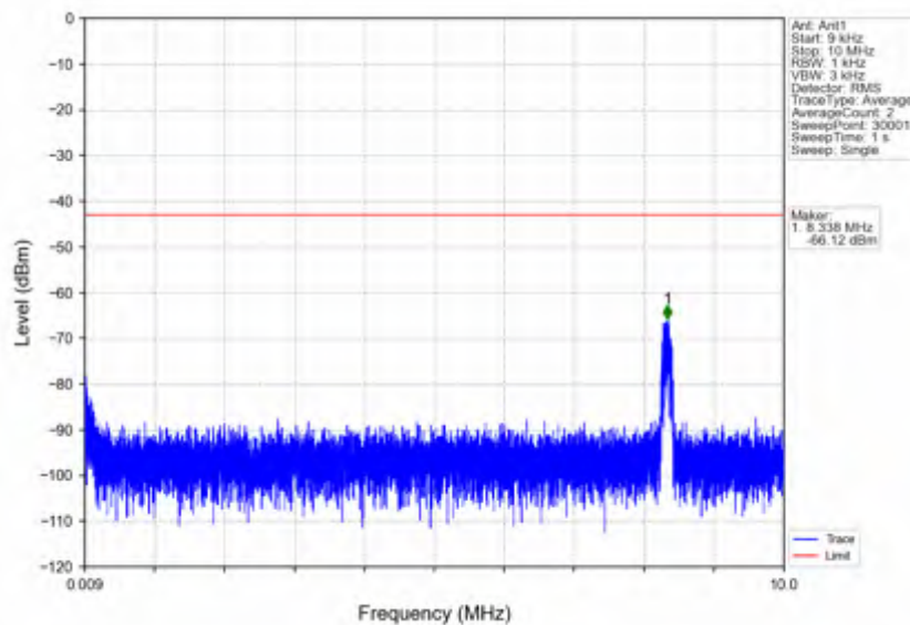
n7_15kHz_SISO_NTNV_10MHz_CP-OFDM QPSK_2565MHz_Edge_1RB_Right
