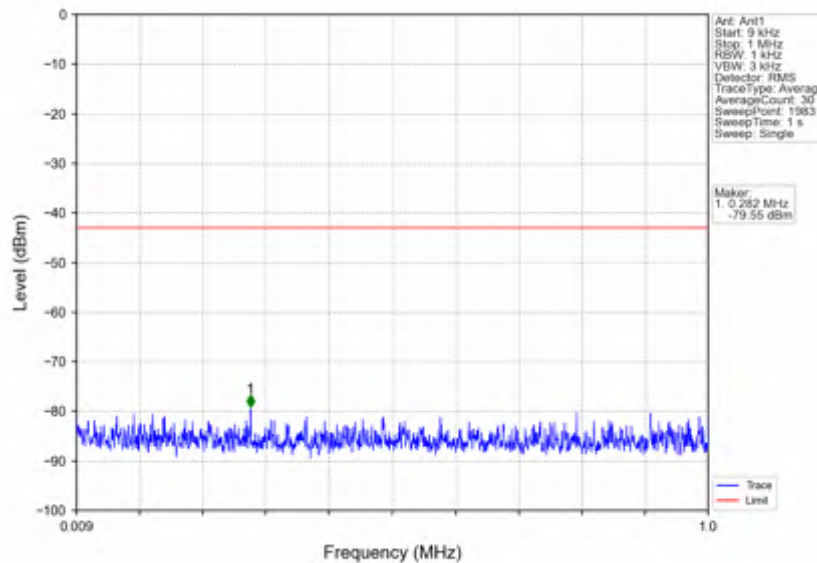
n7_15kHz_SISO_NTNV_20MHz_DFT-s-OFDM QPSK_2560MHz_Outer_Full
