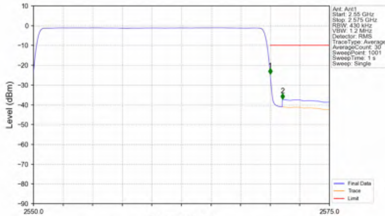
n7_15kHz_SISO_NTNV_20MHz_CP-OFDM QPSK_2560MHz_Outer_Full
