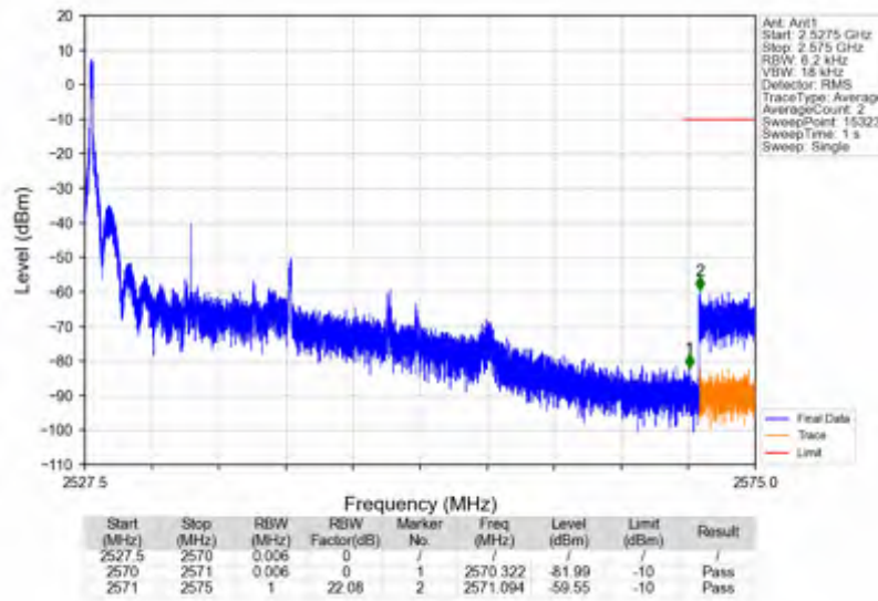
n7_15kHz_SISO_NTNV_15MHz_DFT-s-OFDM PI/2 BPSK_2535MHz_Edge_1RB_Left
