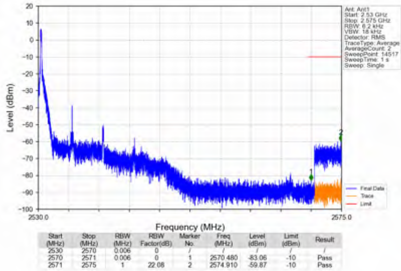
n7_15kHz_SISO_NTNV_10MHz_DFT-s-OFDM PI/2 BPSK_2535MHz_Edge_1RB_Left
