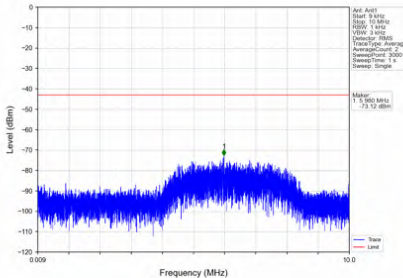
n7_15kHz_SISO_NTNV_5MHz_DFT-s-OFDM QPSK_2567.5MHz_Outer_Full
