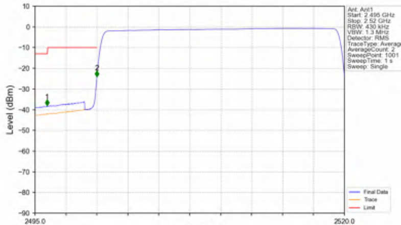
n7_15kHz_SISO_NTNV_20MHz_CP-OFDM QPSK_2510MHz_Outer_Full
