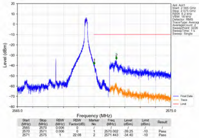
n7_15kHz_SISO_NTNV_5MHz_DFT-s-OFDM QPSK_2567.5MHz_Inner_1RB_Right
