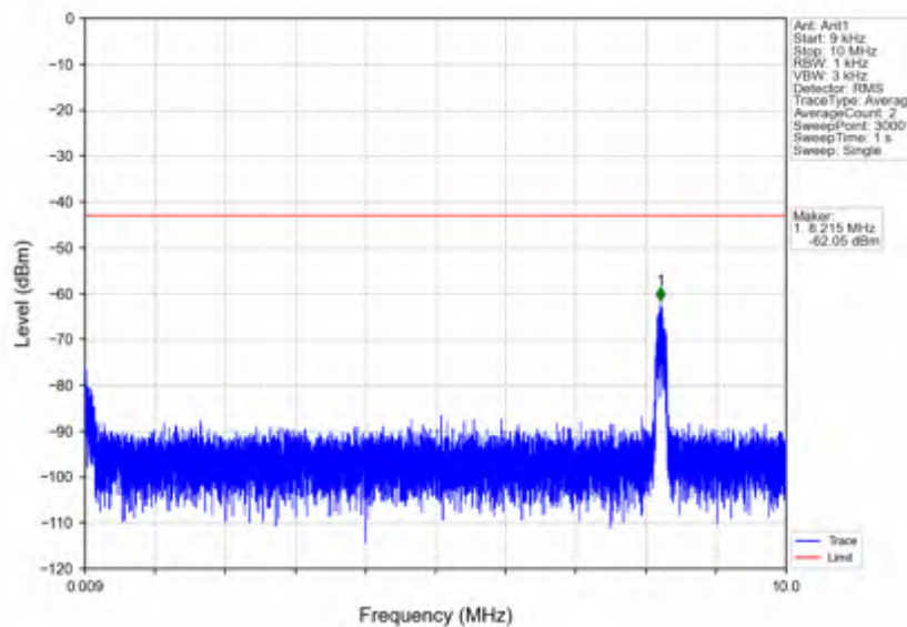
n7_15kHz_SISO_NTV_5MHz_CP-OFDM QPSK_2567.5MHz_Inner_1RB_Right
