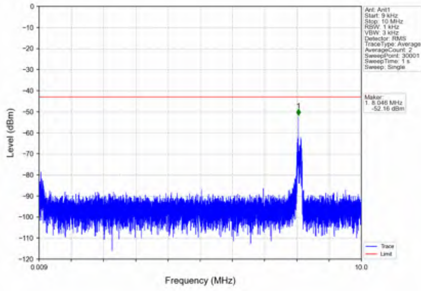
n7_15kHz_SISO_NTNV_15MHz_DFT-s-OFDM PI/2 BPSK_2562.5MHz_Inner_1RB_Right
