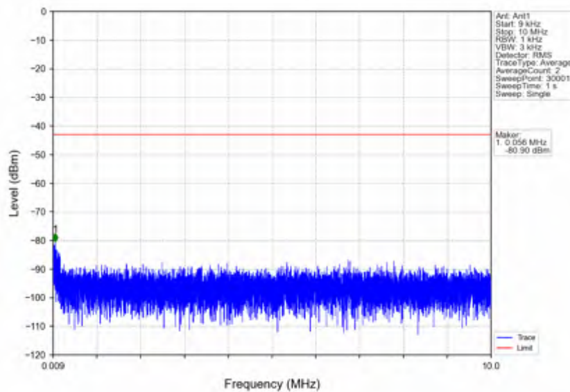
n7_15kHz_SISO_NTNV_10MHz_DFT-s-OFDM_PI/2_BPSK_2505MHz_Edge_1RB_Left
