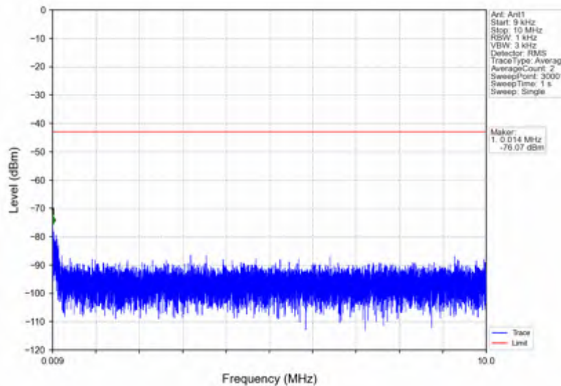
n7_15kHz_SISO_NTNV_15MHz_CP-OFDM QPSK_2507.5MHz_Inner_1RB_Left
