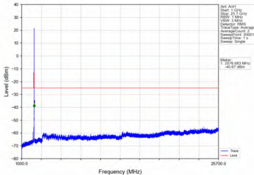
n7_15kHz_SISO_NTV_15MHz_DFT-s-OFDM QPSK_2562.5MHz_Edge_1RB_Right
