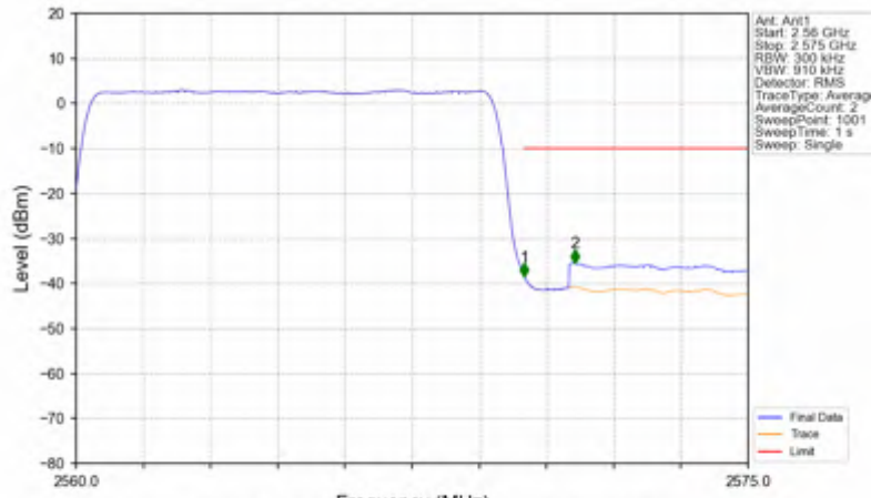
n7_15kHz_SISO_NTNV_10MHz_DFT-s-OFDM QPSK_2565MHz_Outer_Full
