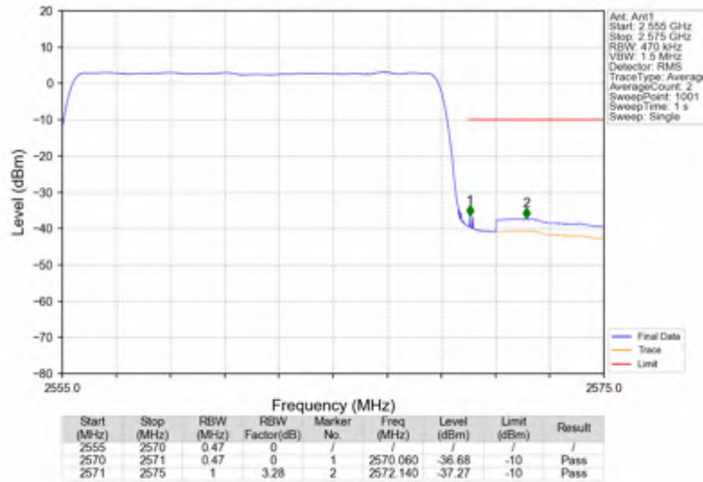
n7_15kHz_SISO_NTNV_15MHz_DFT-s-OFDM QPSK_2562.5MHz_Outer_Full
