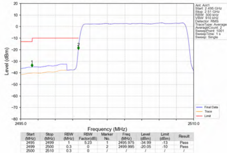
n7_15kHz_SISO_NTNV_10MHz_DFT-s-OFDM QPSK_2505MHz_Outer_Full
