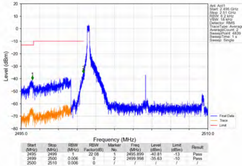
n7_15kHz_SISO_NTNV_10MHz_CP-OFDM QPSK_2505MHz_Edge_1RB_Left
