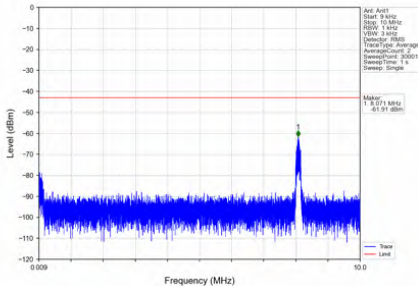
n7_15kHz_SISO_NTV_15MHz_CP-OFDM QPSK_2562.5MHz_Inner_1RB_Right
