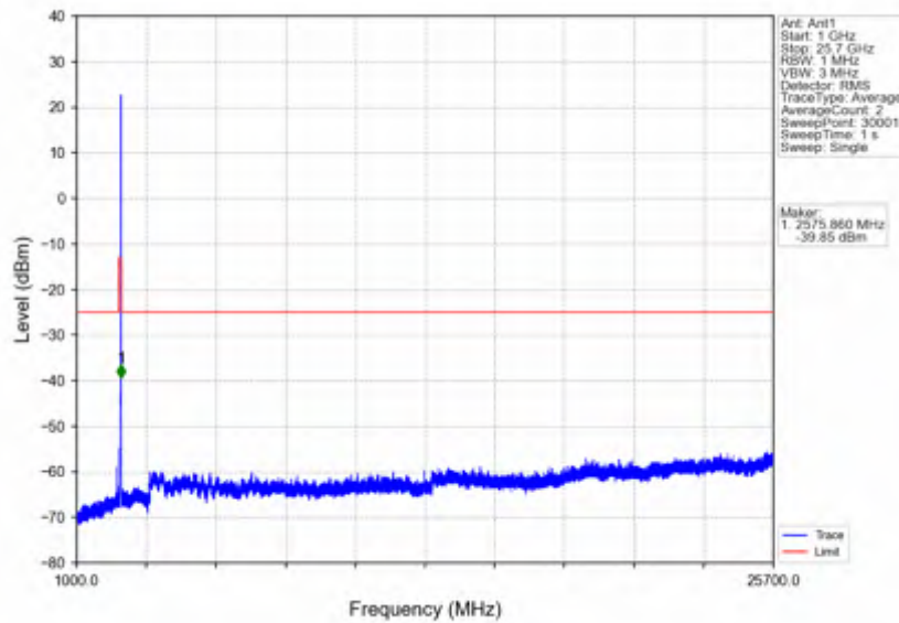
n7_15kHz_SISO_NTNV_15MHz_DFT-s-OFDM QPSK_2507.5MHz_Edge_1RB_Left
