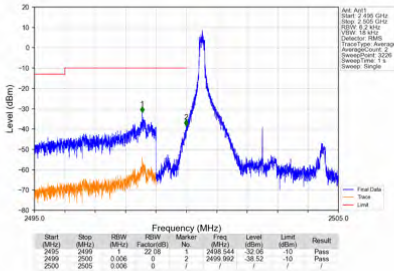
n7_15kHz_SISO_NTNV_5MHz_DFT-s-OFDM QPSK_2502.5MHz_Inner_1RB_Left
