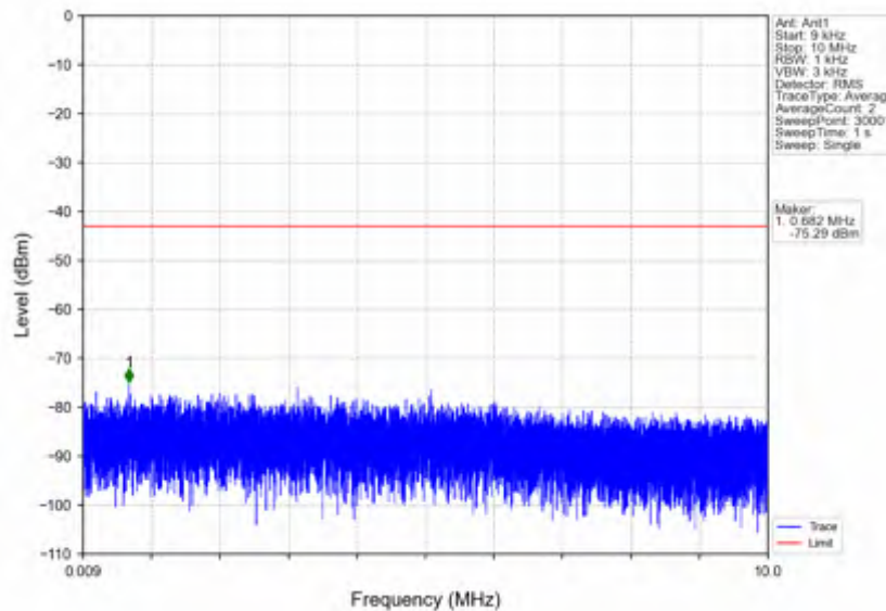
n7_15kHz_SISO_NTNV_15MHz_DFT-s-OFDM QPSK_2562.5MHz_Outer_Full
