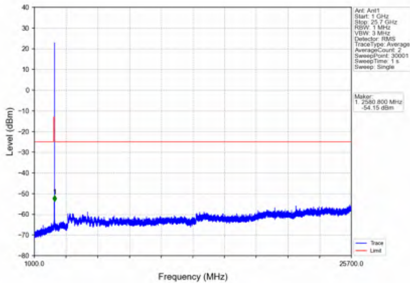
n7_15kHz_SISO_NTNV_10MHz_DFT-s-OFDM QPSK_2505MHz_Edge_1RB_Left
