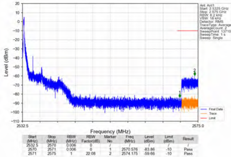
n7_15kHz_SISO_NTNV_5MHz_CP-OFDM QPSK_2535MHz_Edge_1RB_Left
