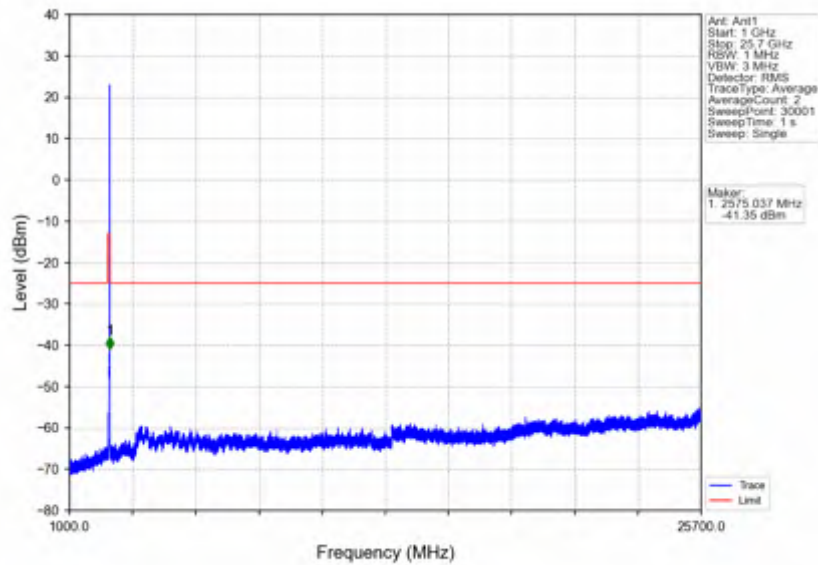
n7_15kHz_SISO_NTV_15MHz_DFT-s-OFDM_QPSK_2562.5MHz_Inner_1RB_Right
