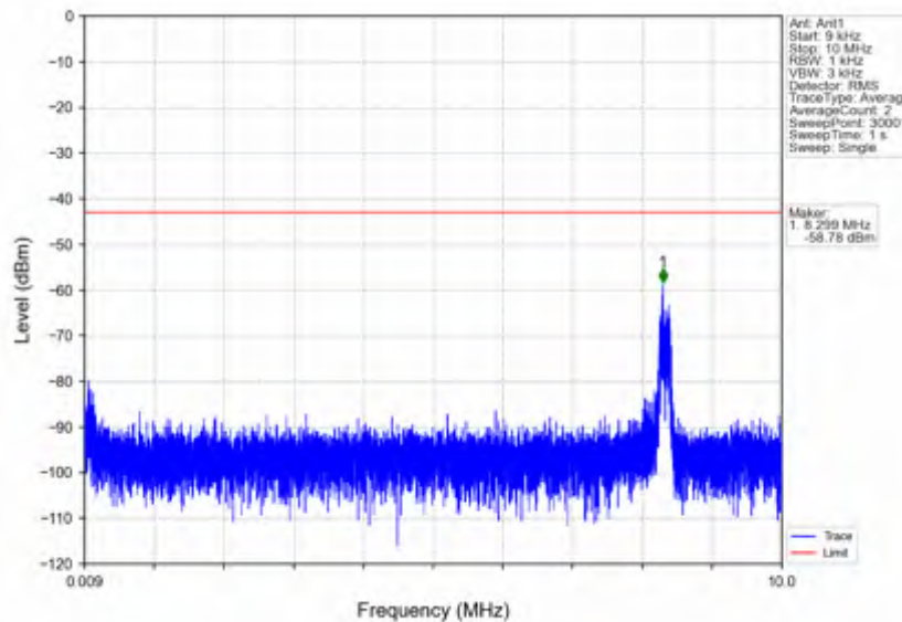
n7_15kHz_SISO_NTNV_10MHz_DFT-s-OFDM PI/2 BPSK_2565MHz_Edge_1RB_Right
