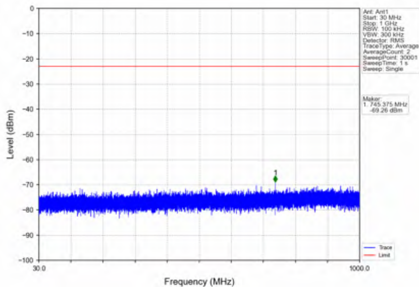
n7_15kHz_SISO_NTNV_15MHz_DFT-s-OFDM PI/2 BPSK_2507.5MHz_Inner_1RB_Left
