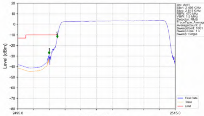
n7_15kHz_SISO_NTNV_15MHz_DFT-s-OFDM PI/2 BPSK_2507.5MHz_Outer_Full
