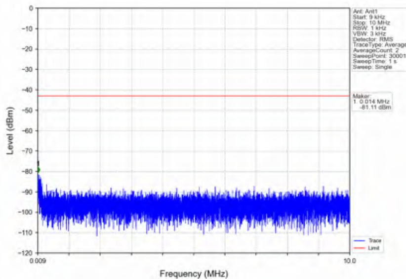
n7_15kHz_SISO_NTNV_15MHz_CP-OFDM QPSK_2507.5MHz_Edge_1RB_Left
