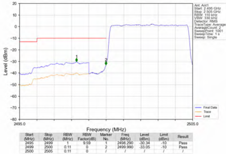
n7_15kHz_SISO_NTNV_5MHz_DFT-s-OFDM QPSK_2502.5MHz_Outer_Full
