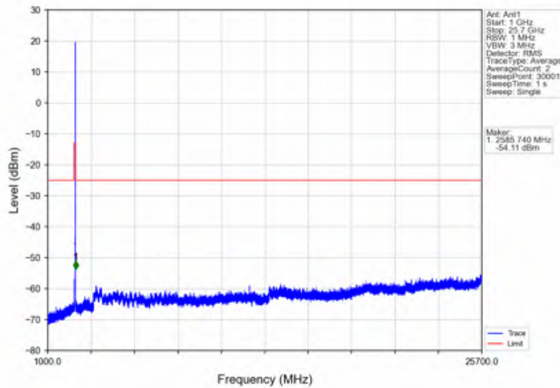
n7_15kHz_SISO_NTV_15MHz_CP-OFDM QPSK_2562.5MHz_Outer_Full
