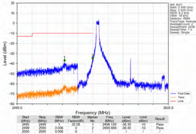
n7_15kHz_SISO_NTV_5MHz_CP-OFDM QPSK_2502.5MHz_Edge_1RB_Left
