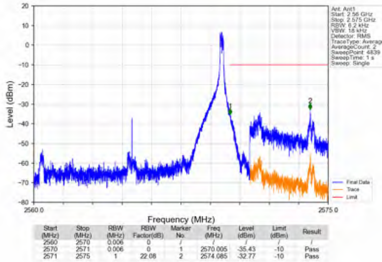
n7_15kHz_SISO_NTNV_10MHz_DFT-s-OFDM PI/2 BPSK_2565MHz_Edge_1RB_Right
