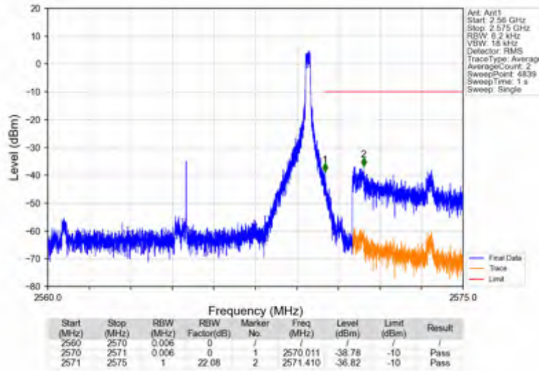
n7_15kHz_SISO_NTNV_10MHz_CP-OFDM QPSK_2565MHz_Inner_1RB_Right
