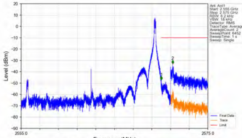
n7_15kHz_SISO_NTNV_15MHz_DFT-s-OFDM PI/2 BPSK_2562.5MHz_Inner_1RB_Right
