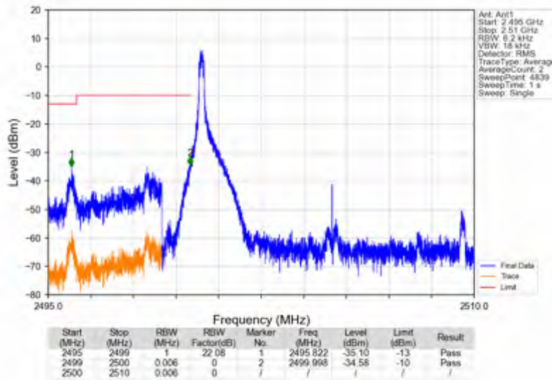
n7_15kHz_SISO_NTNV_10MHz_DFT-s-OFDM QPSK_2505MHz_Edge_1RB_Left
