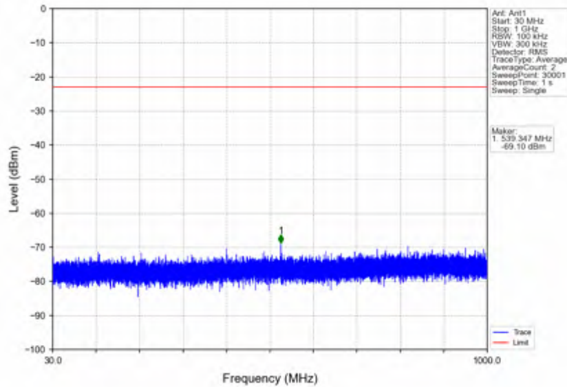
n7_15kHz_SISO_NTNV_5MHz_CP-OFDM QPSK_2502.5MHz_Outer_Full
