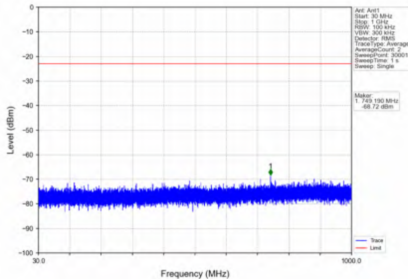
n7_15kHz_SISO_NTV_10MHz_DFT-s-OFDM QPSK_2535MHz_Edge_1RB_Left
