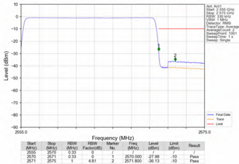
n7_15kHz_SISO_NTV_15MHz_CP-OFDM QPSK_2562.5MHz_Outer_Full
