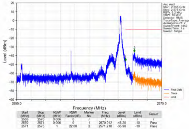
n7_15kHz_SISO_NTV_15MHz_CP-OFDM QPSK_2562.5MHz_Inner_1RB_Right
