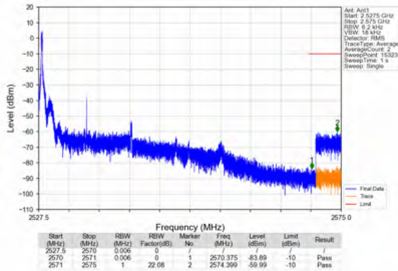
n7_15kHz_SISO_NTNV_15MHz_CP-OFDM QPSK_2535MHz_Edge_1RB_Left
