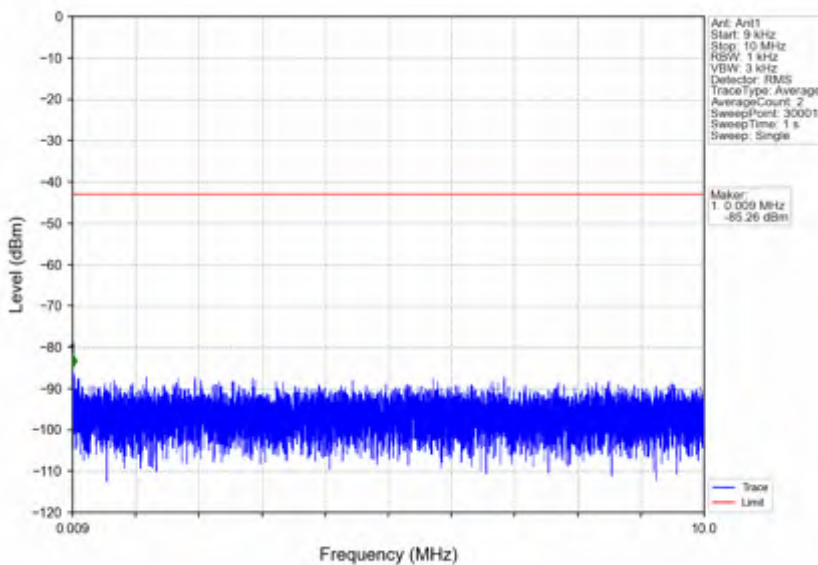
n7_15kHz_SISO_NTNV_10MHz_DFT-s-OFDM QPSK_2505MHz_Outer_Full
