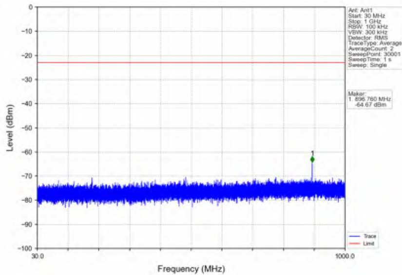
n7_15kHz_SISO_NTV_15MHz_DFT-s-OFDM_QPSK_2562.5MHz_Inner_1RB_Right
