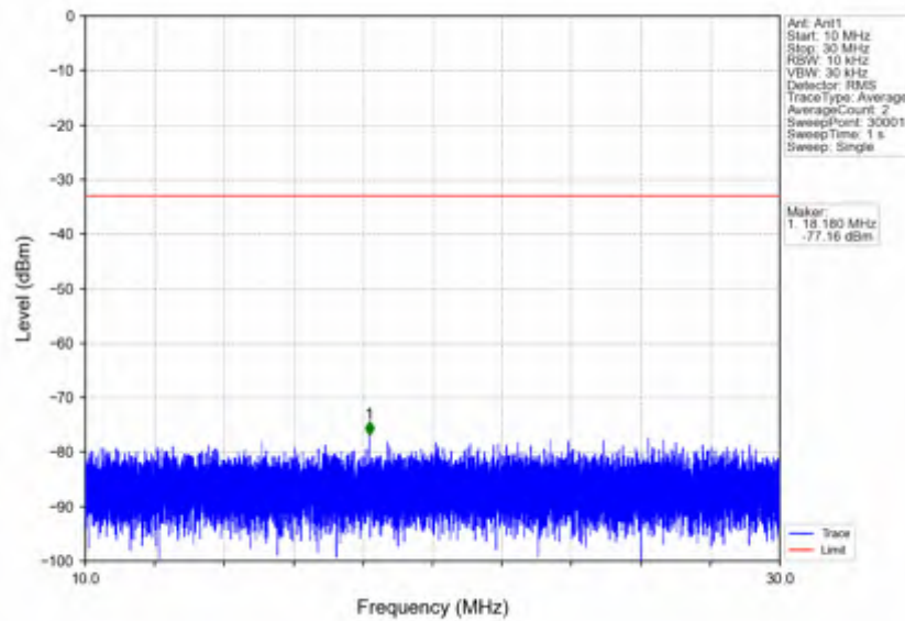
n7_15kHz_SISO_NTV_5MHz_CP-OFDM QPSK_2567.5MHz_Edge_1RB_Right
