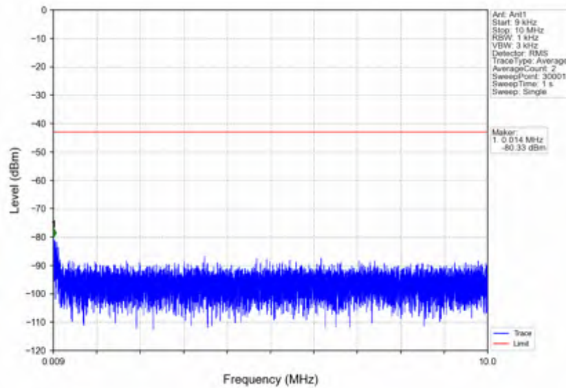
n7_15kHz_SISO_NTNV_5MHz_CP-OFDM QPSK_2535MHz_Edge_1RB_Left
