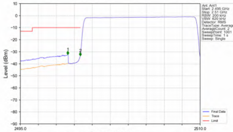
n7_15kHz_SISO_NTNV_10MHz_CP-OFDM QPSK_2505MHz_Outer_Full
