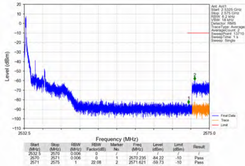
n7_15kHz_SISO_NTNV_5MHz_DFT-s-OFDM QPSK_2535MHz_Edge_1RB_Left
