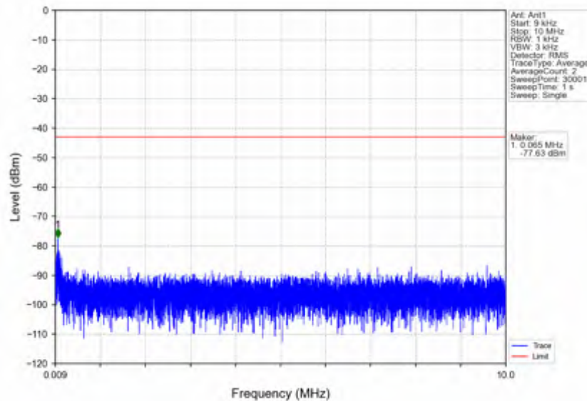
n7_15kHz_SISO_NTV_15MHz_DFT-s-OFDM QPSK_2535MHz_Edge_1RB_Left
