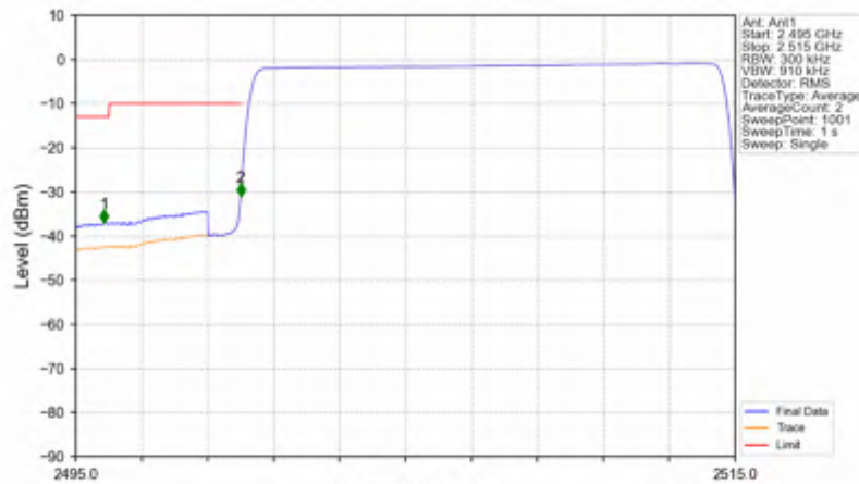
n7_15kHz_SISO_NTNV_15MHz_CP-OFDM QPSK_2507.5MHz_Outer_Full
