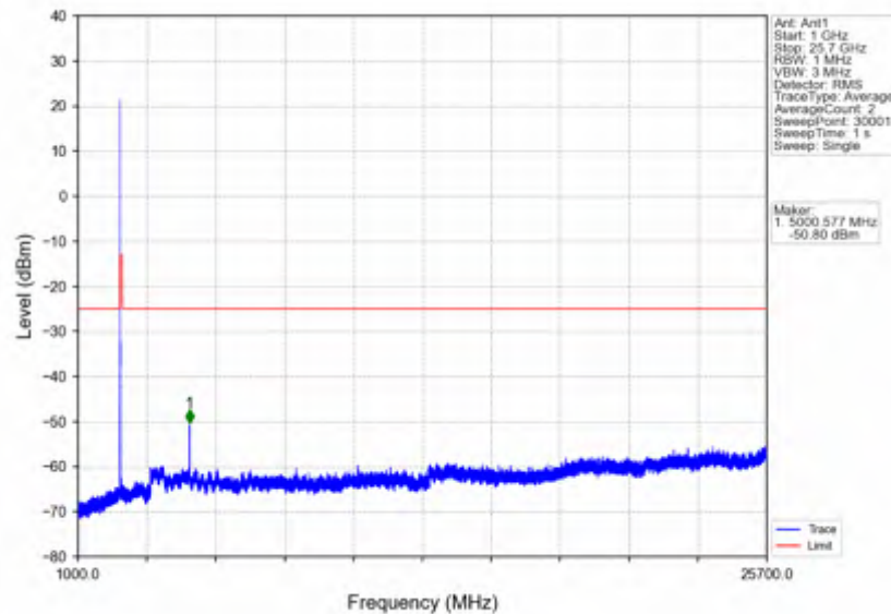
n7_15kHz_SISO_NTV_10MHz_DFT-s-OFDM QPSK_2505MHz_Edge_1RB_Left
