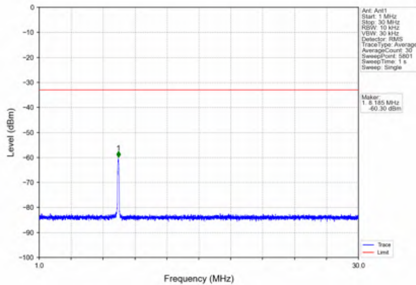
n7_15kHz_SISO_NTNV_20MHz_CP-OFDM QPSK_2560MHz_Edge_1RB_Right
