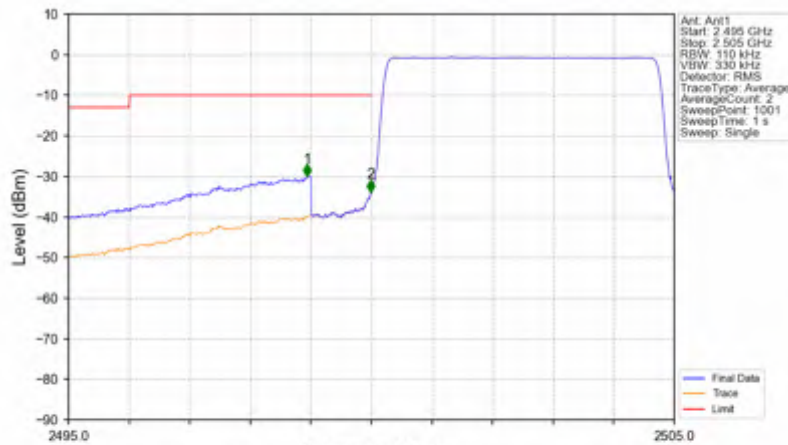
n7_15kHz_SISO_NTNV_5MHz_CP-OFDM QPSK_2502.5MHz_Outer_Full
