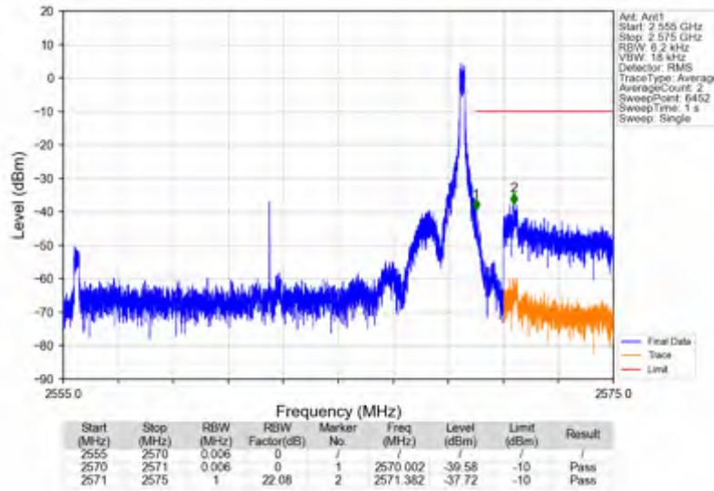
n7_15kHz_SISO_NTNV_15MHz_CP-OFDM QPSK_2562.5MHz_Edge_1RB_Right
