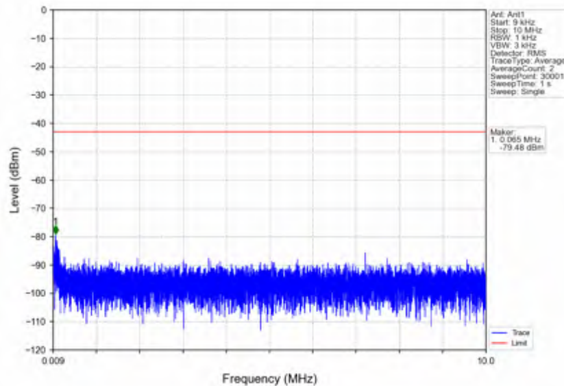
n7_15kHz_SISO_NTNV_20MHz_DFT-s-OFDM QPSK_2535MHz_Edge_1RB_Left
