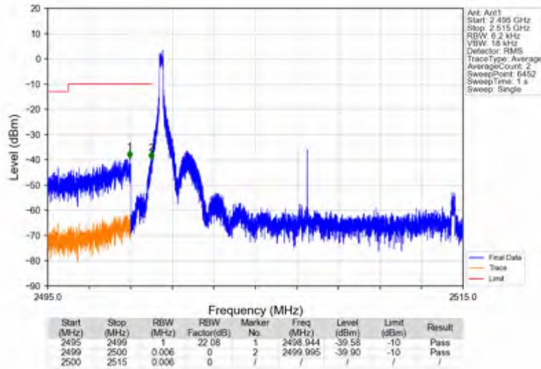
n7_15kHz_SISO_NTNV_15MHz_CP-OFDM QPSK_2507.5MHz_Edge_1RB_Left
