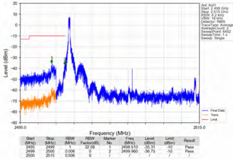
n7_15kHz_SISO_NTNV_15MHz_DFT-s-OFDM PI/2 BPSK_2507.5MHz_Edge_1RB_Left
