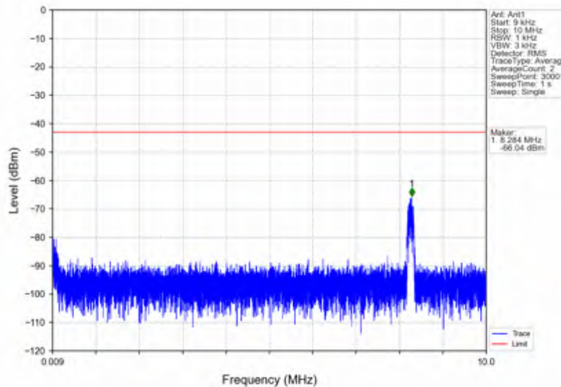
n7_15kHz_SISO_NTNV_15MHz_CP-OFDM QPSK_2562.5MHz_Edge_1RB_Right
