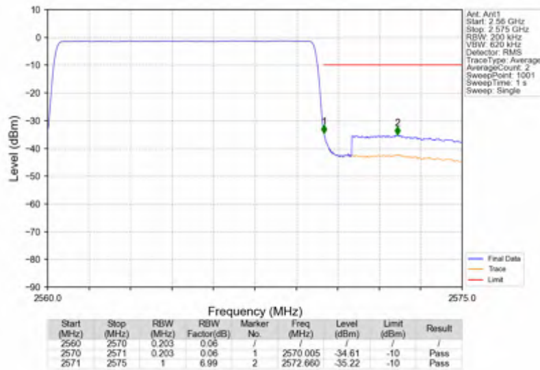
n7_15kHz_SISO_NTNV_10MHz_CP-OFDM QPSK_2565MHz_Outer_Full
