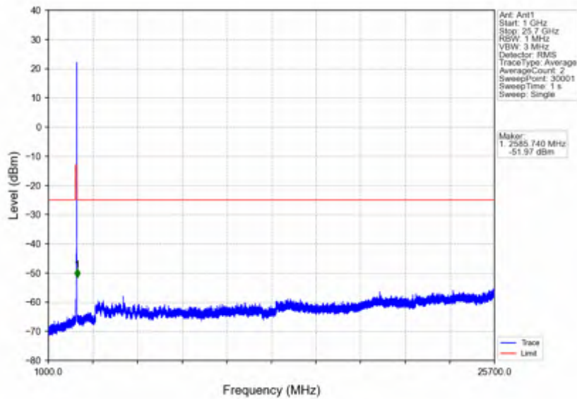
n7_15kHz_SISO_NTNV_15MHz_CP-OFDM QPSK_2562.5MHz_Inner_1RB_Right
