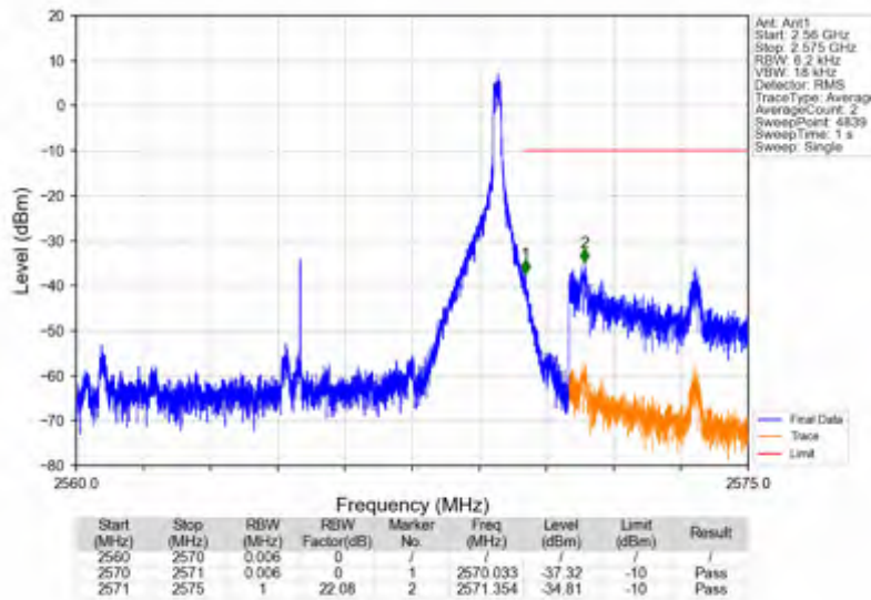
n7_15kHz_SISO_NTNV_10MHz_DFT-s-OFDM QPSK_2565MHz_Inner_1RB_Right
