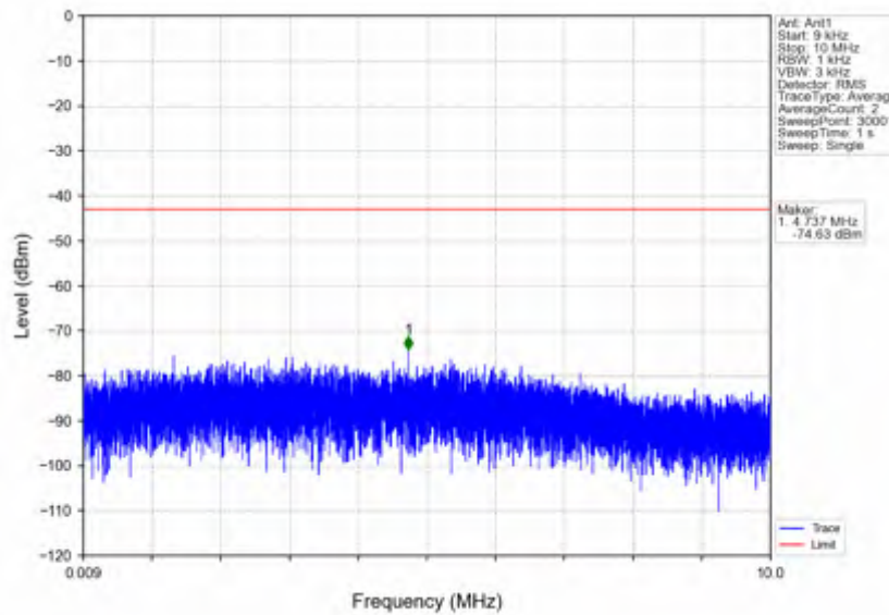
n7_15kHz_SISO_NTNV_10MHz_DFT-s-OFDM QPSK_2565MHz_Outer_Full
