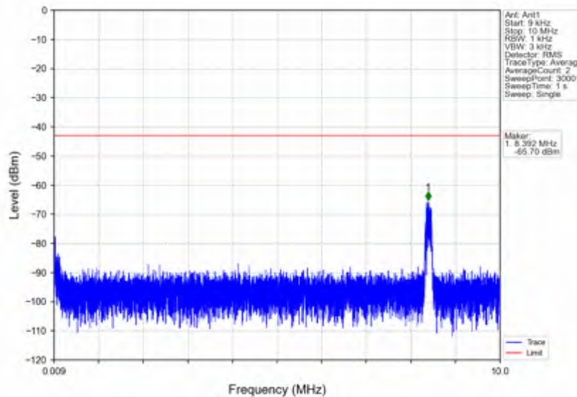
n7_15kHz_SISO_NTV_5MHz_CP-OFDM QPSK_2567.5MHz_Edge_1RB_Right
