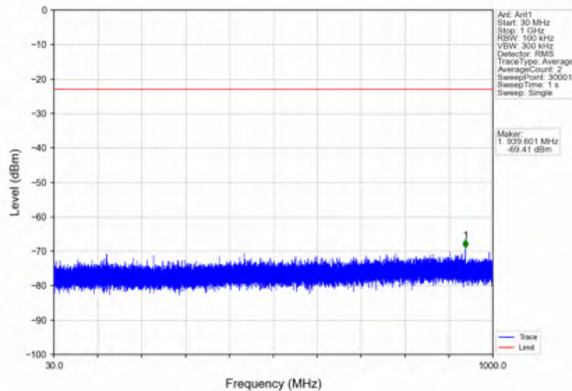
n7_15kHz_SISO_NTV_5MHz_CP-OFDM QPSK_2502.5MHz_Edge_1RB_Left
