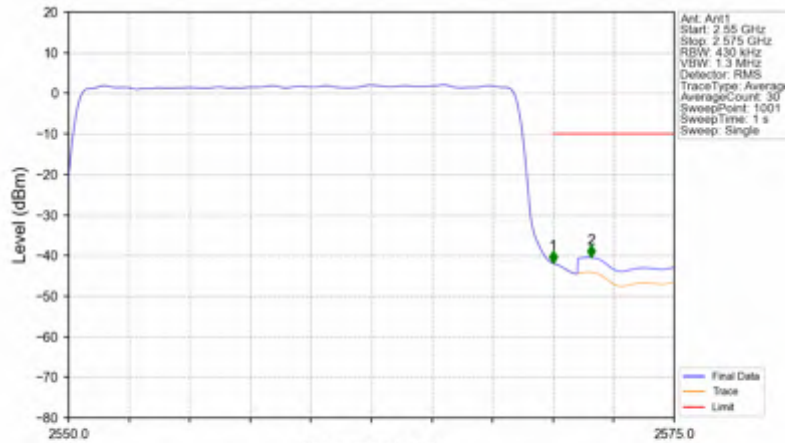
n7_15kHz_SISO_NTNV_20MHz_DFT-s-OFDM PI/2 BPSK_2560MHz_Outer_Full
