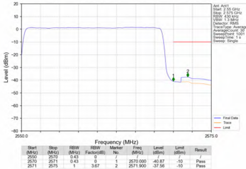
n7_15kHz_SISO_NTNV_20MHz_DFT-s-OFDM QPSK_2560MHz_Outer_Full
