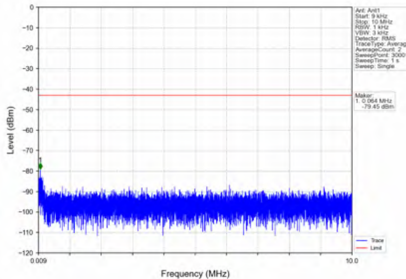
n7_15kHz_SISO_NTV_10MHz_DFT-s-OFDM QPSK_2535MHz_Edge_1RB_Left
