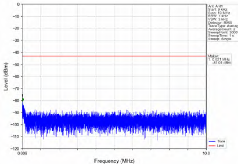
n7_15kHz_SISO_NTV_5MHz_CP-OFDM QPSK_2502.5MHz_Edge_1RB_Left
