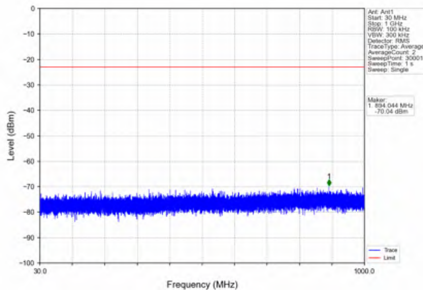
n7_15kHz_SISO_NTV_10MHz_DFT-s-OFDM PI/2 BPSK_2565MHz_Edge_1RB_Right
