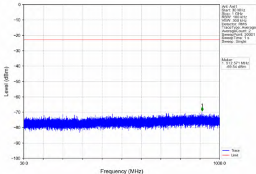
n7_15kHz_SISO_NTNV_10MHz_DFT-s-OFDM QPSK_2565MHz_Inner_1RB_Right
