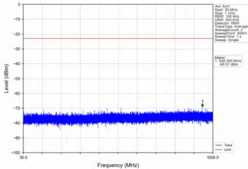
n7_15kHz_SISO_NTNV_5MHz_DFT-s-OFDM QPSK_2535MHz_Edge_1RB_Left
