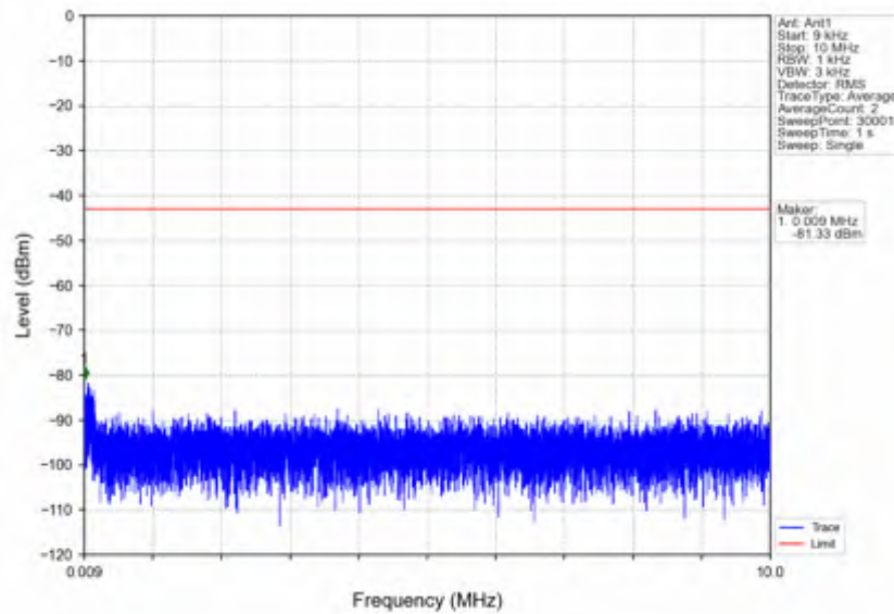
n7_15kHz_SISO_NTV_10MHz_DFT-s-OFDM QPSK_2505MHz_Edge_1RB_Left
