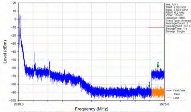
n7_15kHz_SISO_NTV_10MHz_DFT-s-OFDM QPSK_2535MHz_Edge_1RB_Left
