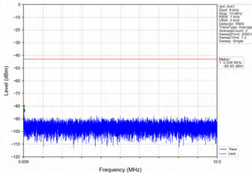
n7_15kHz_SISO_NTNV_20MHz_DFT-s-OFDM_QPSK_2510MHz_Outer_Full
