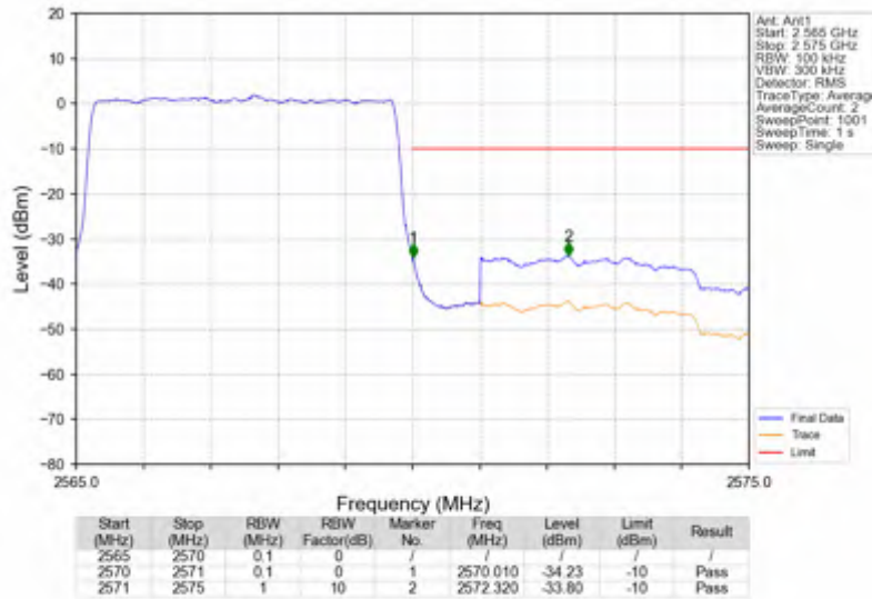
n7_15kHz_SISO_NTNV_5MHz_DFT-s-OFDM QPSK_2567.5MHz_Outer_Full
