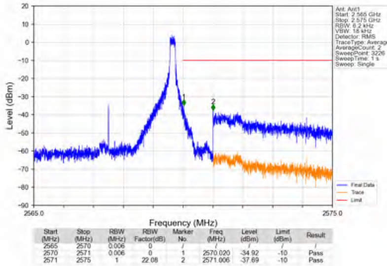
n7_15kHz_SISO_NTV_5MHz_CP-OFDM QPSK_2567.5MHz_Edge_1RB_Right
