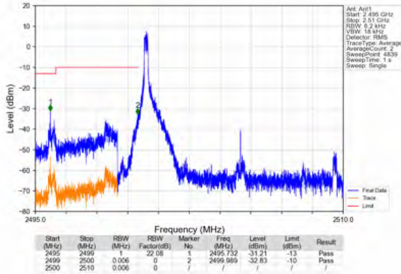
n7_15kHz_SISO_NTNV_10MHz_DFT-s-OFDM_PI/2_BPSK_2505MHz_Edge_1RB_Left
