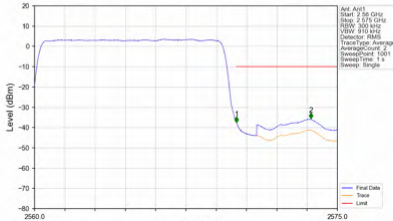
n7_15kHz_SISO_NTNV_10MHz_DFT-s-OFDM PI/2 BPSK_2565MHz_Outer_Full
