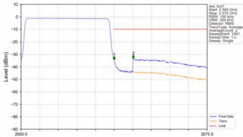
n7_15kHz_SISO_NTNV_5MHz_CP-OFDM QPSK_2567.5MHz_Outer_Full
