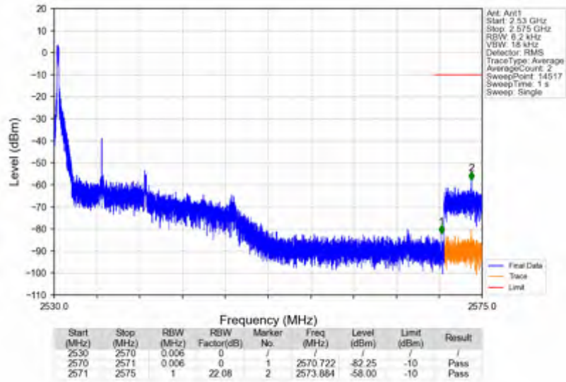
n7_15kHz_SISO_NTNV_10MHz_CP-OFDM QPSK_2535MHz_Edge_1RB_Left
