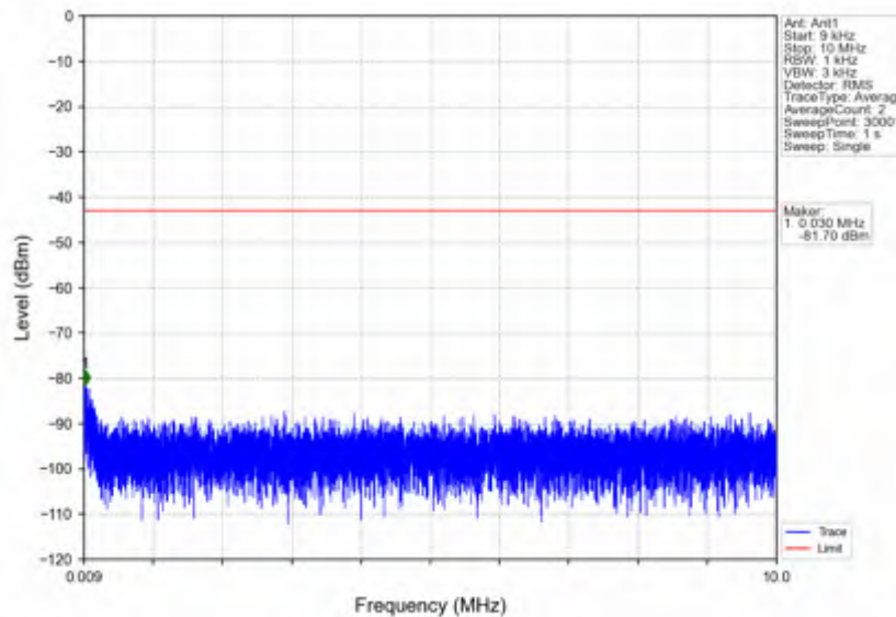
n7_15kHz_SISO_NTNV_10MHz_CP-OFDM QPSK_2505MHz_Edge_1RB_Left
