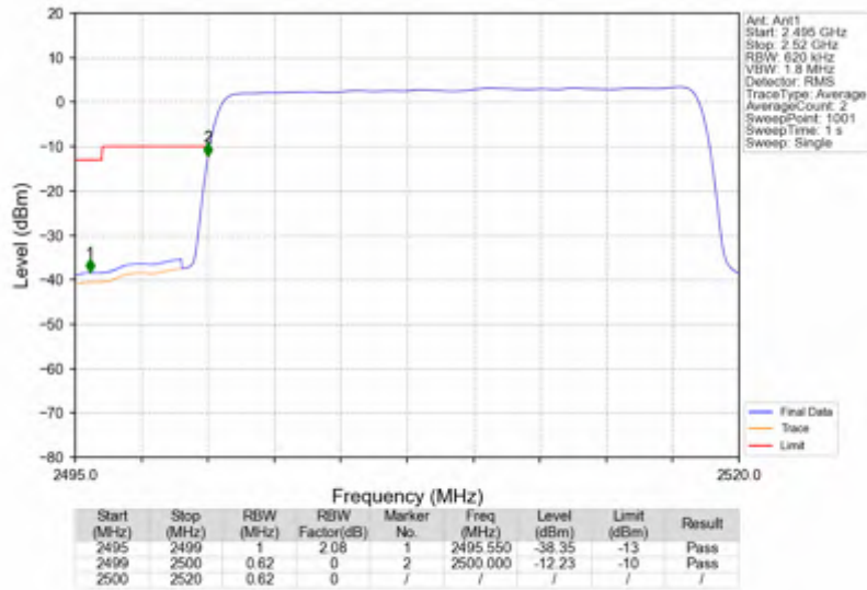
n7_15kHz_SISO_NTNV_20MHz_DFT-s-OFDM_QPSK_2510MHz_Outer_Full
