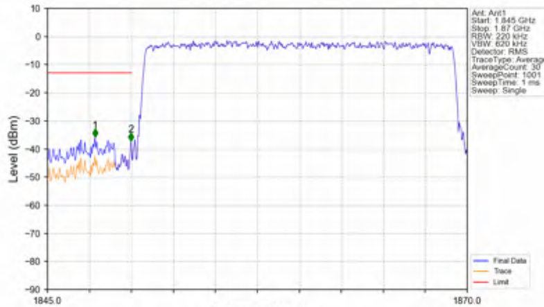
n2_30kHz_SISO_NTNV_20MHz_CP-OFDM QPSK_1860MHz_Outer_Full
