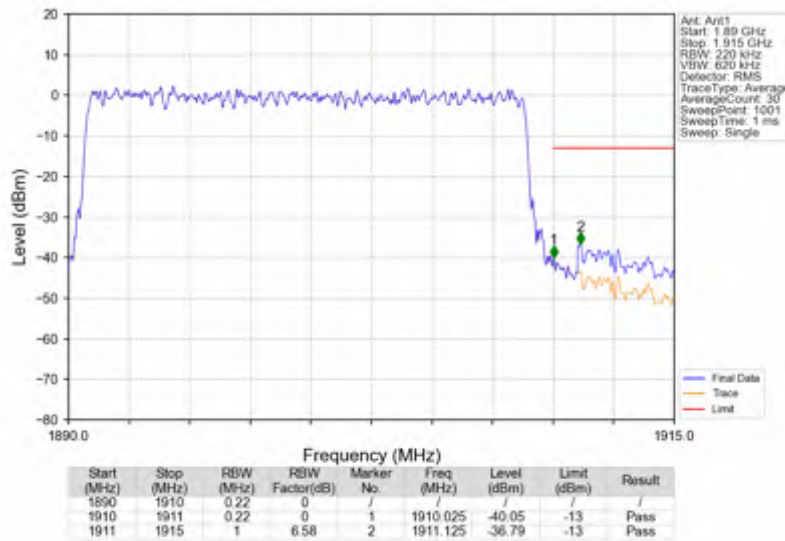
n2_30kHz_SISO_NTNV_20MHz_DFT-s-OFDM PI/2 BPSK_1900MHz_Outer_Full
