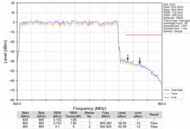
n5_15kHz_SISO_NTNV_15MHz_DFT-s-OFDM QPSK_841.5MHz_Outer_Full
