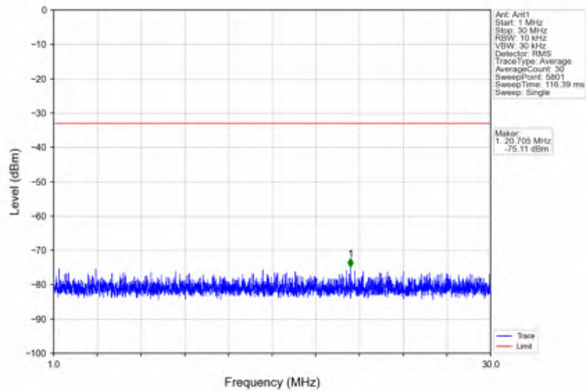
n5_15kHz_SISO_NTNV_10MHz_CP-OFDM QPSK_836.5MHz_Edge_1RB_Left
