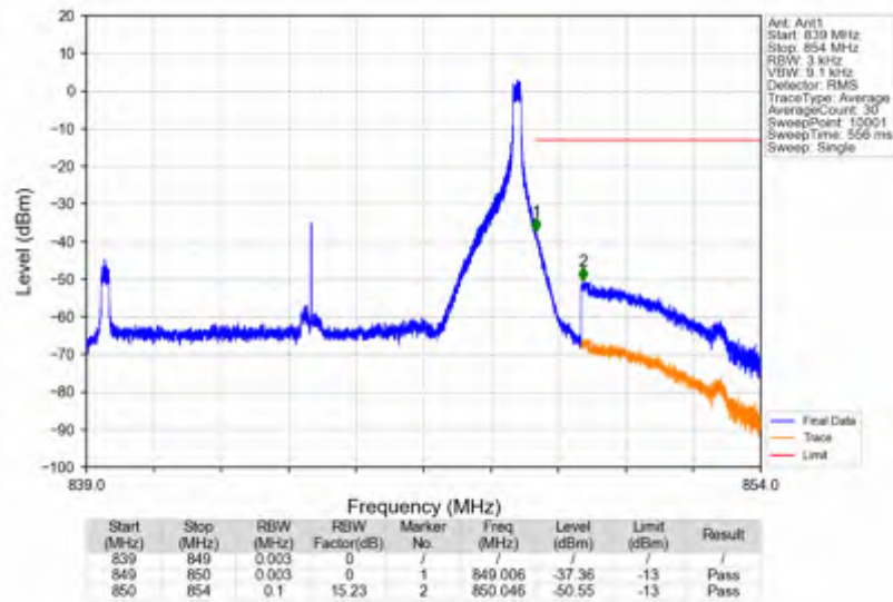
n5_15kHz_SISO_NTNV_10MHz_CP-OFDM QPSK_844MHz_Edge_1RB_Right
