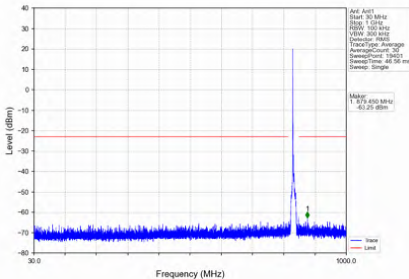
n5_15kHz_SISO_NTNV_5MHz_DFT-s-OFDM QPSK_836.5MHz_Edge_1RB_Left
