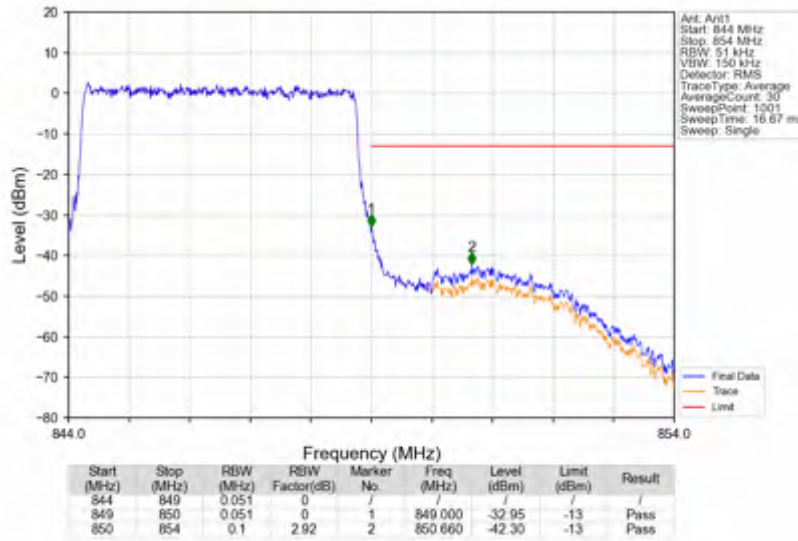
n5_15kHz_SISO_NTNV_5MHz_DFT-s-OFDM PI/2 BPSK_846.5MHz_Outer_Full
