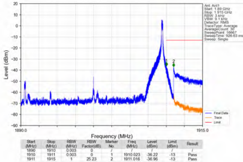
n2_15kHz_SISO_NTNV_20MHz_DFT-s-OFDM QPSK_1900MHz_Edge_1RB_Right
