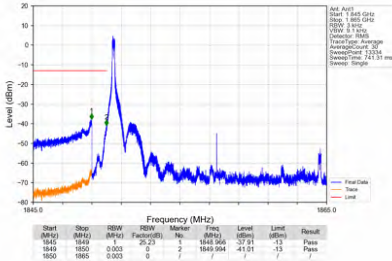
n2_15kHz_SISO_NTNV_15MHz_DFT-s-OFDM QPSK_1857.5MHz_Edge_1RB_Left
