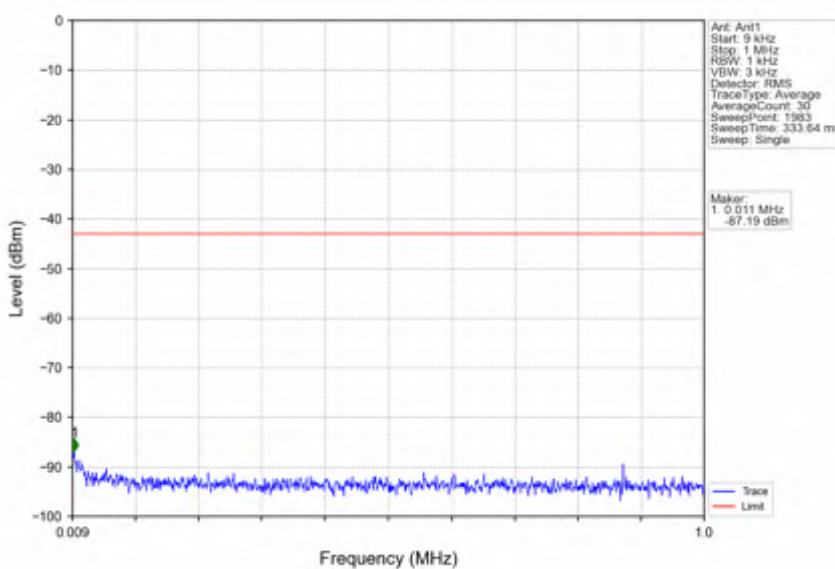
n2_30kHz_SISO_NTNV_10MHz_DFT-s-OFDM QPSK_1905MHz_Outer_Full
