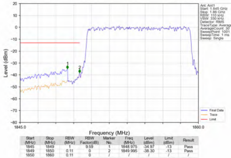
n2_30kHz_SISO_NTNV_10MHz_DFT-s-OFDM_QPSK_1855MHz_Outer_Full
