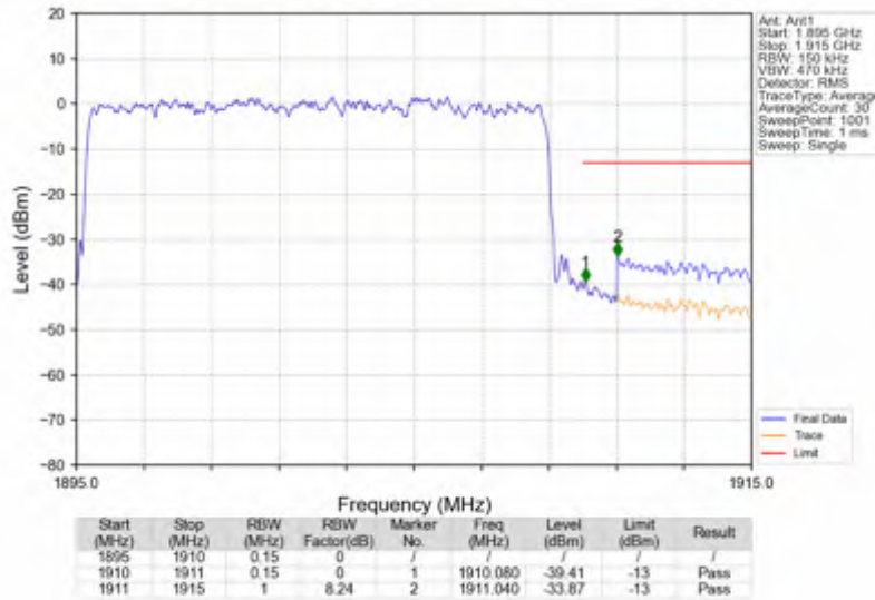
n2_15kHz_SISO_NTNV_15MHz_DFT-s-OFDM QPSK_1902.5MHz_Outer_Full
