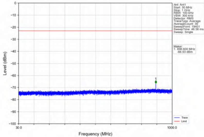
n2_30kHz_SISO_NTNV_10MHz_DFT-s-OFDM QPSK_1905MHz_Edge_1RB_Right
