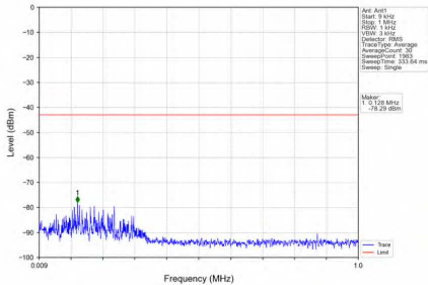
n2_30kHz_SISO_NTNV_15MHz_DFT-s-OFDM QPSK_1857.5MHz_Edge_1RB_Left
