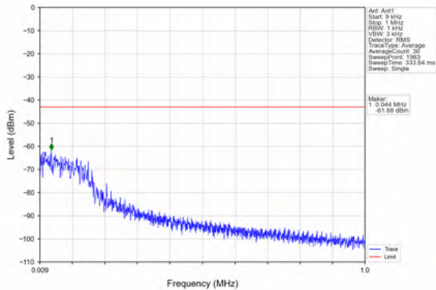
n2_15kHz_SISO_NTNV_20MHz_CP-OFDM QPSK_1900MHz_Edge_1RB_Right
