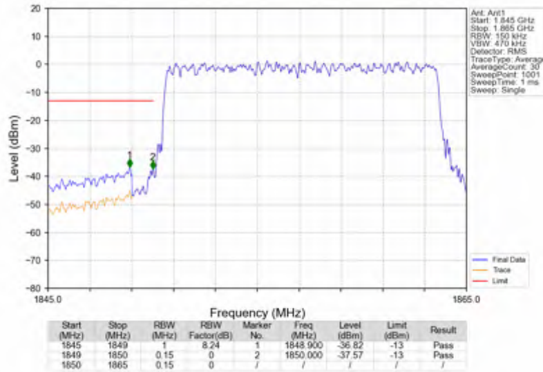
n2_30kHz_SISO_NTNV_15MHz_DFT-s-OFDM QPSK_1857.5MHz_Outer_Full
