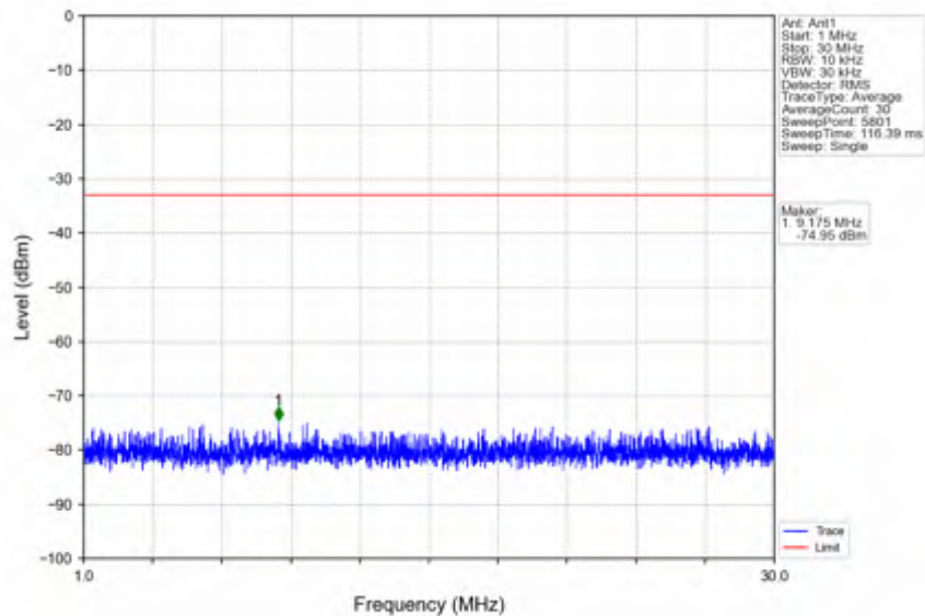
n2_15kHz_SISO_NTNV_5MHz_DFT-s-OFDM QPSK_1907.5MHz_Edge_1RB_Right
