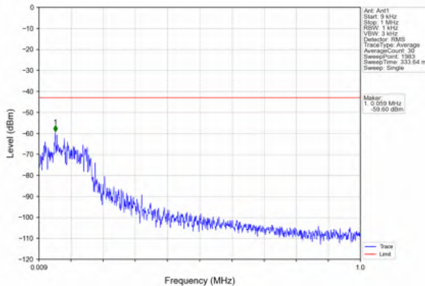
n2_15kHz_SISO_NTNV_5MHz_DFT-s-OFDM QPSK_1852.5MHz_Edge_1RB_Left
