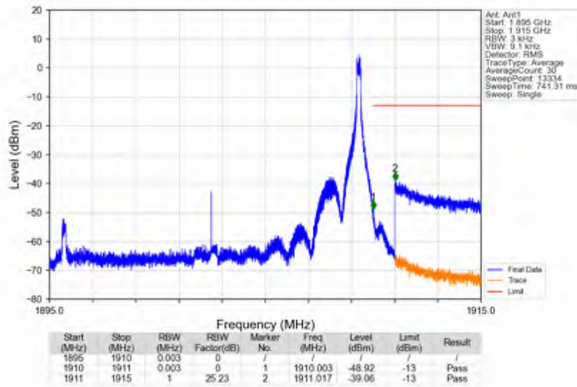
n2_15kHz_SISO_NTNV_15MHz_CP-OFDM QPSK_1902.5MHz_Inner_1RB_Right
