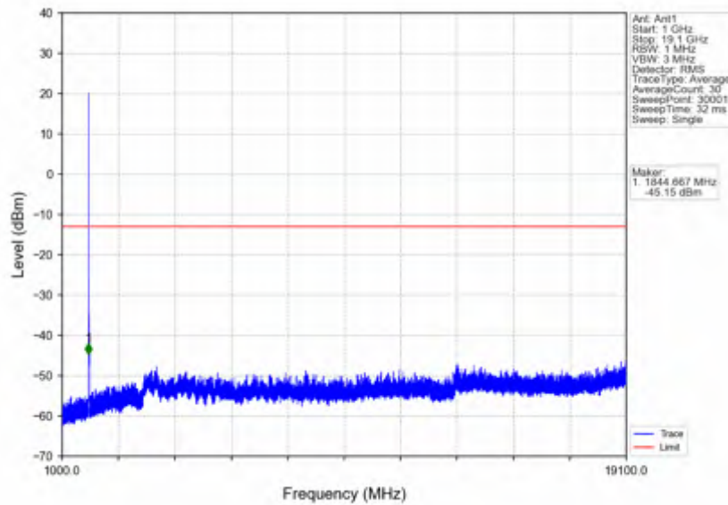
n2_15kHz_SISO_NTNV_15MHz_CP-OFDM QPSK_1857.5MHz_Outer_Full
