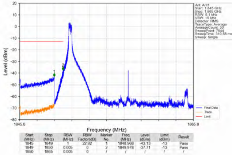
n2_30kHz_SISO_NTNV_15MHz_DFT-s-OFDM_PI/2_BPSK_1857.5MHz_Edge_1RB_Left
