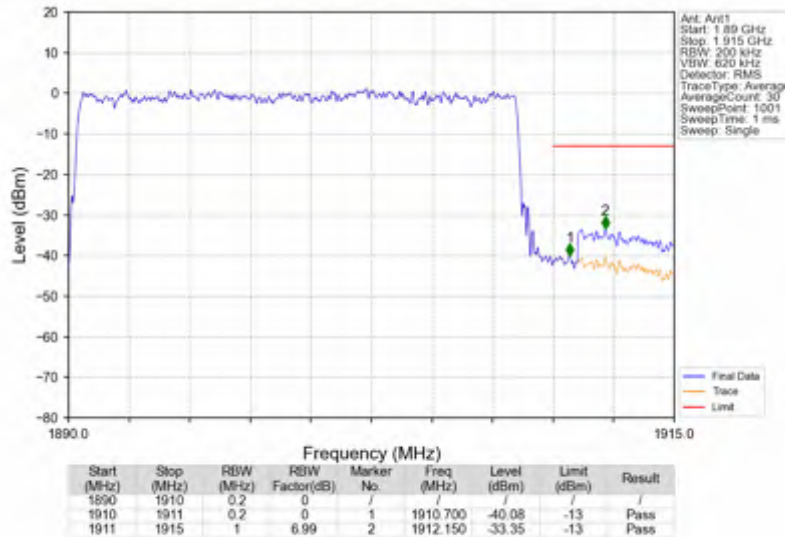
n2_15kHz_SISO_NTNV_20MHz_DFT-s-OFDM QPSK_1900MHz_Outer_Full
