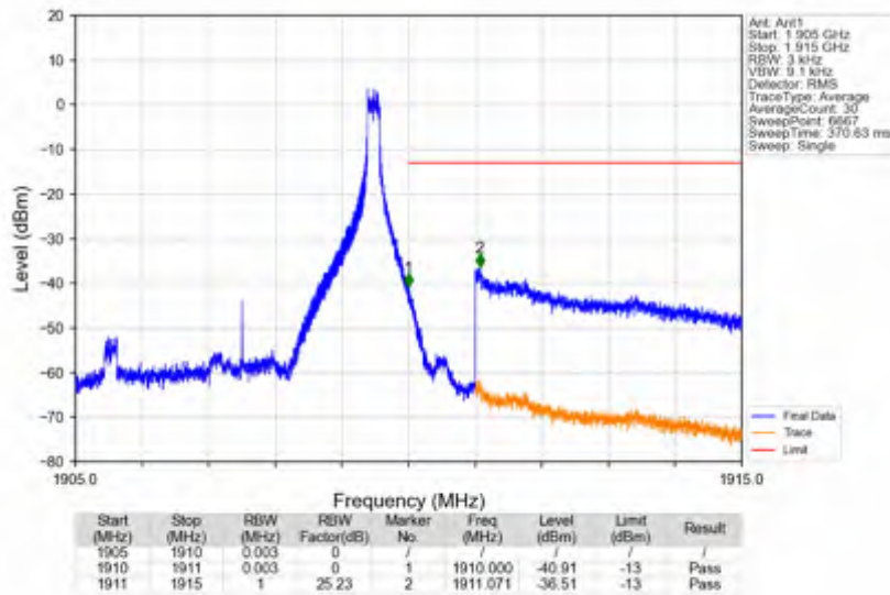
n2_15kHz_SISO_NTNV_5MHz_CP-OFDM QPSK_1907.5MHz_Inner_1RB_Right
