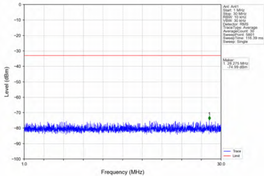
n2_15kHz_SISO_NTNV_5MHz_DFT-s-OFDM QPSK_1852.5MHz_Edge_1RB_Left
