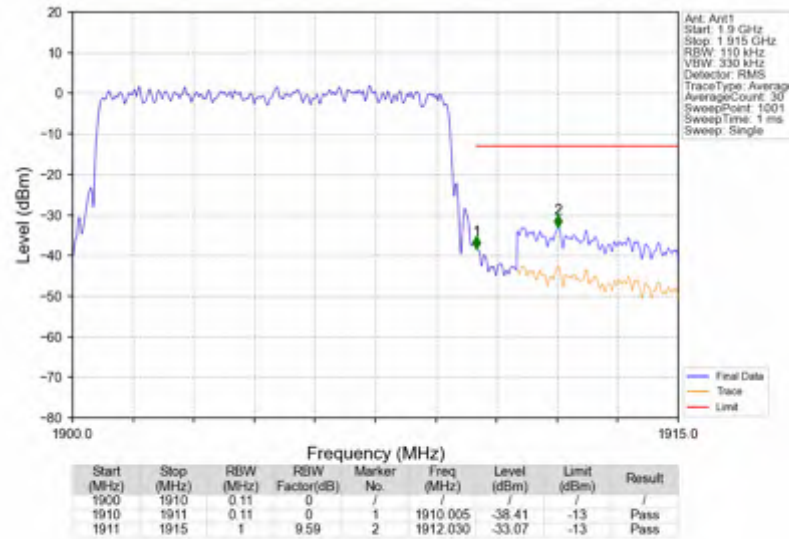
n2_30kHz_SISO_NTNV_10MHz_DFT-s-OFDM QPSK_1905MHz_Outer_Full
