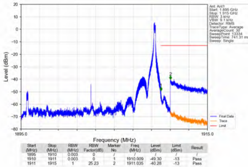
n2_15kHz_SISO_NTNV_15MHz_DFT-s-OFDM QPSK_1902.5MHz_Inner_1RB_Right
