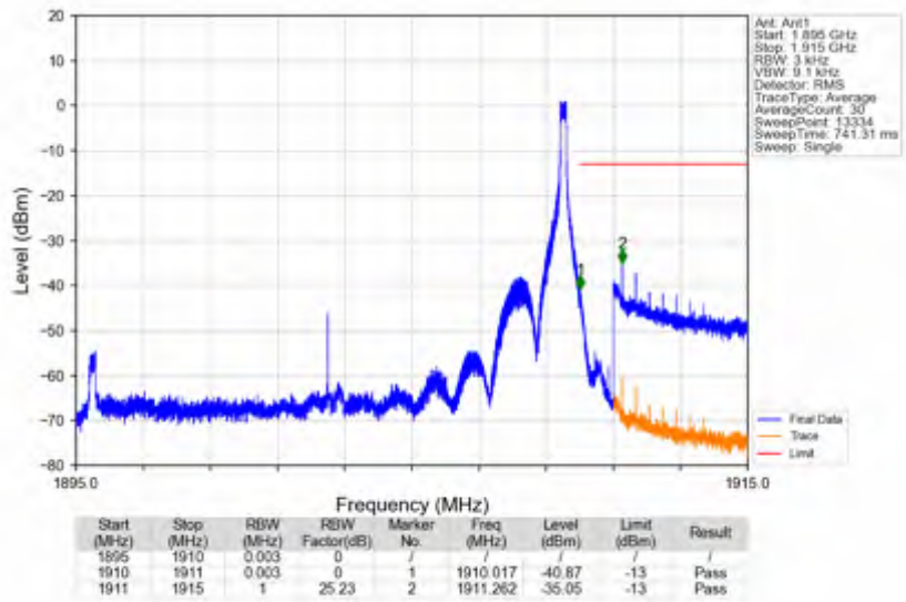
n2_15kHz_SISO_NTNV_15MHz_CP-OFDM QPSK_1902.5MHz_Edge_1RB_Right
