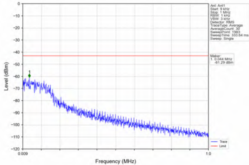
n2_15kHz_SISO_NTV_5MHz_CP-OFDM QPSK_1907.5MHz_Edge_1RB_Right
