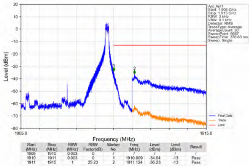
n2_15kHz_SISO_NTNV_5MHz_DFT-s-OFDM QPSK_1907.5MHz_Edge_1RB_Right
