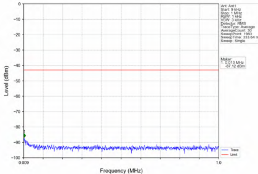
n2_30kHz_SISO_NTNV_10MHz_DFT-s-OFDM_QPSK_1855MHz_Outer_Full
