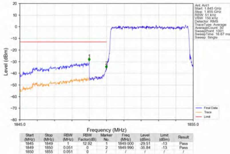
n2_15kHz_SISO_NTNV_5MHz_DFT-s-OFDM QPSK_1852.5MHz_Outer_Full
