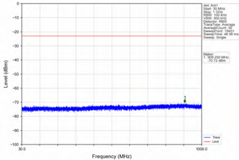
n2_30kHz_SISO_NTNV_15MHz_DFT-s-OFDM QPSK_1857.5MHz_Edge_1RB_Left
