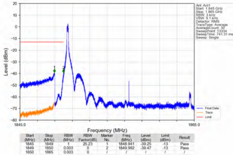
n2_15kHz_SISO_NTNV_15MHz_CP-OFDM QPSK_1857.5MHz_Edge_1RB_Left
