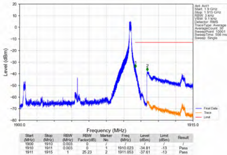
n2_15kHz_SISO_NTNV_10MHz_DFT-s-OFDM QPSK_1905MHz_Edge_1RB_Right
