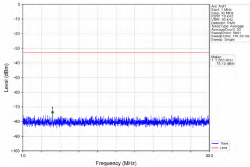
n2_15kHz_SISO_NTNV_15MHz_CP-OFDM QPSK_1880MHz_Edge_1RB_Left
