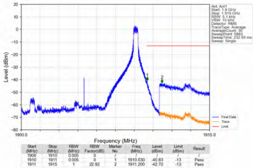
n2_30kHz_SISO_NTNV_10MHz_DFT-s-OFDM QPSK_1905MHz_Edge_1RB_Right
