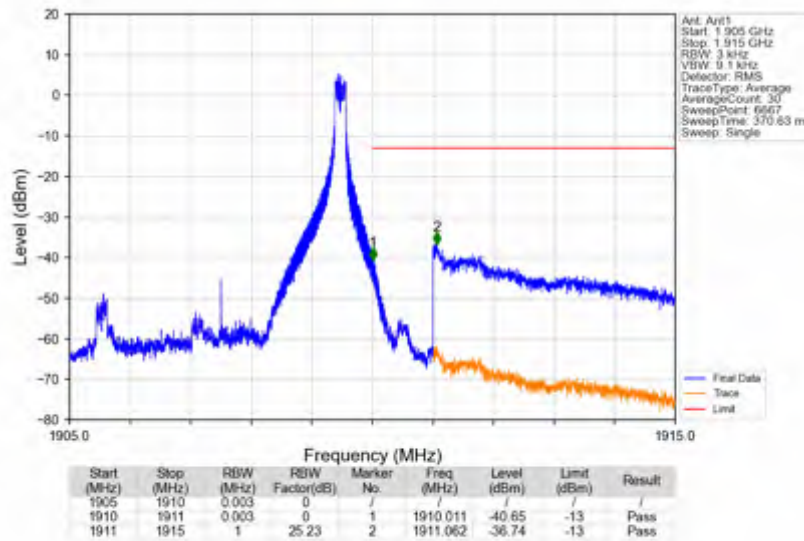
n2_15kHz_SISO_NTNV_5MHz_DFT-s-OFDM QPSK_1907.5MHz_Inner_1RB_Right
