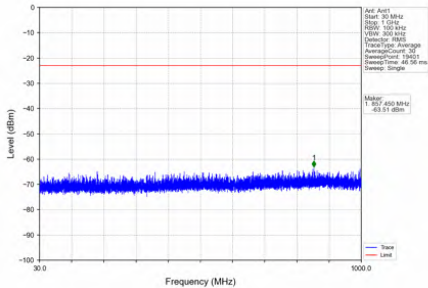
n2_15kHz_SISO_NTNV_10MHz_CP-OFDM QPSK_1905MHz_Edge_1RB_Right
