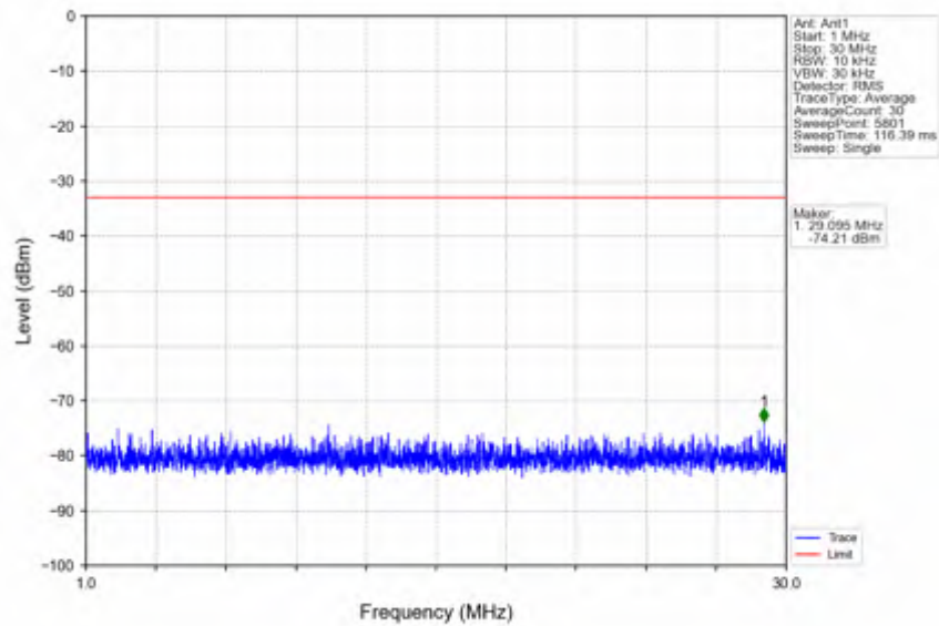
n2_15kHz_SISO_NTV_15MHz_DFT-s-OFDM QPSK_1880MHz_Edge_1RB_Left
