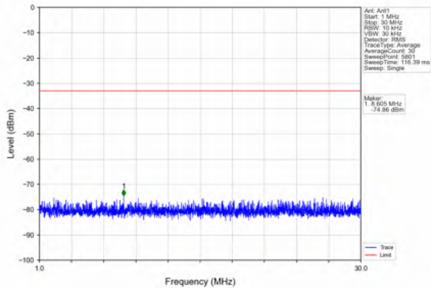
n2_15kHz_SISO_NTNV_5MHz_CP-OFDM QPSK_1852.5MHz_Edge_1RB_Left
