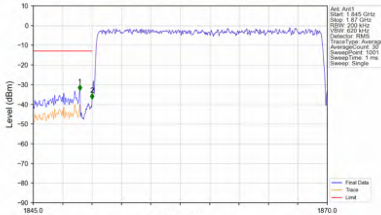
n2_15kHz_SISO_NTNV_20MHz_CP-OFDM QPSK_1860MHz_Outer_Full
