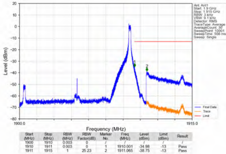
n2_15kHz_SISO_NTNV_10MHz_CP-OFDM QPSK_1905MHz_Edge_1RB_Right
