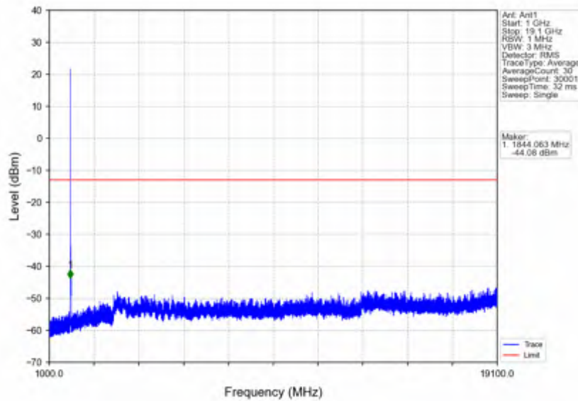
n2_15kHz_SISO_NTNV_15MHz_DFT-s-OFDM QPSK_1857.5MHz_Outer_Full
