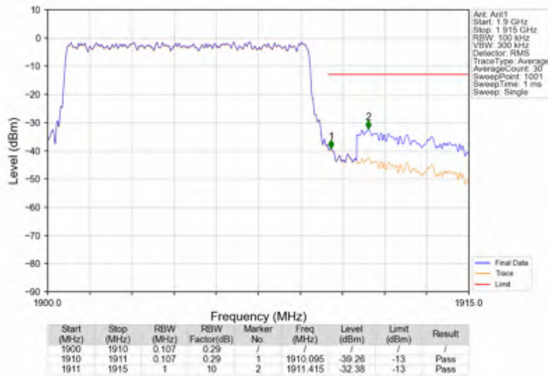
n2_30kHz_SISO_NTNV_10MHz_CP-OFDM QPSK_1905MHz_Outer_Full
