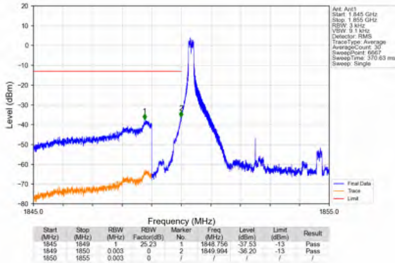
n2_15kHz_SISO_NTNV_5MHz_DFT-s-OFDM QPSK_1852.5MHz_Edge_1RB_Left
