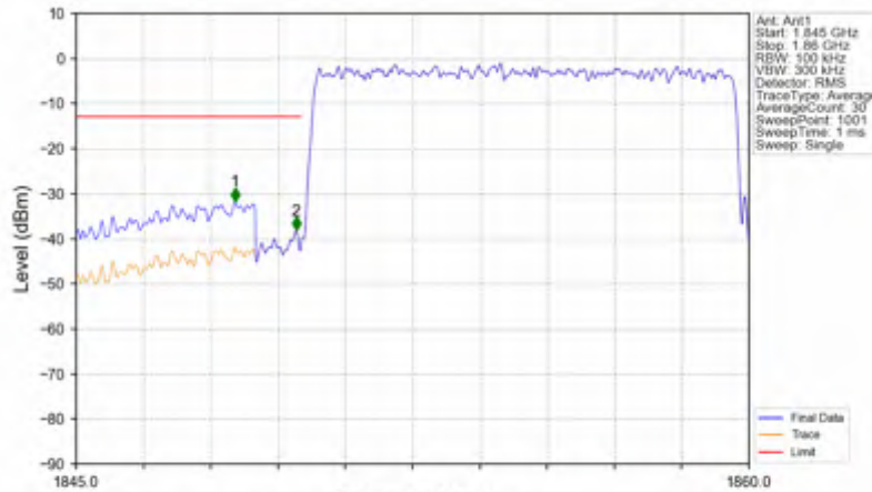
n2_15kHz_SISO_NTNV_10MHz_CP-OFDM QPSK_1855MHz_Outer_Full
