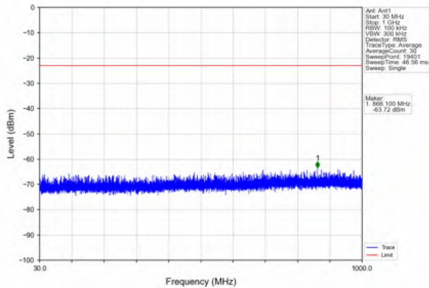
n2_15kHz_SISO_NTNV_5MHz_CP-OFDM QPSK_1907.5MHz_Edge_1RB_Right
