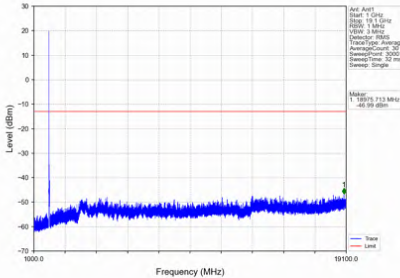
n2_15kHz_SISO_NTNV_20MHz_CP-OFDM QPSK_1900MHz_Edge_1RB_Right
