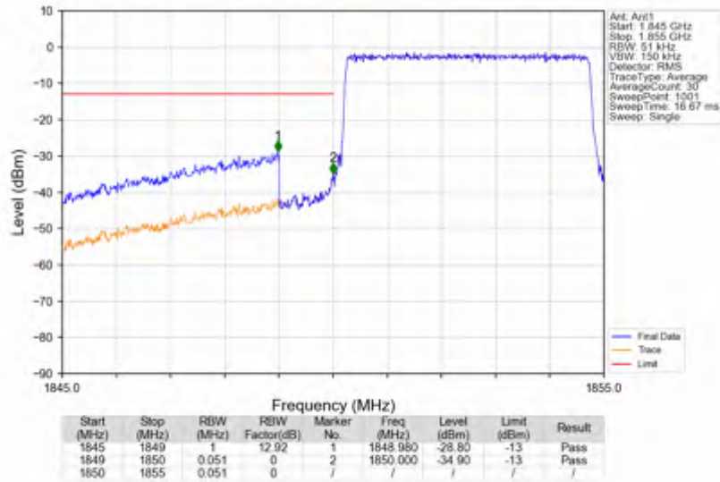
n2_15kHz_SISO_NTNV_5MHz_CP-OFDM QPSK_1852.5MHz_Outer_Full
