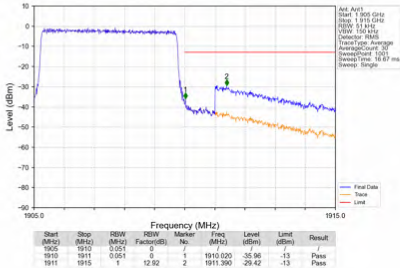
n2_15kHz_SISO_NTNV_5MHz_CP-OFDM QPSK_1907.5MHz_Outer_Full
