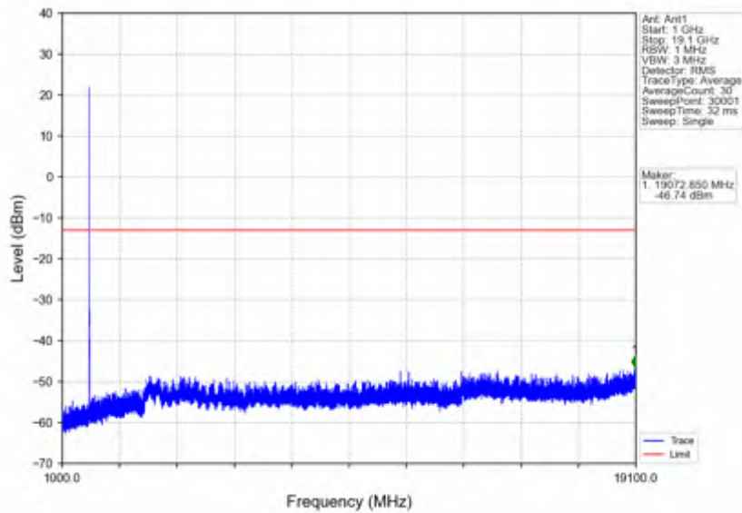
n2_15kHz_SISO_NTV_10MHz_DFT-s-OFDM QPSK_1855MHz_Outer_Full
