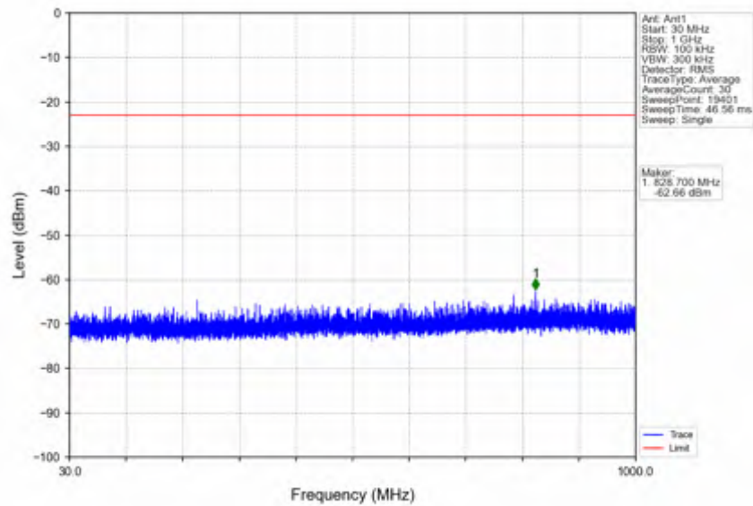
n2_15kHz_SISO_NTNV_20MHz_CP-OFDM QPSK_1900MHz_Edge_1RB_Right
