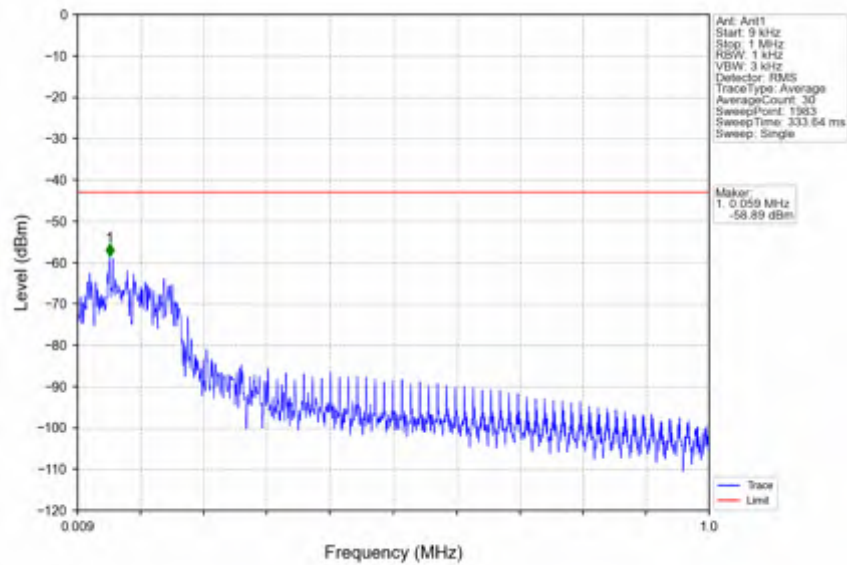
n2_15kHz_SISO_NTV_15MHz_DFT-s-OFDM QPSK_1902.5MHz_Edge_1RB_Right
