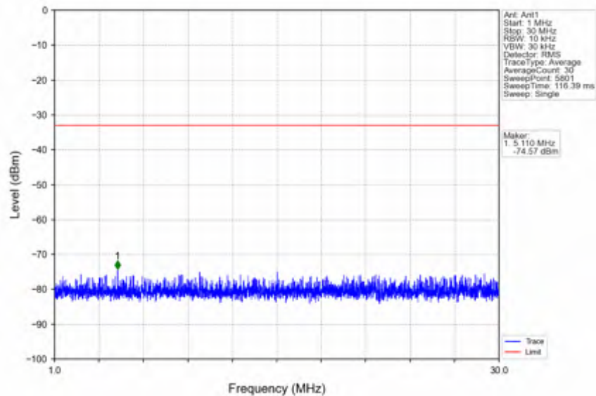
n2_15kHz_SISO_NTNV_10MHz_CP-OFDM QPSK_1905MHz_Edge_1RB_Right
