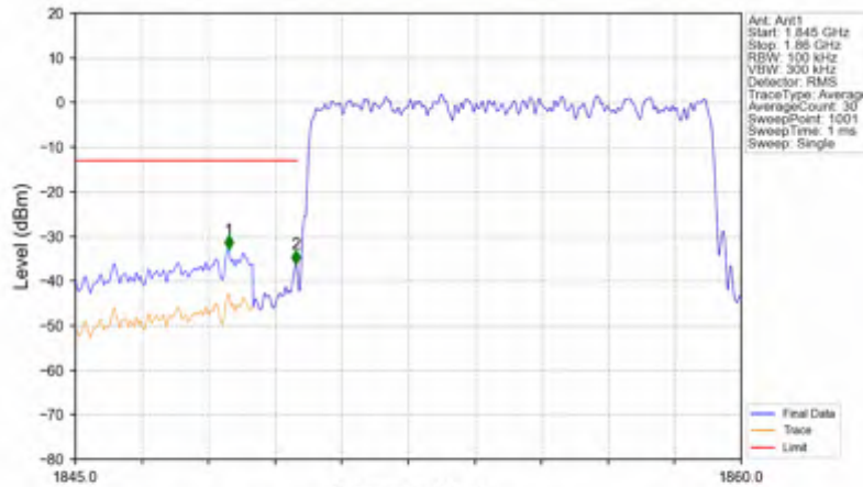
n2_15kHz_SISO_NTV_10MHz_DFT-s-OFDM QPSK_1855MHz_Outer_Full
