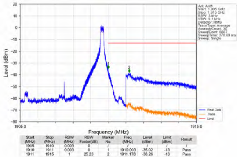
n2_15kHz_SISO_NTNV_5MHz_CP-OFDM QPSK_1907.5MHz_Edge_1RB_Right
