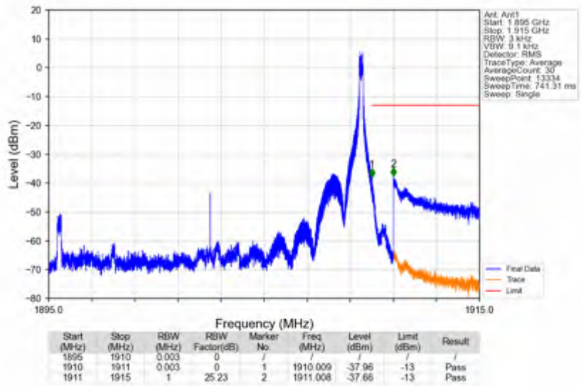
n2_15kHz_SISO_NTV_15MHz_DFT-s-OFDM QPSK_1902.5MHz_Edge_1RB_Right
