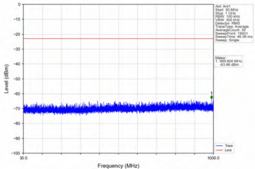
n2_15kHz_SISO_NTNV_15MHz_CP-OFDM QPSK_1857.5MHz_Edge_1RB_Left
