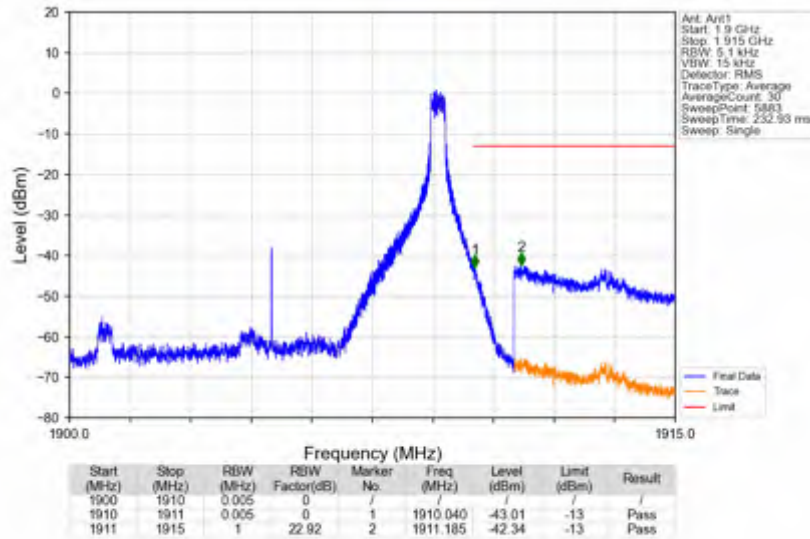
n2_30kHz_SISO_NTNV_10MHz_CP-OFDM QPSK_1905MHz_Edge_1RB_Right
