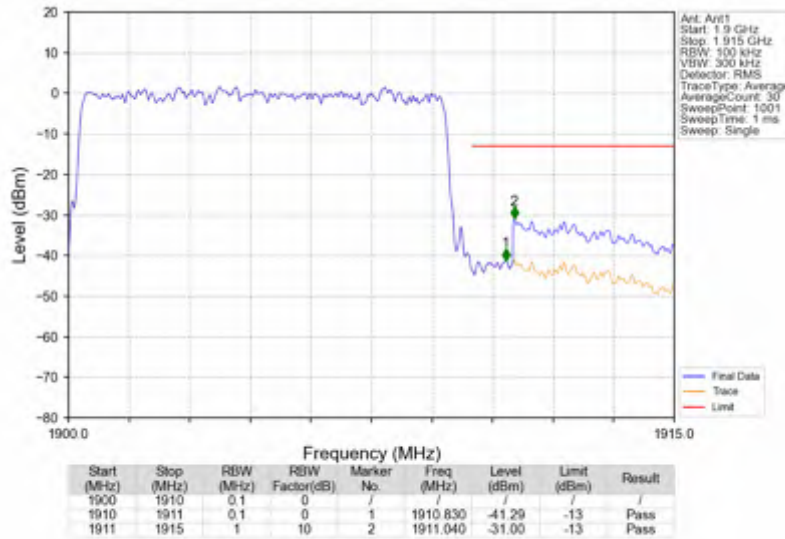
n2_15kHz_SISO_NTNV_10MHz_DFT-s-OFDM QPSK_1905MHz_Outer_Full
