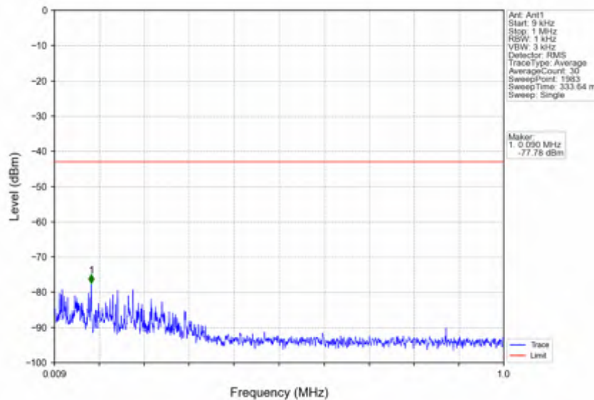
n2_30kHz_SISO_NTNV_10MHz_CP-OFDM QPSK_1905MHz_Edge_1RB_Right
