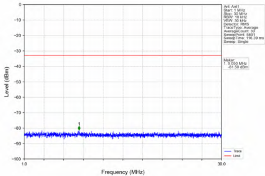
n2_30kHz_SISO_NTNV_15MHz_DFT-s-OFDM QPSK_1857.5MHz_Outer_Full
