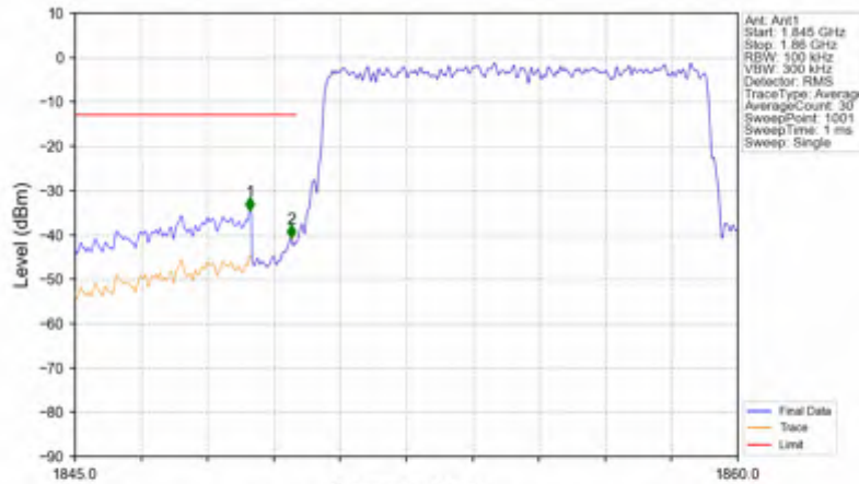
n2_30kHz_SISO_NTNV_10MHz_CP-OFDM QPSK_1855MHz_Outer_Full
