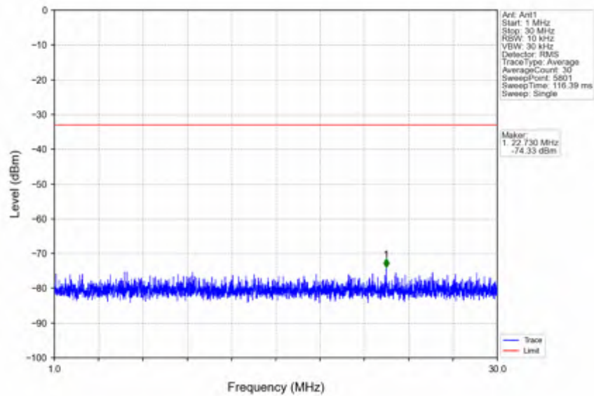
n2_15kHz_SISO_NTNV_5MHz_DFT-s-OFDM QPSK_1880MHz_Edge_1RB_Left
