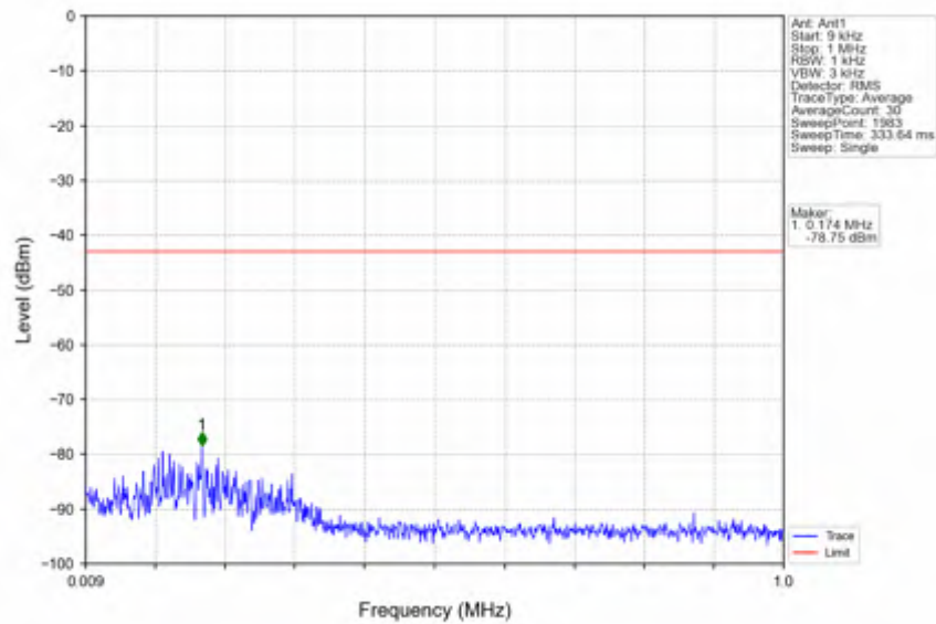
n2_30kHz_SISO_NTNV_10MHz_DFT-s-OFDM QPSK_1905MHz_Edge_1RB_Right
