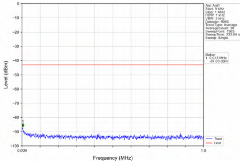
n2_30kHz_SISO_NTNV_15MHz_DFT-s-OFDM QPSK_1857.5MHz_Outer_Full
