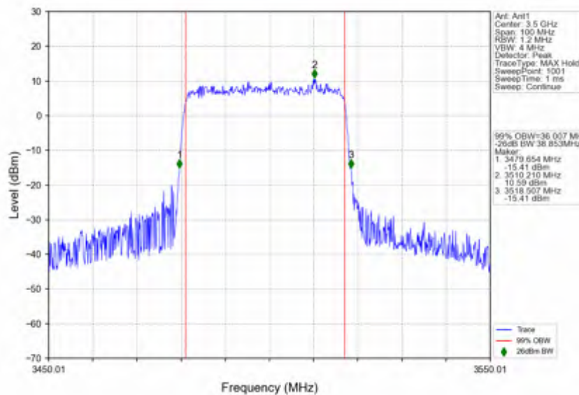
n78e_30kHz_SISO_NTNV_40MHz_DFT-s-OFDM_256_QAM_3500.01MHz_Outer_Full
