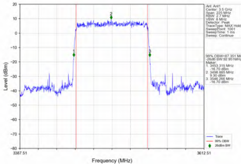
n78e_30kHz_SISO_NTNV_90MHz_DFT-s-OFDM PI/2 BPSK_3500.01MHz_Outer_Full
