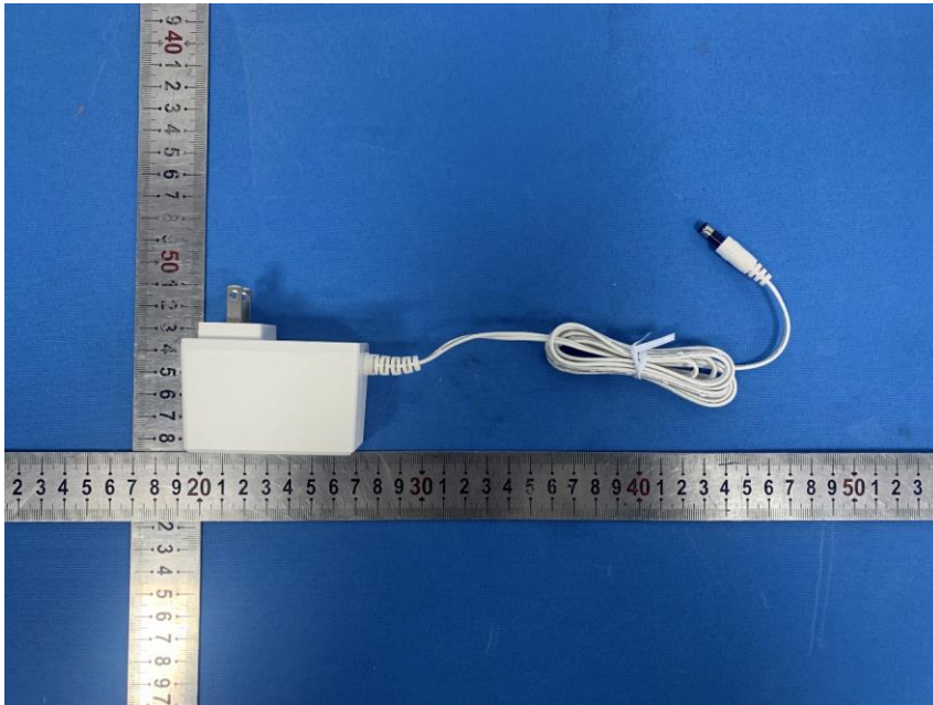
Adapter 2
