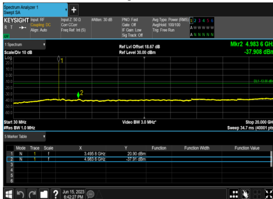
N77(10M)_DFT-s-OFDM_BPSK_Edge_1RB_Left_Mid_CH
