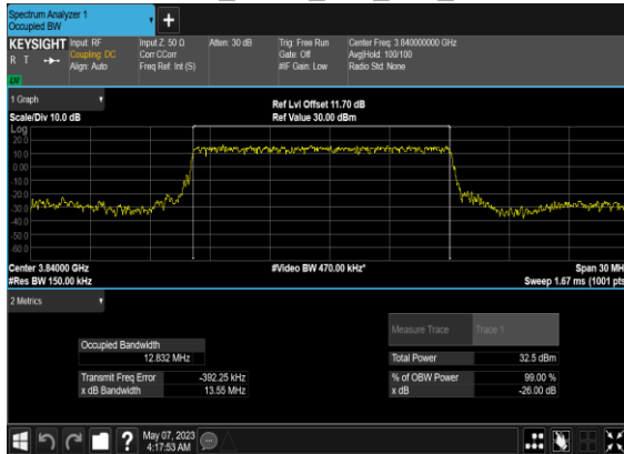
N77(15M)_DFT-s-OFDM_PI_2-BPSK_Outer_Full_Mid_CH
