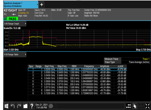
N48(20M)_CP-OFDM_QPSK_Outer_Full_Low_CH
