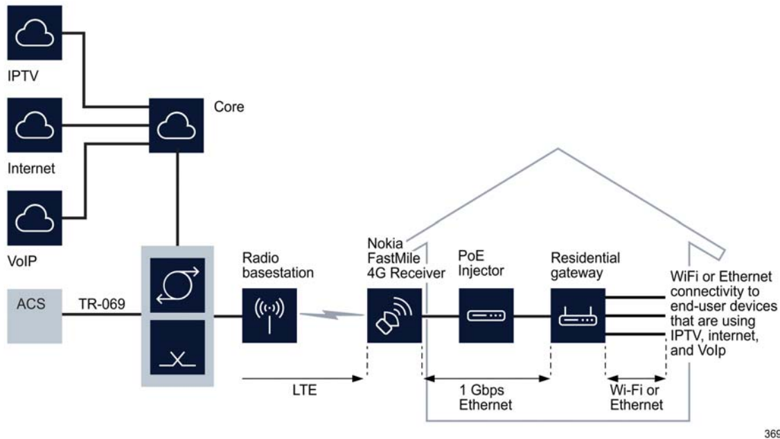
Figure 10 Remote management of the Nokia FastMile 4G Receiver through an ACS
