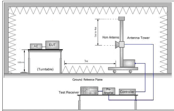
Figure 3. Above 1 GHz
