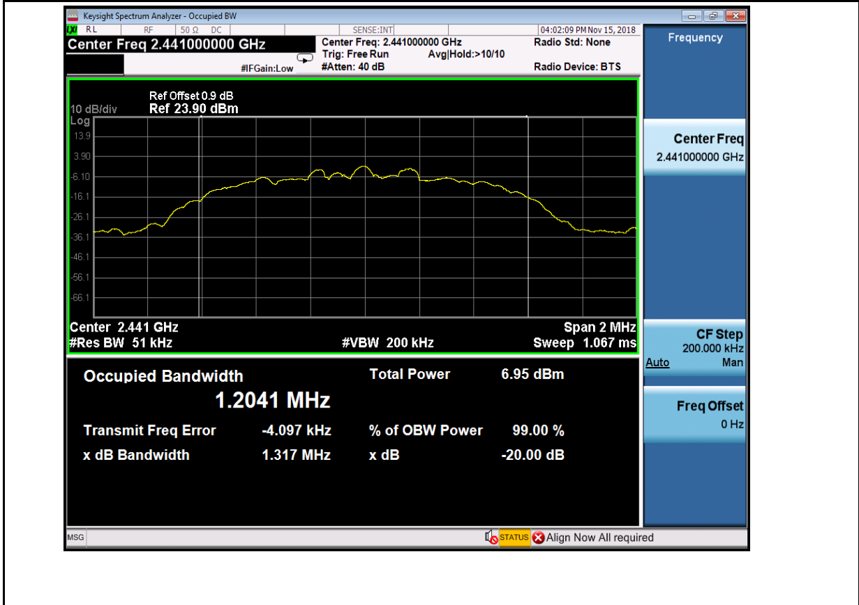
20 dB Bandwidth_3DH5_2441
