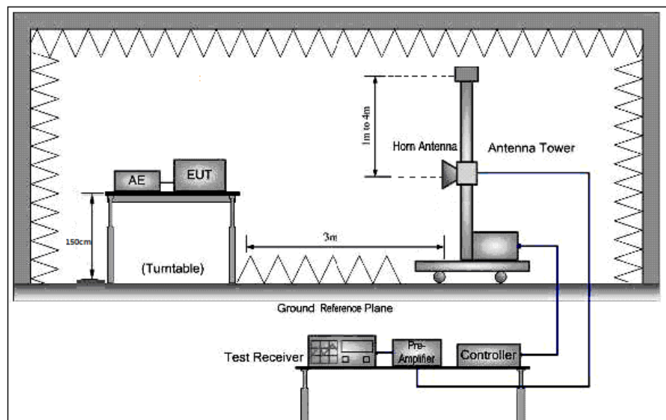
Above 1GHz
