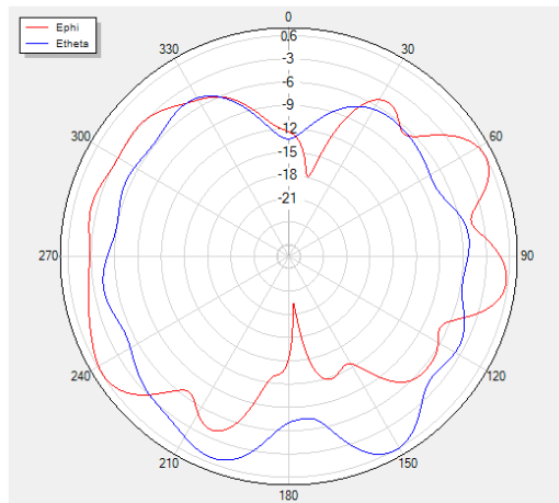
Phi=90 freq=2500MHz
