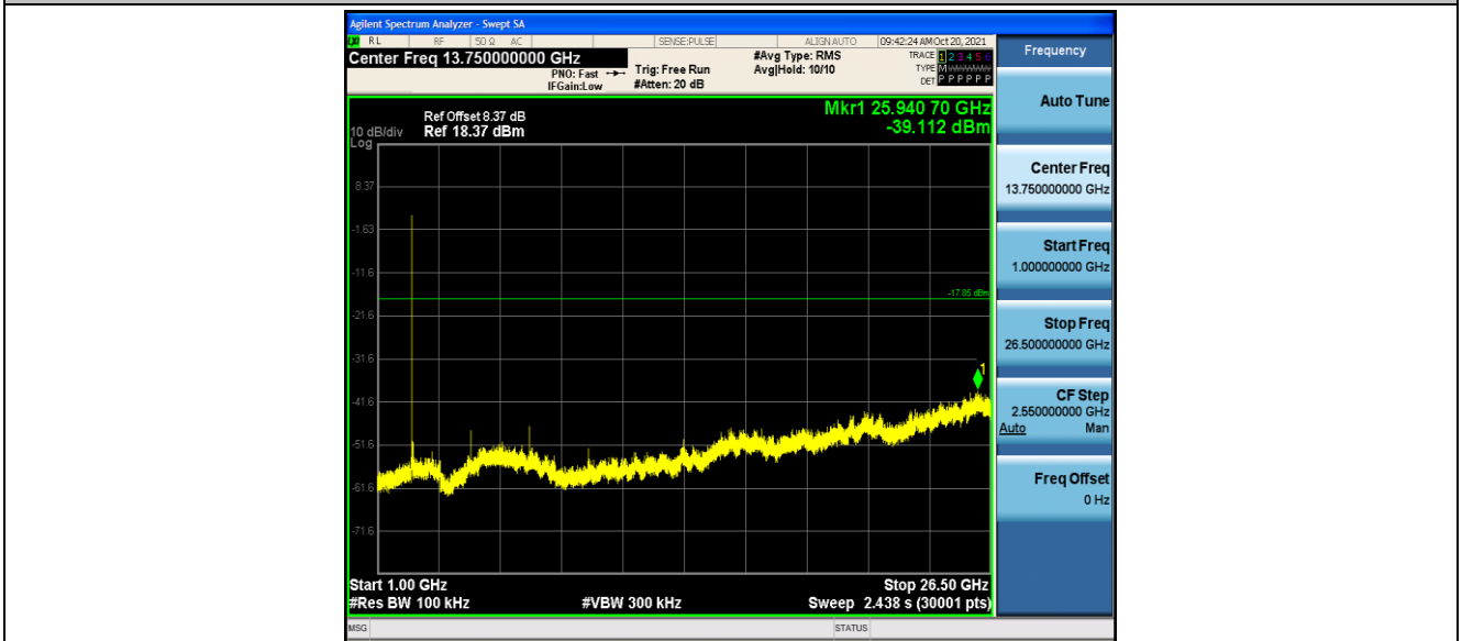
DH5_Ant1_2480_0~Reference
