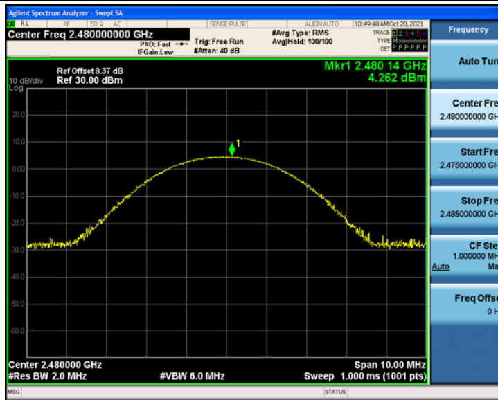
3DH5_Ant1_2480
