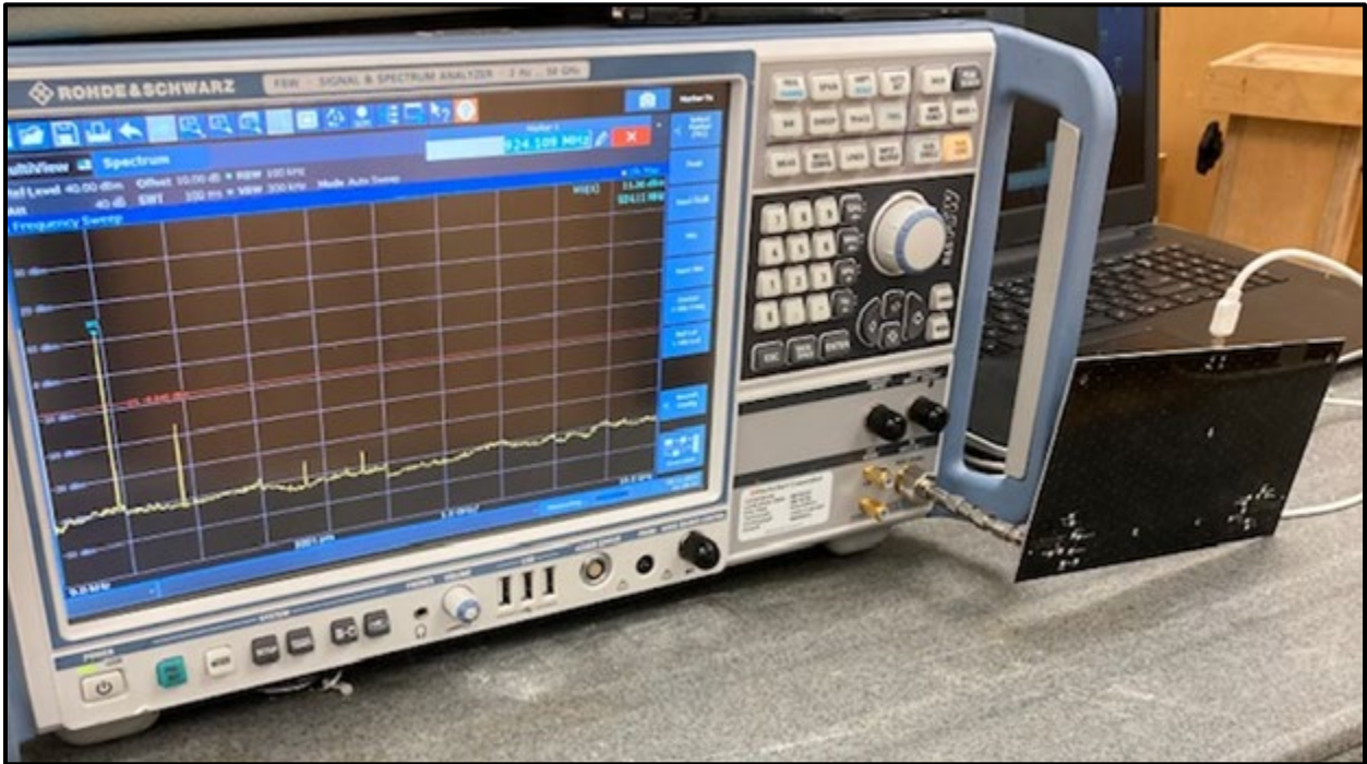
Photograph 5: Conducted Antenna Port
