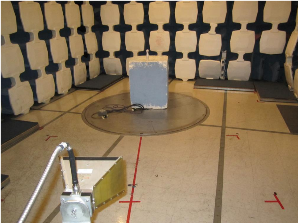
EMI Radiated – Rear (High Range)
