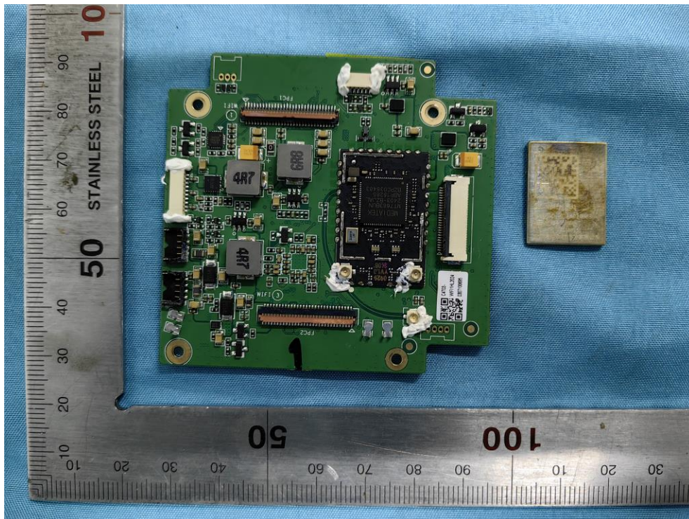
WiFi Board Front
