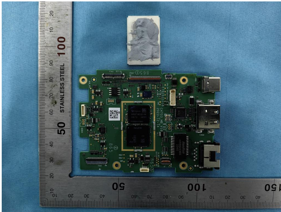
Mainboard Front
