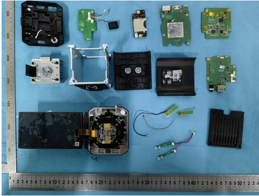
Internal Structure
