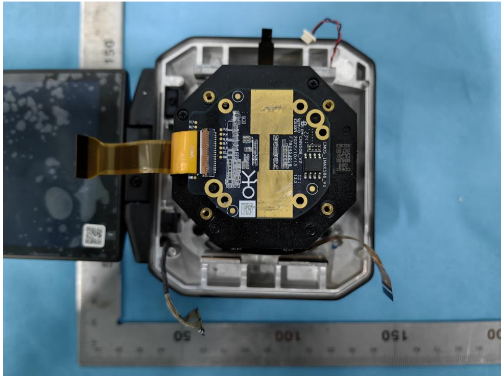
Camera Lens(The smallest whole, indivisible)
