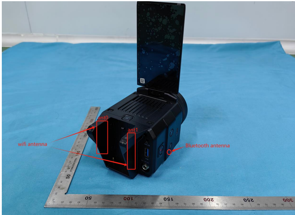
Antenna Location
