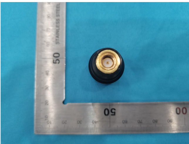
Antenna Appearance 3
