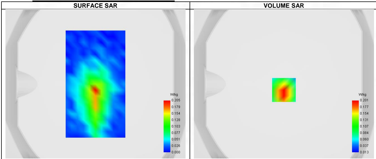
Maximum location: X=0.00, Y=-8.00 ; SAR Peak: 0.37 W/kg
