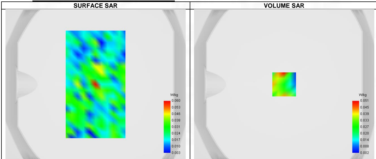
Maximum location: X=0.00, Y=0.00 ; SAR Peak: 0.15 W/kg
