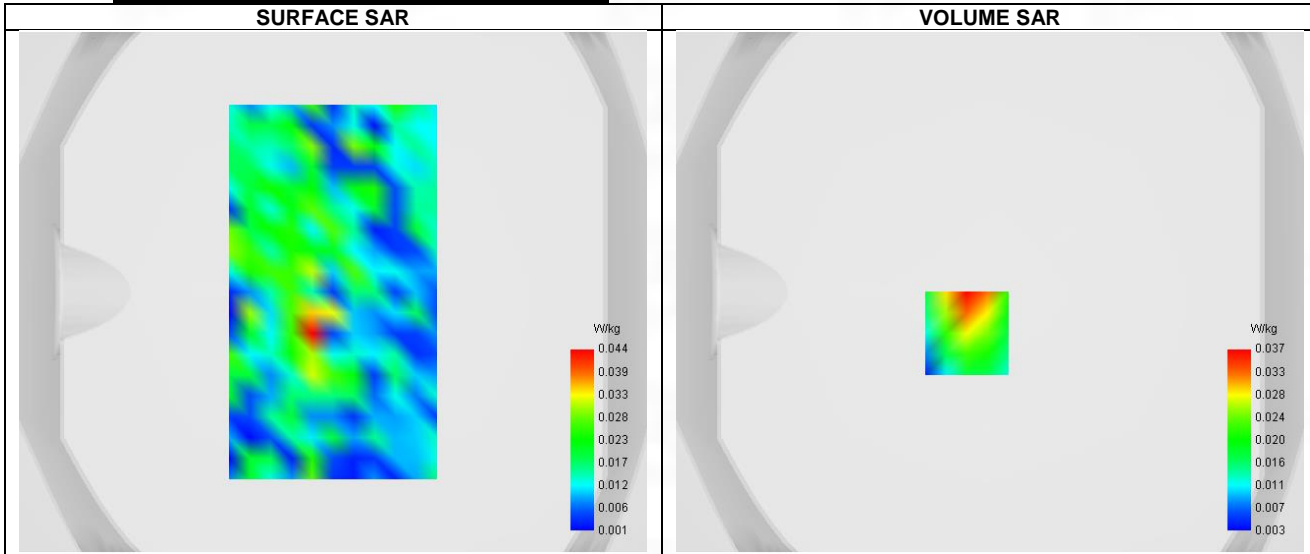
Maximum location: X=-9.00, Y=-16.00 ; SAR Peak: 0.06 W/kg
