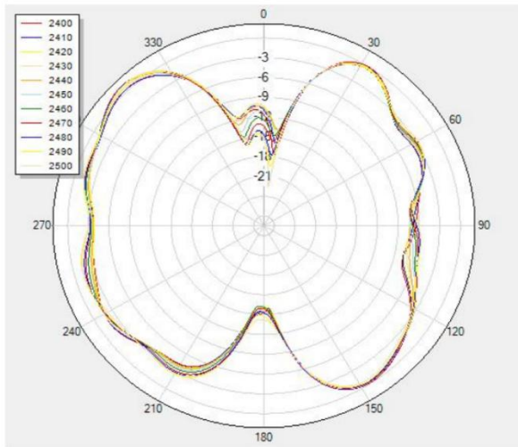
(1) X-Z Plane: V Phi=0
