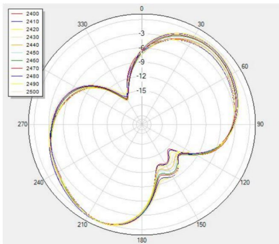
(3) X-Y Plane: H Theta=90
