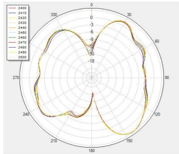
(2) Y-Z Plane: V Phi=90
