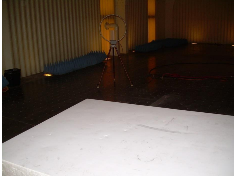
Photograph 3: View of Loop Antenna Placement for measurement of frequencies below 30 MHz
