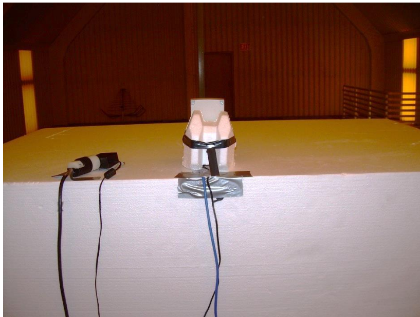
Photograph 2: Back View Radiated Emissions EUT Vertical Configuration
