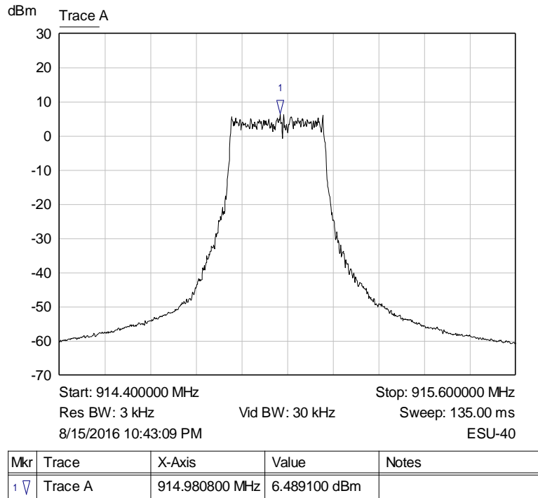
Graph 16: Middle Channel Power Spectral Density as Hybrid
