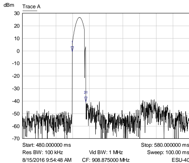
Graph 10: Timing Plot Duration of the Narrow Transmissions Shown in Graph 8
