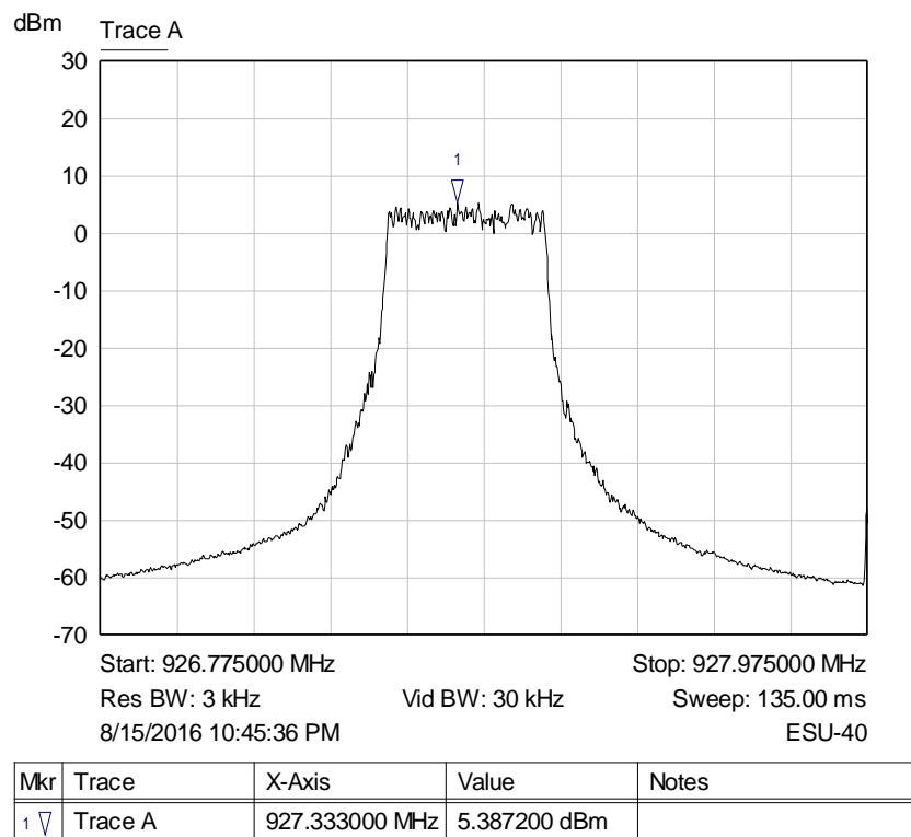
Graph 16: Middle Channel Power Spectral Density as Hybrid
