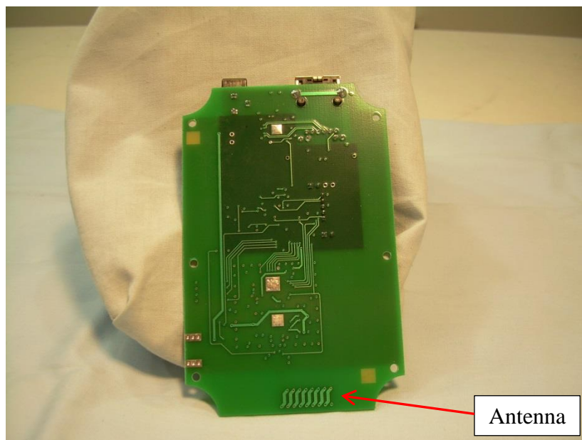
Photograph 4 – View of the Trace Side of the PCB
