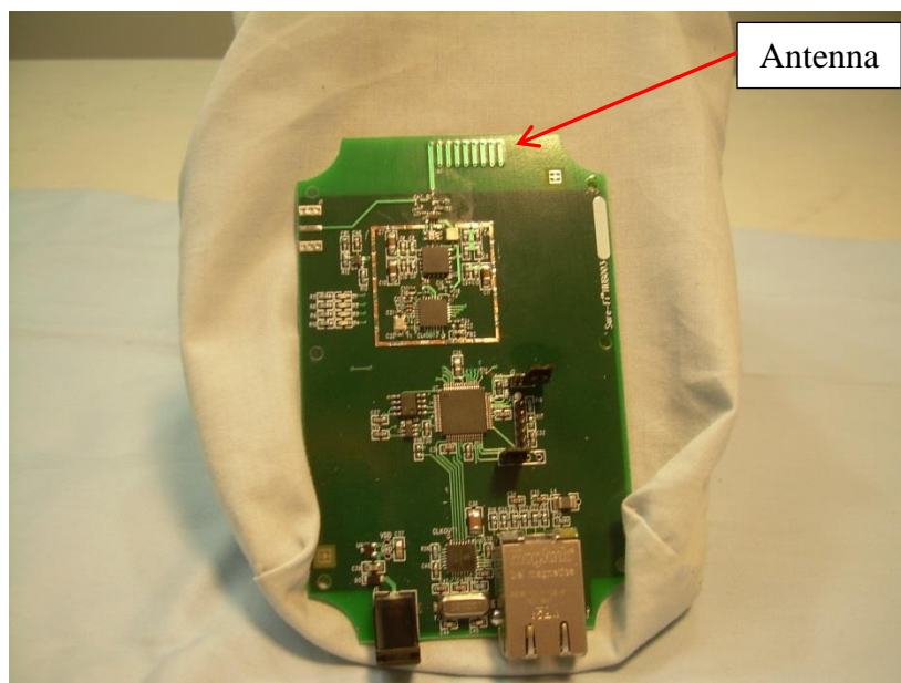
Photograph 2 – Internal View of Circuitry Side of the PCB with RF Shield Removed
