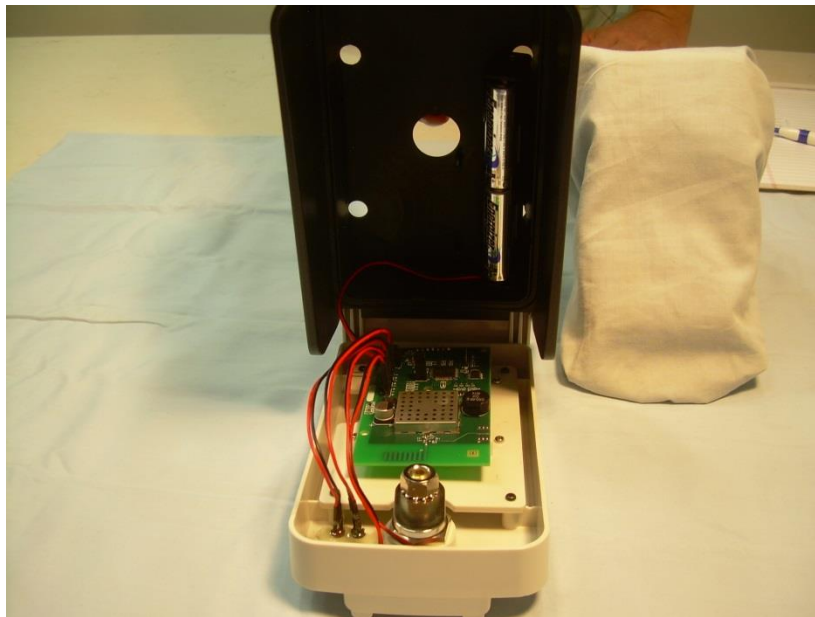
Photograph 1 – Internal View of the EUT with the Housing Open
