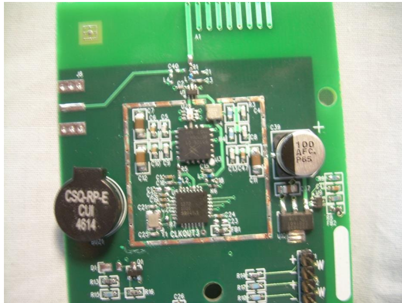
Photograph 3 – Internal View of the Circuitry Under the RF Shield
