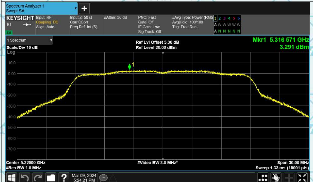
PSD NVNT ac20 5320MHz Ant1
