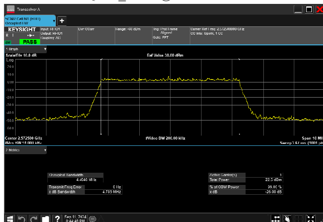
n38_5MHz_15kHz_2572.5MHz_CP-OFDM 16 QAM RB25@0.4463MHz
