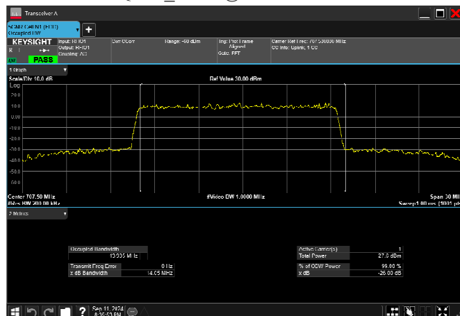
n12_15MHz_15kHz_707.5MHz_CP-OFDM 16 QAM RB79@0 14.115MHz
