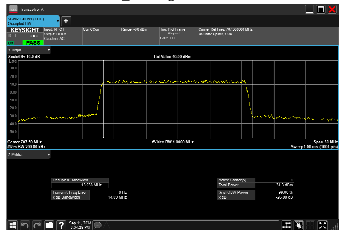
n12_15MHz_15kHz_707.5MHz_DFT-s-OFDM 16 QAM_RB75@0 14.053MHz
