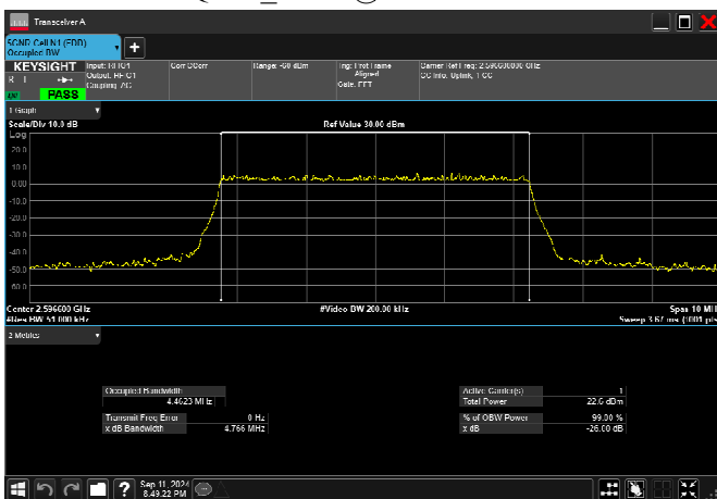
n38_5MHz_15kHz_2595MHz_DFT-s-OFDM 256 QAM_RB25@0 4.462MHz
