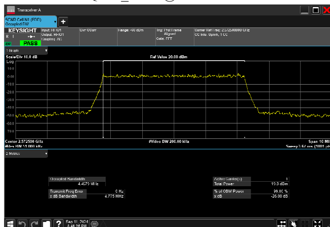
n38_5MHz_15kHz_2572.5MHz_CP-OFDM 256 QAM RB25@0.4468MHz
