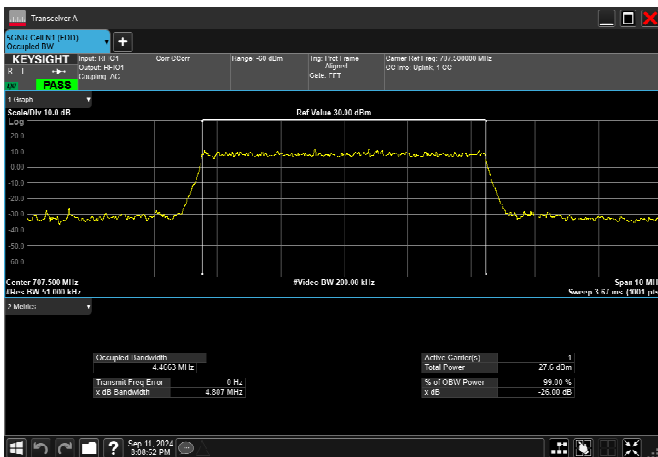
n12_5MHz_15kHz_707.5MHz_CP-OFDM 64 QAM_RB25@0 4.480MHz
