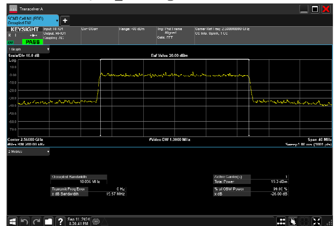
n7_20MHz_15kHz_2560MHz_CP-OFDM 256 QAM_RB106@0 18.896MHz
