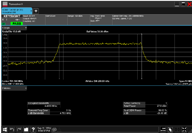
n12_5MHz_15kHz_701.5MHz_CP-OFDM 256 QAM_RB25@0 4.466MHz
