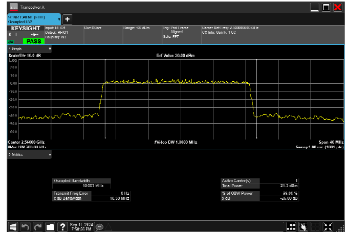
n7_20MHz_15kHz_2560MHz_CP-OFDM 16 QAM_RB106@0 18.899MHz
