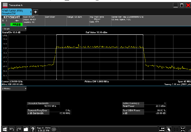
n7_20MHz_15kHz_2560MHz_CP-OFDM 64 QAM_RB106@0 18.910MHz
