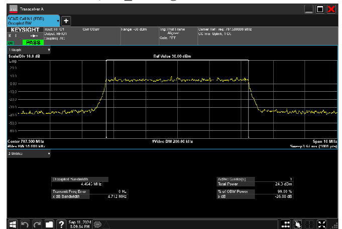
n12_5MHz_15kHz_707.5MHz_CP-OFDM 256 QAM_RB25@0 4.464MHz
