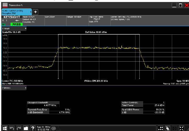
n12_5MHz_15kHz_713.5MHz_DFT-s-OFDM 256 QAM_RB25@0 4.463MHz
