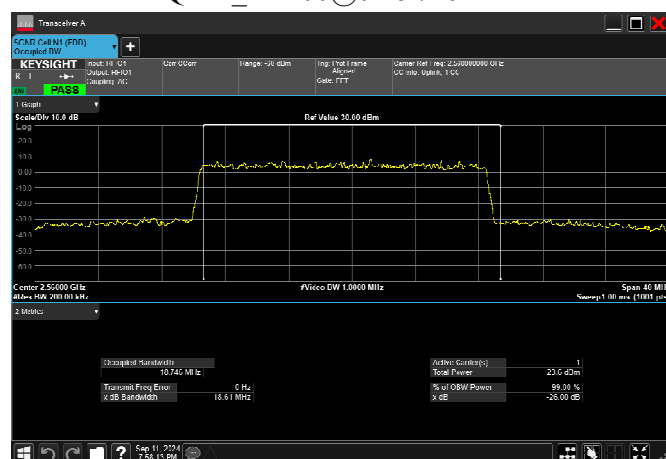
n7_20MHz_15kHz_2560MHz_DFT-s-OFDM 16 OAM RB100@0 18.746MHz
