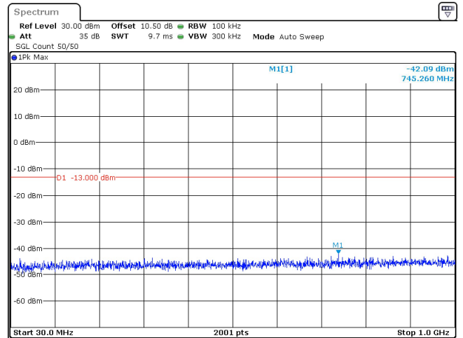
15MHz_15kHz_3500MHz_DFT-s-OFDM QPSK_RB75@0 -42.09 dBm
