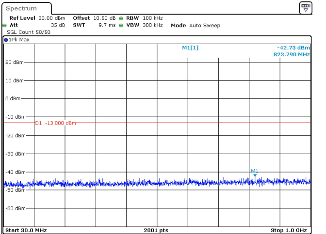
15MHz_30kHz_3457.5MHz_DFT-s-OFDM QPSK_RB1@37 -42.73 dBm
