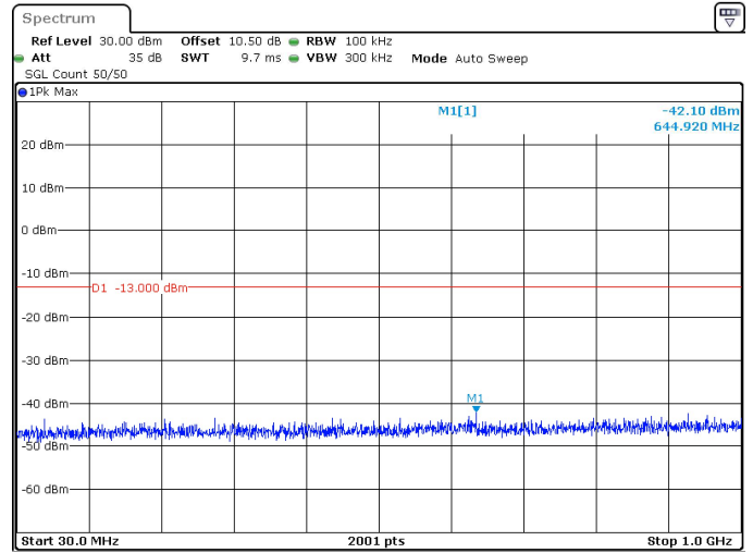
15MHz_15kHz_3500MHz_DFT-s-OFDM QPSK_RB1@0 -42.10 dBm
