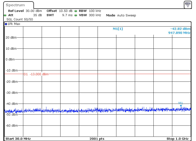
15MHz_30kHz_3457.5MHz_DFT-s-OFDM QPSK_RB36@0 -42.82 dBm
