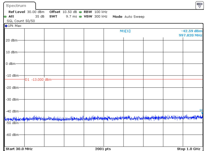
15MHz_15kHz_3542.5MHz_DFT-s-OFDM QPSK_RB1@78 -42.59 dBm
