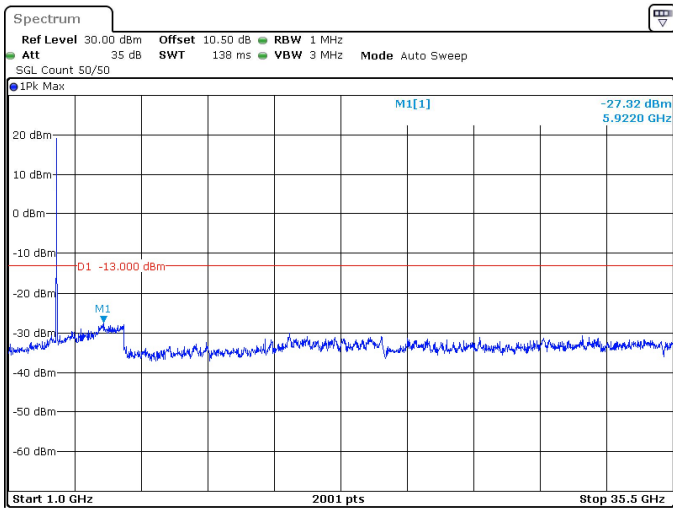
15MHz_15kHz_3500MHz_DFT-s-OFDM QPSK_RB75@0 -27.32 dBm
