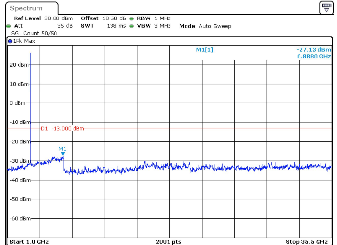
15MHz_30kHz_3457.5MHz_DFT-s-OFDM QPSK_RB1@37 -27.13 dBm
