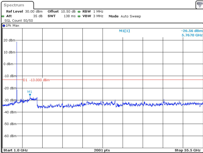
15MHz_15kHz_3500MHz_DFT-s-OFDM QPSK_RB1@0 -26.56 dBm
