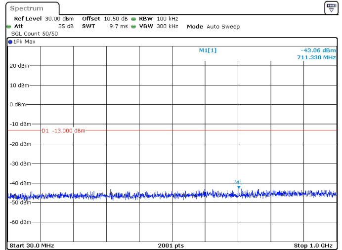
15MHz_15kHz_3500MHz_DFT-s-OFDM QPSK_RB1@78 -43.06 dBm
