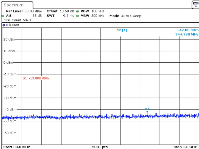
15MHz_30kHz_3457.5MHz_DFT-s-OFDM QPSK_RB1@0 -42.83 dBm
