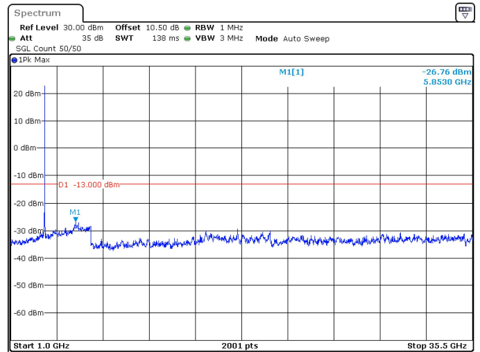
15MHz_15kHz_3542.5MHz_DFT-s-OFDM QPSK_RB1@0 -26.76 dBm
