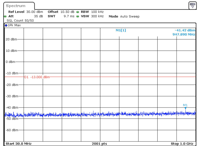
15MHz_15kHz_3542.5MHz_DFT-s-OFDM QPSK_RB75@0 -41.42 dBm
