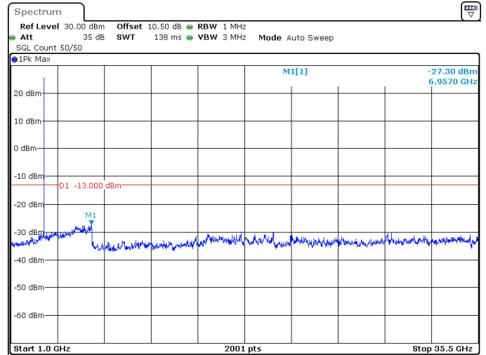
15MHz_30kHz_3457.5MHz_DFT-s-OFDM QPSK_RB1@0 -27.30 dBm
