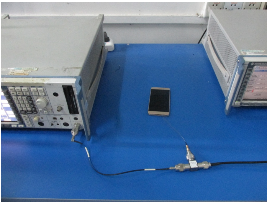
RF TEST
